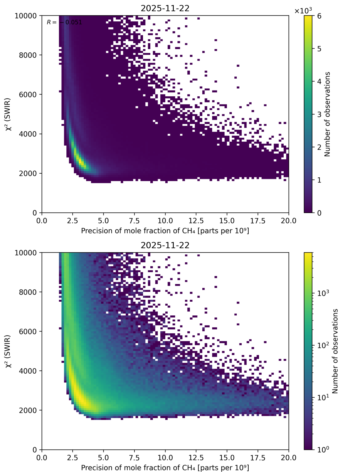
Figure 79: Scatter density plot of “Precision of mole fraction of \text{CH}_4 ” against “ \chi^2 (SWIR)” for 2025-11-21 to 2025-11-23.
