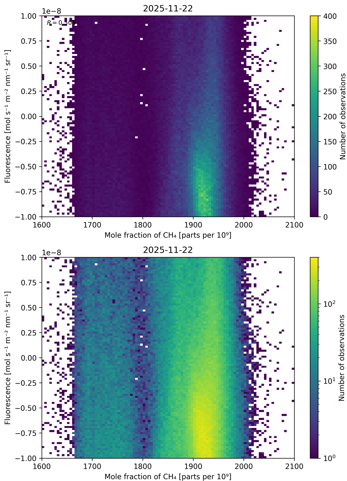
Figure 73: Scatter density plot of “Mole fraction of \text{CH}_4 ” against “Fluorescence” for 2025-11-21 to 2025-11-23.
