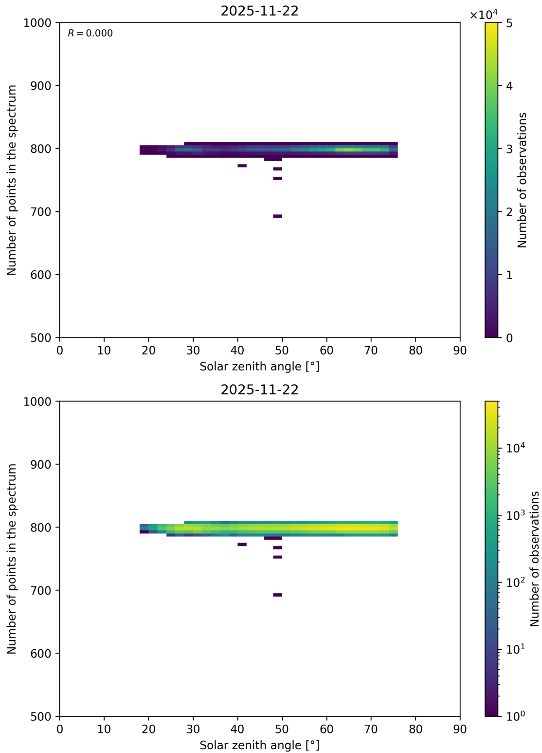
Figure 103: Scatter density plot of “Solar zenith angle” against “Number of points in the spectrum” for 2025-11-21 to 2025-11-23.
