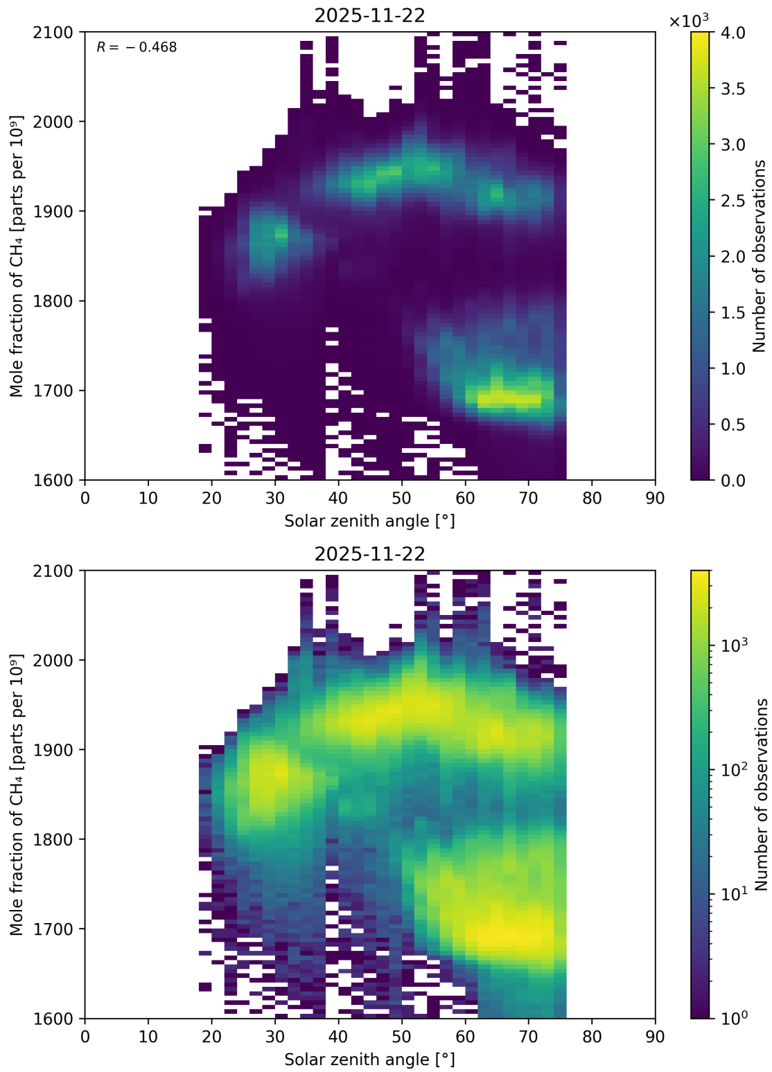
Figure 99: Scatter density plot of “Solar zenith angle” against “Mole fraction of CH 4 ” for 2025-11-21 to 2025-11-23.
