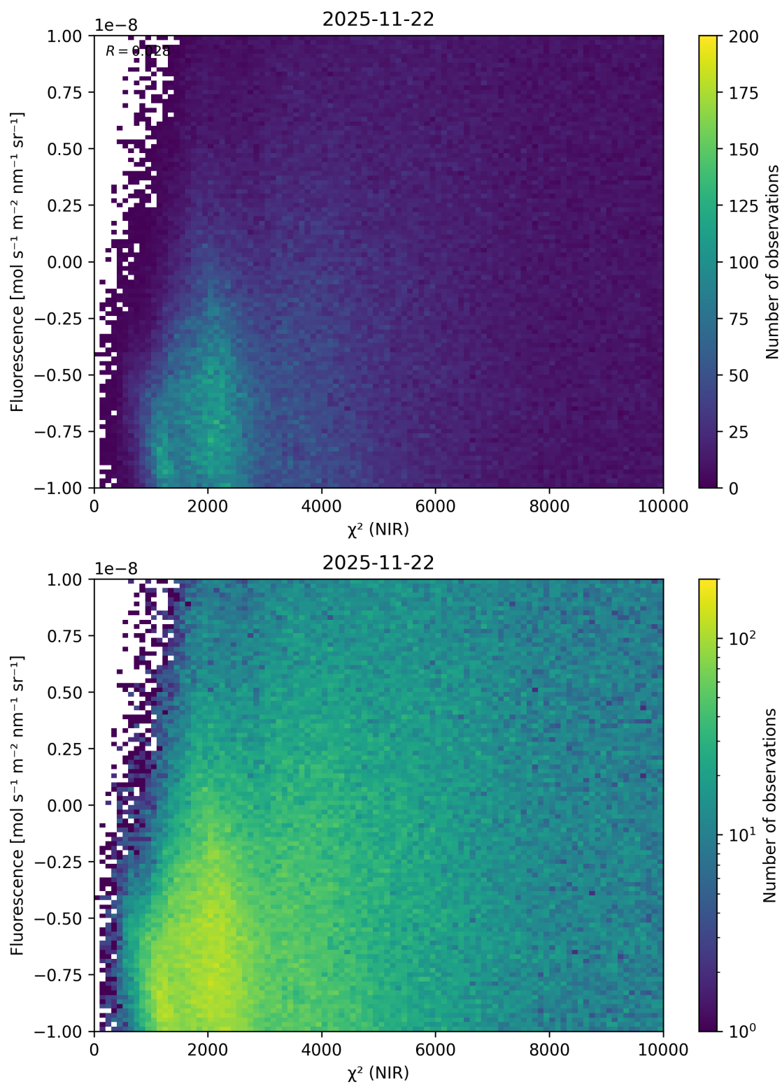
Figure 45: Scatter density plot of “ \chi^2 (NIR)” against “Fluorescence” for 2025-11-21 to 2025-11-23.
