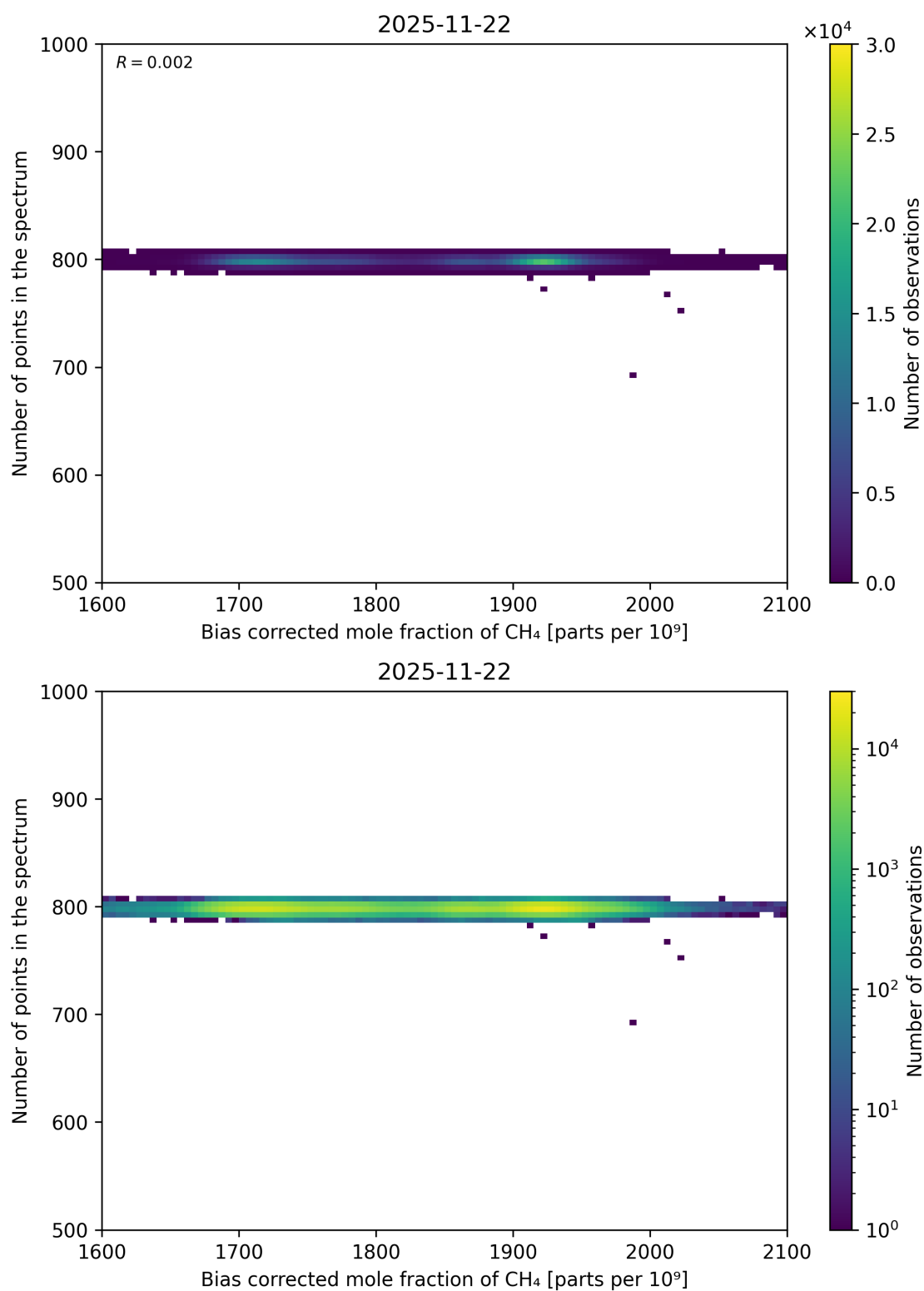
Figure 68: Scatter density plot of “Bias corrected mole fraction of CH 4 ” against “Number of points in the spectrum” for 2025-11-21 to 2025-11-23.
