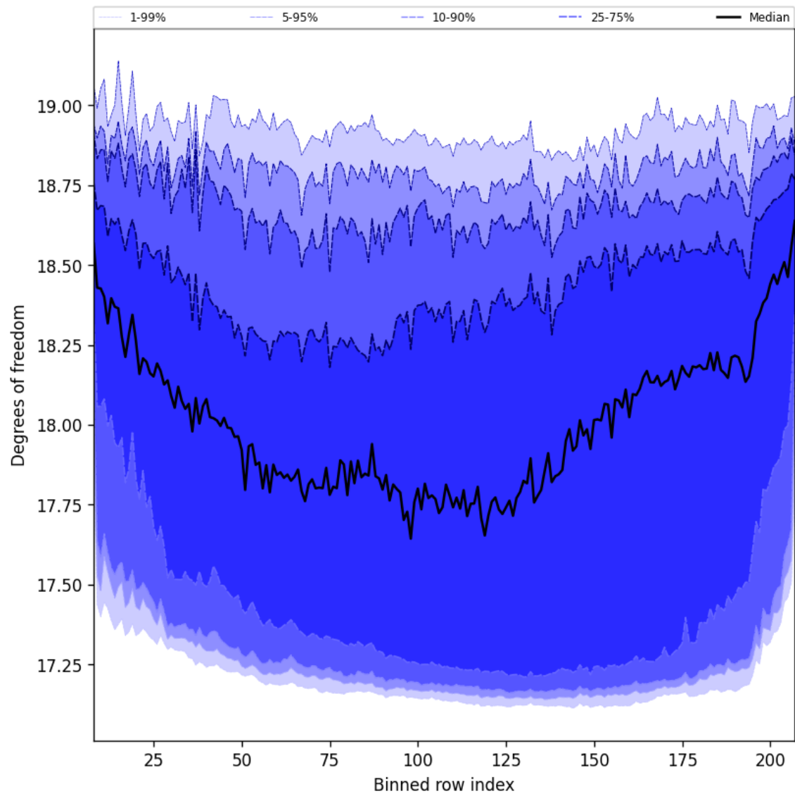
Figure 41: Along track statistics of “Degrees of freedom” for 2025-11-21 to 2025-11-23
