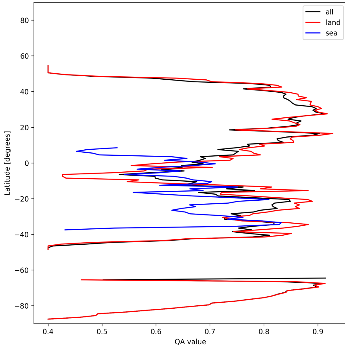
Figure 11: Zonal average of “QA value” for 2025-11-21 to 2025-11-23.
