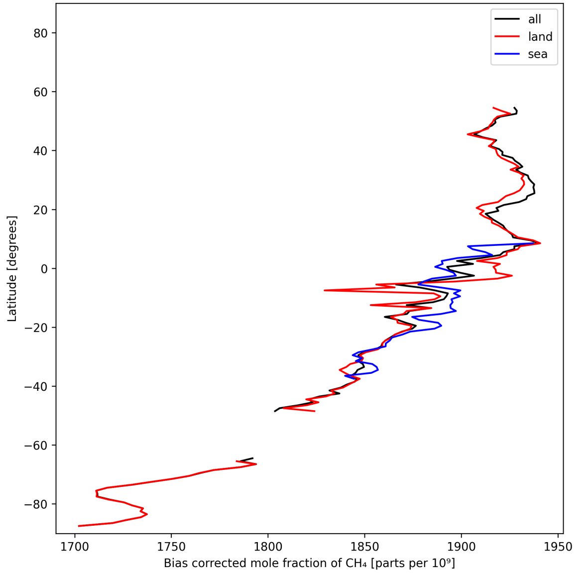
Figure 14: Zonal average of “Bias corrected mole fraction of CH 4 ” for 2025-11-21 to 2025-11-23.
