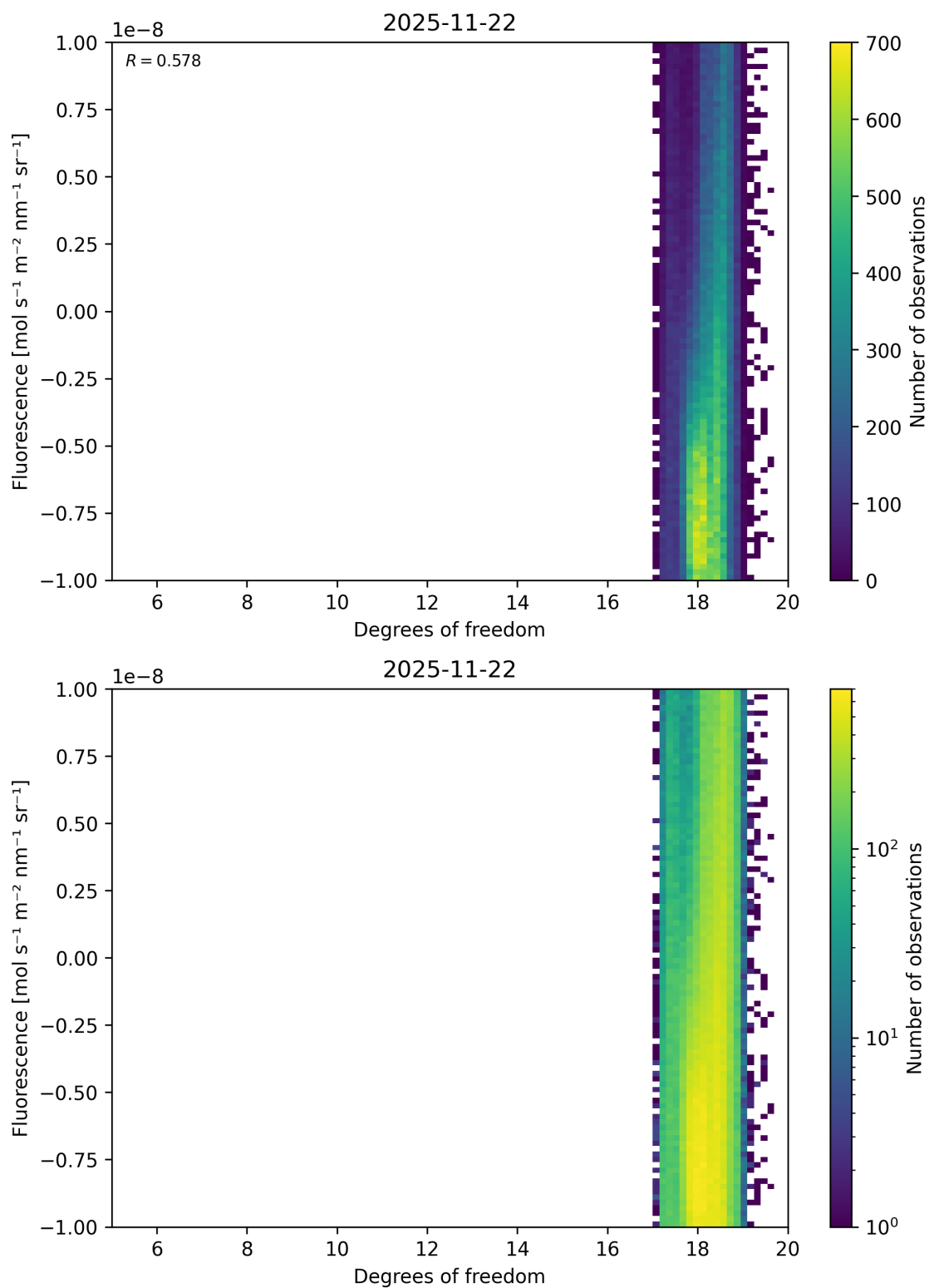
Figure 51: Scatter density plot of “Degrees of freedom” against “Fluorescence” for 2025-11-21 to 2025-11-23.
