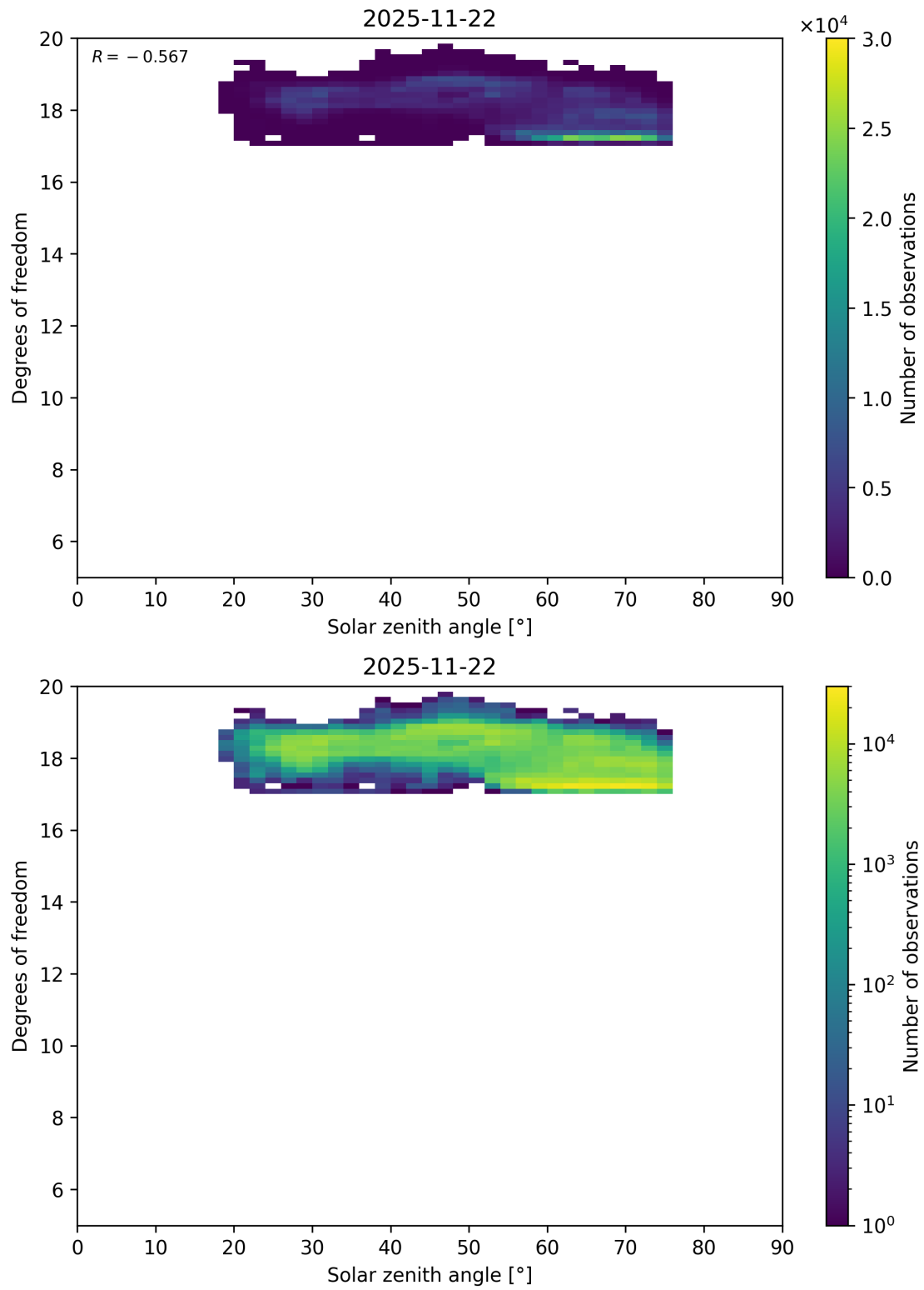
Figure 96: Scatter density plot of “Solar zenith angle” against “Degrees of freedom” for 2025-11-21 to 2025-11-23.
