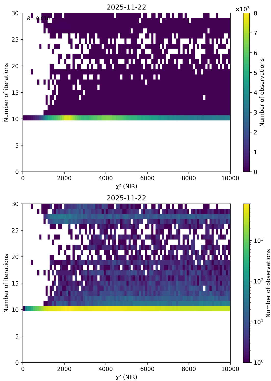
Figure 46: Scatter density plot of “ \chi^2 (NIR)” against “Number of iterations” for 2025-11-21 to 2025-11-23.
