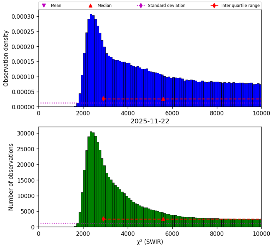
Figure 28: Histogram of “ \chi^2 (SWIR)” for 2025-11-21 to 2025-11-23
