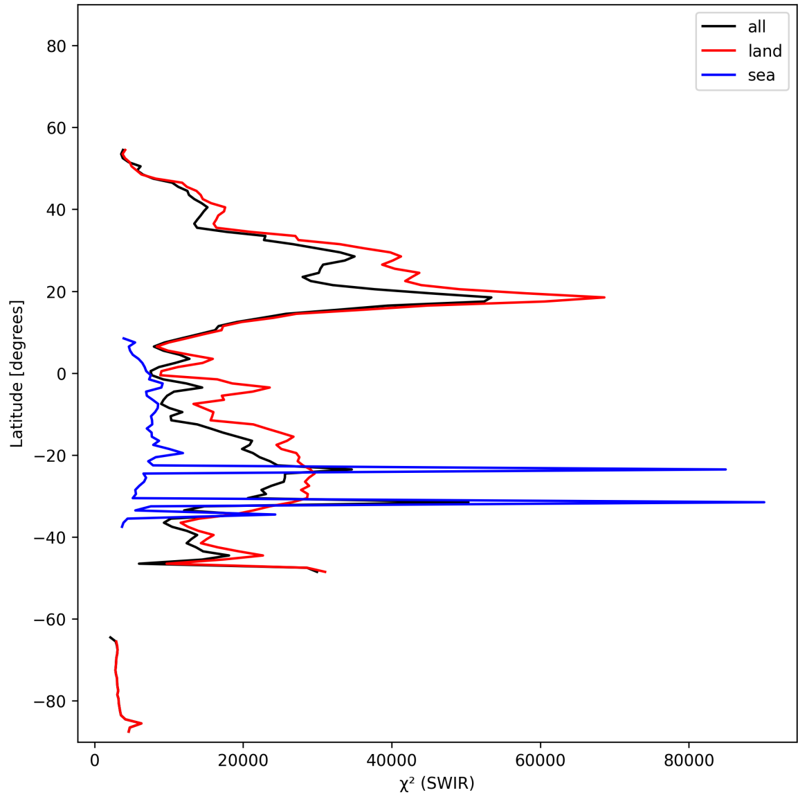
Figure 17: Zonal average of “ \chi^2 (SWIR)” for 2025-11-21 to 2025-11-23.
