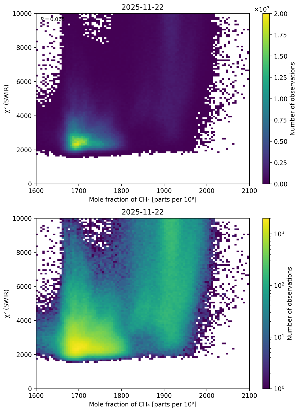
Figure 71: Scatter density plot of “Mole fraction of \text{CH}_4 ” against “ \chi^2 (SWIR)” for 2025-11-21 to 2025-11-23.
