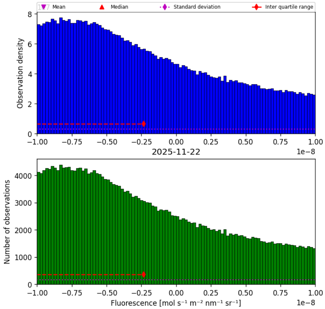
Figure 32: Histogram of “Fluorescence” for 2025-11-21 to 2025-11-23
