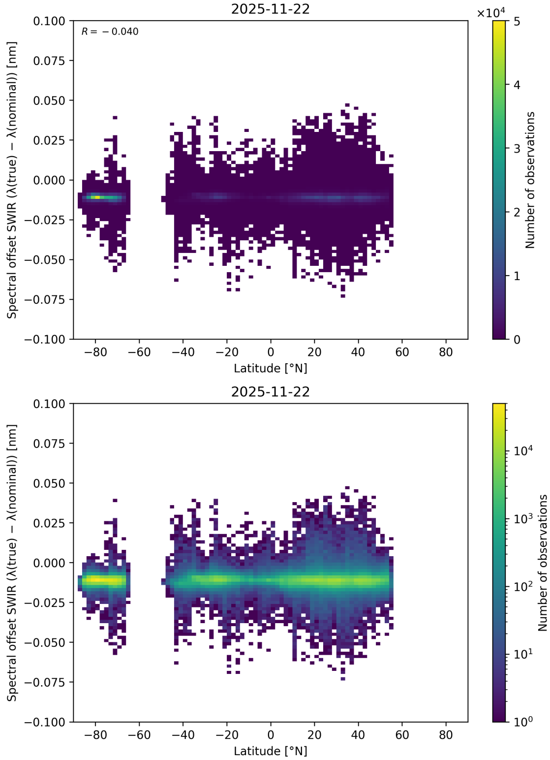
Figure 62: Scatter density plot of “Latitude” against “Spectral offset SWIR ( \lambda_{\text{true}} - \lambda_{\text{nominal}} )” for 2025-11-21 to 2025-11-23.
