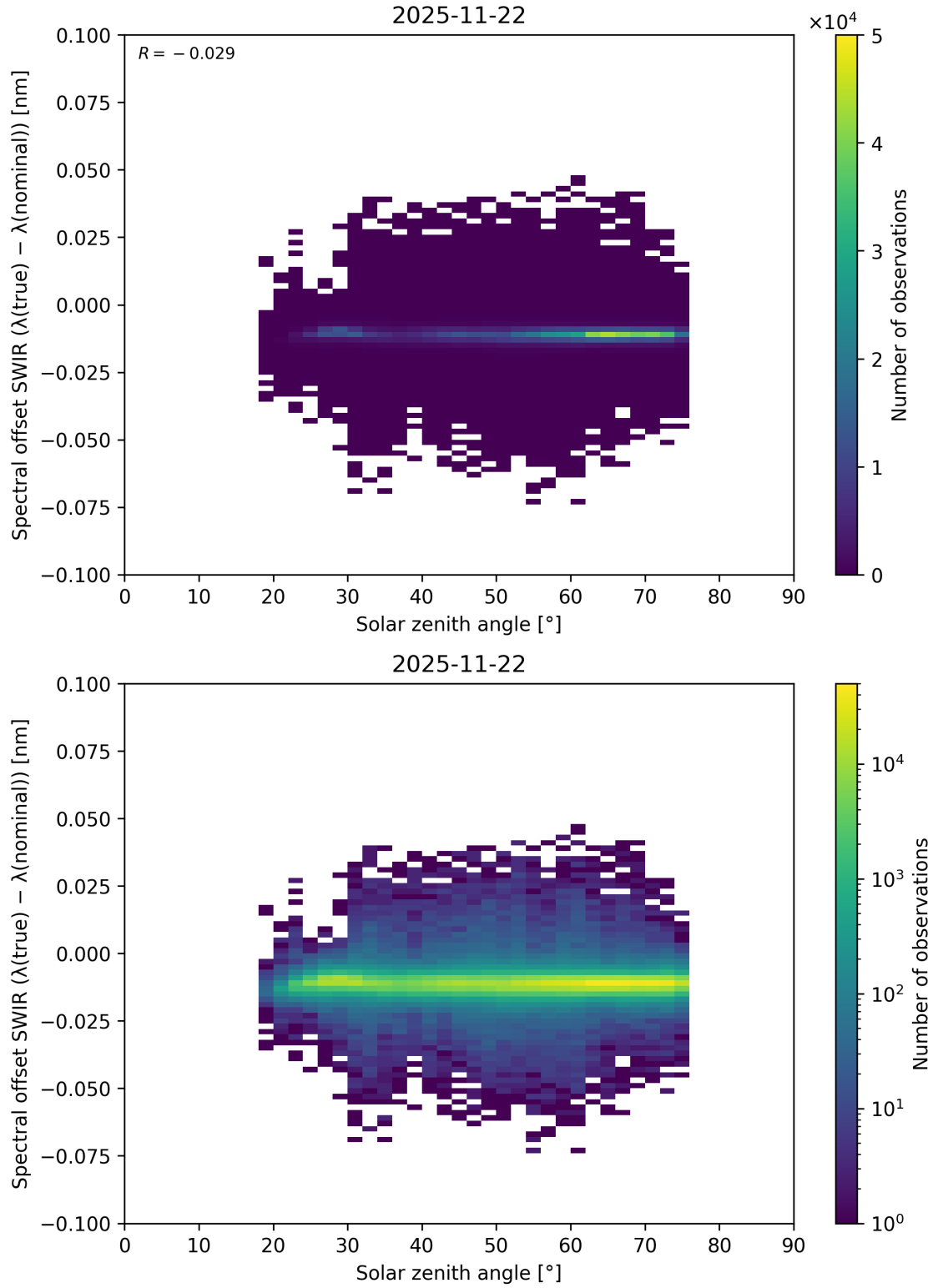
Figure 104: Scatter density plot of “Solar zenith angle” against “Spectral offset SWIR ( \lambda_{\text{true}} - \lambda_{\text{nominal}} )” for 2025-11-21 to 2025-11-23.
