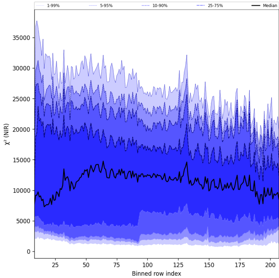
Figure 40: Along track statistics of “ \chi^2 (NIR)” for 2025-11-21 to 2025-11-23
