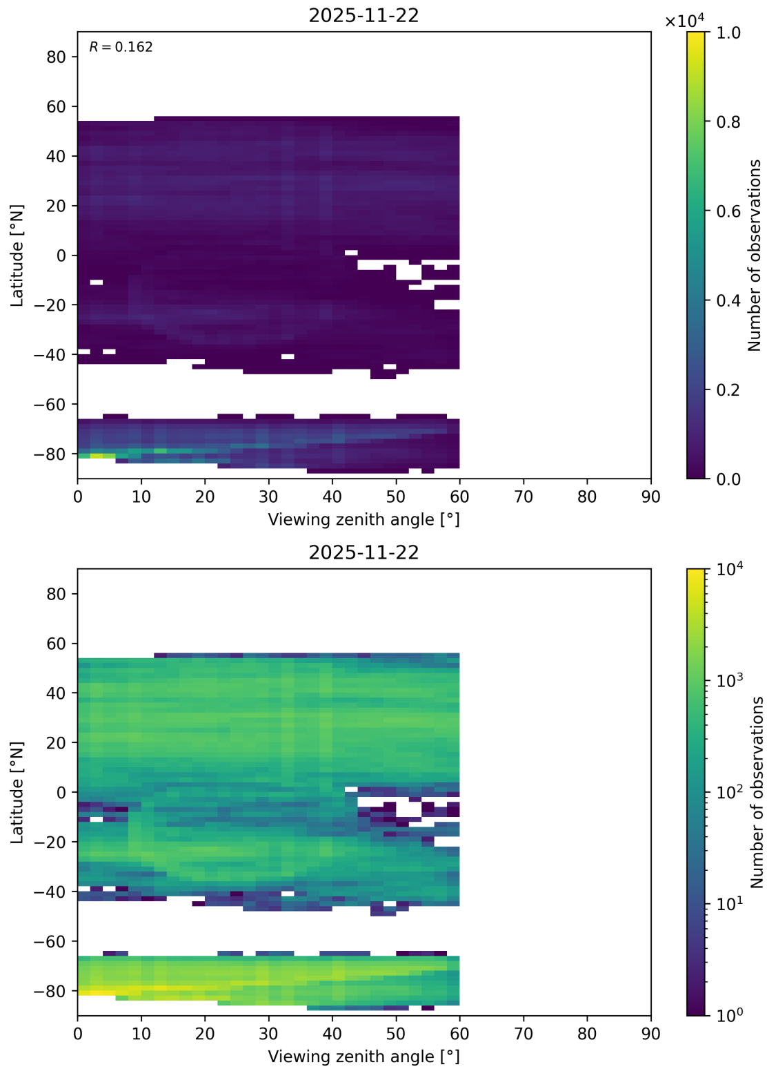
Figure 109: Scatter density plot of “Viewing zenith angle” against “Latitude” for 2025-11-21 to 2025-11-23.
