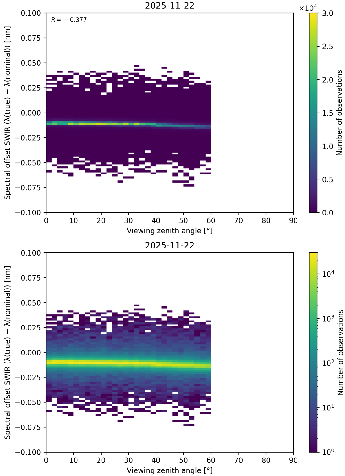
Figure 116: Scatter density plot of “Viewing zenith angle” against “Spectral offset SWIR ( \lambda_{\text{true}} - \lambda_{\text{nominal}} )” for 2025-11-21 to 2025-11-23.
