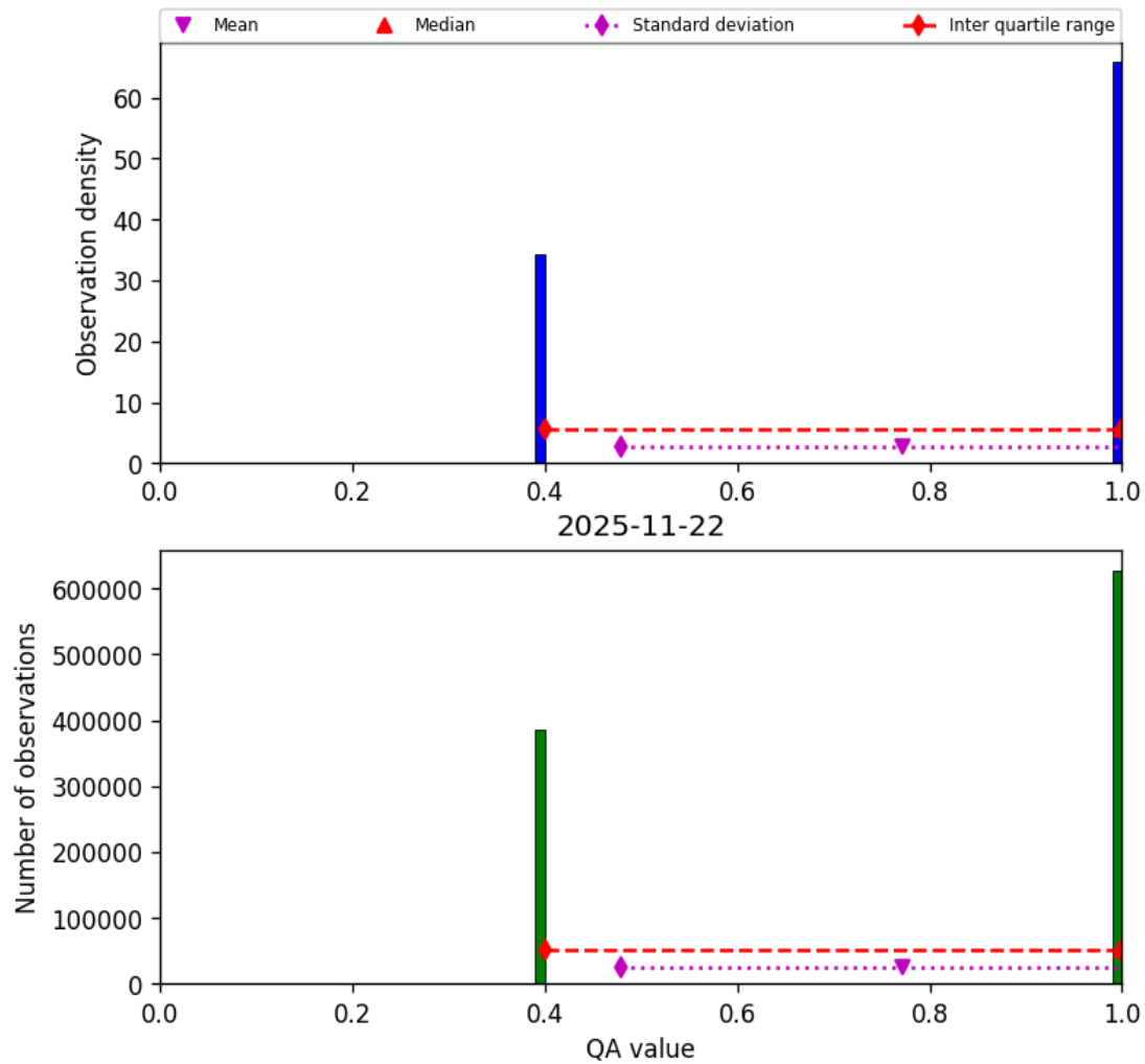
Figure 22: Histogram of “QA value” for 2025-11-21 to 2025-11-23
