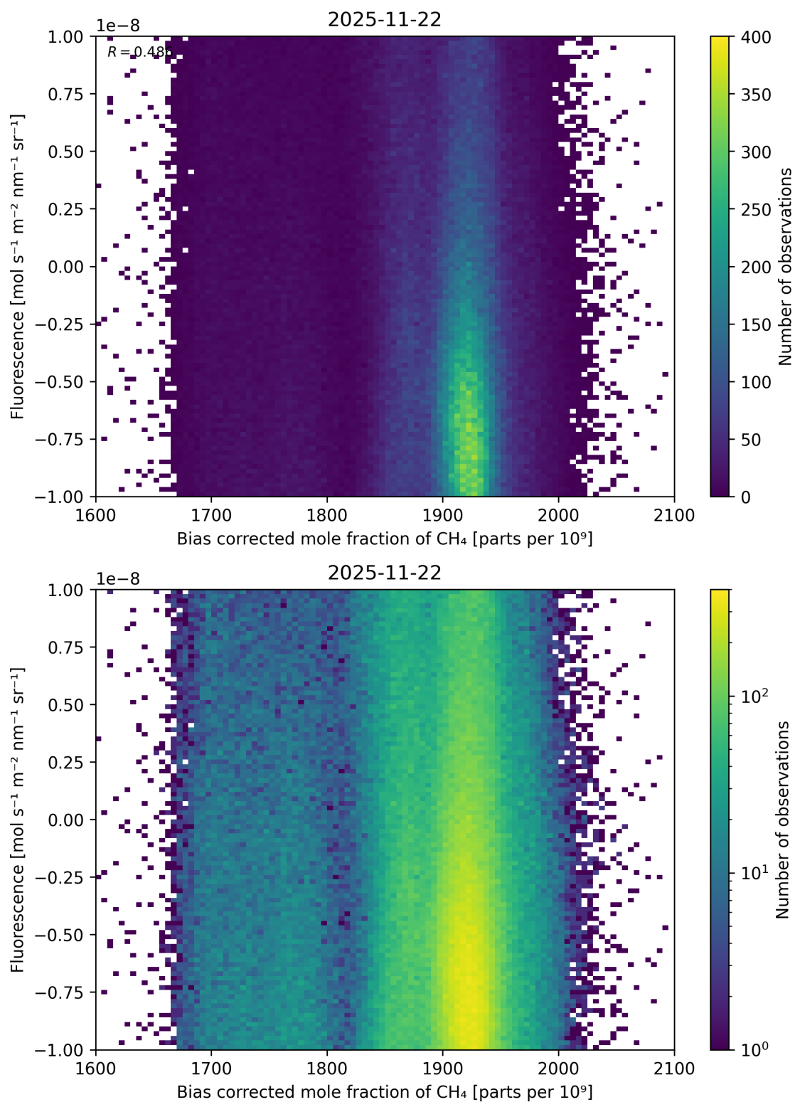
Figure 66: Scatter density plot of “Bias corrected mole fraction of \text{CH}_4 ” against “Fluorescence” for 2025-11-21 to 2025-11-23.
