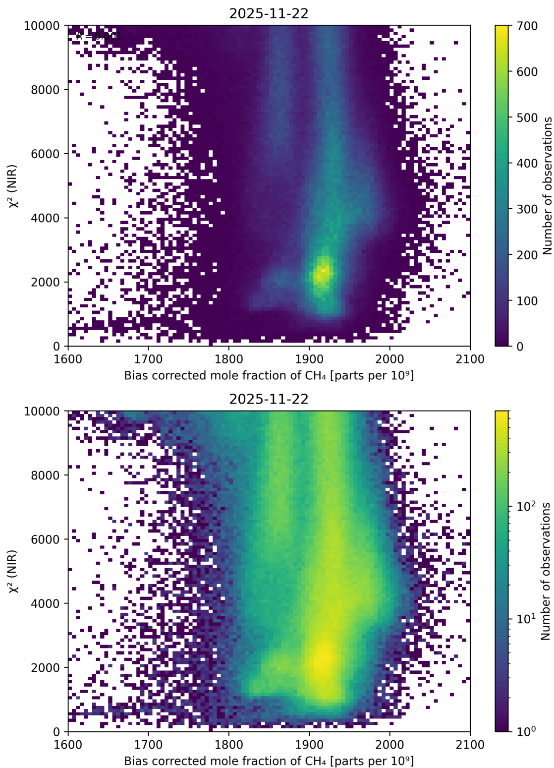
Figure 63: Scatter density plot of “Bias corrected mole fraction of \text{CH}_4 ” against “ \chi^2 (NIR)” for 2025-11-21 to 2025-11-23.
