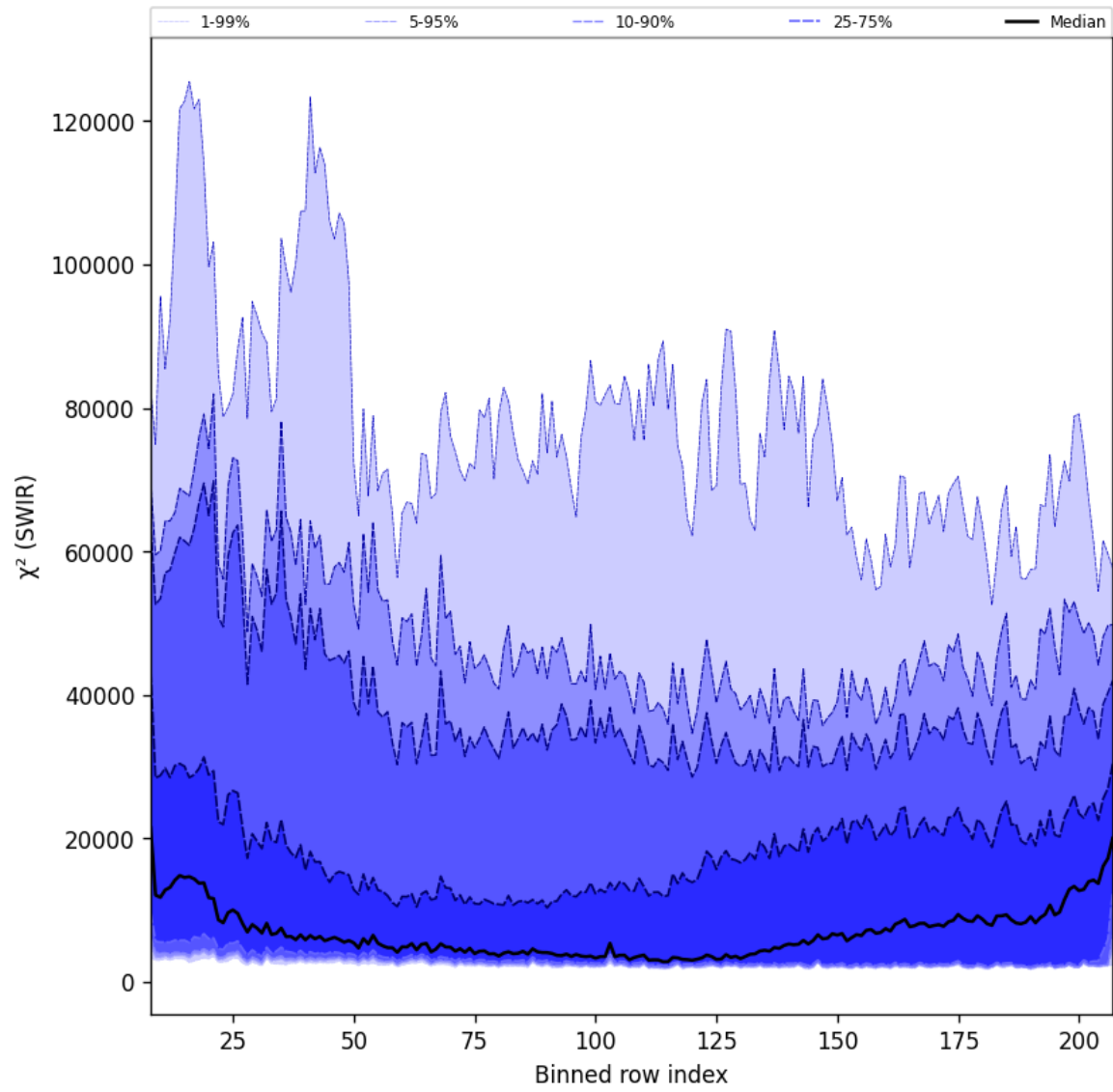
Figure 39: Along track statistics of “ \chi^2 (SWIR)” for 2025-11-21 to 2025-11-23
