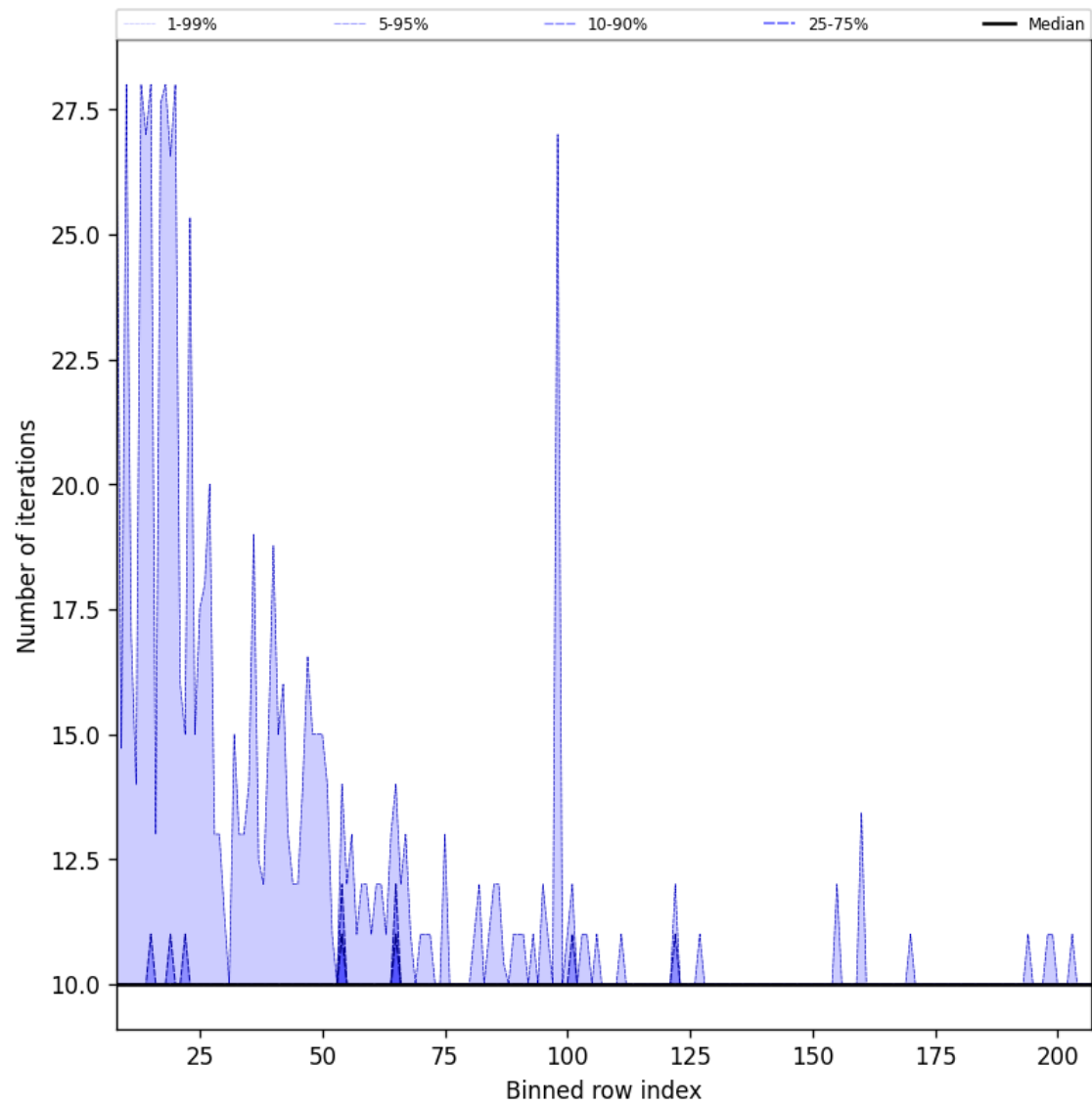
Figure 42: Along track statistics of “Number of iterations” for 2025-11-21 to 2025-11-23
