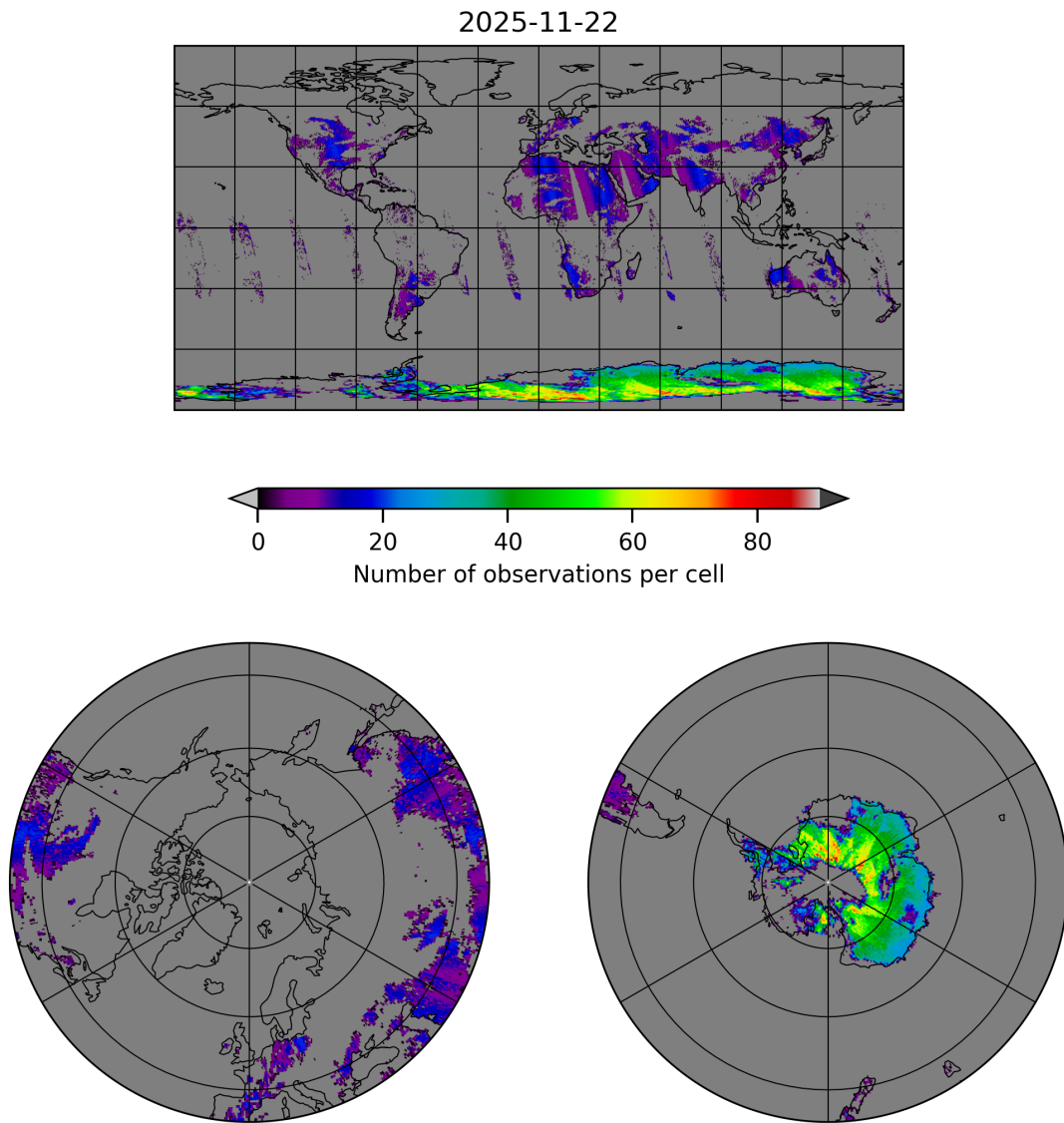
Figure 10: Map of the number of observations for 2025-11-21 to 2025-11-23
