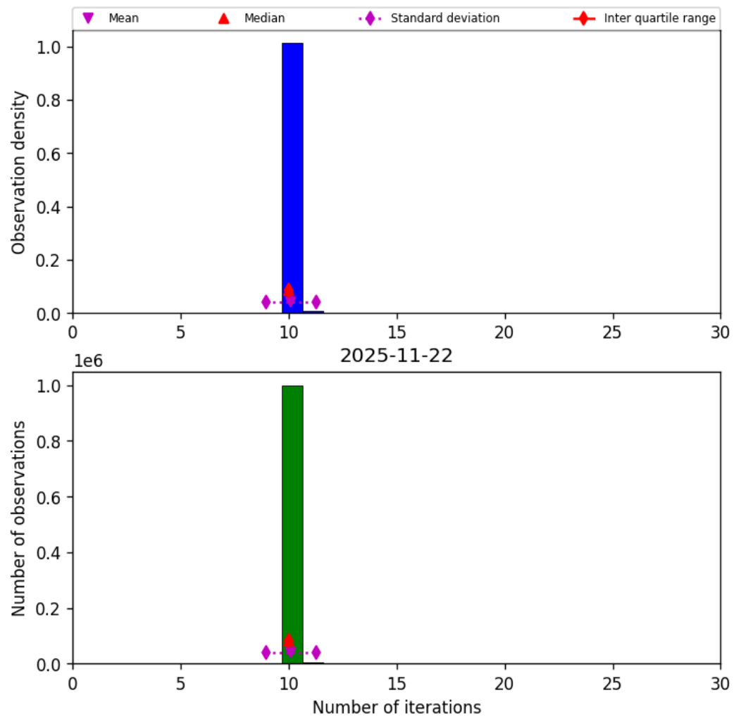
Figure 31: Histogram of “Number of iterations” for 2025-11-21 to 2025-11-23
