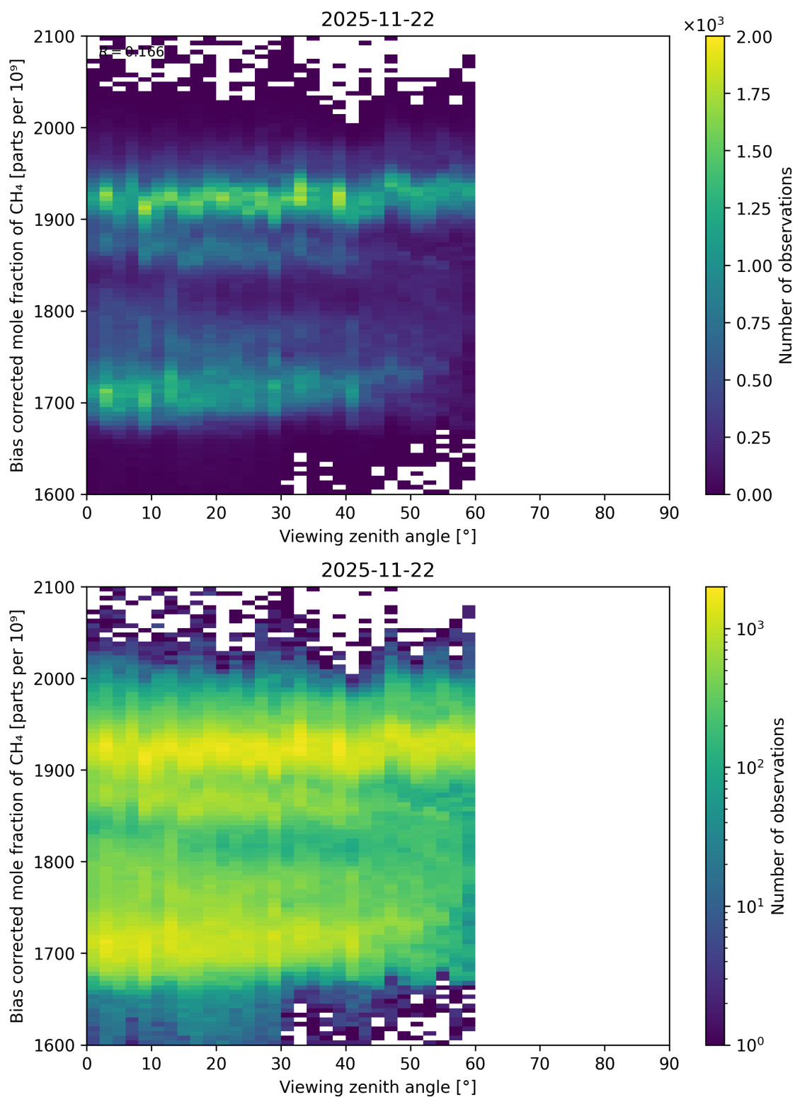
Figure 111: Scatter density plot of “Viewing zenith angle” against “Bias corrected mole fraction of \text{CH}_4 ” for 2025-11-21 to 2025-11-23.
