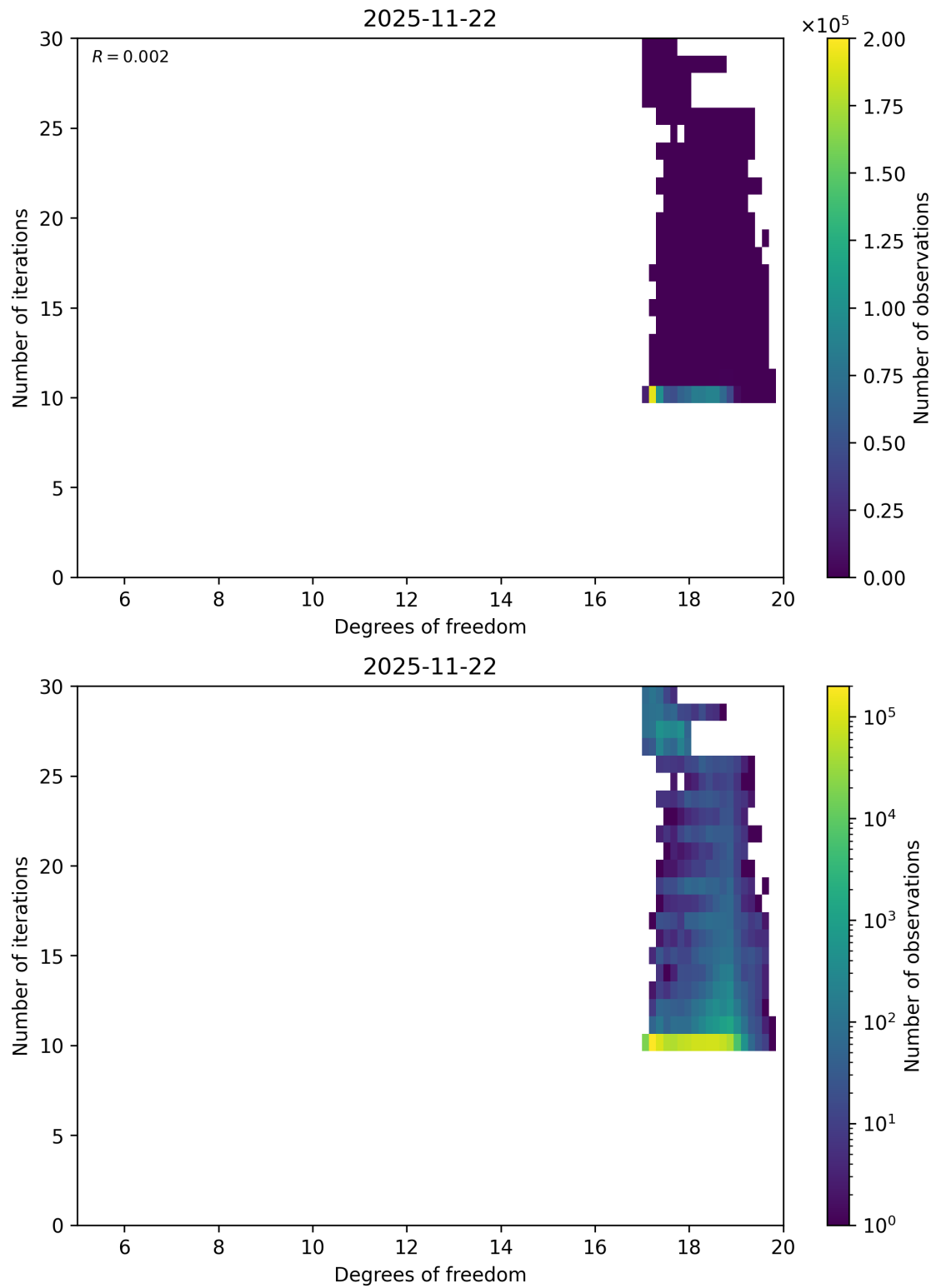
Figure 52: Scatter density plot of “Degrees of freedom” against “Number of iterations” for 2025-11-21 to 2025-11-23.
