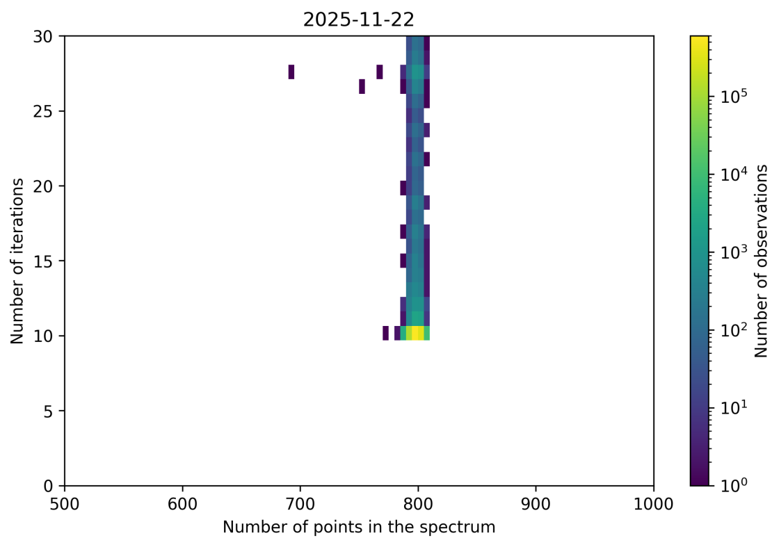
Figure 92: Scatter density plot of “Number of points in the spectrum” against “Number of iterations” for 2025-11-21 to 2025-11-23.
