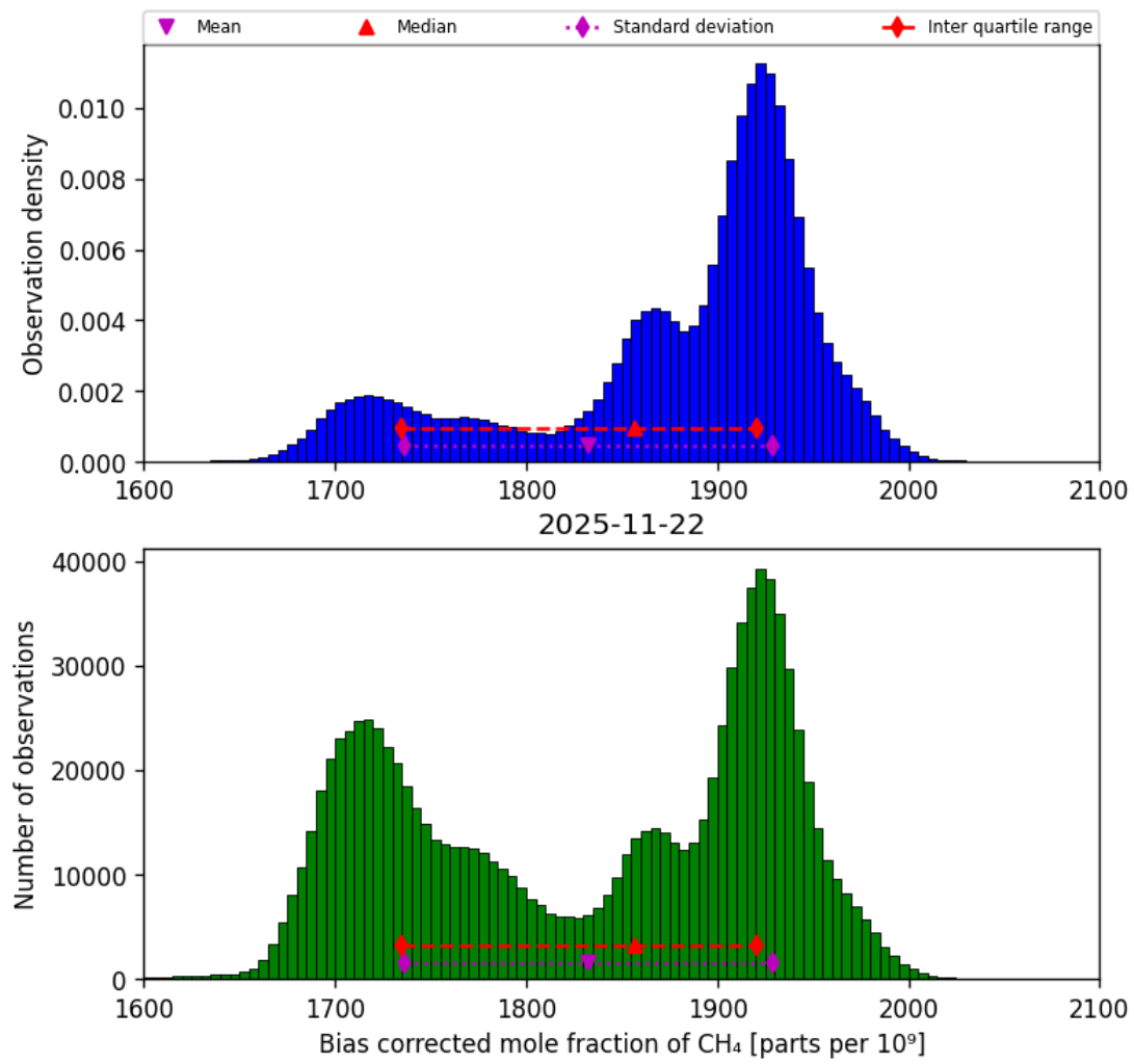
Figure 25: Histogram of “Bias corrected mole fraction of CH 4 ” for 2025-11-21 to 2025-11-23
