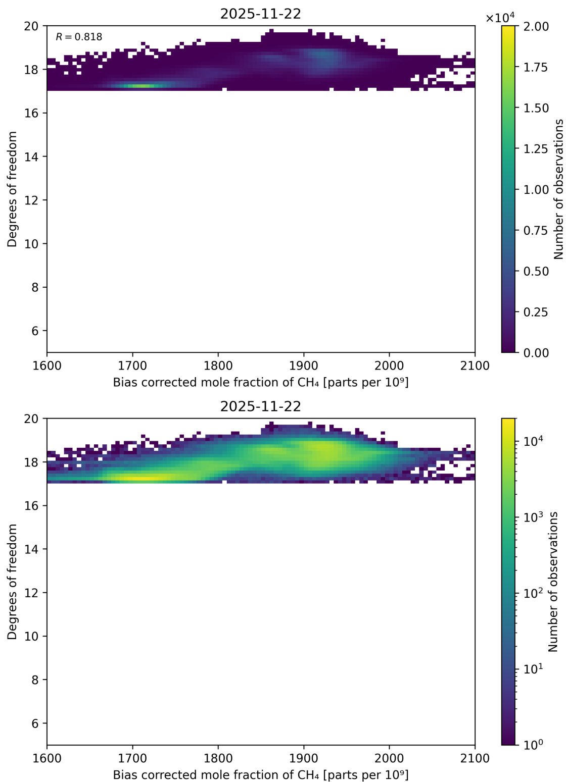
Figure 65: Scatter density plot of “Bias corrected mole fraction of \text{CH}_4 ” against “Degrees of freedom” for 2025-11-21 to 2025-11-23.
