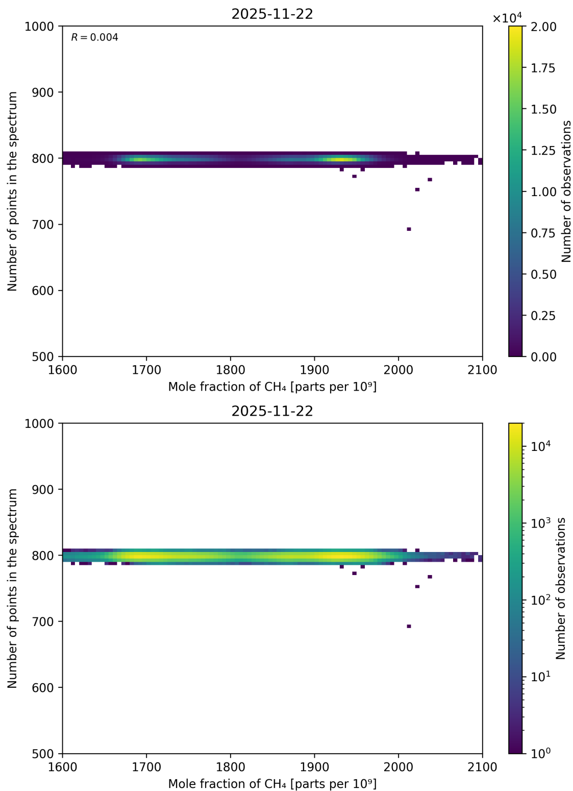
Figure 77: Scatter density plot of “Mole fraction of CH 4 ” against “Number of points in the spectrum” for 2025-11-21 to 2025-11-23.
