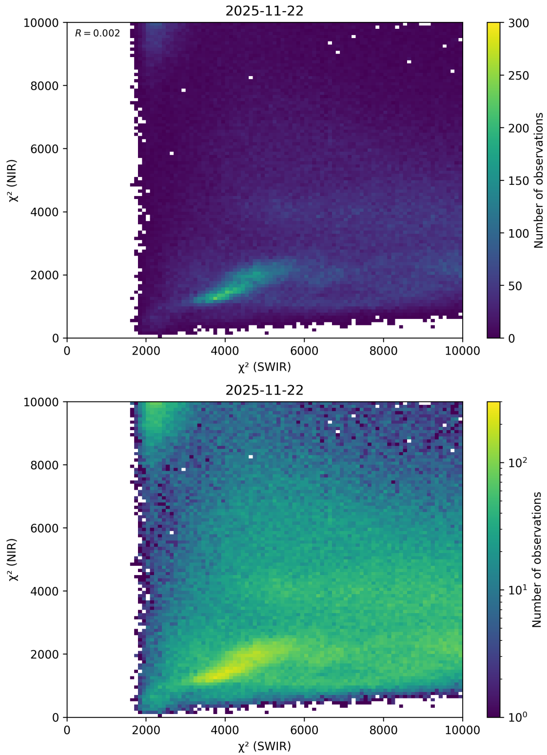
Figure 47: Scatter density plot of “ \chi^2 (SWIR)” against “ \chi^2 (NIR)” for 2025-11-21 to 2025-11-23.
