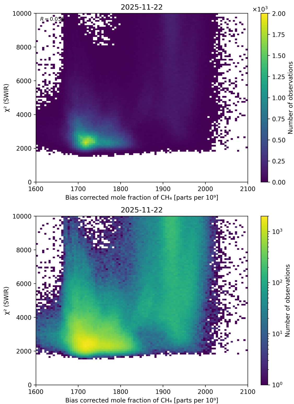
Figure 64: Scatter density plot of “Bias corrected mole fraction of \text{CH}_4 ” against “ \chi^2 (SWIR)” for 2025-11-21 to 2025-11-23.
