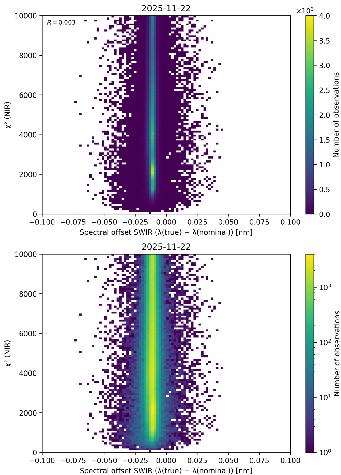
Figure 117: Scatter density plot of “Spectral offset SWIR ( \lambda_{\text{true}} - \lambda_{\text{nominal}} )” against “ \chi^2 (NIR)” for 2025-11-21 to 2025-11-23.
