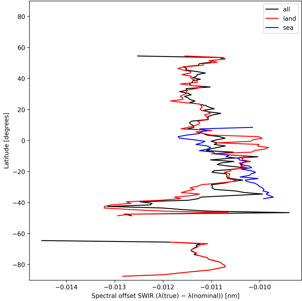
Figure 16: Zonal average of “Spectral offset SWIR ( \lambda_{\text{true}} - \lambda_{\text{nominal}} )” for 2025-11-21 to 2025-11-23.
