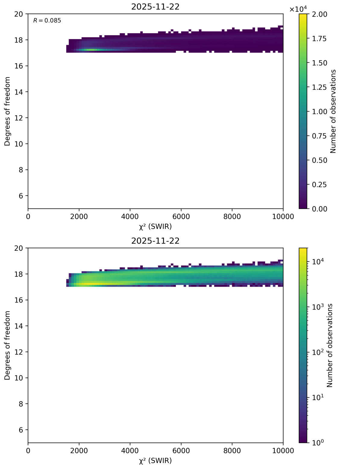
Figure 48: Scatter density plot of “ \chi^2 (SWIR)” against “Degrees of freedom” for 2025-11-21 to 2025-11-23.
