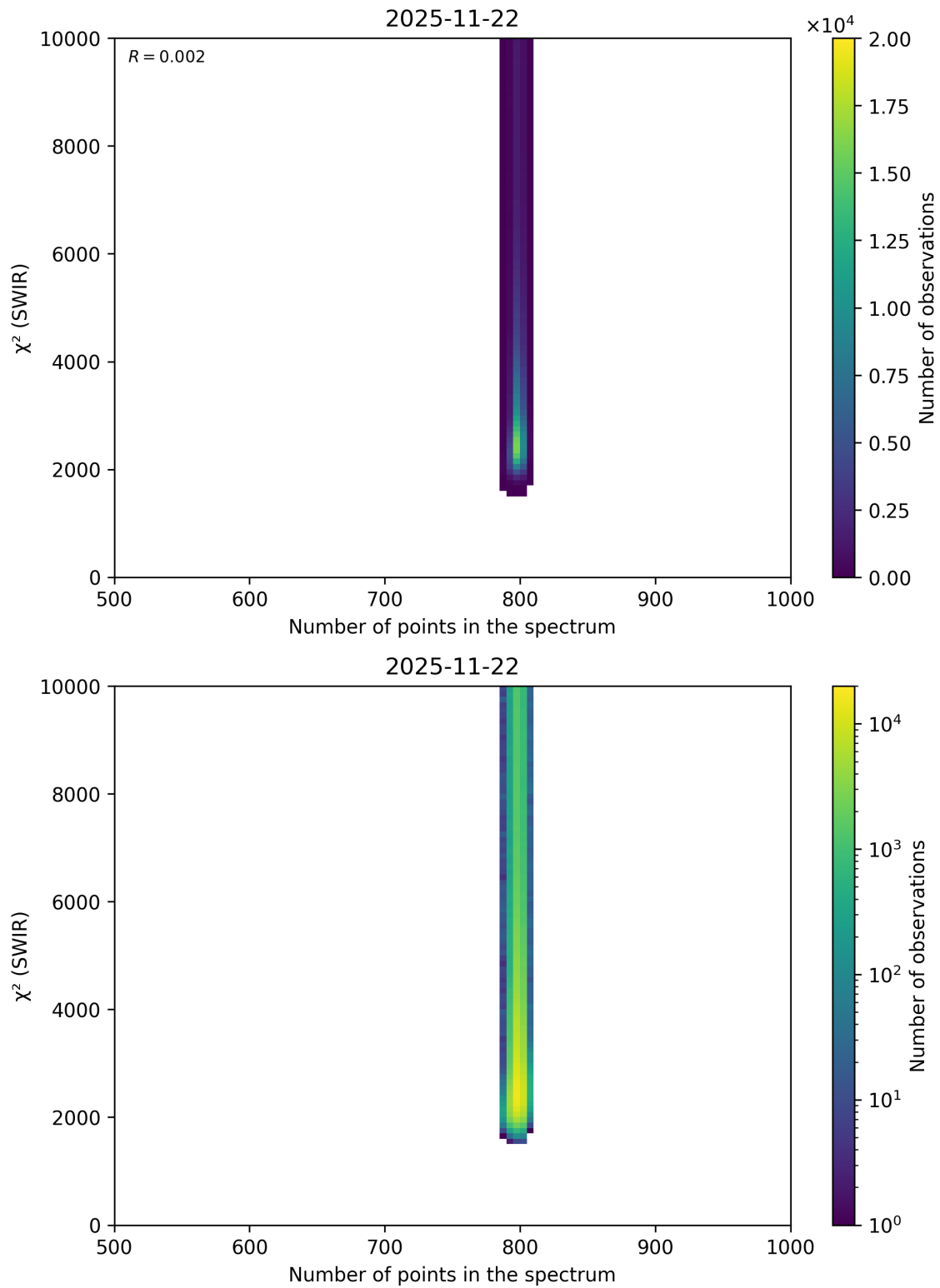
Figure 89: Scatter density plot of “Number of points in the spectrum” against “ \chi^2 (SWIR)” for 2025-11-21 to 2025-11-23.
