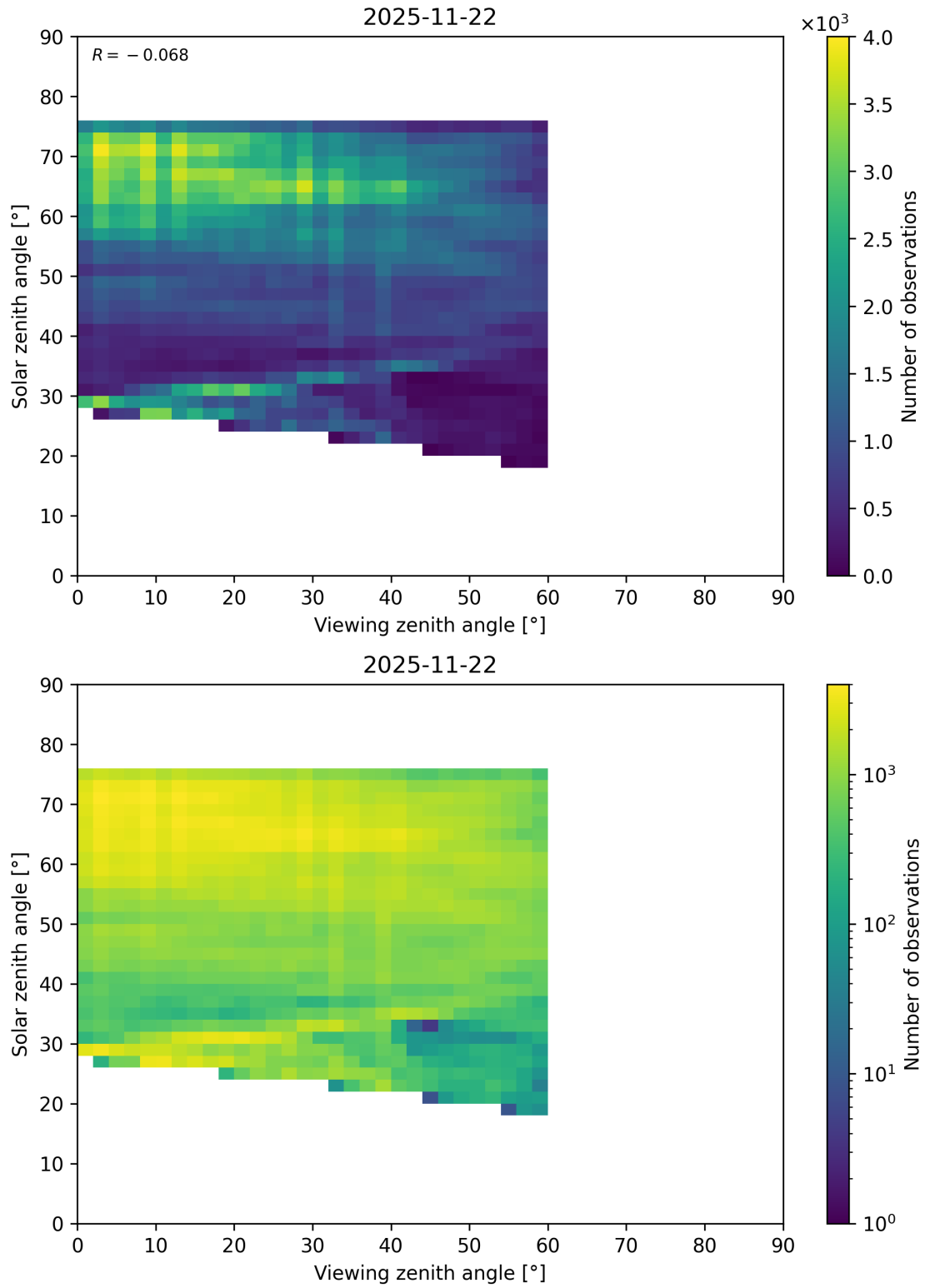
Figure 115: Scatter density plot of “Viewing zenith angle” against “Solar zenith angle” for 2025-11-21 to 2025-11-23.
