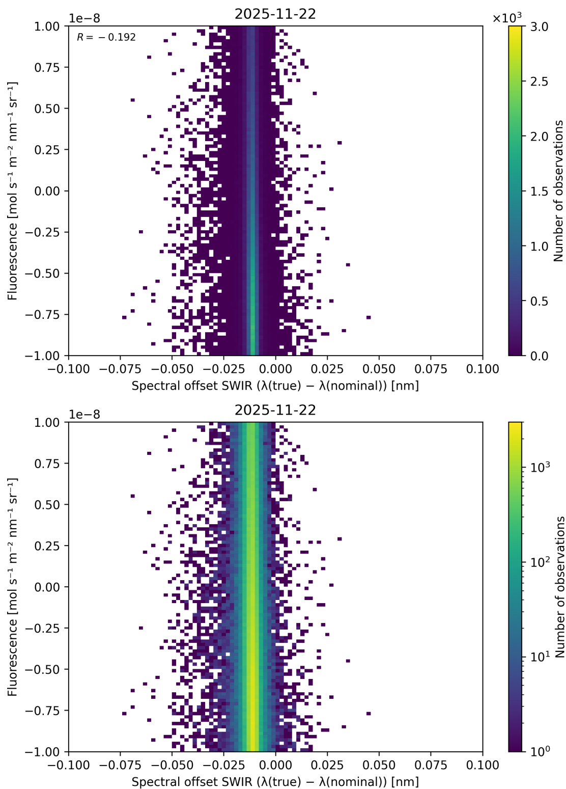
Figure 120: Scatter density plot of “Spectral offset SWIR ( \lambda_{\text{true}} - \lambda_{\text{nominal}} )” against “Fluorescence” for 2025-11-21 to 2025-11-23.
