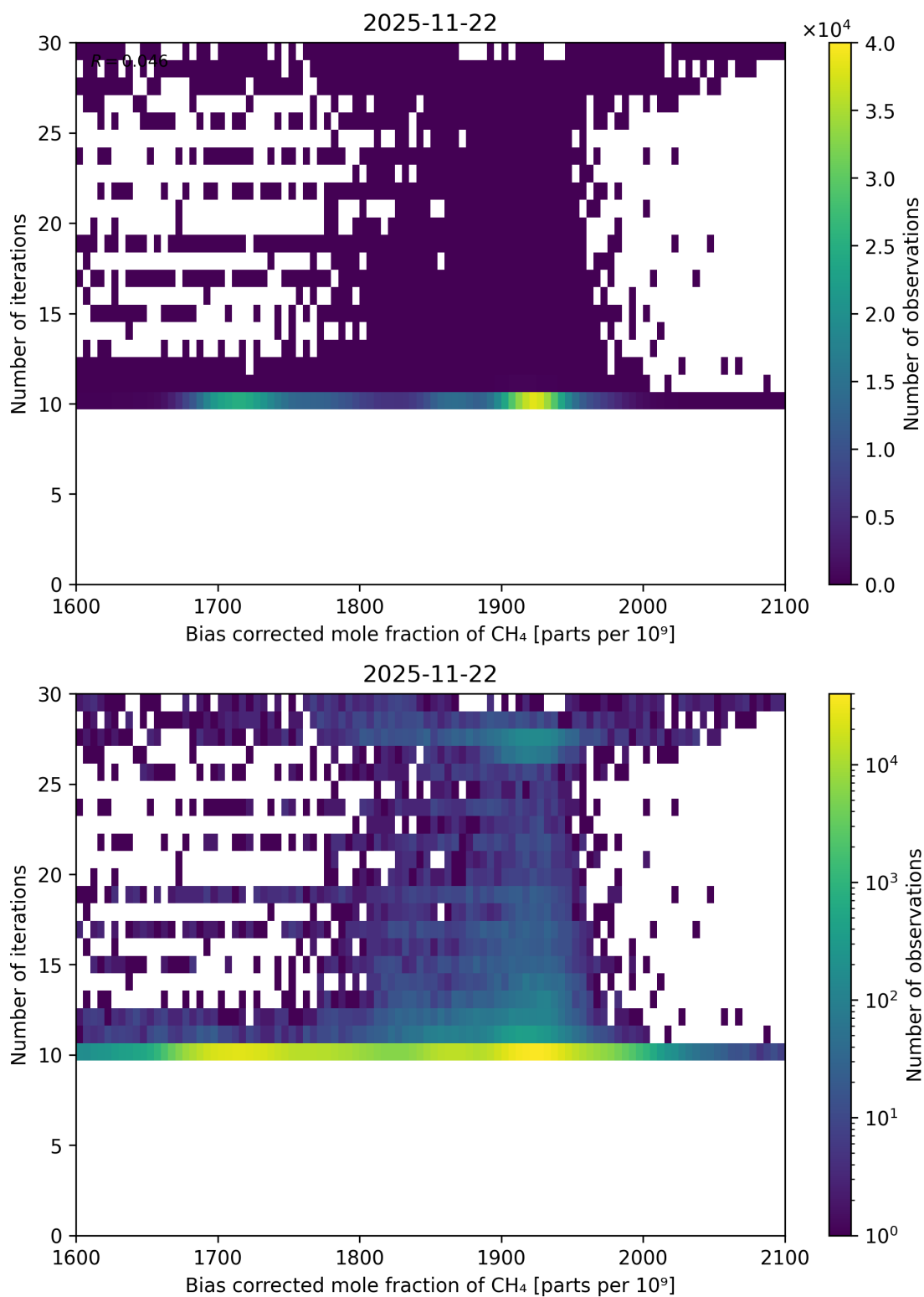
Figure 67: Scatter density plot of “Bias corrected mole fraction of \text{CH}_4 ” against “Number of iterations” for 2025-11-21 to 2025-11-23.
