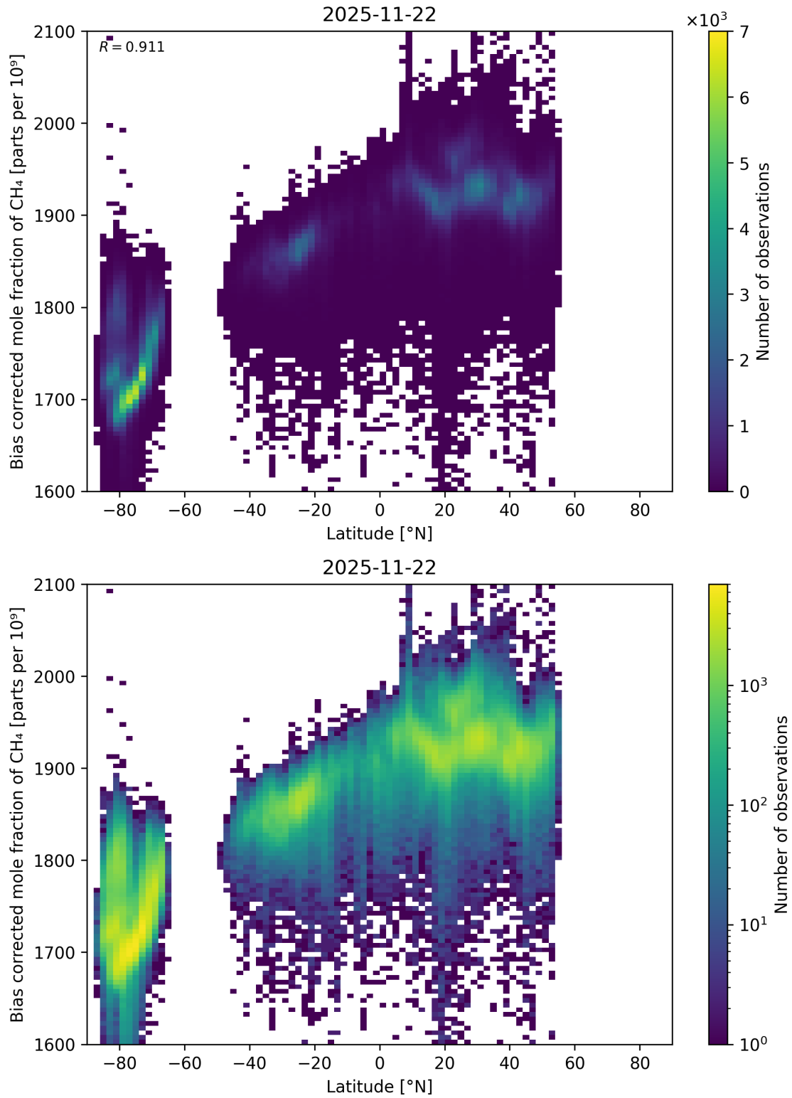
Figure 58: Scatter density plot of “Latitude” against “Bias corrected mole fraction of CH 4 ” for 2025-11-21 to 2025-11-23.
