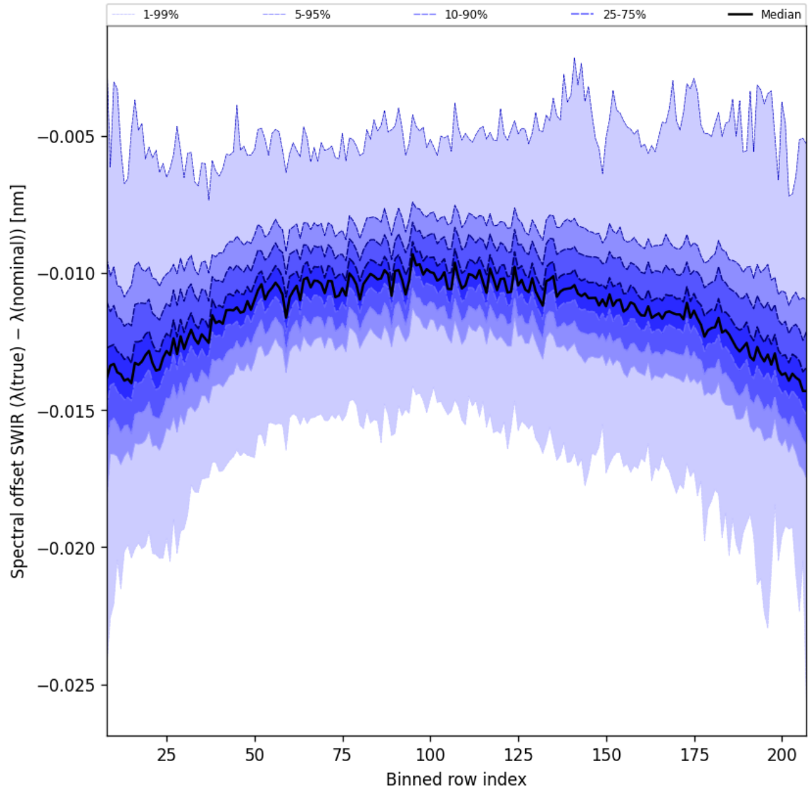
Figure 38: Along track statistics of “Spectral offset SWIR ( \lambda_{\text{true}} - \lambda_{\text{nominal}} )” for 2025-11-21 to 2025-11-23
