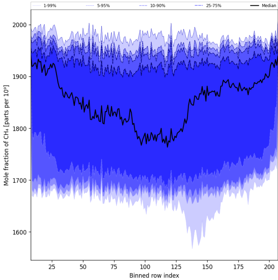
Figure 34: Along track statistics of “Mole fraction of CH 4 ” for 2025-11-21 to 2025-11-23
