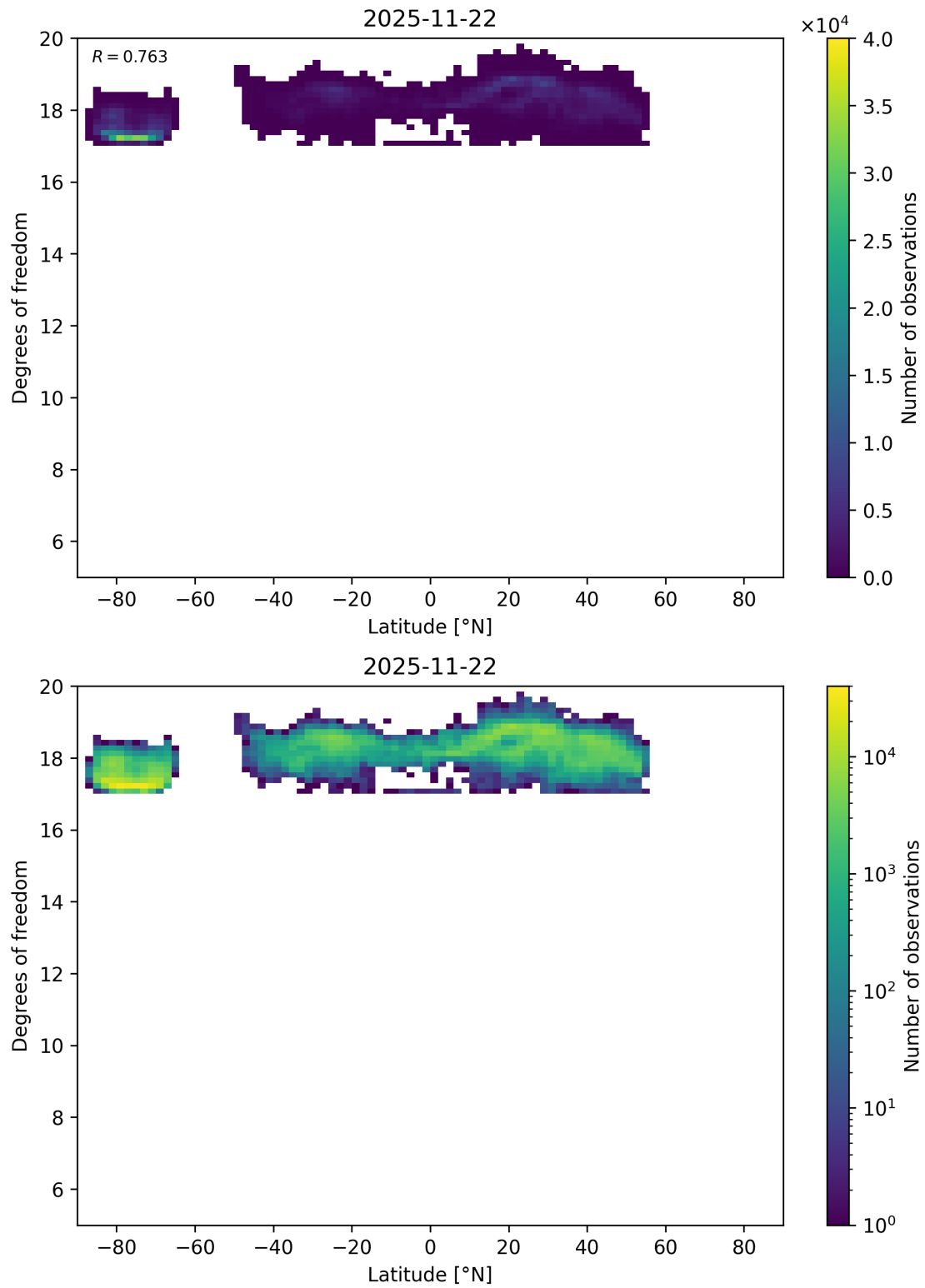
Figure 55: Scatter density plot of “Latitude” against “Degrees of freedom” for 2025-11-21 to 2025-11-23.
