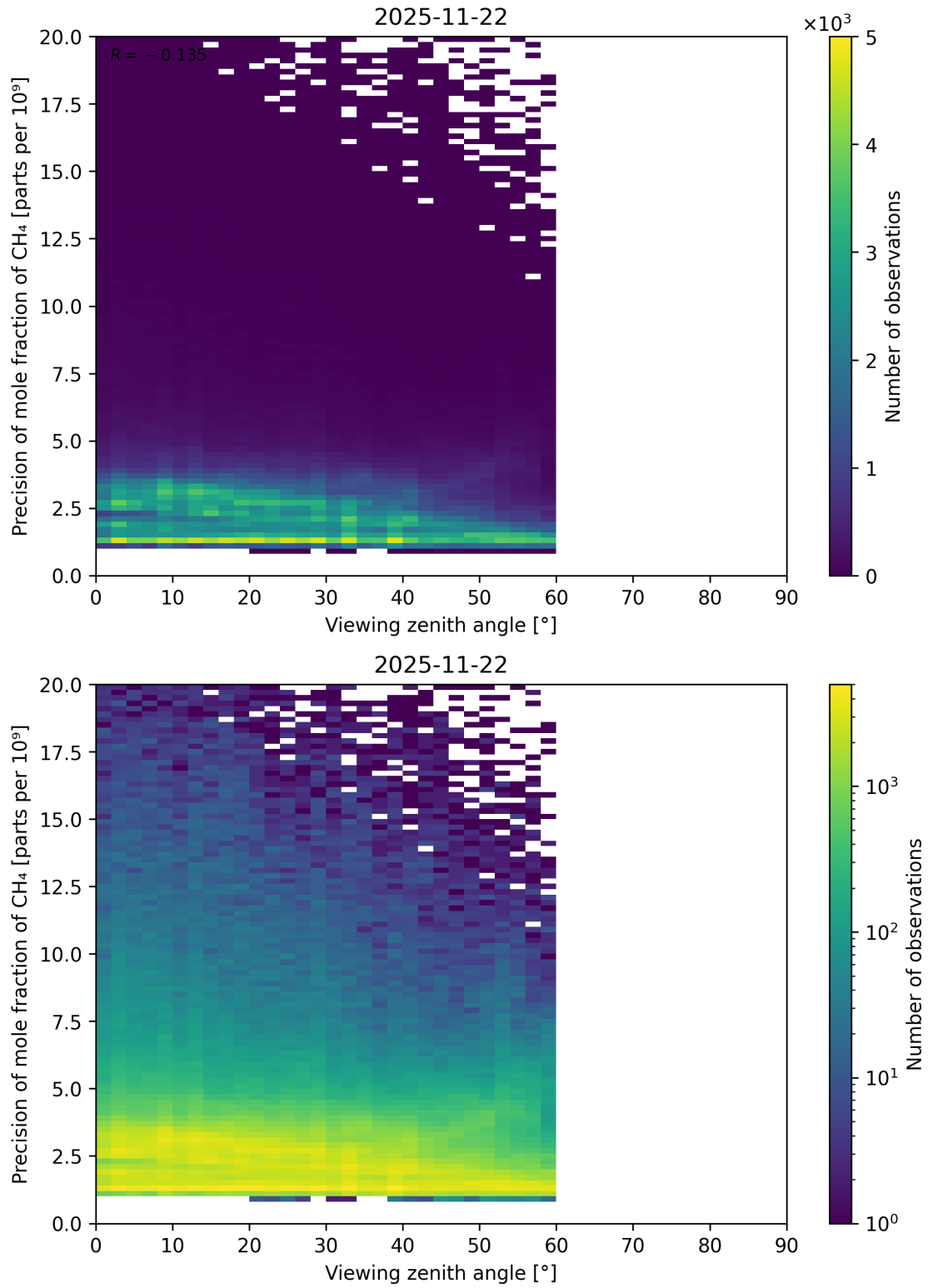
Figure 112: Scatter density plot of “Viewing zenith angle” against “Precision of mole fraction of CH 4 ” for 2025-11-21 to 2025-11-23.
