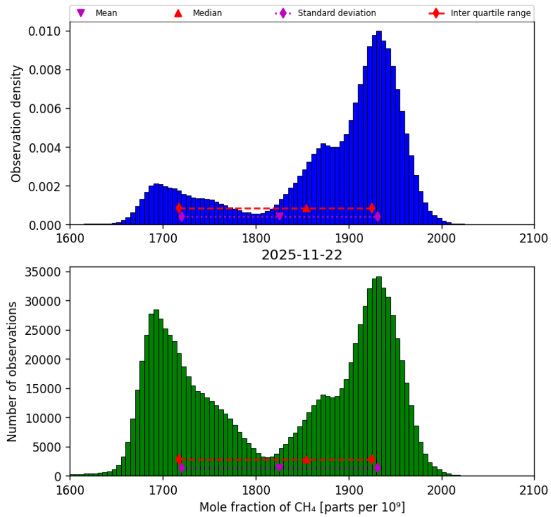
Figure 23: Histogram of “Mole fraction of CH 4 ” for 2025-11-21 to 2025-11-23
