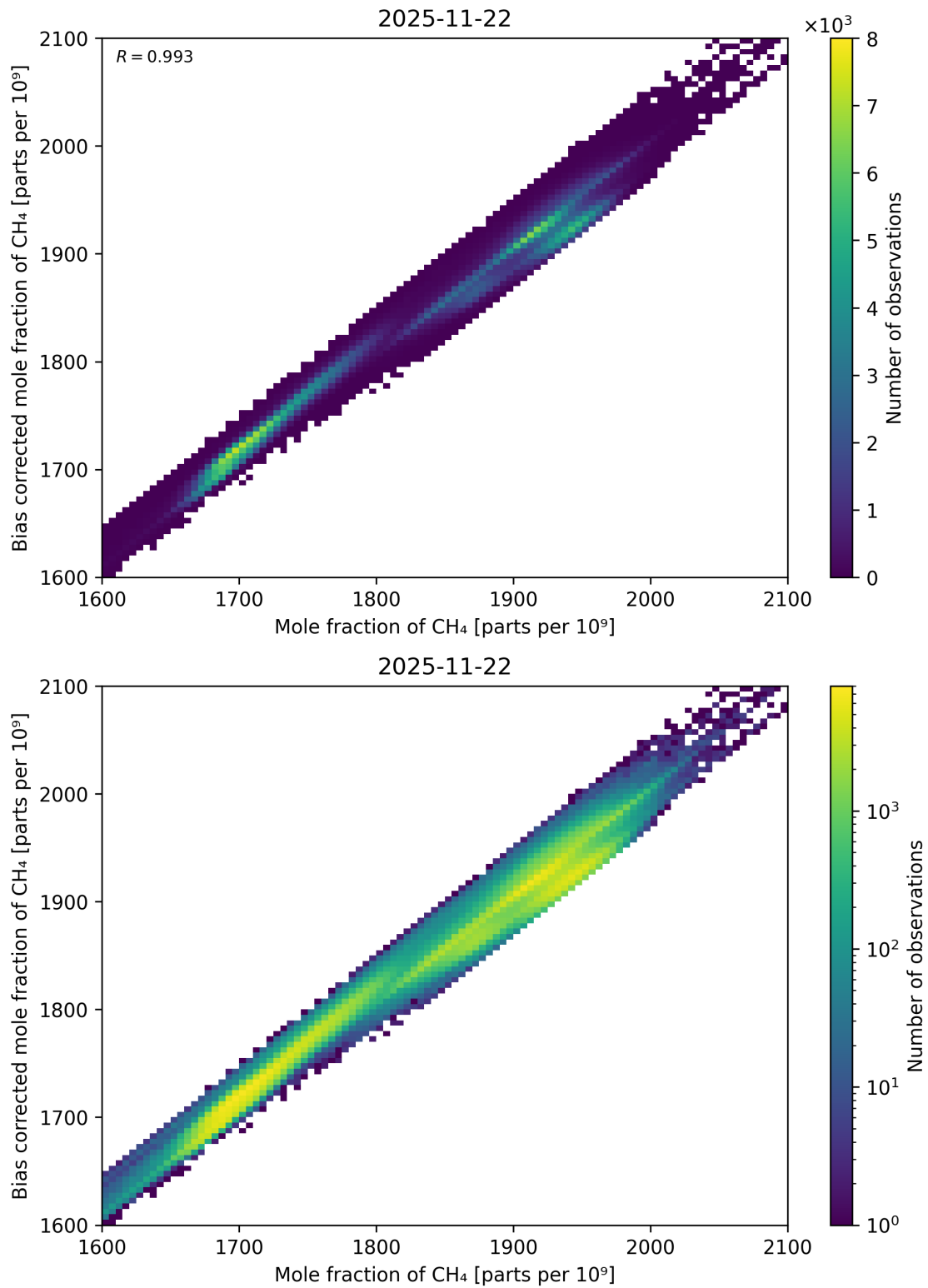
Figure 74: Scatter density plot of “Mole fraction of CH 4 ” against “Bias corrected mole fraction of CH 4 ” for 2025-11-21 to 2025-11-23.
