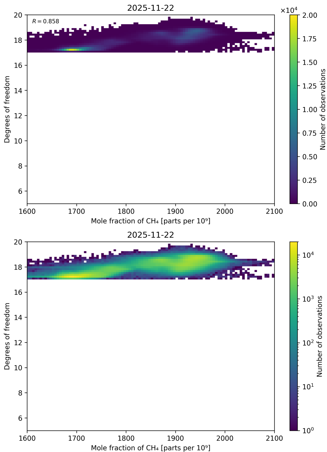
Figure 72: Scatter density plot of “Mole fraction of CH 4 ” against “Degrees of freedom” for 2025-11-21 to 2025-11-23.
