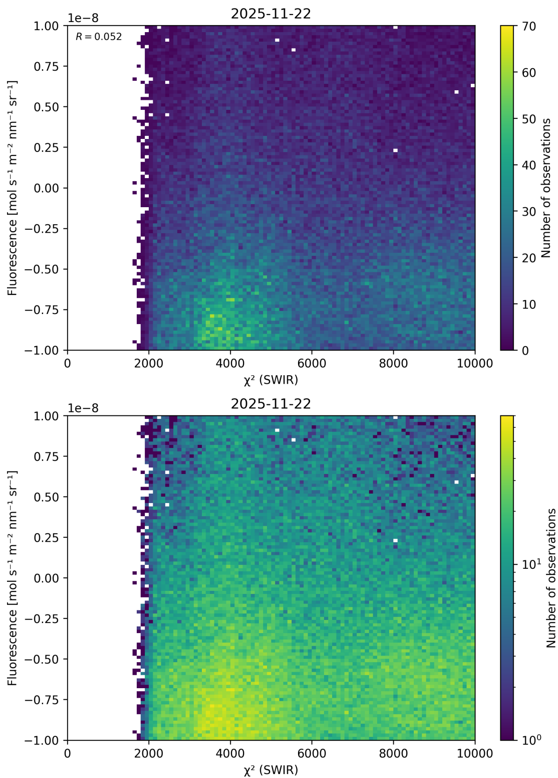
Figure 49: Scatter density plot of “ \chi^2 (SWIR)” against “Fluorescence” for 2025-11-21 to 2025-11-23.
