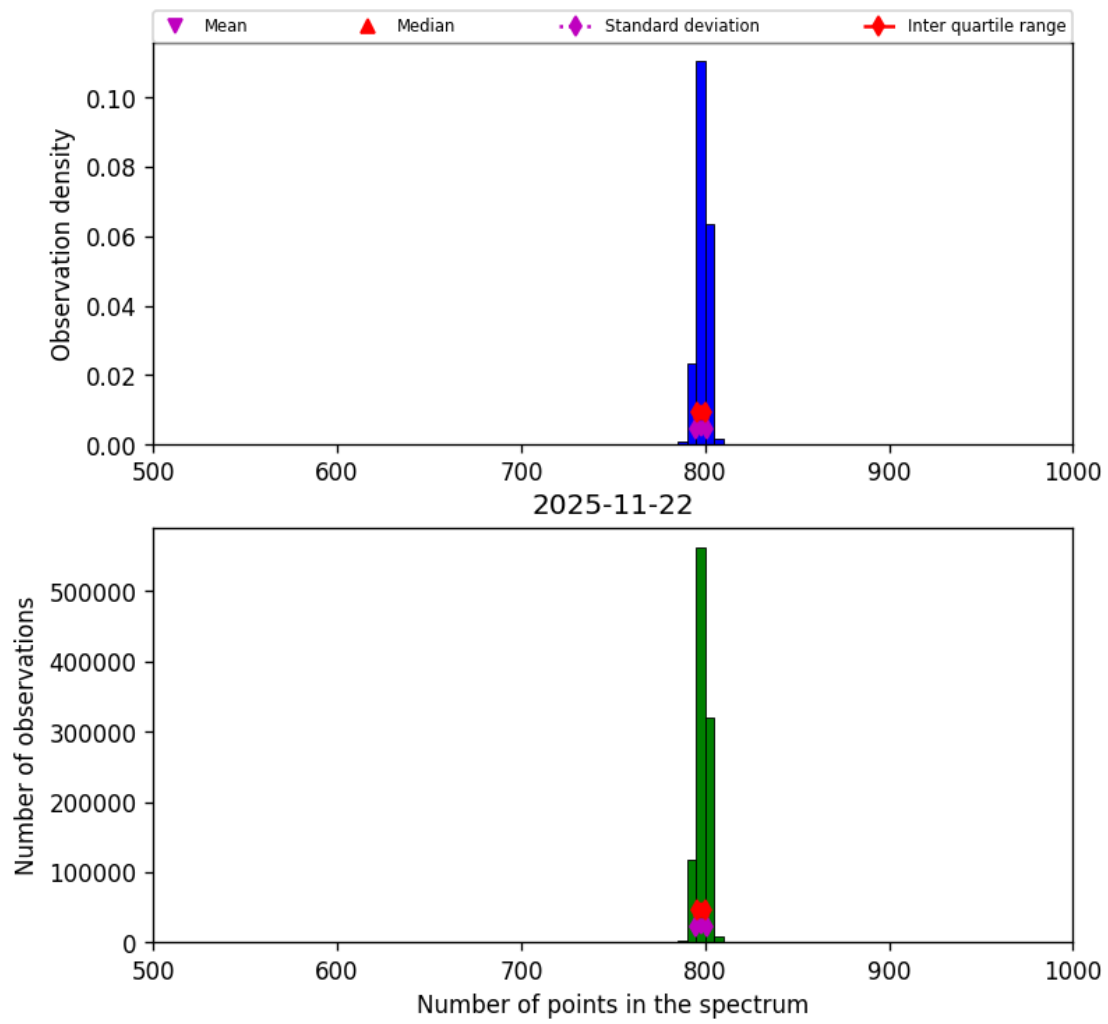
Figure 26: Histogram of “Number of points in the spectrum” for 2025-11-21 to 2025-11-23
