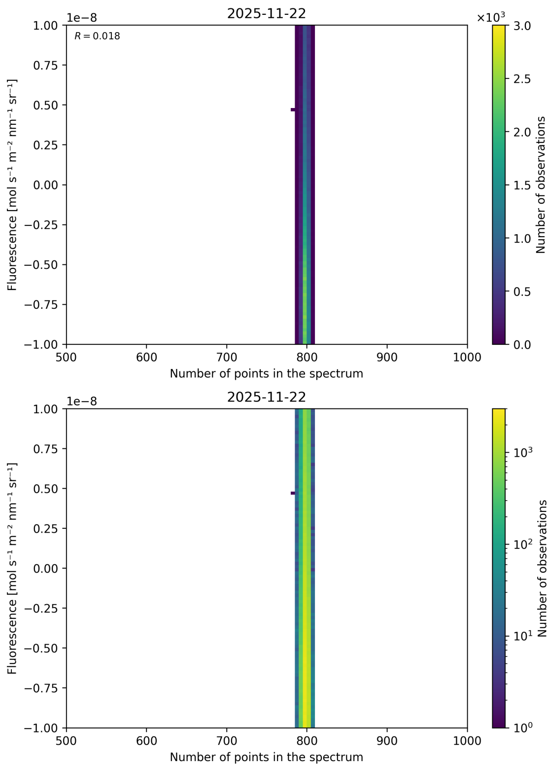
Figure 91: Scatter density plot of “Number of points in the spectrum” against “Fluorescence” for 2025-11-21 to 2025-11-23.
