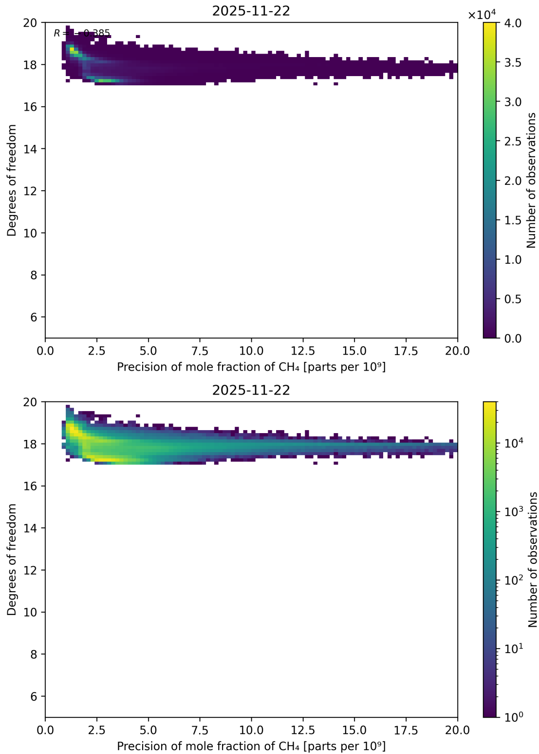
Figure 80: Scatter density plot of “Precision of mole fraction of CH 4 ” against “Degrees of freedom” for 2025-11-21 to 2025-11-23.
