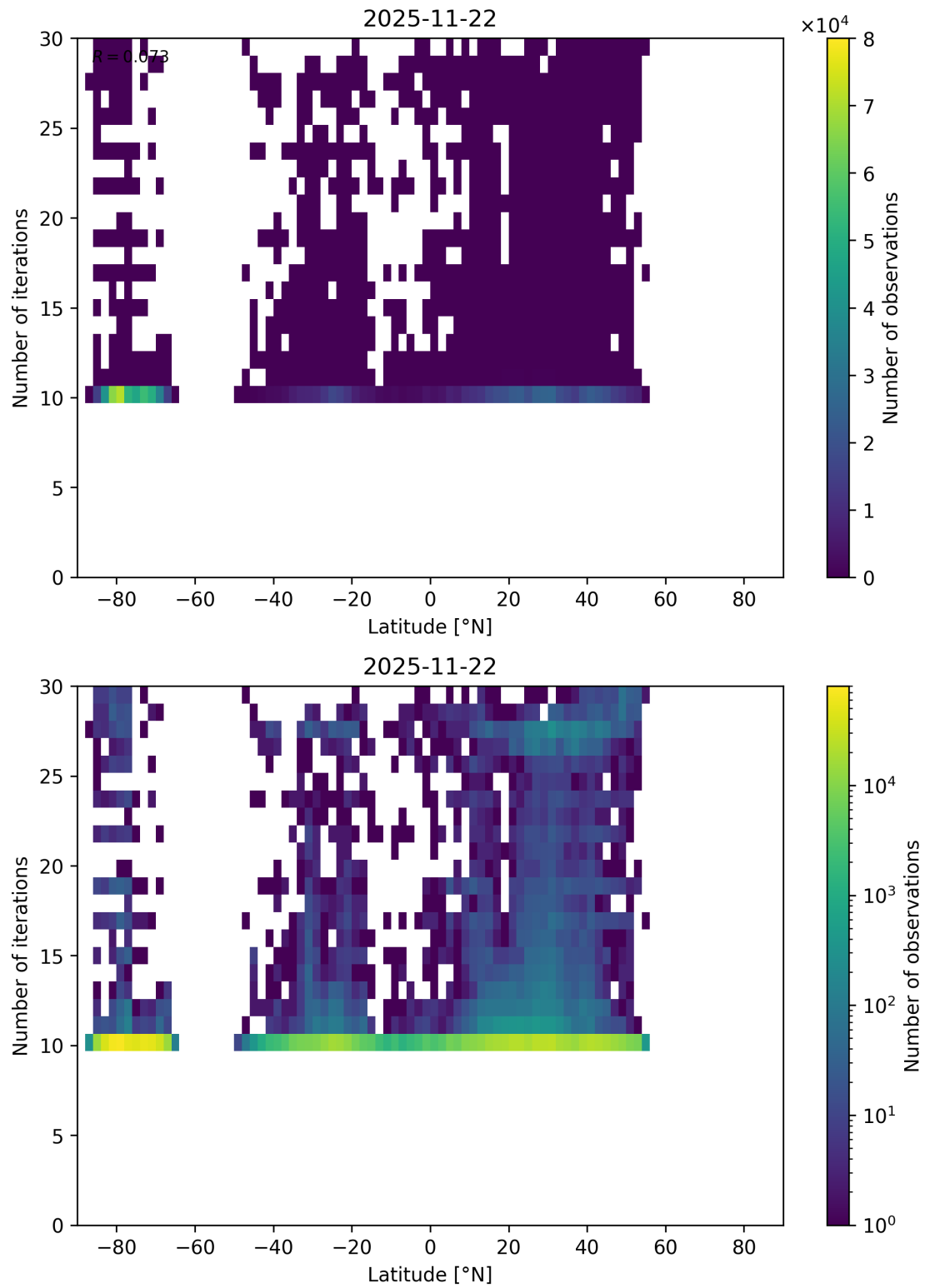
Figure 60: Scatter density plot of “Latitude” against “Number of iterations” for 2025-11-21 to 2025-11-23.
