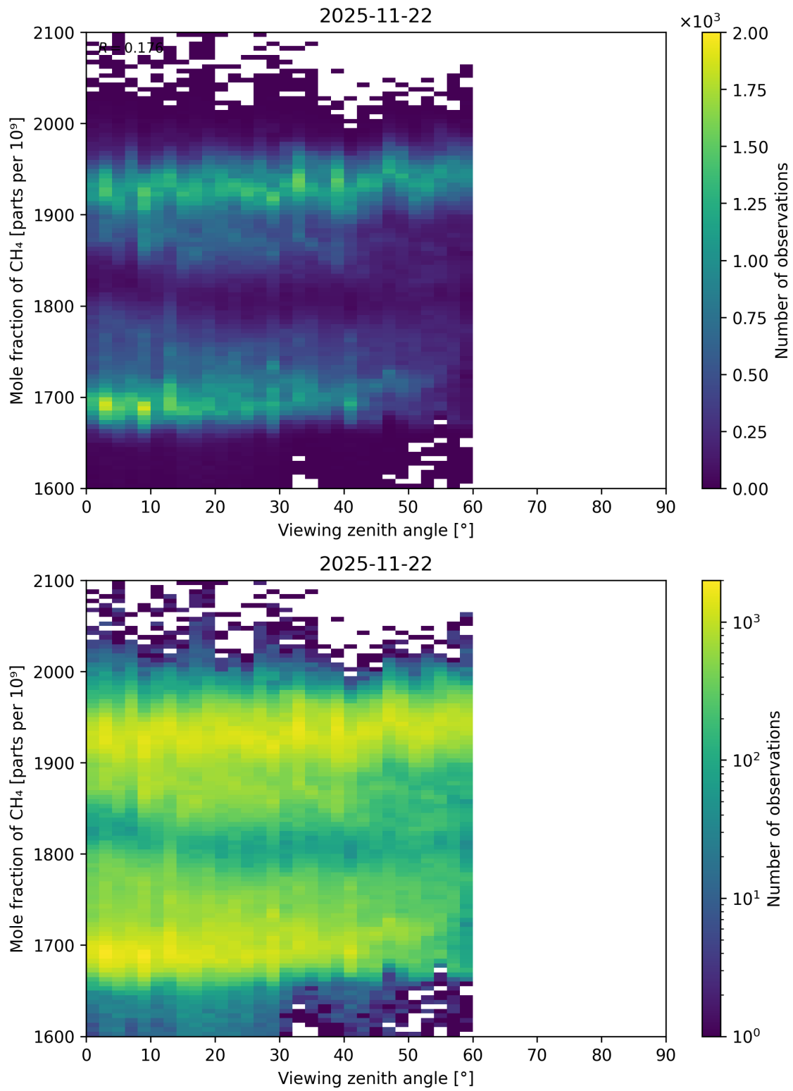
Figure 110: Scatter density plot of “Viewing zenith angle” against “Mole fraction of CH 4 ” for 2025-11-21 to 2025-11-23.
