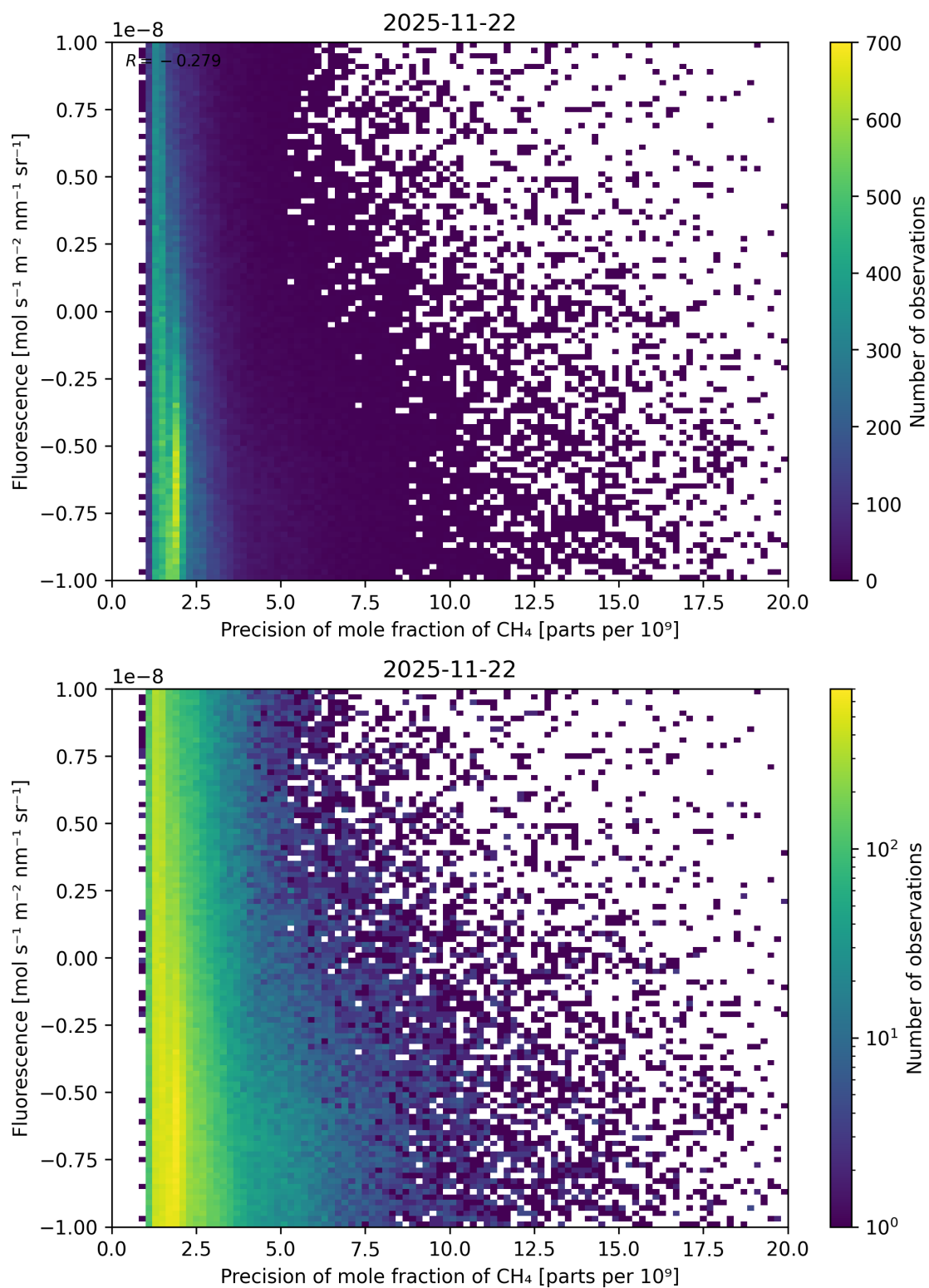
Figure 81: Scatter density plot of “Precision of mole fraction of CH 4 ” against “Fluorescence” for 2025-11-21 to 2025-11-23.
