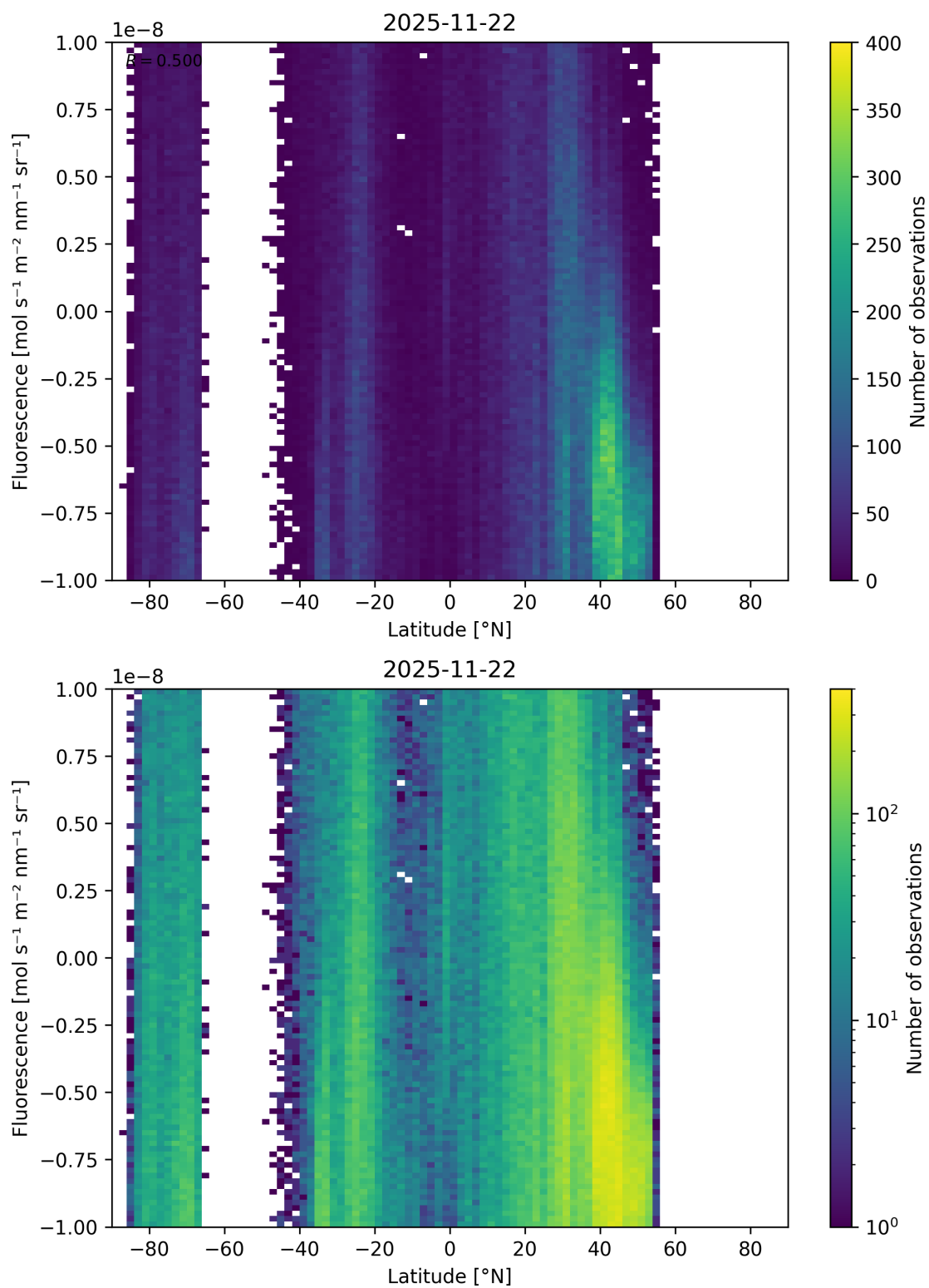
Figure 56: Scatter density plot of “Latitude” against “Fluorescence” for 2025-11-21 to 2025-11-23.
