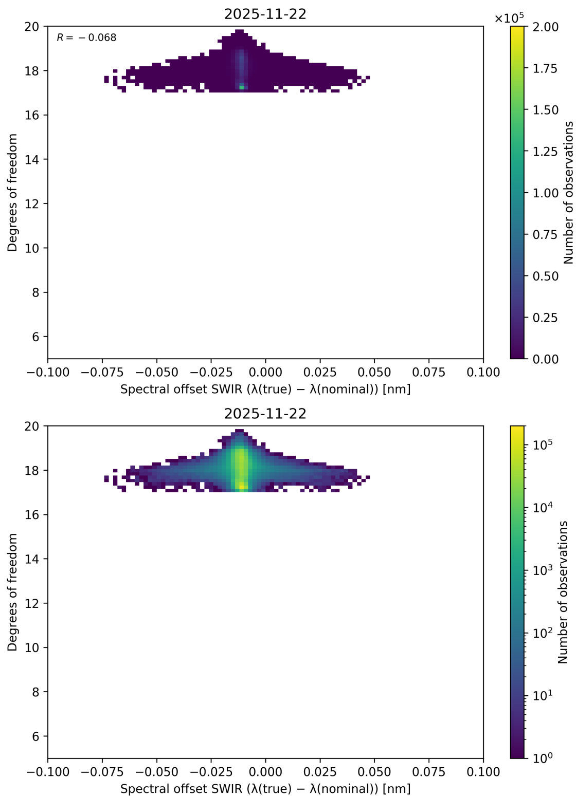
Figure 119: Scatter density plot of “Spectral offset SWIR ( \lambda_{\text{true}} - \lambda_{\text{nominal}} )” against “Degrees of freedom” for 2025-11-21 to 2025-11-23.
