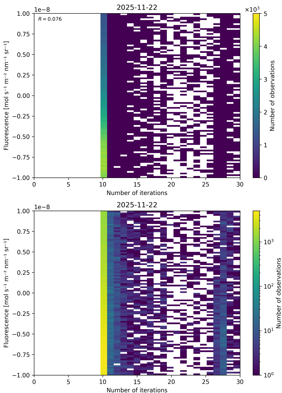
Figure 87: Scatter density plot of “Number of iterations” against “Fluorescence” for 2025-11-21 to 2025-11-23.
