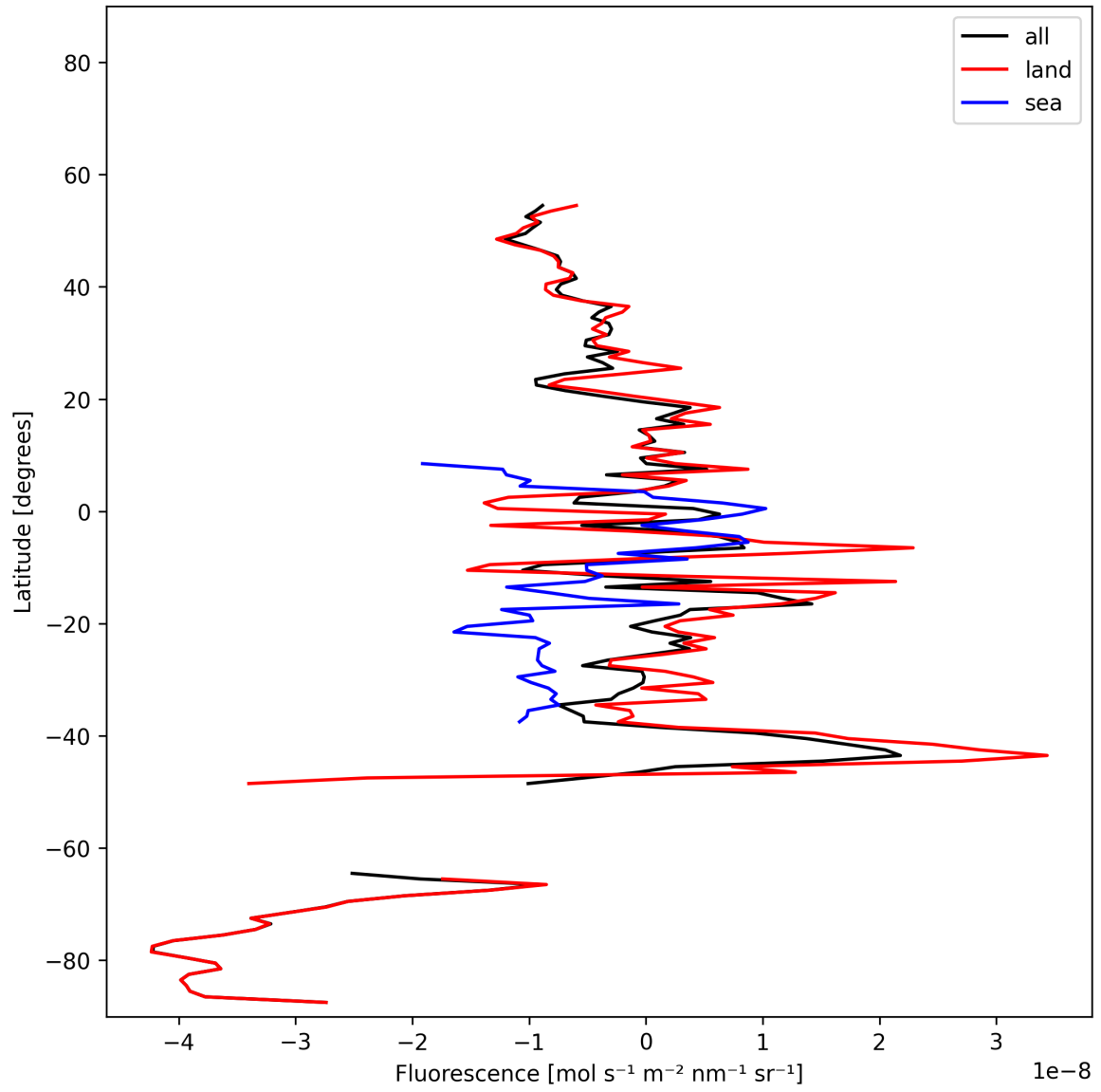
Figure 21: Zonal average of “Fluorescence” for 2025-11-21 to 2025-11-23.
