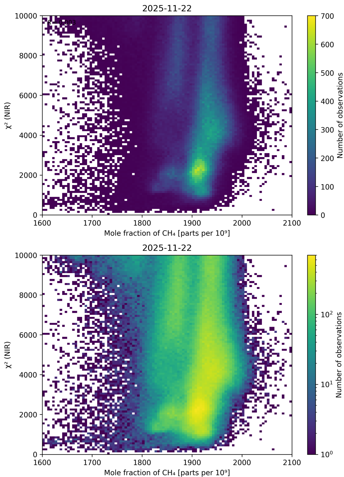
Figure 70: Scatter density plot of “Mole fraction of CH 4 ” against “ \chi^2 (NIR)” for 2025-11-21 to 2025-11-23.
