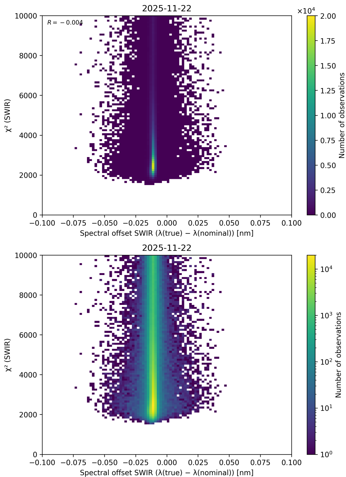
Figure 118: Scatter density plot of “Spectral offset SWIR ( \lambda_{\text{true}} - \lambda_{\text{nominal}} )” against “ \chi^2 (SWIR)” for 2025-11-21 to 2025-11-23.
