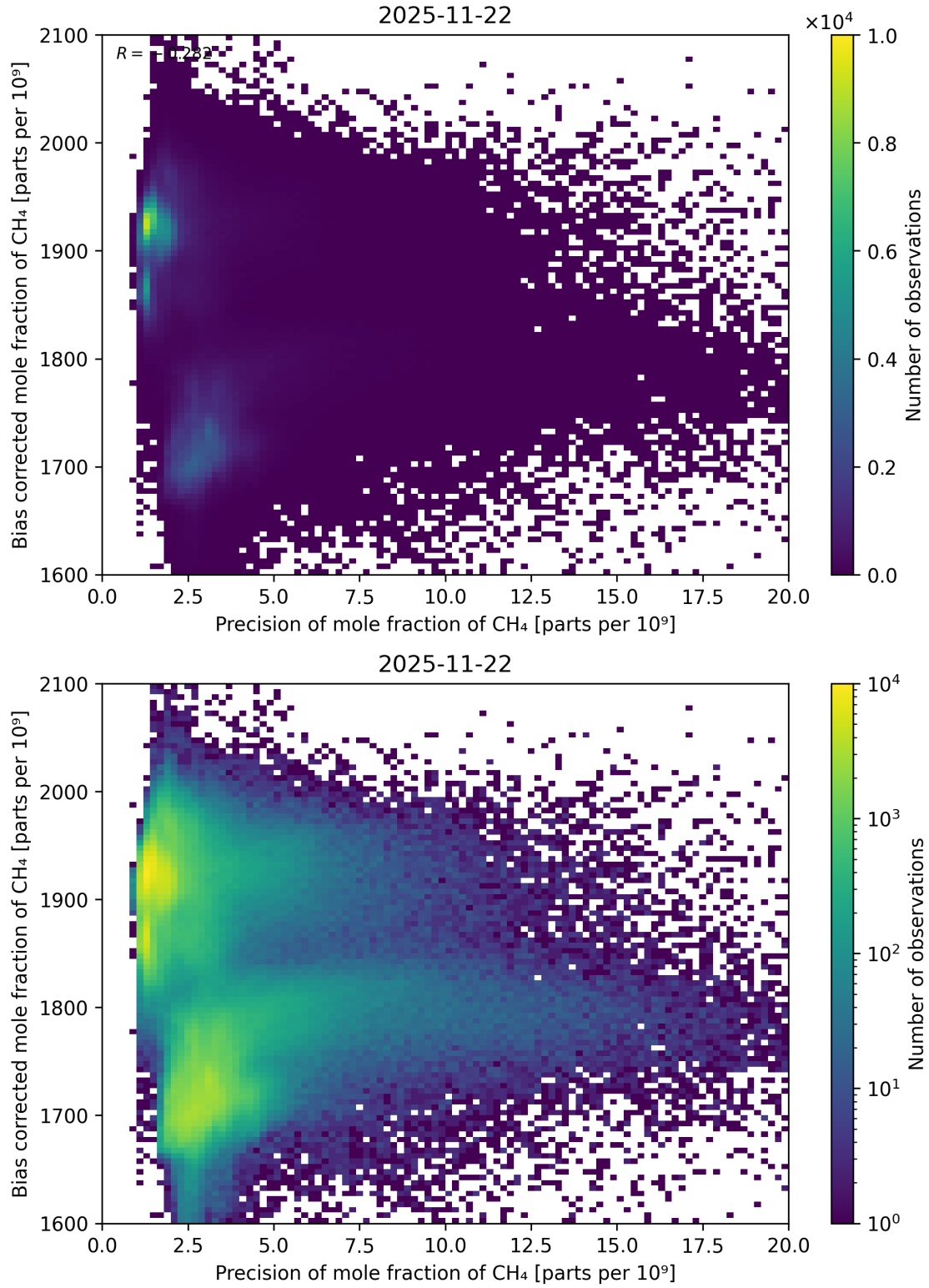
Figure 82: Scatter density plot of “Precision of mole fraction of CH 4 ” against “Bias corrected mole fraction of CH 4 ” for 2025-11-21 to 2025-11-23.
