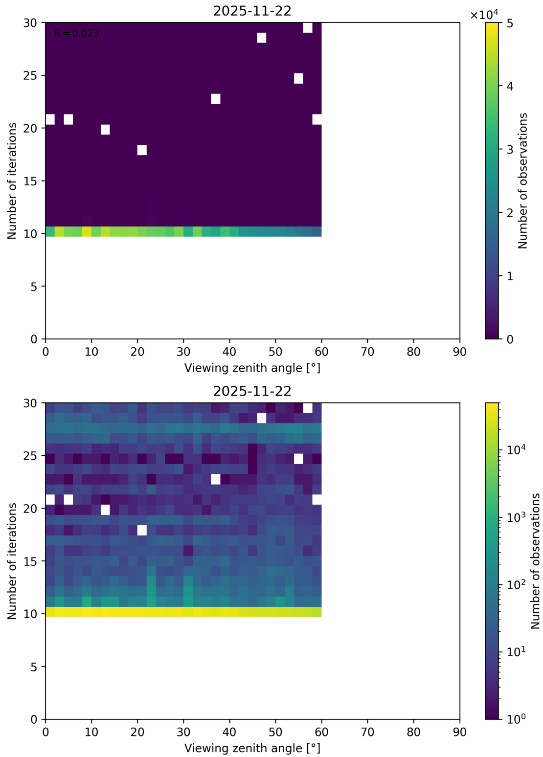
Figure 113: Scatter density plot of “Viewing zenith angle” against “Number of iterations” for 2025-11-21 to 2025-11-23.
