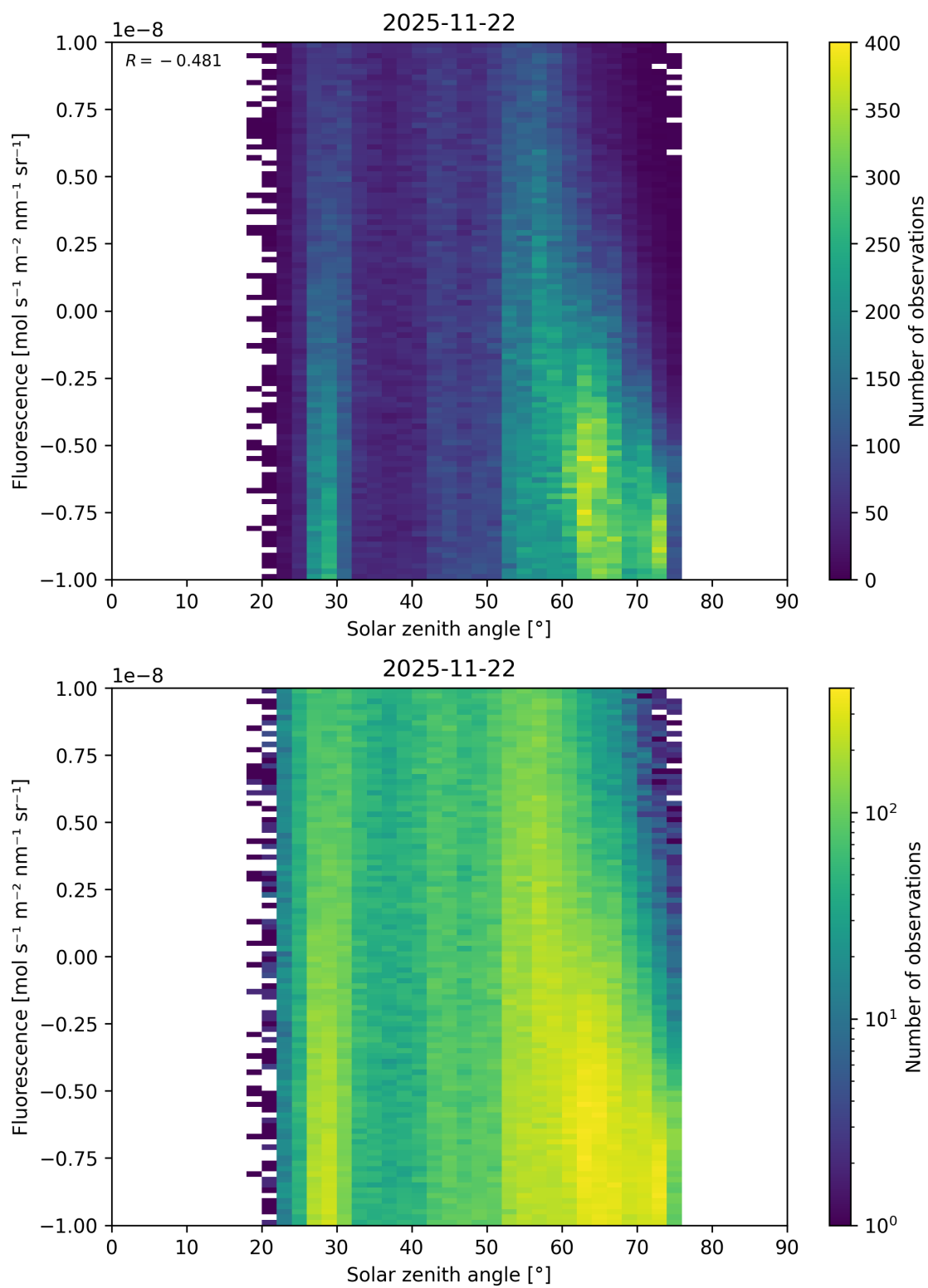
Figure 97: Scatter density plot of “Solar zenith angle” against “Fluorescence” for 2025-11-21 to 2025-11-23.
