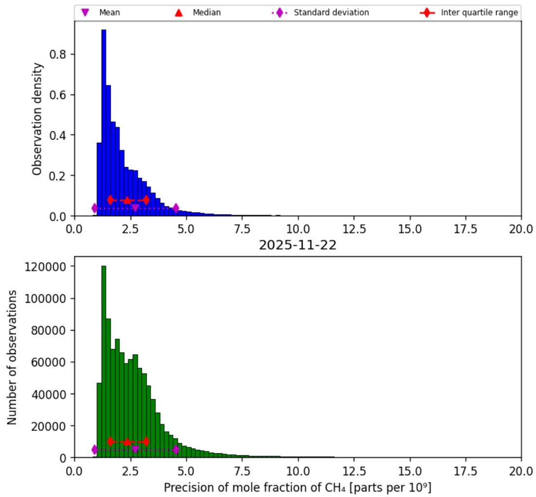
Figure 24: Histogram of “Precision of mole fraction of CH 4 ” for 2025-11-21 to 2025-11-23
