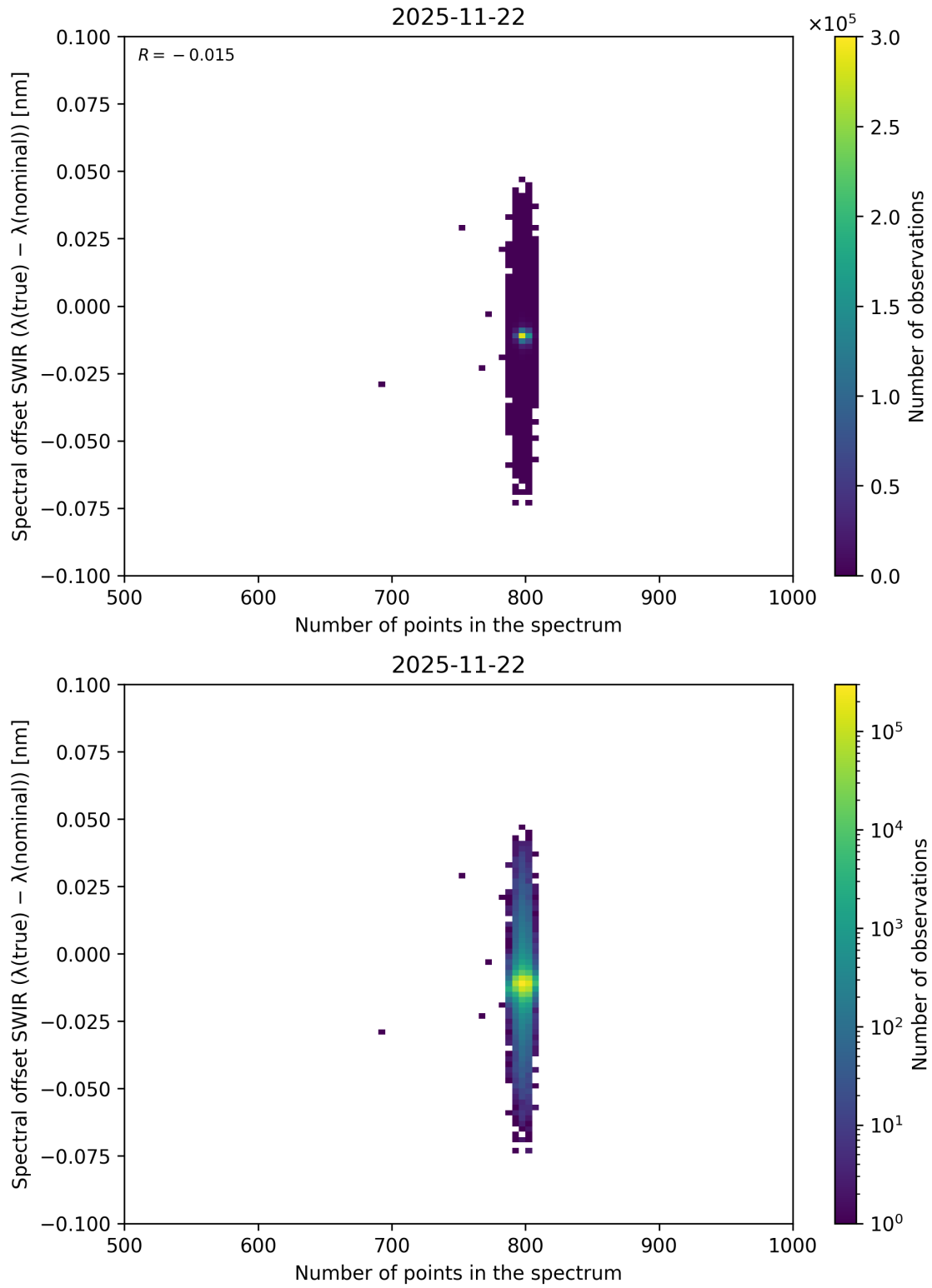
Figure 93: Scatter density plot of “Number of points in the spectrum” against “Spectral offset SWIR ( \lambda_{\text{true}} - \lambda_{\text{nominal}} )” for 2025-11-21 to 2025-11-23.
