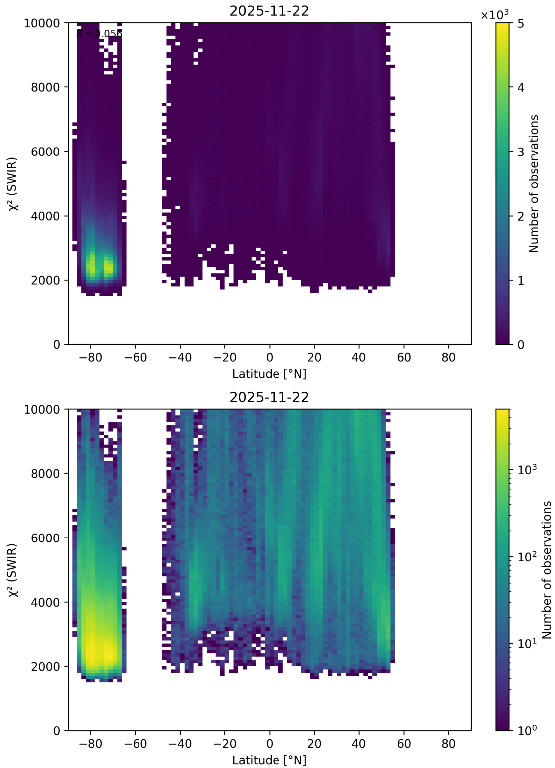
Figure 54: Scatter density plot of “Latitude” against “ \chi^2 (SWIR)” for 2025-11-21 to 2025-11-23.
