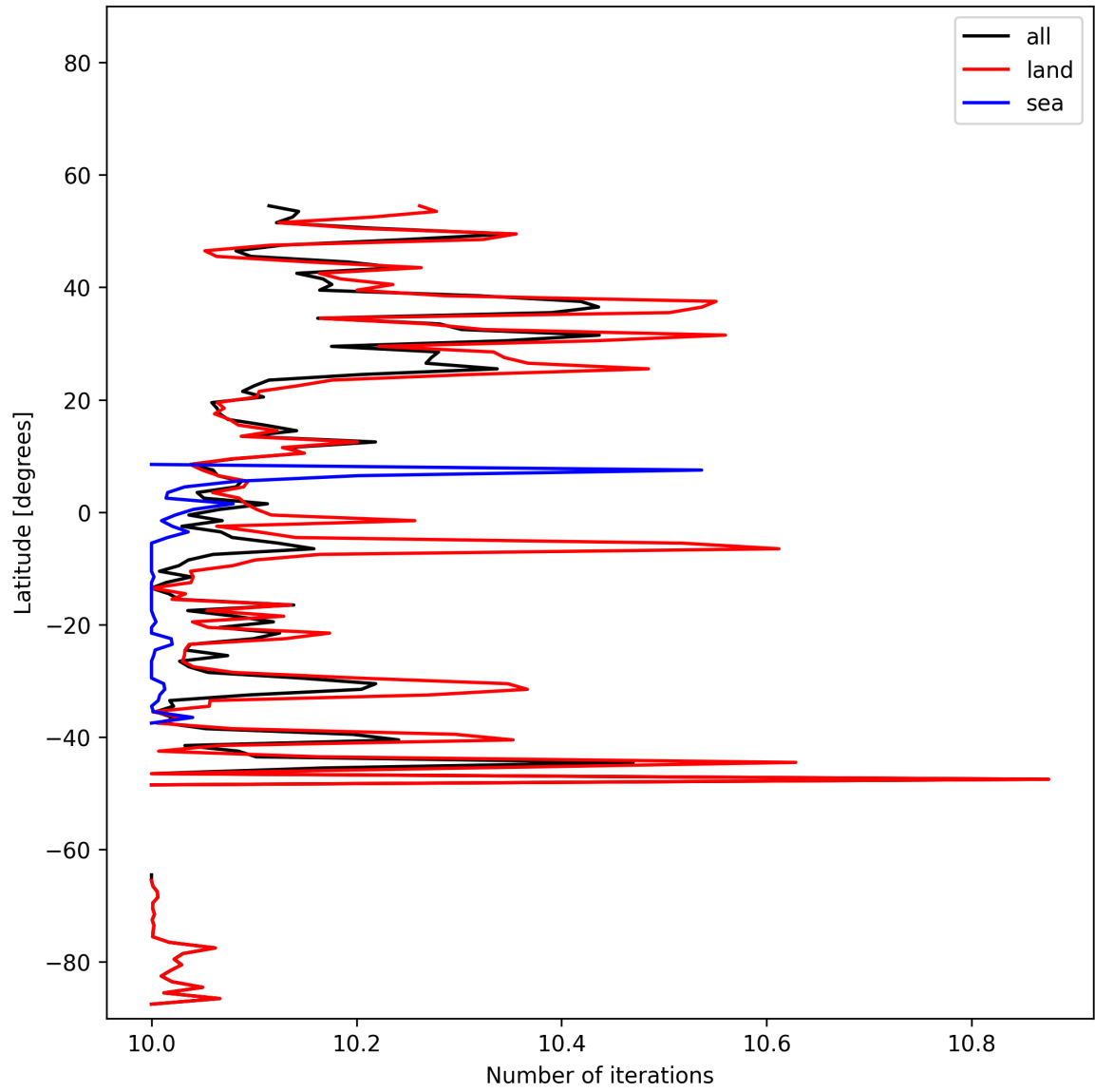
Figure 20: Zonal average of “Number of iterations” for 2025-11-21 to 2025-11-23.
