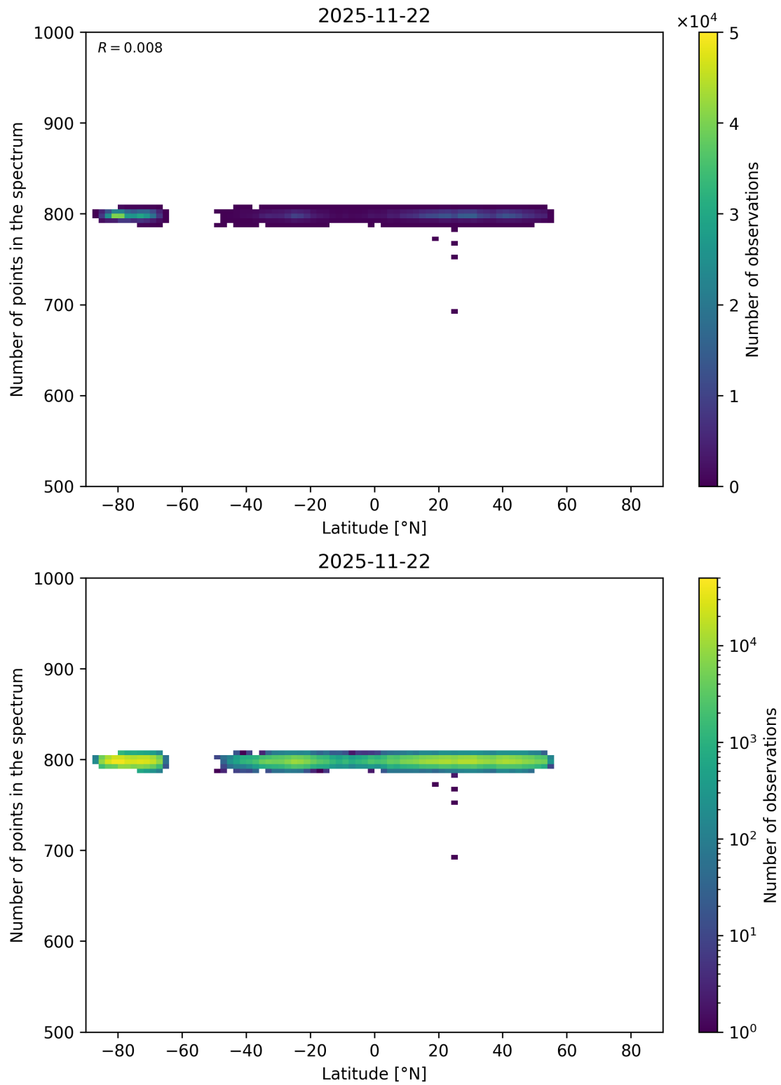
Figure 61: Scatter density plot of “Latitude” against “Number of points in the spectrum” for 2025-11-21 to 2025-11-23.
