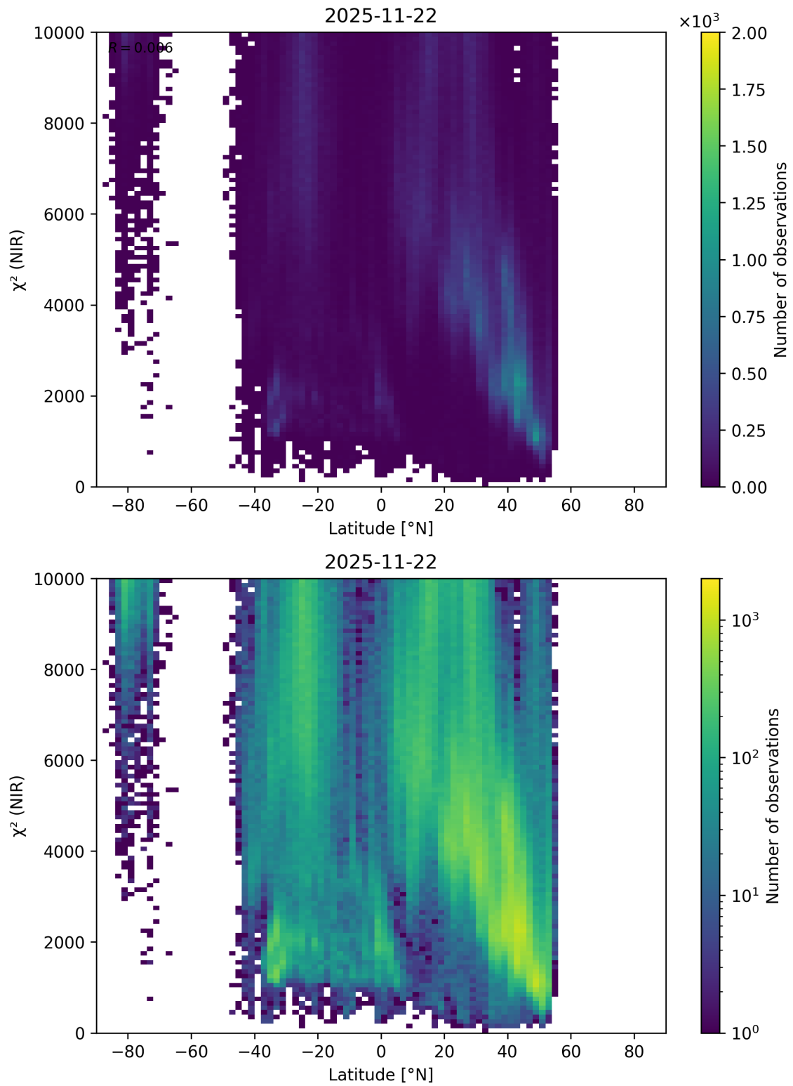
Figure 53: Scatter density plot of “Latitude” against “ \chi^2 (NIR)” for 2025-11-21 to 2025-11-23.
