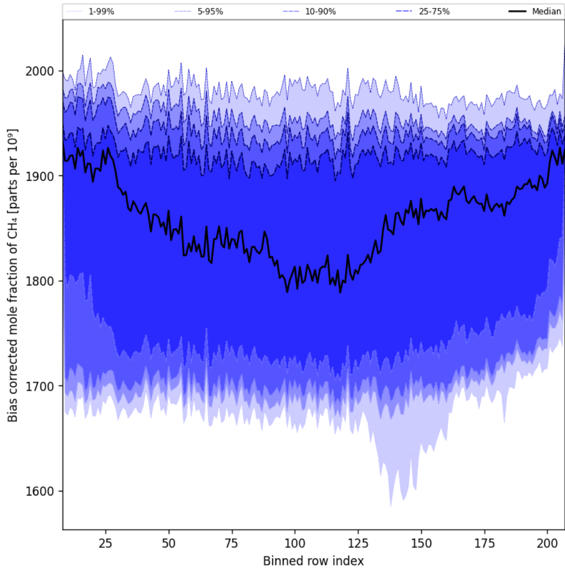
Figure 36: Along track statistics of “Bias corrected mole fraction of CH 4 ” for 2025-11-21 to 2025-11-23
