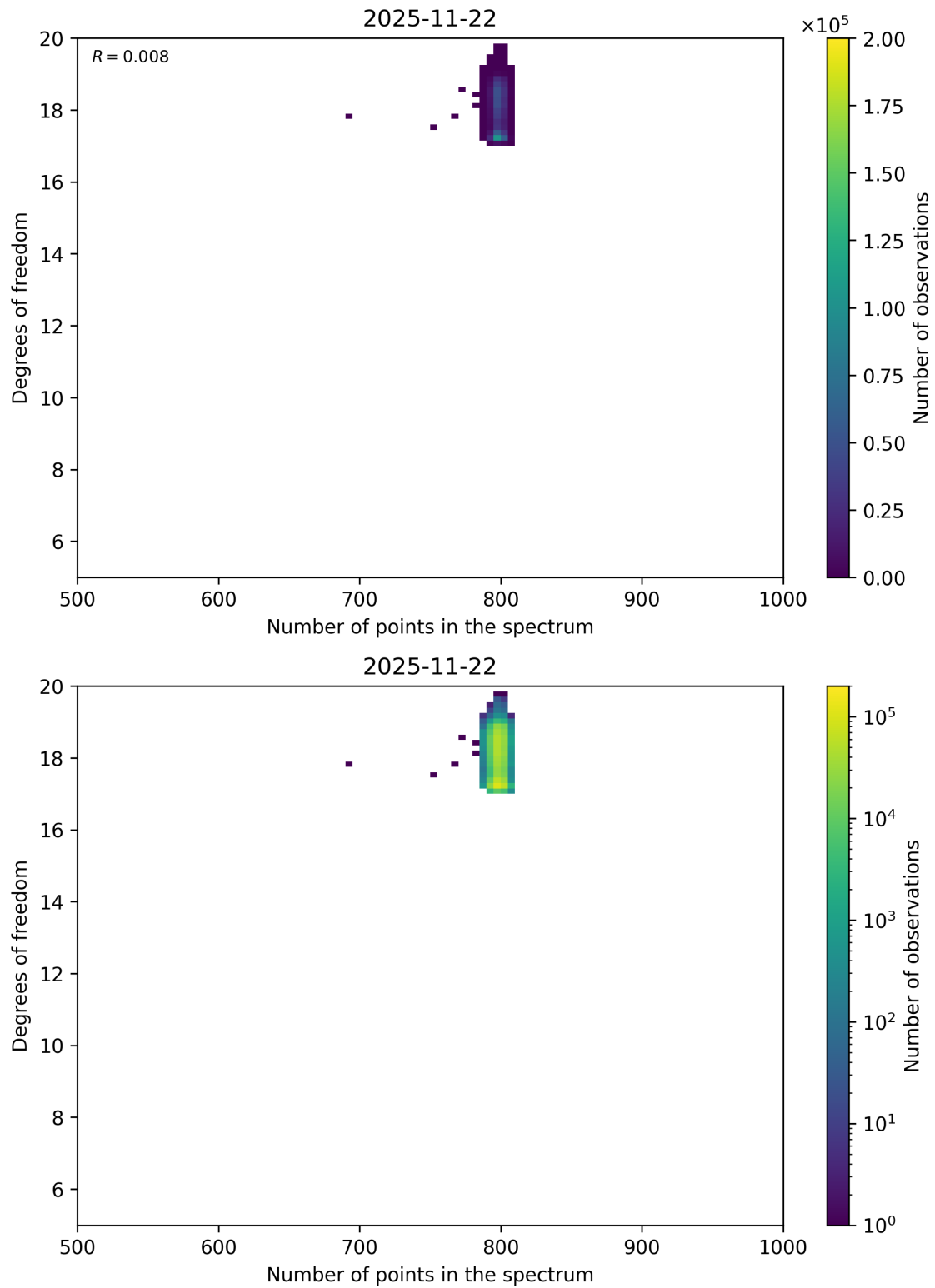
Figure 90: Scatter density plot of “Number of points in the spectrum” against “Degrees of freedom” for 2025-11-21 to 2025-11-23.
