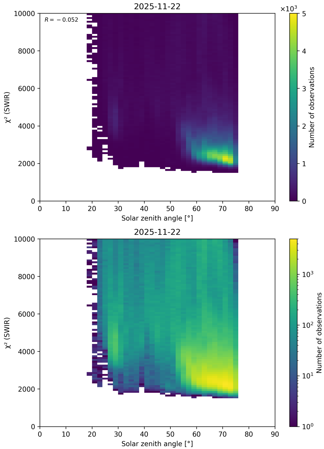
Figure 95: Scatter density plot of “Solar zenith angle” against “ \chi^2 (SWIR)” for 2025-11-21 to 2025-11-23.
