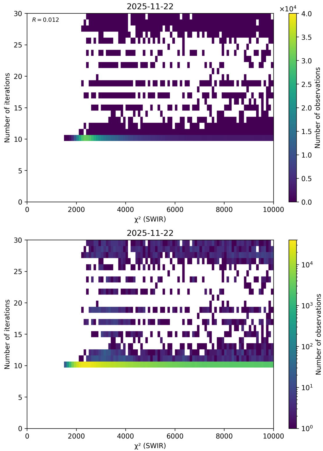
Figure 50: Scatter density plot of “ \chi^2 (SWIR)” against “Number of iterations” for 2025-11-21 to 2025-11-23.
