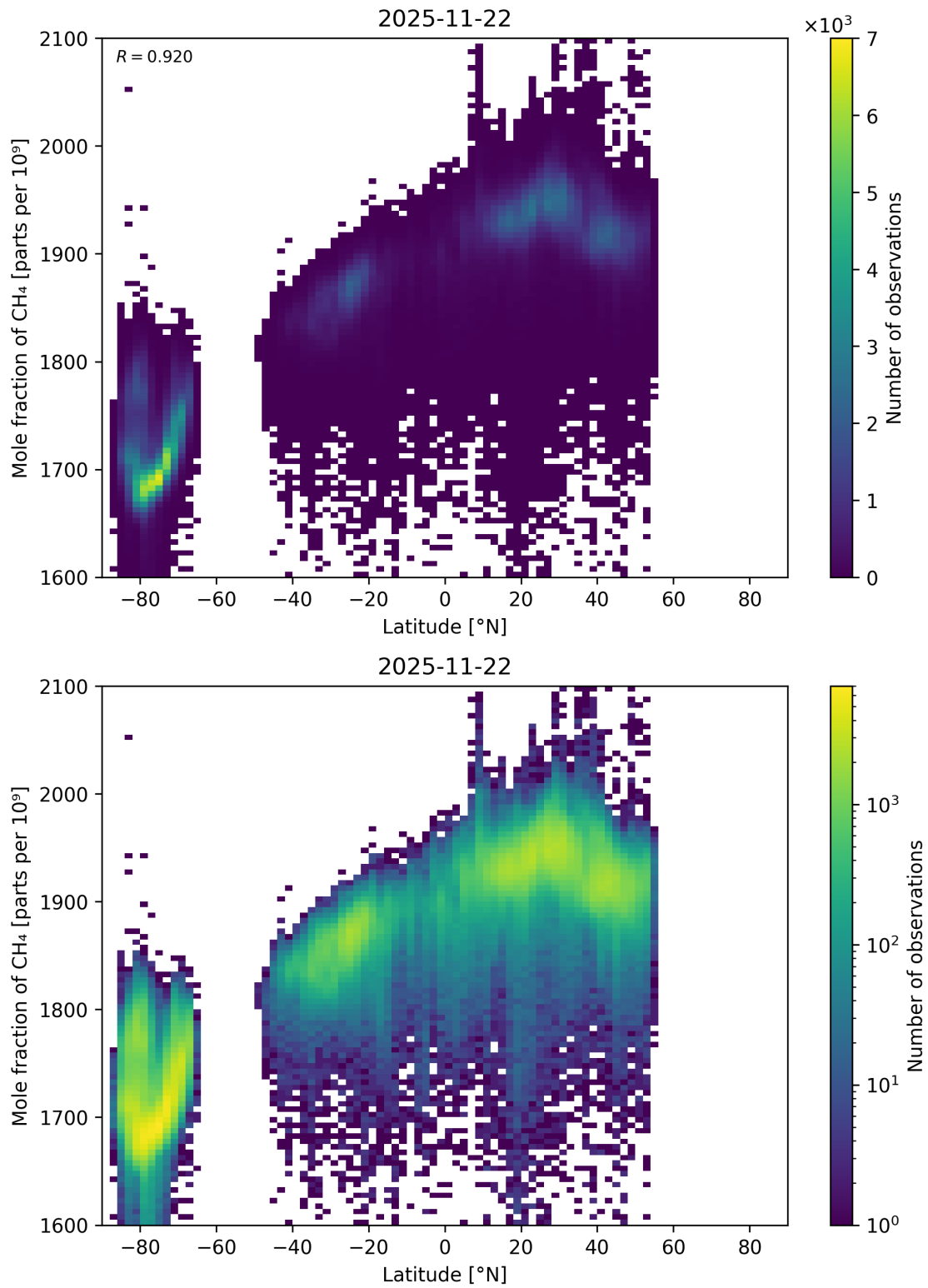
Figure 57: Scatter density plot of “Latitude” against “Mole fraction of \text{CH}_4 ” for 2025-11-21 to 2025-11-23.
