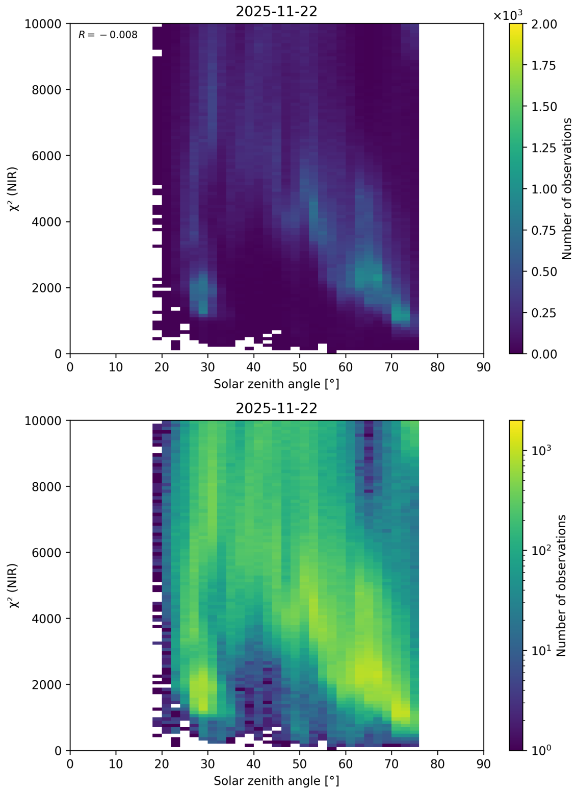
Figure 94: Scatter density plot of “Solar zenith angle” against “ \chi^2 (NIR)” for 2025-11-21 to 2025-11-23.
