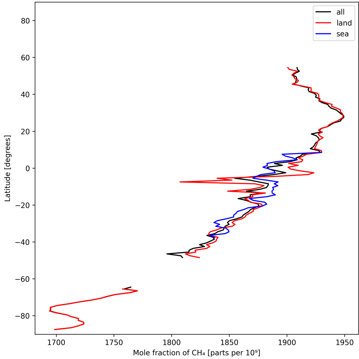
Figure 12: Zonal average of “Mole fraction of CH 4 ” for 2025-11-21 to 2025-11-23.
