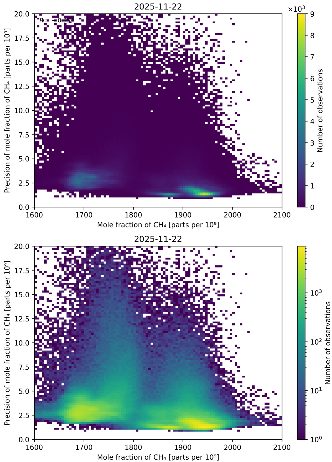
Figure 75: Scatter density plot of “Mole fraction of CH 4 ” against “Precision of mole fraction of CH 4 ” for 2025-11-21 to 2025-11-23.
