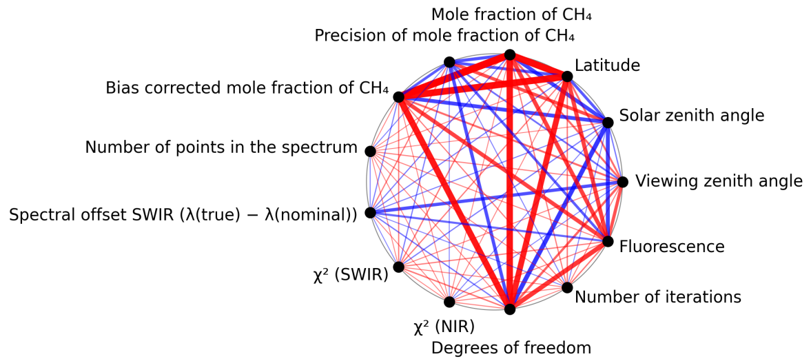
Figure 1: Map of correlation graph for 2025-11-21 to 2025-11-23.
