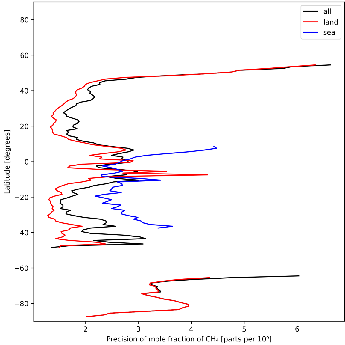
Figure 13: Zonal average of “Precision of mole fraction of CH 4 ” for 2025-11-21 to 2025-11-23.
