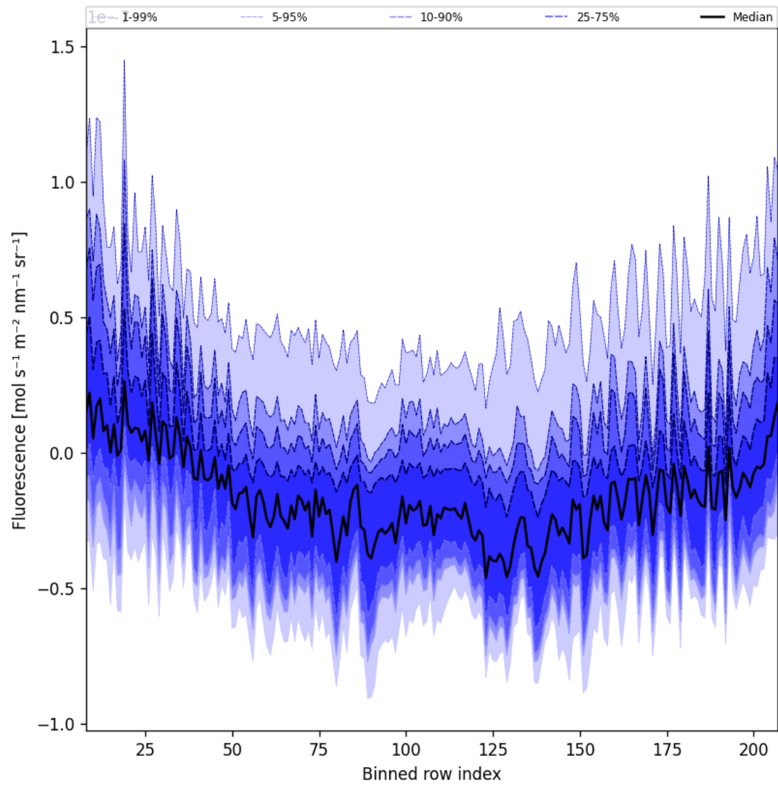
Figure 43: Along track statistics of “Fluorescence” for 2025-11-21 to 2025-11-23
