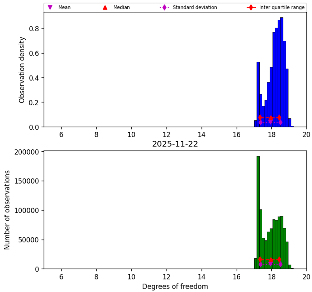
Figure 30: Histogram of “Degrees of freedom” for 2025-11-21 to 2025-11-23
