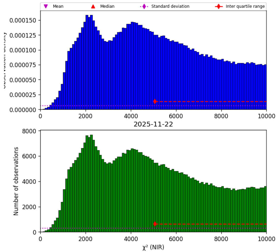
Figure 29: Histogram of “ \chi^2 (NIR)” for 2025-11-21 to 2025-11-23
