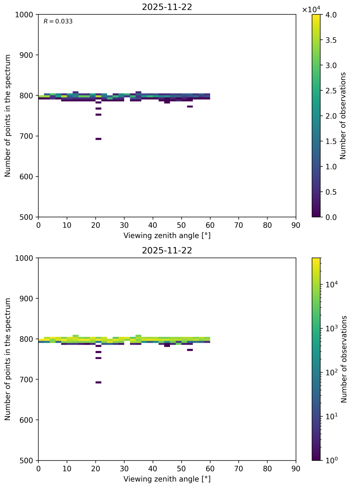
Figure 114: Scatter density plot of “Viewing zenith angle” against “Number of points in the spectrum” for 2025-11-21 to 2025-11-23.
