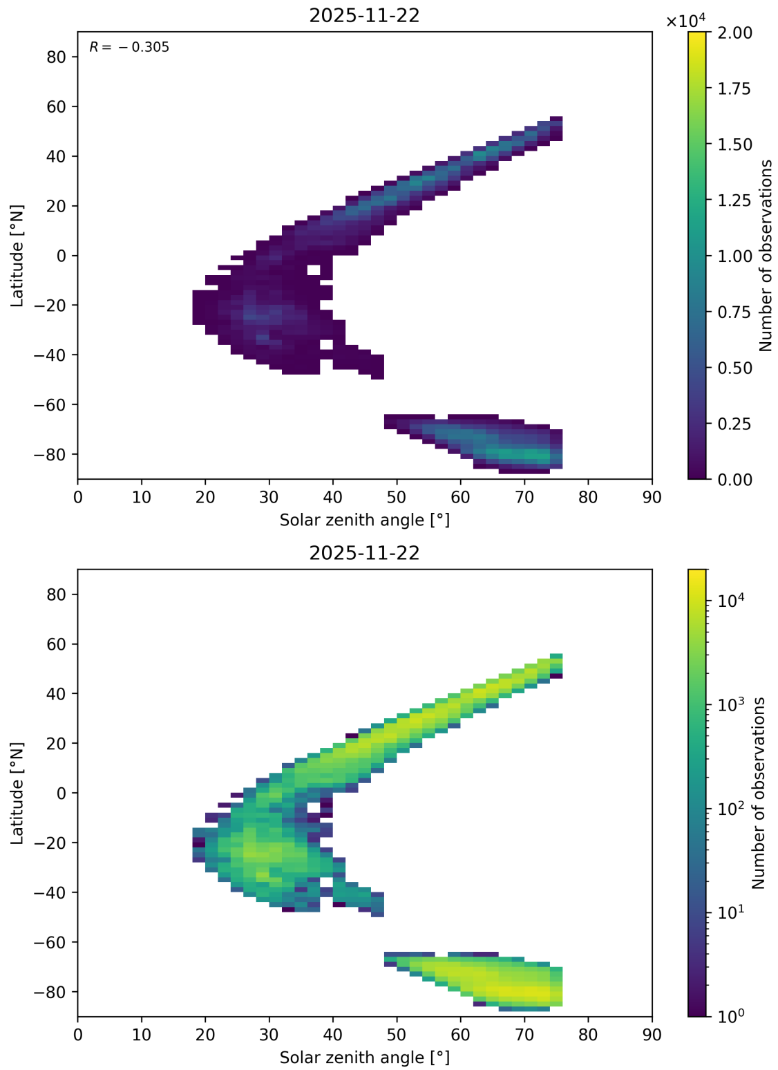
Figure 98: Scatter density plot of “Solar zenith angle” against “Latitude” for 2025-11-21 to 2025-11-23.
