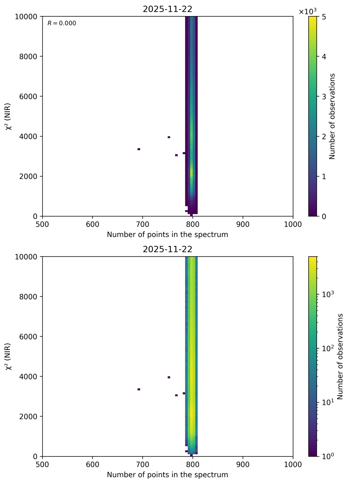
Figure 88: Scatter density plot of “Number of points in the spectrum” against “ \chi^2 (NIR)” for 2025-11-21 to 2025-11-23.
