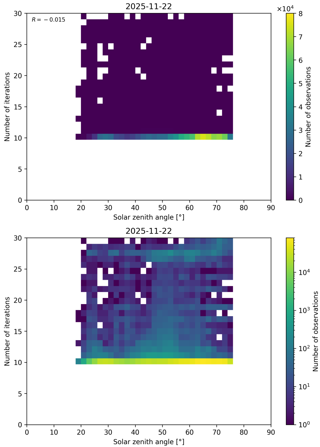
Figure 102: Scatter density plot of “Solar zenith angle” against “Number of iterations” for 2025-11-21 to 2025-11-23.
