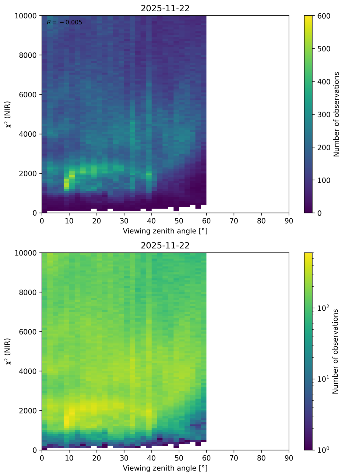
Figure 105: Scatter density plot of “Viewing zenith angle” against “ \chi^2 (NIR)” for 2025-11-21 to 2025-11-23.
