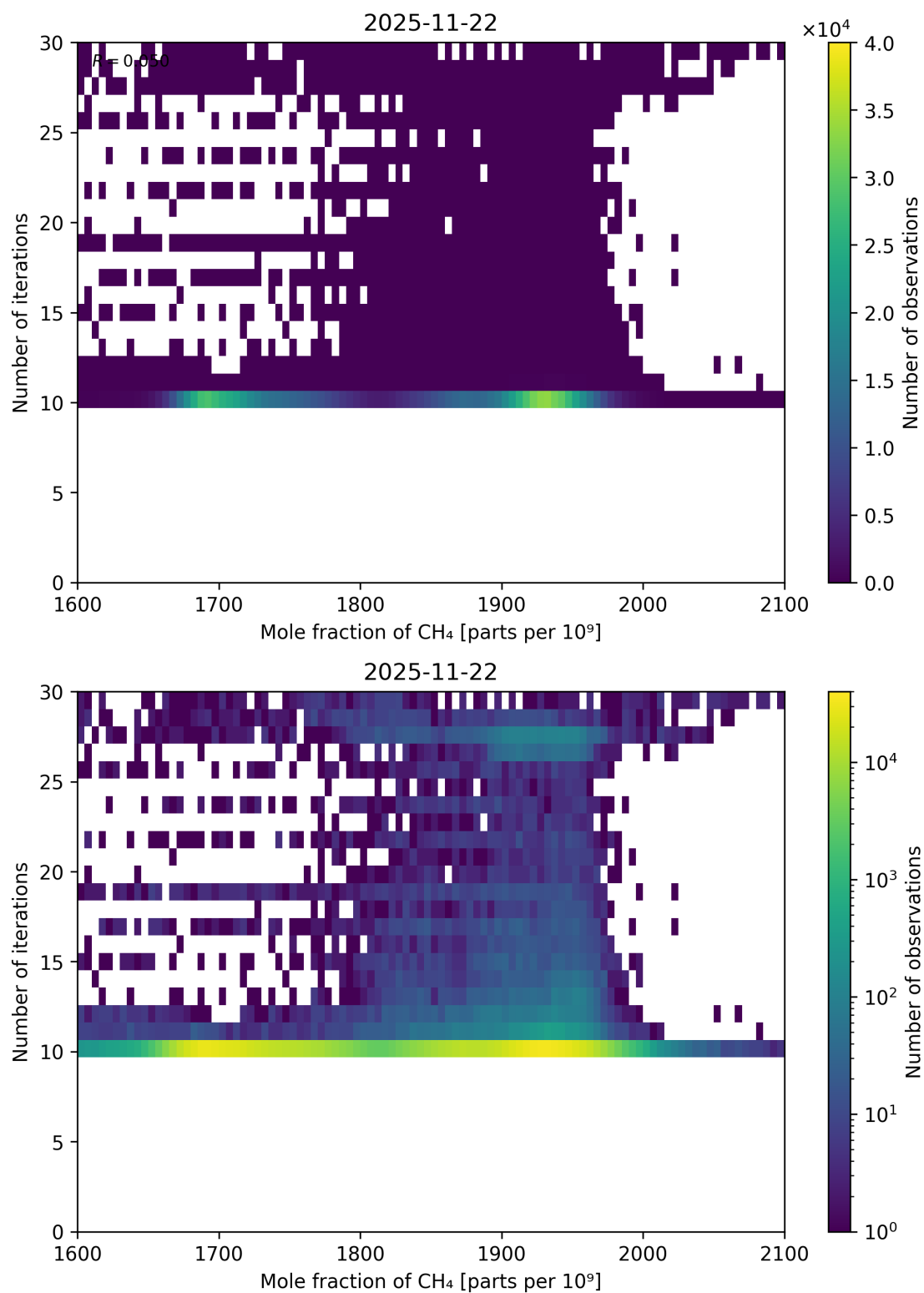
Figure 76: Scatter density plot of “Mole fraction of CH 4 ” against “Number of iterations” for 2025-11-21 to 2025-11-23.
