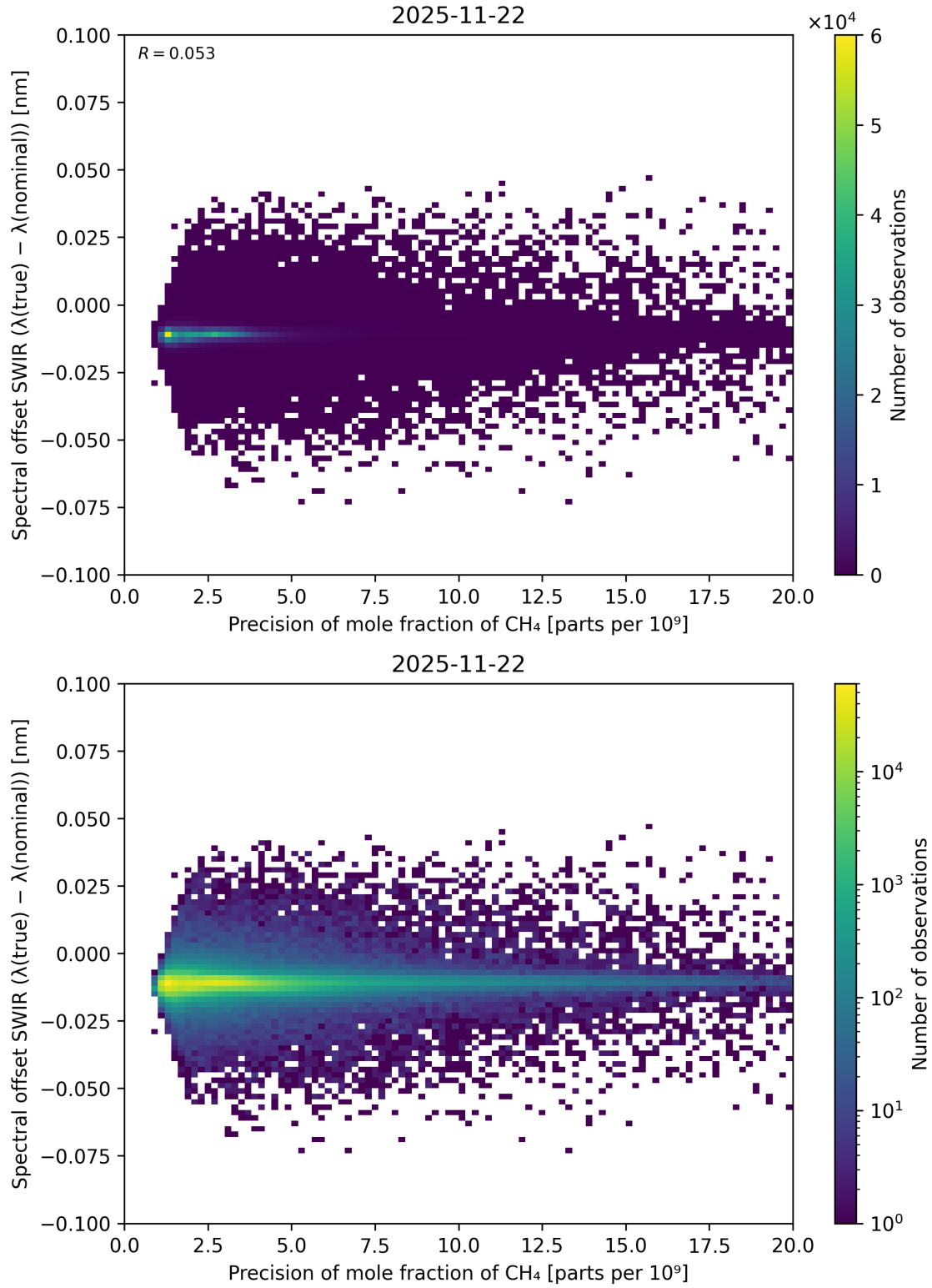
Figure 85: Scatter density plot of “Precision of mole fraction of CH 4 ” against “Spectral offset SWIR ( \lambda_{\text{true}} - \lambda_{\text{nominal}} )” for 2025-11-21 to 2025-11-23.
