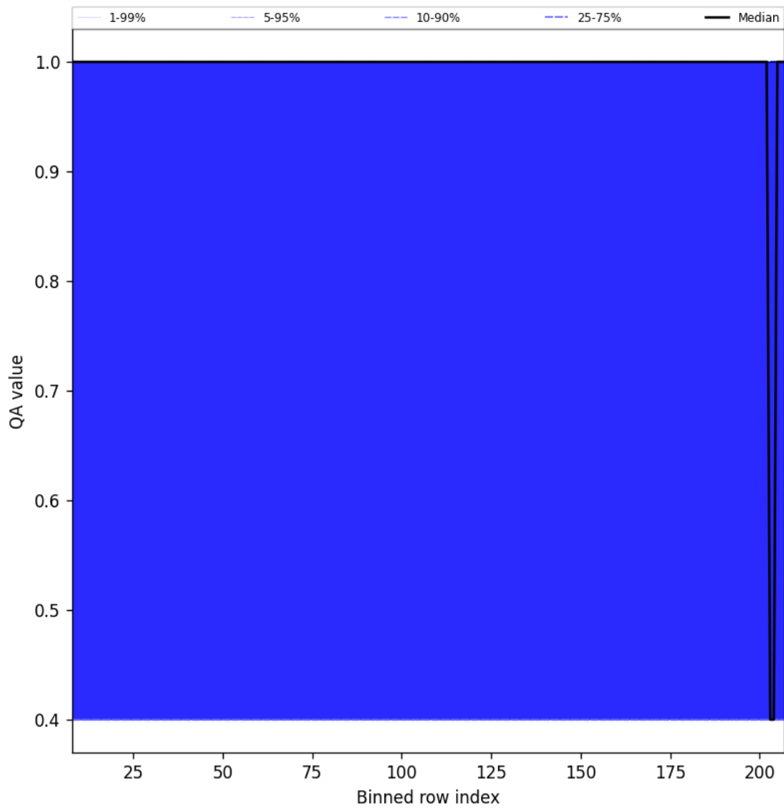
Figure 33: Along track statistics of “QA value” for 2025-11-21 to 2025-11-23
