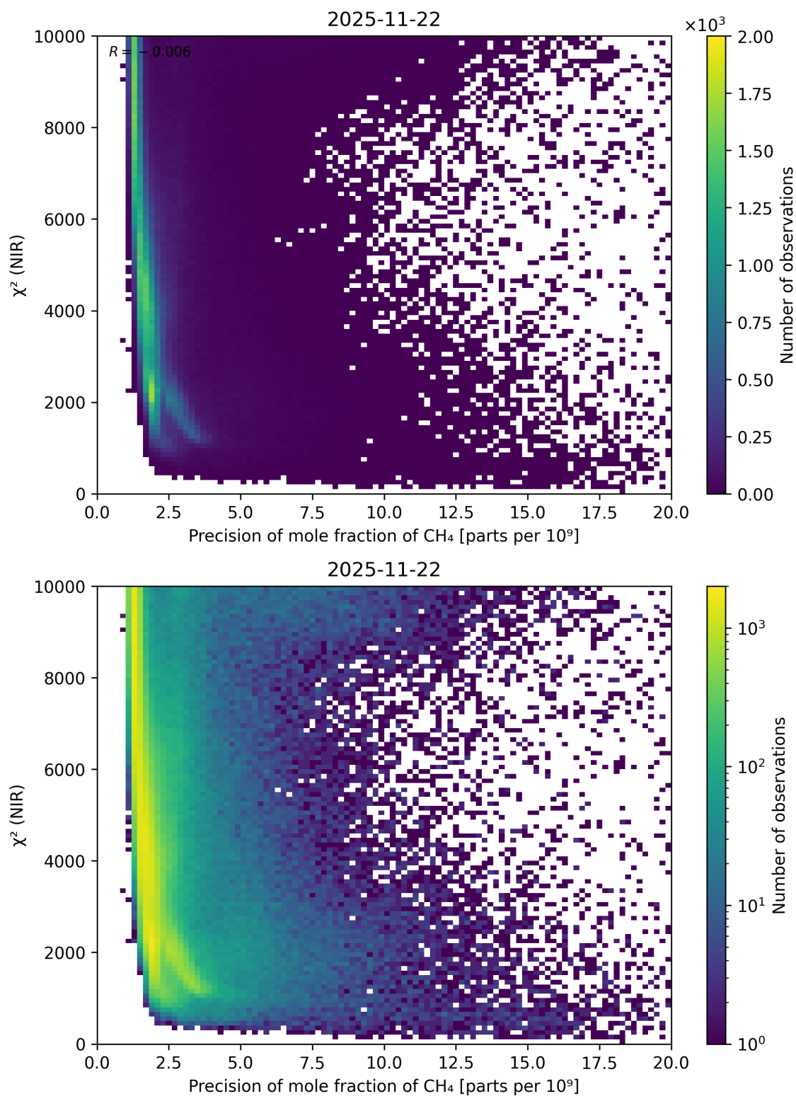
Figure 78: Scatter density plot of “Precision of mole fraction of CH 4 ” against “ \chi^2 (NIR)” for 2025-11-21 to 2025-11-23.
