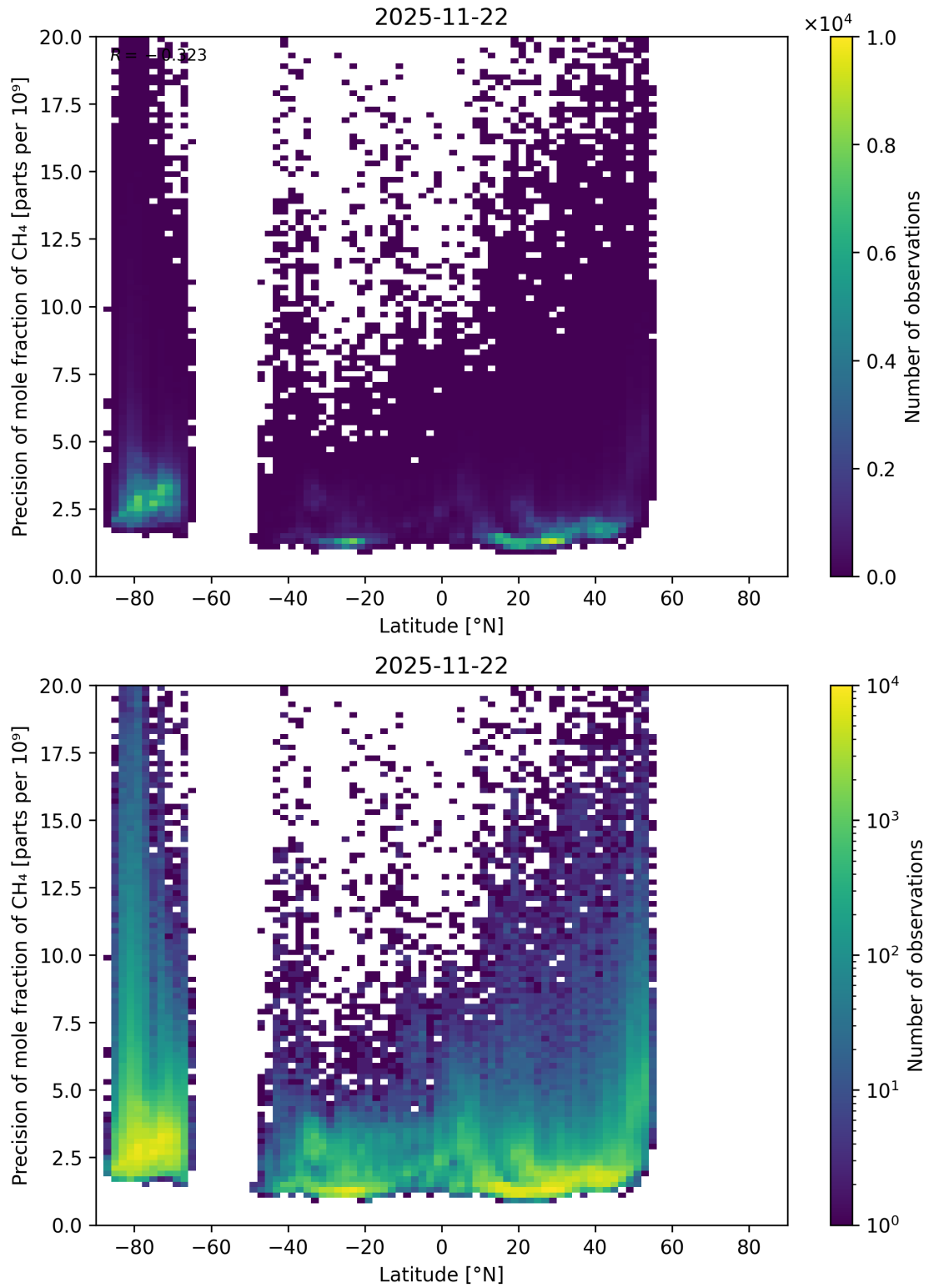
Figure 59: Scatter density plot of “Latitude” against “Precision of mole fraction of CH 4 ” for 2025-11-21 to 2025-11-23.
