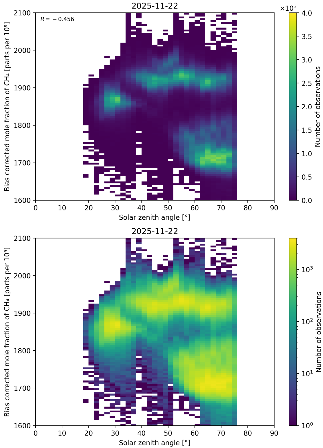
Figure 100: Scatter density plot of “Solar zenith angle” against “Bias corrected mole fraction of CH 4 ” for 2025-11-21 to 2025-11-23.
