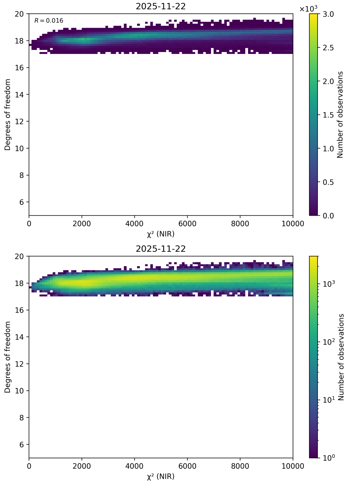
Figure 44: Scatter density plot of “ \chi^2 (NIR)” against “Degrees of freedom” for 2025-11-21 to 2025-11-23.
