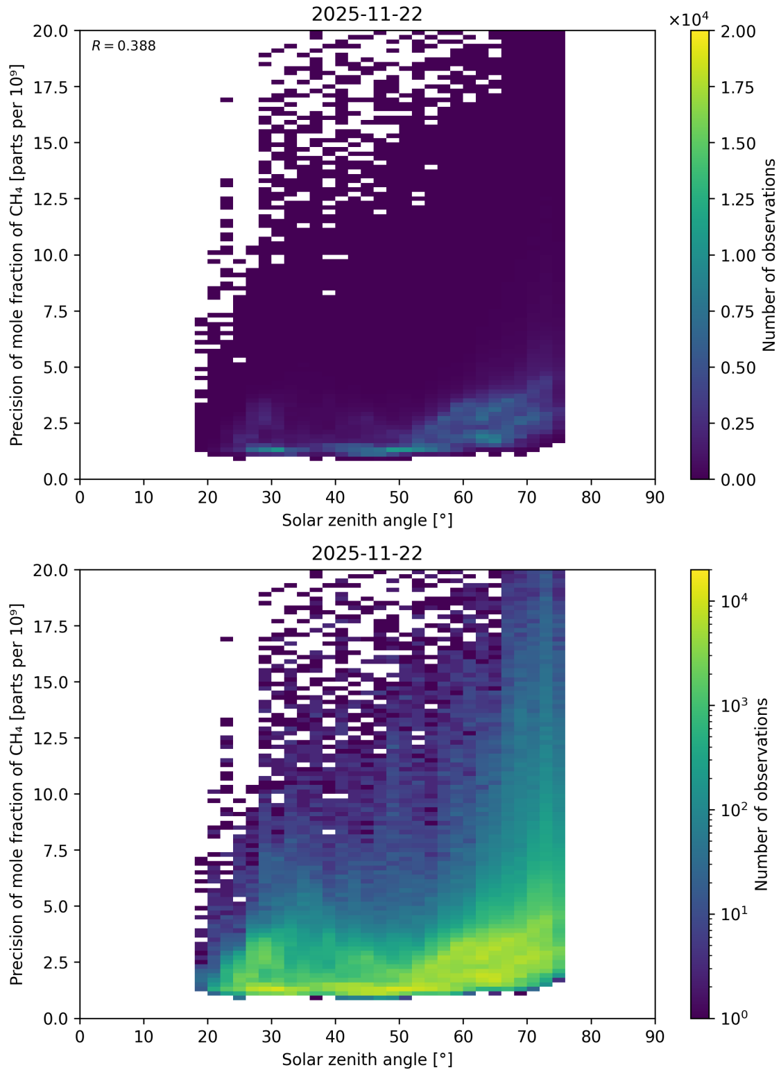
Figure 101: Scatter density plot of “Solar zenith angle” against “Precision of mole fraction of \text{CH}_4 ” for 2025-11-21 to 2025-11-23.
