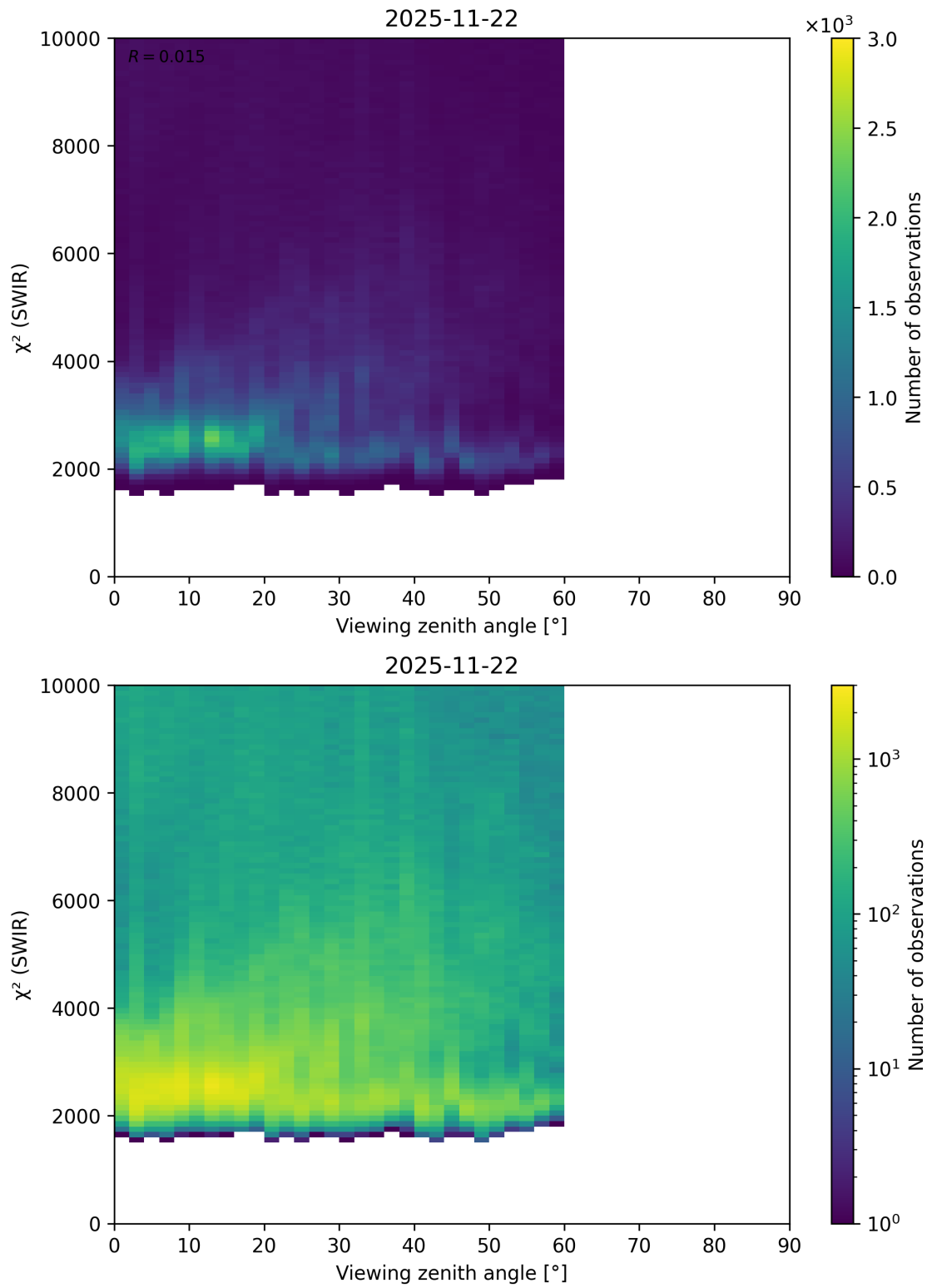
Figure 106: Scatter density plot of “Viewing zenith angle” against “ \chi^2 (SWIR)” for 2025-11-21 to 2025-11-23.
