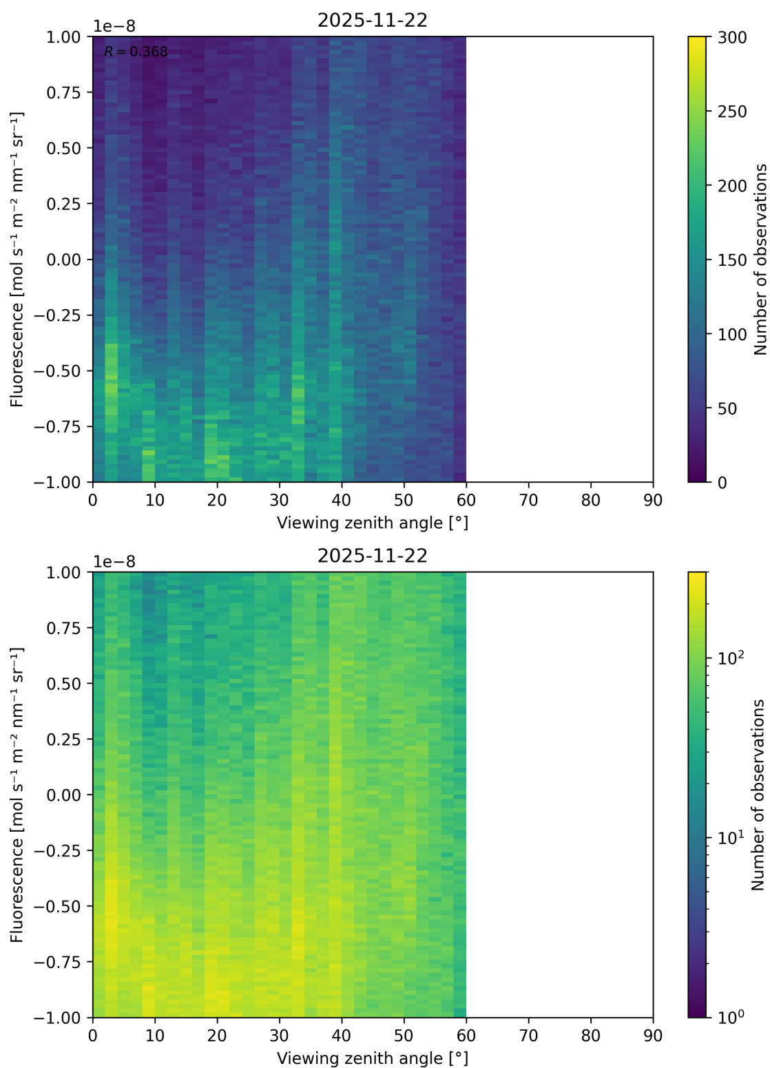
Figure 108: Scatter density plot of “Viewing zenith angle” against “Fluorescence” for 2025-11-21 to 2025-11-23.
