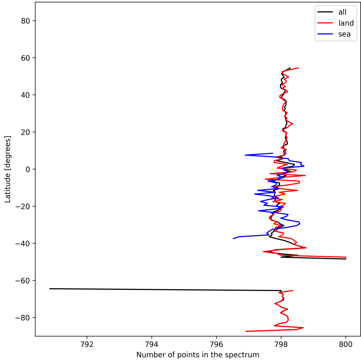
Figure 15: Zonal average of “Number of points in the spectrum” for 2025-11-21 to 2025-11-23.
