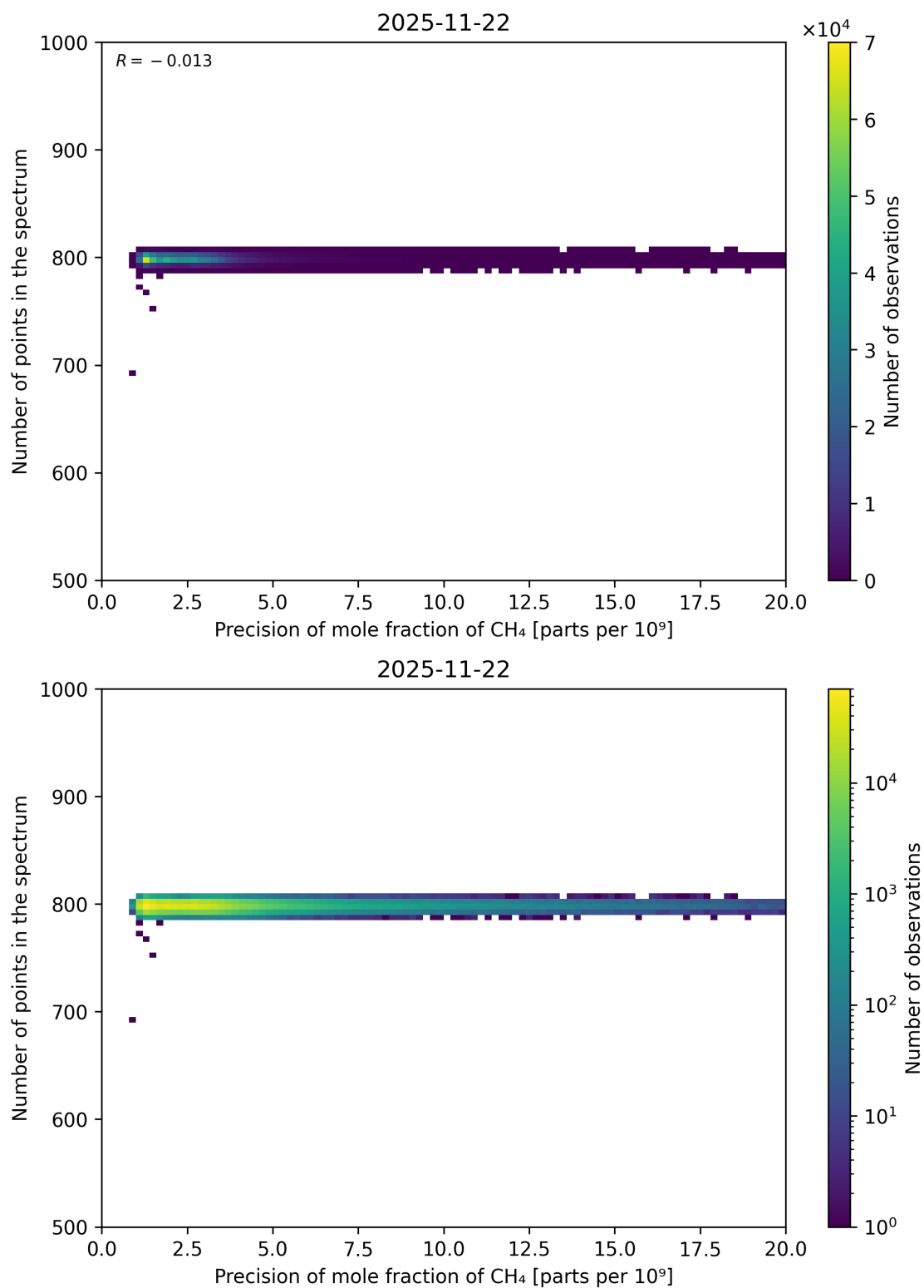
Figure 84: Scatter density plot of “Precision of mole fraction of CH 4 ” against “Number of points in the spectrum” for 2025-11-21 to 2025-11-23.
