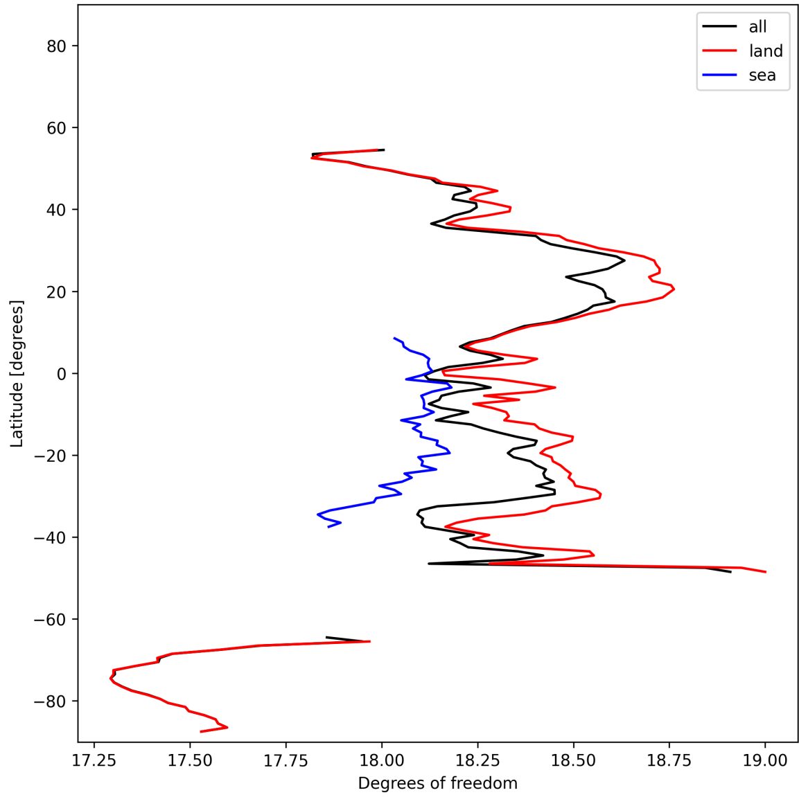
Figure 19: Zonal average of “Degrees of freedom” for 2025-11-21 to 2025-11-23.
