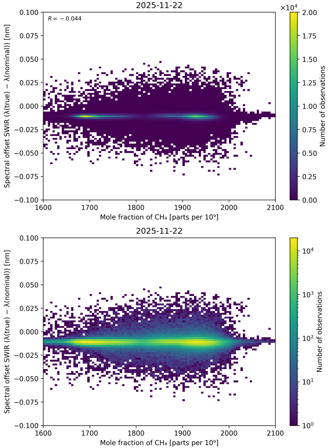
Figure 86: Scatter density plot of “Mole fraction of CH 4 ” against “Spectral offset SWIR ( \lambda_{\text{true}} - \lambda_{\text{nominal}} )” for 2025-11-21 to 2025-11-23.
