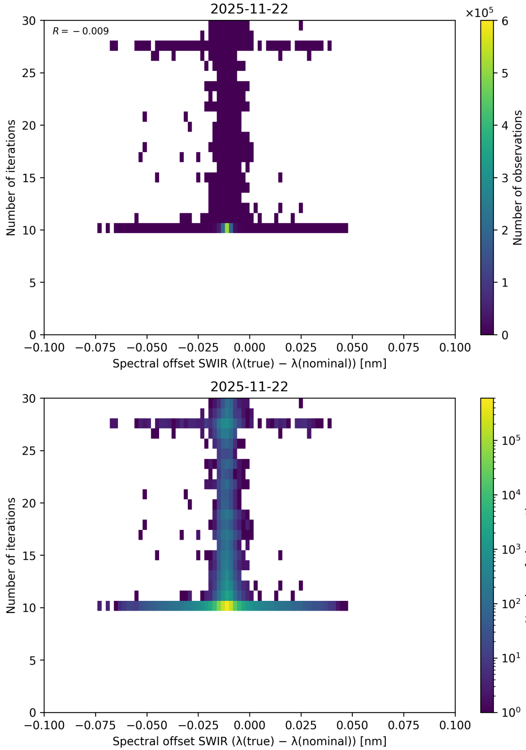
Figure 121: Scatter density plot of “Spectral offset SWIR ( \lambda_{\text{true}} - \lambda_{\text{nominal}} )” against “Number of iterations” for 2025-11-21 to 2025-11-23.
