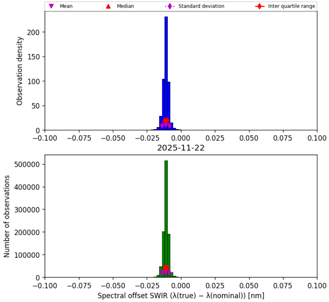
Figure 27: Histogram of “Spectral offset SWIR ( \lambda_{\text{true}} - \lambda_{\text{nominal}} )” for 2025-11-21 to 2025-11-23
