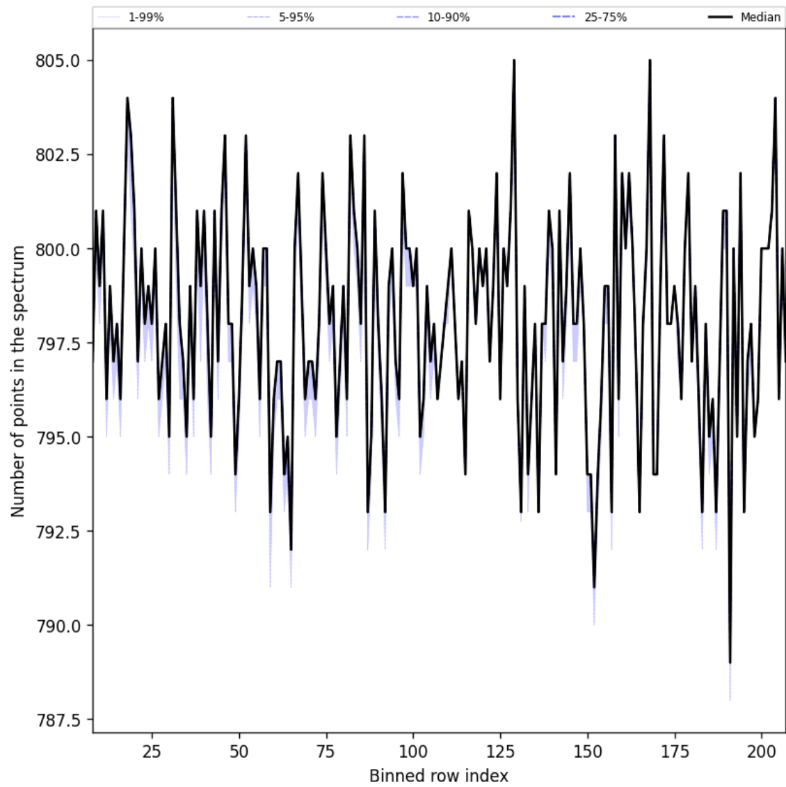
Figure 37: Along track statistics of “Number of points in the spectrum” for 2025-11-21 to 2025-11-23
