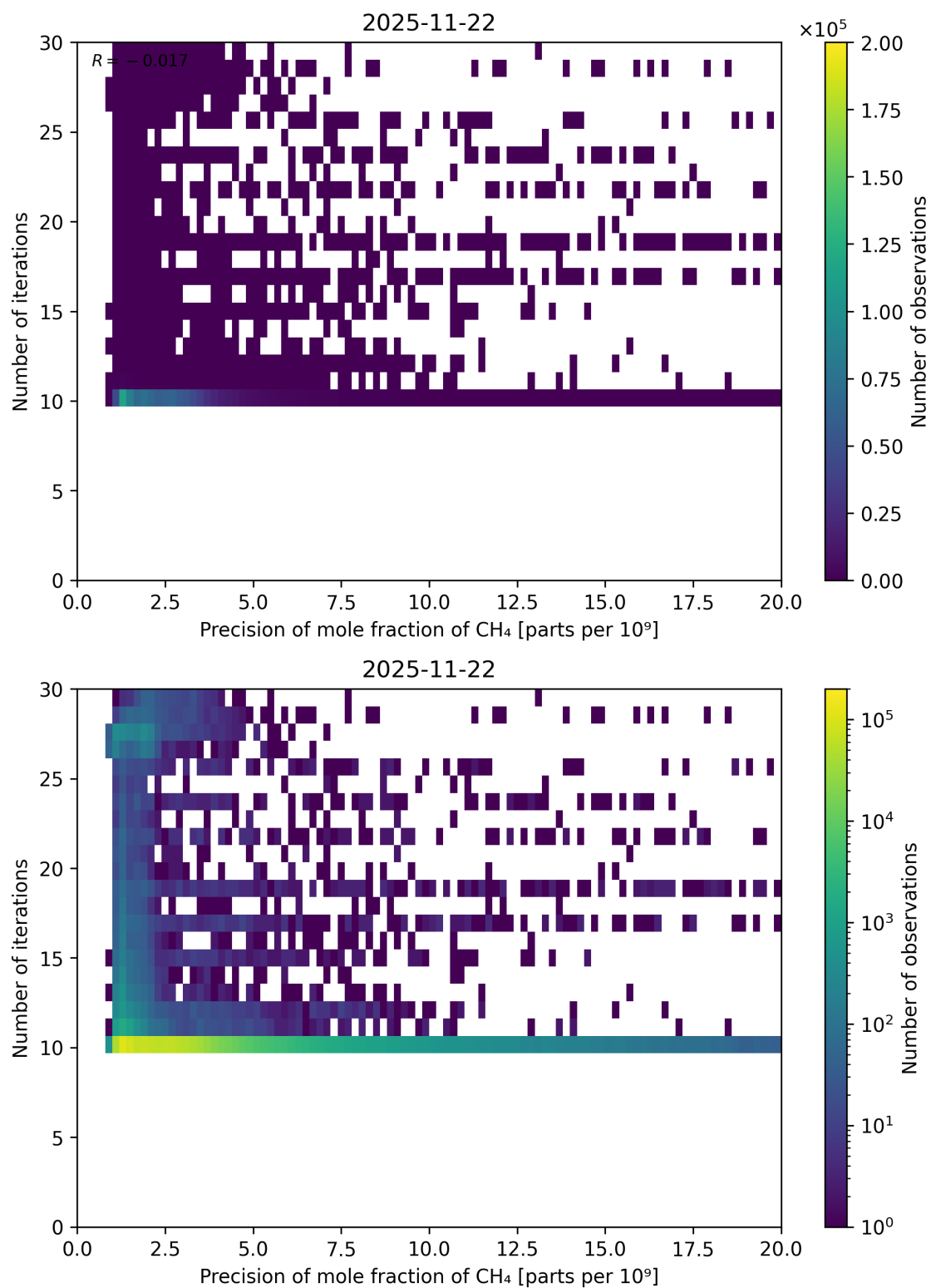
Figure 83: Scatter density plot of “Precision of mole fraction of CH 4 ” against “Number of iterations” for 2025-11-21 to 2025-11-23.
