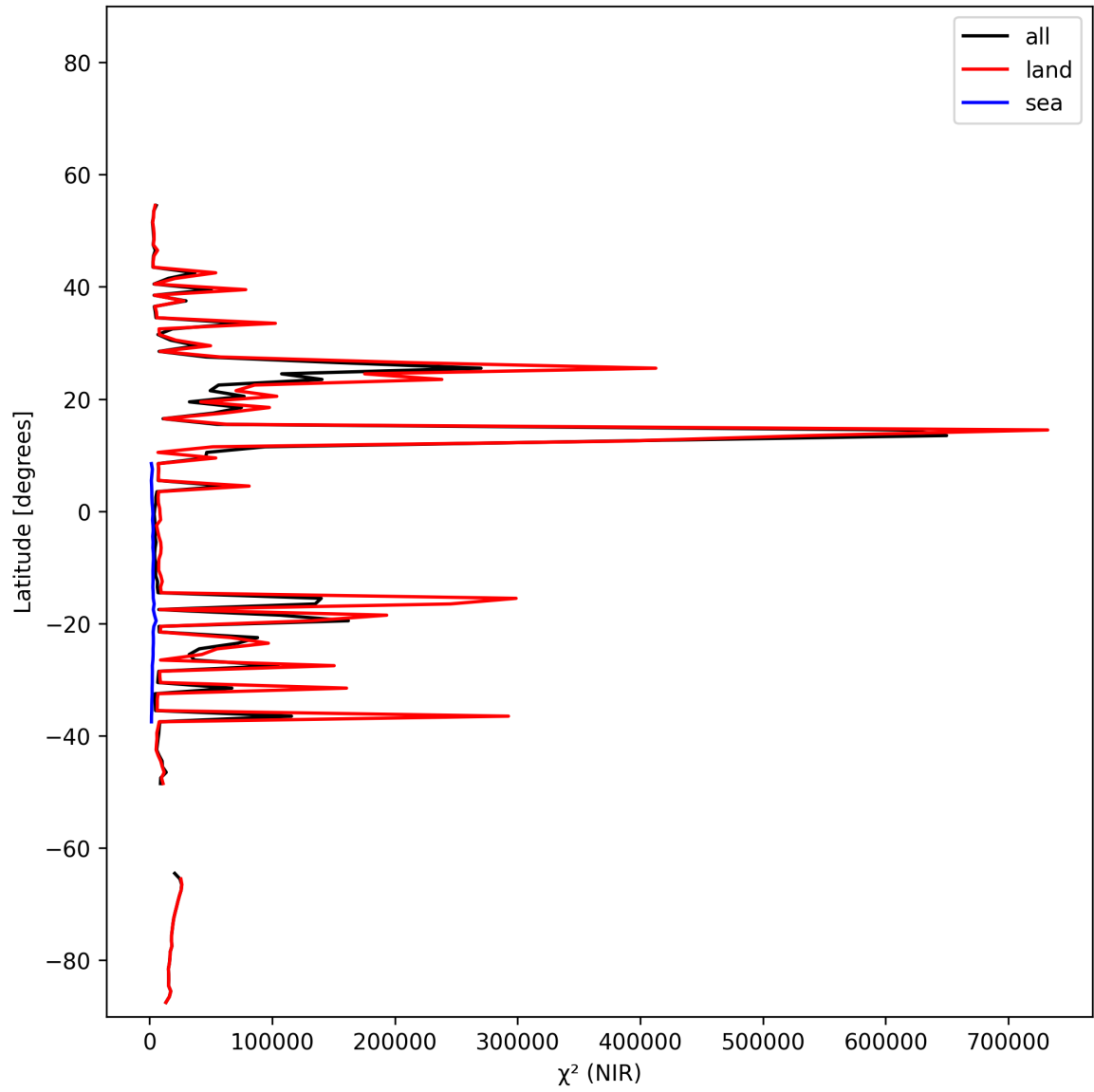
Figure 18: Zonal average of “ \chi^2 (NIR)” for 2025-11-21 to 2025-11-23.
