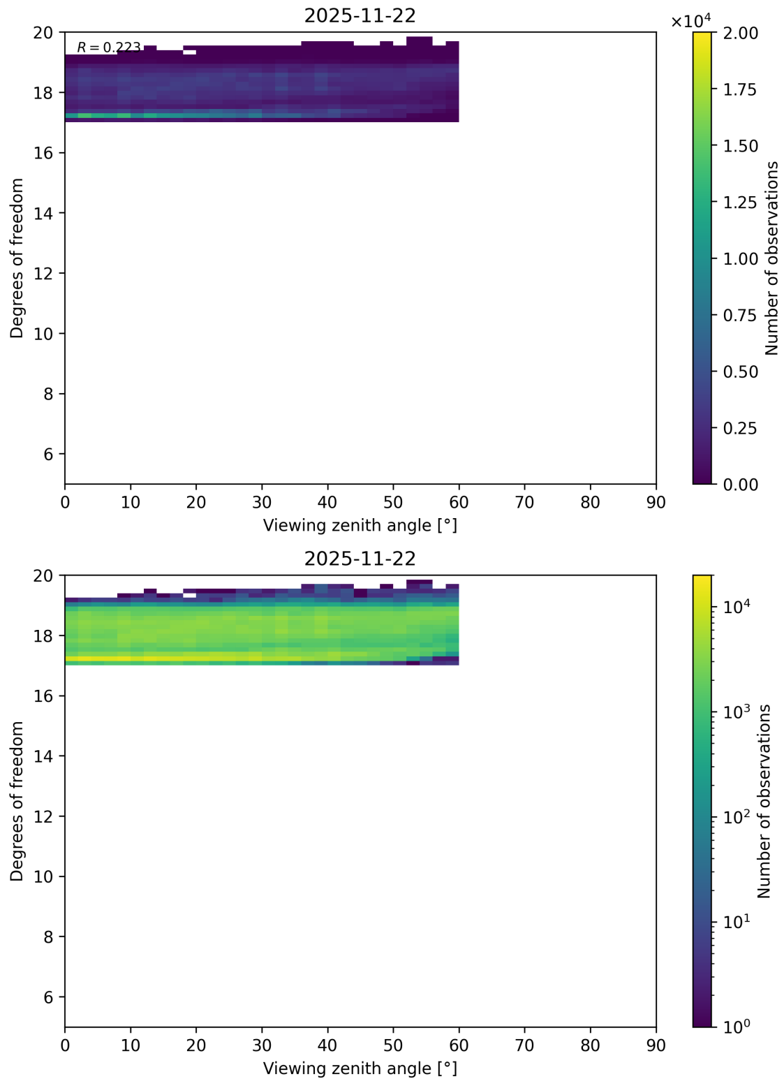
Figure 107: Scatter density plot of “Viewing zenith angle” against “Degrees of freedom” for 2025-11-21 to 2025-11-23.
