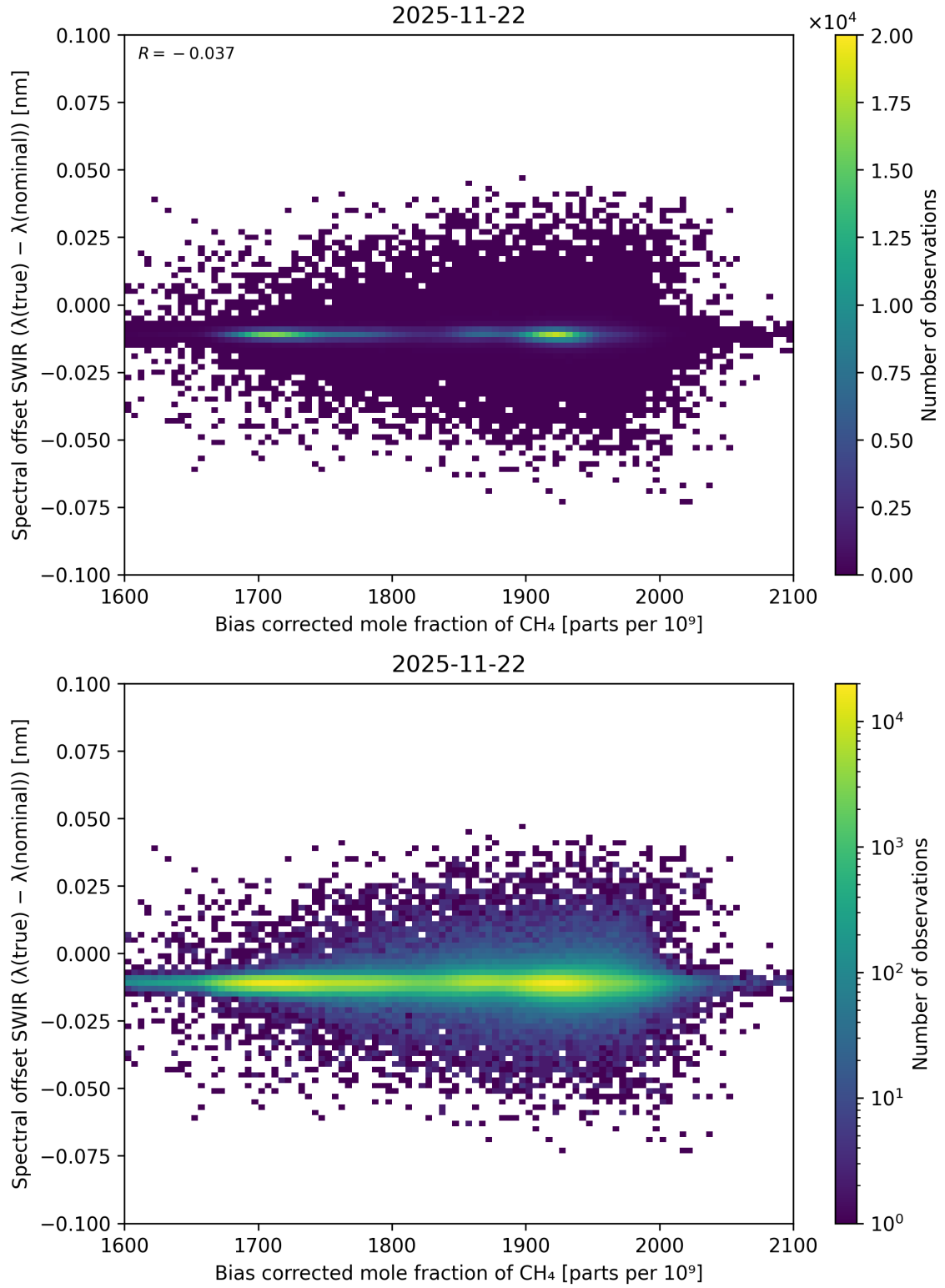
Figure 69: Scatter density plot of “Bias corrected mole fraction of \text{CH}_4 ” against “Spectral offset SWIR ( \lambda_{\text{true}} - \lambda_{\text{nominal}} )” for 2025-11-21 to 2025-11-23.
