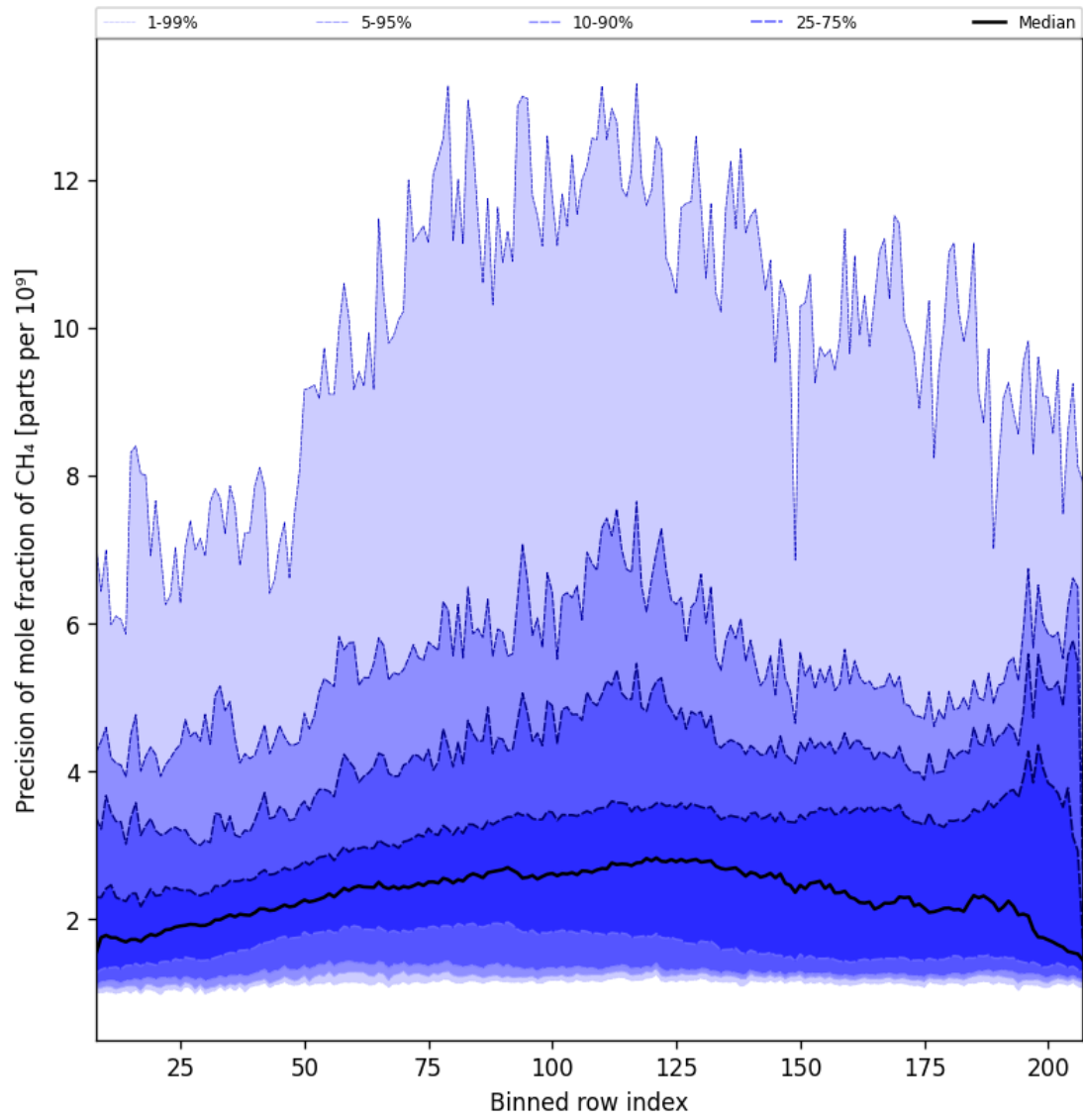
Figure 35: Along track statistics of “Precision of mole fraction of CH 4 ” for 2025-11-21 to 2025-11-23
