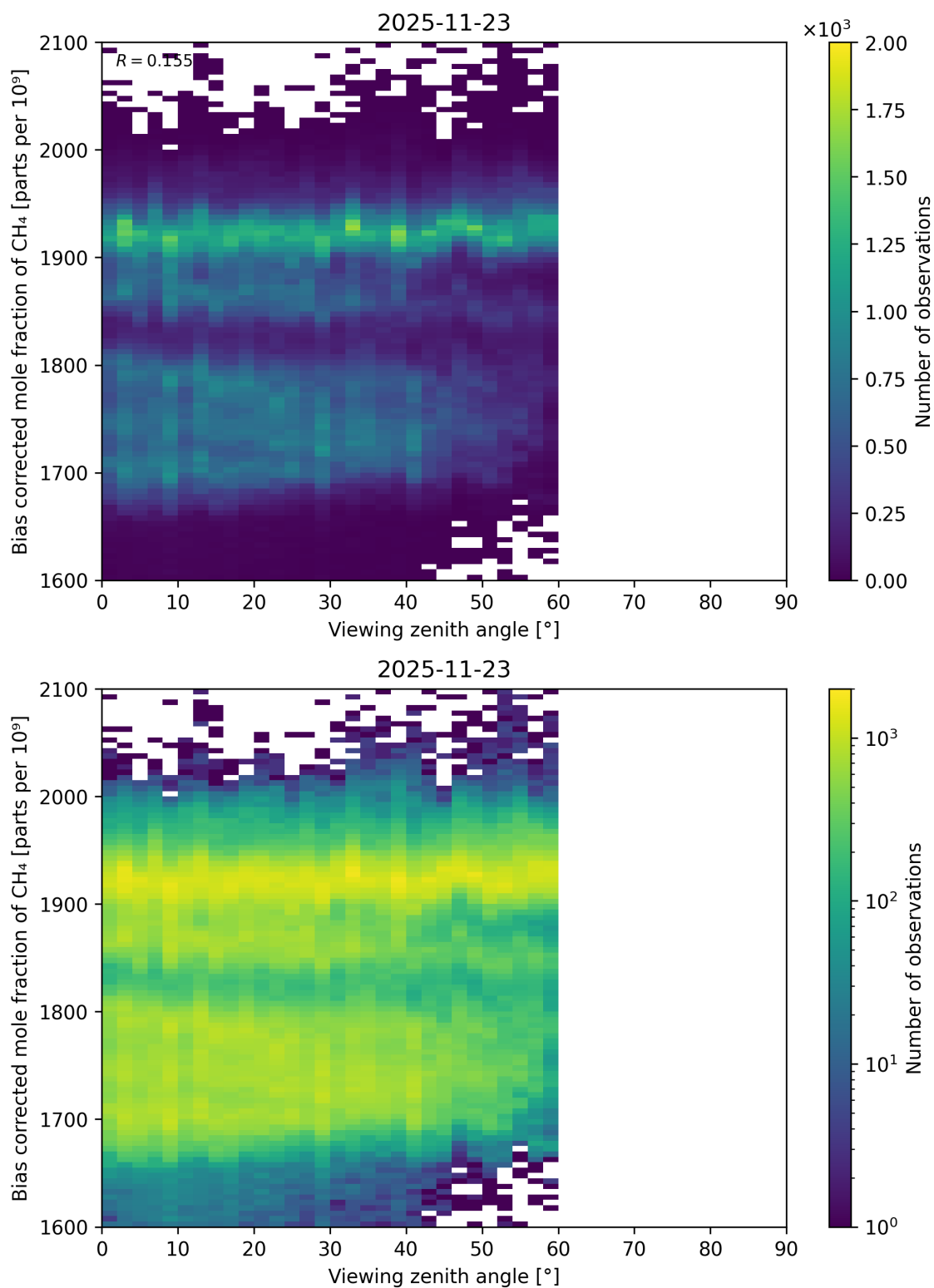
Figure 127: Scatter density plot of “Viewing zenith angle” against “Bias corrected mole fraction of \text{CH}_4 ” for 2025-11-23 to 2025-11-24.
