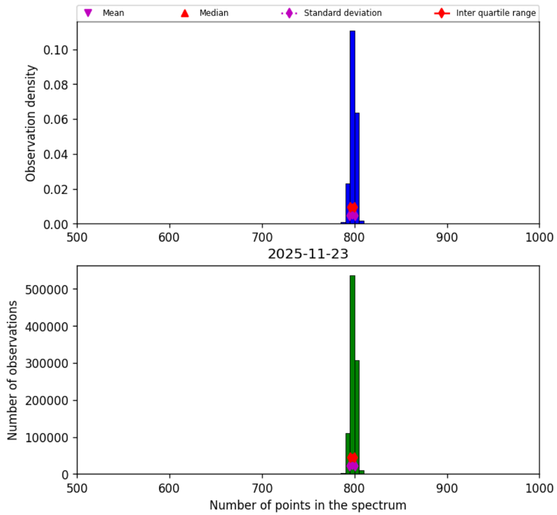
Figure 28: Histogram of “Number of points in the spectrum” for 2025-11-23 to 2025-11-24
