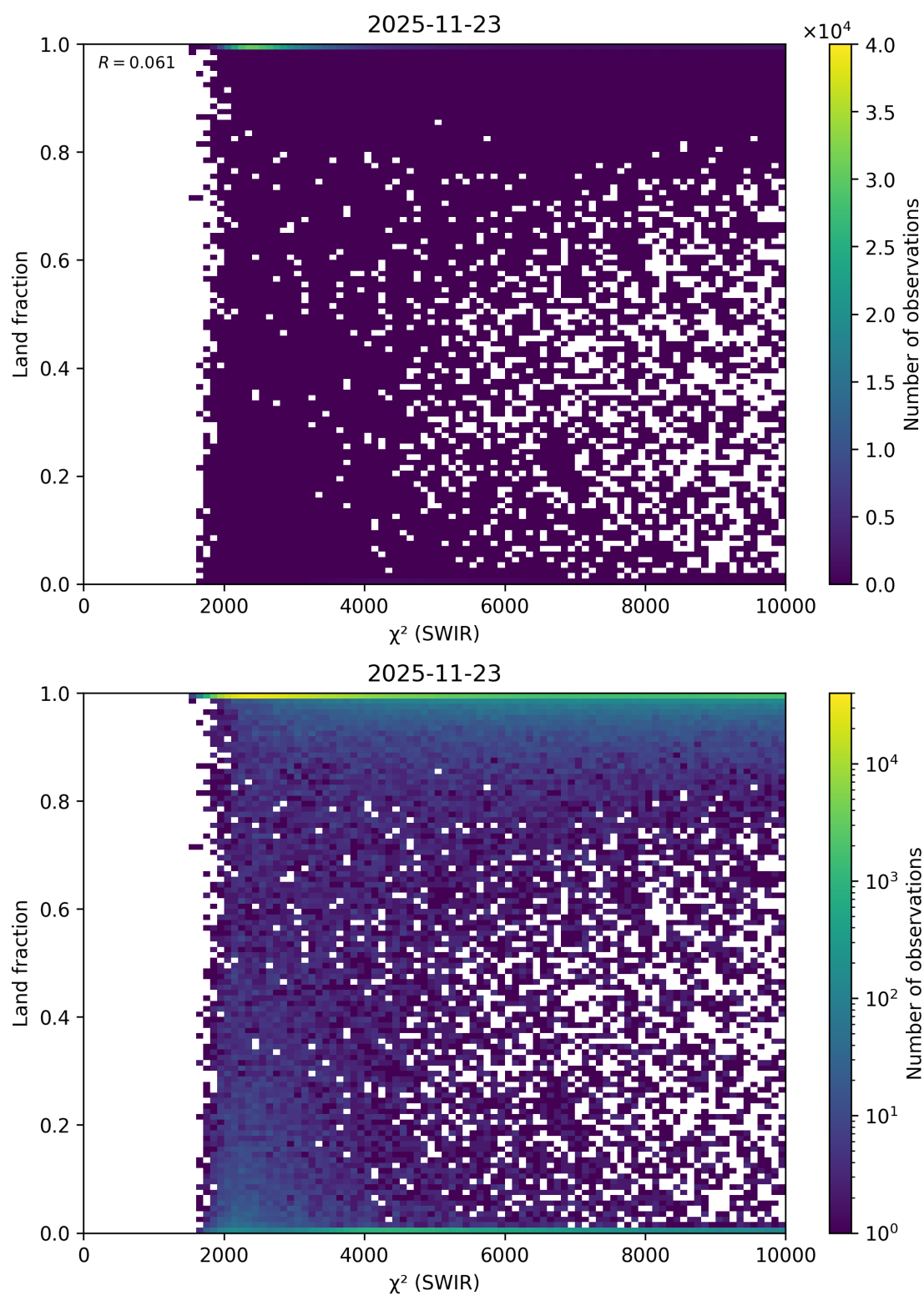
Figure 55: Scatter density plot of “ \chi^2 (SWIR)” against “Land fraction” for 2025-11-23 to 2025-11-24.
