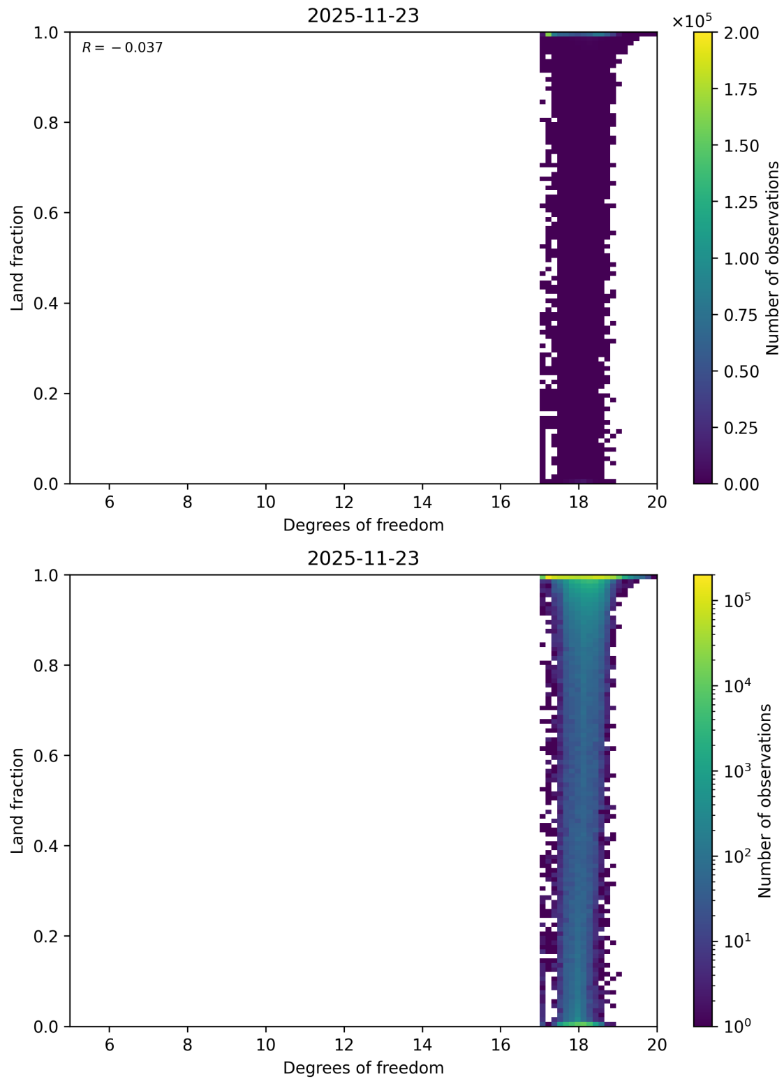
Figure 58: Scatter density plot of “Degrees of freedom” against “Land fraction” for 2025-11-23 to 2025-11-24.
