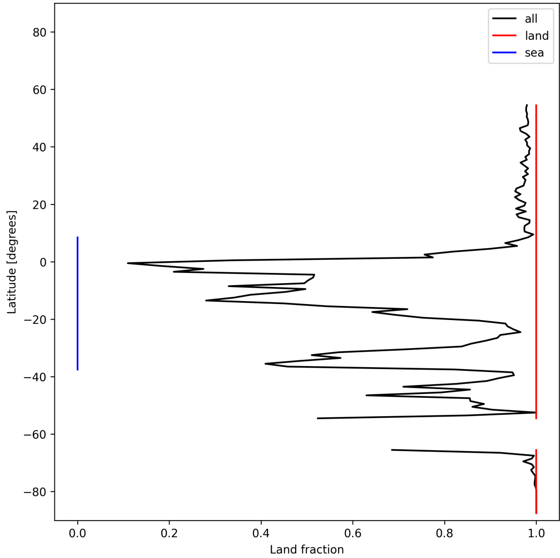
Figure 23: Zonal average of “Land fraction” for 2025-11-23 to 2025-11-24.
