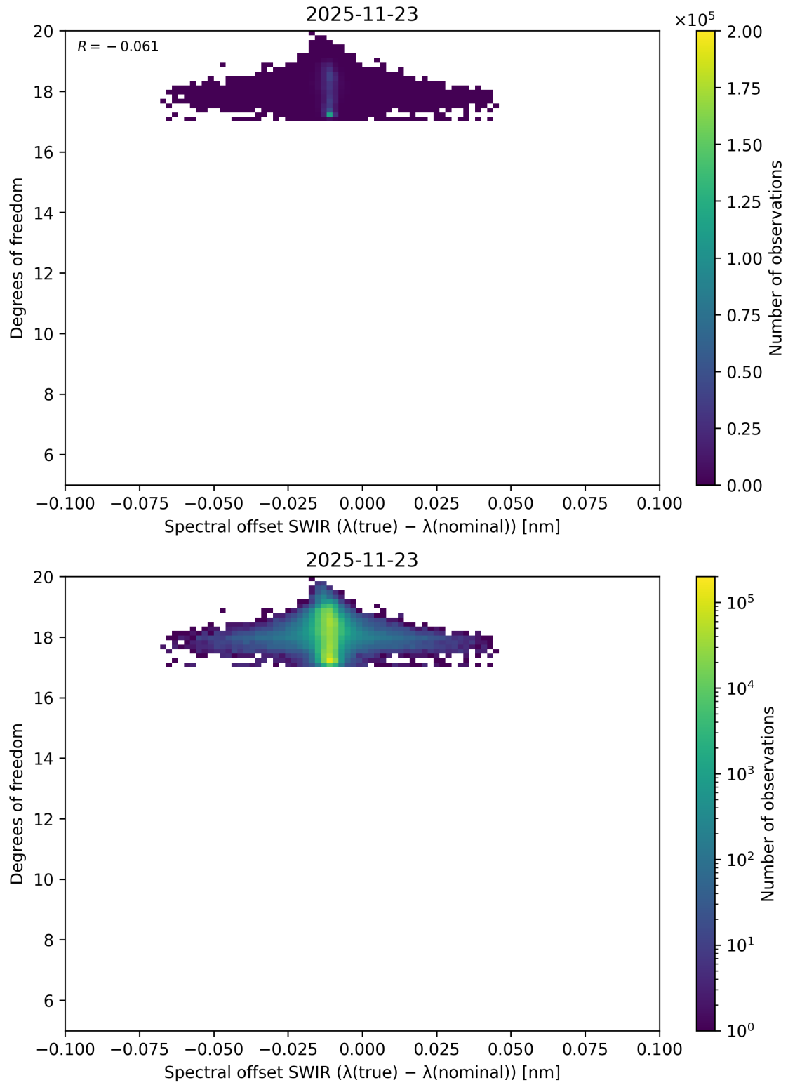
Figure 135: Scatter density plot of “Spectral offset SWIR ( \lambda_{\text{true}} - \lambda_{\text{nominal}} )” against “Degrees of freedom” for 2025-11-23 to 2025-11-24.
