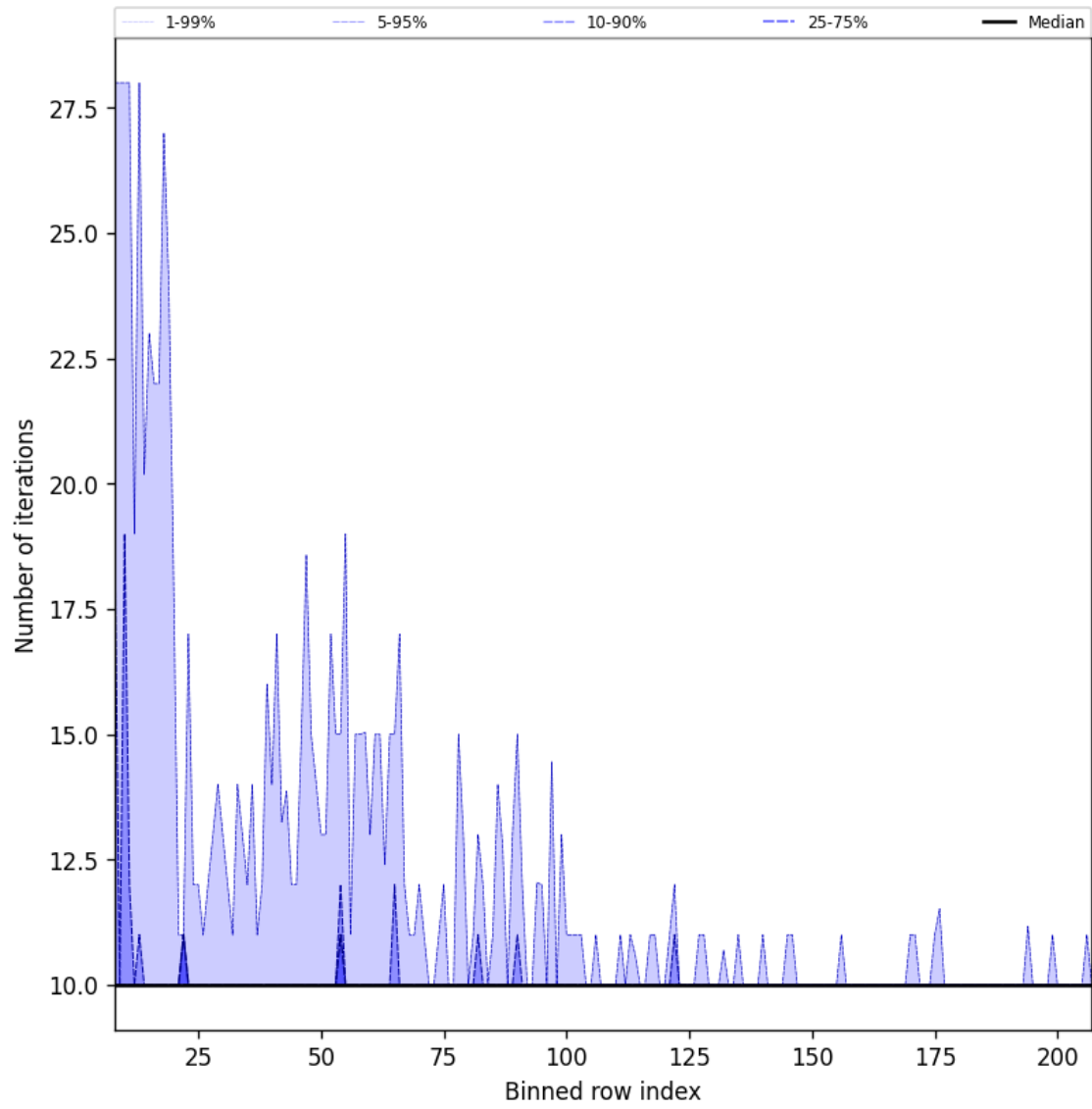
Figure 45: Along track statistics of “Number of iterations” for 2025-11-23 to 2025-11-24
