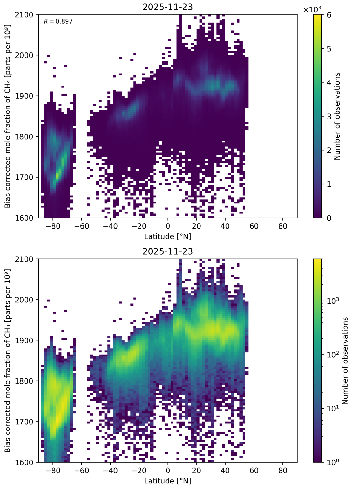
Figure 67: Scatter density plot of “Latitude” against “Bias corrected mole fraction of CH 4 ” for 2025-11-23 to 2025-11-24.
