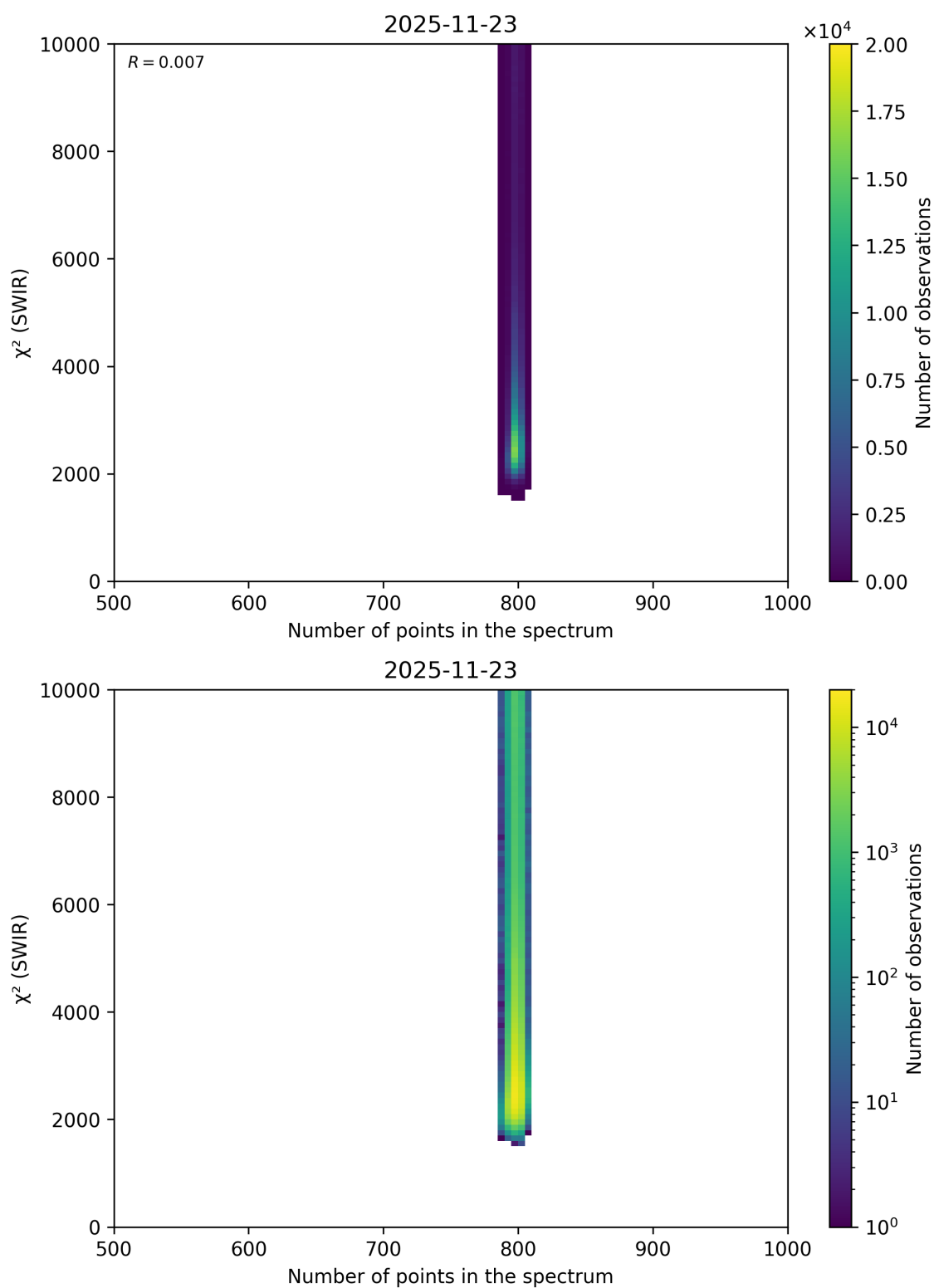
Figure 102: Scatter density plot of “Number of points in the spectrum” against “ \chi^2 (SWIR)” for 2025-11-23 to 2025-11-24.
