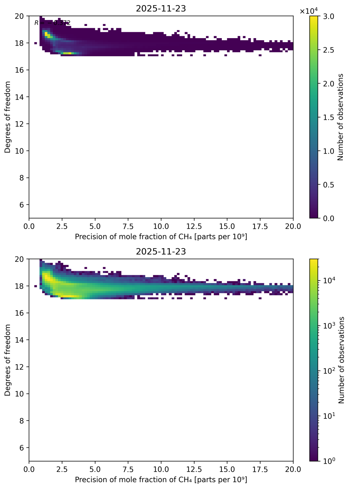
Figure 91: Scatter density plot of “Precision of mole fraction of CH 4 ” against “Degrees of freedom” for 2025-11-23 to 2025-11-24.
