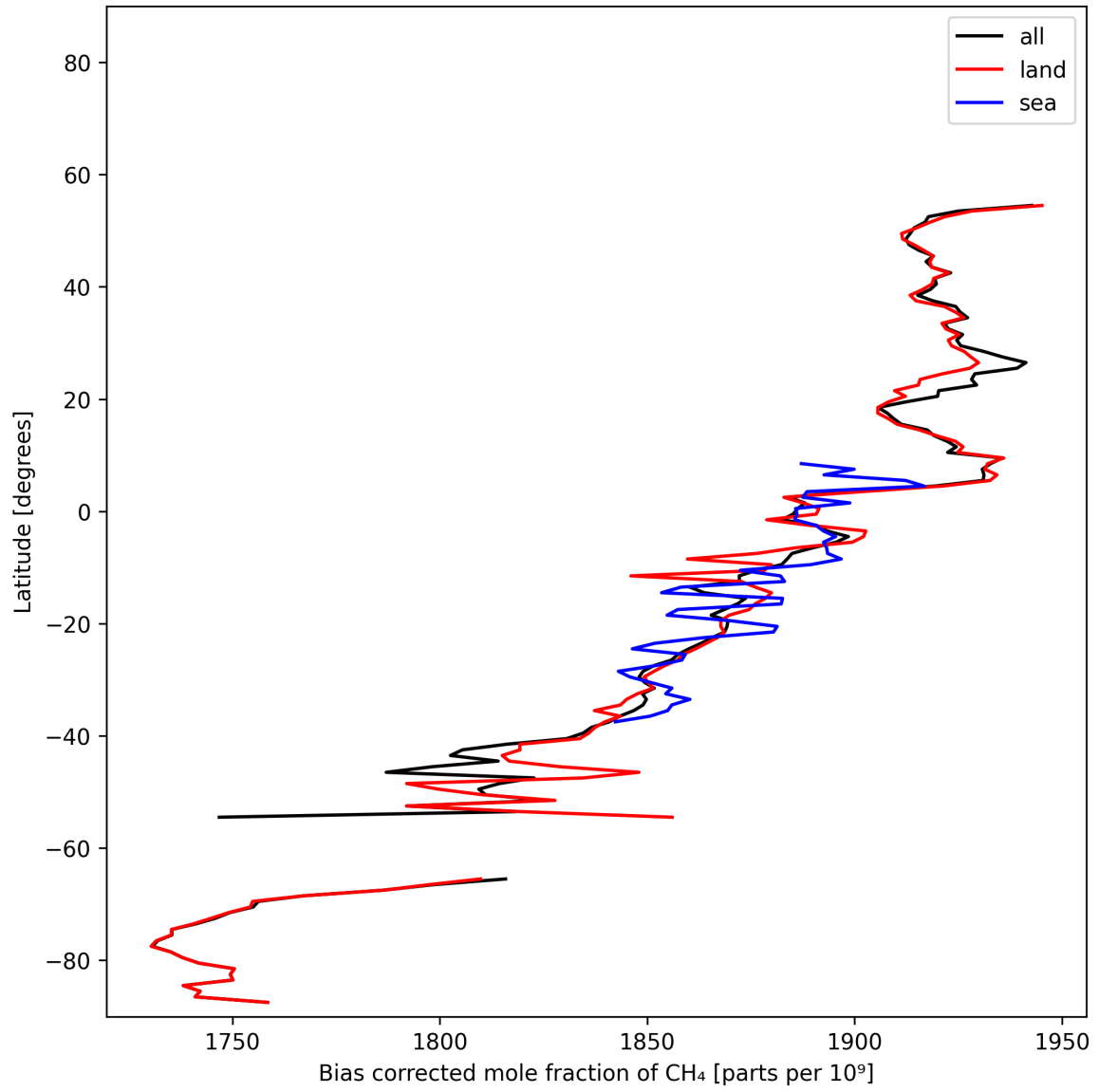
Figure 15: Zonal average of “Bias corrected mole fraction of CH 4 ” for 2025-11-23 to 2025-11-24.
