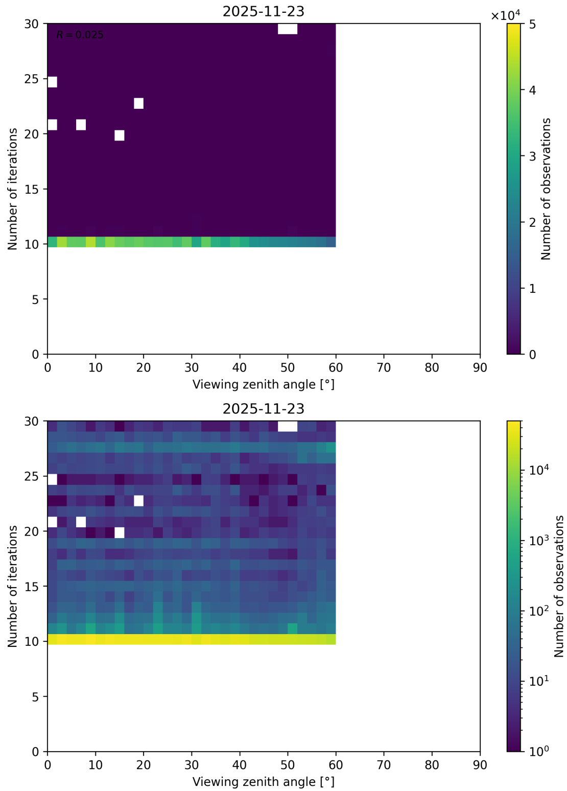
Figure 129: Scatter density plot of “Viewing zenith angle” against “Number of iterations” for 2025-11-23 to 2025-11-24.
