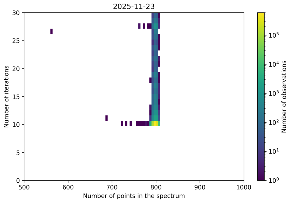
Figure 106: Scatter density plot of “Number of points in the spectrum” against “Number of iterations” for 2025-11-23 to 2025-11-24.
