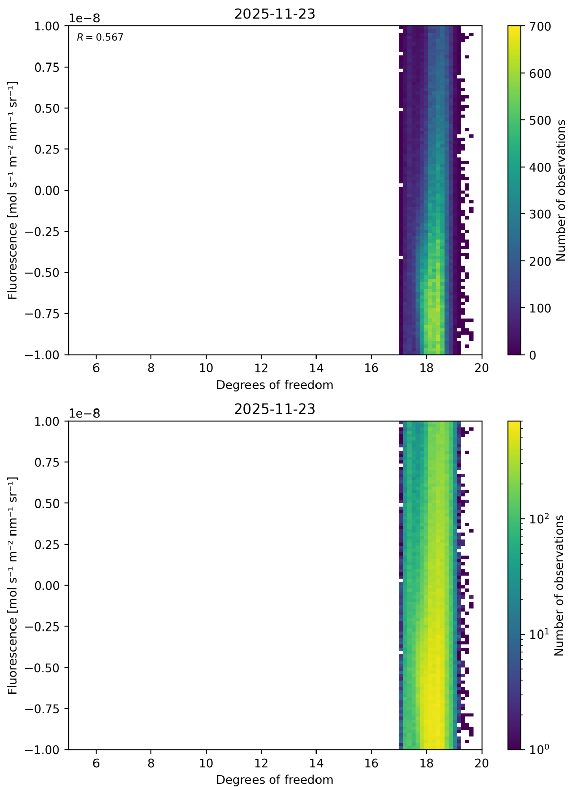
Figure 57: Scatter density plot of “Degrees of freedom” against “Fluorescence” for 2025-11-23 to 2025-11-24.
