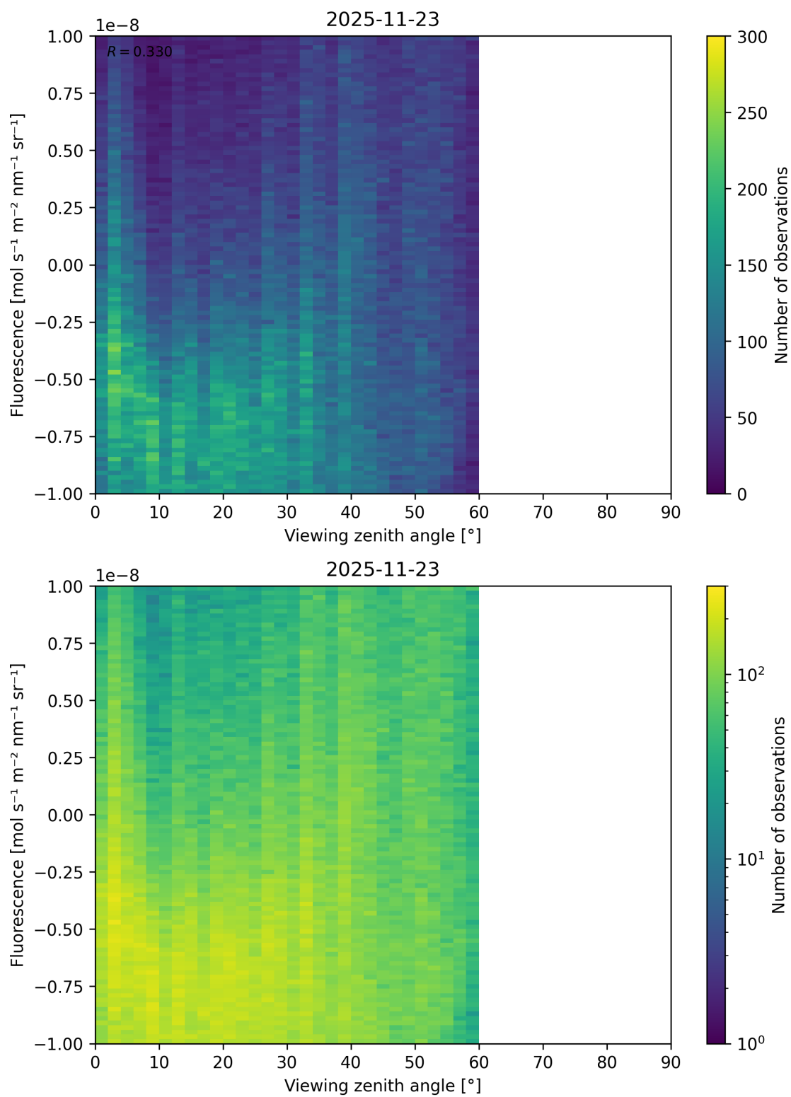
Figure 123: Scatter density plot of “Viewing zenith angle” against “Fluorescence” for 2025-11-23 to 2025-11-24.
