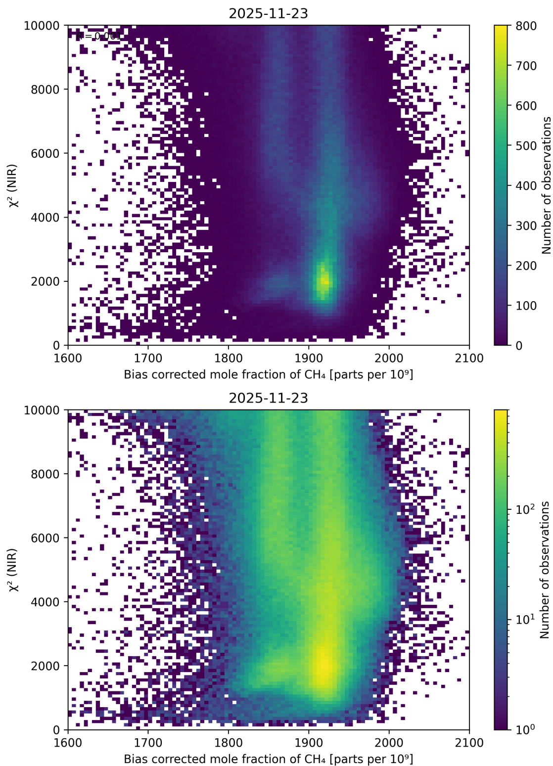
Figure 72: Scatter density plot of “Bias corrected mole fraction of CH 4 ” against “ \chi^2 (NIR)” for 2025-11-23 to 2025-11-24.
