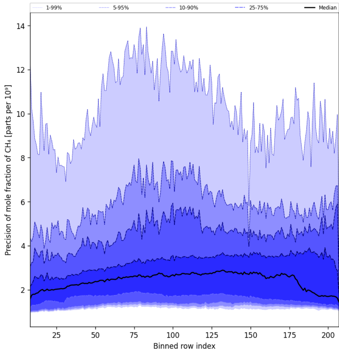
Figure 38: Along track statistics of “Precision of mole fraction of CH 4 ” for 2025-11-23 to 2025-11-24
