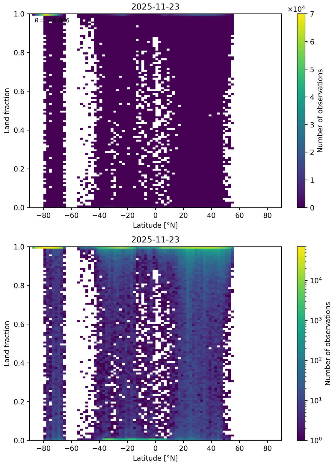
Figure 65: Scatter density plot of “Latitude” against “Land fraction” for 2025-11-23 to 2025-11-24.
