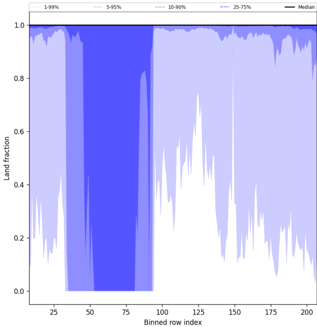
Figure 47: Along track statistics of "Land fraction" for 2025-11-23 to 2025-11-24
