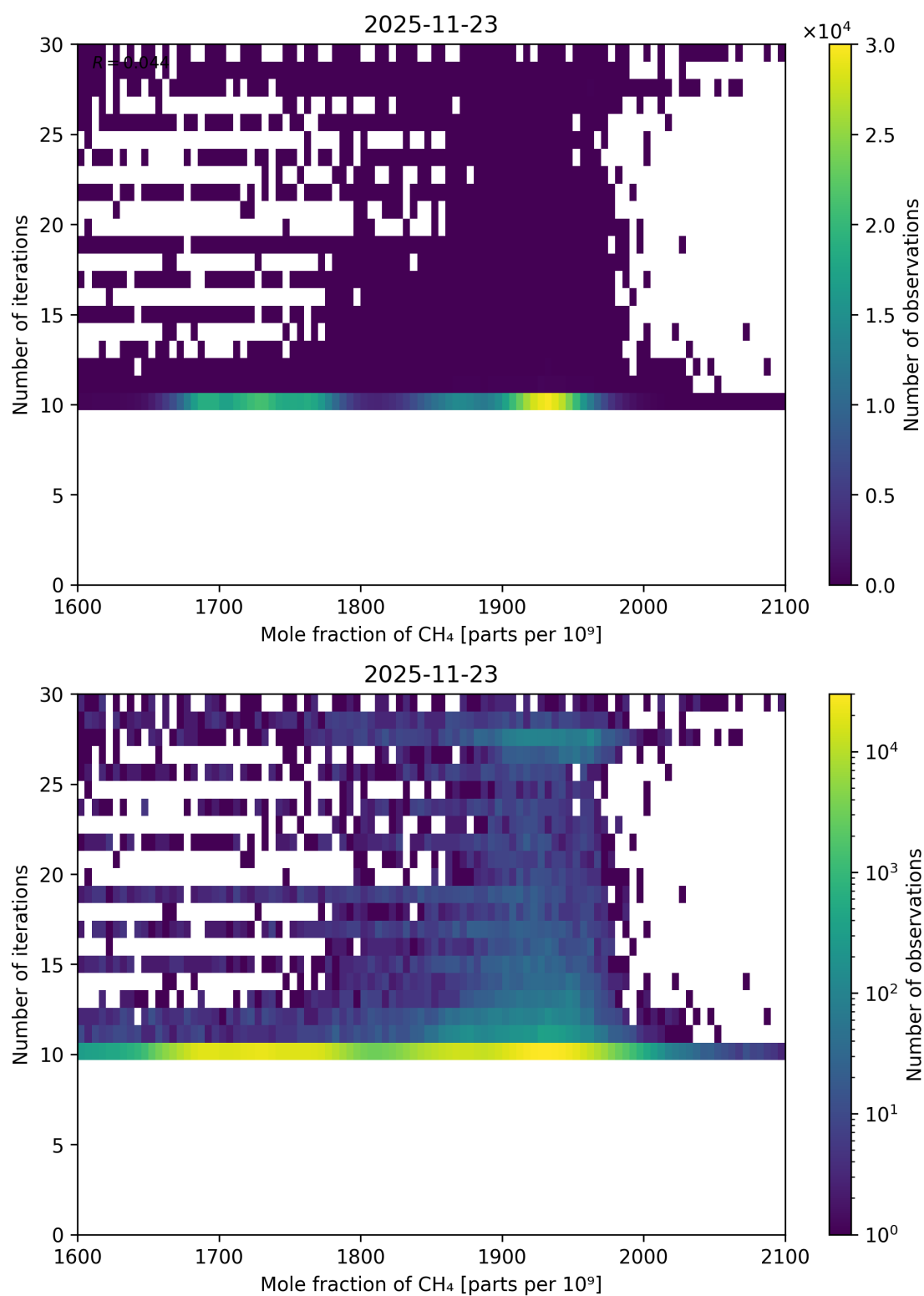
Figure 87: Scatter density plot of “Mole fraction of CH 4 ” against “Number of iterations” for 2025-11-23 to 2025-11-24.
