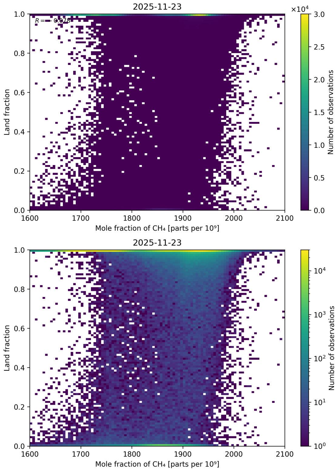
Figure 84: Scatter density plot of “Mole fraction of CH 4 ” against “Land fraction” for 2025-11-23 to 2025-11-24.
