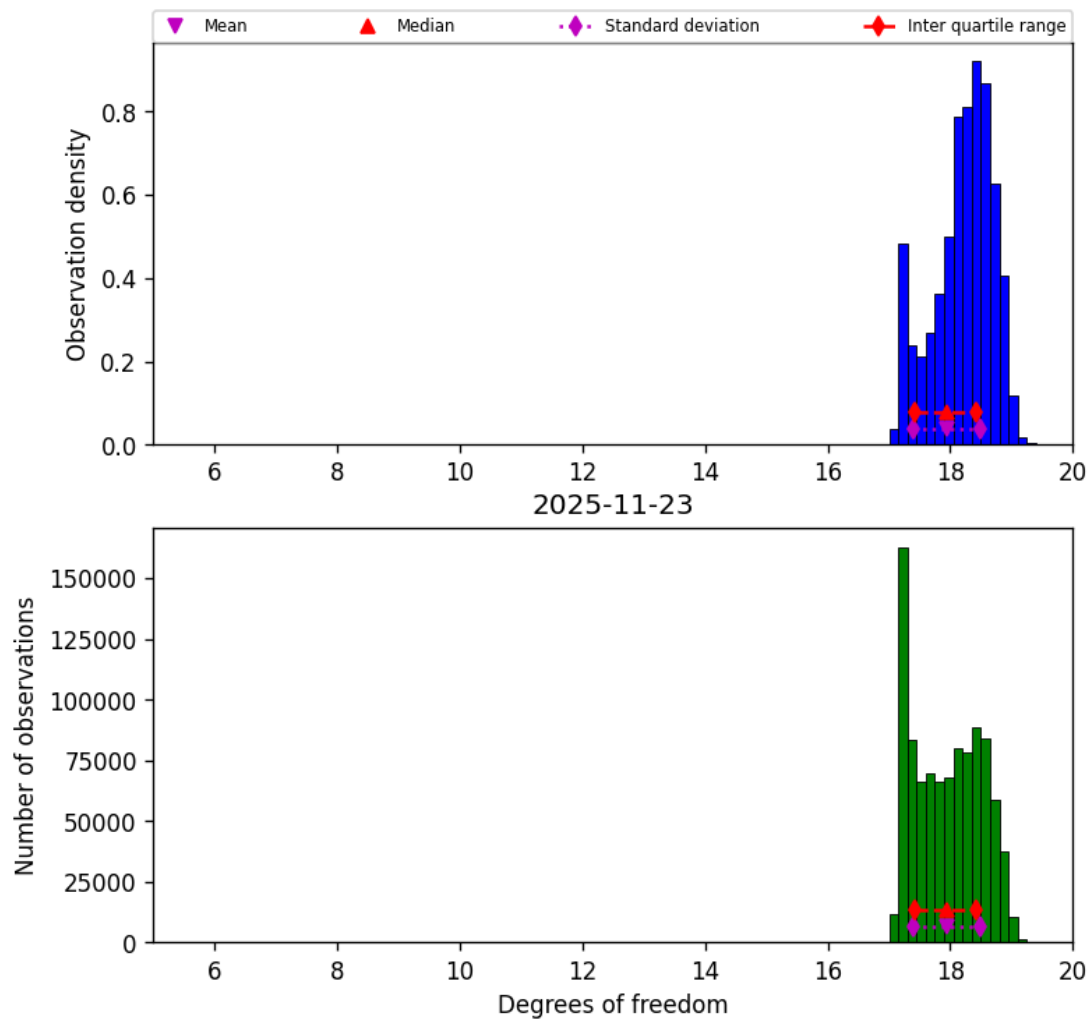
Figure 32: Histogram of “Degrees of freedom” for 2025-11-23 to 2025-11-24
