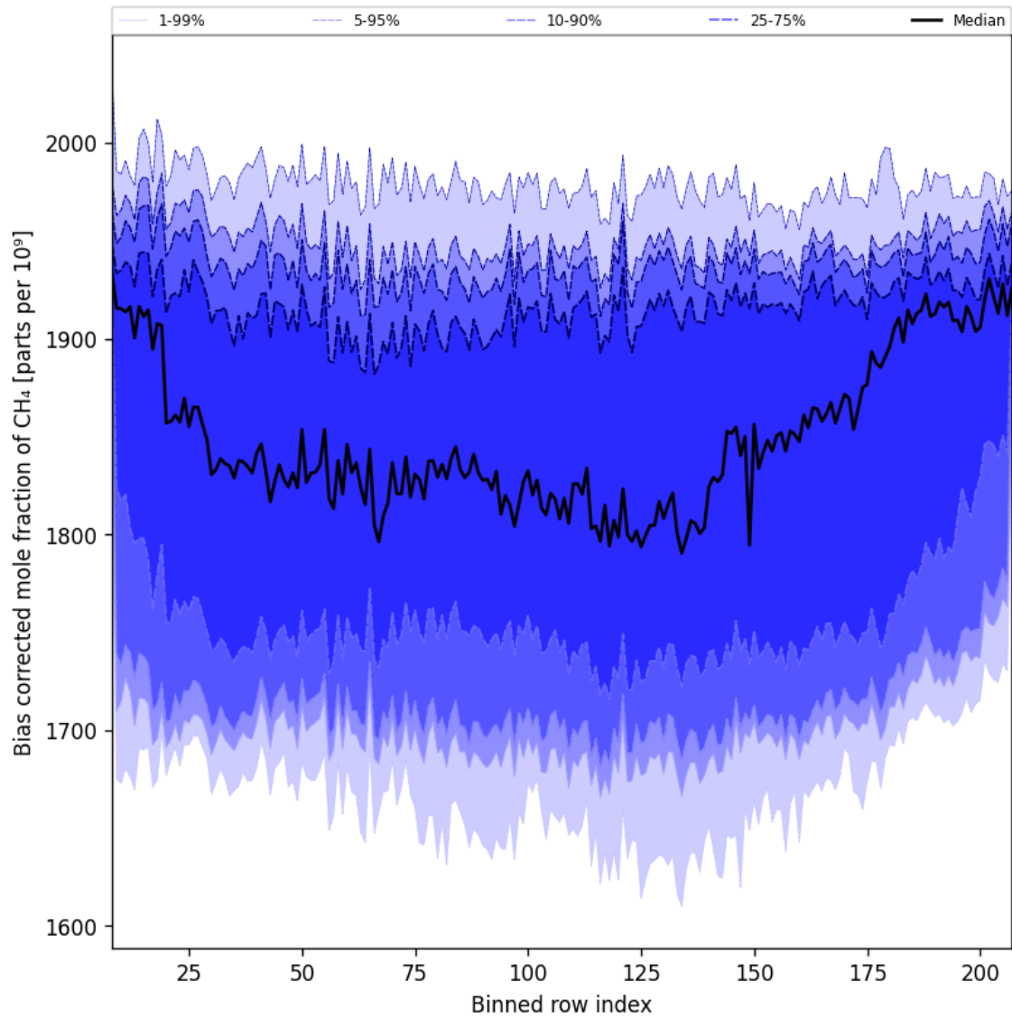
Figure 39: Along track statistics of “Bias corrected mole fraction of CH 4 ” for 2025-11-23 to 2025-11-24
