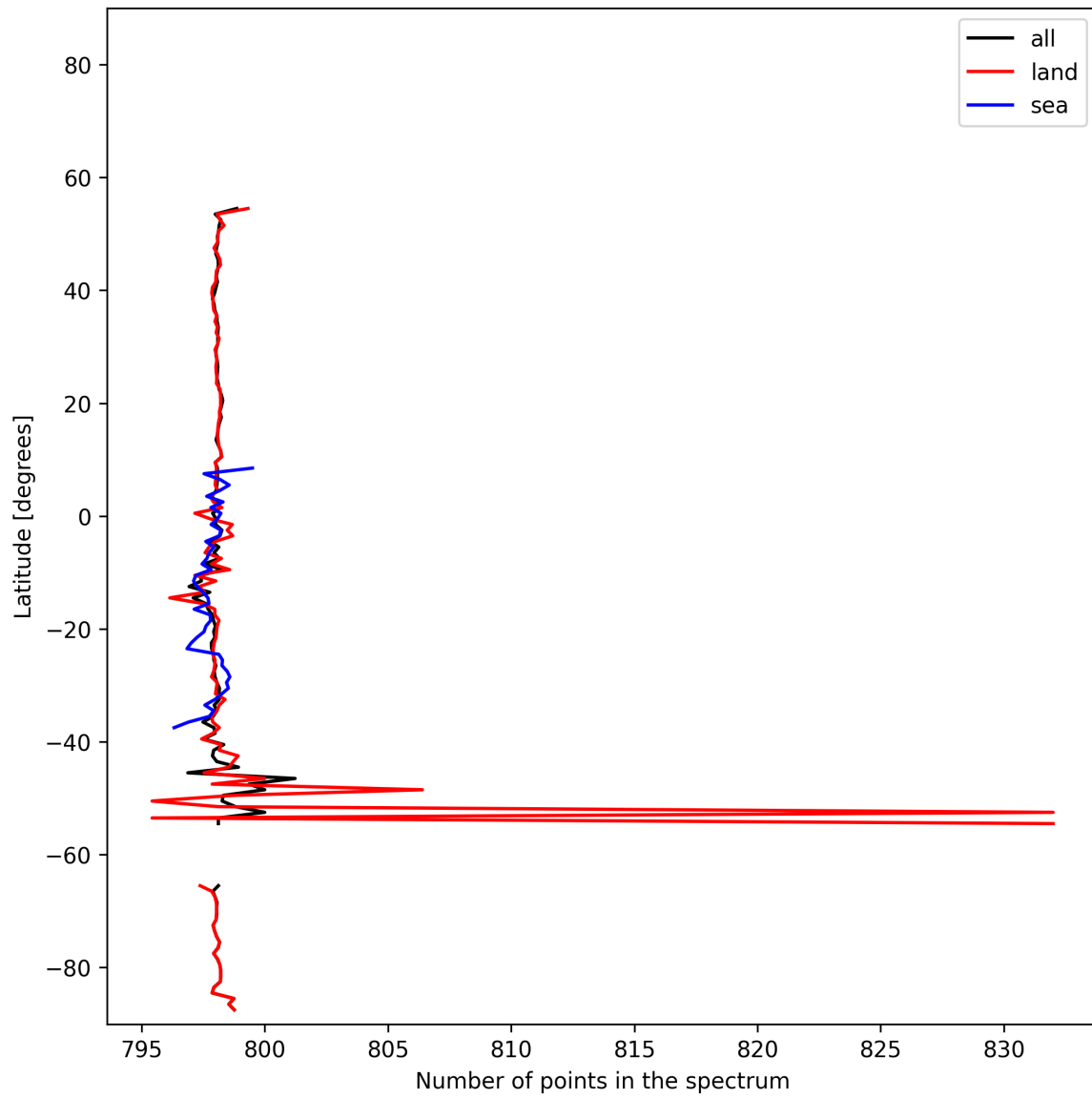
Figure 16: Zonal average of “Number of points in the spectrum” for 2025-11-23 to 2025-11-24.
