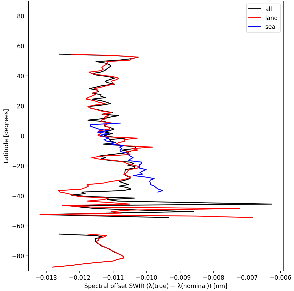
Figure 17: Zonal average of “Spectral offset SWIR ( \lambda_{\text{true}} - \lambda_{\text{nominal}} )” for 2025-11-23 to 2025-11-24.
