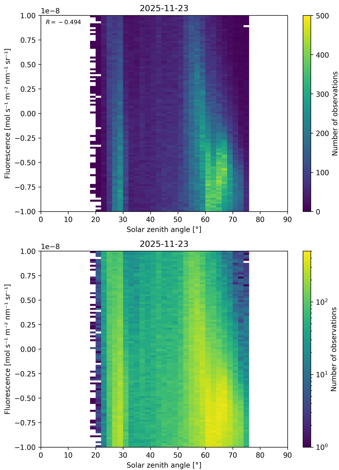
Figure 111: Scatter density plot of “Solar zenith angle” against “Fluorescence” for 2025-11-23 to 2025-11-24.
