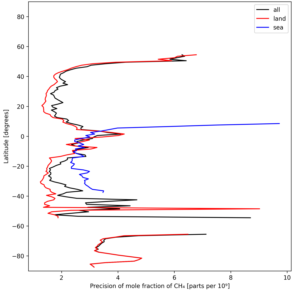
Figure 14: Zonal average of “Precision of mole fraction of CH 4 ” for 2025-11-23 to 2025-11-24.
