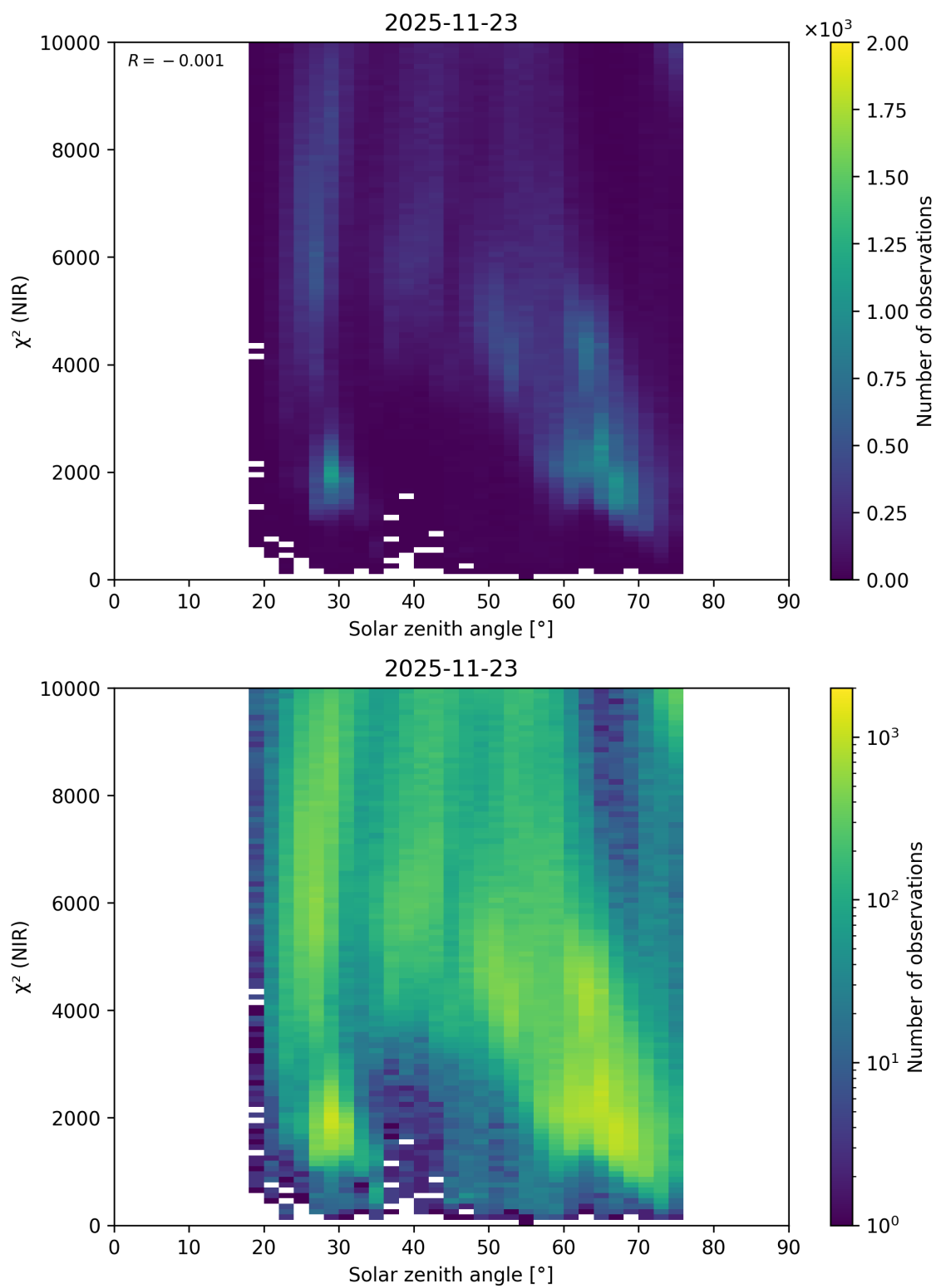
Figure 108: Scatter density plot of “Solar zenith angle” against “ \chi^2 (NIR)” for 2025-11-23 to 2025-11-24.
