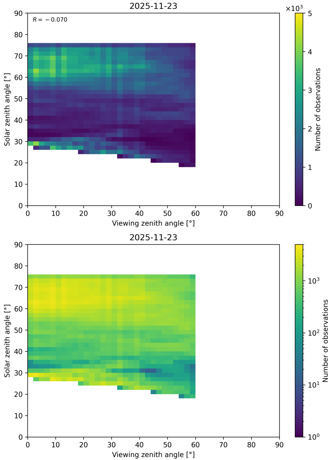
Figure 131: Scatter density plot of “Viewing zenith angle” against “Solar zenith angle” for 2025-11-23 to 2025-11-24.
