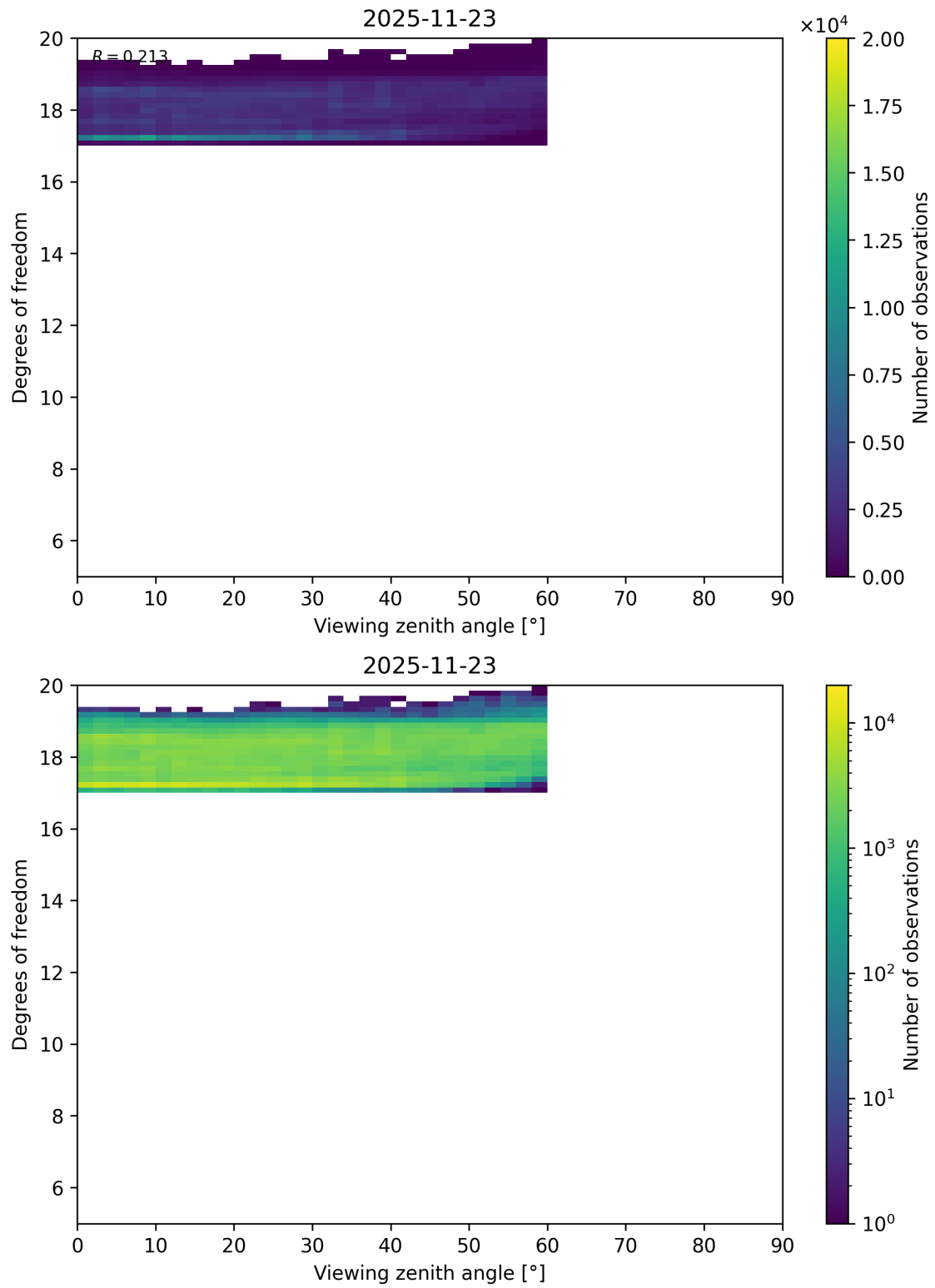
Figure 122: Scatter density plot of “Viewing zenith angle” against “Degrees of freedom” for 2025-11-23 to 2025-11-24.
