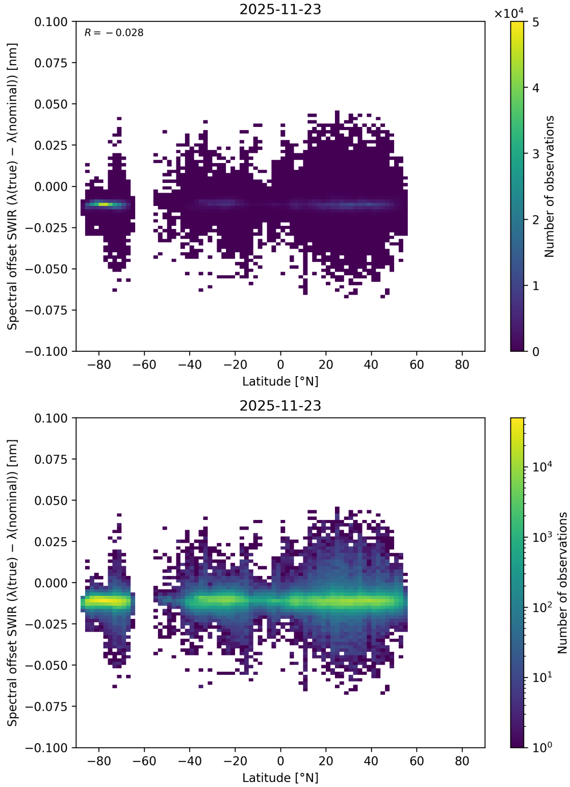
Figure 71: Scatter density plot of “Latitude” against “Spectral offset SWIR ( \lambda_{\text{true}} - \lambda_{\text{nominal}} )” for 2025-11-23 to 2025-11-24.
