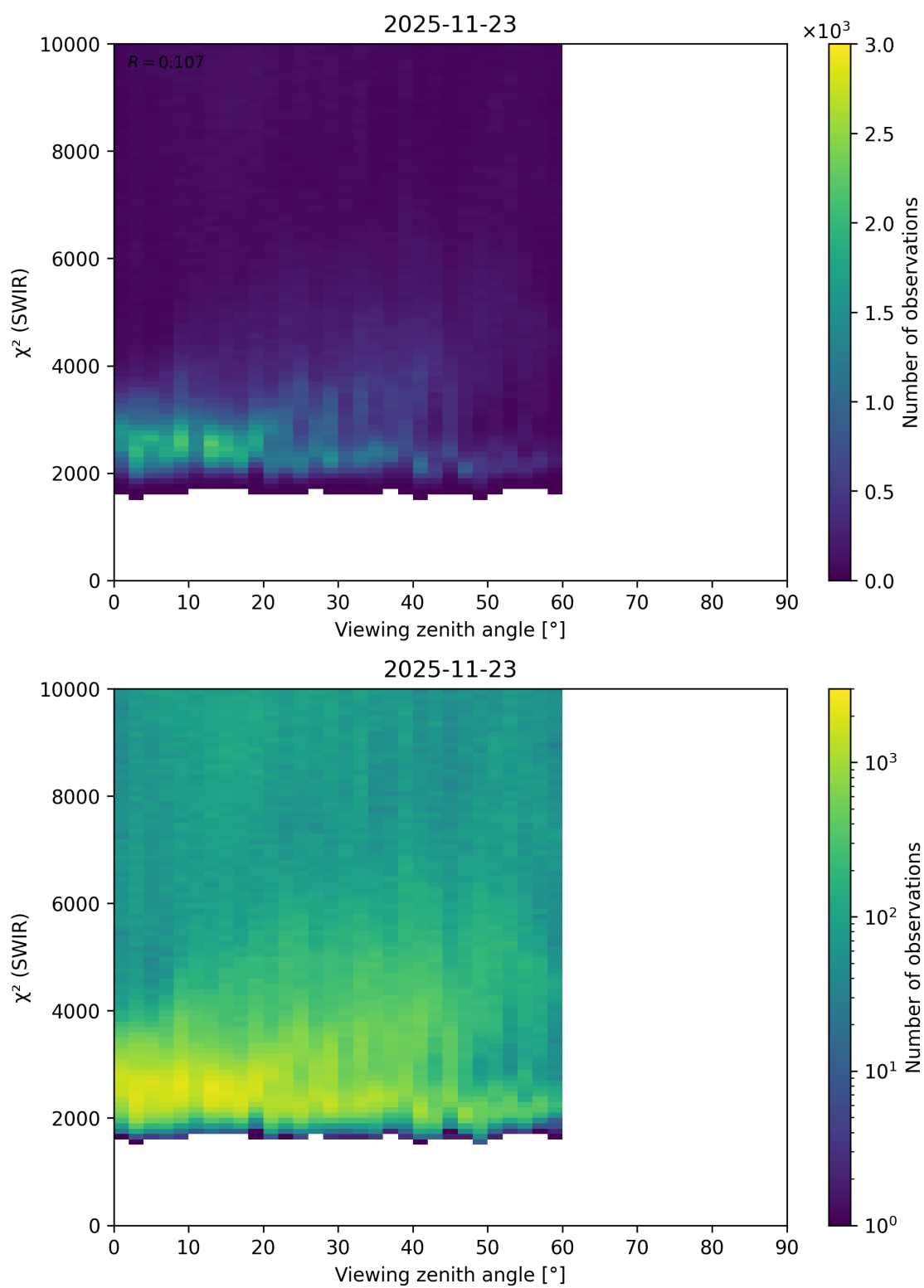
Figure 121: Scatter density plot of “Viewing zenith angle” against “ \chi^2 (SWIR)” for 2025-11-23 to 2025-11-24.
