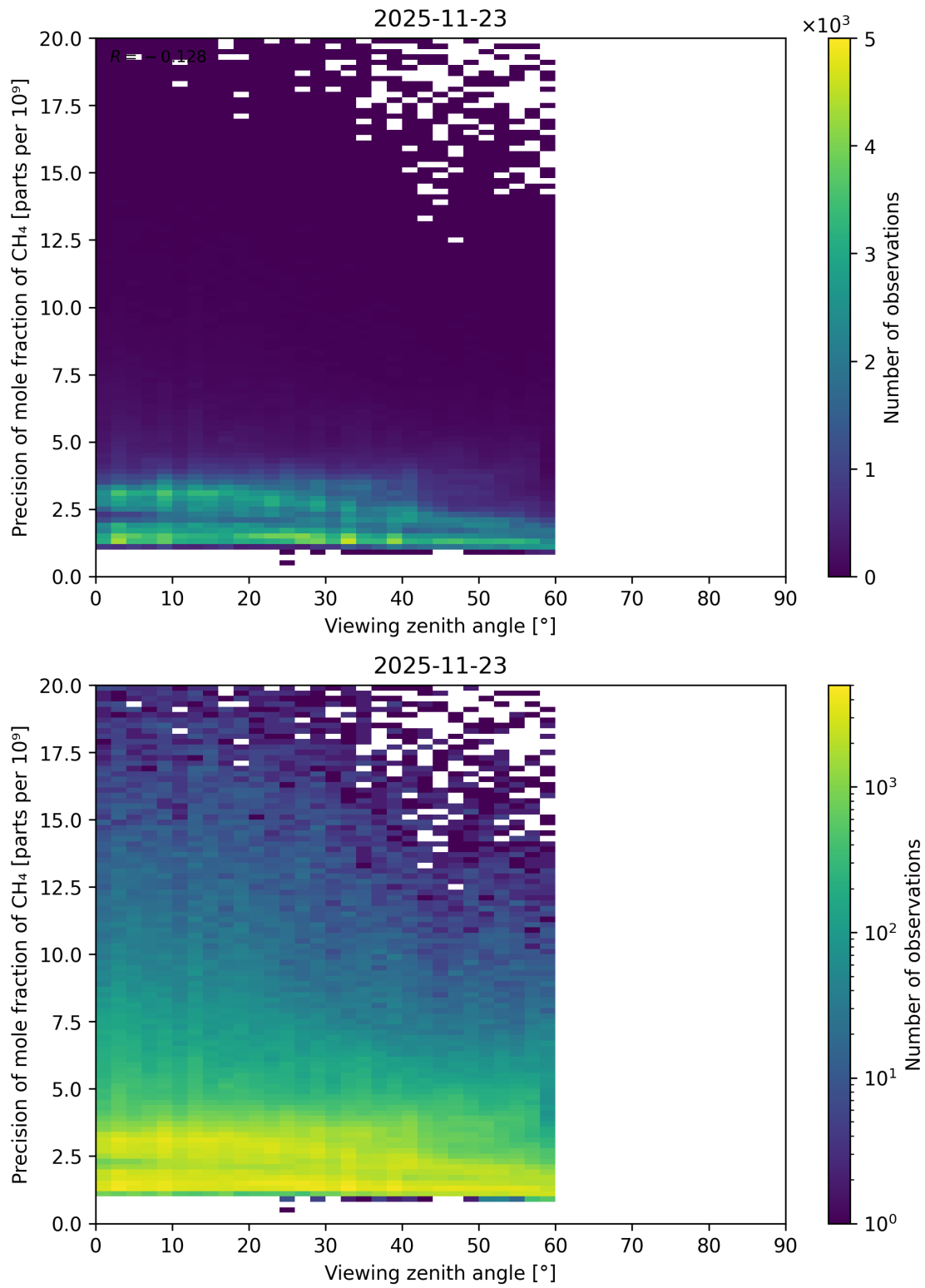
Figure 128: Scatter density plot of “Viewing zenith angle” against “Precision of mole fraction of CH 4 ” for 2025-11-23 to 2025-11-24.
