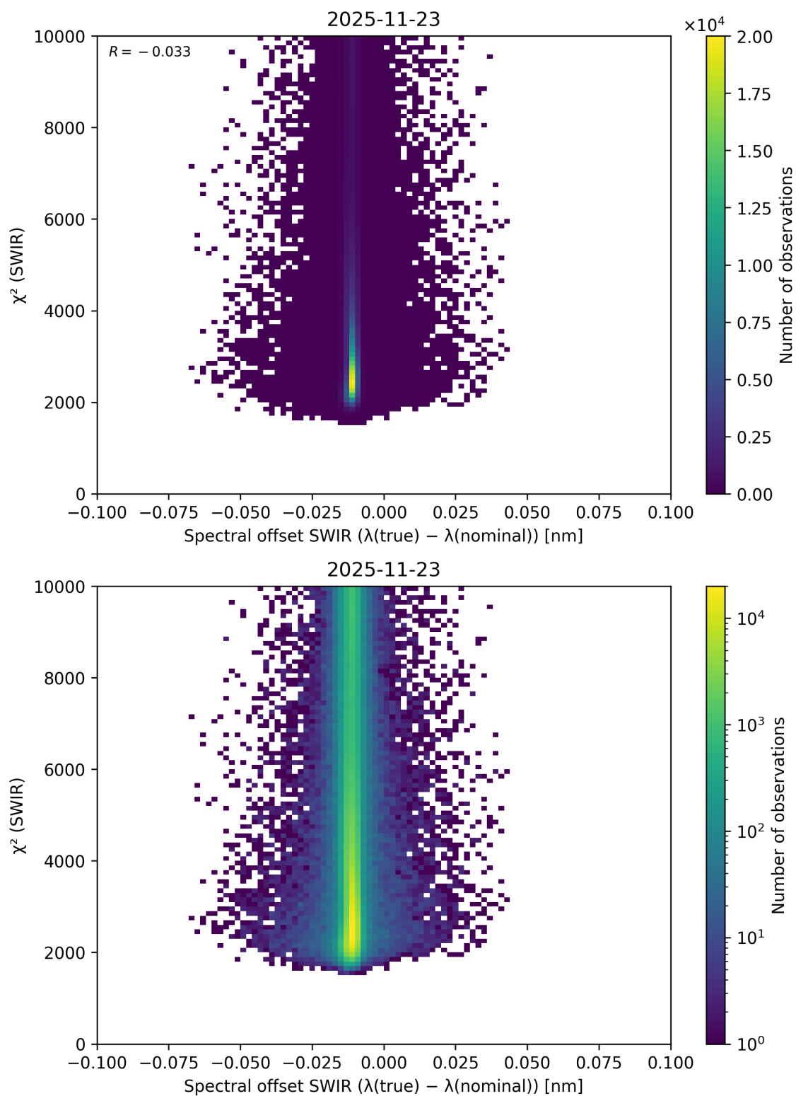
Figure 134: Scatter density plot of “Spectral offset SWIR ( \lambda_{\text{true}} - \lambda_{\text{nominal}} )” against “ \chi^2 (SWIR)” for 2025-11-23 to 2025-11-24.
