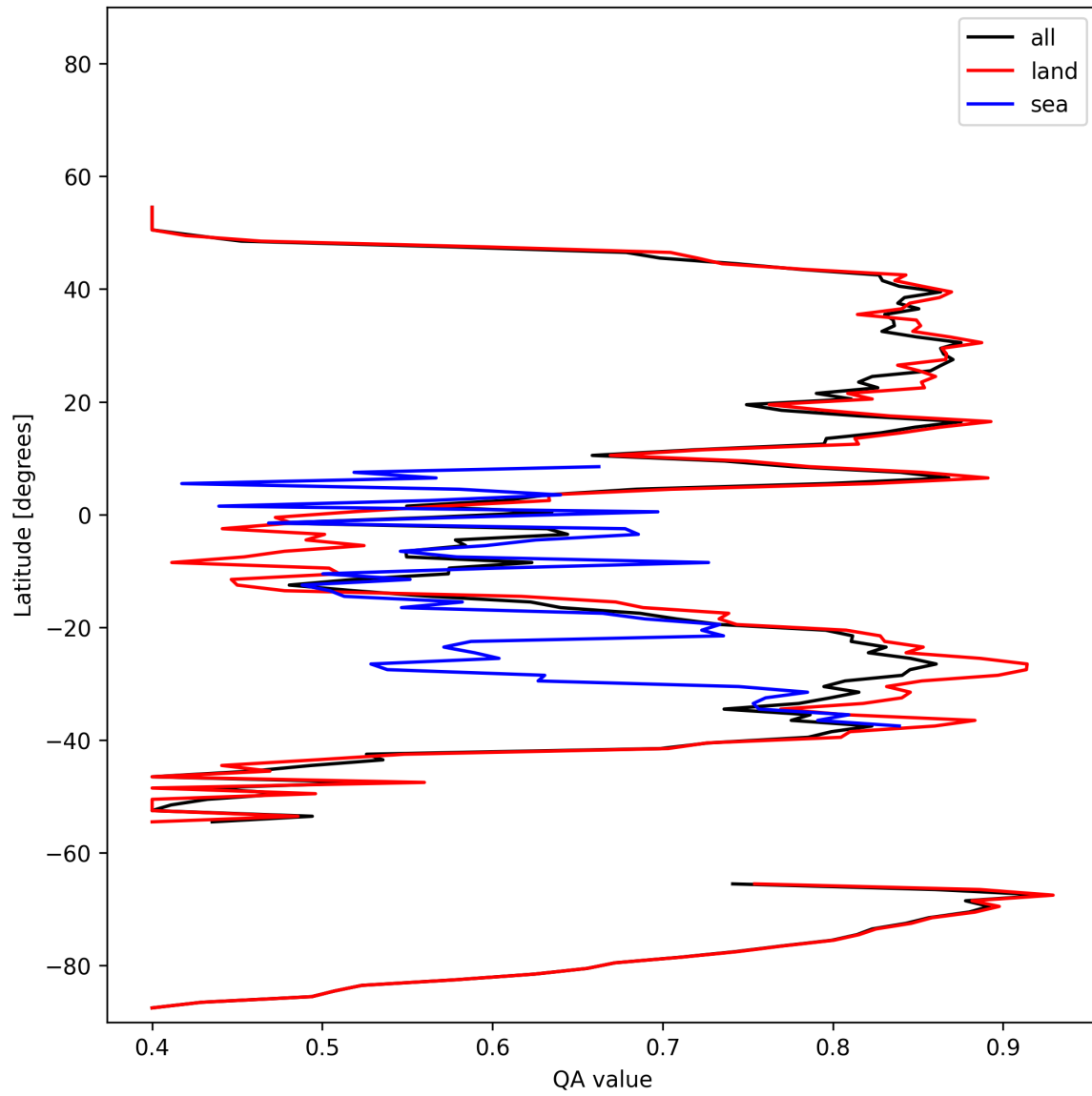
Figure 12: Zonal average of “QA value” for 2025-11-23 to 2025-11-24.
