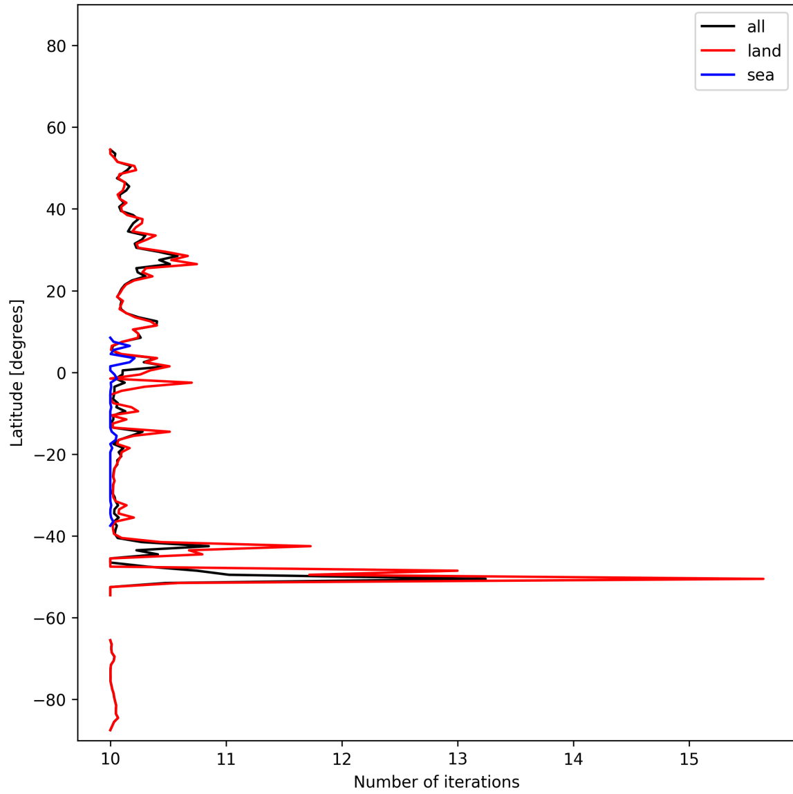
Figure 21: Zonal average of “Number of iterations” for 2025-11-23 to 2025-11-24.
