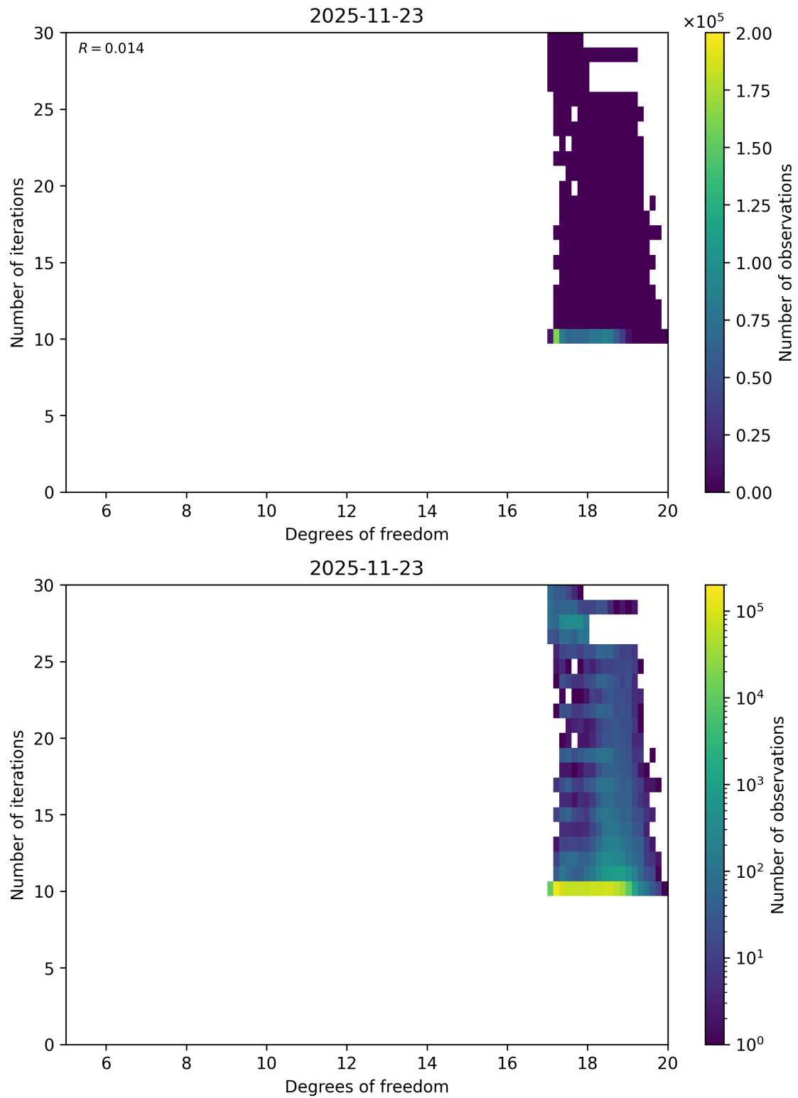
Figure 59: Scatter density plot of “Degrees of freedom” against “Number of iterations” for 2025-11-23 to 2025-11-24.
