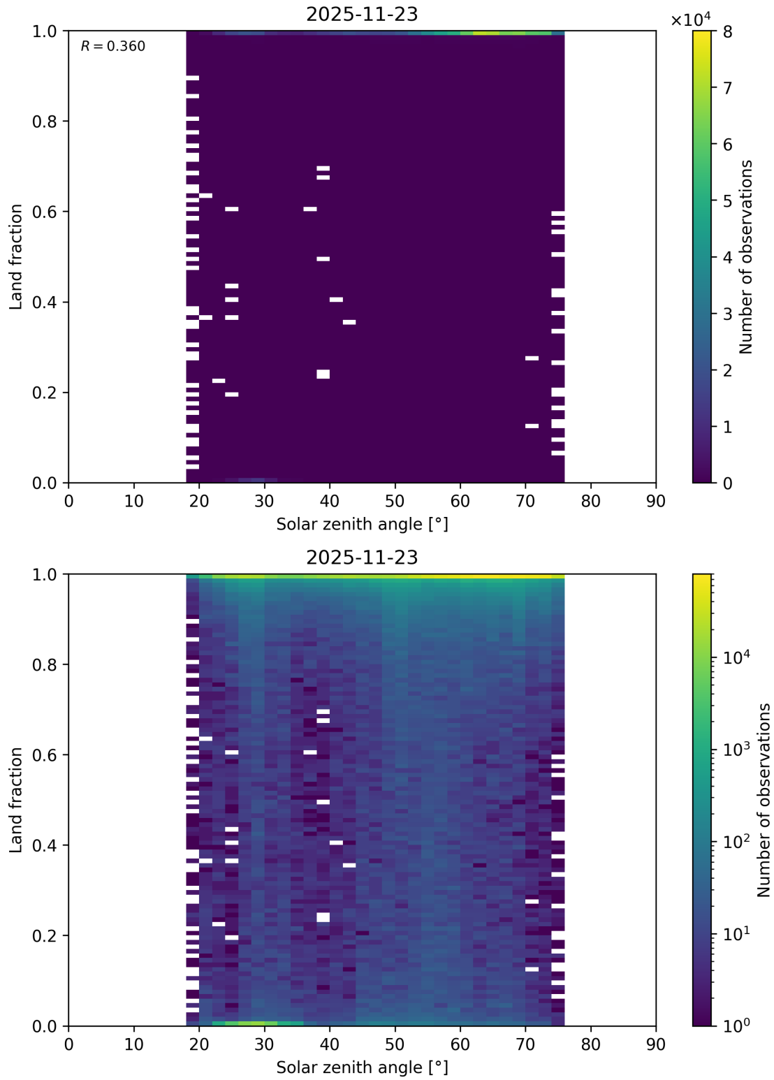
Figure 112: Scatter density plot of “Solar zenith angle” against “Land fraction” for 2025-11-23 to 2025-11-24.
