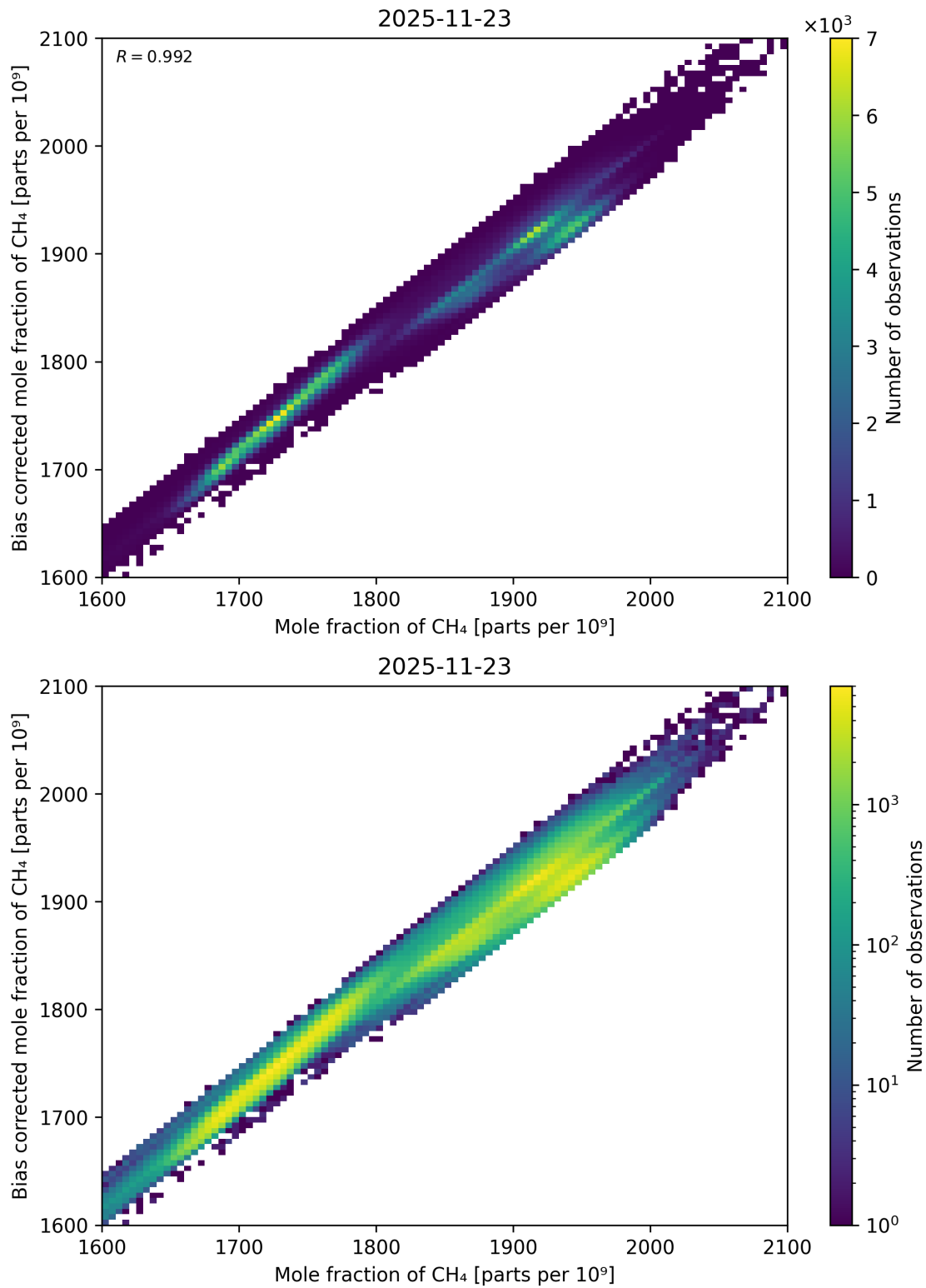
Figure 85: Scatter density plot of “Mole fraction of CH 4 ” against “Bias corrected mole fraction of CH 4 ” for 2025-11-23 to 2025-11-24.
