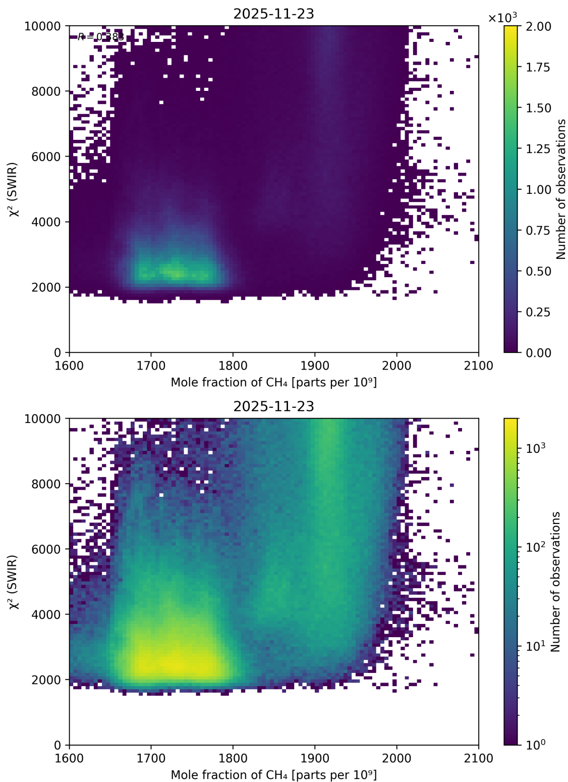
Figure 81: Scatter density plot of “Mole fraction of \text{CH}_4 ” against “ \chi^2 (SWIR)” for 2025-11-23 to 2025-11-24.
