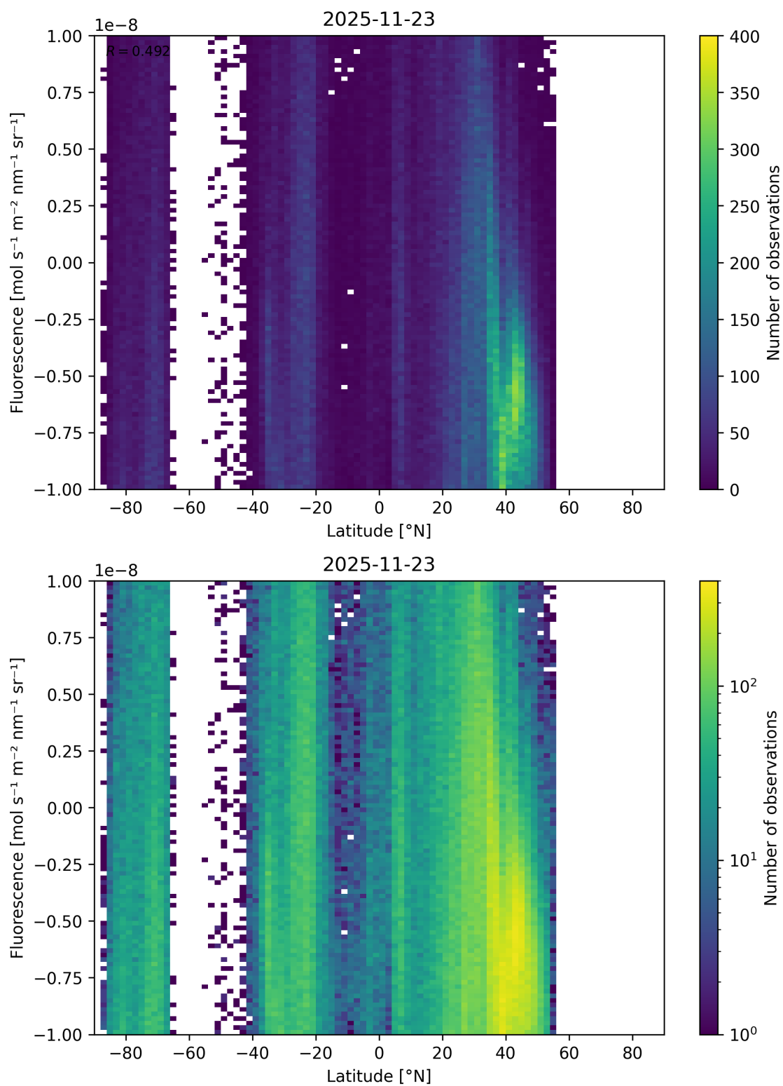
Figure 64: Scatter density plot of “Latitude” against “Fluorescence” for 2025-11-23 to 2025-11-24.
