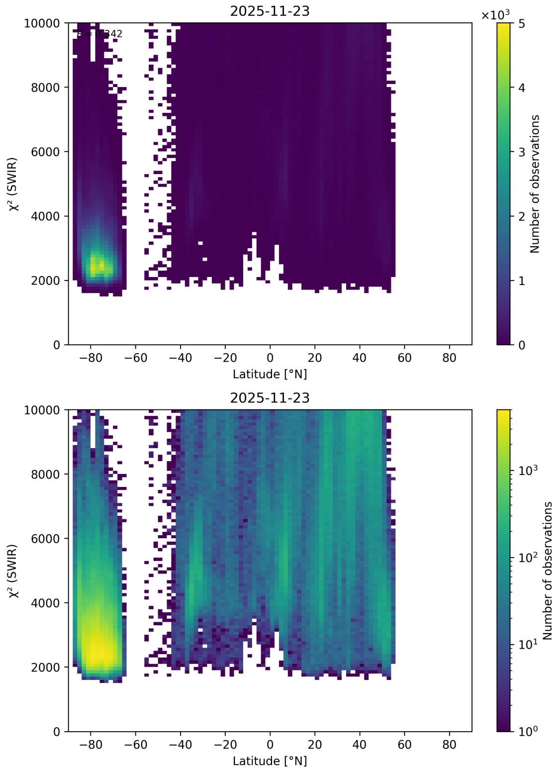
Figure 62: Scatter density plot of “Latitude” against “ \chi^2 (SWIR)” for 2025-11-23 to 2025-11-24.
