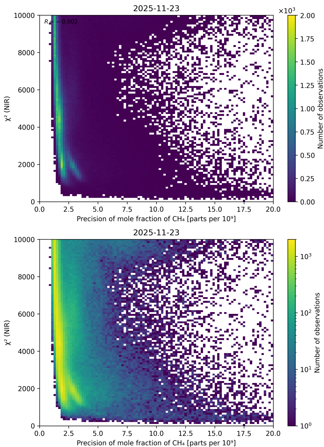
Figure 89: Scatter density plot of “Precision of mole fraction of CH 4 ” against “ \chi^2 (NIR)” for 2025-11-23 to 2025-11-24.
