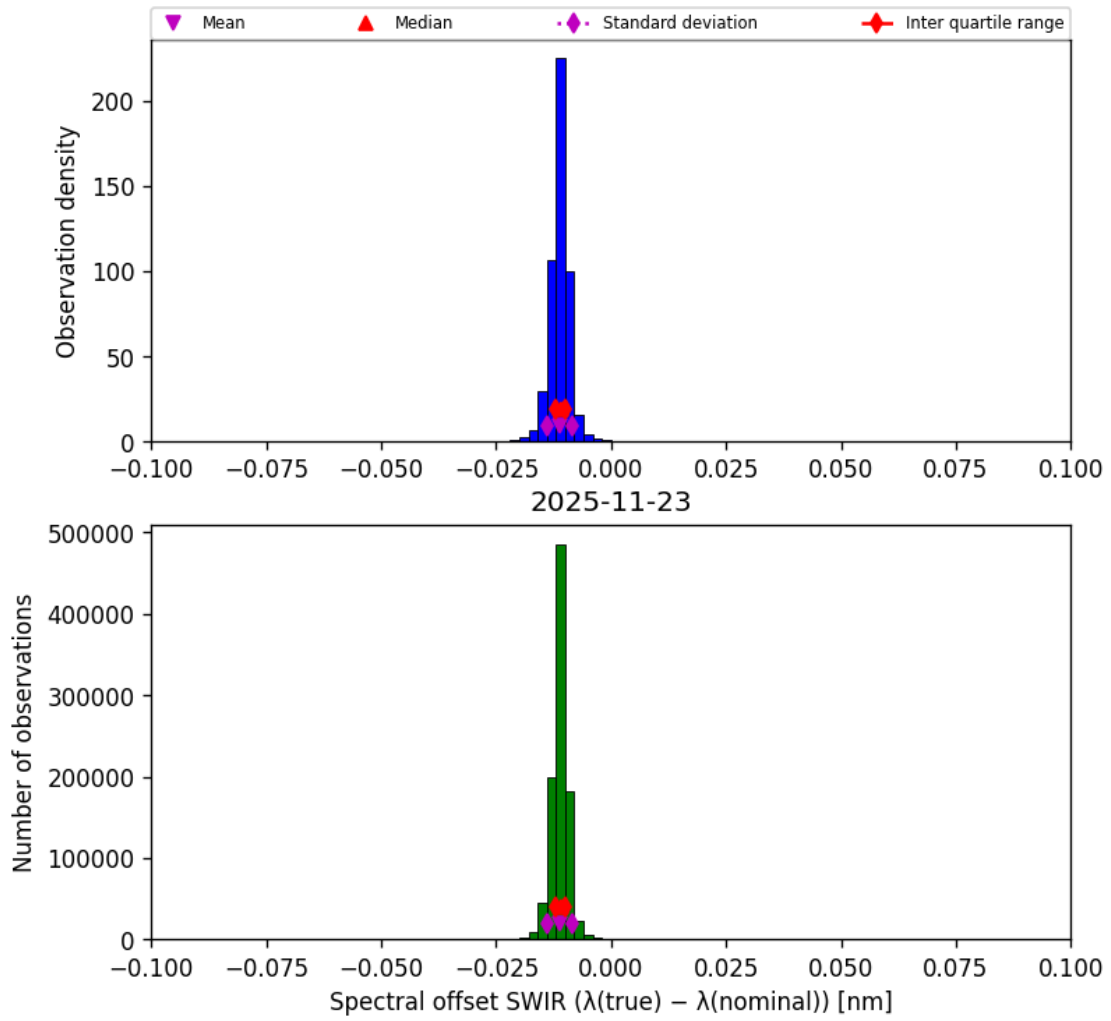
Figure 29: Histogram of “Spectral offset SWIR ( \lambda_{\text{true}} - \lambda_{\text{nominal}} )” for 2025-11-23 to 2025-11-24
