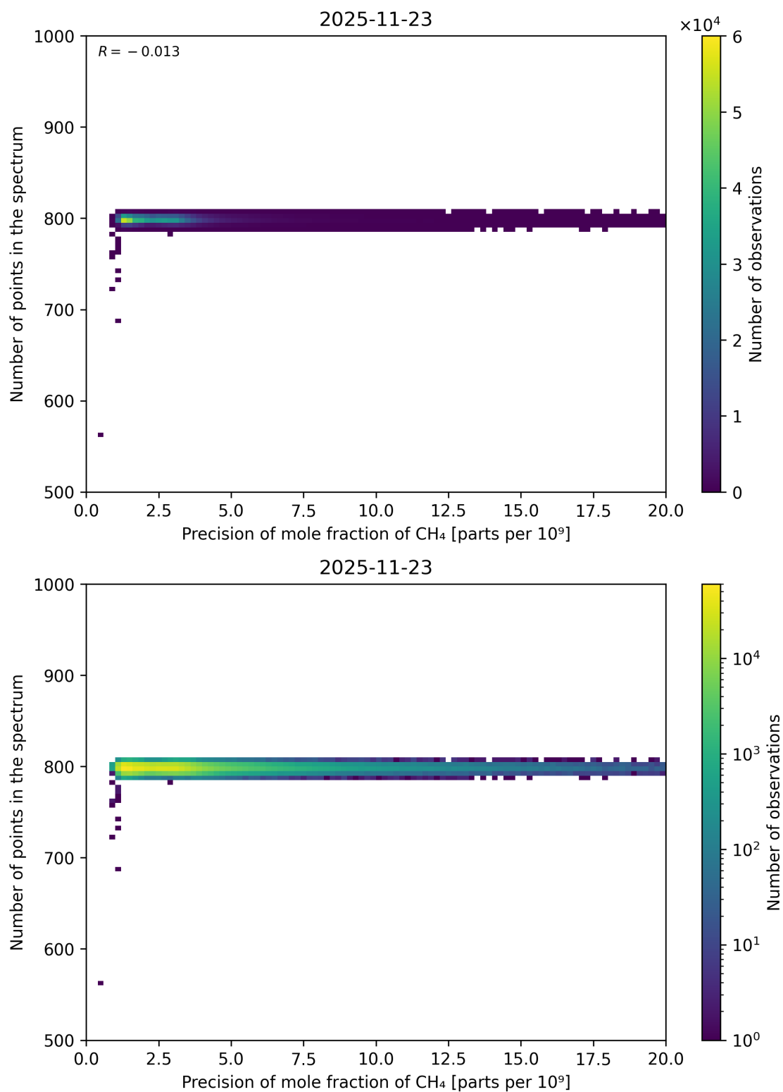
Figure 96: Scatter density plot of “Precision of mole fraction of CH 4 ” against “Number of points in the spectrum” for 2025-11-23 to 2025-11-24.
