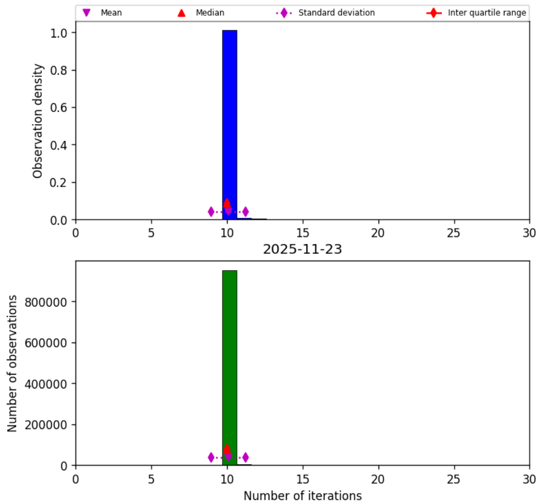
Figure 33: Histogram of “Number of iterations” for 2025-11-23 to 2025-11-24
