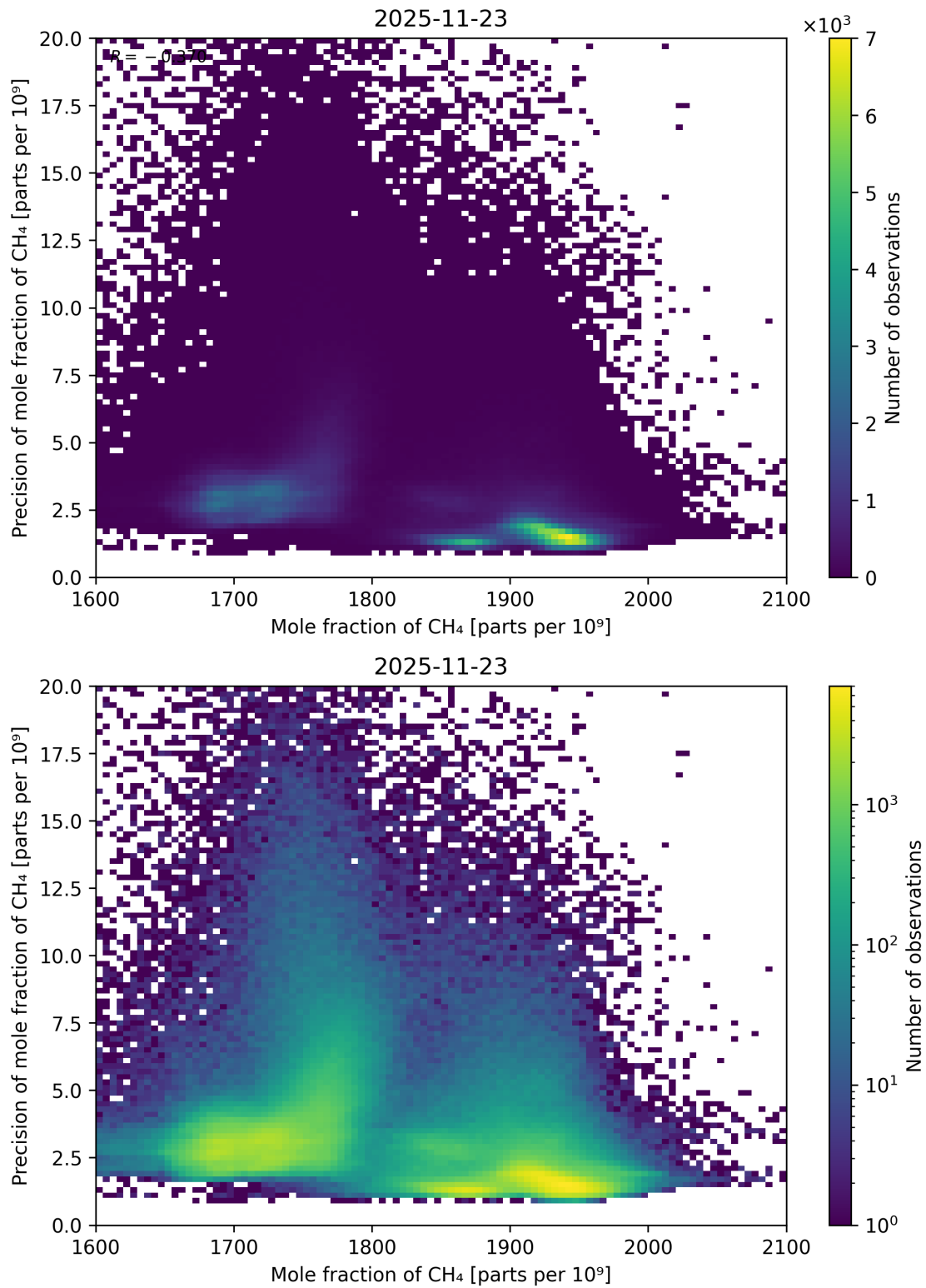
Figure 86: Scatter density plot of “Mole fraction of CH 4 ” against “Precision of mole fraction of CH 4 ” for 2025-11-23 to 2025-11-24.
