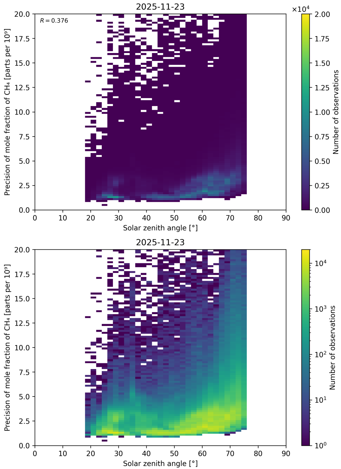
Figure 116: Scatter density plot of “Solar zenith angle” against “Precision of mole fraction of \text{CH}_4 ” for 2025-11-23 to 2025-11-24.
