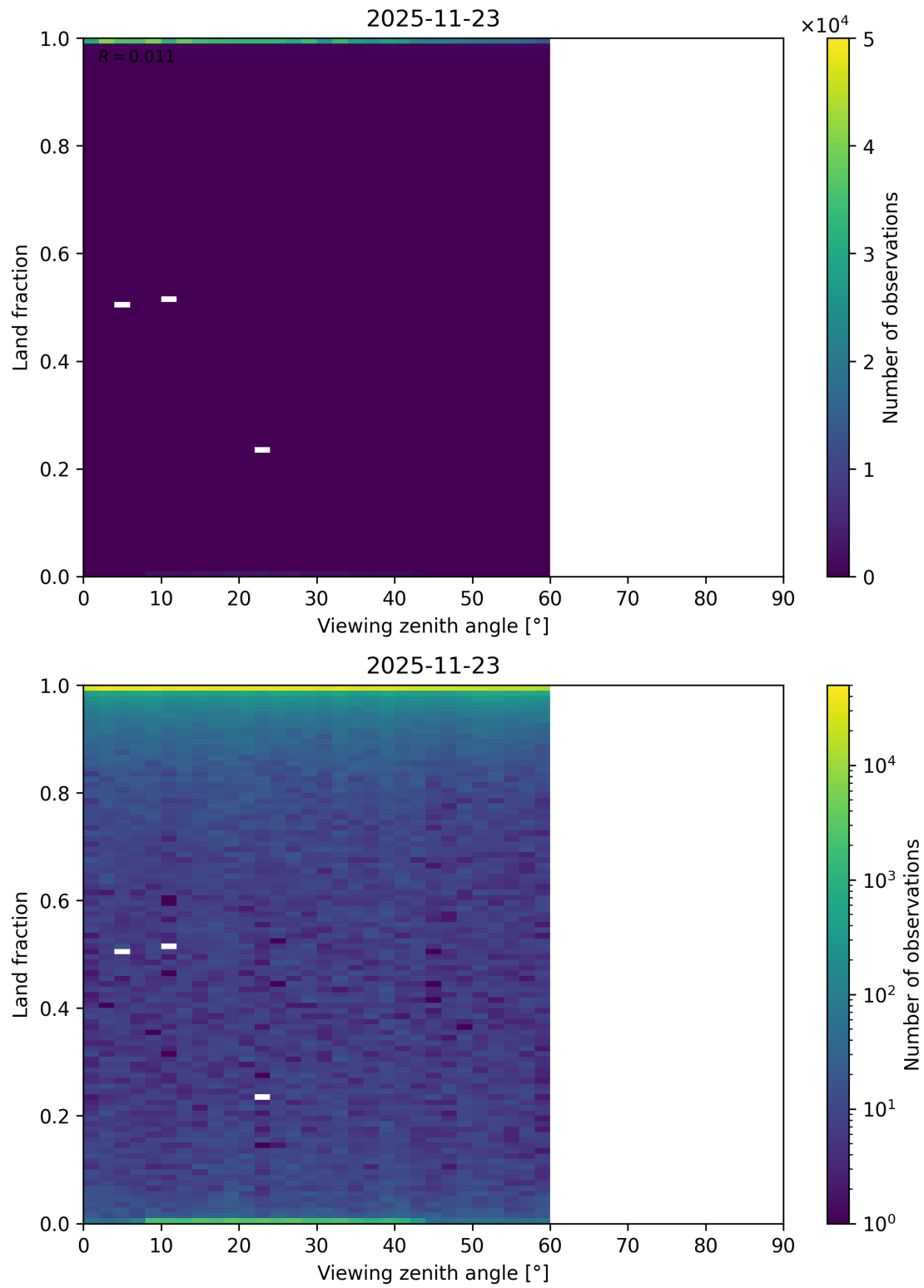
Figure 124: Scatter density plot of “Viewing zenith angle” against “Land fraction” for 2025-11-23 to 2025-11-24.
