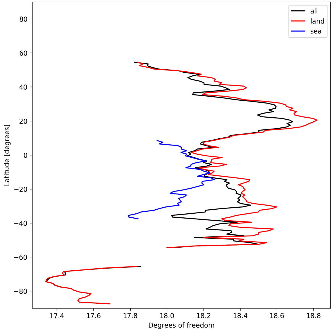
Figure 20: Zonal average of “Degrees of freedom” for 2025-11-23 to 2025-11-24.
