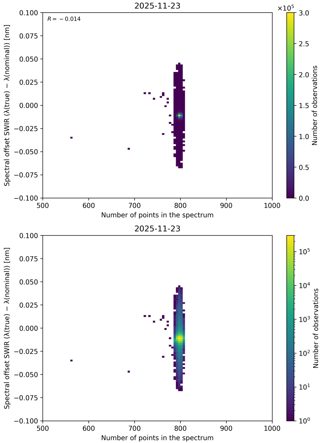
Figure 107: Scatter density plot of “Number of points in the spectrum” against “Spectral offset SWIR ( \lambda_{\text{true}} - \lambda_{\text{nominal}} )” for 2025-11-23 to 2025-11-24.
