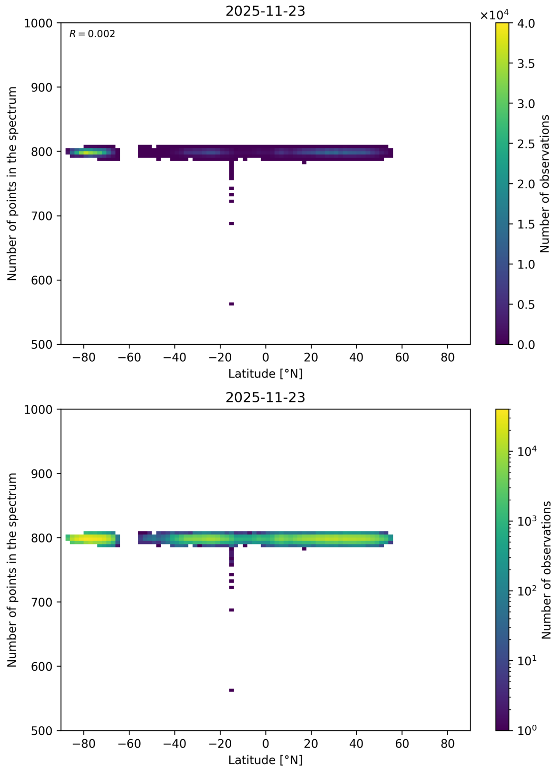
Figure 70: Scatter density plot of “Latitude” against “Number of points in the spectrum” for 2025-11-23 to 2025-11-24.
