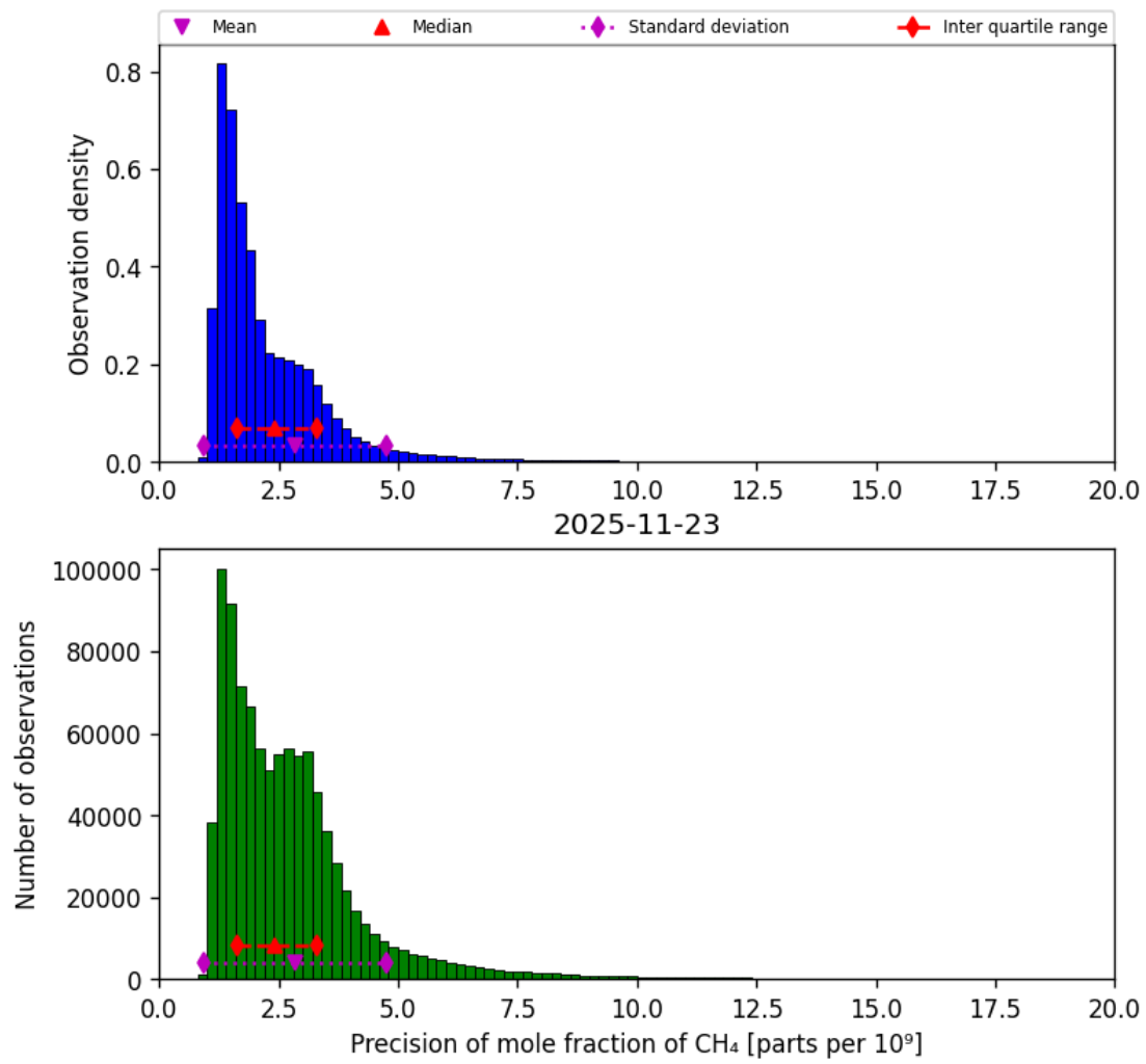
Figure 26: Histogram of “Precision of mole fraction of CH 4 ” for 2025-11-23 to 2025-11-24
