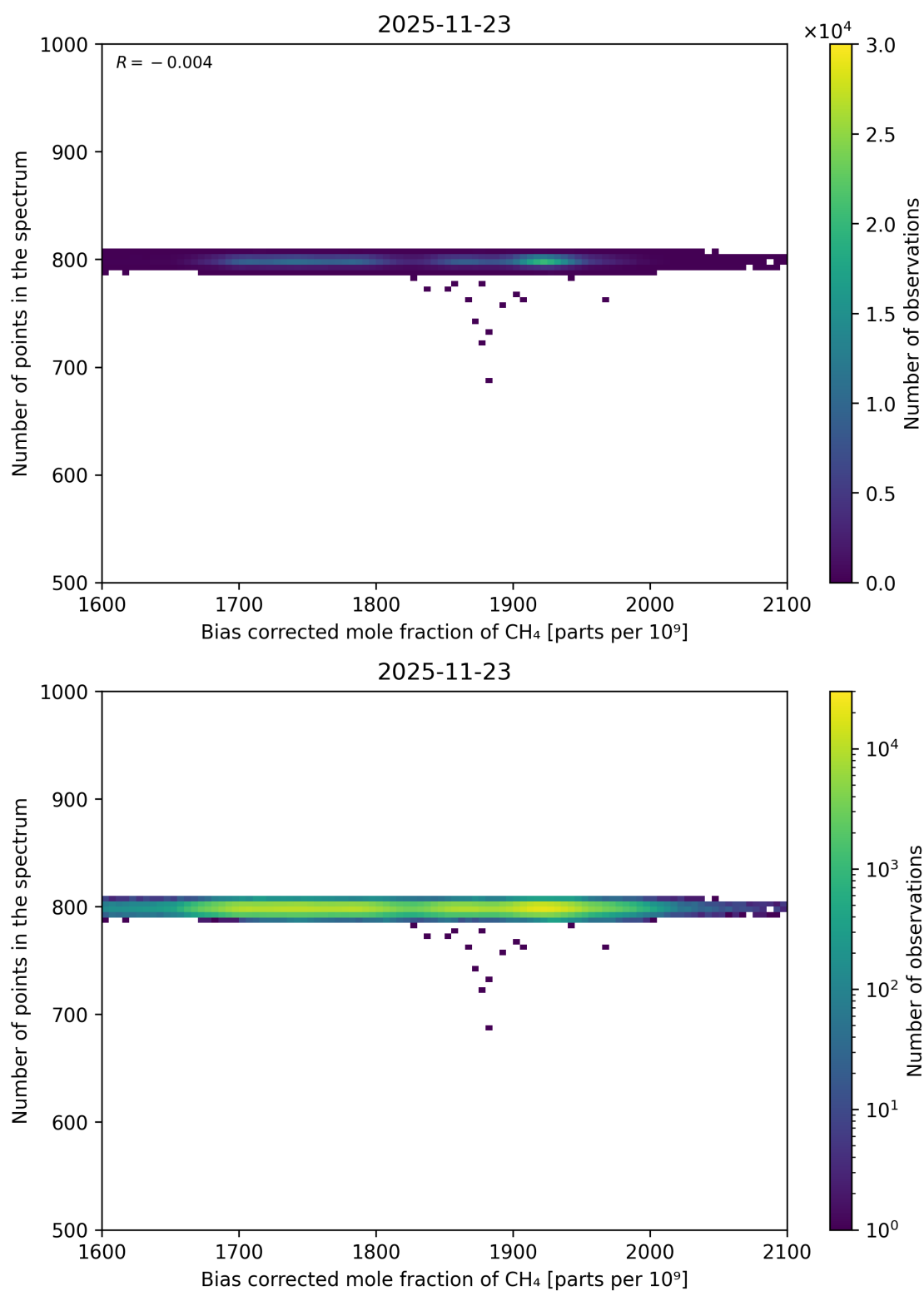
Figure 78: Scatter density plot of “Bias corrected mole fraction of CH 4 ” against “Number of points in the spectrum” for 2025-11-23 to 2025-11-24.
