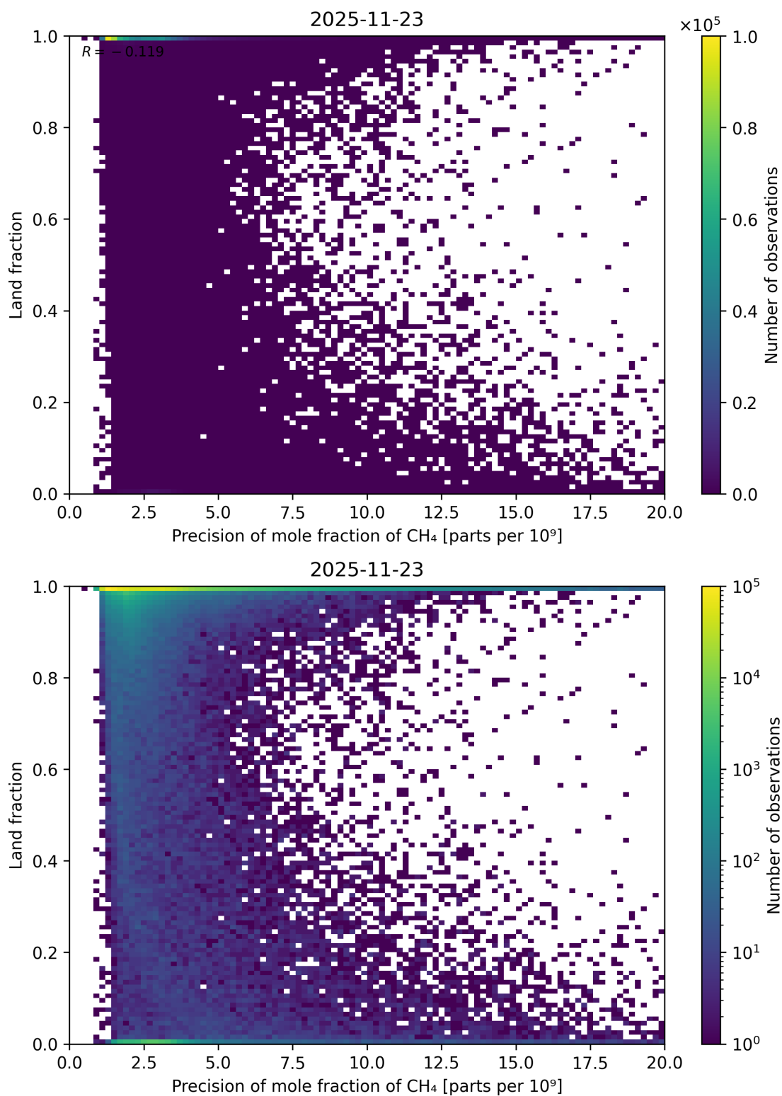
Figure 93: Scatter density plot of “Precision of mole fraction of CH 4 ” against “Land fraction” for 2025-11-23 to 2025-11-24.
