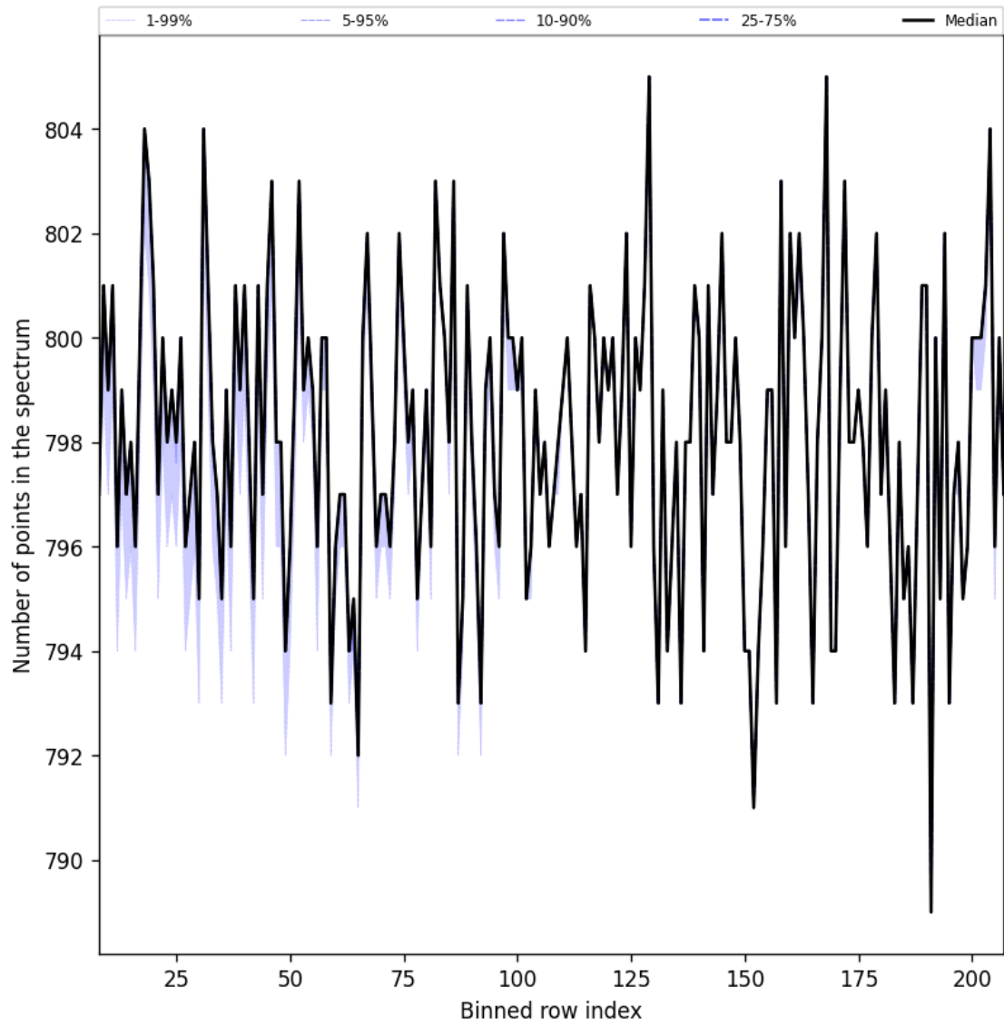
Figure 40: Along track statistics of “Number of points in the spectrum” for 2025-11-23 to 2025-11-24
