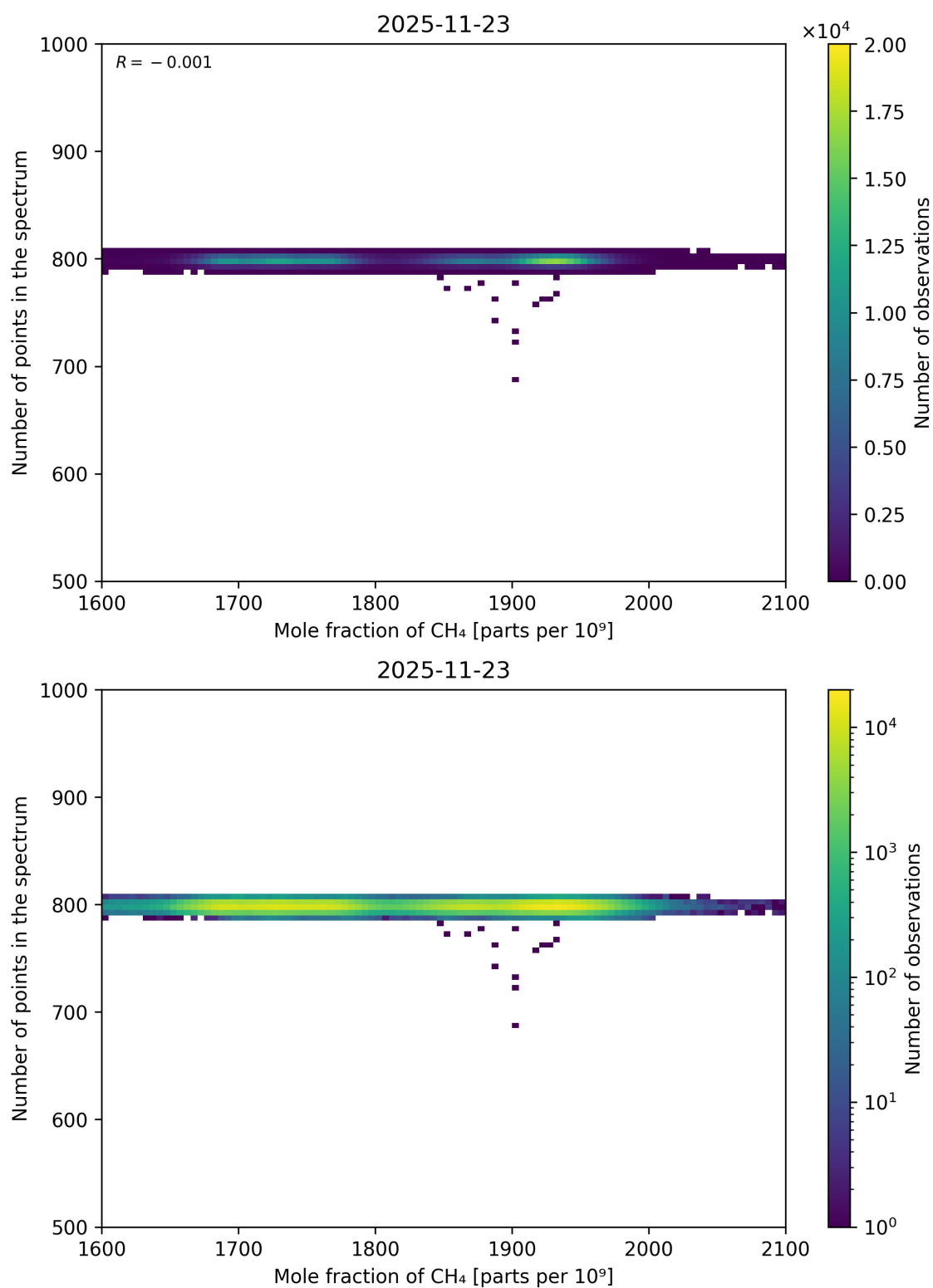
Figure 88: Scatter density plot of “Mole fraction of CH 4 ” against “Number of points in the spectrum” for 2025-11-23 to 2025-11-24.
