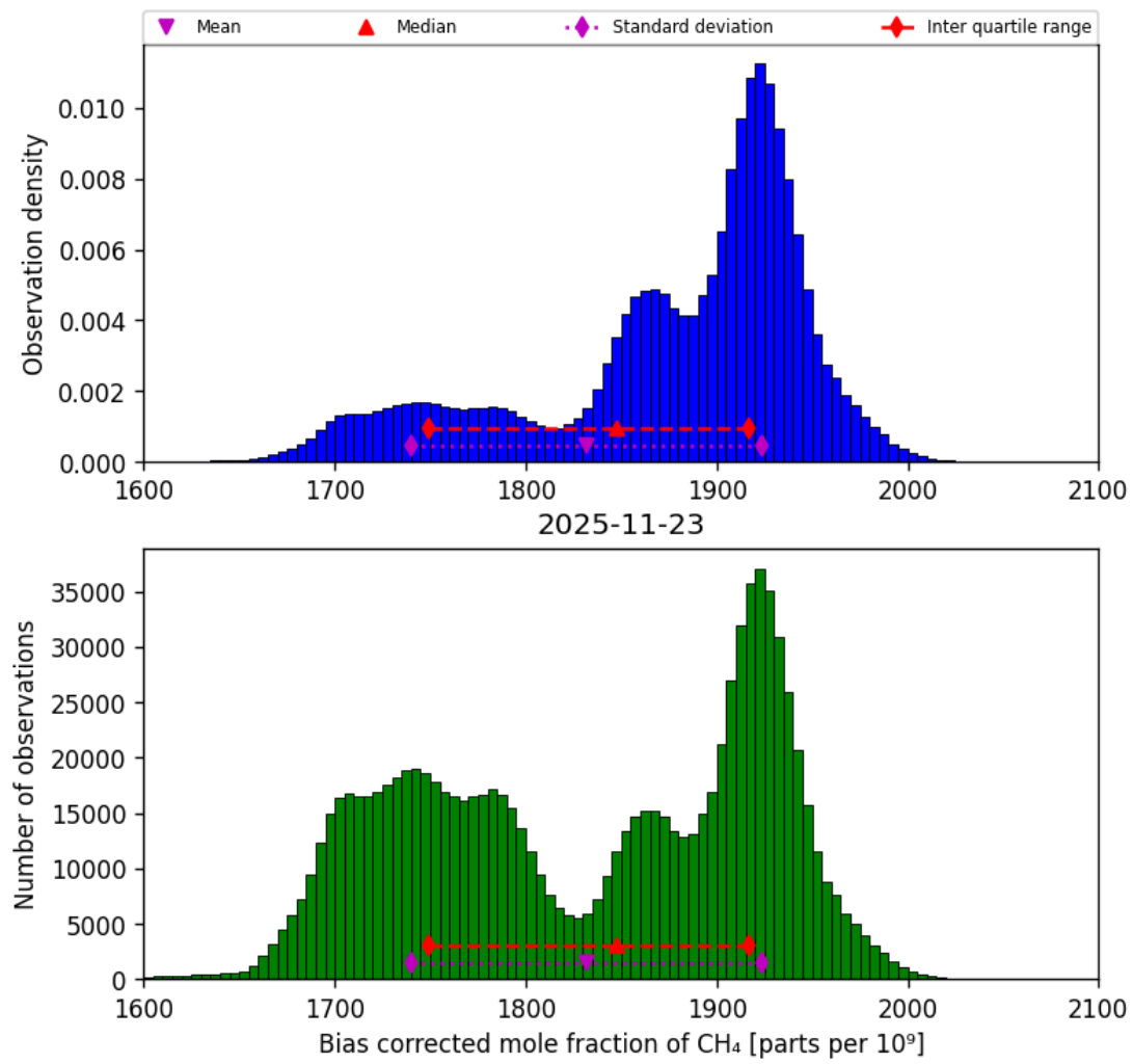
Figure 27: Histogram of “Bias corrected mole fraction of CH 4 ” for 2025-11-23 to 2025-11-24
