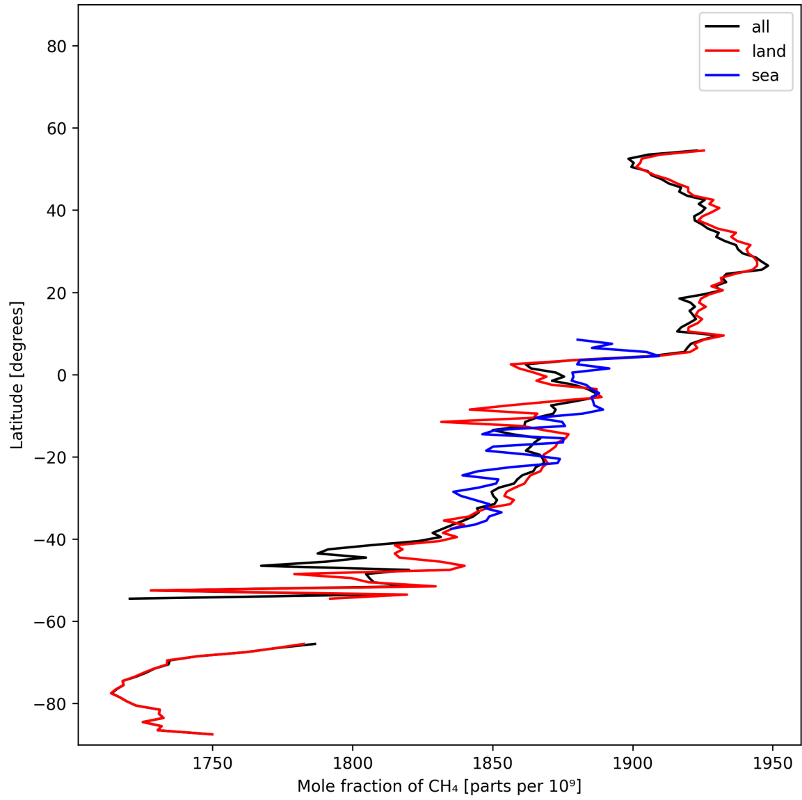
Figure 13: Zonal average of “Mole fraction of CH 4 ” for 2025-11-23 to 2025-11-24.
