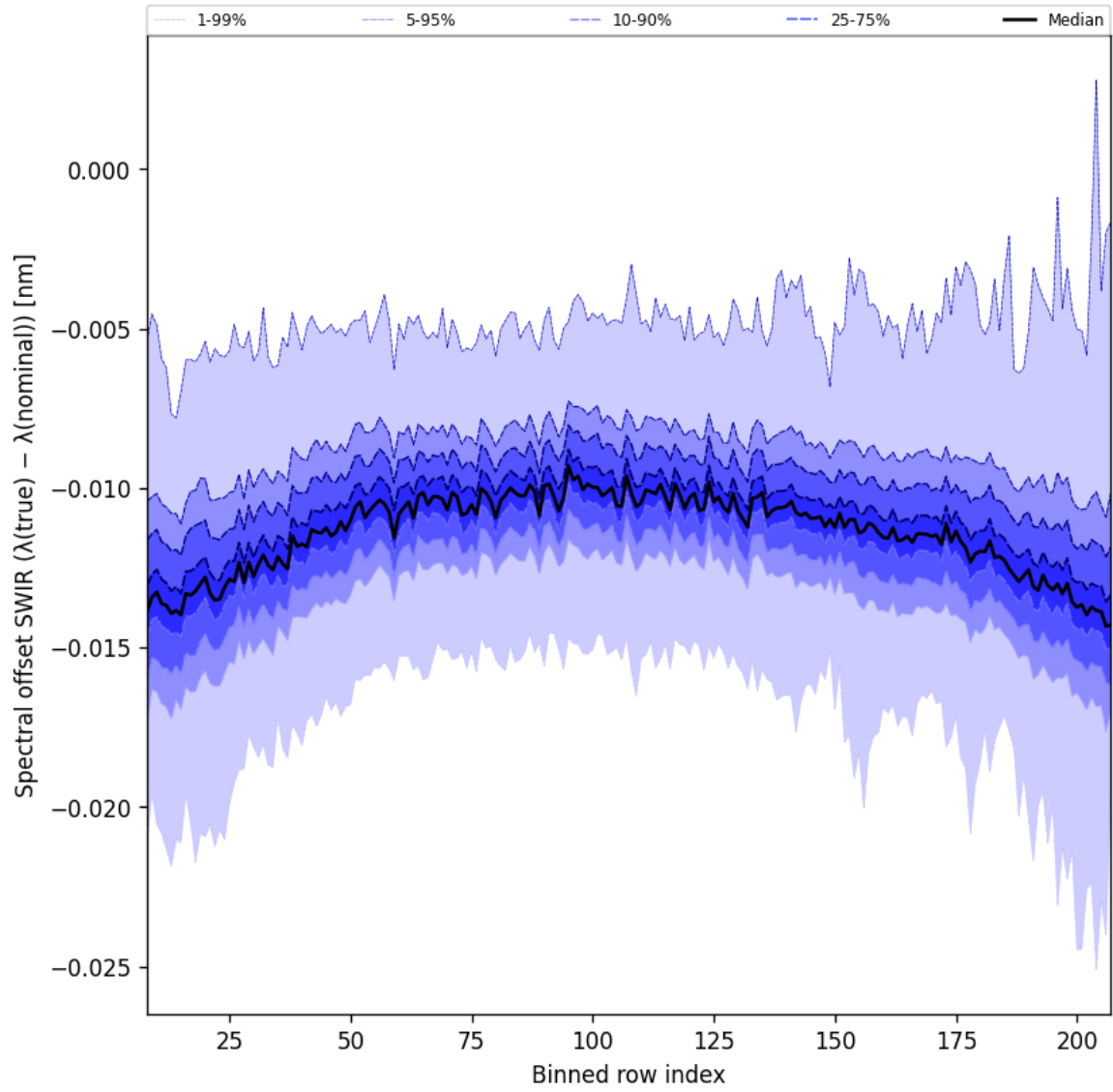
Figure 41: Along track statistics of “Spectral offset SWIR ( \lambda_{\text{true}} - \lambda_{\text{nominal}} )” for 2025-11-23 to 2025-11-24
