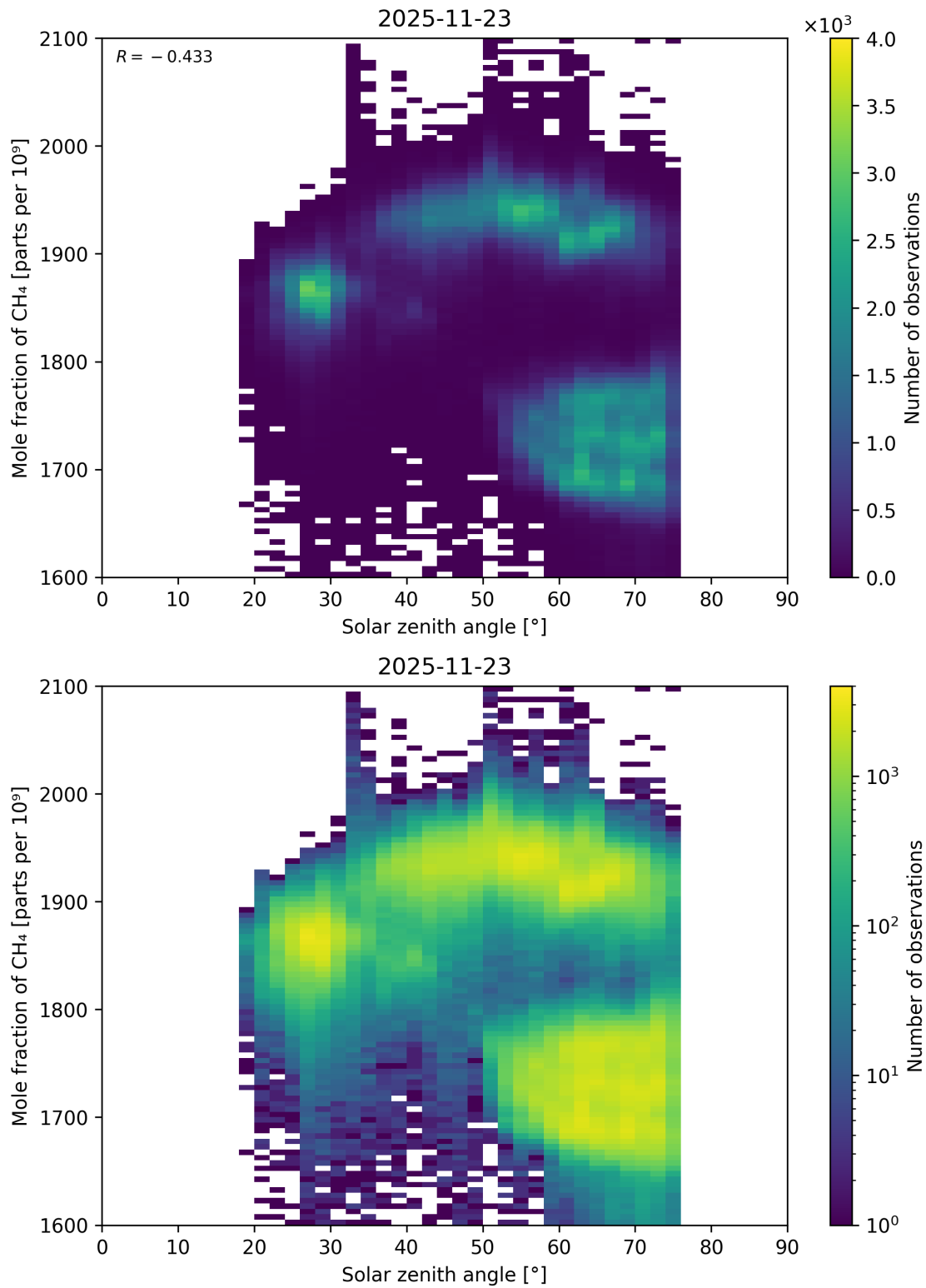
Figure 114: Scatter density plot of “Solar zenith angle” against “Mole fraction of CH 4 ” for 2025-11-23 to 2025-11-24.
