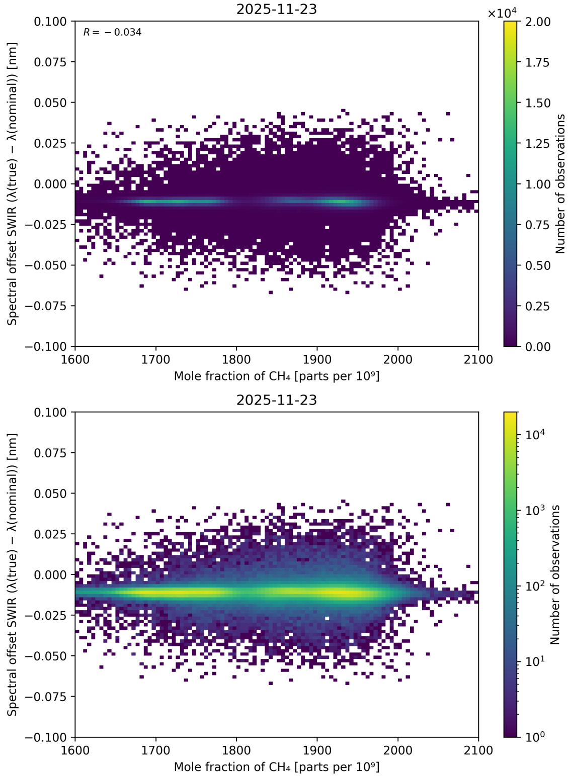
Figure 98: Scatter density plot of “Mole fraction of \text{CH}_4 ” against “Spectral offset SWIR ( \lambda_{\text{true}} - \lambda_{\text{nominal}} )” for 2025-11-23 to 2025-11-24.
