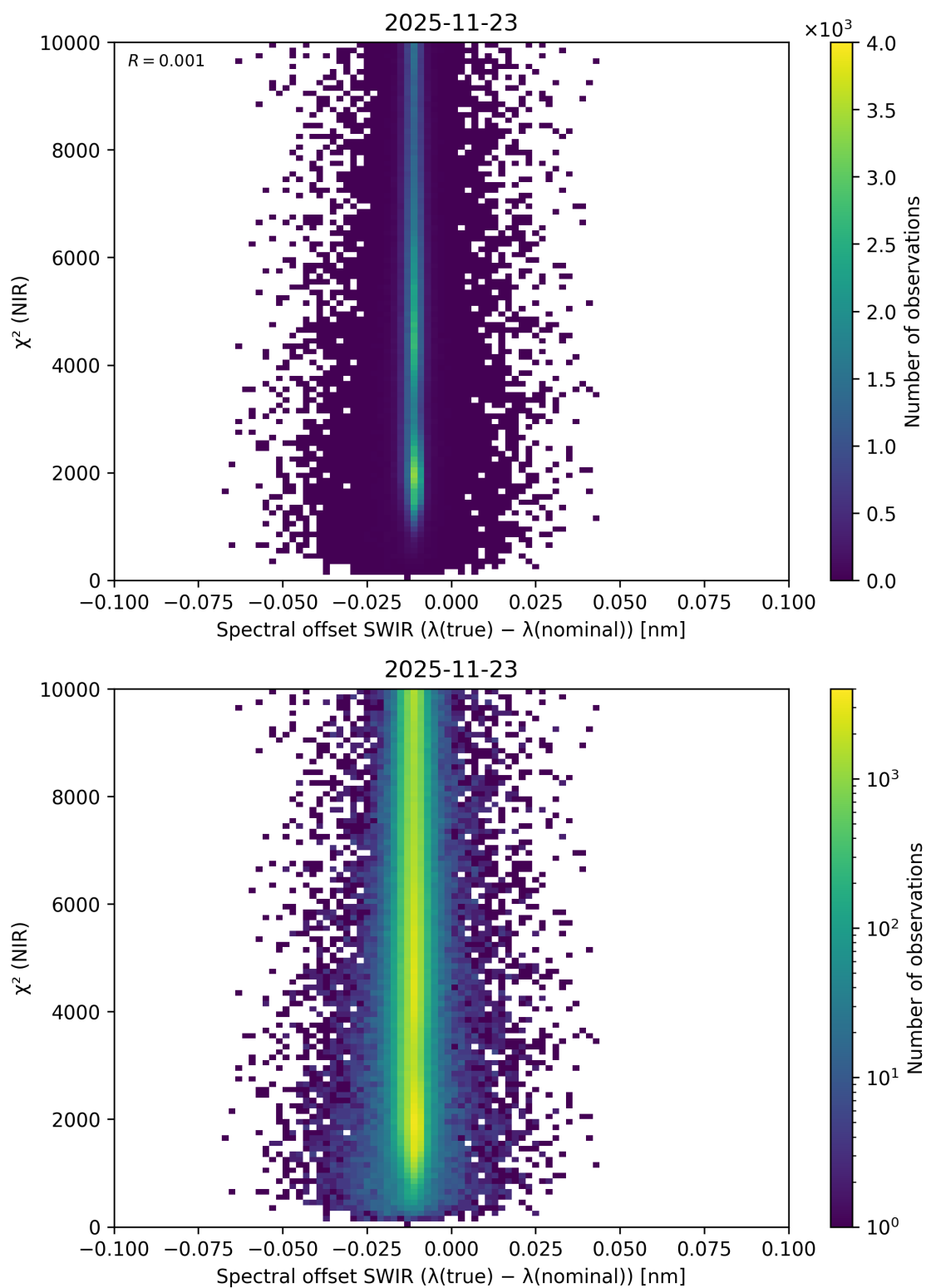
Figure 133: Scatter density plot of “Spectral offset SWIR ( \lambda_{\text{true}} - \lambda_{\text{nominal}} )” against “ \chi^2 (NIR)” for 2025-11-23 to 2025-11-24.
