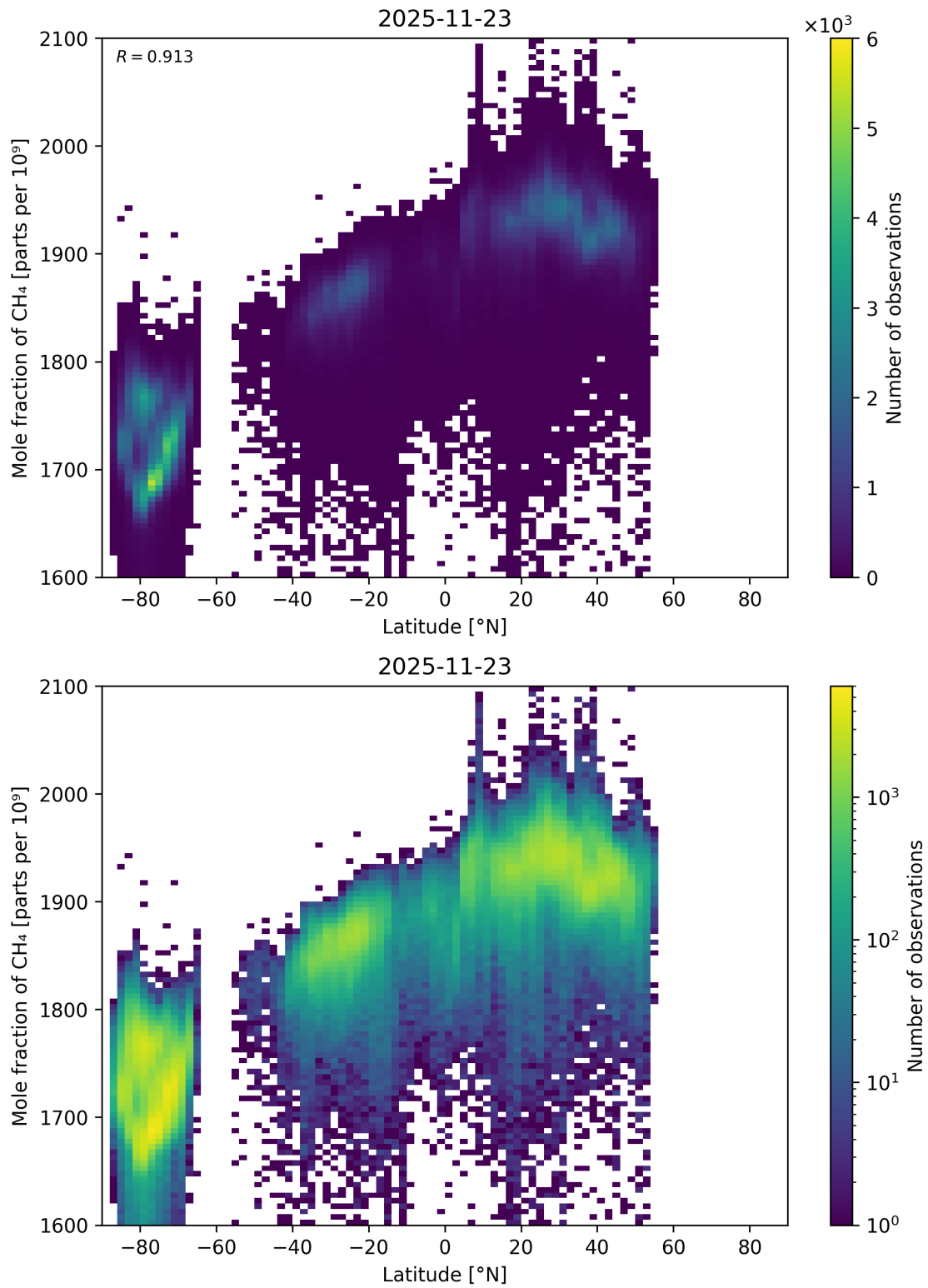
Figure 66: Scatter density plot of “Latitude” against “Mole fraction of CH 4 ” for 2025-11-23 to 2025-11-24.
