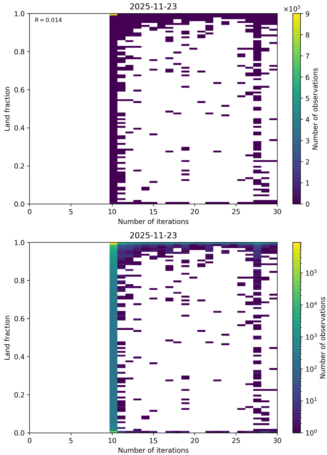
Figure 100: Scatter density plot of “Number of iterations” against “Land fraction” for 2025-11-23 to 2025-11-24.
