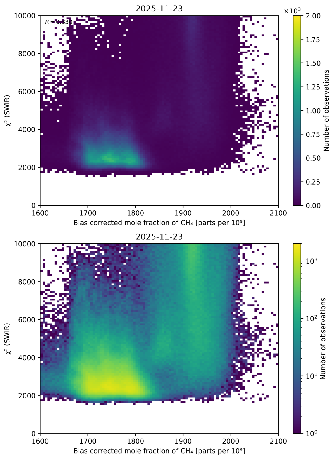
Figure 73: Scatter density plot of “Bias corrected mole fraction of \text{CH}_4 ” against “ \chi^2 (SWIR)” for 2025-11-23 to 2025-11-24.
