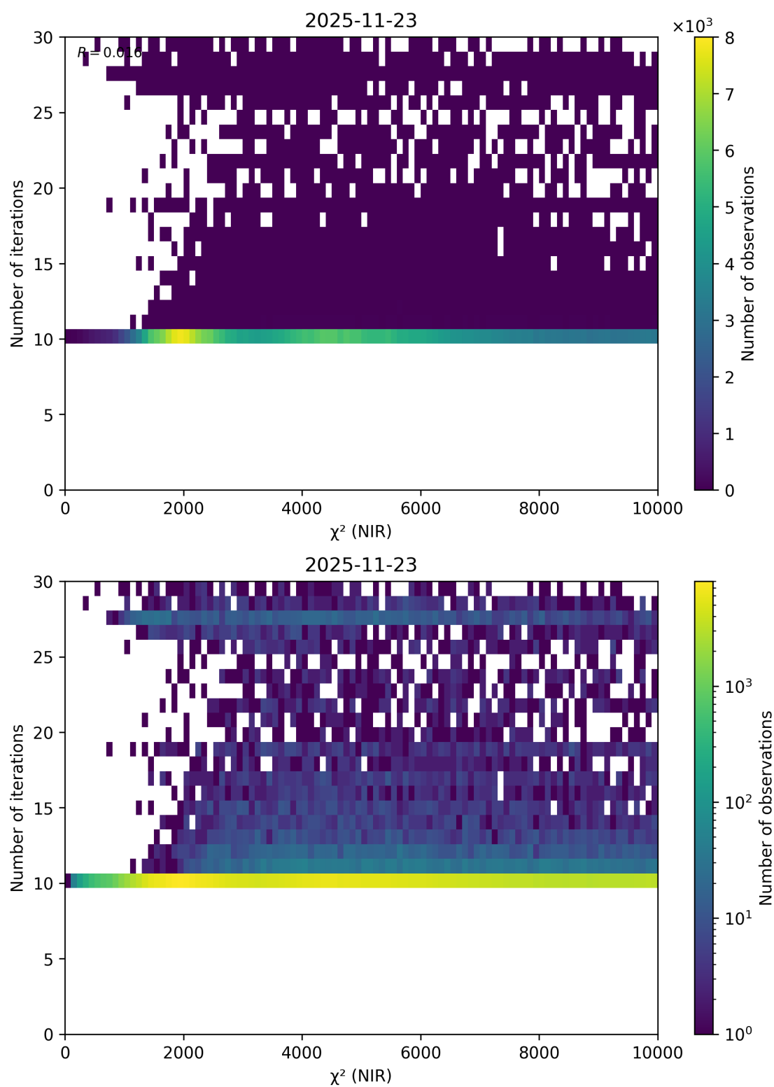
Figure 51: Scatter density plot of “ \chi^2 (NIR)” against “Number of iterations” for 2025-11-23 to 2025-11-24.
