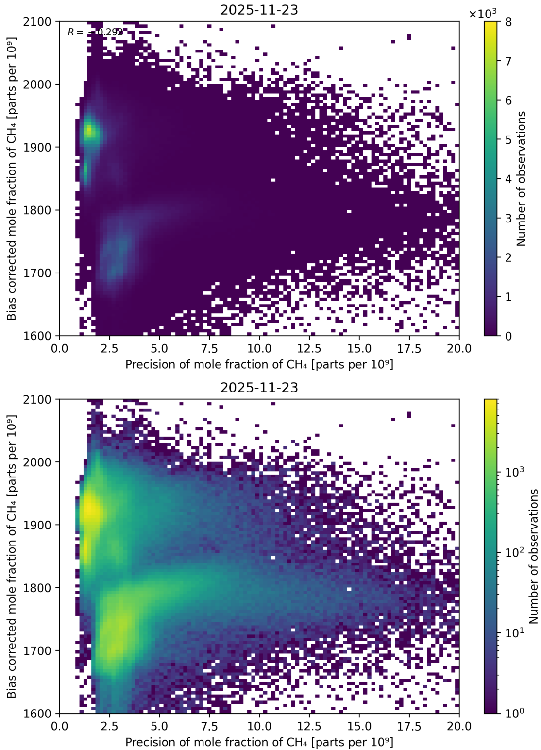
Figure 94: Scatter density plot of “Precision of mole fraction of CH 4 ” against “Bias corrected mole fraction of CH 4 ” for 2025-11-23 to 2025-11-24.
