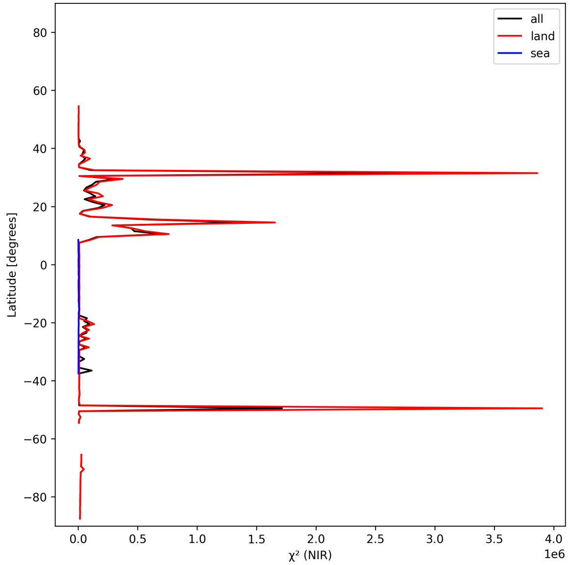
Figure 19: Zonal average of “ \chi^2 (NIR)” for 2025-11-23 to 2025-11-24.
