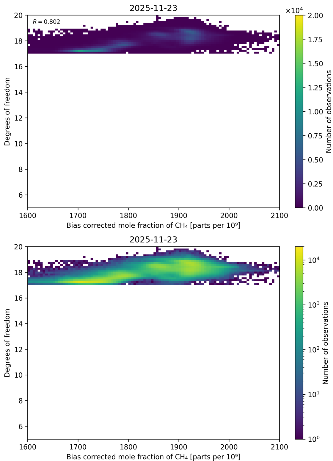
Figure 74: Scatter density plot of “Bias corrected mole fraction of CH 4 ” against “Degrees of freedom” for 2025-11-23 to 2025-11-24.
