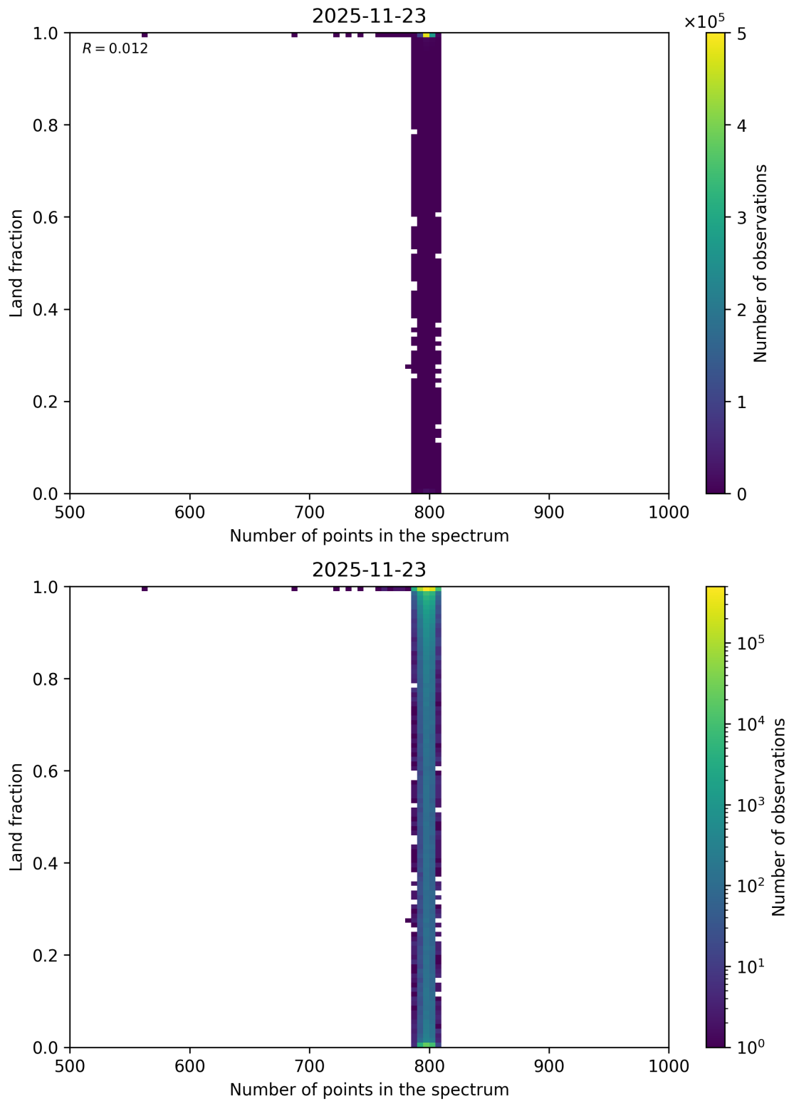
Figure 105: Scatter density plot of “Number of points in the spectrum” against “Land fraction” for 2025-11-23 to 2025-11-24.
