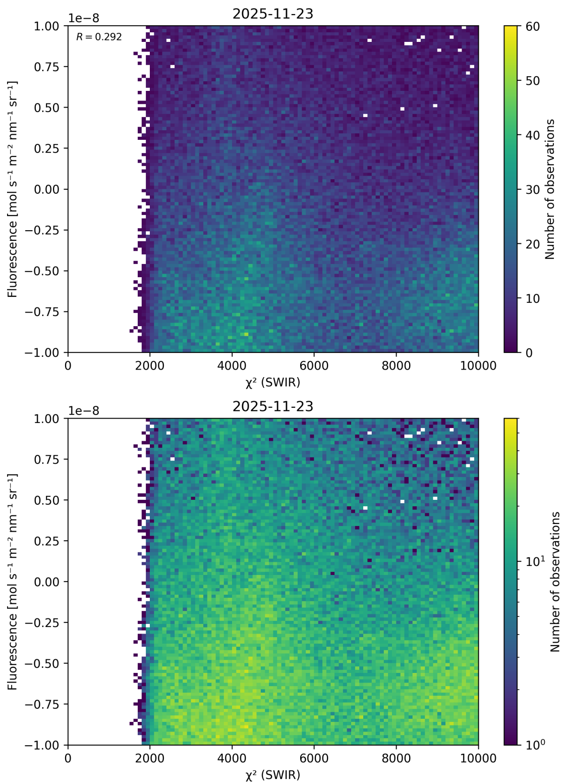
Figure 54: Scatter density plot of “ \chi^2 (SWIR)” against “Fluorescence” for 2025-11-23 to 2025-11-24.
