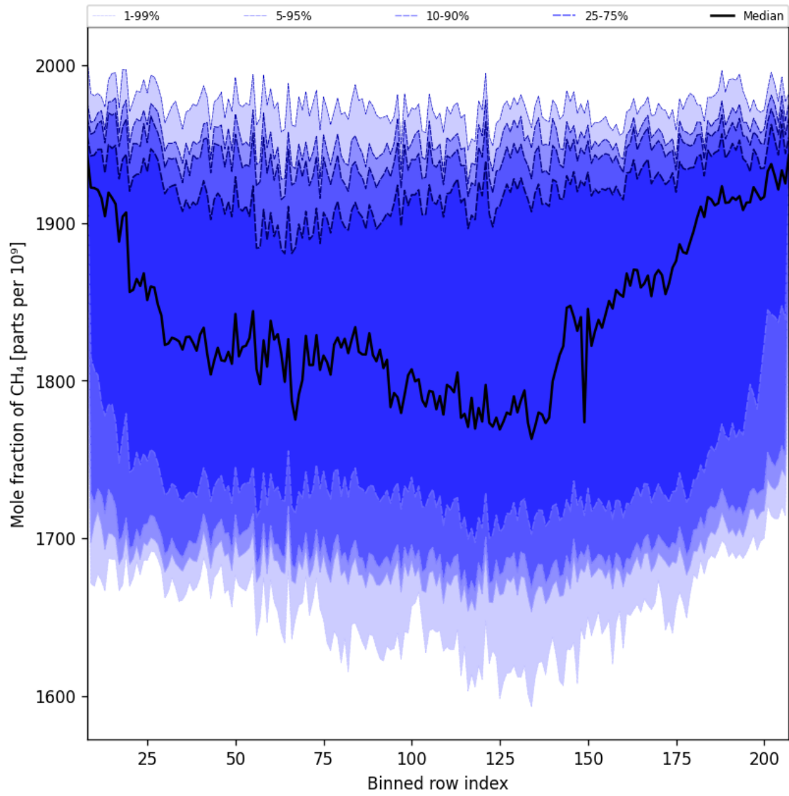
Figure 37: Along track statistics of “Mole fraction of CH 4 ” for 2025-11-23 to 2025-11-24
