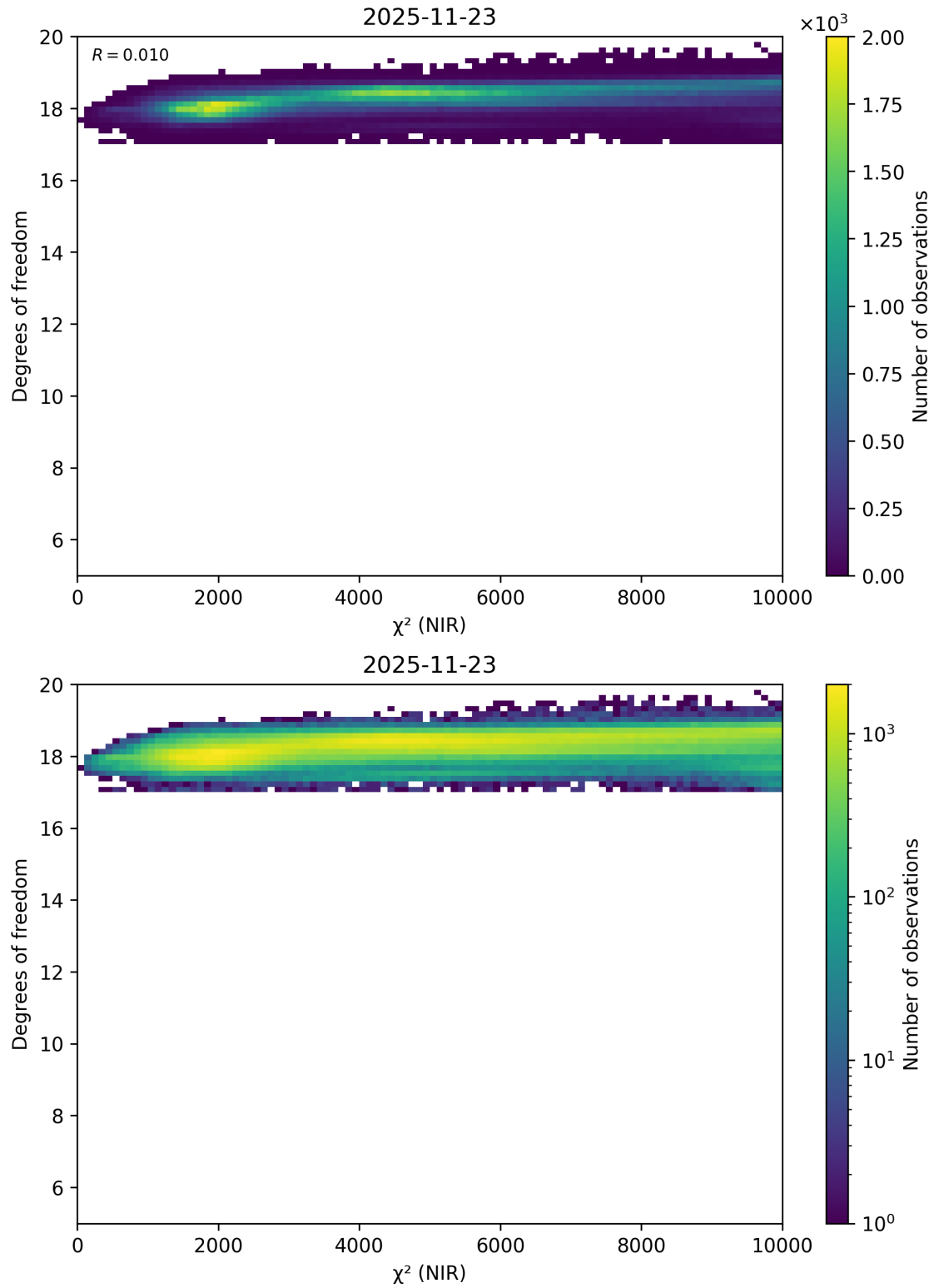
Figure 48: Scatter density plot of “ \chi^2 (NIR)” against “Degrees of freedom” for 2025-11-23 to 2025-11-24.
