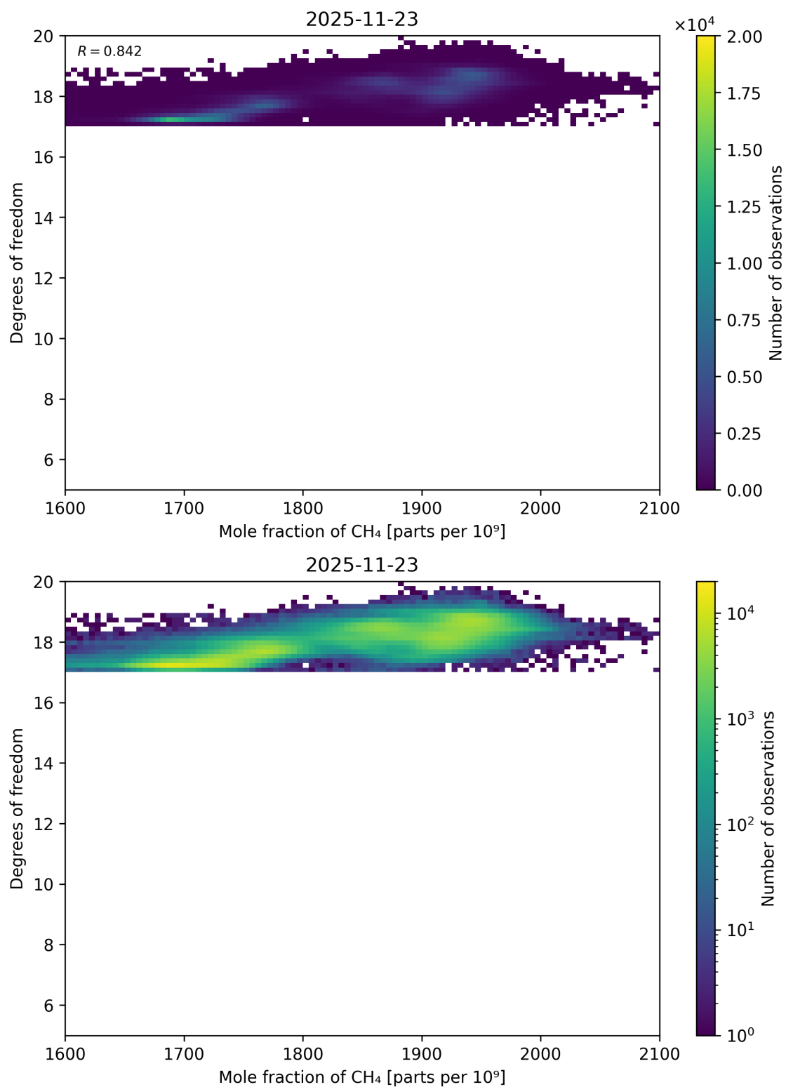
Figure 82: Scatter density plot of “Mole fraction of CH 4 ” against “Degrees of freedom” for 2025-11-23 to 2025-11-24.
