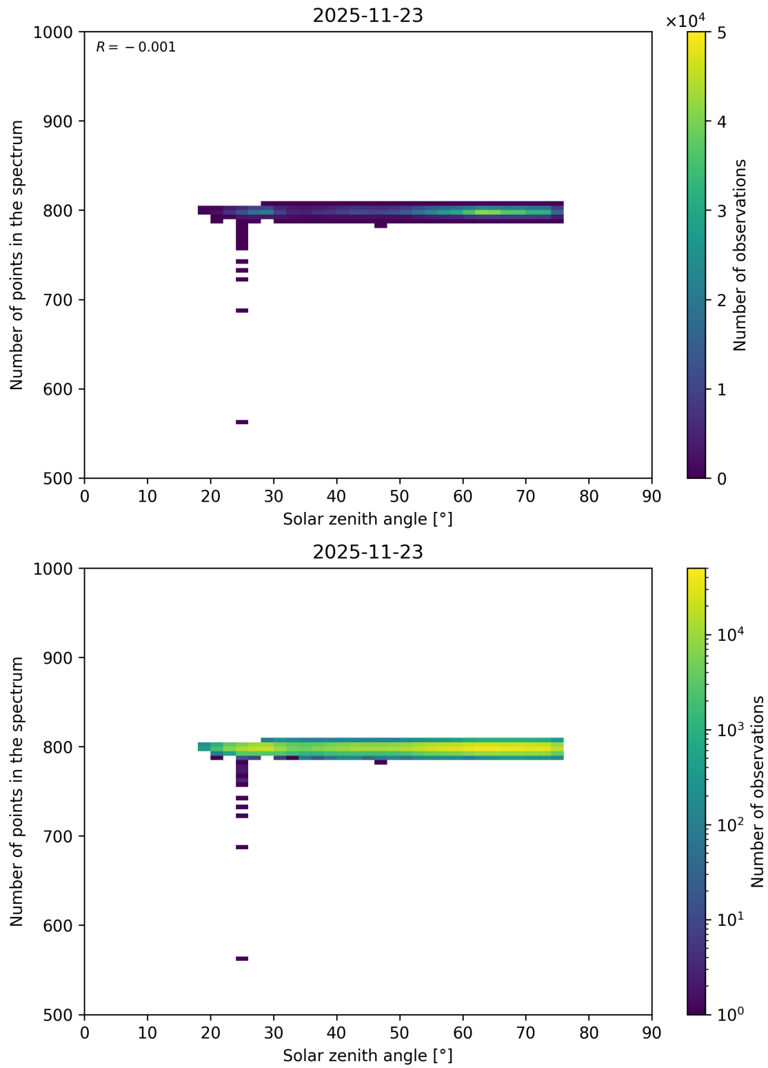
Figure 118: Scatter density plot of “Solar zenith angle” against “Number of points in the spectrum” for 2025-11-23 to 2025-11-24.
