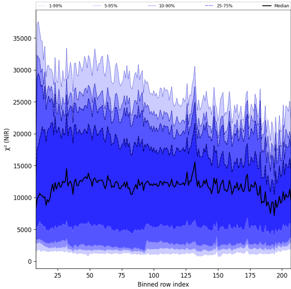
Figure 43: Along track statistics of “ \chi^2 (NIR)” for 2025-11-23 to 2025-11-24
