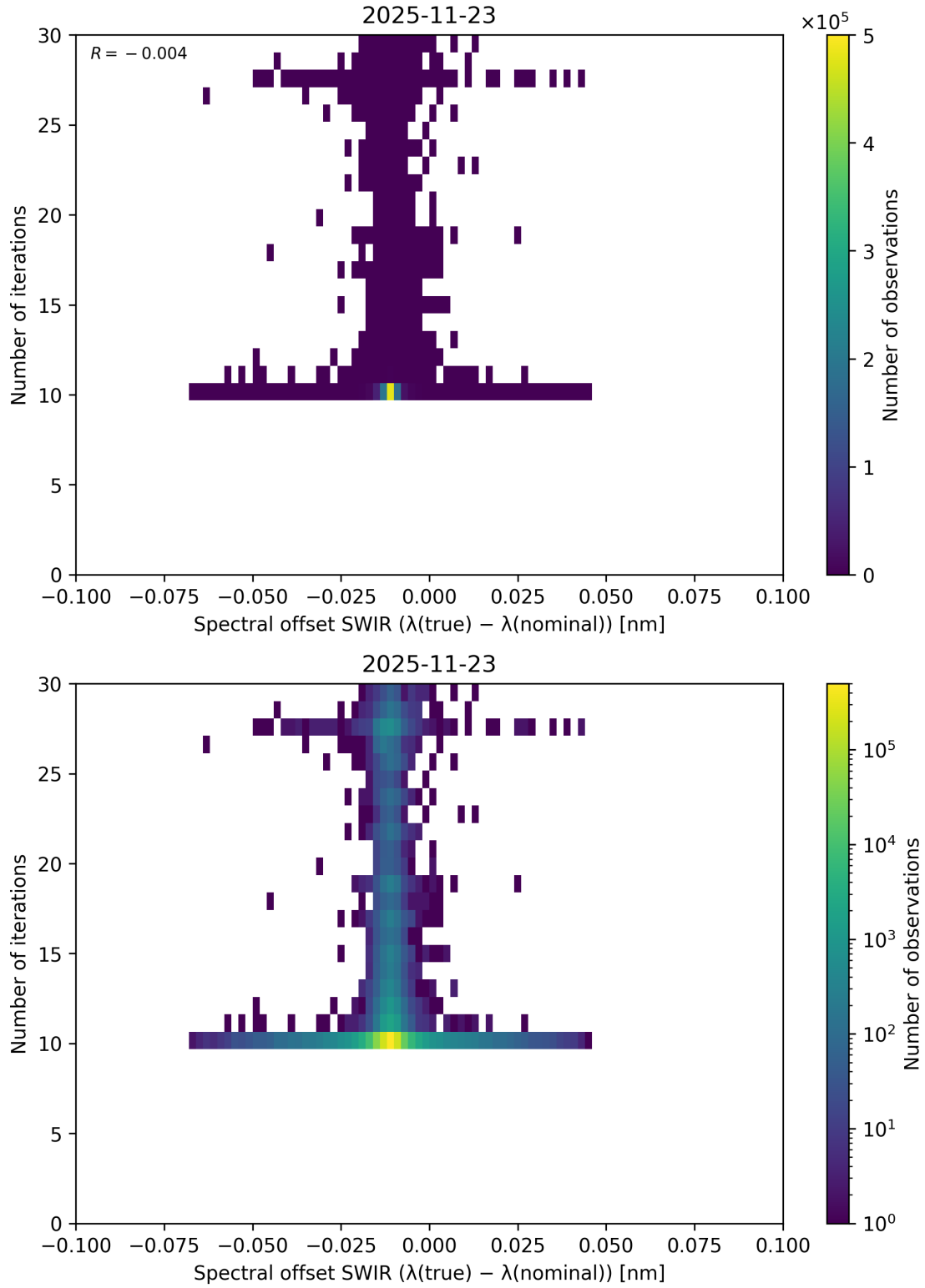
Figure 138: Scatter density plot of “Spectral offset SWIR ( \lambda_{\text{true}} - \lambda_{\text{nominal}} )” against “Number of iterations” for 2025-11-23 to 2025-11-24.
