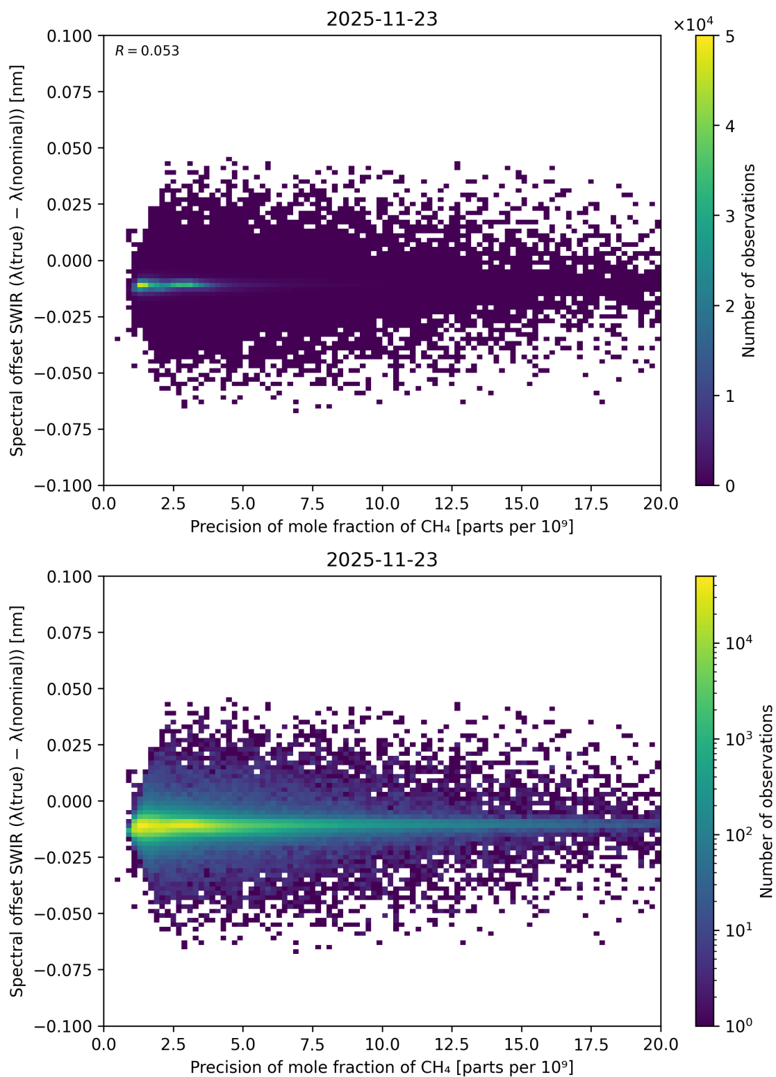
Figure 97: Scatter density plot of “Precision of mole fraction of \text{CH}_4 ” against “Spectral offset SWIR ( \lambda_{\text{true}} - \lambda_{\text{nominal}} )” for 2025-11-23 to 2025-11-24.
