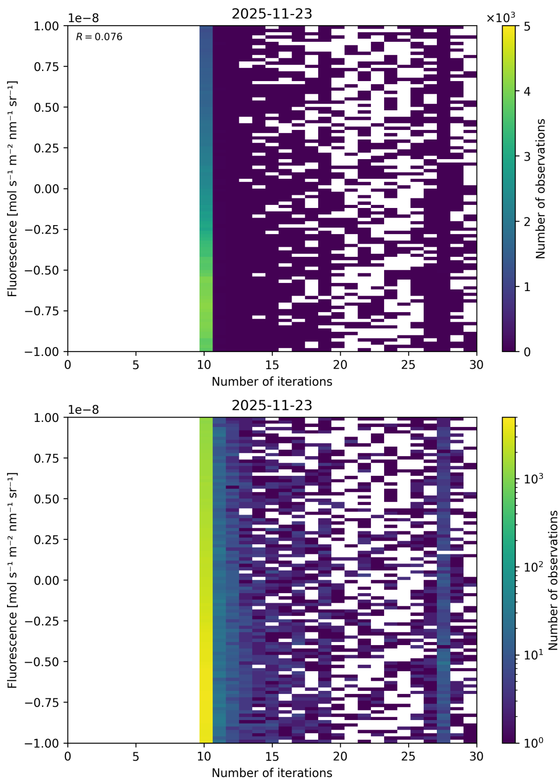
Figure 99: Scatter density plot of “Number of iterations” against “Fluorescence” for 2025-11-23 to 2025-11-24.
