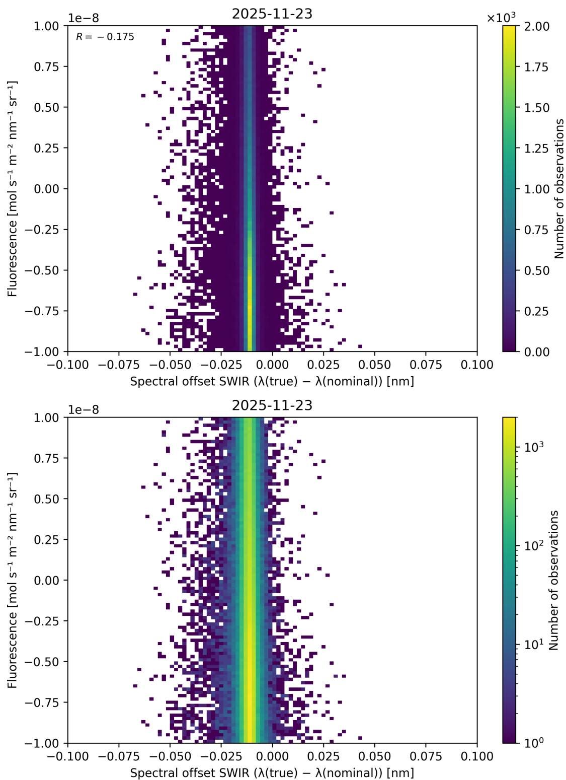
Figure 136: Scatter density plot of “Spectral offset SWIR ( \lambda_{\text{true}} - \lambda_{\text{nominal}} )” against “Fluorescence” for 2025-11-23 to 2025-11-24.
