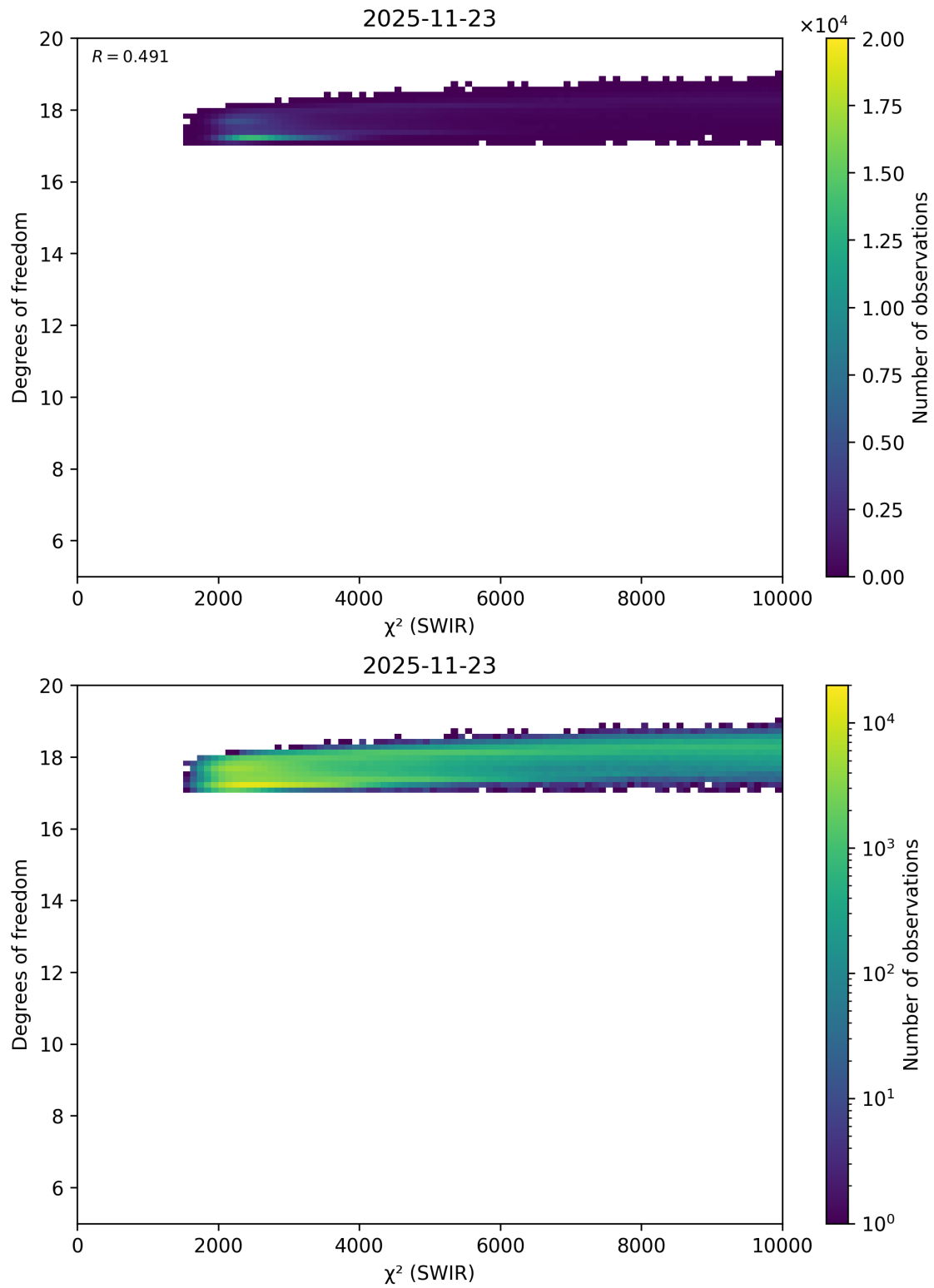
Figure 53: Scatter density plot of “ \chi^2 (SWIR)” against “Degrees of freedom” for 2025-11-23 to 2025-11-24.
