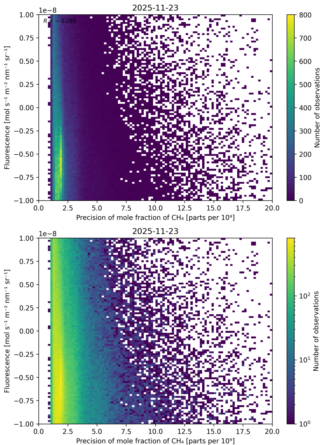
Figure 92: Scatter density plot of “Precision of mole fraction of CH 4 ” against “Fluorescence” for 2025-11-23 to 2025-11-24.
