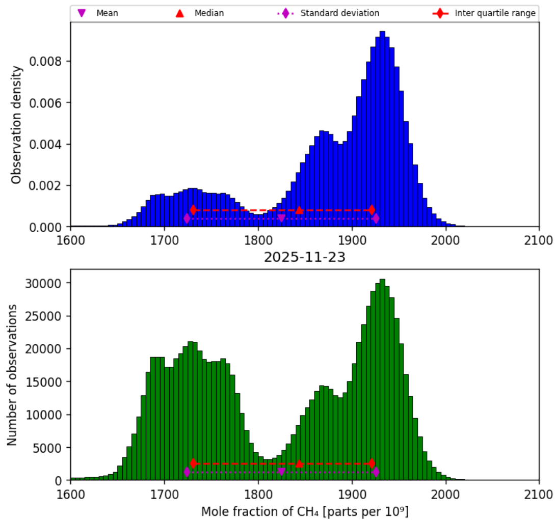
Figure 25: Histogram of “Mole fraction of CH 4 ” for 2025-11-23 to 2025-11-24
