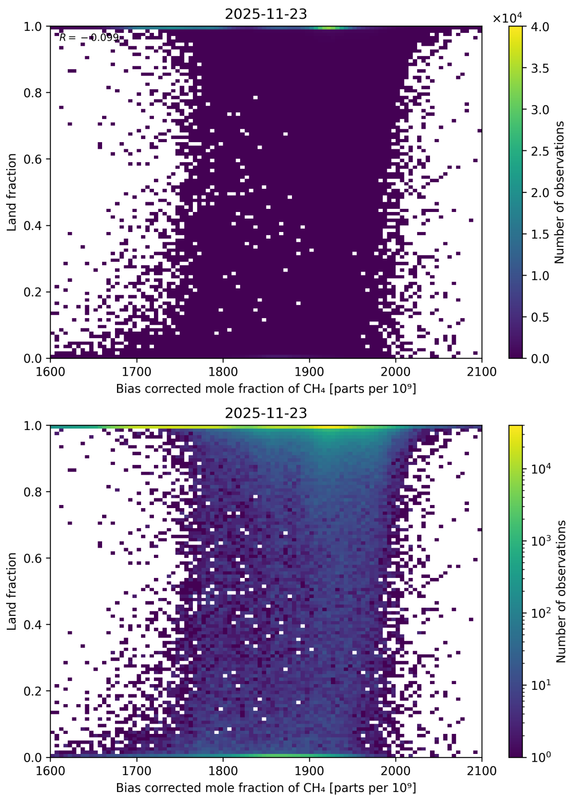
Figure 76: Scatter density plot of “Bias corrected mole fraction of CH 4 ” against “Land fraction” for 2025-11-23 to 2025-11-24.
