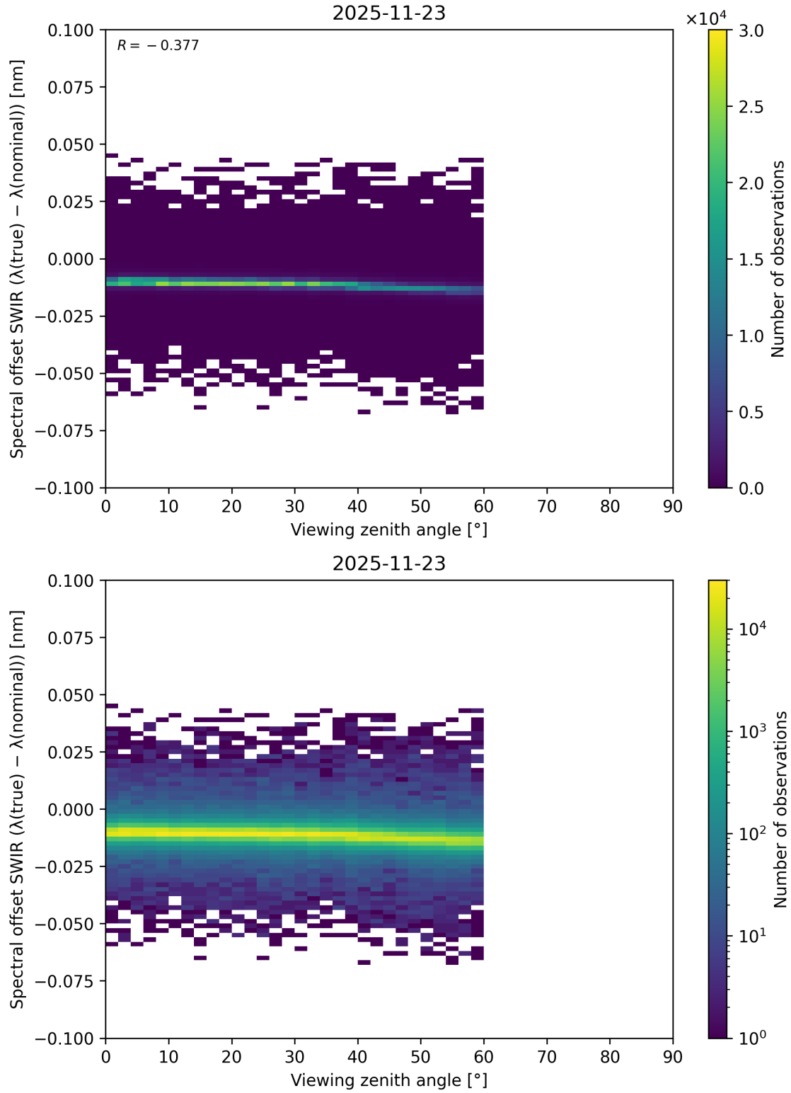
Figure 132: Scatter density plot of “Viewing zenith angle” against “Spectral offset SWIR ( \lambda_{\text{true}} - \lambda_{\text{nominal}} )” for 2025-11-23 to 2025-11-24.
