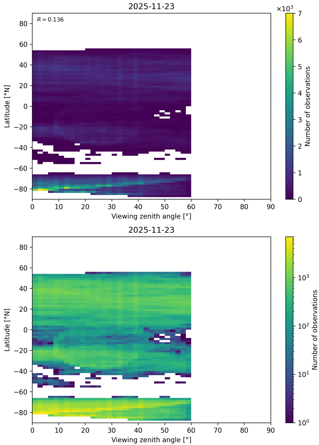
Figure 125: Scatter density plot of “Viewing zenith angle” against “Latitude” for 2025-11-23 to 2025-11-24.
