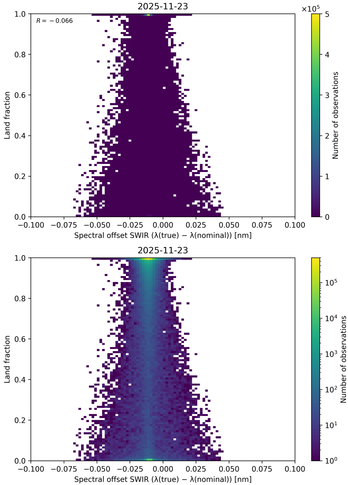
Figure 137: Scatter density plot of “Spectral offset SWIR ( \lambda_{\text{true}} - \lambda_{\text{nominal}} )” against “Land fraction” for 2025-11-23 to 2025-11-24.
