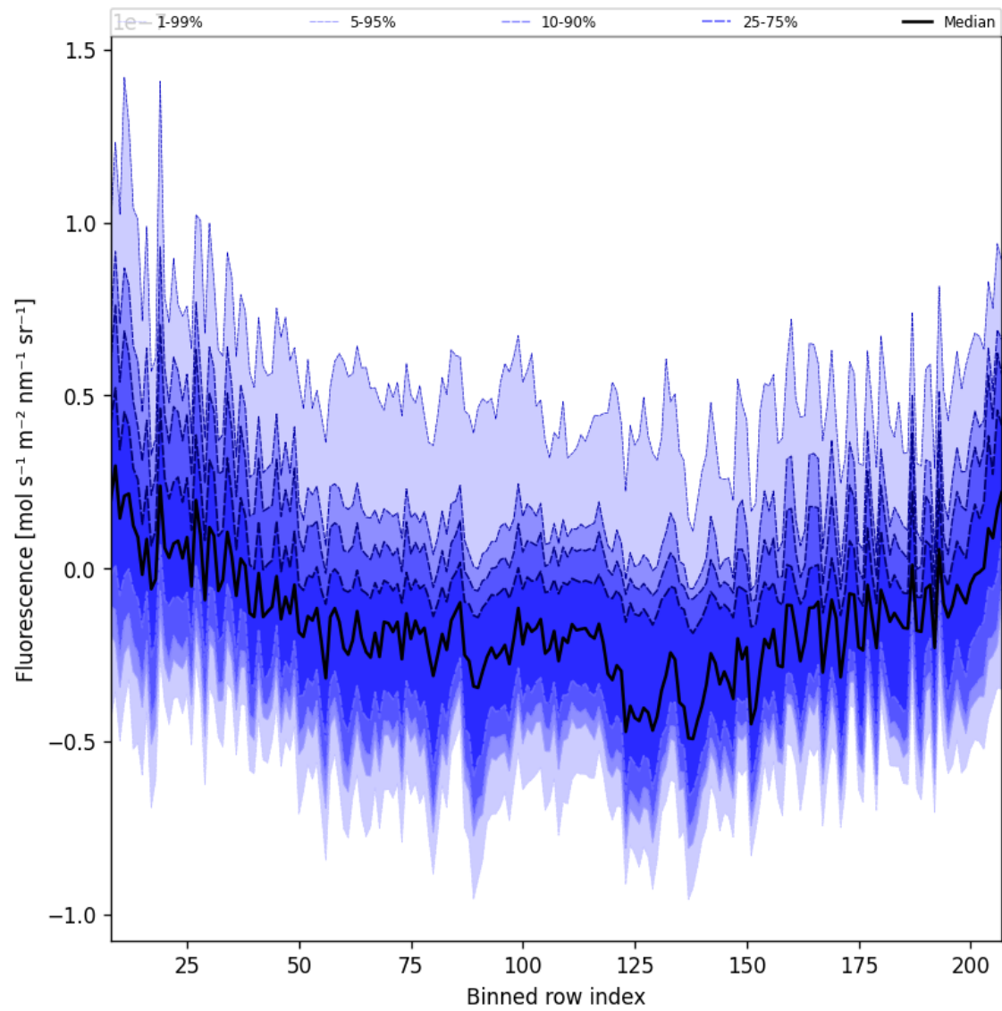
Figure 46: Along track statistics of “Fluorescence” for 2025-11-23 to 2025-11-24
