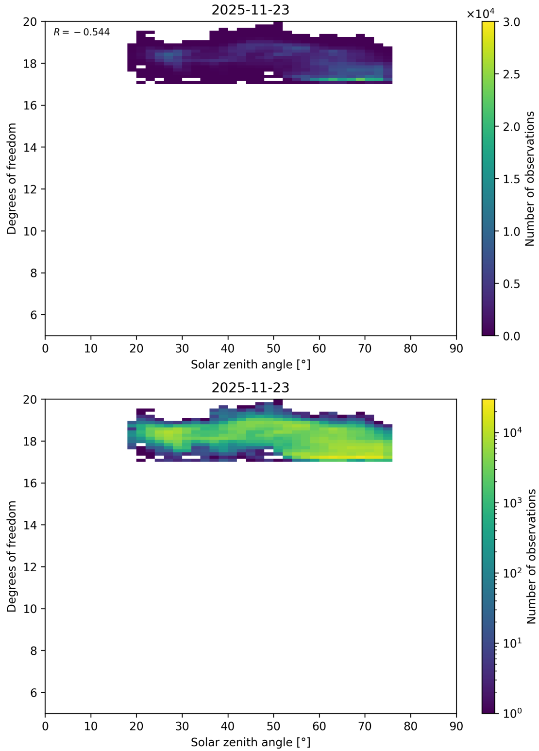
Figure 110: Scatter density plot of “Solar zenith angle” against “Degrees of freedom” for 2025-11-23 to 2025-11-24.
