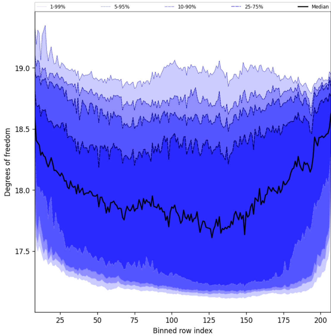
Figure 44: Along track statistics of “Degrees of freedom” for 2025-11-23 to 2025-11-24
