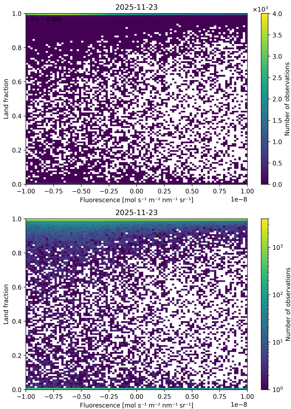
Figure 60: Scatter density plot of “Fluorescence” against “Land fraction” for 2025-11-23 to 2025-11-24.
