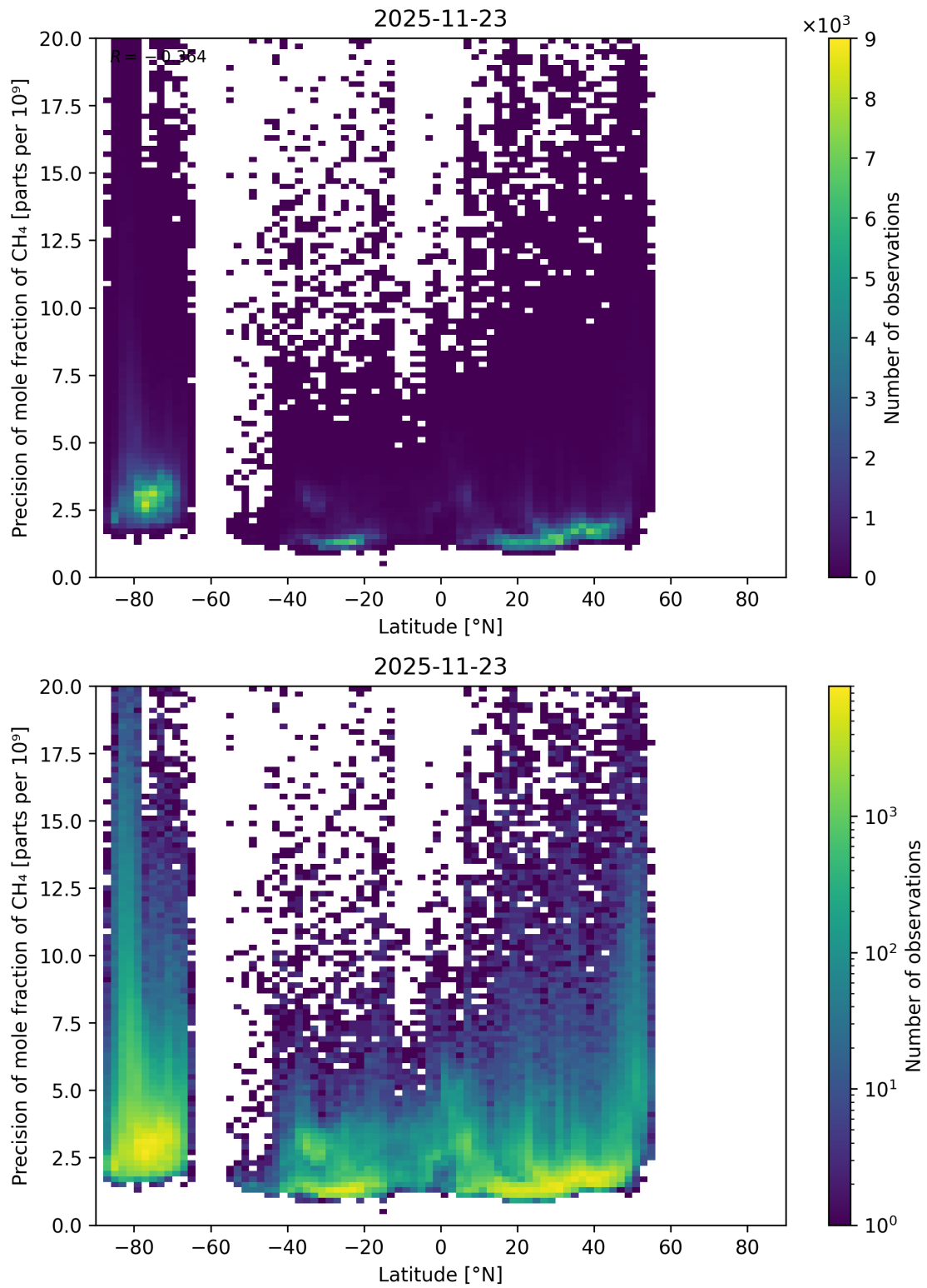
Figure 68: Scatter density plot of “Latitude” against “Precision of mole fraction of CH 4 ” for 2025-11-23 to 2025-11-24.
