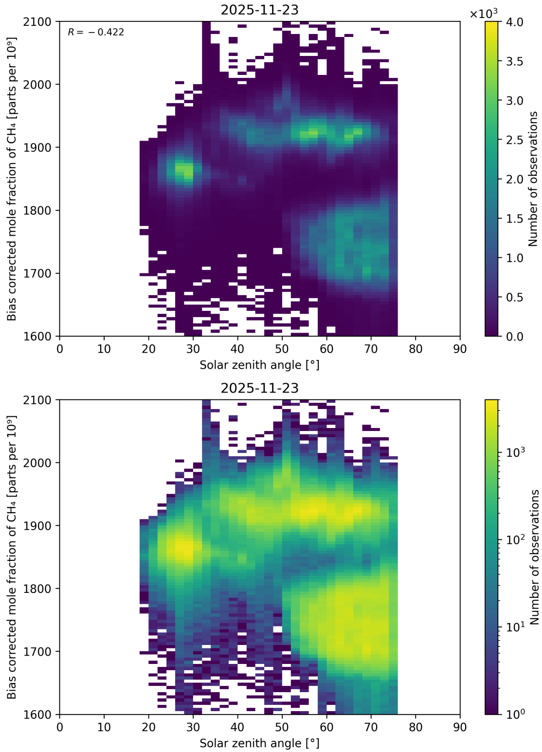
Figure 115: Scatter density plot of “Solar zenith angle” against “Bias corrected mole fraction of CH 4 ” for 2025-11-23 to 2025-11-24.
