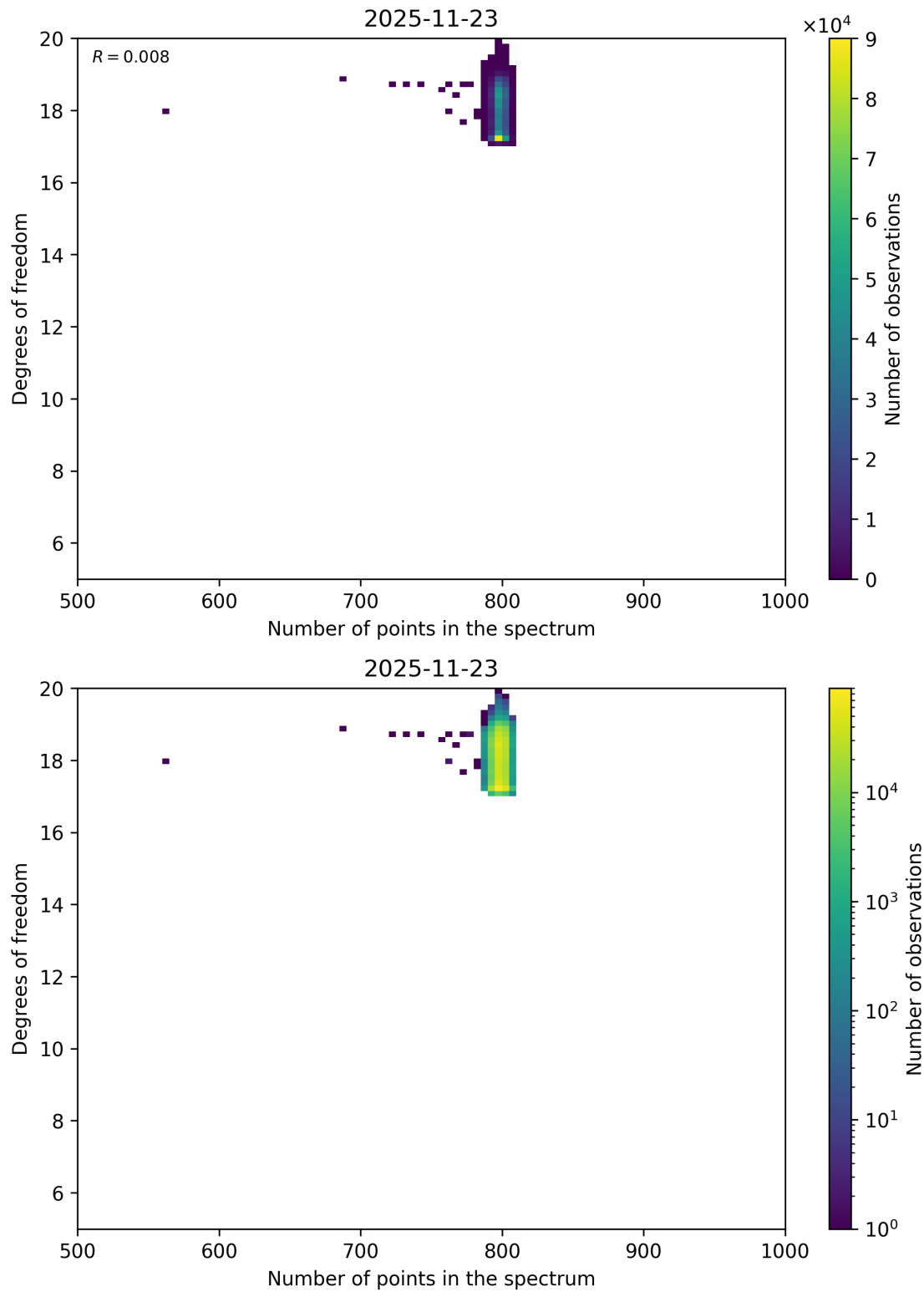
Figure 103: Scatter density plot of “Number of points in the spectrum” against “Degrees of freedom” for 2025-11-23 to 2025-11-24.
