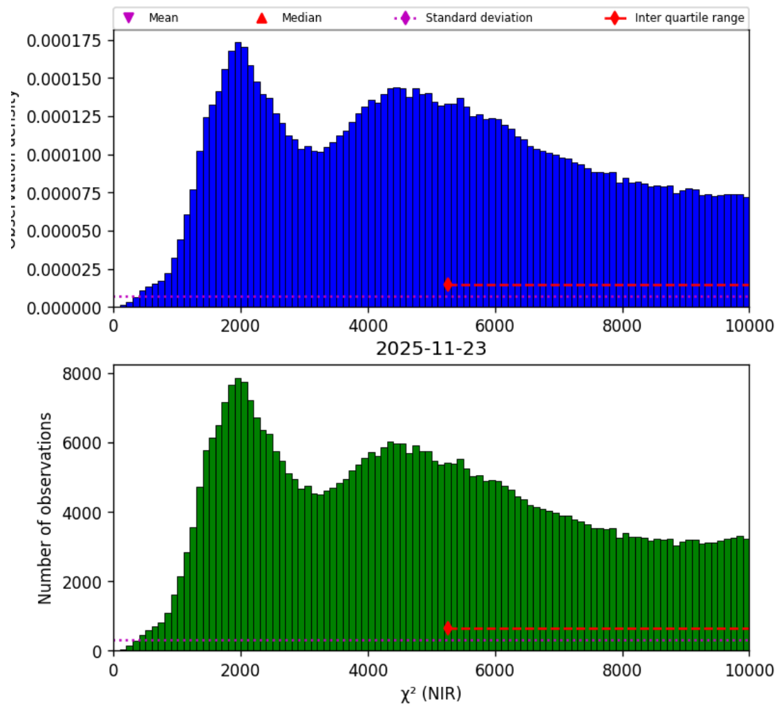
Figure 31: Histogram of “ \chi^2 (NIR)” for 2025-11-23 to 2025-11-24
