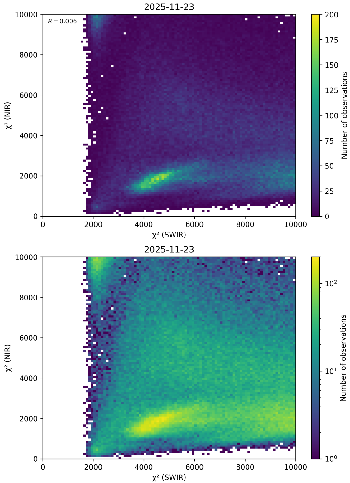
Figure 52: Scatter density plot of “ \chi^2 (SWIR)” against “ \chi^2 (NIR)” for 2025-11-23 to 2025-11-24.
