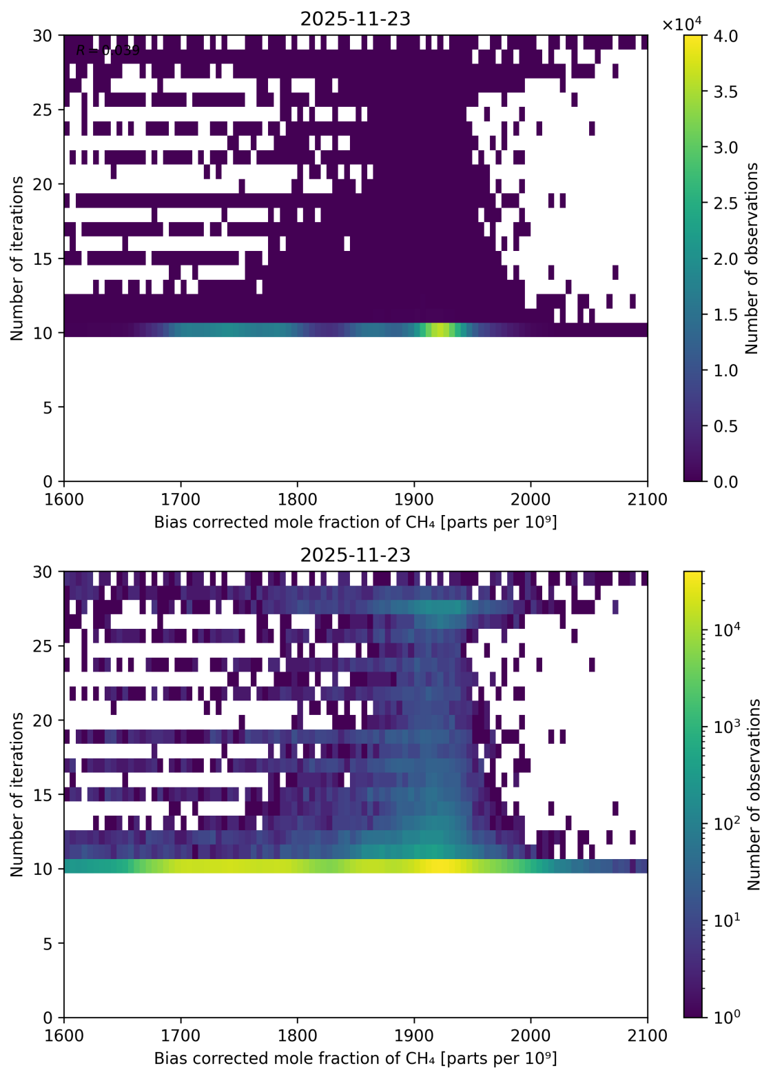
Figure 77: Scatter density plot of “Bias corrected mole fraction of CH 4 ” against “Number of iterations” for 2025-11-23 to 2025-11-24.
