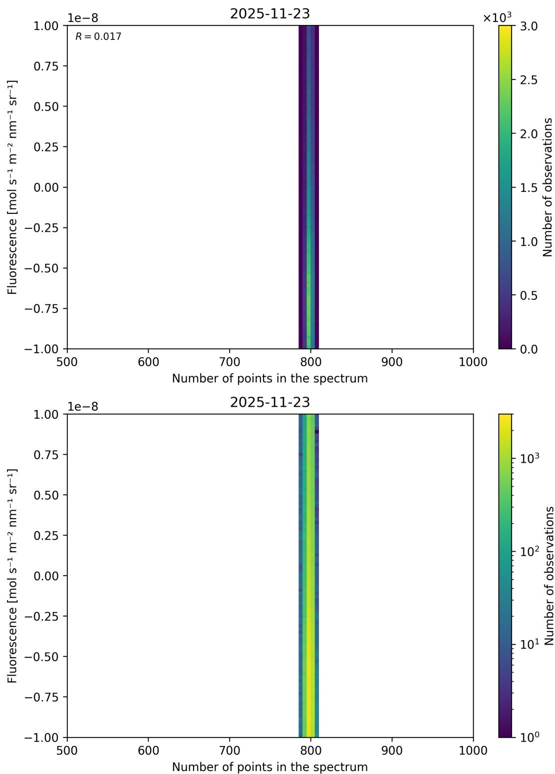
Figure 104: Scatter density plot of “Number of points in the spectrum” against “Fluorescence” for 2025-11-23 to 2025-11-24.
