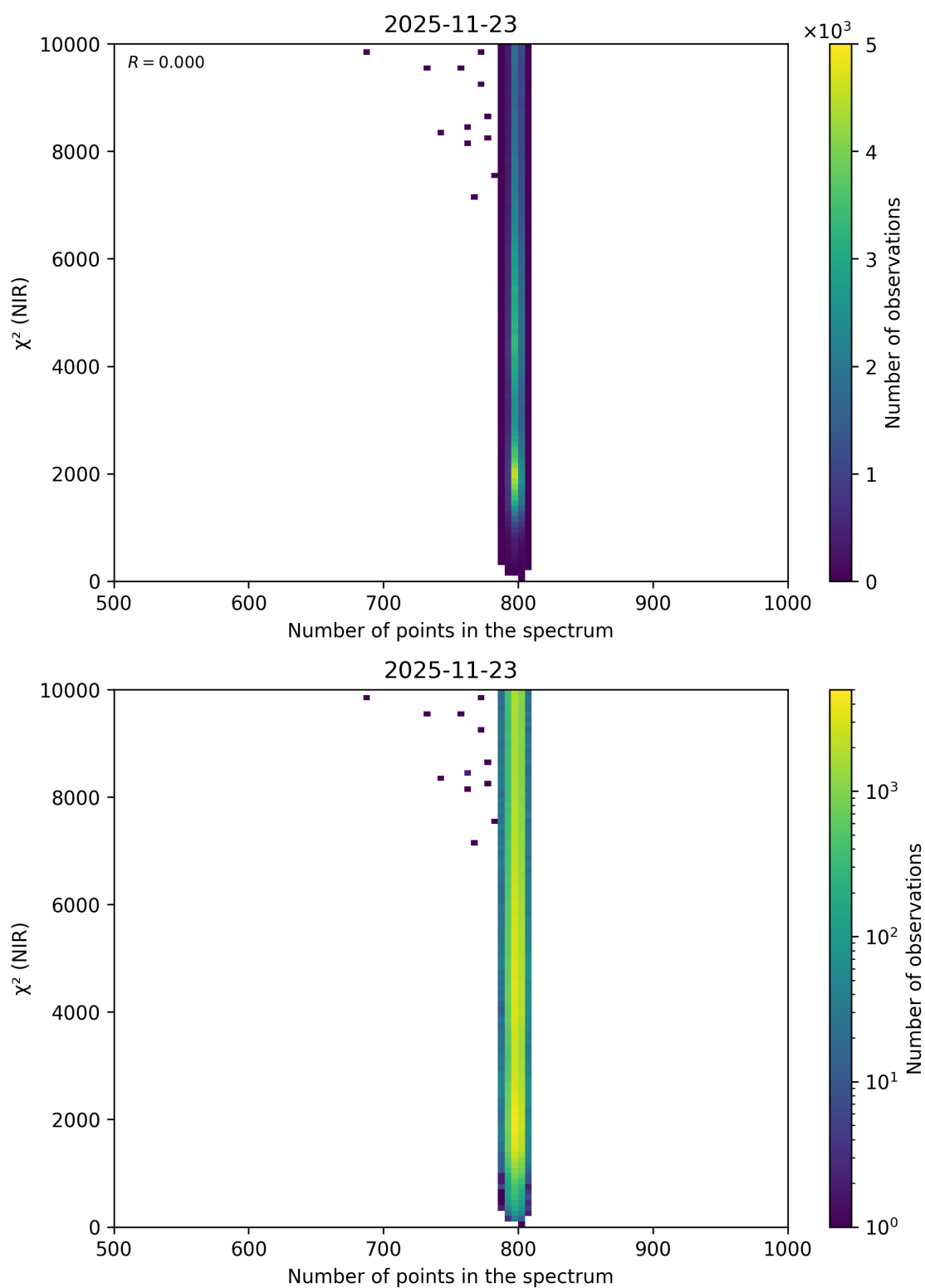
Figure 101: Scatter density plot of “Number of points in the spectrum” against “ \chi^2 (NIR)” for 2025-11-23 to 2025-11-24.
