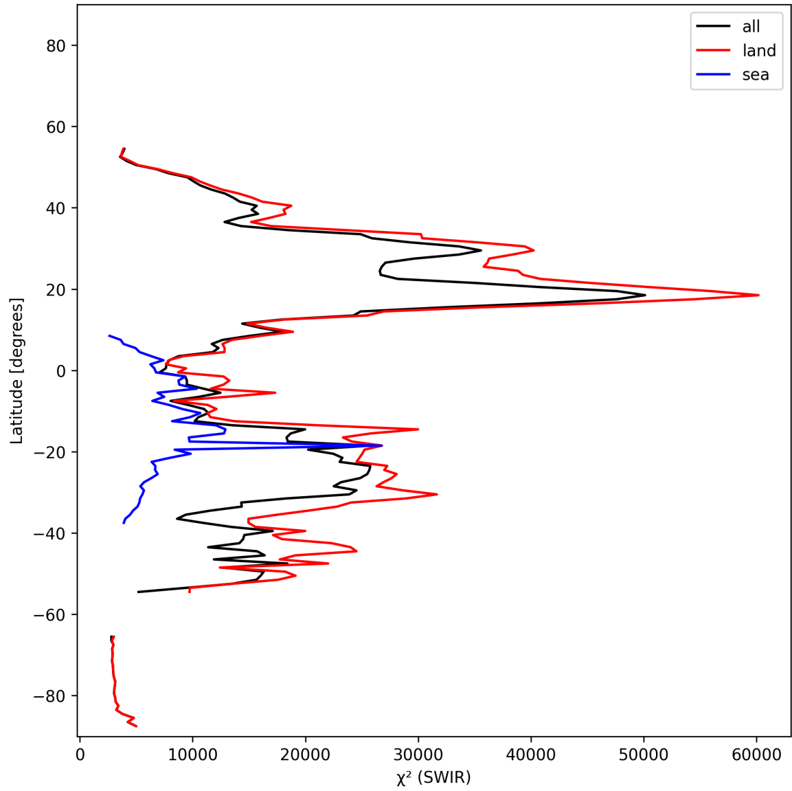
Figure 18: Zonal average of “ \chi^2 (SWIR)” for 2025-11-23 to 2025-11-24.
