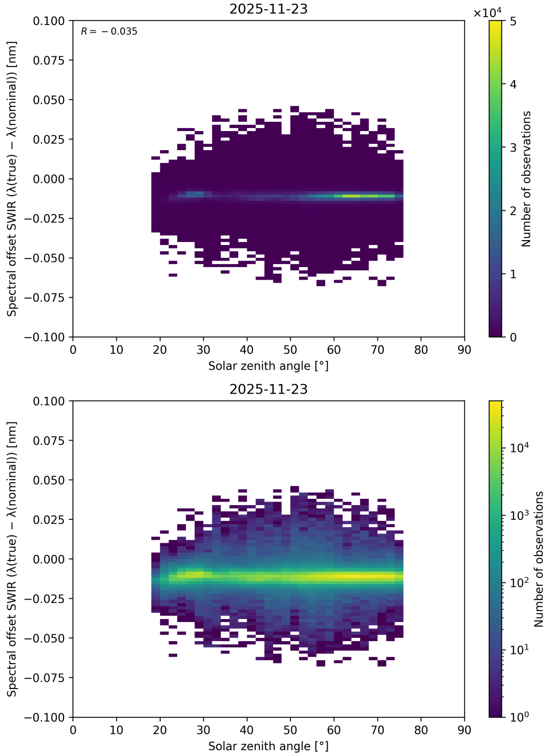
Figure 119: Scatter density plot of “Solar zenith angle” against “Spectral offset SWIR ( \lambda_{\text{true}} - \lambda_{\text{nominal}} )” for 2025-11-23 to 2025-11-24.
