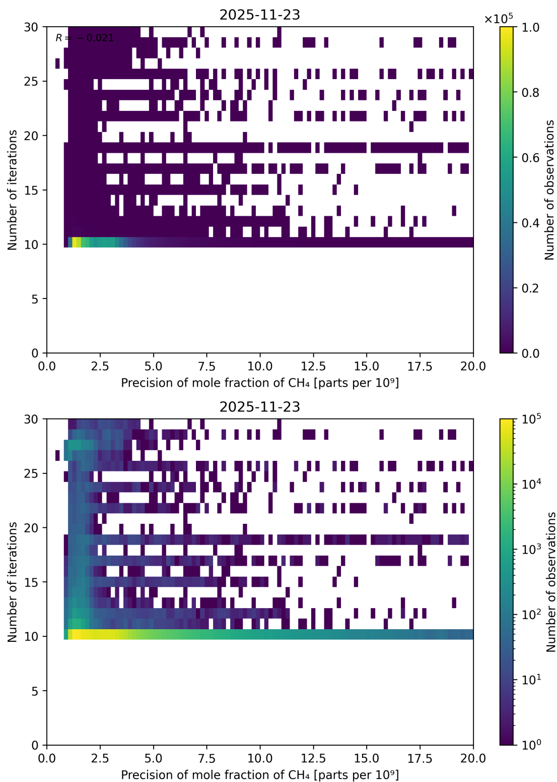
Figure 95: Scatter density plot of “Precision of mole fraction of CH 4 ” against “Number of iterations” for 2025-11-23 to 2025-11-24.
