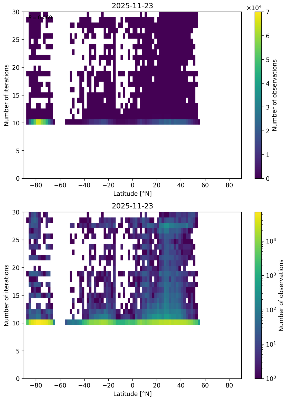
Figure 69: Scatter density plot of “Latitude” against “Number of iterations” for 2025-11-23 to 2025-11-24.
