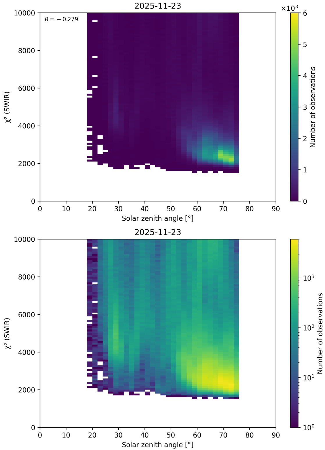
Figure 109: Scatter density plot of “Solar zenith angle” against “ \chi^2 (SWIR)” for 2025-11-23 to 2025-11-24.
