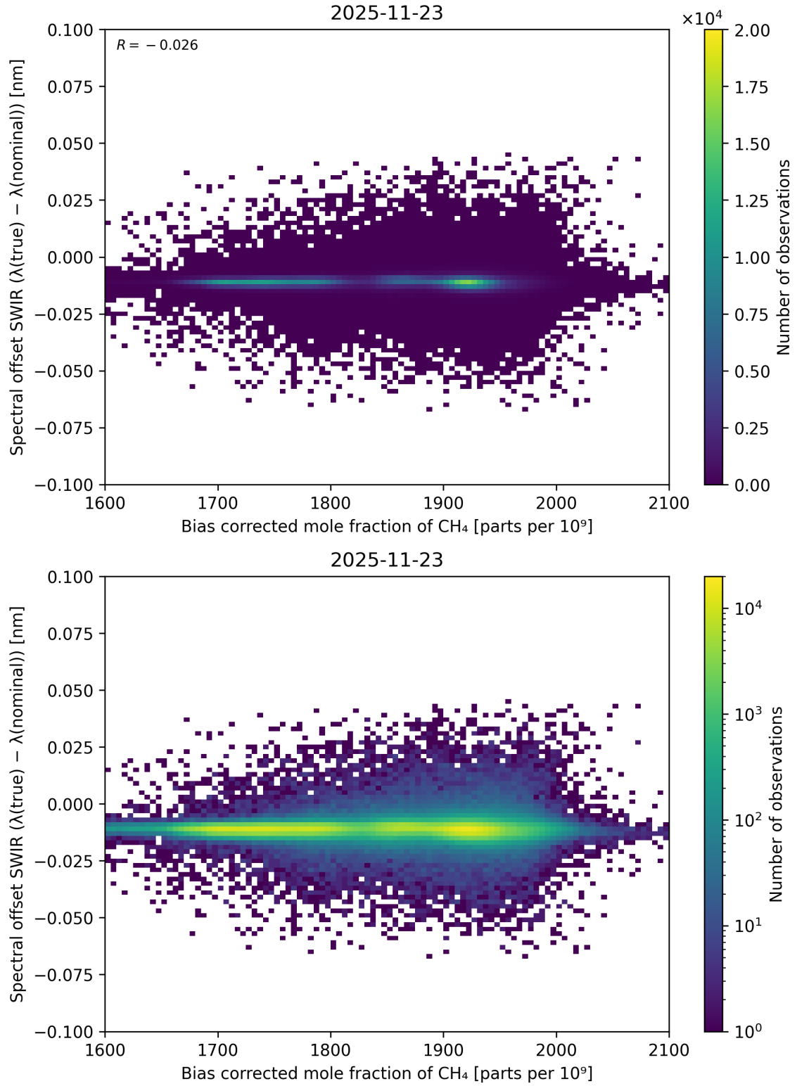
Figure 79: Scatter density plot of “Bias corrected mole fraction of \text{CH}_4 ” against “Spectral offset SWIR ( \lambda_{\text{true}} - \lambda_{\text{nominal}} )” for 2025-11-23 to 2025-11-24.
