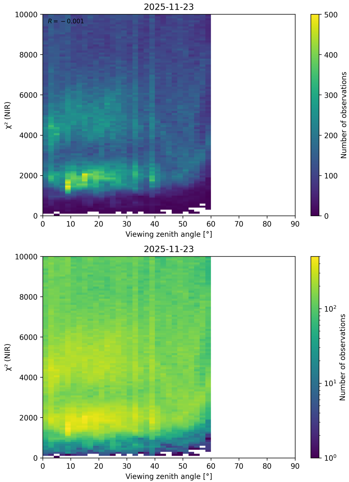
Figure 120: Scatter density plot of “Viewing zenith angle” against “ \chi^2 (NIR)” for 2025-11-23 to 2025-11-24.
