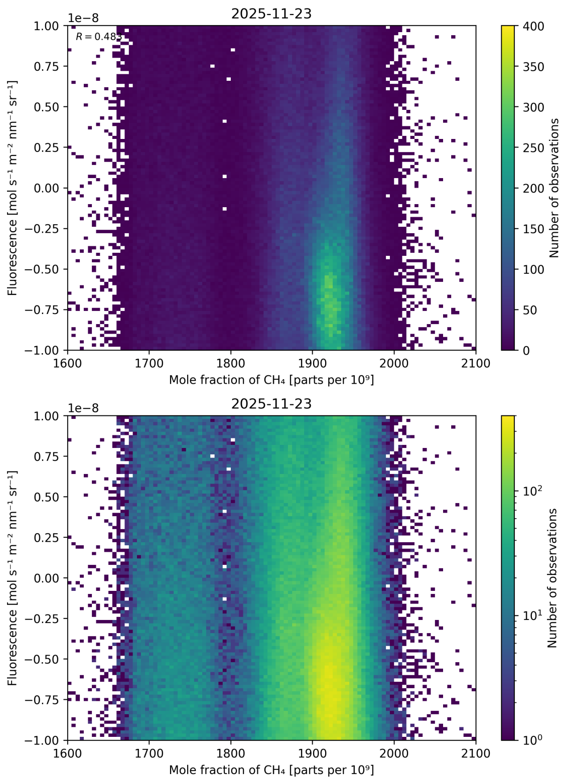
Figure 83: Scatter density plot of “Mole fraction of CH 4 ” against “Fluorescence” for 2025-11-23 to 2025-11-24.
