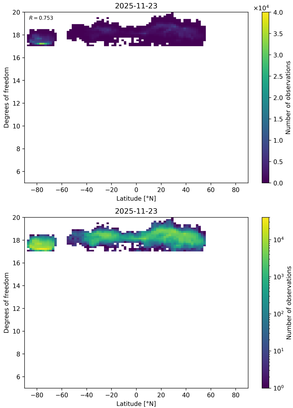
Figure 63: Scatter density plot of “Latitude” against “Degrees of freedom” for 2025-11-23 to 2025-11-24.
