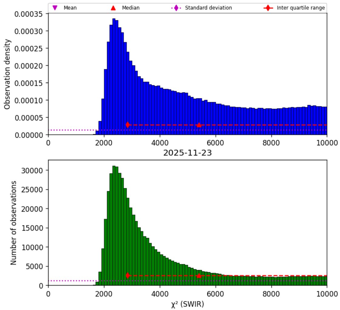
Figure 30: Histogram of “ \chi^2 (SWIR)” for 2025-11-23 to 2025-11-24
