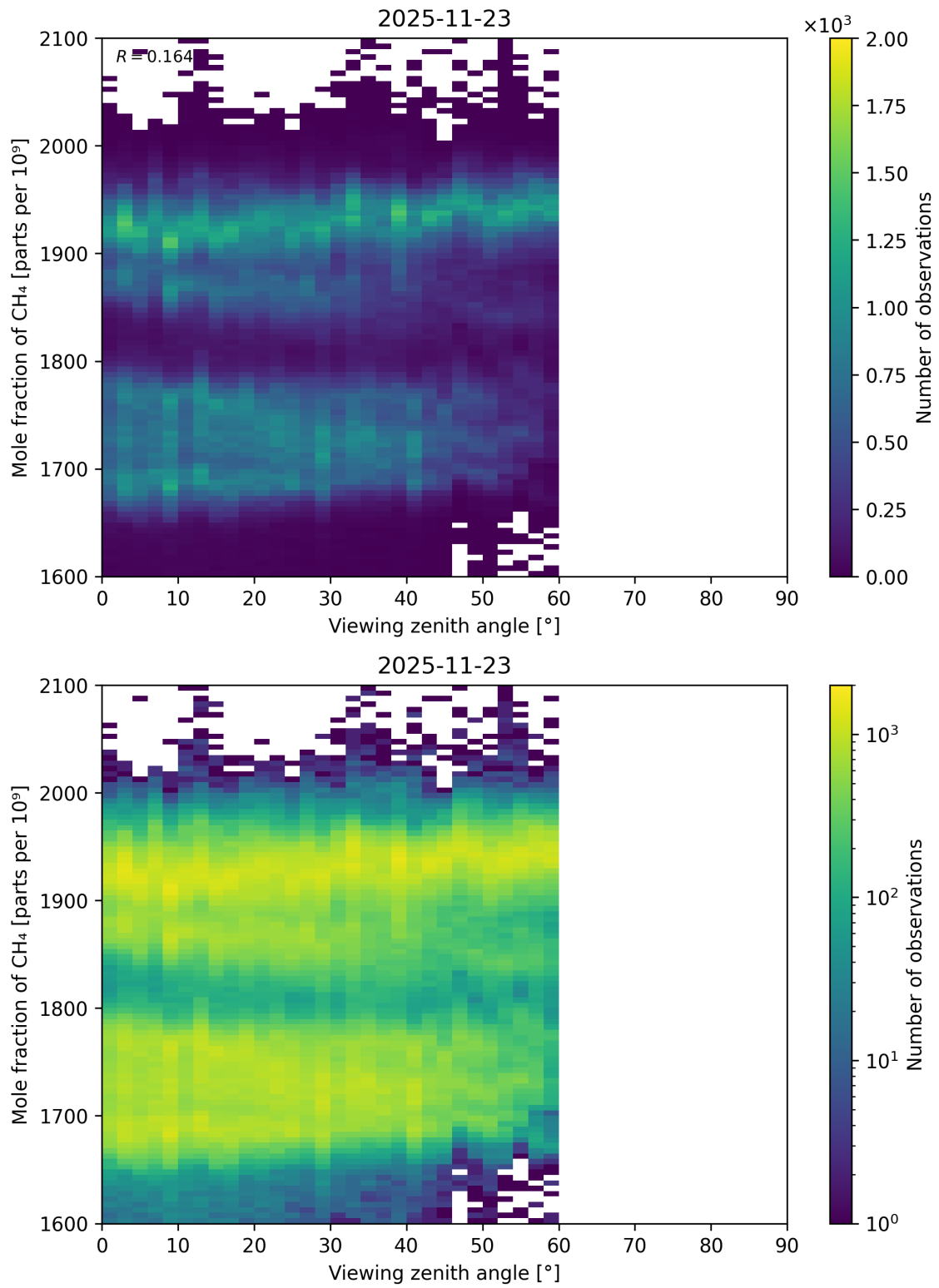
Figure 126: Scatter density plot of “Viewing zenith angle” against “Mole fraction of CH 4 ” for 2025-11-23 to 2025-11-24.
