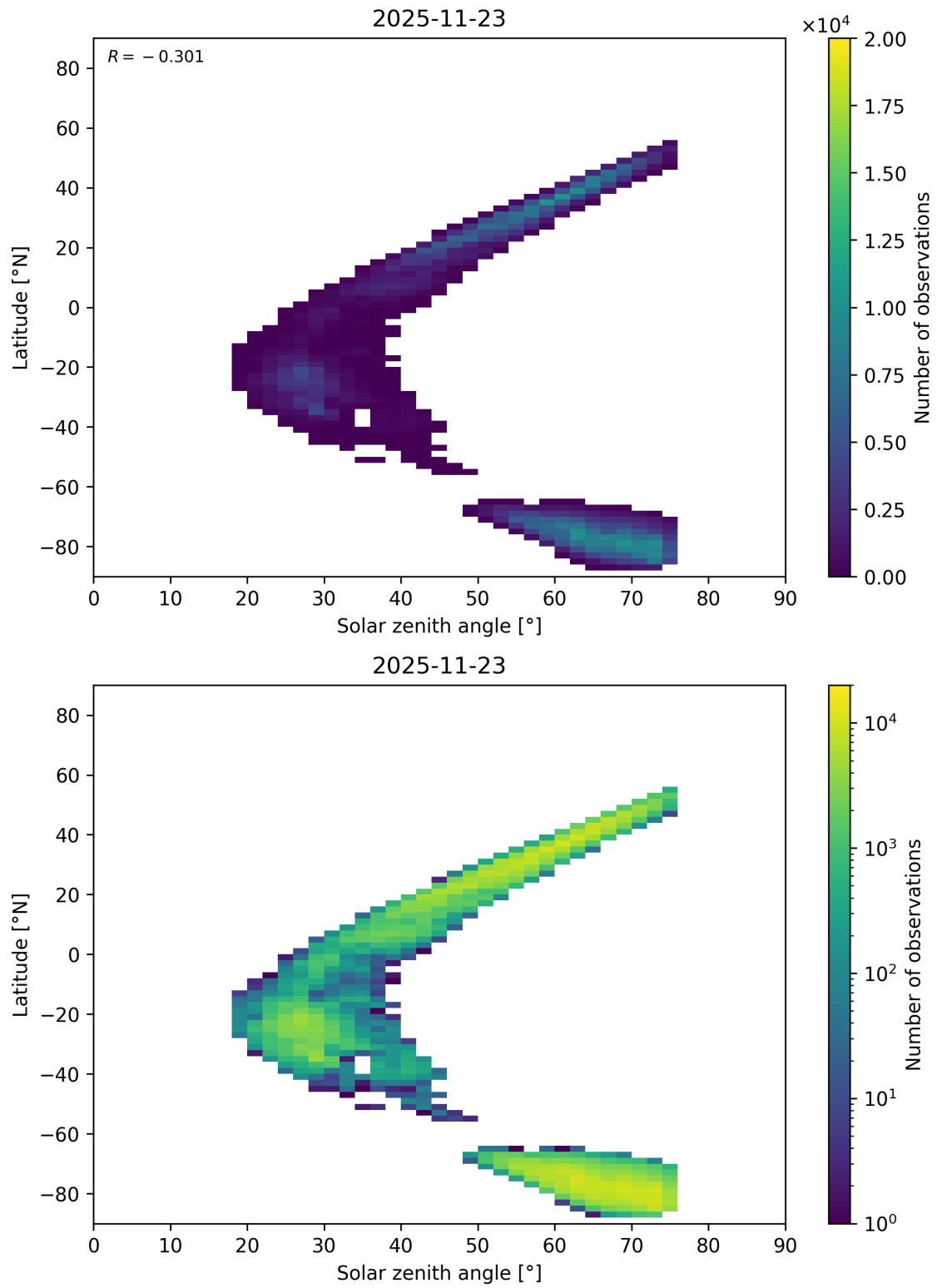
Figure 113: Scatter density plot of “Solar zenith angle” against “Latitude” for 2025-11-23 to 2025-11-24.
