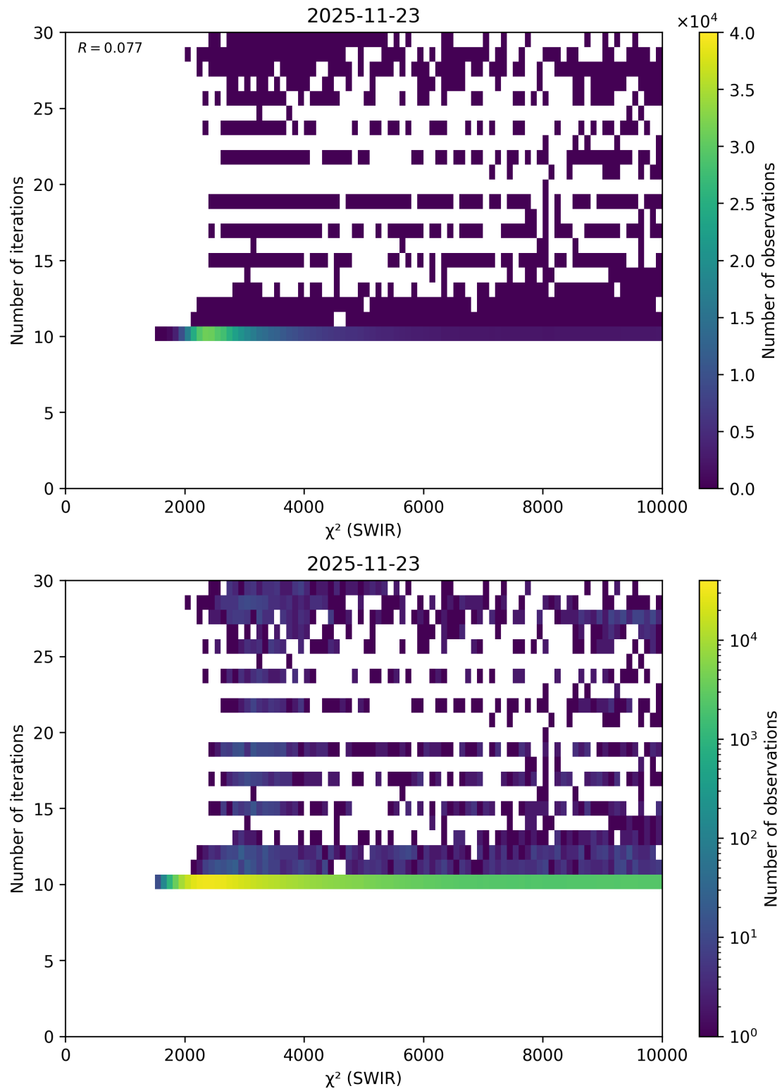
Figure 56: Scatter density plot of “ \chi^2 (SWIR)” against “Number of iterations” for 2025-11-23 to 2025-11-24.
