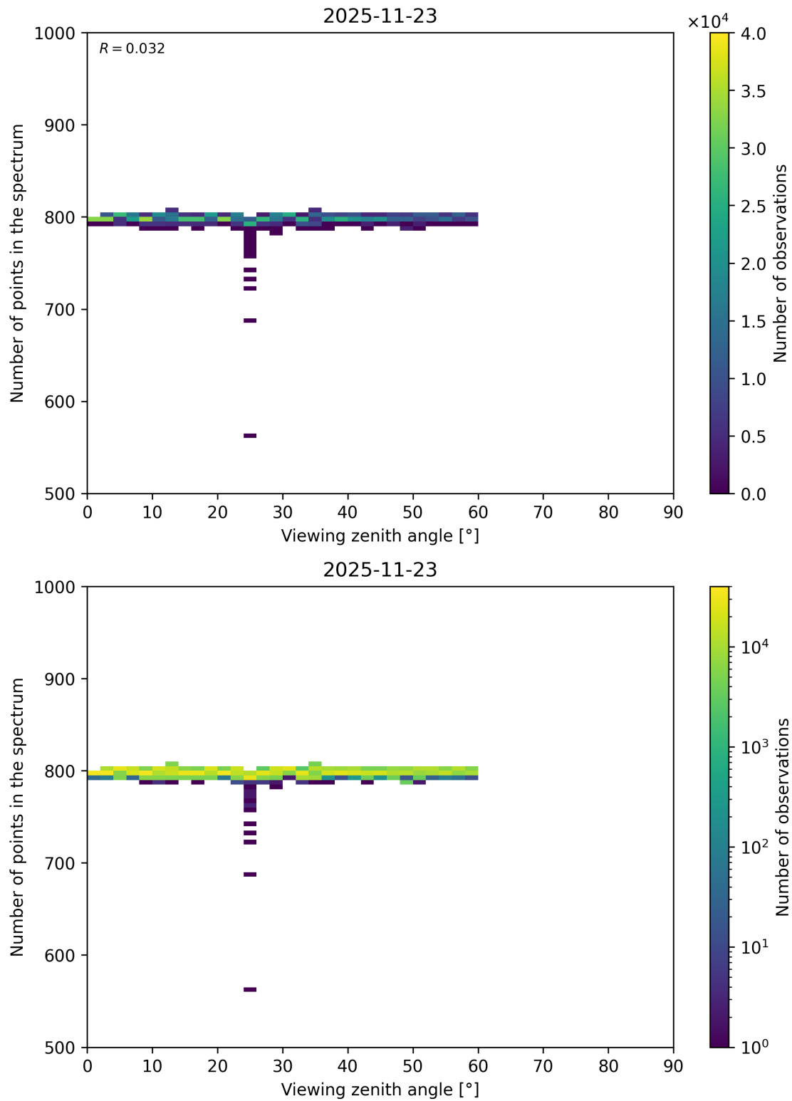
Figure 130: Scatter density plot of “Viewing zenith angle” against “Number of points in the spectrum” for 2025-11-23 to 2025-11-24.
