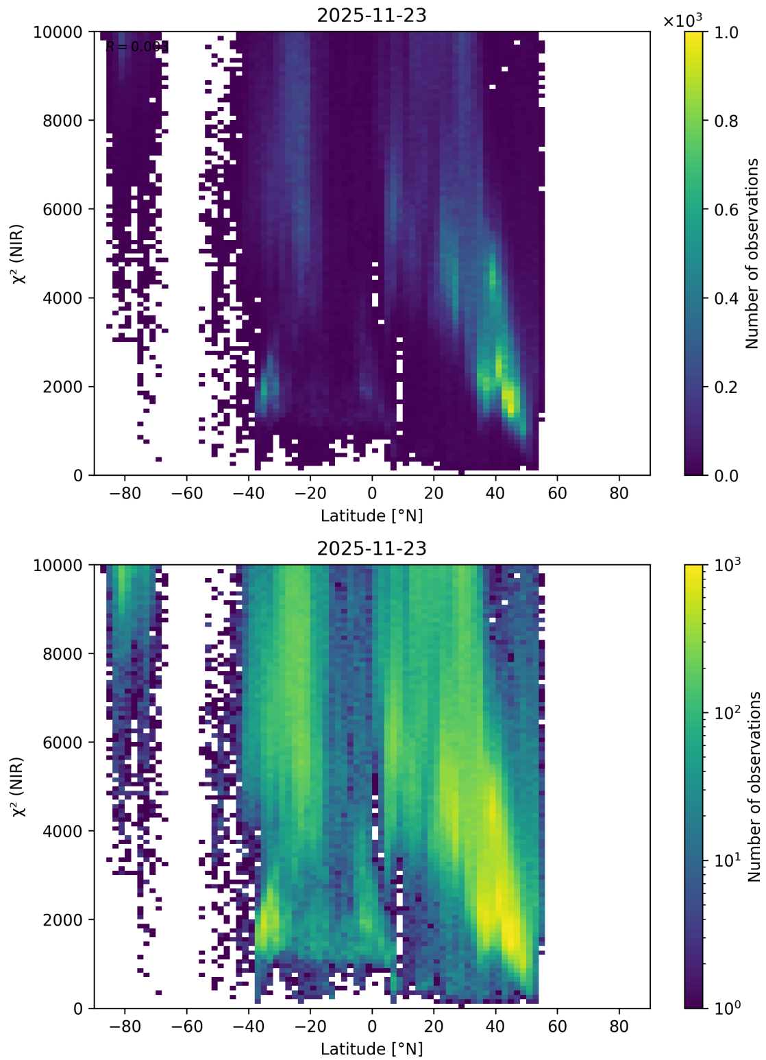
Figure 61: Scatter density plot of “Latitude” against “ \chi^2 (NIR)” for 2025-11-23 to 2025-11-24.
