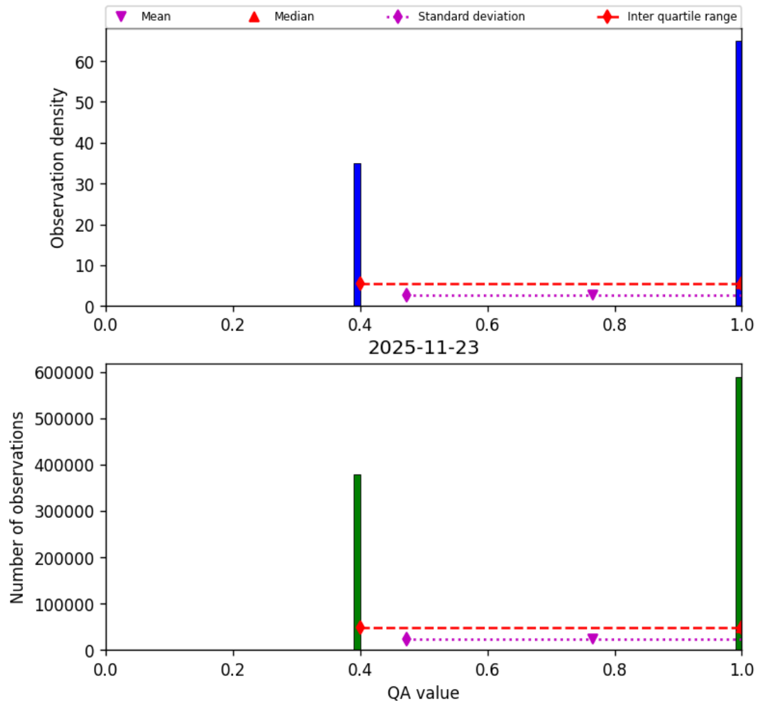
Figure 24: Histogram of “QA value” for 2025-11-23 to 2025-11-24
