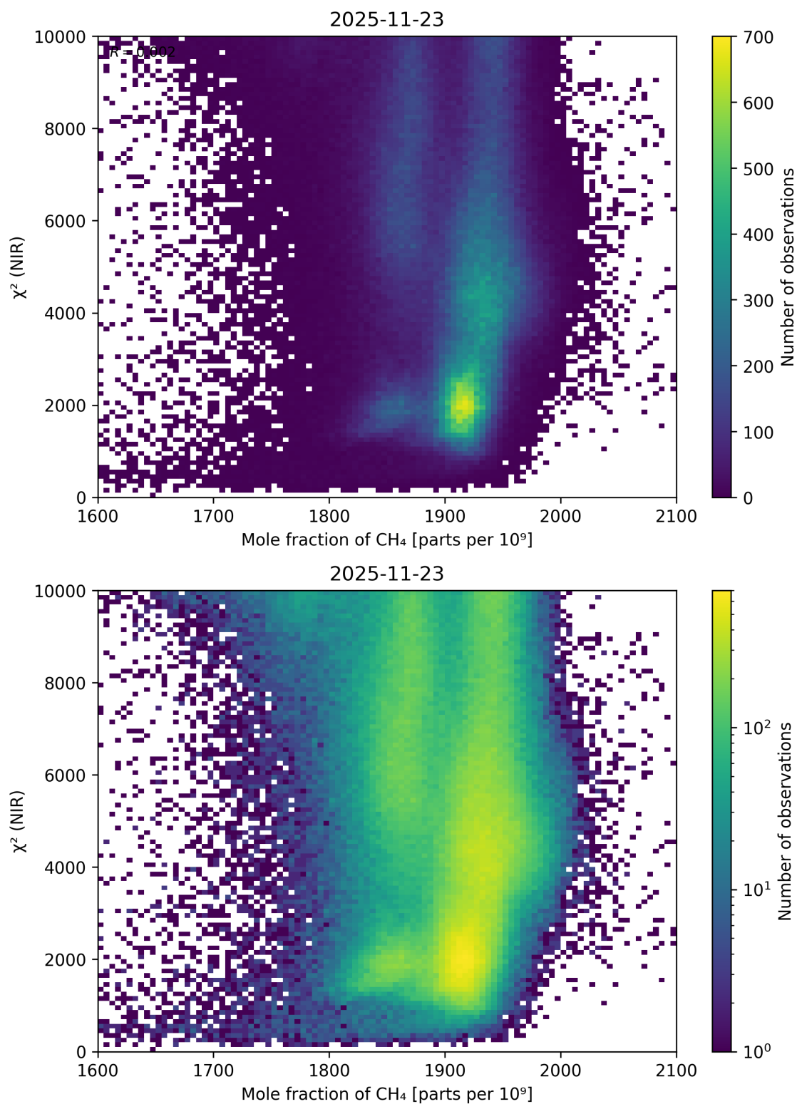
Figure 80: Scatter density plot of “Mole fraction of \text{CH}_4 ” against “ \chi^2 (NIR)” for 2025-11-23 to 2025-11-24.
