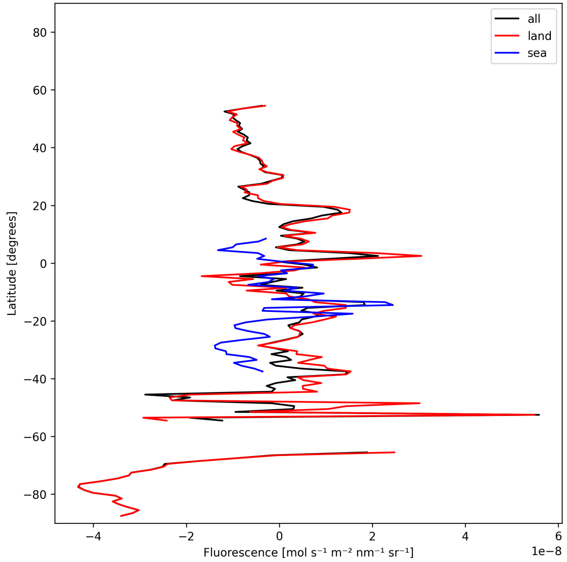
Figure 22: Zonal average of “Fluorescence” for 2025-11-23 to 2025-11-24.
