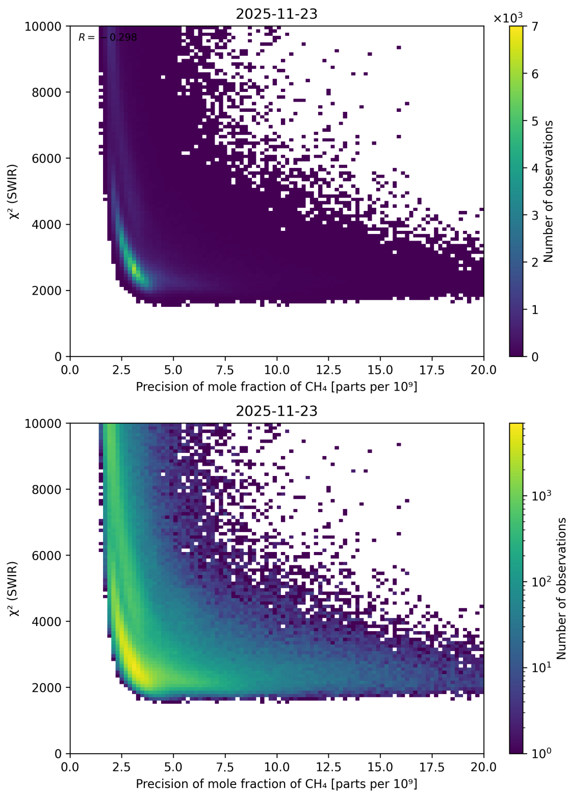
Figure 90: Scatter density plot of “Precision of mole fraction of \text{CH}_4 ” against “ \chi^2 (SWIR)” for 2025-11-23 to 2025-11-24.
