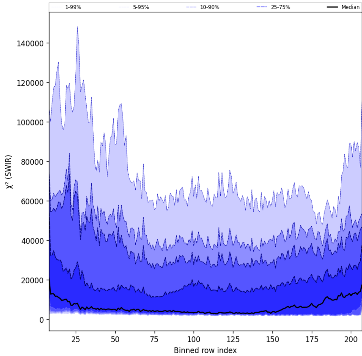
Figure 42: Along track statistics of “ \chi^2 (SWIR)” for 2025-11-23 to 2025-11-24
