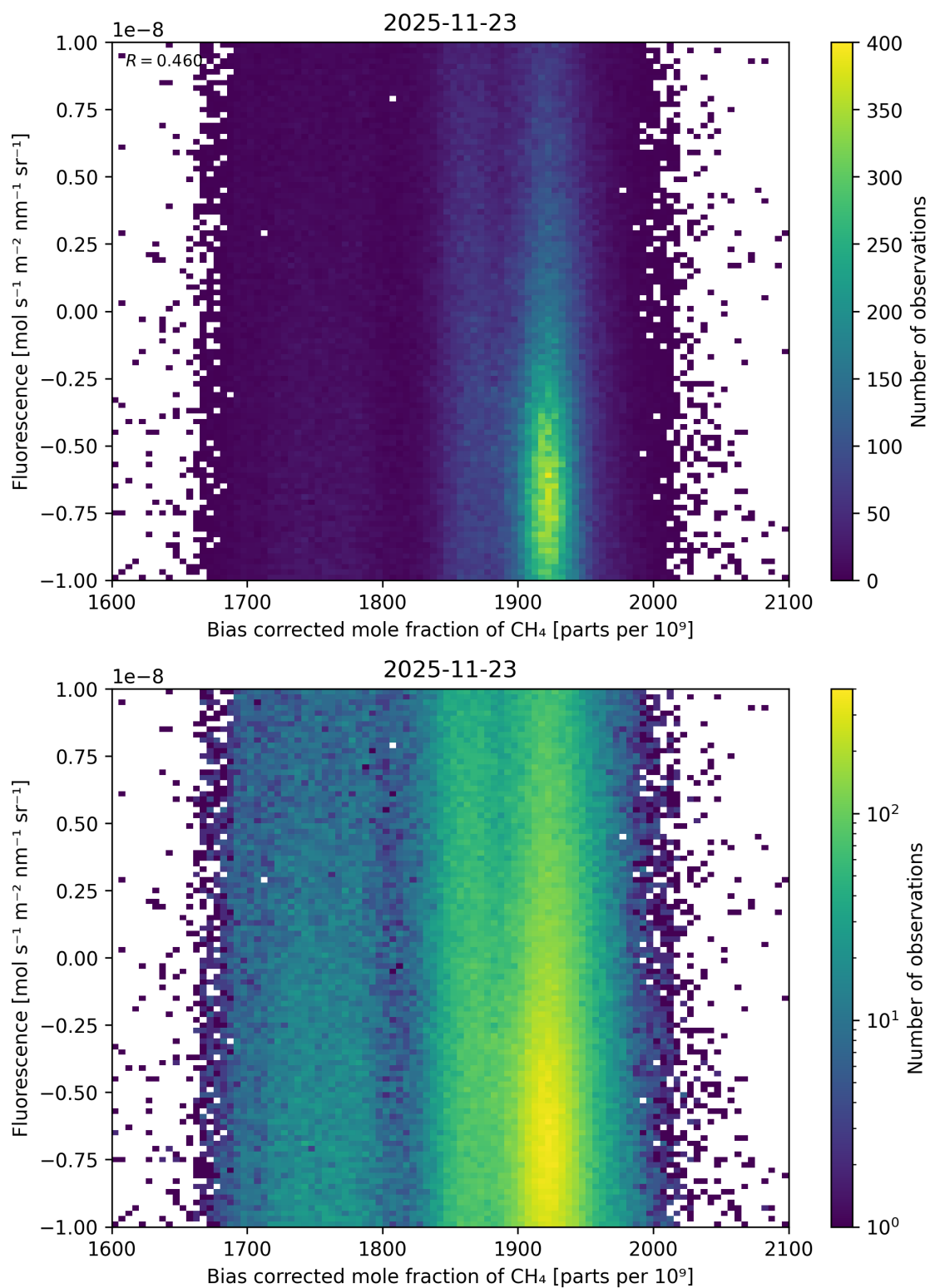
Figure 75: Scatter density plot of “Bias corrected mole fraction of \text{CH}_4 ” against “Fluorescence” for 2025-11-23 to 2025-11-24.
