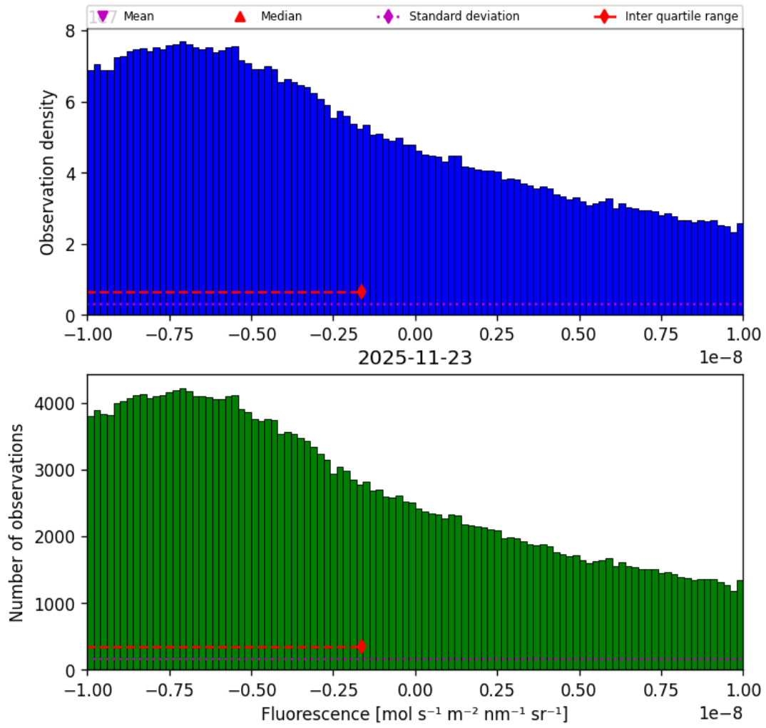
Figure 34: Histogram of “Fluorescence” for 2025-11-23 to 2025-11-24
