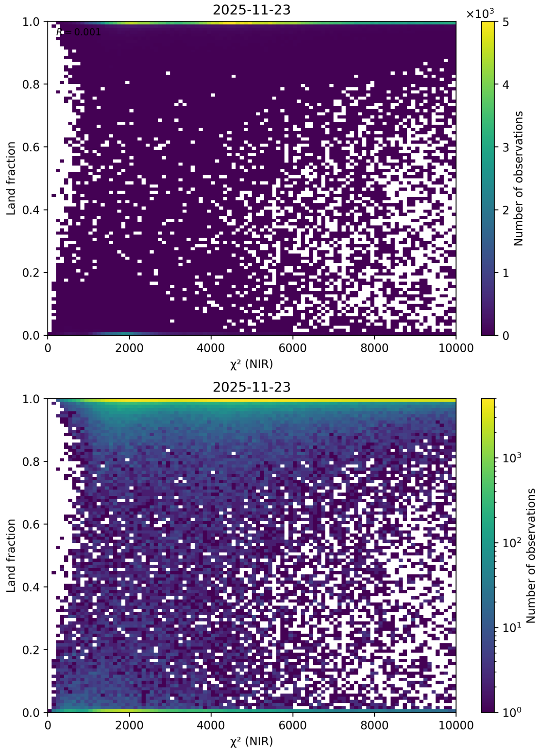
Figure 50: Scatter density plot of “ \chi^2 (NIR)” against “Land fraction” for 2025-11-23 to 2025-11-24.
