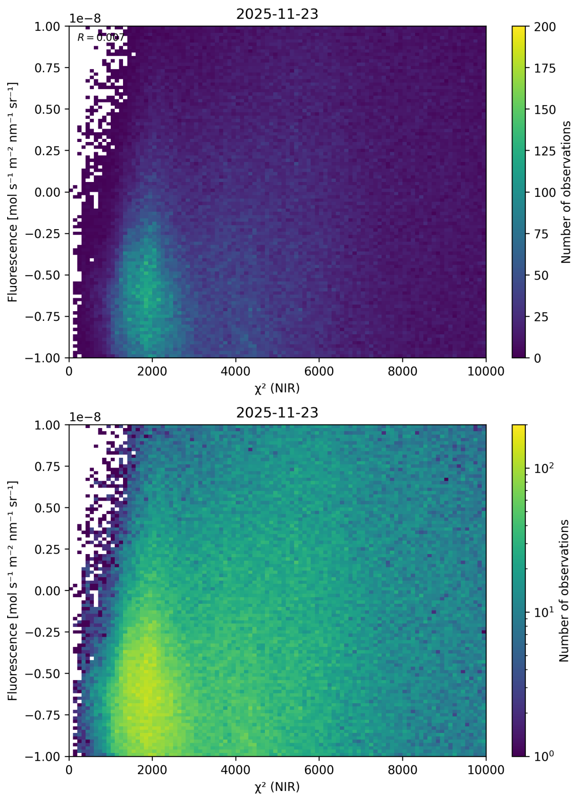
Figure 49: Scatter density plot of “ \chi^2 (NIR)” against “Fluorescence” for 2025-11-23 to 2025-11-24.
