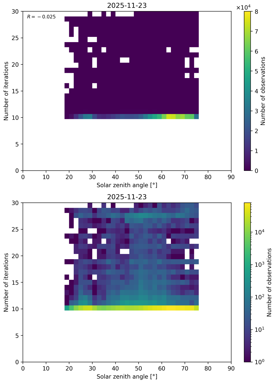
Figure 117: Scatter density plot of “Solar zenith angle” against “Number of iterations” for 2025-11-23 to 2025-11-24.
