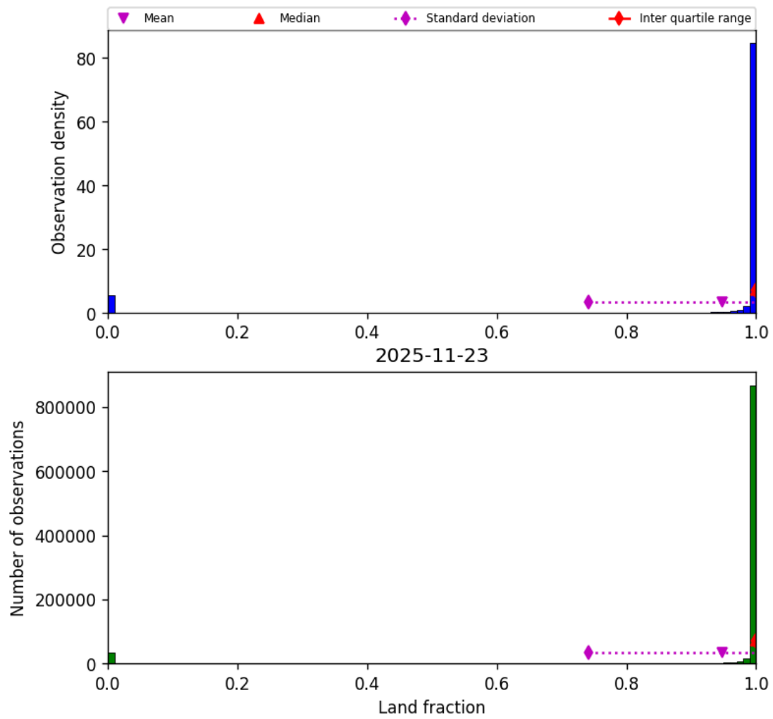
Figure 35: Histogram of “Land fraction” for 2025-11-23 to 2025-11-24
