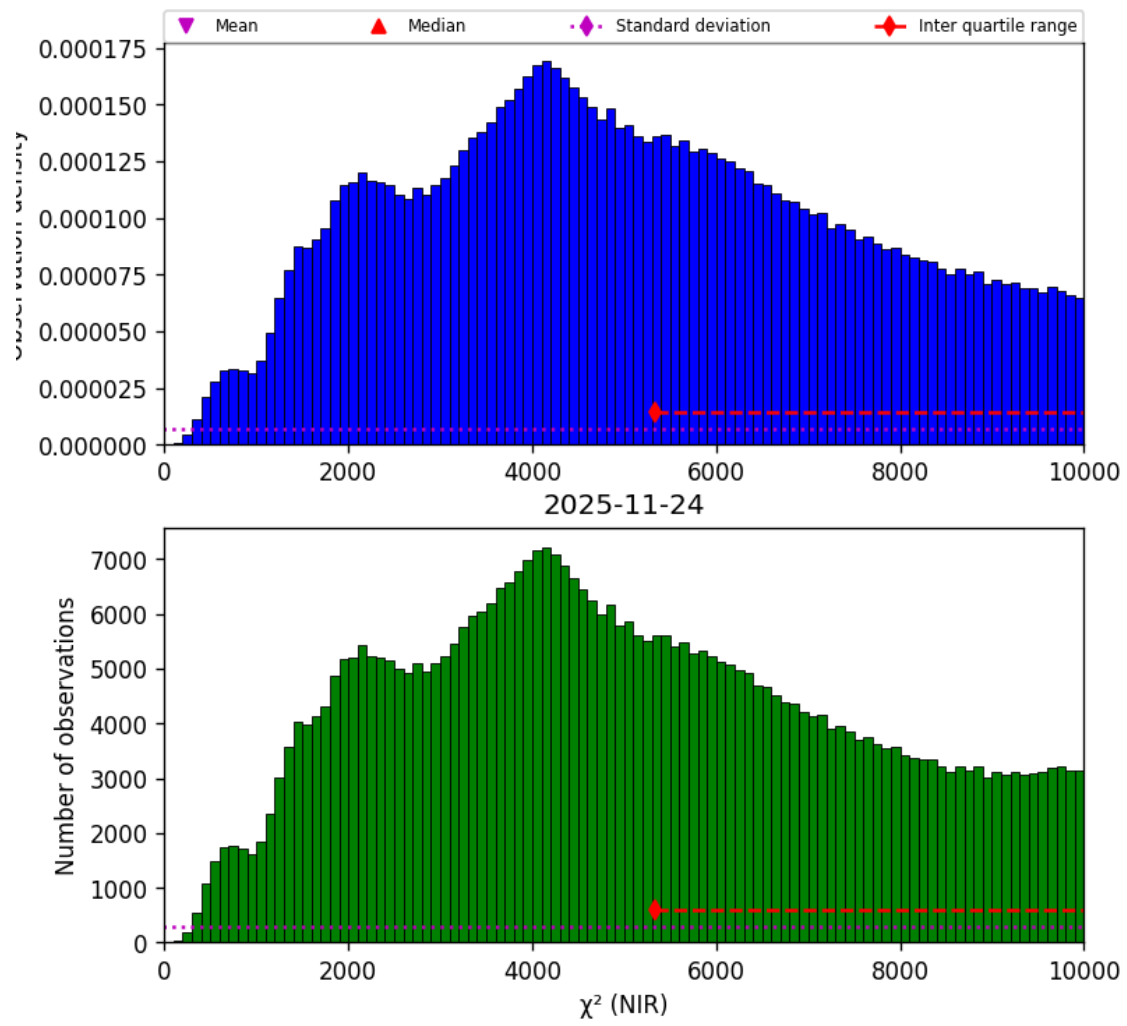
Figure 31: Histogram of “ \chi^2 (NIR)” for 2025-11-23 to 2025-11-25
