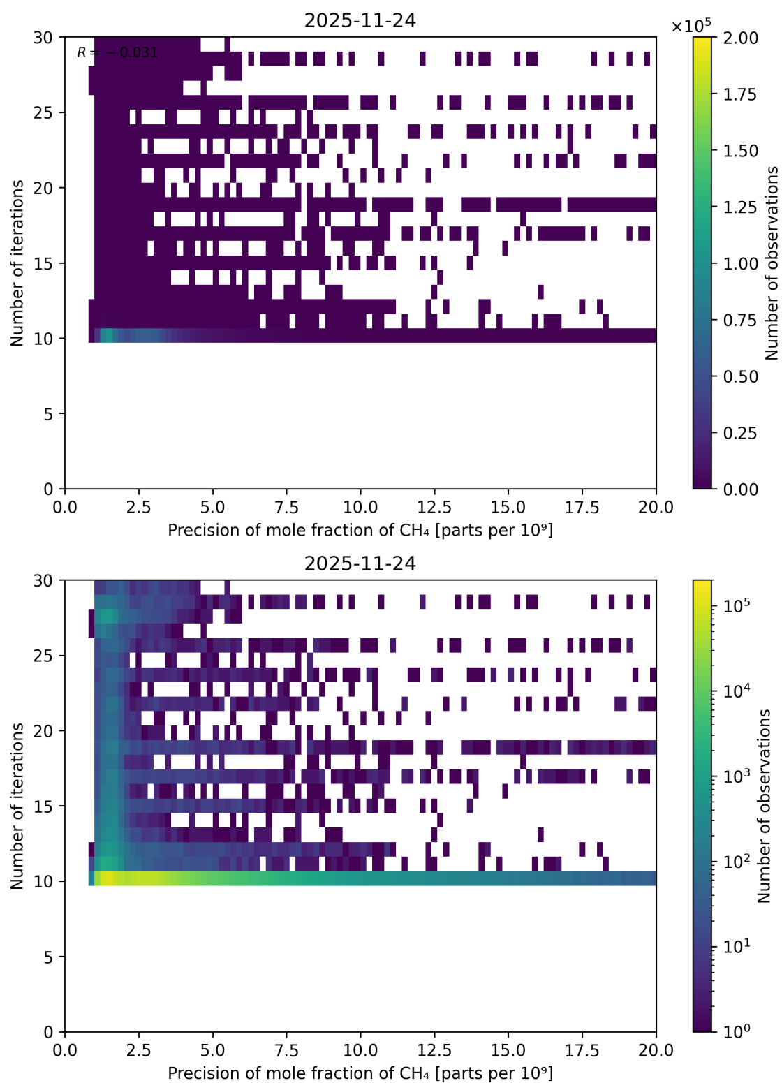
Figure 95: Scatter density plot of “Precision of mole fraction of CH 4 ” against “Number of iterations” for 2025-11-23 to 2025-11-25.
