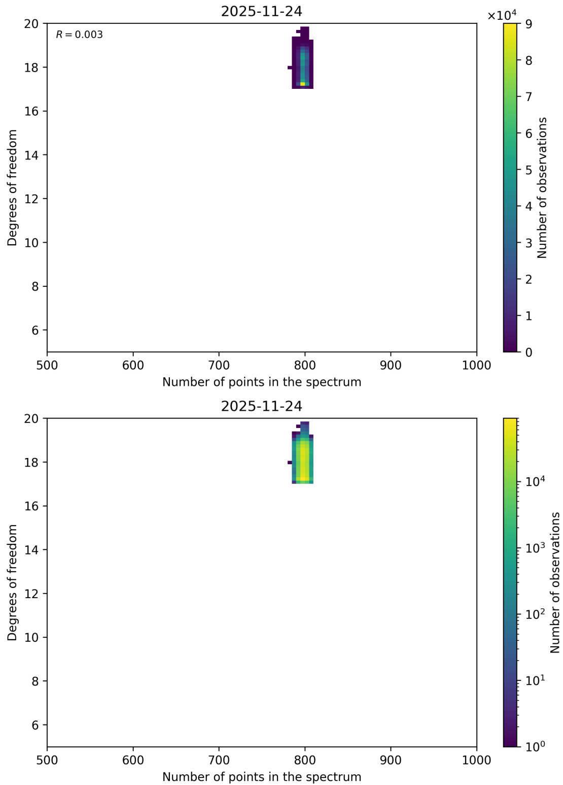
Figure 103: Scatter density plot of “Number of points in the spectrum” against “Degrees of freedom” for 2025-11-23 to 2025-11-25.
