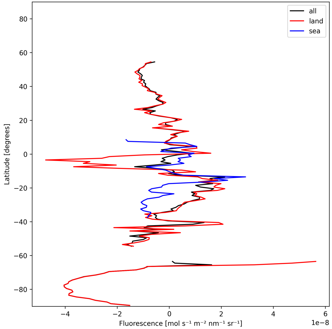
Figure 22: Zonal average of “Fluorescence” for 2025-11-23 to 2025-11-25.
