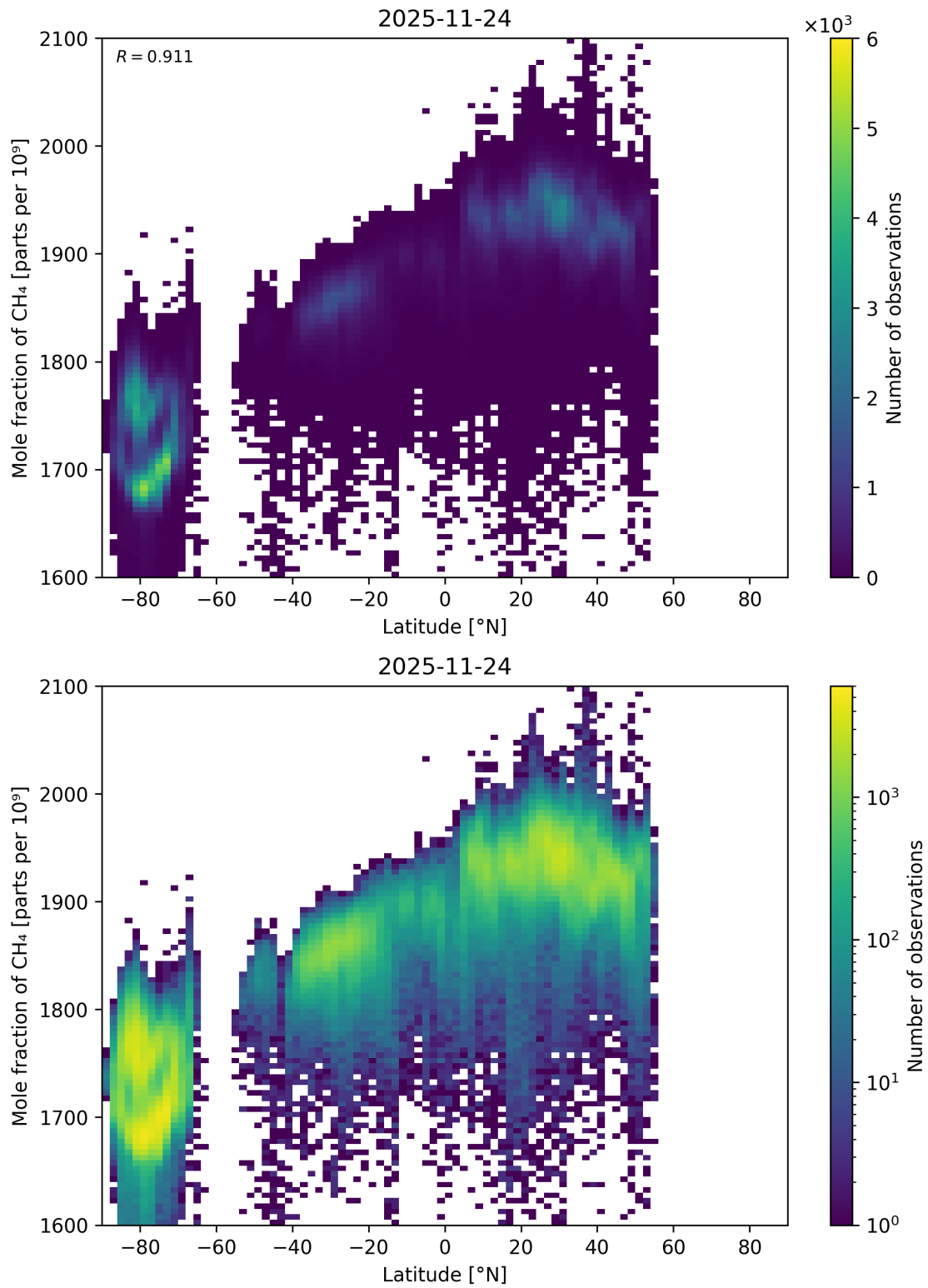
Figure 66: Scatter density plot of “Latitude” against “Mole fraction of CH 4 ” for 2025-11-23 to 2025-11-25.
