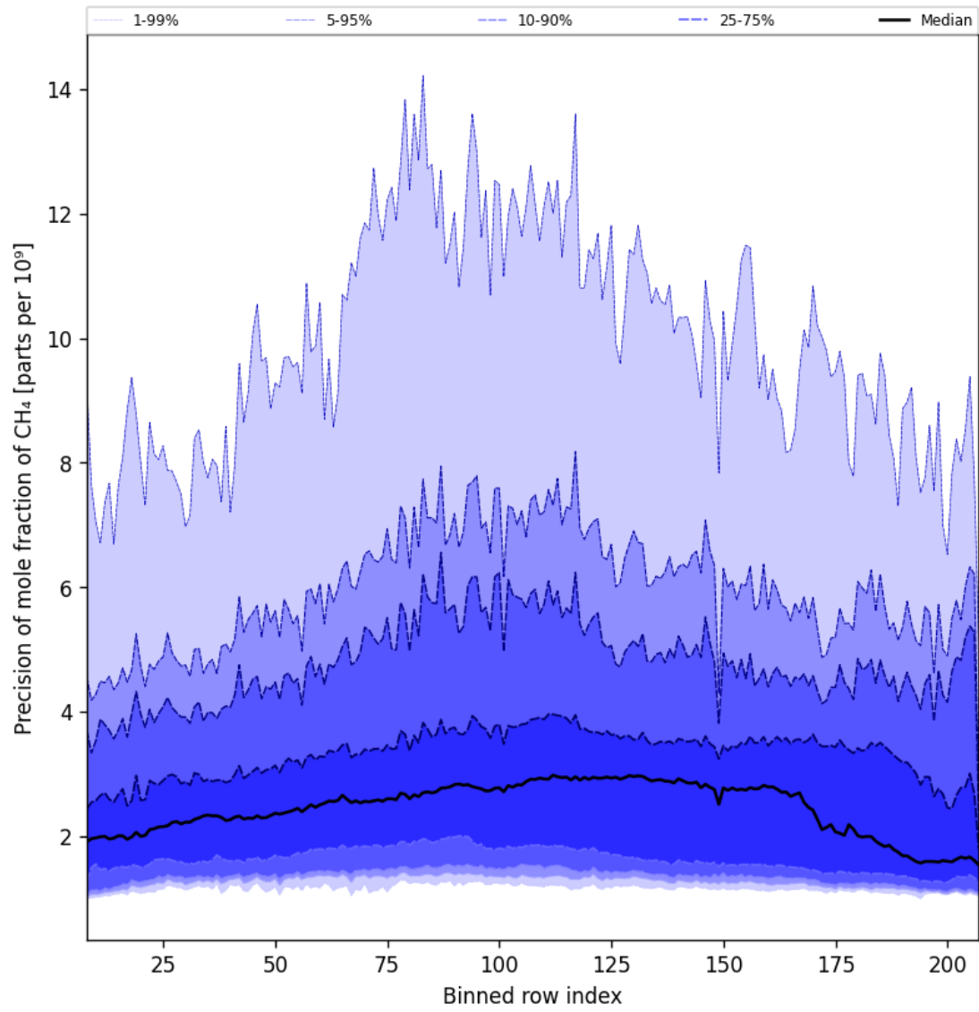
Figure 38: Along track statistics of “Precision of mole fraction of CH 4 ” for 2025-11-23 to 2025-11-25
