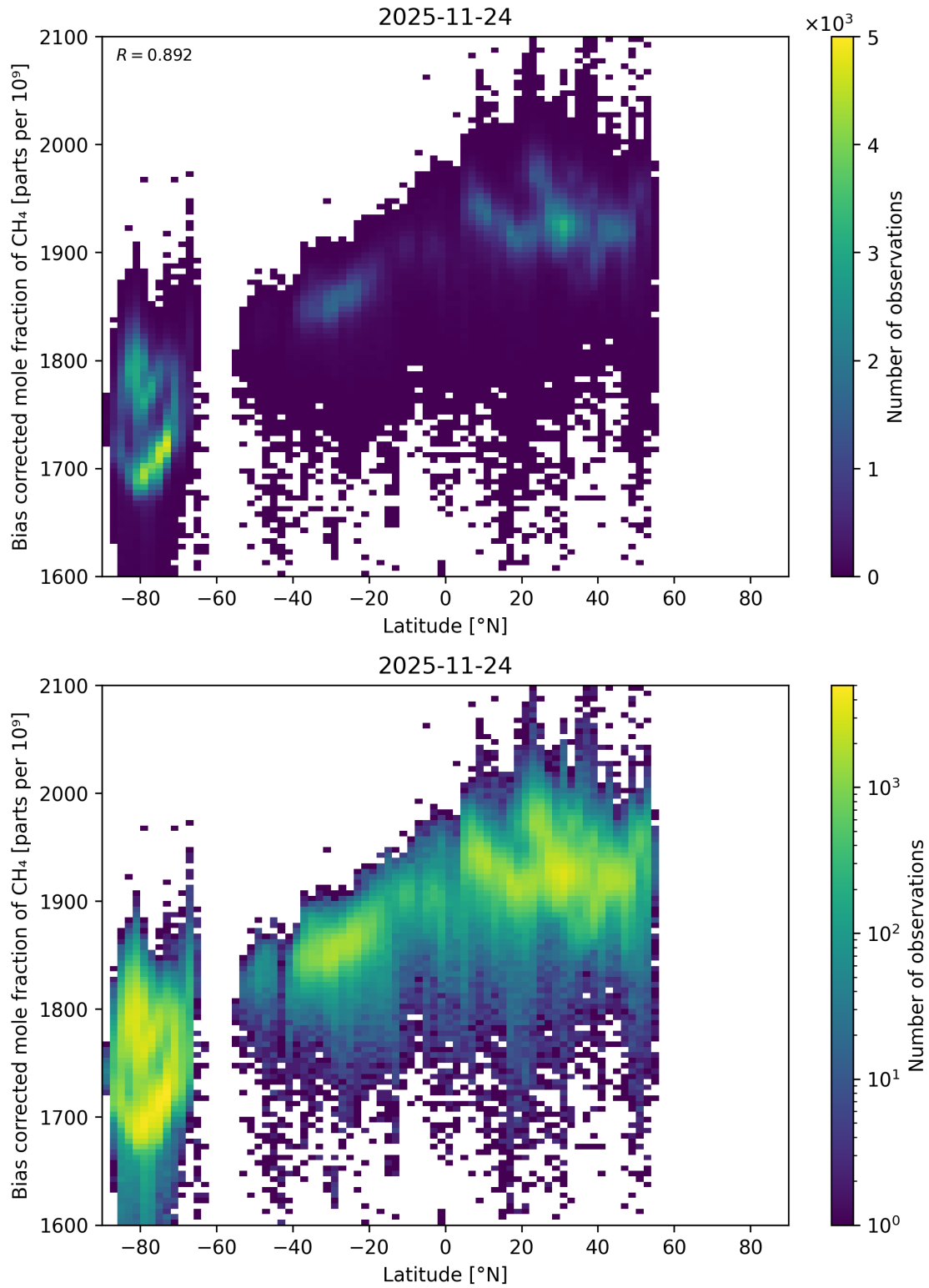
Figure 67: Scatter density plot of “Latitude” against “Bias corrected mole fraction of \text{CH}_4 ” for 2025-11-23 to 2025-11-25.
