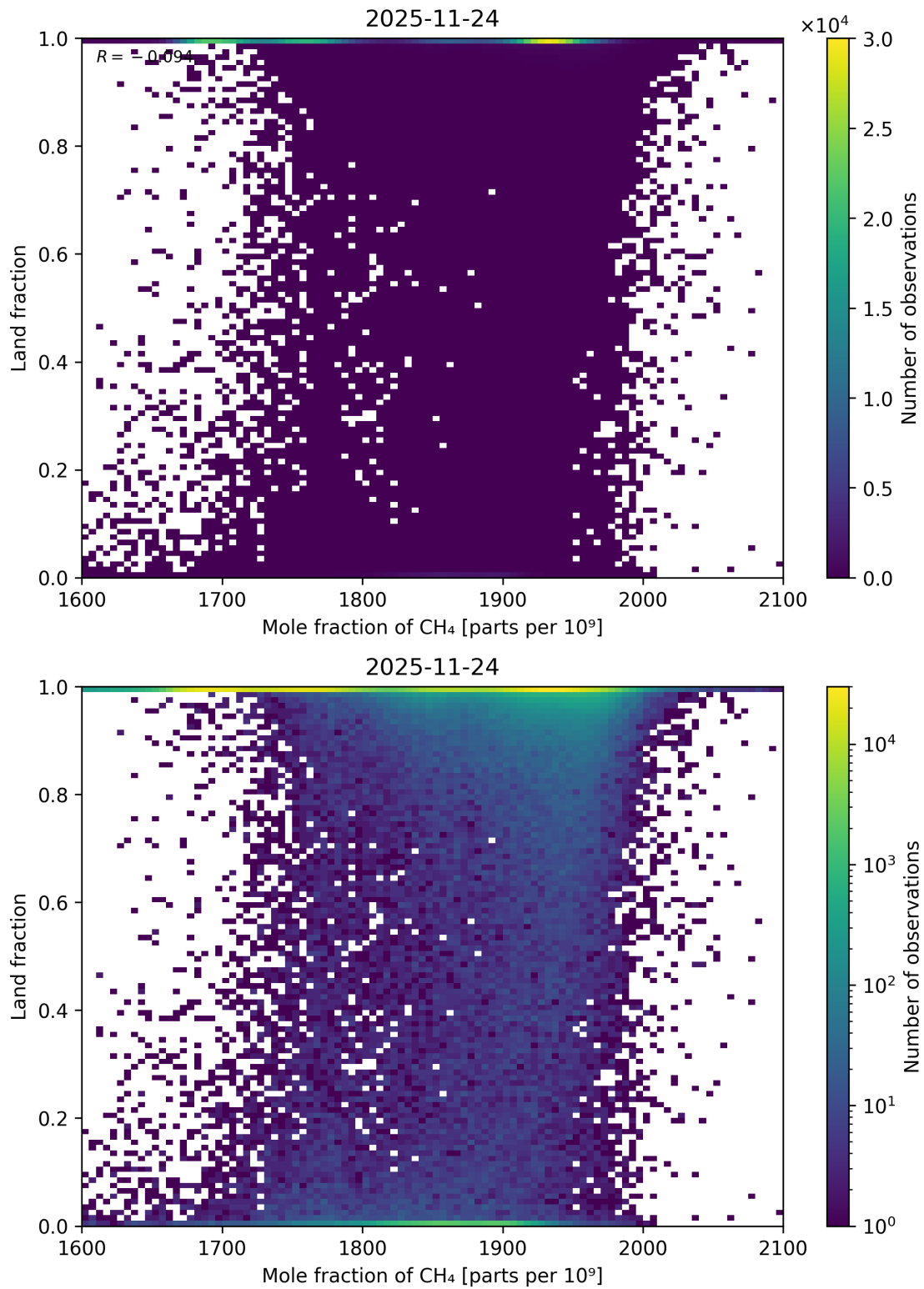
Figure 84: Scatter density plot of “Mole fraction of CH 4 ” against “Land fraction” for 2025-11-23 to 2025-11-25.
