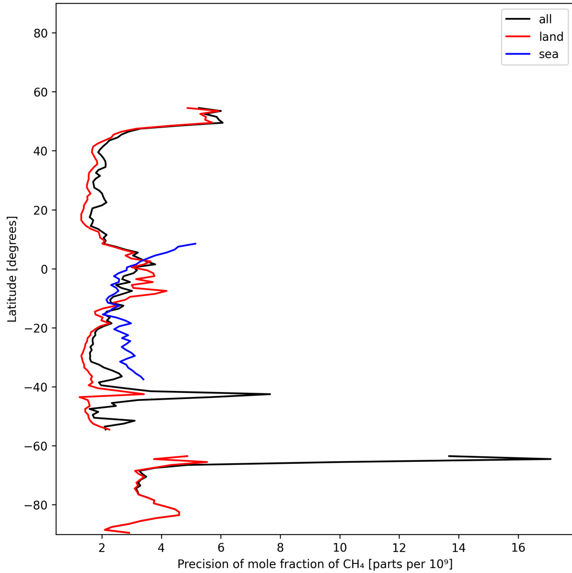
Figure 14: Zonal average of “Precision of mole fraction of CH 4 ” for 2025-11-23 to 2025-11-25.
