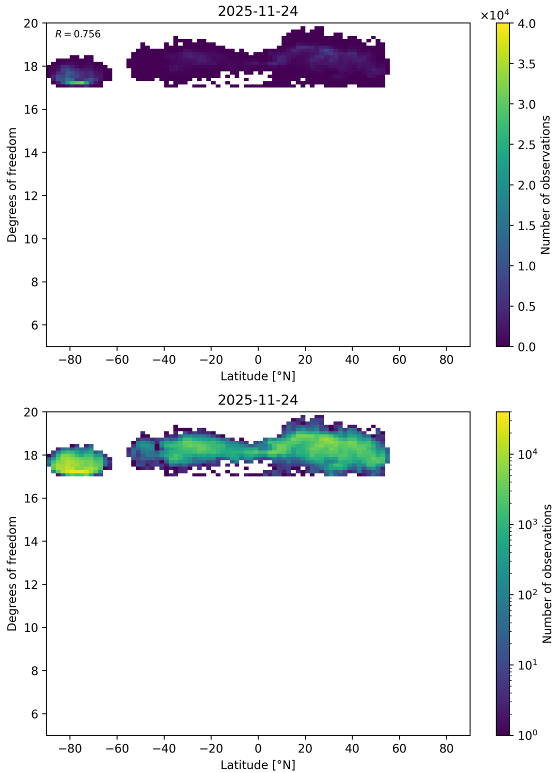
Figure 63: Scatter density plot of “Latitude” against “Degrees of freedom” for 2025-11-23 to 2025-11-25.
