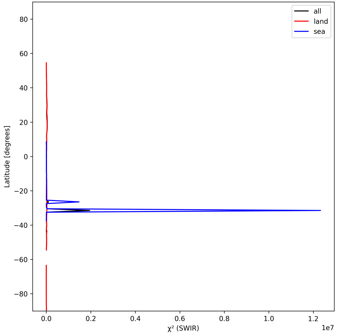
Figure 18: Zonal average of “ \chi^2 (SWIR)” for 2025-11-23 to 2025-11-25.
