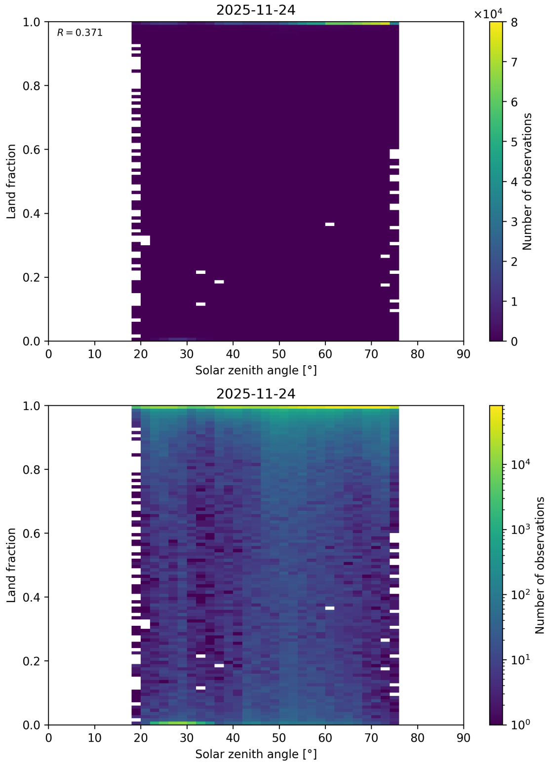
Figure 112: Scatter density plot of “Solar zenith angle” against “Land fraction” for 2025-11-23 to 2025-11-25.
