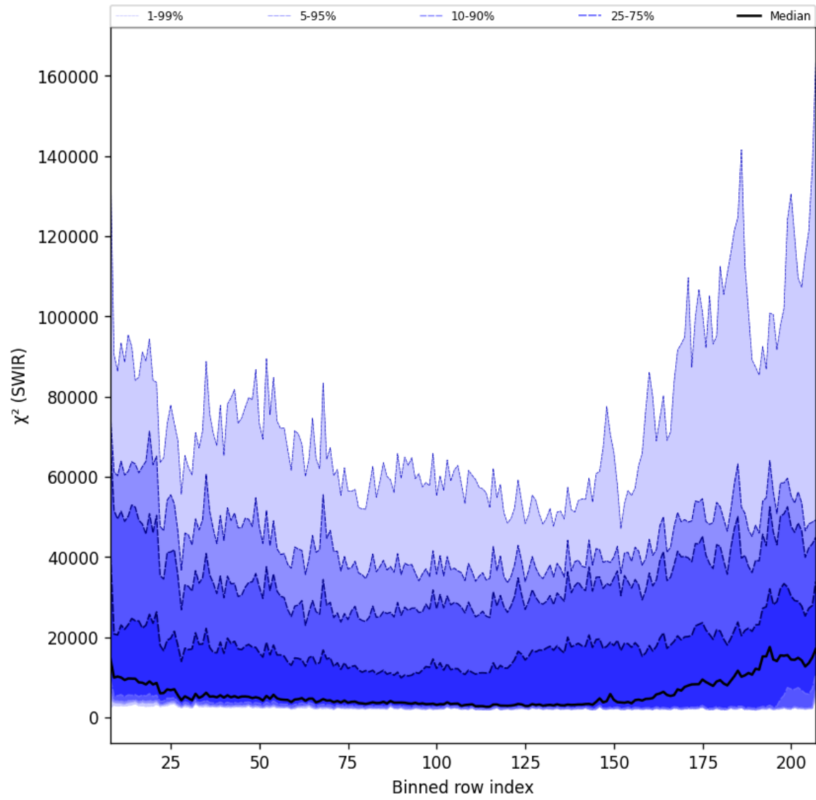
Figure 42: Along track statistics of “ \chi^2 (SWIR)” for 2025-11-23 to 2025-11-25
