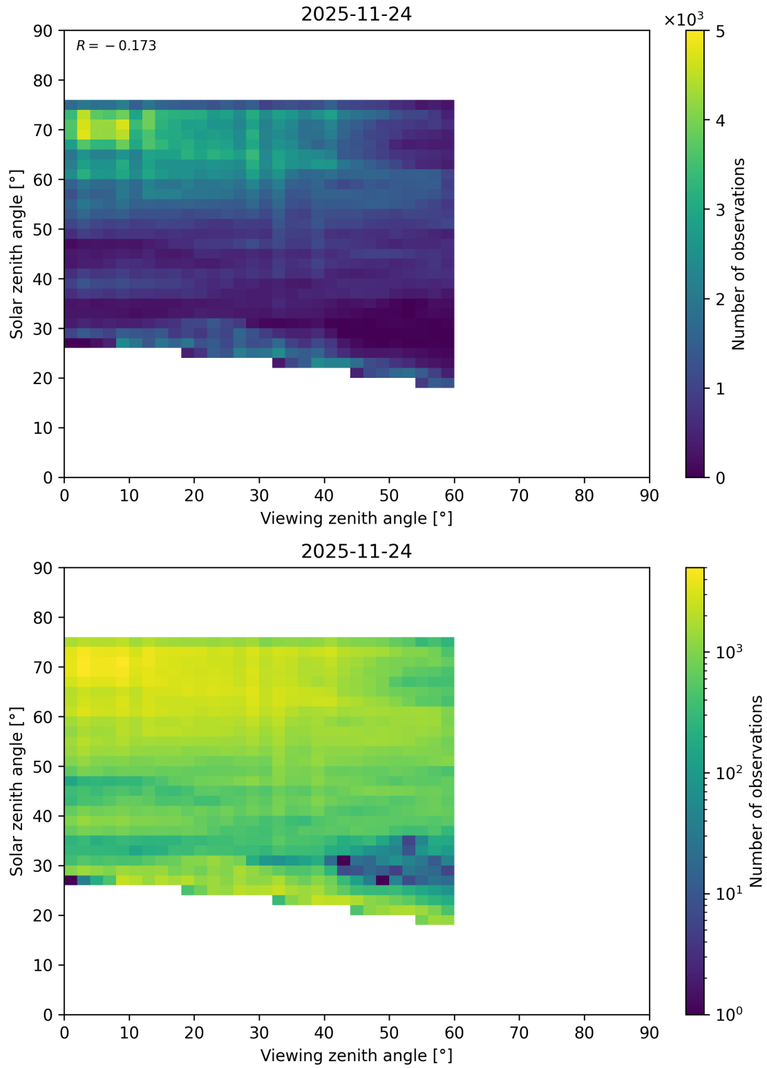
Figure 131: Scatter density plot of “Viewing zenith angle” against “Solar zenith angle” for 2025-11-23 to 2025-11-25.
