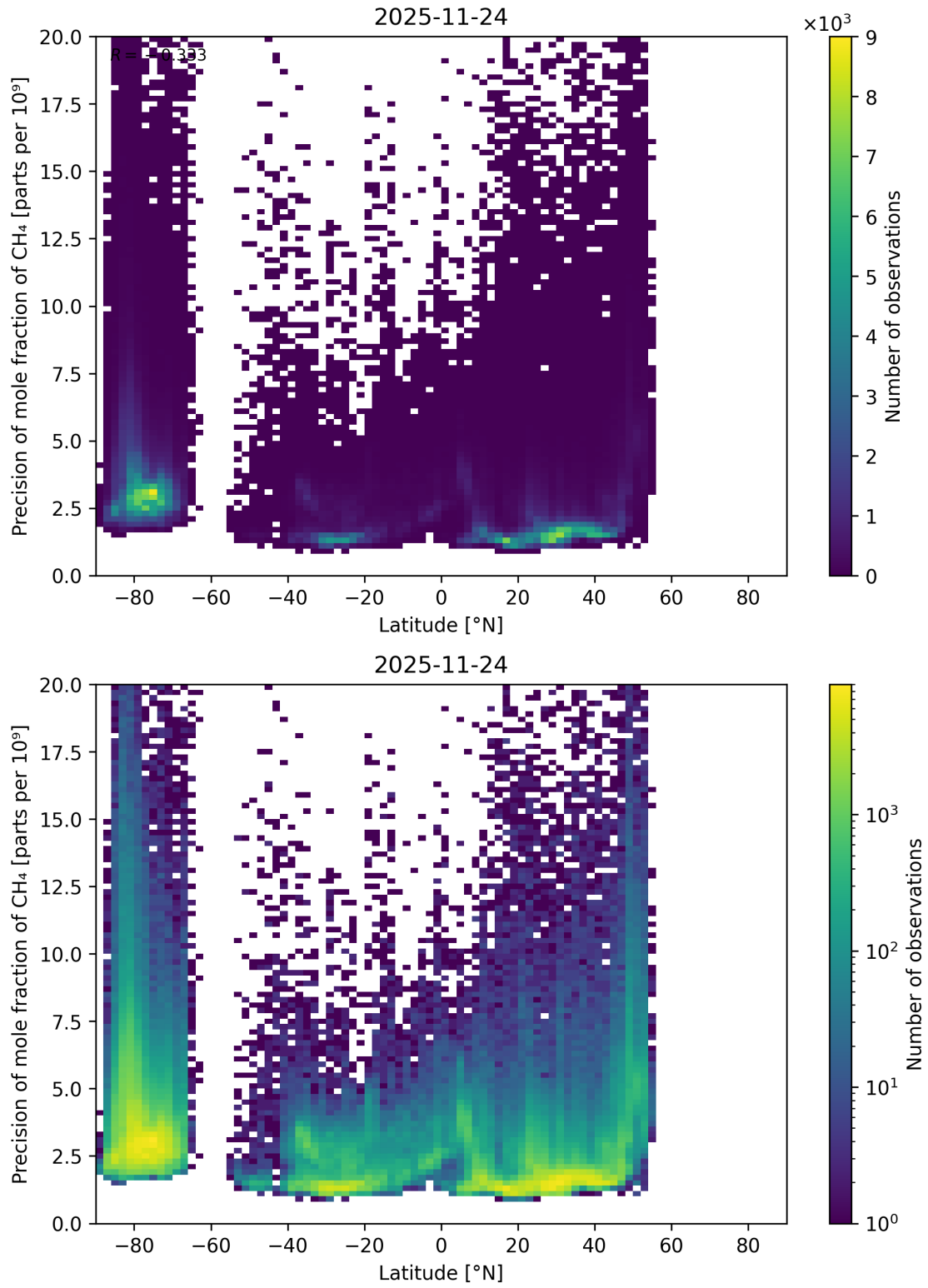
Figure 68: Scatter density plot of “Latitude” against “Precision of mole fraction of CH 4 ” for 2025-11-23 to 2025-11-25.
