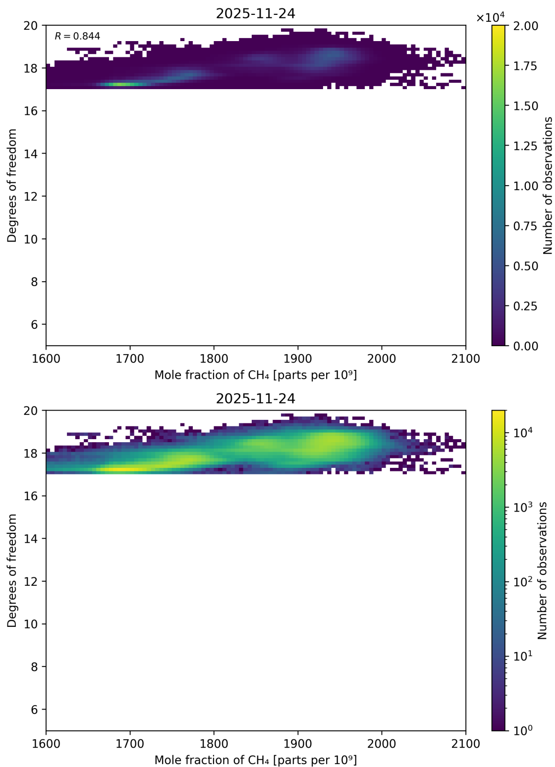
Figure 82: Scatter density plot of “Mole fraction of CH 4 ” against “Degrees of freedom” for 2025-11-23 to 2025-11-25.
