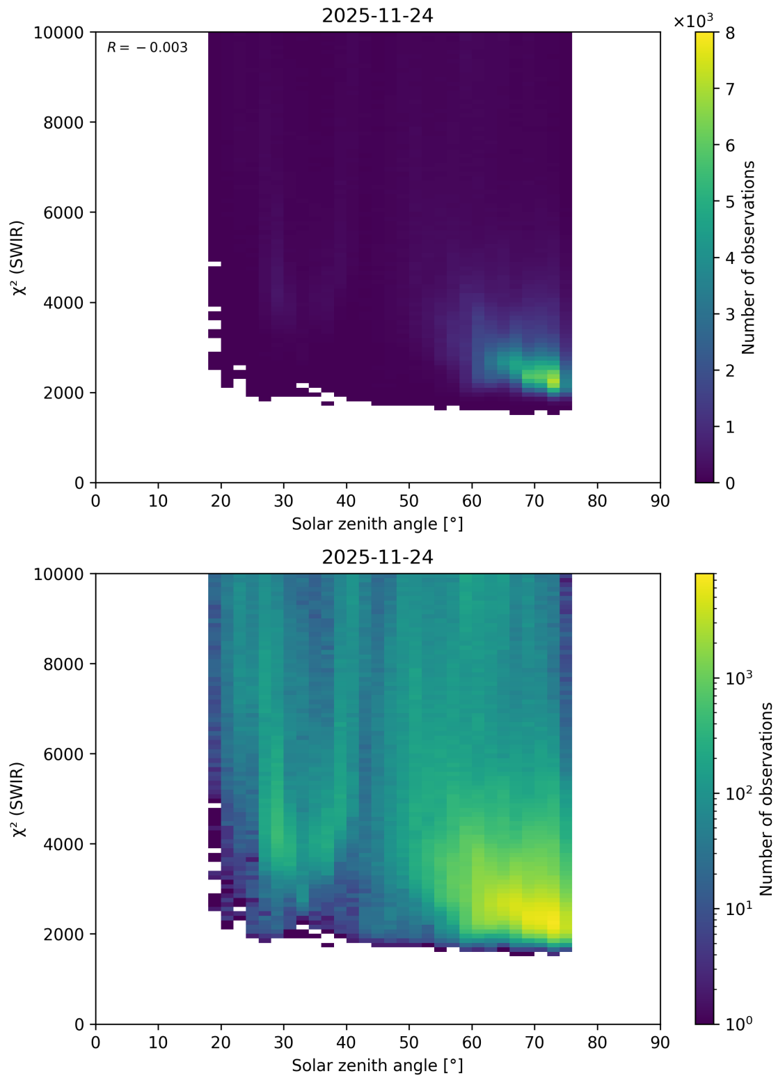
Figure 109: Scatter density plot of “Solar zenith angle” against “ \chi^2 (SWIR)” for 2025-11-23 to 2025-11-25.
