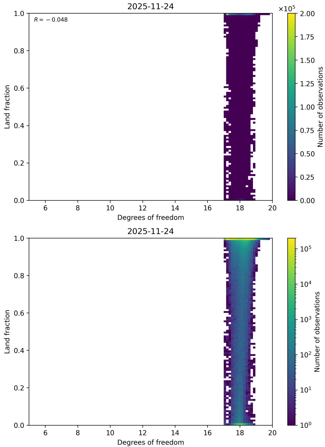
Figure 58: Scatter density plot of “Degrees of freedom” against “Land fraction” for 2025-11-23 to 2025-11-25.
