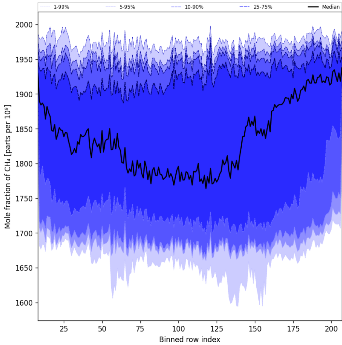
Figure 37: Along track statistics of “Mole fraction of CH 4 ” for 2025-11-23 to 2025-11-25
