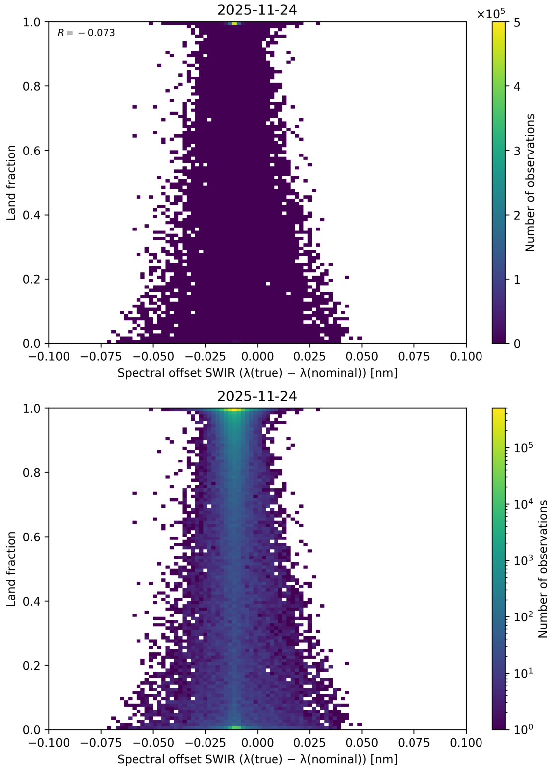
Figure 137: Scatter density plot of “Spectral offset SWIR ( \lambda_{\text{true}} - \lambda_{\text{nominal}} )” against “Land fraction” for 2025-11-23 to 2025-11-25.
