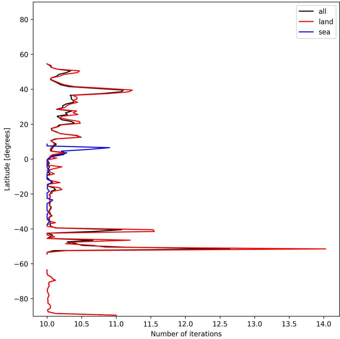
Figure 21: Zonal average of “Number of iterations” for 2025-11-23 to 2025-11-25.
