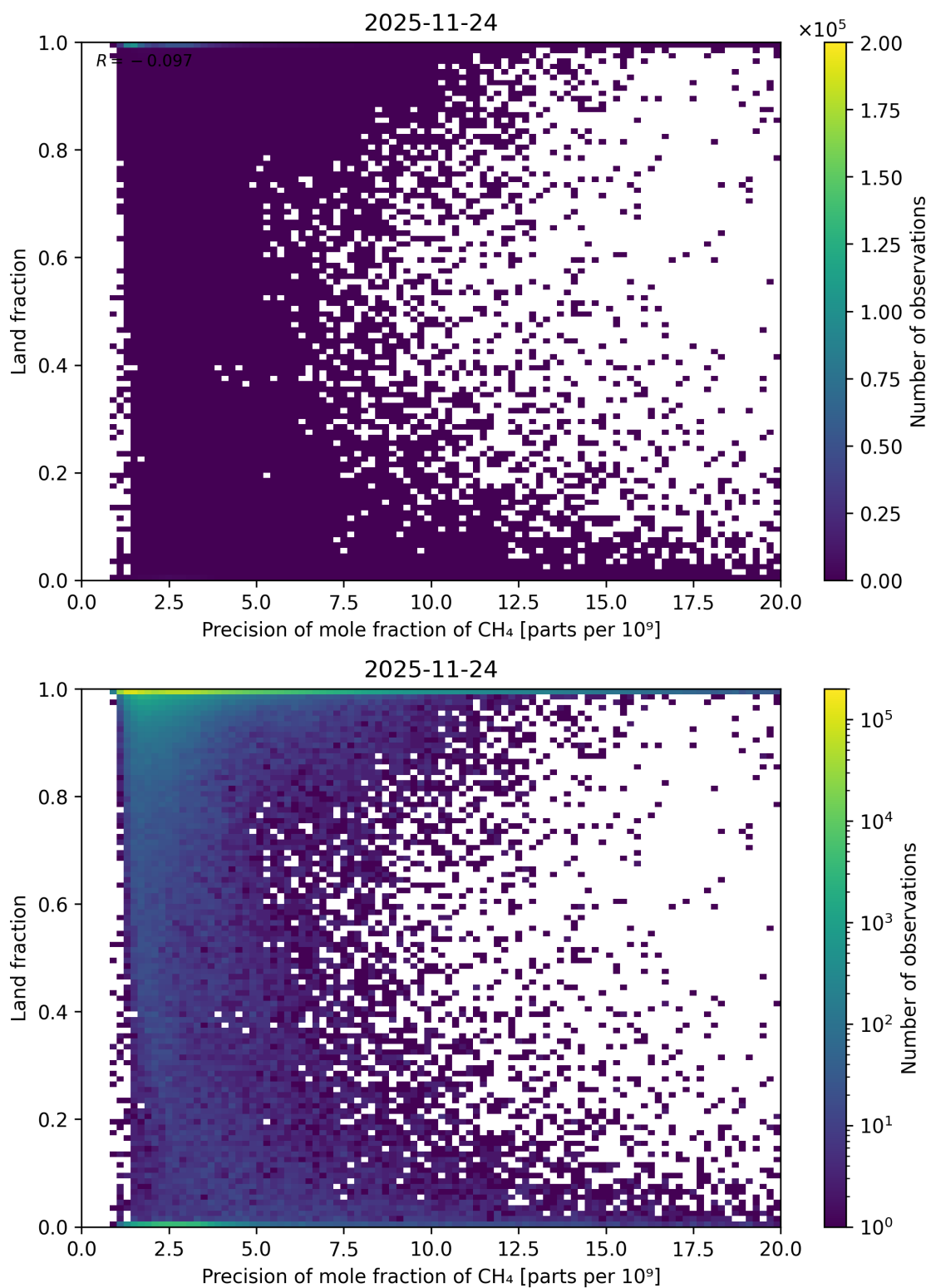
Figure 93: Scatter density plot of “Precision of mole fraction of CH 4 ” against “Land fraction” for 2025-11-23 to 2025-11-25.
