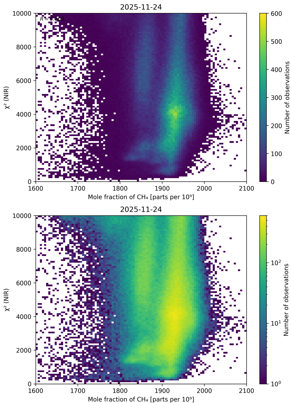
Figure 80: Scatter density plot of “Mole fraction of \text{CH}_4 ” against “ \chi^2 (NIR)” for 2025-11-23 to 2025-11-25.
