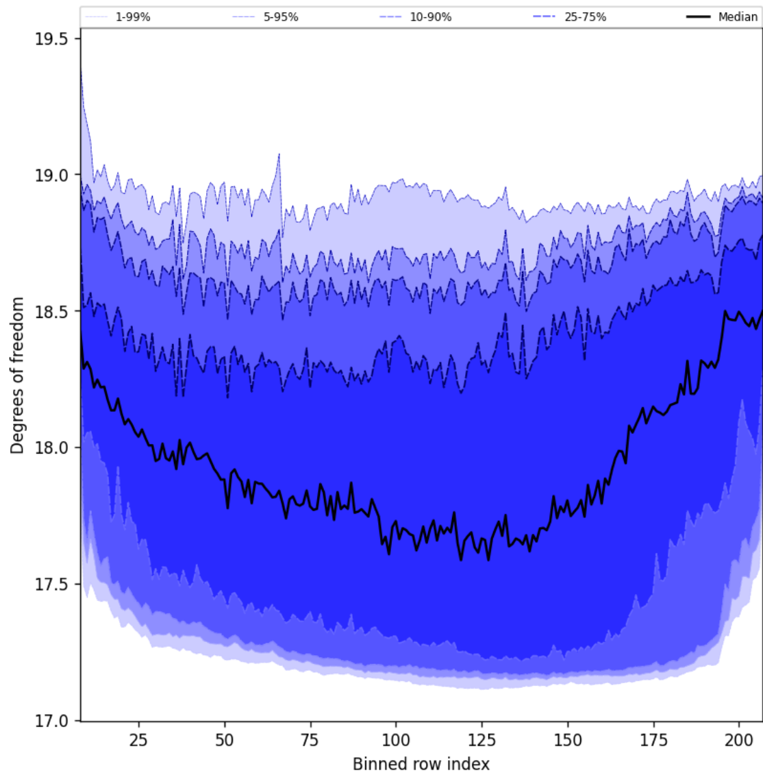
Figure 44: Along track statistics of “Degrees of freedom” for 2025-11-23 to 2025-11-25
