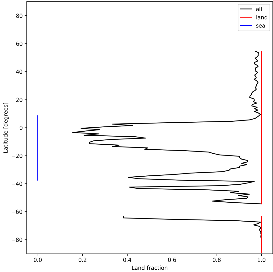
Figure 23: Zonal average of “Land fraction” for 2025-11-23 to 2025-11-25.
