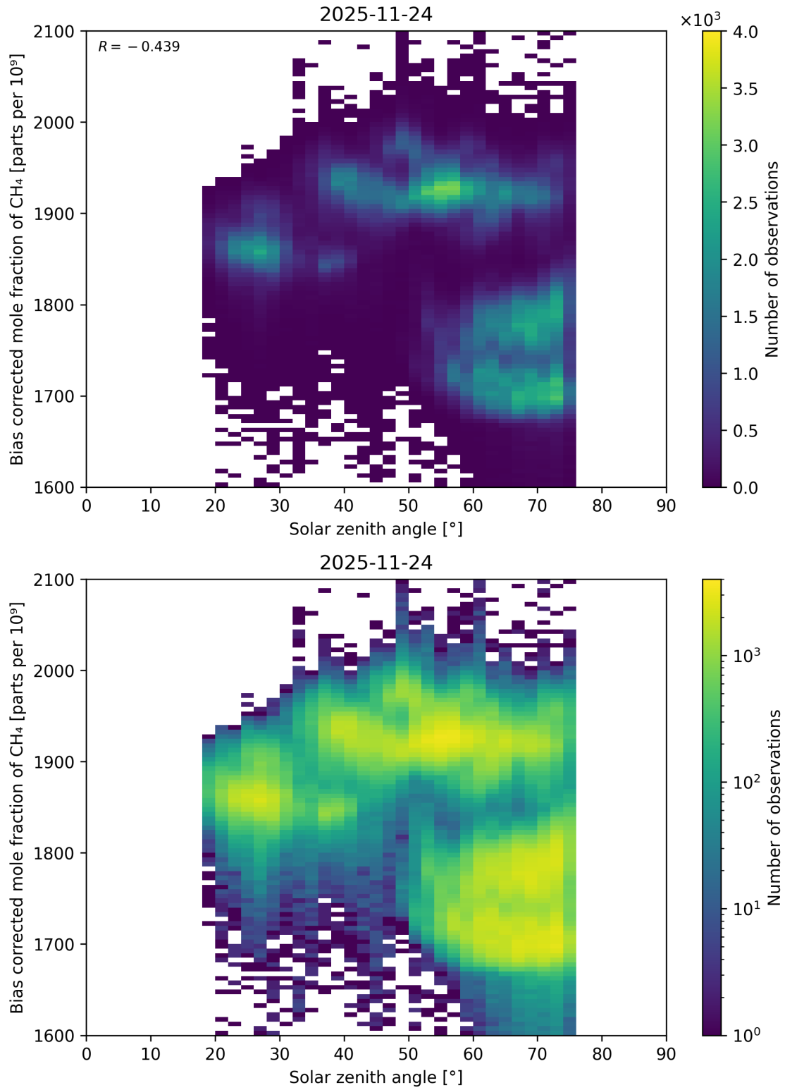
Figure 115: Scatter density plot of “Solar zenith angle” against “Bias corrected mole fraction of \text{CH}_4 ” for 2025-11-23 to 2025-11-25.
