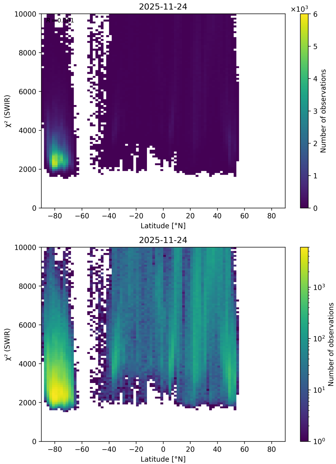
Figure 62: Scatter density plot of “Latitude” against “ \chi^2 (SWIR)” for 2025-11-23 to 2025-11-25.
