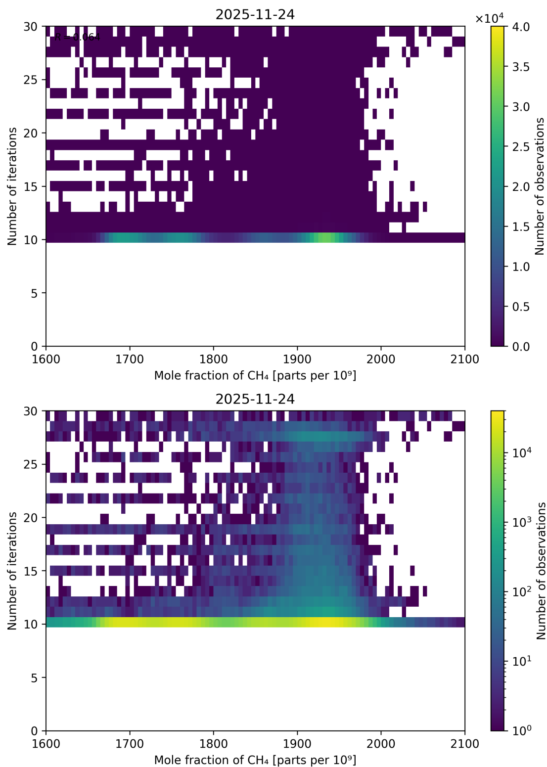
Figure 87: Scatter density plot of “Mole fraction of CH 4 ” against “Number of iterations” for 2025-11-23 to 2025-11-25.
