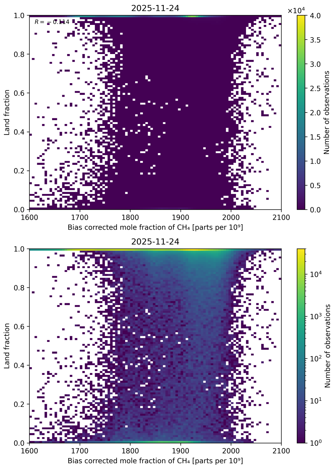
Figure 76: Scatter density plot of “Bias corrected mole fraction of CH 4 ” against “Land fraction” for 2025-11-23 to 2025-11-25.
