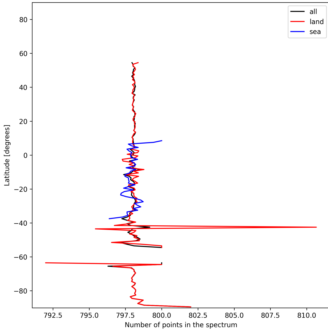
Figure 16: Zonal average of “Number of points in the spectrum” for 2025-11-23 to 2025-11-25.
