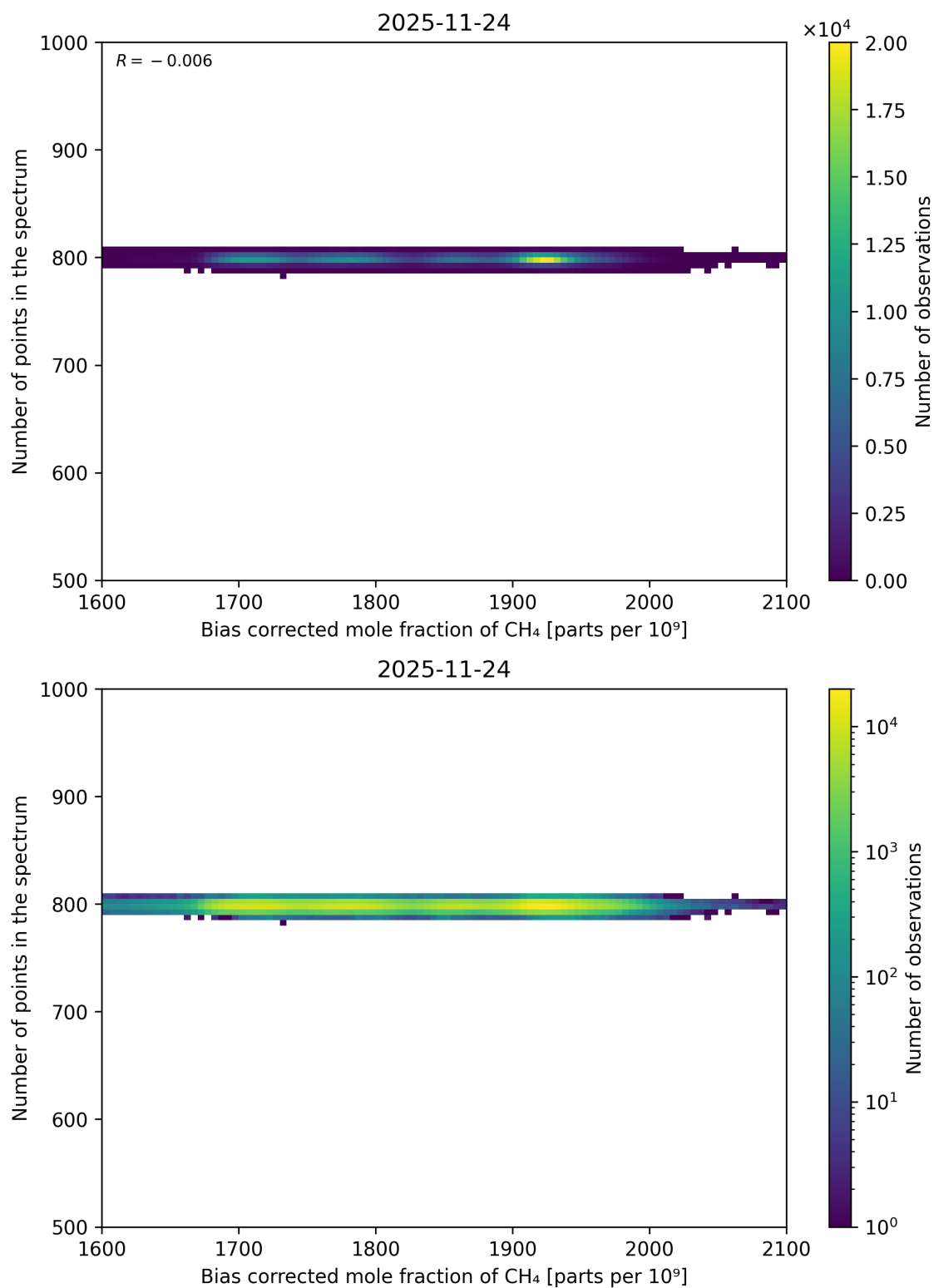
Figure 78: Scatter density plot of “Bias corrected mole fraction of CH 4 ” against “Number of points in the spectrum” for 2025-11-23 to 2025-11-25.
