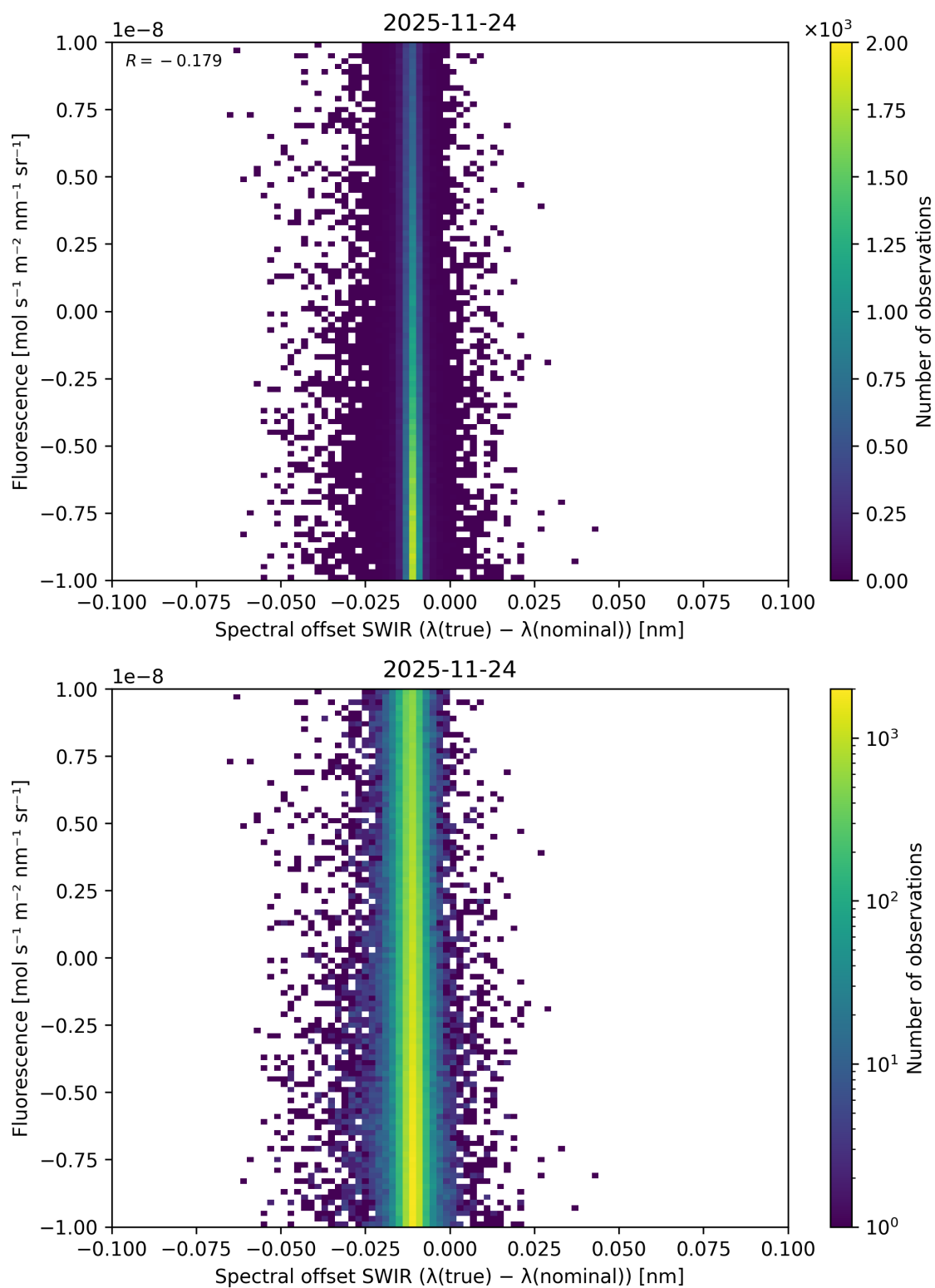
Figure 136: Scatter density plot of “Spectral offset SWIR ( \lambda_{\text{true}} - \lambda_{\text{nominal}} )” against “Fluorescence” for 2025-11-23 to 2025-11-25.
