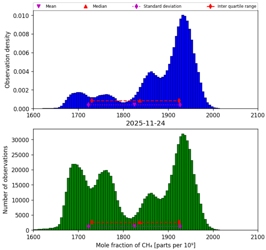
Figure 25: Histogram of “Mole fraction of CH 4 ” for 2025-11-23 to 2025-11-25
