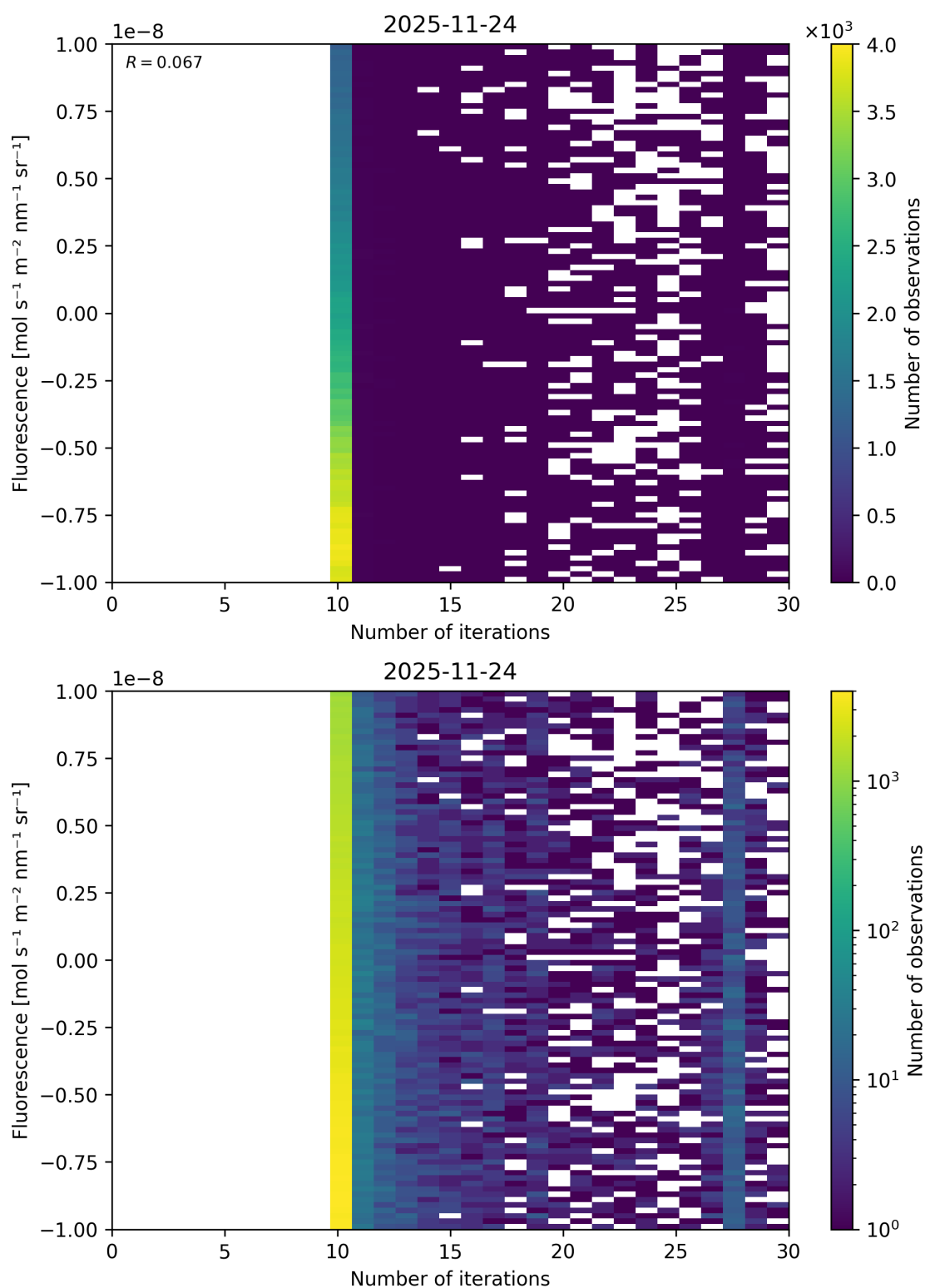
Figure 99: Scatter density plot of “Number of iterations” against “Fluorescence” for 2025-11-23 to 2025-11-25.
