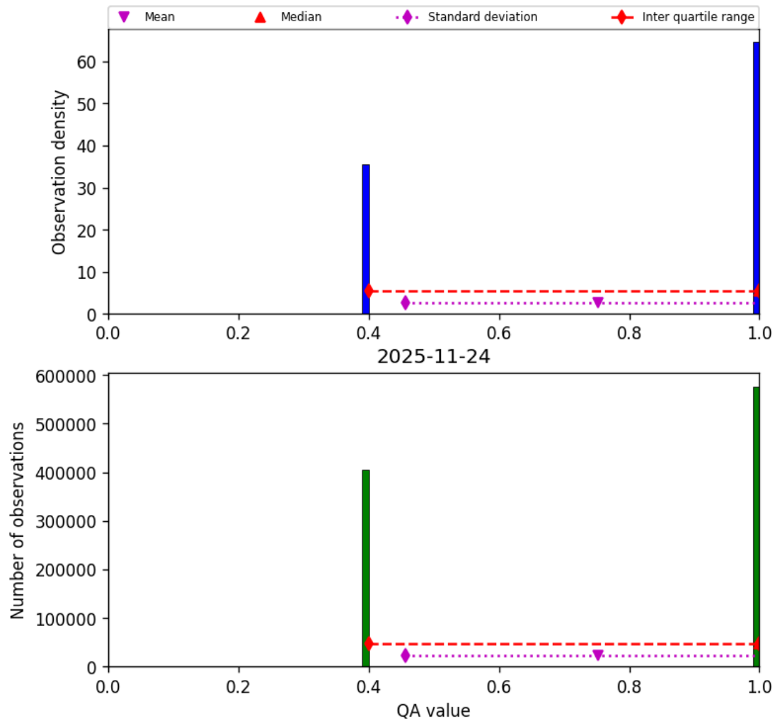
Figure 24: Histogram of “QA value” for 2025-11-23 to 2025-11-25
