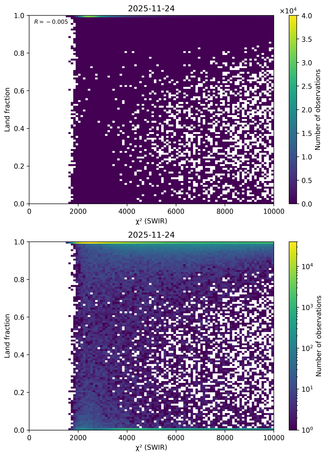
Figure 55: Scatter density plot of “ \chi^2 (SWIR)” against “Land fraction” for 2025-11-23 to 2025-11-25.
