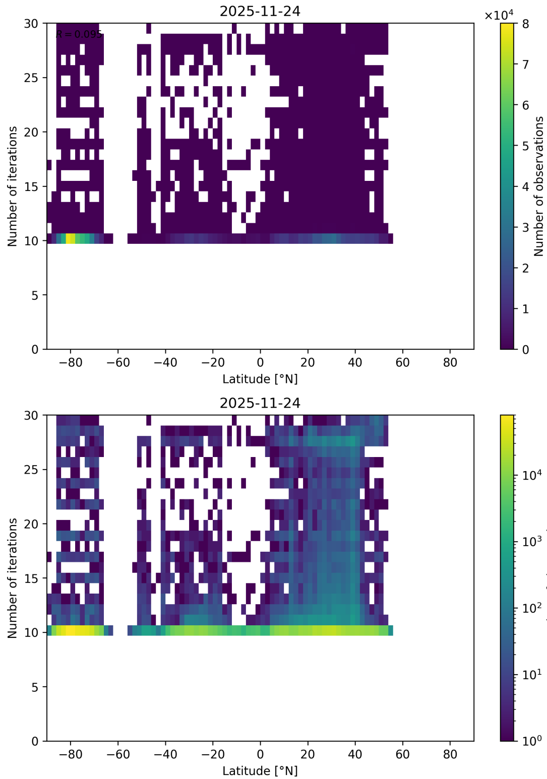
Figure 69: Scatter density plot of “Latitude” against “Number of iterations” for 2025-11-23 to 2025-11-25.
