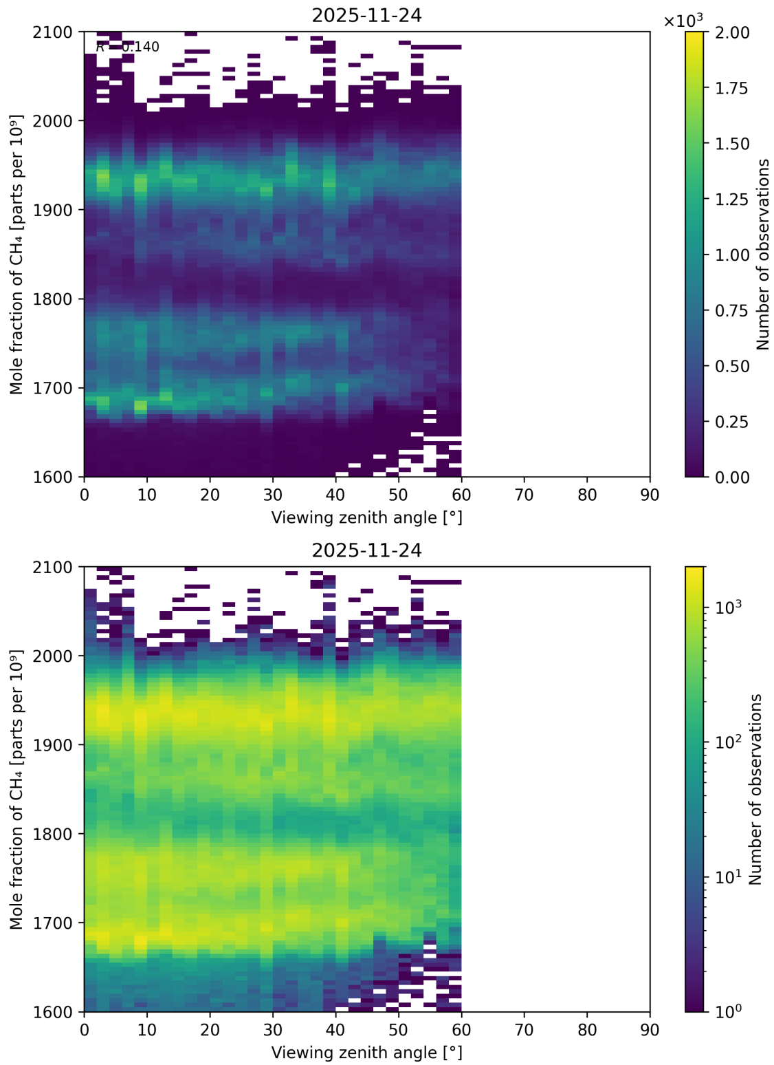
Figure 126: Scatter density plot of “Viewing zenith angle” against “Mole fraction of CH 4 ” for 2025-11-23 to 2025-11-25.
