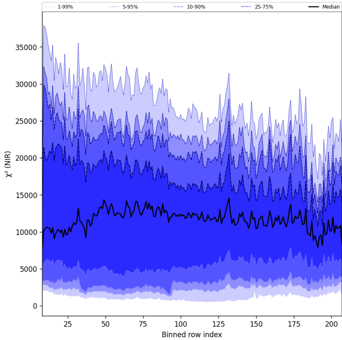
Figure 43: Along track statistics of “ \chi^2 (NIR)” for 2025-11-23 to 2025-11-25
