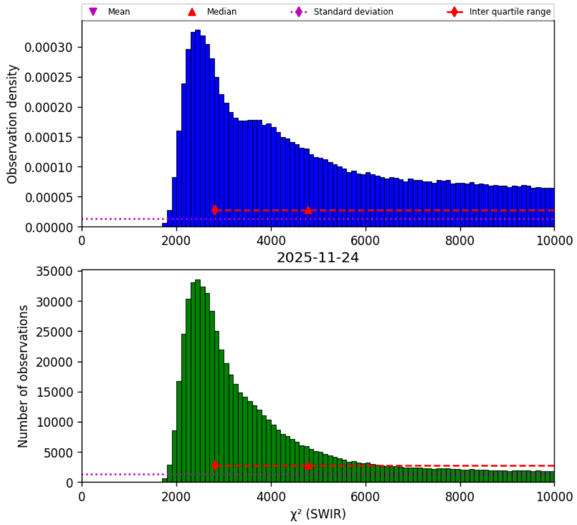
Figure 30: Histogram of " \chi^2 (SWIR)" for 2025-11-23 to 2025-11-25
