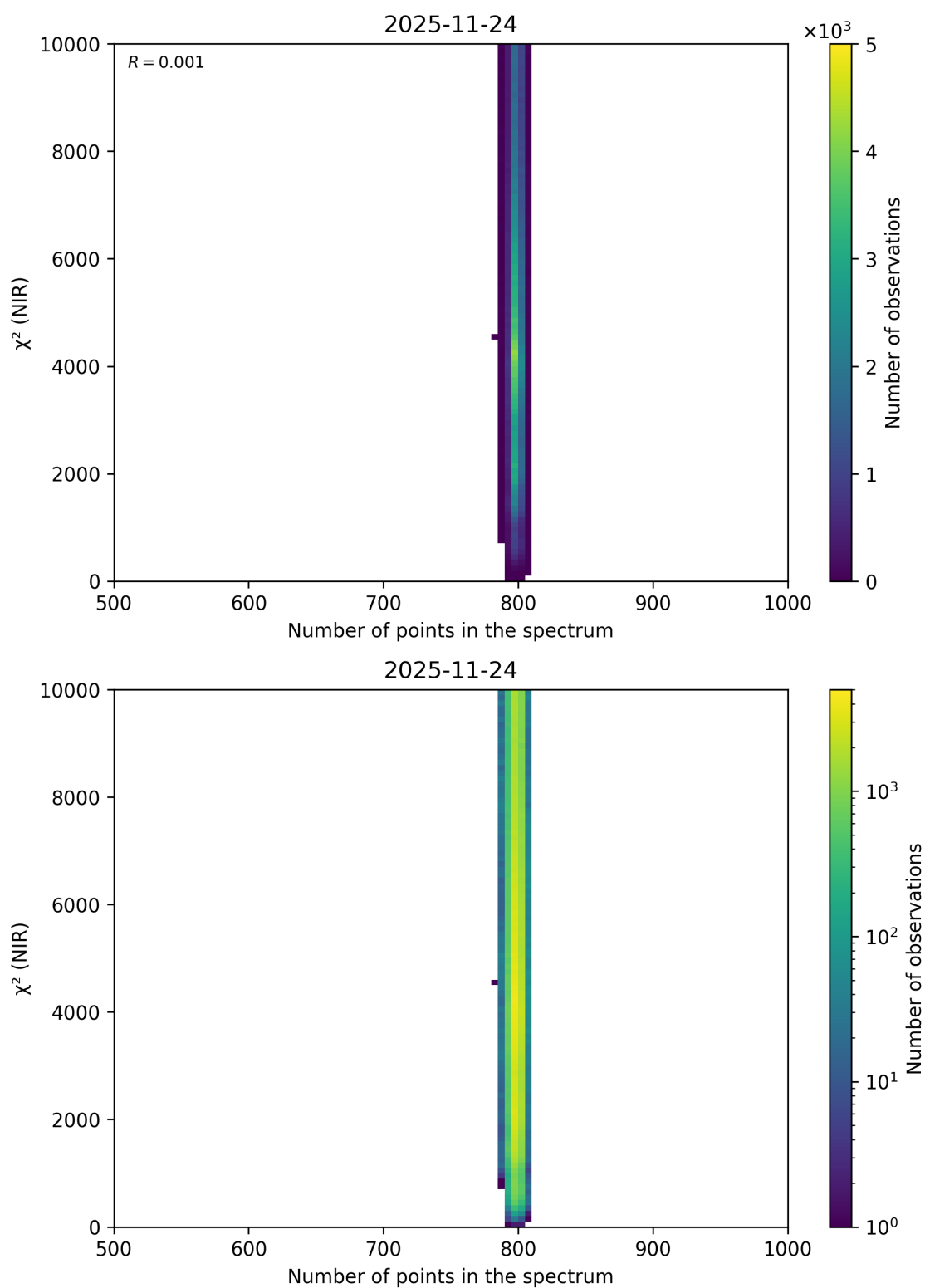
Figure 101: Scatter density plot of “Number of points in the spectrum” against “ \chi^2 (NIR)” for 2025-11-23 to 2025-11-25.
