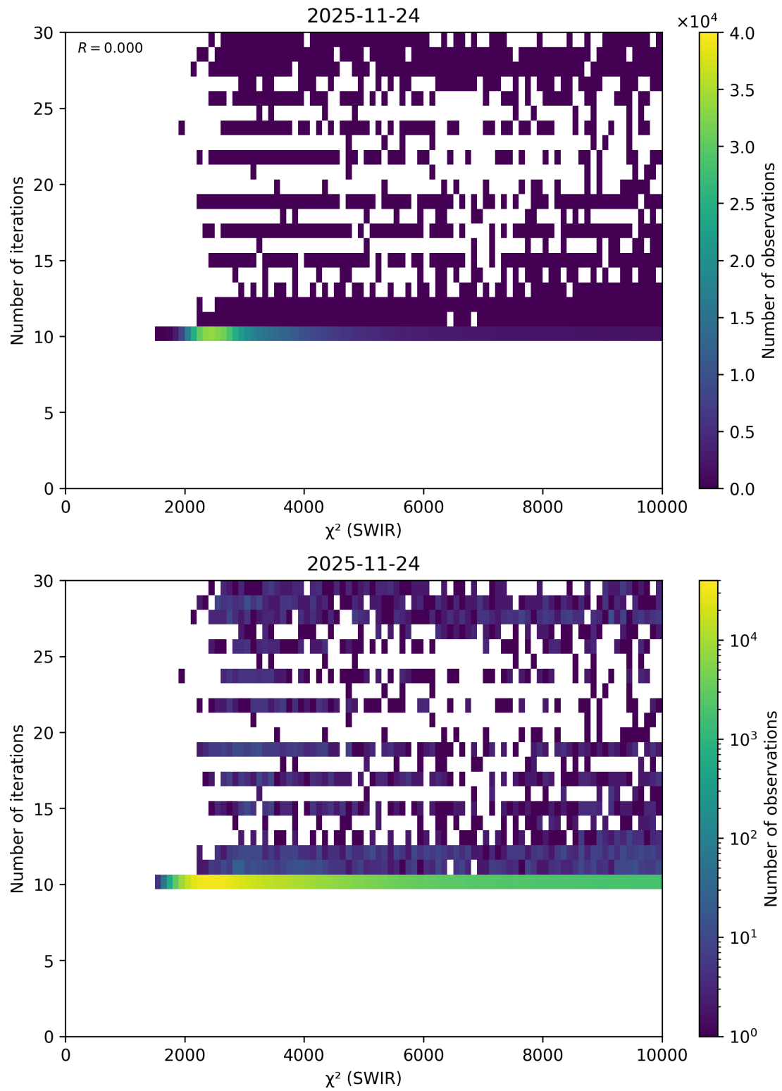
Figure 56: Scatter density plot of “ \chi^2 (SWIR)” against “Number of iterations” for 2025-11-23 to 2025-11-25.
