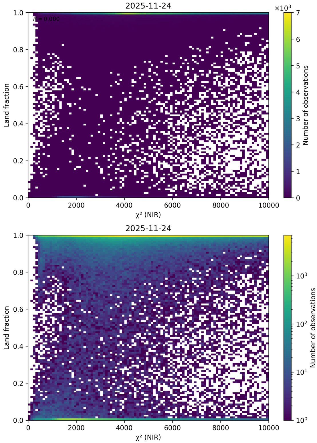
Figure 50: Scatter density plot of “ \chi^2 (NIR)” against “Land fraction” for 2025-11-23 to 2025-11-25.
