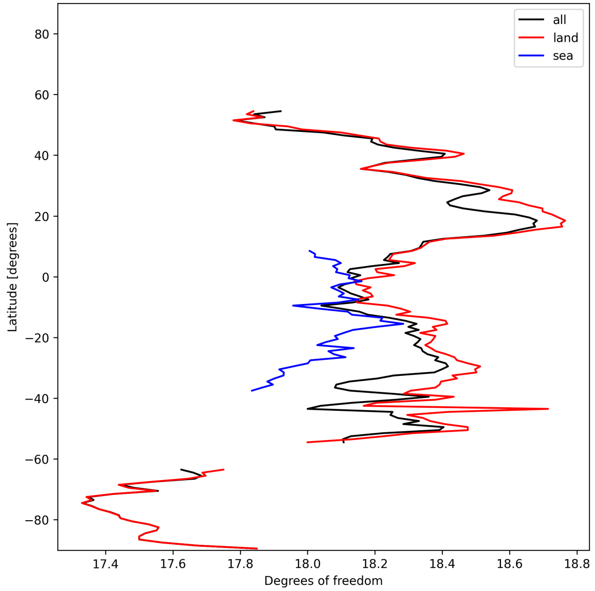
Figure 20: Zonal average of “Degrees of freedom” for 2025-11-23 to 2025-11-25.
