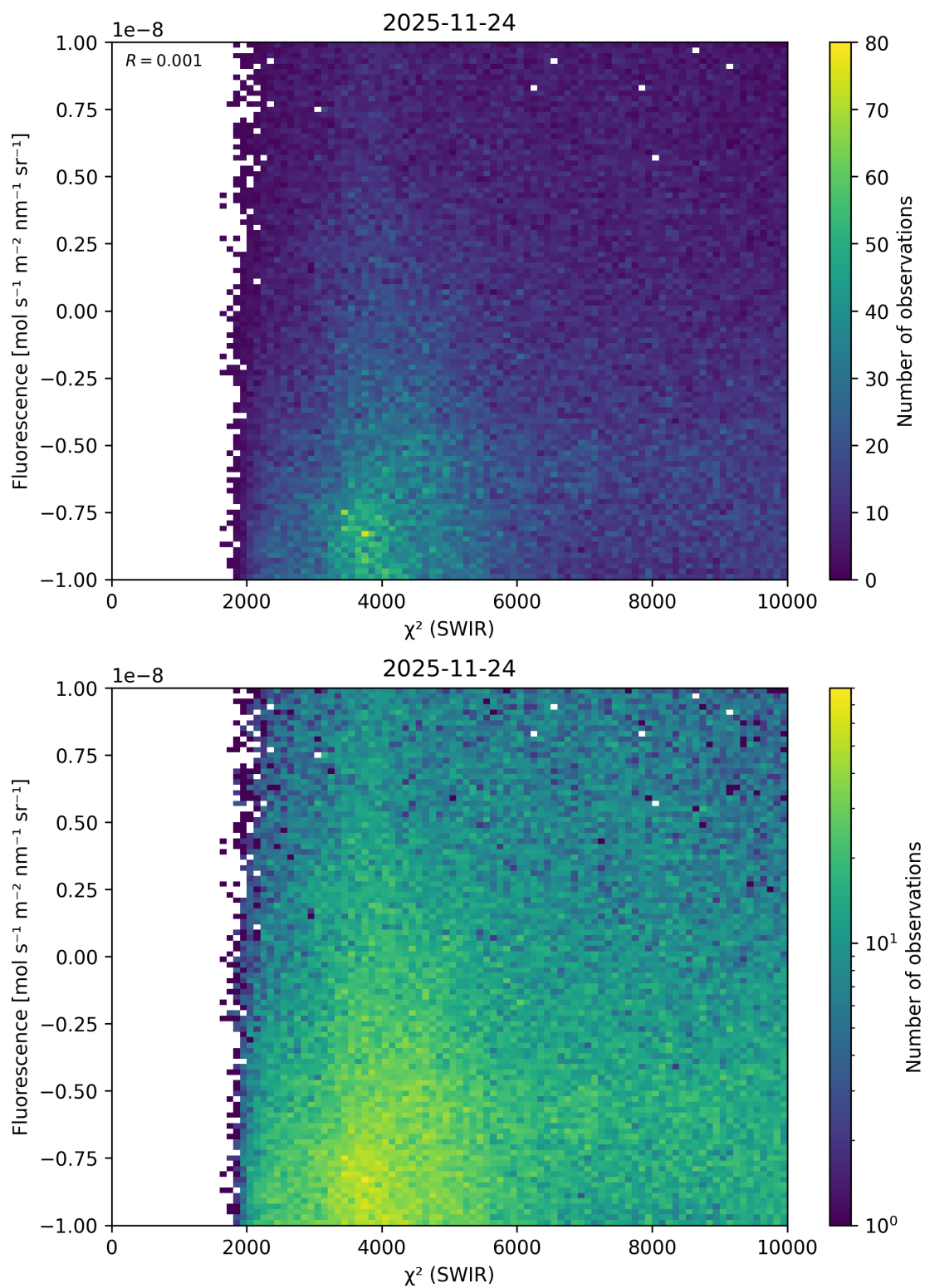
Figure 54: Scatter density plot of “ \chi^2 (SWIR)” against “Fluorescence” for 2025-11-23 to 2025-11-25.
