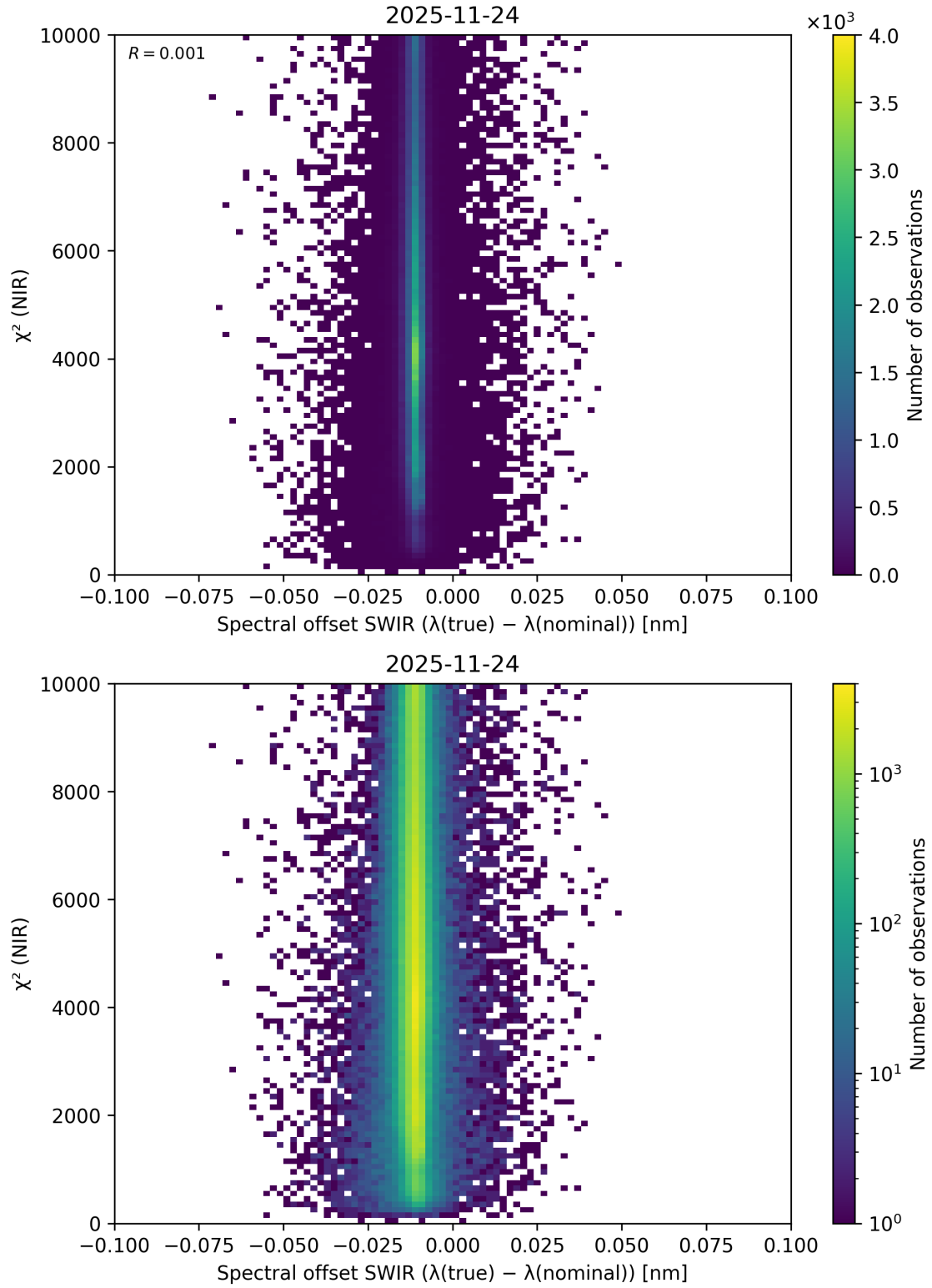
Figure 133: Scatter density plot of “Spectral offset SWIR ( \lambda_{\text{true}} - \lambda_{\text{nominal}} )” against “ \chi^2 (NIR)” for 2025-11-23 to 2025-11-25.
