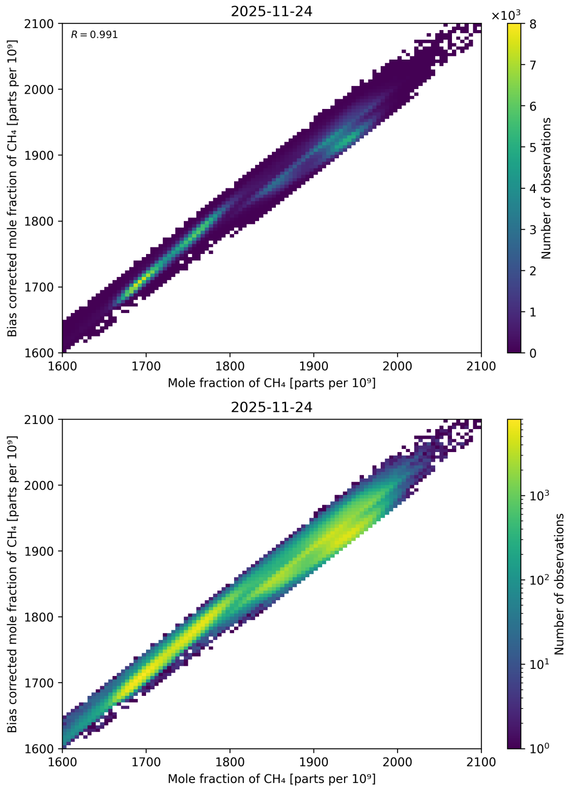
Figure 85: Scatter density plot of “Mole fraction of CH 4 ” against “Bias corrected mole fraction of CH 4 ” for 2025-11-23 to 2025-11-25.
