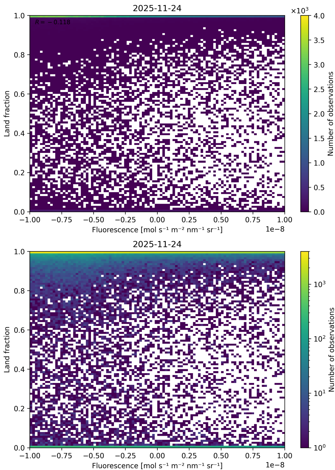
Figure 60: Scatter density plot of “Fluorescence” against “Land fraction” for 2025-11-23 to 2025-11-25.
