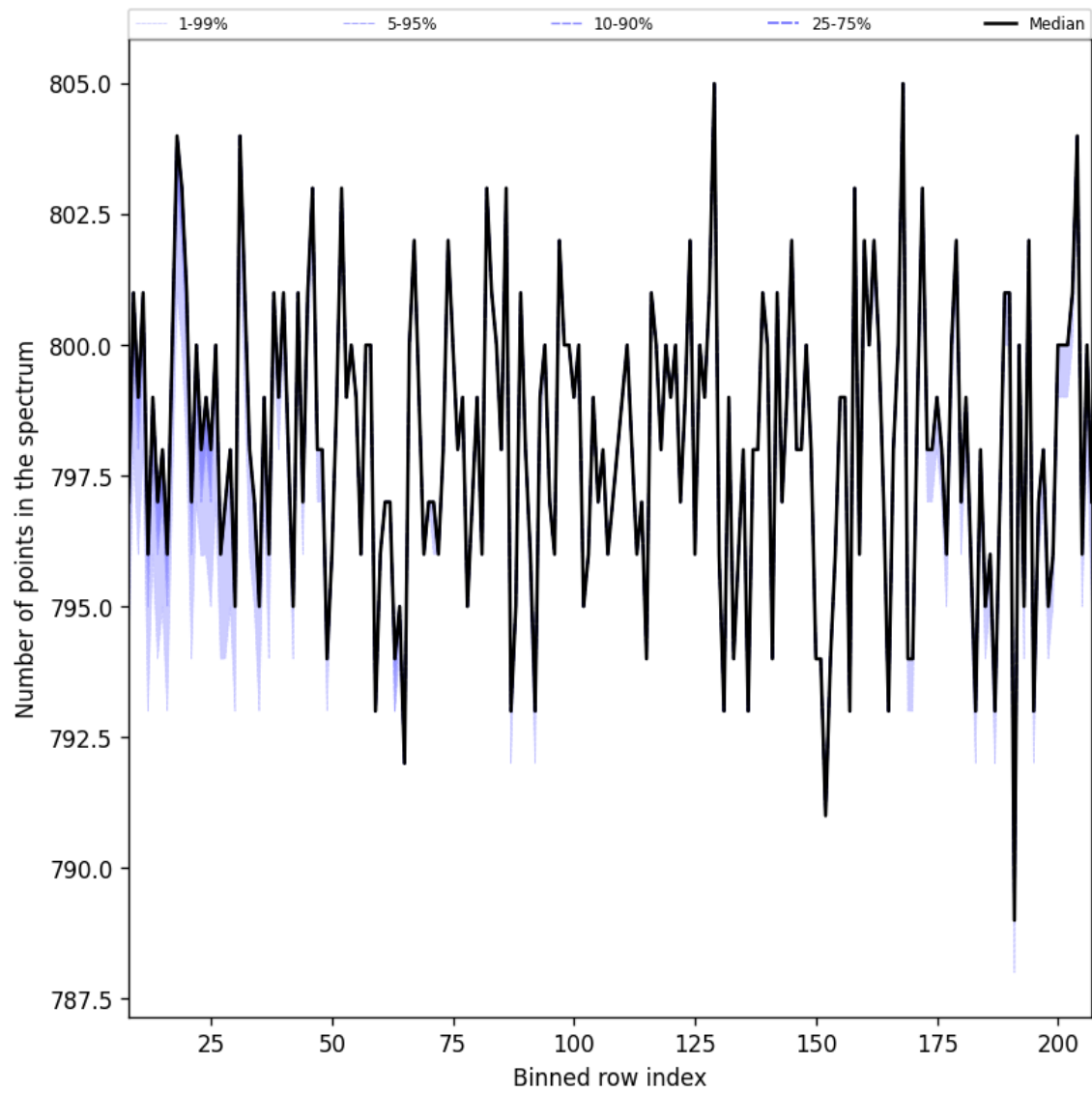
Figure 40: Along track statistics of “Number of points in the spectrum” for 2025-11-23 to 2025-11-25
