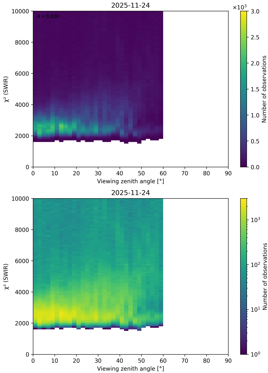
Figure 121: Scatter density plot of “Viewing zenith angle” against “ \chi^2 (SWIR)” for 2025-11-23 to 2025-11-25.
