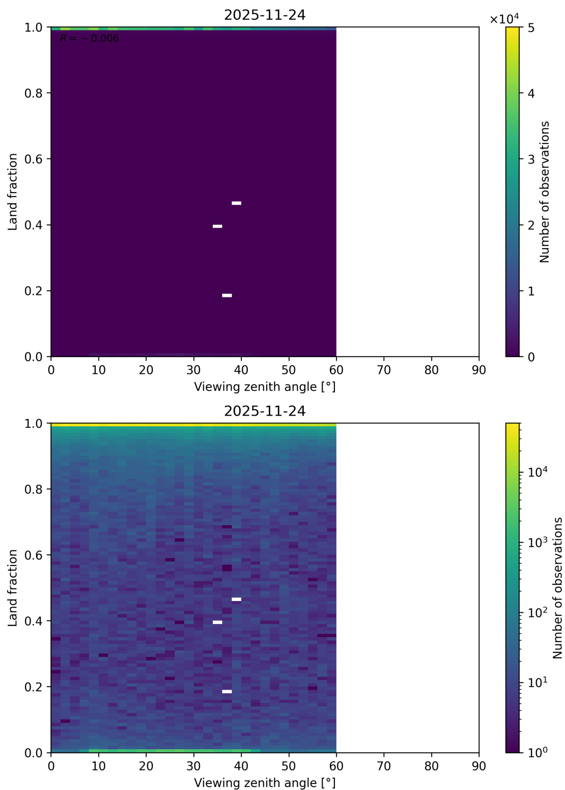
Figure 124: Scatter density plot of “Viewing zenith angle” against “Land fraction” for 2025-11-23 to 2025-11-25.
