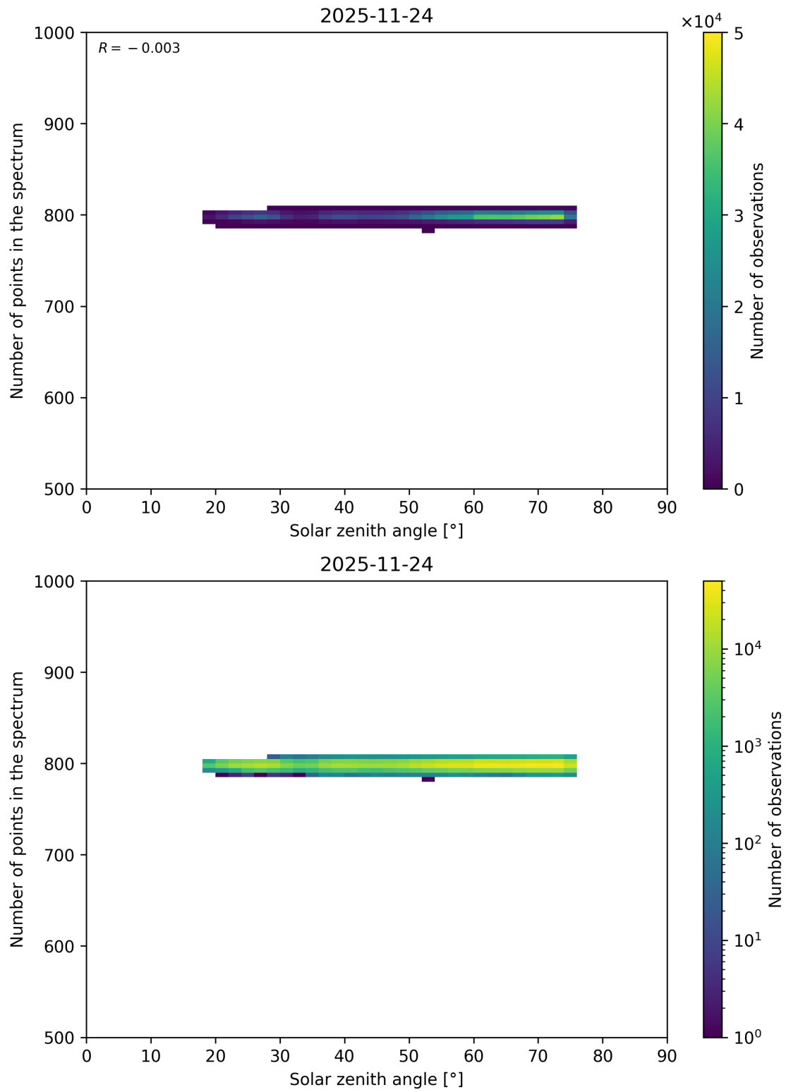
Figure 118: Scatter density plot of “Solar zenith angle” against “Number of points in the spectrum” for 2025-11-23 to 2025-11-25.
