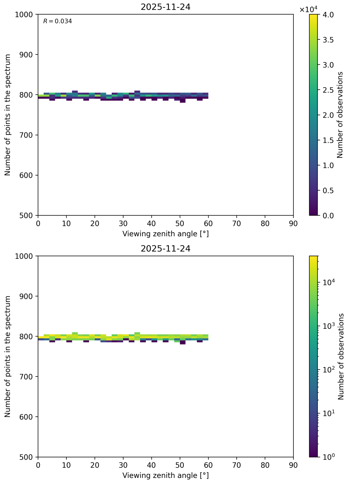
Figure 130: Scatter density plot of “Viewing zenith angle” against “Number of points in the spectrum” for 2025-11-23 to 2025-11-25.
