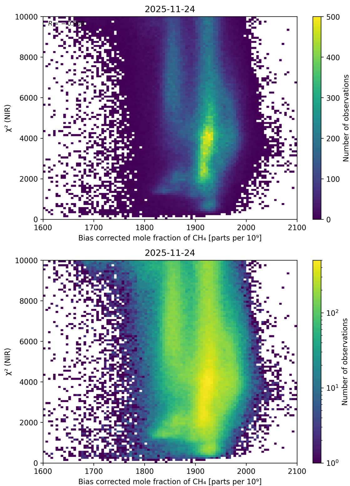
Figure 72: Scatter density plot of “Bias corrected mole fraction of \text{CH}_4 ” against “ \chi^2 (NIR)” for 2025-11-23 to 2025-11-25.
