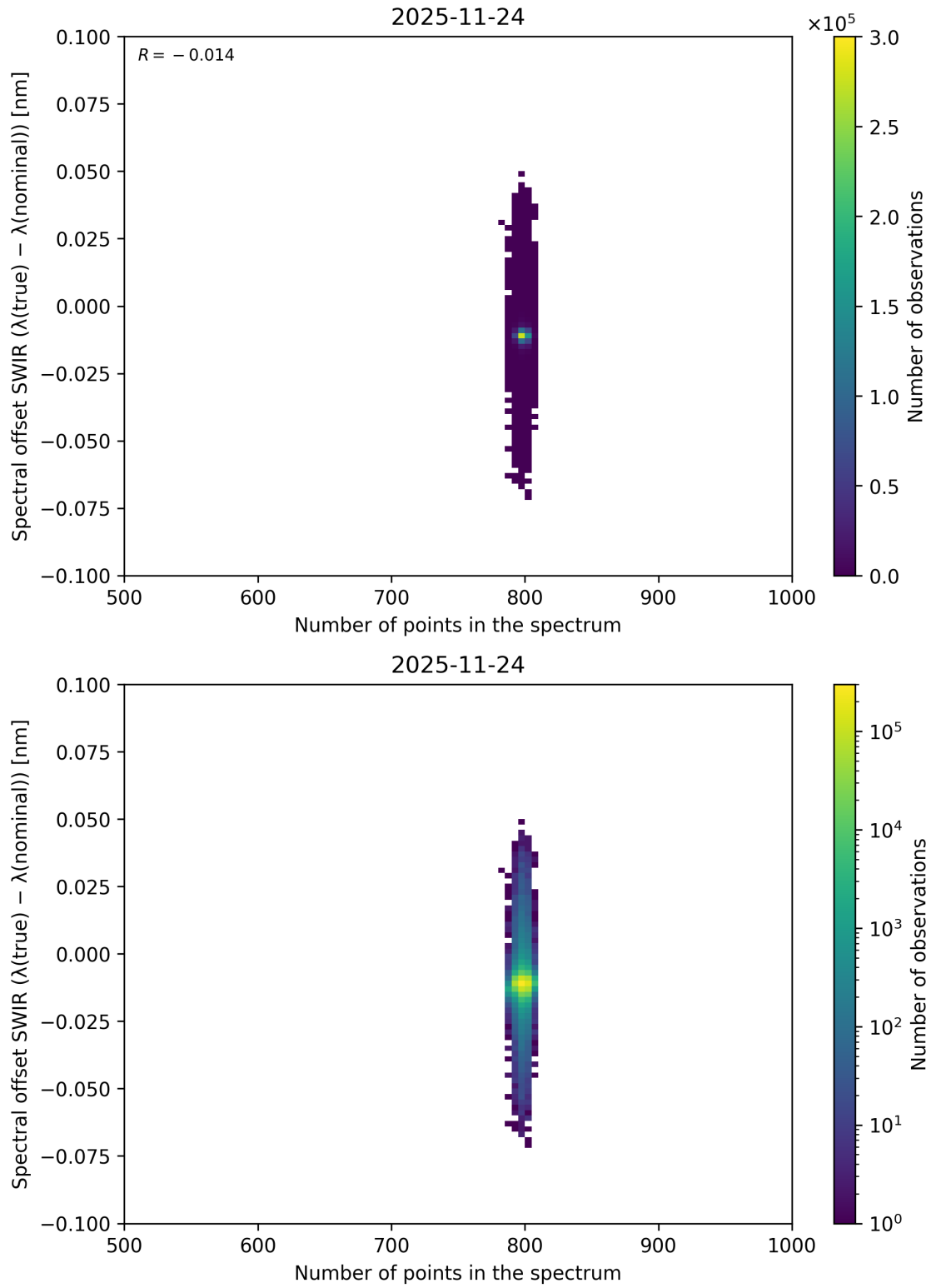
Figure 107: Scatter density plot of “Number of points in the spectrum” against “Spectral offset SWIR ( \lambda_{\text{true}} - \lambda_{\text{nominal}} )” for 2025-11-23 to 2025-11-25.
