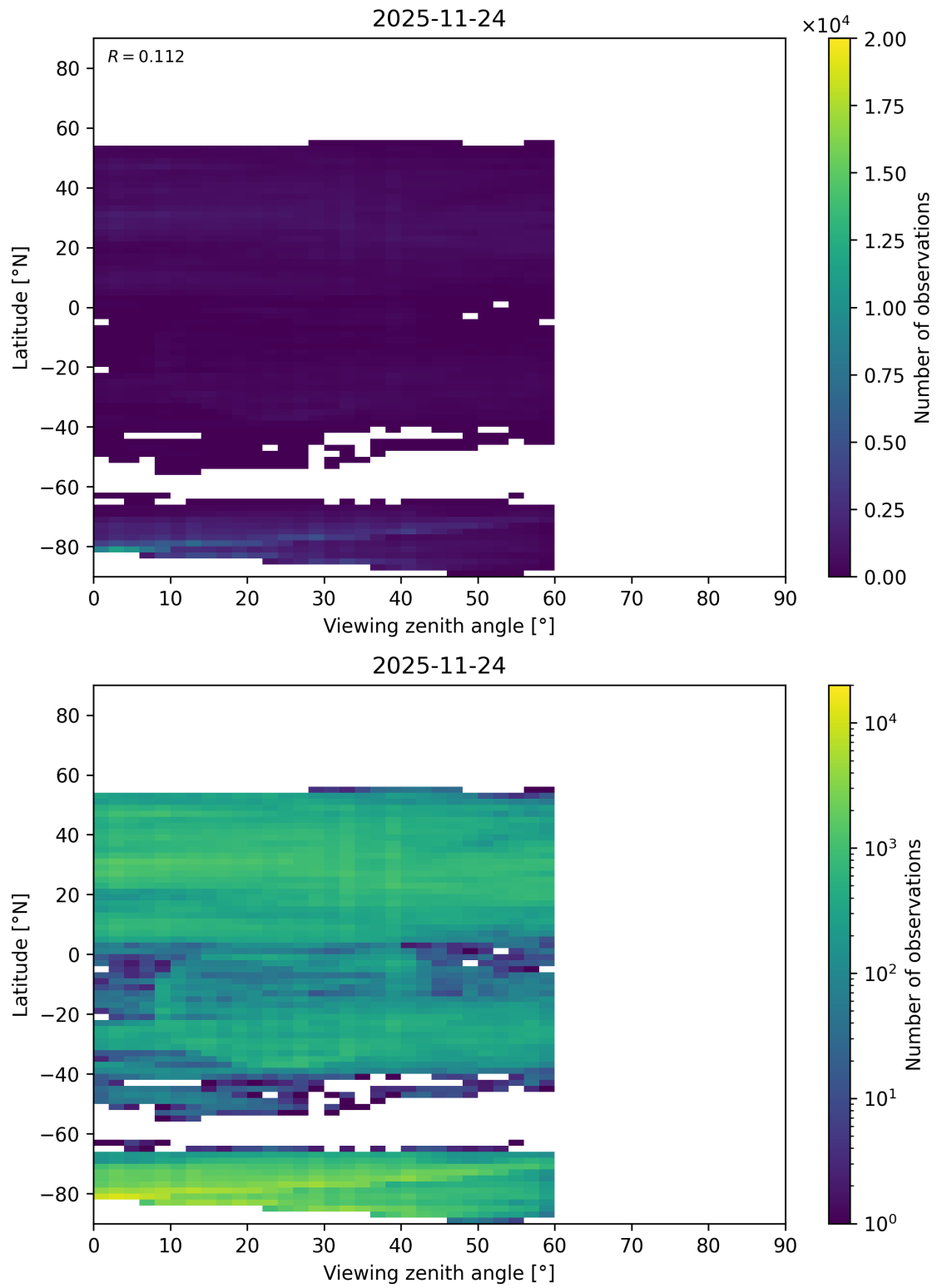
Figure 125: Scatter density plot of “Viewing zenith angle” against “Latitude” for 2025-11-23 to 2025-11-25.
