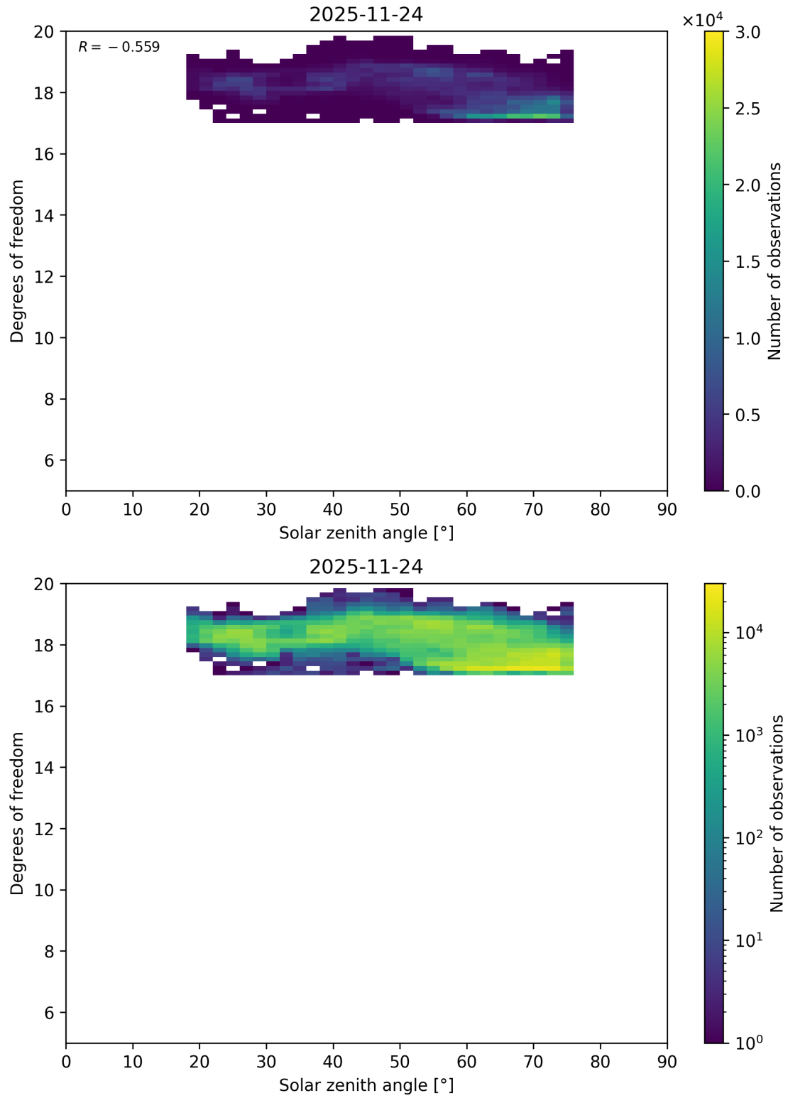
Figure 110: Scatter density plot of “Solar zenith angle” against “Degrees of freedom” for 2025-11-23 to 2025-11-25.
