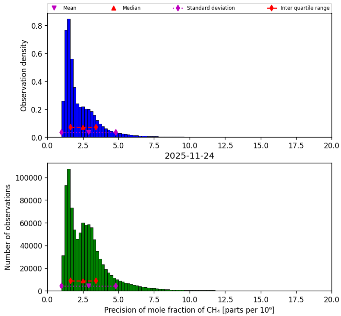
Figure 26: Histogram of “Precision of mole fraction of CH 4 ” for 2025-11-23 to 2025-11-25
