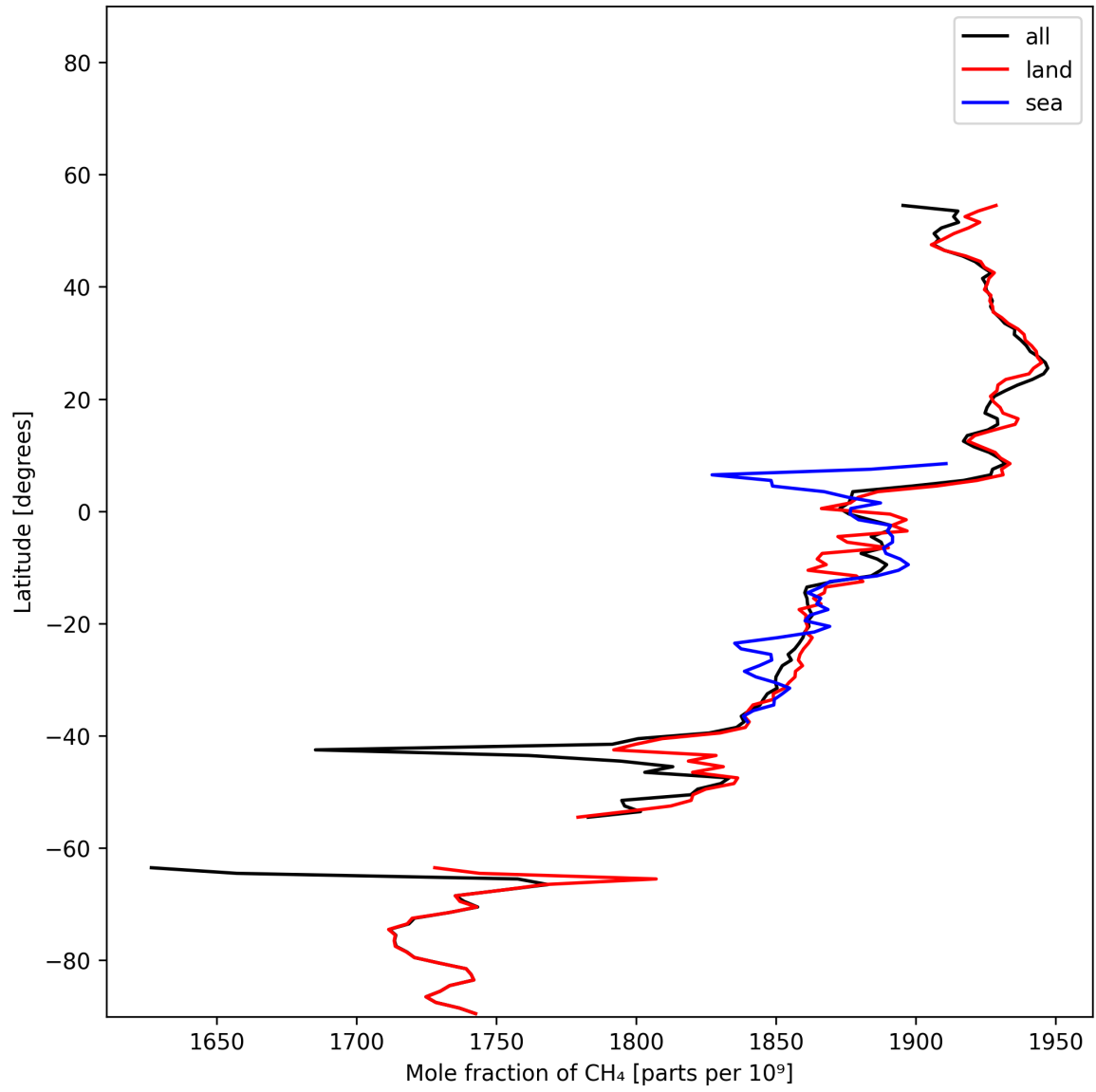
Figure 13: Zonal average of “Mole fraction of CH 4 ” for 2025-11-23 to 2025-11-25.
