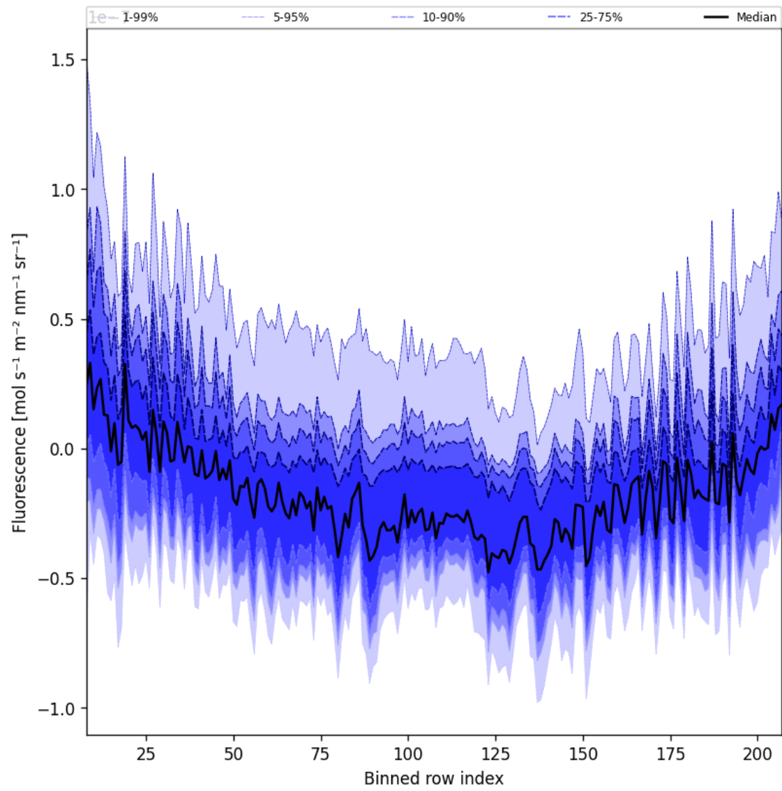
Figure 46: Along track statistics of “Fluorescence” for 2025-11-23 to 2025-11-25
