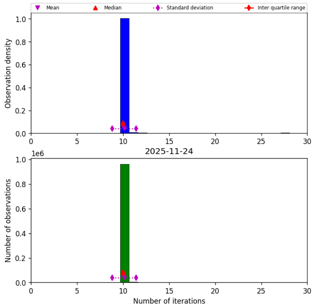
Figure 33: Histogram of “Number of iterations” for 2025-11-23 to 2025-11-25
