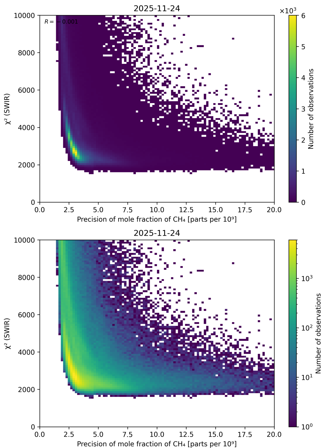
Figure 90: Scatter density plot of “Precision of mole fraction of \text{CH}_4 ” against “ \chi^2 (SWIR)” for 2025-11-23 to 2025-11-25.
