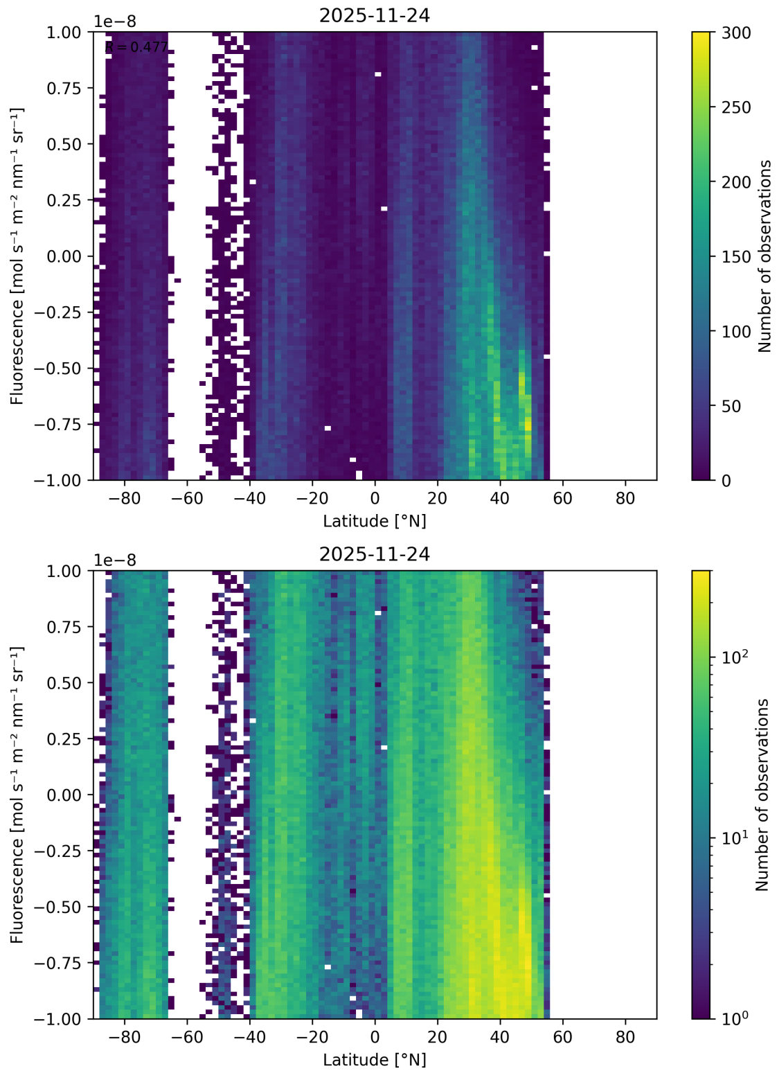
Figure 64: Scatter density plot of “Latitude” against “Fluorescence” for 2025-11-23 to 2025-11-25.
