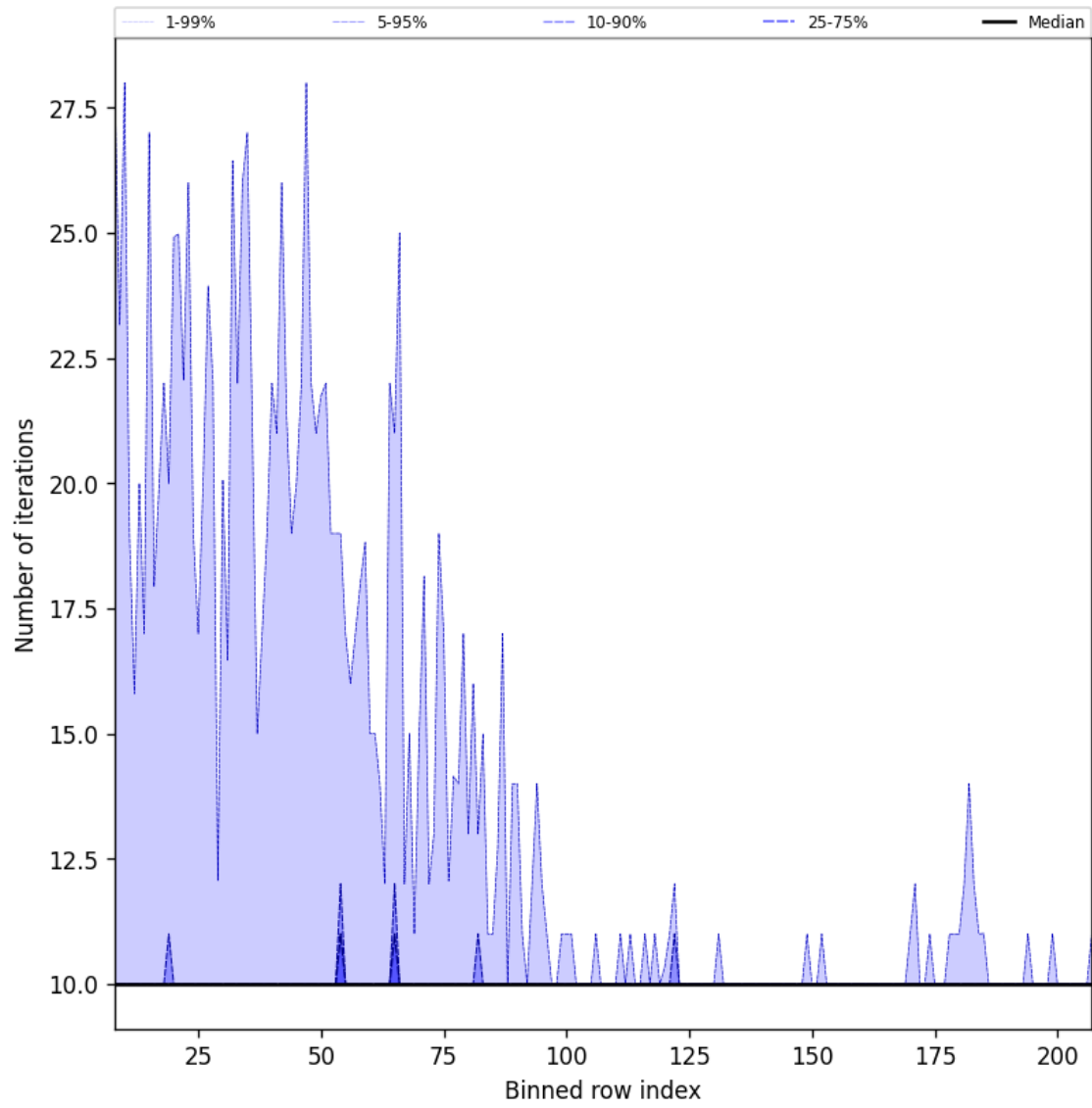
Figure 45: Along track statistics of “Number of iterations” for 2025-11-23 to 2025-11-25
