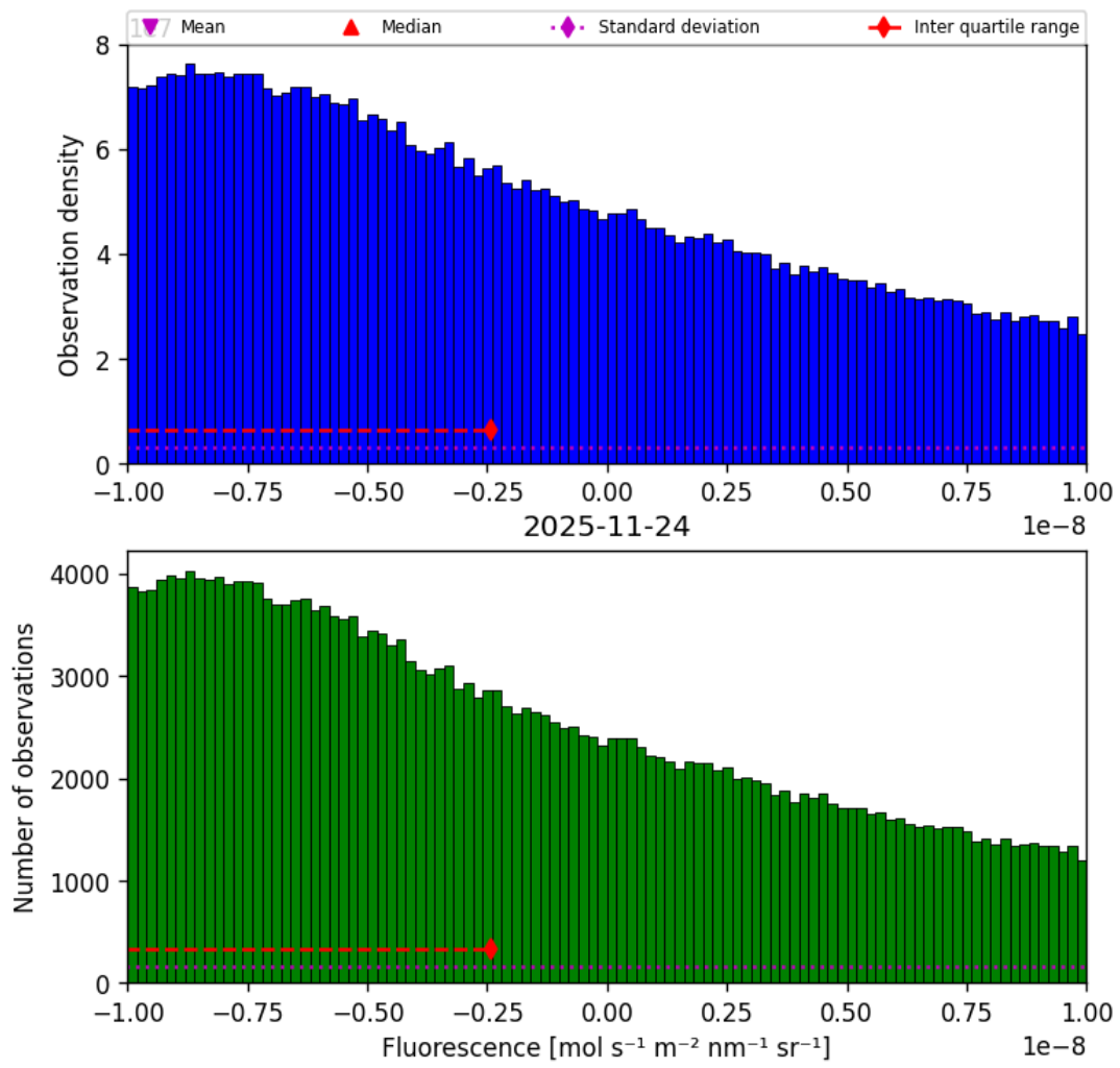
Figure 34: Histogram of “Fluorescence” for 2025-11-23 to 2025-11-25
