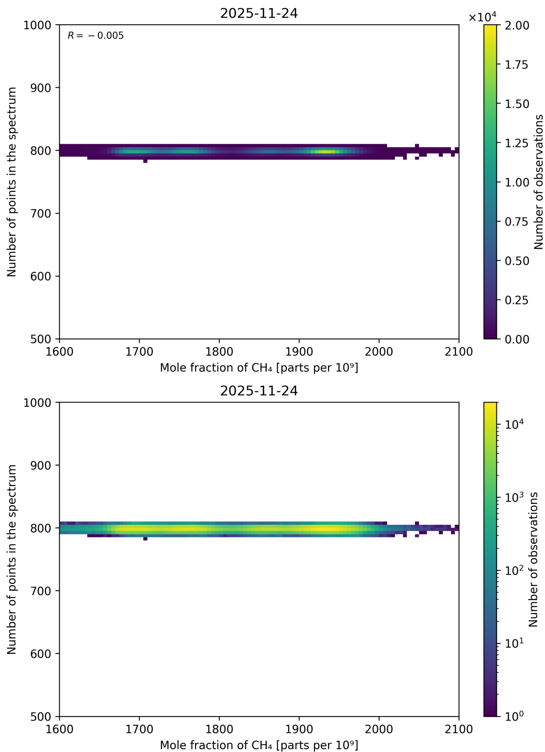
Figure 88: Scatter density plot of “Mole fraction of CH 4 ” against “Number of points in the spectrum” for 2025-11-23 to 2025-11-25.
