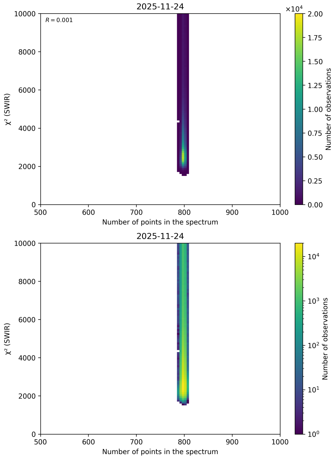
Figure 102: Scatter density plot of “Number of points in the spectrum” against “ \chi^2 (SWIR)” for 2025-11-23 to 2025-11-25.
