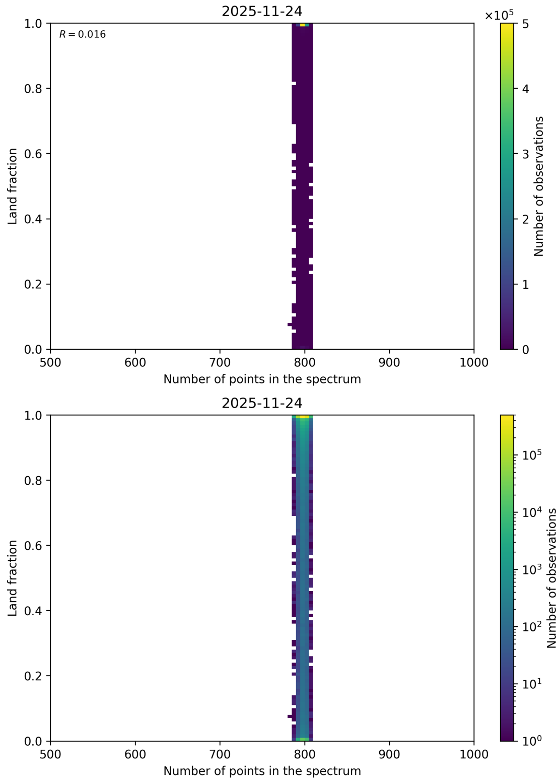
Figure 105: Scatter density plot of “Number of points in the spectrum” against “Land fraction” for 2025-11-23 to 2025-11-25.
