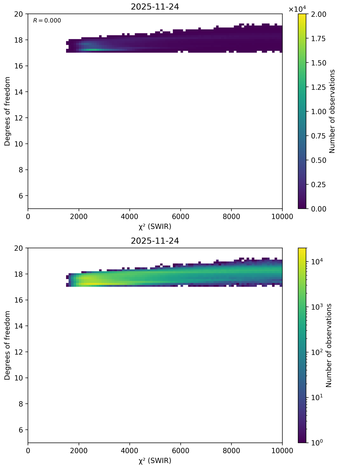
Figure 53: Scatter density plot of “ \chi^2 (SWIR)” against “Degrees of freedom” for 2025-11-23 to 2025-11-25.
