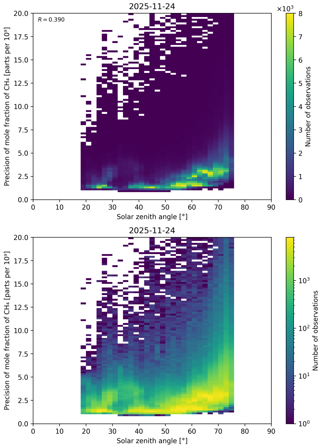
Figure 116: Scatter density plot of “Solar zenith angle” against “Precision of mole fraction of \text{CH}_4 ” for 2025-11-23 to 2025-11-25.
