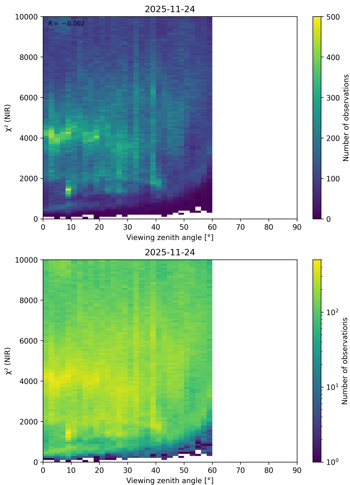
Figure 120: Scatter density plot of “Viewing zenith angle” against “ \chi^2 (NIR)” for 2025-11-23 to 2025-11-25.
