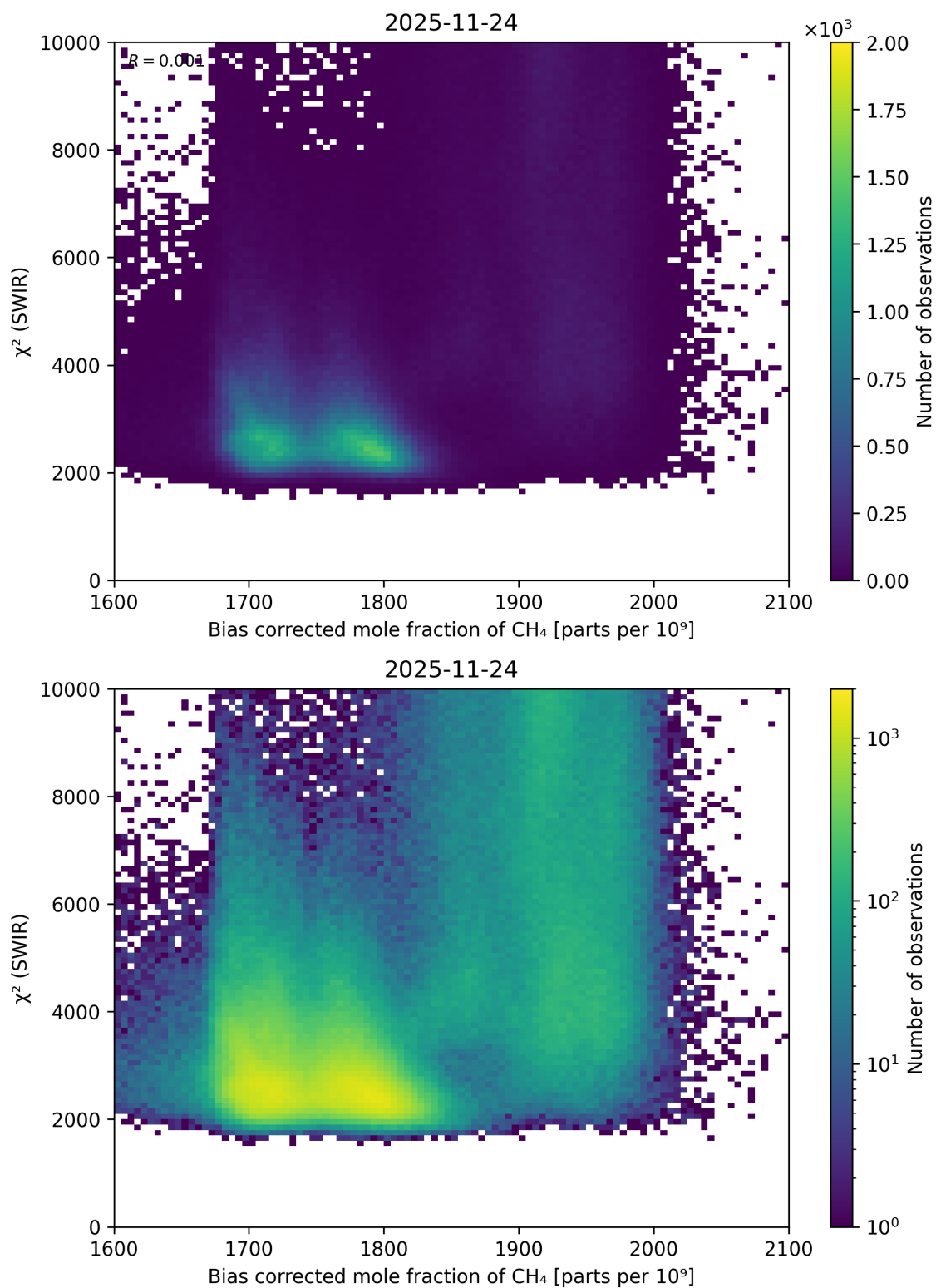
Figure 73: Scatter density plot of “Bias corrected mole fraction of CH 4 ” against “ \chi^2 (SWIR)” for 2025-11-23 to 2025-11-25.
