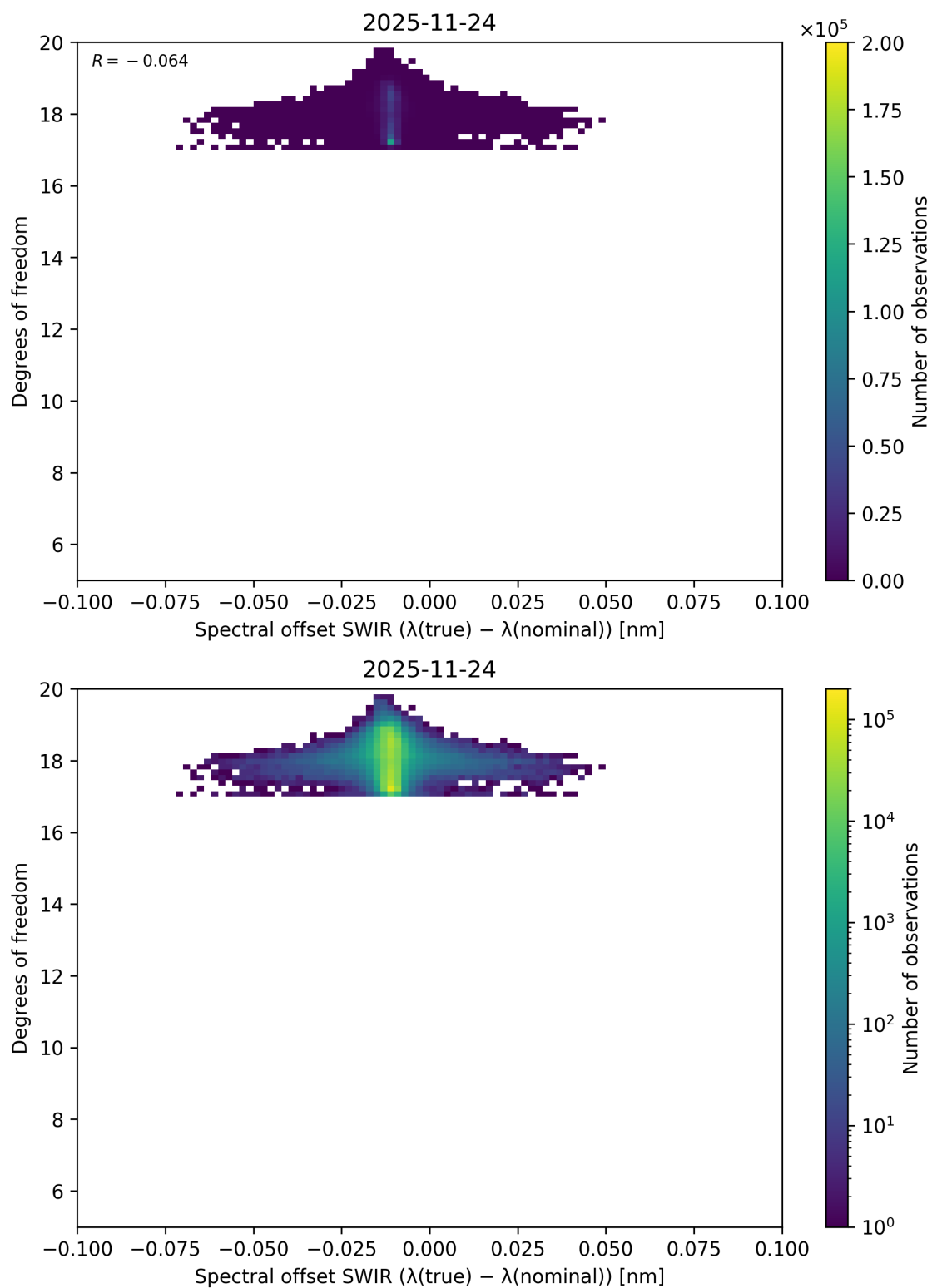
Figure 135: Scatter density plot of “Spectral offset SWIR ( \lambda_{\text{true}} - \lambda_{\text{nominal}} )” against “Degrees of freedom” for 2025-11-23 to 2025-11-25.
