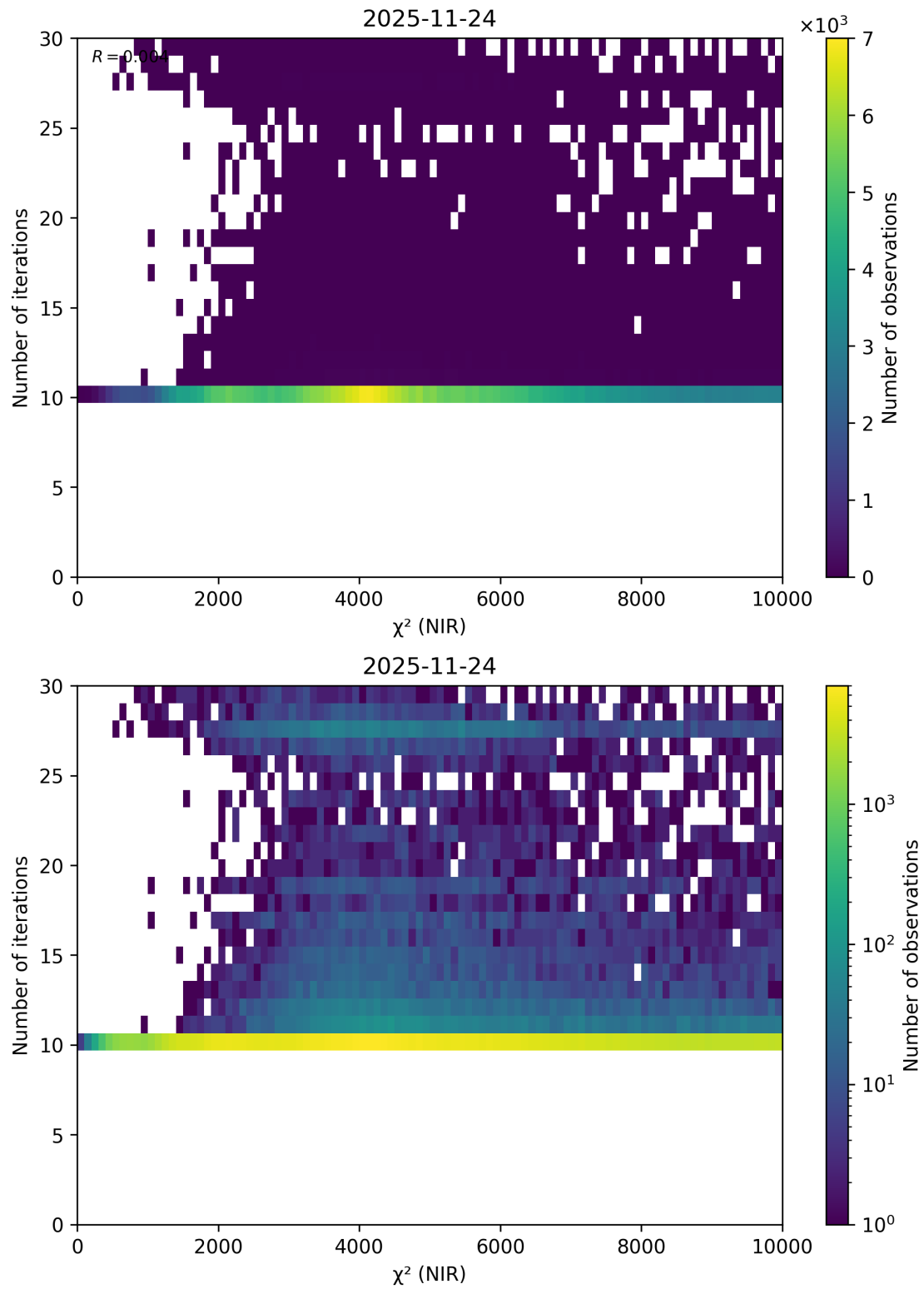
Figure 51: Scatter density plot of “ \chi^2 (NIR)” against “Number of iterations” for 2025-11-23 to 2025-11-25.
