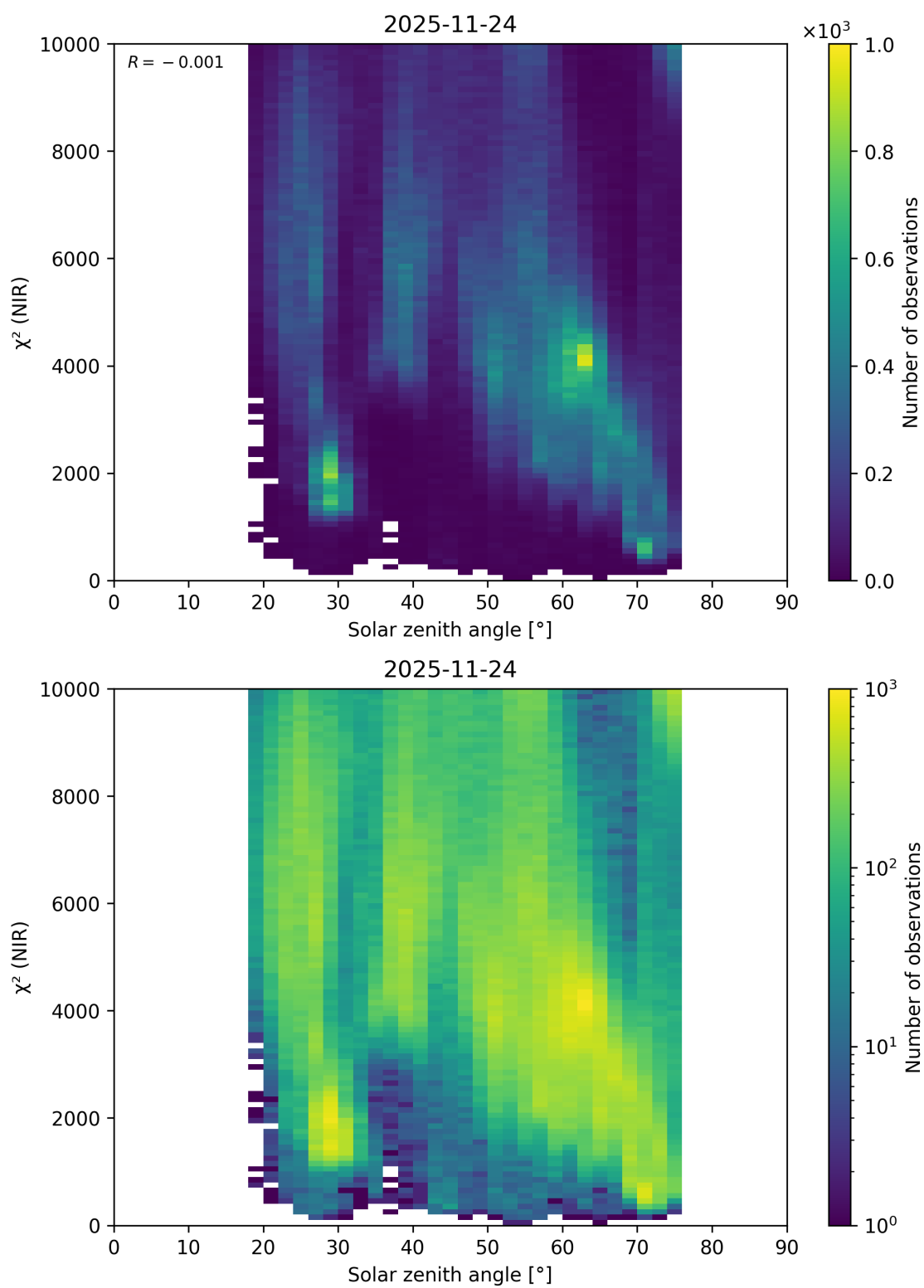
Figure 108: Scatter density plot of “Solar zenith angle” against “ \chi^2 (NIR)” for 2025-11-23 to 2025-11-25.
