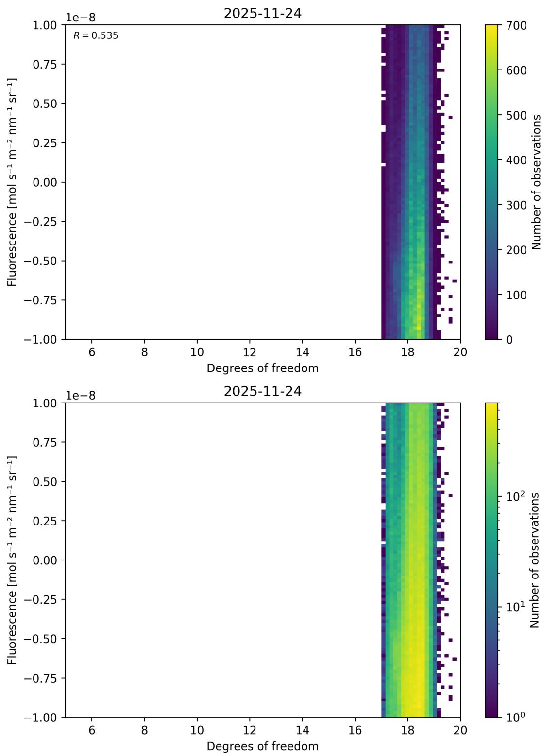
Figure 57: Scatter density plot of “Degrees of freedom” against “Fluorescence” for 2025-11-23 to 2025-11-25.
