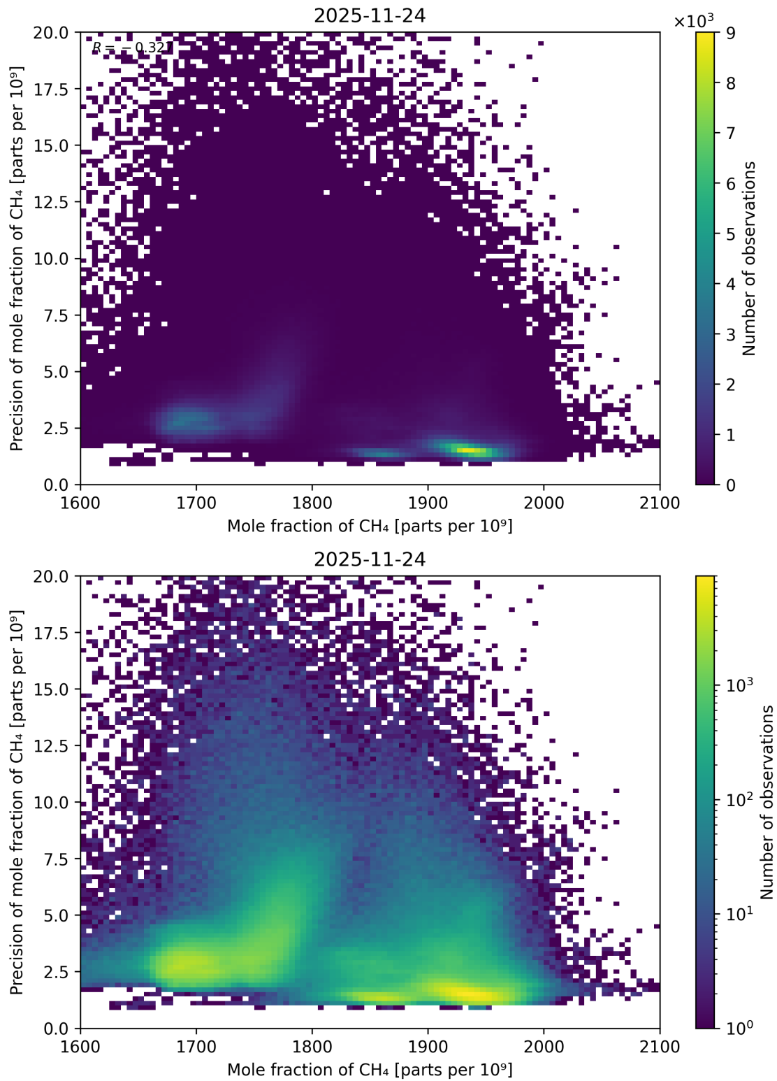
Figure 86: Scatter density plot of “Mole fraction of CH 4 ” against “Precision of mole fraction of CH 4 ” for 2025-11-23 to 2025-11-25.
