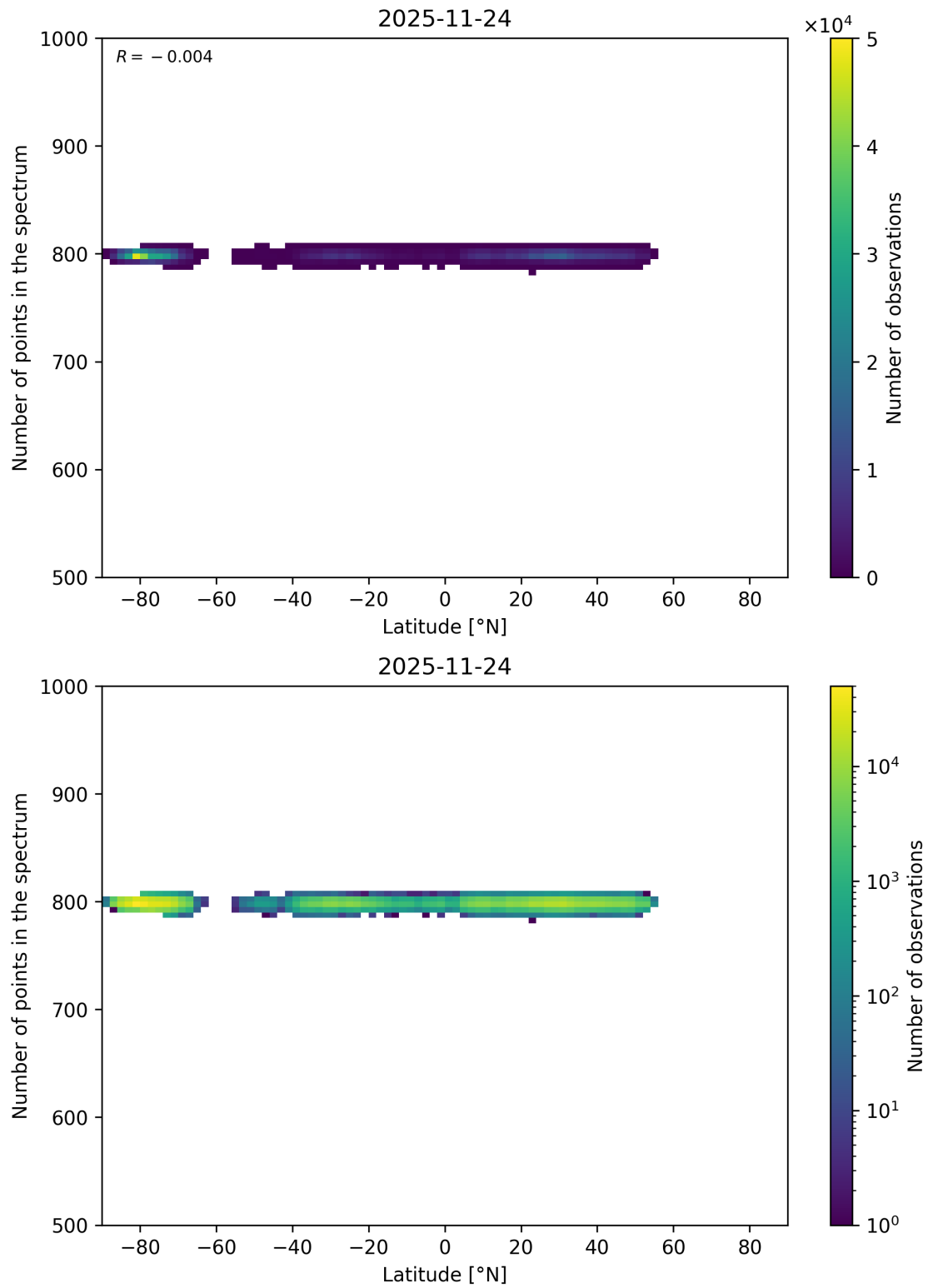
Figure 70: Scatter density plot of “Latitude” against “Number of points in the spectrum” for 2025-11-23 to 2025-11-25.
