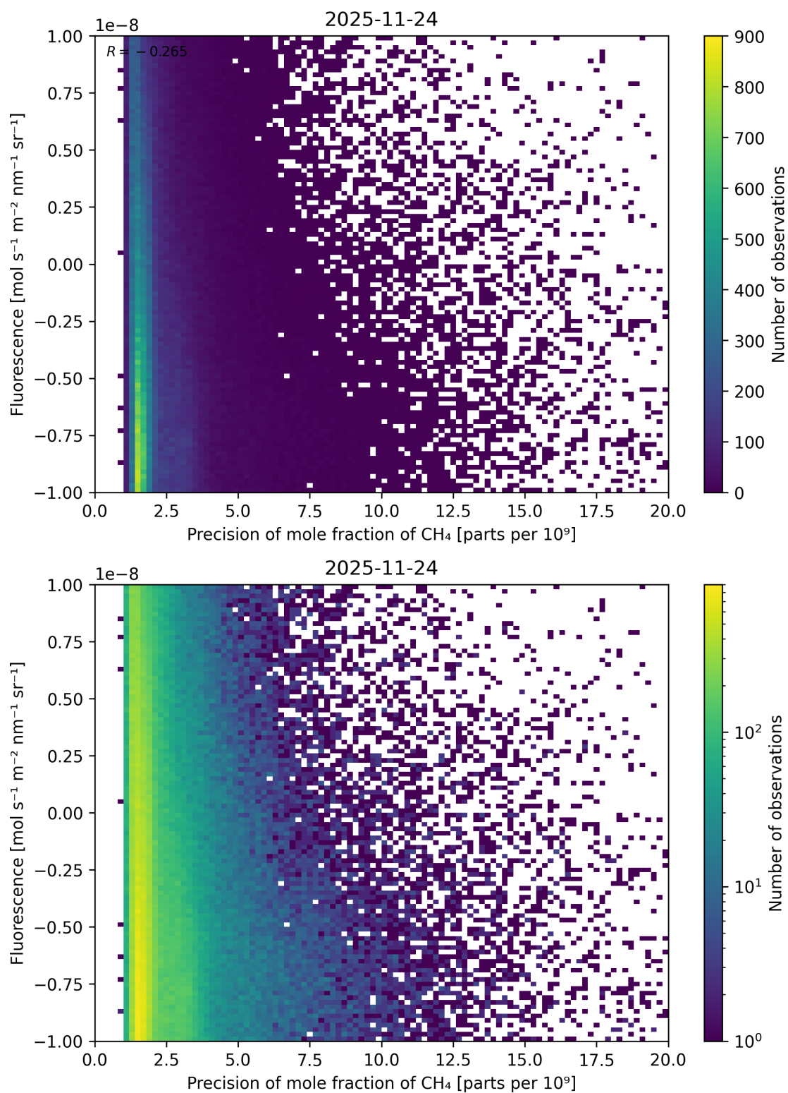
Figure 92: Scatter density plot of “Precision of mole fraction of \text{CH}_4 ” against “Fluorescence” for 2025-11-23 to 2025-11-25.
