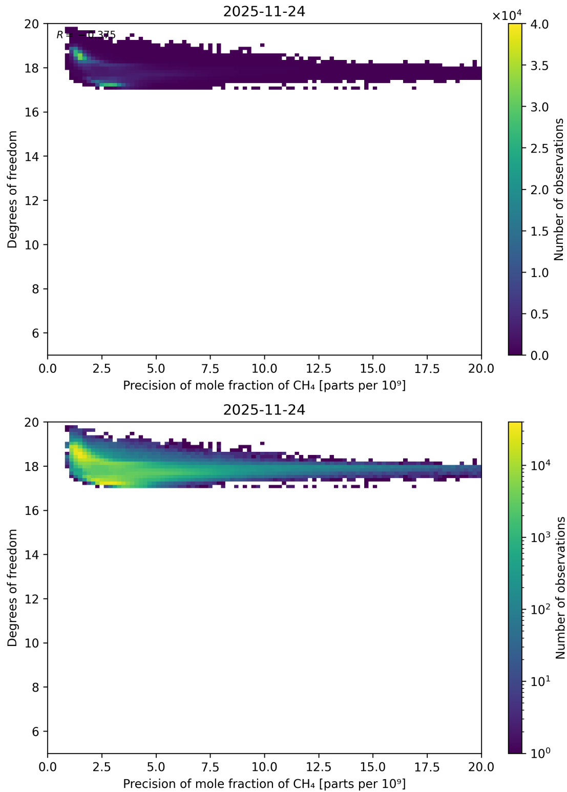
Figure 91: Scatter density plot of “Precision of mole fraction of CH 4 ” against “Degrees of freedom” for 2025-11-23 to 2025-11-25.
