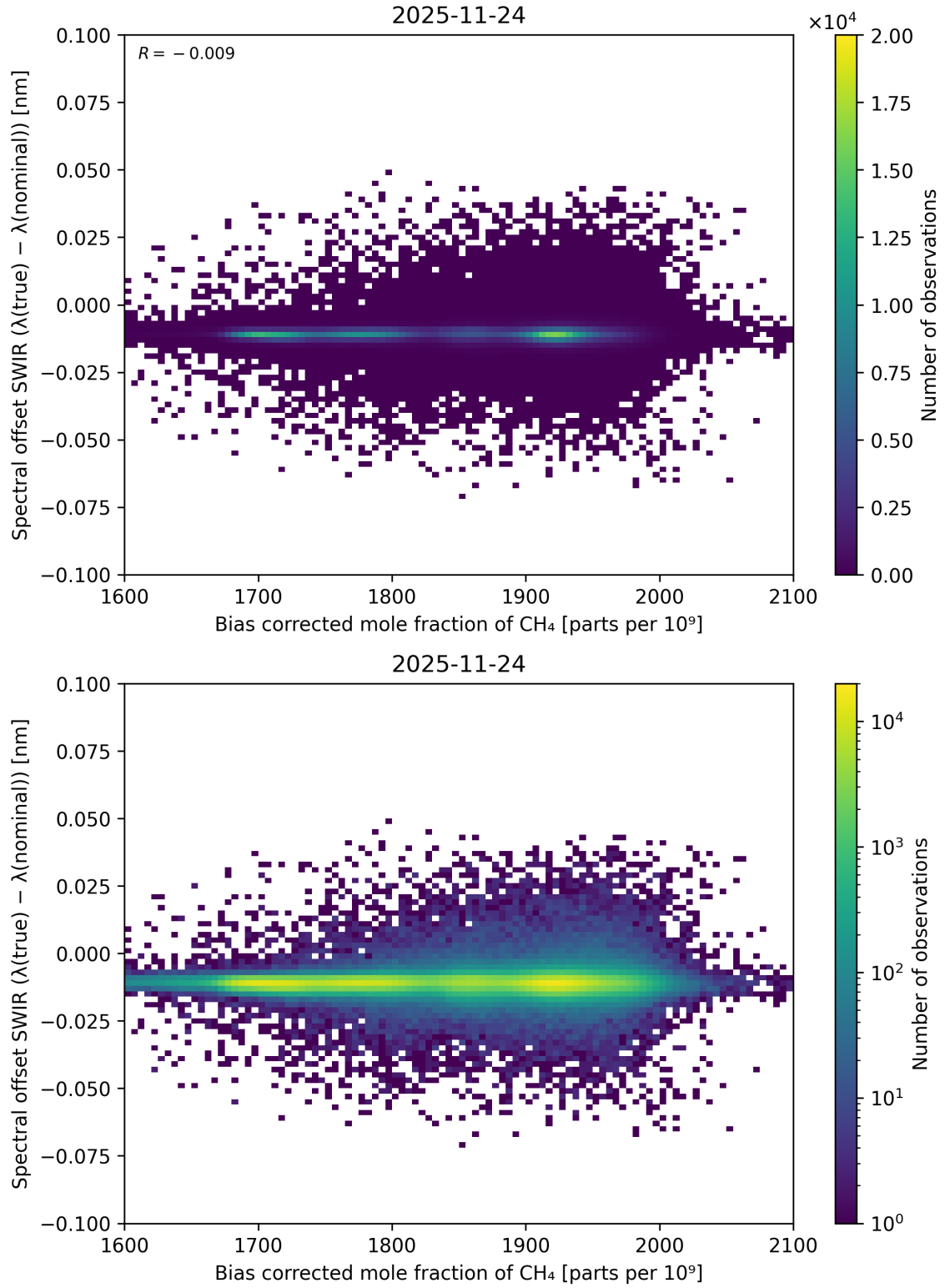
Figure 79: Scatter density plot of “Bias corrected mole fraction of \text{CH}_4 ” against “Spectral offset SWIR ( \lambda_{\text{true}} - \lambda_{\text{nominal}} )” for 2025-11-23 to 2025-11-25.
