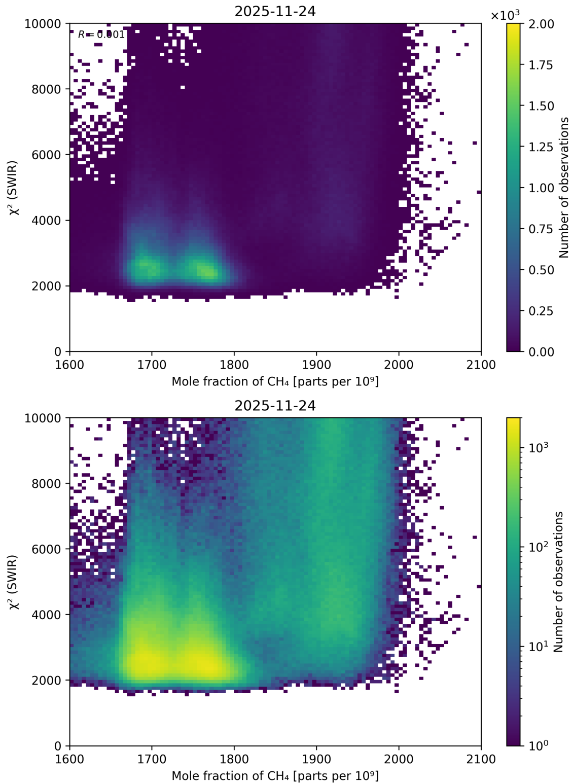
Figure 81: Scatter density plot of “Mole fraction of \text{CH}_4 ” against “ \chi^2 (SWIR)” for 2025-11-23 to 2025-11-25.
