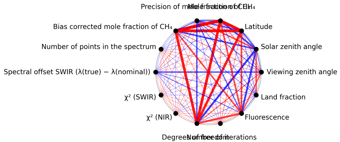
Figure 1: Map of correlation graph for 2025-11-23 to 2025-11-25.
