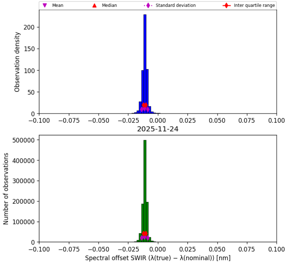
Figure 29: Histogram of “Spectral offset SWIR ( \lambda_{\text{true}} - \lambda_{\text{nominal}} )” for 2025-11-23 to 2025-11-25
