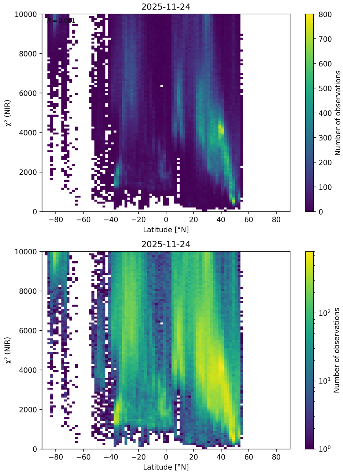
Figure 61: Scatter density plot of “Latitude” against “ \chi^2 (NIR)” for 2025-11-23 to 2025-11-25.
