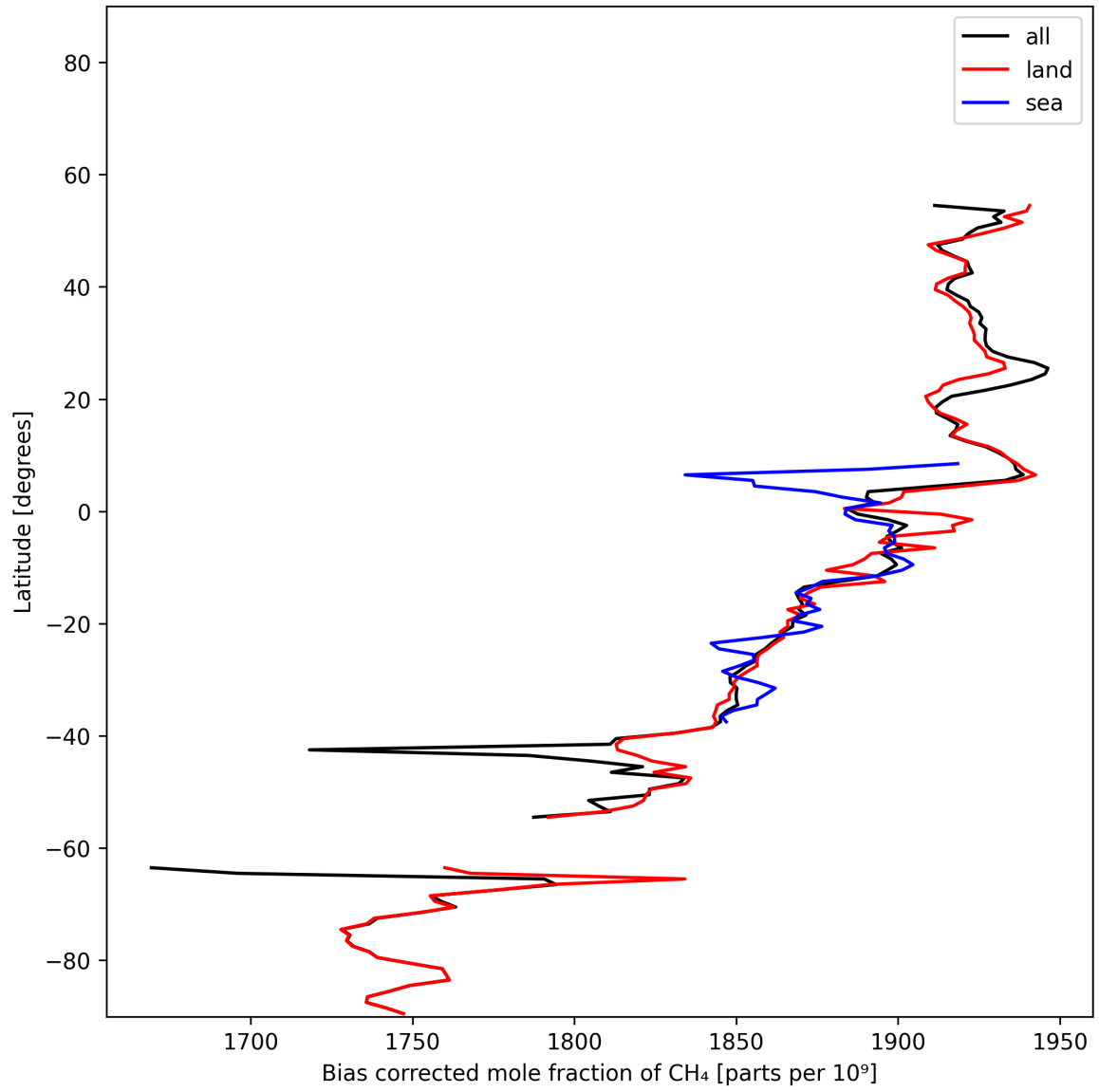
Figure 15: Zonal average of “Bias corrected mole fraction of CH 4 ” for 2025-11-23 to 2025-11-25.
