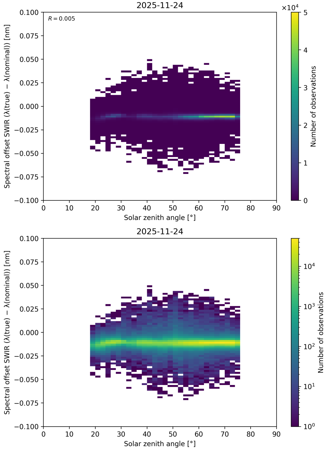
Figure 119: Scatter density plot of “Solar zenith angle” against “Spectral offset SWIR ( \lambda_{\text{true}} - \lambda_{\text{nominal}} )” for 2025-11-23 to 2025-11-25.
