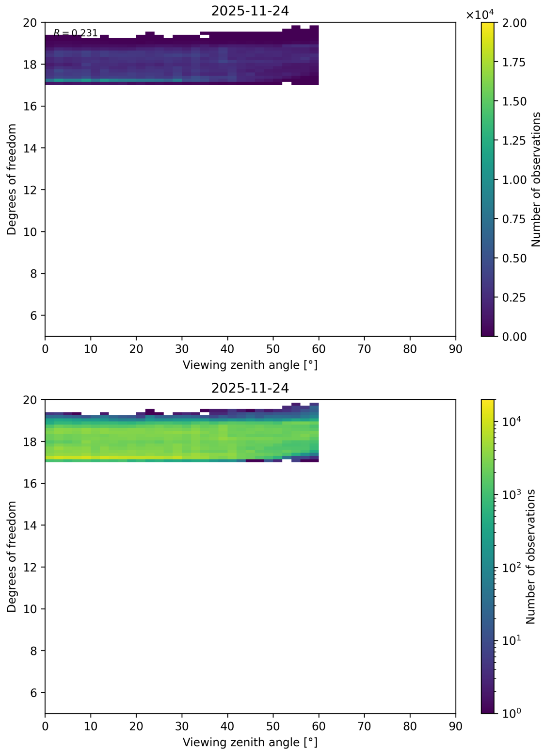
Figure 122: Scatter density plot of “Viewing zenith angle” against “Degrees of freedom” for 2025-11-23 to 2025-11-25.
