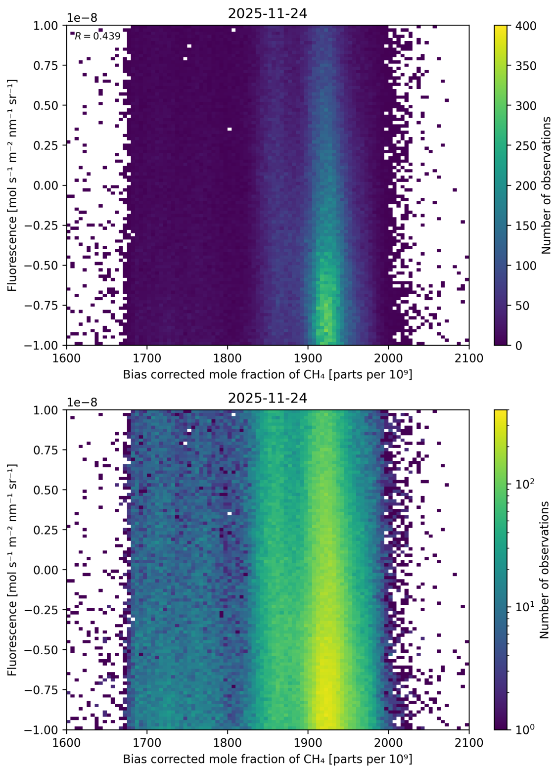
Figure 75: Scatter density plot of “Bias corrected mole fraction of \text{CH}_4 ” against “Fluorescence” for 2025-11-23 to 2025-11-25.
