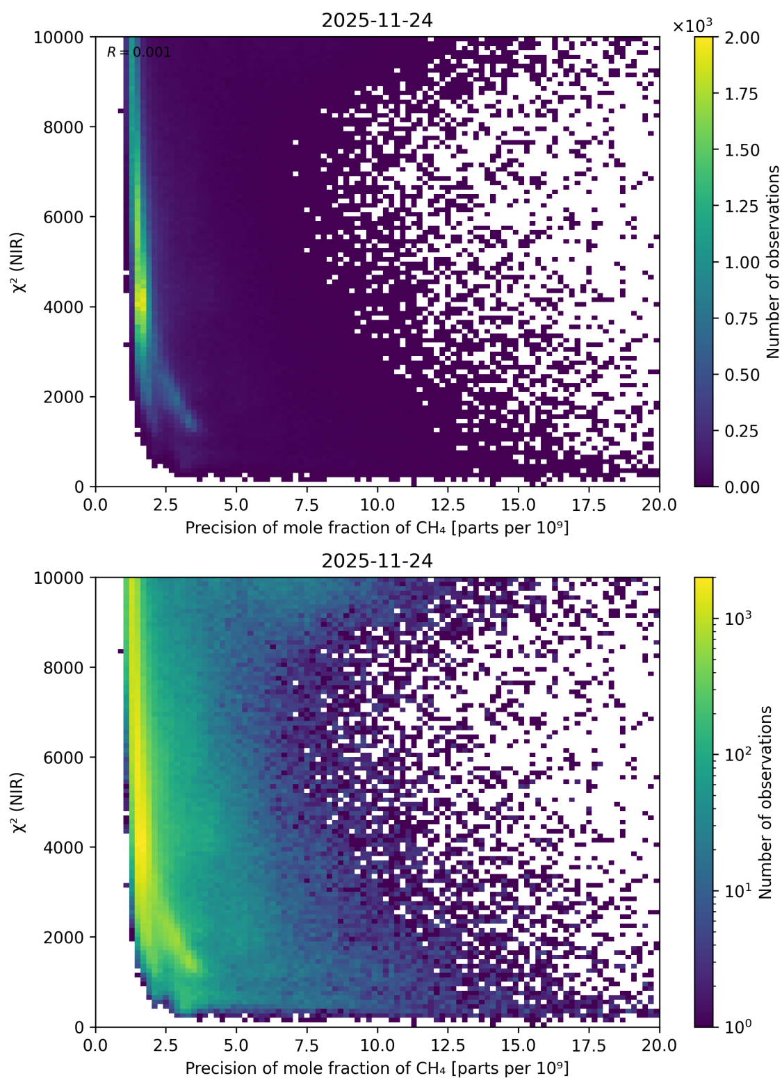
Figure 89: Scatter density plot of “Precision of mole fraction of \text{CH}_4 ” against “ \chi^2 (NIR)” for 2025-11-23 to 2025-11-25.
