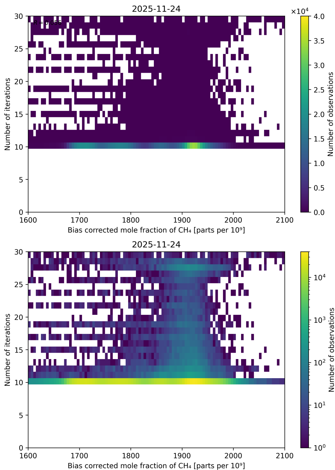
Figure 77: Scatter density plot of “Bias corrected mole fraction of \text{CH}_4 ” against “Number of iterations” for 2025-11-23 to 2025-11-25.
