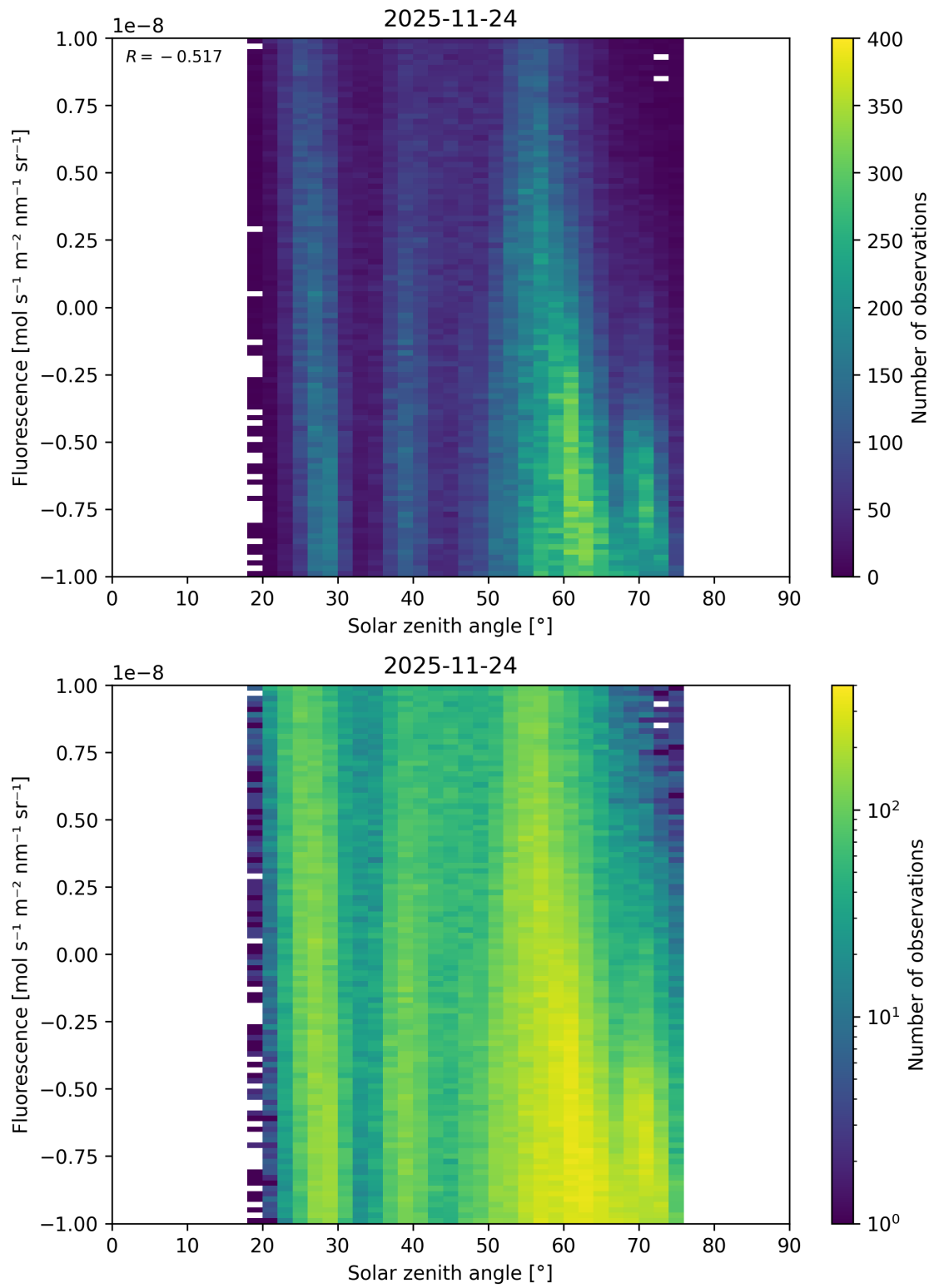
Figure 111: Scatter density plot of “Solar zenith angle” against “Fluorescence” for 2025-11-23 to 2025-11-25.
