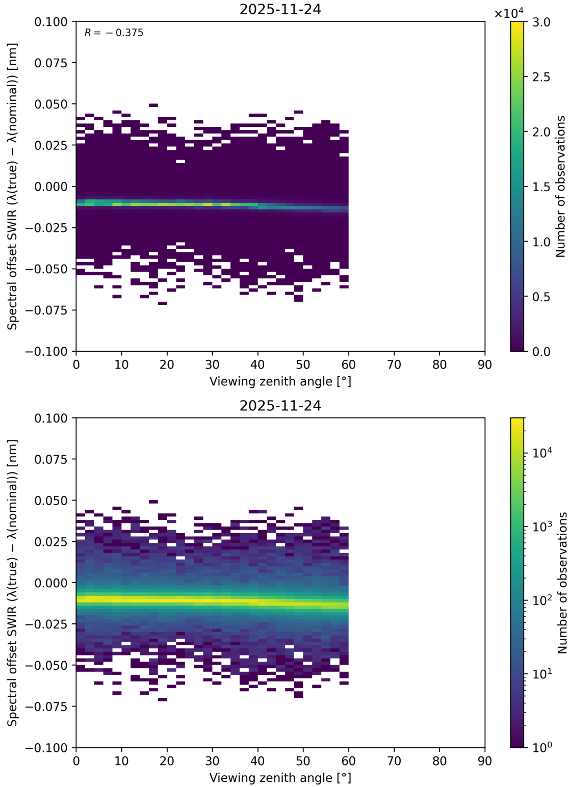
Figure 132: Scatter density plot of “Viewing zenith angle” against “Spectral offset SWIR ( \lambda_{\text{true}} - \lambda_{\text{nominal}} )” for 2025-11-23 to 2025-11-25.
