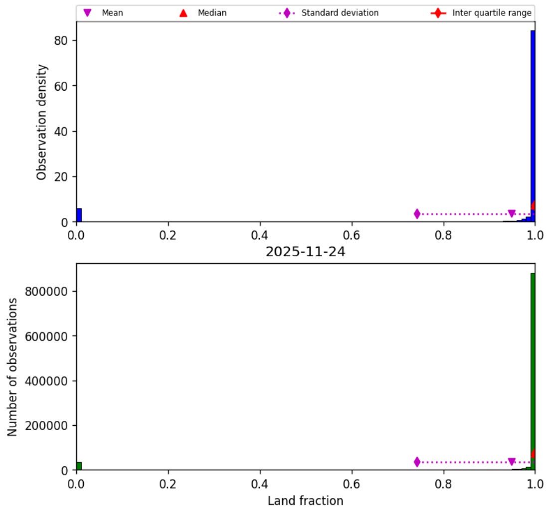
Figure 35: Histogram of “Land fraction” for 2025-11-23 to 2025-11-25
