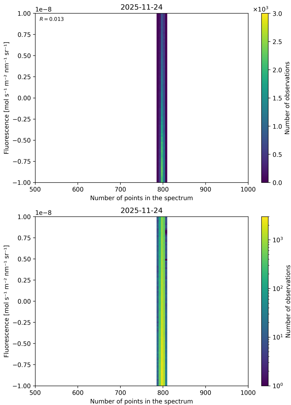
Figure 104: Scatter density plot of “Number of points in the spectrum” against “Fluorescence” for 2025-11-23 to 2025-11-25.
