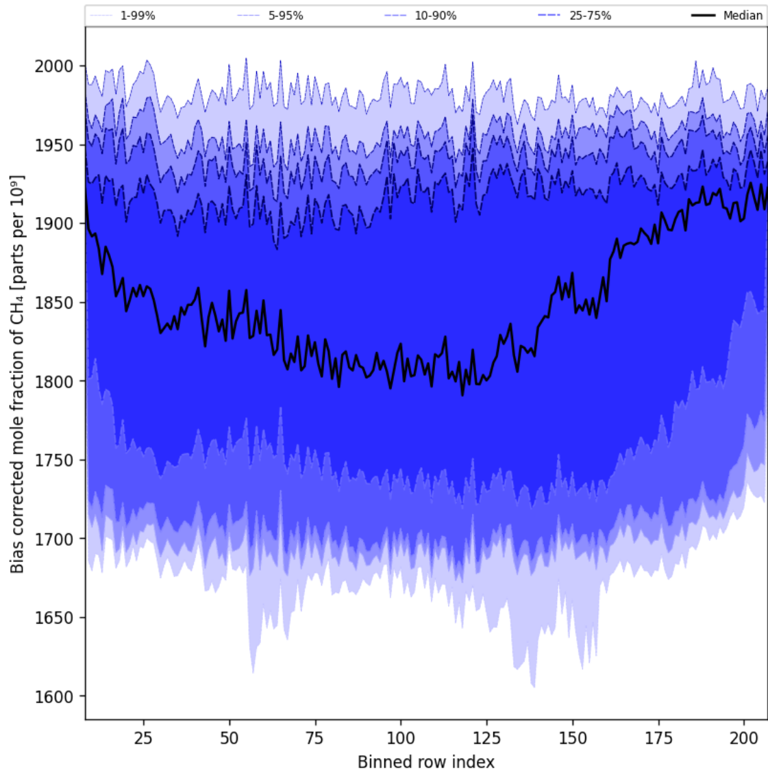
Figure 39: Along track statistics of “Bias corrected mole fraction of CH 4 ” for 2025-11-23 to 2025-11-25
