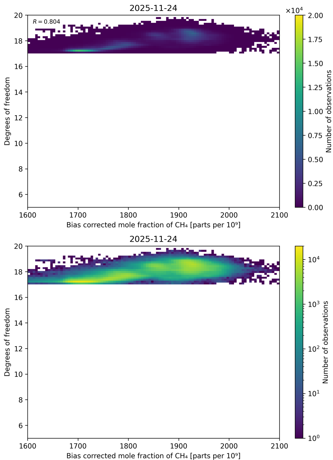
Figure 74: Scatter density plot of “Bias corrected mole fraction of CH 4 ” against “Degrees of freedom” for 2025-11-23 to 2025-11-25.
