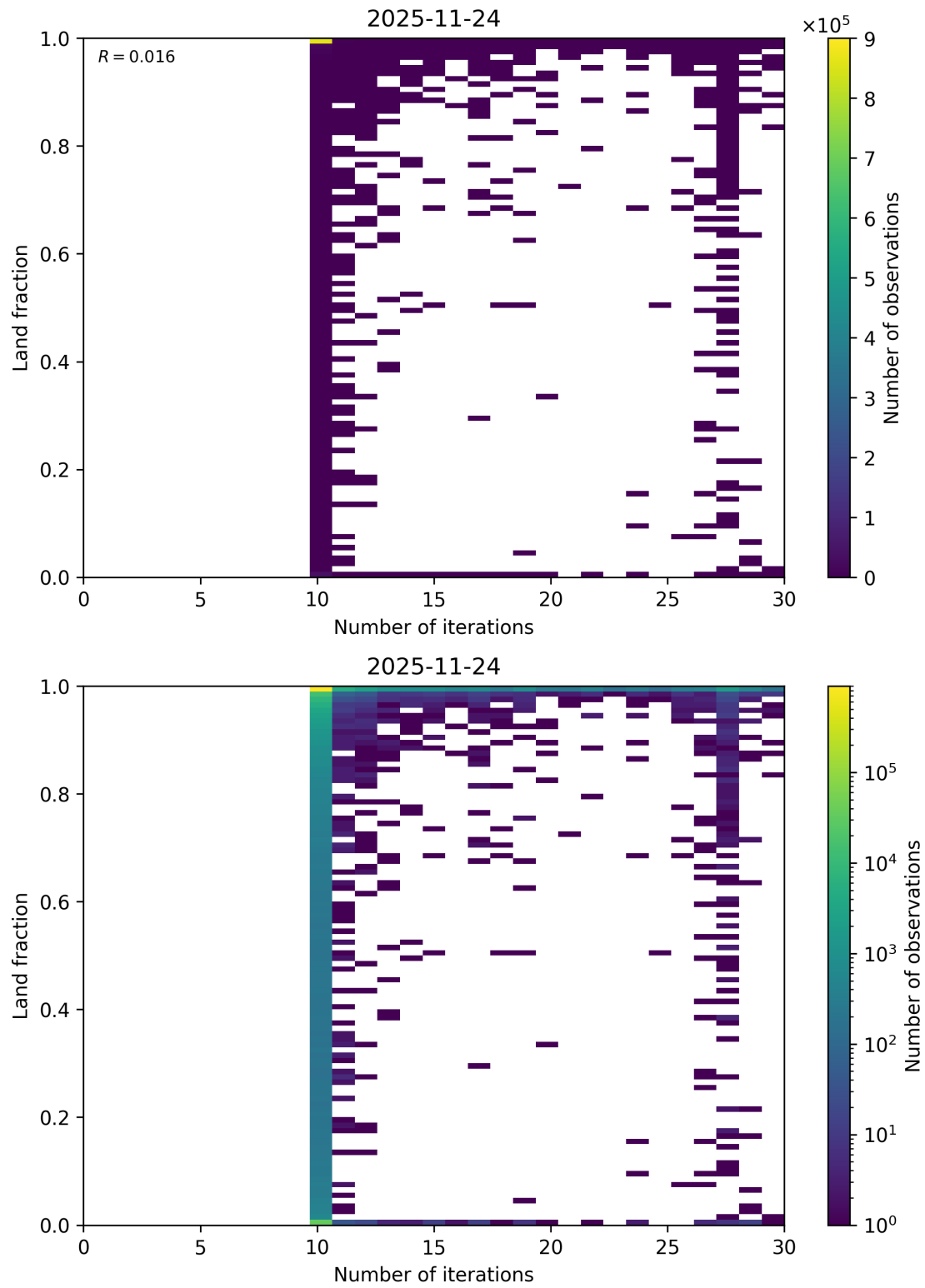
Figure 100: Scatter density plot of “Number of iterations” against “Land fraction” for 2025-11-23 to 2025-11-25.
