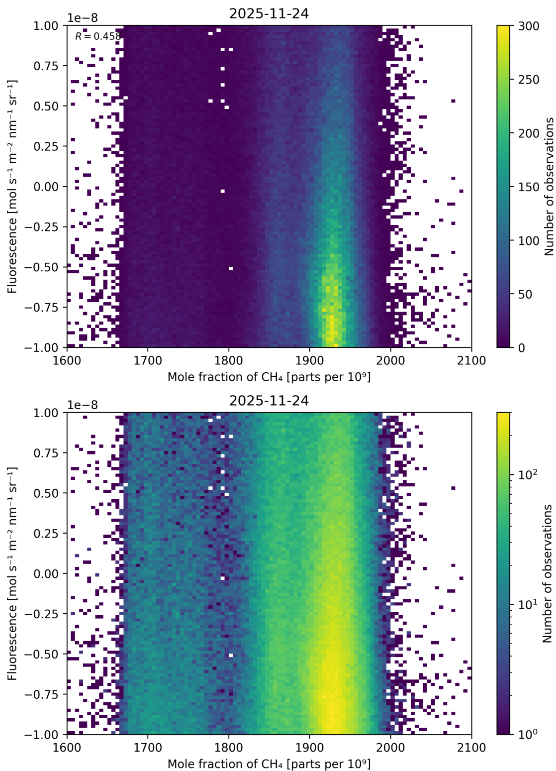
Figure 83: Scatter density plot of “Mole fraction of \text{CH}_4 ” against “Fluorescence” for 2025-11-23 to 2025-11-25.
