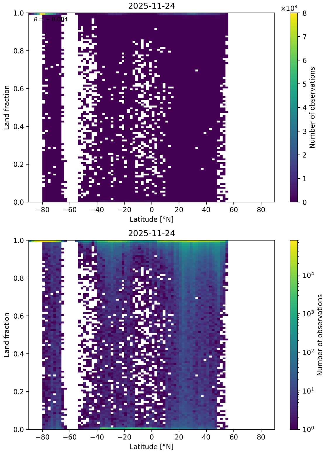
Figure 65: Scatter density plot of “Latitude” against “Land fraction” for 2025-11-23 to 2025-11-25.
