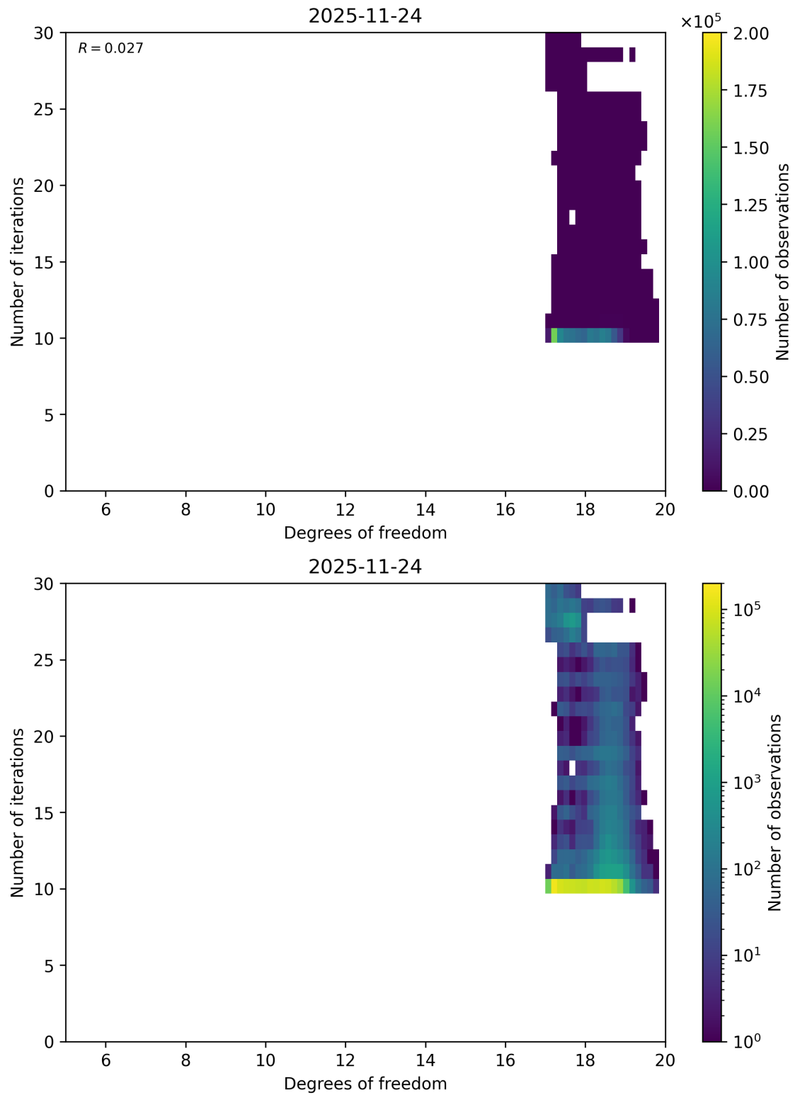
Figure 59: Scatter density plot of “Degrees of freedom” against “Number of iterations” for 2025-11-23 to 2025-11-25.
