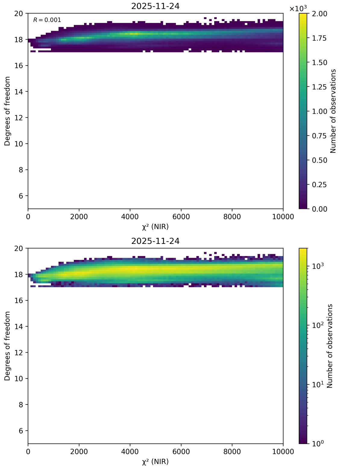
Figure 48: Scatter density plot of “ \chi^2 (NIR)” against “Degrees of freedom” for 2025-11-23 to 2025-11-25.
