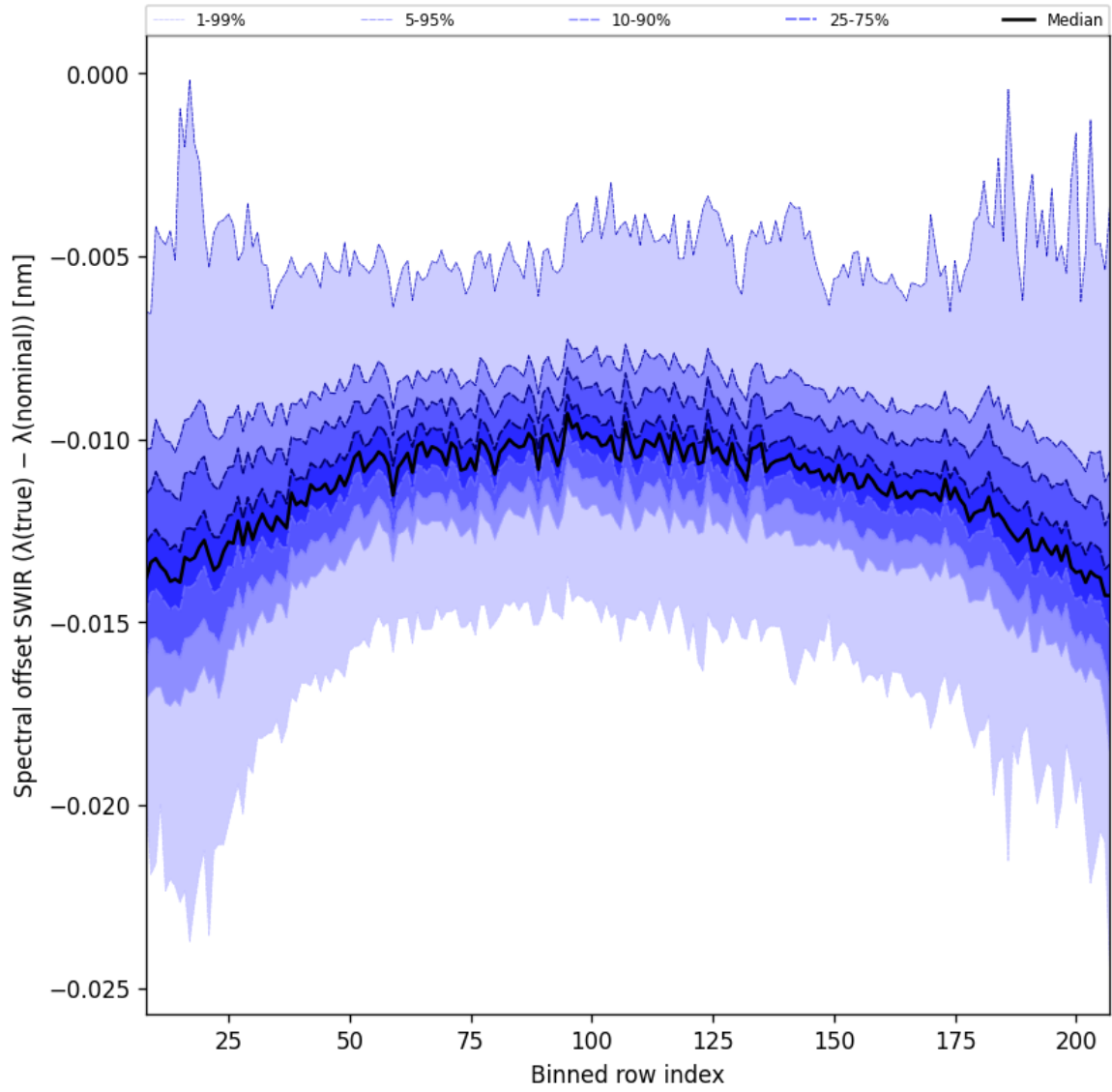
Figure 41: Along track statistics of “Spectral offset SWIR ( \lambda_{\text{true}} - \lambda_{\text{nominal}} )” for 2025-11-23 to 2025-11-25
