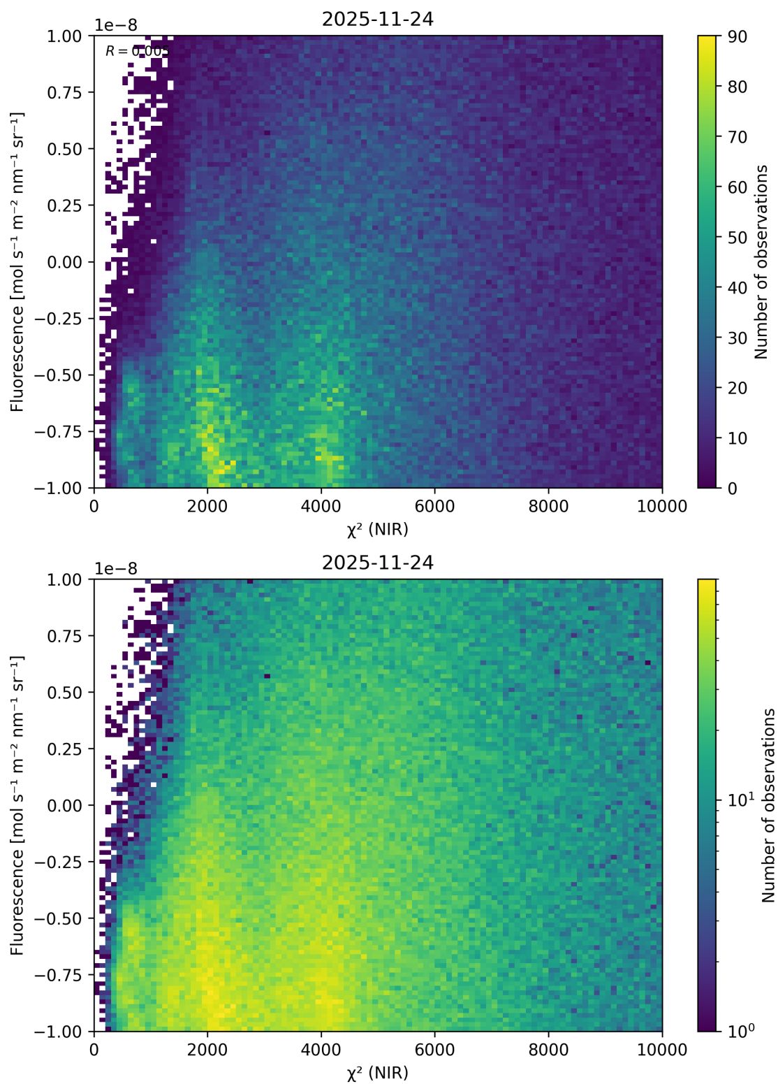
Figure 49: Scatter density plot of “ \chi^2 (NIR)” against “Fluorescence” for 2025-11-23 to 2025-11-25.
