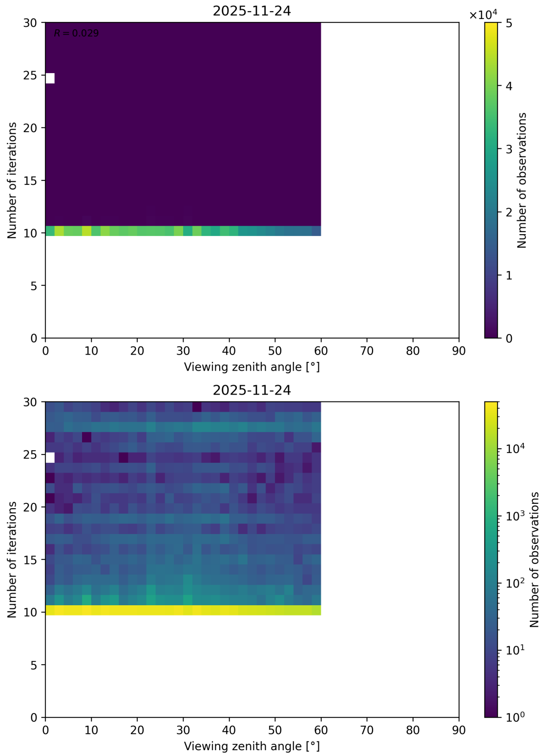
Figure 129: Scatter density plot of “Viewing zenith angle” against “Number of iterations” for 2025-11-23 to 2025-11-25.
