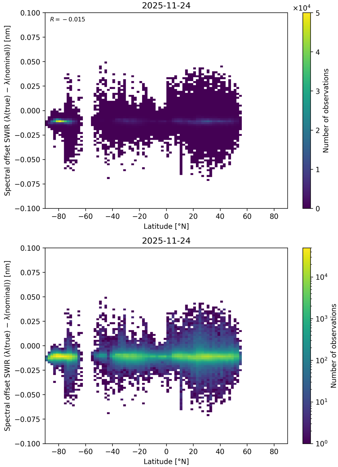
Figure 71: Scatter density plot of “Latitude” against “Spectral offset SWIR ( \lambda_{\text{true}} - \lambda_{\text{nominal}} )” for 2025-11-23 to 2025-11-25.
