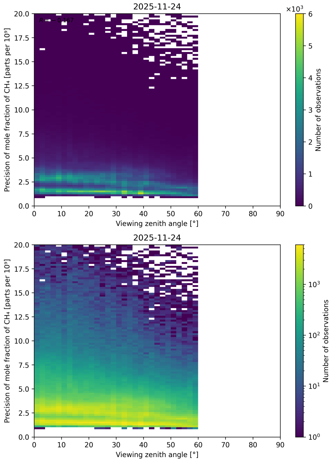
Figure 128: Scatter density plot of “Viewing zenith angle” against “Precision of mole fraction of CH 4 ” for 2025-11-23 to 2025-11-25.
