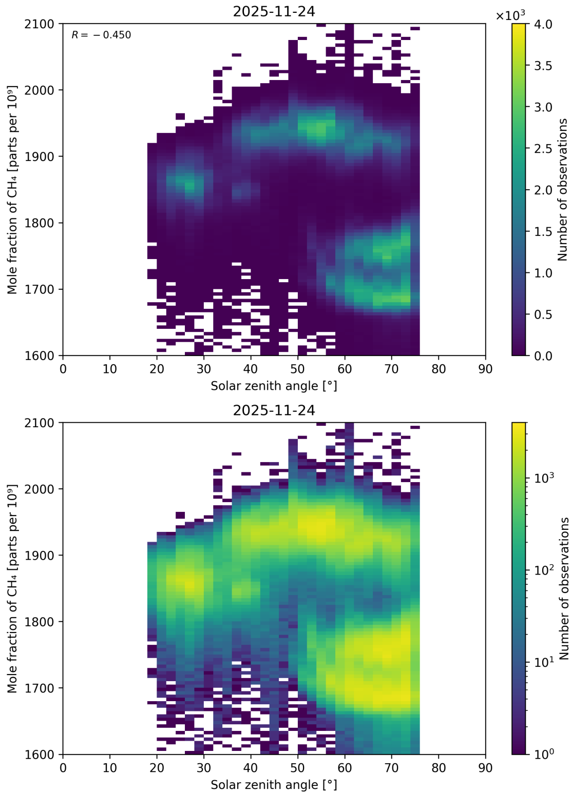
Figure 114: Scatter density plot of “Solar zenith angle” against “Mole fraction of CH 4 ” for 2025-11-23 to 2025-11-25.
