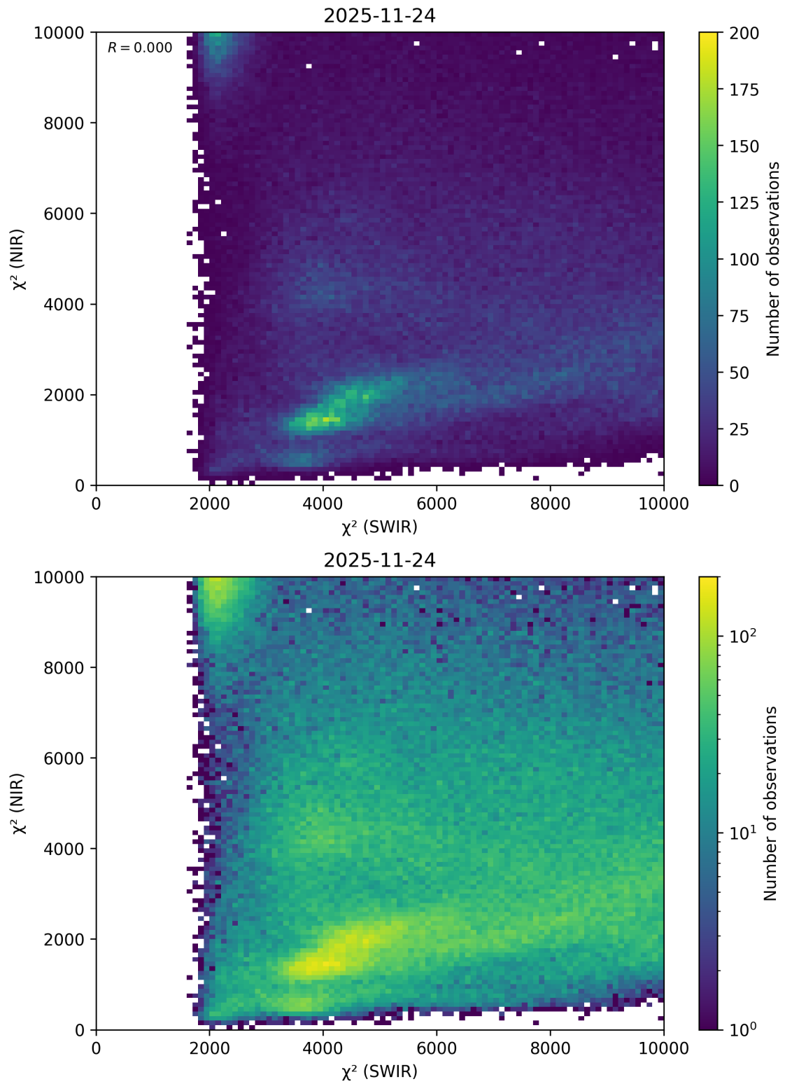
Figure 52: Scatter density plot of “ \chi^2 (SWIR)” against “ \chi^2 (NIR)” for 2025-11-23 to 2025-11-25.
