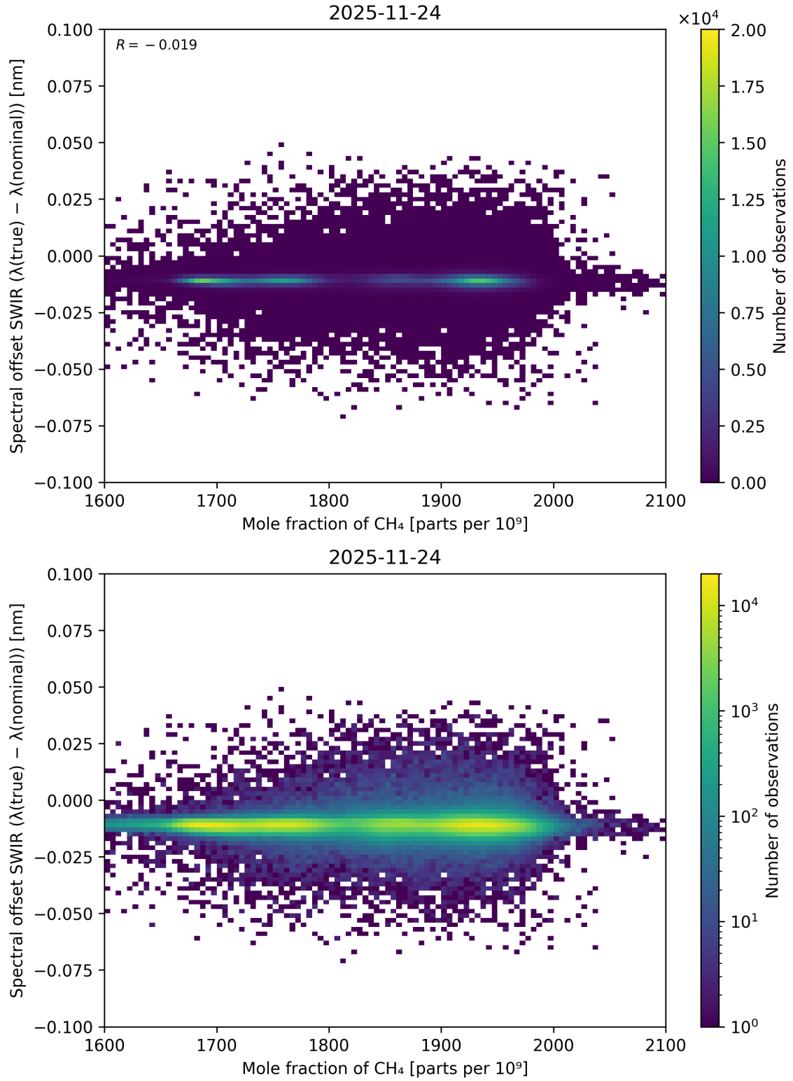
Figure 98: Scatter density plot of “Mole fraction of CH 4 ” against “Spectral offset SWIR ( \lambda_{\text{true}} - \lambda_{\text{nominal}} )” for 2025-11-23 to 2025-11-25.
