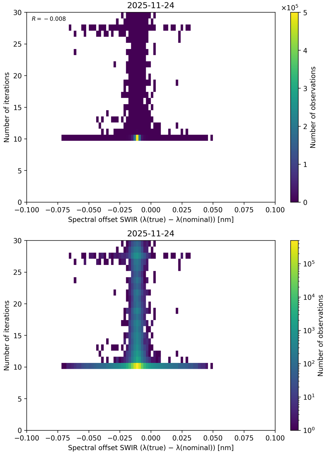
Figure 138: Scatter density plot of “Spectral offset SWIR ( \lambda_{\text{true}} - \lambda_{\text{nominal}} )” against “Number of iterations” for 2025-11-23 to 2025-11-25.
