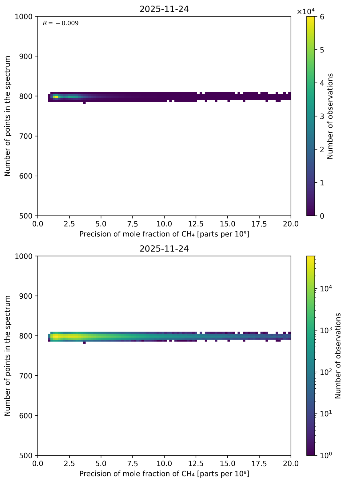
Figure 96: Scatter density plot of “Precision of mole fraction of CH 4 ” against “Number of points in the spectrum” for 2025-11-23 to 2025-11-25.
