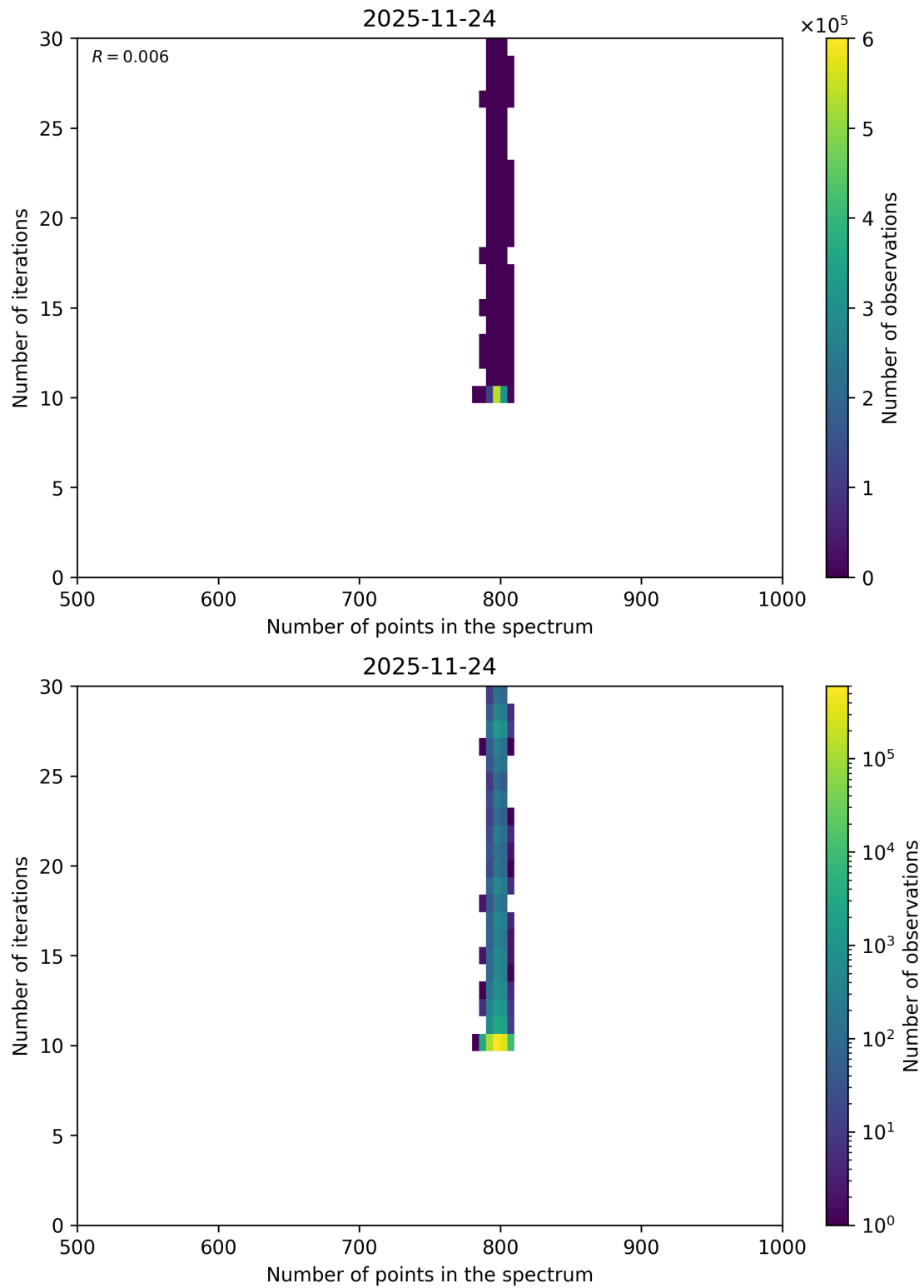
Figure 106: Scatter density plot of “Number of points in the spectrum” against “Number of iterations” for 2025-11-23 to 2025-11-25.
