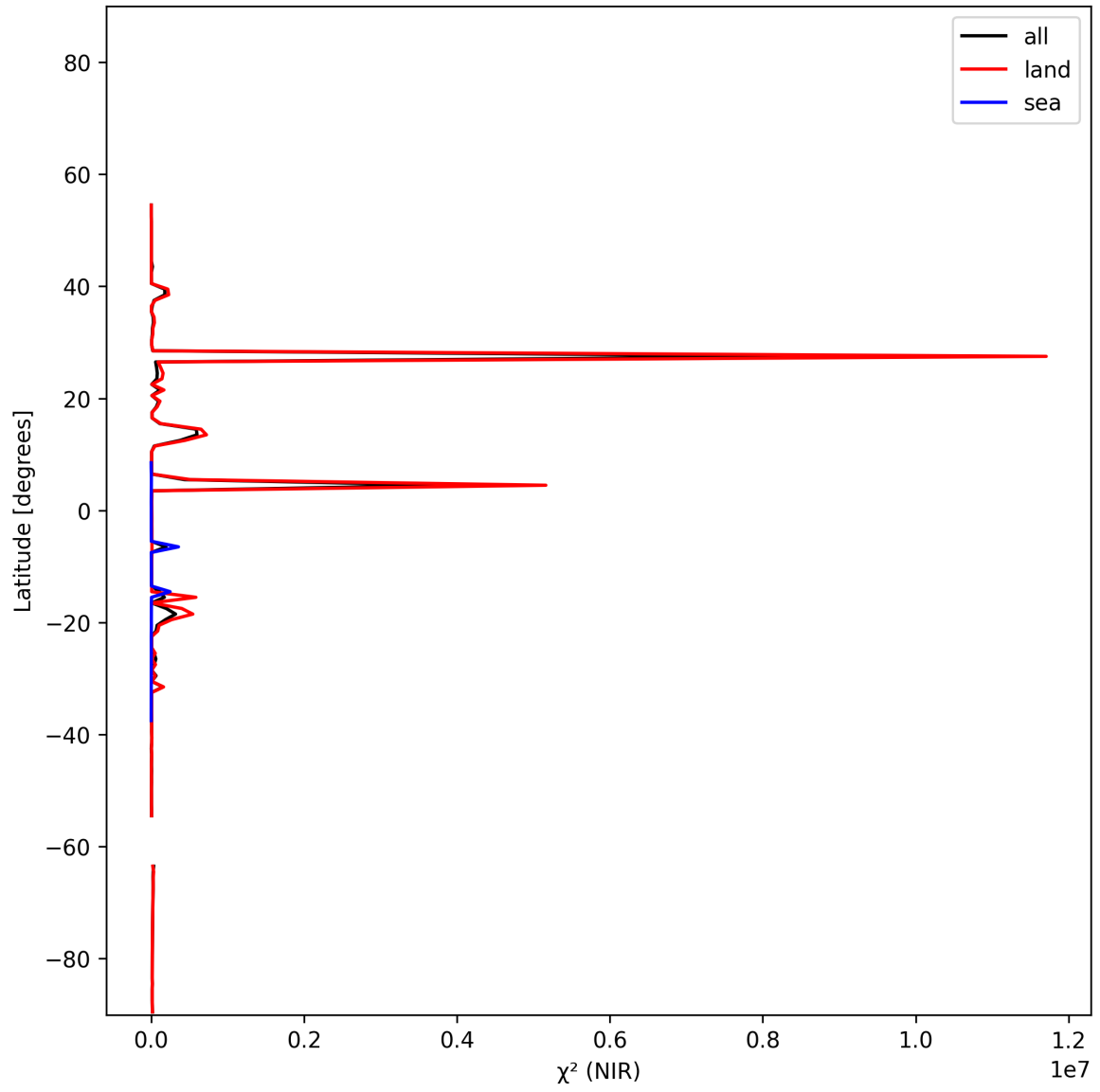
Figure 19: Zonal average of “ \chi^2 (NIR)” for 2025-11-23 to 2025-11-25.
