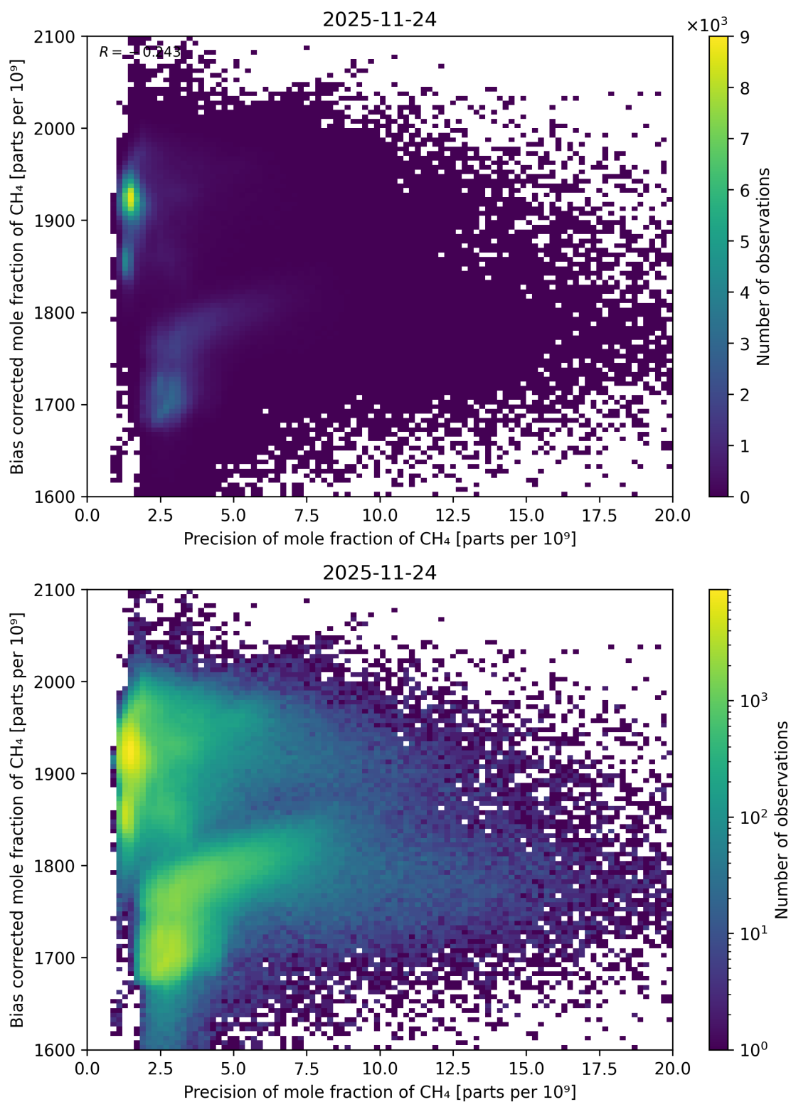
Figure 94: Scatter density plot of “Precision of mole fraction of CH 4 ” against “Bias corrected mole fraction of CH 4 ” for 2025-11-23 to 2025-11-25.
