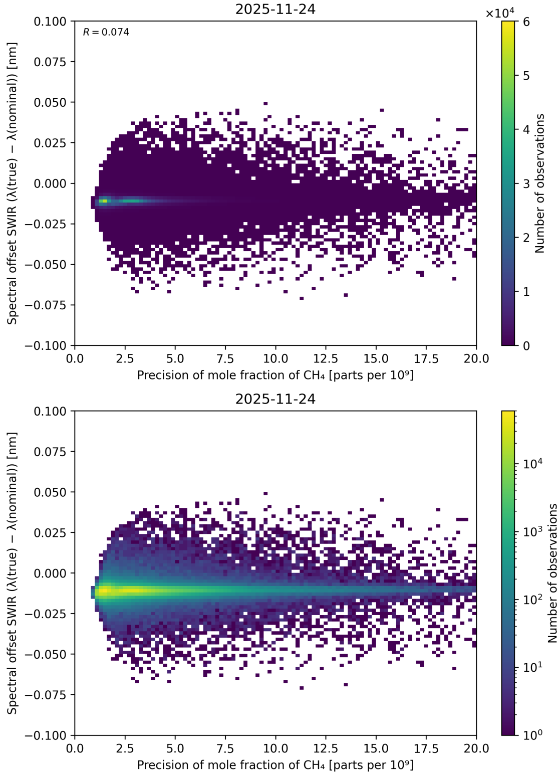
Figure 97: Scatter density plot of “Precision of mole fraction of CH 4 ” against “Spectral offset SWIR ( \lambda_{\text{true}} - \lambda_{\text{nominal}} )” for 2025-11-23 to 2025-11-25.
