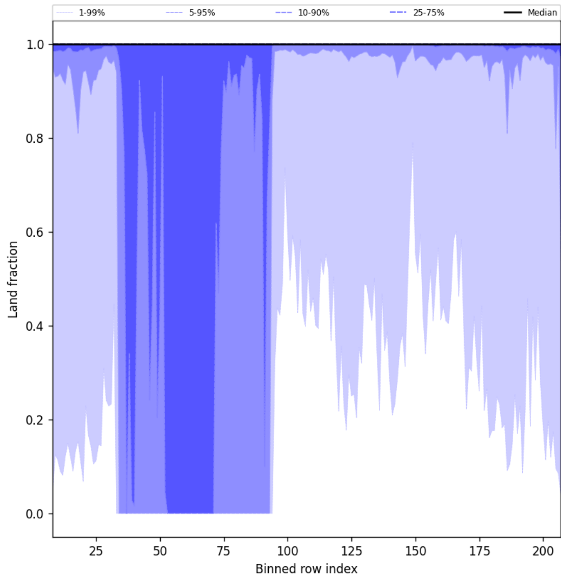
Figure 47: Along track statistics of "Land fraction" for 2025-11-23 to 2025-11-25
