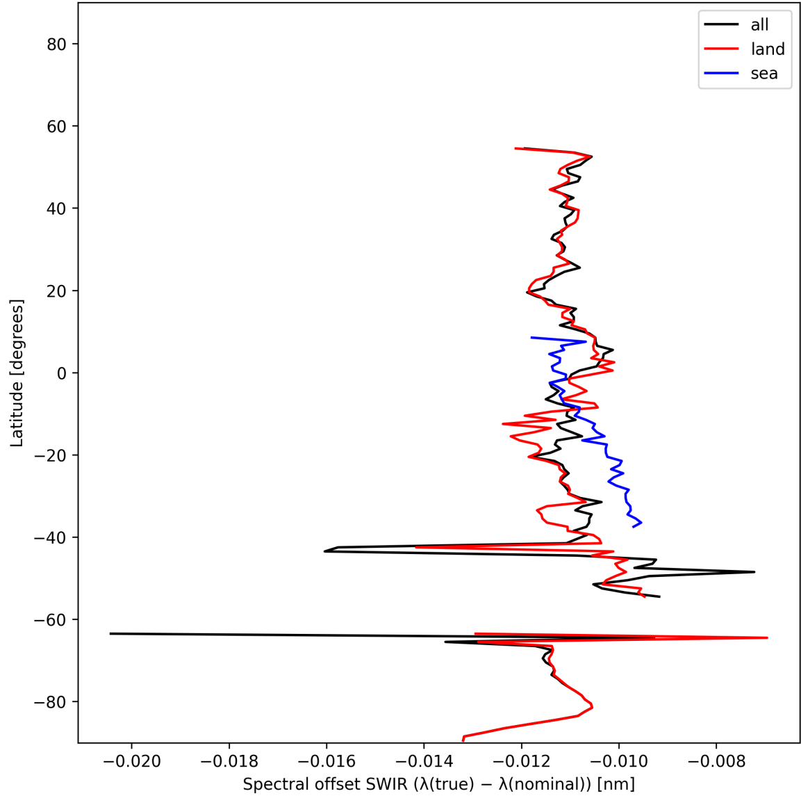
Figure 17: Zonal average of “Spectral offset SWIR ( \lambda_{\text{true}} - \lambda_{\text{nominal}} )” for 2025-11-23 to 2025-11-25.
