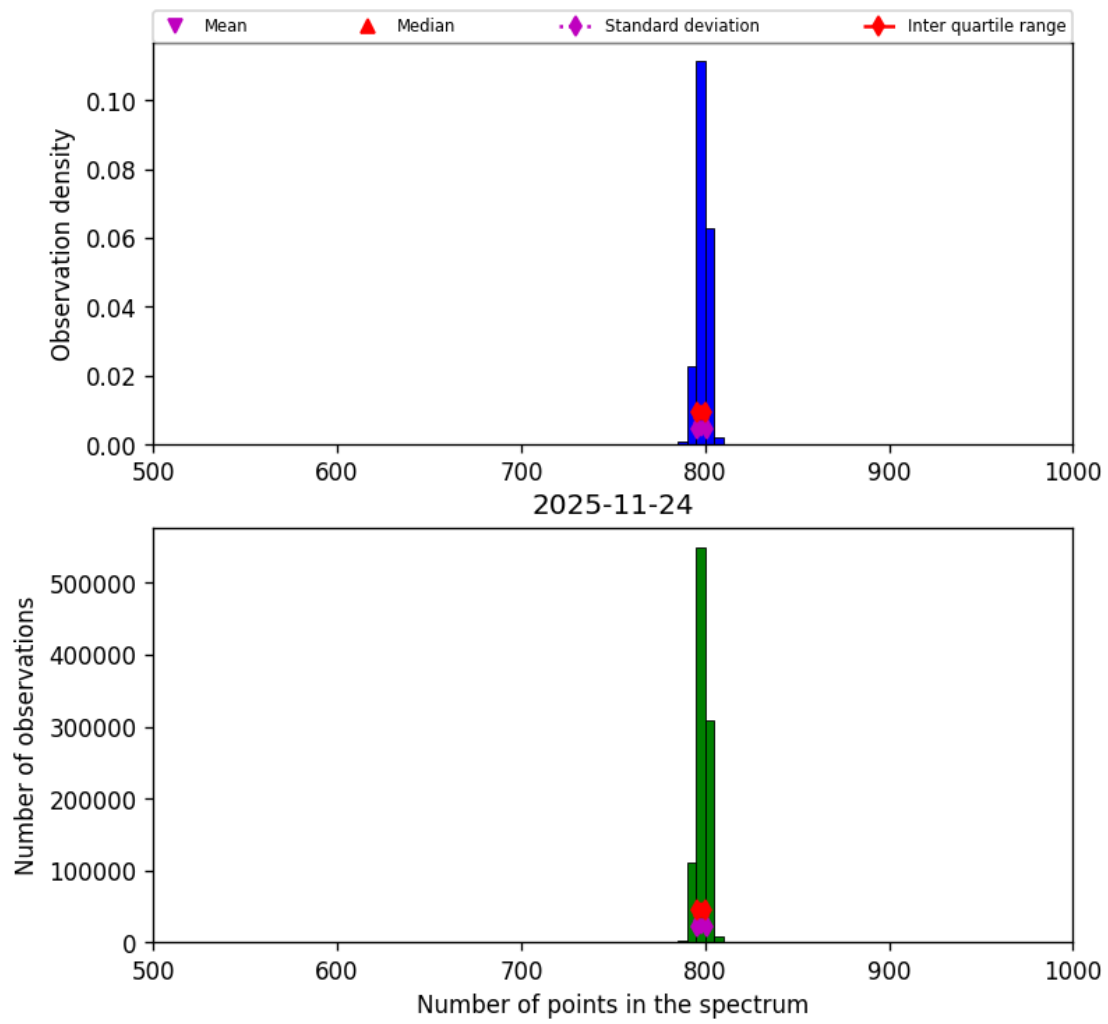
Figure 28: Histogram of “Number of points in the spectrum” for 2025-11-23 to 2025-11-25
