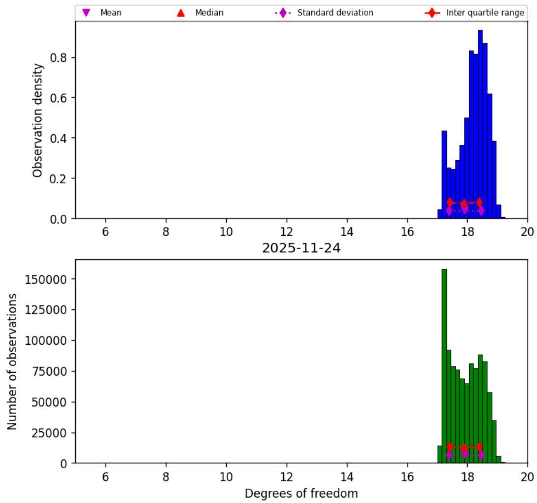
Figure 32: Histogram of “Degrees of freedom” for 2025-11-23 to 2025-11-25
