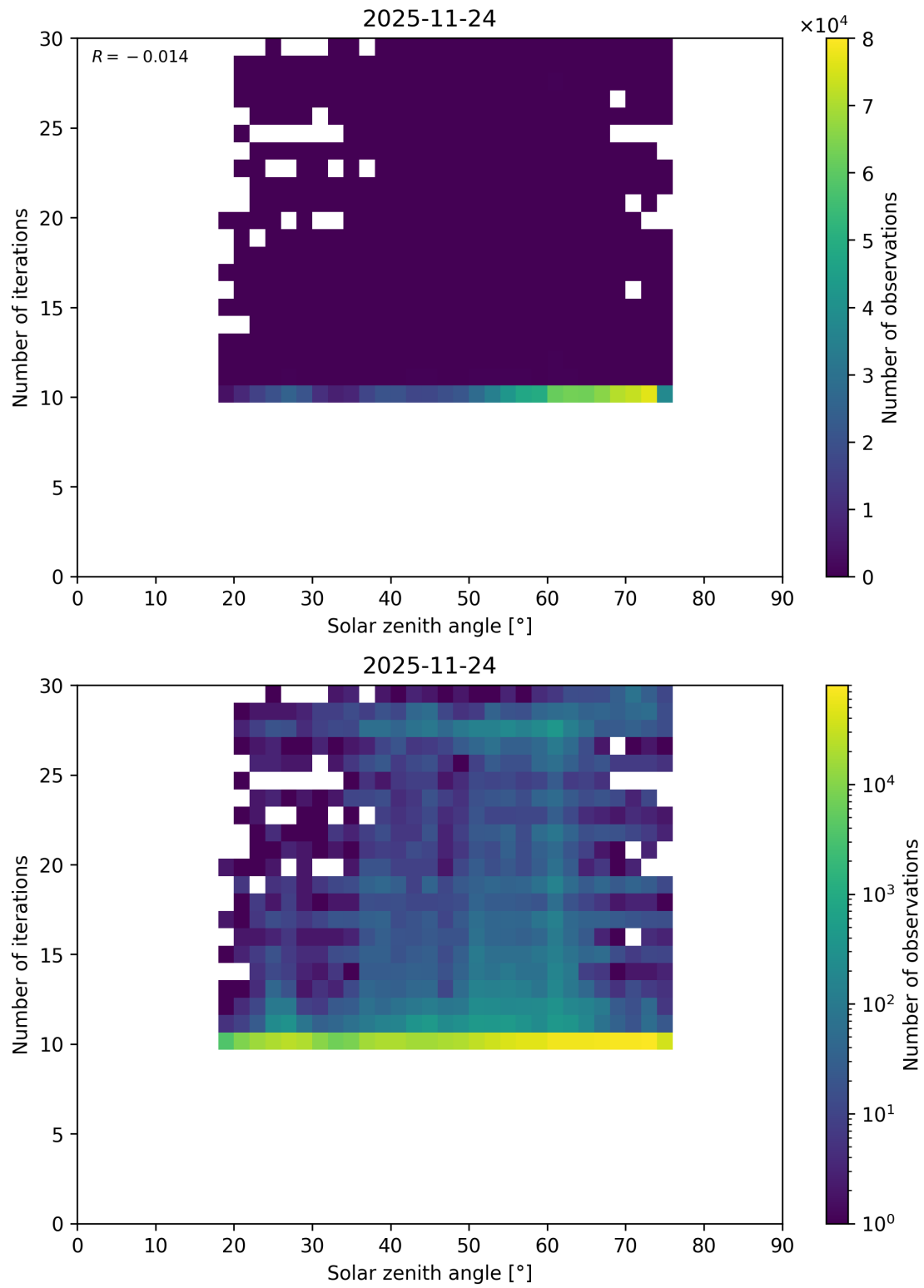
Figure 117: Scatter density plot of “Solar zenith angle” against “Number of iterations” for 2025-11-23 to 2025-11-25.
