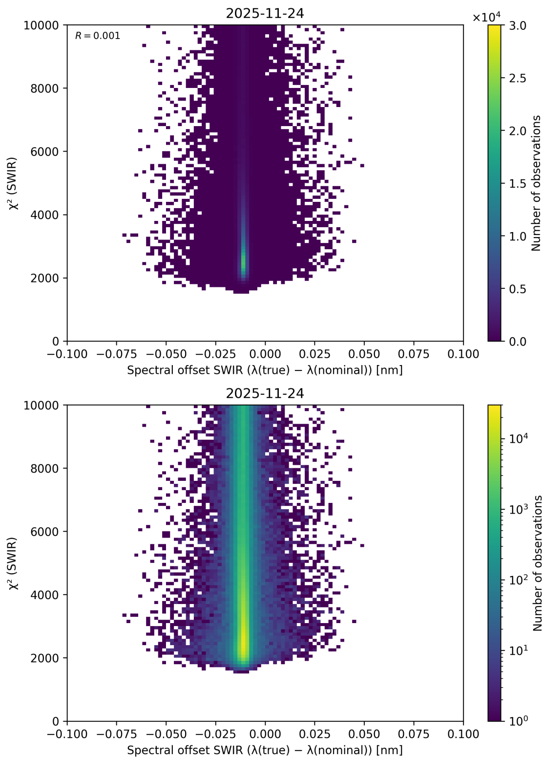
Figure 134: Scatter density plot of “Spectral offset SWIR ( \lambda_{\text{true}} - \lambda_{\text{nominal}} )” against “ \chi^2 (SWIR)” for 2025-11-23 to 2025-11-25.
