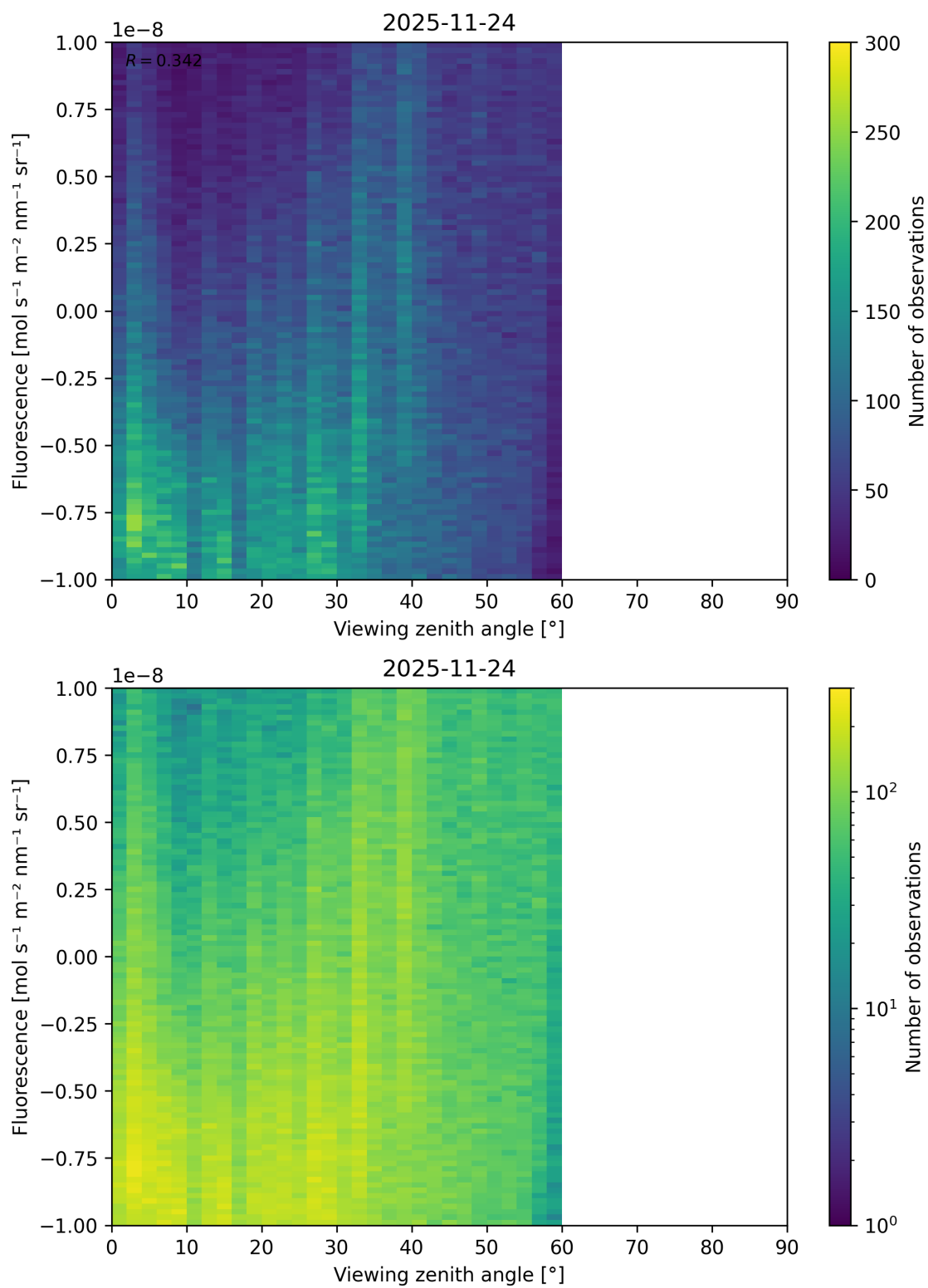
Figure 123: Scatter density plot of “Viewing zenith angle” against “Fluorescence” for 2025-11-23 to 2025-11-25.
