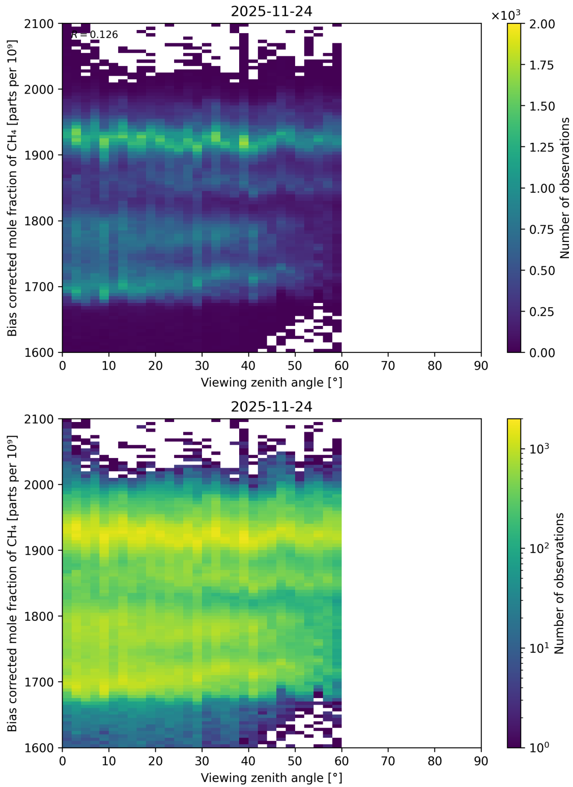
Figure 127: Scatter density plot of “Viewing zenith angle” against “Bias corrected mole fraction of CH 4 ” for 2025-11-23 to 2025-11-25.
