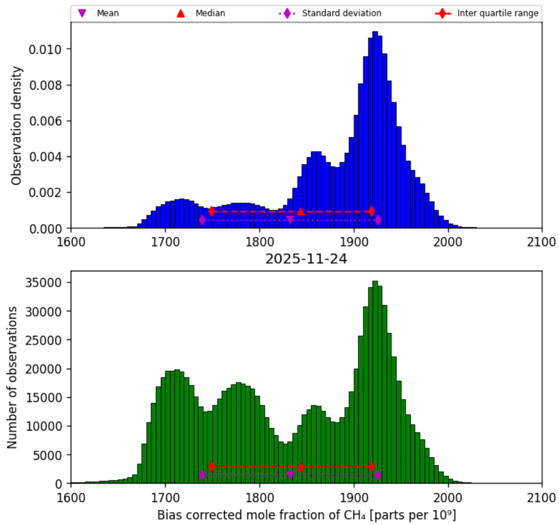
Figure 27: Histogram of “Bias corrected mole fraction of CH 4 ” for 2025-11-23 to 2025-11-25
