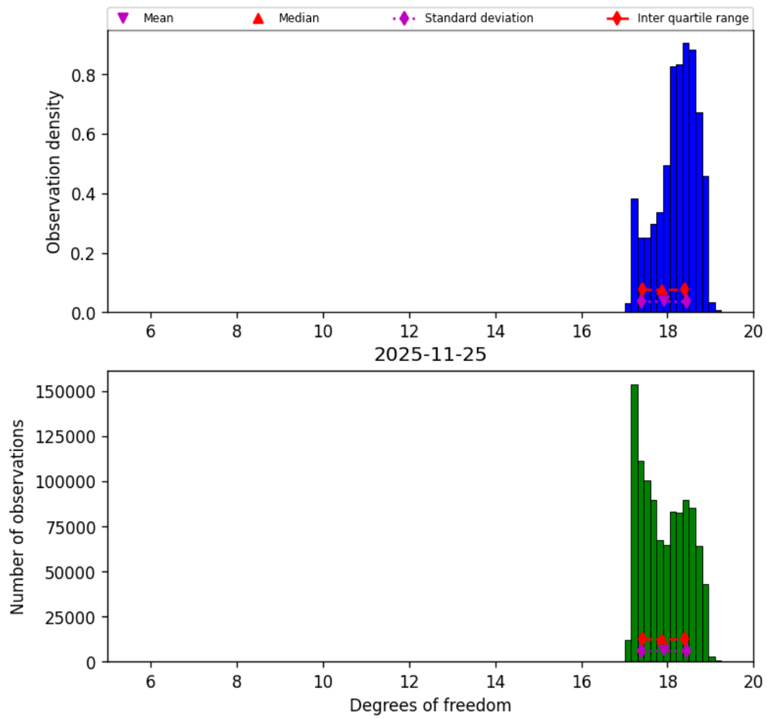
Figure 32: Histogram of “Degrees of freedom” for 2025-11-24 to 2025-11-26
