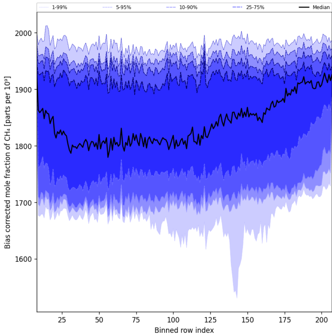
Figure 39: Along track statistics of “Bias corrected mole fraction of CH 4 ” for 2025-11-24 to 2025-11-26
