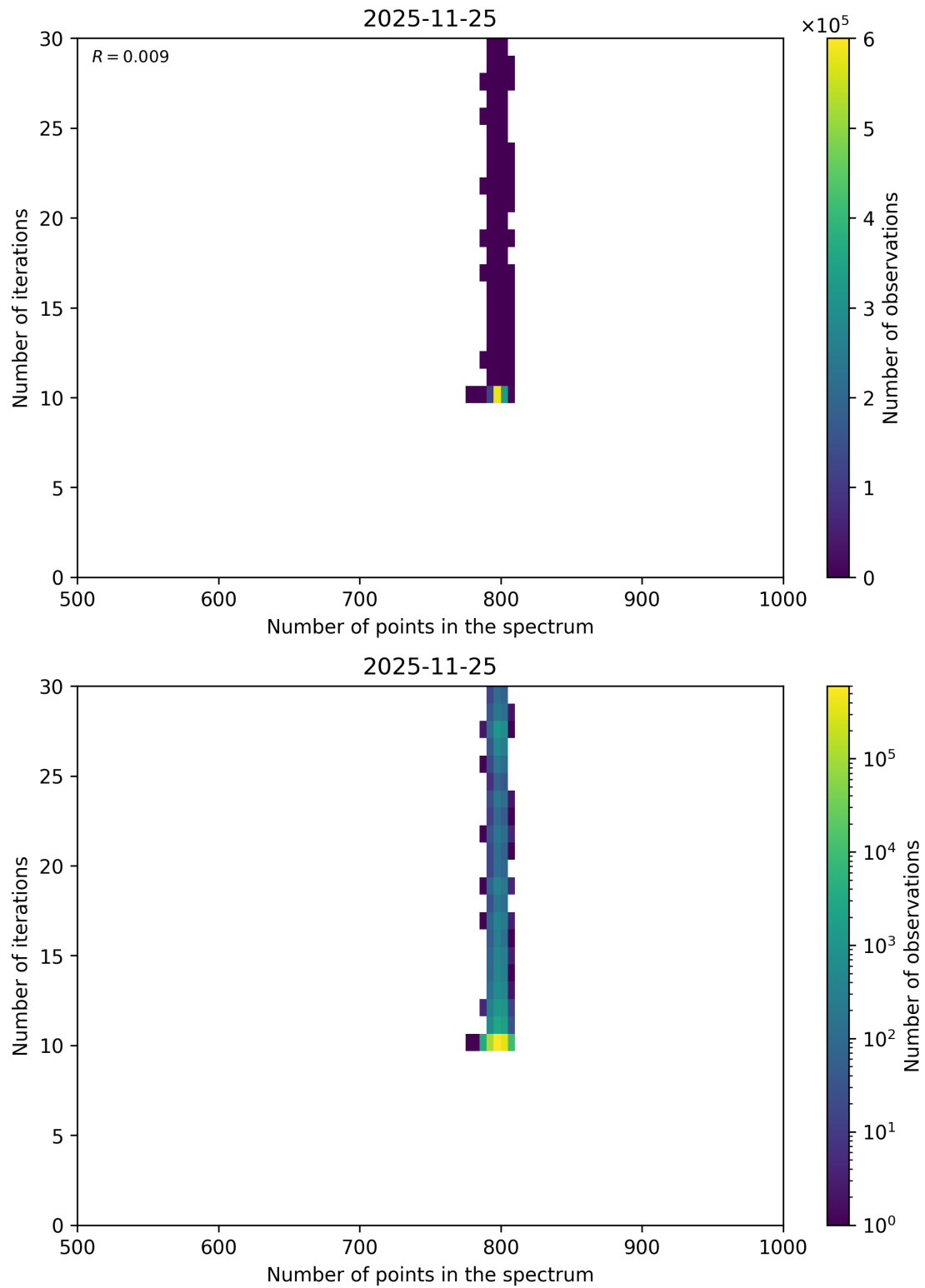
Figure 106: Scatter density plot of “Number of points in the spectrum” against “Number of iterations” for 2025-11-24 to 2025-11-26.
