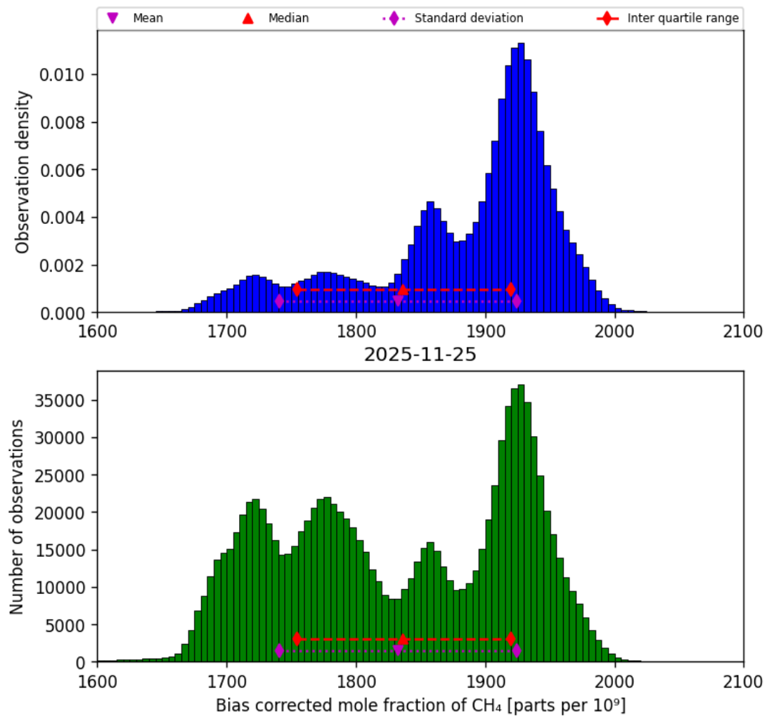
Figure 27: Histogram of “Bias corrected mole fraction of CH 4 ” for 2025-11-24 to 2025-11-26
