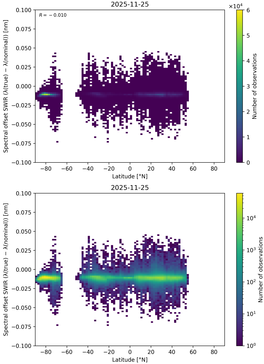
Figure 71: Scatter density plot of “Latitude” against “Spectral offset SWIR ( \lambda_{\text{true}} - \lambda_{\text{nominal}} )” for 2025-11-24 to 2025-11-26.
