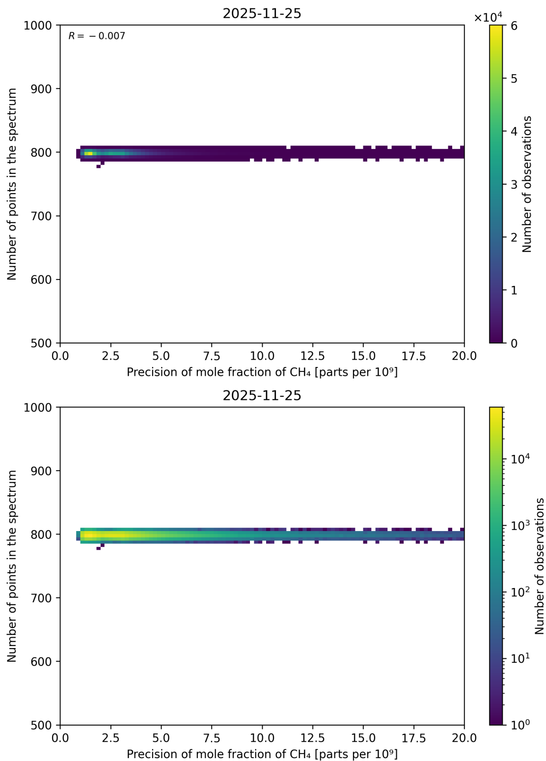
Figure 96: Scatter density plot of “Precision of mole fraction of CH 4 ” against “Number of points in the spectrum” for 2025-11-24 to 2025-11-26.
