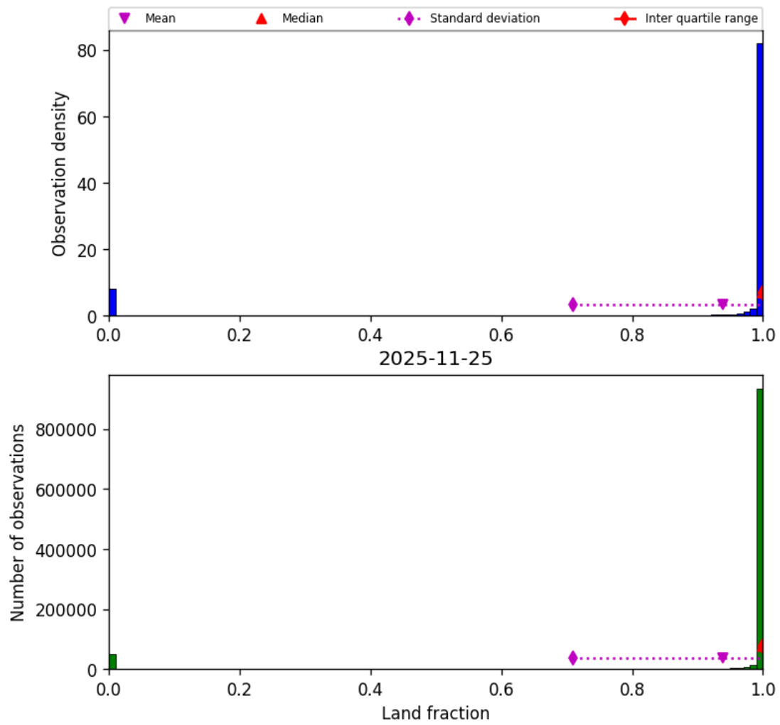
Figure 35: Histogram of “Land fraction” for 2025-11-24 to 2025-11-26
