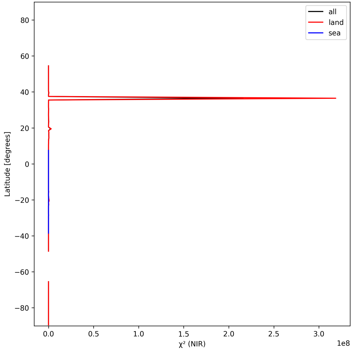
Figure 19: Zonal average of “ \chi^2 (NIR)” for 2025-11-24 to 2025-11-26.
