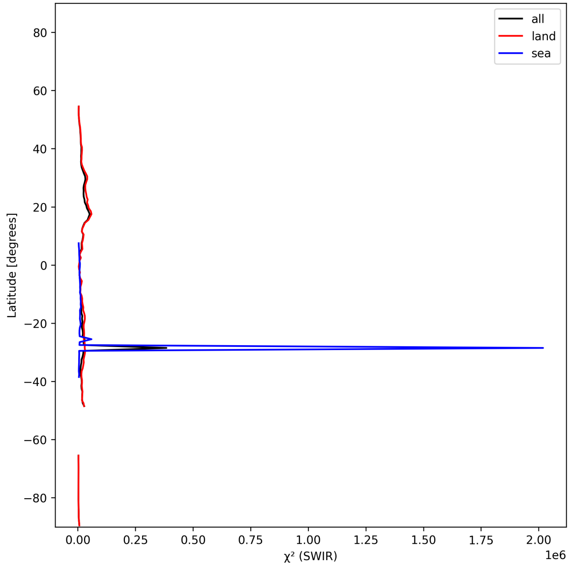
Figure 18: Zonal average of “ \chi^2 (SWIR)” for 2025-11-24 to 2025-11-26.
