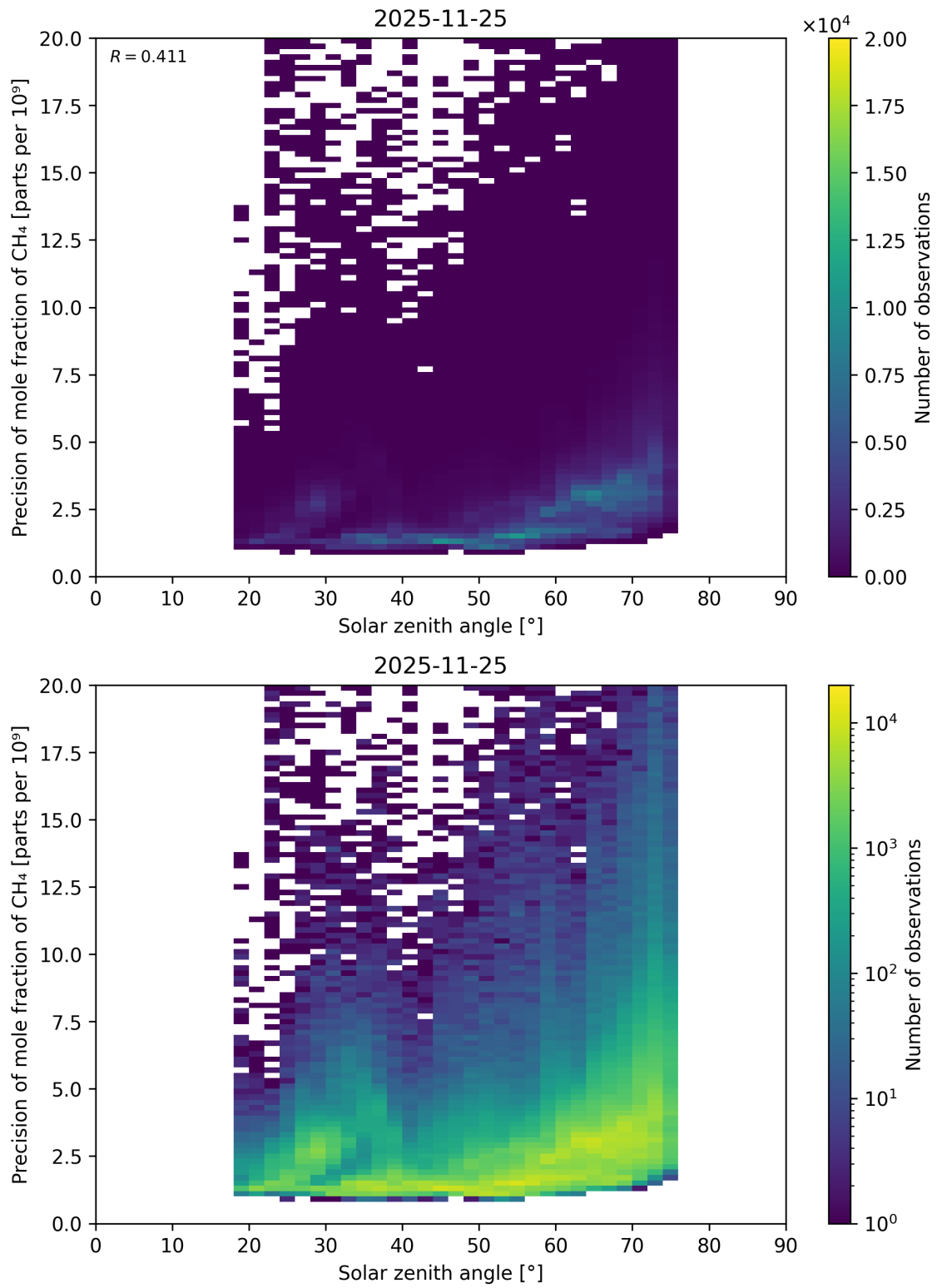
Figure 116: Scatter density plot of “Solar zenith angle” against “Precision of mole fraction of \text{CH}_4 ” for 2025-11-24 to 2025-11-26.
