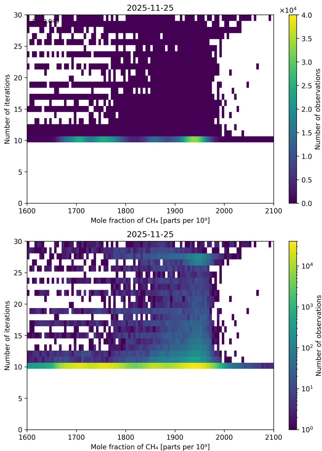
Figure 87: Scatter density plot of “Mole fraction of CH 4 ” against “Number of iterations” for 2025-11-24 to 2025-11-26.
