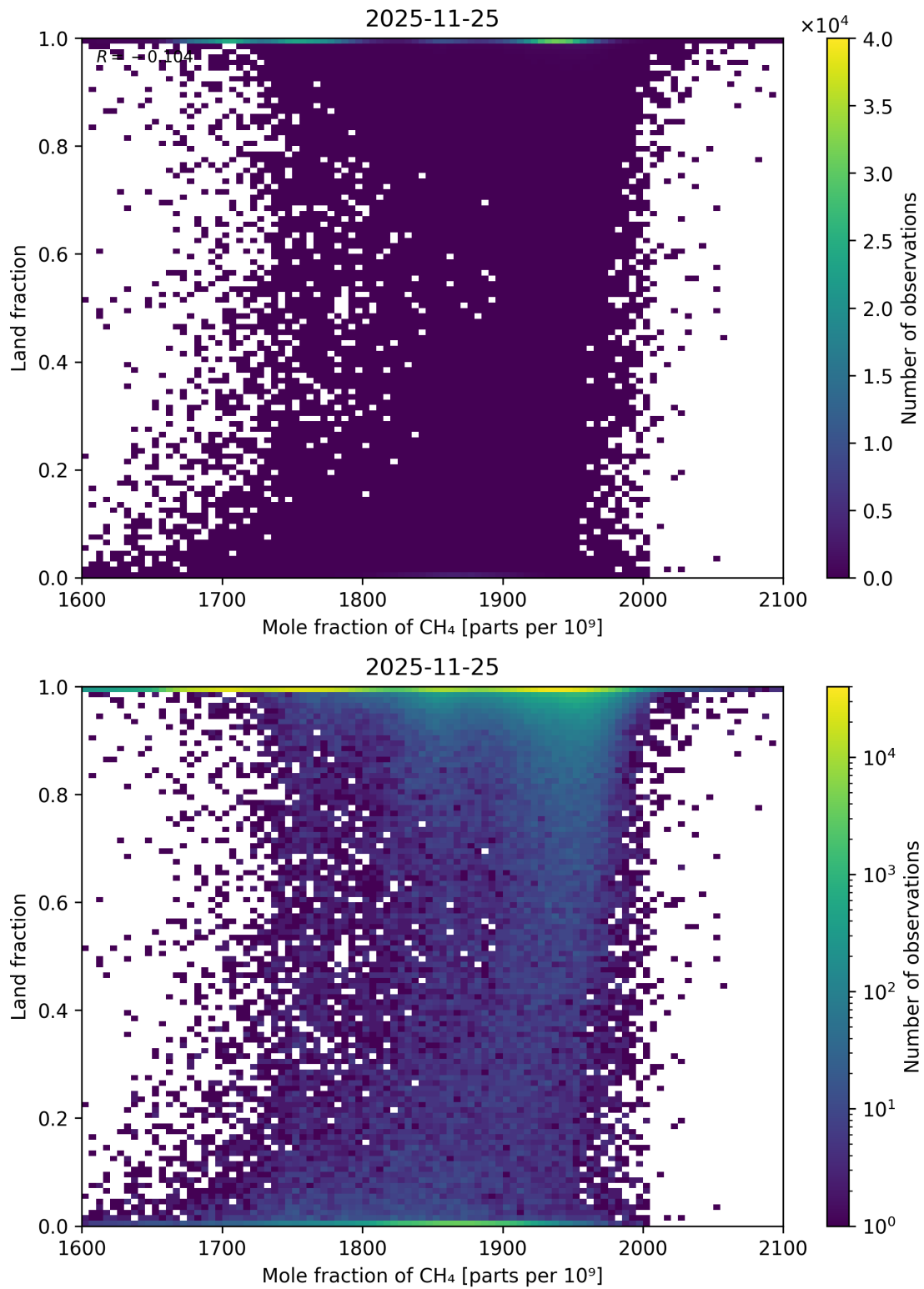
Figure 84: Scatter density plot of “Mole fraction of CH 4 ” against “Land fraction” for 2025-11-24 to 2025-11-26.
