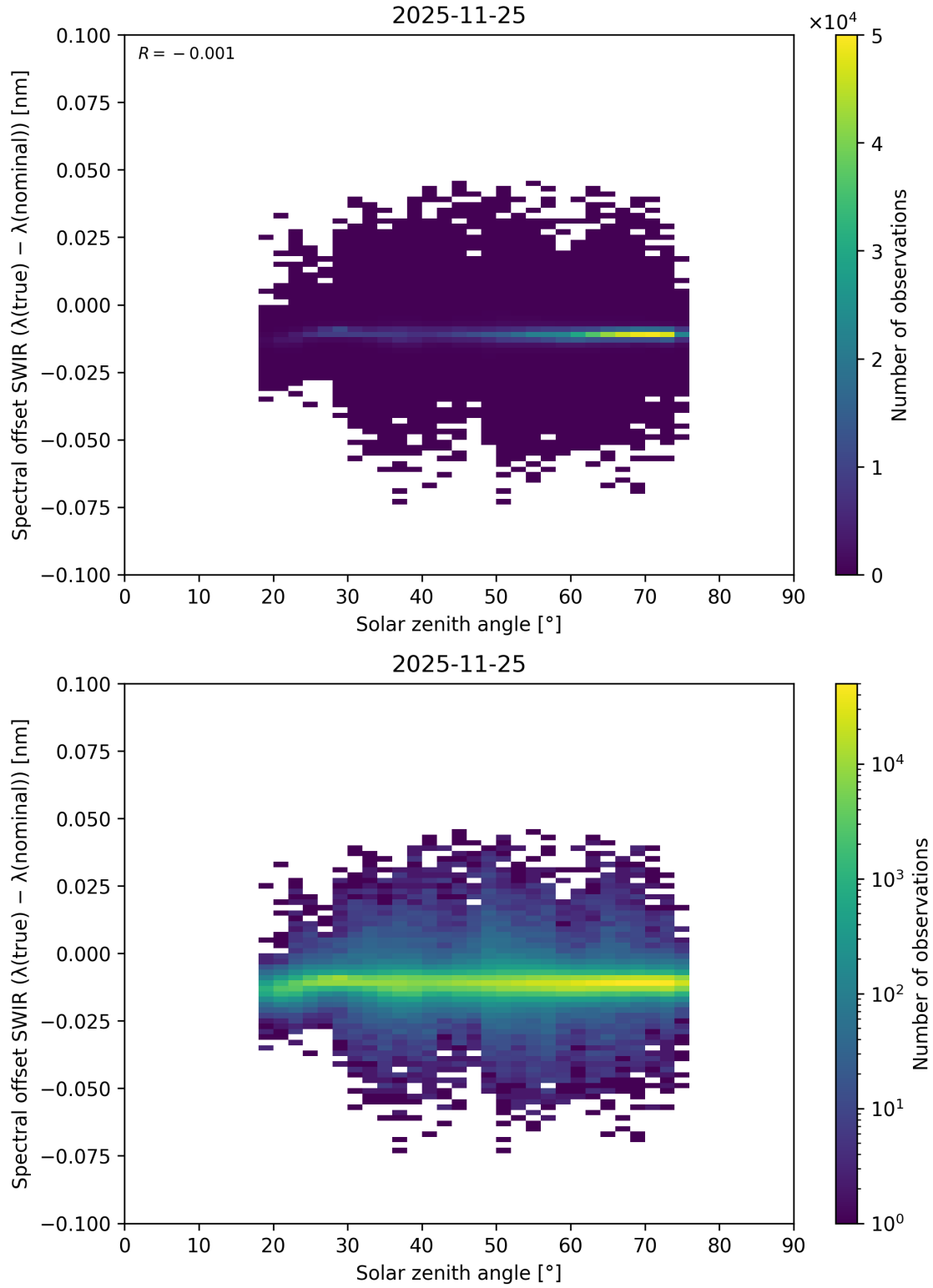
Figure 119: Scatter density plot of “Solar zenith angle” against “Spectral offset SWIR ( \lambda_{\text{true}} - \lambda_{\text{nominal}} )” for 2025-11-24 to 2025-11-26.
