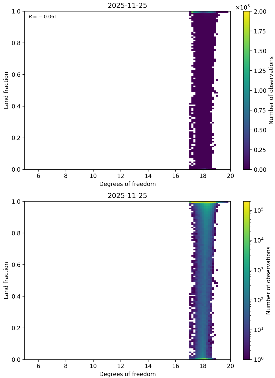
Figure 58: Scatter density plot of “Degrees of freedom” against “Land fraction” for 2025-11-24 to 2025-11-26.
