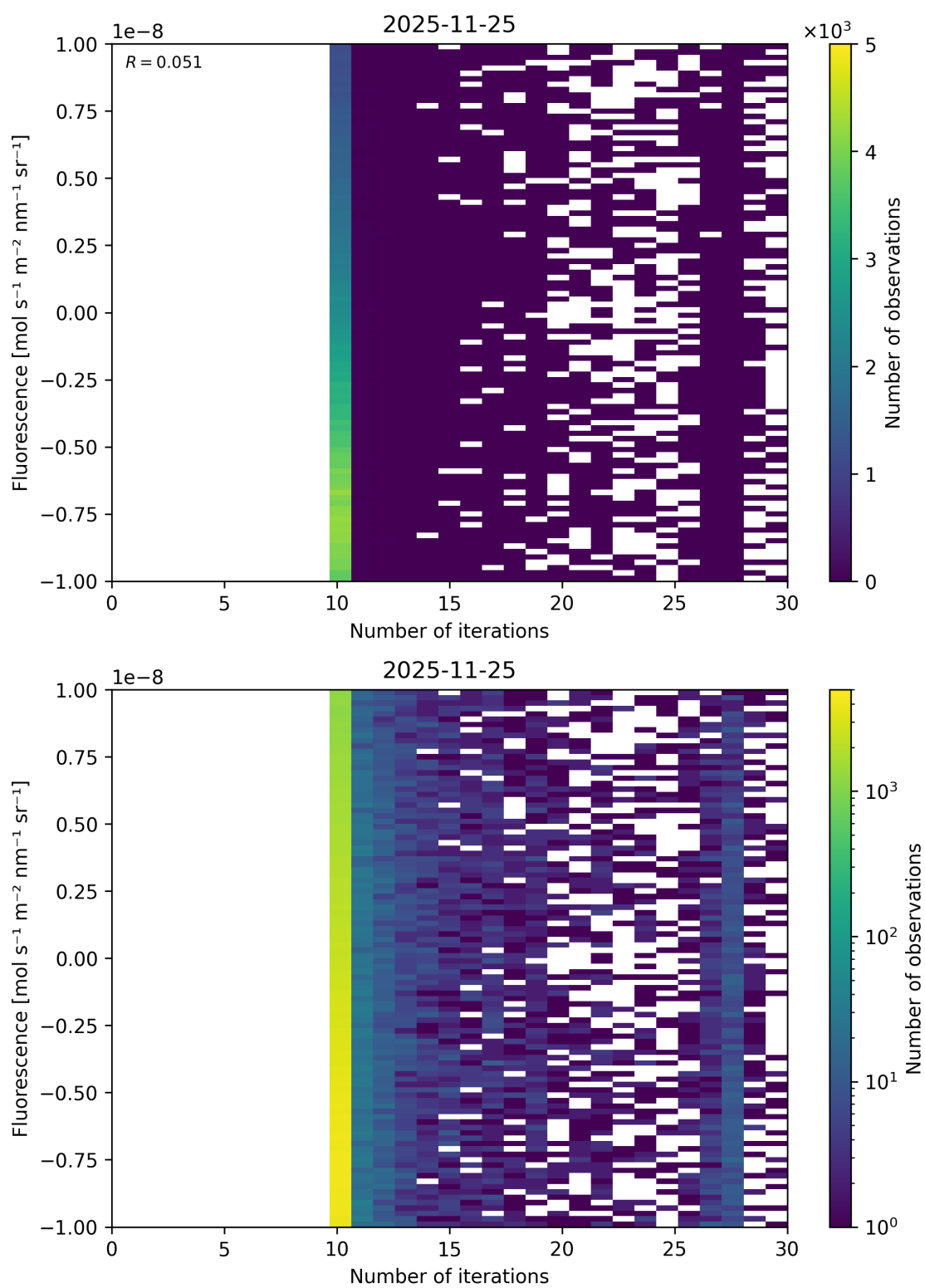
Figure 99: Scatter density plot of “Number of iterations” against “Fluorescence” for 2025-11-24 to 2025-11-26.
