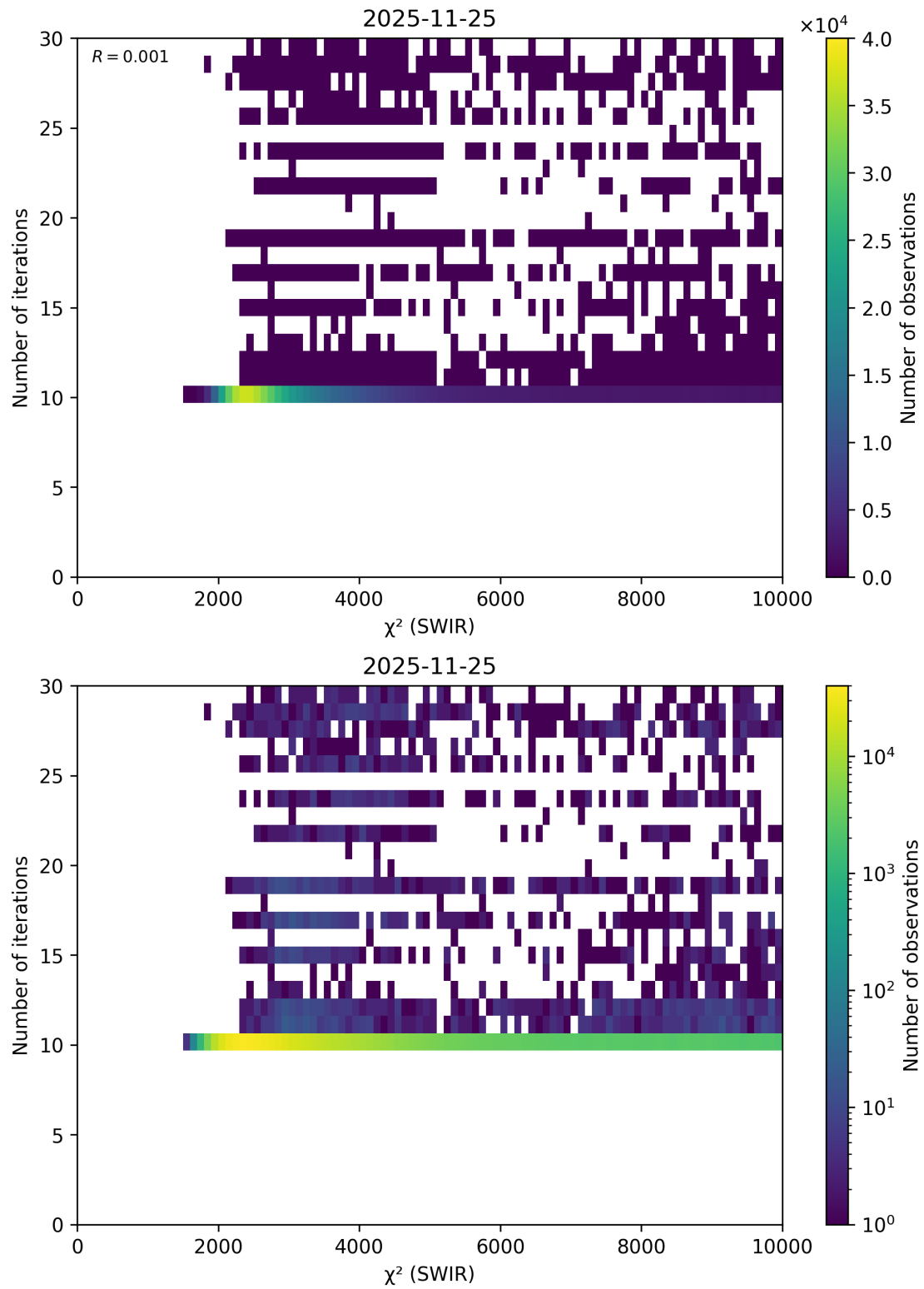
Figure 56: Scatter density plot of “ \chi^2 (SWIR)” against “Number of iterations” for 2025-11-24 to 2025-11-26.
