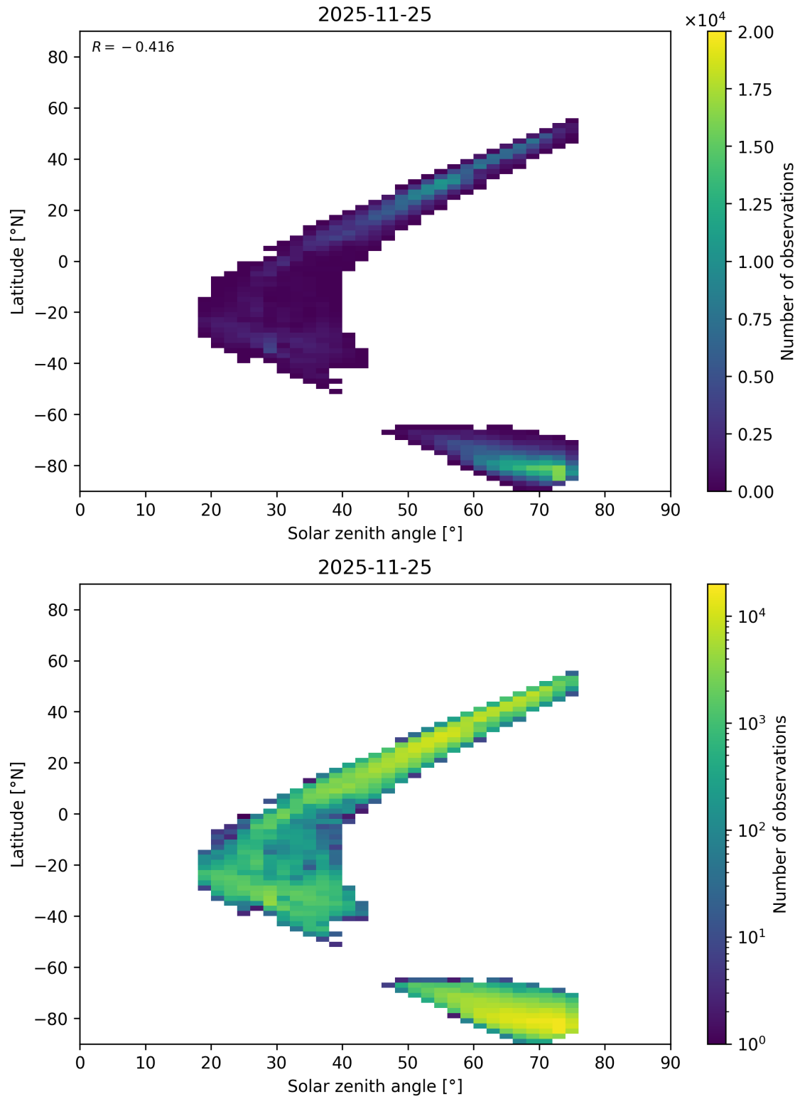
Figure 113: Scatter density plot of “Solar zenith angle” against “Latitude” for 2025-11-24 to 2025-11-26.
