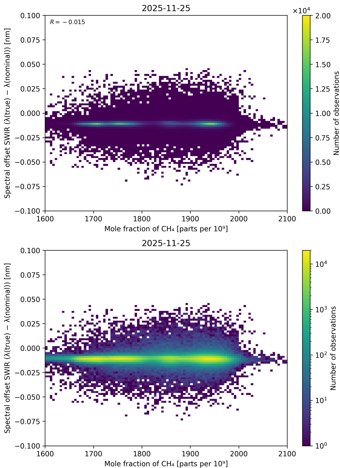
Figure 98: Scatter density plot of “Mole fraction of CH 4 ” against “Spectral offset SWIR ( \lambda_{\text{true}} - \lambda_{\text{nominal}} )” for 2025-11-24 to 2025-11-26.
