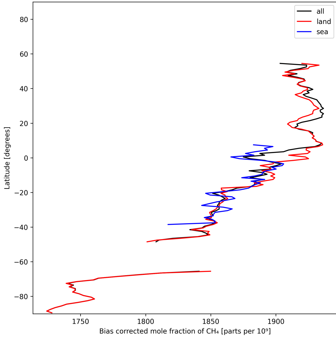
Figure 15: Zonal average of “Bias corrected mole fraction of CH 4 ” for 2025-11-24 to 2025-11-26.
