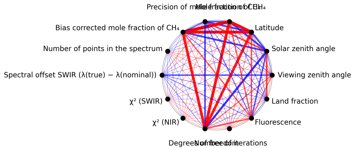
Figure 1: Map of correlation graph for 2025-11-24 to 2025-11-26.
