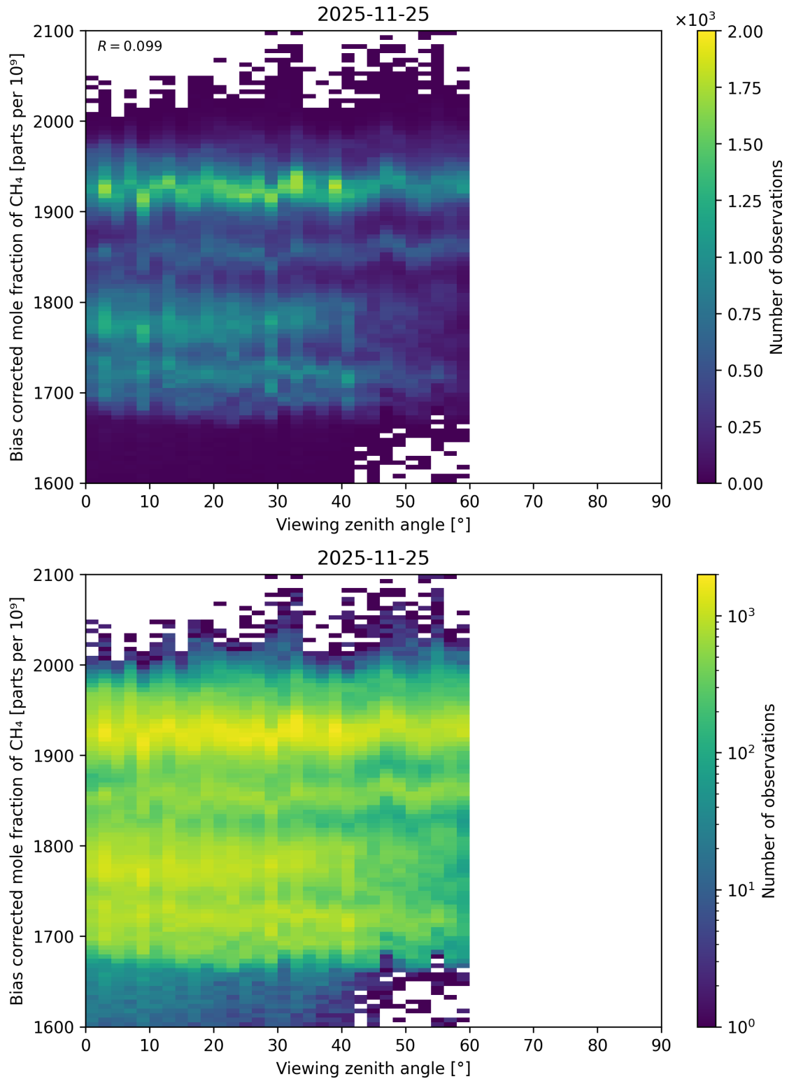
Figure 127: Scatter density plot of “Viewing zenith angle” against “Bias corrected mole fraction of CH 4 ” for 2025-11-24 to 2025-11-26.
