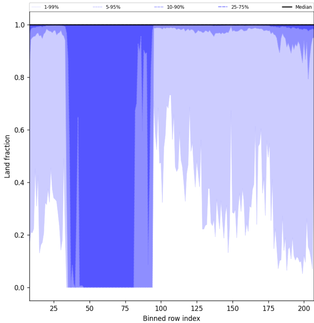
Figure 47: Along track statistics of "Land fraction" for 2025-11-24 to 2025-11-26
