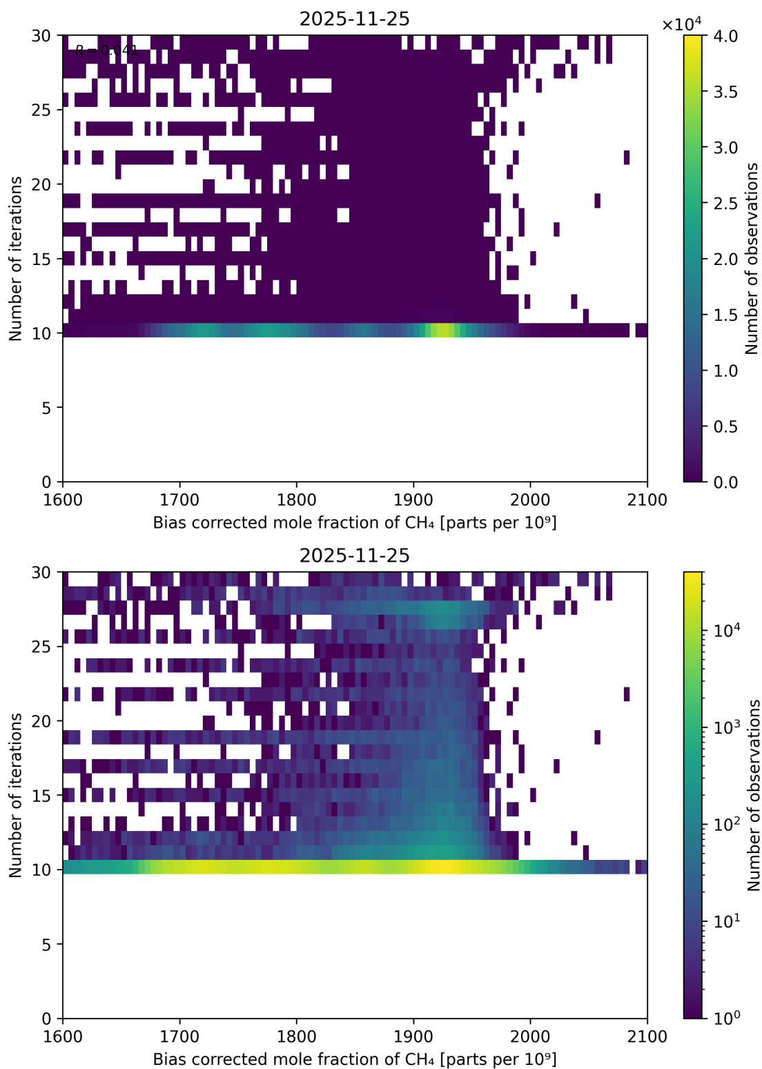
Figure 77: Scatter density plot of “Bias corrected mole fraction of CH 4 ” against “Number of iterations” for 2025-11-24 to 2025-11-26.
