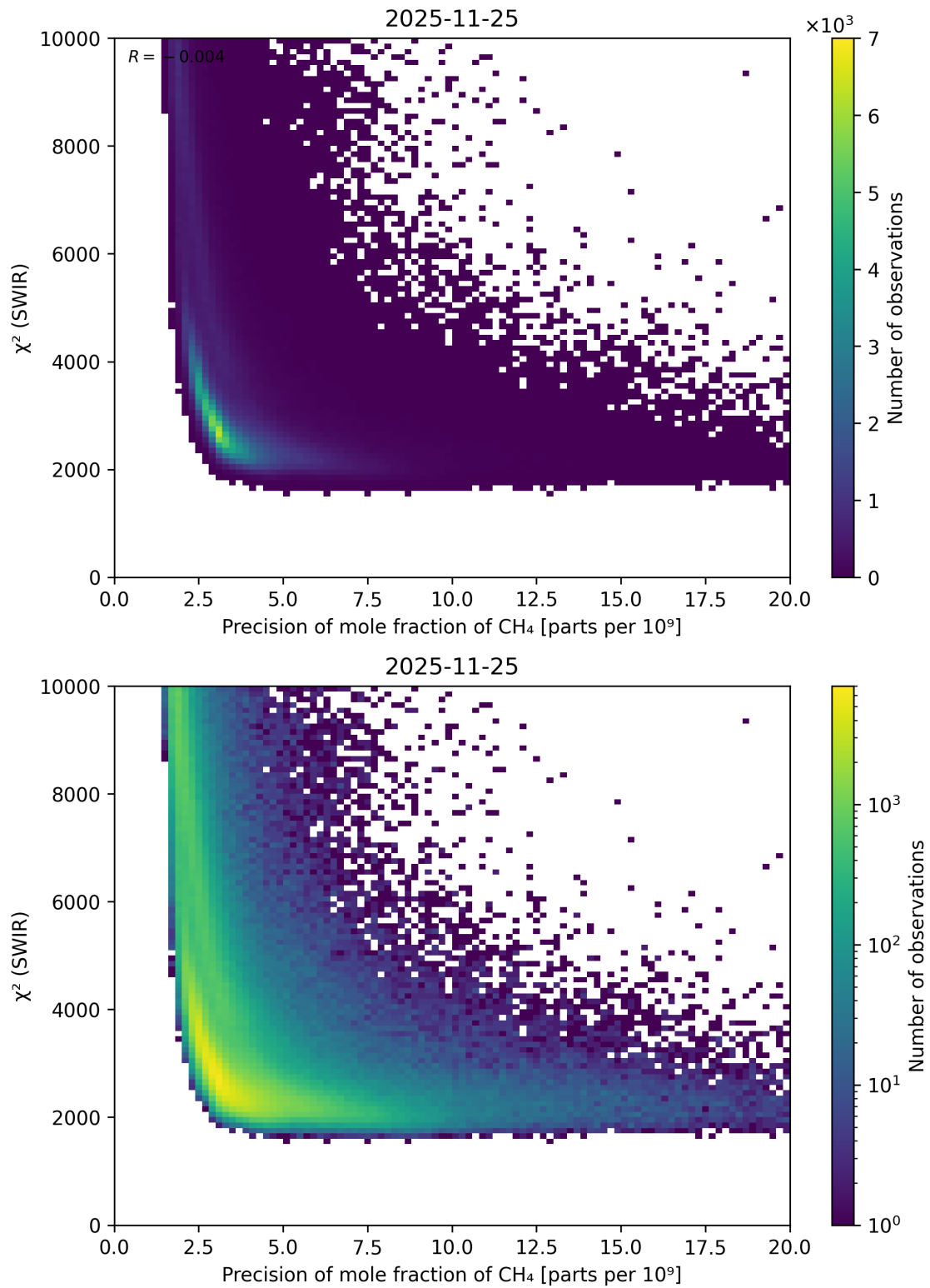
Figure 90: Scatter density plot of “Precision of mole fraction of CH 4 ” against “ \chi^2 (SWIR)” for 2025-11-24 to 2025-11-26.
