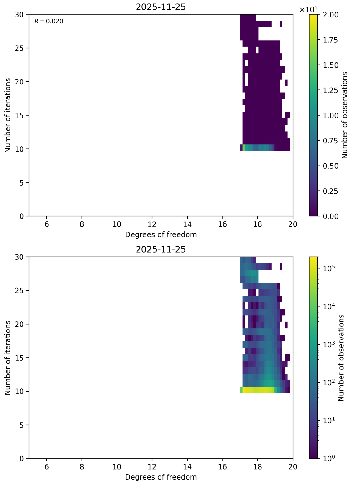
Figure 59: Scatter density plot of “Degrees of freedom” against “Number of iterations” for 2025-11-24 to 2025-11-26.
