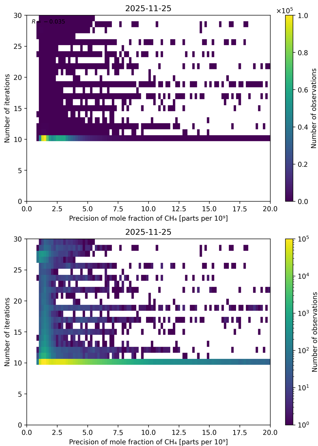
Figure 95: Scatter density plot of “Precision of mole fraction of CH 4 ” against “Number of iterations” for 2025-11-24 to 2025-11-26.
