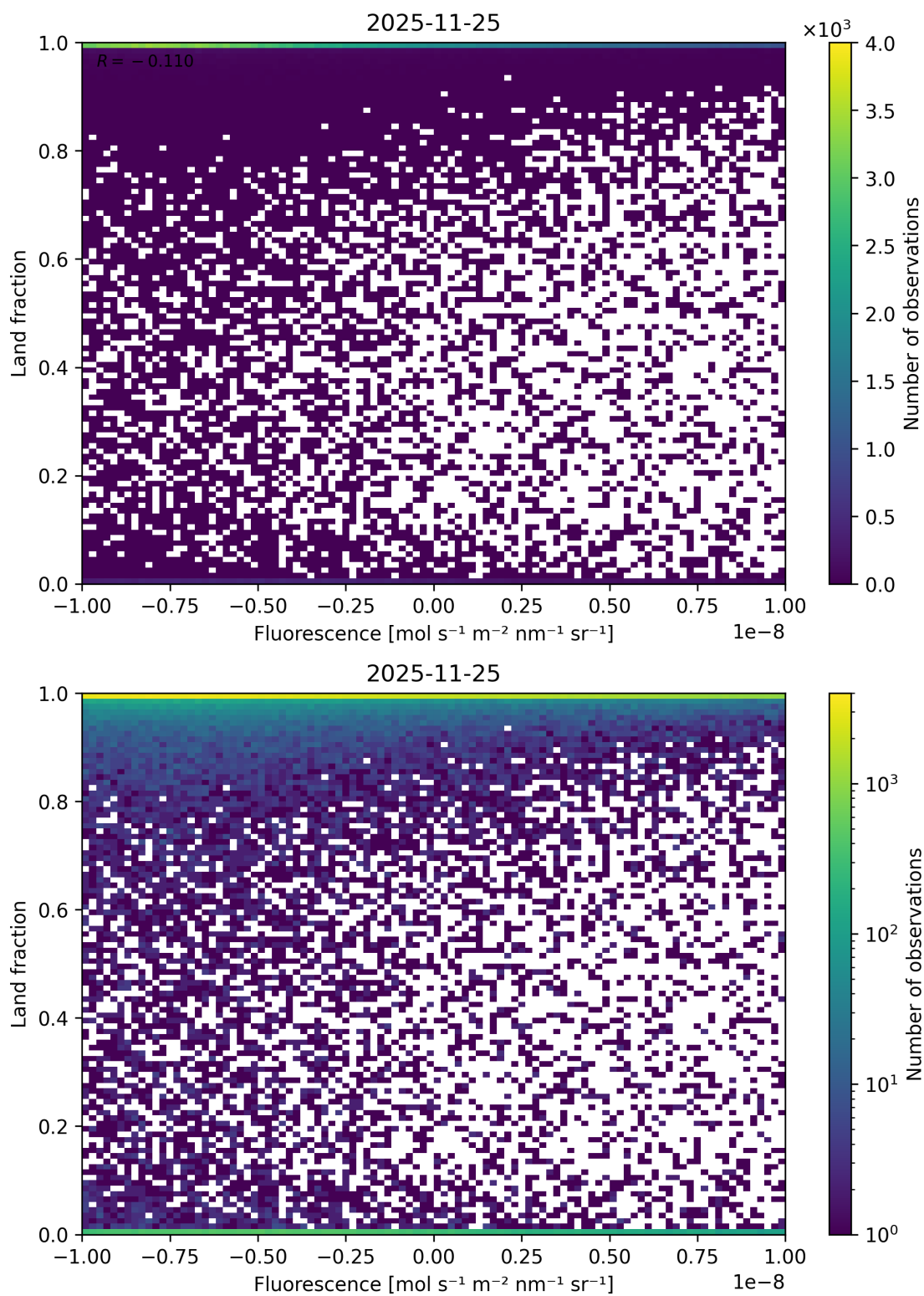
Figure 60: Scatter density plot of “Fluorescence” against “Land fraction” for 2025-11-24 to 2025-11-26.
