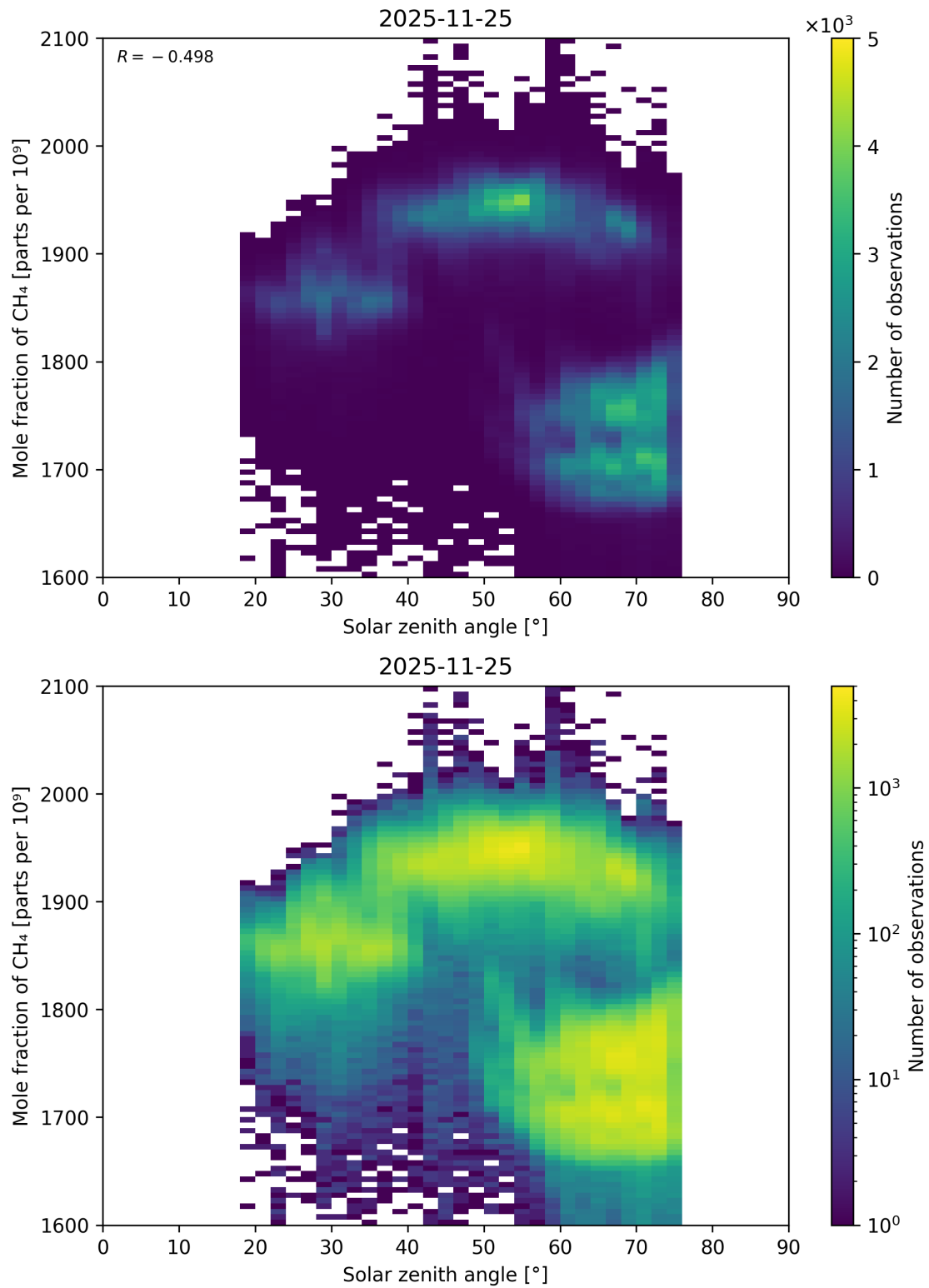
Figure 114: Scatter density plot of “Solar zenith angle” against “Mole fraction of CH 4 ” for 2025-11-24 to 2025-11-26.
