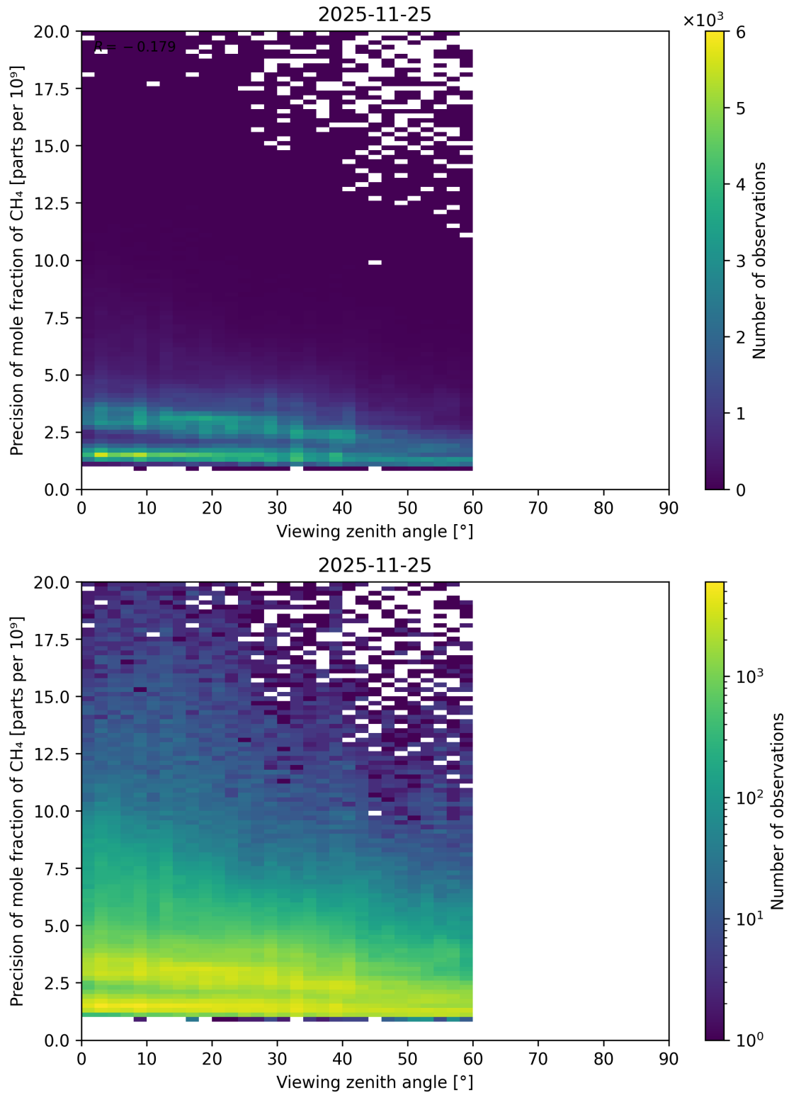
Figure 128: Scatter density plot of “Viewing zenith angle” against “Precision of mole fraction of CH 4 ” for 2025-11-24 to 2025-11-26.
