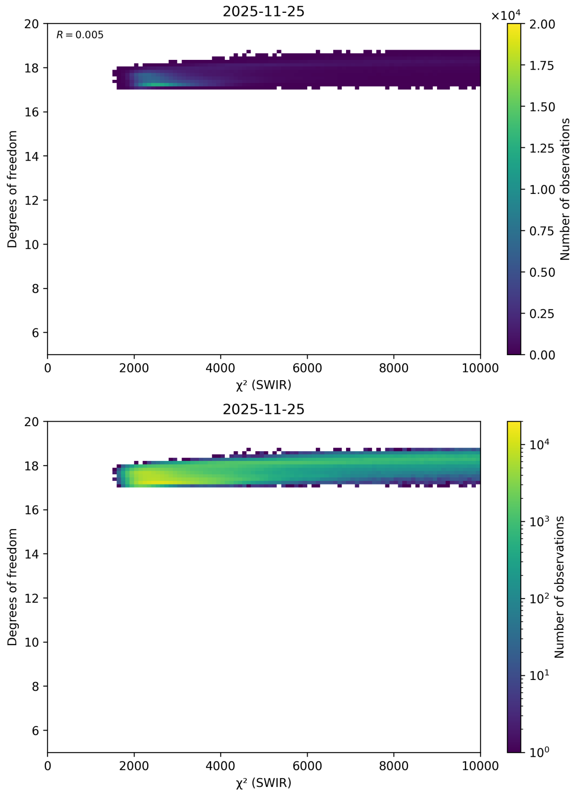
Figure 53: Scatter density plot of “ \chi^2 (SWIR)” against “Degrees of freedom” for 2025-11-24 to 2025-11-26.
