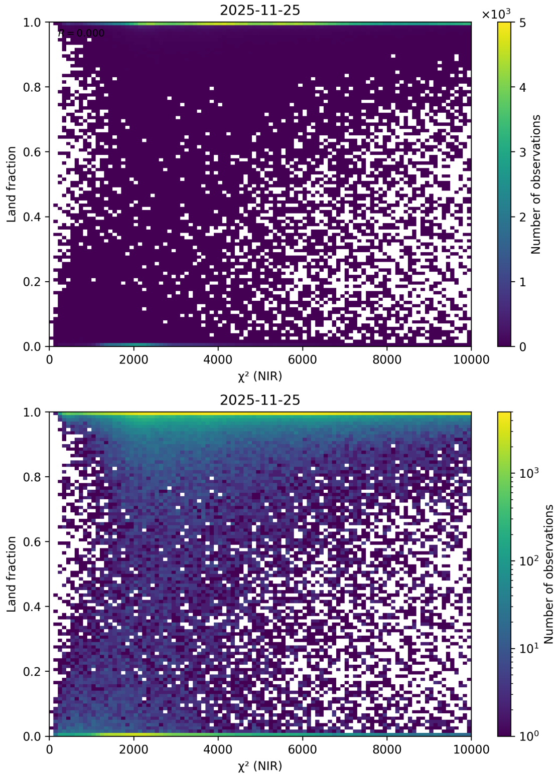
Figure 50: Scatter density plot of " \chi^2 (NIR)" against "Land fraction" for 2025-11-24 to 2025-11-26.
