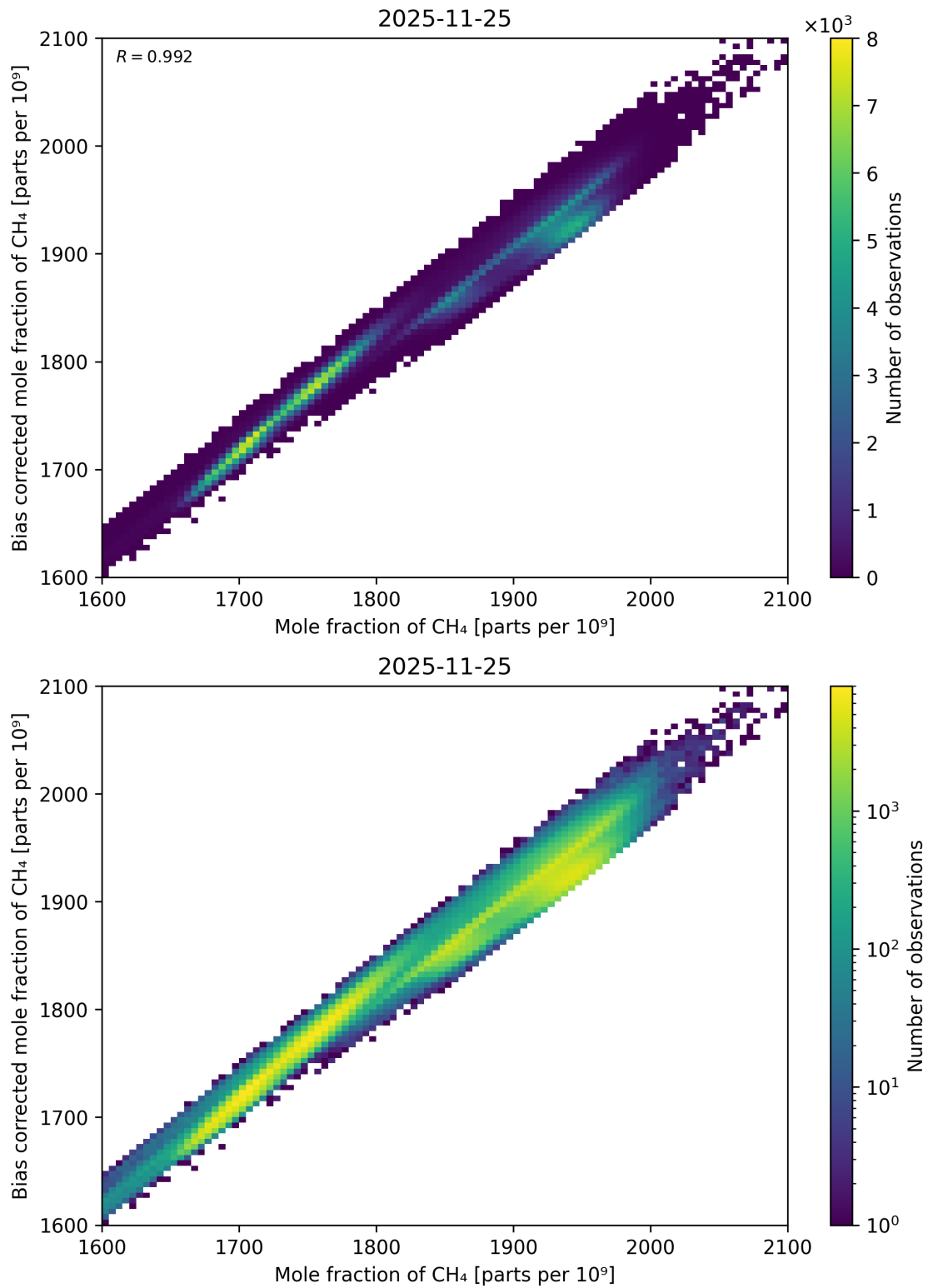
Figure 85: Scatter density plot of “Mole fraction of CH 4 ” against “Bias corrected mole fraction of CH 4 ” for 2025-11-24 to 2025-11-26.
