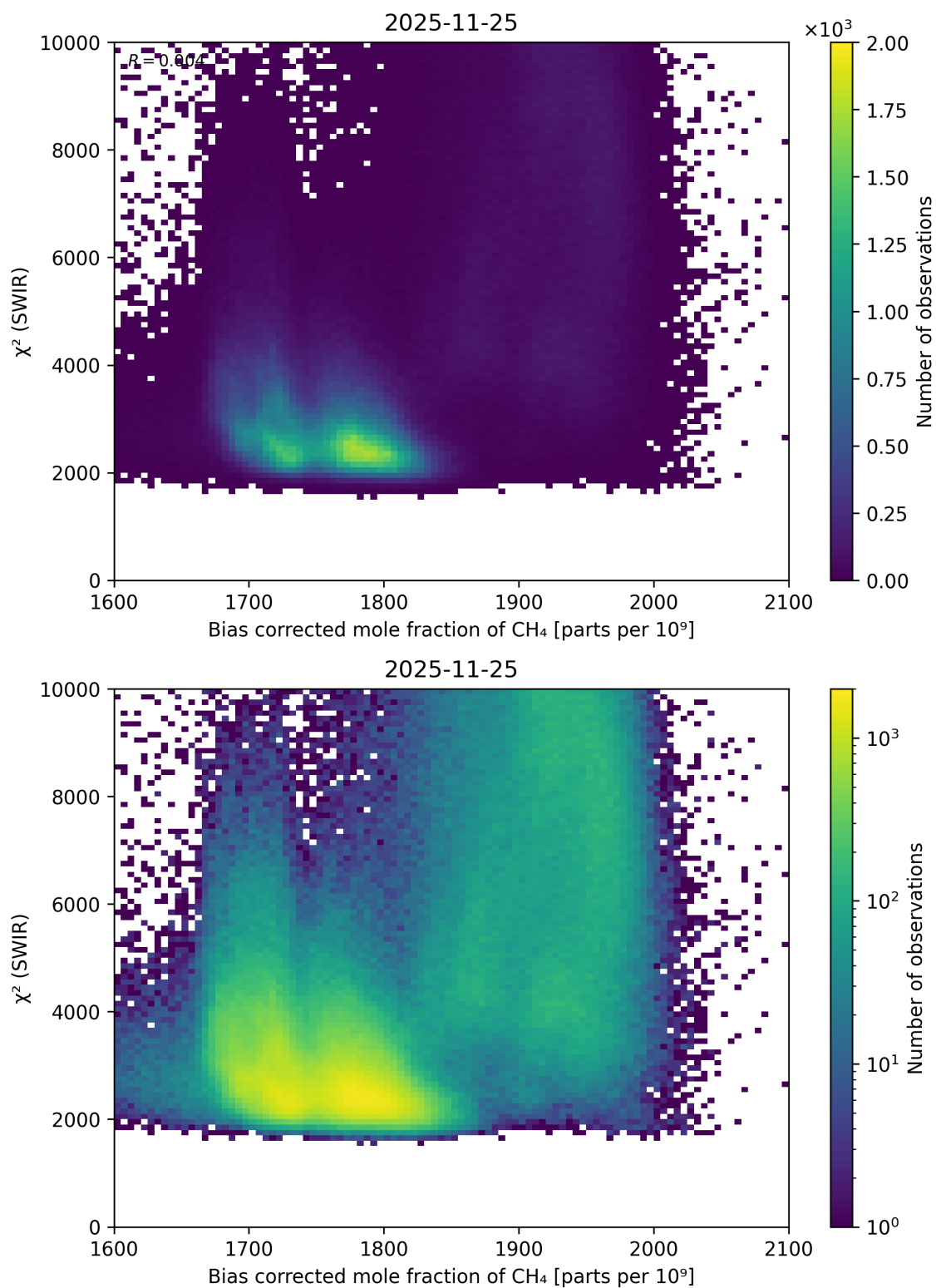
Figure 73: Scatter density plot of “Bias corrected mole fraction of CH 4 ” against “ \chi^2 (SWIR)” for 2025-11-24 to 2025-11-26.
