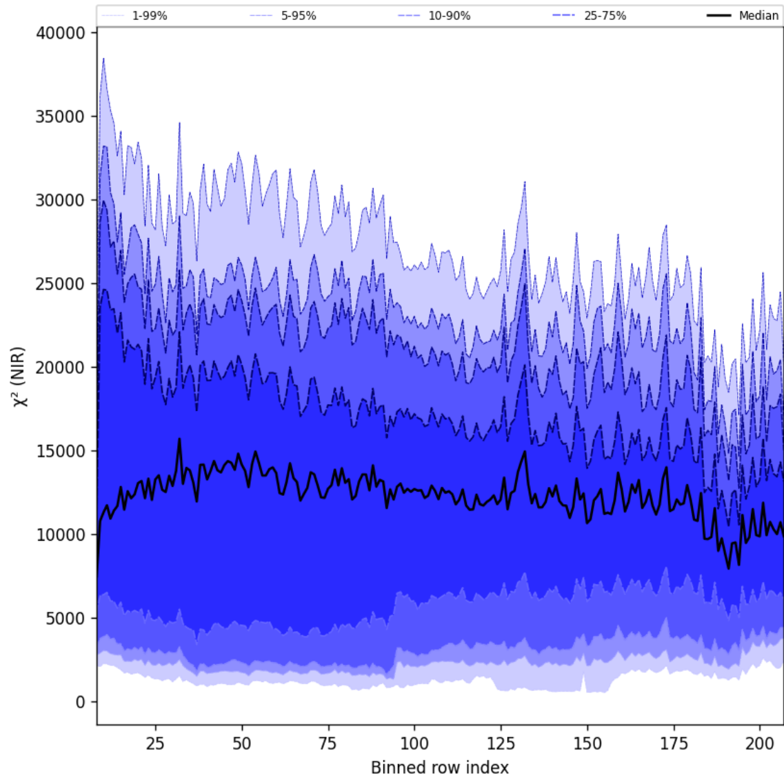
Figure 43: Along track statistics of “ \chi^2 (NIR)” for 2025-11-24 to 2025-11-26
