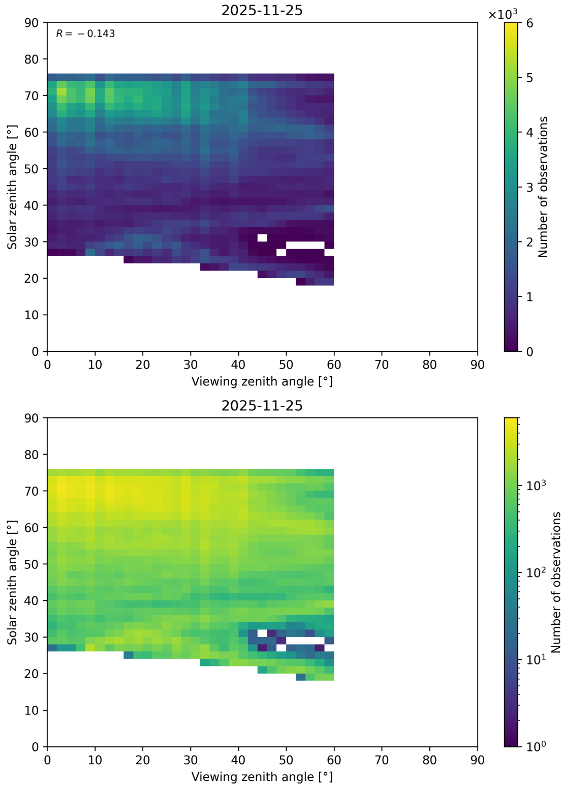
Figure 131: Scatter density plot of “Viewing zenith angle” against “Solar zenith angle” for 2025-11-24 to 2025-11-26.
