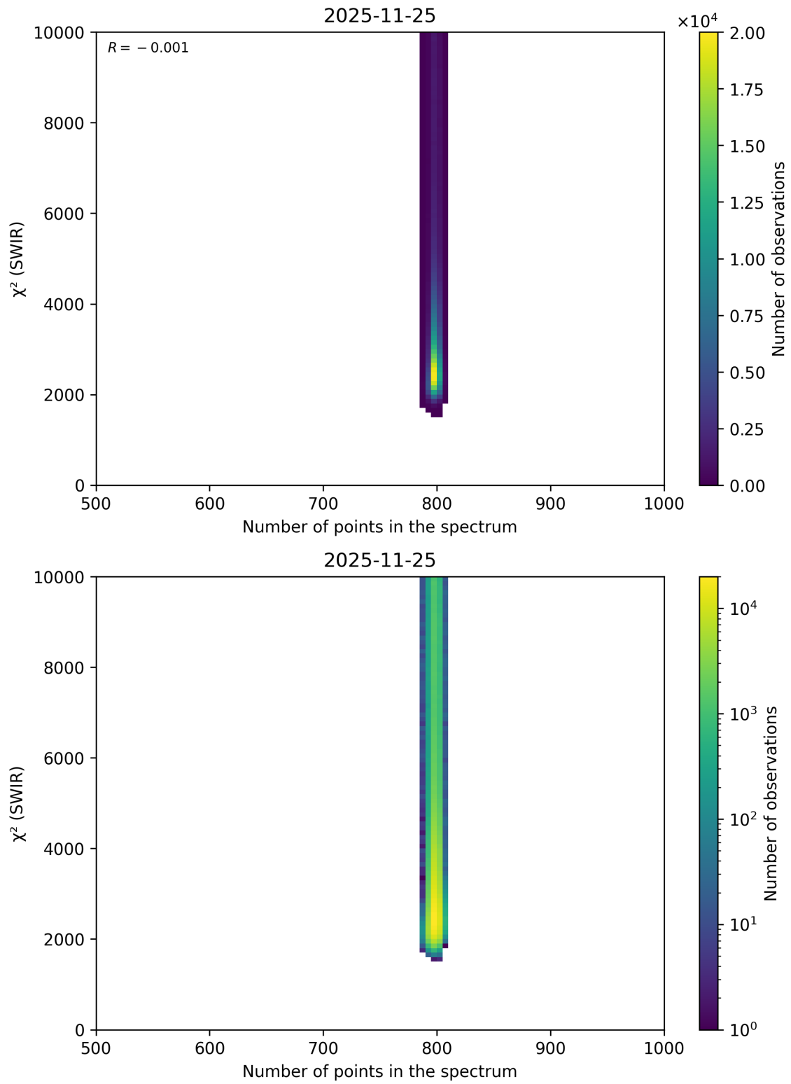
Figure 102: Scatter density plot of “Number of points in the spectrum” against “ \chi^2 (SWIR)” for 2025-11-24 to 2025-11-26.
