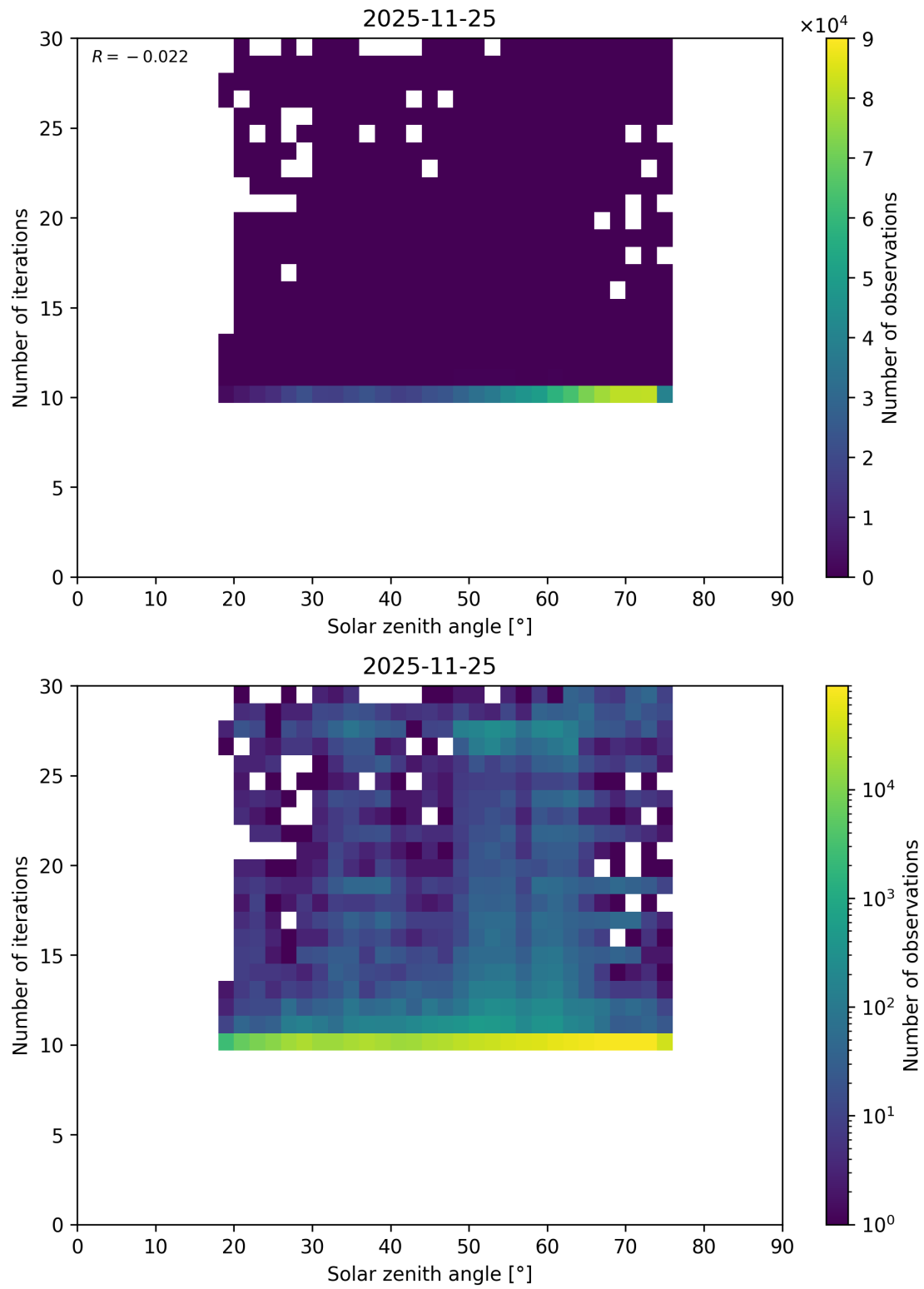
Figure 117: Scatter density plot of “Solar zenith angle” against “Number of iterations” for 2025-11-24 to 2025-11-26.
