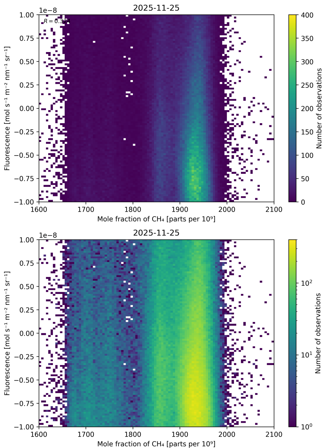
Figure 83: Scatter density plot of “Mole fraction of \text{CH}_4 ” against “Fluorescence” for 2025-11-24 to 2025-11-26.
