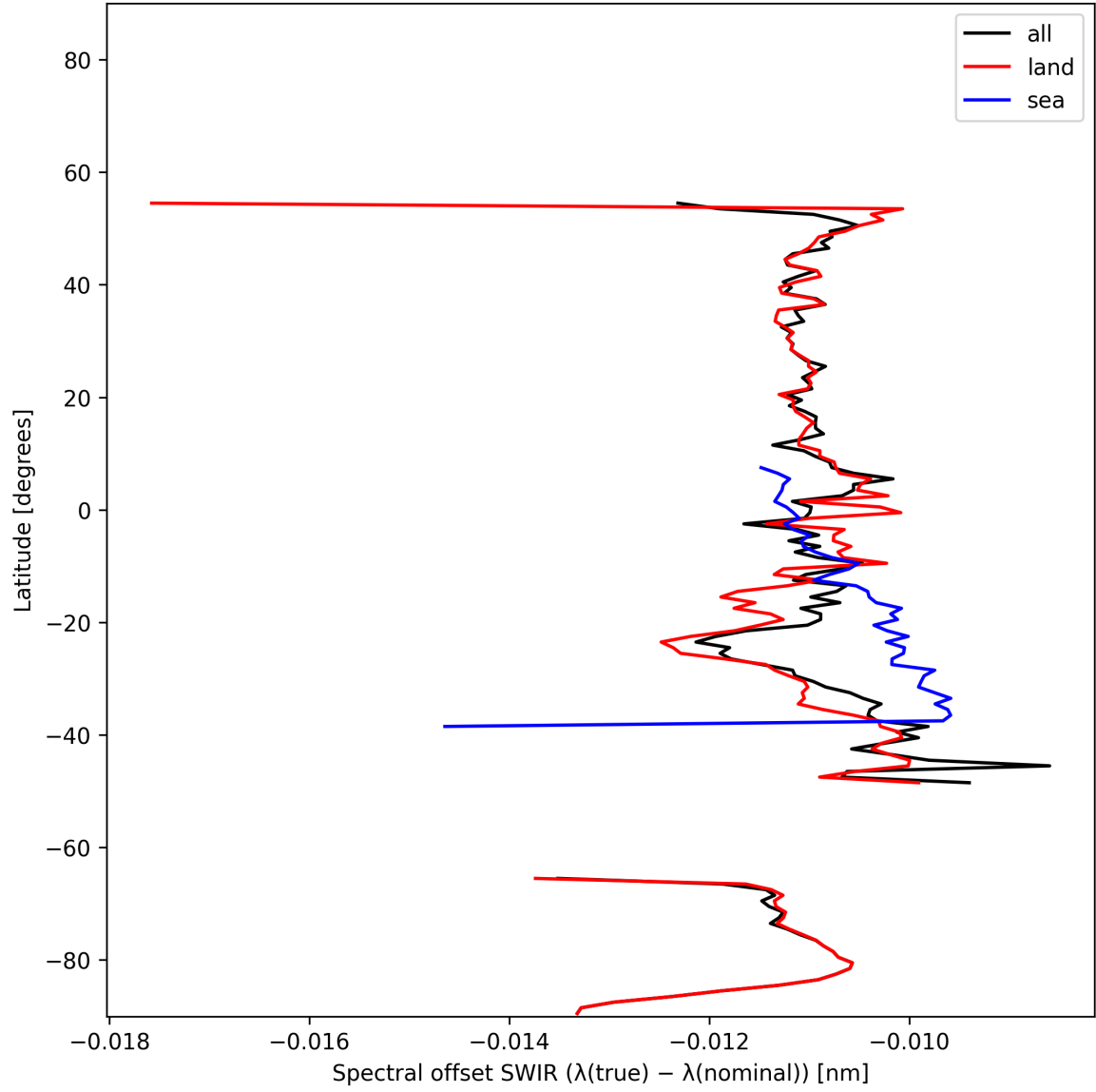
Figure 17: Zonal average of “Spectral offset SWIR ( \lambda_{\text{true}} - \lambda_{\text{nominal}} )” for 2025-11-24 to 2025-11-26.
