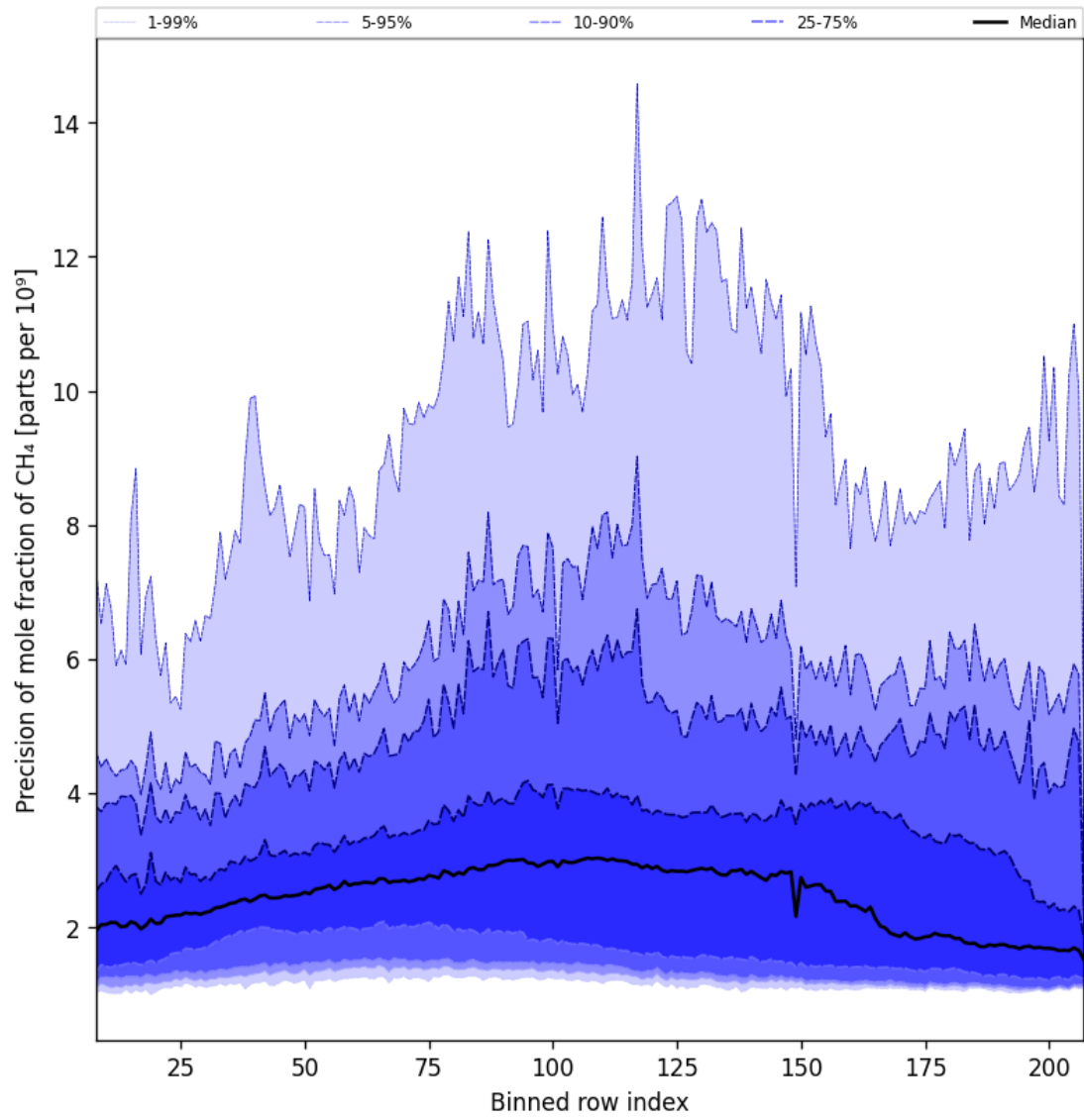
Figure 38: Along track statistics of “Precision of mole fraction of CH 4 ” for 2025-11-24 to 2025-11-26
