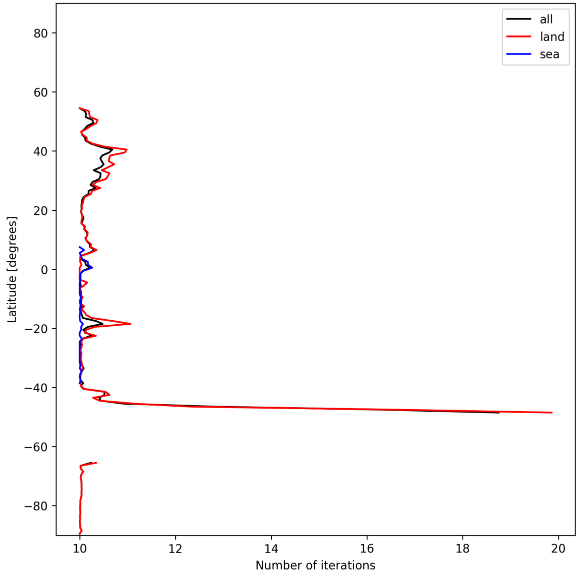
Figure 21: Zonal average of “Number of iterations” for 2025-11-24 to 2025-11-26.
