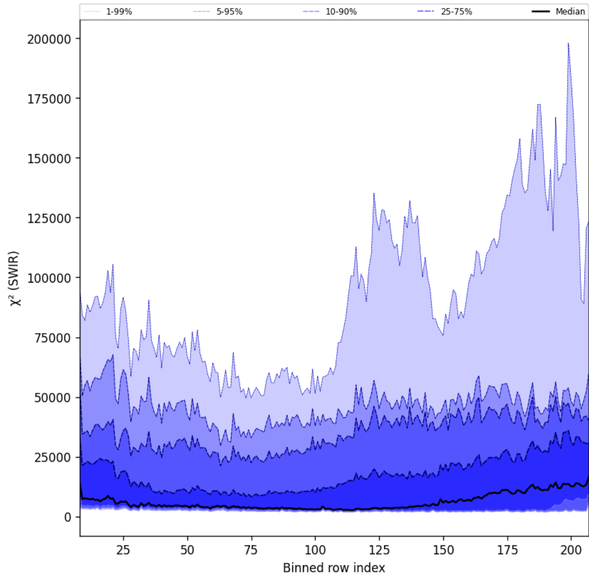
Figure 42: Along track statistics of “ \chi^2 (SWIR)” for 2025-11-24 to 2025-11-26
