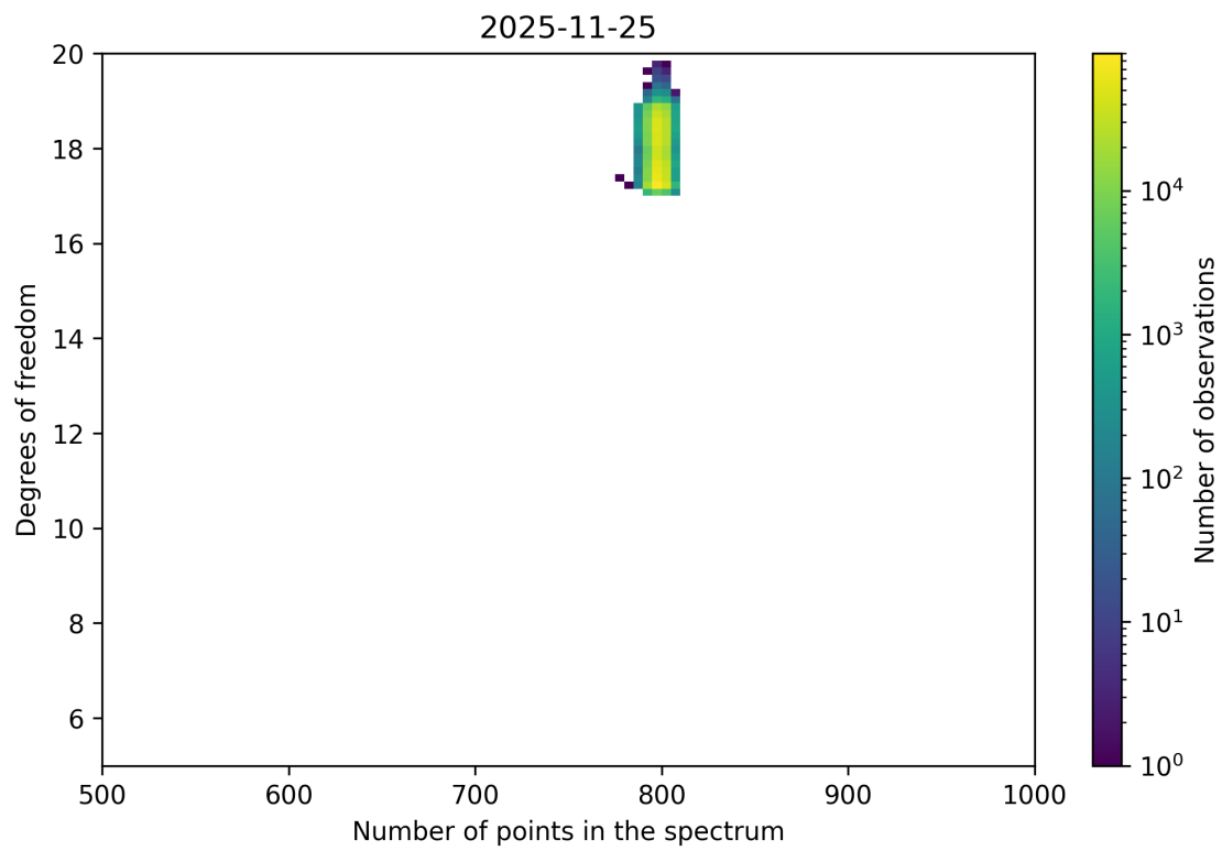
Figure 103: Scatter density plot of “Number of points in the spectrum” against “Degrees of freedom” for 2025-11-24 to 2025-11-26.
