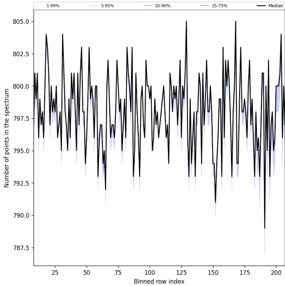
Figure 40: Along track statistics of “Number of points in the spectrum” for 2025-11-24 to 2025-11-26
