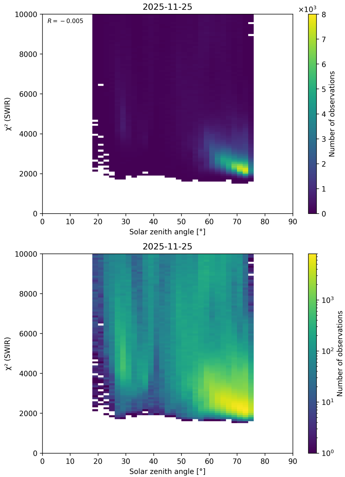
Figure 109: Scatter density plot of “Solar zenith angle” against “ \chi^2 (SWIR)” for 2025-11-24 to 2025-11-26.
