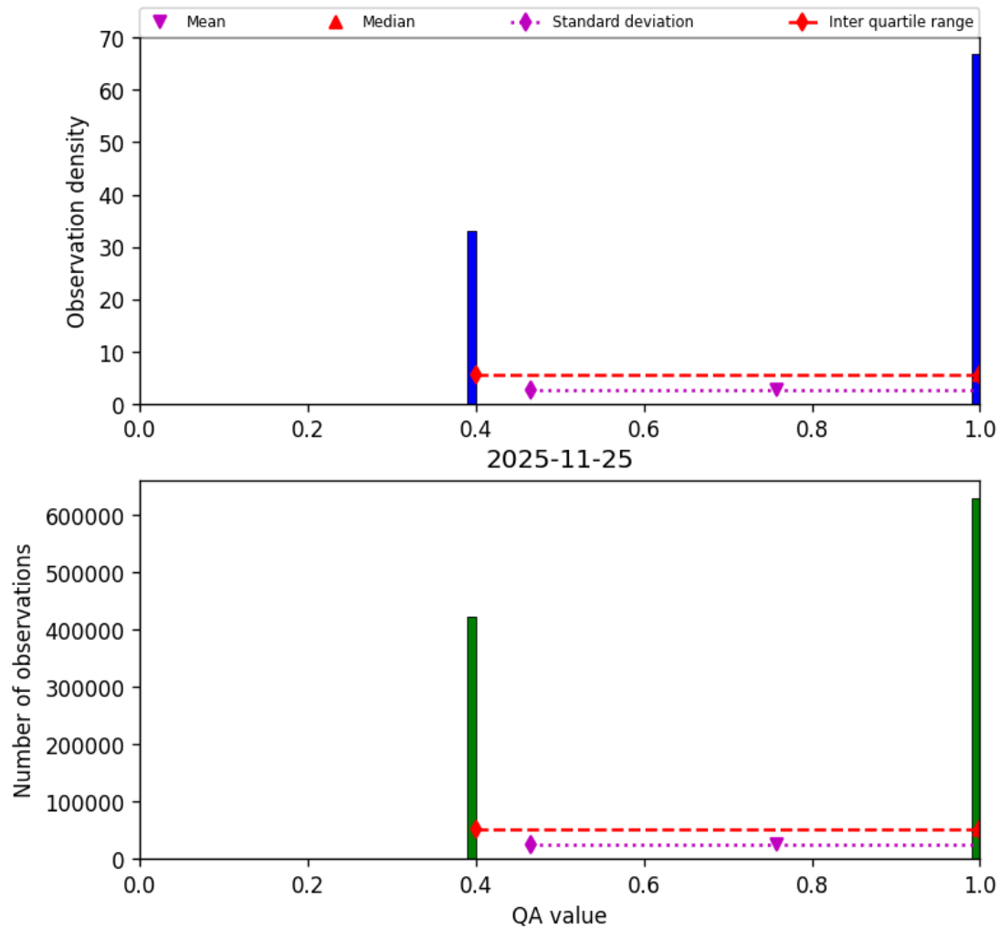
Figure 24: Histogram of “QA value” for 2025-11-24 to 2025-11-26
