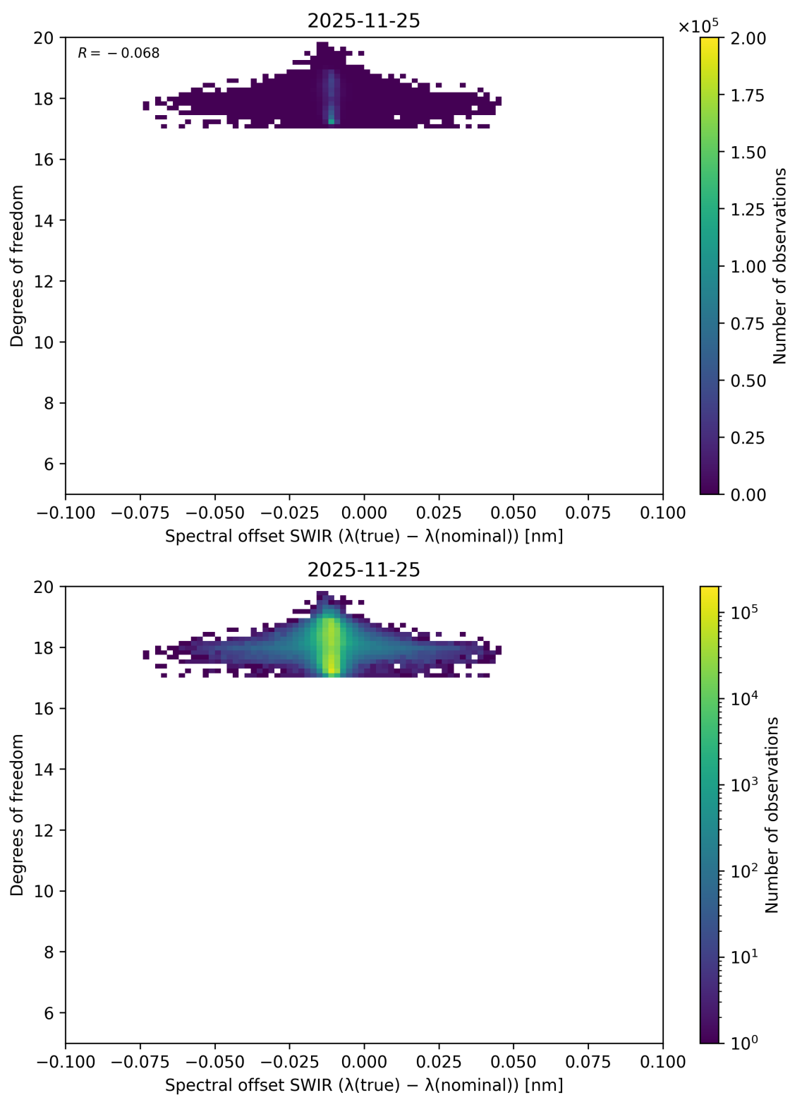
Figure 135: Scatter density plot of “Spectral offset SWIR ( \lambda_{\text{true}} - \lambda_{\text{nominal}} )” against “Degrees of freedom” for 2025-11-24 to 2025-11-26.
