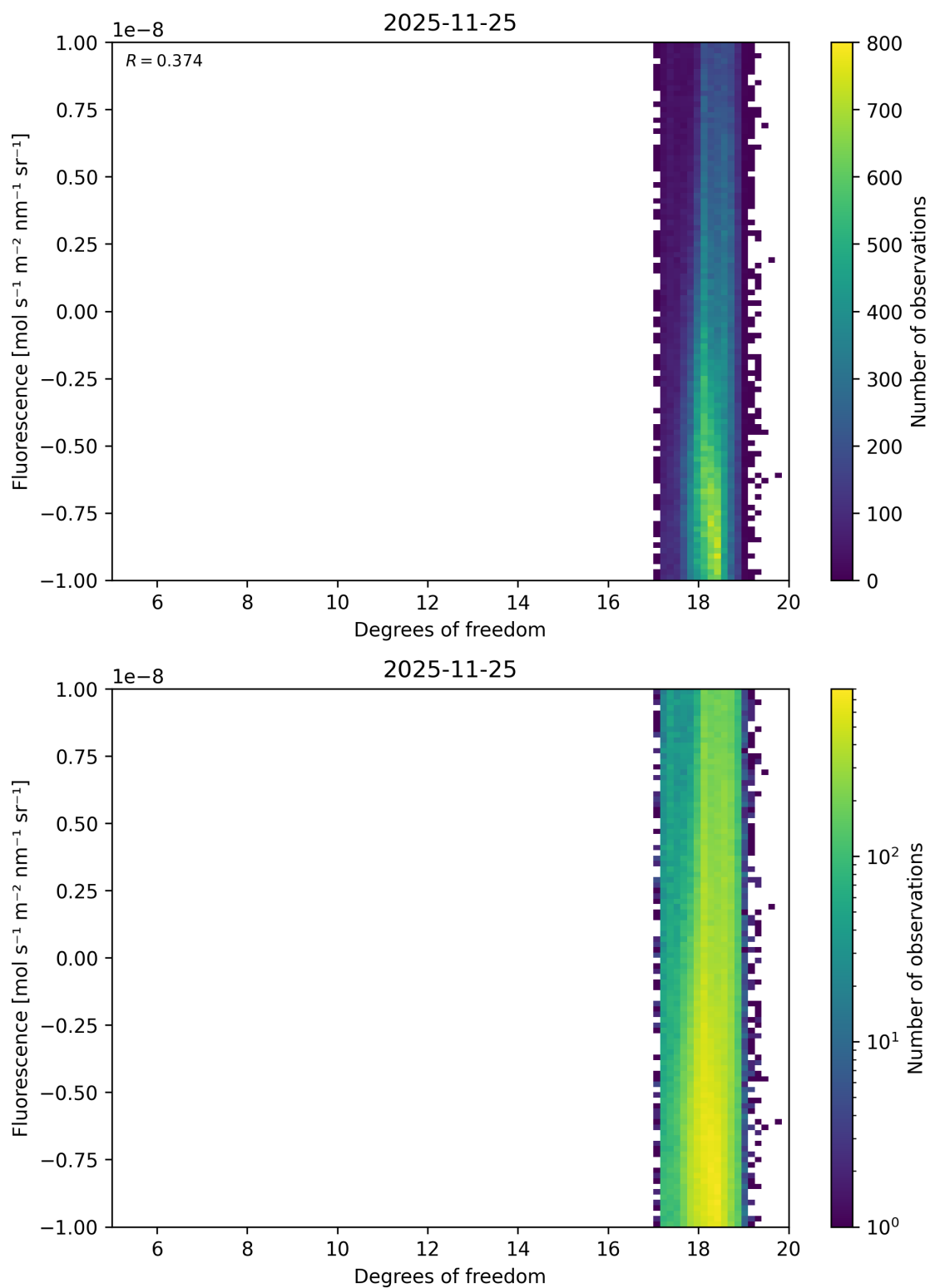
Figure 57: Scatter density plot of “Degrees of freedom” against “Fluorescence” for 2025-11-24 to 2025-11-26.
