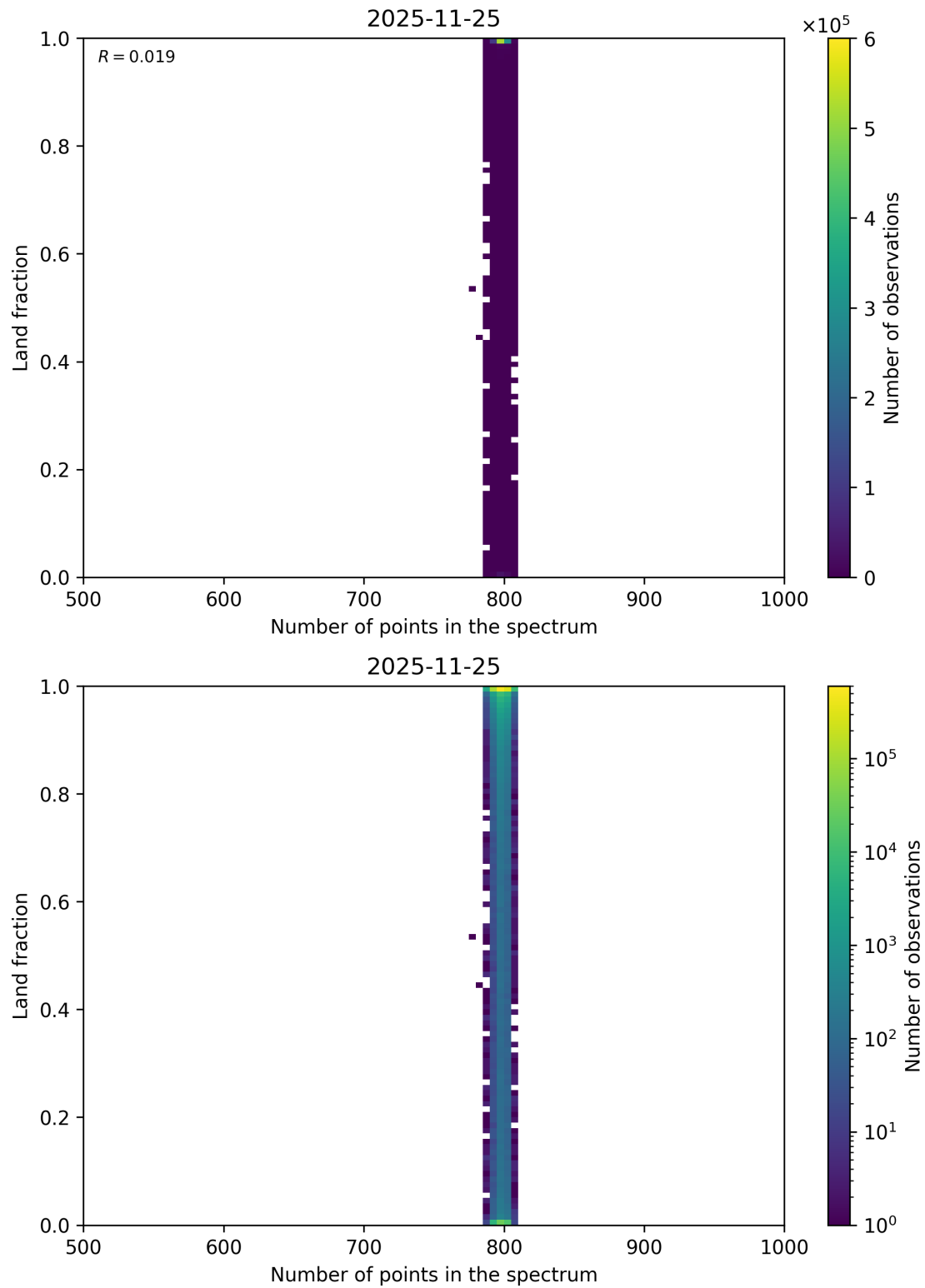
Figure 105: Scatter density plot of “Number of points in the spectrum” against “Land fraction” for 2025-11-24 to 2025-11-26.
