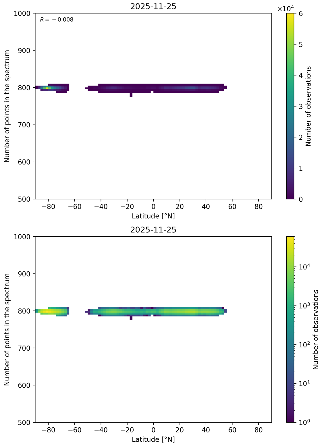
Figure 70: Scatter density plot of “Latitude” against “Number of points in the spectrum” for 2025-11-24 to 2025-11-26.
