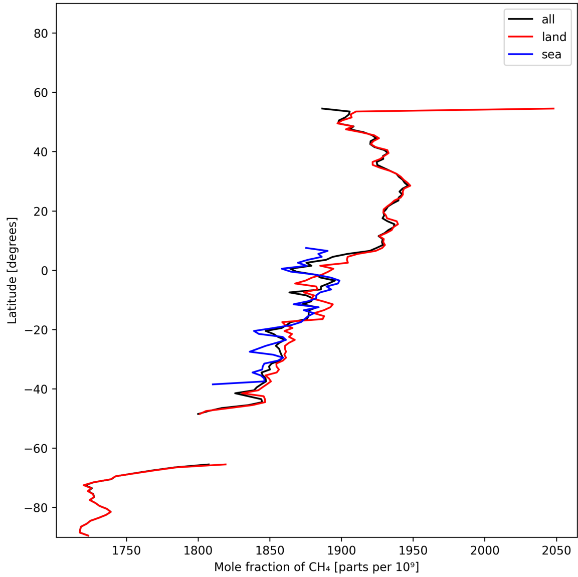
Figure 13: Zonal average of “Mole fraction of CH 4 ” for 2025-11-24 to 2025-11-26.
