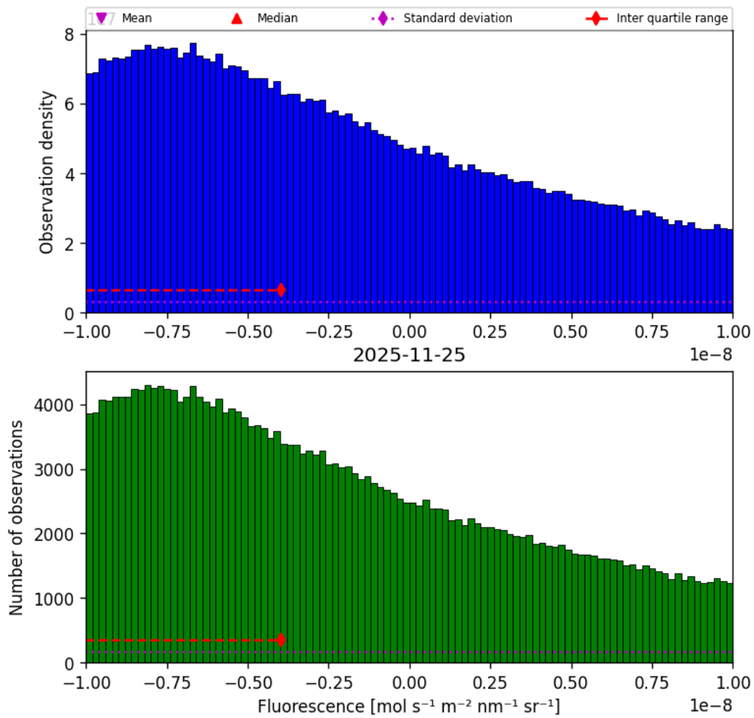
Figure 34: Histogram of “Fluorescence” for 2025-11-24 to 2025-11-26
