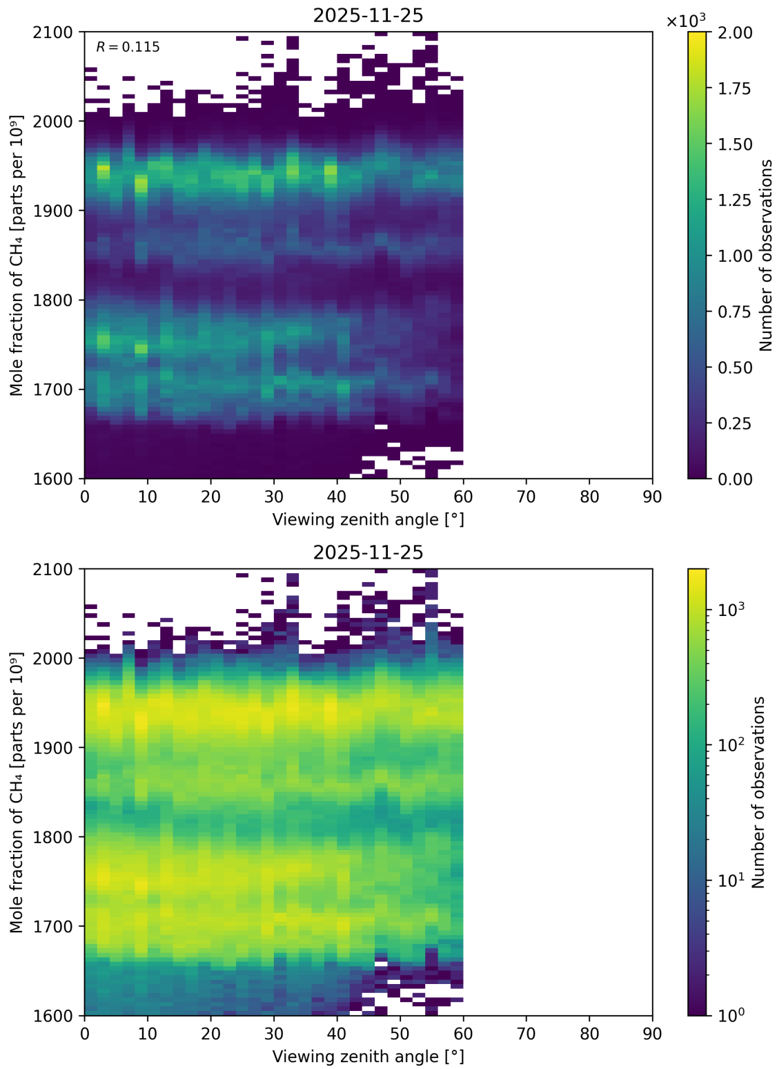
Figure 126: Scatter density plot of “Viewing zenith angle” against “Mole fraction of \text{CH}_4 ” for 2025-11-24 to 2025-11-26.
