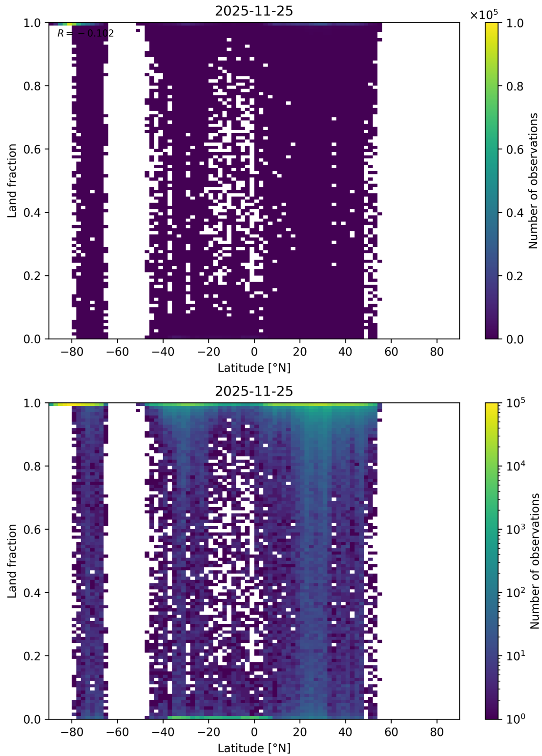
Figure 65: Scatter density plot of “Latitude” against “Land fraction” for 2025-11-24 to 2025-11-26.
