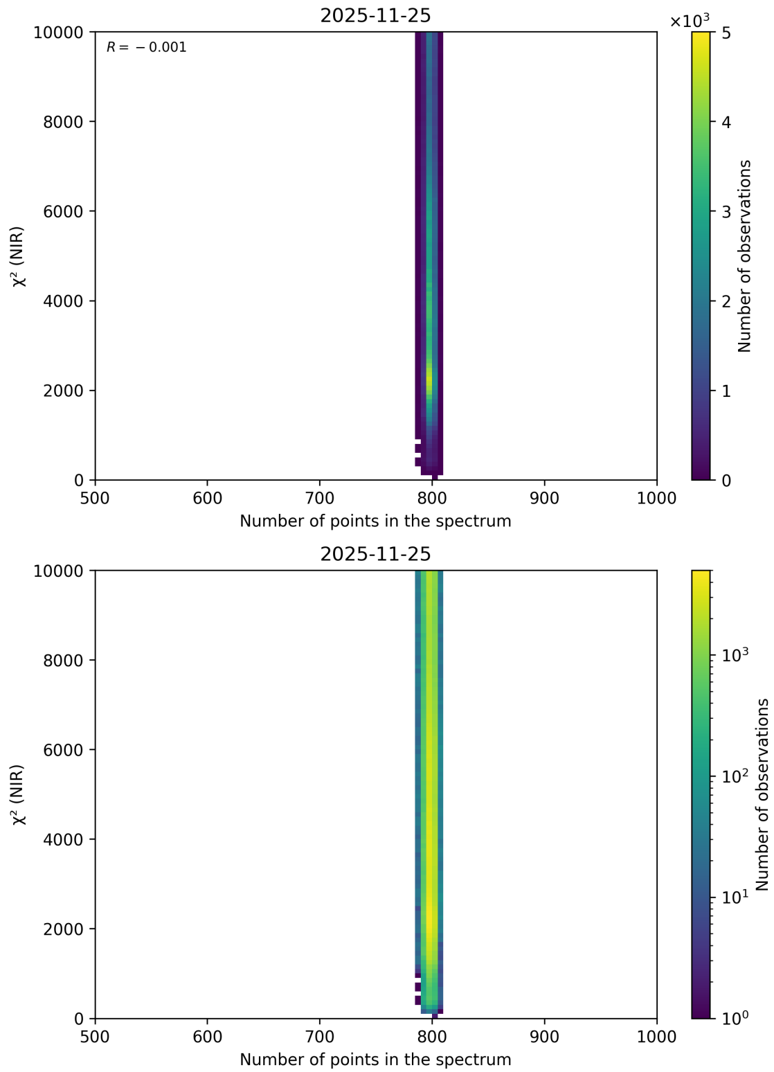
Figure 101: Scatter density plot of “Number of points in the spectrum” against “ \chi^2 (NIR)” for 2025-11-24 to 2025-11-26.
