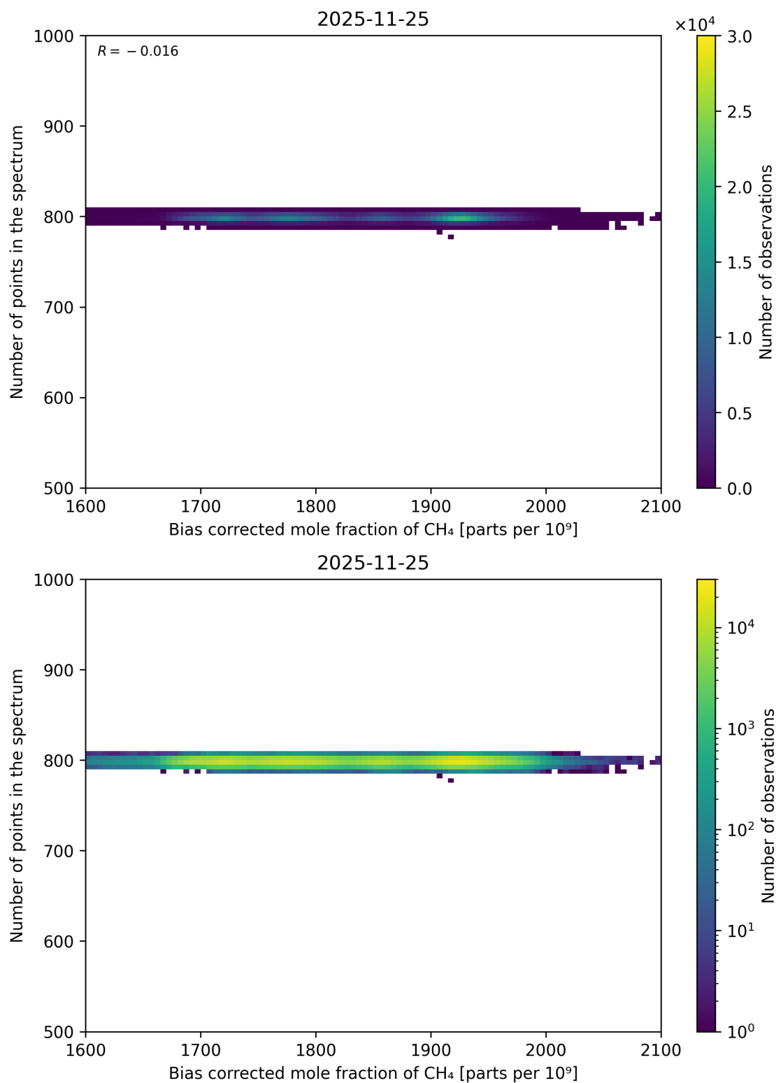
Figure 78: Scatter density plot of “Bias corrected mole fraction of CH 4 ” against “Number of points in the spectrum” for 2025-11-24 to 2025-11-26.
