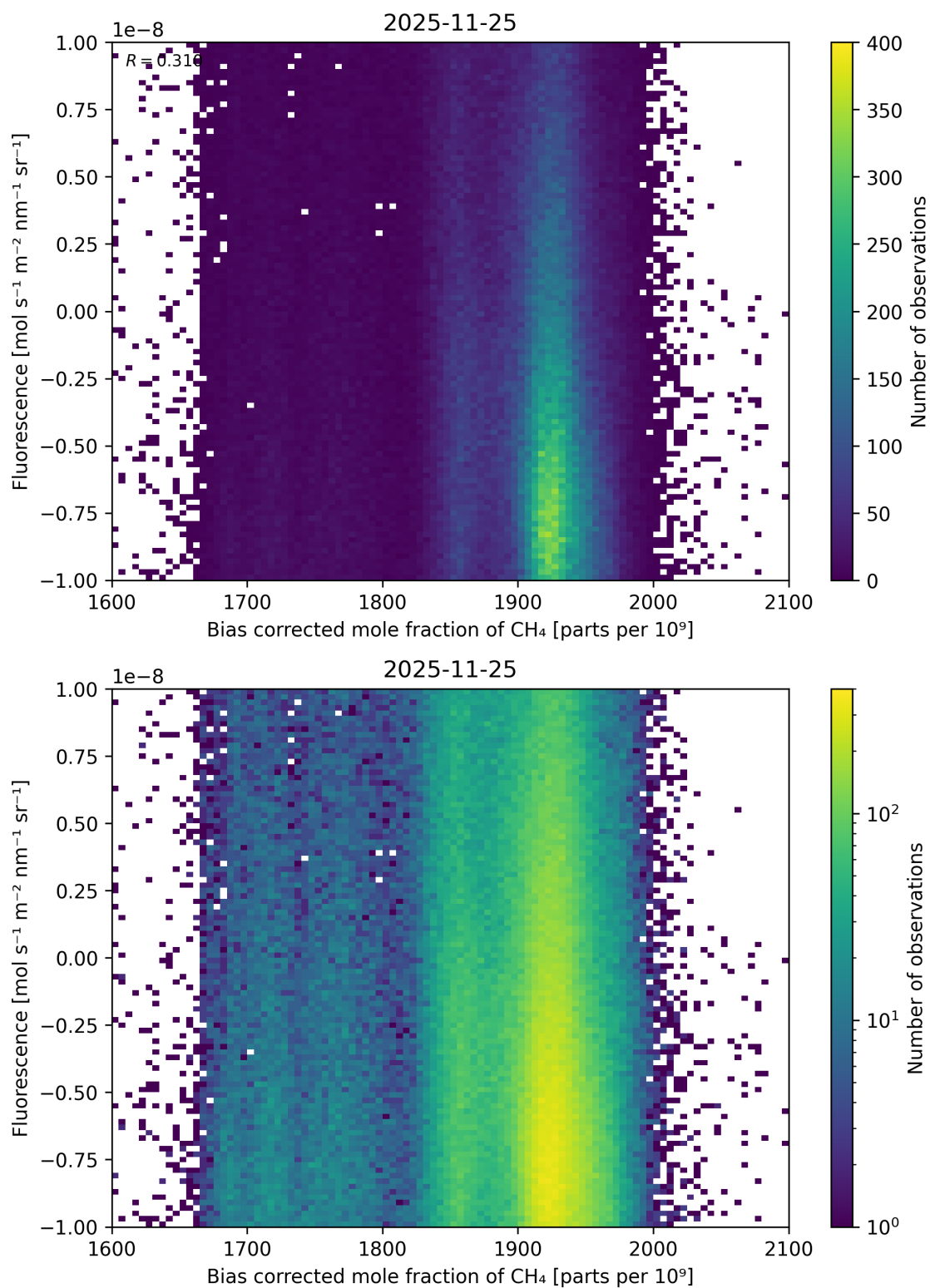
Figure 75: Scatter density plot of “Bias corrected mole fraction of \text{CH}_4 ” against “Fluorescence” for 2025-11-24 to 2025-11-26.
