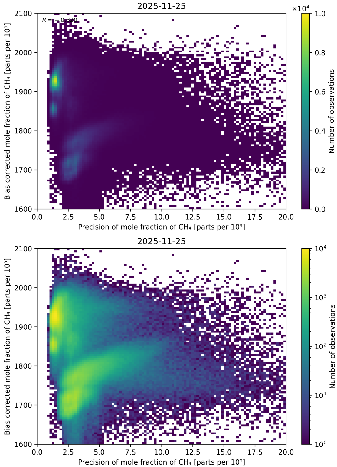
Figure 94: Scatter density plot of “Precision of mole fraction of CH 4 ” against “Bias corrected mole fraction of CH 4 ” for 2025-11-24 to 2025-11-26.
