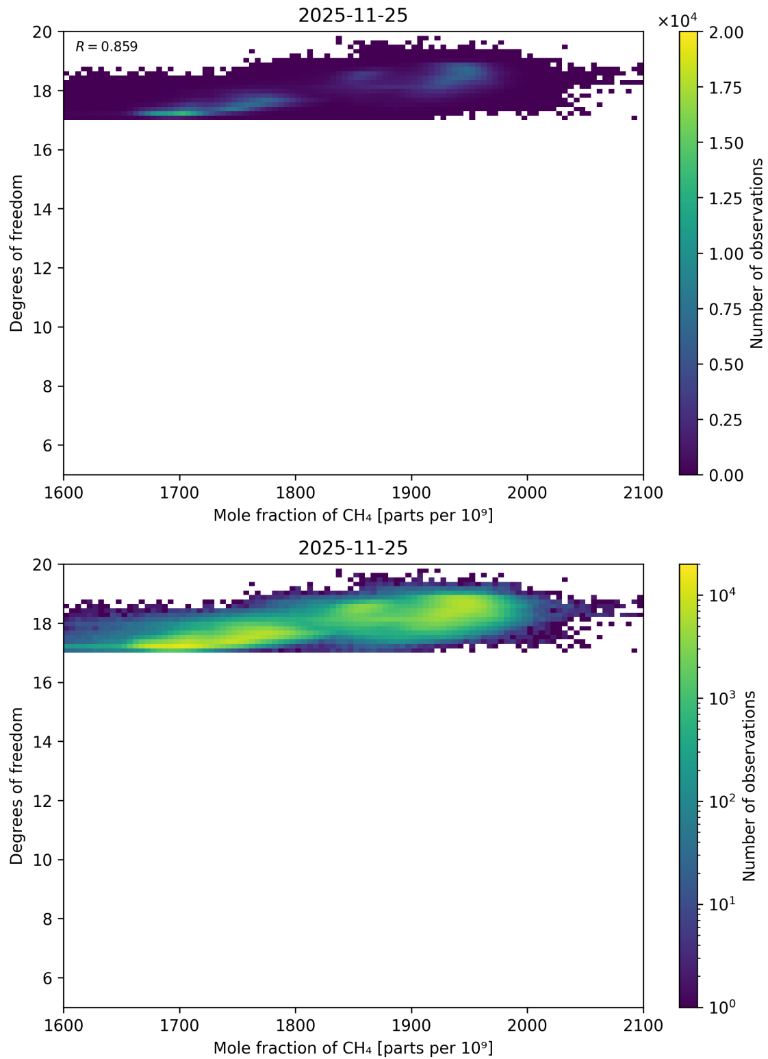
Figure 82: Scatter density plot of “Mole fraction of CH 4 ” against “Degrees of freedom” for 2025-11-24 to 2025-11-26.
