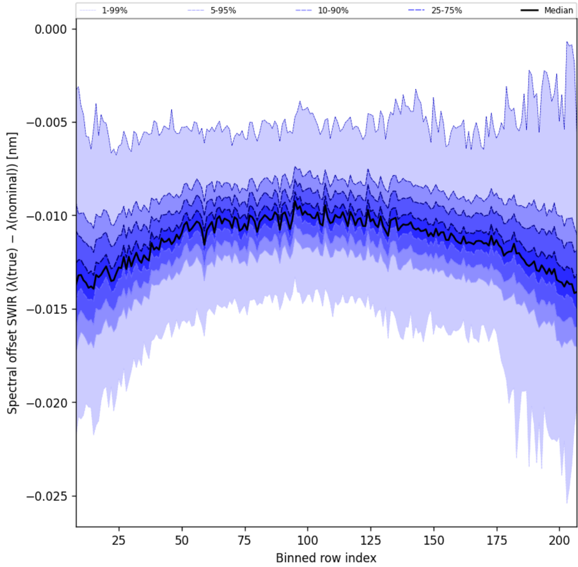
Figure 41: Along track statistics of “Spectral offset SWIR ( \lambda_{\text{true}} - \lambda_{\text{nominal}} )” for 2025-11-24 to 2025-11-26
