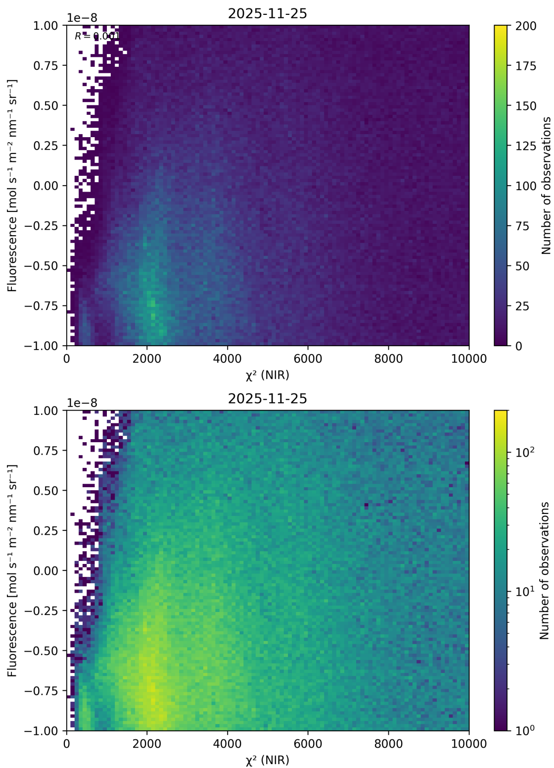
Figure 49: Scatter density plot of “ \chi^2 (NIR)” against “Fluorescence” for 2025-11-24 to 2025-11-26.
