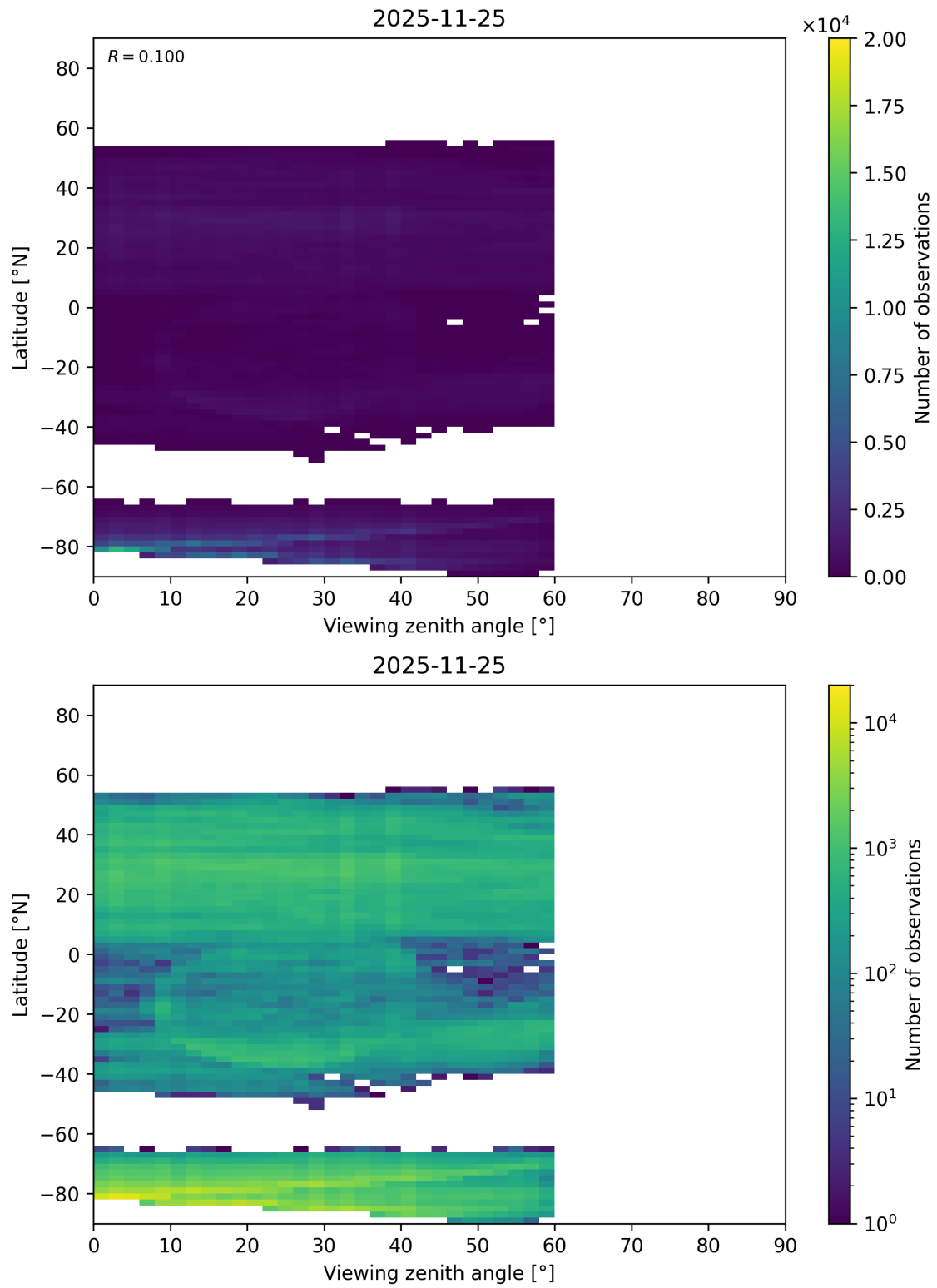
Figure 125: Scatter density plot of “Viewing zenith angle” against “Latitude” for 2025-11-24 to 2025-11-26.
