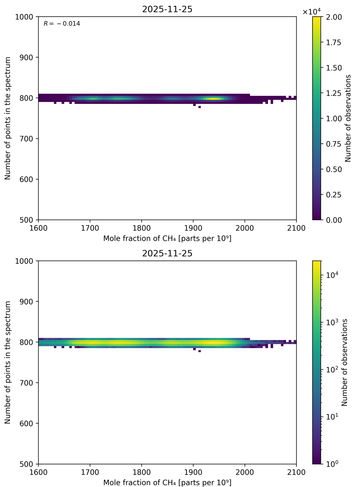
Figure 88: Scatter density plot of “Mole fraction of CH 4 ” against “Number of points in the spectrum” for 2025-11-24 to 2025-11-26.
