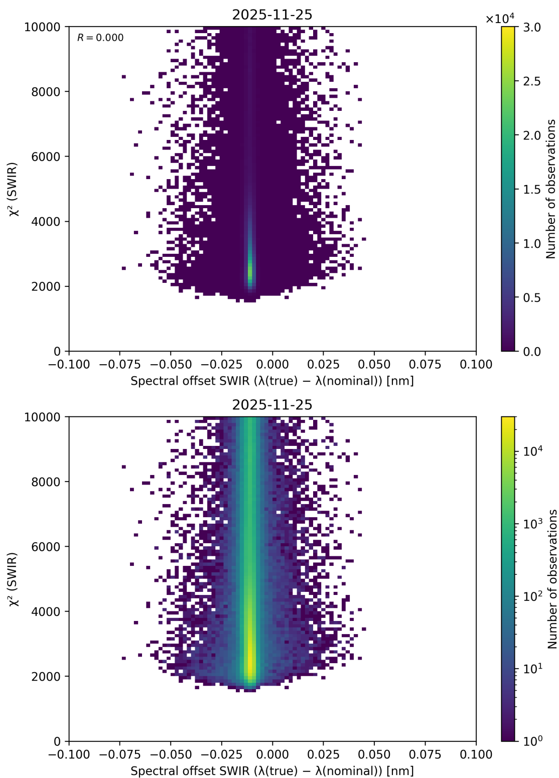
Figure 134: Scatter density plot of “Spectral offset SWIR ( \lambda_{\text{true}} - \lambda_{\text{nominal}} )” against “ \chi^2 (SWIR)” for 2025-11-24 to 2025-11-26.
