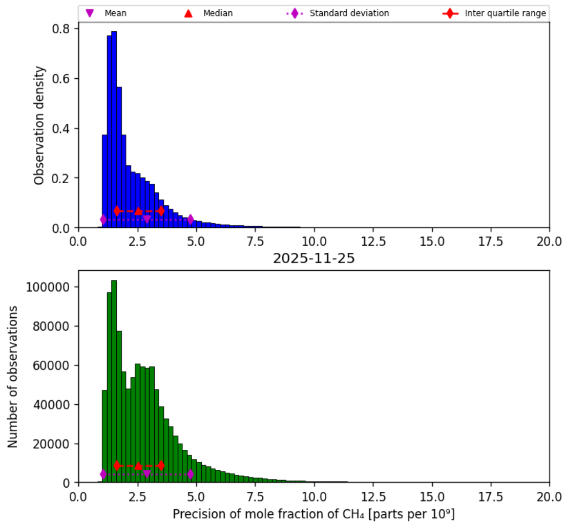
Figure 26: Histogram of “Precision of mole fraction of CH 4 ” for 2025-11-24 to 2025-11-26
