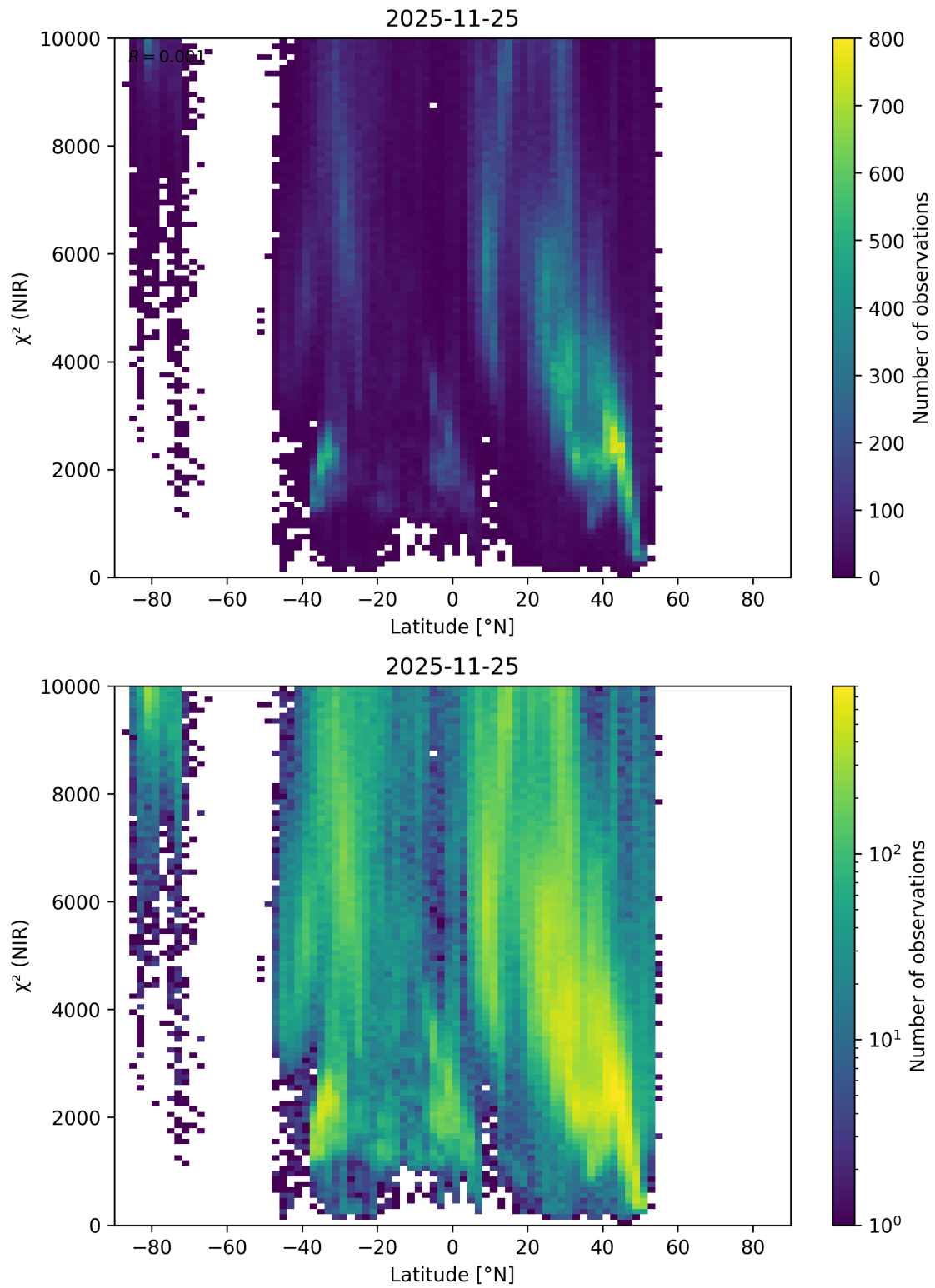
Figure 61: Scatter density plot of “Latitude” against “ \chi^2 (NIR)” for 2025-11-24 to 2025-11-26.
