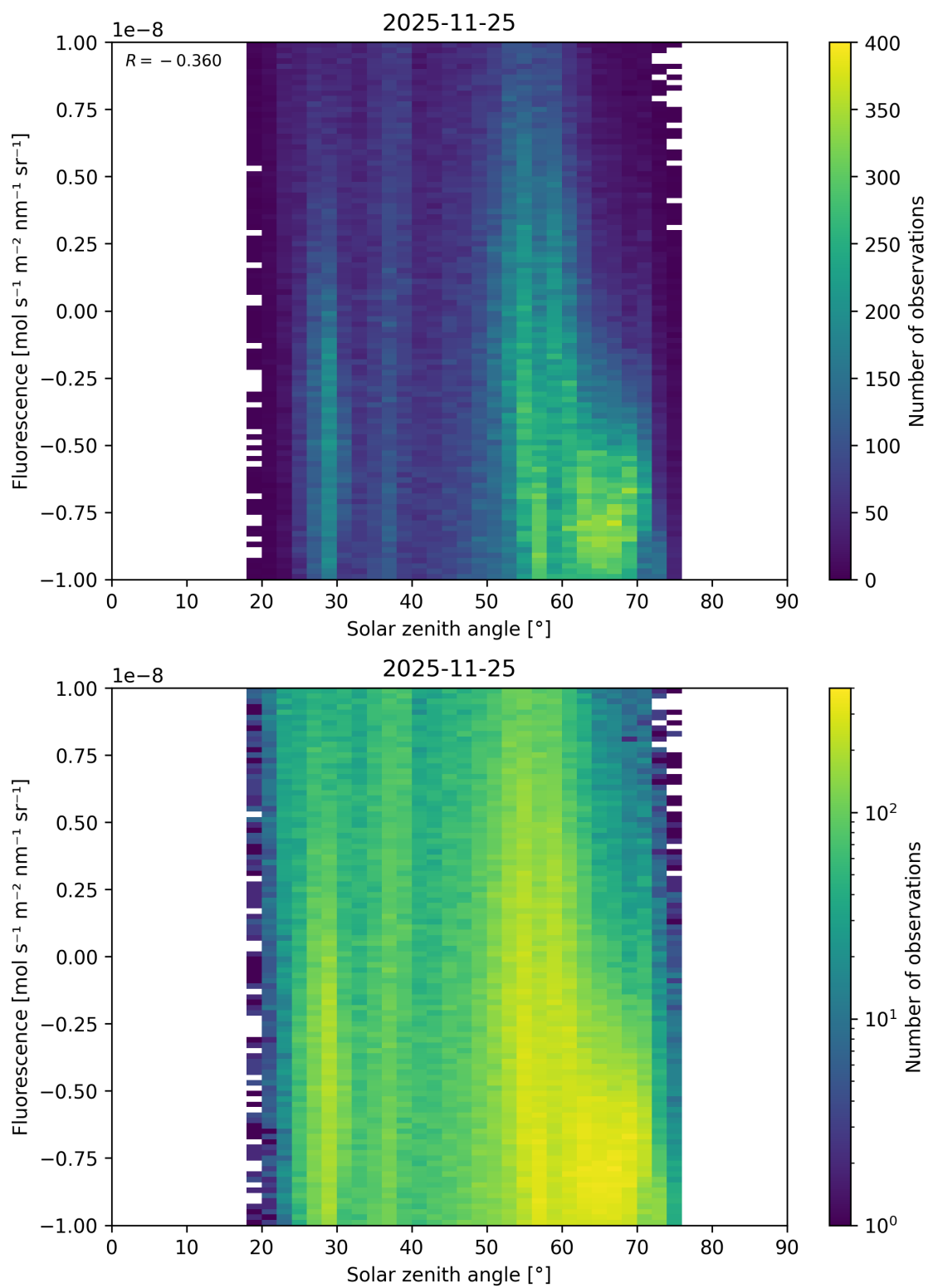
Figure 111: Scatter density plot of “Solar zenith angle” against “Fluorescence” for 2025-11-24 to 2025-11-26.
