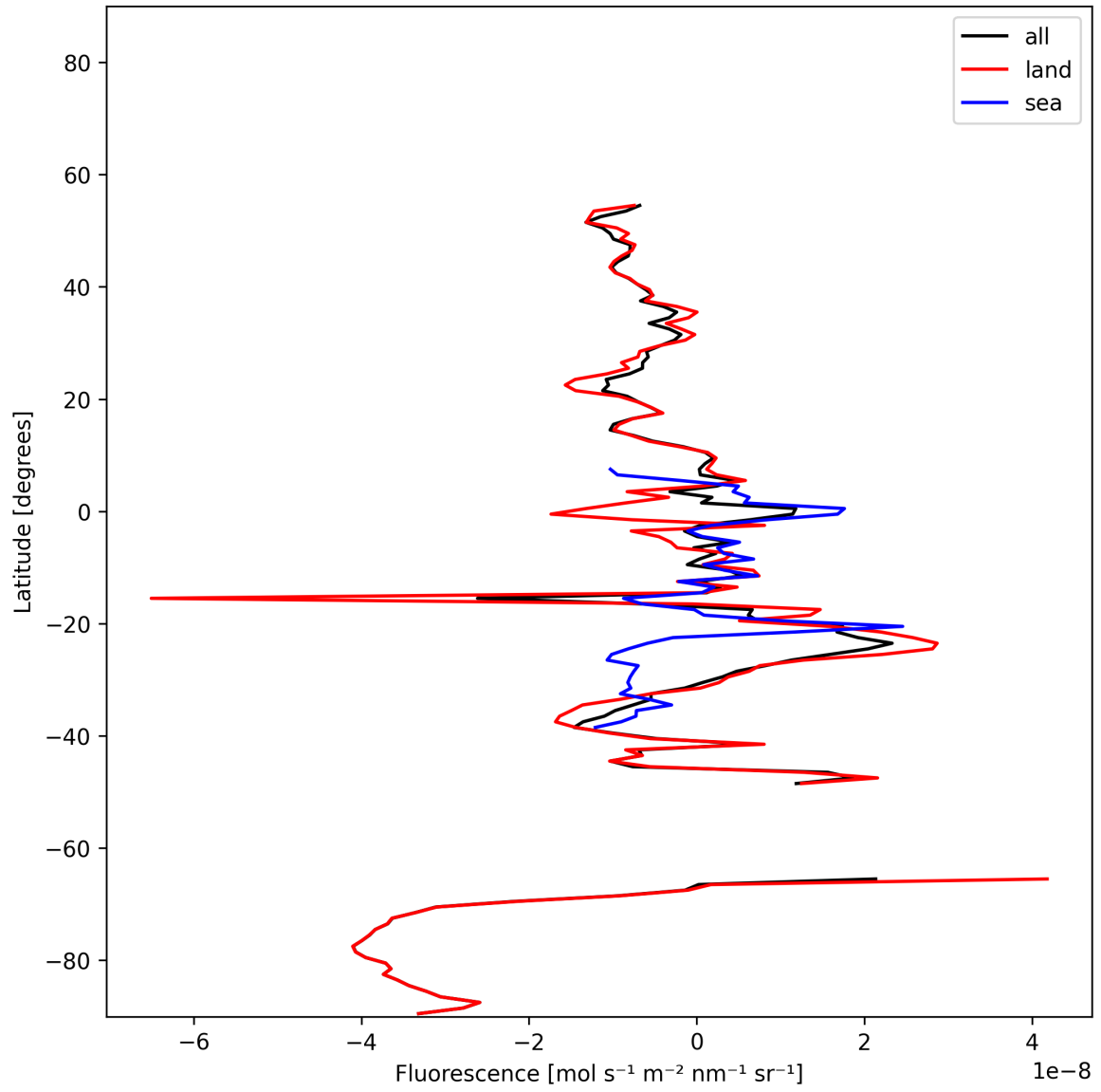
Figure 22: Zonal average of “Fluorescence” for 2025-11-24 to 2025-11-26.
