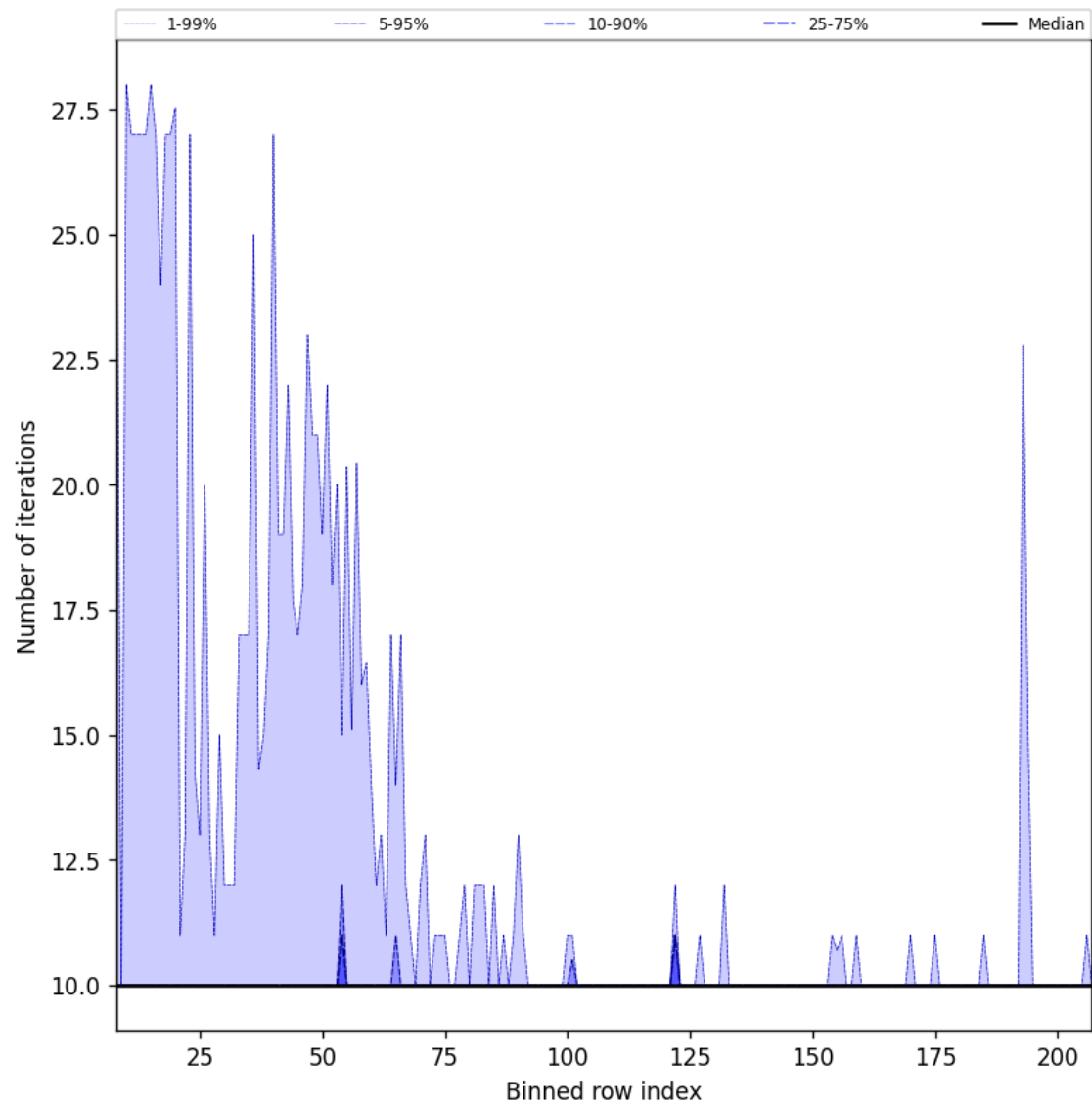
Figure 45: Along track statistics of “Number of iterations” for 2025-11-24 to 2025-11-26
