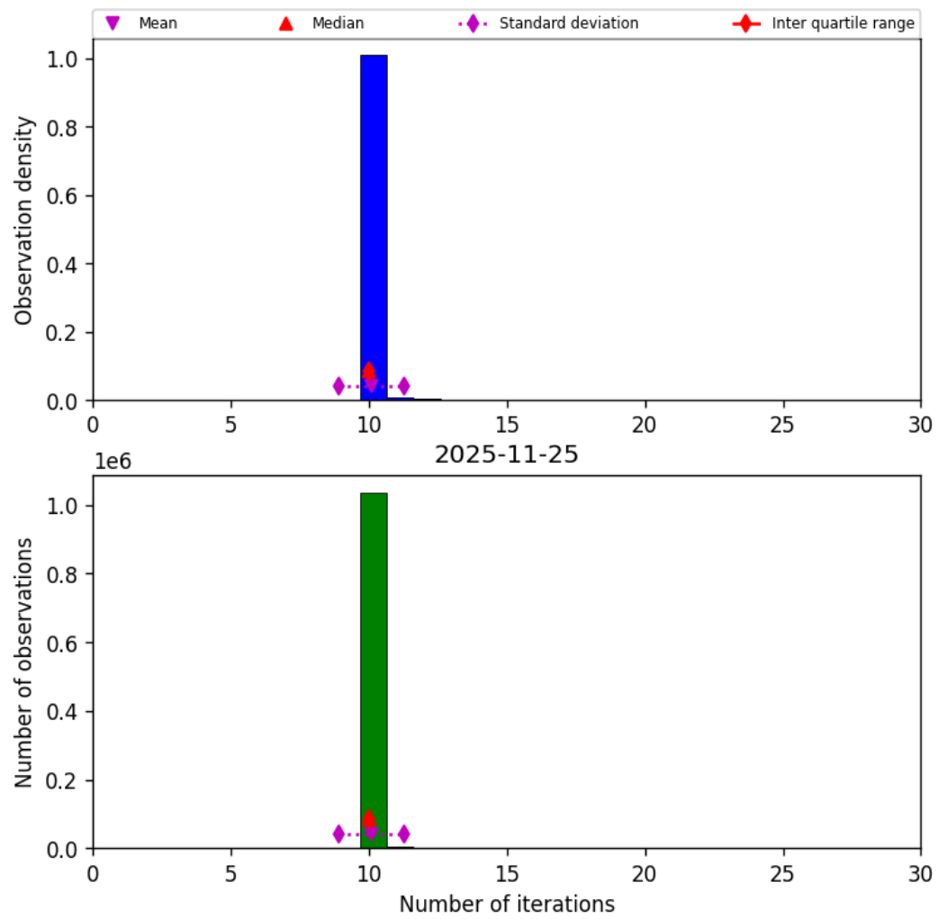
Figure 33: Histogram of “Number of iterations” for 2025-11-24 to 2025-11-26
