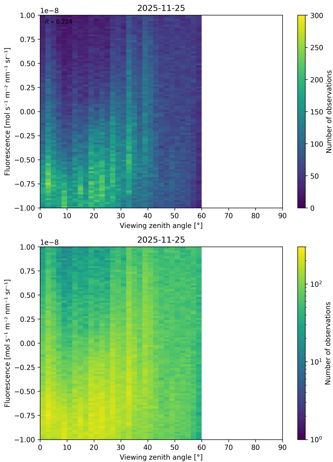
Figure 123: Scatter density plot of “Viewing zenith angle” against “Fluorescence” for 2025-11-24 to 2025-11-26.
