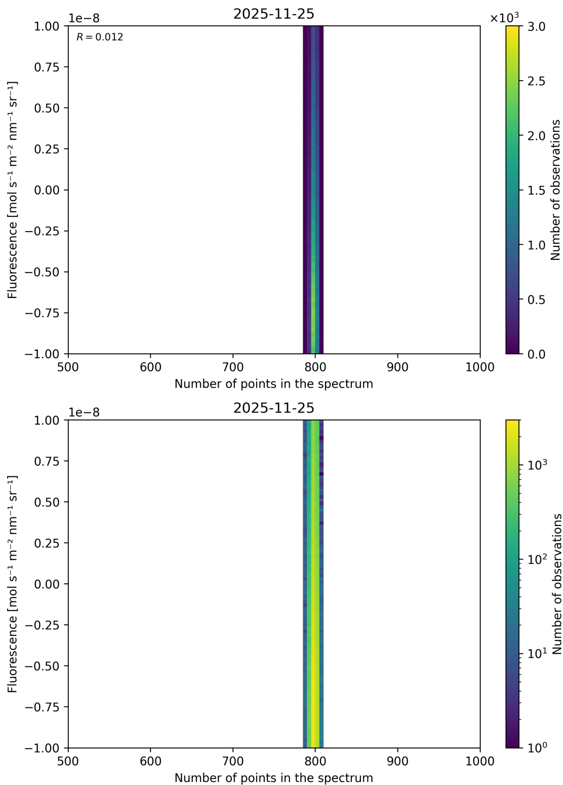
Figure 104: Scatter density plot of “Number of points in the spectrum” against “Fluorescence” for 2025-11-24 to 2025-11-26.
