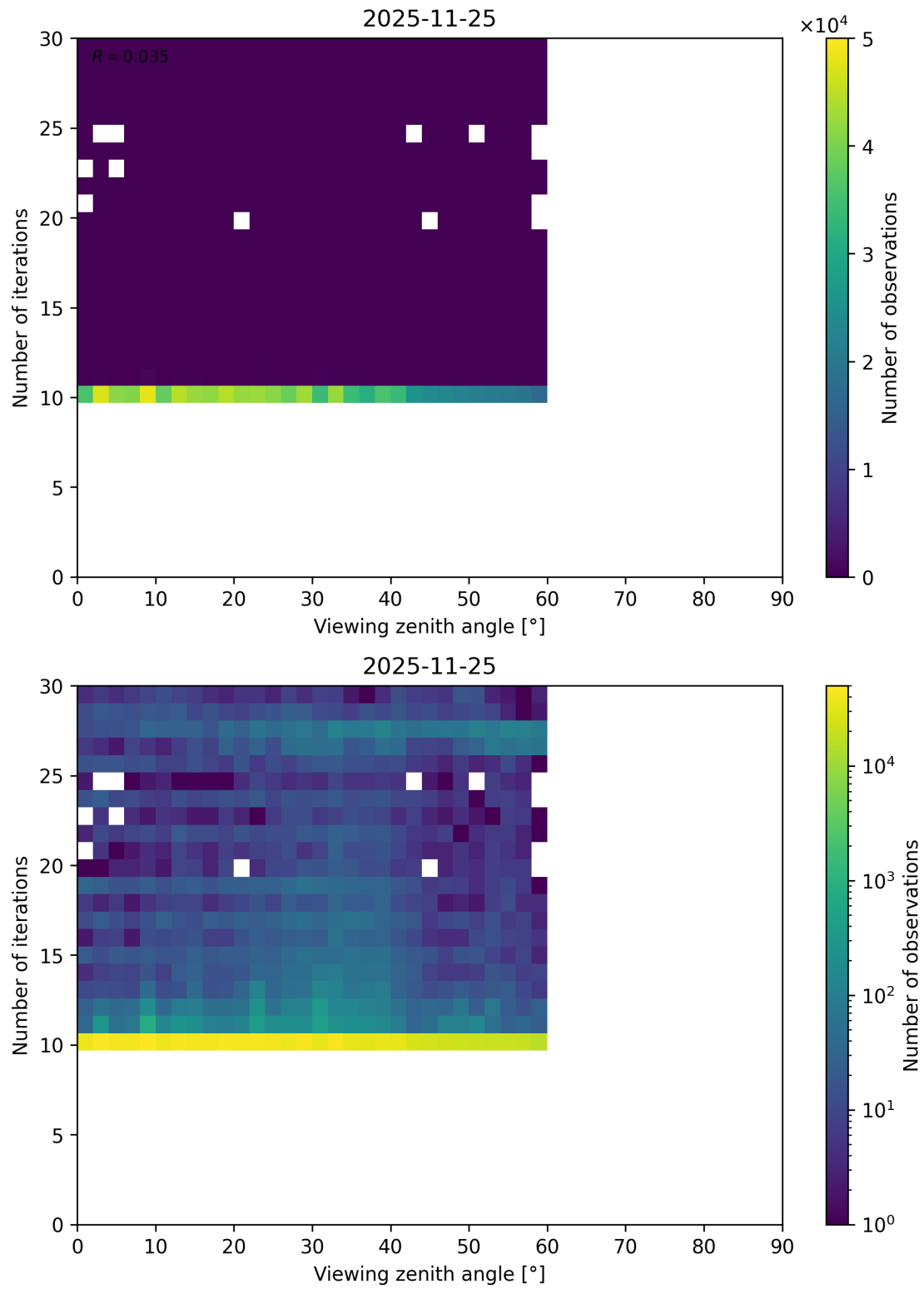
Figure 129: Scatter density plot of “Viewing zenith angle” against “Number of iterations” for 2025-11-24 to 2025-11-26.
