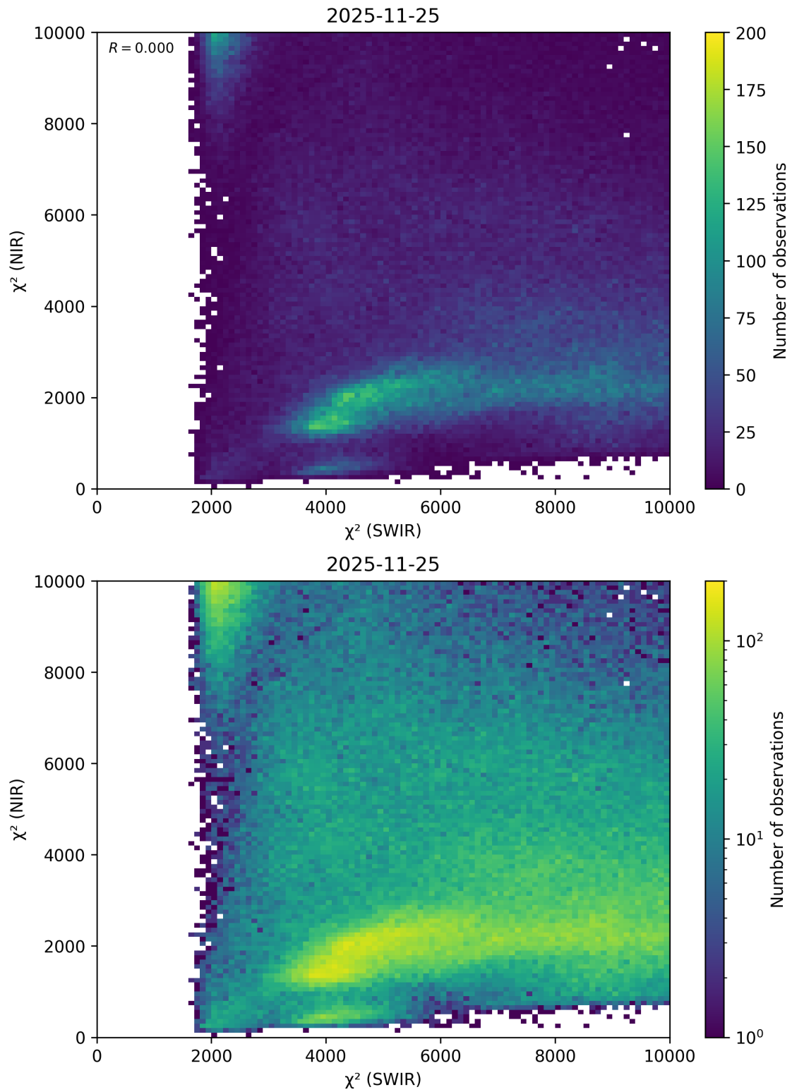
Figure 52: Scatter density plot of “ \chi^2 (SWIR)” against “ \chi^2 (NIR)” for 2025-11-24 to 2025-11-26.
