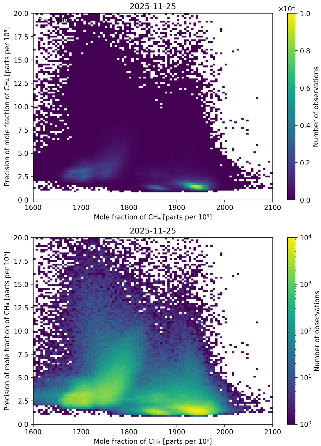
Figure 86: Scatter density plot of “Mole fraction of CH 4 ” against “Precision of mole fraction of CH 4 ” for 2025-11-24 to 2025-11-26.
