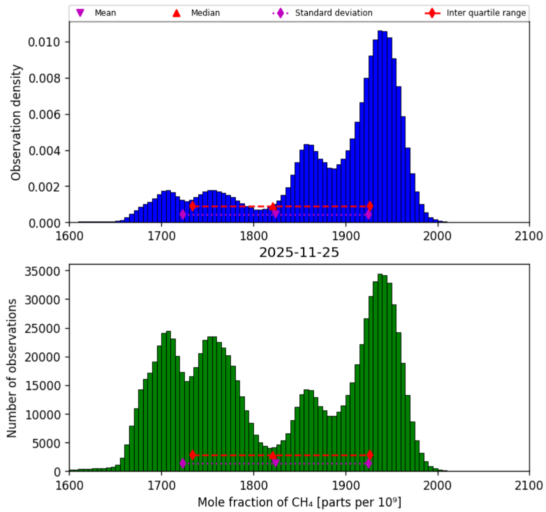
Figure 25: Histogram of “Mole fraction of CH 4 ” for 2025-11-24 to 2025-11-26
