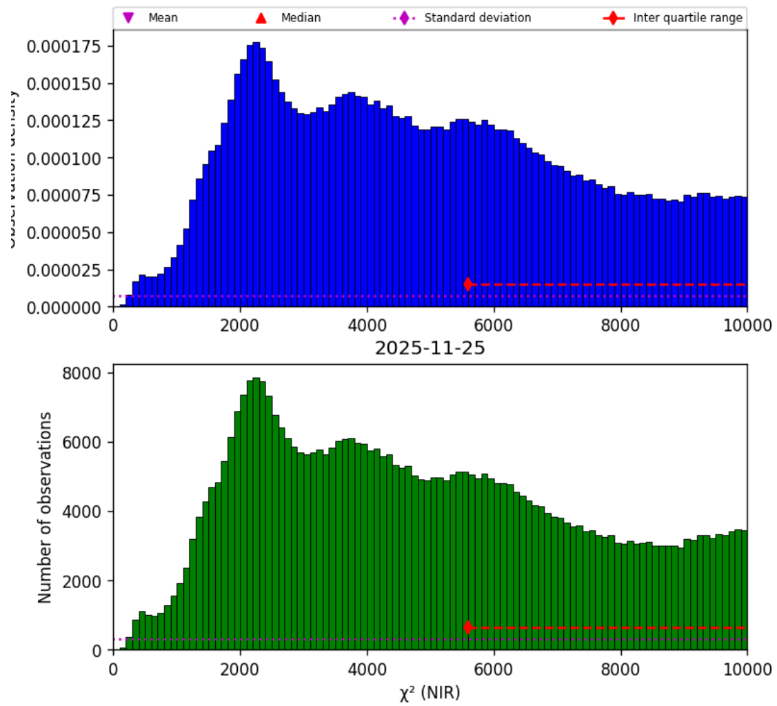
Figure 31: Histogram of “ \chi^2 (NIR)” for 2025-11-24 to 2025-11-26
