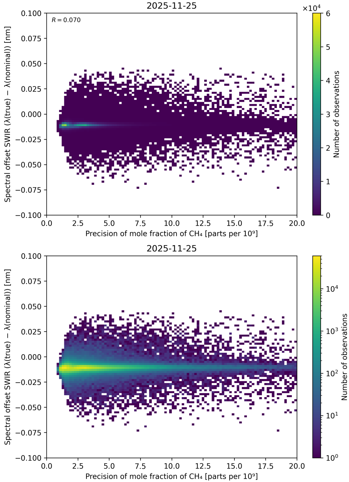
Figure 97: Scatter density plot of “Precision of mole fraction of CH 4 ” against “Spectral offset SWIR ( \lambda_{\text{true}} - \lambda_{\text{nominal}} )” for 2025-11-24 to 2025-11-26.
