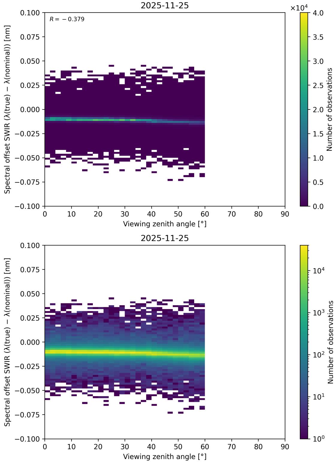
Figure 132: Scatter density plot of “Viewing zenith angle” against “Spectral offset SWIR ( \lambda_{\text{true}} - \lambda_{\text{nominal}} )” for 2025-11-24 to 2025-11-26.
