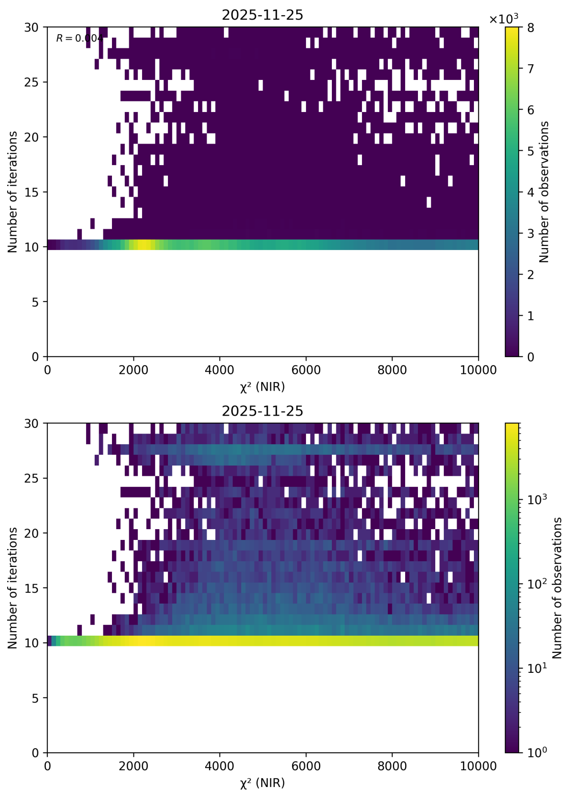
Figure 51: Scatter density plot of “ \chi^2 (NIR)” against “Number of iterations” for 2025-11-24 to 2025-11-26.
