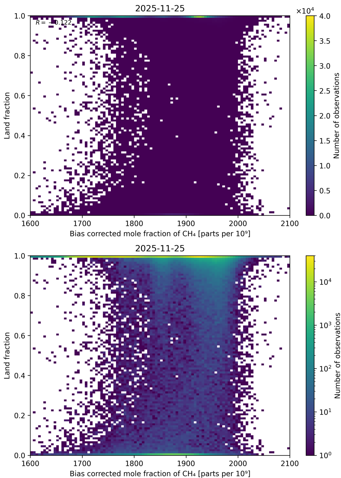
Figure 76: Scatter density plot of “Bias corrected mole fraction of CH 4 ” against “Land fraction” for 2025-11-24 to 2025-11-26.
