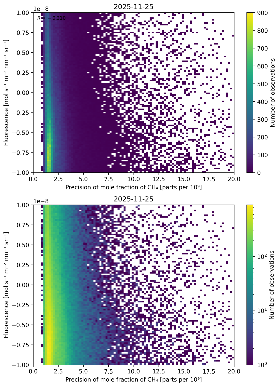
Figure 92: Scatter density plot of “Precision of mole fraction of \text{CH}_4 ” against “Fluorescence” for 2025-11-24 to 2025-11-26.
