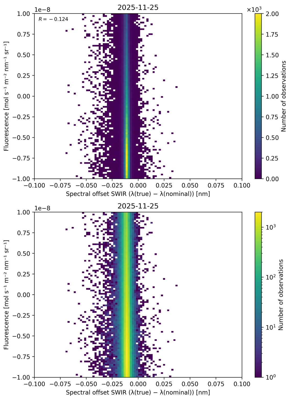
Figure 136: Scatter density plot of “Spectral offset SWIR ( \lambda_{\text{true}} - \lambda_{\text{nominal}} )” against “Fluorescence” for 2025-11-24 to 2025-11-26.
