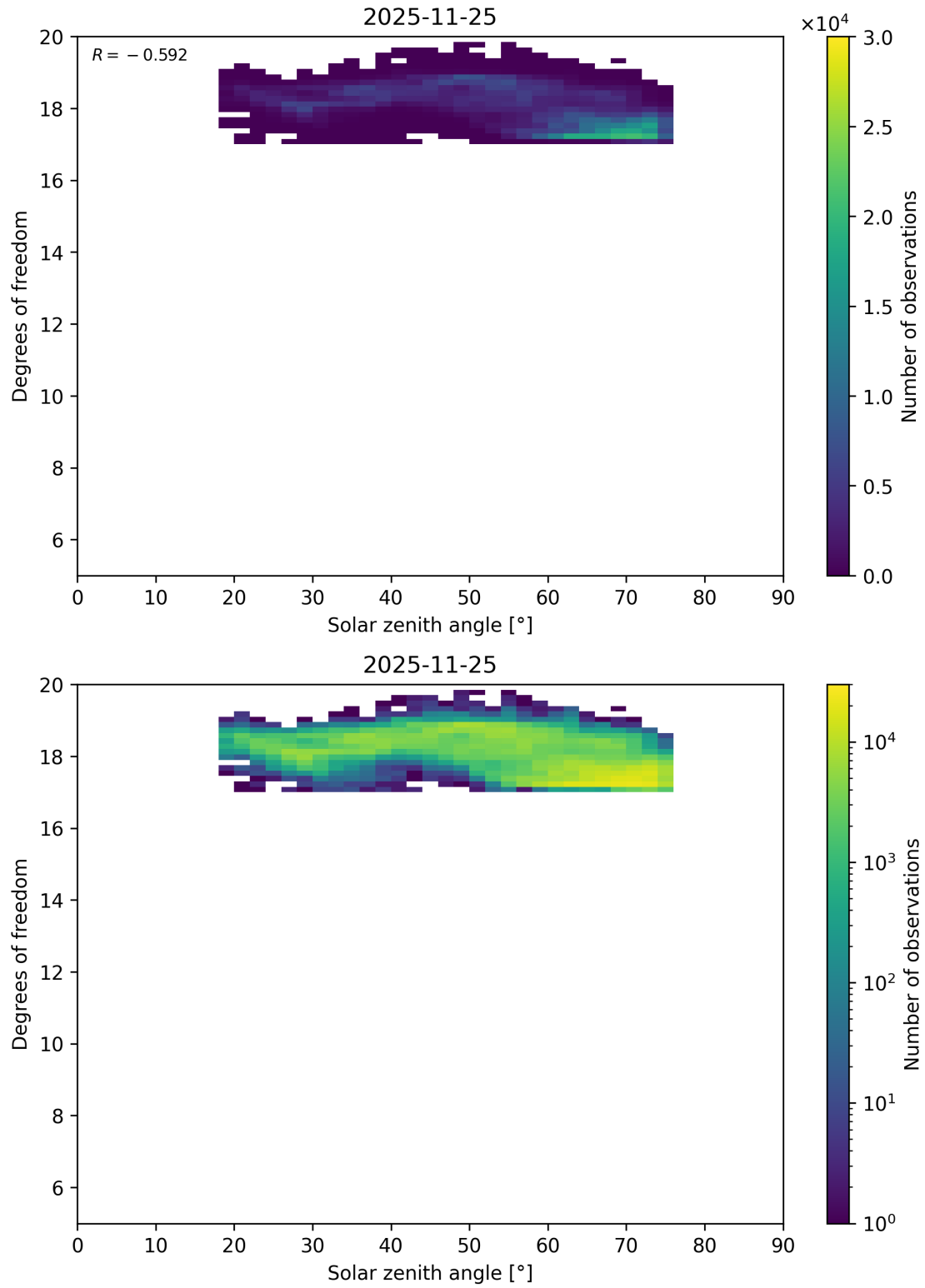
Figure 110: Scatter density plot of “Solar zenith angle” against “Degrees of freedom” for 2025-11-24 to 2025-11-26.
