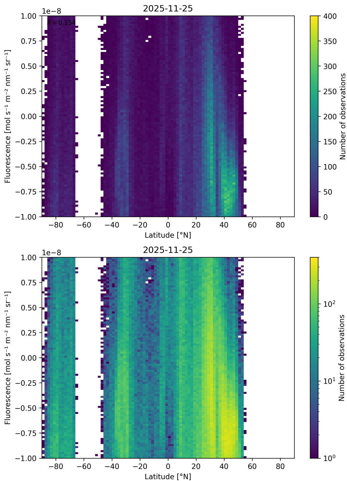
Figure 64: Scatter density plot of “Latitude” against “Fluorescence” for 2025-11-24 to 2025-11-26.
