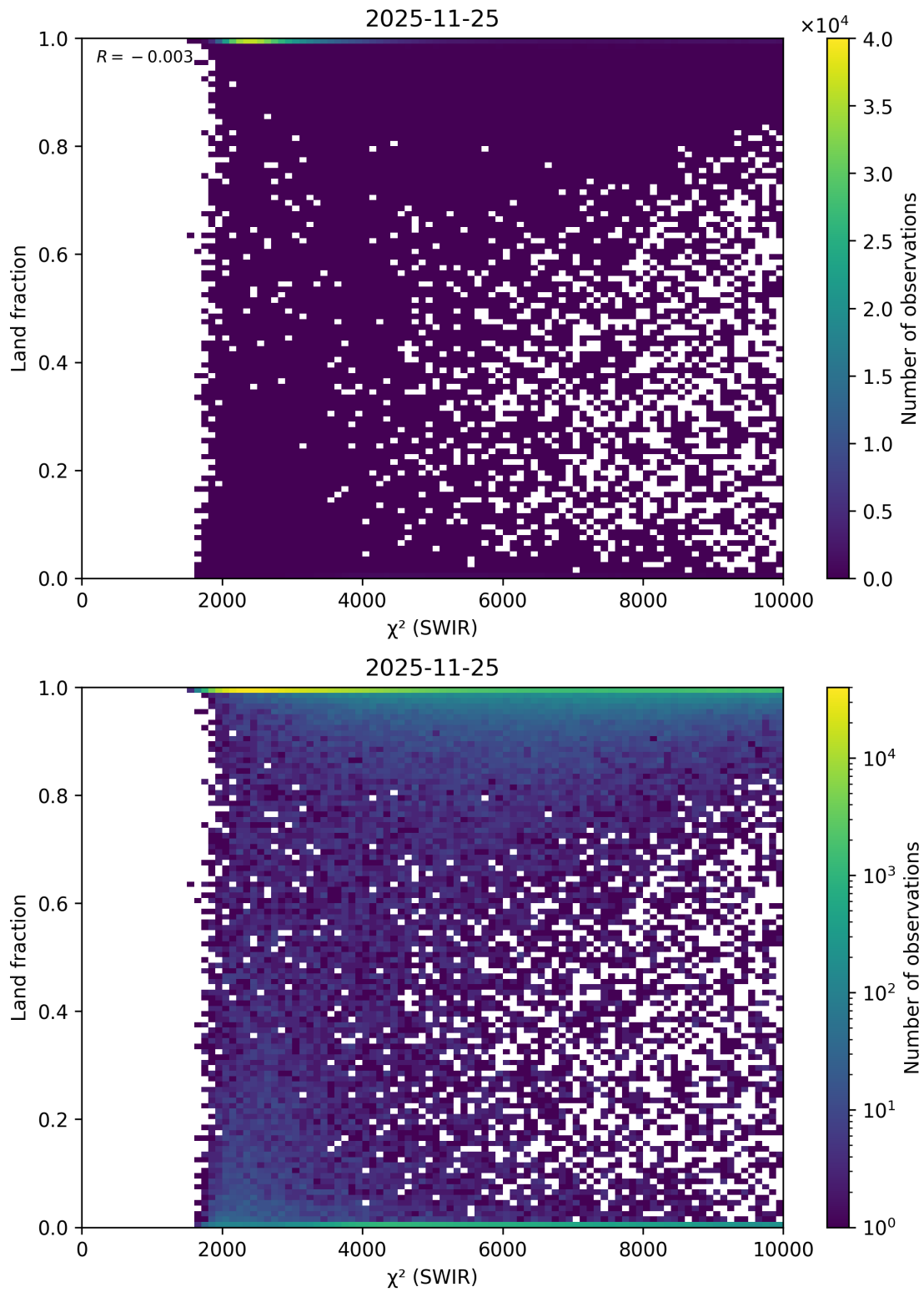
Figure 55: Scatter density plot of “ \chi^2 (SWIR)” against “Land fraction” for 2025-11-24 to 2025-11-26.
