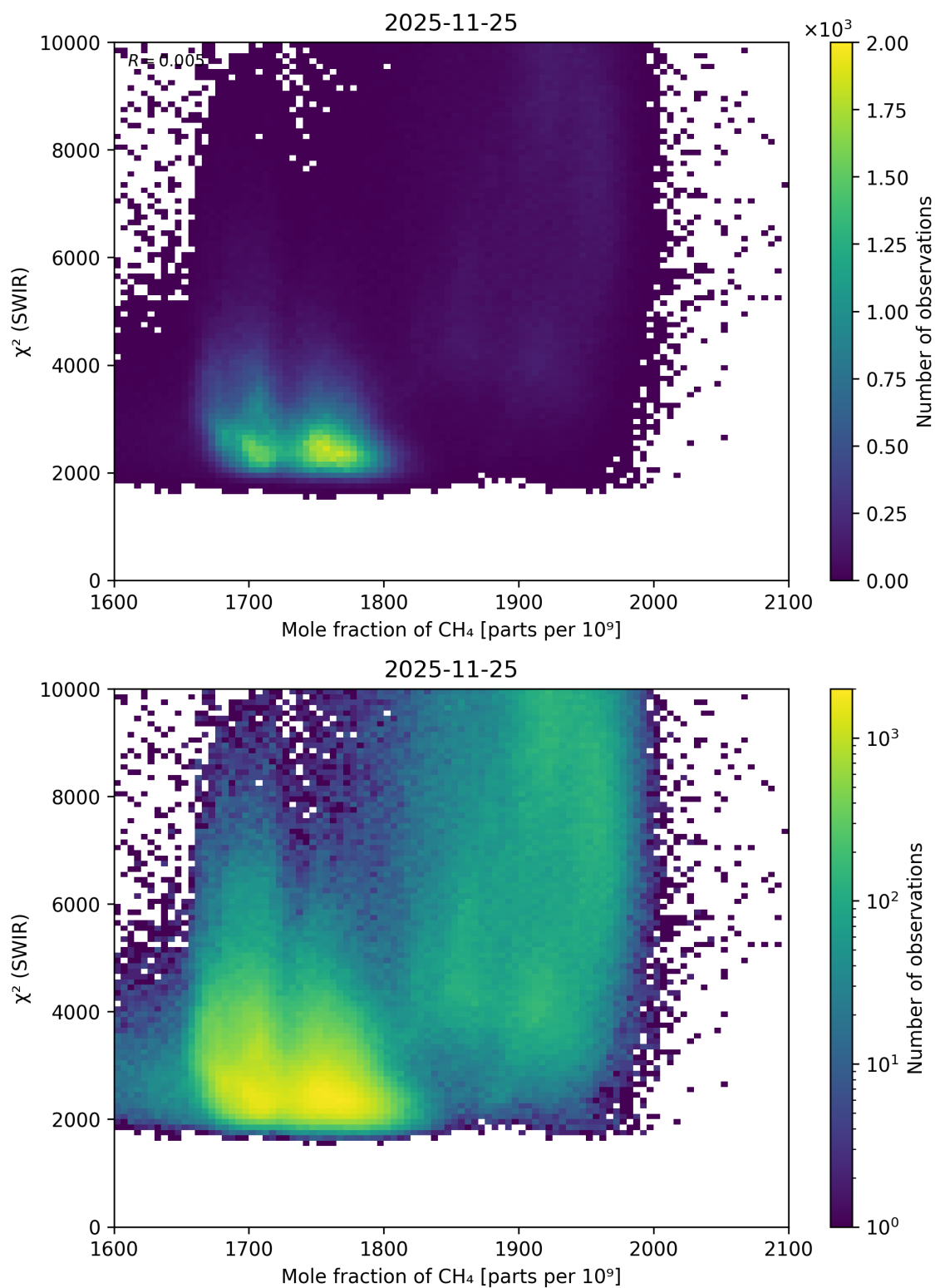
Figure 81: Scatter density plot of “Mole fraction of \text{CH}_4 ” against “ \chi^2 (SWIR)” for 2025-11-24 to 2025-11-26.
