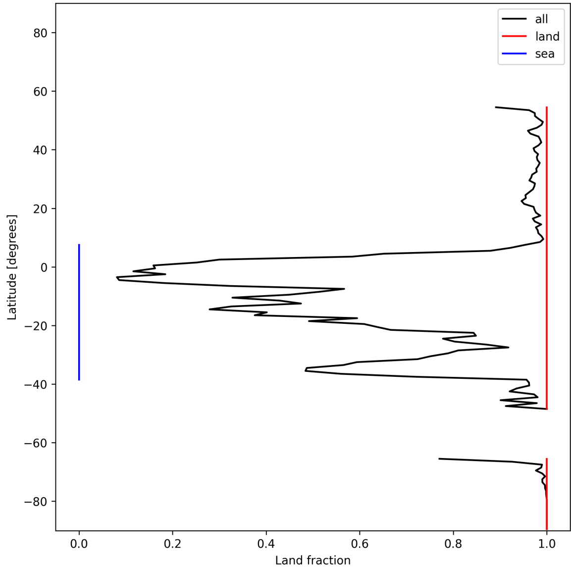
Figure 23: Zonal average of “Land fraction” for 2025-11-24 to 2025-11-26.
