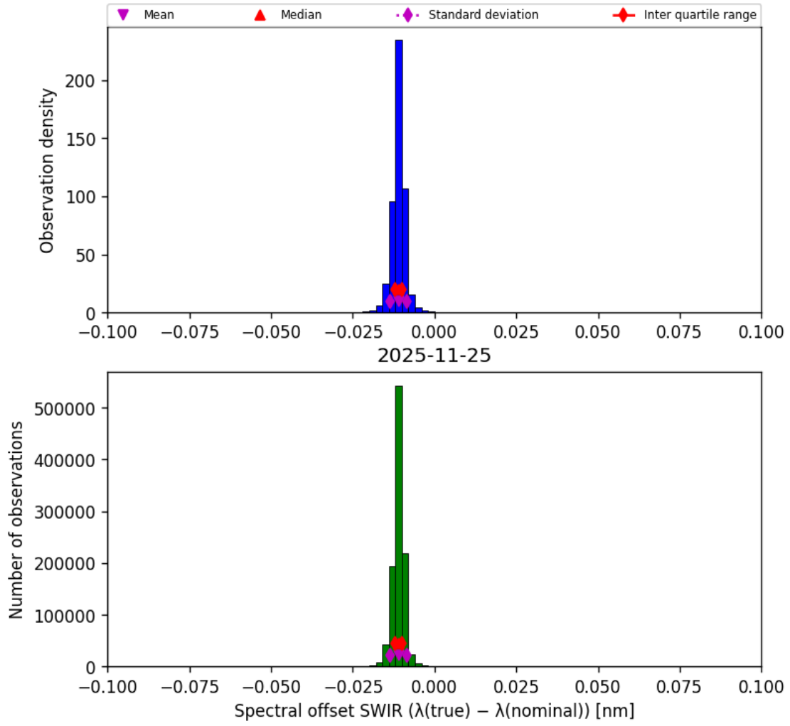
Figure 29: Histogram of “Spectral offset SWIR ( \lambda_{\text{true}} - \lambda_{\text{nominal}} )” for 2025-11-24 to 2025-11-26
