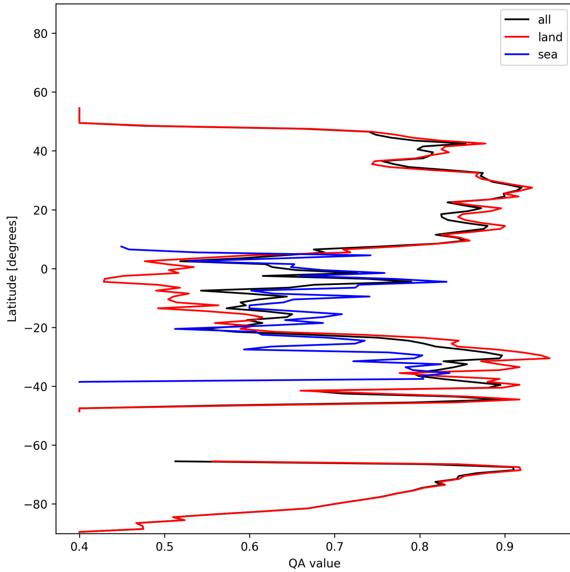
Figure 12: Zonal average of “QA value” for 2025-11-24 to 2025-11-26.
