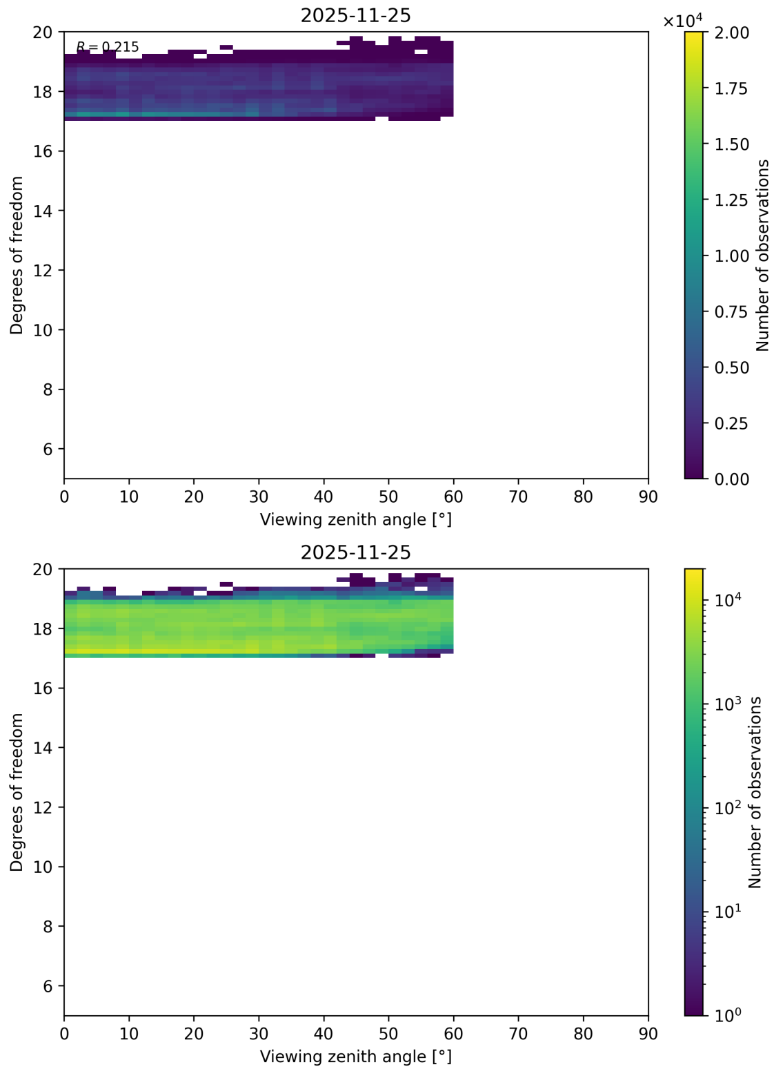
Figure 122: Scatter density plot of “Viewing zenith angle” against “Degrees of freedom” for 2025-11-24 to 2025-11-26.
