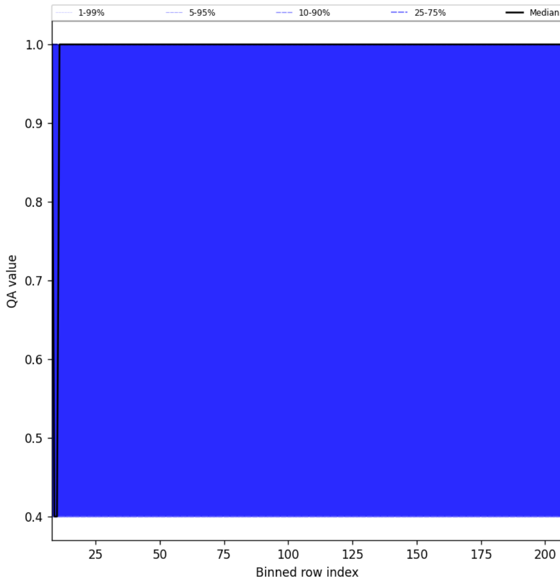
Figure 36: Along track statistics of “QA value” for 2025-11-24 to 2025-11-26
