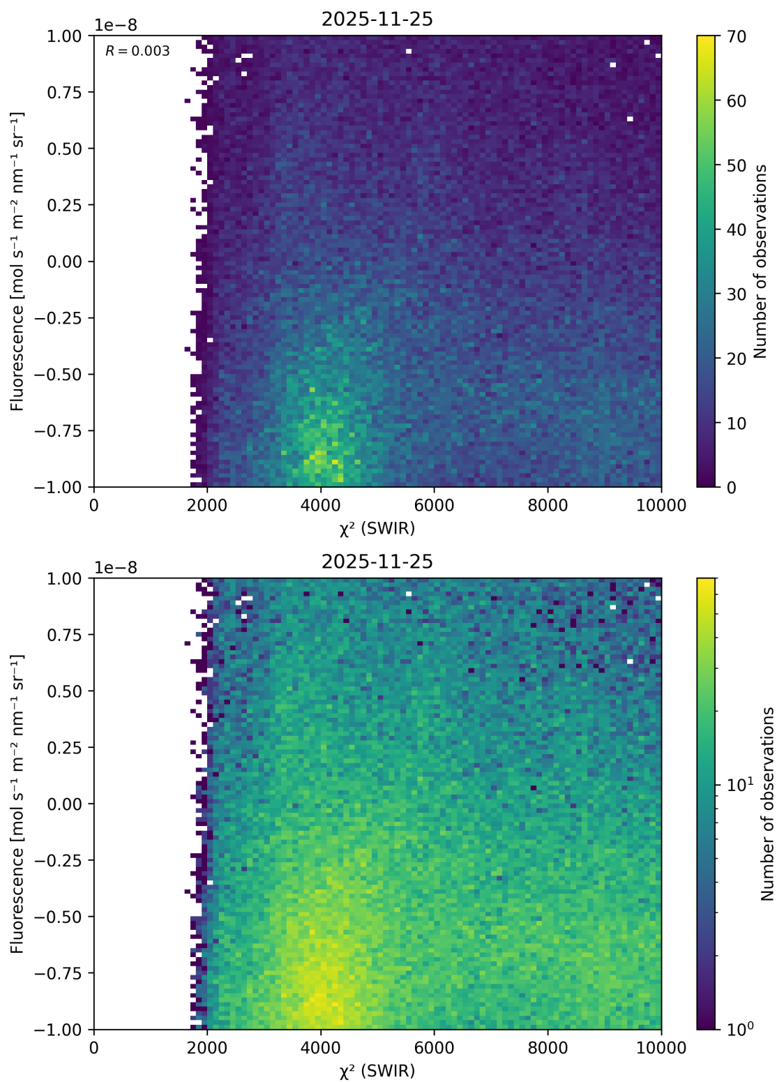
Figure 54: Scatter density plot of “ \chi^2 (SWIR)” against “Fluorescence” for 2025-11-24 to 2025-11-26.
