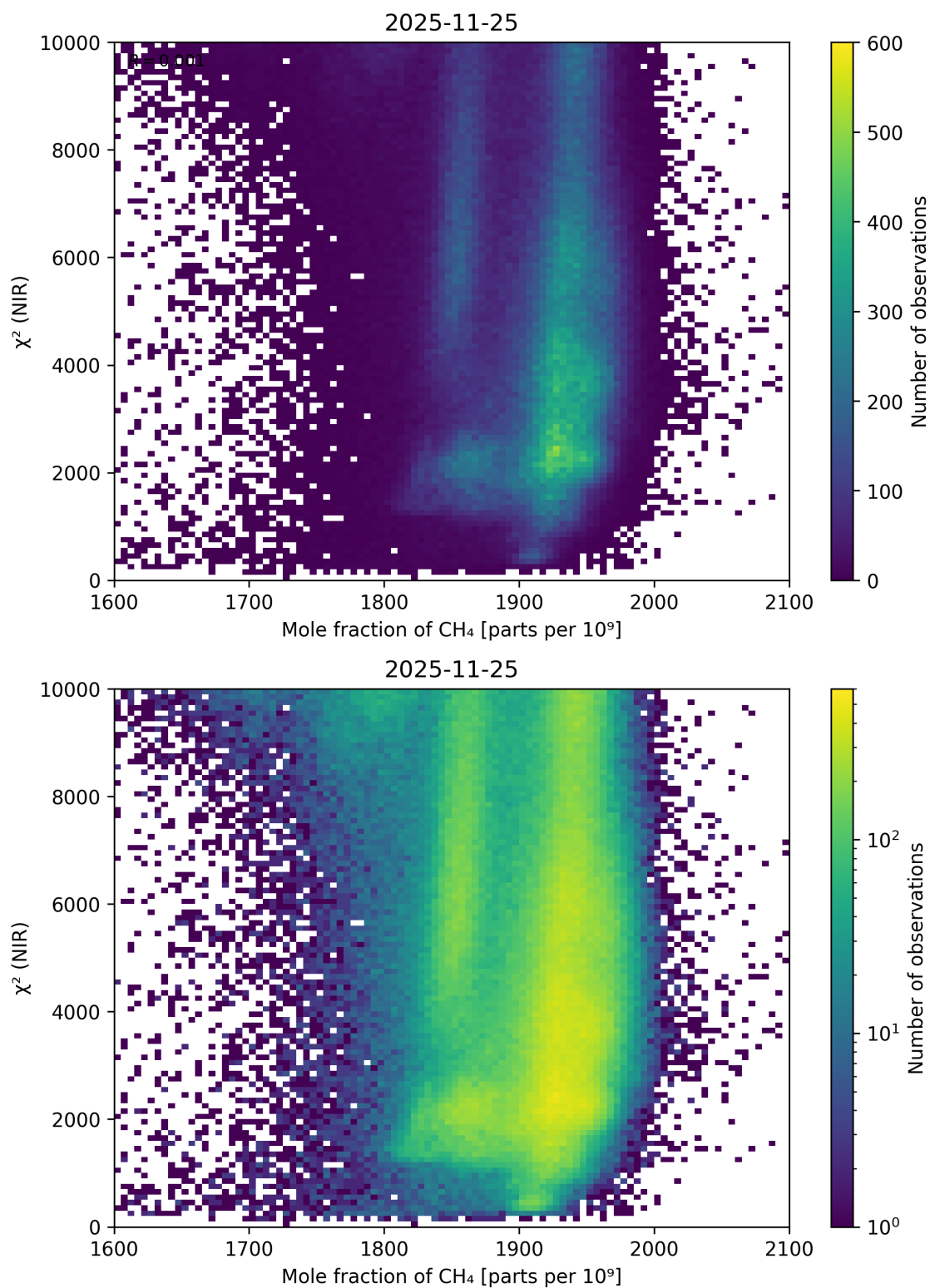
Figure 80: Scatter density plot of “Mole fraction of \text{CH}_4 ” against “ \chi^2 (NIR)” for 2025-11-24 to 2025-11-26.
