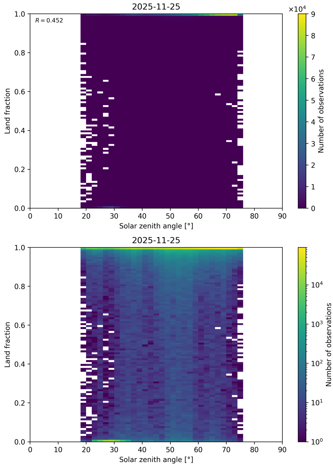
Figure 112: Scatter density plot of “Solar zenith angle” against “Land fraction” for 2025-11-24 to 2025-11-26.
