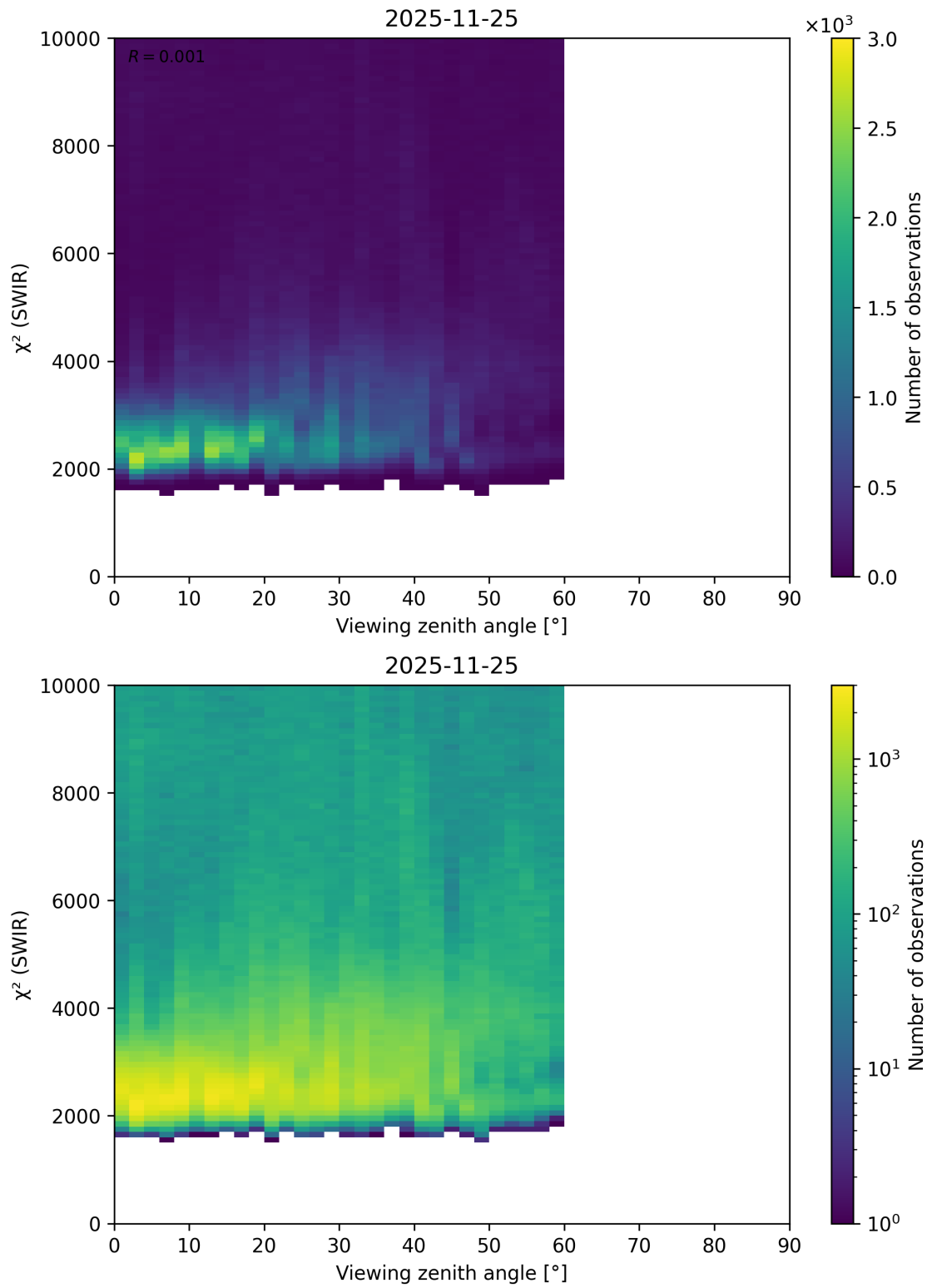
Figure 121: Scatter density plot of “Viewing zenith angle” against “ \chi^2 (SWIR)” for 2025-11-24 to 2025-11-26.
