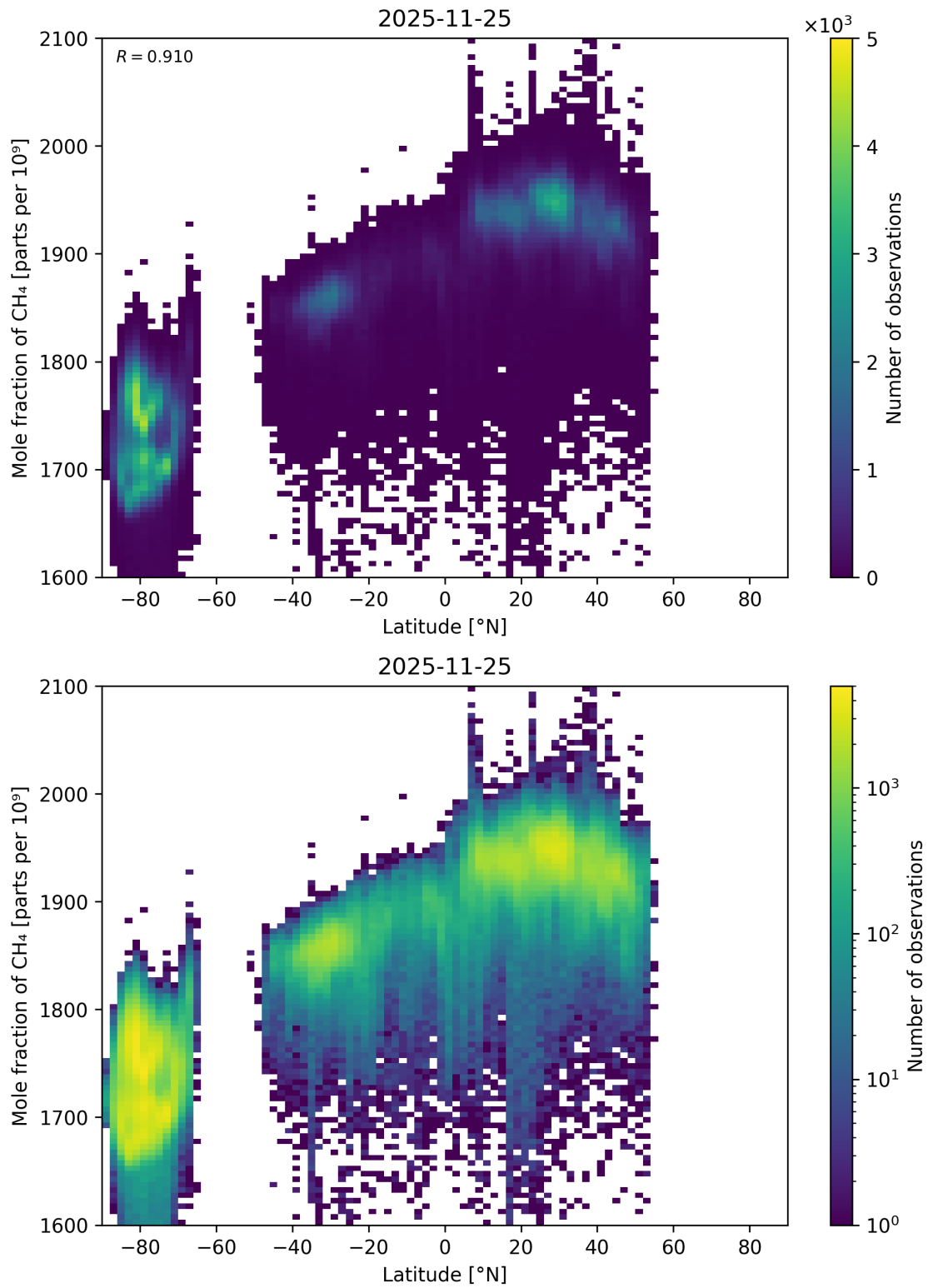
Figure 66: Scatter density plot of “Latitude” against “Mole fraction of CH 4 ” for 2025-11-24 to 2025-11-26.
