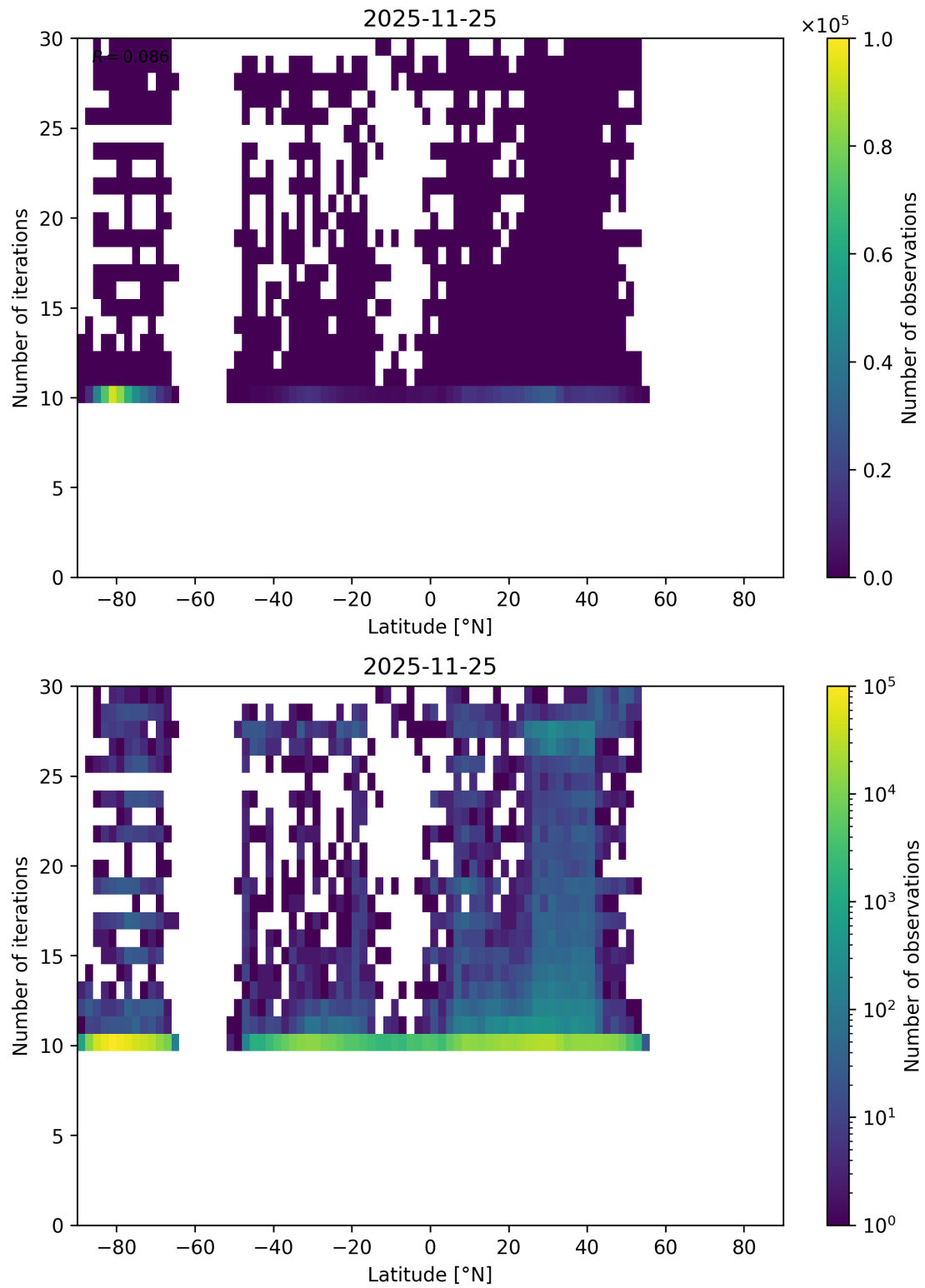
Figure 69: Scatter density plot of “Latitude” against “Number of iterations” for 2025-11-24 to 2025-11-26.
