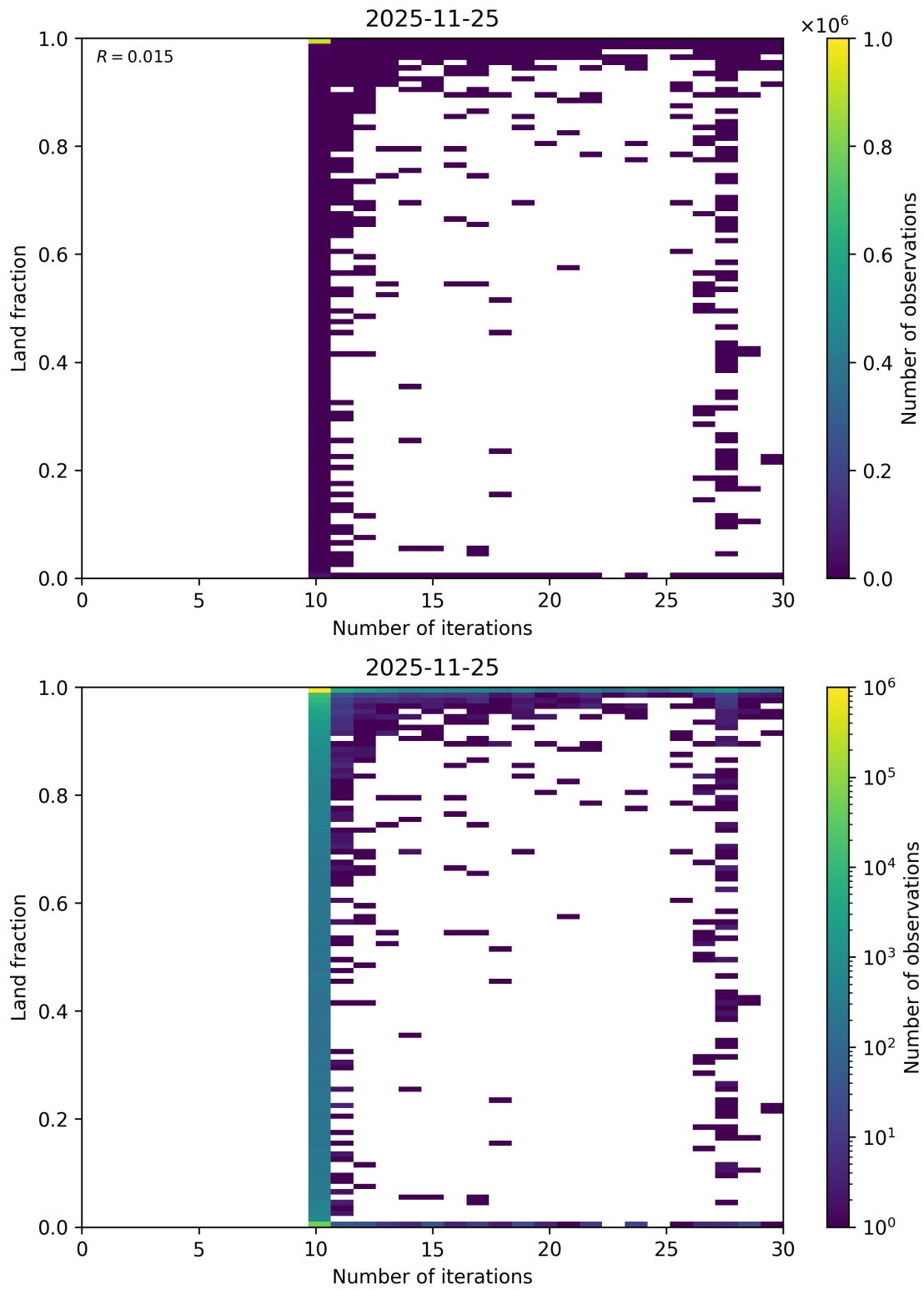
Figure 100: Scatter density plot of “Number of iterations” against “Land fraction” for 2025-11-24 to 2025-11-26.
