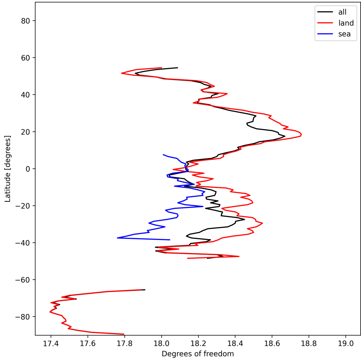
Figure 20: Zonal average of “Degrees of freedom” for 2025-11-24 to 2025-11-26.
