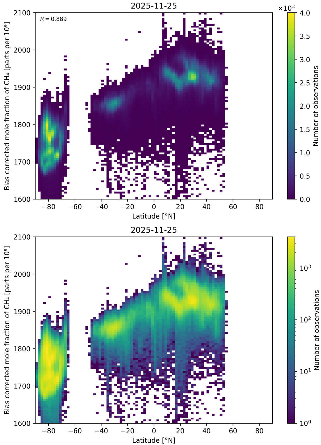
Figure 67: Scatter density plot of “Latitude” against “Bias corrected mole fraction of \text{CH}_4 ” for 2025-11-24 to 2025-11-26.
