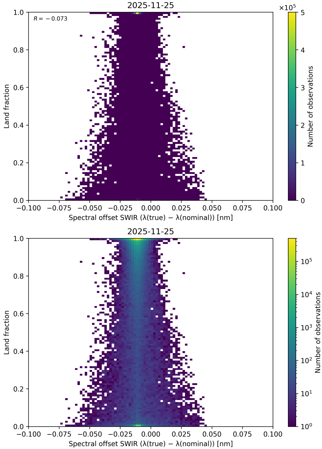
Figure 137: Scatter density plot of “Spectral offset SWIR ( \lambda_{\text{true}} - \lambda_{\text{nominal}} )” against “Land fraction” for 2025-11-24 to 2025-11-26.
