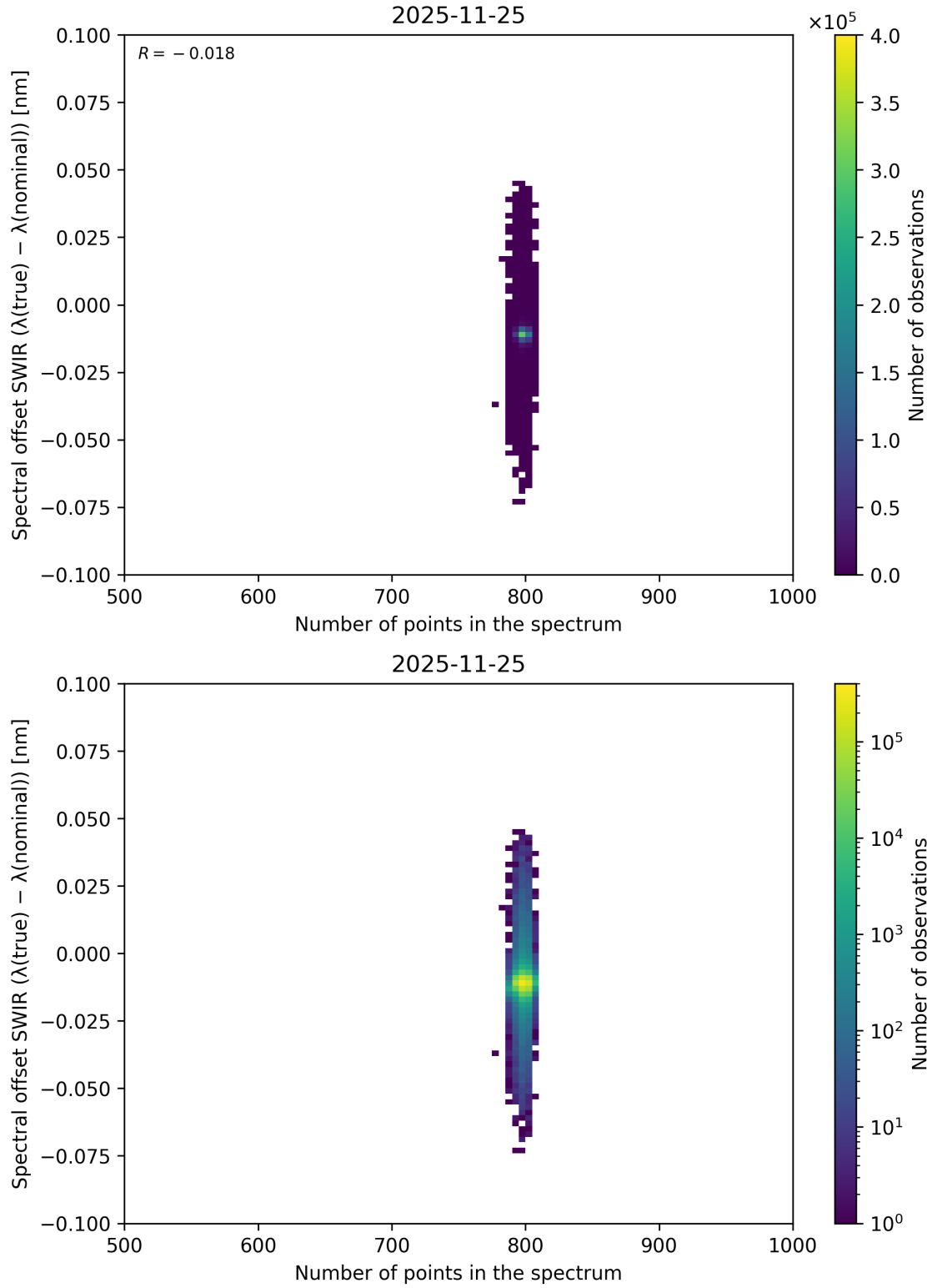
Figure 107: Scatter density plot of “Number of points in the spectrum” against “Spectral offset SWIR ( \lambda_{\text{true}} - \lambda_{\text{nominal}} )” for 2025-11-24 to 2025-11-26.
