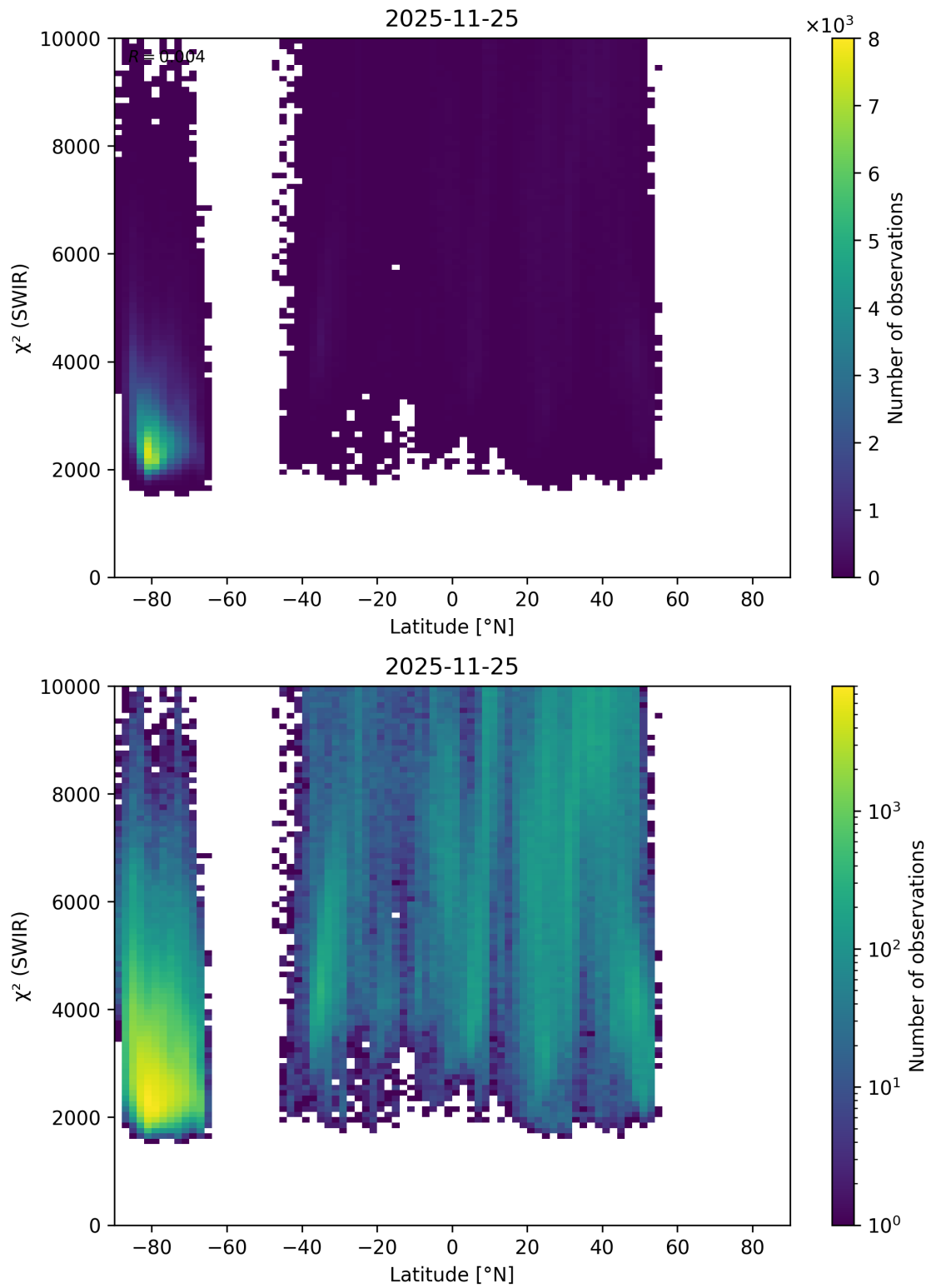
Figure 62: Scatter density plot of “Latitude” against “ \chi^2 (SWIR)” for 2025-11-24 to 2025-11-26.
