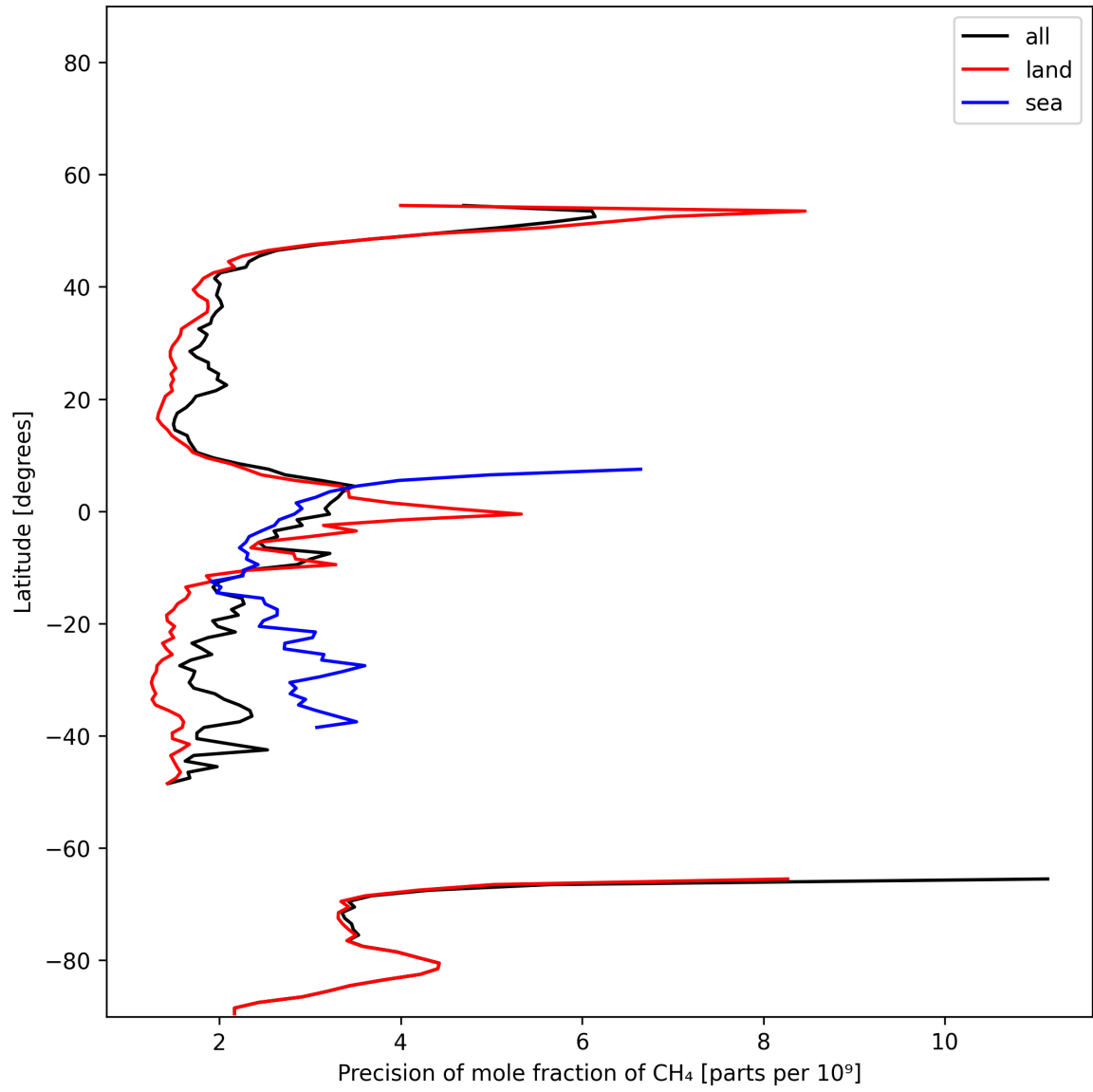
Figure 14: Zonal average of “Precision of mole fraction of CH 4 ” for 2025-11-24 to 2025-11-26.
