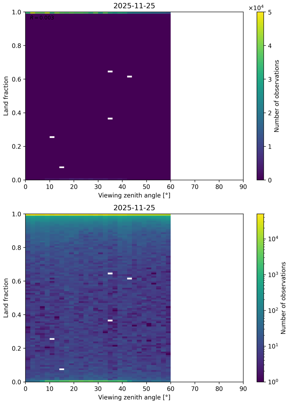
Figure 124: Scatter density plot of “Viewing zenith angle” against “Land fraction” for 2025-11-24 to 2025-11-26.
