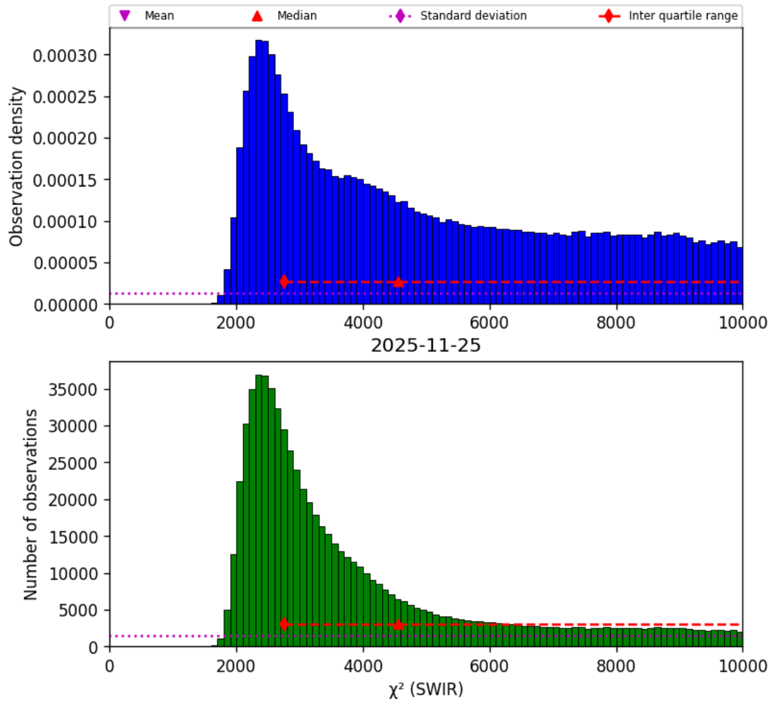
Figure 30: Histogram of “ \chi^2 (SWIR)” for 2025-11-24 to 2025-11-26
