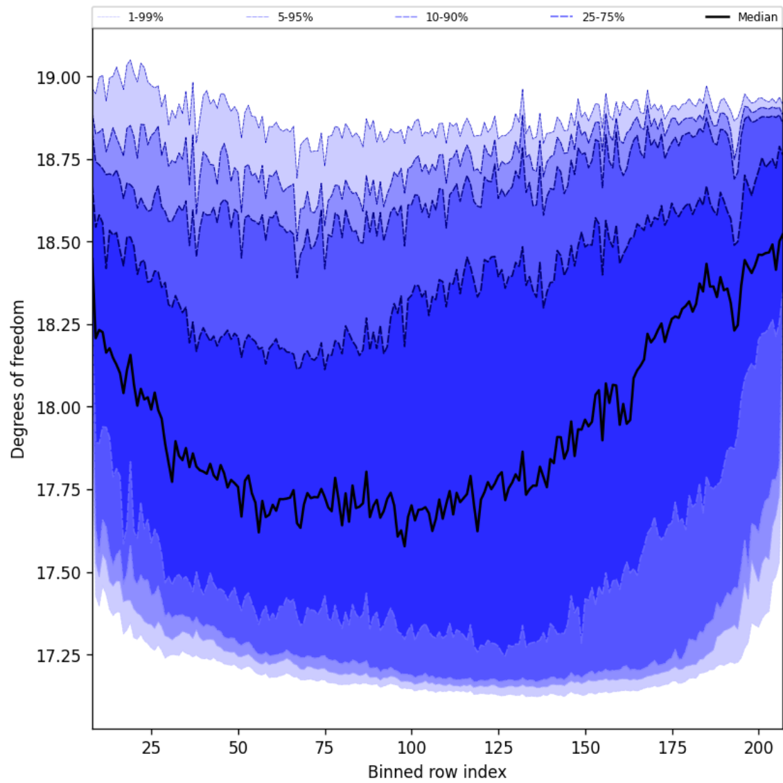
Figure 44: Along track statistics of “Degrees of freedom” for 2025-11-24 to 2025-11-26
