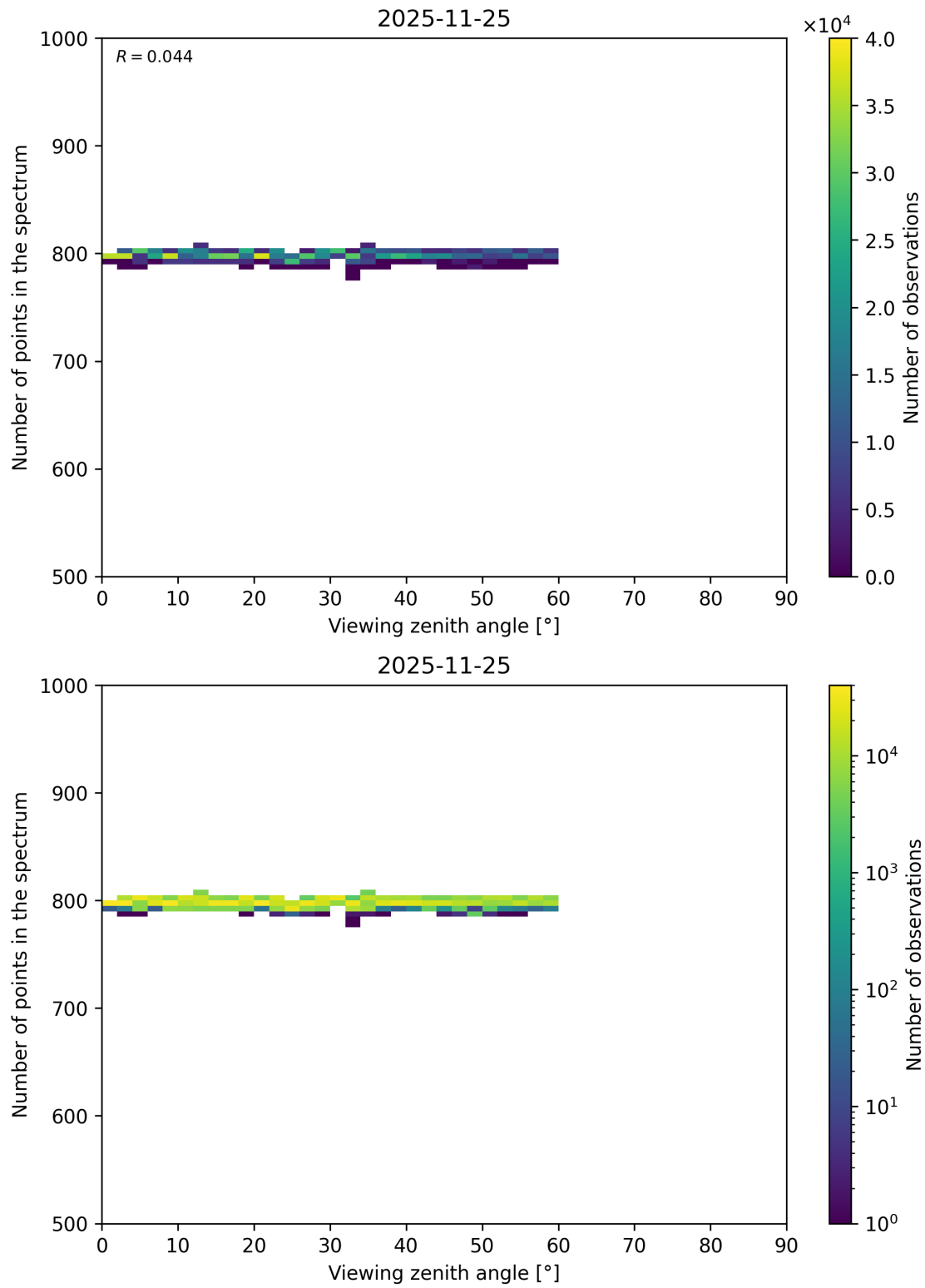
Figure 130: Scatter density plot of “Viewing zenith angle” against “Number of points in the spectrum” for 2025-11-24 to 2025-11-26.
