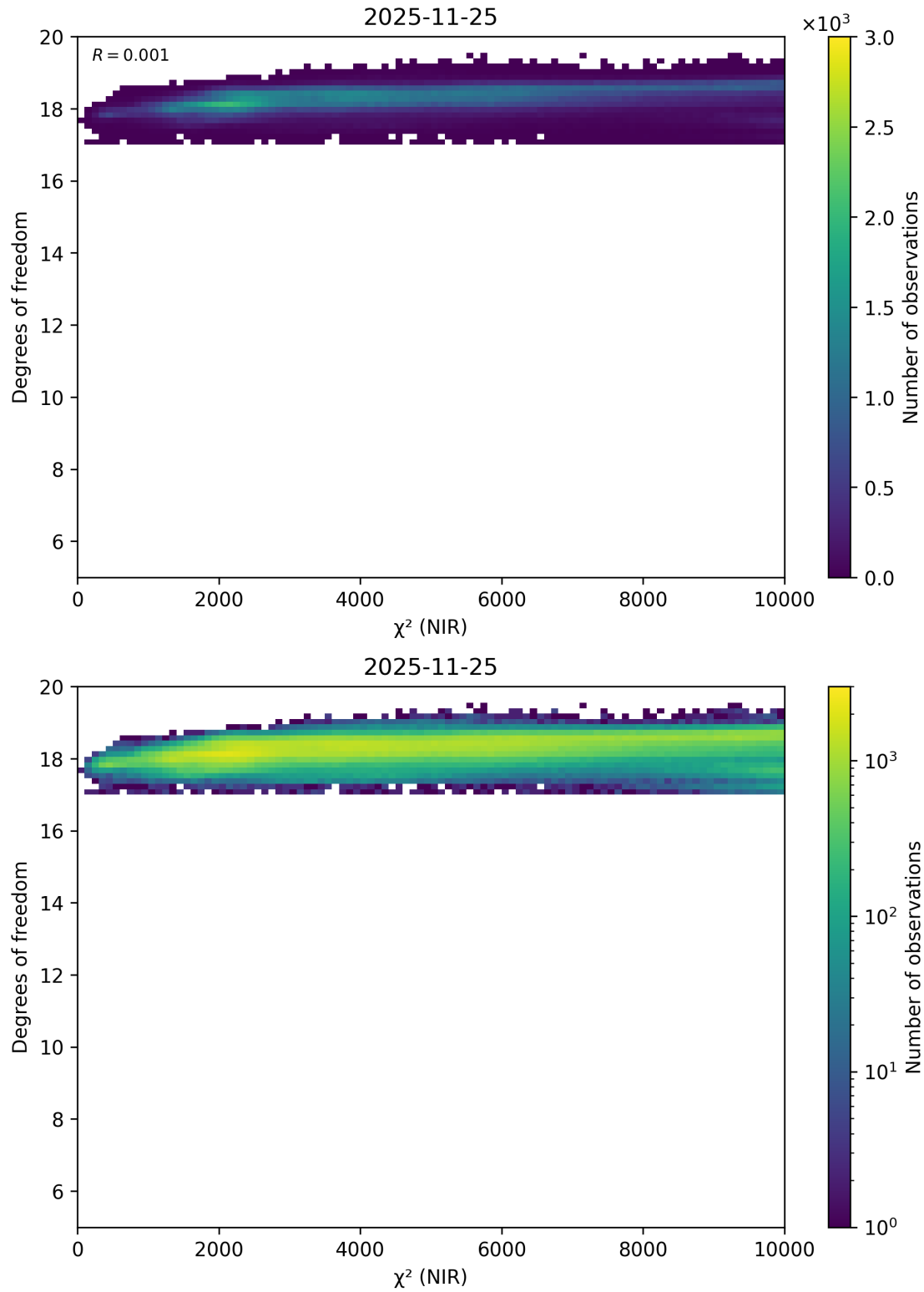
Figure 48: Scatter density plot of “ \chi^2 (NIR)” against “Degrees of freedom” for 2025-11-24 to 2025-11-26.
