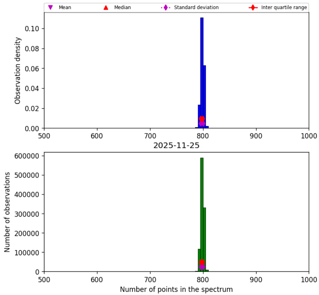
Figure 28: Histogram of “Number of points in the spectrum” for 2025-11-24 to 2025-11-26
