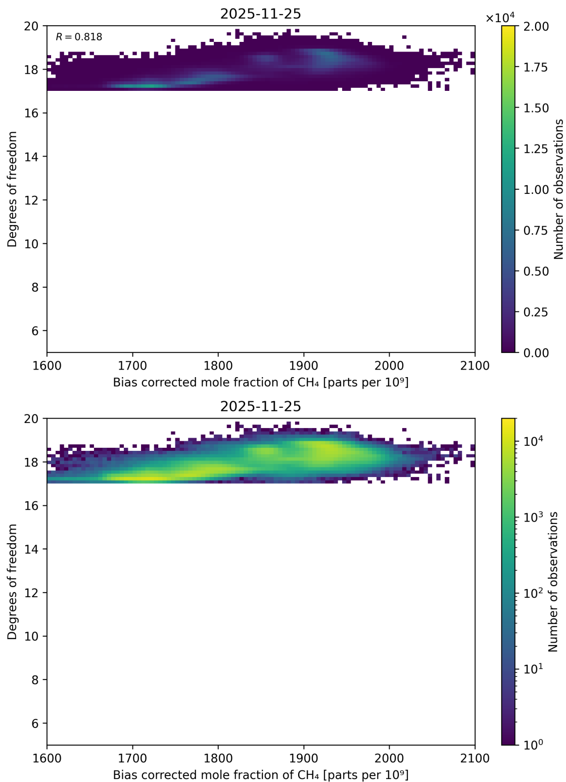
Figure 74: Scatter density plot of “Bias corrected mole fraction of CH 4 ” against “Degrees of freedom” for 2025-11-24 to 2025-11-26.
