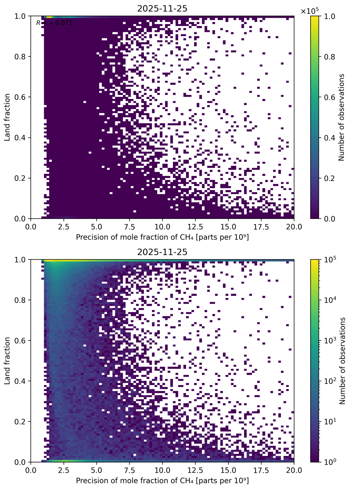
Figure 93: Scatter density plot of “Precision of mole fraction of CH 4 ” against “Land fraction” for 2025-11-24 to 2025-11-26.
