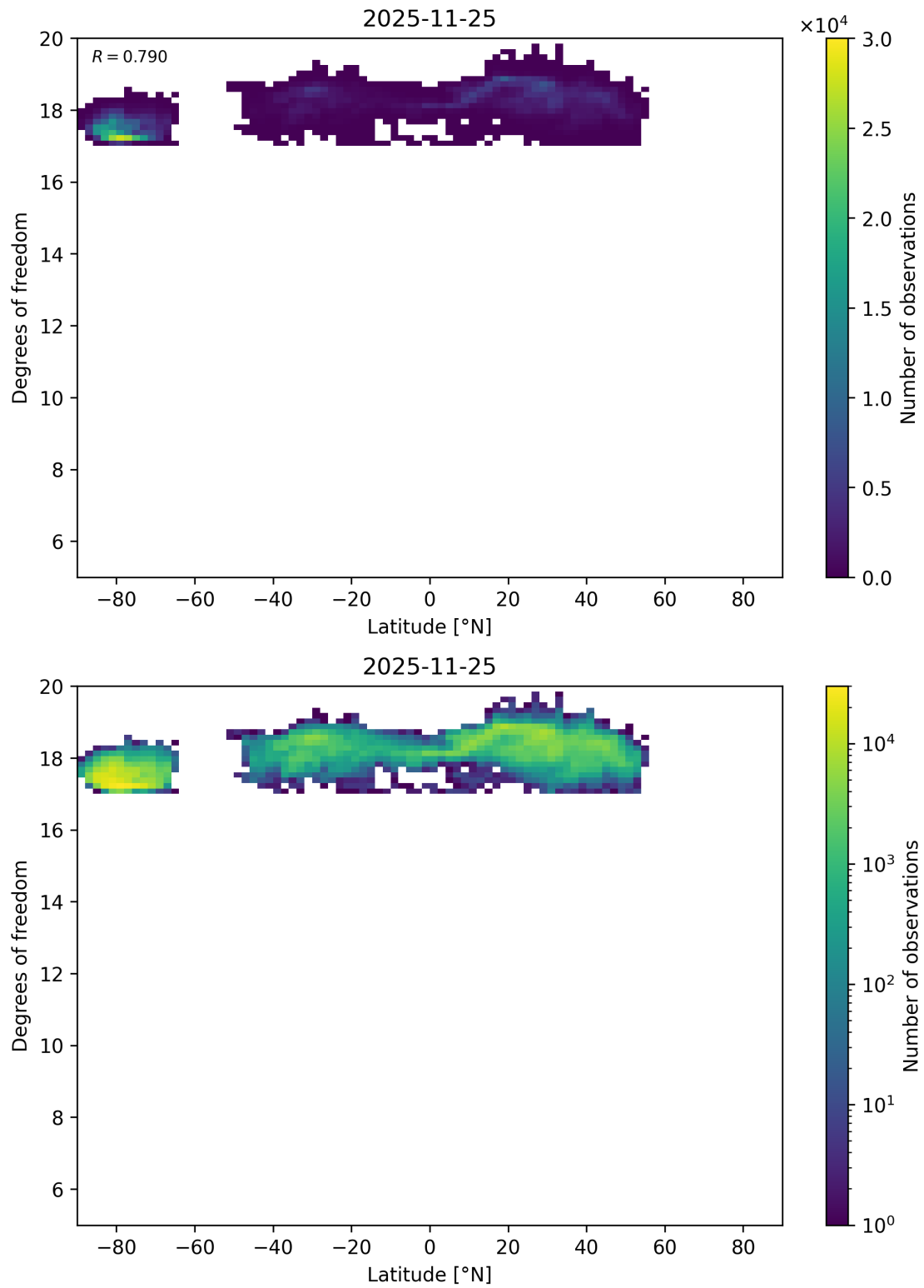
Figure 63: Scatter density plot of “Latitude” against “Degrees of freedom” for 2025-11-24 to 2025-11-26.
