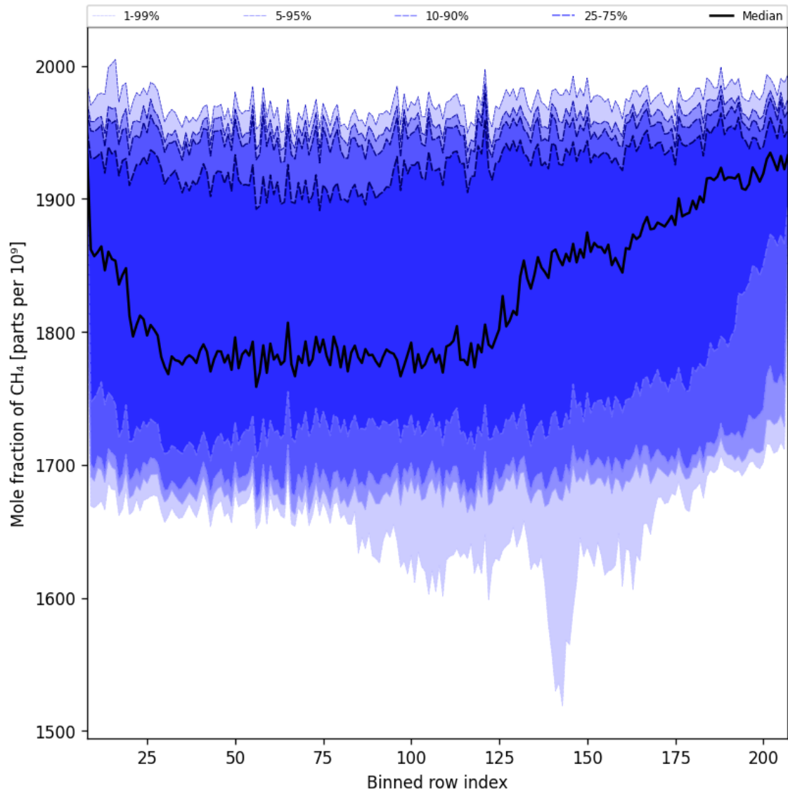
Figure 37: Along track statistics of “Mole fraction of CH 4 ” for 2025-11-24 to 2025-11-26
