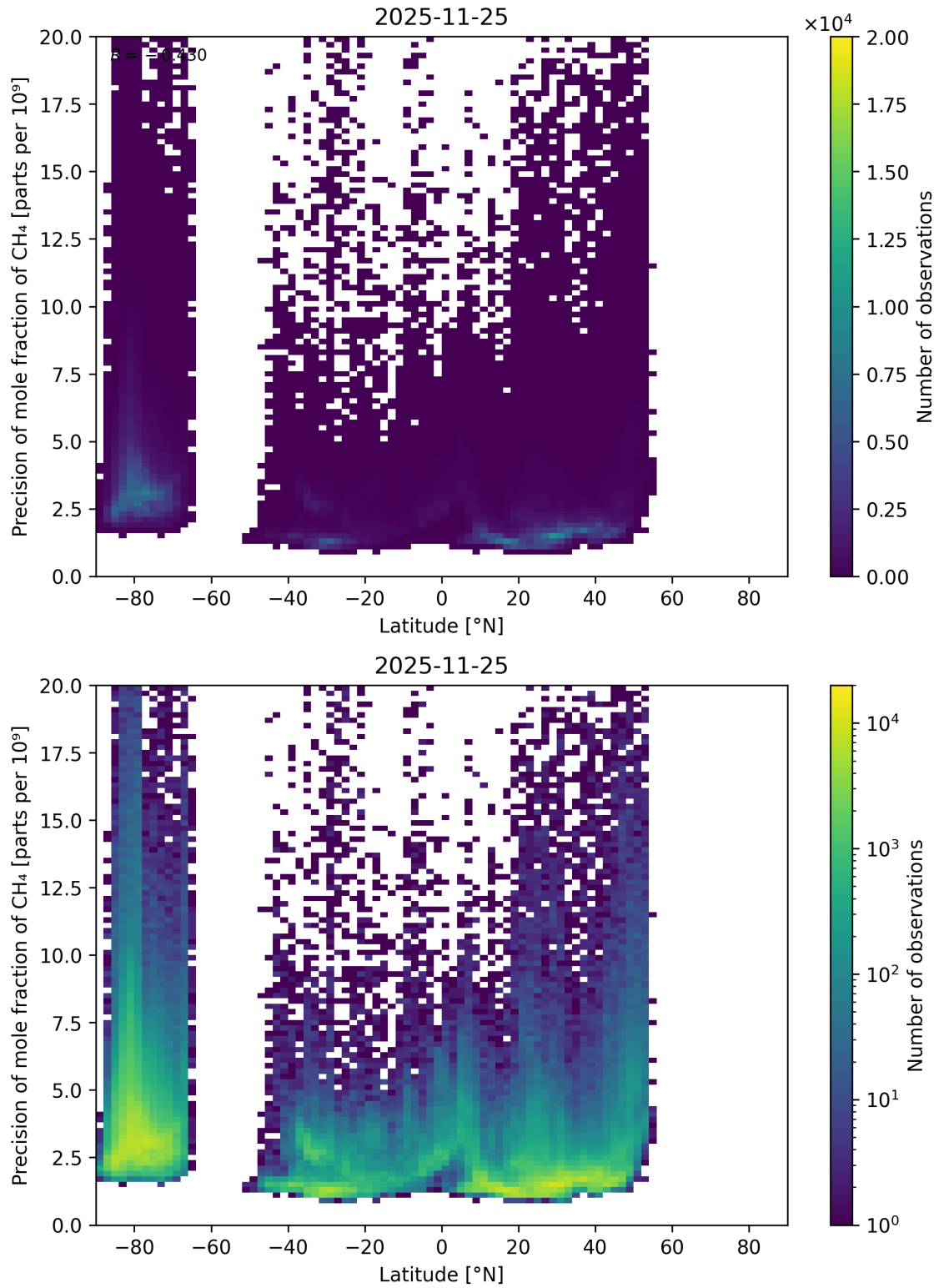
Figure 68: Scatter density plot of “Latitude” against “Precision of mole fraction of CH 4 ” for 2025-11-24 to 2025-11-26.
