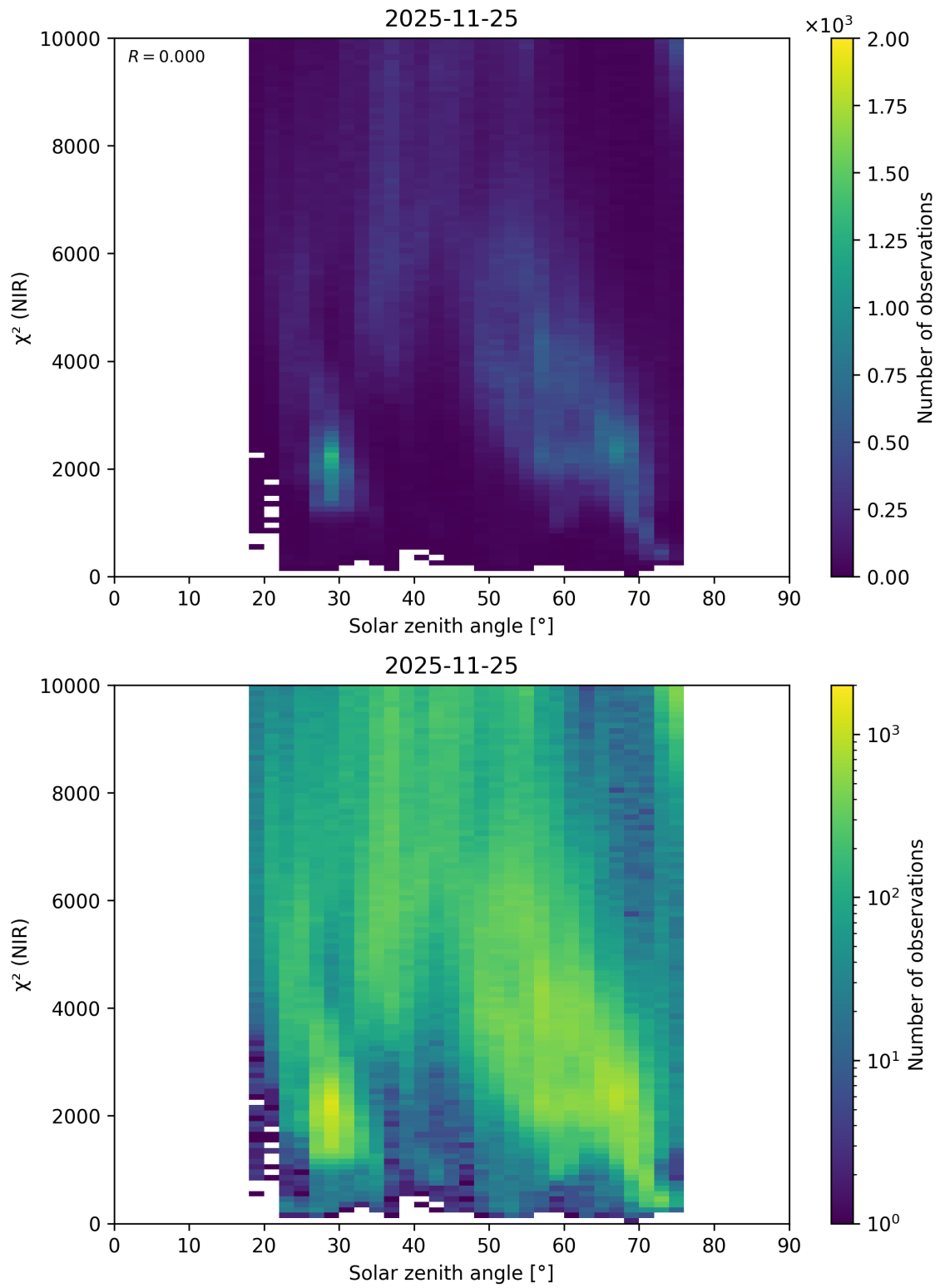
Figure 108: Scatter density plot of “Solar zenith angle” against “ \chi^2 (NIR)” for 2025-11-24 to 2025-11-26.
