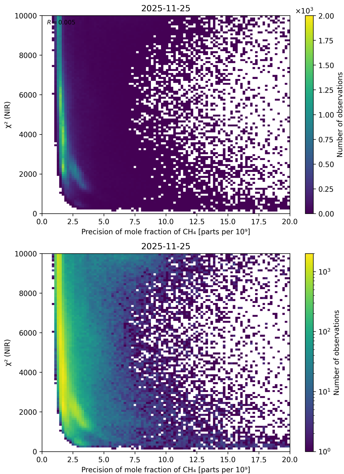
Figure 89: Scatter density plot of “Precision of mole fraction of \text{CH}_4 ” against “ \chi^2 (NIR)” for 2025-11-24 to 2025-11-26.
