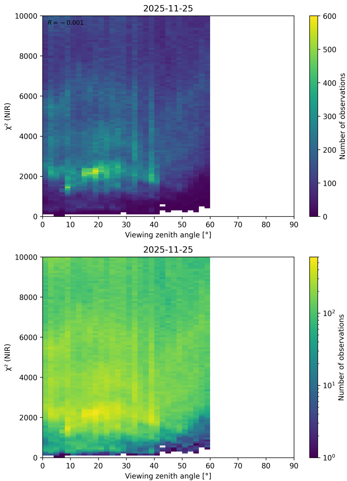
Figure 120: Scatter density plot of “Viewing zenith angle” against “ \chi^2 (NIR)” for 2025-11-24 to 2025-11-26.
