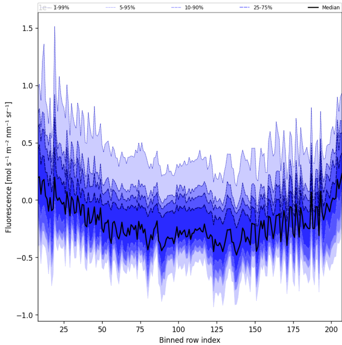
Figure 46: Along track statistics of “Fluorescence” for 2025-11-24 to 2025-11-26
