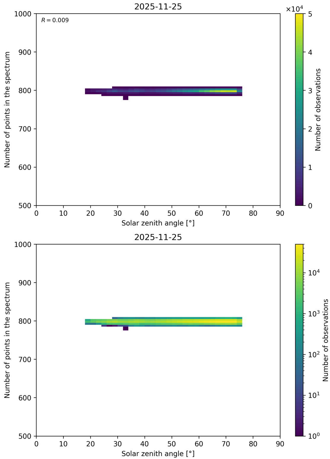
Figure 118: Scatter density plot of “Solar zenith angle” against “Number of points in the spectrum” for 2025-11-24 to 2025-11-26.
