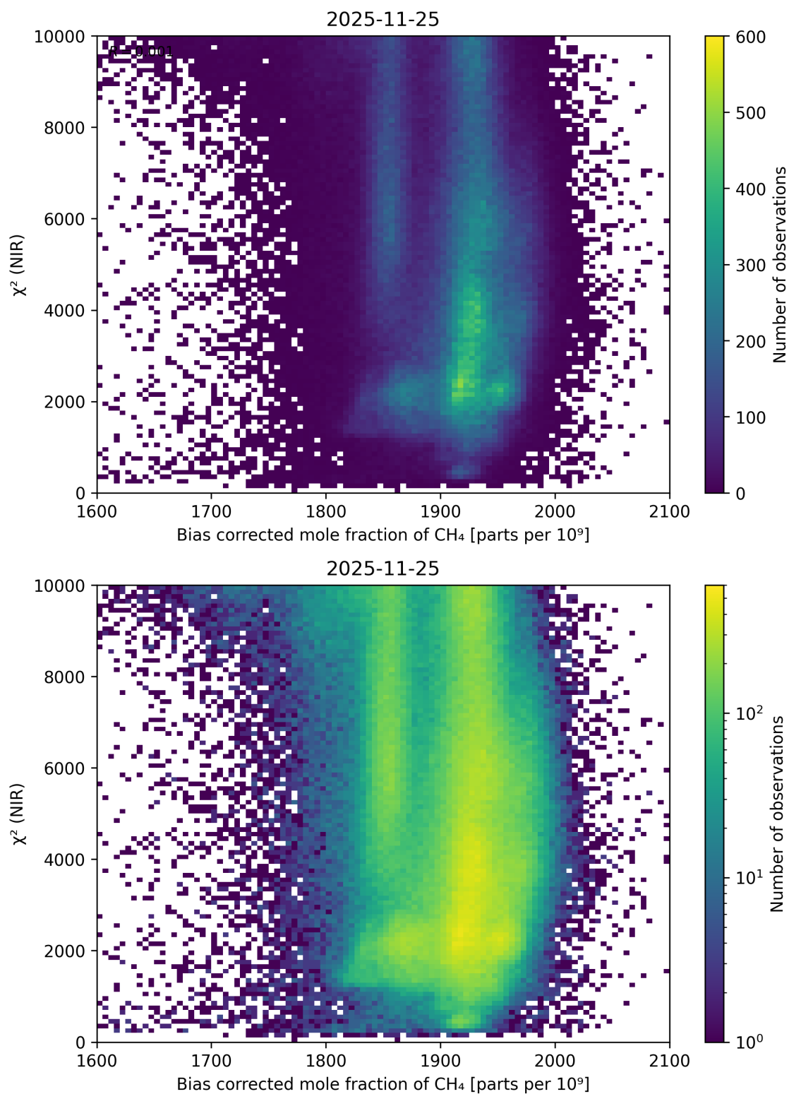
Figure 72: Scatter density plot of “Bias corrected mole fraction of CH 4 ” against “ \chi^2 (NIR)” for 2025-11-24 to 2025-11-26.
