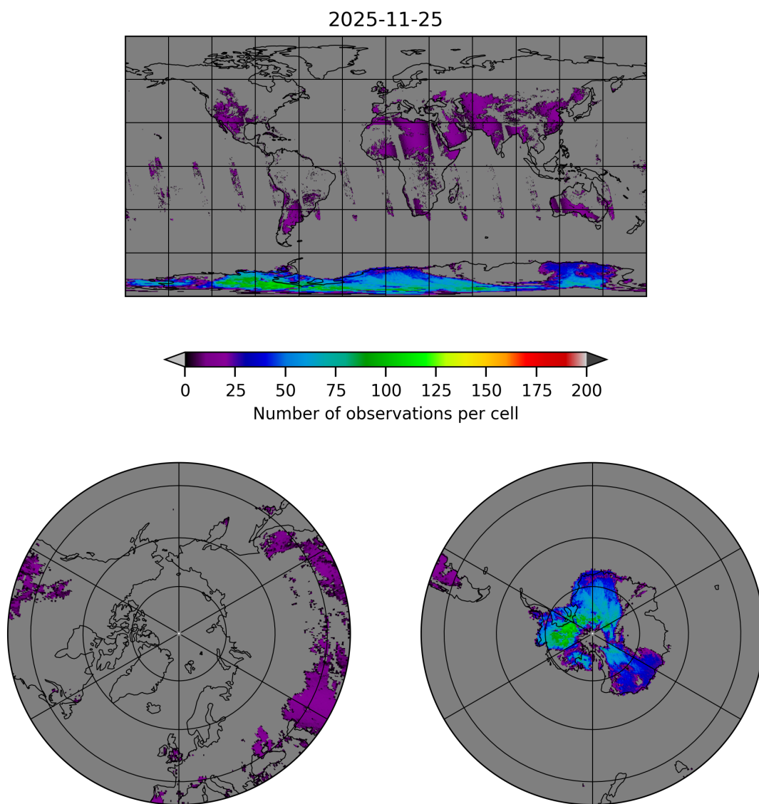
Figure 11: Map of the number of observations for 2025-11-24 to 2025-11-26
