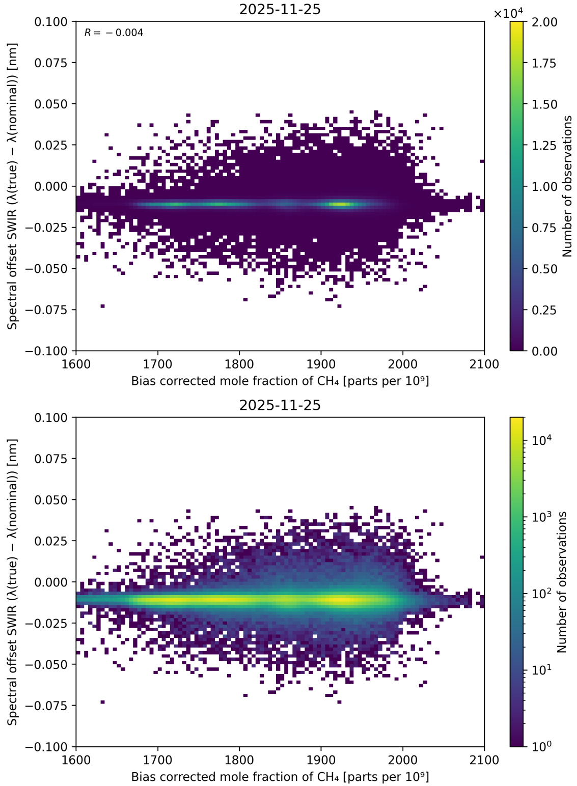
Figure 79: Scatter density plot of “Bias corrected mole fraction of \text{CH}_4 ” against “Spectral offset SWIR ( \lambda_{\text{true}} - \lambda_{\text{nominal}} )” for 2025-11-24 to 2025-11-26.
