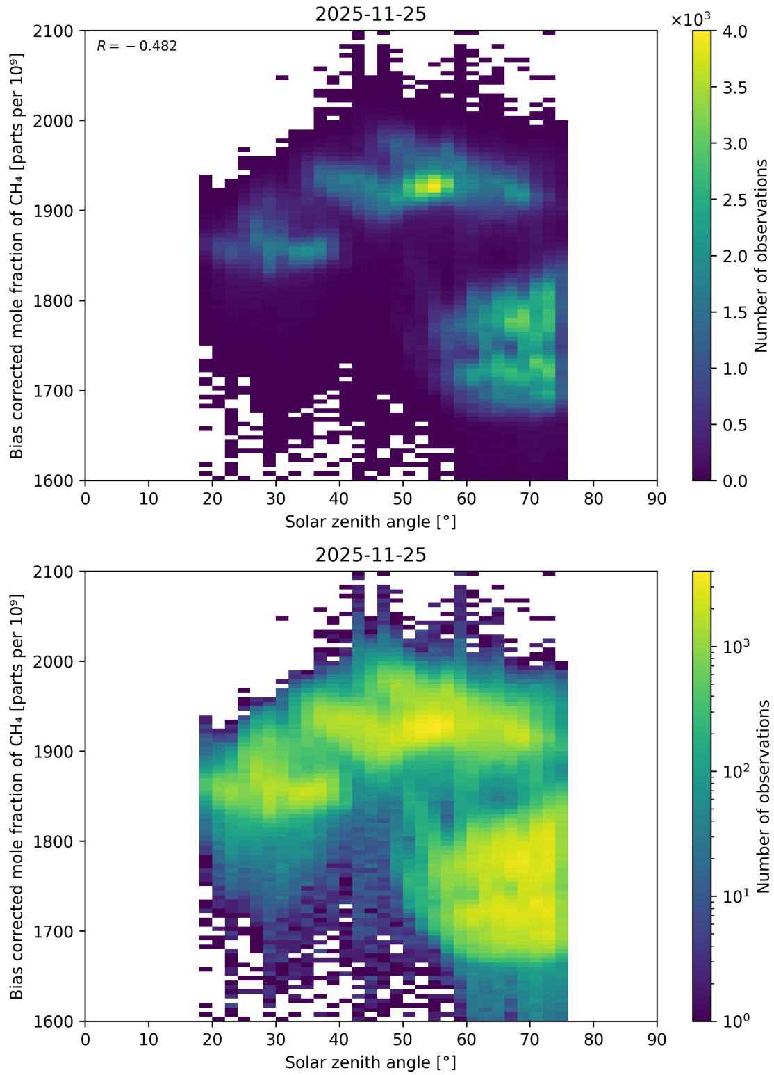
Figure 115: Scatter density plot of “Solar zenith angle” against “Bias corrected mole fraction of CH 4 ” for 2025-11-24 to 2025-11-26.
