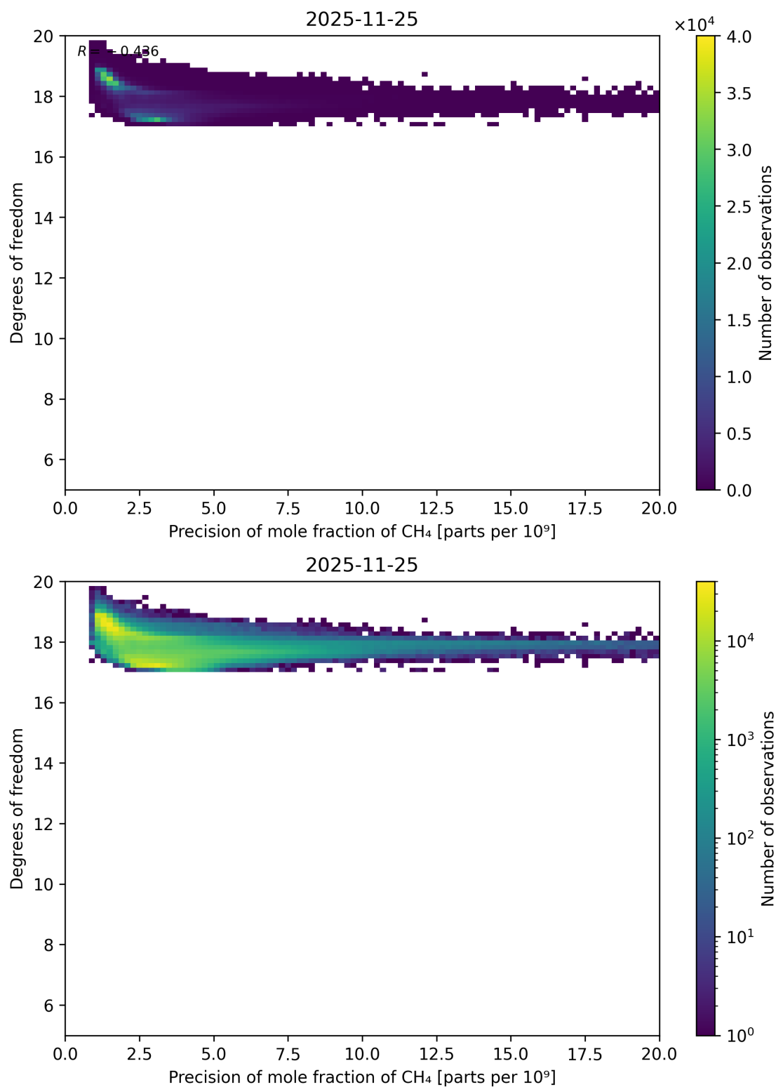
Figure 91: Scatter density plot of “Precision of mole fraction of CH 4 ” against “Degrees of freedom” for 2025-11-24 to 2025-11-26.
