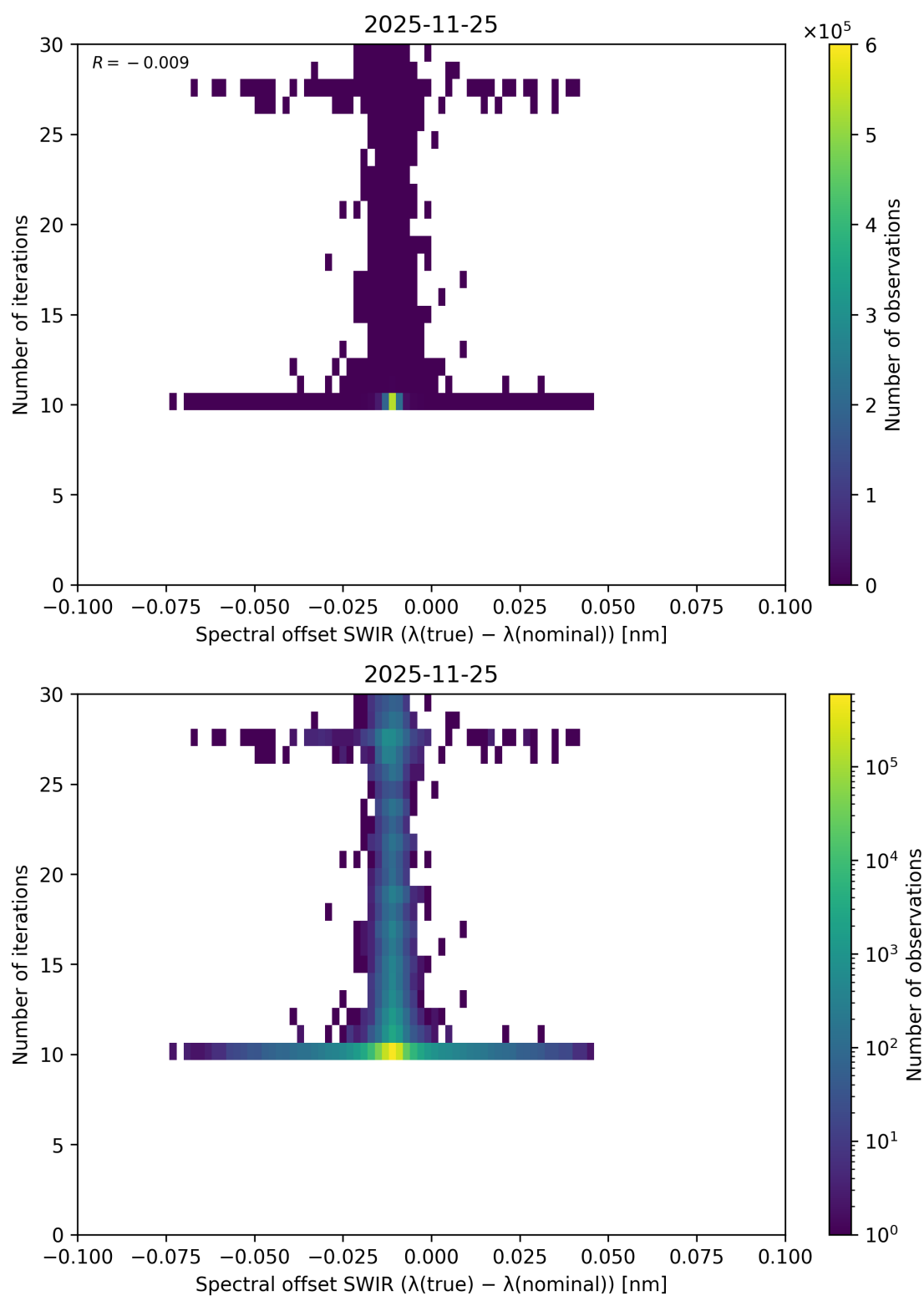
Figure 138: Scatter density plot of “Spectral offset SWIR ( \lambda_{\text{true}} - \lambda_{\text{nominal}} )” against “Number of iterations” for 2025-11-24 to 2025-11-26.
