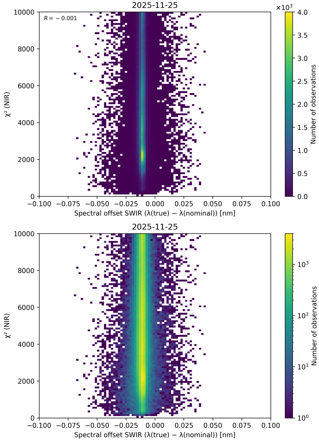
Figure 133: Scatter density plot of “Spectral offset SWIR ( \lambda_{\text{true}} - \lambda_{\text{nominal}} )” against “ \chi^2 (NIR)” for 2025-11-24 to 2025-11-26.
