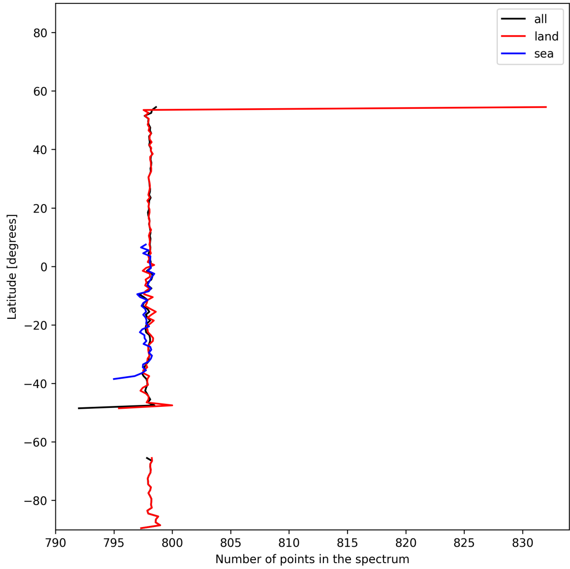
Figure 16: Zonal average of “Number of points in the spectrum” for 2025-11-24 to 2025-11-26.
