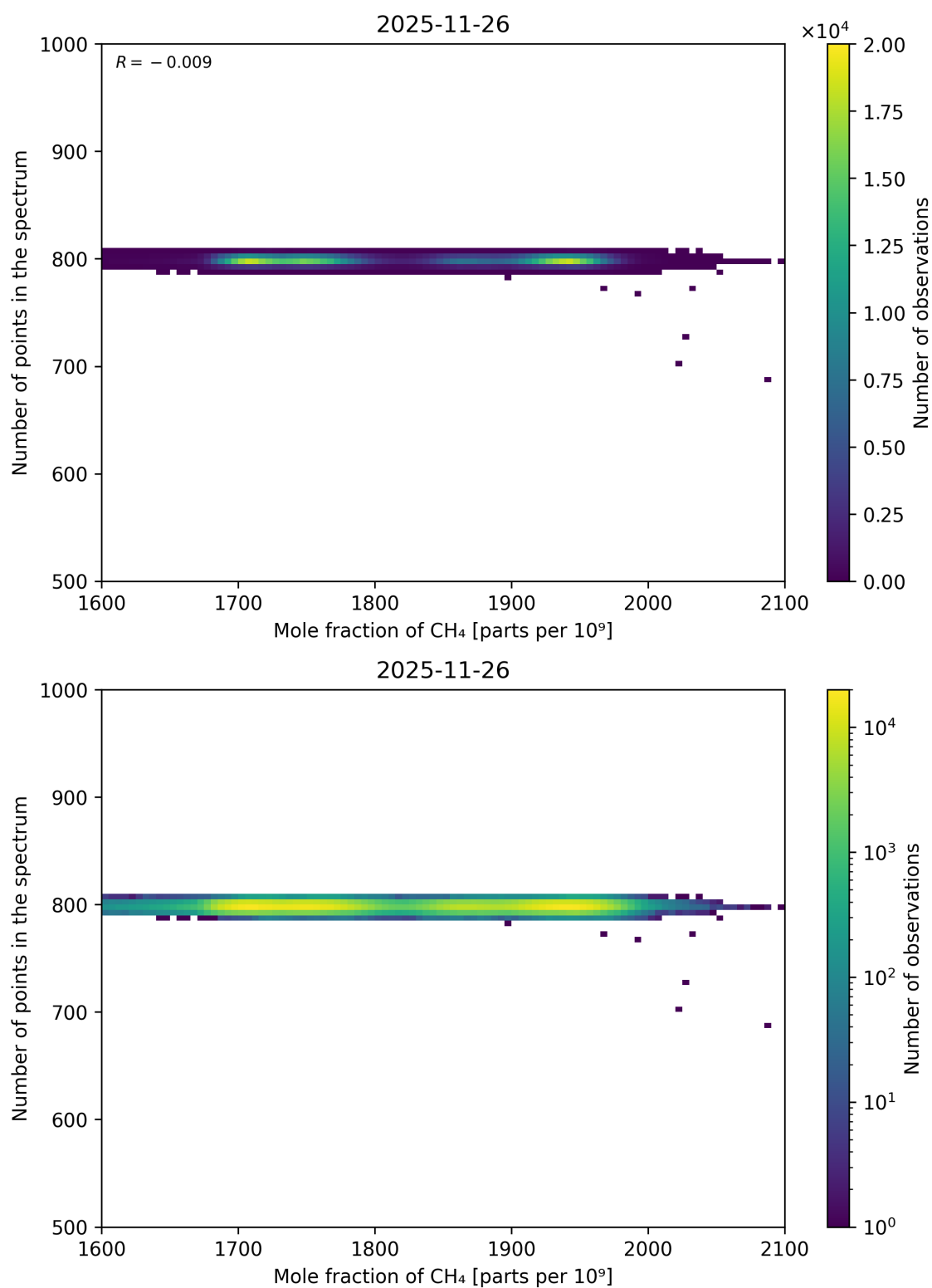
Figure 88: Scatter density plot of “Mole fraction of CH 4 ” against “Number of points in the spectrum” for 2025-11-25 to 2025-11-27.
