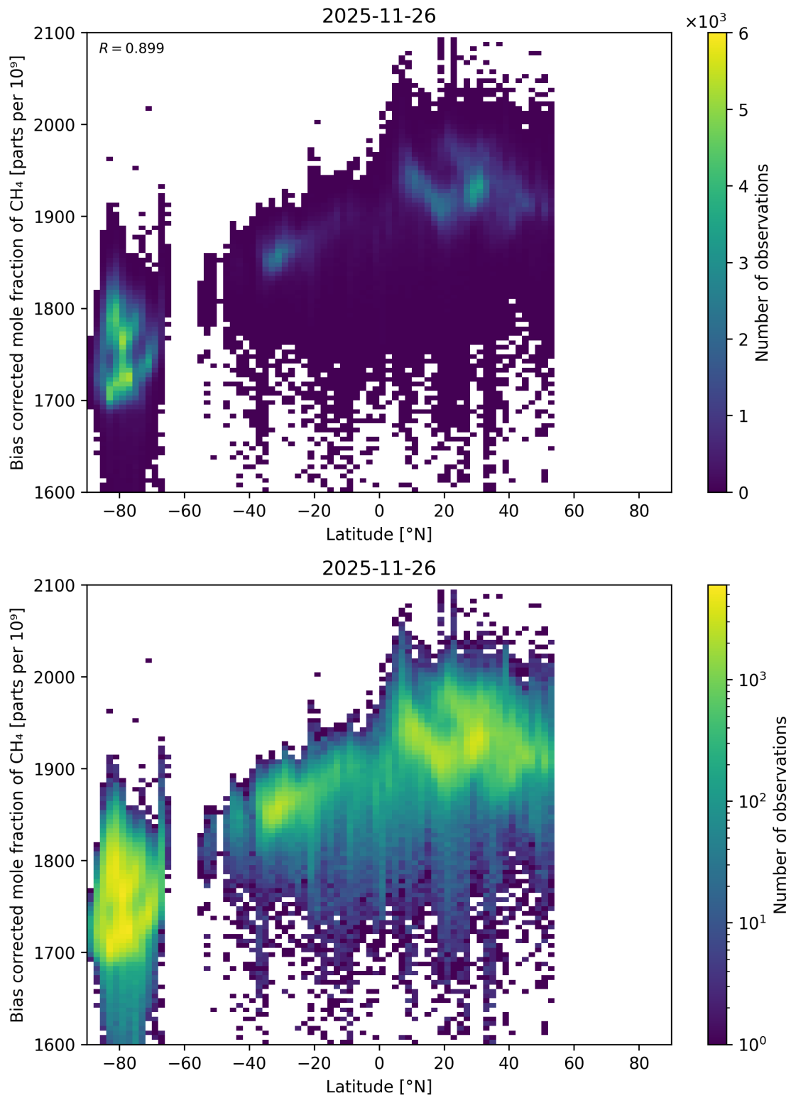
Figure 67: Scatter density plot of “Latitude” against “Bias corrected mole fraction of \text{CH}_4 ” for 2025-11-25 to 2025-11-27.
