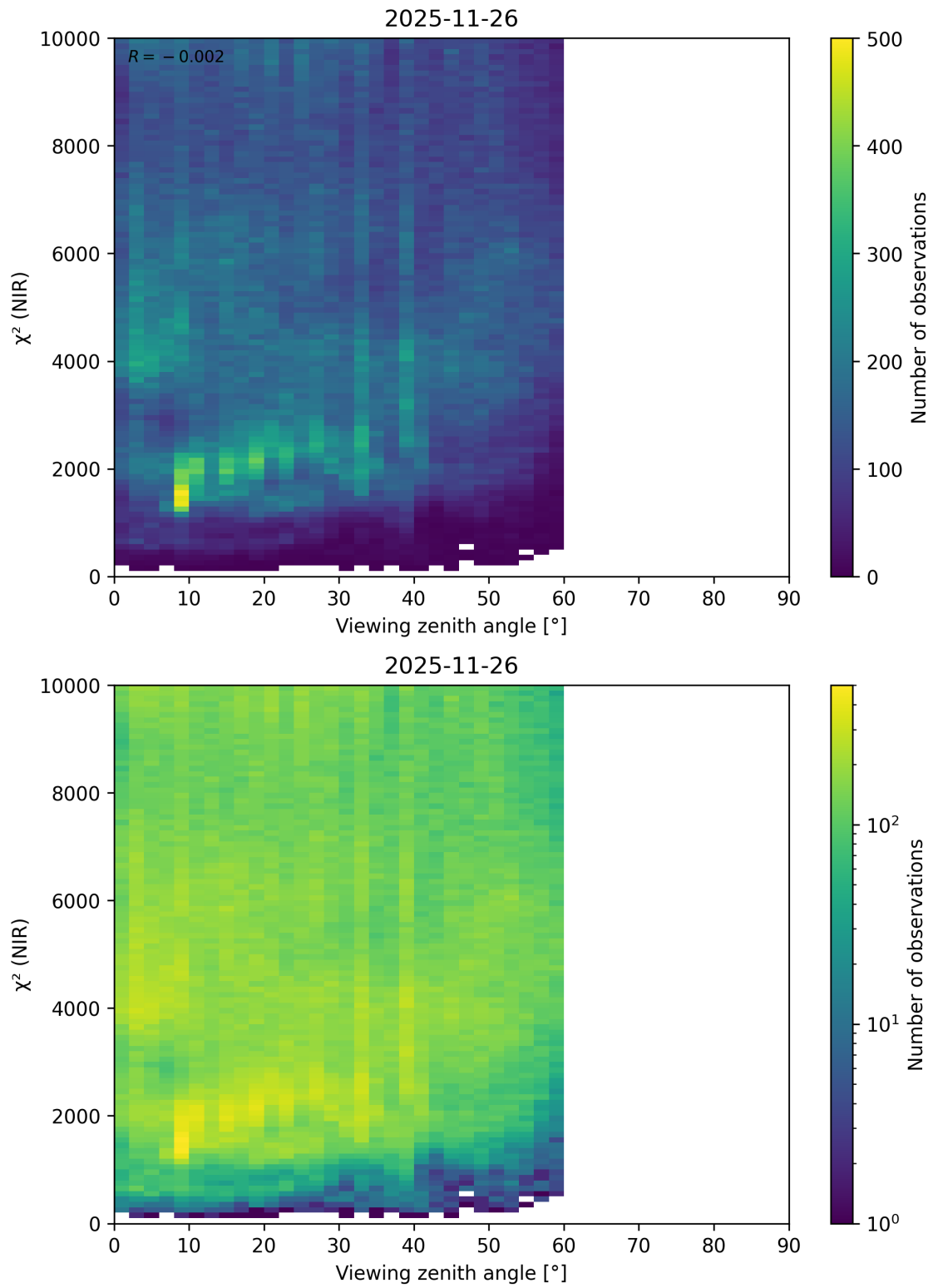
Figure 120: Scatter density plot of “Viewing zenith angle” against “ \chi^2 (NIR)” for 2025-11-25 to 2025-11-27.
