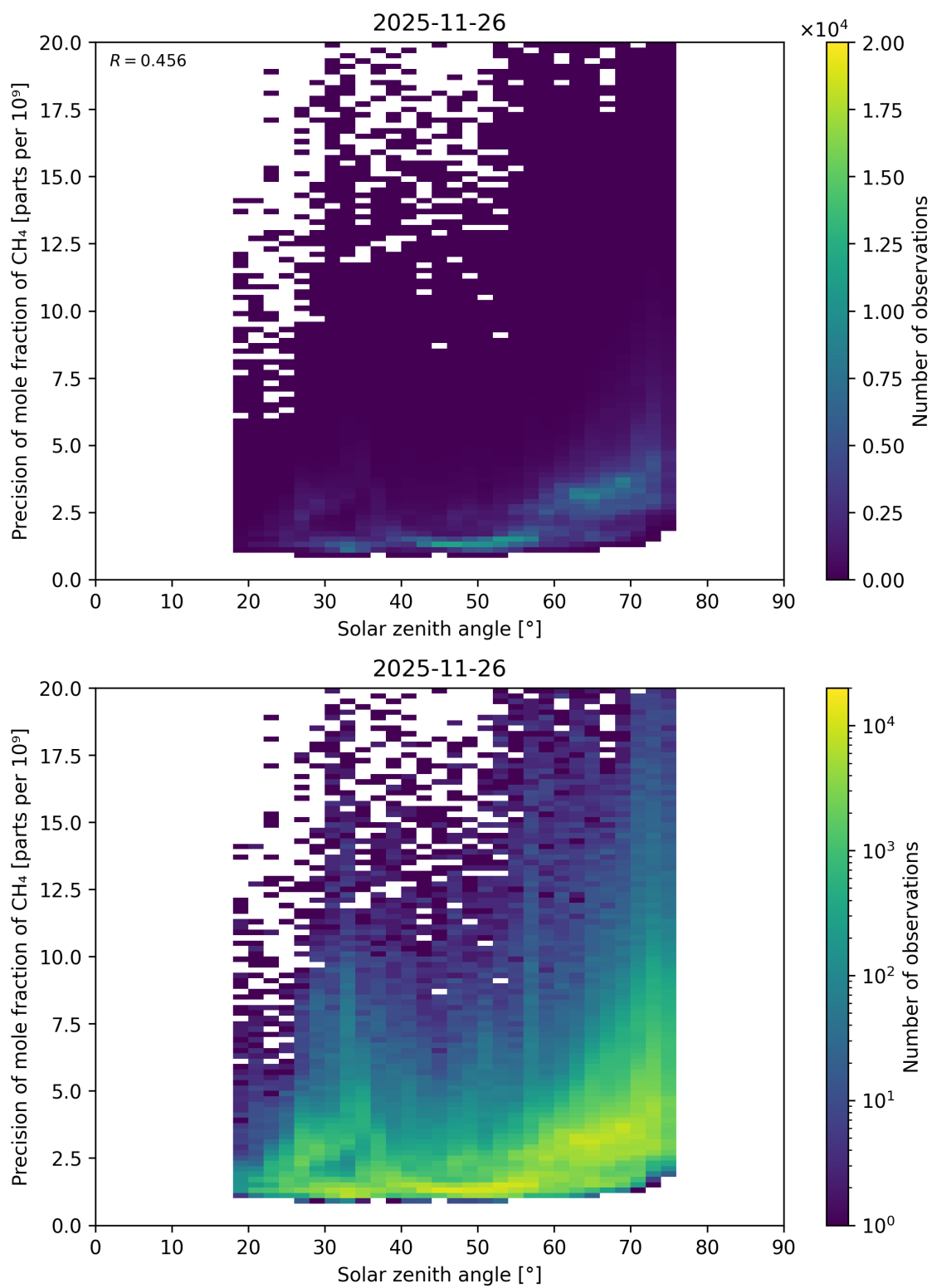
Figure 116: Scatter density plot of “Solar zenith angle” against “Precision of mole fraction of \text{CH}_4 ” for 2025-11-25 to 2025-11-27.
