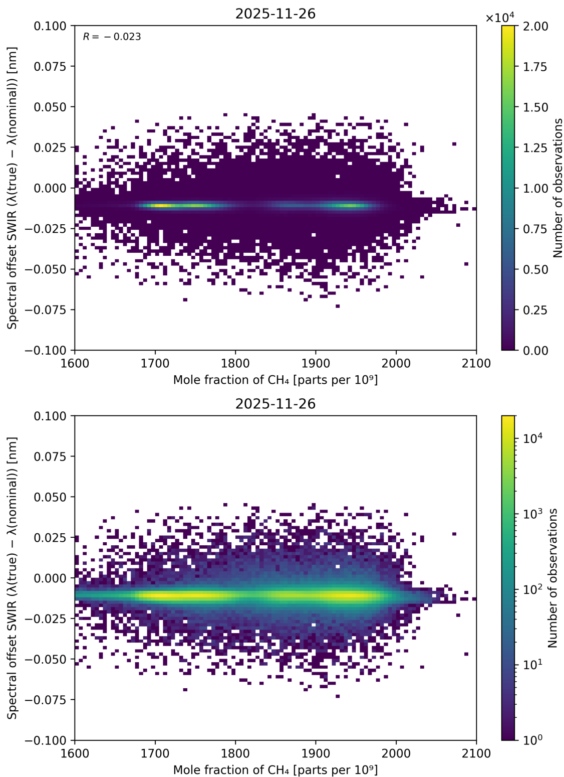
Figure 98: Scatter density plot of “Mole fraction of CH 4 ” against “Spectral offset SWIR ( \lambda_{\text{true}} - \lambda_{\text{nominal}} )” for 2025-11-25 to 2025-11-27.
