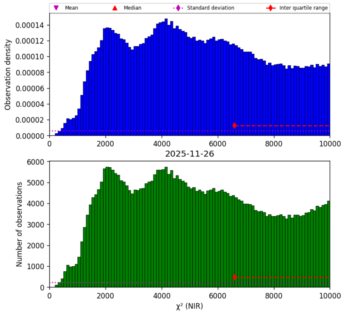
Figure 31: Histogram of " \chi^2 (NIR)" for 2025-11-25 to 2025-11-27
