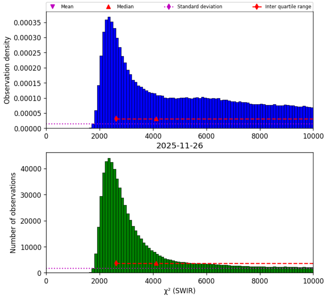
Figure 30: Histogram of " \chi^2 (SWIR)" for 2025-11-25 to 2025-11-27
