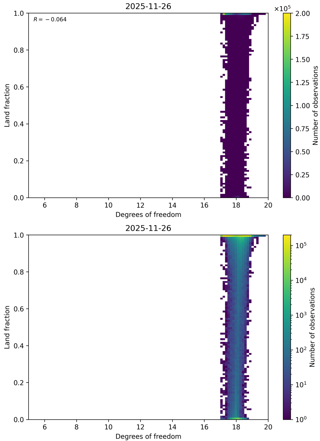
Figure 58: Scatter density plot of “Degrees of freedom” against “Land fraction” for 2025-11-25 to 2025-11-27.
