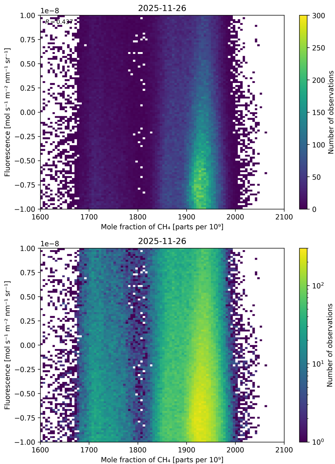
Figure 83: Scatter density plot of “Mole fraction of \text{CH}_4 ” against “Fluorescence” for 2025-11-25 to 2025-11-27.
