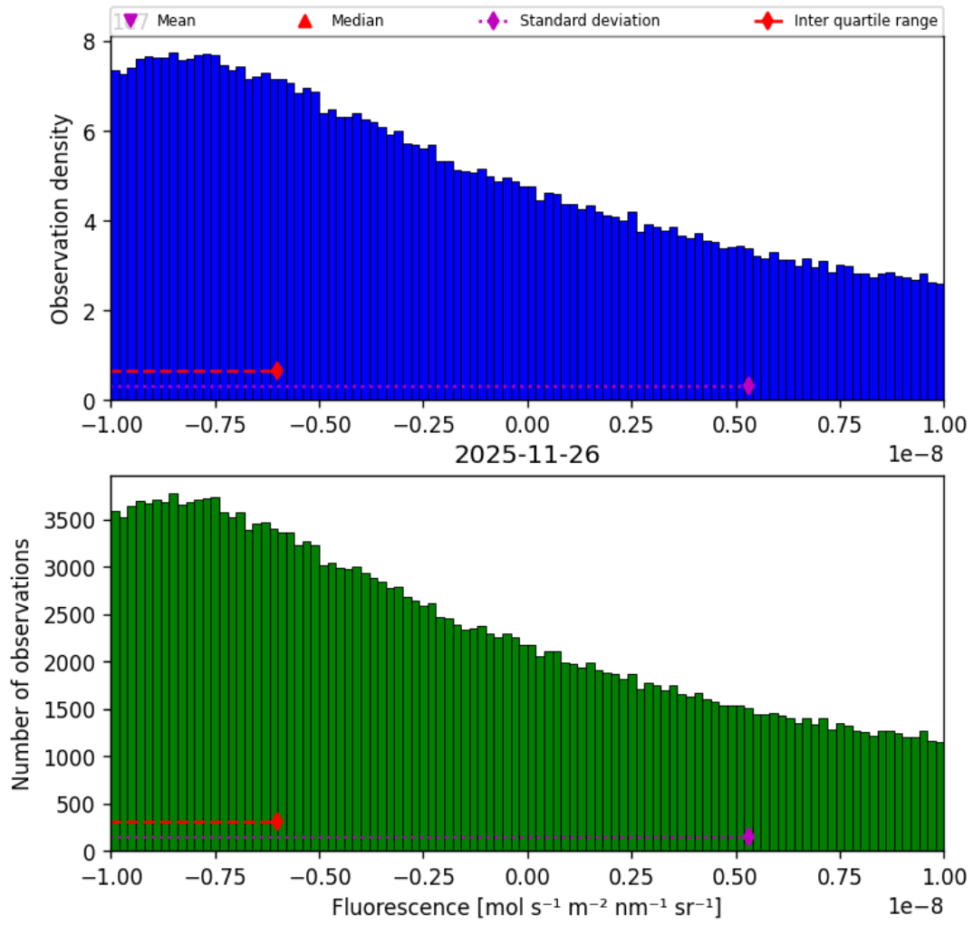
Figure 34: Histogram of “Fluorescence” for 2025-11-25 to 2025-11-27
