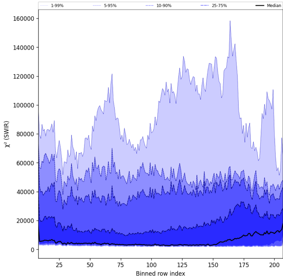
Figure 42: Along track statistics of “ \chi^2 (SWIR)” for 2025-11-25 to 2025-11-27
