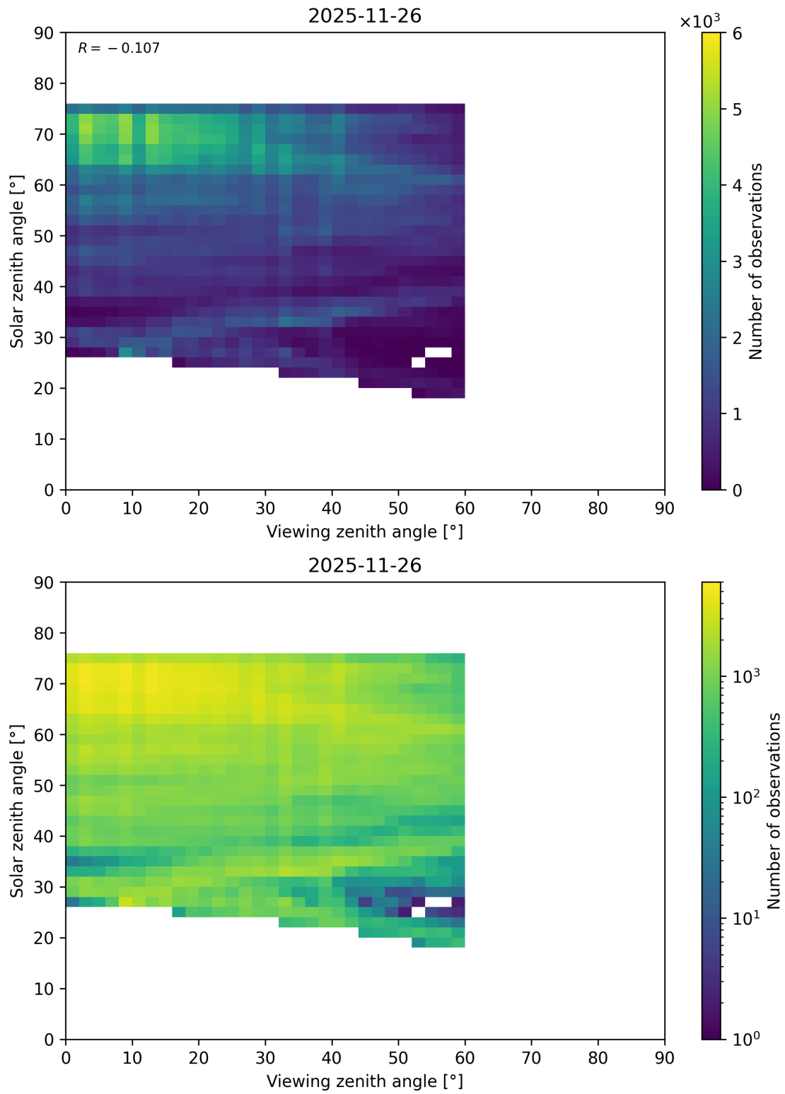
Figure 131: Scatter density plot of “Viewing zenith angle” against “Solar zenith angle” for 2025-11-25 to 2025-11-27.
