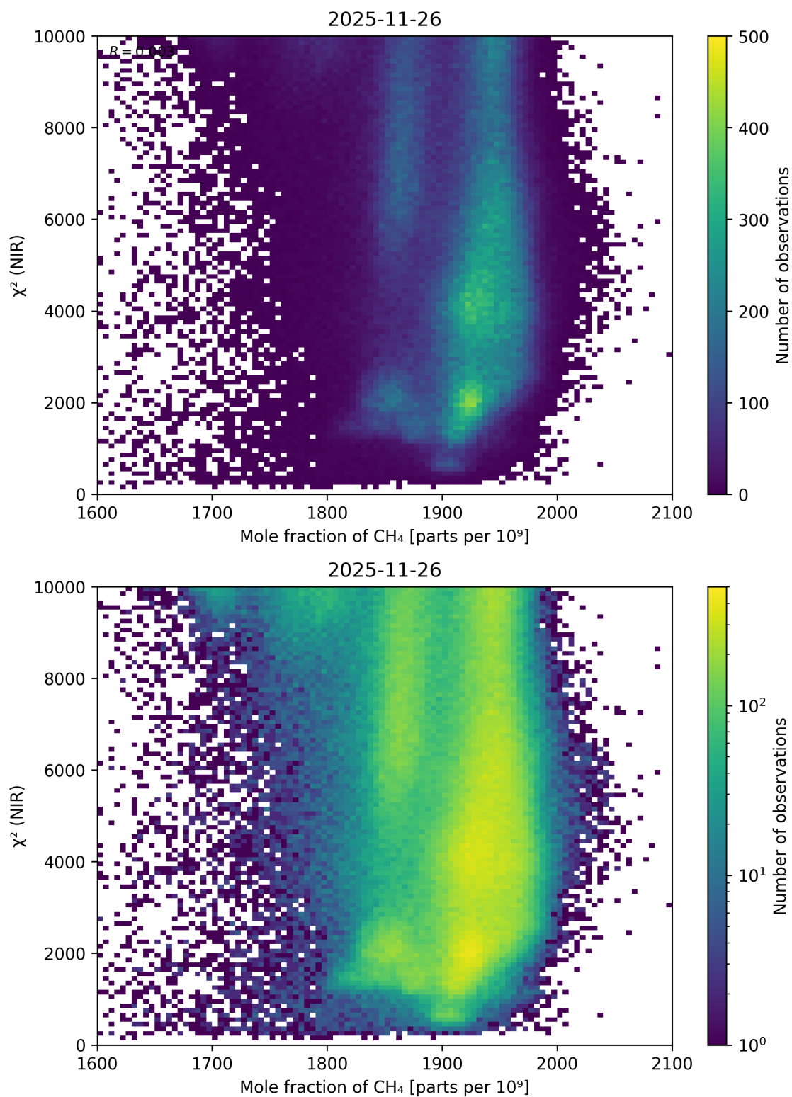
Figure 80: Scatter density plot of “Mole fraction of CH 4 ” against “ \chi^2 (NIR)” for 2025-11-25 to 2025-11-27.
