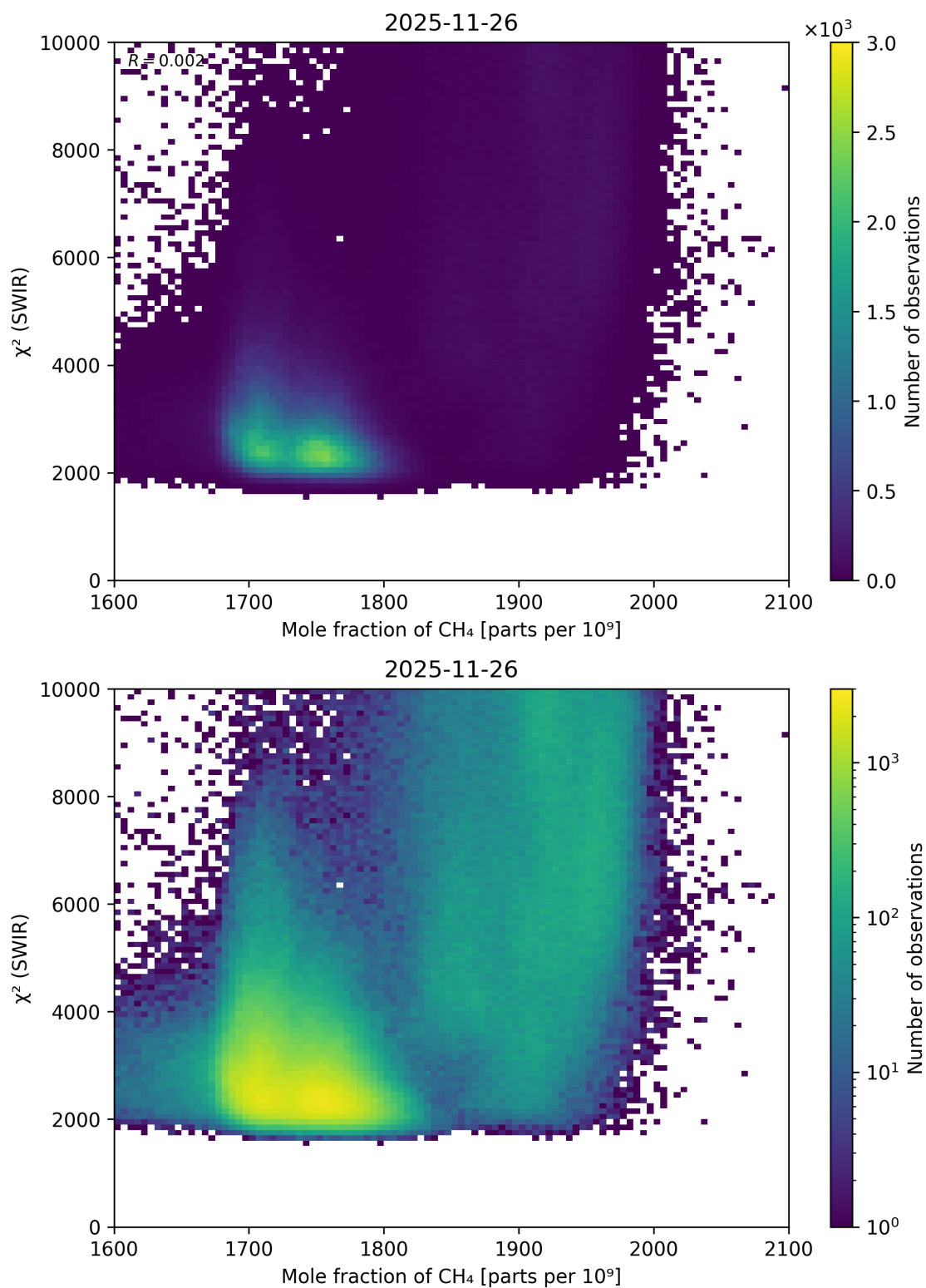
Figure 81: Scatter density plot of “Mole fraction of \text{CH}_4 ” against “ \chi^2 (SWIR)” for 2025-11-25 to 2025-11-27.
