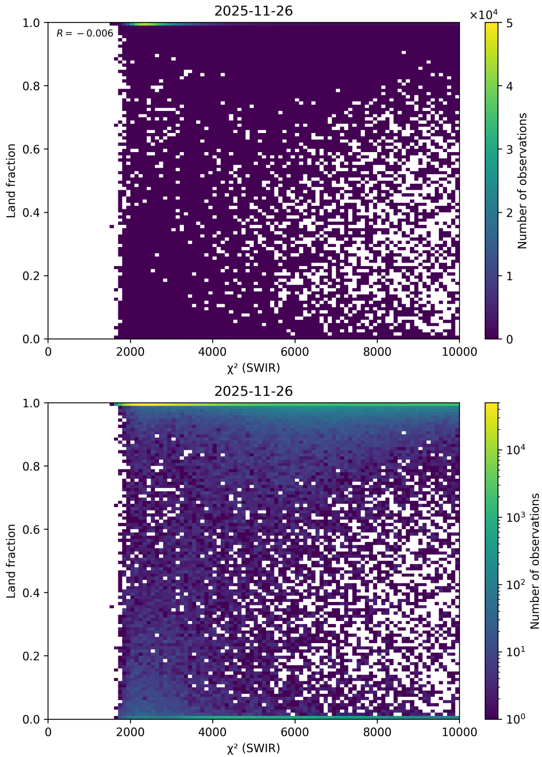
Figure 55: Scatter density plot of “ \chi^2 (SWIR)” against “Land fraction” for 2025-11-25 to 2025-11-27.
