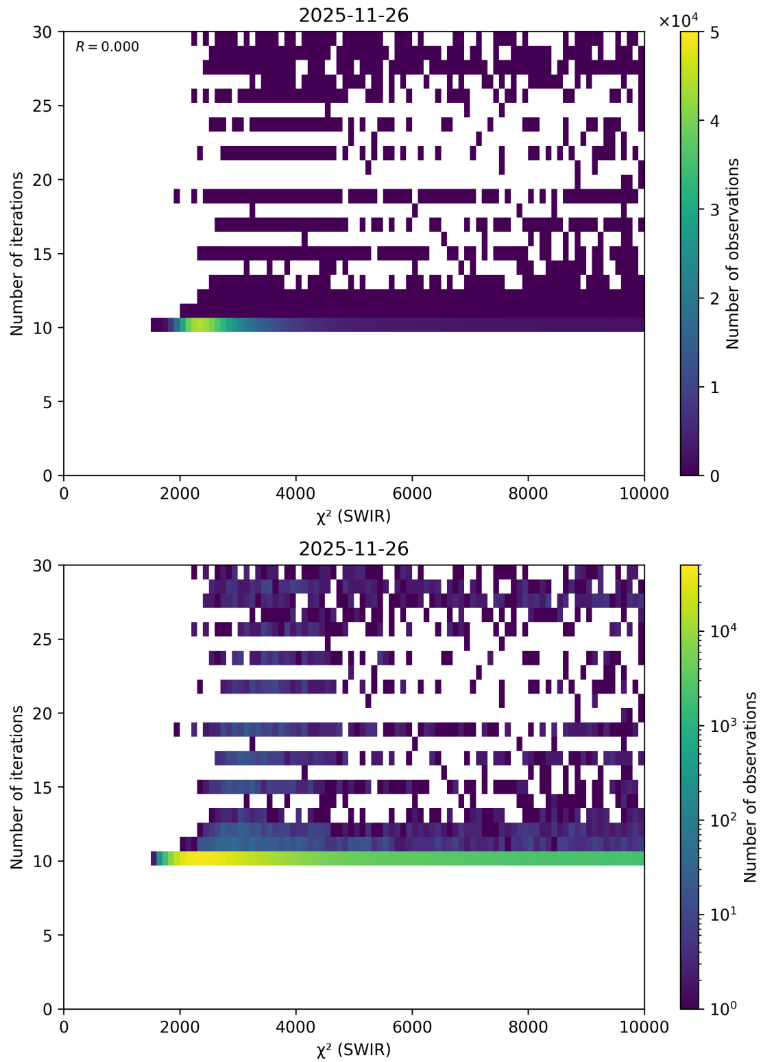
Figure 56: Scatter density plot of “ \chi^2 (SWIR)” against “Number of iterations” for 2025-11-25 to 2025-11-27.
