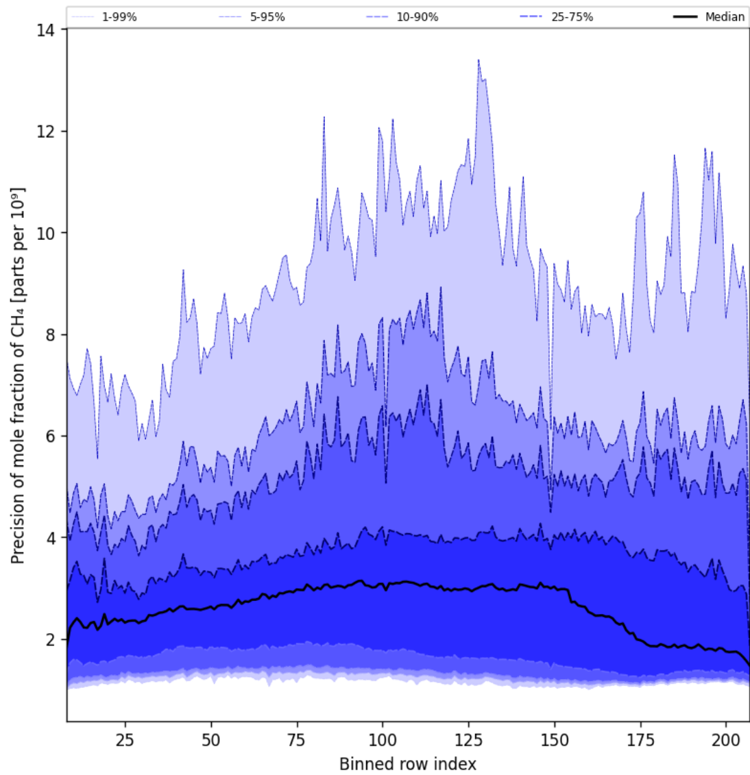
Figure 38: Along track statistics of “Precision of mole fraction of CH 4 ” for 2025-11-25 to 2025-11-27
