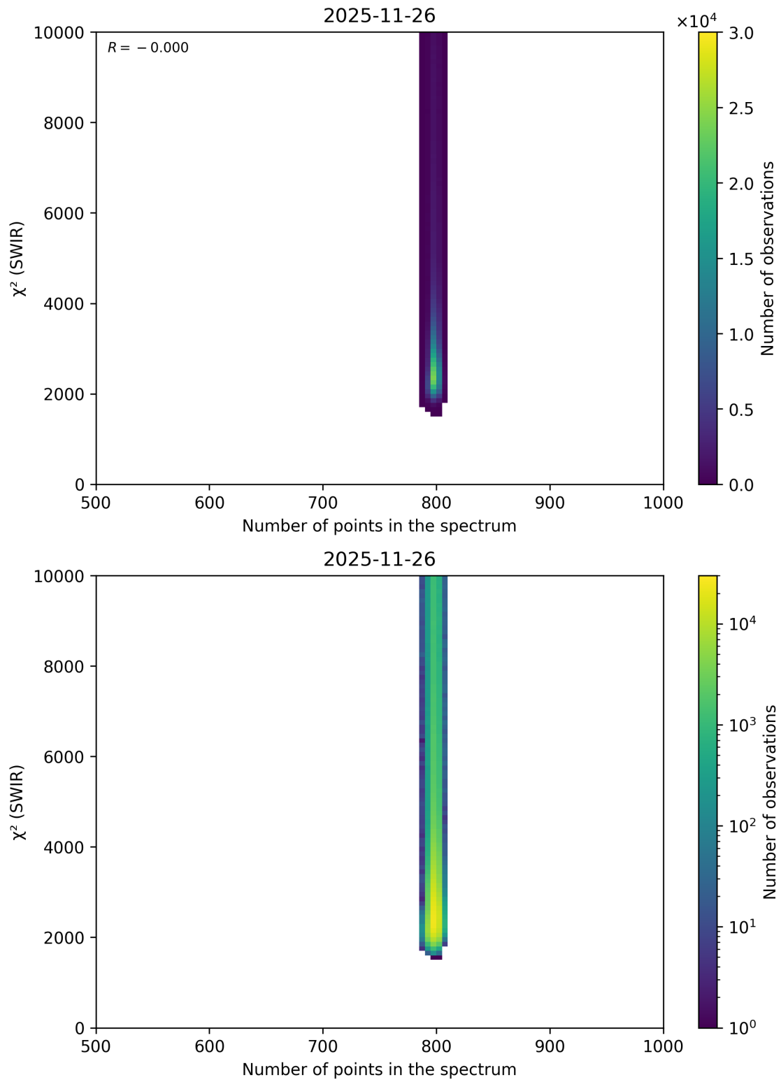
Figure 102: Scatter density plot of “Number of points in the spectrum” against “ \chi^2 (SWIR)” for 2025-11-25 to 2025-11-27.
