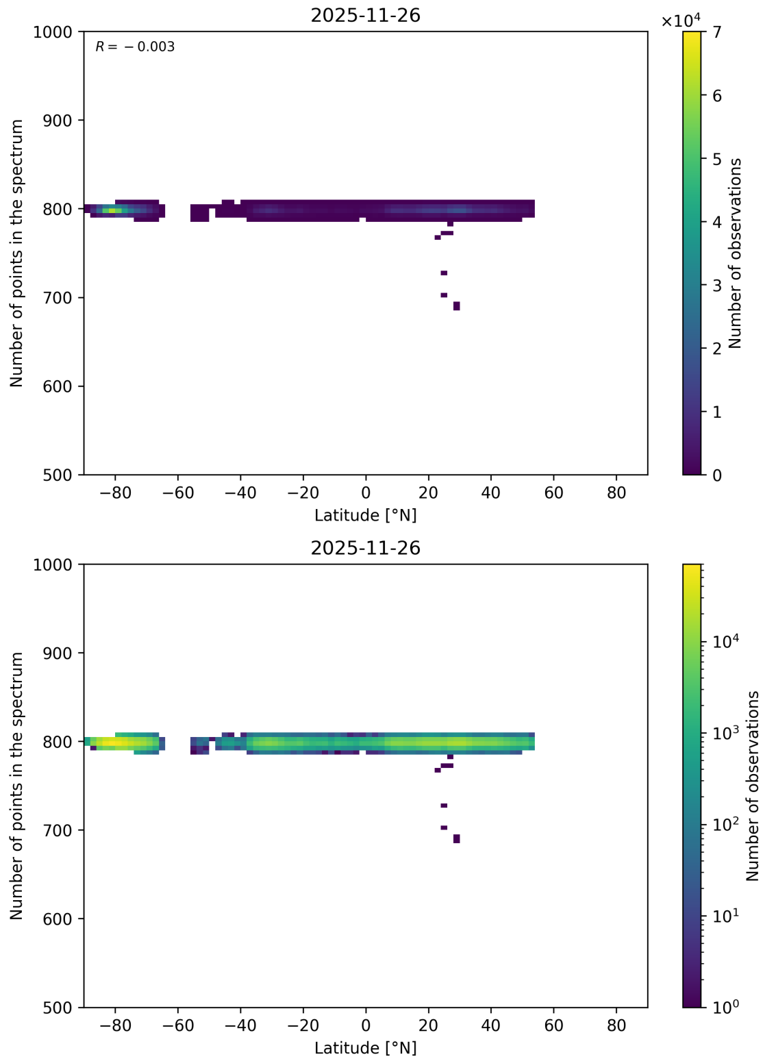
Figure 70: Scatter density plot of “Latitude” against “Number of points in the spectrum” for 2025-11-25 to 2025-11-27.
