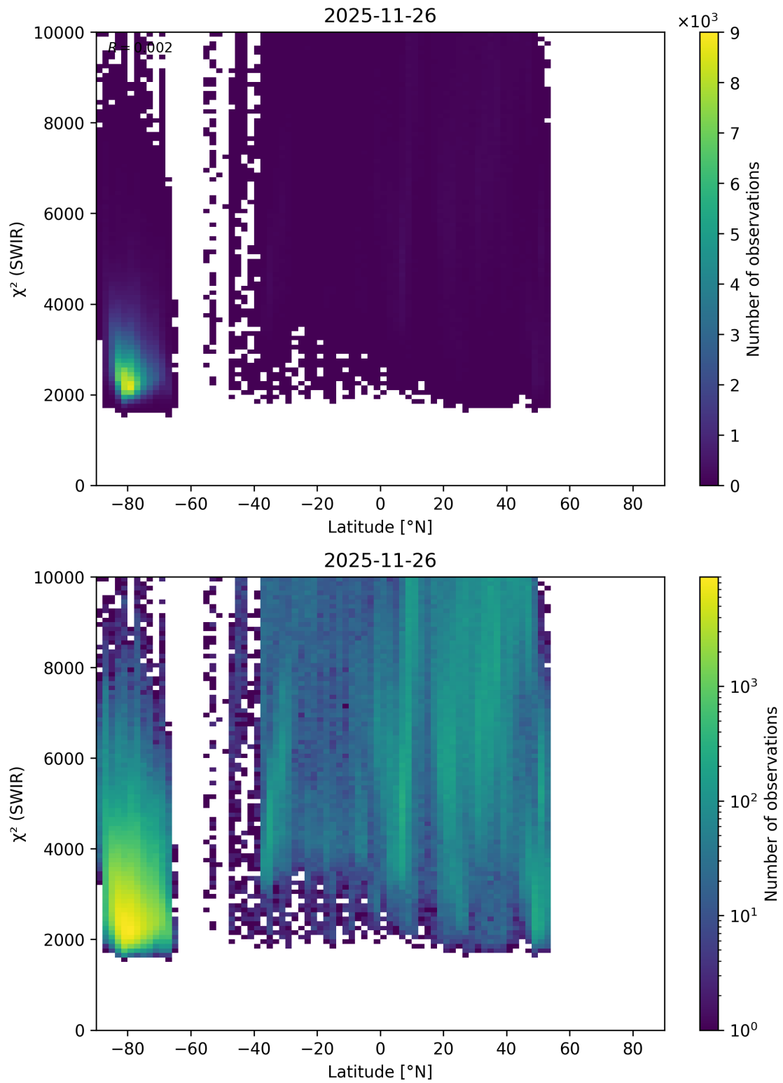
Figure 62: Scatter density plot of “Latitude” against “ \chi^2 (SWIR)” for 2025-11-25 to 2025-11-27.
