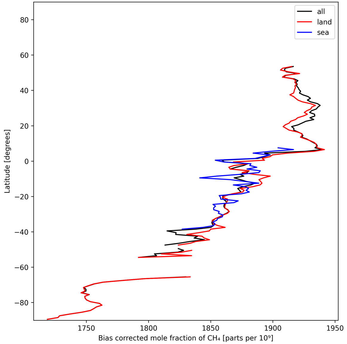
Figure 15: Zonal average of “Bias corrected mole fraction of CH 4 ” for 2025-11-25 to 2025-11-27.
