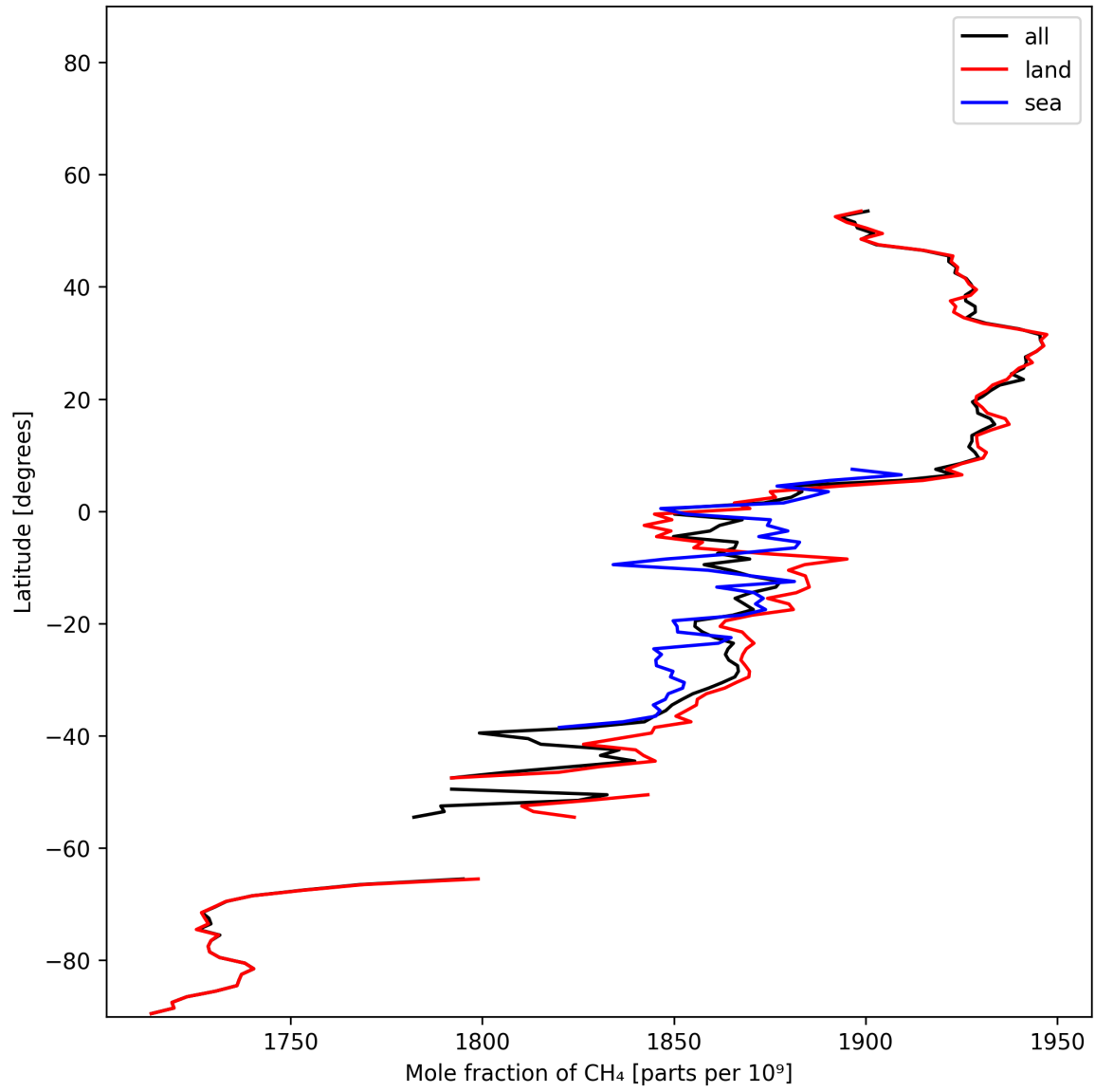
Figure 13: Zonal average of “Mole fraction of \text{CH}_4 ” for 2025-11-25 to 2025-11-27.
