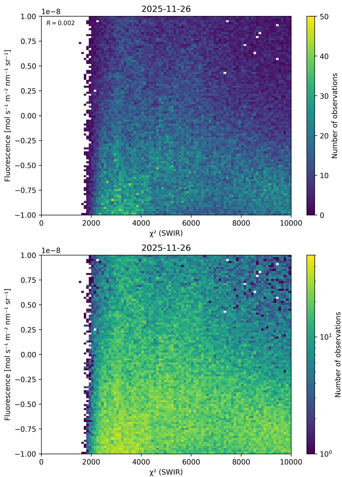
Figure 54: Scatter density plot of “ \chi^2 (SWIR)” against “Fluorescence” for 2025-11-25 to 2025-11-27.
