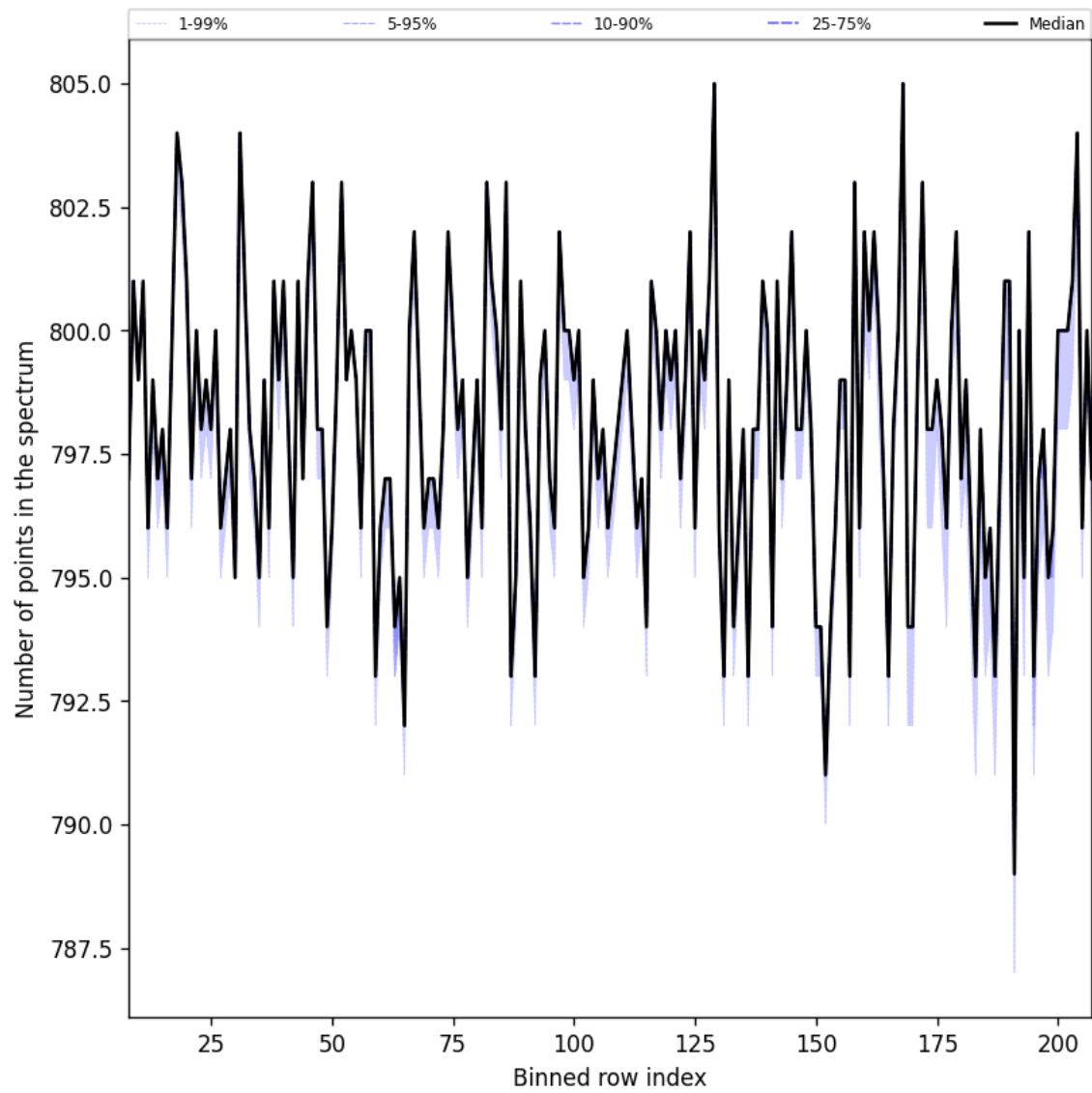
Figure 40: Along track statistics of “Number of points in the spectrum” for 2025-11-25 to 2025-11-27
