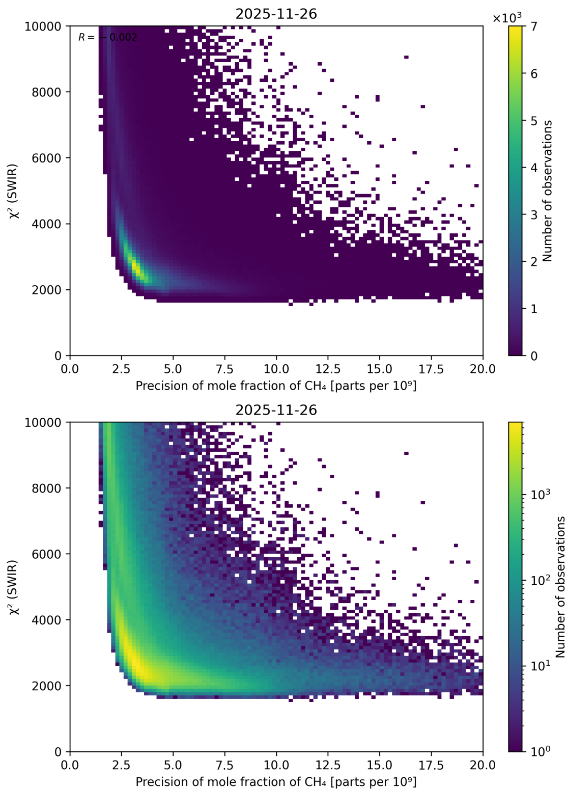
Figure 90: Scatter density plot of “Precision of mole fraction of \text{CH}_4 ” against “ \chi^2 (SWIR)” for 2025-11-25 to 2025-11-27.
