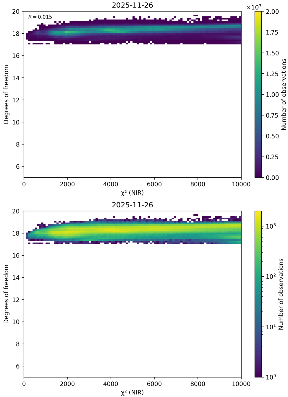
Figure 48: Scatter density plot of “ \chi^2 (NIR)” against “Degrees of freedom” for 2025-11-25 to 2025-11-27.
