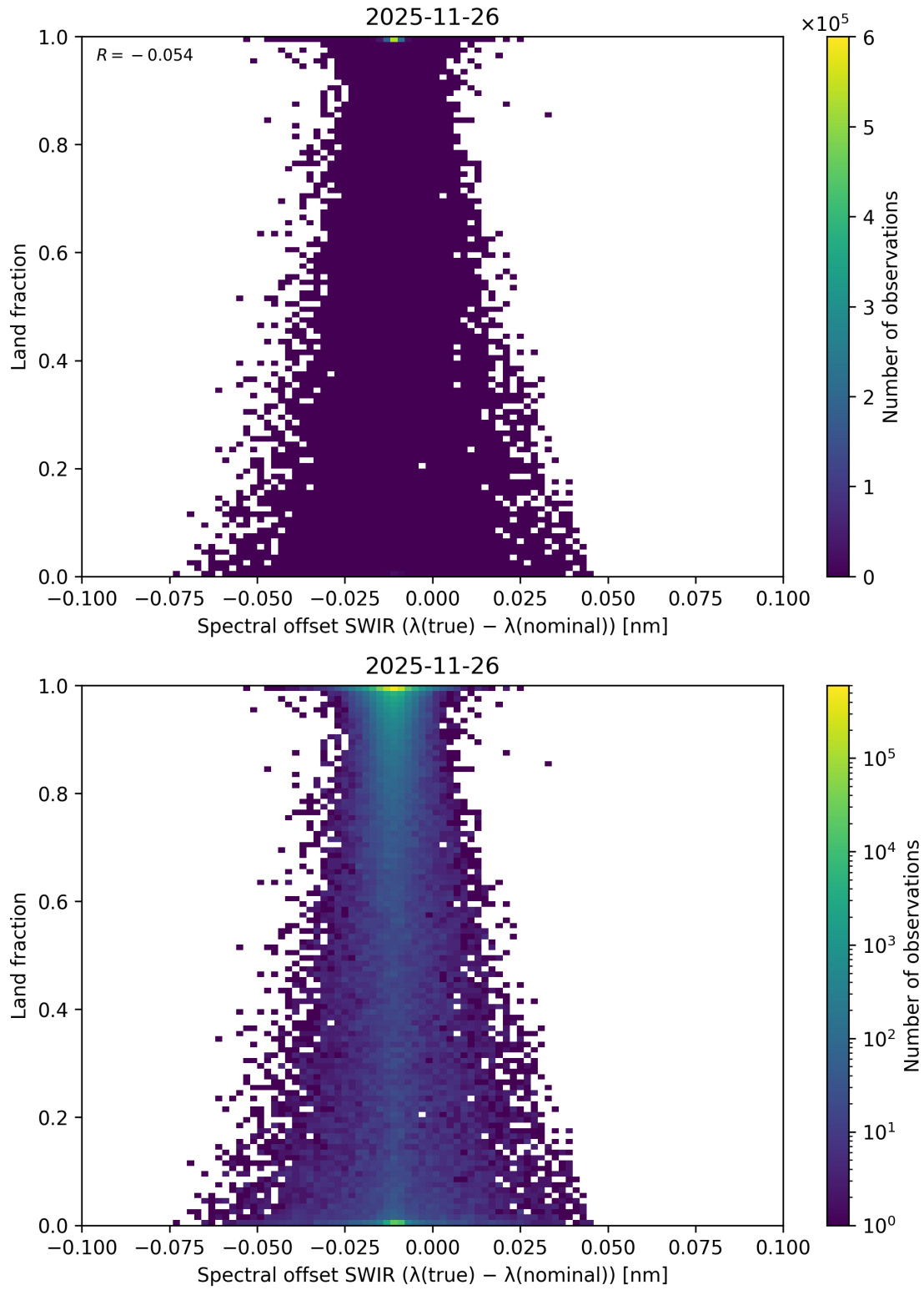
Figure 137: Scatter density plot of “Spectral offset SWIR ( \lambda_{\text{true}} - \lambda_{\text{nominal}} )” against “Land fraction” for 2025-11-25 to 2025-11-27.
