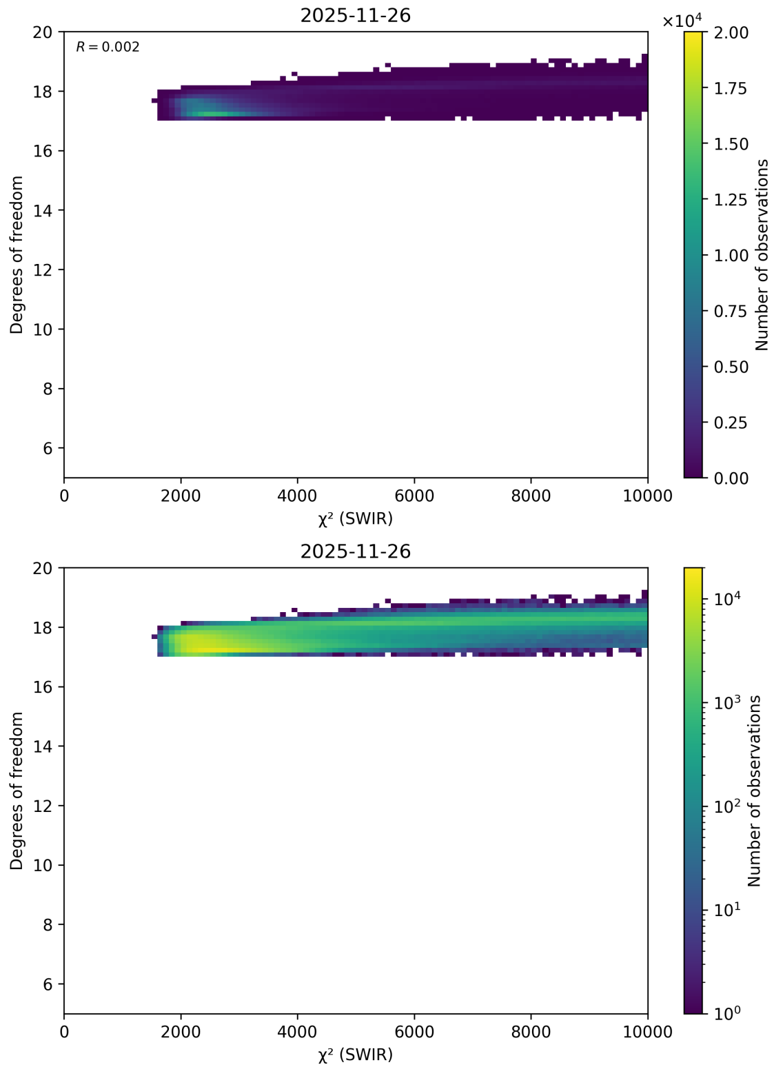
Figure 53: Scatter density plot of “ \chi^2 (SWIR)” against “Degrees of freedom” for 2025-11-25 to 2025-11-27.
