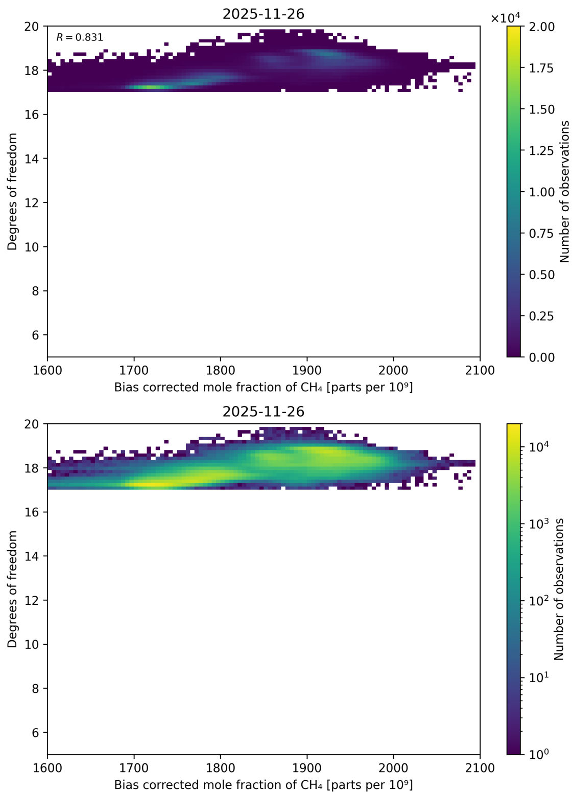
Figure 74: Scatter density plot of “Bias corrected mole fraction of CH 4 ” against “Degrees of freedom” for 2025-11-25 to 2025-11-27.
