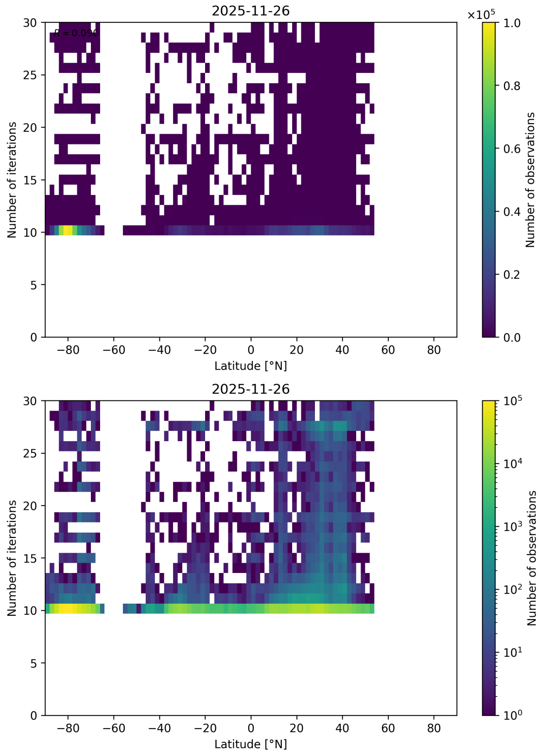
Figure 69: Scatter density plot of “Latitude” against “Number of iterations” for 2025-11-25 to 2025-11-27.
