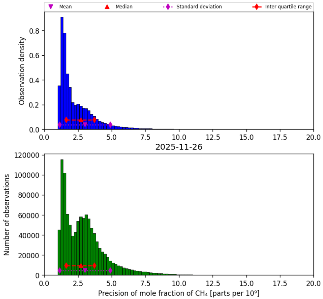
Figure 26: Histogram of “Precision of mole fraction of CH 4 ” for 2025-11-25 to 2025-11-27
