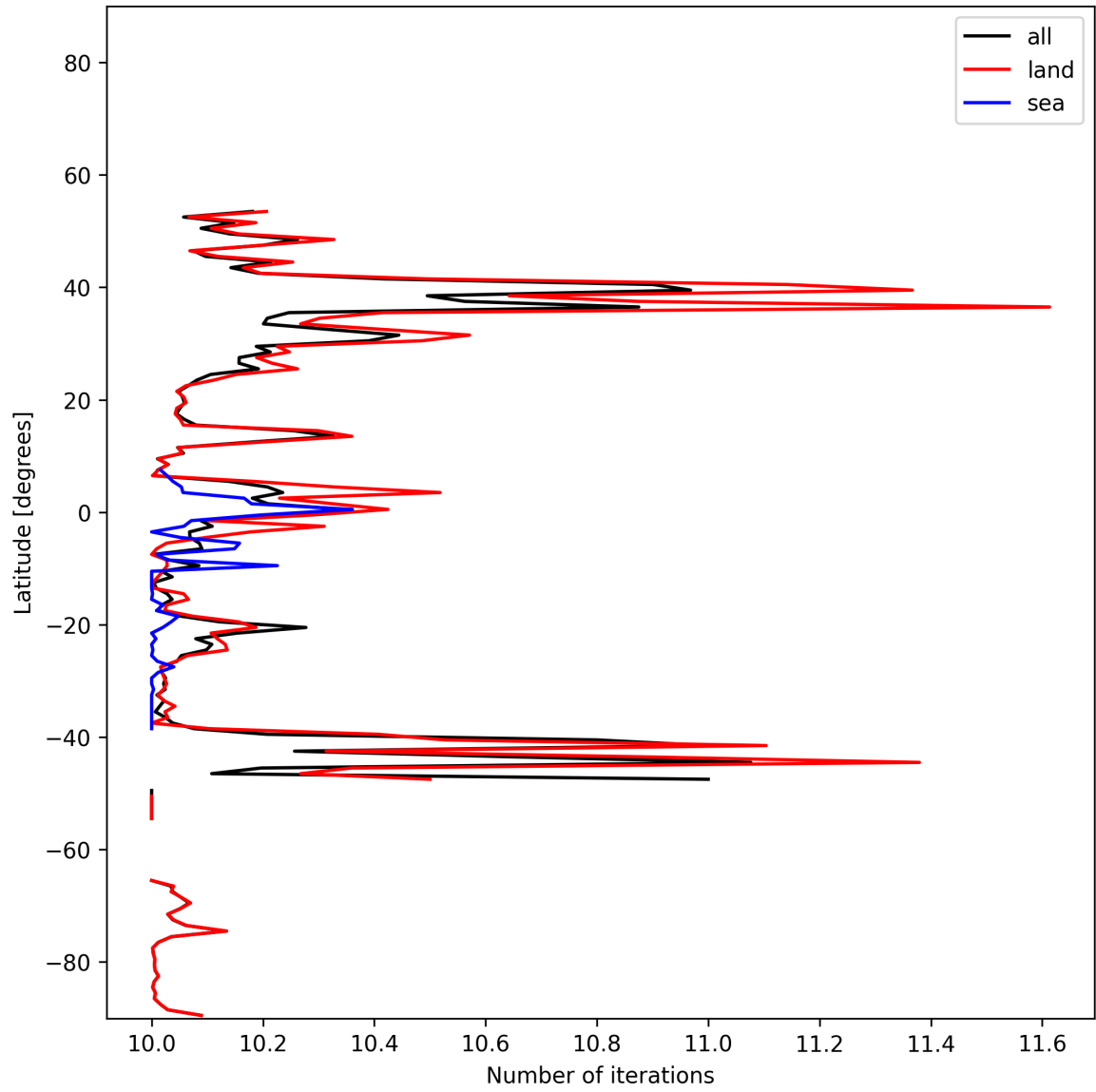
Figure 21: Zonal average of “Number of iterations” for 2025-11-25 to 2025-11-27.
