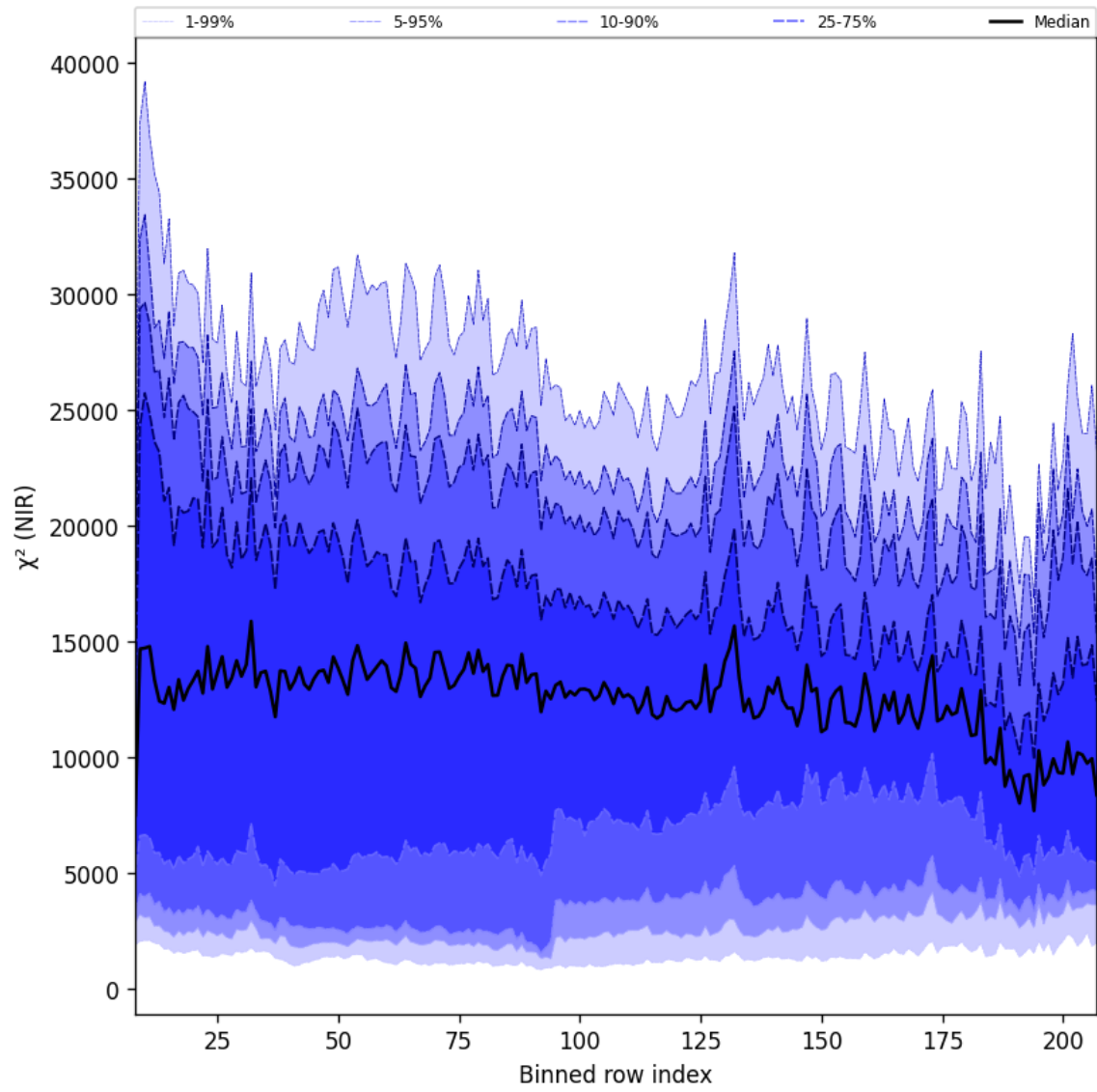
Figure 43: Along track statistics of “ \chi^2 (NIR)” for 2025-11-25 to 2025-11-27
