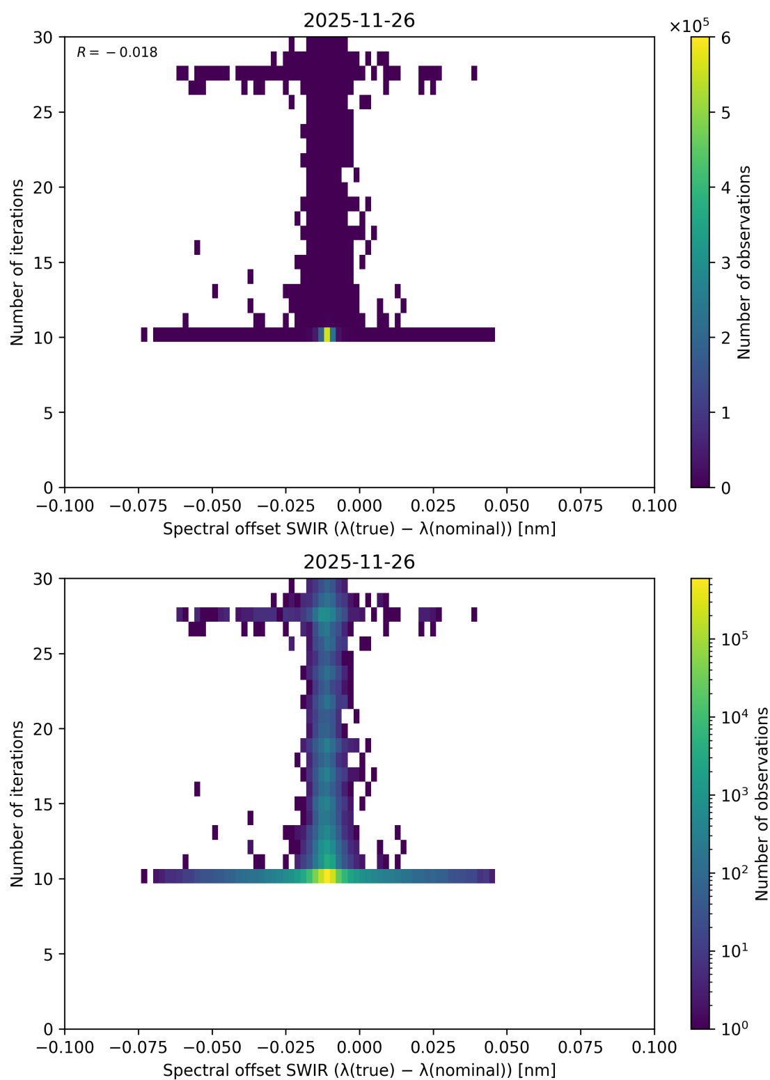
Figure 138: Scatter density plot of “Spectral offset SWIR ( \lambda_{\text{true}} - \lambda_{\text{nominal}} )” against “Number of iterations” for 2025-11-25 to 2025-11-27.
