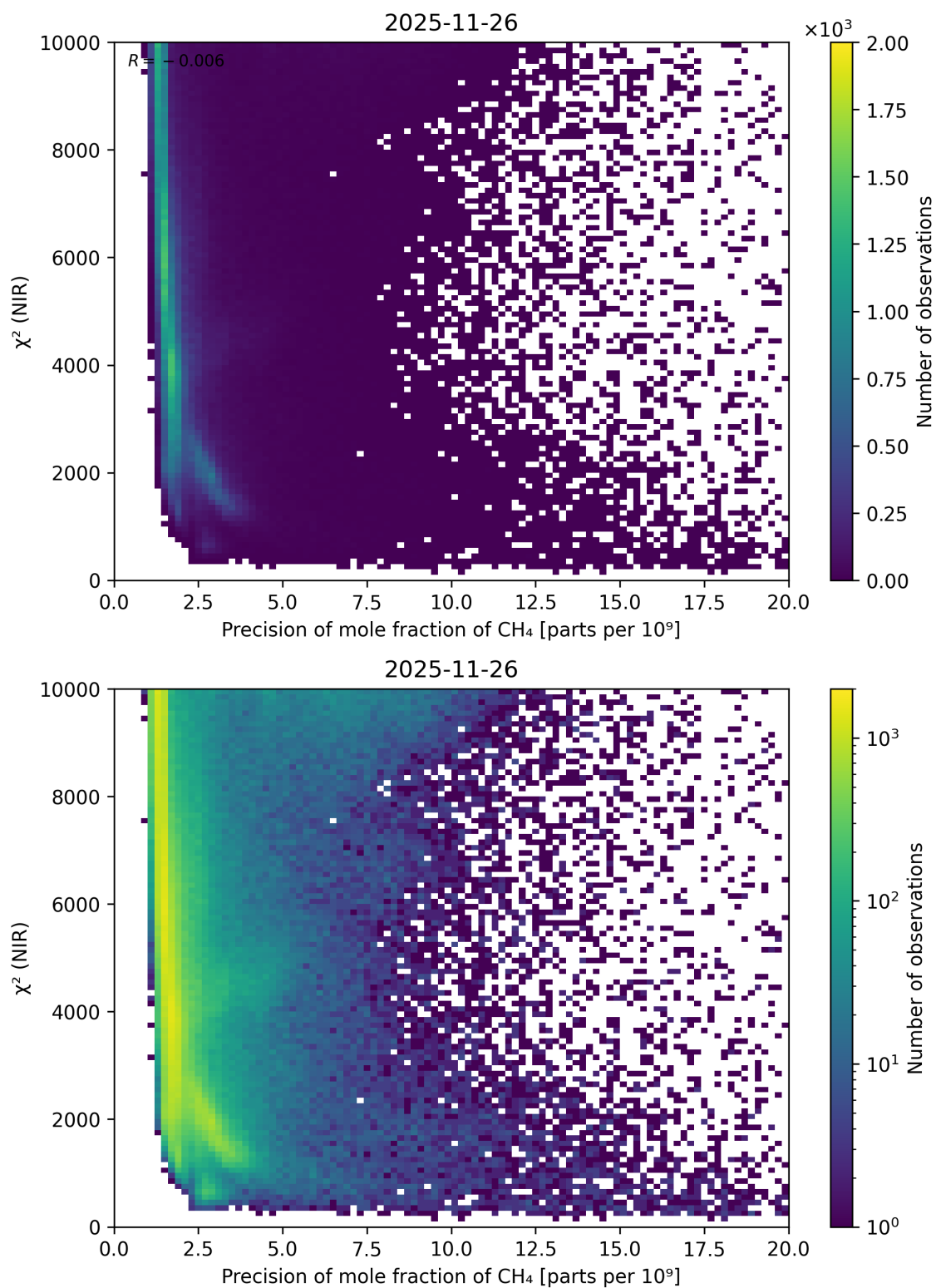
Figure 89: Scatter density plot of “Precision of mole fraction of CH 4 ” against “ \chi^2 (NIR)” for 2025-11-25 to 2025-11-27.
