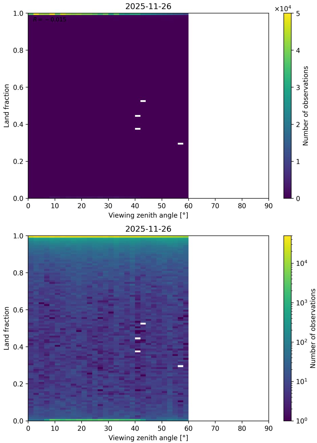
Figure 124: Scatter density plot of “Viewing zenith angle” against “Land fraction” for 2025-11-25 to 2025-11-27.
