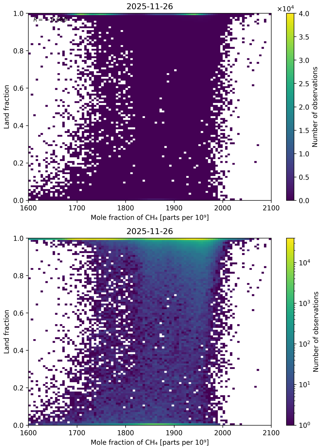
Figure 84: Scatter density plot of “Mole fraction of CH 4 ” against “Land fraction” for 2025-11-25 to 2025-11-27.
