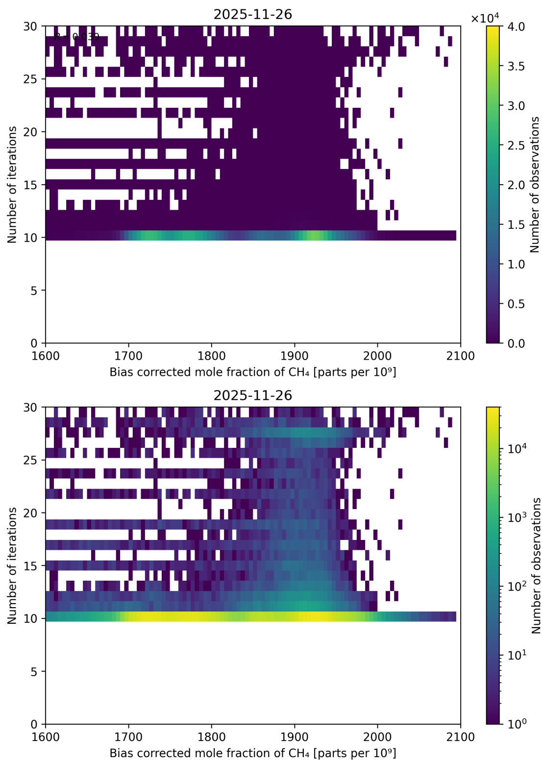
Figure 77: Scatter density plot of “Bias corrected mole fraction of \text{CH}_4 ” against “Number of iterations” for 2025-11-25 to 2025-11-27.
