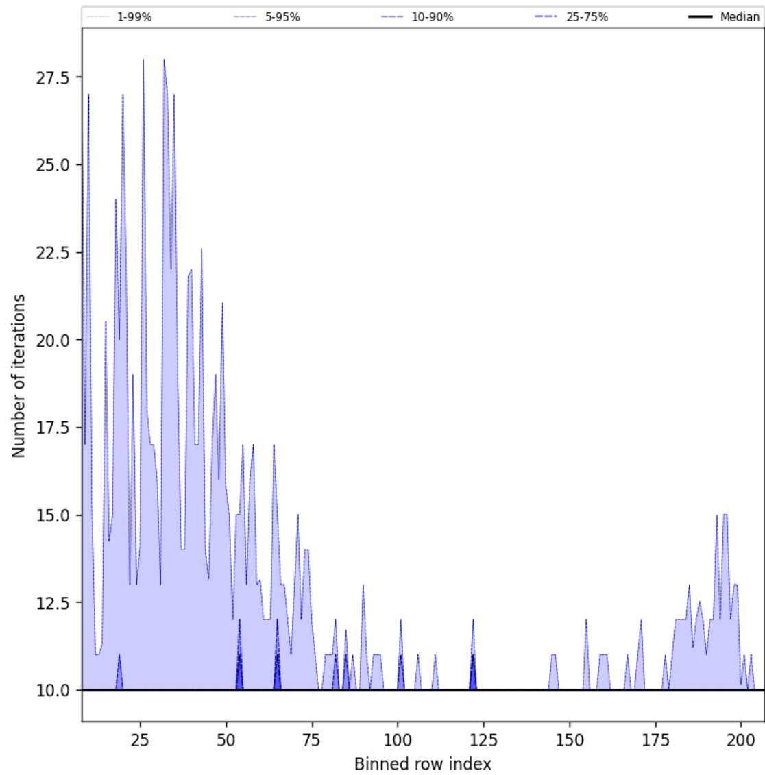
Figure 45: Along track statistics of “Number of iterations” for 2025-11-25 to 2025-11-27
