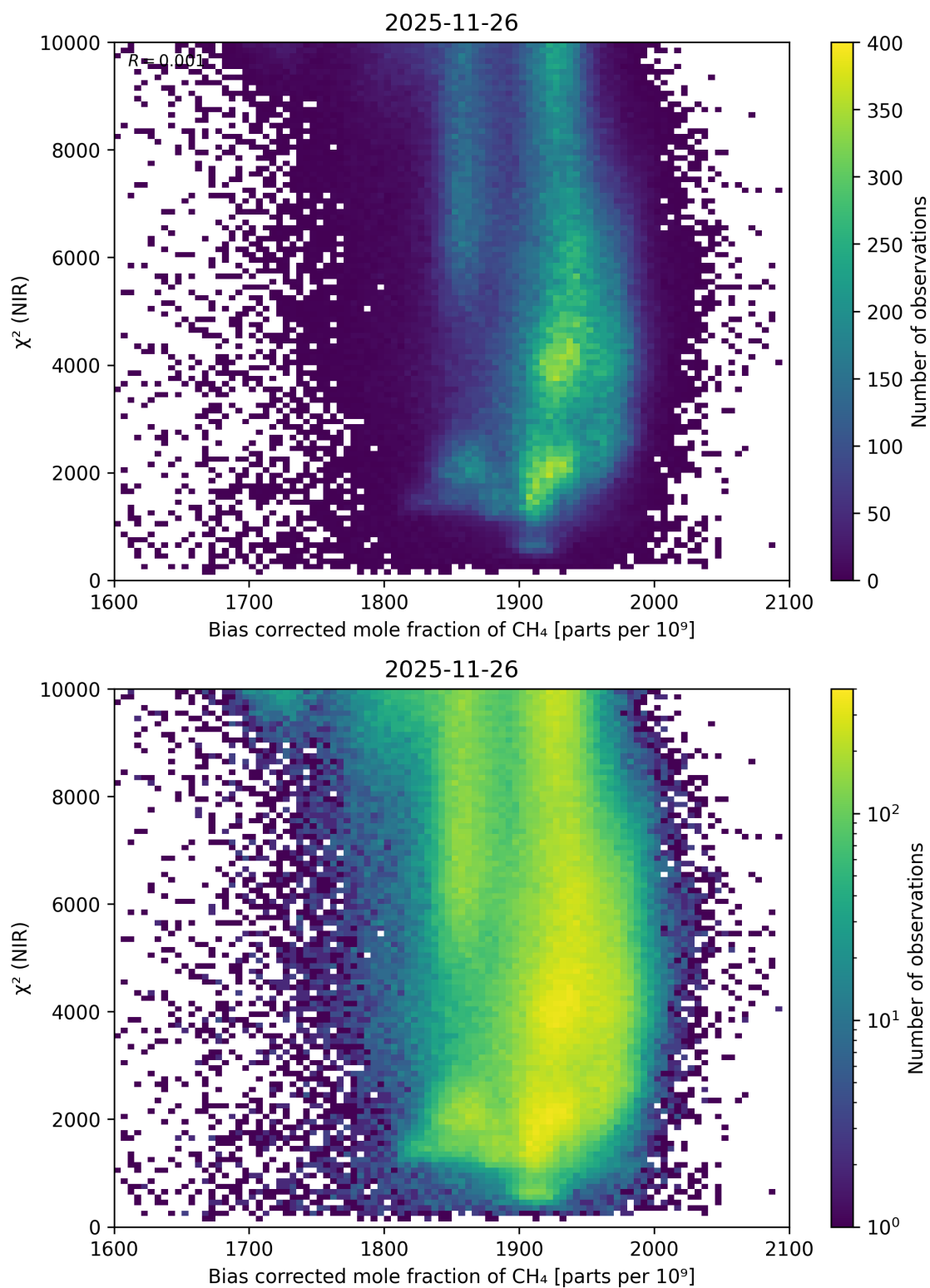
Figure 72: Scatter density plot of “Bias corrected mole fraction of CH 4 ” against “ \chi^2 (NIR)” for 2025-11-25 to 2025-11-27.
