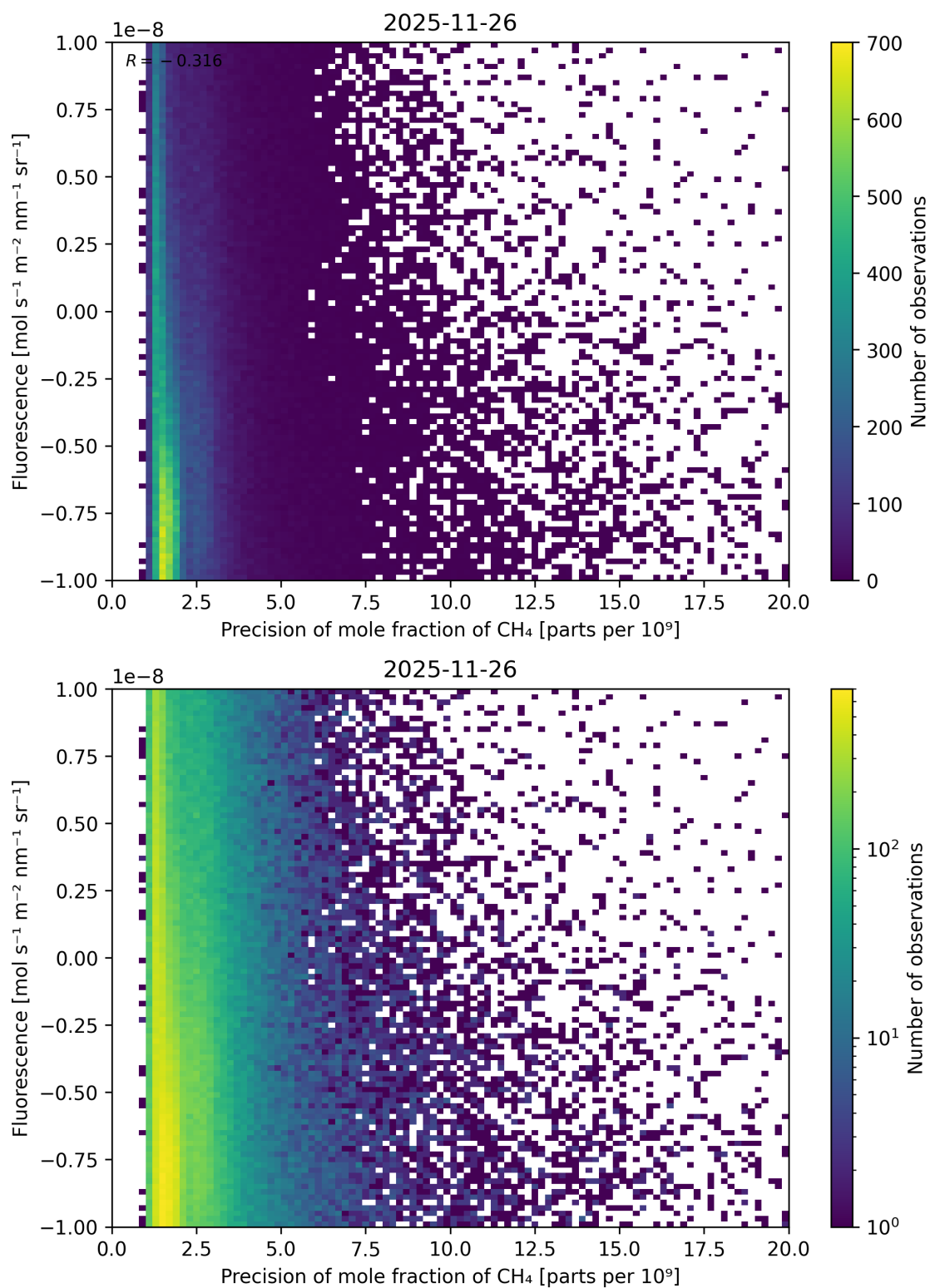
Figure 92: Scatter density plot of “Precision of mole fraction of \text{CH}_4 ” against “Fluorescence” for 2025-11-25 to 2025-11-27.
