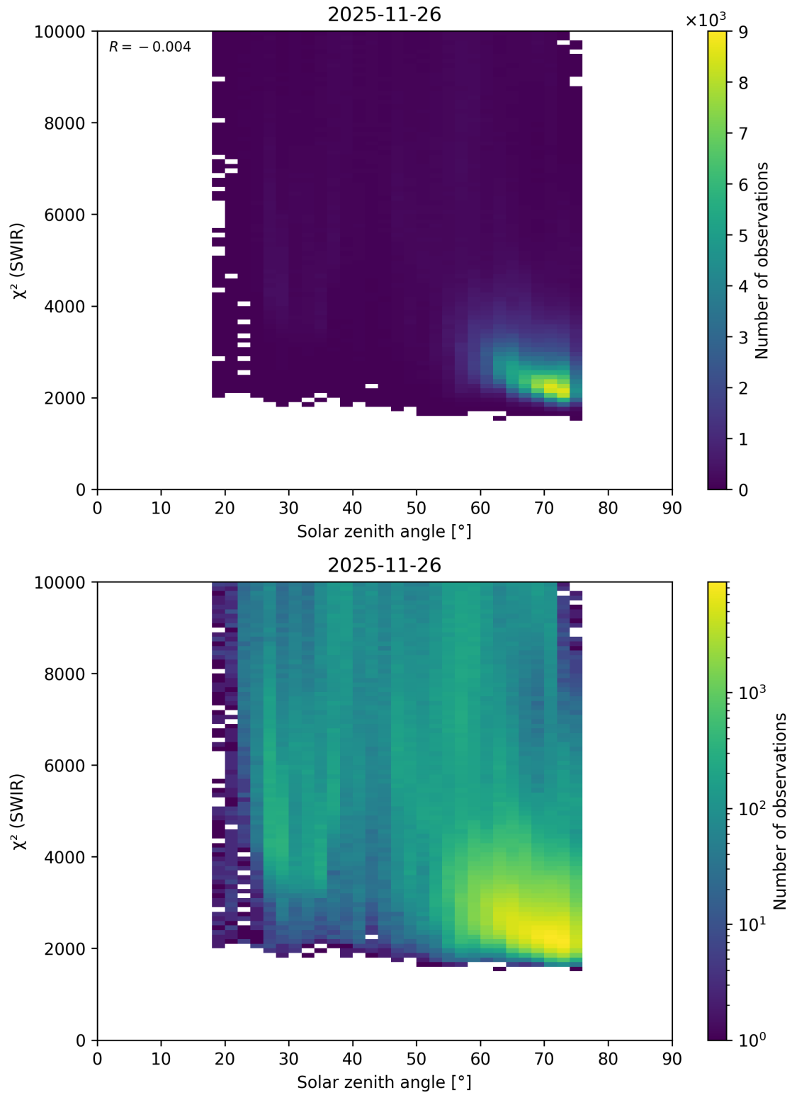
Figure 109: Scatter density plot of “Solar zenith angle” against “ \chi^2 (SWIR)” for 2025-11-25 to 2025-11-27.
