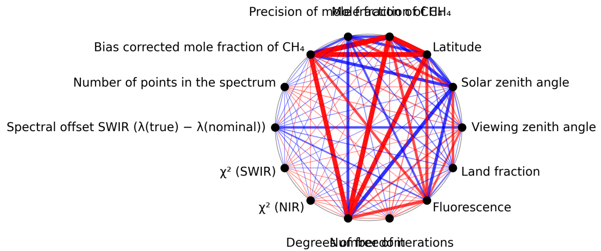
Figure 1: Map of correlation graph for 2025-11-25 to 2025-11-27.
