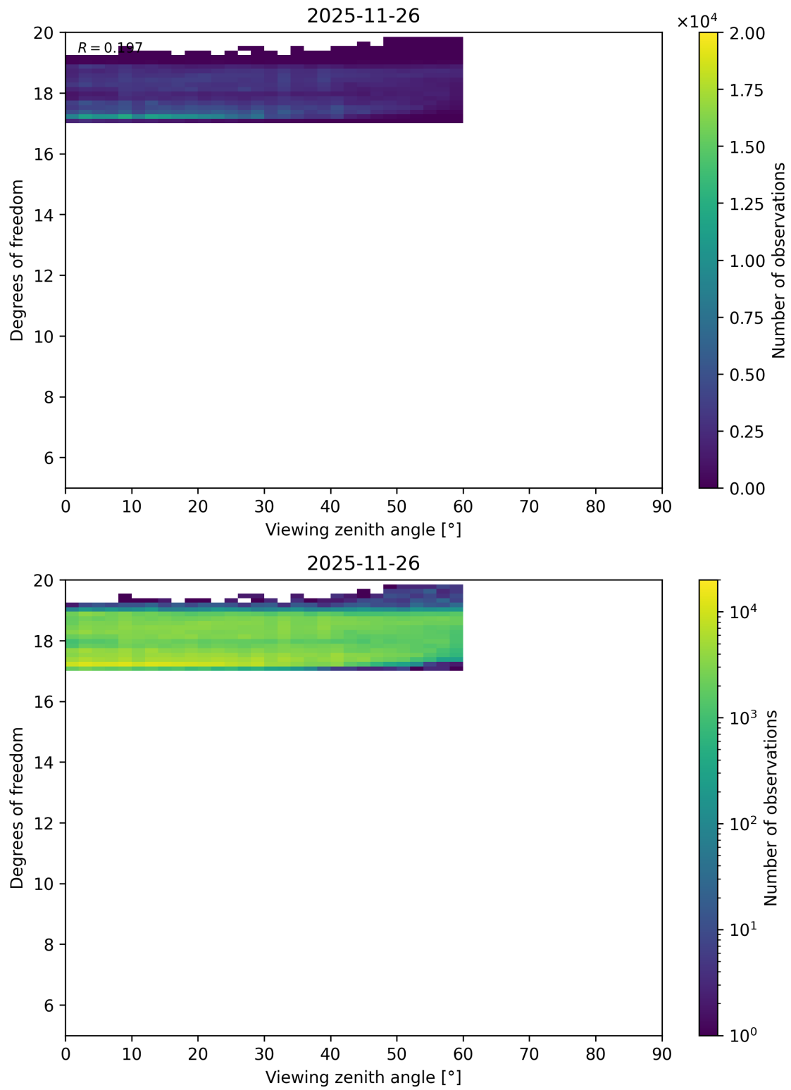
Figure 122: Scatter density plot of “Viewing zenith angle” against “Degrees of freedom” for 2025-11-25 to 2025-11-27.
