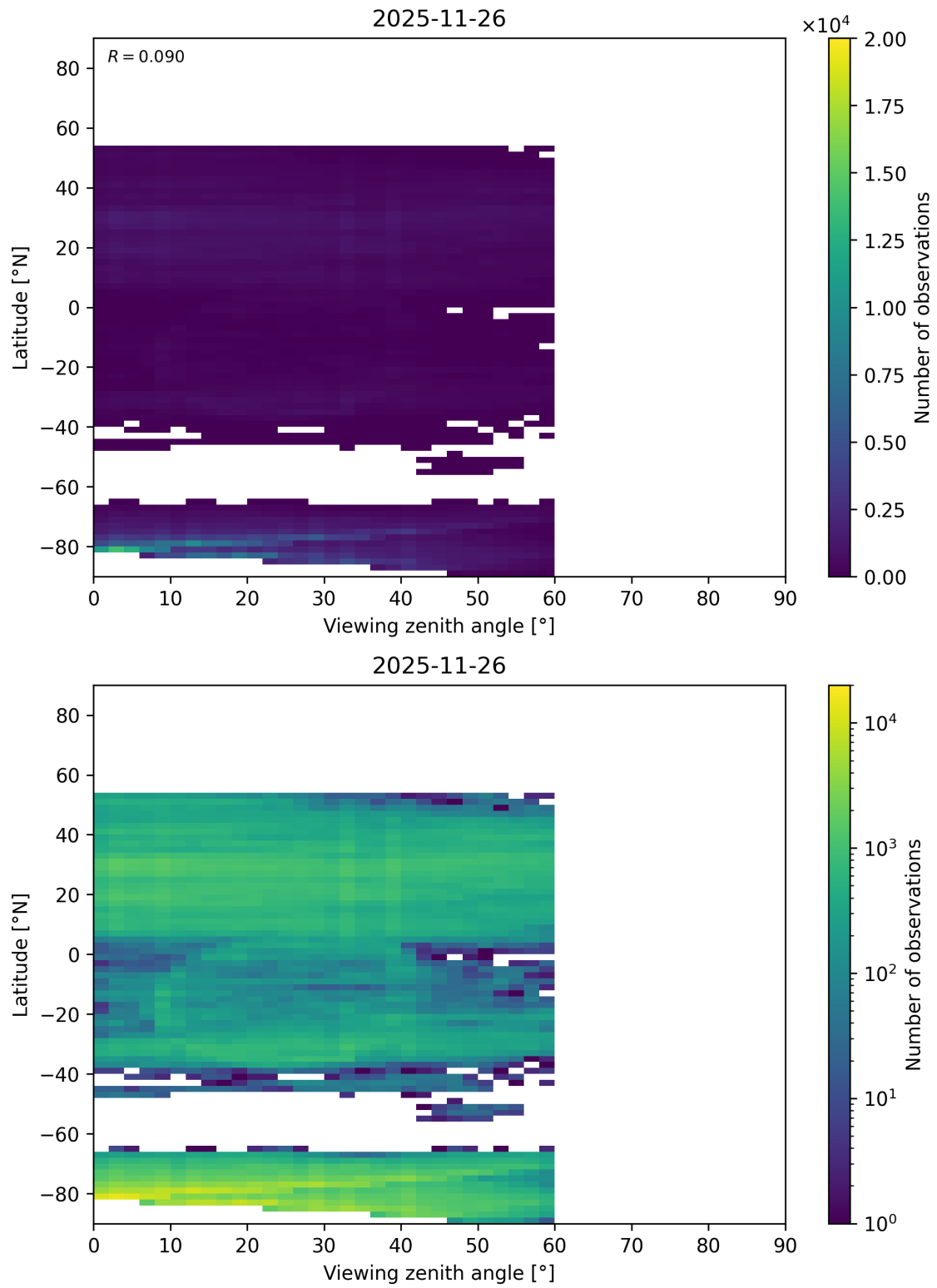
Figure 125: Scatter density plot of “Viewing zenith angle” against “Latitude” for 2025-11-25 to 2025-11-27.
