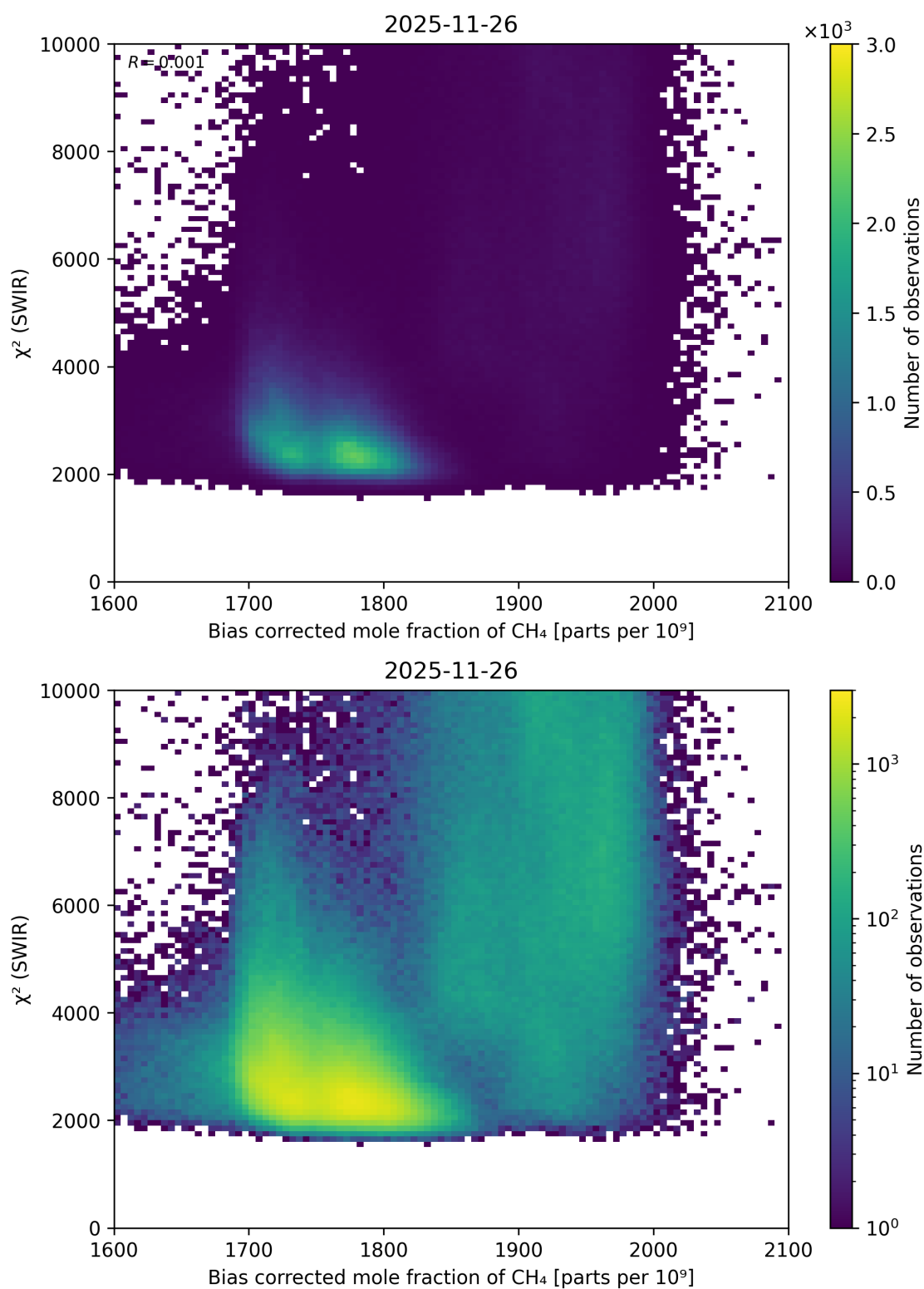
Figure 73: Scatter density plot of “Bias corrected mole fraction of \text{CH}_4 ” against “ \chi^2 (SWIR)” for 2025-11-25 to 2025-11-27.
