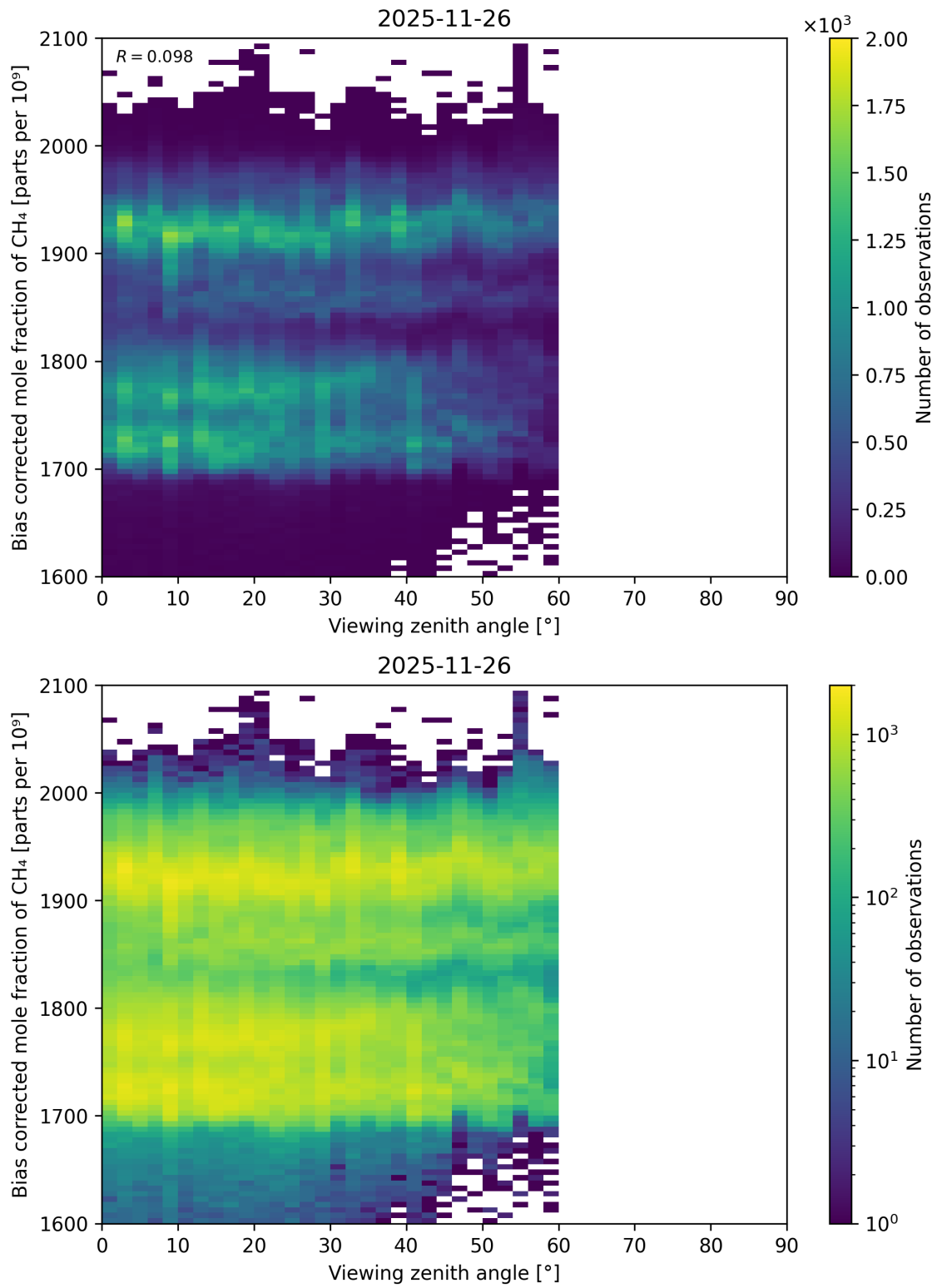
Figure 127: Scatter density plot of “Viewing zenith angle” against “Bias corrected mole fraction of CH 4 ” for 2025-11-25 to 2025-11-27.
