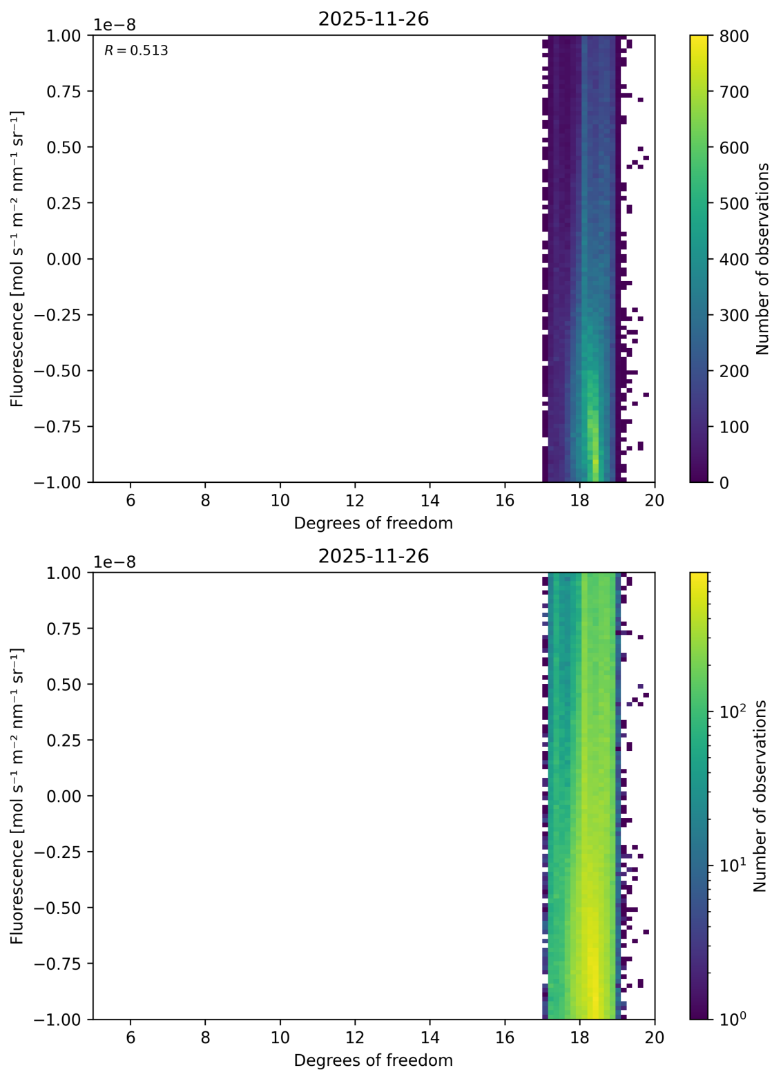
Figure 57: Scatter density plot of “Degrees of freedom” against “Fluorescence” for 2025-11-25 to 2025-11-27.
