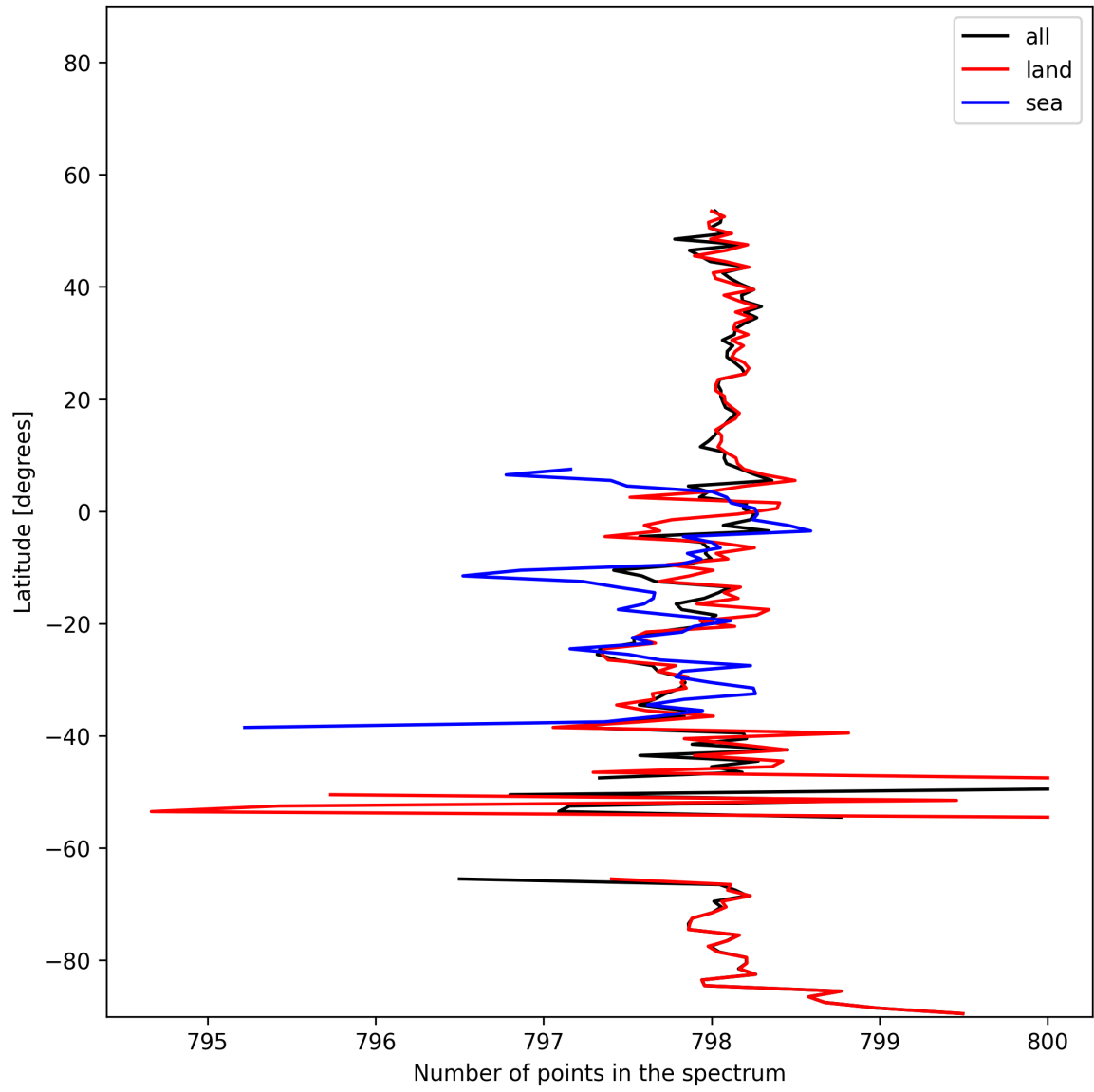
Figure 16: Zonal average of “Number of points in the spectrum” for 2025-11-25 to 2025-11-27.
