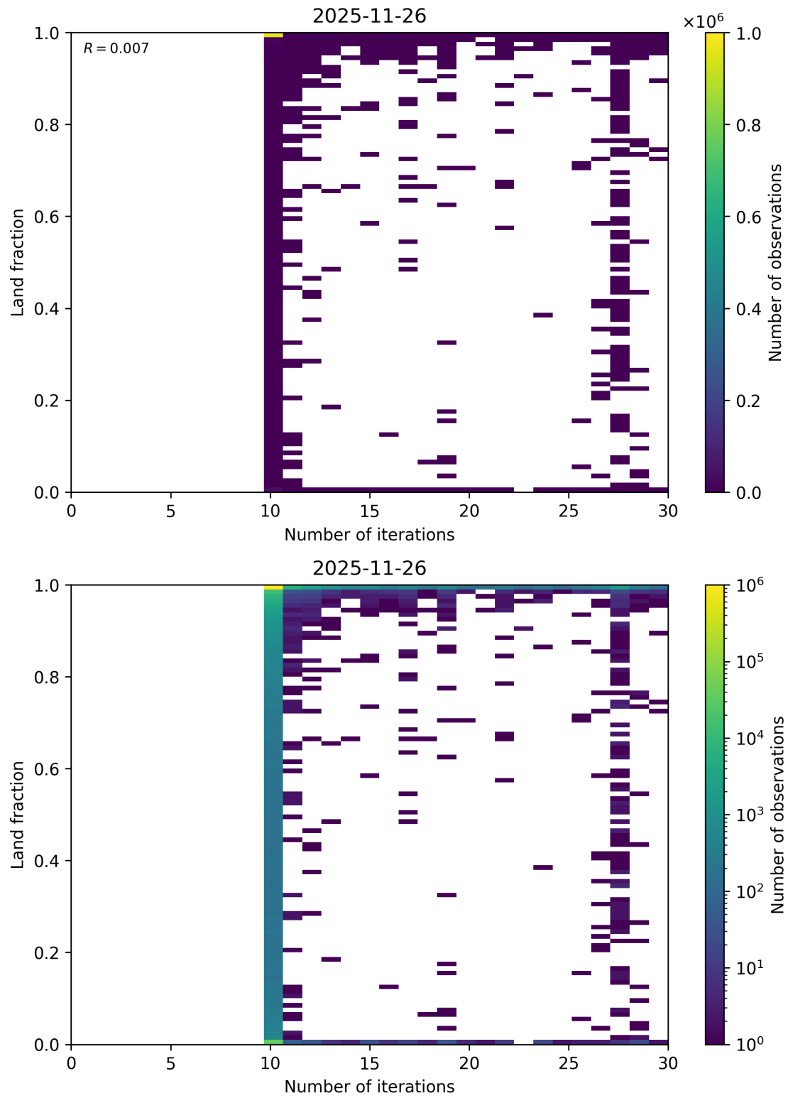
Figure 100: Scatter density plot of “Number of iterations” against “Land fraction” for 2025-11-25 to 2025-11-27.
