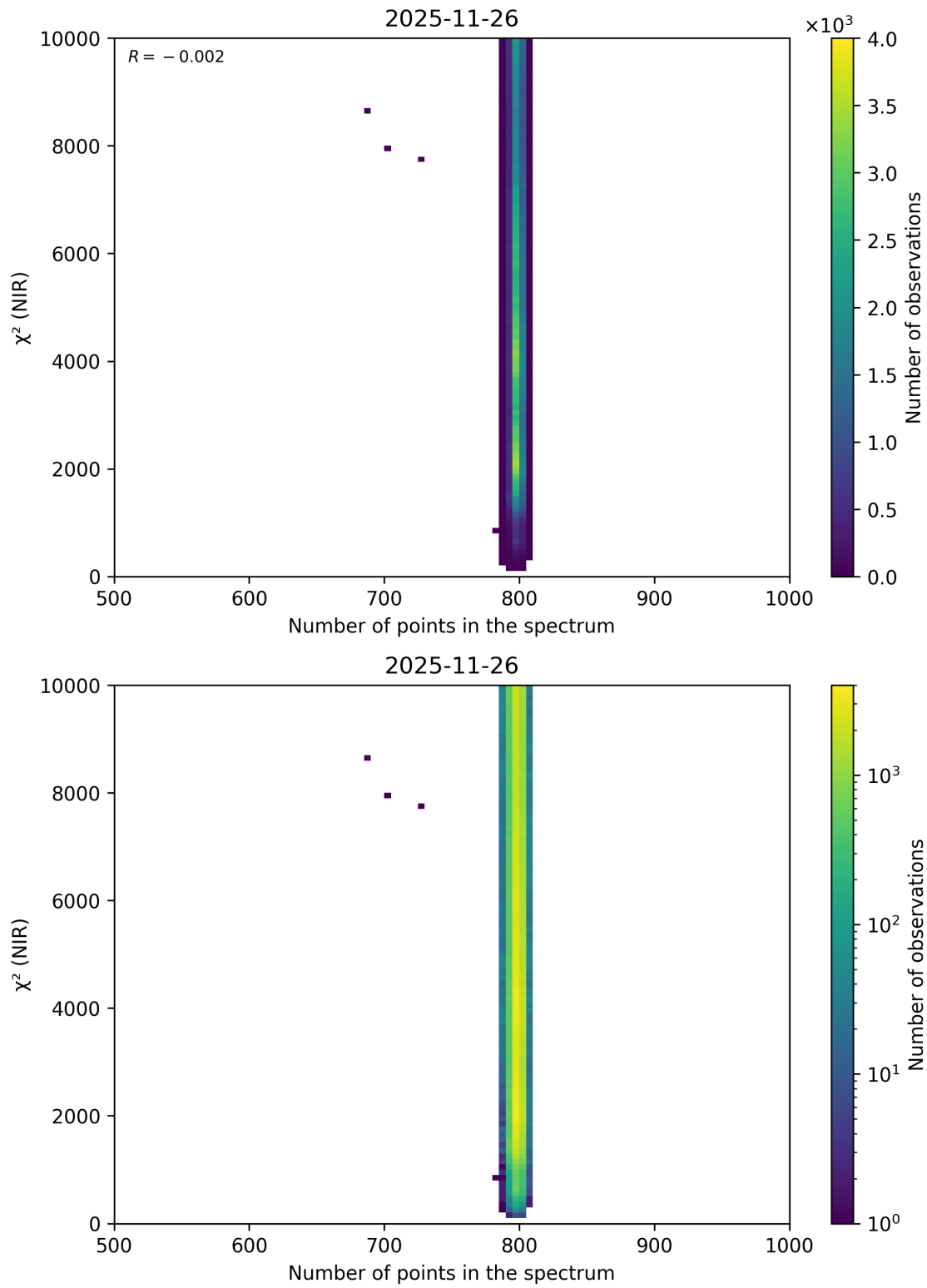
Figure 101: Scatter density plot of “Number of points in the spectrum” against “ \chi^2 (NIR)” for 2025-11-25 to 2025-11-27.
