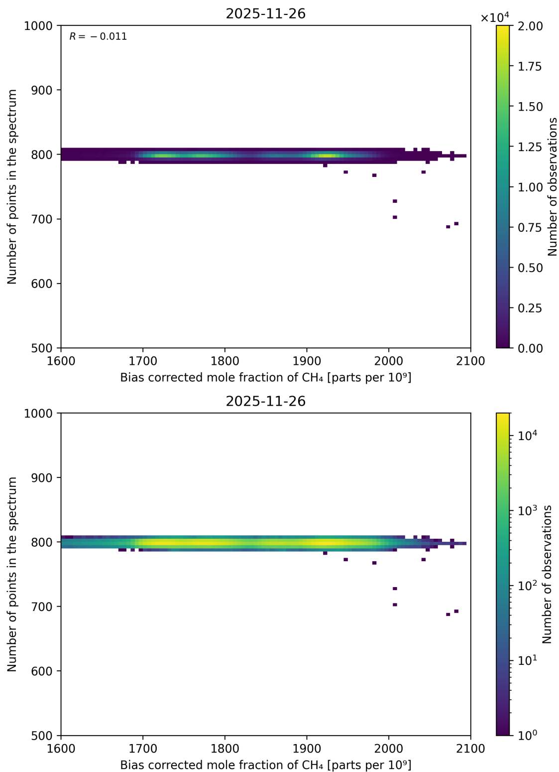
Figure 78: Scatter density plot of “Bias corrected mole fraction of CH 4 ” against “Number of points in the spectrum” for 2025-11-25 to 2025-11-27.
