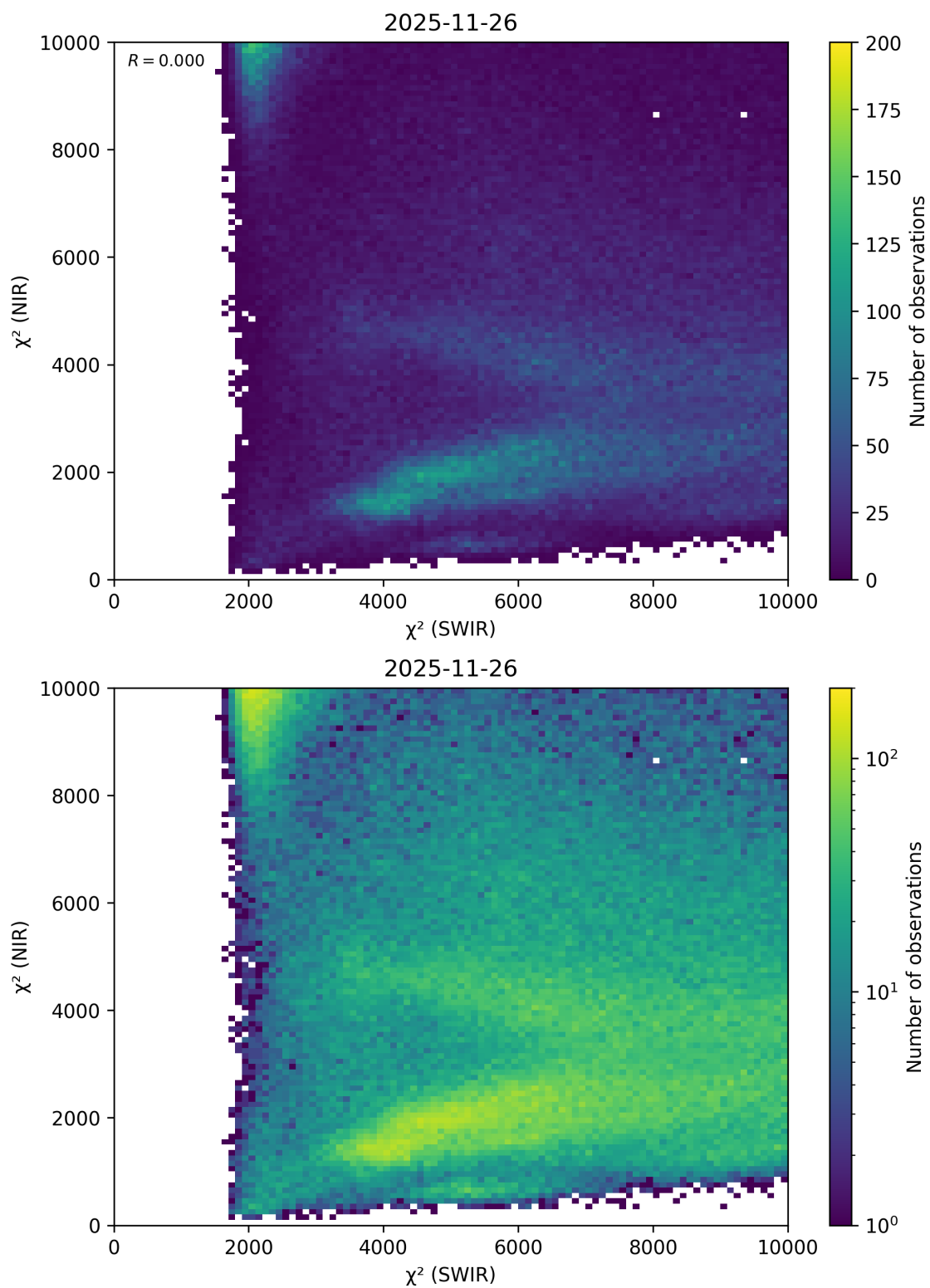
Figure 52: Scatter density plot of “ \chi^2 (SWIR)” against “ \chi^2 (NIR)” for 2025-11-25 to 2025-11-27.
