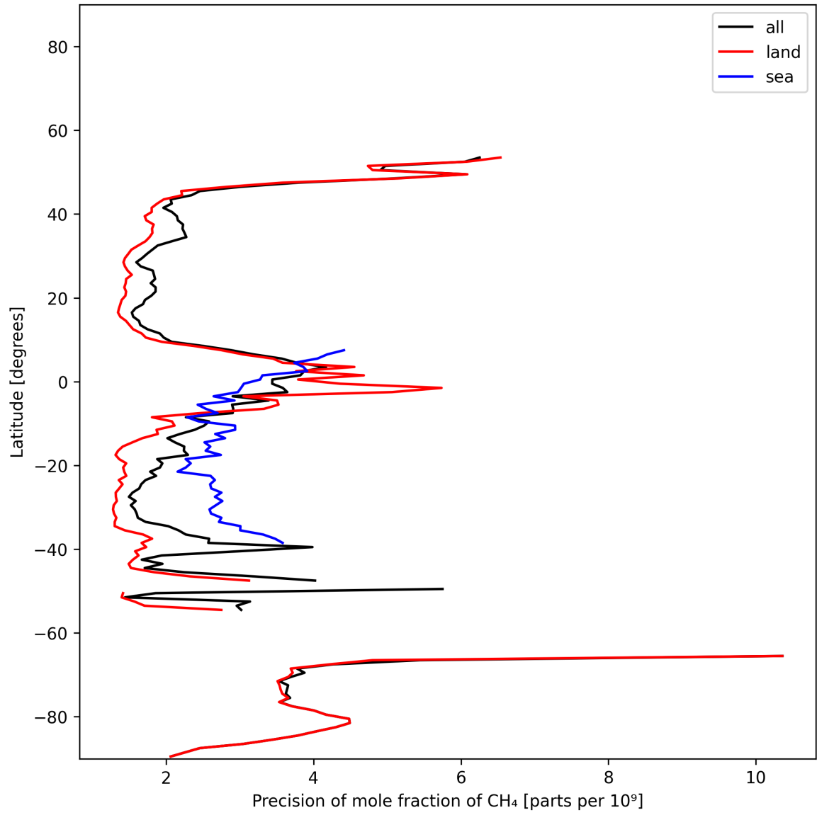
Figure 14: Zonal average of “Precision of mole fraction of CH 4 ” for 2025-11-25 to 2025-11-27.
