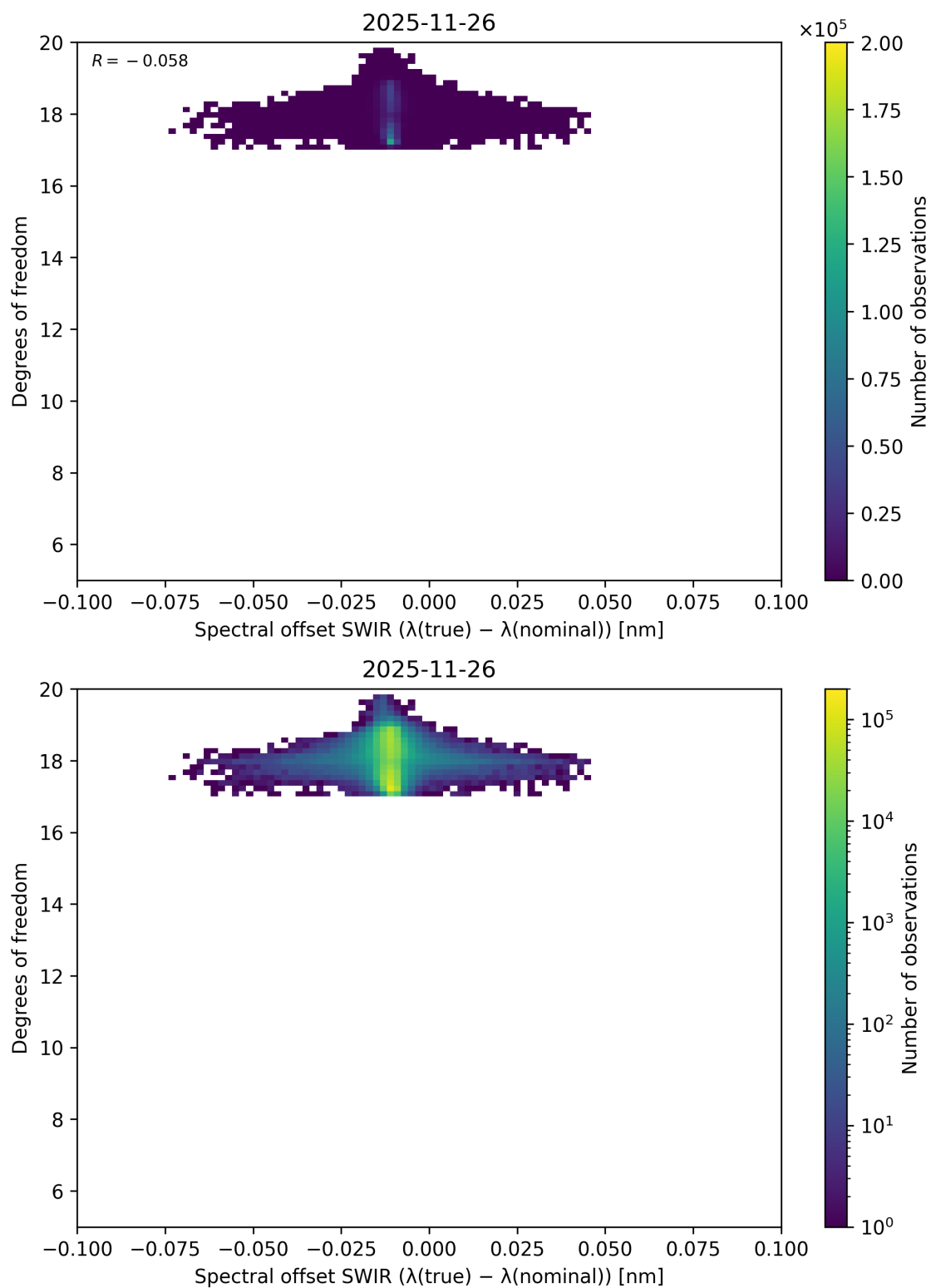
Figure 135: Scatter density plot of “Spectral offset SWIR ( \lambda_{\text{true}} - \lambda_{\text{nominal}} )” against “Degrees of freedom” for 2025-11-25 to 2025-11-27.
