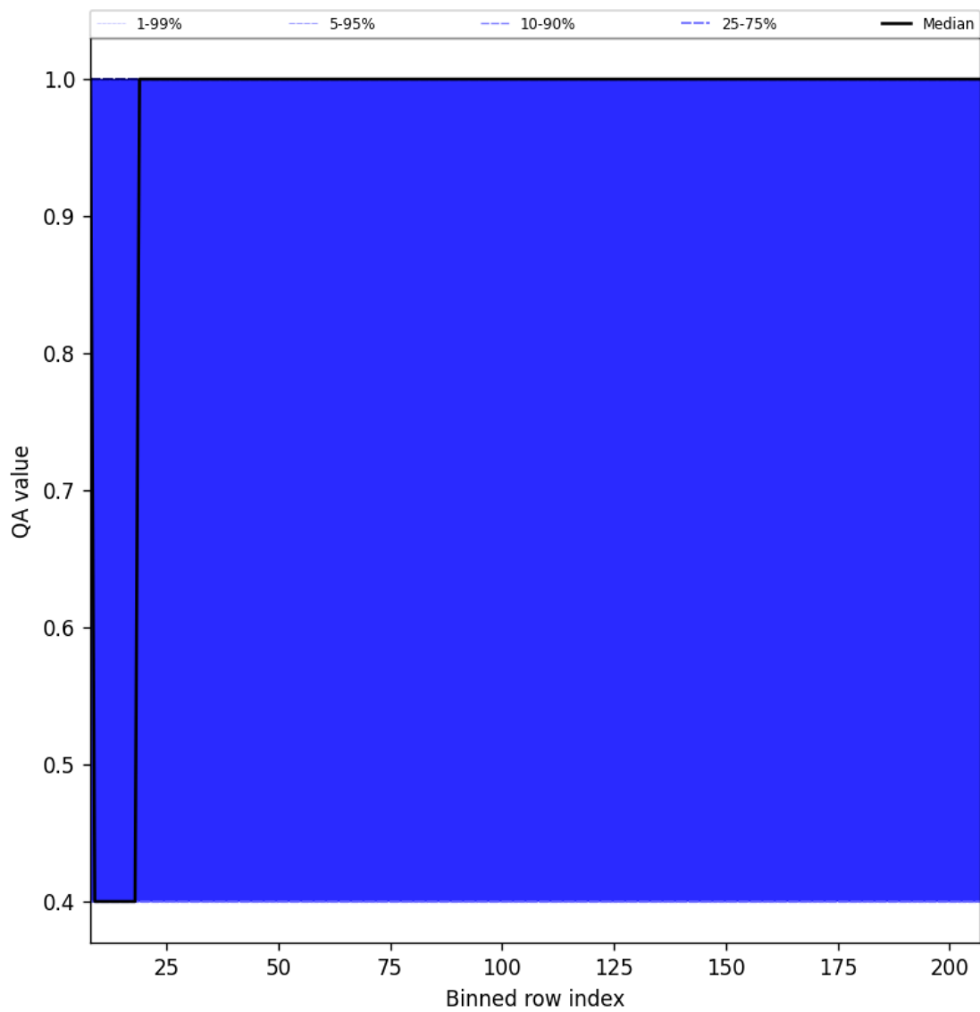
Figure 36: Along track statistics of “QA value” for 2025-11-25 to 2025-11-27
