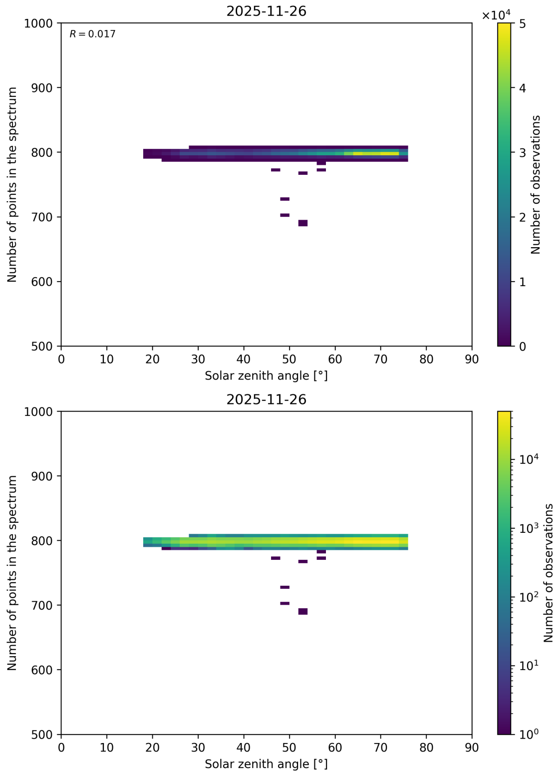
Figure 118: Scatter density plot of “Solar zenith angle” against “Number of points in the spectrum” for 2025-11-25 to 2025-11-27.
