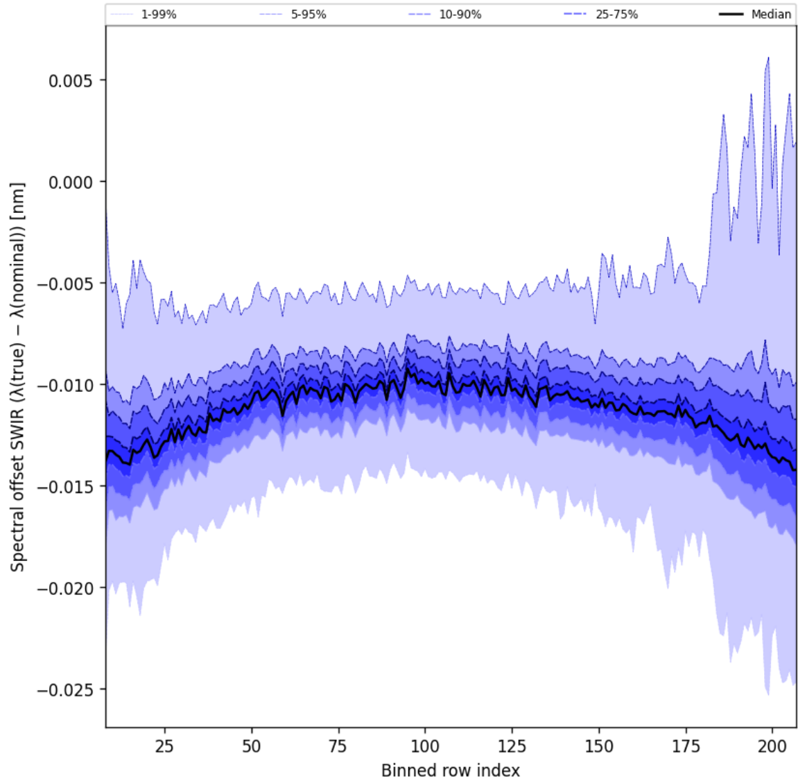
Figure 41: Along track statistics of “Spectral offset SWIR ( \lambda_{\text{true}} - \lambda_{\text{nominal}} )” for 2025-11-25 to 2025-11-27
