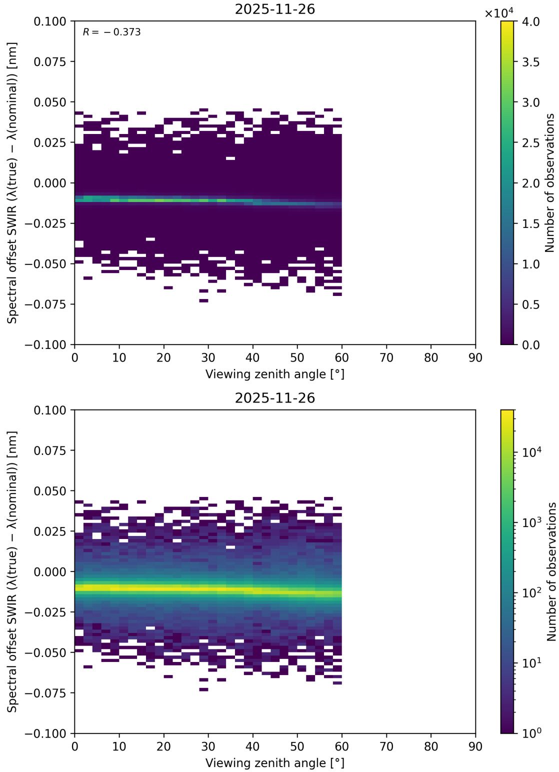
Figure 132: Scatter density plot of “Viewing zenith angle” against “Spectral offset SWIR ( \lambda_{\text{true}} - \lambda_{\text{nominal}} )” for 2025-11-25 to 2025-11-27.
