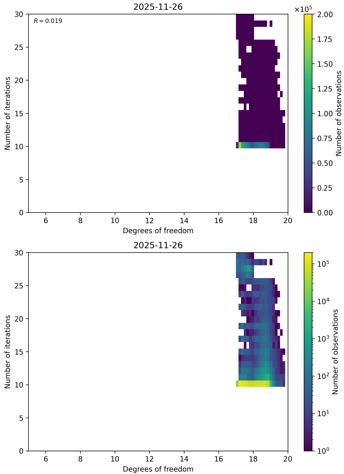
Figure 59: Scatter density plot of “Degrees of freedom” against “Number of iterations” for 2025-11-25 to 2025-11-27.
