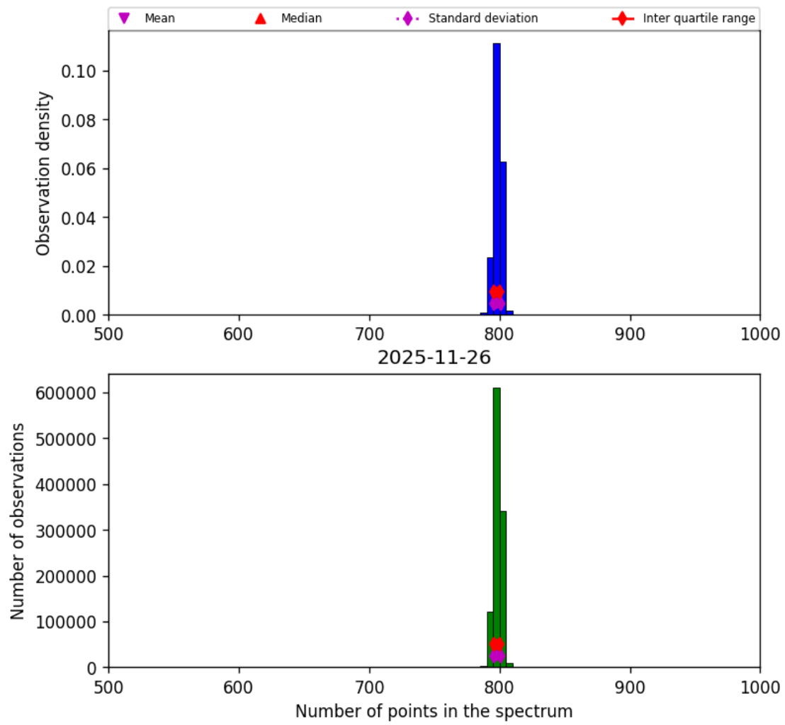
Figure 28: Histogram of “Number of points in the spectrum” for 2025-11-25 to 2025-11-27
