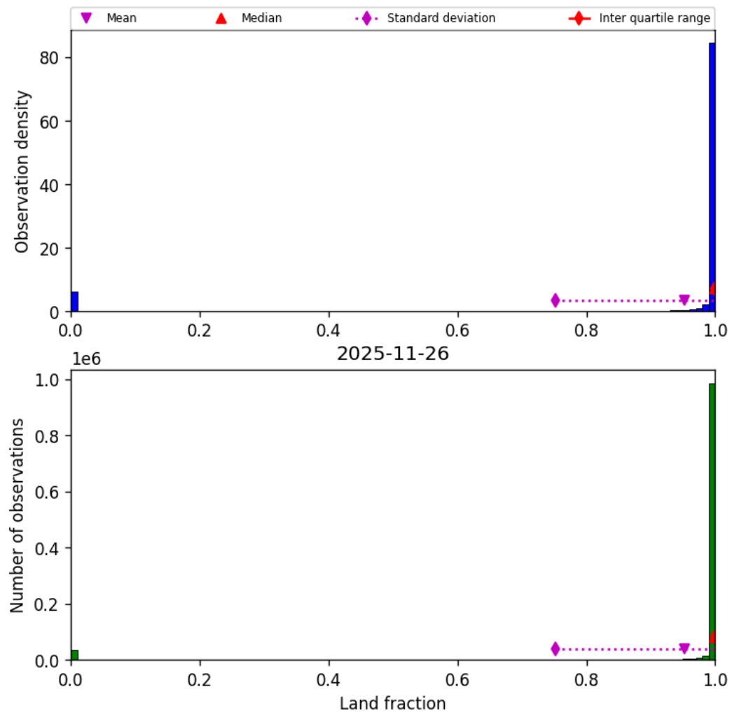
Figure 35: Histogram of "Land fraction" for 2025-11-25 to 2025-11-27
