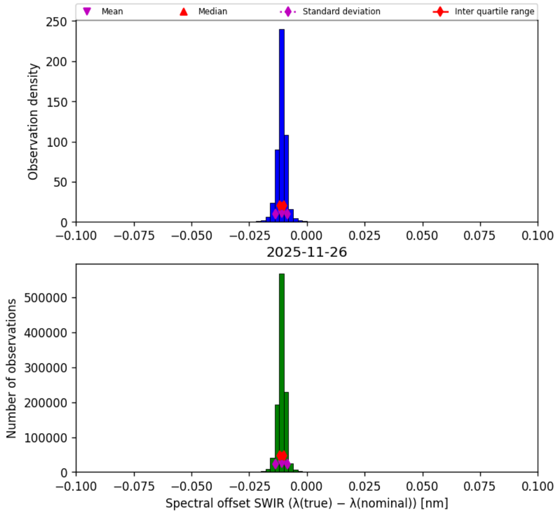
Figure 29: Histogram of “Spectral offset SWIR ( \lambda_{\text{true}} - \lambda_{\text{nominal}} )” for 2025-11-25 to 2025-11-27
