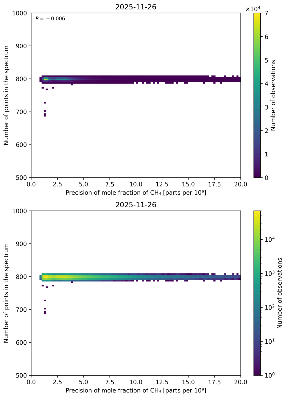
Figure 96: Scatter density plot of “Precision of mole fraction of CH 4 ” against “Number of points in the spectrum” for 2025-11-25 to 2025-11-27.
