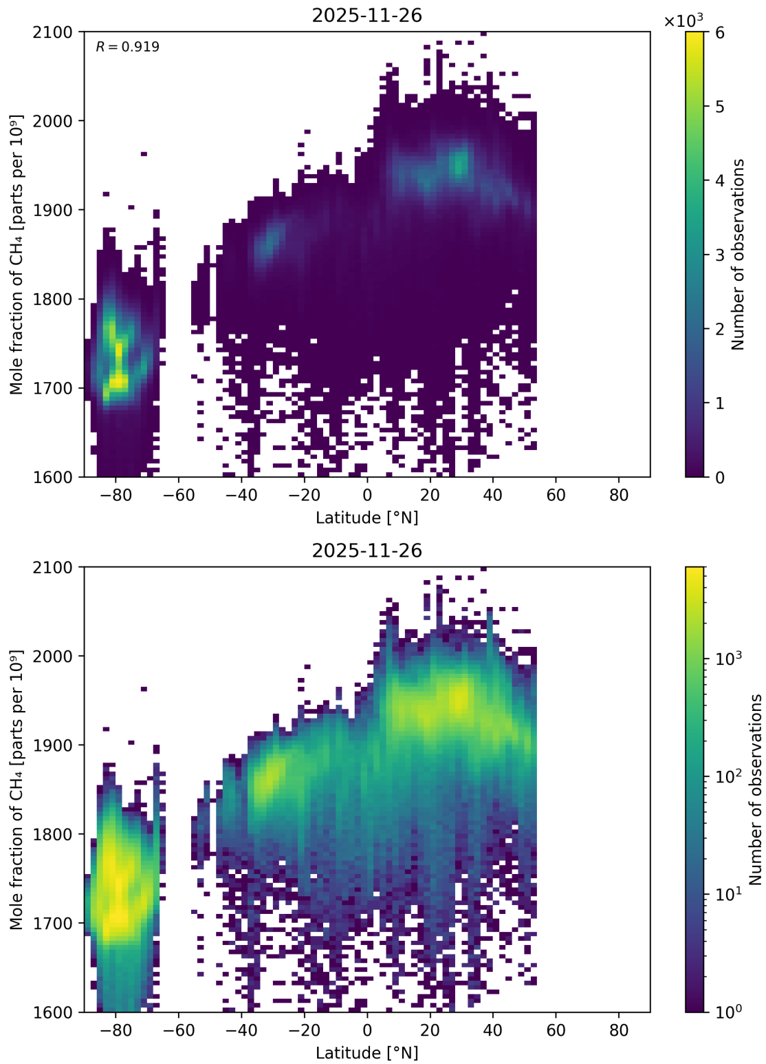
Figure 66: Scatter density plot of “Latitude” against “Mole fraction of \text{CH}_4 ” for 2025-11-25 to 2025-11-27.
