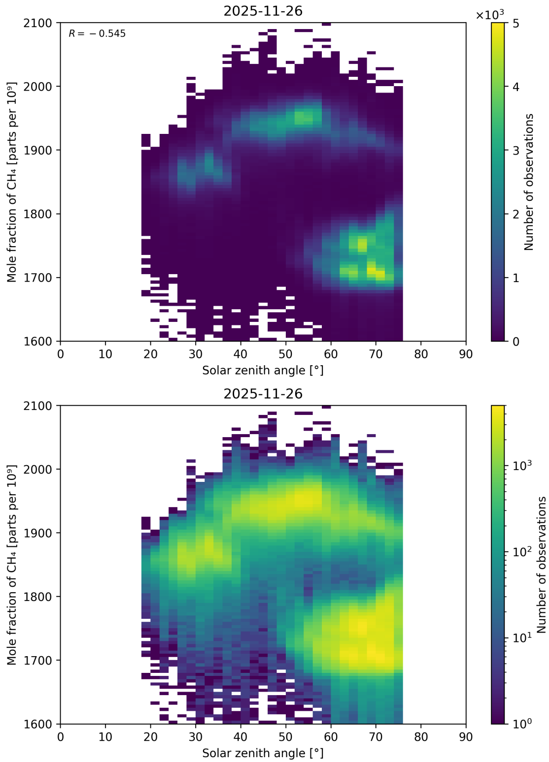
Figure 114: Scatter density plot of “Solar zenith angle” against “Mole fraction of CH 4 ” for 2025-11-25 to 2025-11-27.
