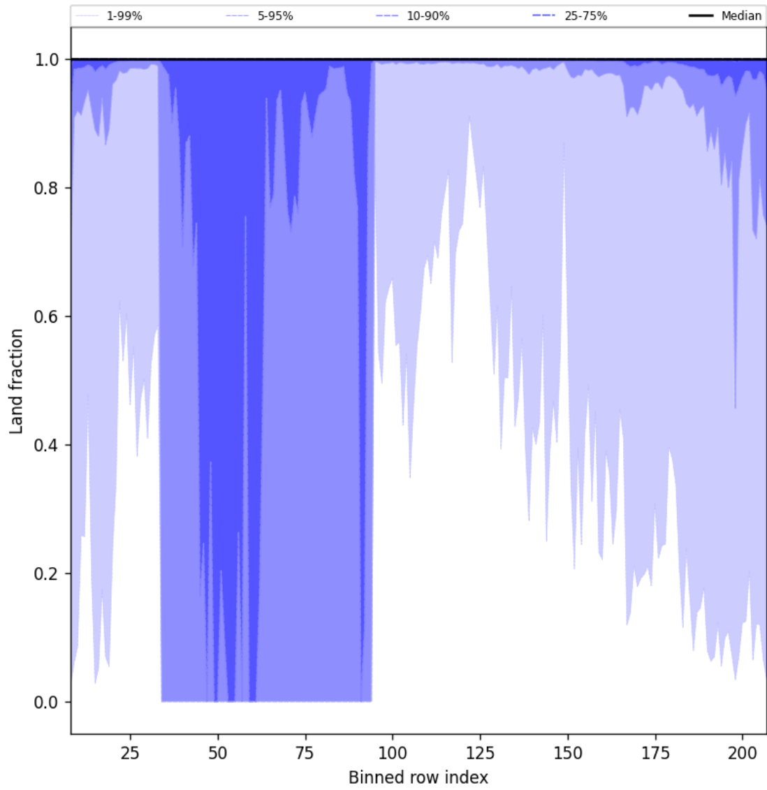
Figure 47: Along track statistics of “Land fraction” for 2025-11-25 to 2025-11-27
