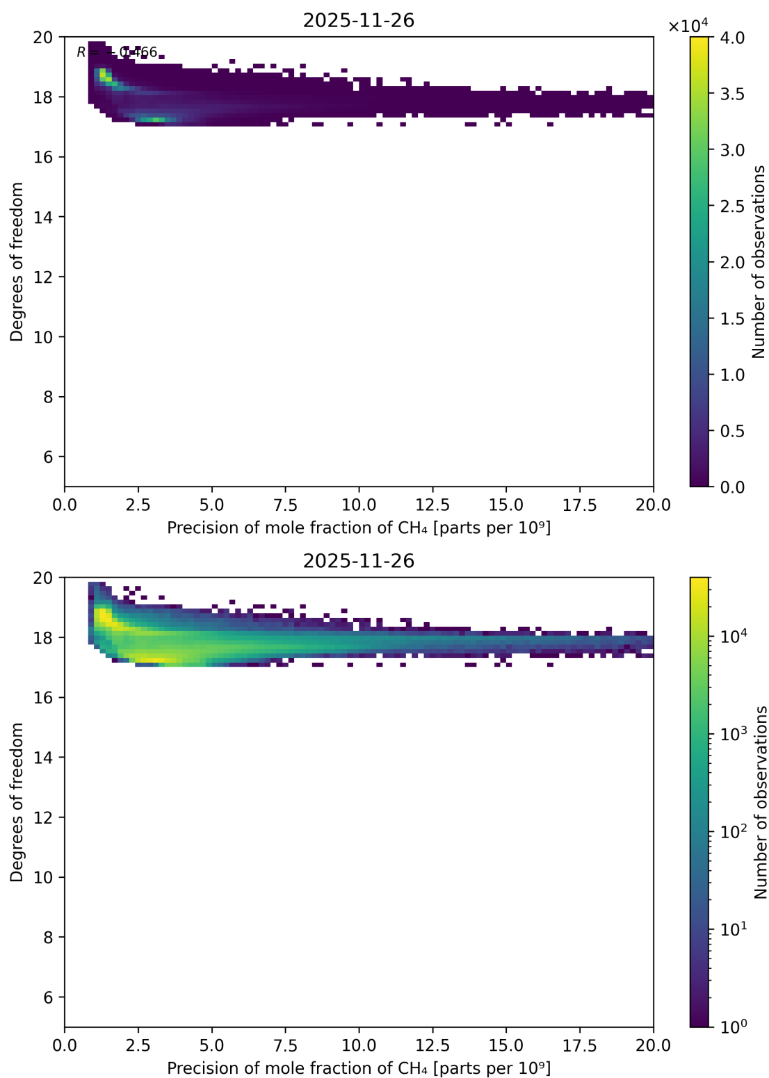
Figure 91: Scatter density plot of “Precision of mole fraction of CH 4 ” against “Degrees of freedom” for 2025-11-25 to 2025-11-27.
