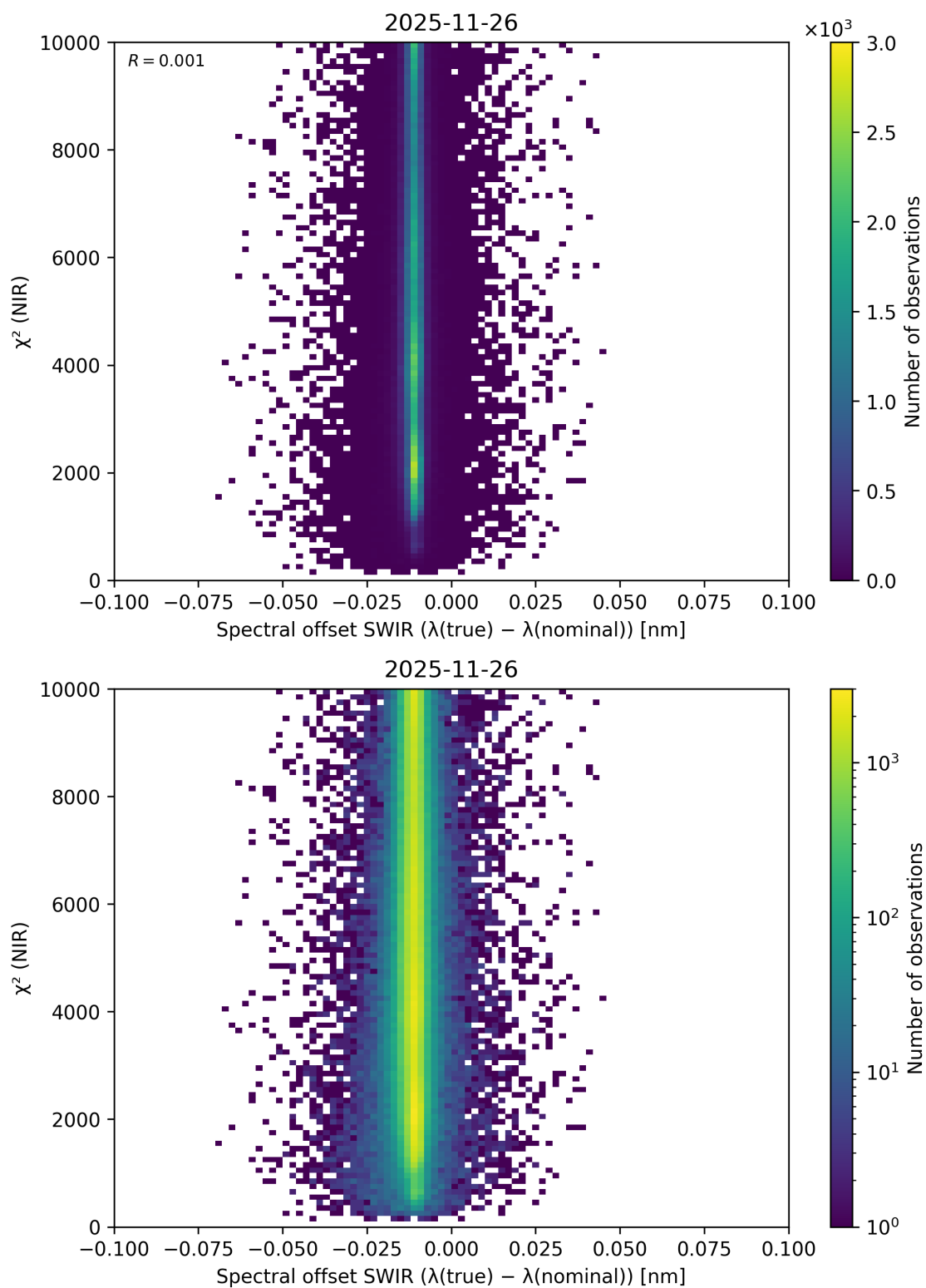
Figure 133: Scatter density plot of “Spectral offset SWIR ( \lambda_{\text{true}} - \lambda_{\text{nominal}} )” against “ \chi^2 (NIR)” for 2025-11-25 to 2025-11-27.
