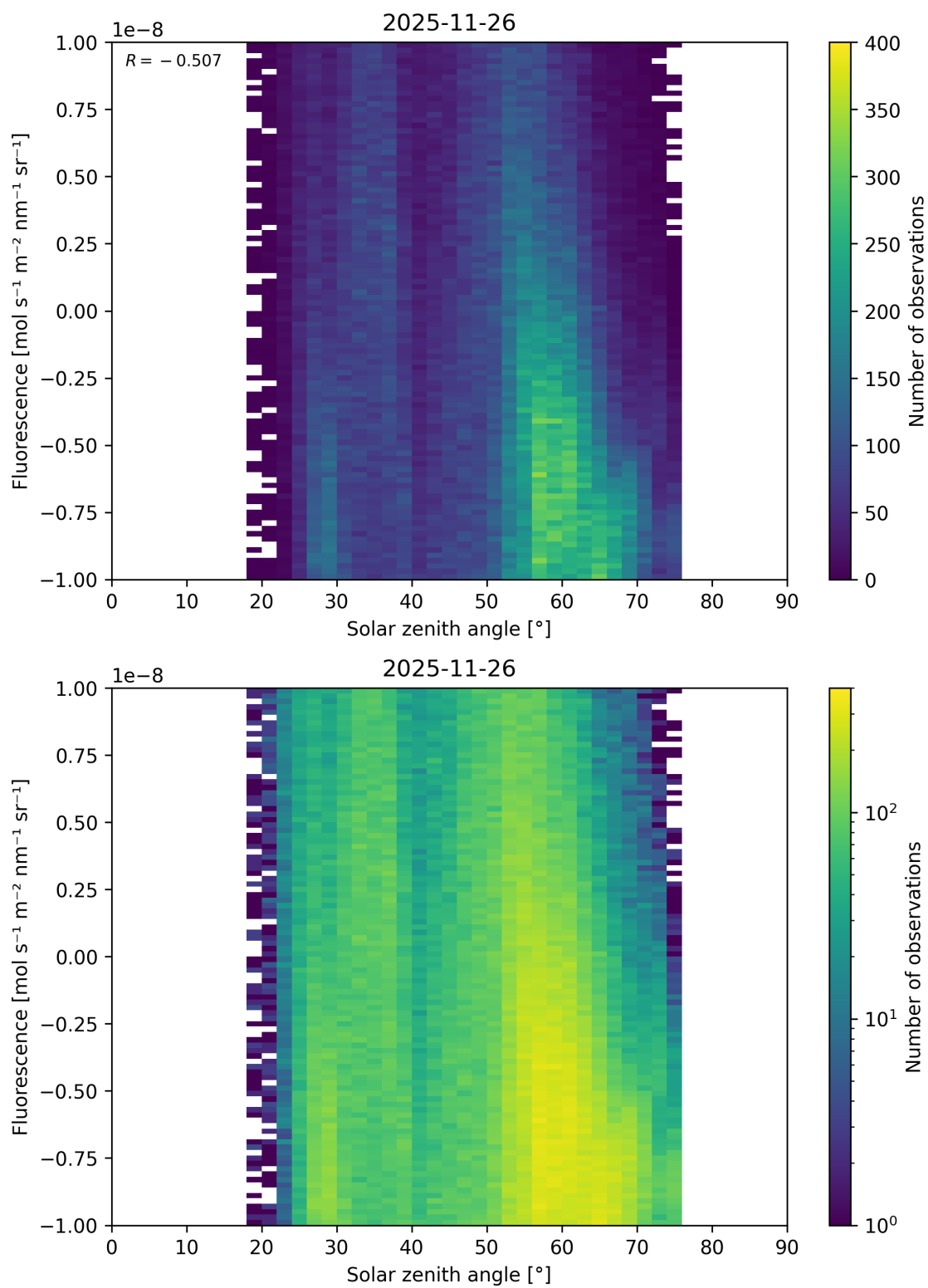
Figure 111: Scatter density plot of “Solar zenith angle” against “Fluorescence” for 2025-11-25 to 2025-11-27.
