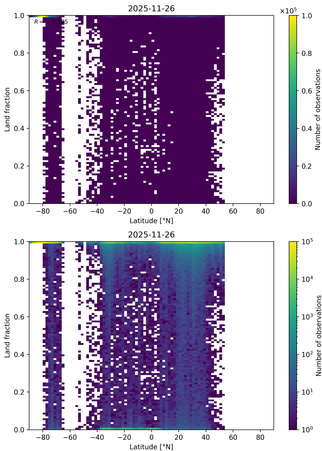
Figure 65: Scatter density plot of “Latitude” against “Land fraction” for 2025-11-25 to 2025-11-27.
