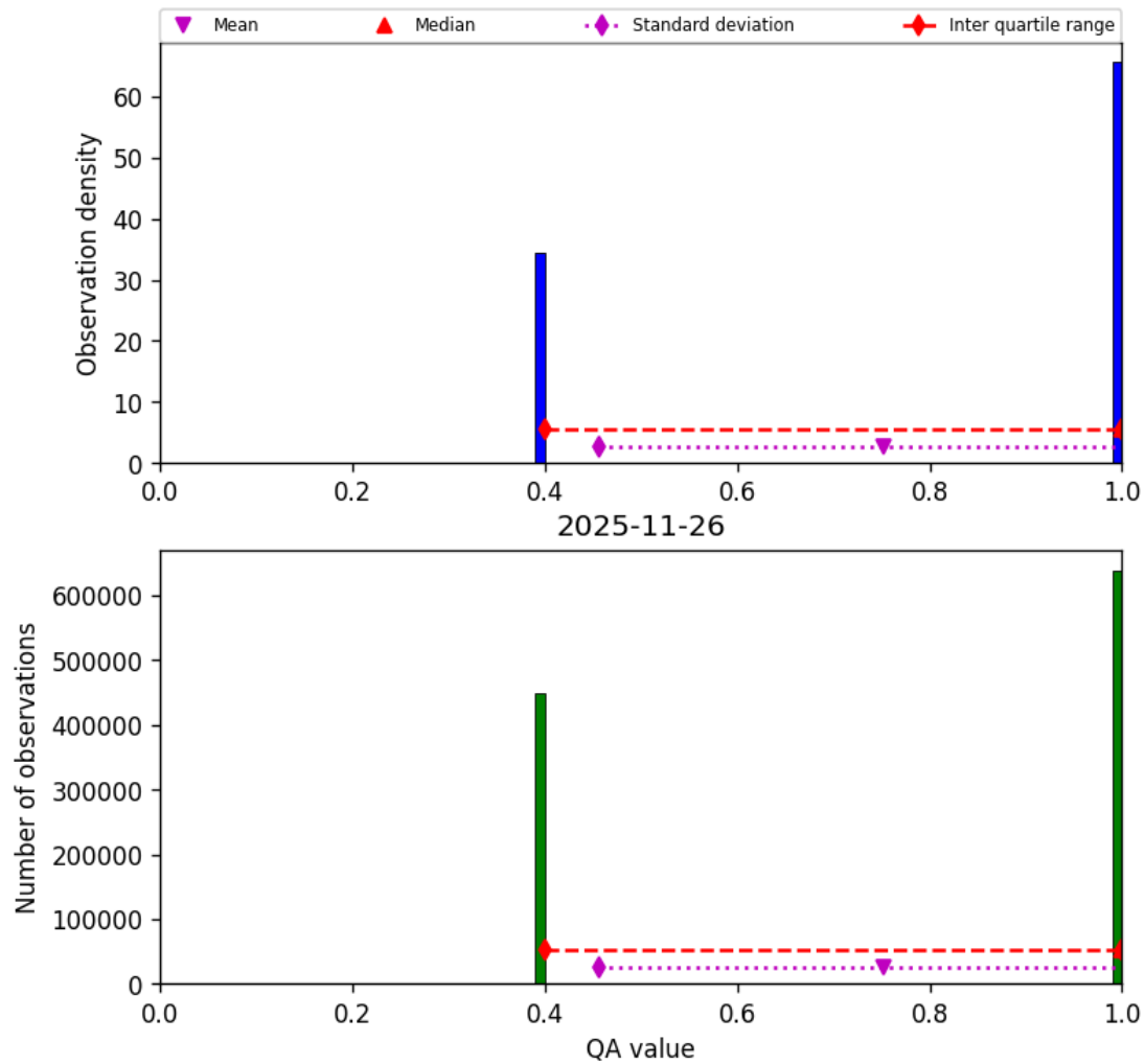
Figure 24: Histogram of “QA value” for 2025-11-25 to 2025-11-27
