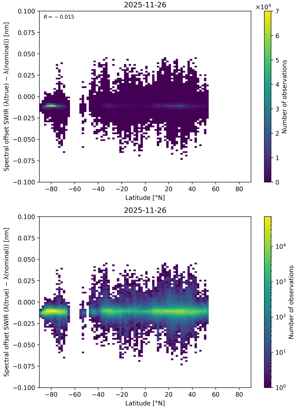
Figure 71: Scatter density plot of “Latitude” against “Spectral offset SWIR ( \lambda_{\text{true}} - \lambda_{\text{nominal}} )” for 2025-11-25 to 2025-11-27.
