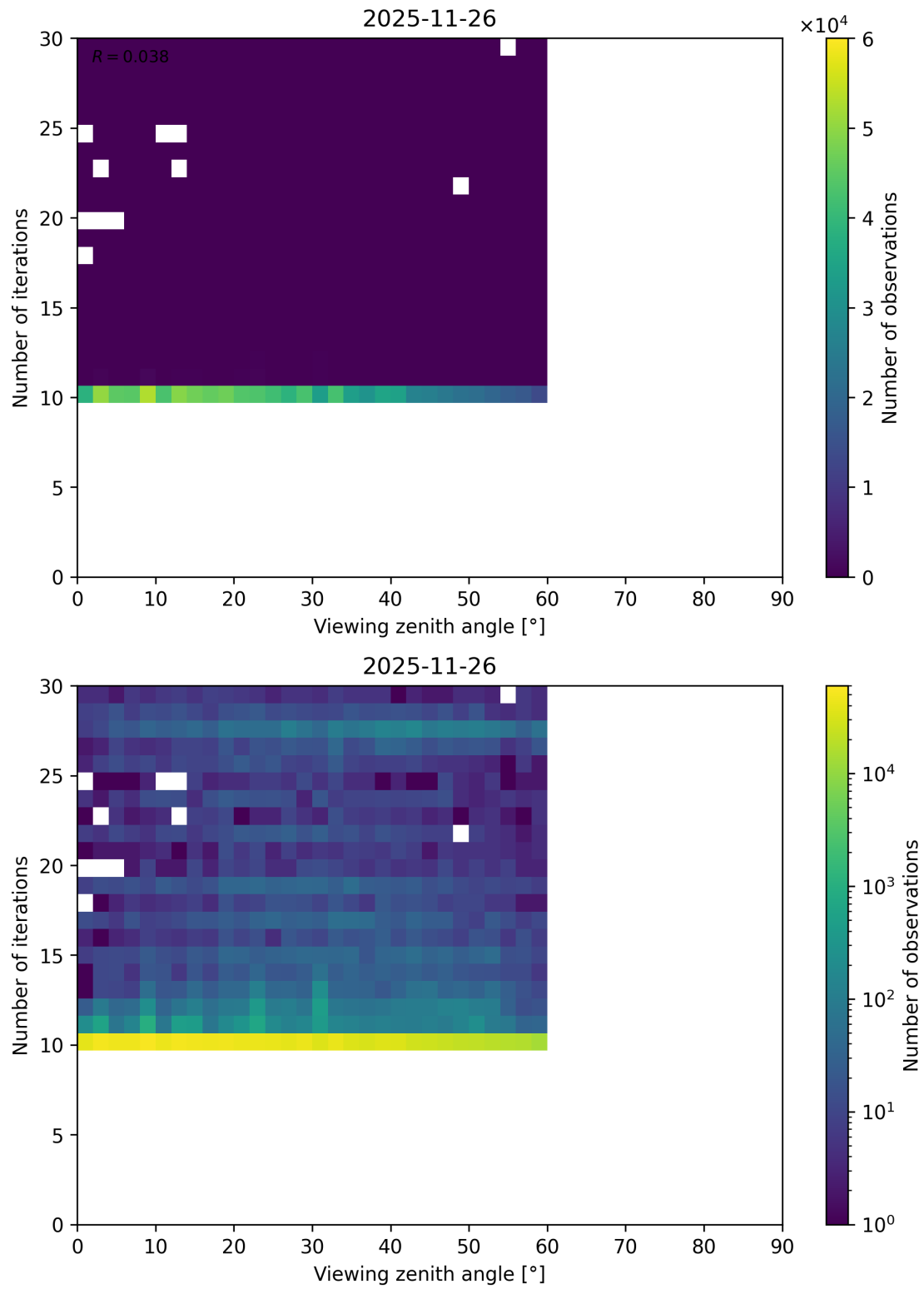
Figure 129: Scatter density plot of “Viewing zenith angle” against “Number of iterations” for 2025-11-25 to 2025-11-27.
