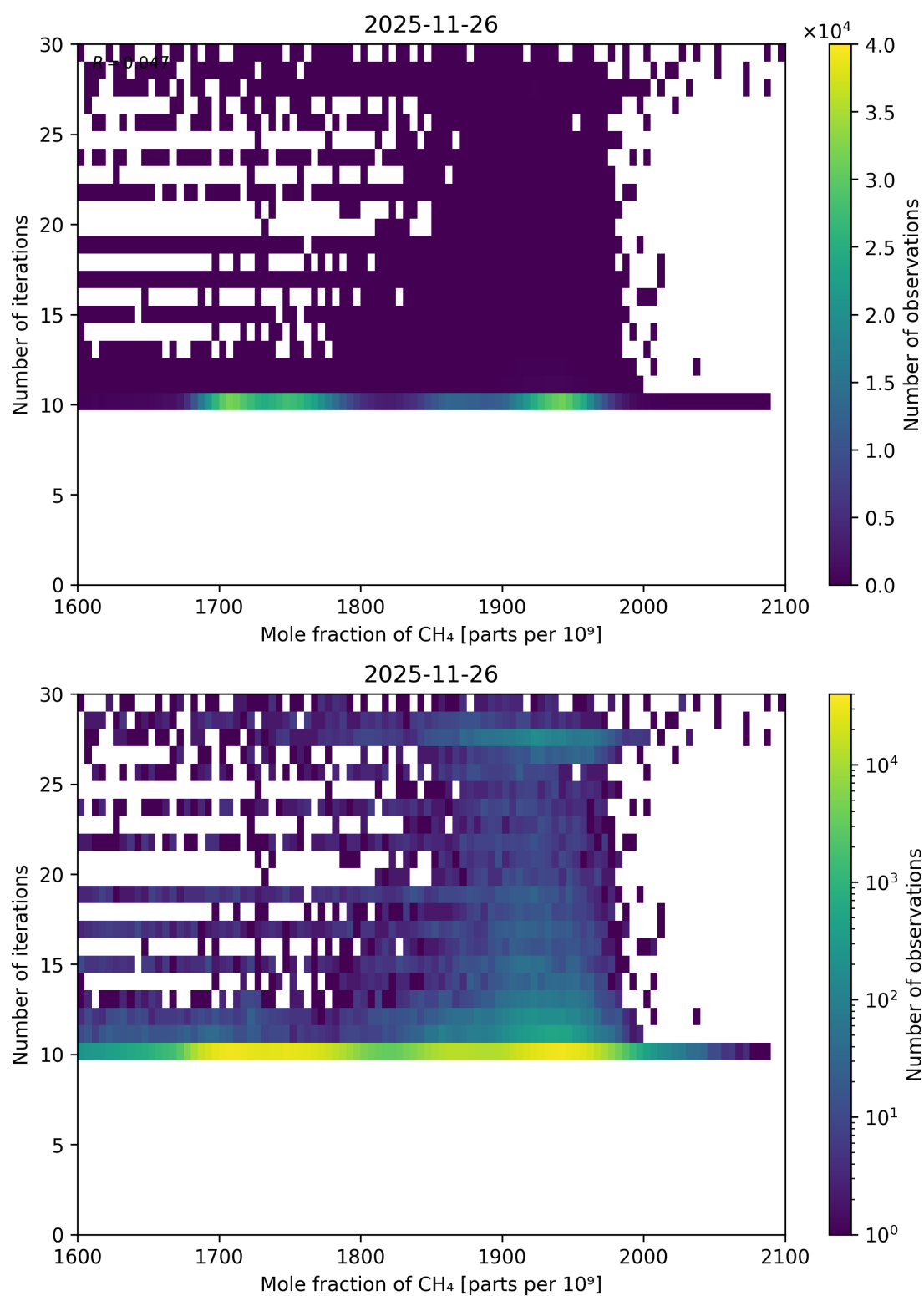
Figure 87: Scatter density plot of “Mole fraction of CH 4 ” against “Number of iterations” for 2025-11-25 to 2025-11-27.
