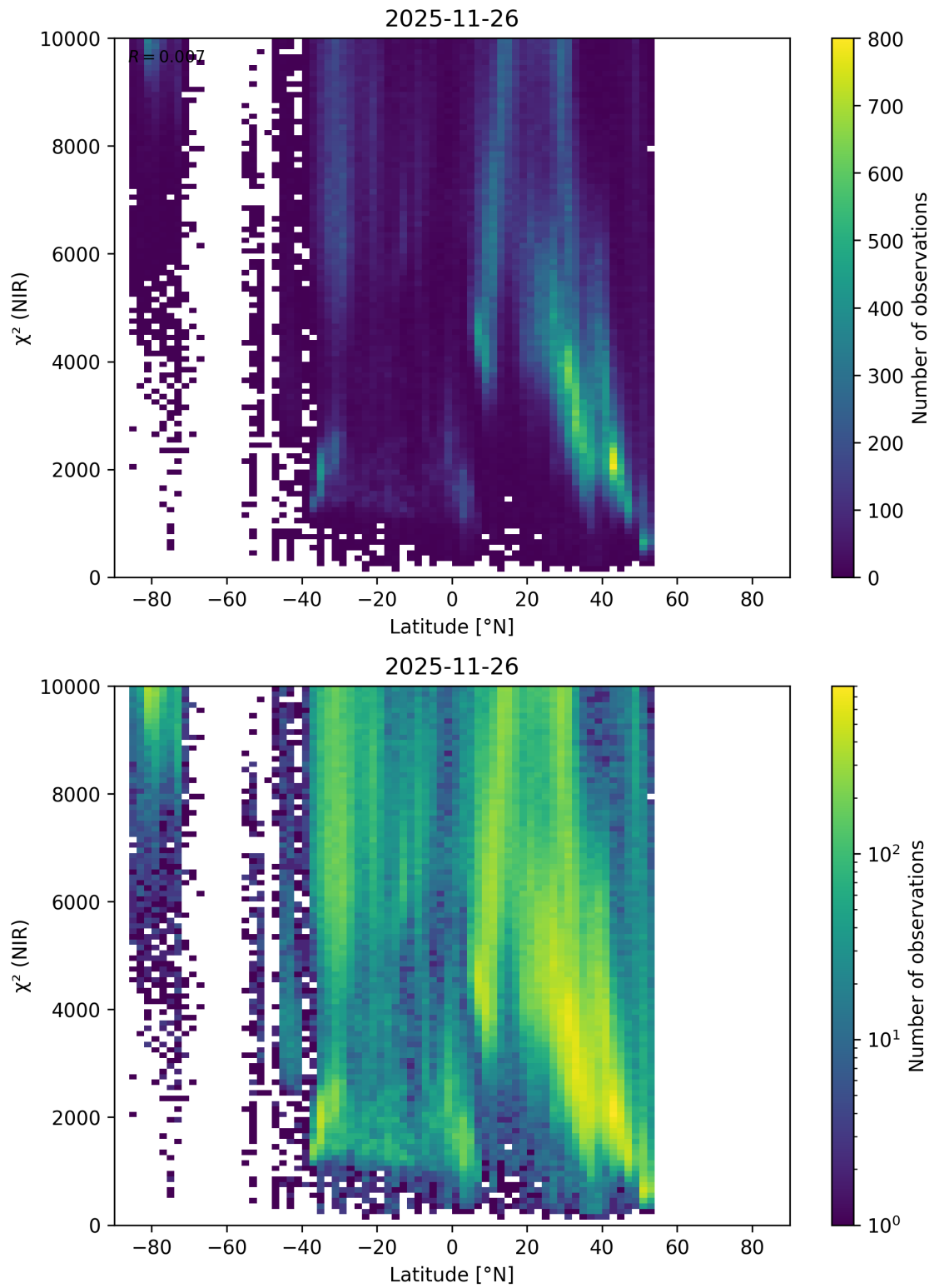
Figure 61: Scatter density plot of “Latitude” against “ \chi^2 (NIR)” for 2025-11-25 to 2025-11-27.
