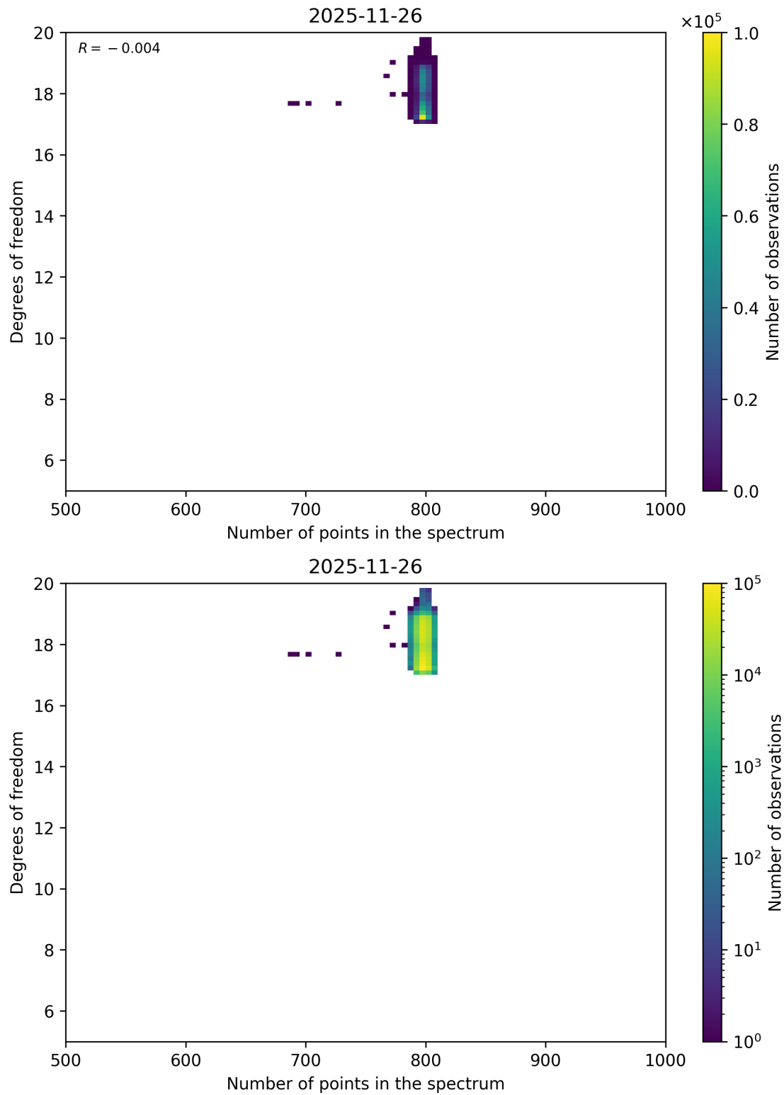
Figure 103: Scatter density plot of “Number of points in the spectrum” against “Degrees of freedom” for 2025-11-25 to 2025-11-27.
