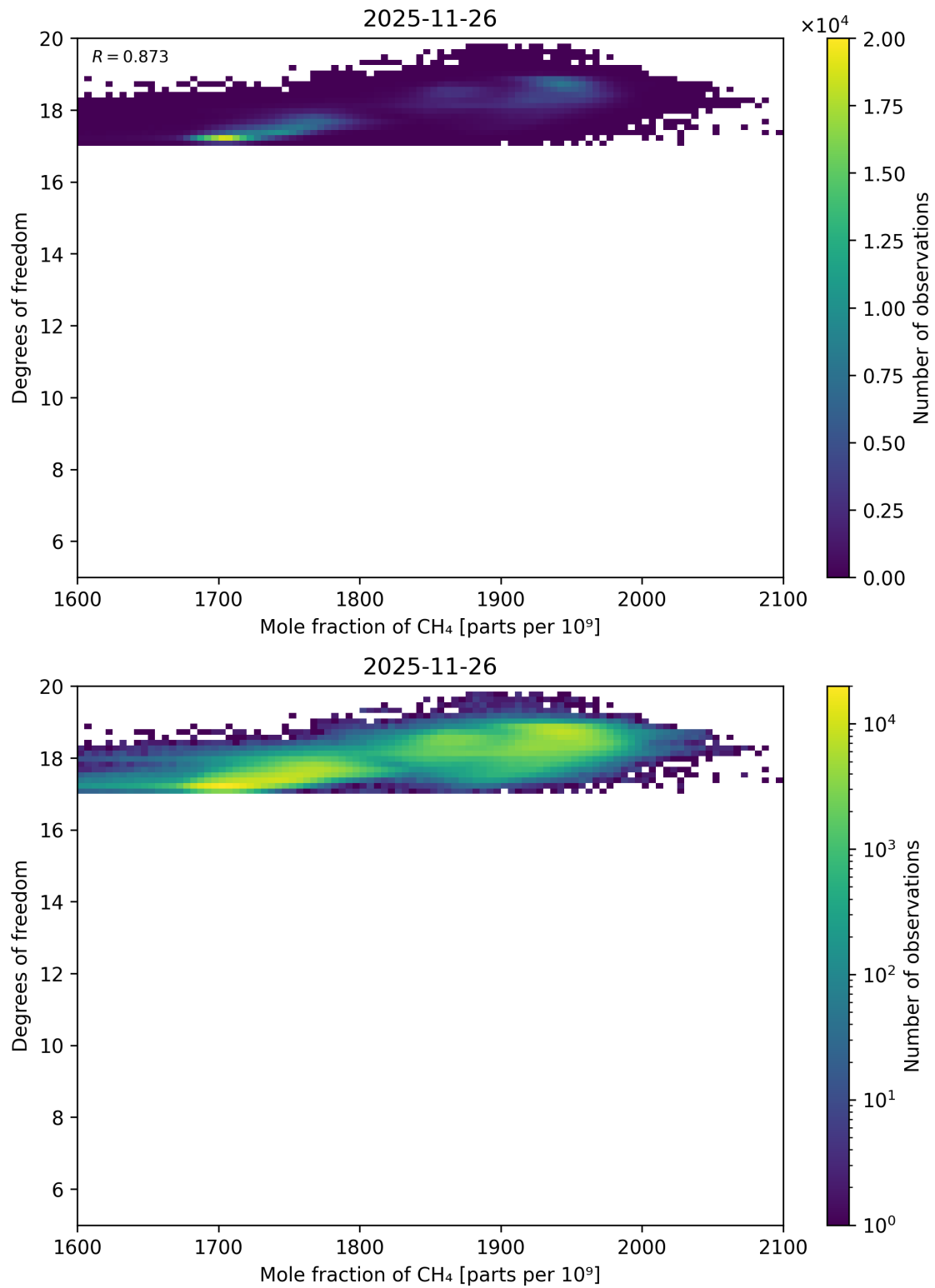
Figure 82: Scatter density plot of “Mole fraction of CH 4 ” against “Degrees of freedom” for 2025-11-25 to 2025-11-27.
