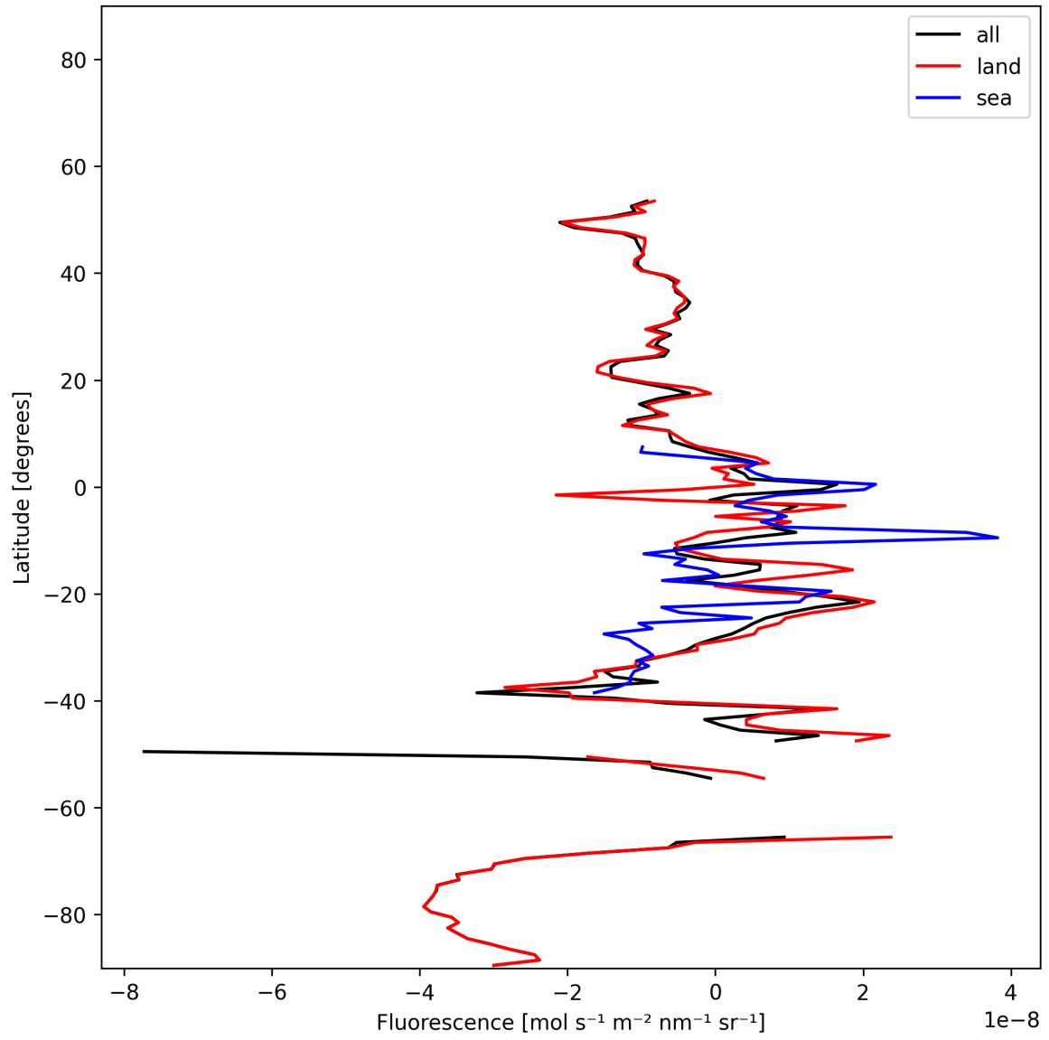
Figure 22: Zonal average of “Fluorescence” for 2025-11-25 to 2025-11-27.
