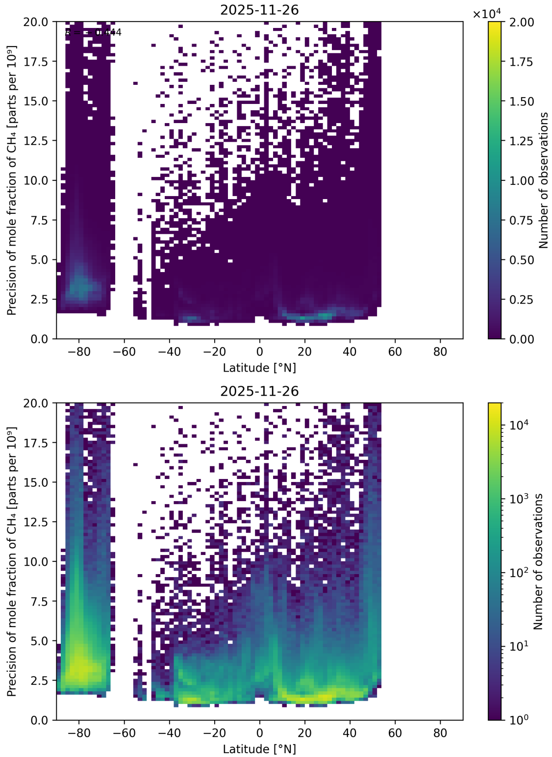
Figure 68: Scatter density plot of “Latitude” against “Precision of mole fraction of CH 4 ” for 2025-11-25 to 2025-11-27.
