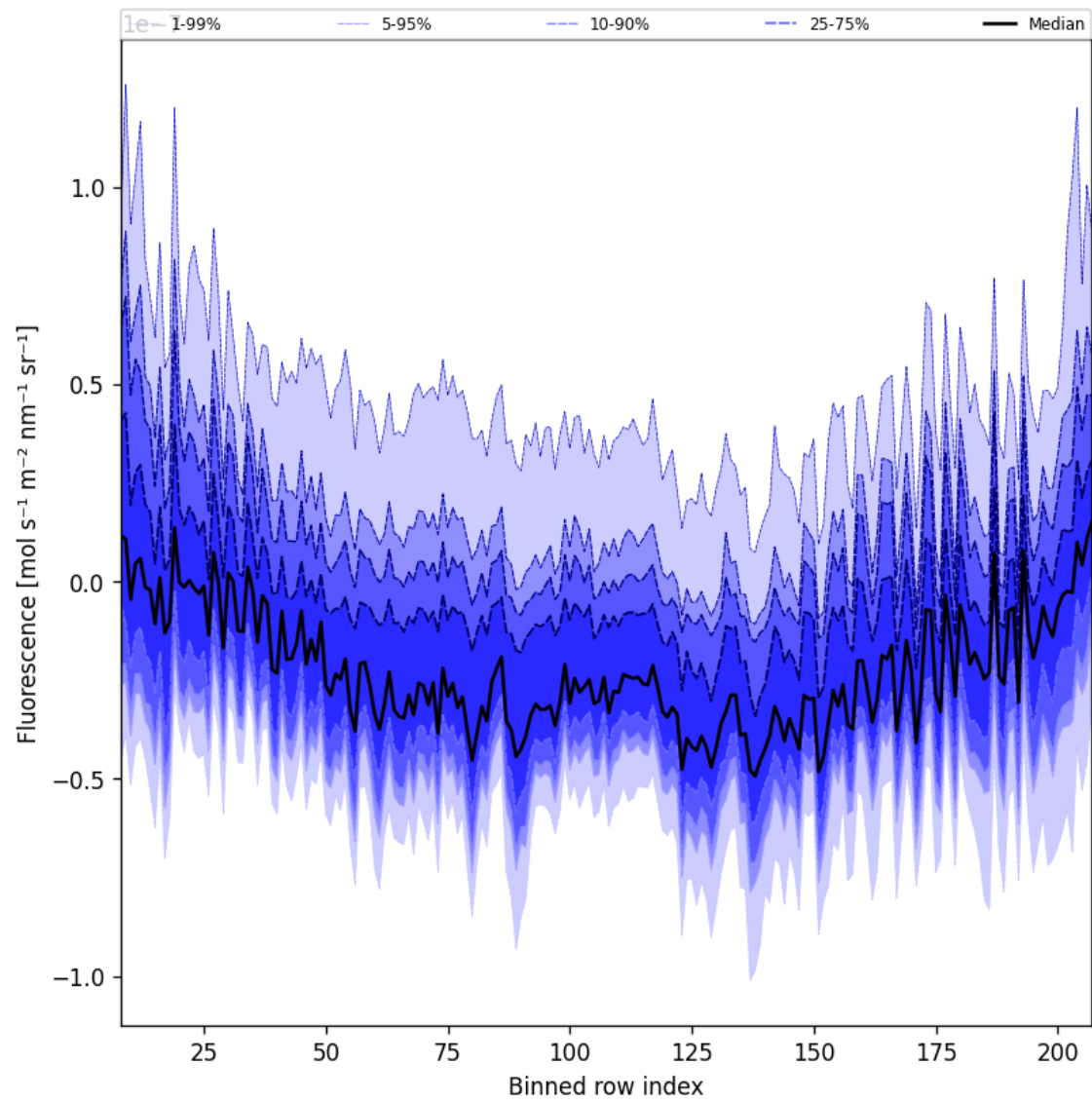
Figure 46: Along track statistics of “Fluorescence” for 2025-11-25 to 2025-11-27
