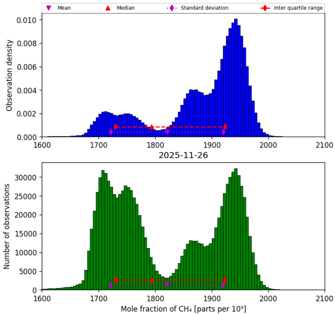
Figure 25: Histogram of “Mole fraction of CH 4 ” for 2025-11-25 to 2025-11-27
