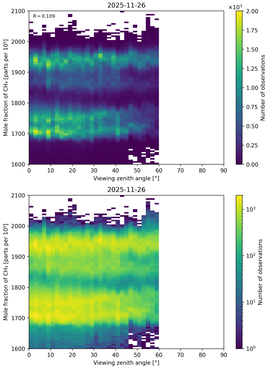
Figure 126: Scatter density plot of “Viewing zenith angle” against “Mole fraction of \text{CH}_4 ” for 2025-11-25 to 2025-11-27.
