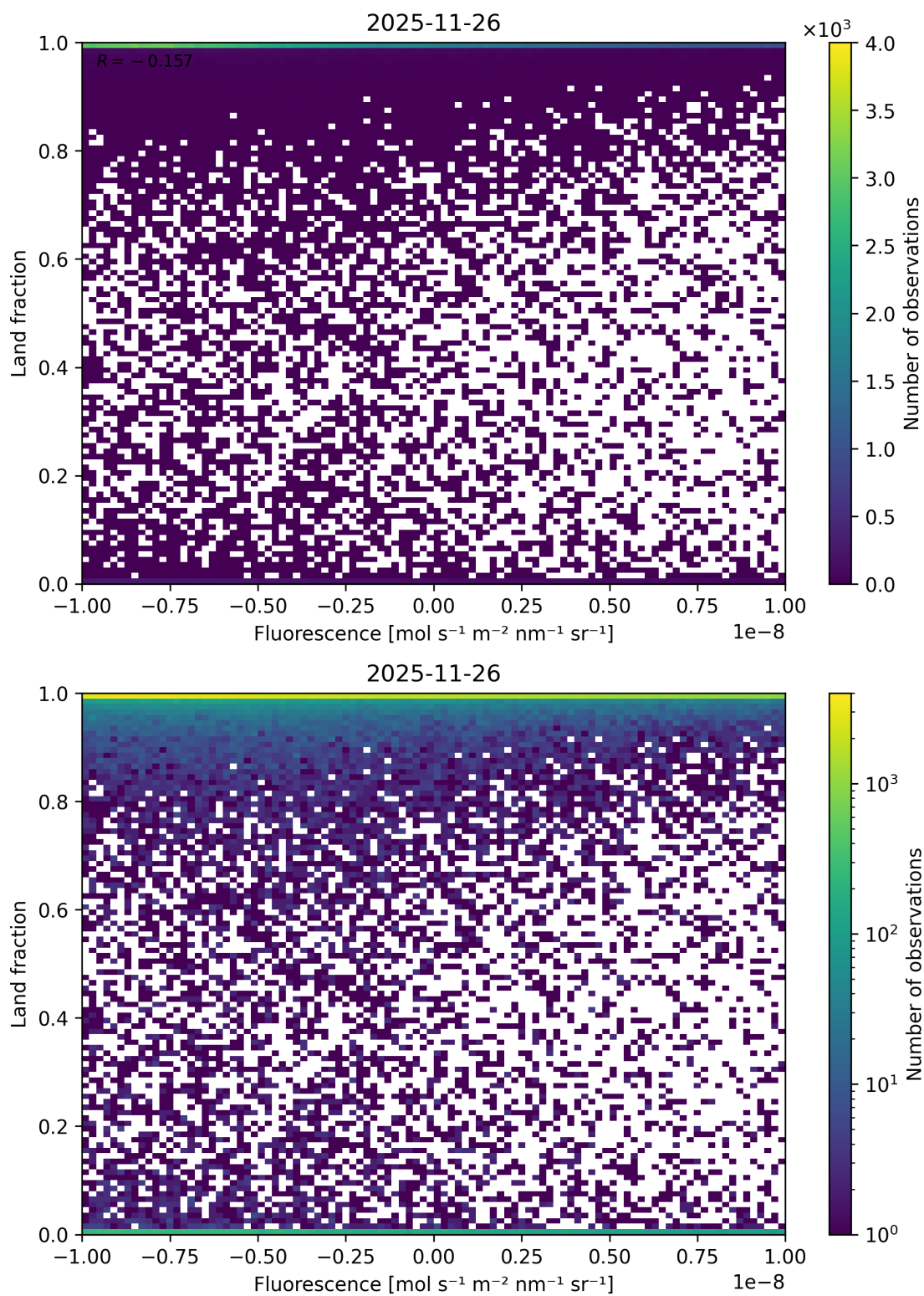
Figure 60: Scatter density plot of “Fluorescence” against “Land fraction” for 2025-11-25 to 2025-11-27.
