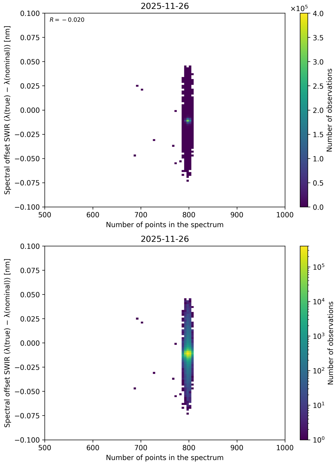
Figure 107: Scatter density plot of “Number of points in the spectrum” against “Spectral offset SWIR ( \lambda_{\text{true}} - \lambda_{\text{nominal}} )” for 2025-11-25 to 2025-11-27.
