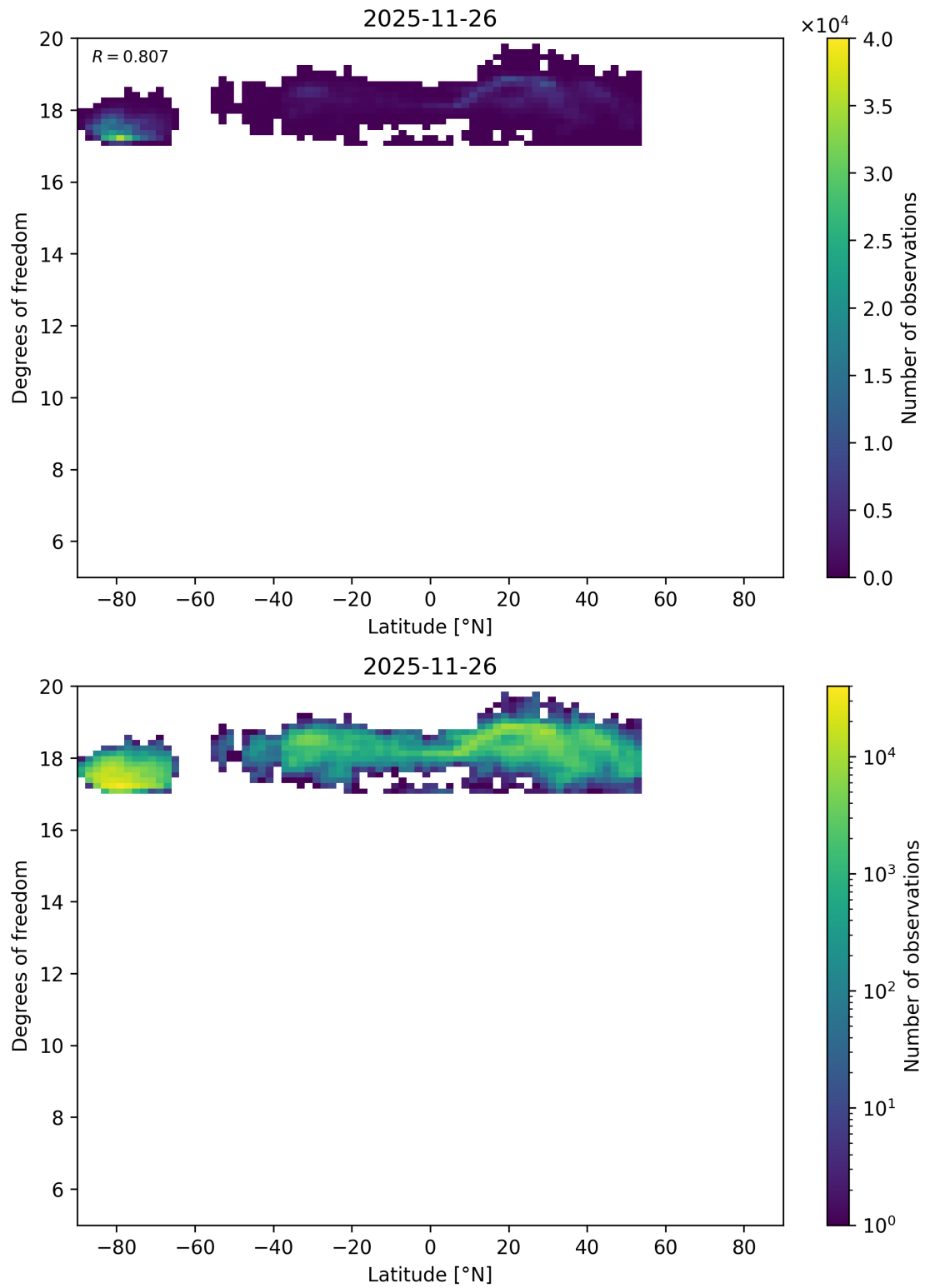
Figure 63: Scatter density plot of “Latitude” against “Degrees of freedom” for 2025-11-25 to 2025-11-27.
