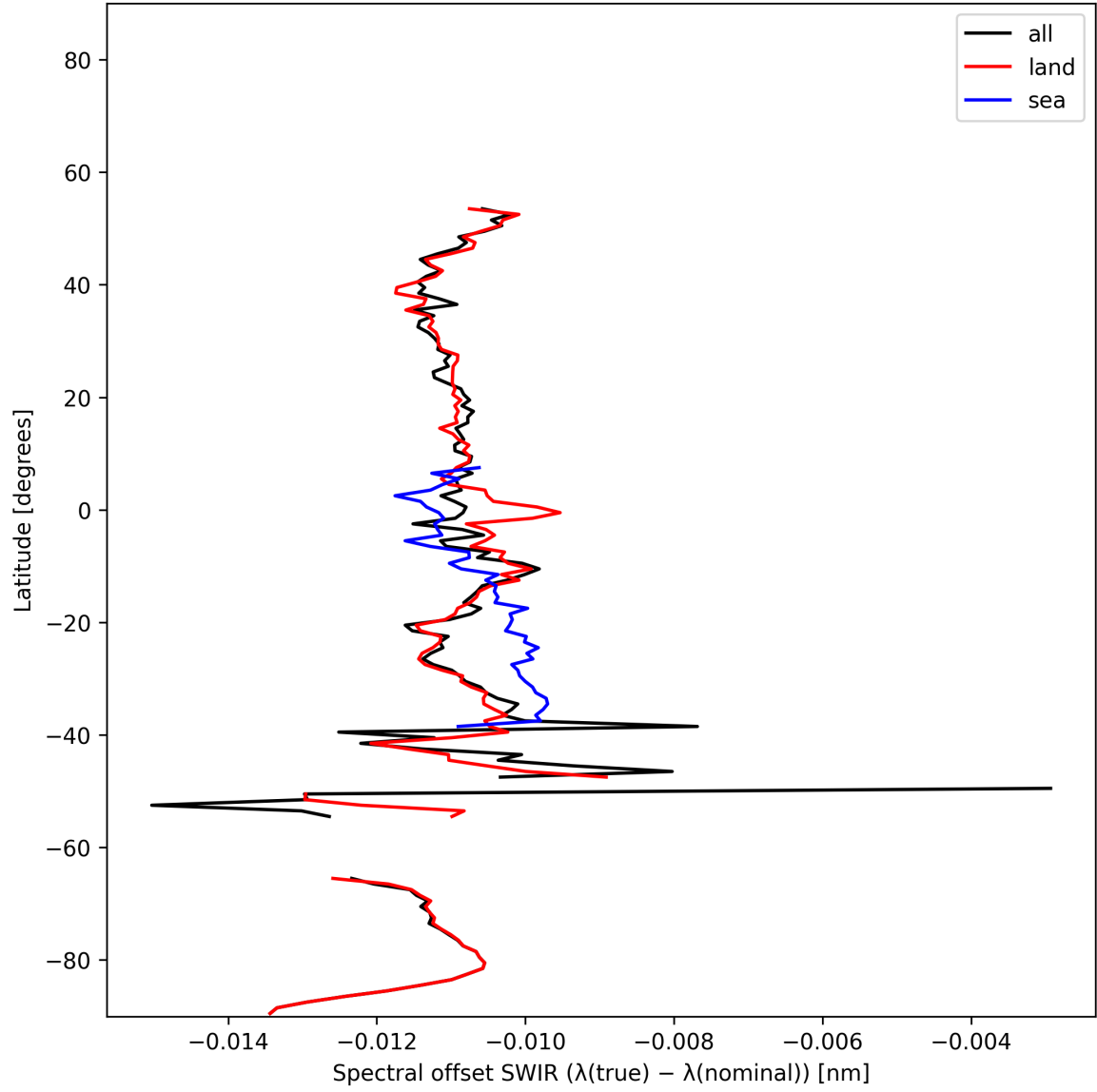
Figure 17: Zonal average of “Spectral offset SWIR ( \lambda_{\text{true}} - \lambda_{\text{nominal}} )” for 2025-11-25 to 2025-11-27.
