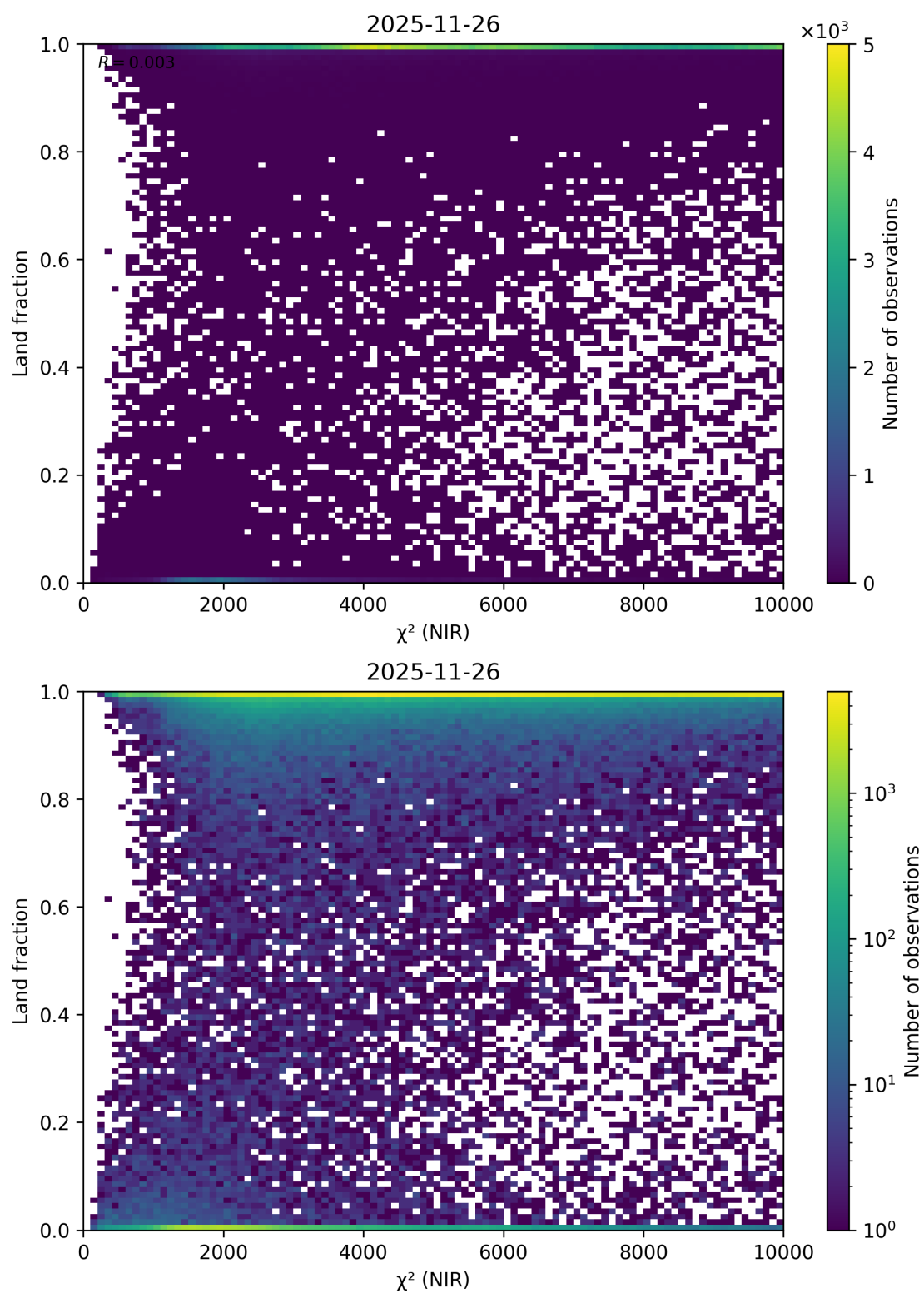
Figure 50: Scatter density plot of “ \chi^2 (NIR)” against “Land fraction” for 2025-11-25 to 2025-11-27.
