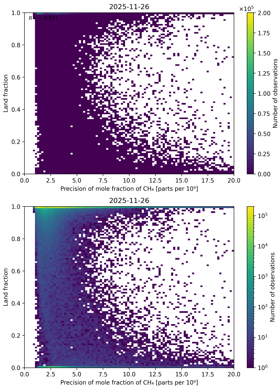
Figure 93: Scatter density plot of “Precision of mole fraction of CH 4 ” against “Land fraction” for 2025-11-25 to 2025-11-27.
