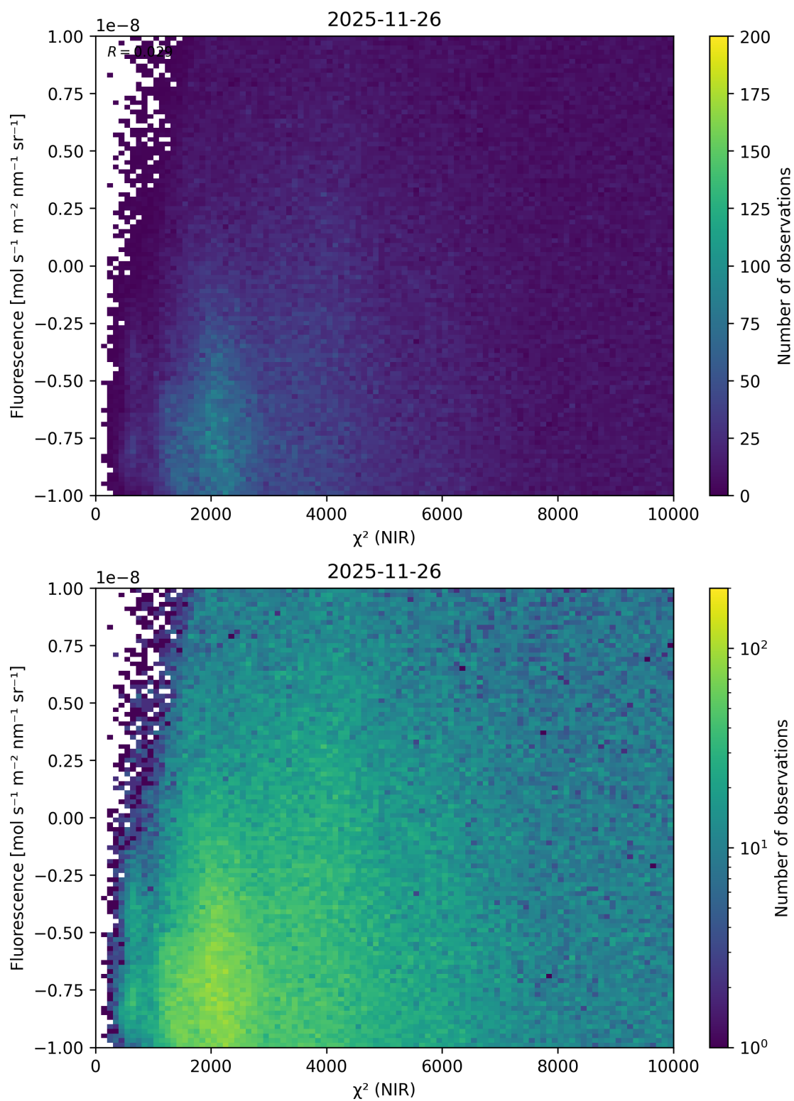
Figure 49: Scatter density plot of “ \chi^2 (NIR)” against “Fluorescence” for 2025-11-25 to 2025-11-27.
