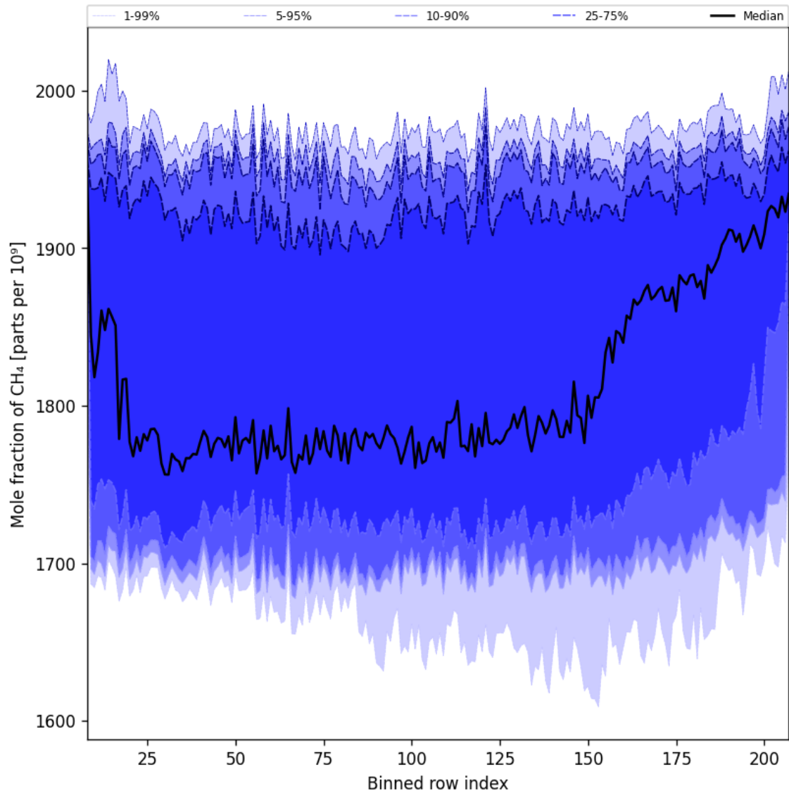
Figure 37: Along track statistics of “Mole fraction of CH 4 ” for 2025-11-25 to 2025-11-27
