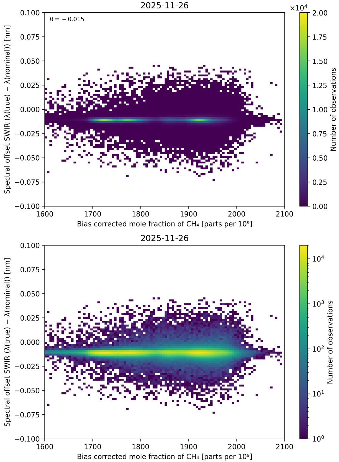
Figure 79: Scatter density plot of “Bias corrected mole fraction of CH 4 ” against “Spectral offset SWIR ( \lambda_{\text{true}} - \lambda_{\text{nominal}} )” for 2025-11-25 to 2025-11-27.
