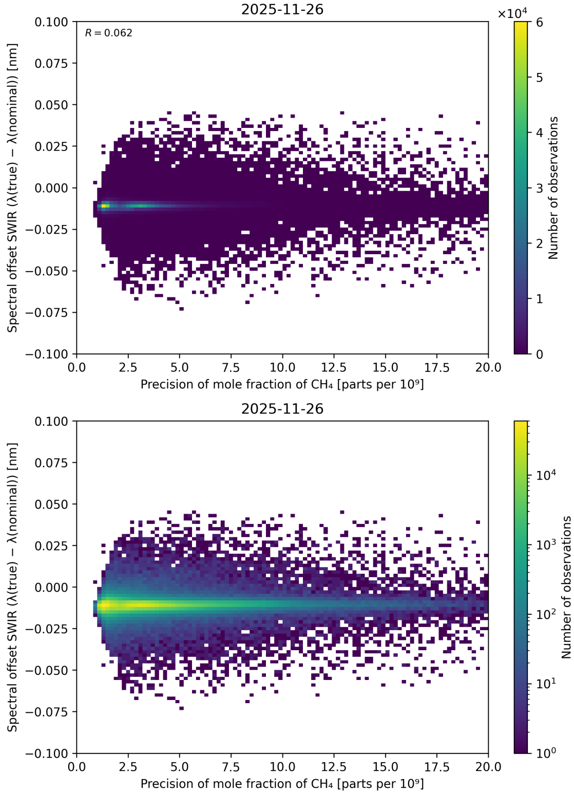
Figure 97: Scatter density plot of “Precision of mole fraction of CH 4 ” against “Spectral offset SWIR ( \lambda_{\text{true}} - \lambda_{\text{nominal}} )” for 2025-11-25 to 2025-11-27.
