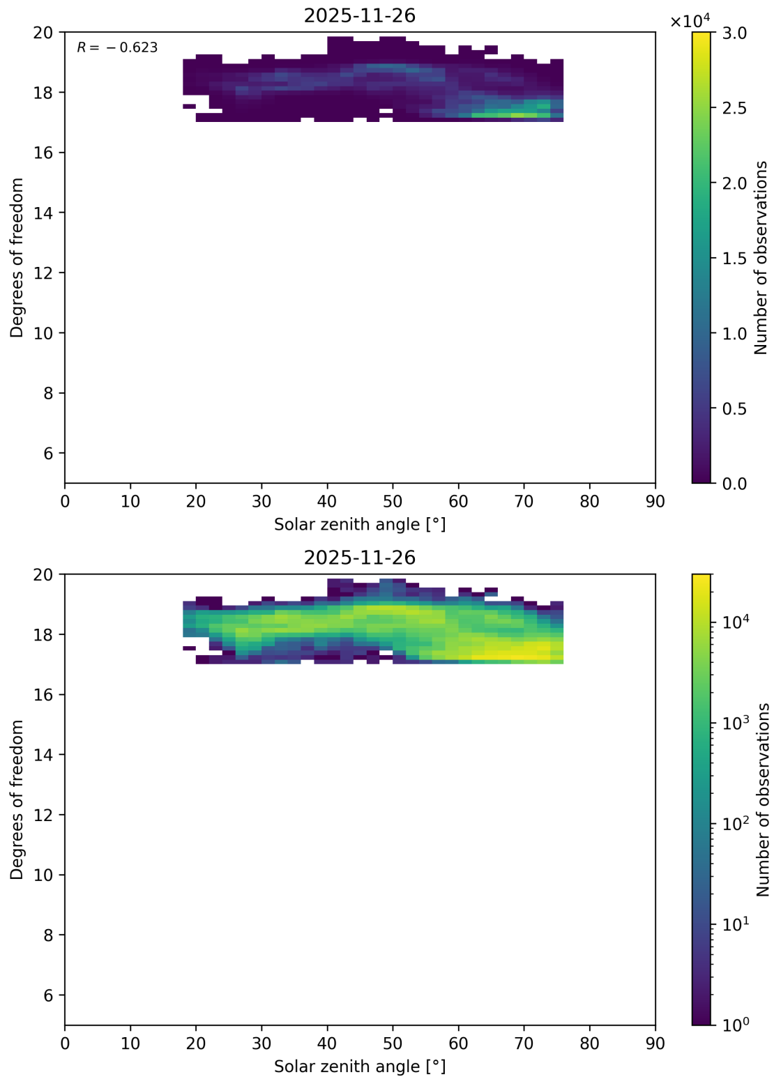
Figure 110: Scatter density plot of “Solar zenith angle” against “Degrees of freedom” for 2025-11-25 to 2025-11-27.
