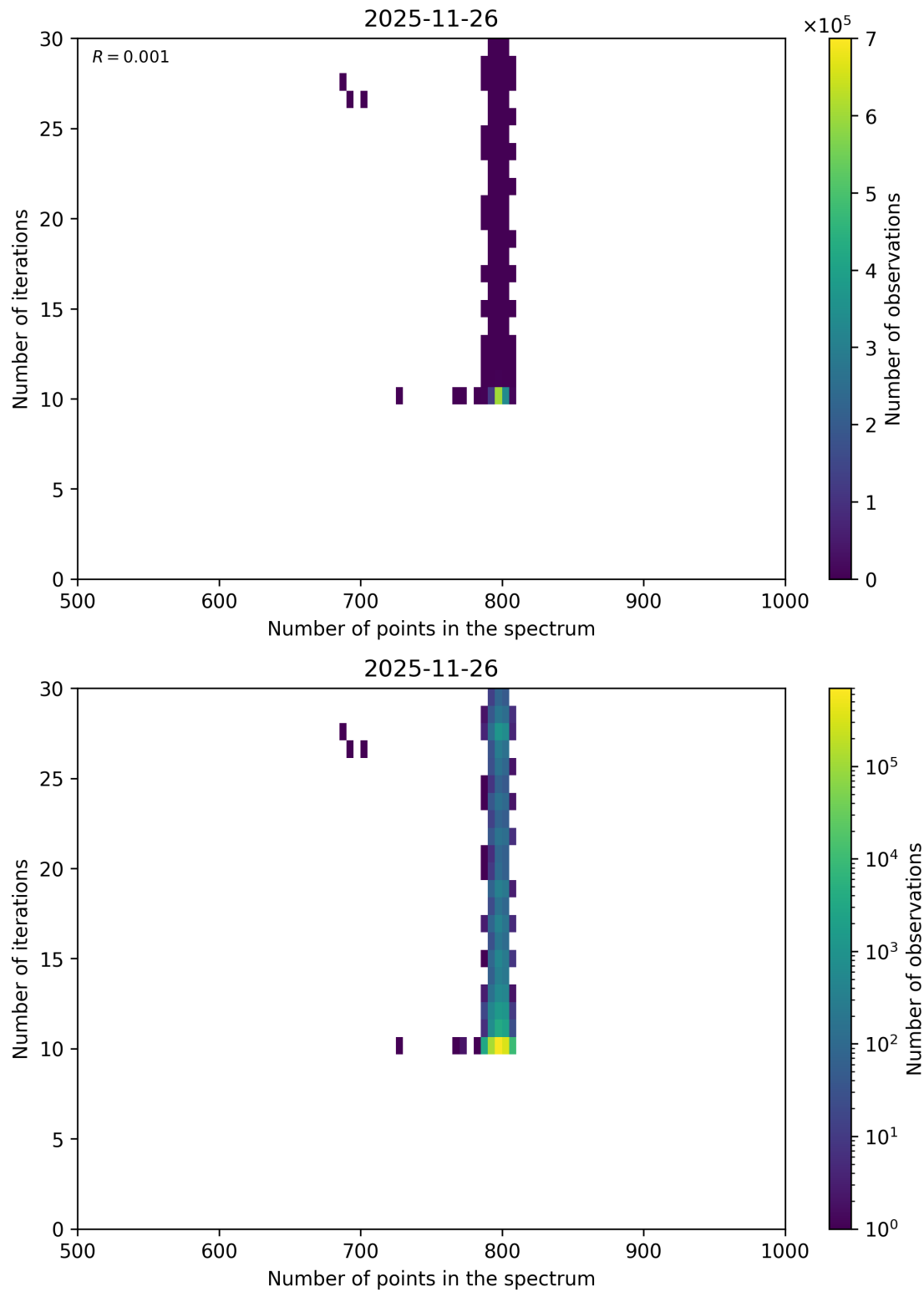
Figure 106: Scatter density plot of “Number of points in the spectrum” against “Number of iterations” for 2025-11-25 to 2025-11-27.
