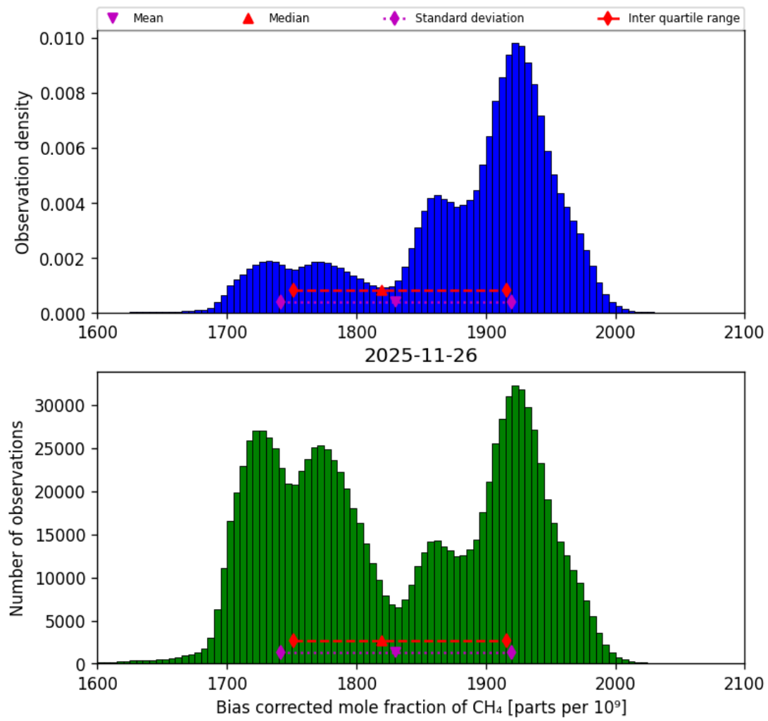
Figure 27: Histogram of “Bias corrected mole fraction of CH 4 ” for 2025-11-25 to 2025-11-27
