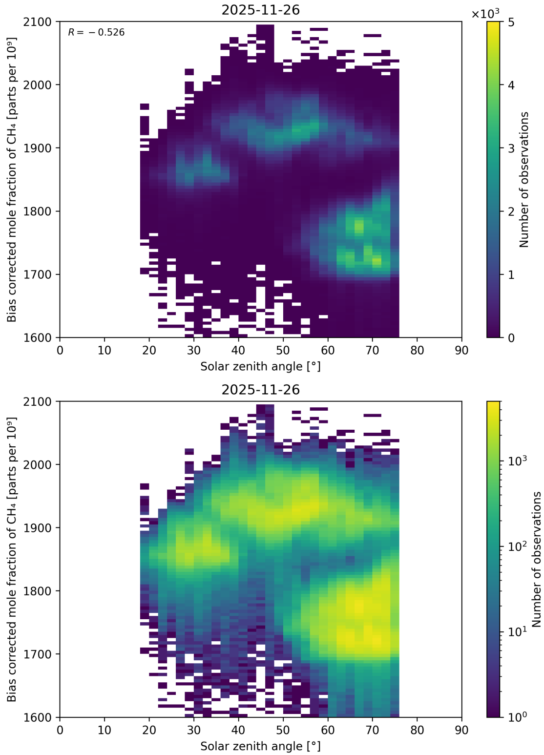
Figure 115: Scatter density plot of “Solar zenith angle” against “Bias corrected mole fraction of \text{CH}_4 ” for 2025-11-25 to 2025-11-27.
