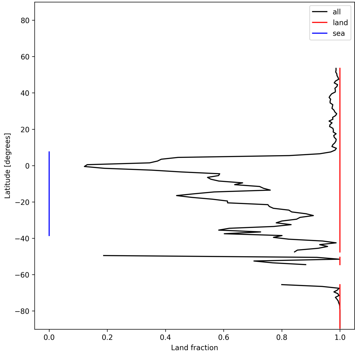
Figure 23: Zonal average of “Land fraction” for 2025-11-25 to 2025-11-27.
