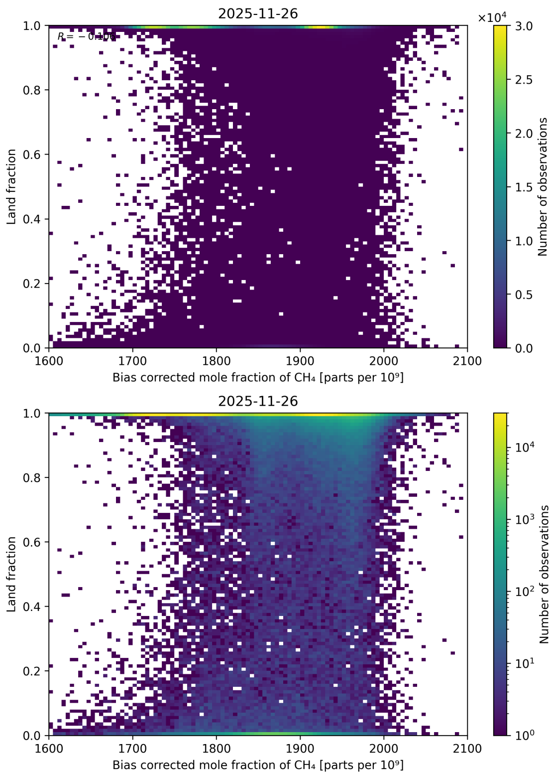
Figure 76: Scatter density plot of “Bias corrected mole fraction of CH 4 ” against “Land fraction” for 2025-11-25 to 2025-11-27.
