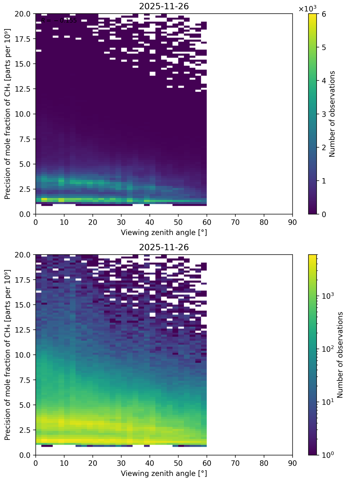
Figure 128: Scatter density plot of “Viewing zenith angle” against “Precision of mole fraction of CH 4 ” for 2025-11-25 to 2025-11-27.
