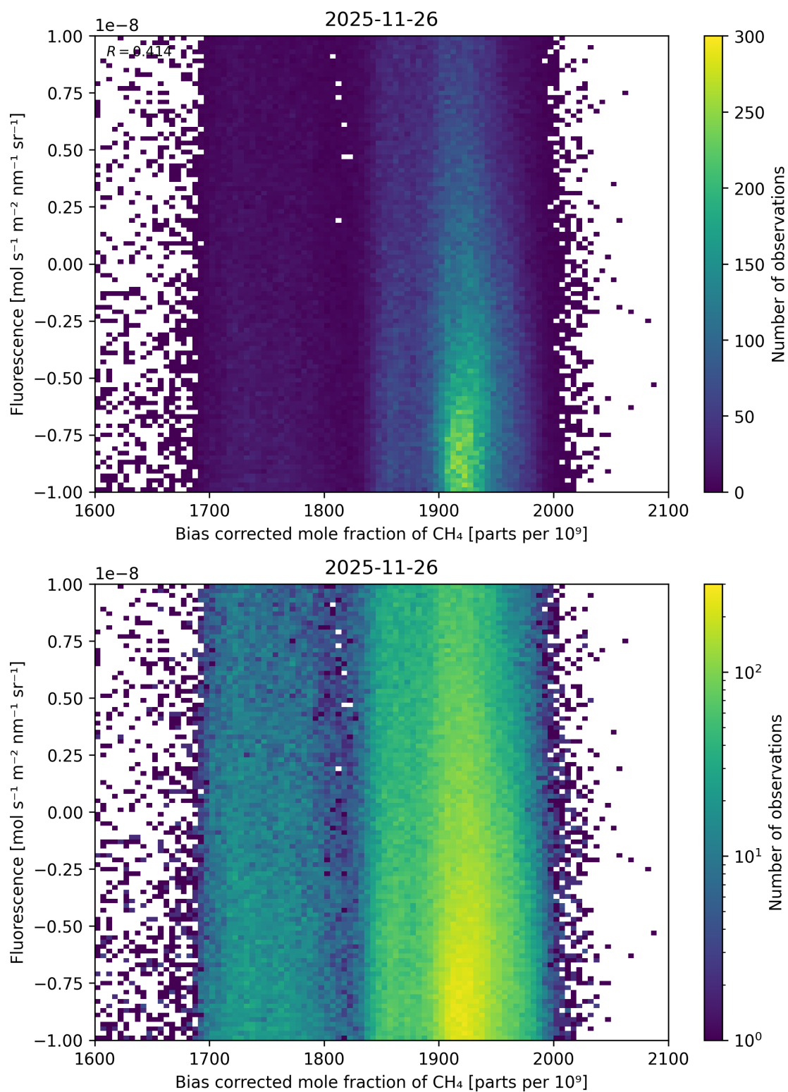
Figure 75: Scatter density plot of “Bias corrected mole fraction of \text{CH}_4 ” against “Fluorescence” for 2025-11-25 to 2025-11-27.
