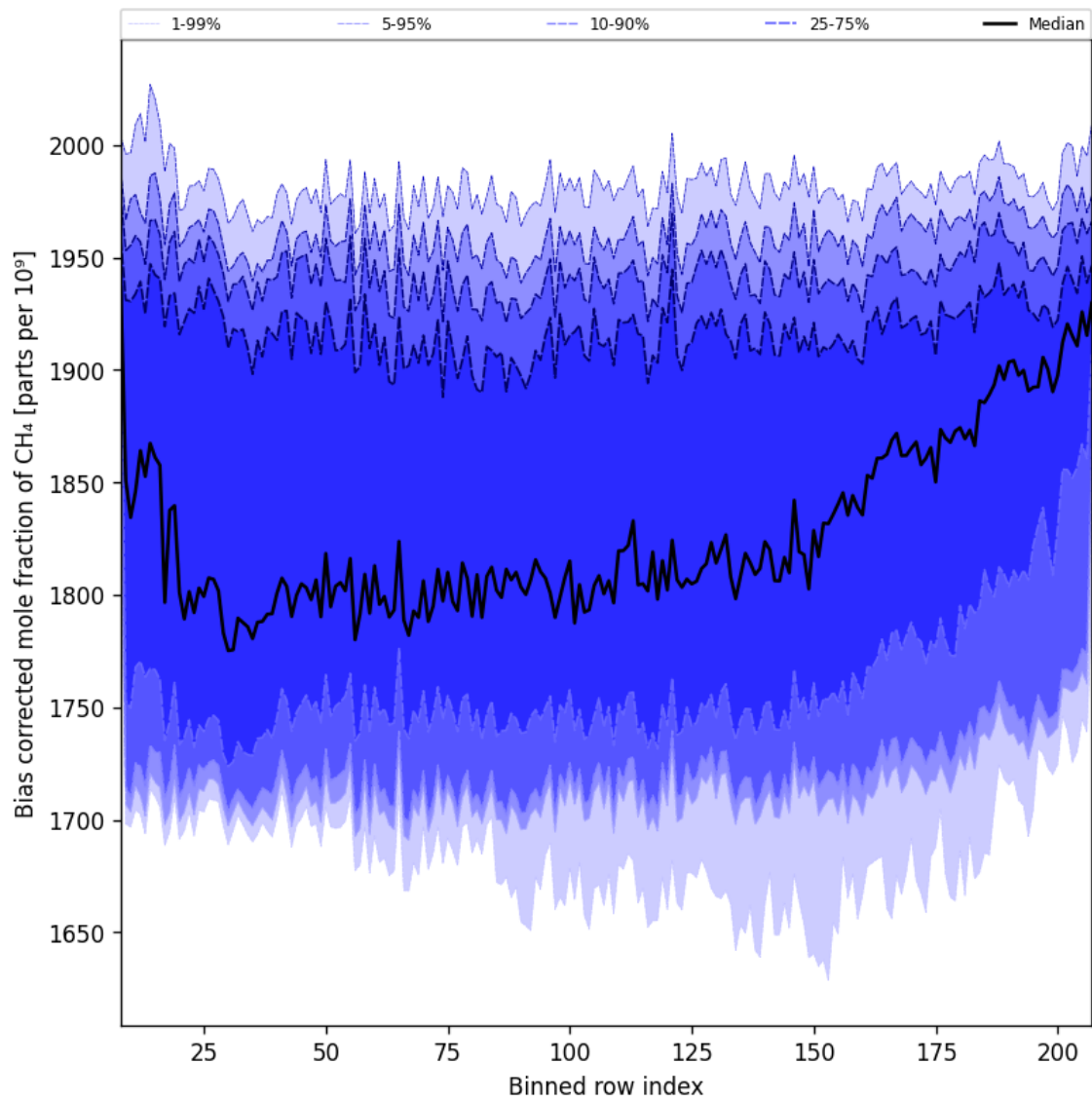
Figure 39: Along track statistics of “Bias corrected mole fraction of CH 4 ” for 2025-11-25 to 2025-11-27
