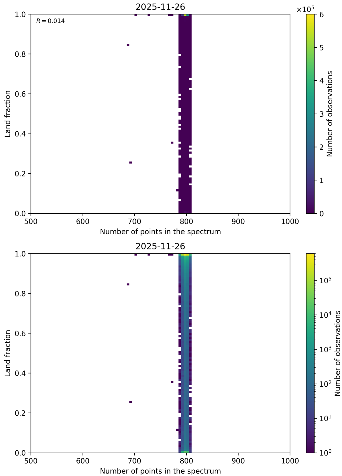
Figure 105: Scatter density plot of “Number of points in the spectrum” against “Land fraction” for 2025-11-25 to 2025-11-27.
