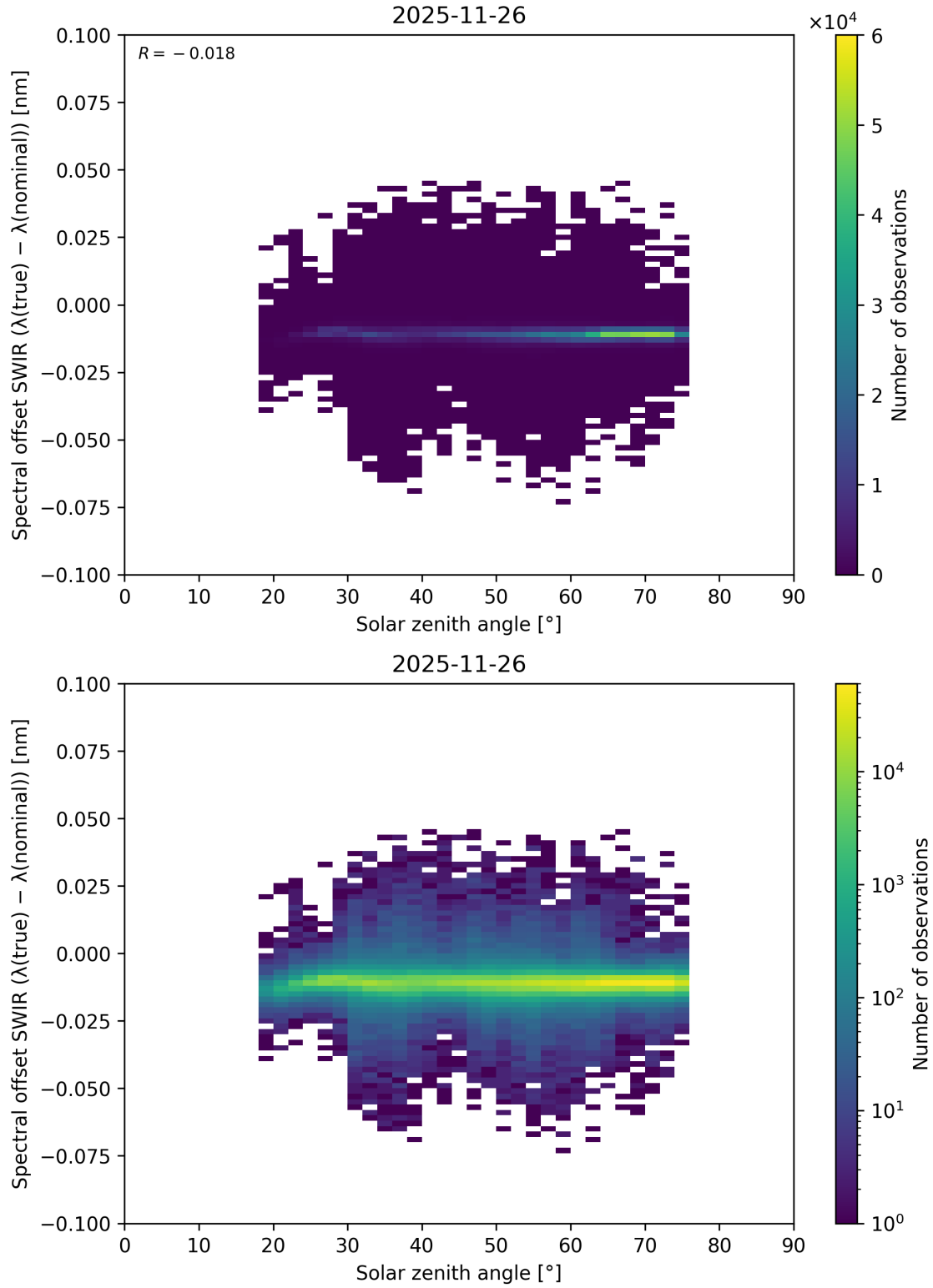
Figure 119: Scatter density plot of “Solar zenith angle” against “Spectral offset SWIR ( \lambda_{\text{true}} - \lambda_{\text{nominal}} )” for 2025-11-25 to 2025-11-27.
