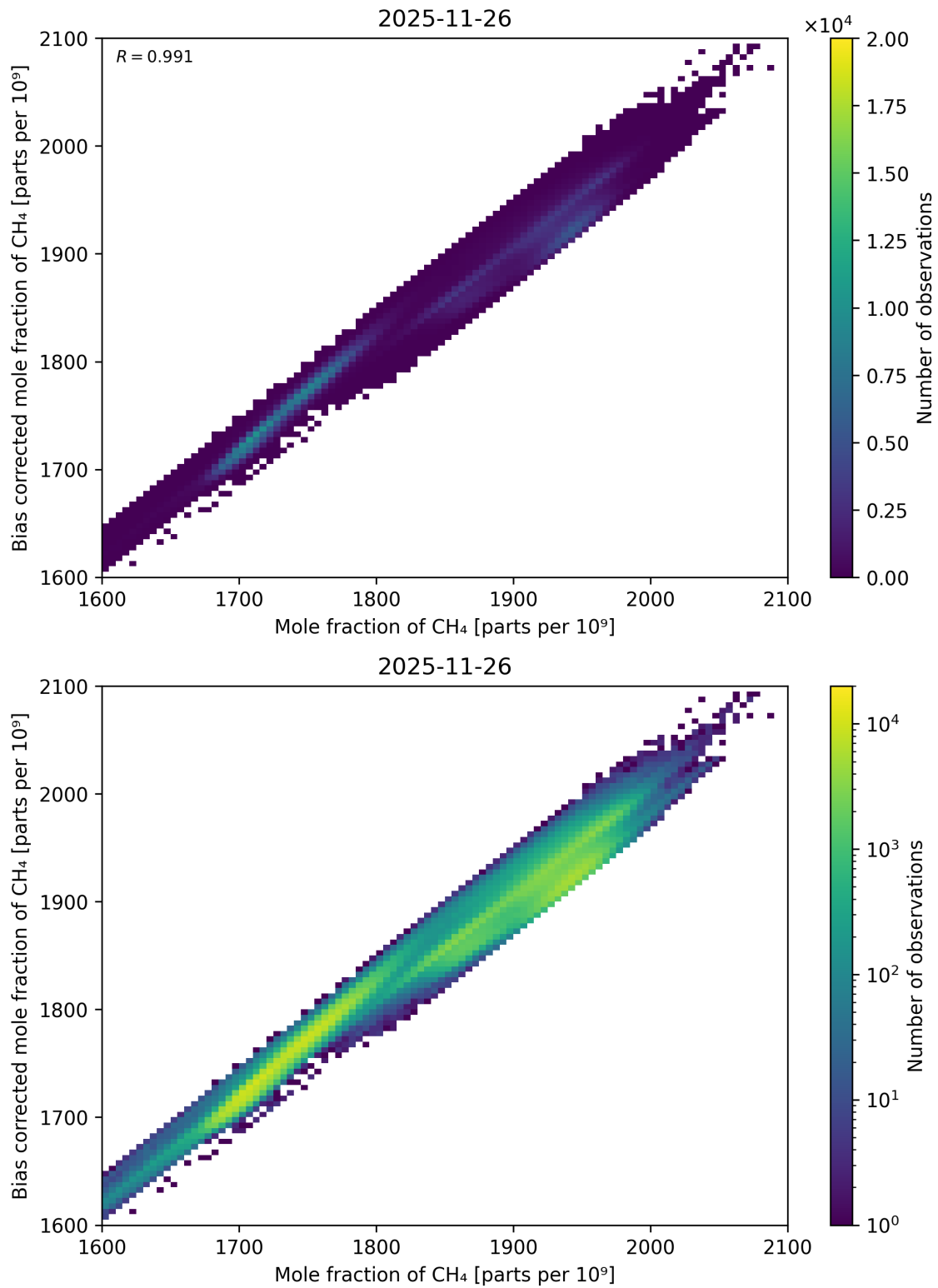
Figure 85: Scatter density plot of “Mole fraction of CH 4 ” against “Bias corrected mole fraction of CH 4 ” for 2025-11-25 to 2025-11-27.
