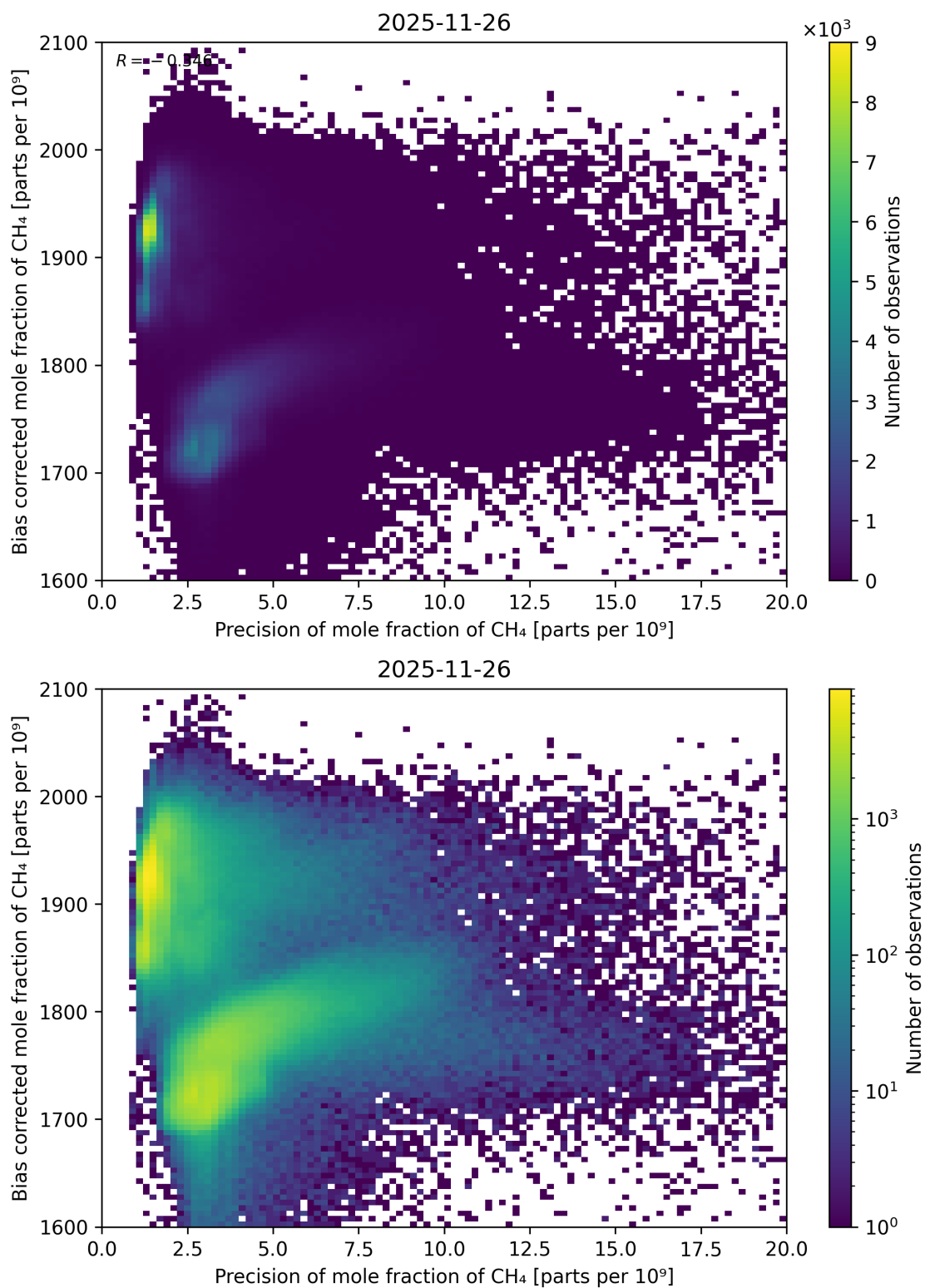
Figure 94: Scatter density plot of “Precision of mole fraction of CH 4 ” against “Bias corrected mole fraction of CH 4 ” for 2025-11-25 to 2025-11-27.
