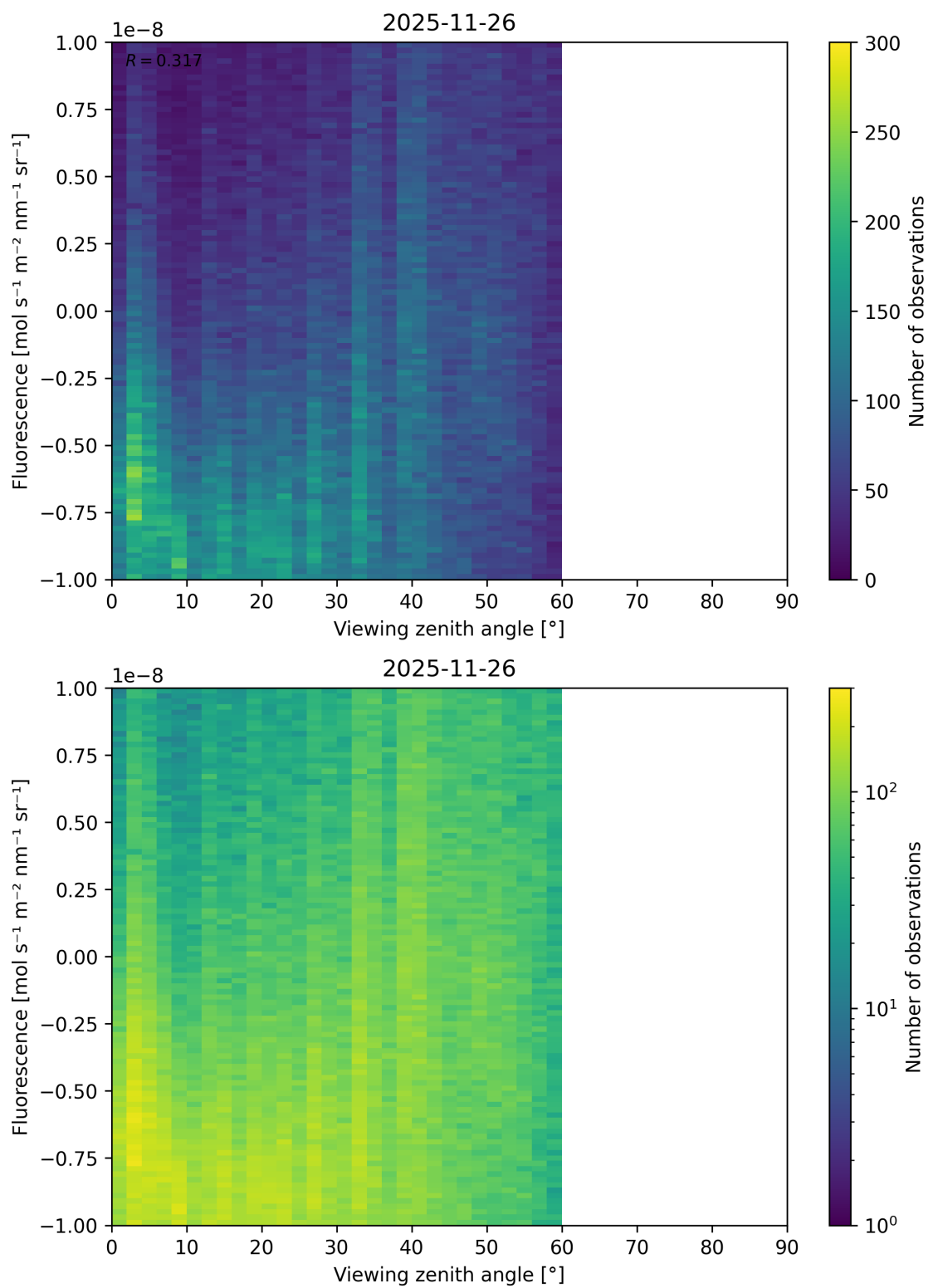
Figure 123: Scatter density plot of “Viewing zenith angle” against “Fluorescence” for 2025-11-25 to 2025-11-27.
