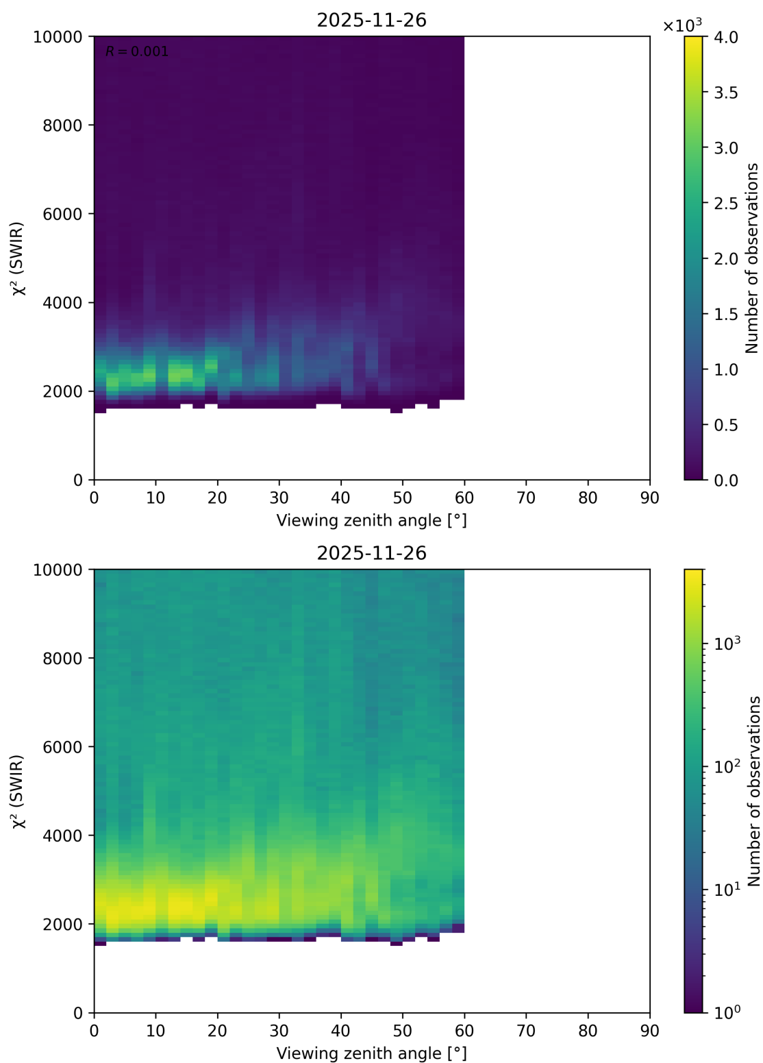
Figure 121: Scatter density plot of “Viewing zenith angle” against “ \chi^2 (SWIR)” for 2025-11-25 to 2025-11-27.
