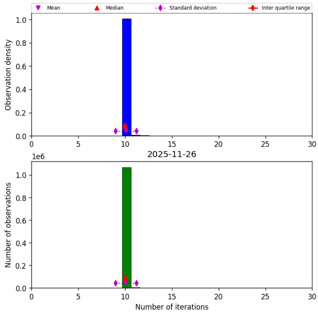
Figure 33: Histogram of “Number of iterations” for 2025-11-25 to 2025-11-27
