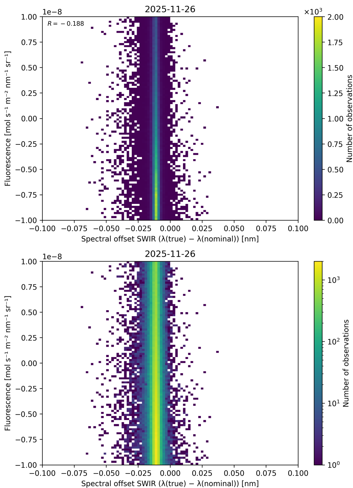
Figure 136: Scatter density plot of “Spectral offset SWIR ( \lambda_{\text{true}} - \lambda_{\text{nominal}} )” against “Fluorescence” for 2025-11-25 to 2025-11-27.
