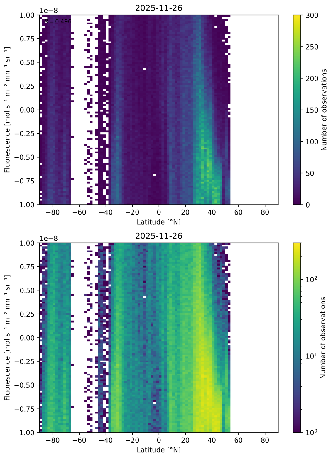
Figure 64: Scatter density plot of “Latitude” against “Fluorescence” for 2025-11-25 to 2025-11-27.
