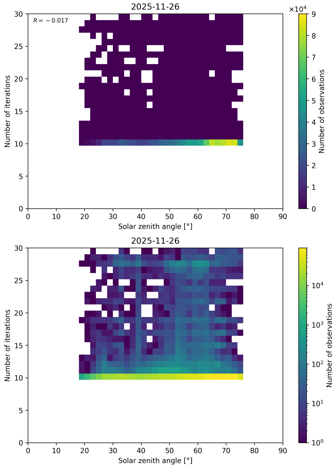
Figure 117: Scatter density plot of “Solar zenith angle” against “Number of iterations” for 2025-11-25 to 2025-11-27.
