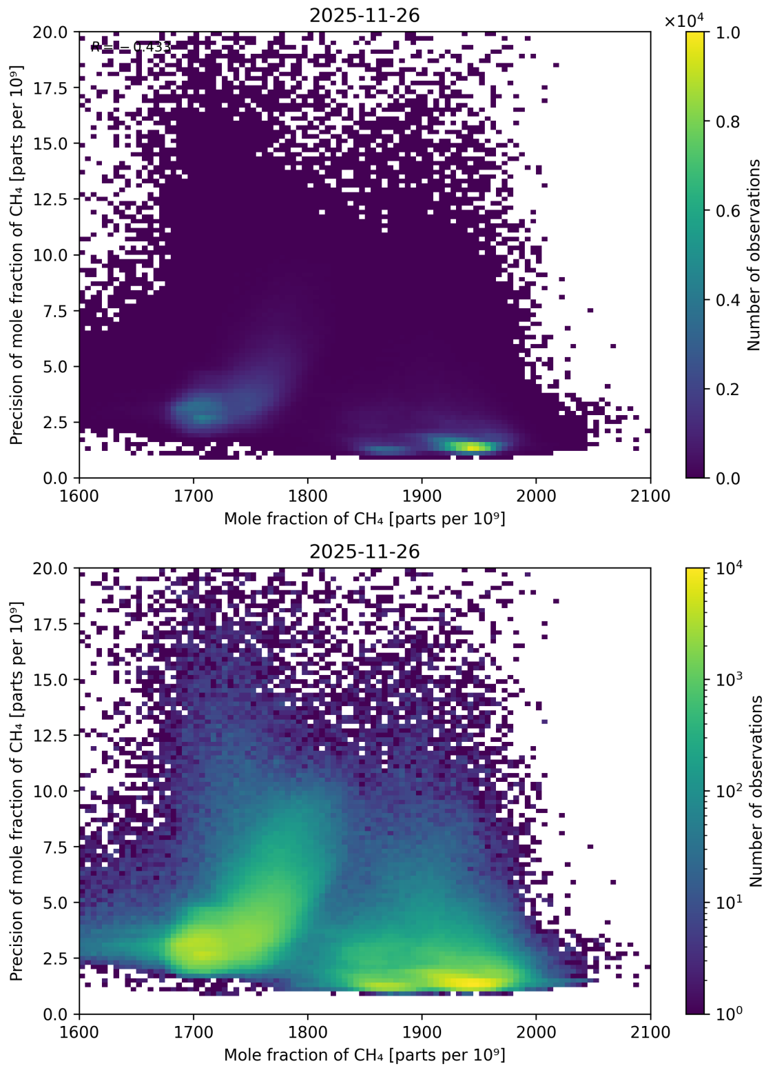
Figure 86: Scatter density plot of “Mole fraction of CH 4 ” against “Precision of mole fraction of CH 4 ” for 2025-11-25 to 2025-11-27.
