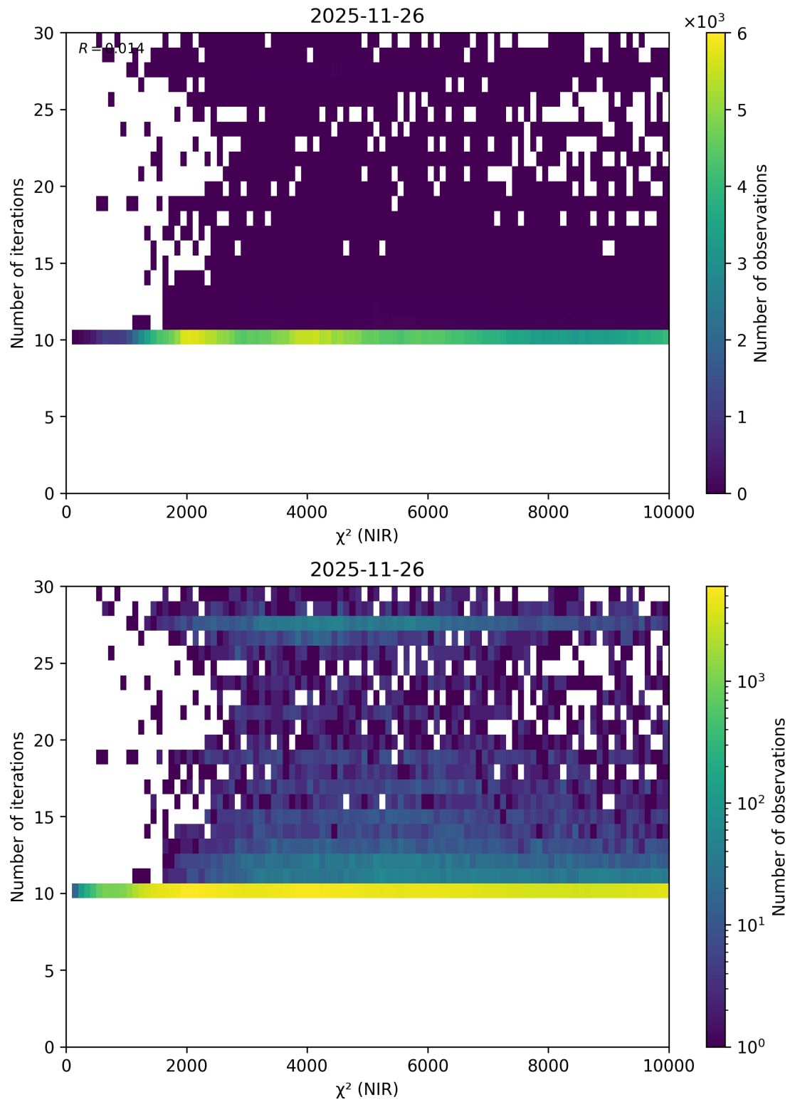
Figure 51: Scatter density plot of “ \chi^2 (NIR)” against “Number of iterations” for 2025-11-25 to 2025-11-27.
