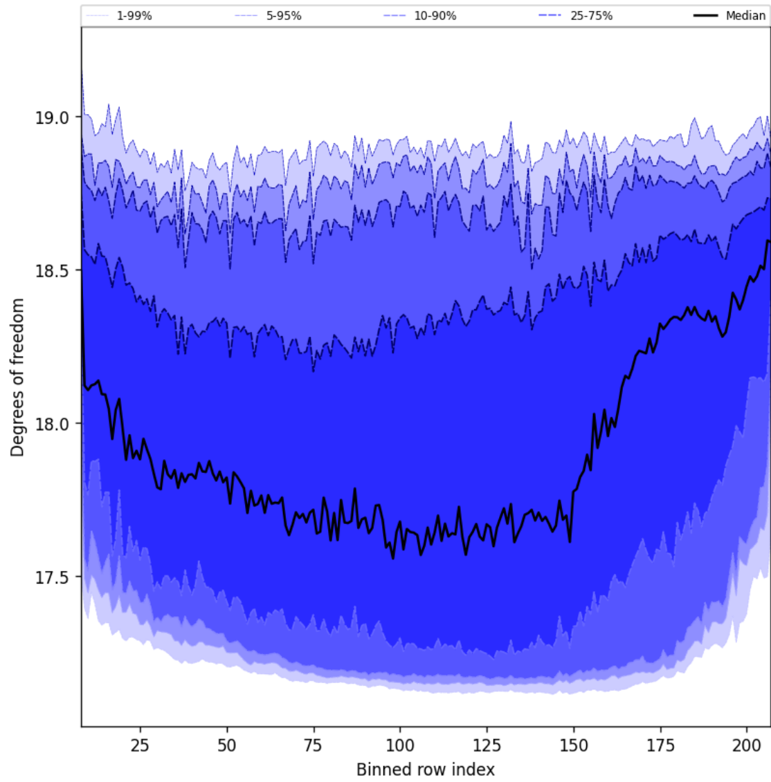
Figure 44: Along track statistics of “Degrees of freedom” for 2025-11-25 to 2025-11-27
