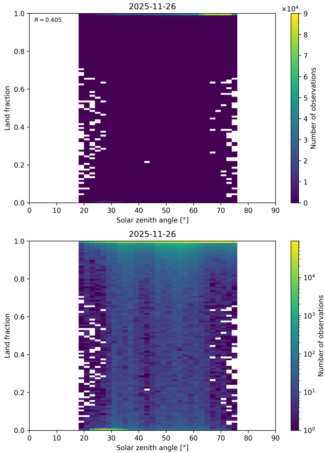
Figure 112: Scatter density plot of “Solar zenith angle” against “Land fraction” for 2025-11-25 to 2025-11-27.
