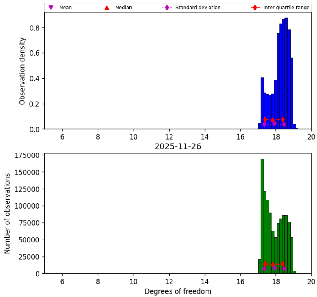
Figure 32: Histogram of “Degrees of freedom” for 2025-11-25 to 2025-11-27
