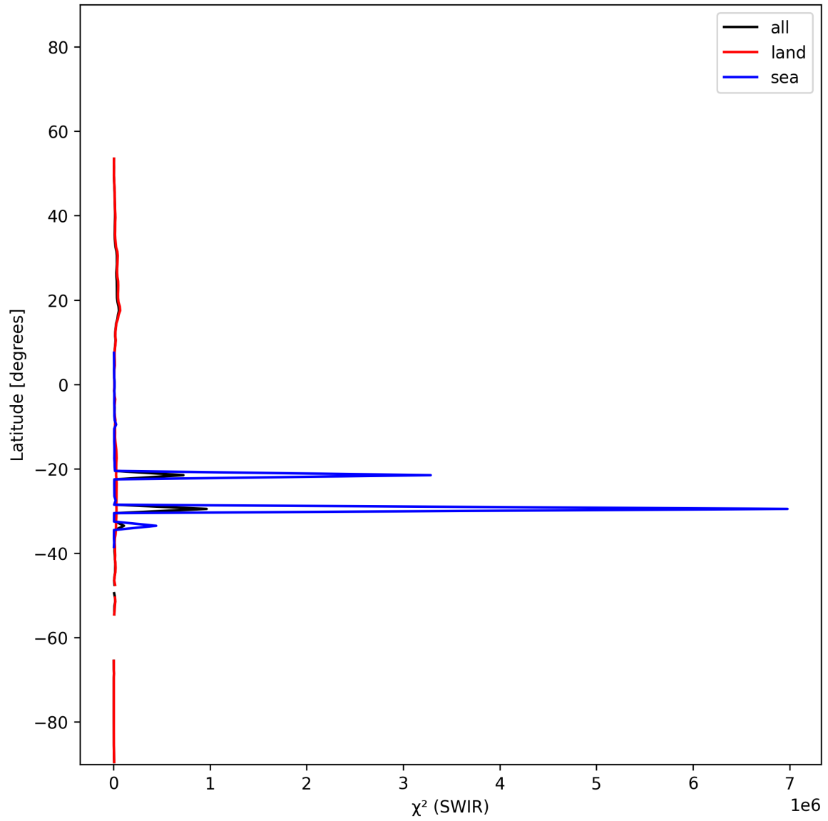
Figure 18: Zonal average of “ \chi^2 (SWIR)” for 2025-11-25 to 2025-11-27.
