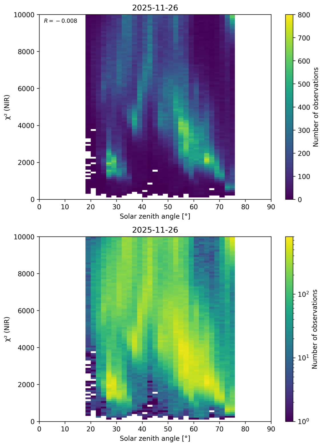
Figure 108: Scatter density plot of “Solar zenith angle” against “ \chi^2 (NIR)” for 2025-11-25 to 2025-11-27.
