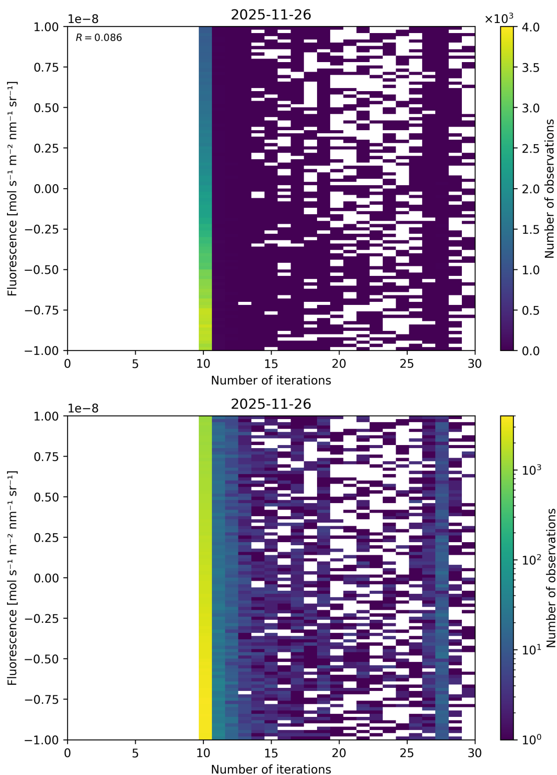
Figure 99: Scatter density plot of “Number of iterations” against “Fluorescence” for 2025-11-25 to 2025-11-27.
