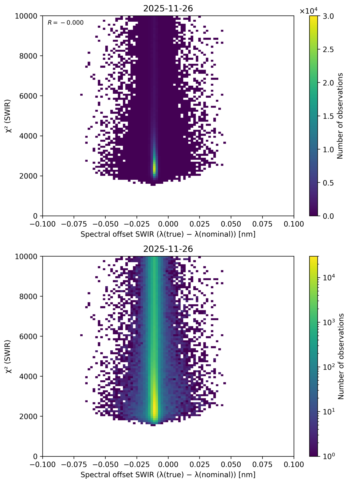
Figure 134: Scatter density plot of “Spectral offset SWIR ( \lambda_{\text{true}} - \lambda_{\text{nominal}} )” against “ \chi^2 (SWIR)” for 2025-11-25 to 2025-11-27.
