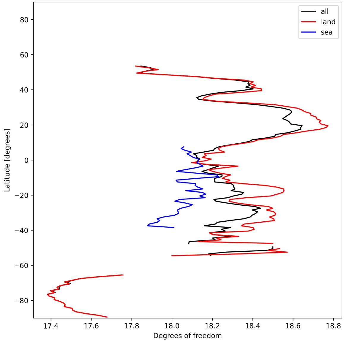
Figure 20: Zonal average of “Degrees of freedom” for 2025-11-25 to 2025-11-27.
