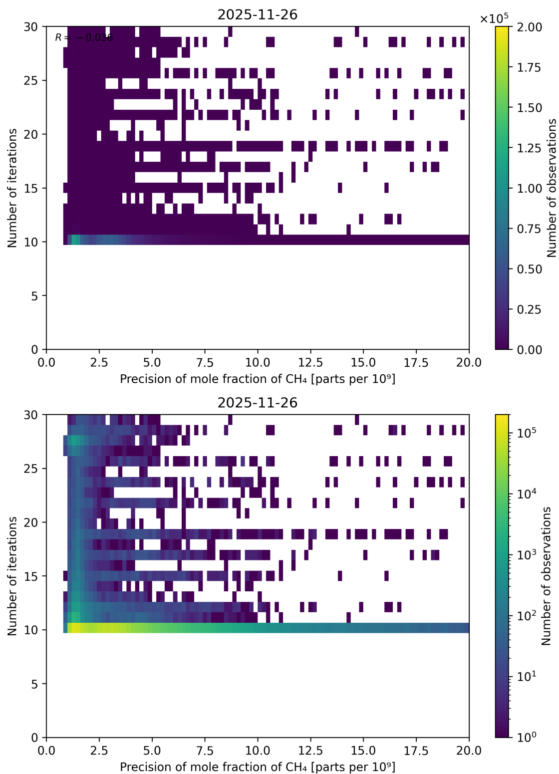
Figure 95: Scatter density plot of “Precision of mole fraction of \text{CH}_4 ” against “Number of iterations” for 2025-11-25 to 2025-11-27.
