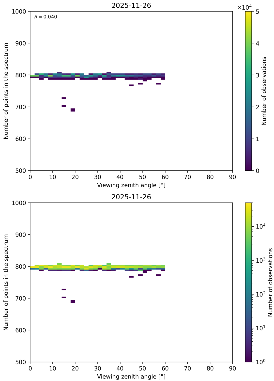
Figure 130: Scatter density plot of “Viewing zenith angle” against “Number of points in the spectrum” for 2025-11-25 to 2025-11-27.
