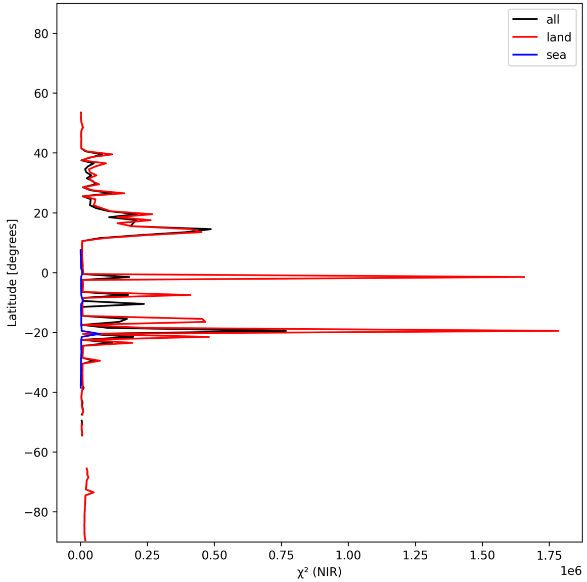
Figure 19: Zonal average of “ \chi^2 (NIR)” for 2025-11-25 to 2025-11-27.
