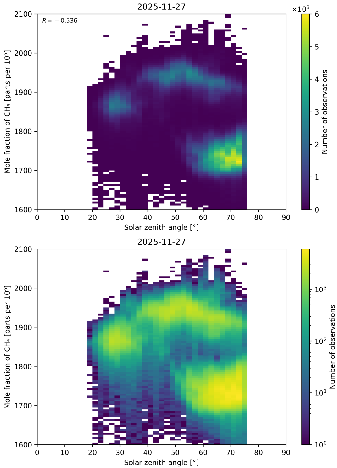
Figure 114: Scatter density plot of “Solar zenith angle” against “Mole fraction of CH 4 ” for 2025-11-26 to 2025-11-28.
