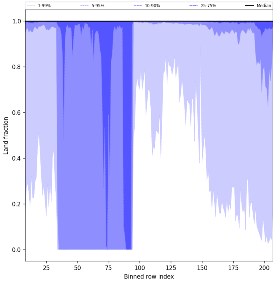
Figure 47: Along track statistics of “Land fraction” for 2025-11-26 to 2025-11-28
