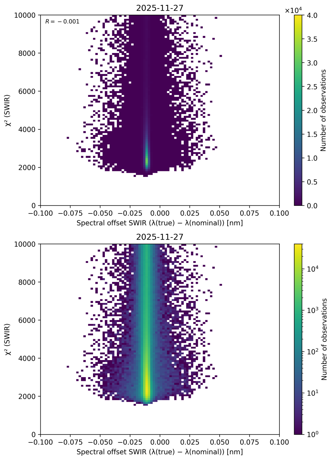
Figure 134: Scatter density plot of “Spectral offset SWIR ( \lambda_{\text{true}} - \lambda_{\text{nominal}} )” against “ \chi^2 (SWIR)” for 2025-11-26 to 2025-11-28.
