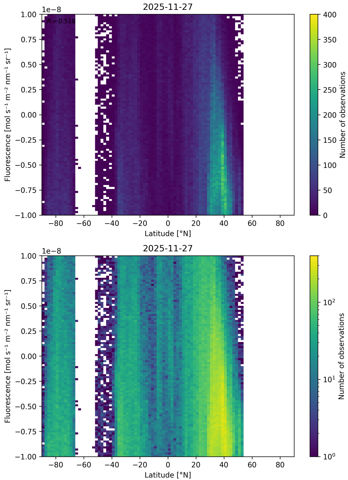
Figure 64: Scatter density plot of “Latitude” against “Fluorescence” for 2025-11-26 to 2025-11-28.
