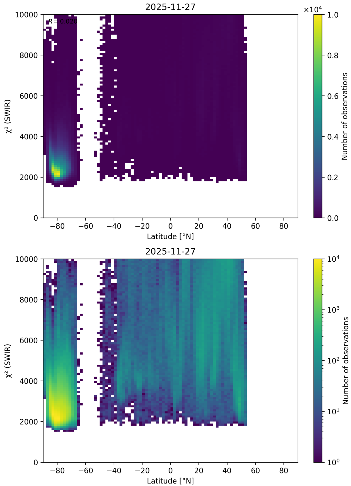
Figure 62: Scatter density plot of “Latitude” against “ \chi^2 (SWIR)” for 2025-11-26 to 2025-11-28.
