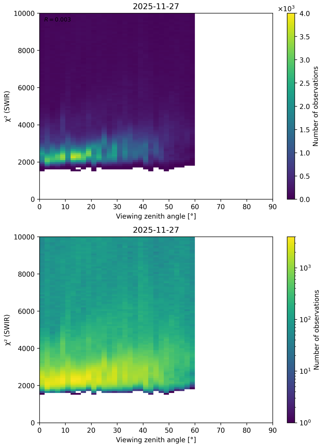
Figure 121: Scatter density plot of “Viewing zenith angle” against “ \chi^2 (SWIR)” for 2025-11-26 to 2025-11-28.
