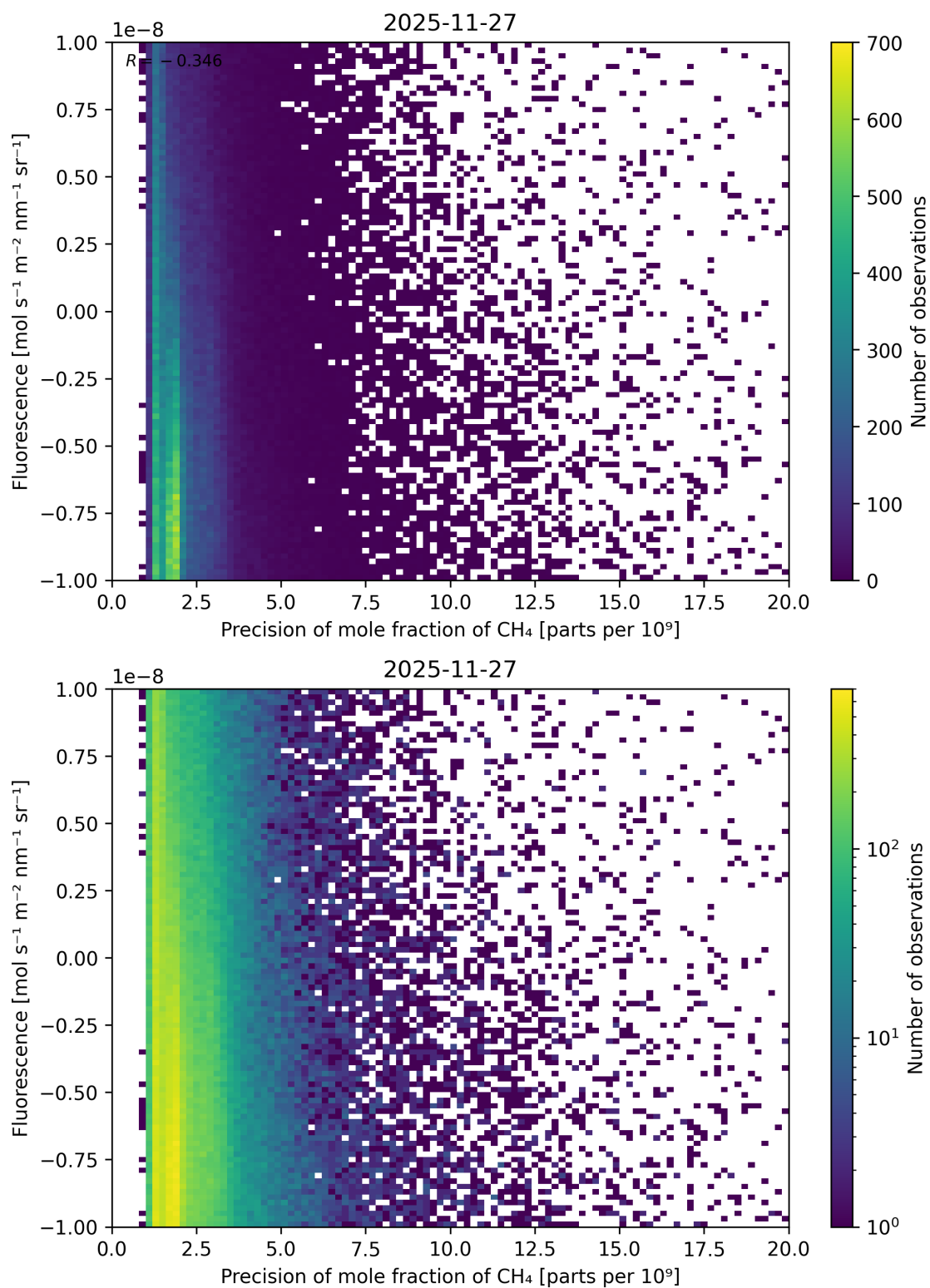
Figure 92: Scatter density plot of “Precision of mole fraction of CH 4 ” against “Fluorescence” for 2025-11-26 to 2025-11-28.
