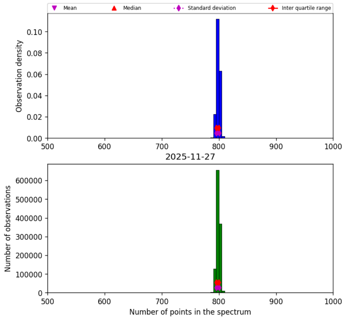
Figure 28: Histogram of “Number of points in the spectrum” for 2025-11-26 to 2025-11-28
