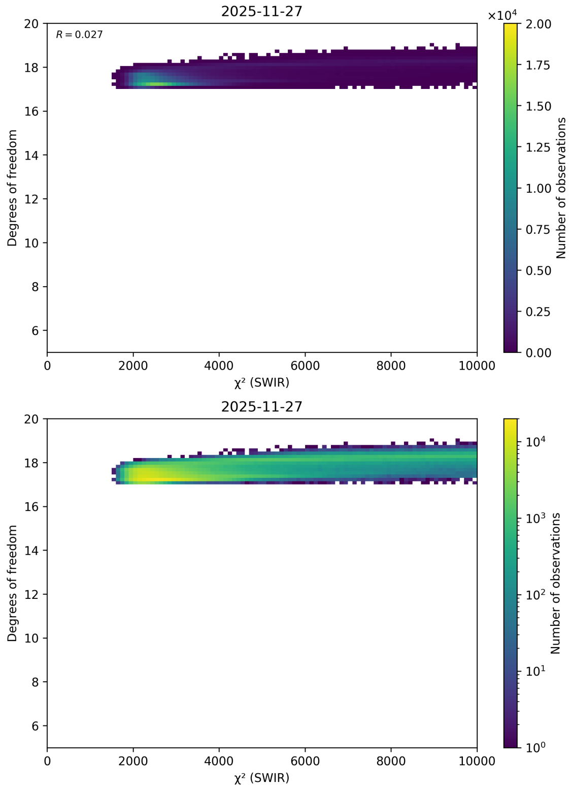
Figure 53: Scatter density plot of “ \chi^2 (SWIR)” against “Degrees of freedom” for 2025-11-26 to 2025-11-28.
