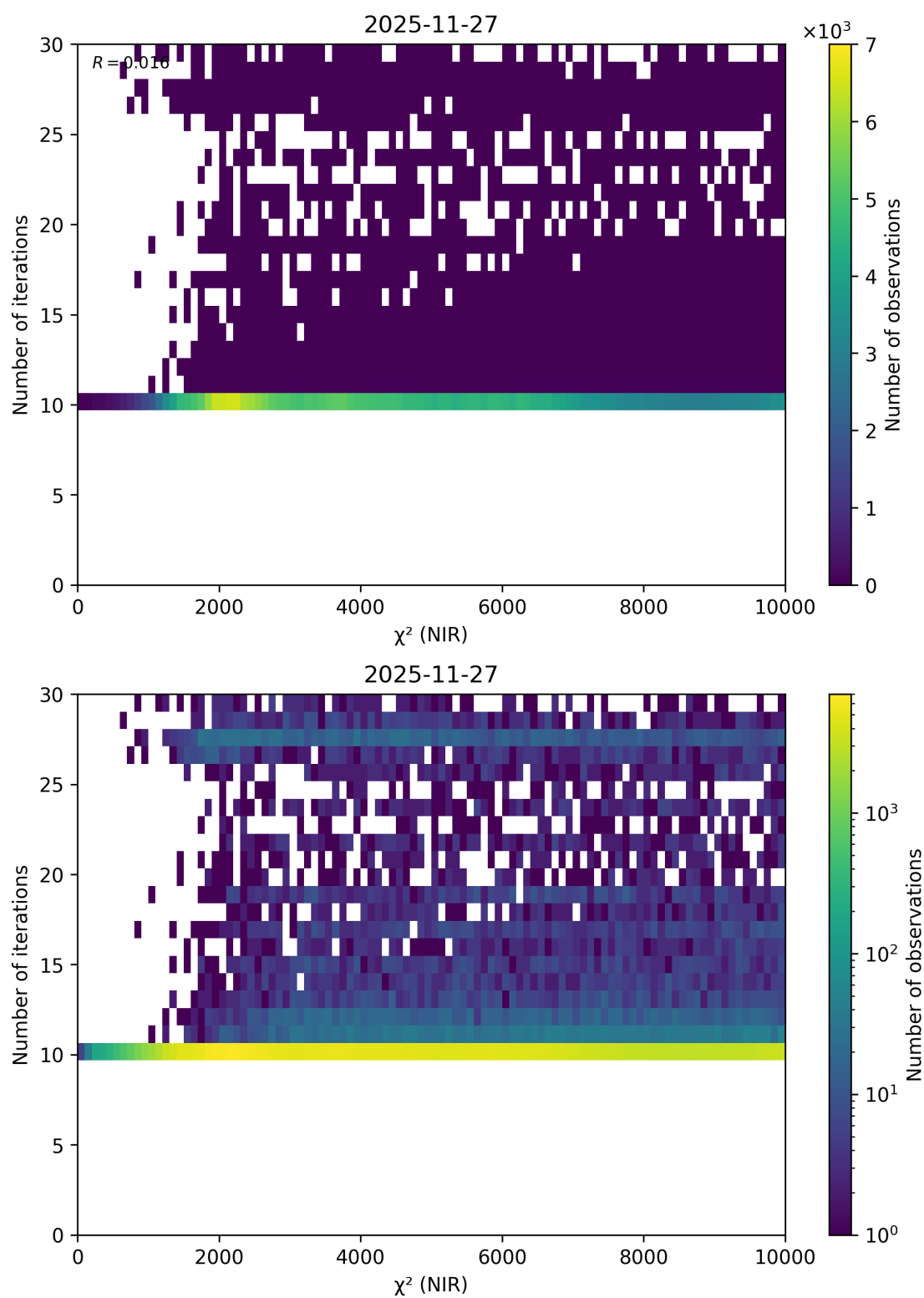
Figure 51: Scatter density plot of “ \chi^2 (NIR)” against “Number of iterations” for 2025-11-26 to 2025-11-28.
