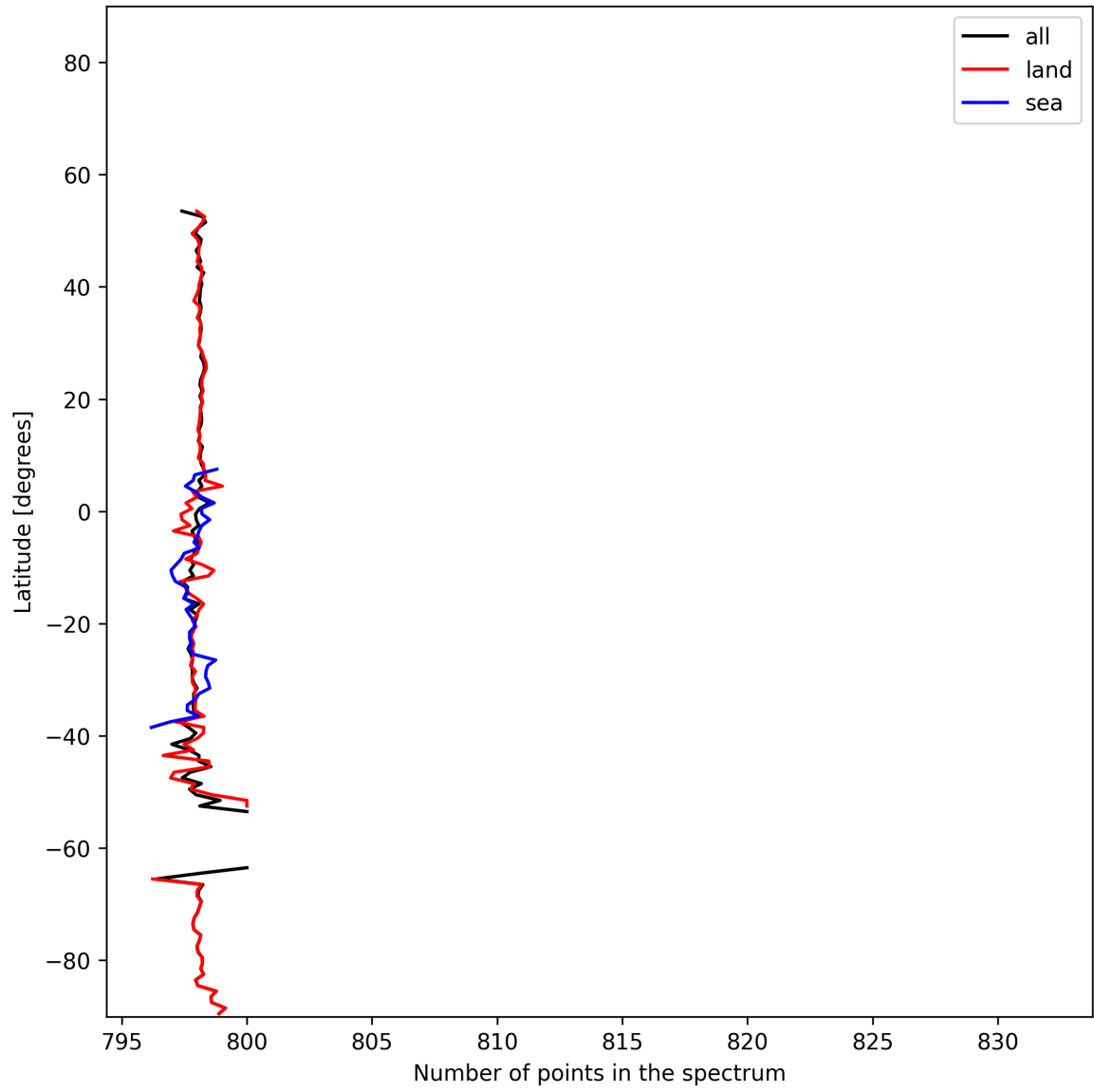
Figure 16: Zonal average of “Number of points in the spectrum” for 2025-11-26 to 2025-11-28.
