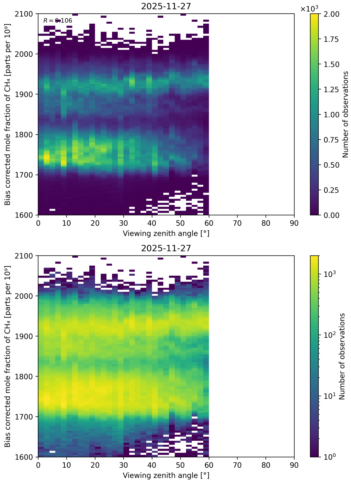
Figure 127: Scatter density plot of “Viewing zenith angle” against “Bias corrected mole fraction of CH 4 ” for 2025-11-26 to 2025-11-28.
