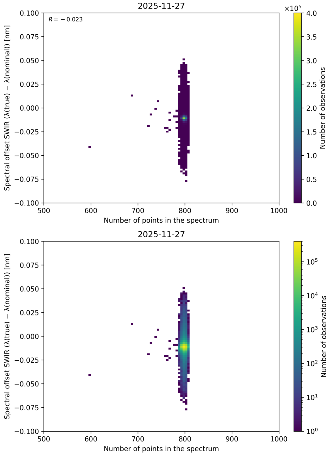
Figure 107: Scatter density plot of “Number of points in the spectrum” against “Spectral offset SWIR ( \lambda_{\text{true}} - \lambda_{\text{nominal}} )” for 2025-11-26 to 2025-11-28.
