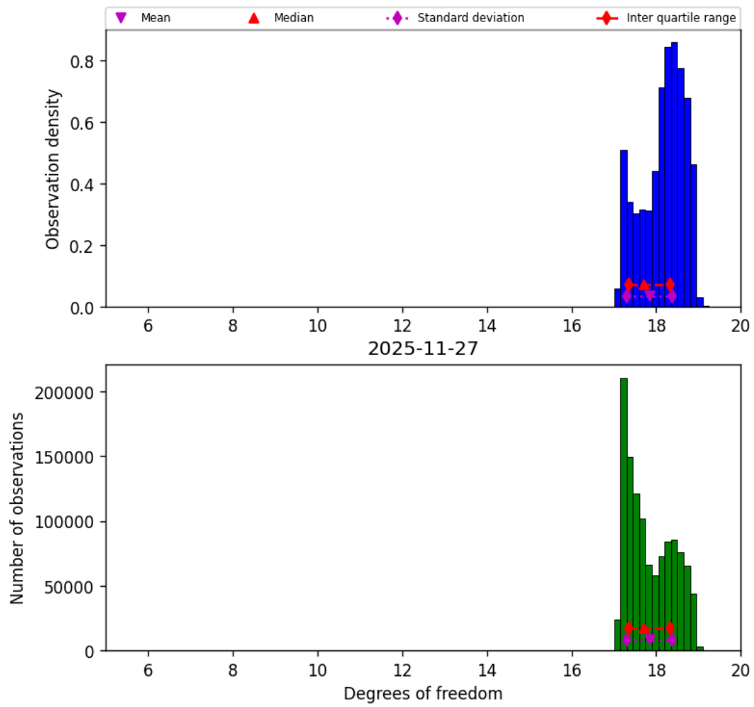
Figure 32: Histogram of “Degrees of freedom” for 2025-11-26 to 2025-11-28
