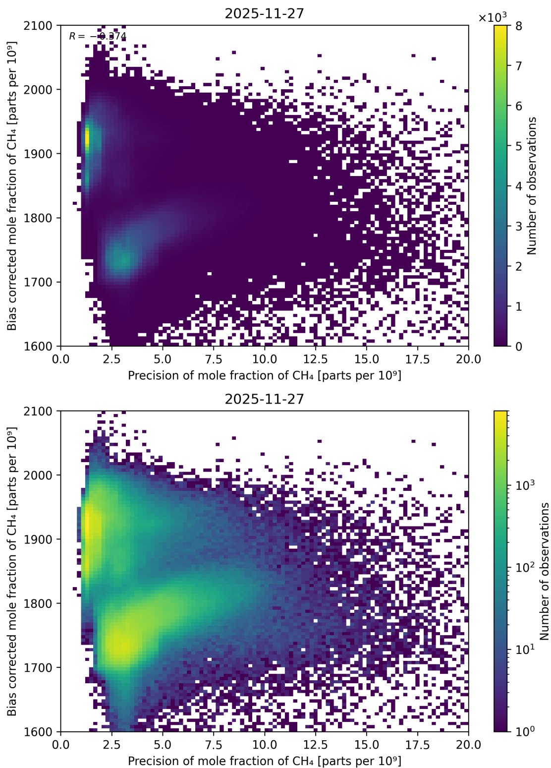
Figure 94: Scatter density plot of “Precision of mole fraction of CH 4 ” against “Bias corrected mole fraction of CH 4 ” for 2025-11-26 to 2025-11-28.
