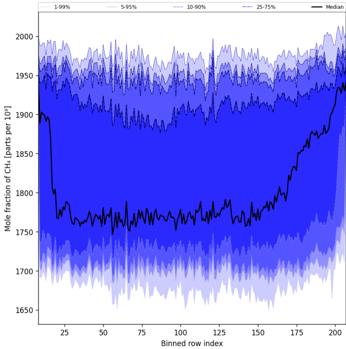
Figure 37: Along track statistics of “Mole fraction of CH 4 ” for 2025-11-26 to 2025-11-28
