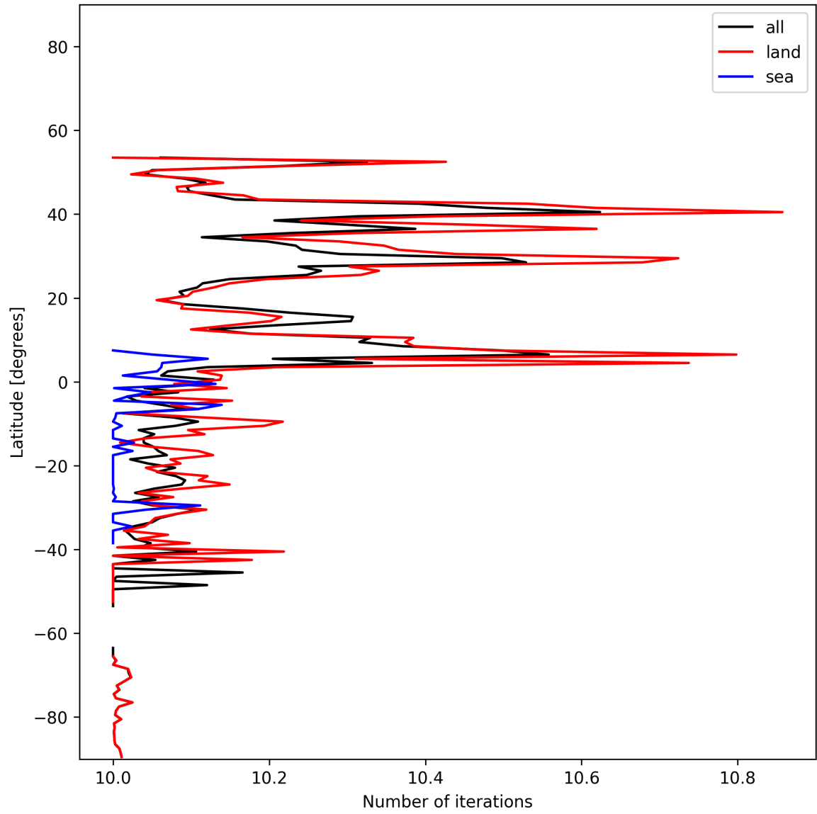
Figure 21: Zonal average of “Number of iterations” for 2025-11-26 to 2025-11-28.
