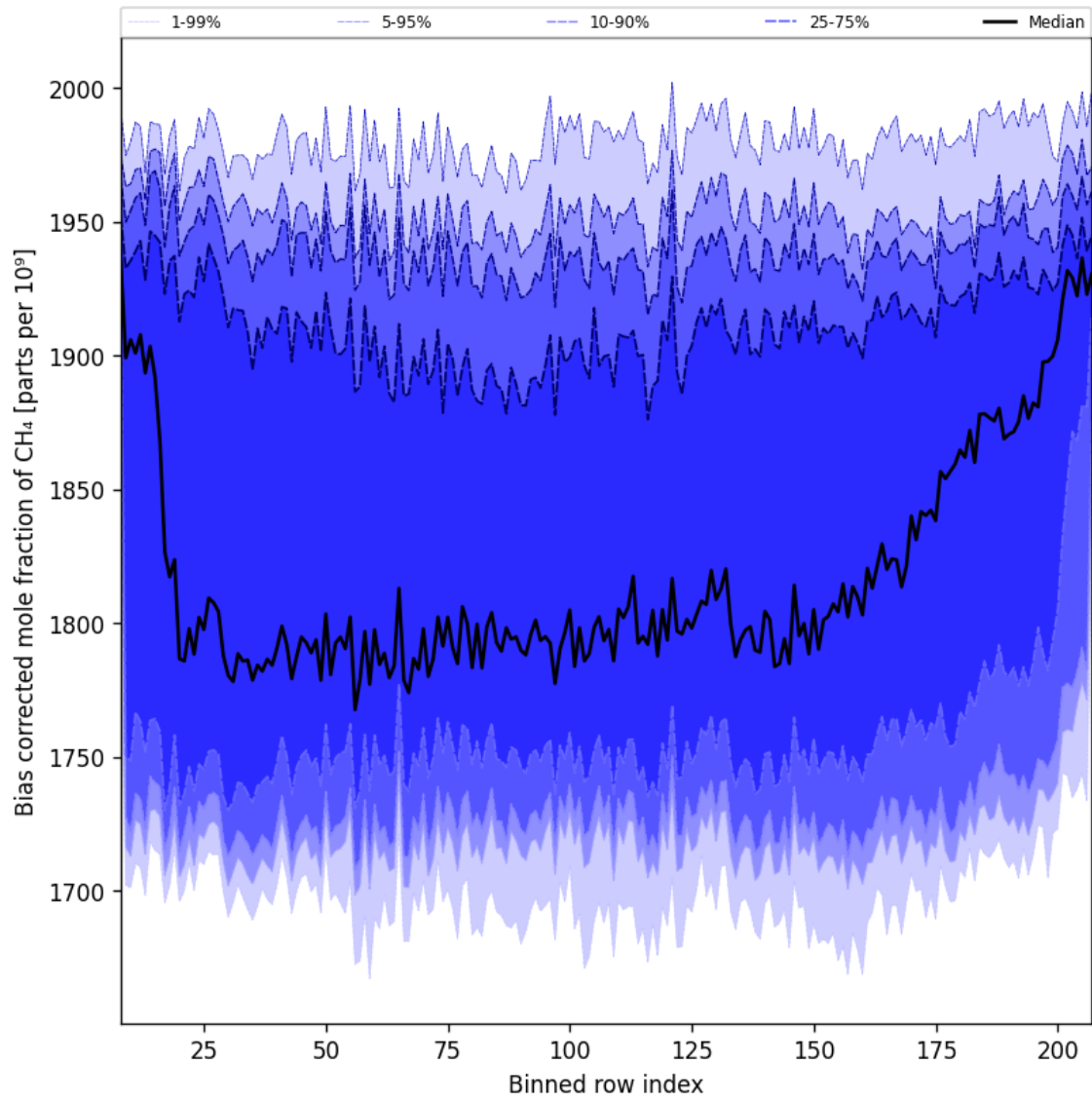
Figure 39: Along track statistics of “Bias corrected mole fraction of CH 4 ” for 2025-11-26 to 2025-11-28
