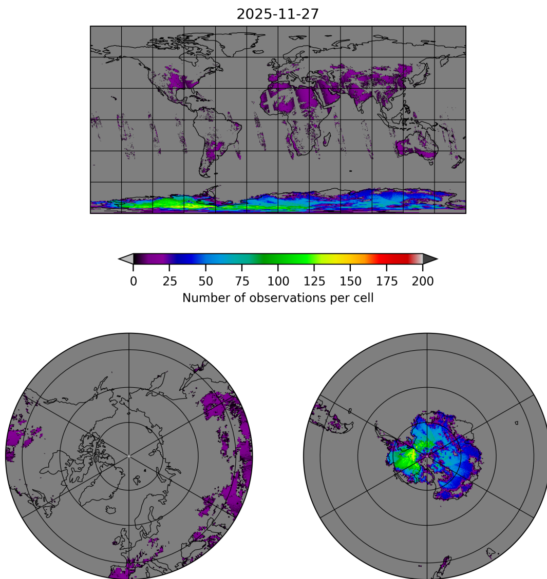
Figure 11: Map of the number of observations for 2025-11-26 to 2025-11-28
