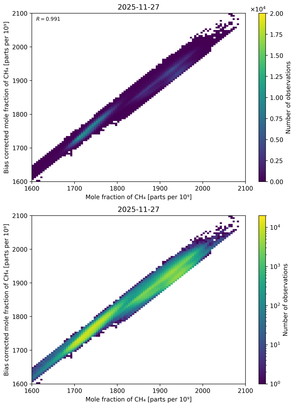
Figure 85: Scatter density plot of “Mole fraction of CH 4 ” against “Bias corrected mole fraction of CH 4 ” for 2025-11-26 to 2025-11-28.
