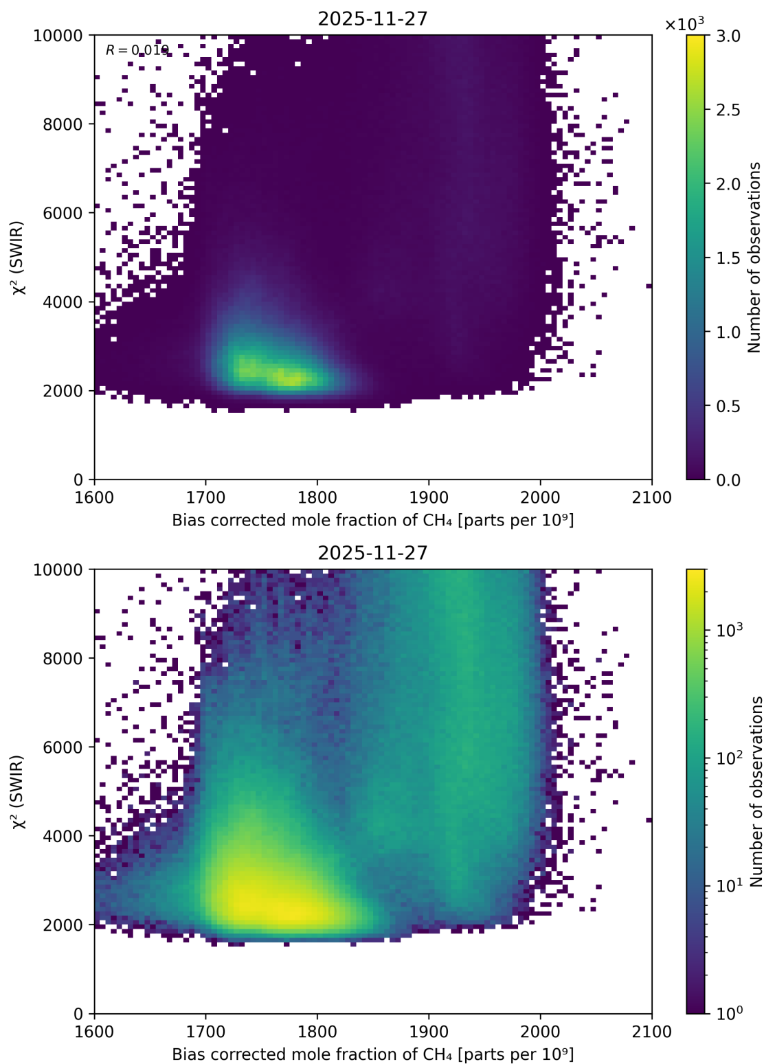
Figure 73: Scatter density plot of “Bias corrected mole fraction of \text{CH}_4 ” against “ \chi^2 (SWIR)” for 2025-11-26 to 2025-11-28.
