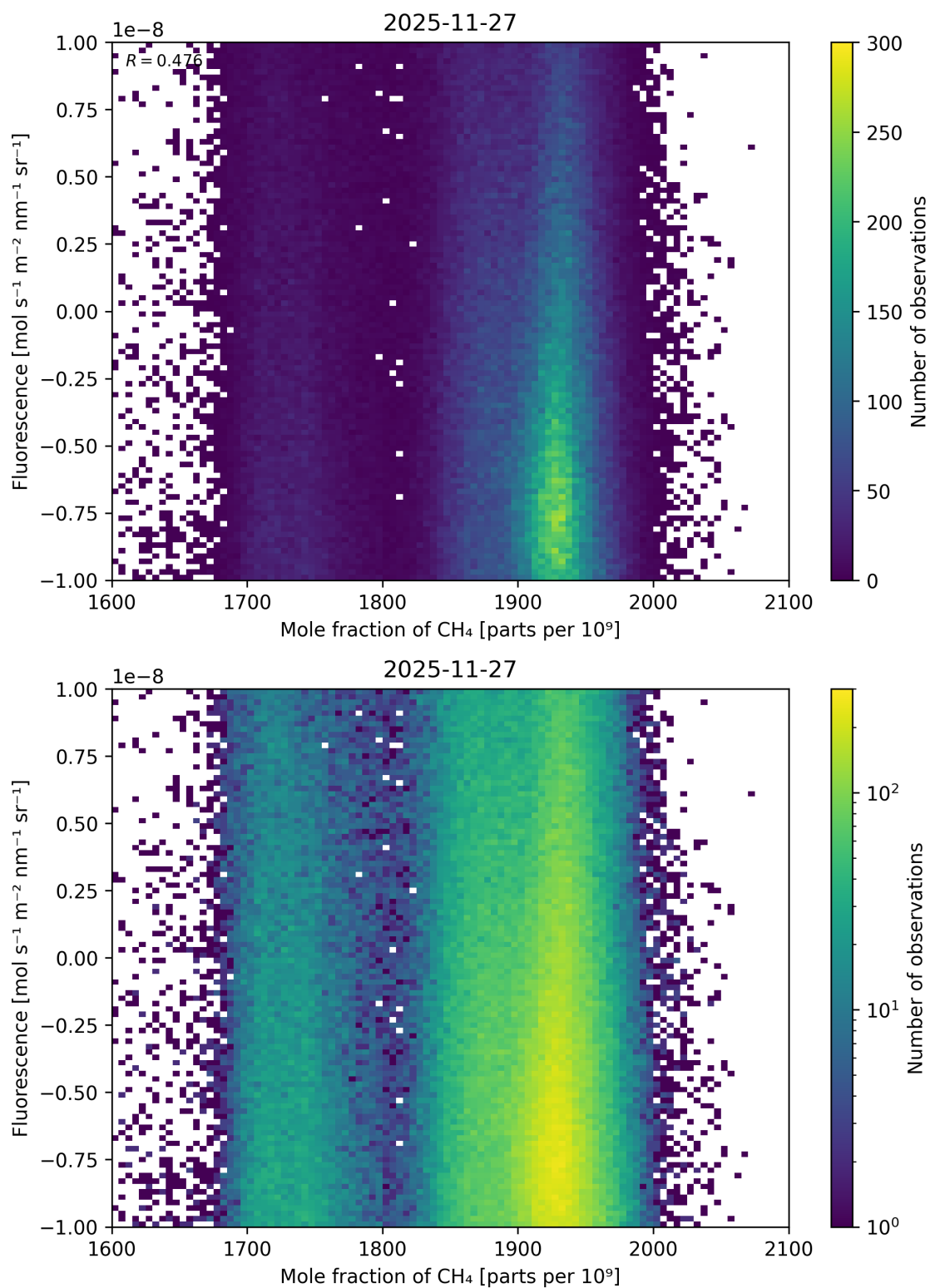
Figure 83: Scatter density plot of “Mole fraction of \text{CH}_4 ” against “Fluorescence” for 2025-11-26 to 2025-11-28.
