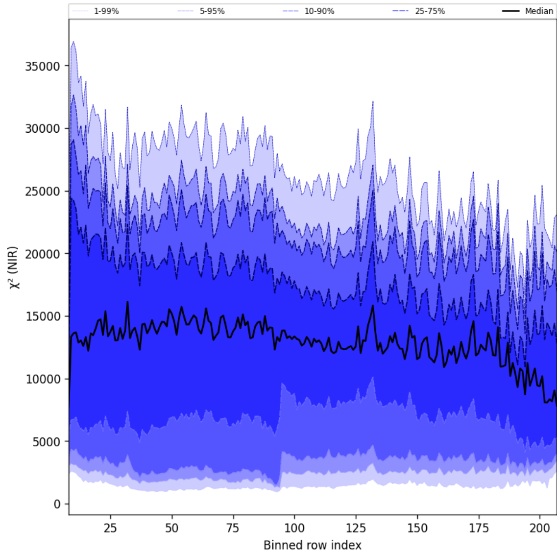
Figure 43: Along track statistics of “ \chi^2 (NIR)” for 2025-11-26 to 2025-11-28
