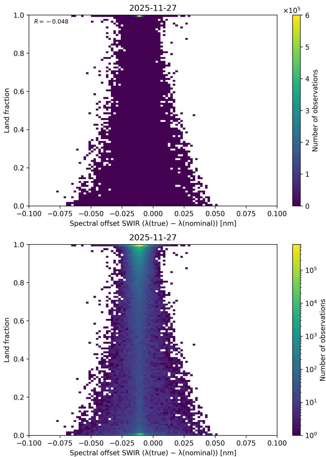
Figure 137: Scatter density plot of “Spectral offset SWIR ( \lambda_{\text{true}} - \lambda_{\text{nominal}} )” against “Land fraction” for 2025-11-26 to 2025-11-28.
