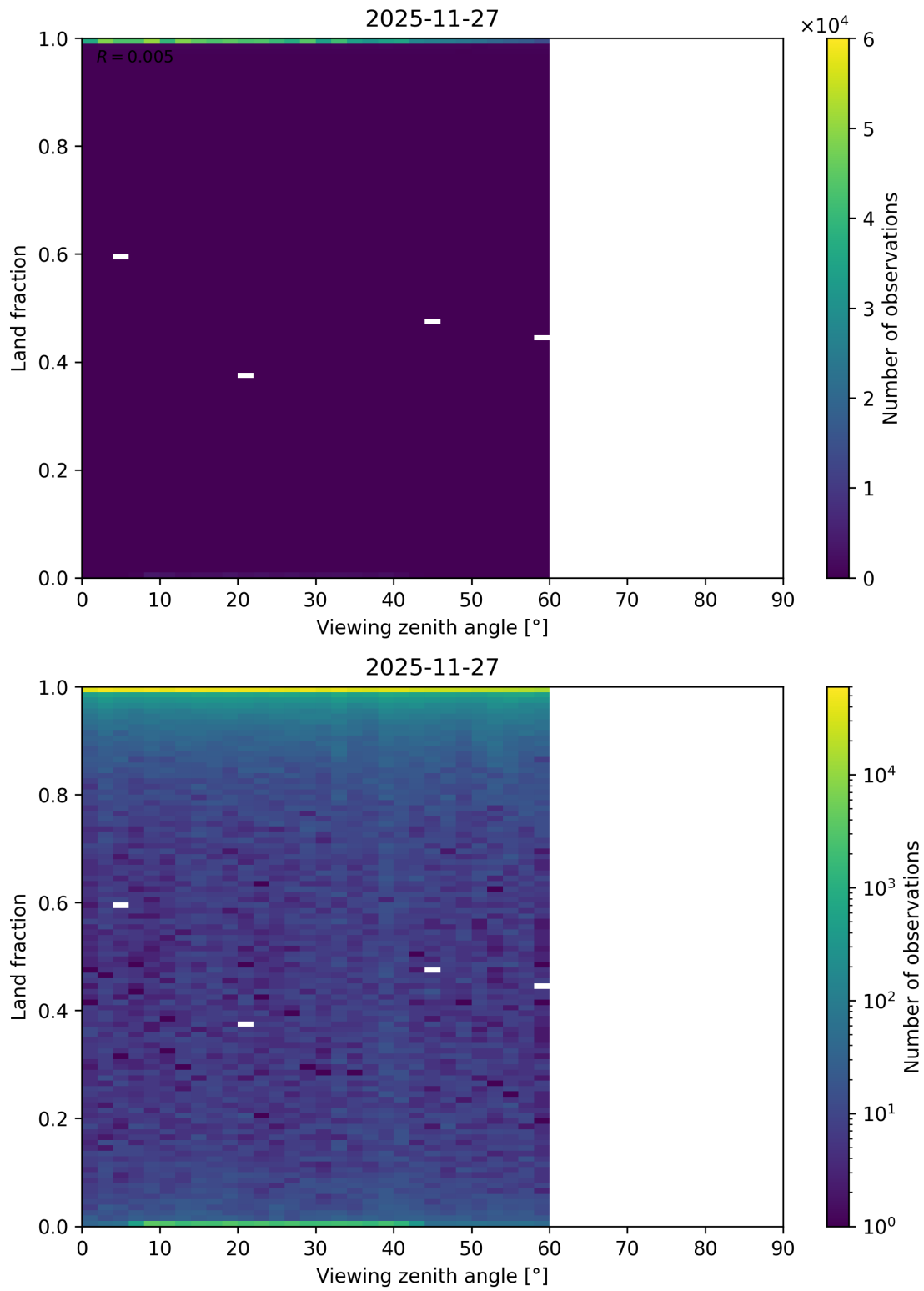
Figure 124: Scatter density plot of “Viewing zenith angle” against “Land fraction” for 2025-11-26 to 2025-11-28.
