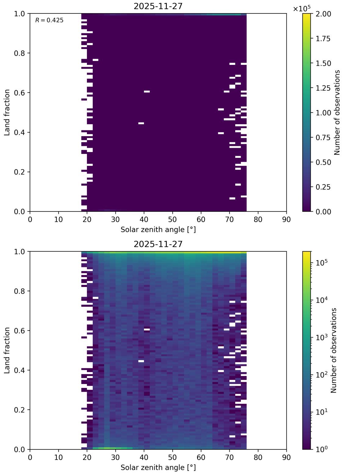
Figure 112: Scatter density plot of “Solar zenith angle” against “Land fraction” for 2025-11-26 to 2025-11-28.
