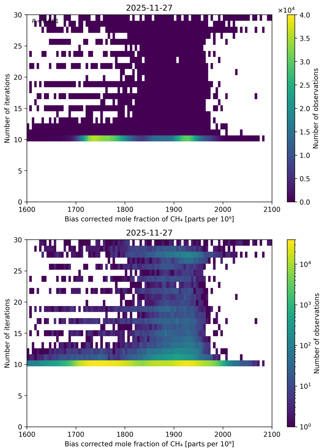
Figure 77: Scatter density plot of “Bias corrected mole fraction of CH 4 ” against “Number of iterations” for 2025-11-26 to 2025-11-28.
