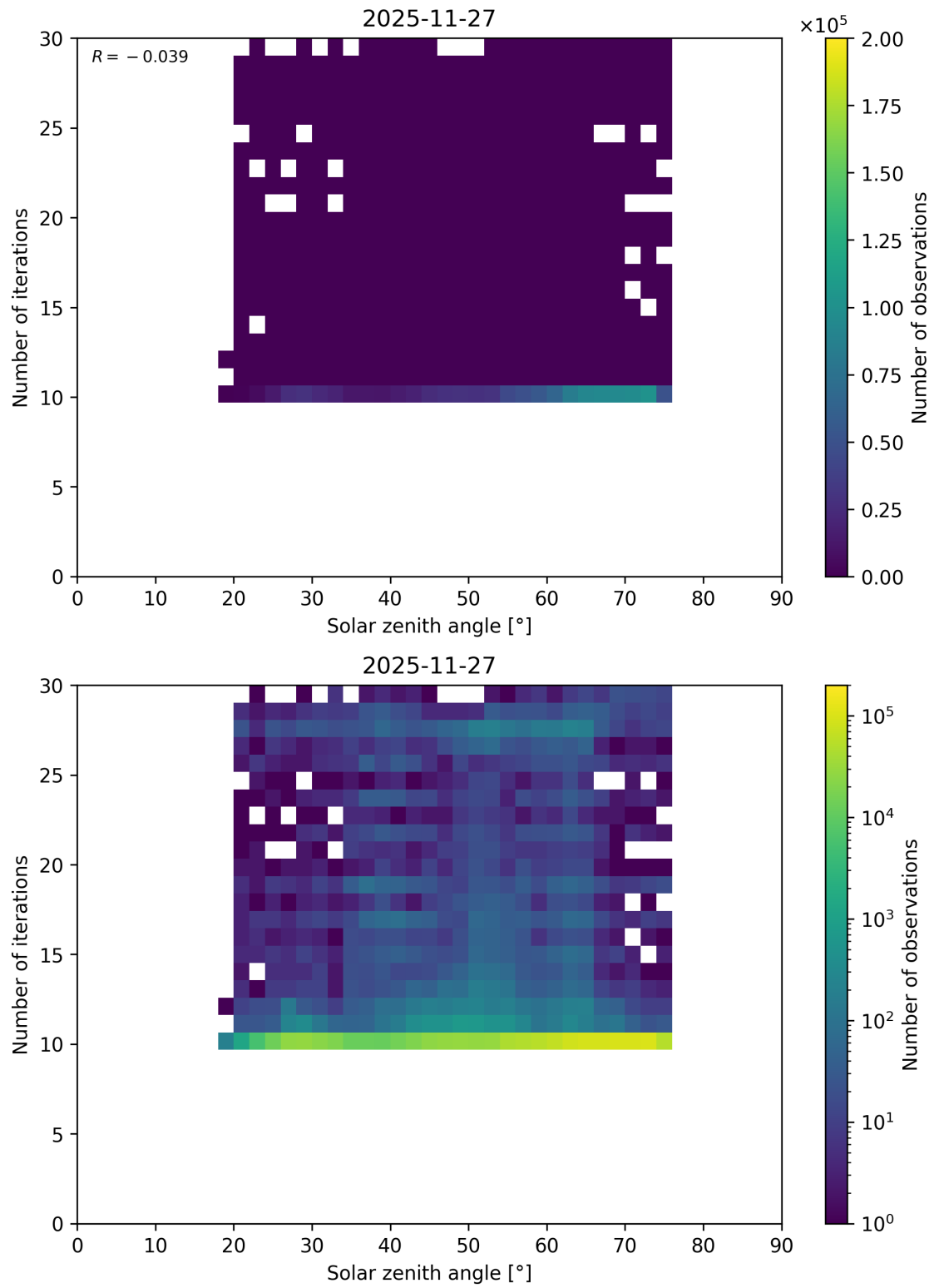
Figure 117: Scatter density plot of “Solar zenith angle” against “Number of iterations” for 2025-11-26 to 2025-11-28.
