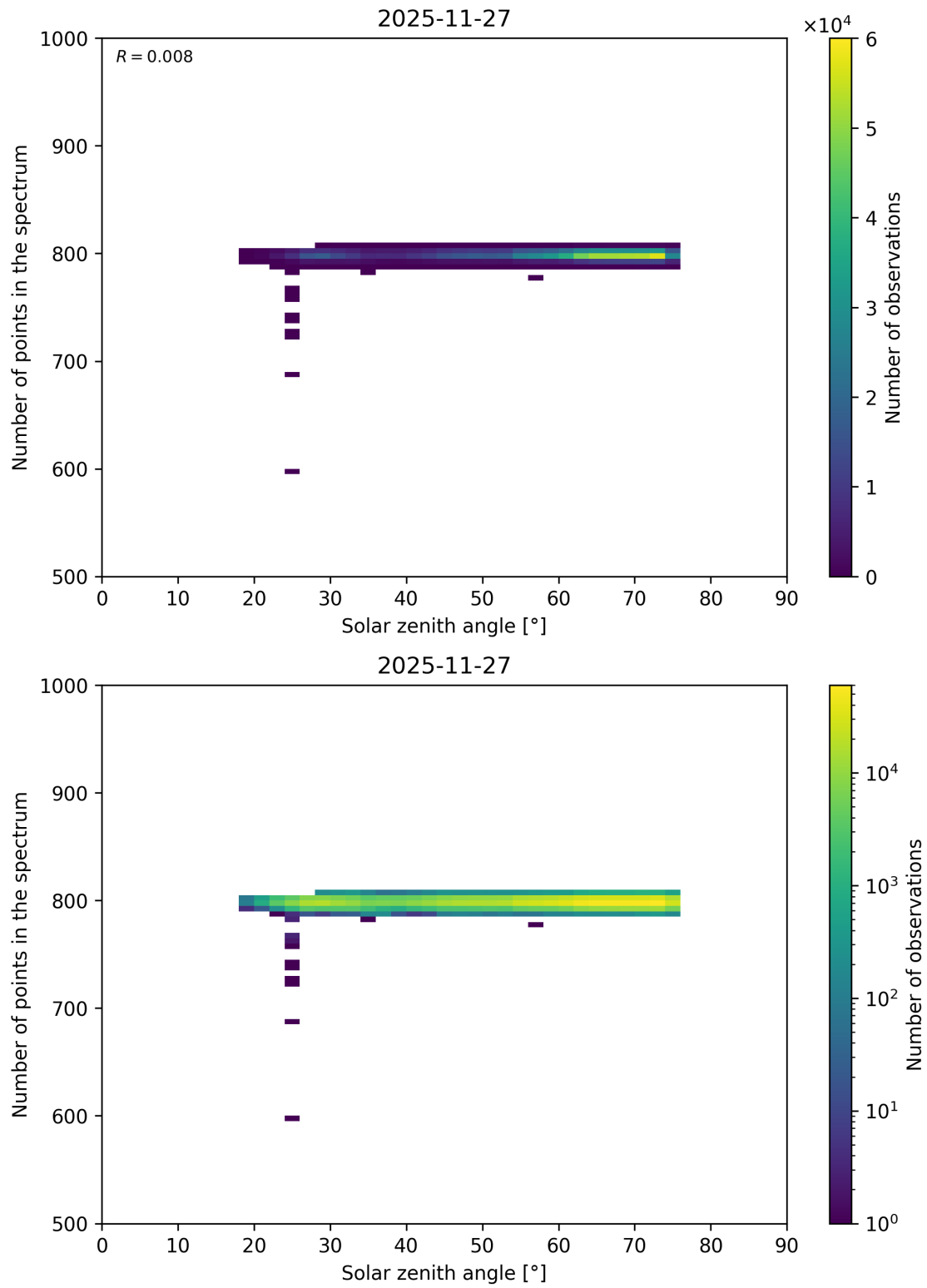
Figure 118: Scatter density plot of “Solar zenith angle” against “Number of points in the spectrum” for 2025-11-26 to 2025-11-28.
