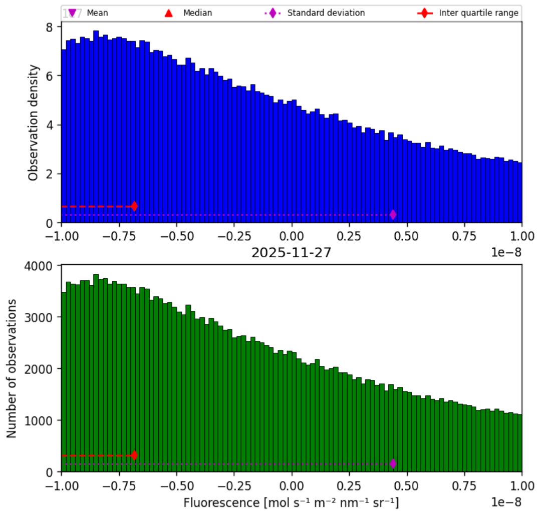
Figure 34: Histogram of “Fluorescence” for 2025-11-26 to 2025-11-28
