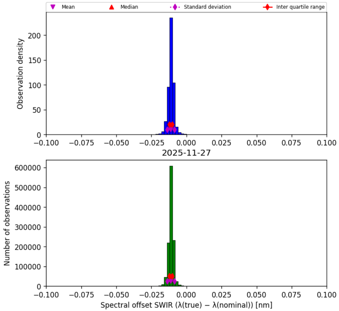
Figure 29: Histogram of “Spectral offset SWIR ( \lambda_{\text{true}} - \lambda_{\text{nominal}} )” for 2025-11-26 to 2025-11-28
