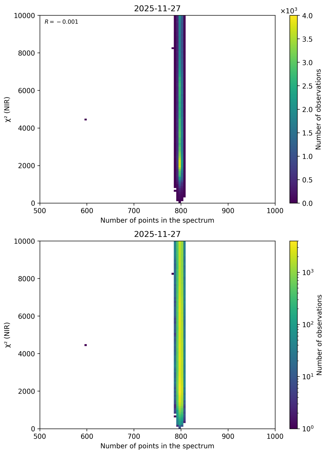
Figure 101: Scatter density plot of “Number of points in the spectrum” against “ \chi^2 (NIR)” for 2025-11-26 to 2025-11-28.
