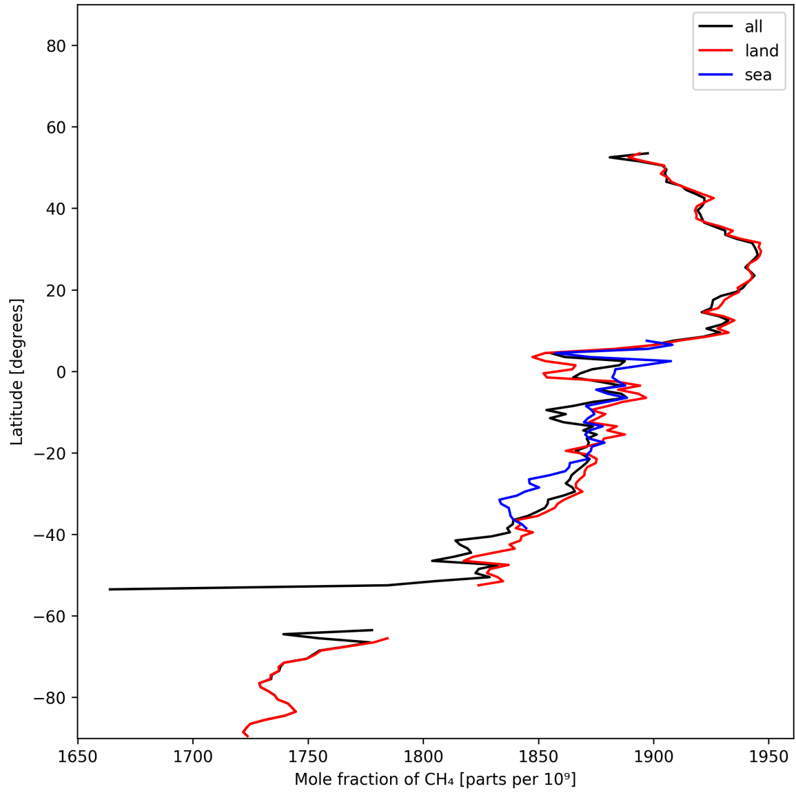
Figure 13: Zonal average of “Mole fraction of CH 4 ” for 2025-11-26 to 2025-11-28.
