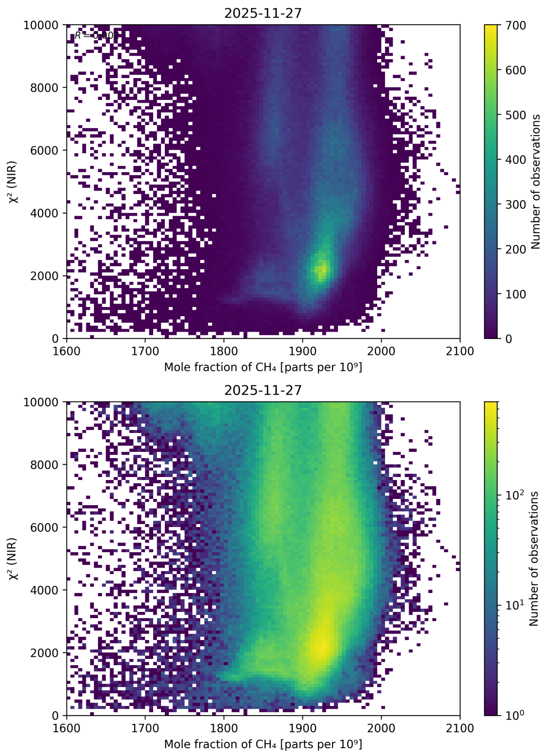
Figure 80: Scatter density plot of “Mole fraction of CH 4 ” against “ \chi^2 (NIR)” for 2025-11-26 to 2025-11-28.
