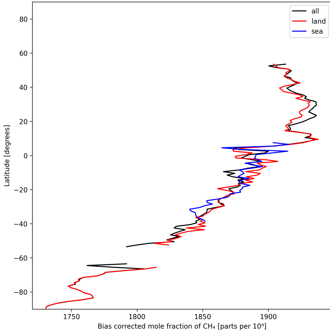
Figure 15: Zonal average of “Bias corrected mole fraction of CH 4 ” for 2025-11-26 to 2025-11-28.
