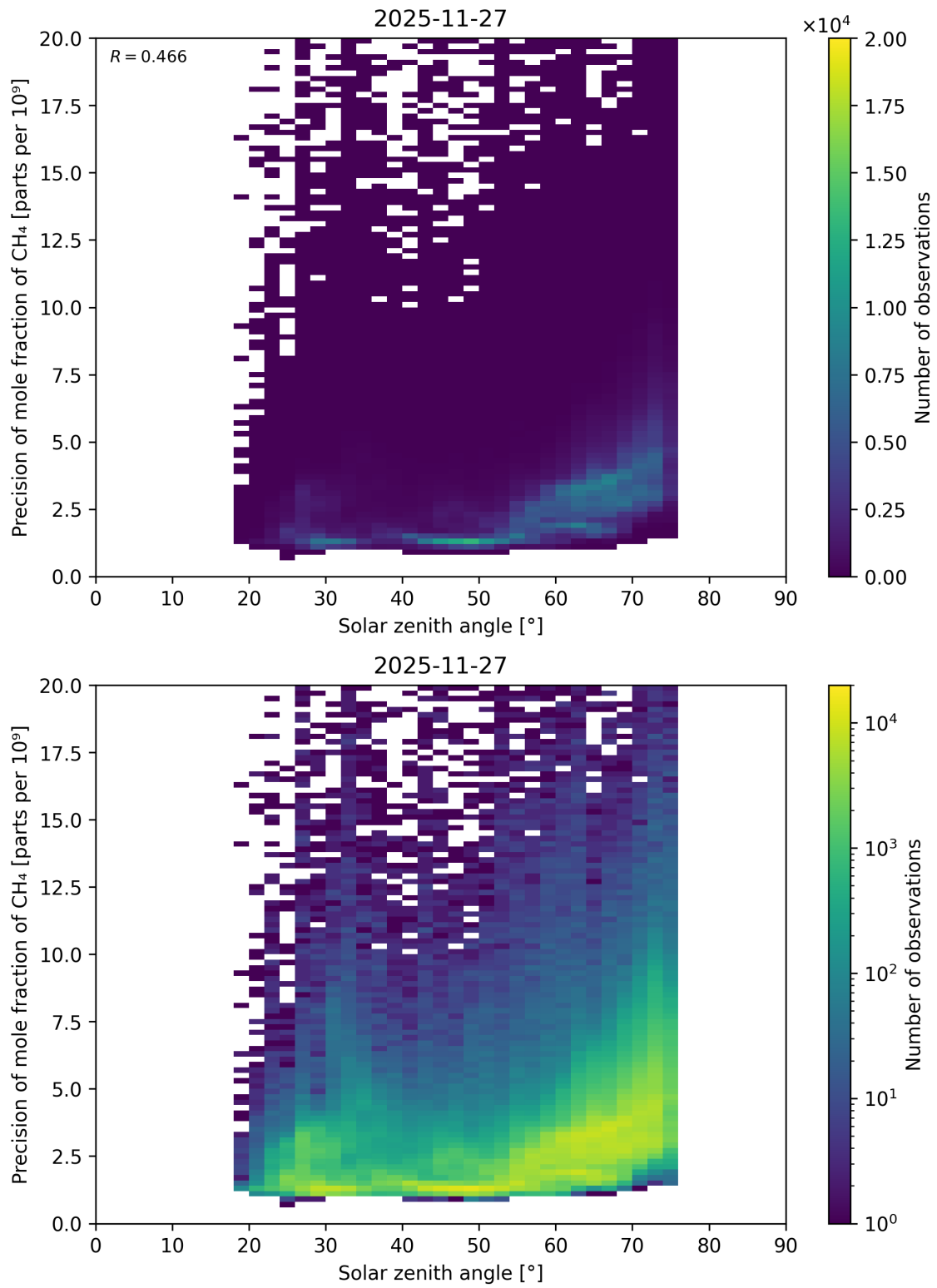
Figure 116: Scatter density plot of “Solar zenith angle” against “Precision of mole fraction of \text{CH}_4 ” for 2025-11-26 to 2025-11-28.
