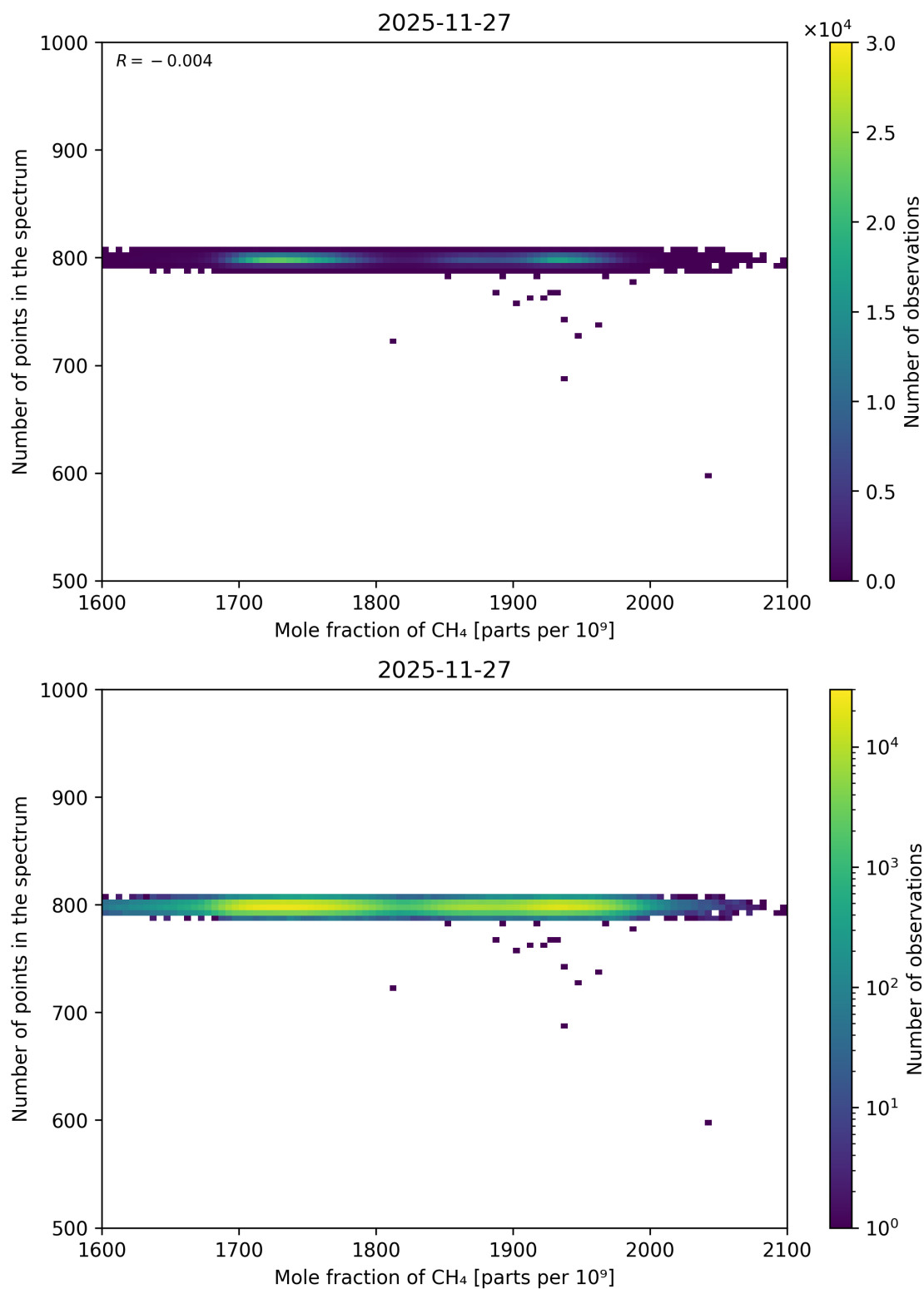
Figure 88: Scatter density plot of “Mole fraction of CH 4 ” against “Number of points in the spectrum” for 2025-11-26 to 2025-11-28.
