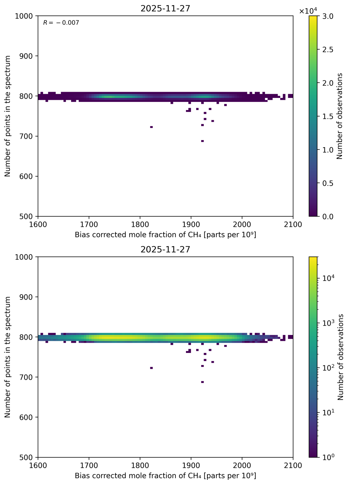
Figure 78: Scatter density plot of “Bias corrected mole fraction of \text{CH}_4 ” against “Number of points in the spectrum” for 2025-11-26 to 2025-11-28.
