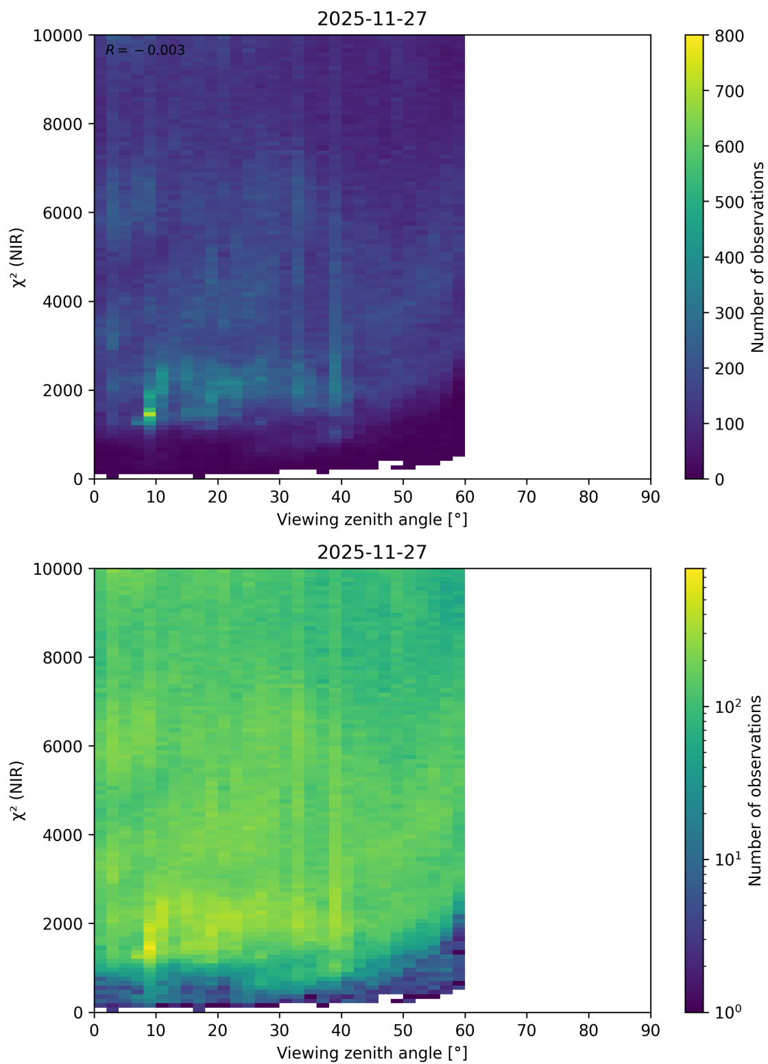
Figure 120: Scatter density plot of “Viewing zenith angle” against “ \chi^2 (NIR)” for 2025-11-26 to 2025-11-28.
