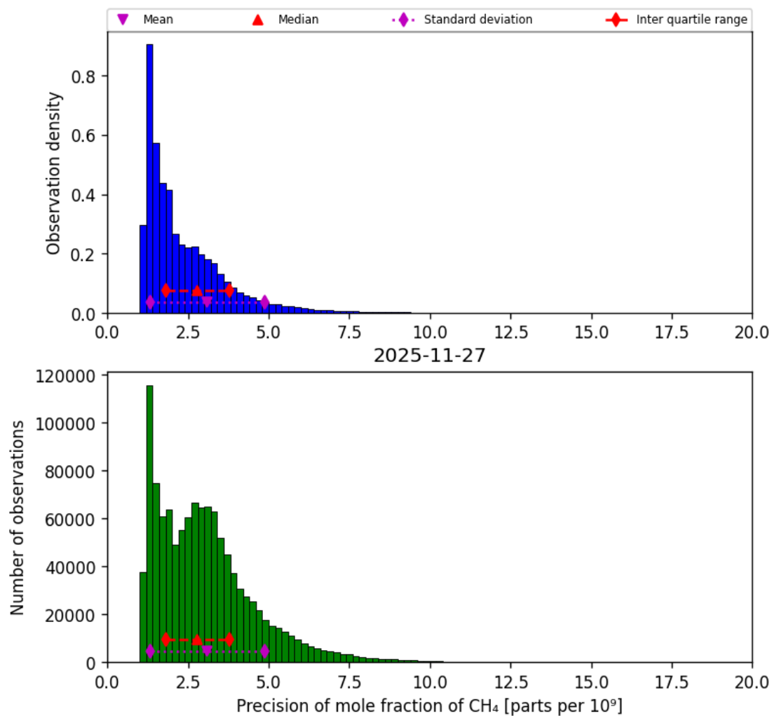
Figure 26: Histogram of “Precision of mole fraction of CH 4 ” for 2025-11-26 to 2025-11-28
