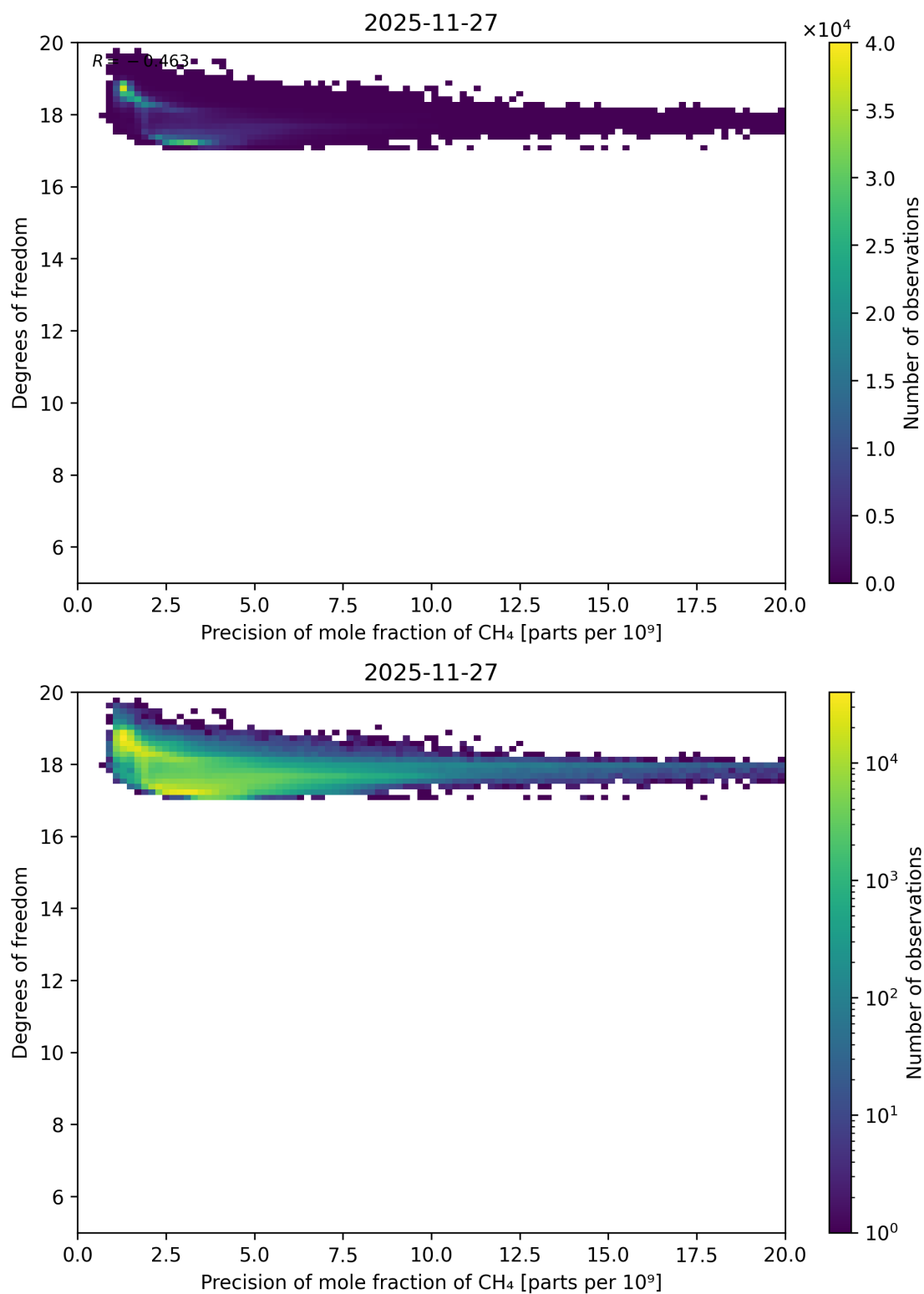
Figure 91: Scatter density plot of “Precision of mole fraction of CH 4 ” against “Degrees of freedom” for 2025-11-26 to 2025-11-28.
