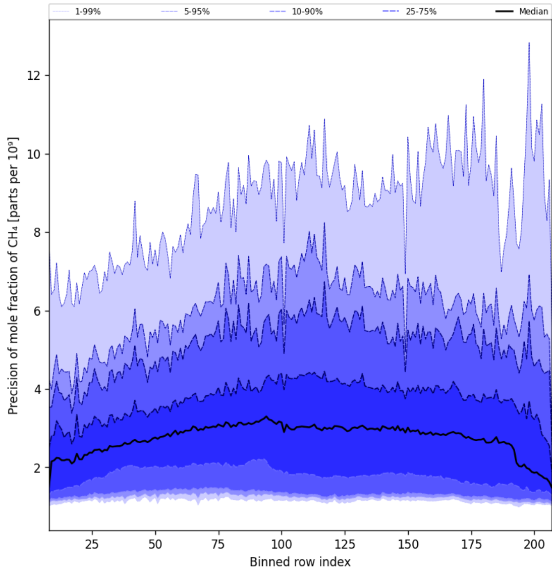
Figure 38: Along track statistics of “Precision of mole fraction of CH 4 ” for 2025-11-26 to 2025-11-28
