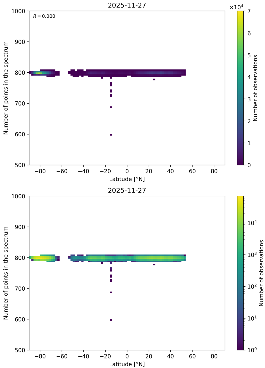
Figure 70: Scatter density plot of “Latitude” against “Number of points in the spectrum” for 2025-11-26 to 2025-11-28.
