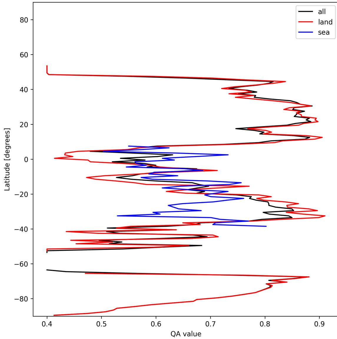
Figure 12: Zonal average of “QA value” for 2025-11-26 to 2025-11-28.
