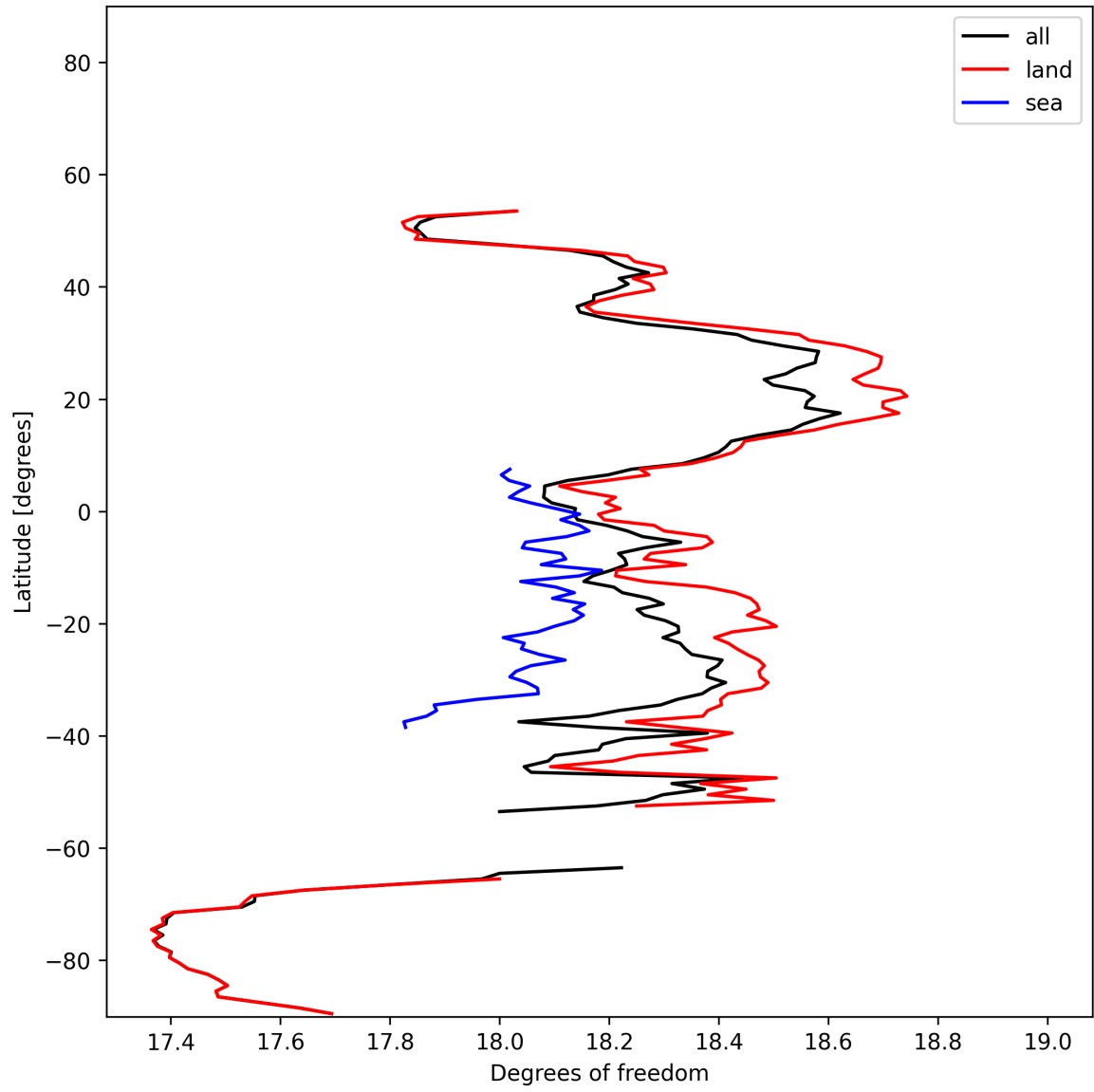
Figure 20: Zonal average of “Degrees of freedom” for 2025-11-26 to 2025-11-28.
