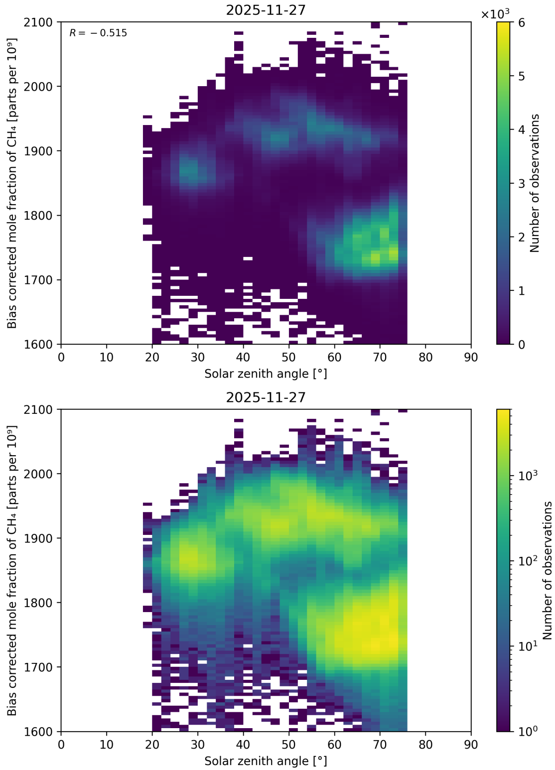
Figure 115: Scatter density plot of “Solar zenith angle” against “Bias corrected mole fraction of \text{CH}_4 ” for 2025-11-26 to 2025-11-28.
