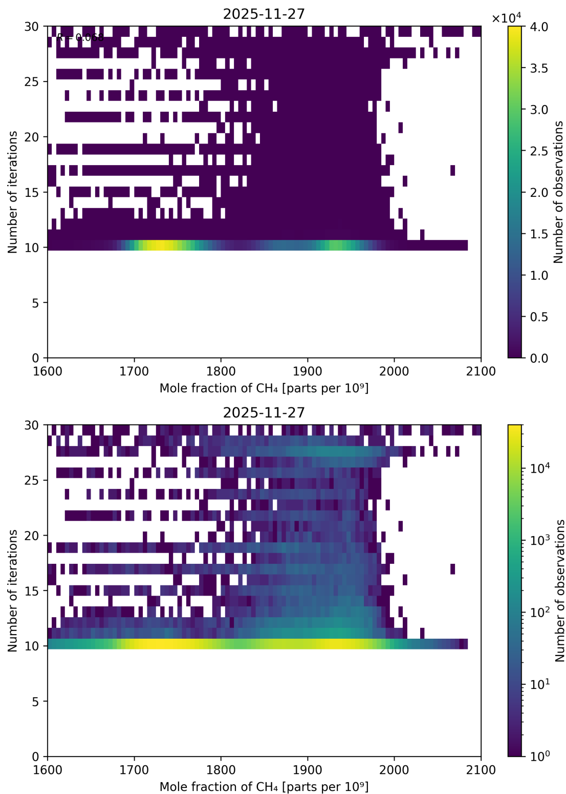
Figure 87: Scatter density plot of “Mole fraction of CH 4 ” against “Number of iterations” for 2025-11-26 to 2025-11-28.
