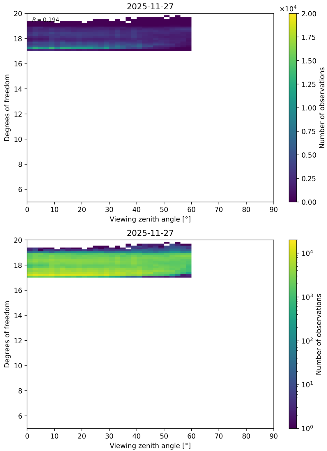
Figure 122: Scatter density plot of “Viewing zenith angle” against “Degrees of freedom” for 2025-11-26 to 2025-11-28.
