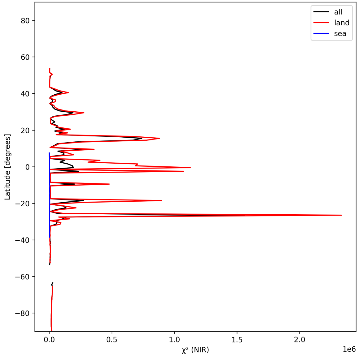
Figure 19: Zonal average of “ \chi^2 (NIR)” for 2025-11-26 to 2025-11-28.
