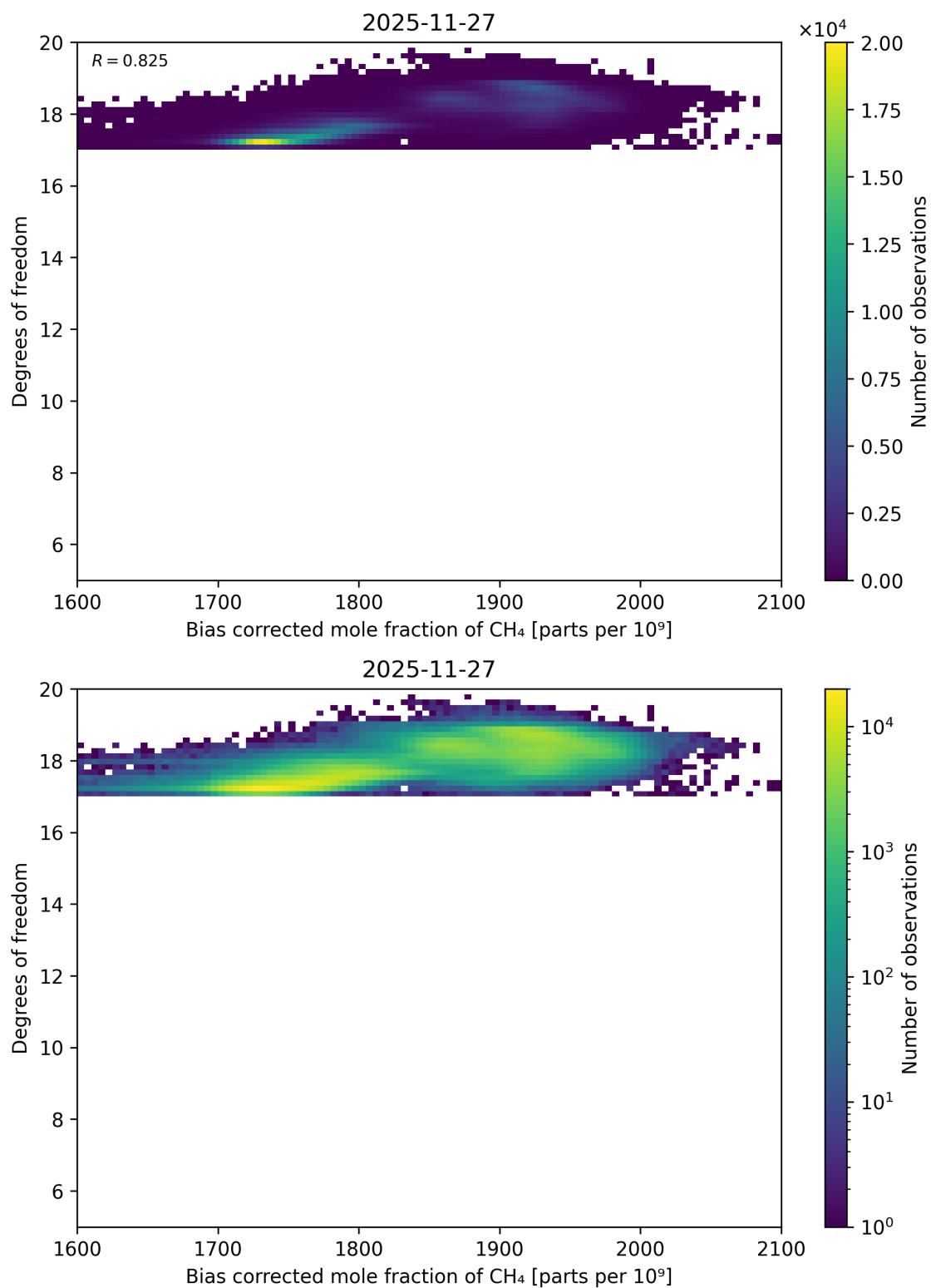
Figure 74: Scatter density plot of “Bias corrected mole fraction of \text{CH}_4 ” against “Degrees of freedom” for 2025-11-26 to 2025-11-28.
