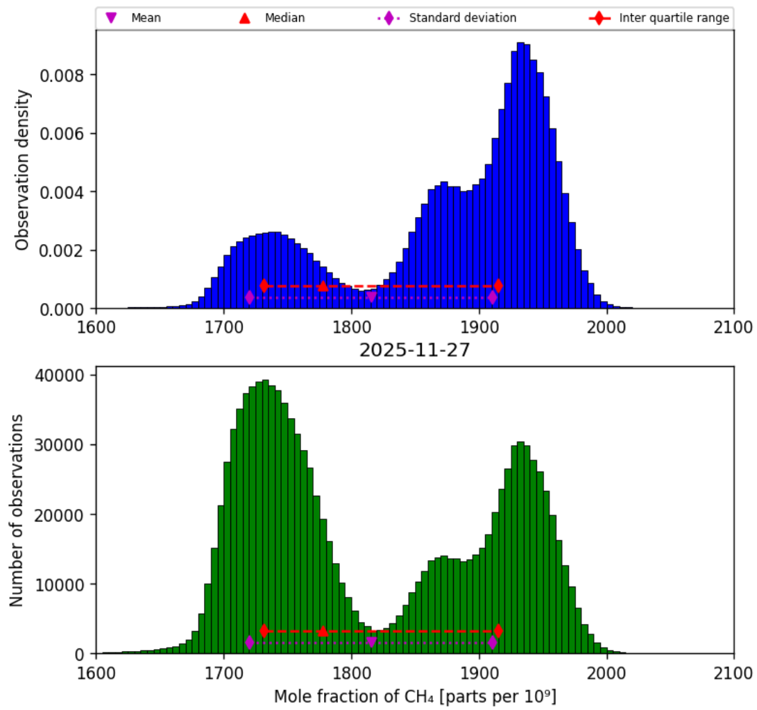
Figure 25: Histogram of “Mole fraction of CH 4 ” for 2025-11-26 to 2025-11-28
