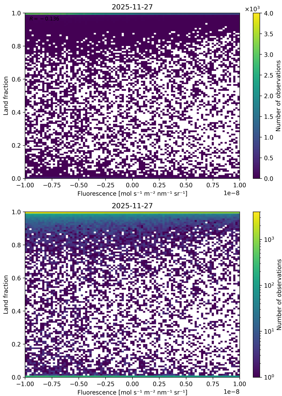
Figure 60: Scatter density plot of “Fluorescence” against “Land fraction” for 2025-11-26 to 2025-11-28.
