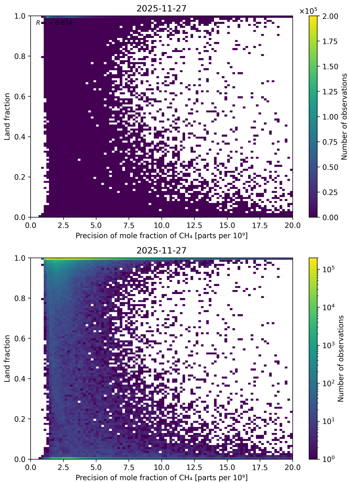
Figure 93: Scatter density plot of “Precision of mole fraction of CH 4 ” against “Land fraction” for 2025-11-26 to 2025-11-28.
