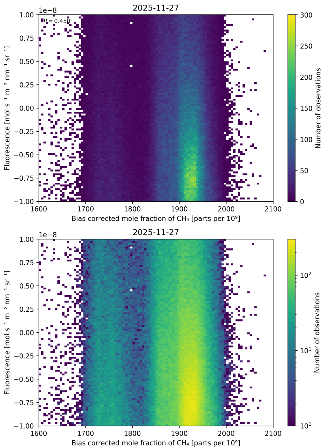
Figure 75: Scatter density plot of “Bias corrected mole fraction of \text{CH}_4 ” against “Fluorescence” for 2025-11-26 to 2025-11-28.
