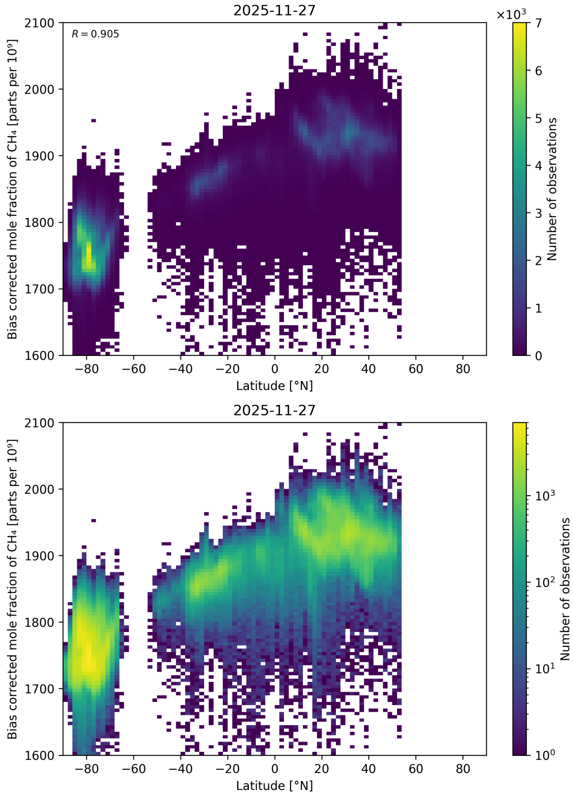
Figure 67: Scatter density plot of “Latitude” against “Bias corrected mole fraction of CH 4 ” for 2025-11-26 to 2025-11-28.
