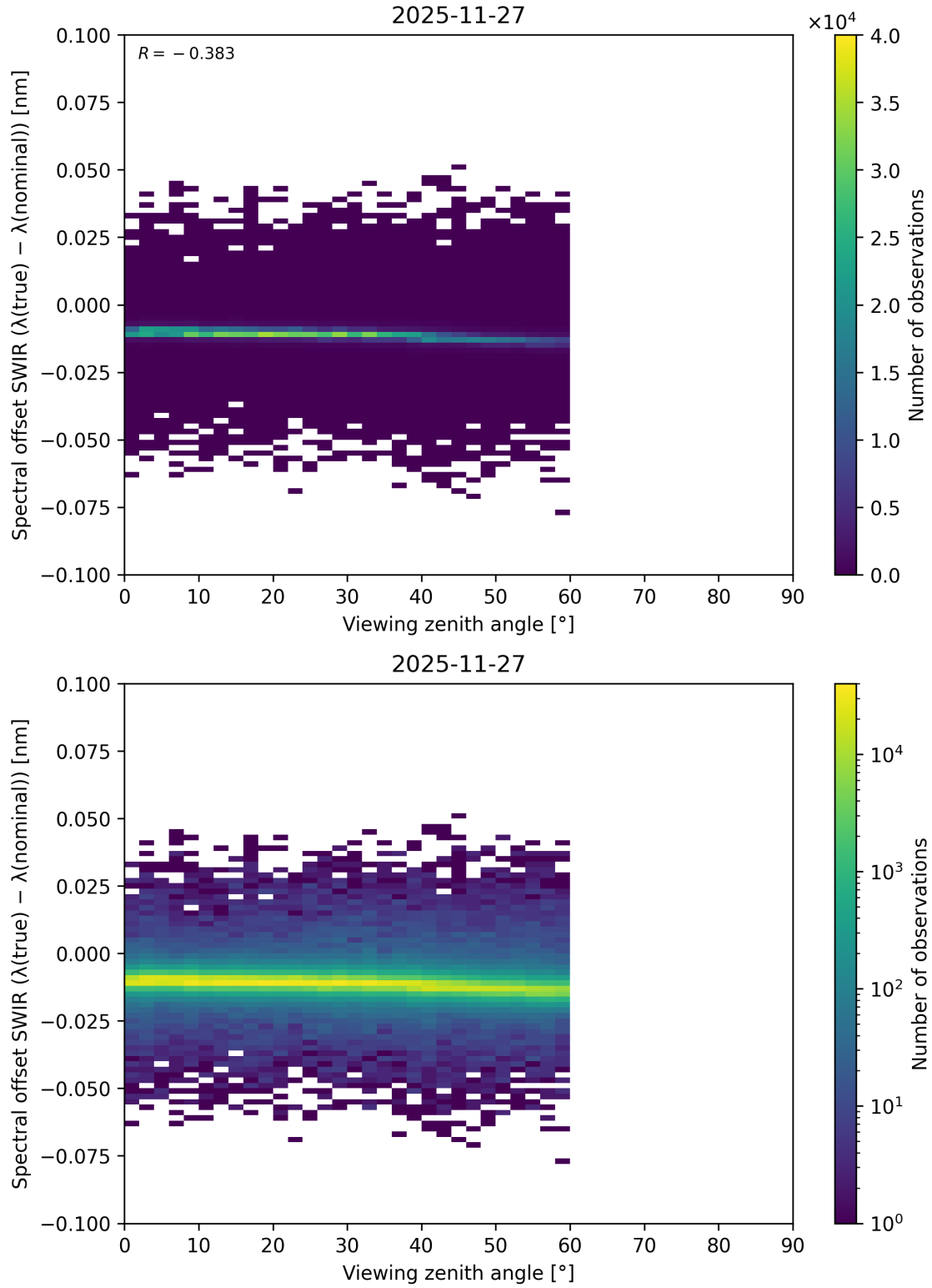
Figure 132: Scatter density plot of “Viewing zenith angle” against “Spectral offset SWIR ( \lambda_{\text{true}} - \lambda_{\text{nominal}} )” for 2025-11-26 to 2025-11-28.
