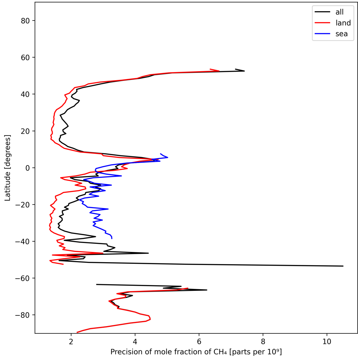
Figure 14: Zonal average of “Precision of mole fraction of CH 4 ” for 2025-11-26 to 2025-11-28.
