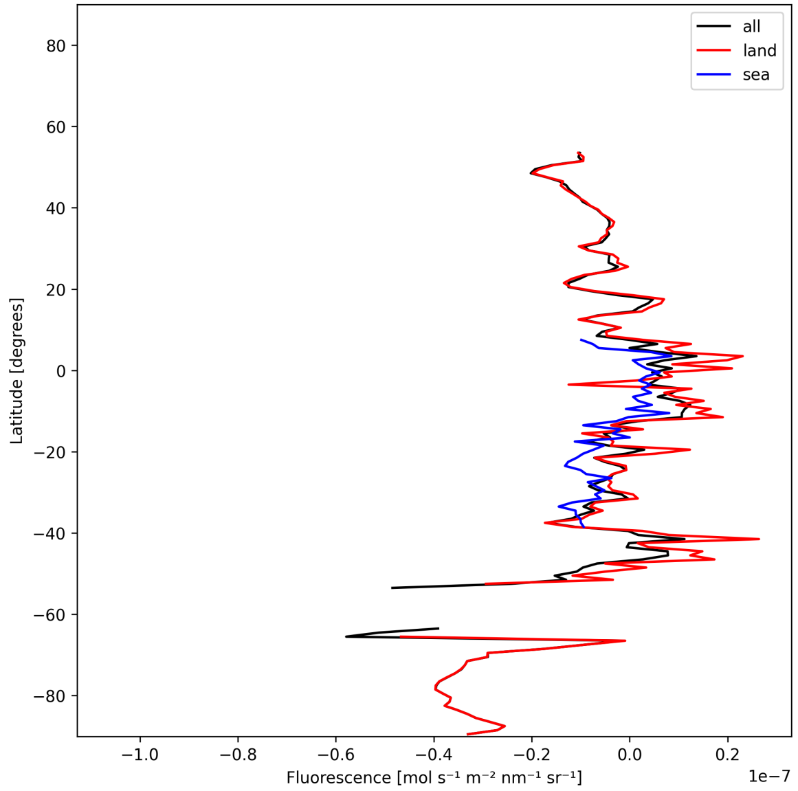
Figure 22: Zonal average of “Fluorescence” for 2025-11-26 to 2025-11-28.
