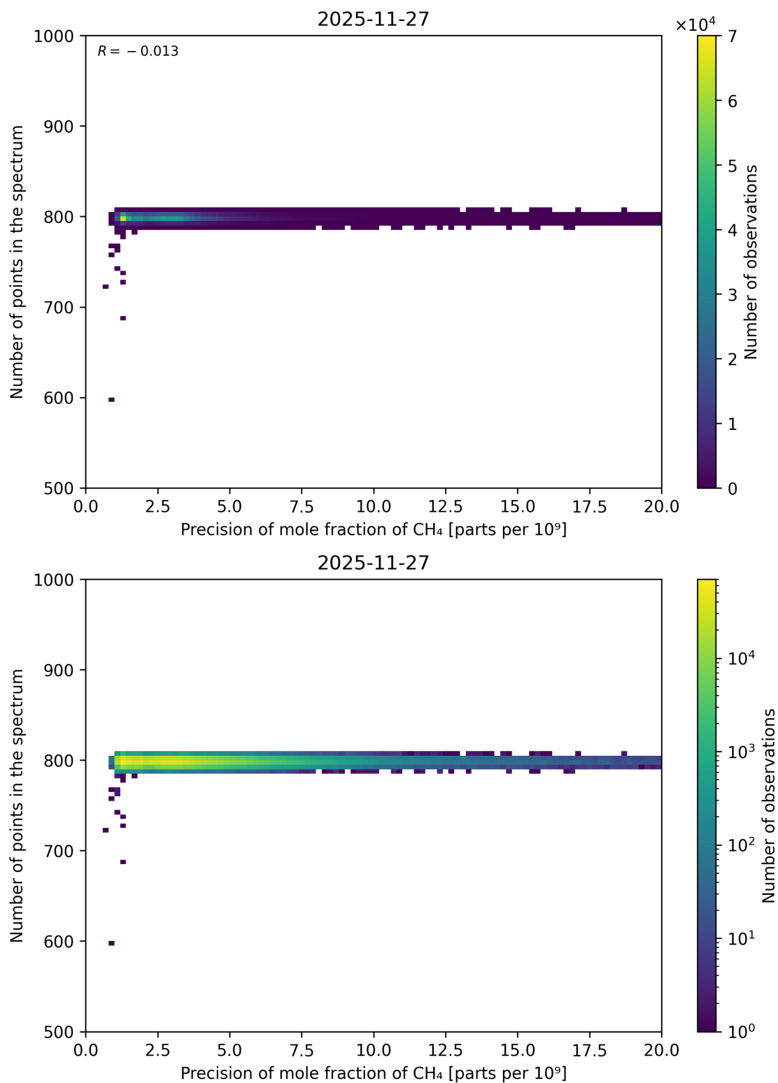
Figure 96: Scatter density plot of “Precision of mole fraction of CH 4 ” against “Number of points in the spectrum” for 2025-11-26 to 2025-11-28.
