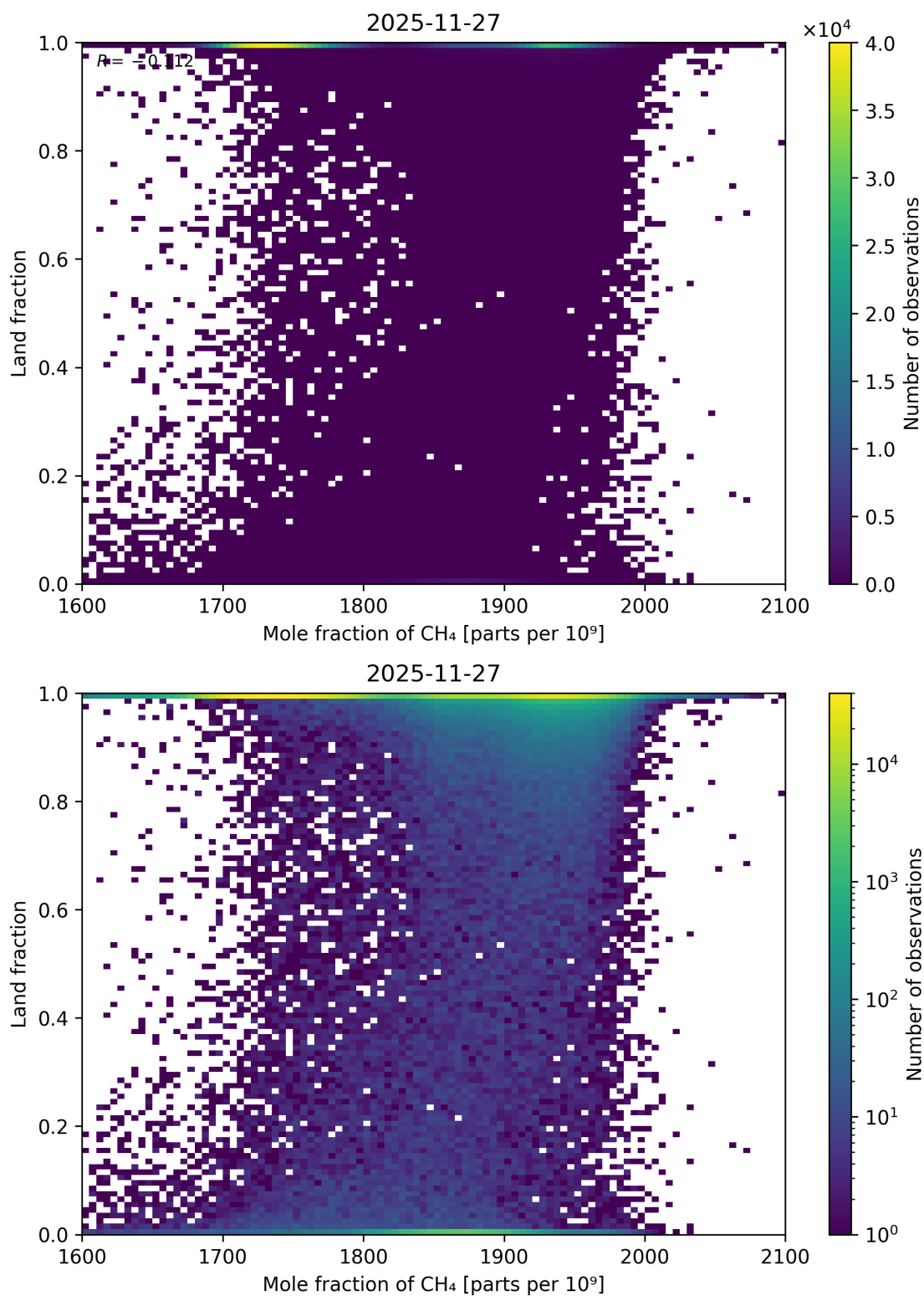
Figure 84: Scatter density plot of “Mole fraction of CH 4 ” against “Land fraction” for 2025-11-26 to 2025-11-28.
