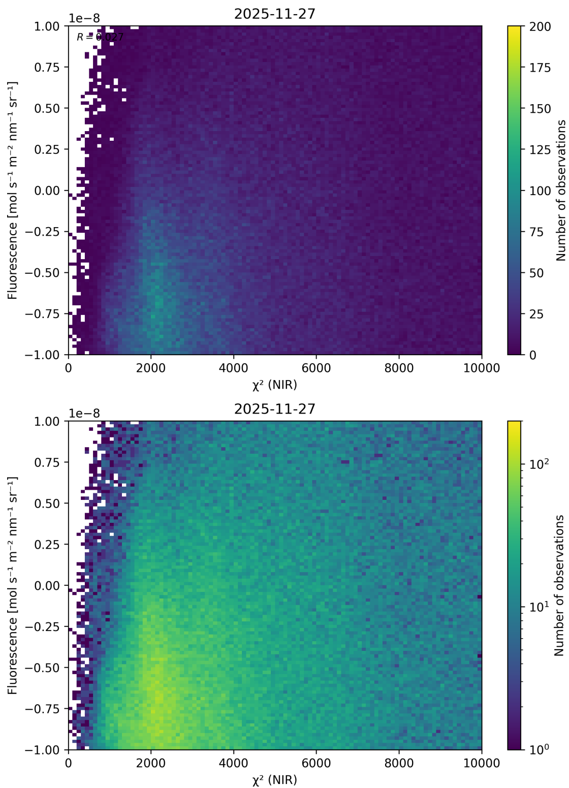
Figure 49: Scatter density plot of “ \chi^2 (NIR)” against “Fluorescence” for 2025-11-26 to 2025-11-28.
