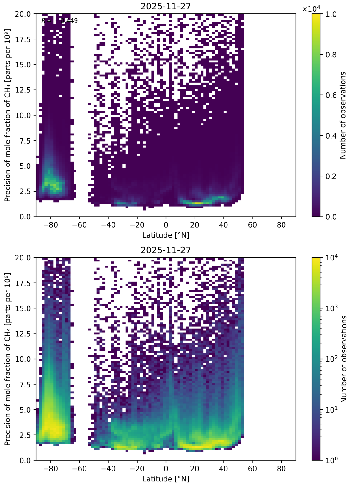
Figure 68: Scatter density plot of “Latitude” against “Precision of mole fraction of \text{CH}_4 ” for 2025-11-26 to 2025-11-28.
