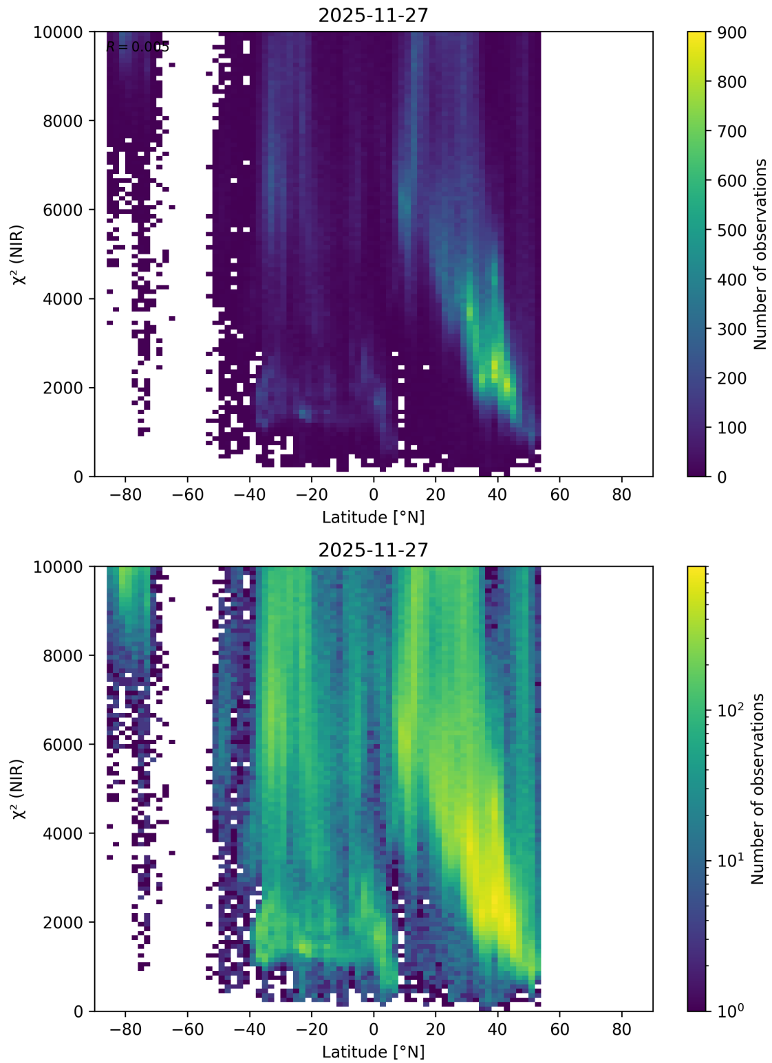
Figure 61: Scatter density plot of “Latitude” against “ \chi^2 (NIR)” for 2025-11-26 to 2025-11-28.
