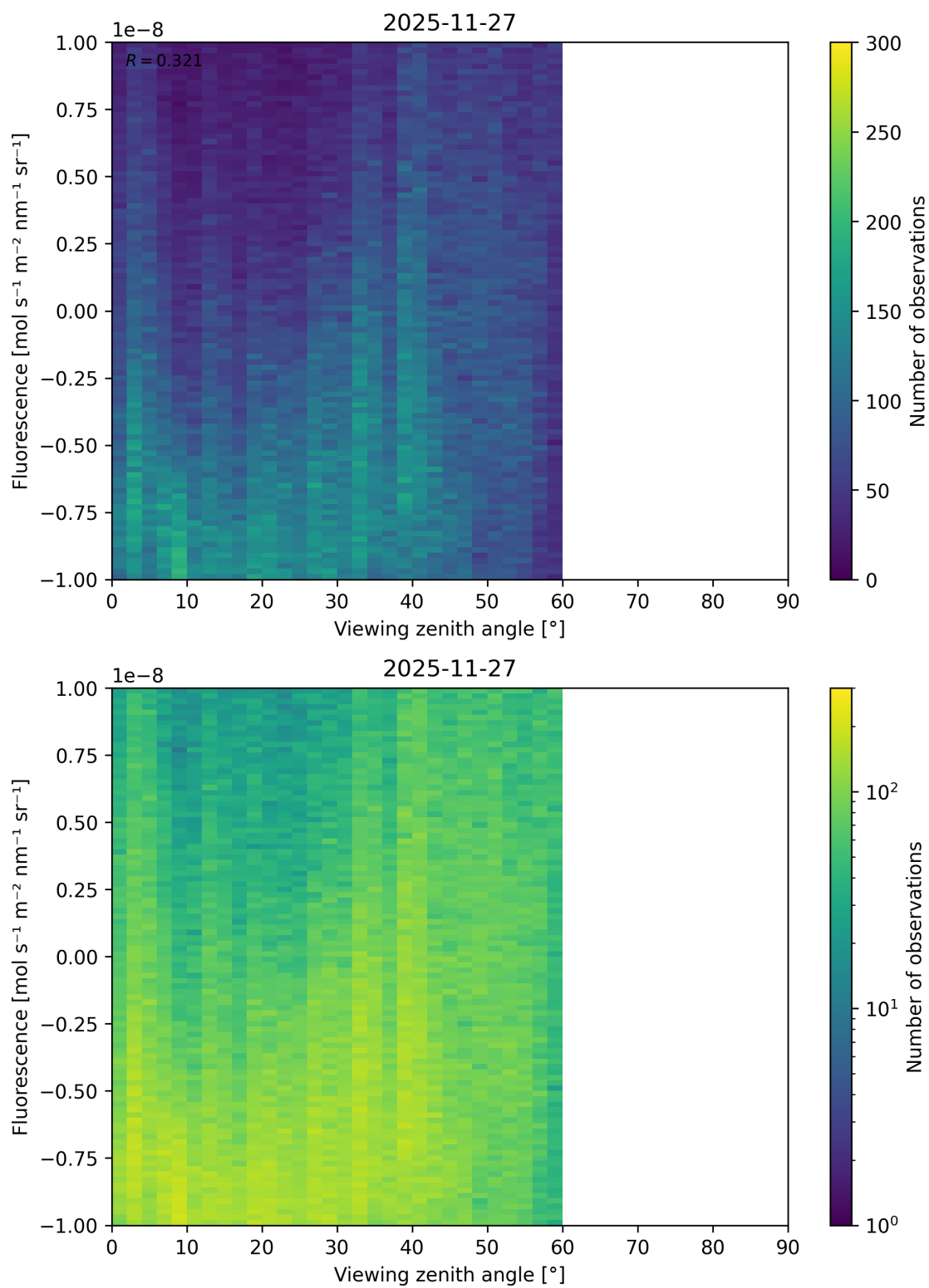
Figure 123: Scatter density plot of “Viewing zenith angle” against “Fluorescence” for 2025-11-26 to 2025-11-28.
