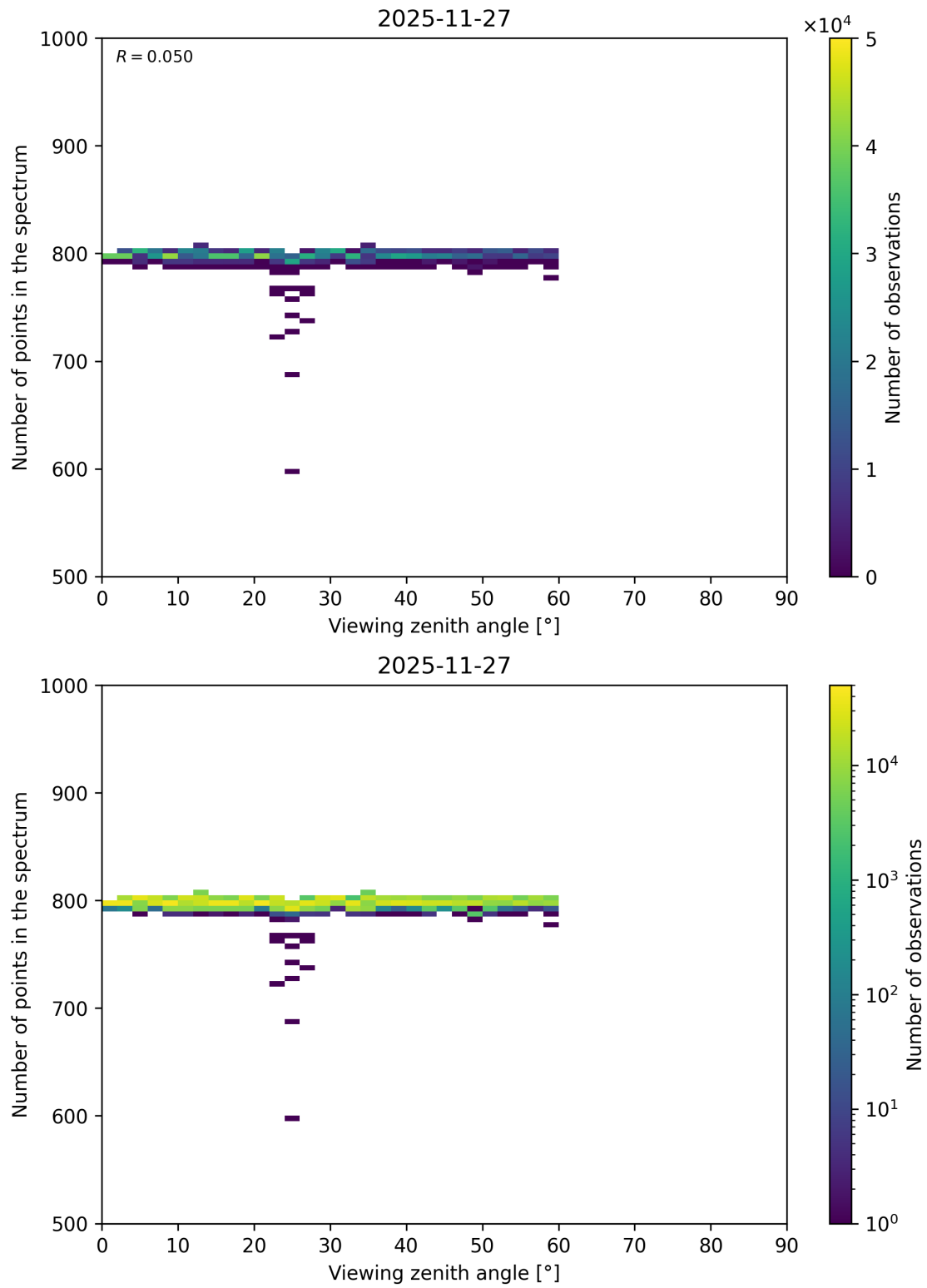
Figure 130: Scatter density plot of “Viewing zenith angle” against “Number of points in the spectrum” for 2025-11-26 to 2025-11-28.
