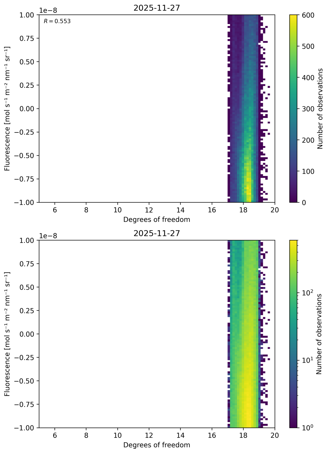
Figure 57: Scatter density plot of “Degrees of freedom” against “Fluorescence” for 2025-11-26 to 2025-11-28.
