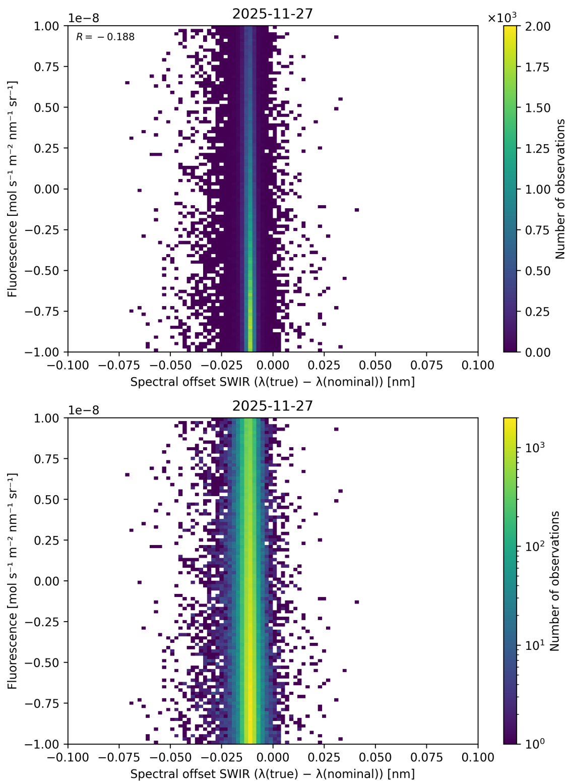
Figure 136: Scatter density plot of “Spectral offset SWIR ( \lambda_{\text{true}} - \lambda_{\text{nominal}} )” against “Fluorescence” for 2025-11-26 to 2025-11-28.
