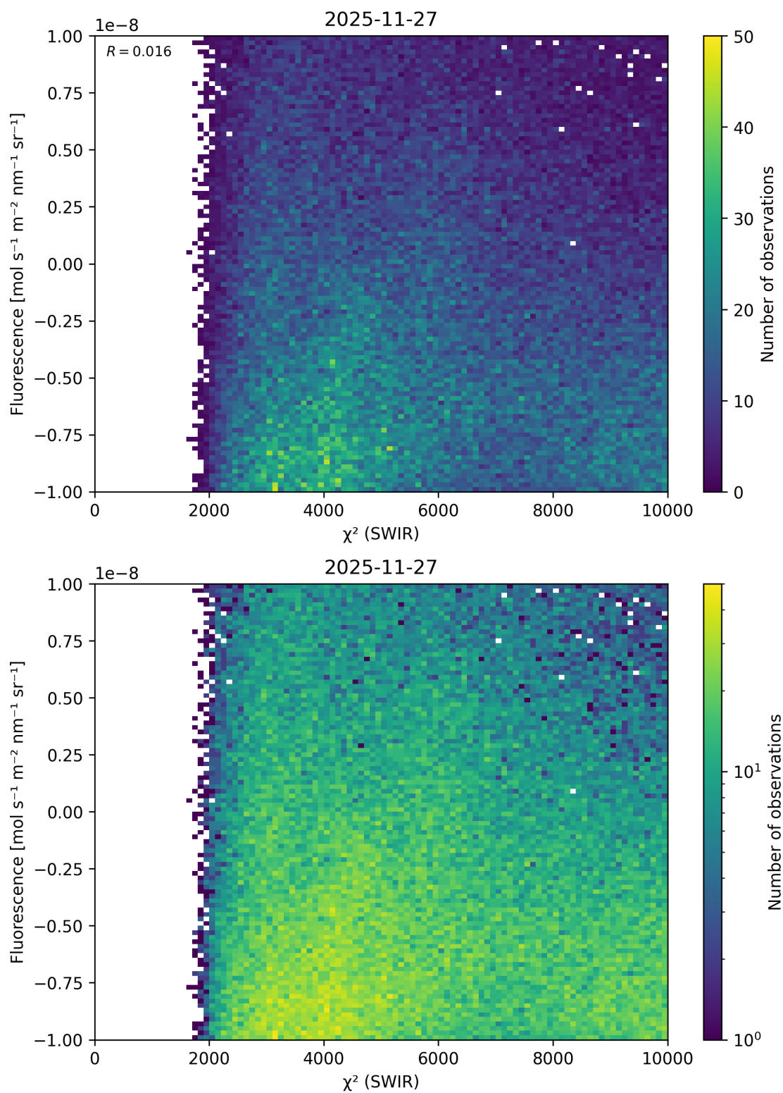
Figure 54: Scatter density plot of “ \chi^2 (SWIR)” against “Fluorescence” for 2025-11-26 to 2025-11-28.
