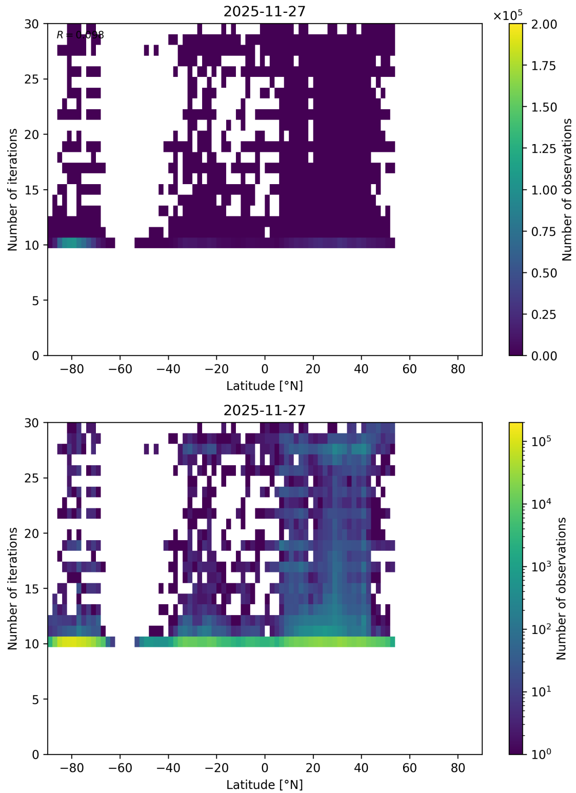
Figure 69: Scatter density plot of “Latitude” against “Number of iterations” for 2025-11-26 to 2025-11-28.
