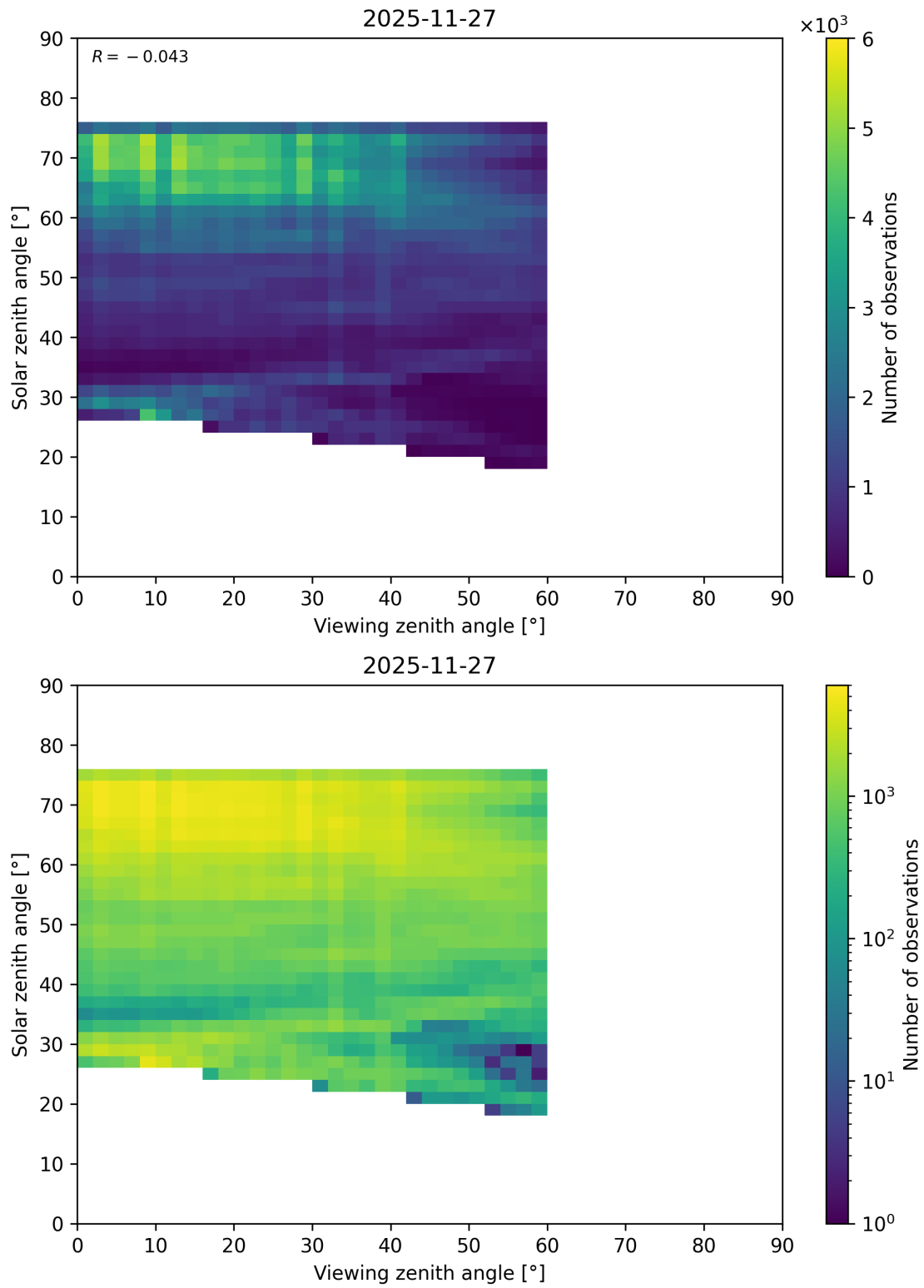
Figure 131: Scatter density plot of “Viewing zenith angle” against “Solar zenith angle” for 2025-11-26 to 2025-11-28.
