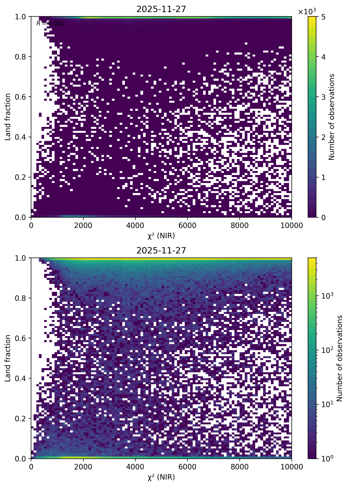
Figure 50: Scatter density plot of “ \chi^2 (NIR)” against “Land fraction” for 2025-11-26 to 2025-11-28.
