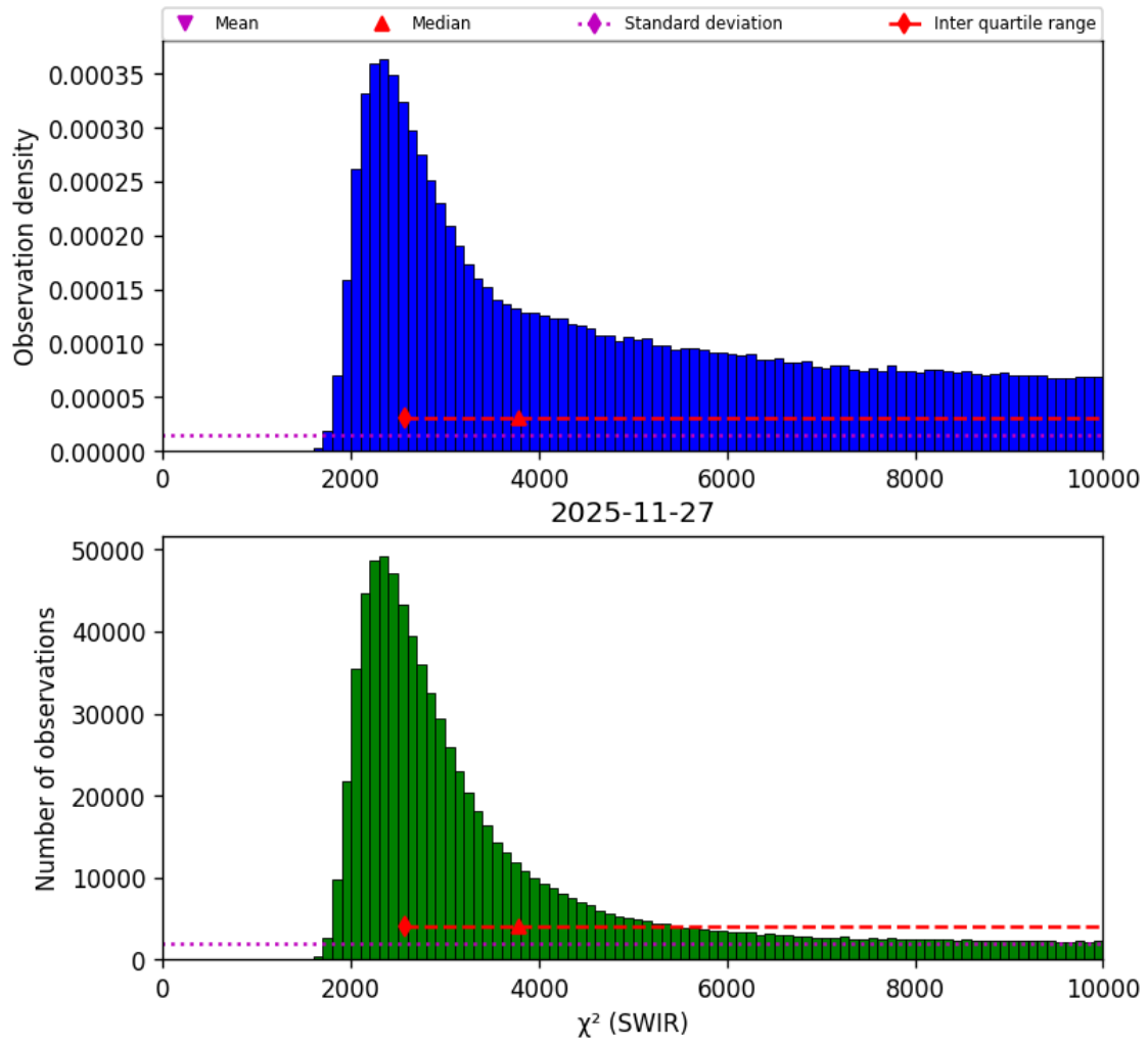
Figure 30: Histogram of “ \chi^2 (SWIR)” for 2025-11-26 to 2025-11-28
