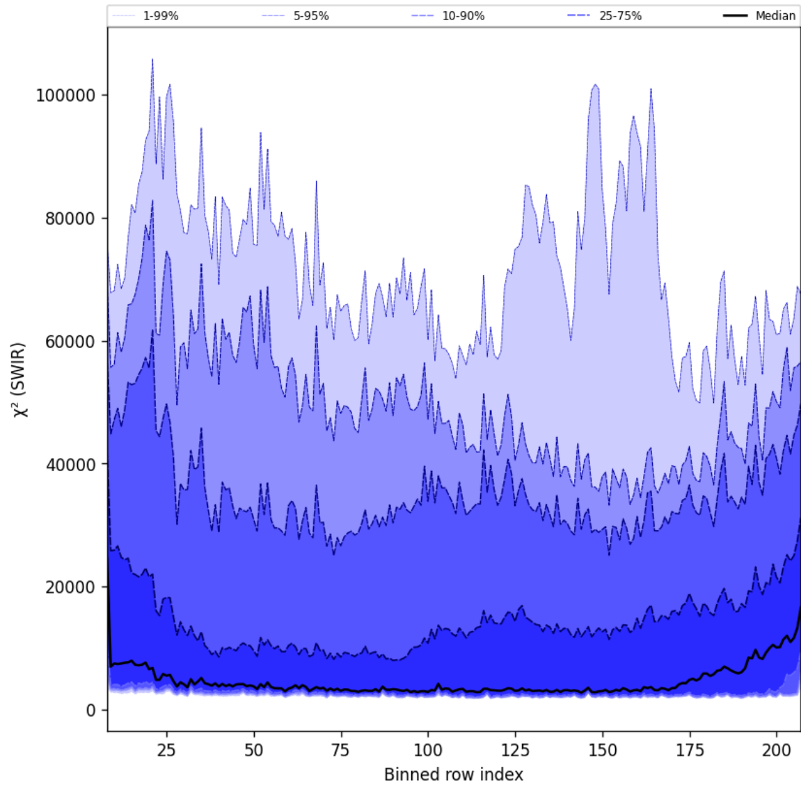
Figure 42: Along track statistics of “ \chi^2 (SWIR)” for 2025-11-26 to 2025-11-28
