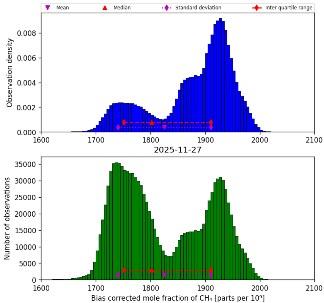
Figure 27: Histogram of “Bias corrected mole fraction of CH 4 ” for 2025-11-26 to 2025-11-28
