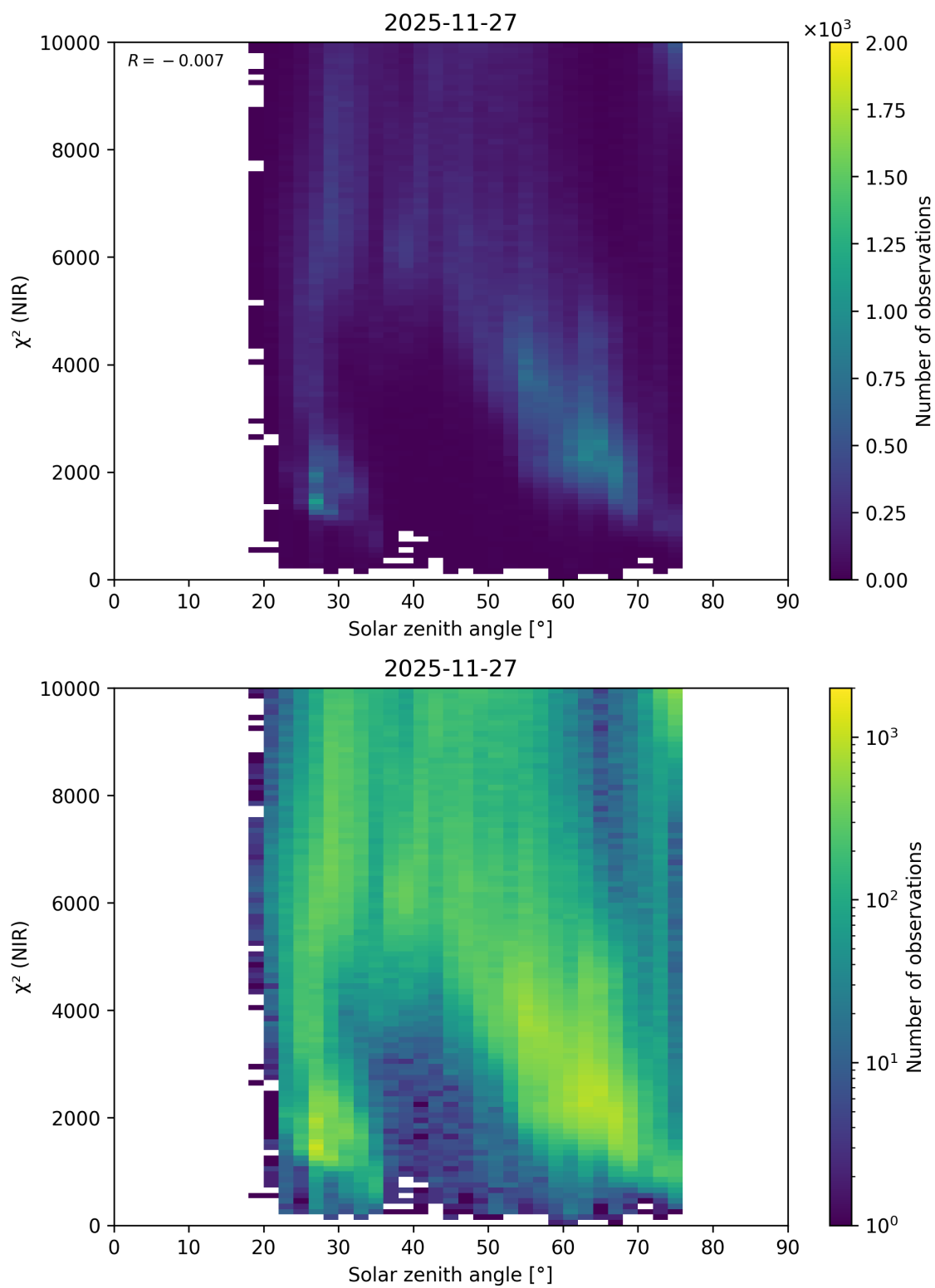
Figure 108: Scatter density plot of “Solar zenith angle” against “ \chi^2 (NIR)” for 2025-11-26 to 2025-11-28.
