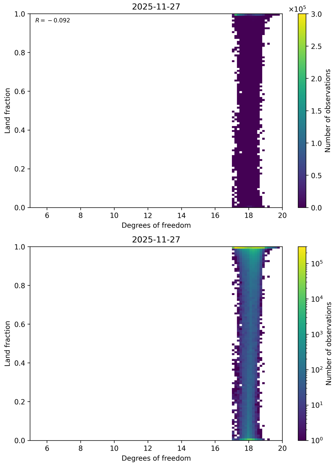
Figure 58: Scatter density plot of “Degrees of freedom” against “Land fraction” for 2025-11-26 to 2025-11-28.
