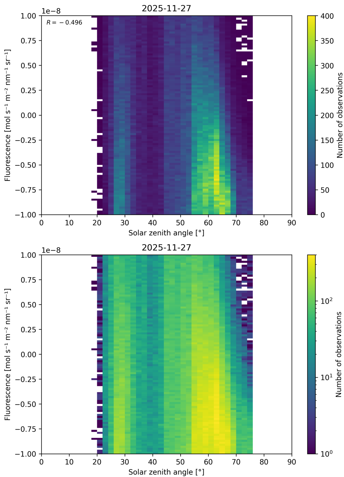
Figure 111: Scatter density plot of “Solar zenith angle” against “Fluorescence” for 2025-11-26 to 2025-11-28.
