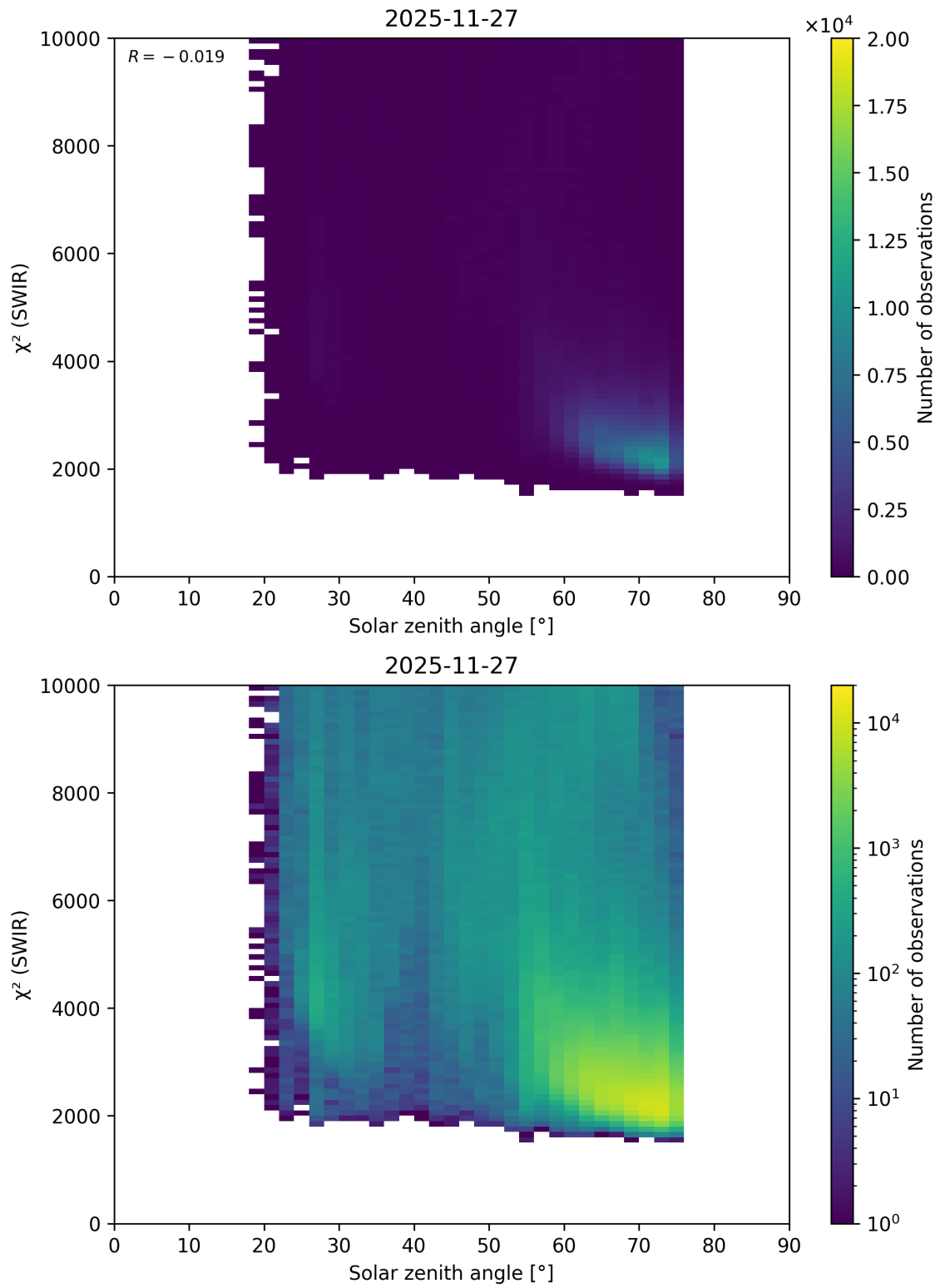
Figure 109: Scatter density plot of “Solar zenith angle” against “ \chi^2 (SWIR)” for 2025-11-26 to 2025-11-28.
