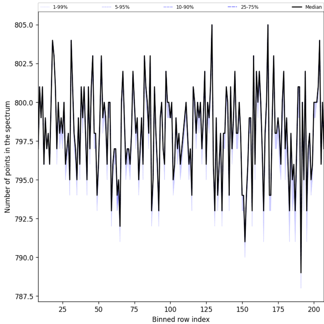
Figure 40: Along track statistics of “Number of points in the spectrum” for 2025-11-26 to 2025-11-28
