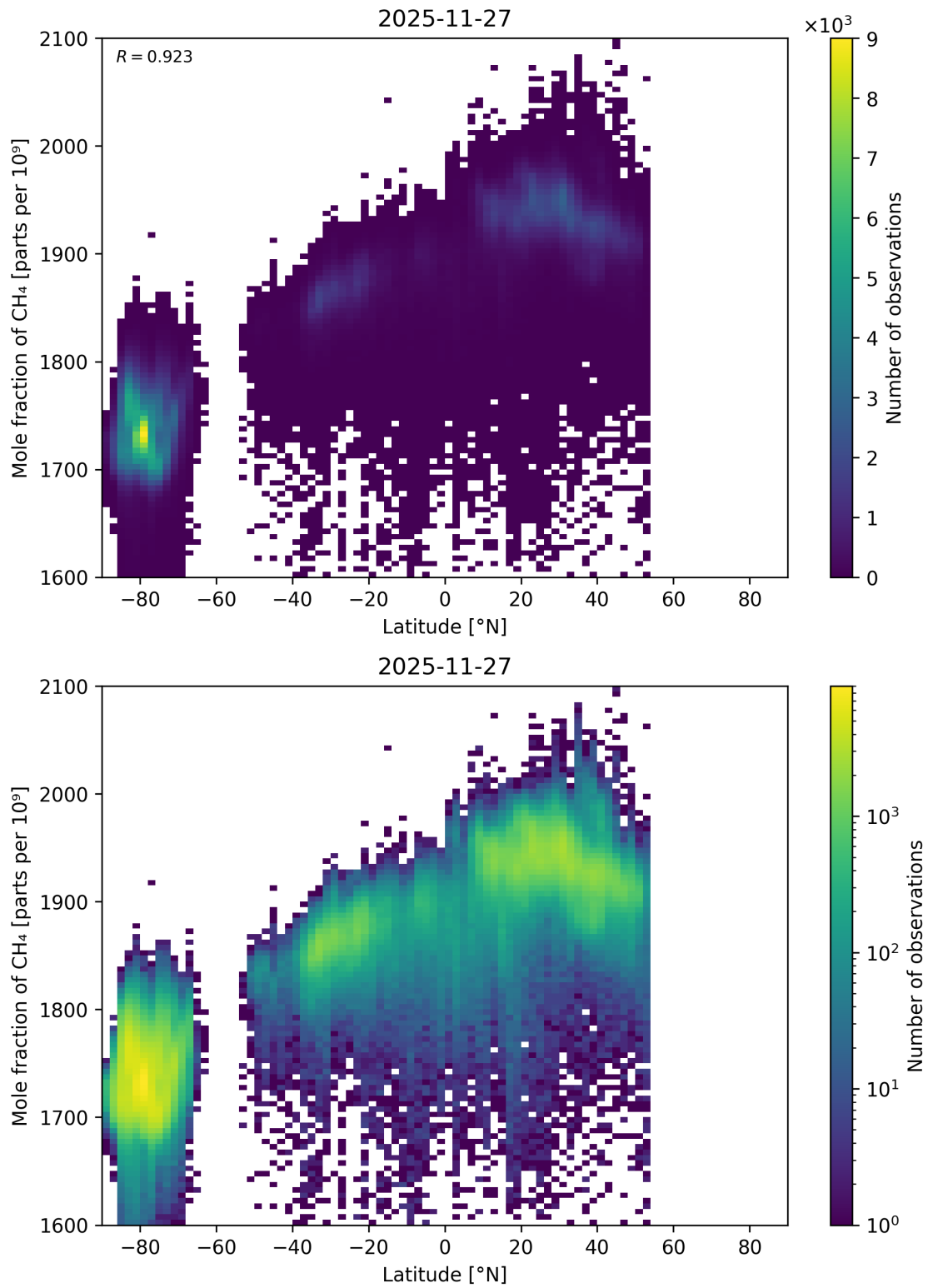
Figure 66: Scatter density plot of “Latitude” against “Mole fraction of CH 4 ” for 2025-11-26 to 2025-11-28.
