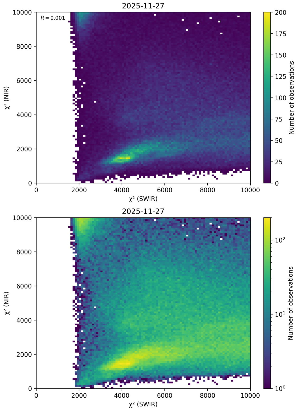
Figure 52: Scatter density plot of “ \chi^2 (SWIR)” against “ \chi^2 (NIR)” for 2025-11-26 to 2025-11-28.
