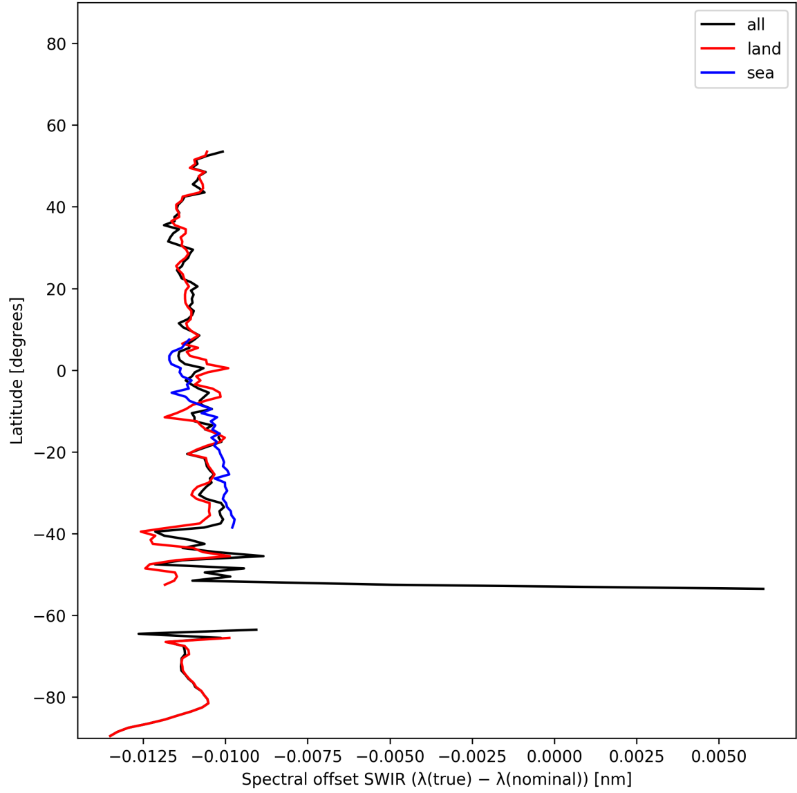
Figure 17: Zonal average of “Spectral offset SWIR ( \lambda_{\text{true}} - \lambda_{\text{nominal}} )” for 2025-11-26 to 2025-11-28.
