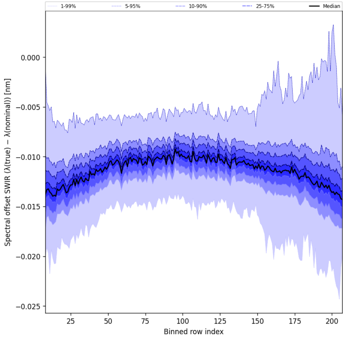
Figure 41: Along track statistics of “Spectral offset SWIR ( \lambda_{\text{true}} - \lambda_{\text{nominal}} )” for 2025-11-26 to 2025-11-28
