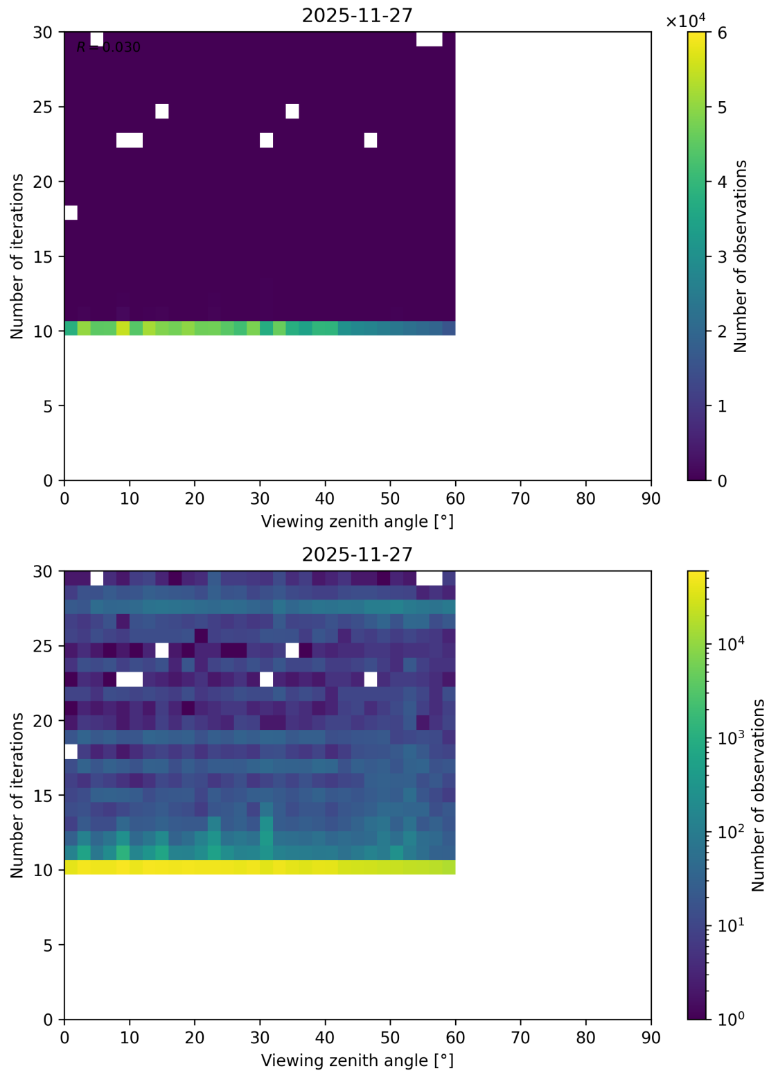
Figure 129: Scatter density plot of “Viewing zenith angle” against “Number of iterations” for 2025-11-26 to 2025-11-28.
