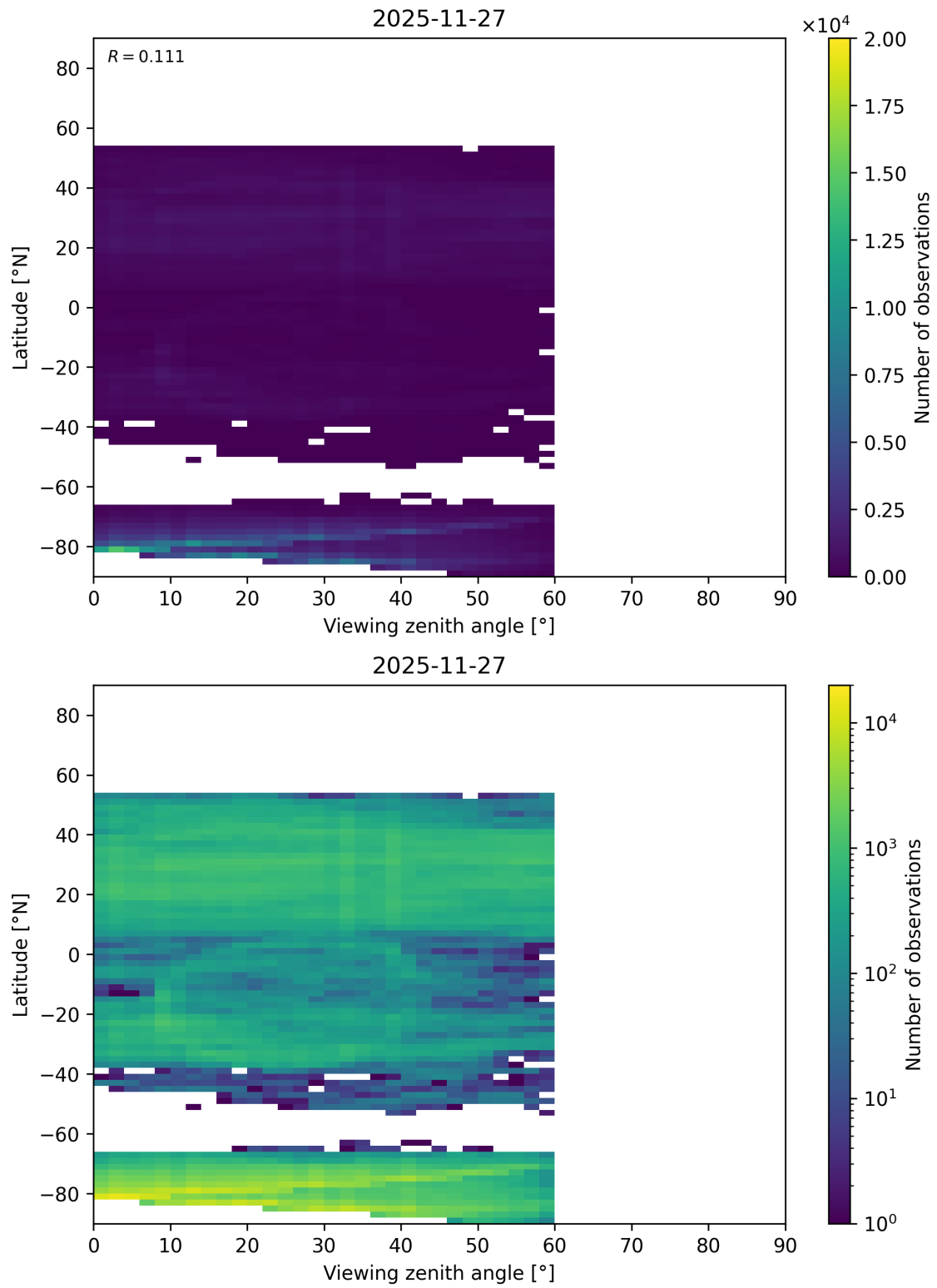
Figure 125: Scatter density plot of “Viewing zenith angle” against “Latitude” for 2025-11-26 to 2025-11-28.
