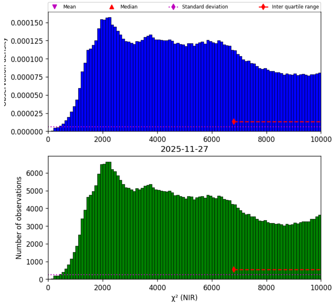
Figure 31: Histogram of “ \chi^2 (NIR)” for 2025-11-26 to 2025-11-28
