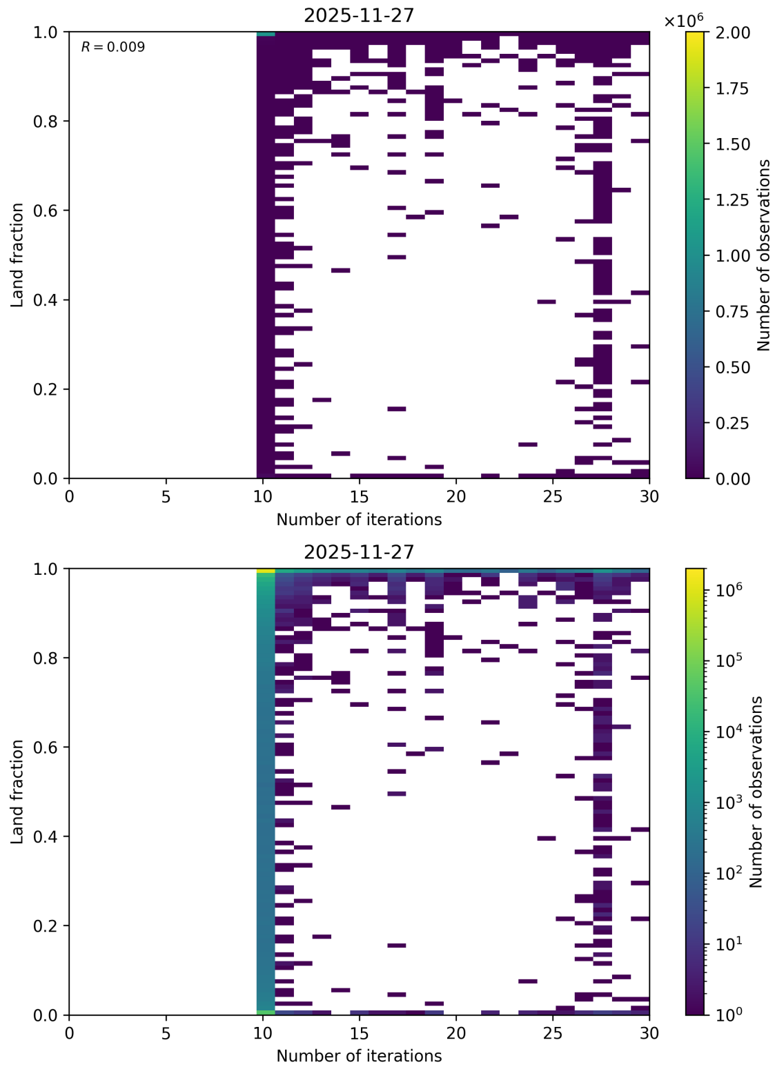
Figure 100: Scatter density plot of “Number of iterations” against “Land fraction” for 2025-11-26 to 2025-11-28.
