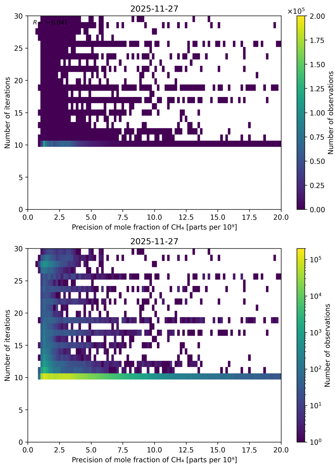
Figure 95: Scatter density plot of “Precision of mole fraction of CH 4 ” against “Number of iterations” for 2025-11-26 to 2025-11-28.
