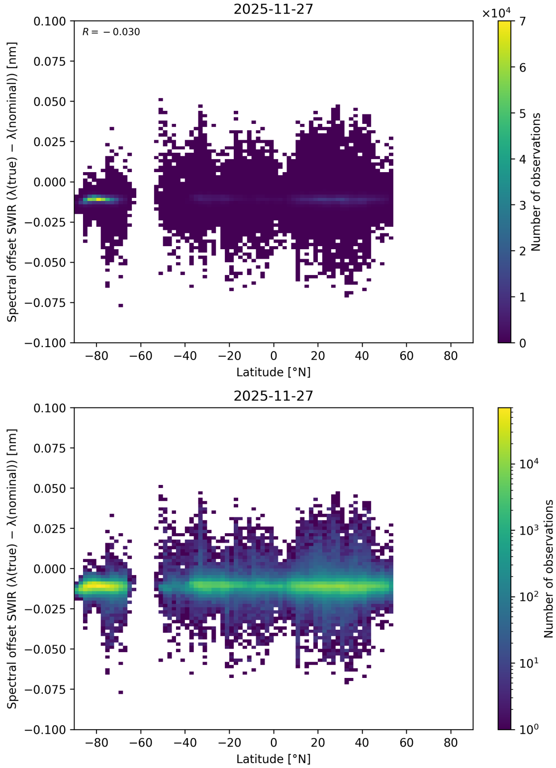
Figure 71: Scatter density plot of “Latitude” against “Spectral offset SWIR ( \lambda_{\text{true}} - \lambda_{\text{nominal}} )” for 2025-11-26 to 2025-11-28.
