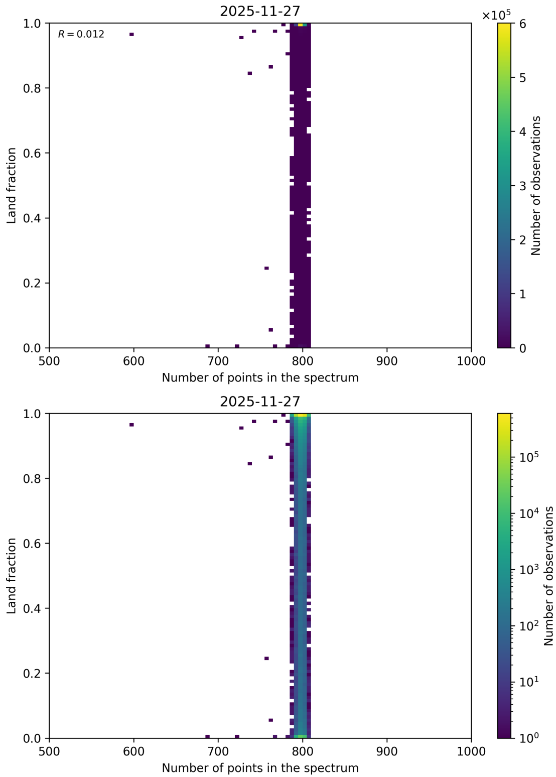
Figure 105: Scatter density plot of “Number of points in the spectrum” against “Land fraction” for 2025-11-26 to 2025-11-28.
