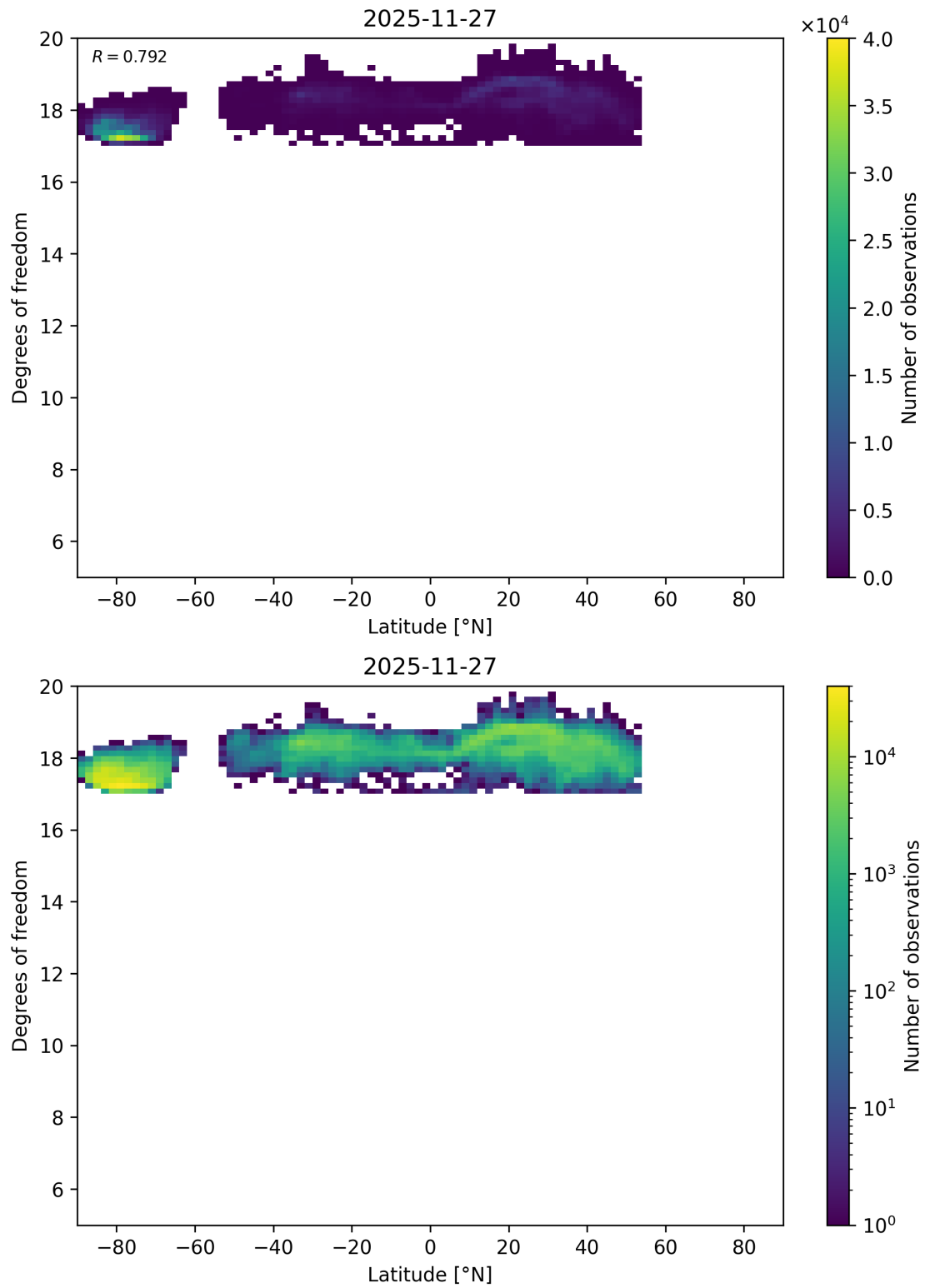
Figure 63: Scatter density plot of “Latitude” against “Degrees of freedom” for 2025-11-26 to 2025-11-28.
