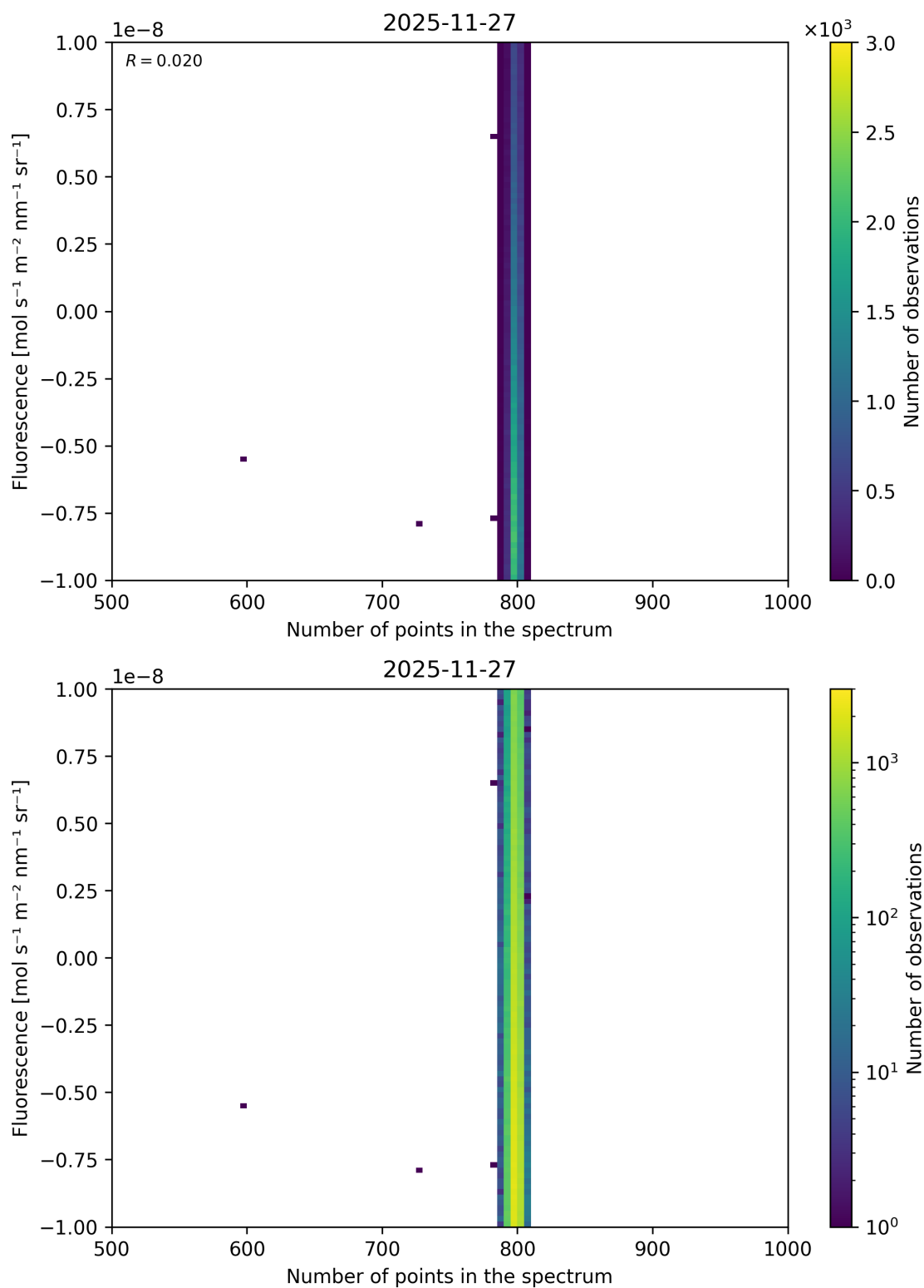
Figure 104: Scatter density plot of “Number of points in the spectrum” against “Fluorescence” for 2025-11-26 to 2025-11-28.
