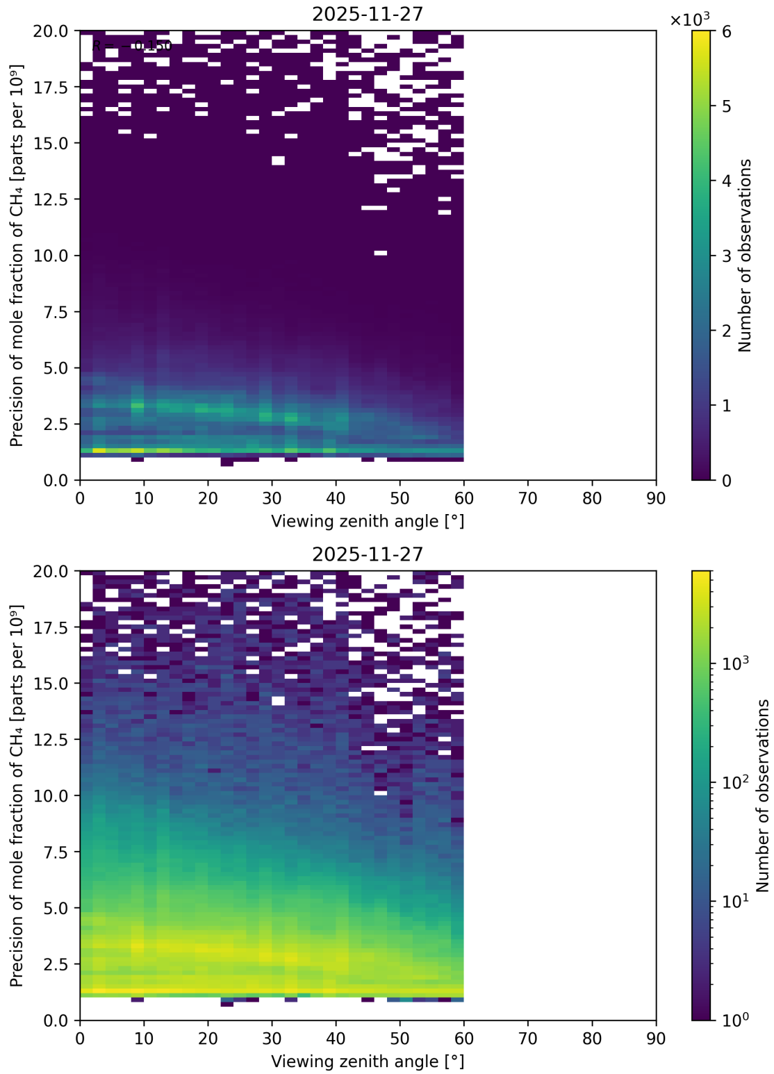
Figure 128: Scatter density plot of “Viewing zenith angle” against “Precision of mole fraction of CH 4 ” for 2025-11-26 to 2025-11-28.
