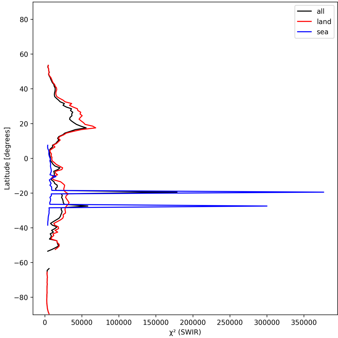
Figure 18: Zonal average of “ \chi^2 (SWIR)” for 2025-11-26 to 2025-11-28.
