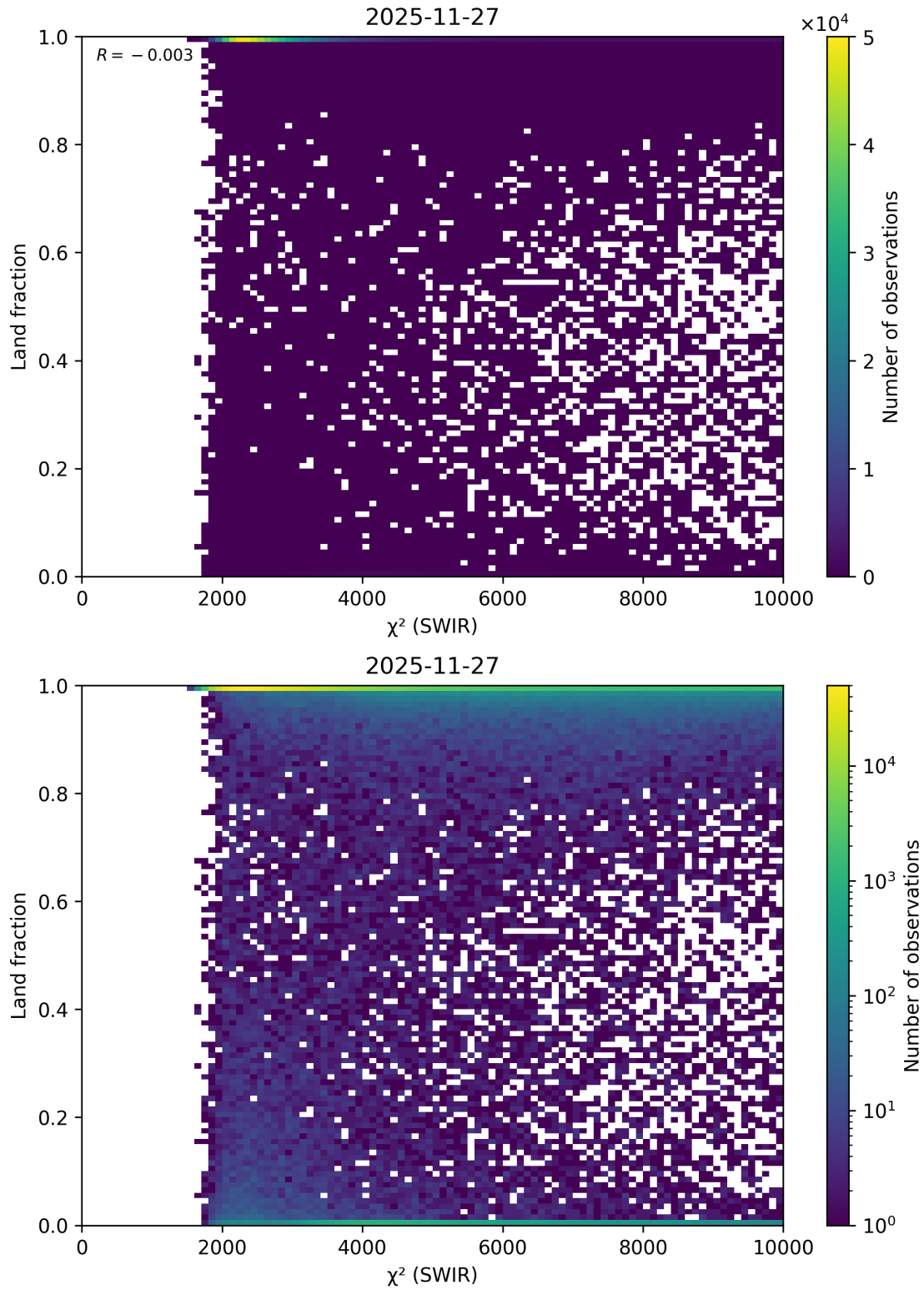
Figure 55: Scatter density plot of “ \chi^2 (SWIR)” against “Land fraction” for 2025-11-26 to 2025-11-28.
