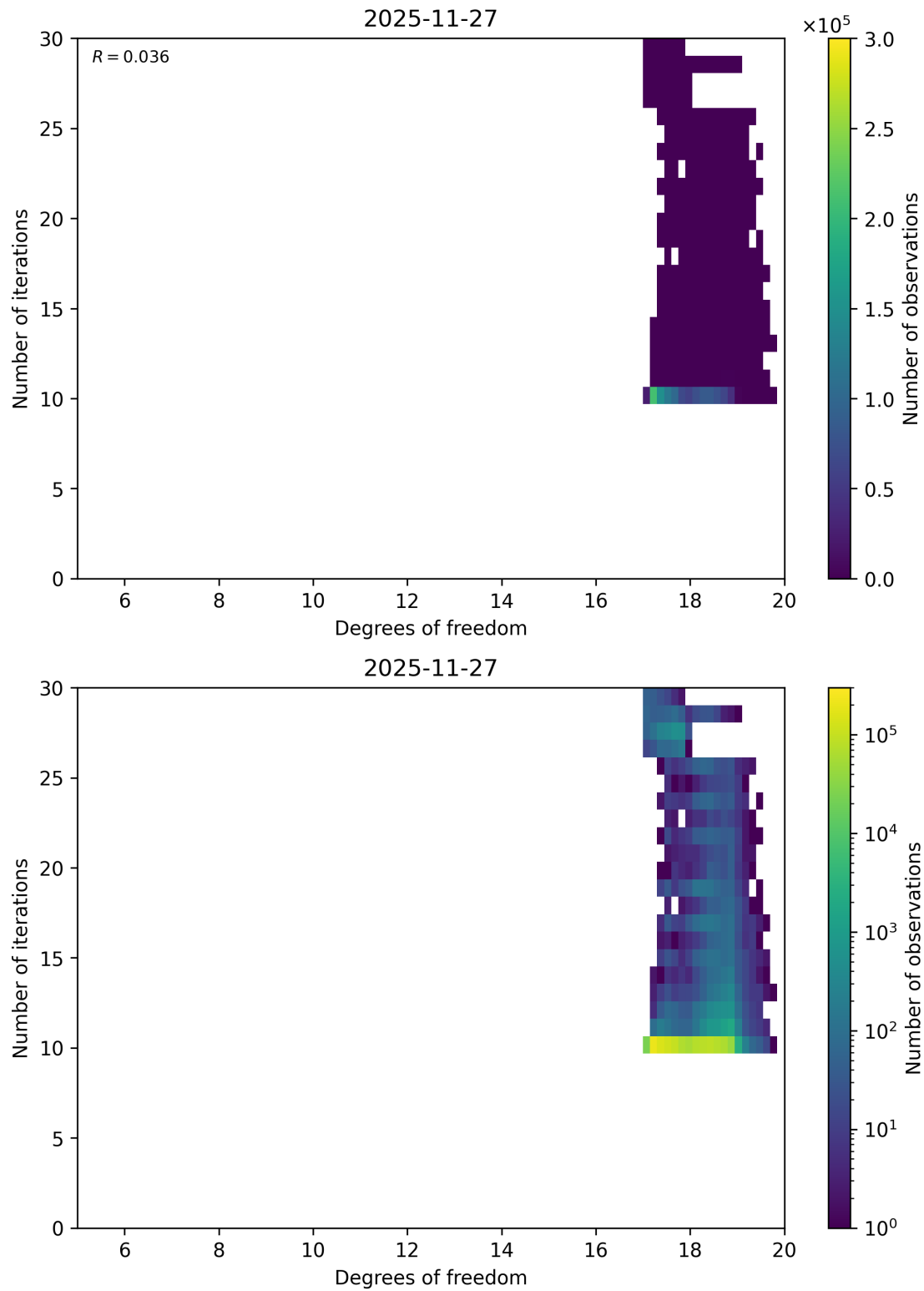
Figure 59: Scatter density plot of “Degrees of freedom” against “Number of iterations” for 2025-11-26 to 2025-11-28.
