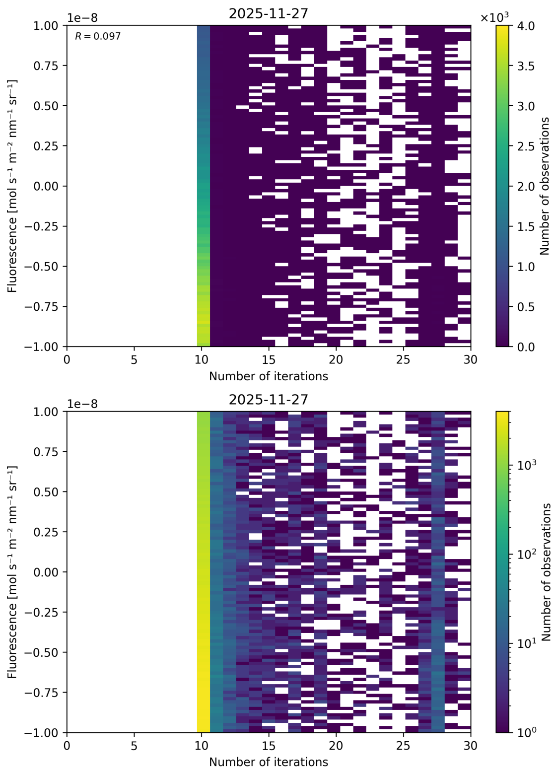
Figure 99: Scatter density plot of “Number of iterations” against “Fluorescence” for 2025-11-26 to 2025-11-28.
