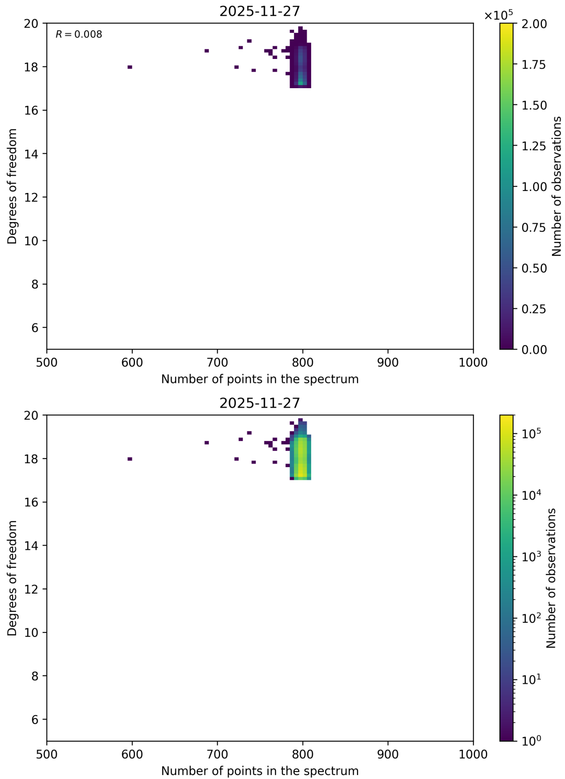
Figure 103: Scatter density plot of “Number of points in the spectrum” against “Degrees of freedom” for 2025-11-26 to 2025-11-28.
