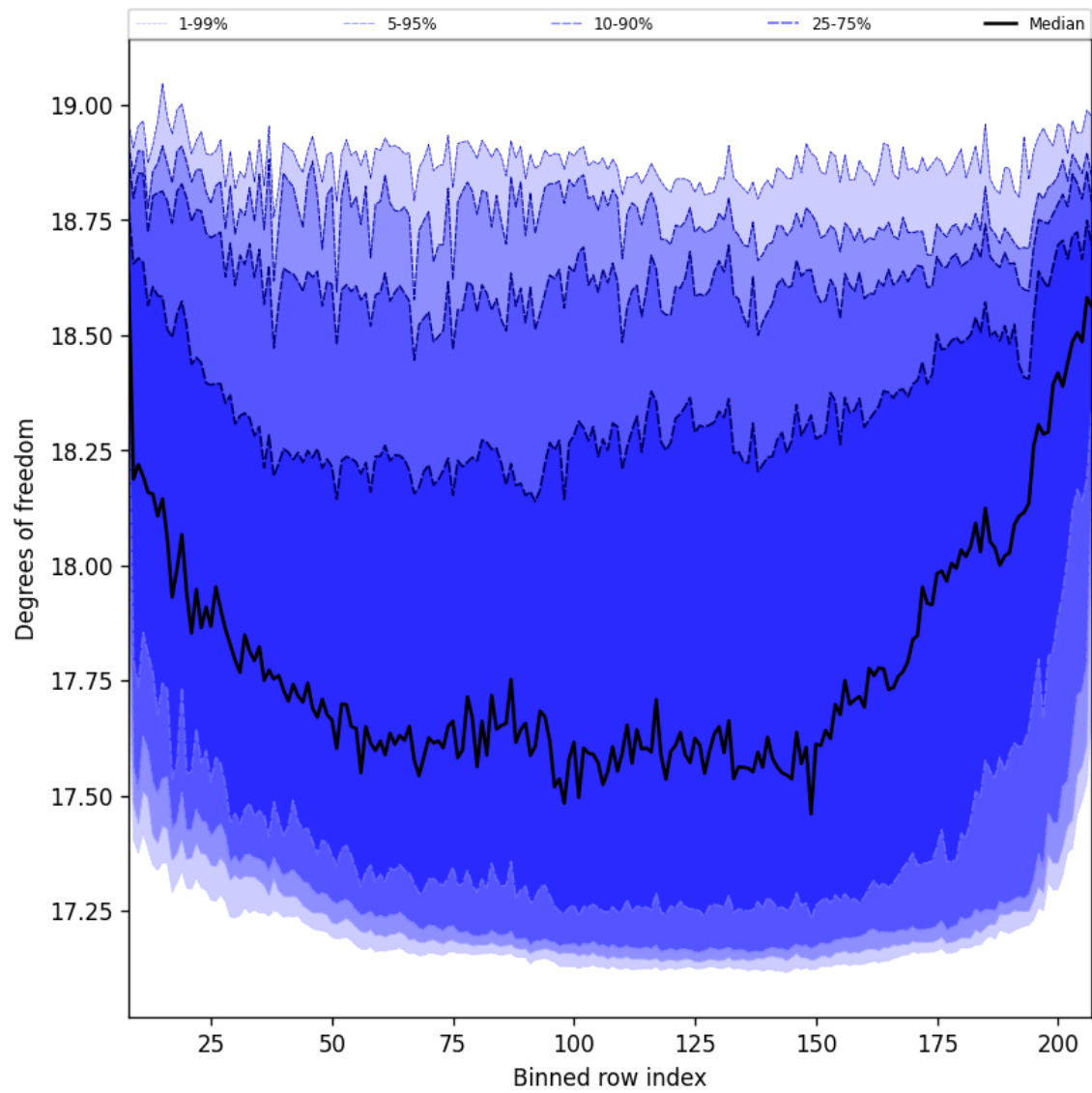
Figure 44: Along track statistics of “Degrees of freedom” for 2025-11-26 to 2025-11-28
