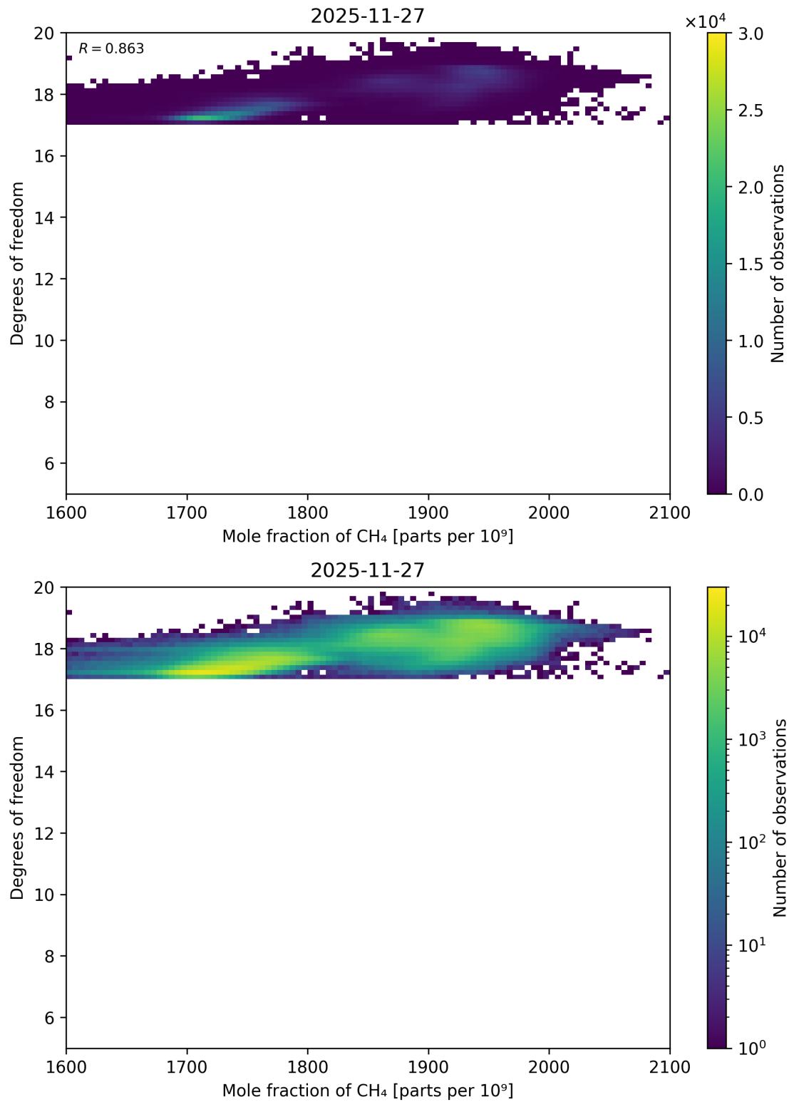
Figure 82: Scatter density plot of “Mole fraction of CH 4 ” against “Degrees of freedom” for 2025-11-26 to 2025-11-28.
