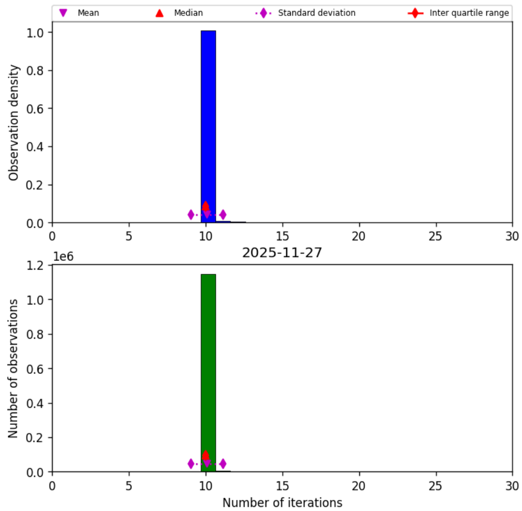
Figure 33: Histogram of “Number of iterations” for 2025-11-26 to 2025-11-28
