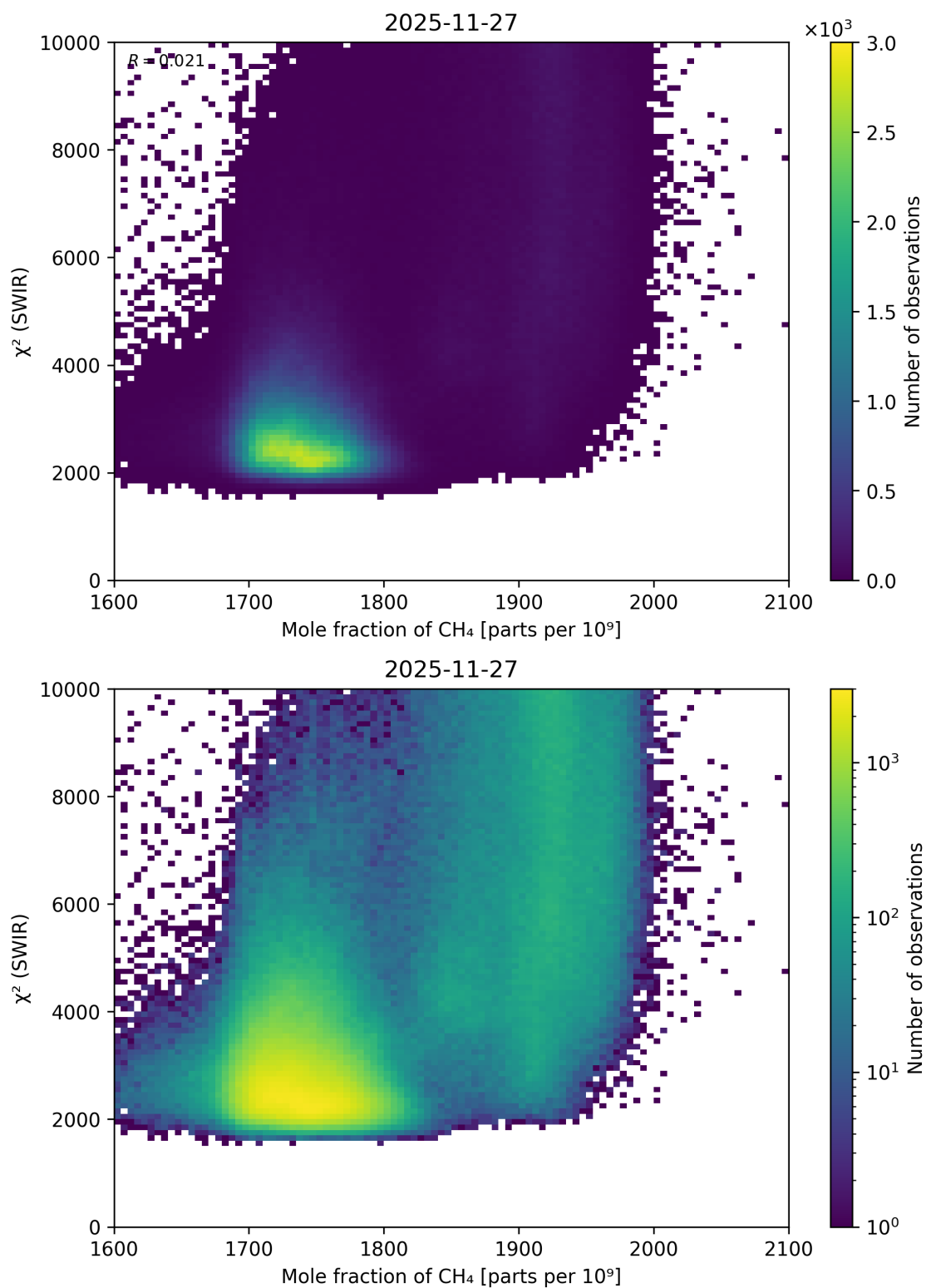
Figure 81: Scatter density plot of “Mole fraction of \text{CH}_4 ” against “ \chi^2 (SWIR)” for 2025-11-26 to 2025-11-28.
