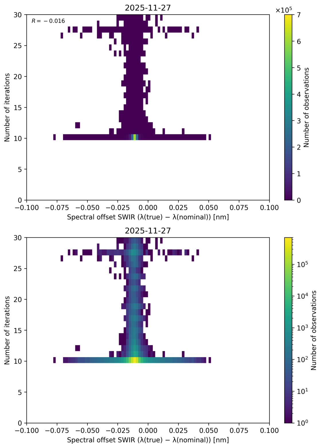
Figure 138: Scatter density plot of “Spectral offset SWIR ( \lambda_{\text{true}} - \lambda_{\text{nominal}} )” against “Number of iterations” for 2025-11-26 to 2025-11-28.
