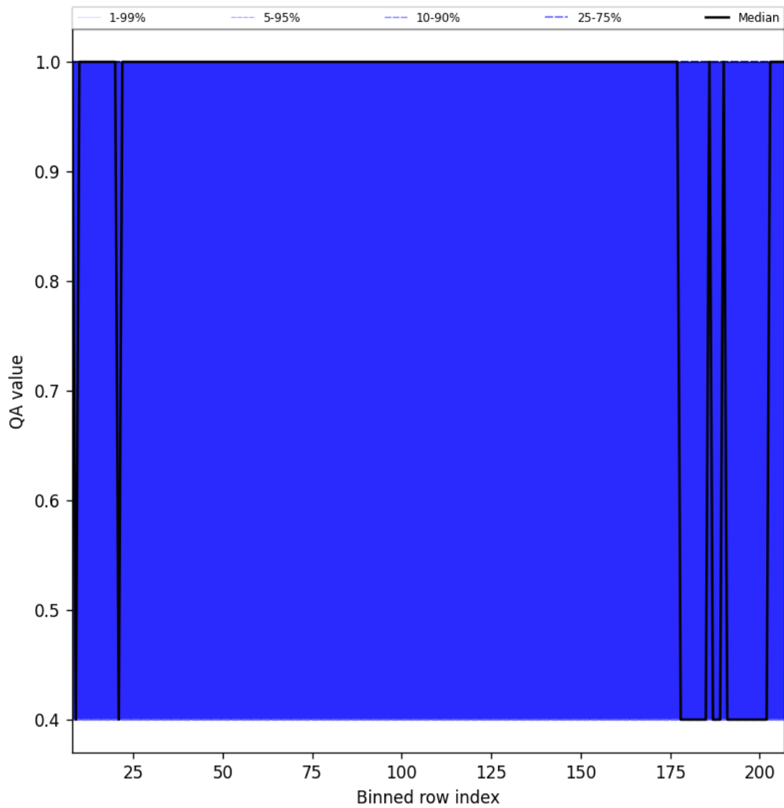
Figure 36: Along track statistics of “QA value” for 2025-11-26 to 2025-11-28
