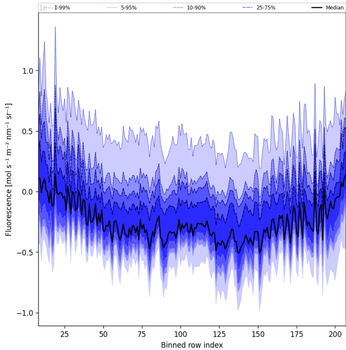
Figure 46: Along track statistics of “Fluorescence” for 2025-11-26 to 2025-11-28
