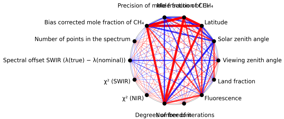
Figure 1: Map of correlation graph for 2025-11-26 to 2025-11-28.
