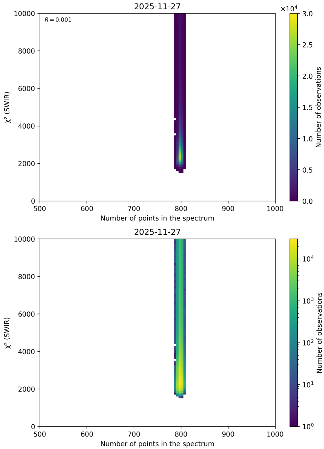
Figure 102: Scatter density plot of “Number of points in the spectrum” against “ \chi^2 (SWIR)” for 2025-11-26 to 2025-11-28.
