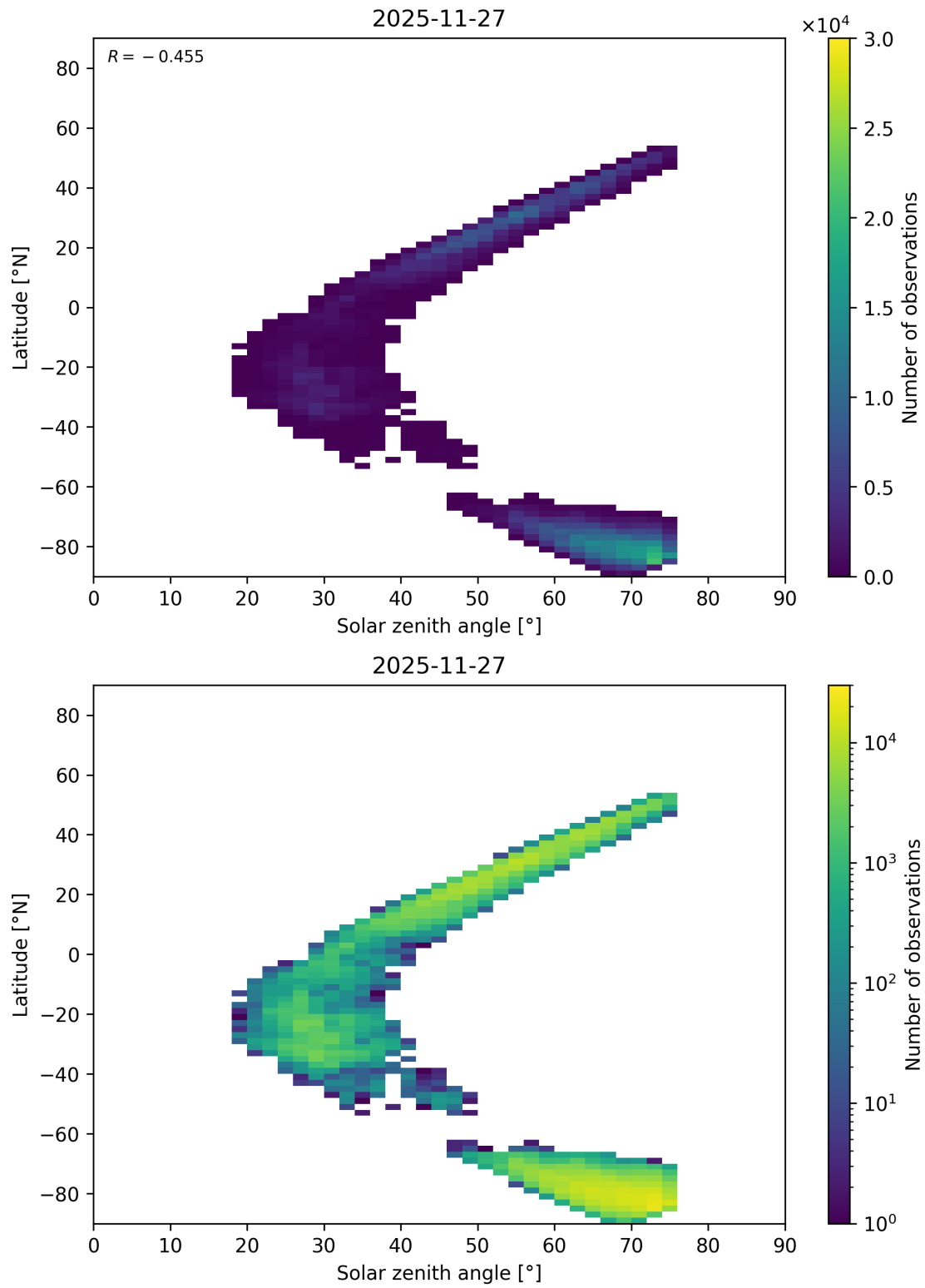
Figure 113: Scatter density plot of “Solar zenith angle” against “Latitude” for 2025-11-26 to 2025-11-28.
