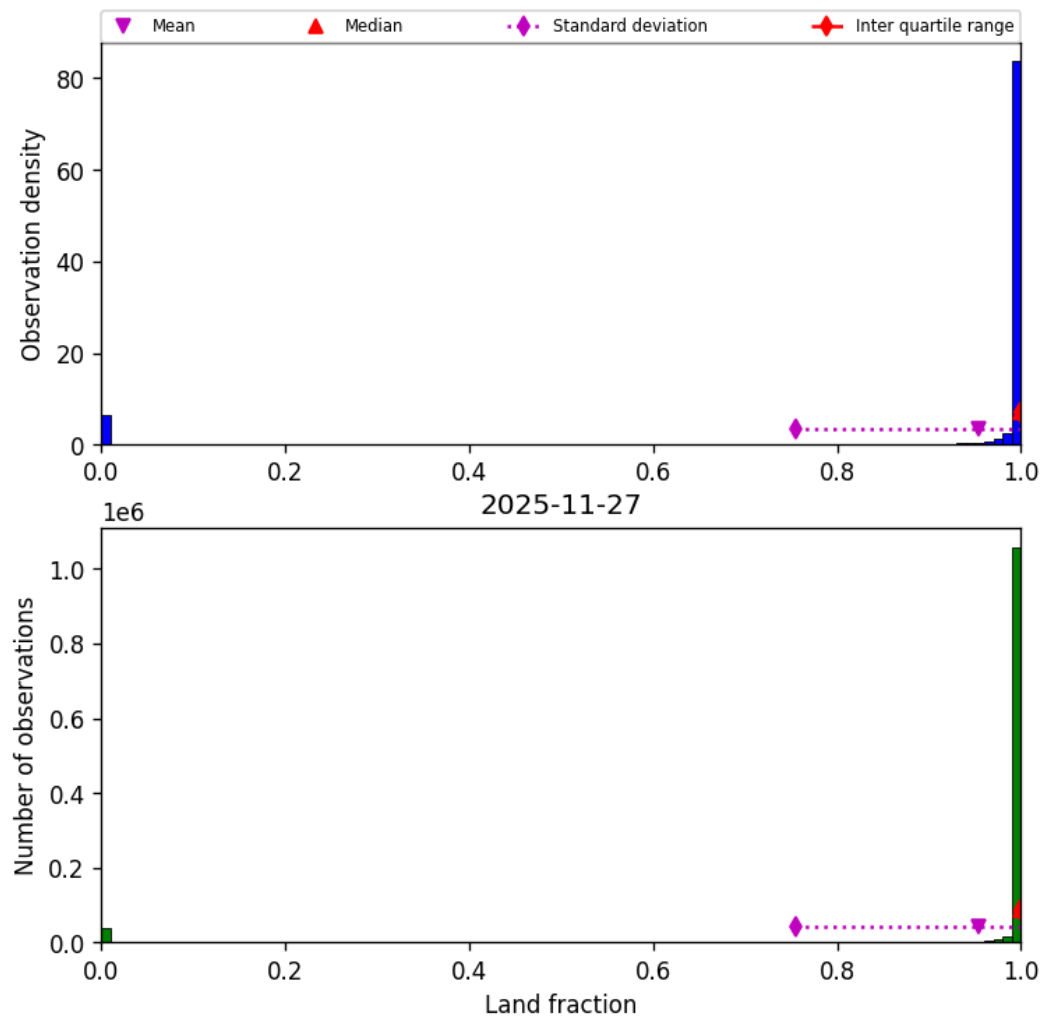
Figure 35: Histogram of “Land fraction” for 2025-11-26 to 2025-11-28
