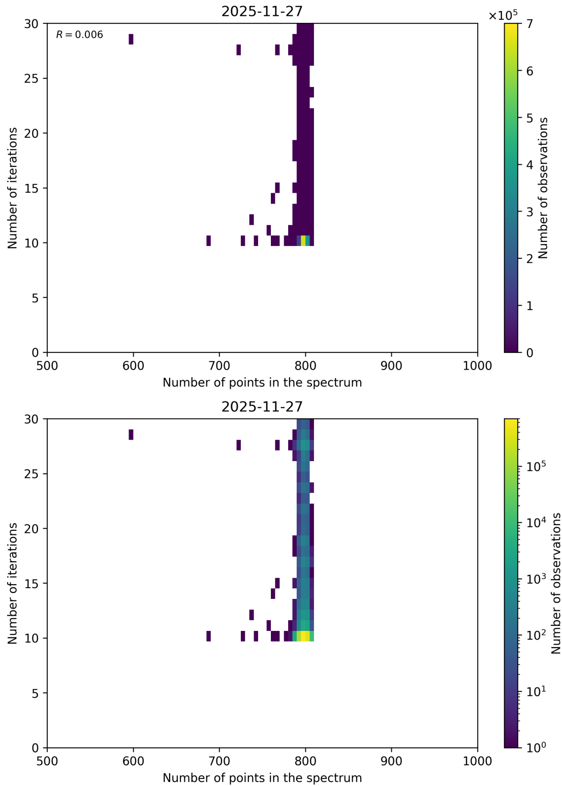
Figure 106: Scatter density plot of “Number of points in the spectrum” against “Number of iterations” for 2025-11-26 to 2025-11-28.
