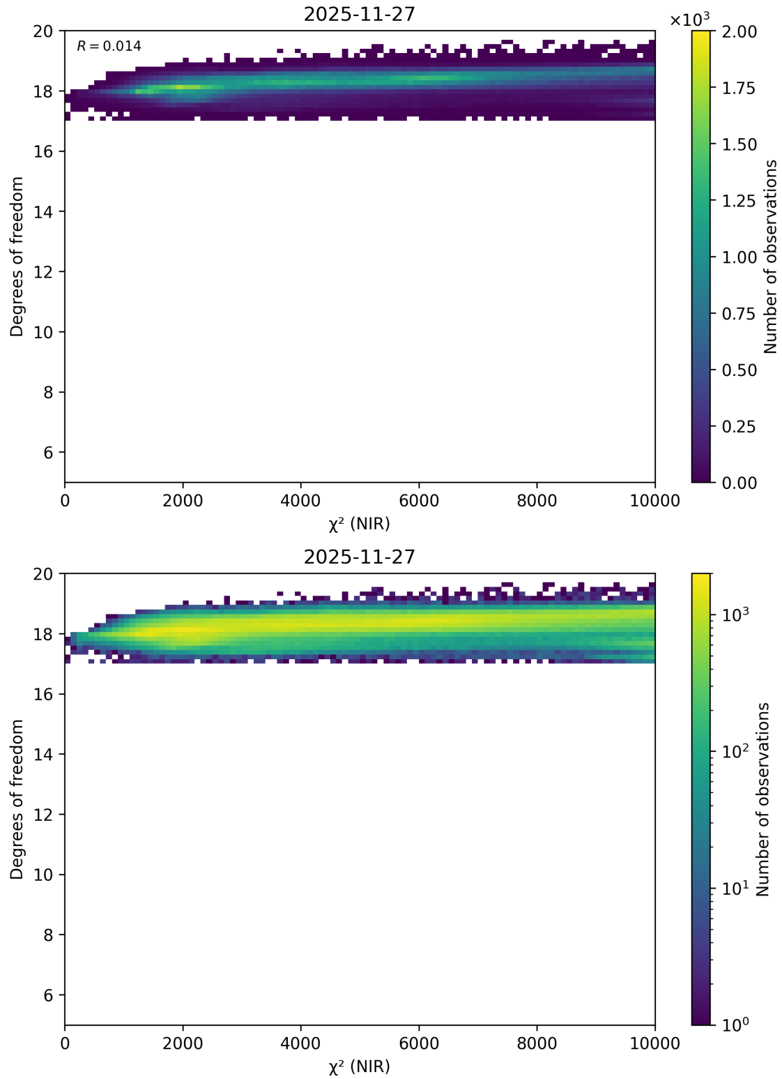
Figure 48: Scatter density plot of “ \chi^2 (NIR)” against “Degrees of freedom” for 2025-11-26 to 2025-11-28.
