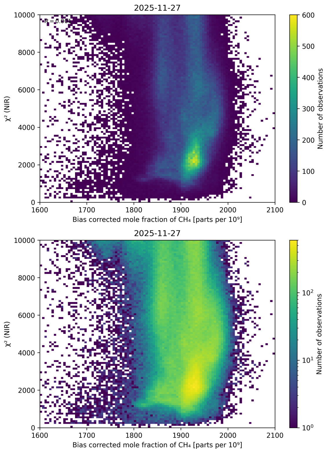
Figure 72: Scatter density plot of “Bias corrected mole fraction of CH 4 ” against “ \chi^2 (NIR)” for 2025-11-26 to 2025-11-28.
