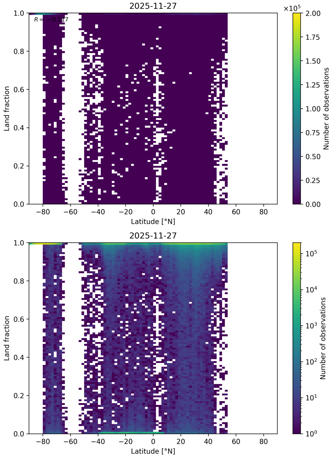
Figure 65: Scatter density plot of “Latitude” against “Land fraction” for 2025-11-26 to 2025-11-28.
