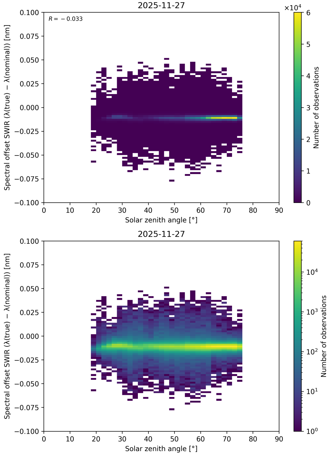
Figure 119: Scatter density plot of “Solar zenith angle” against “Spectral offset SWIR ( \lambda_{\text{true}} - \lambda_{\text{nominal}} )” for 2025-11-26 to 2025-11-28.
