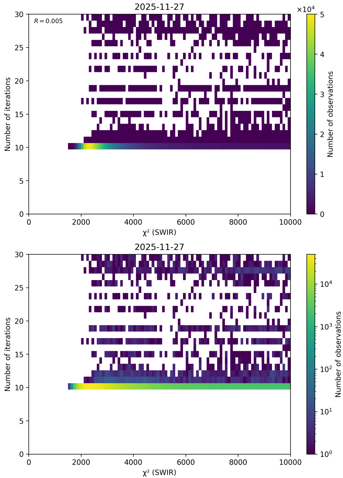
Figure 56: Scatter density plot of “ \chi^2 (SWIR)” against “Number of iterations” for 2025-11-26 to 2025-11-28.
