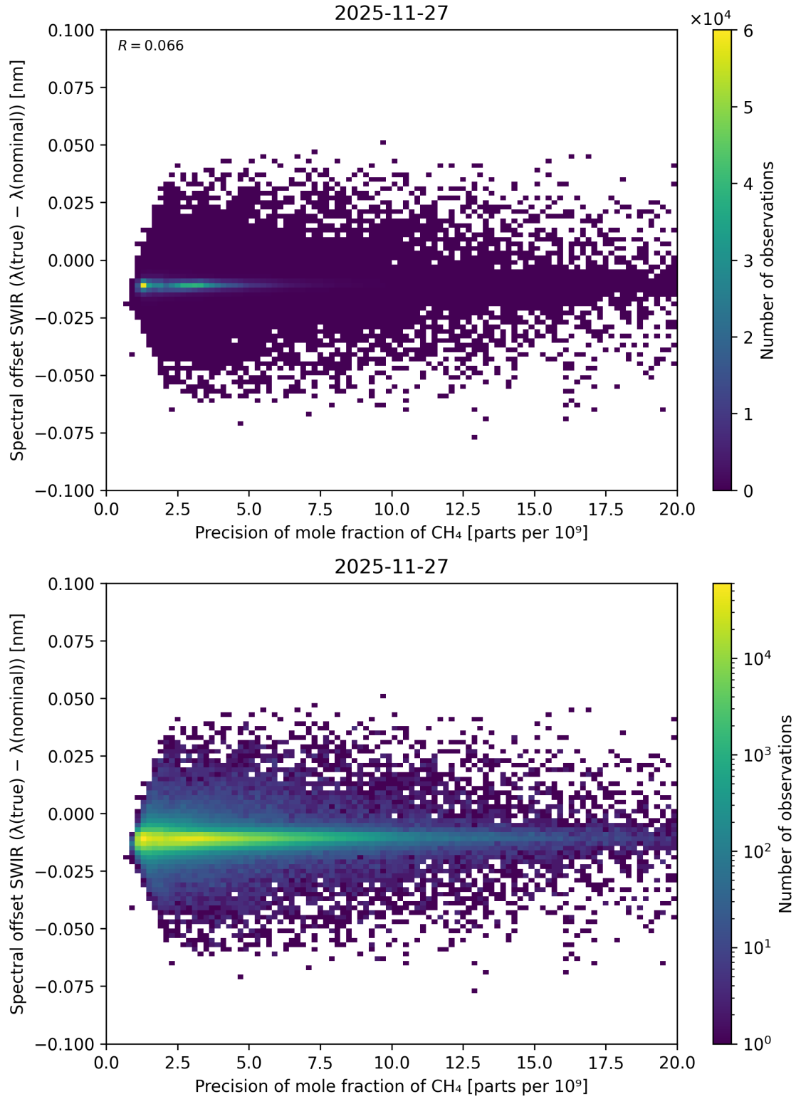
Figure 97: Scatter density plot of “Precision of mole fraction of \text{CH}_4 ” against “Spectral offset SWIR ( \lambda_{\text{true}} - \lambda_{\text{nominal}} )” for 2025-11-26 to 2025-11-28.
