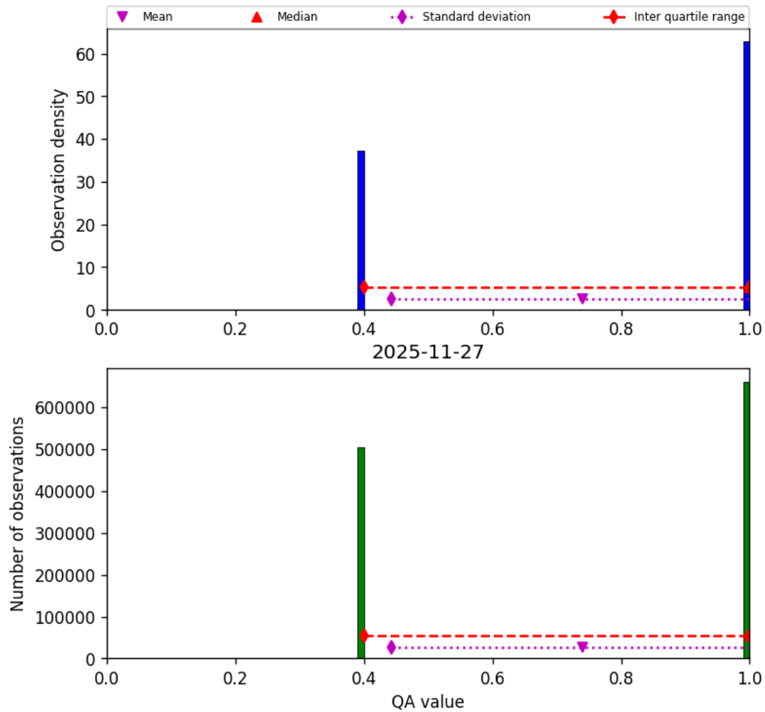
Figure 24: Histogram of “QA value” for 2025-11-26 to 2025-11-28
