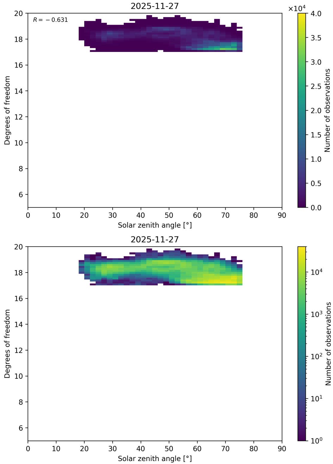
Figure 110: Scatter density plot of “Solar zenith angle” against “Degrees of freedom” for 2025-11-26 to 2025-11-28.
