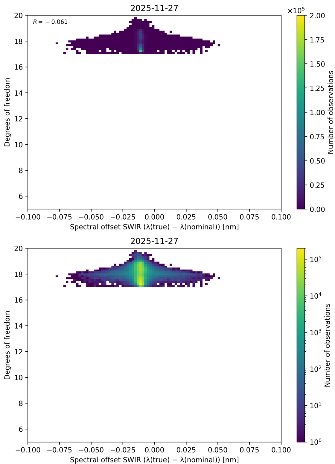
Figure 135: Scatter density plot of “Spectral offset SWIR ( \lambda_{\text{true}} - \lambda_{\text{nominal}} )” against “Degrees of freedom” for 2025-11-26 to 2025-11-28.
