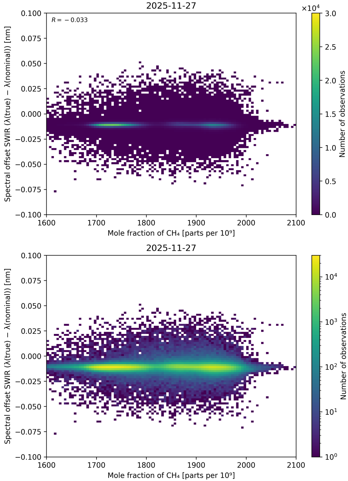
Figure 98: Scatter density plot of “Mole fraction of CH 4 ” against “Spectral offset SWIR ( \lambda_{\text{true}} - \lambda_{\text{nominal}} )” for 2025-11-26 to 2025-11-28.
