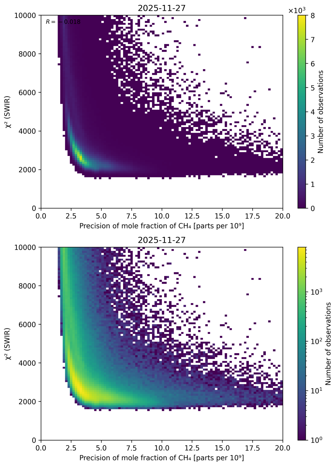
Figure 90: Scatter density plot of “Precision of mole fraction of \text{CH}_4 ” against “ \chi^2 (SWIR)” for 2025-11-26 to 2025-11-28.
