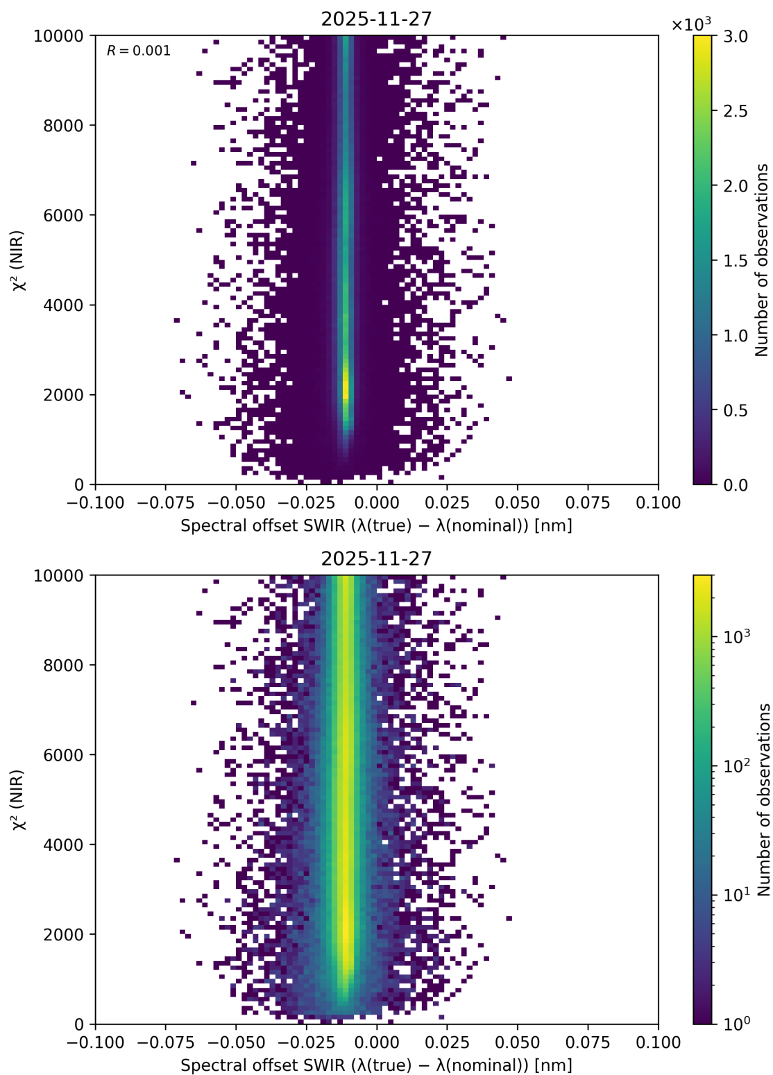
Figure 133: Scatter density plot of “Spectral offset SWIR ( \lambda_{\text{true}} - \lambda_{\text{nominal}} )” against “ \chi^2 (NIR)” for 2025-11-26 to 2025-11-28.
