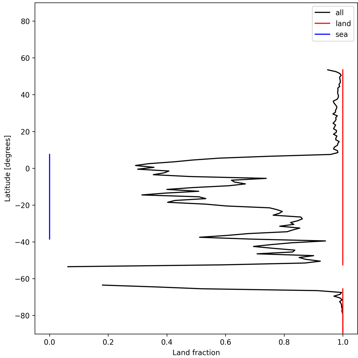
Figure 23: Zonal average of “Land fraction” for 2025-11-26 to 2025-11-28.
