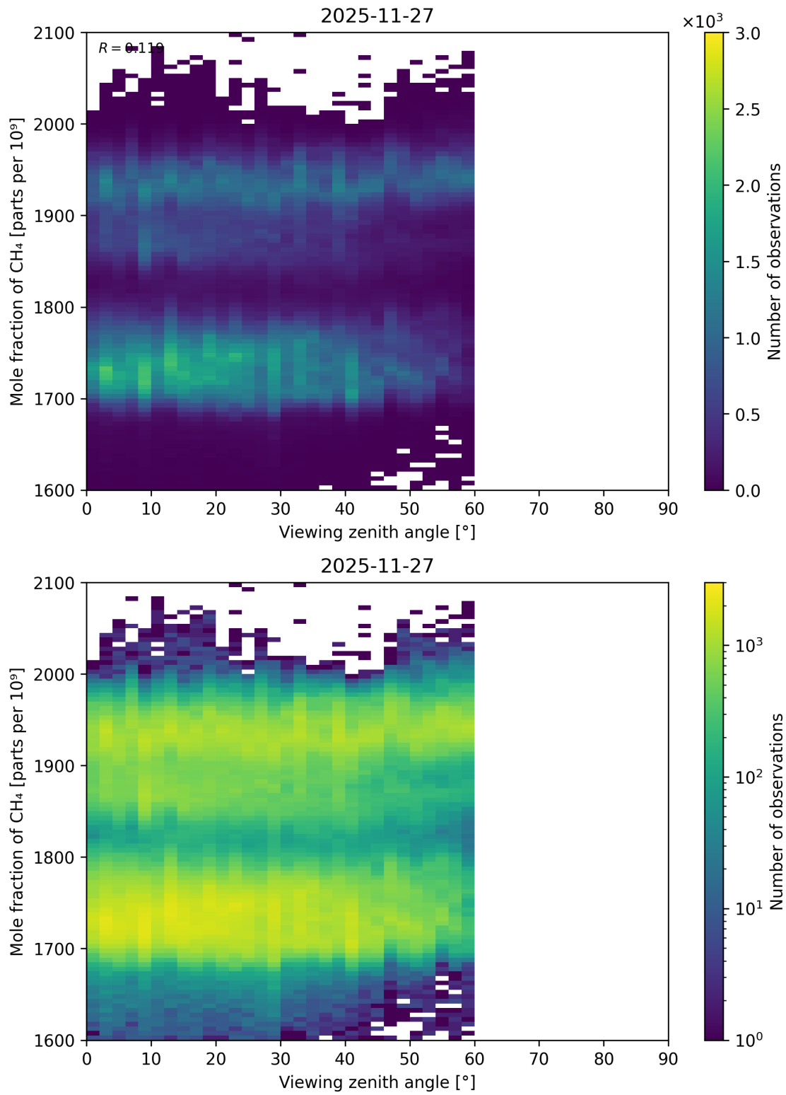
Figure 126: Scatter density plot of “Viewing zenith angle” against “Mole fraction of CH 4 ” for 2025-11-26 to 2025-11-28.
