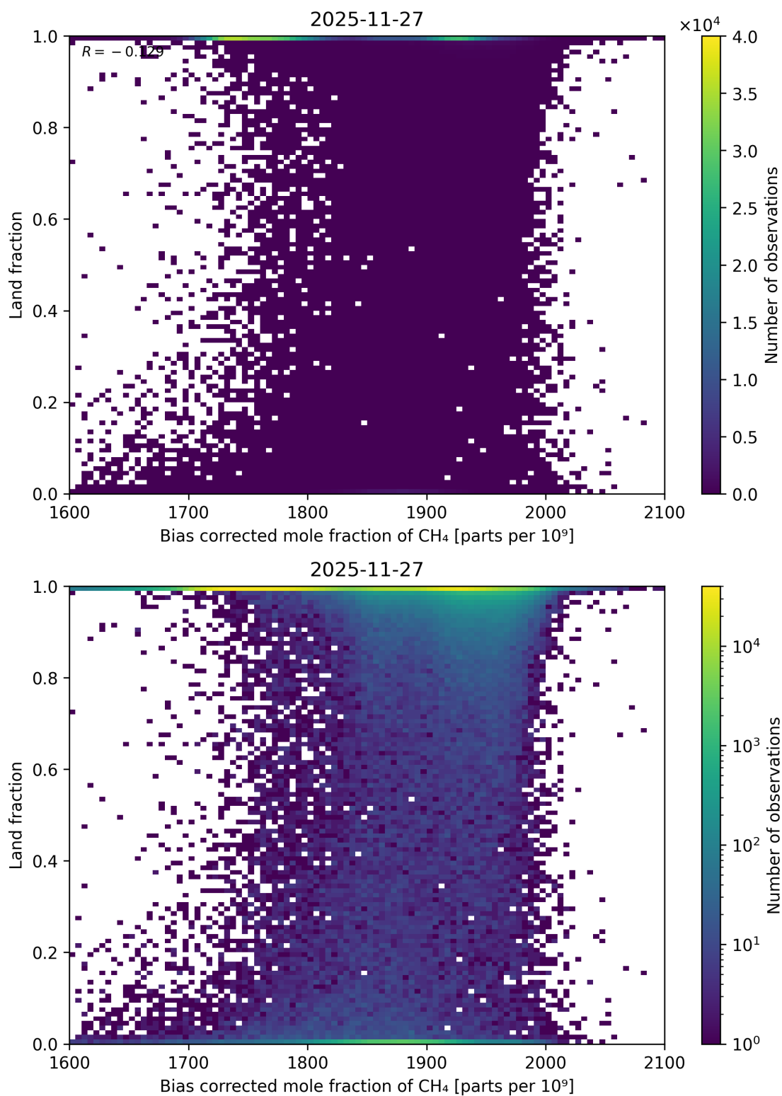
Figure 76: Scatter density plot of “Bias corrected mole fraction of CH 4 ” against “Land fraction” for 2025-11-26 to 2025-11-28.
