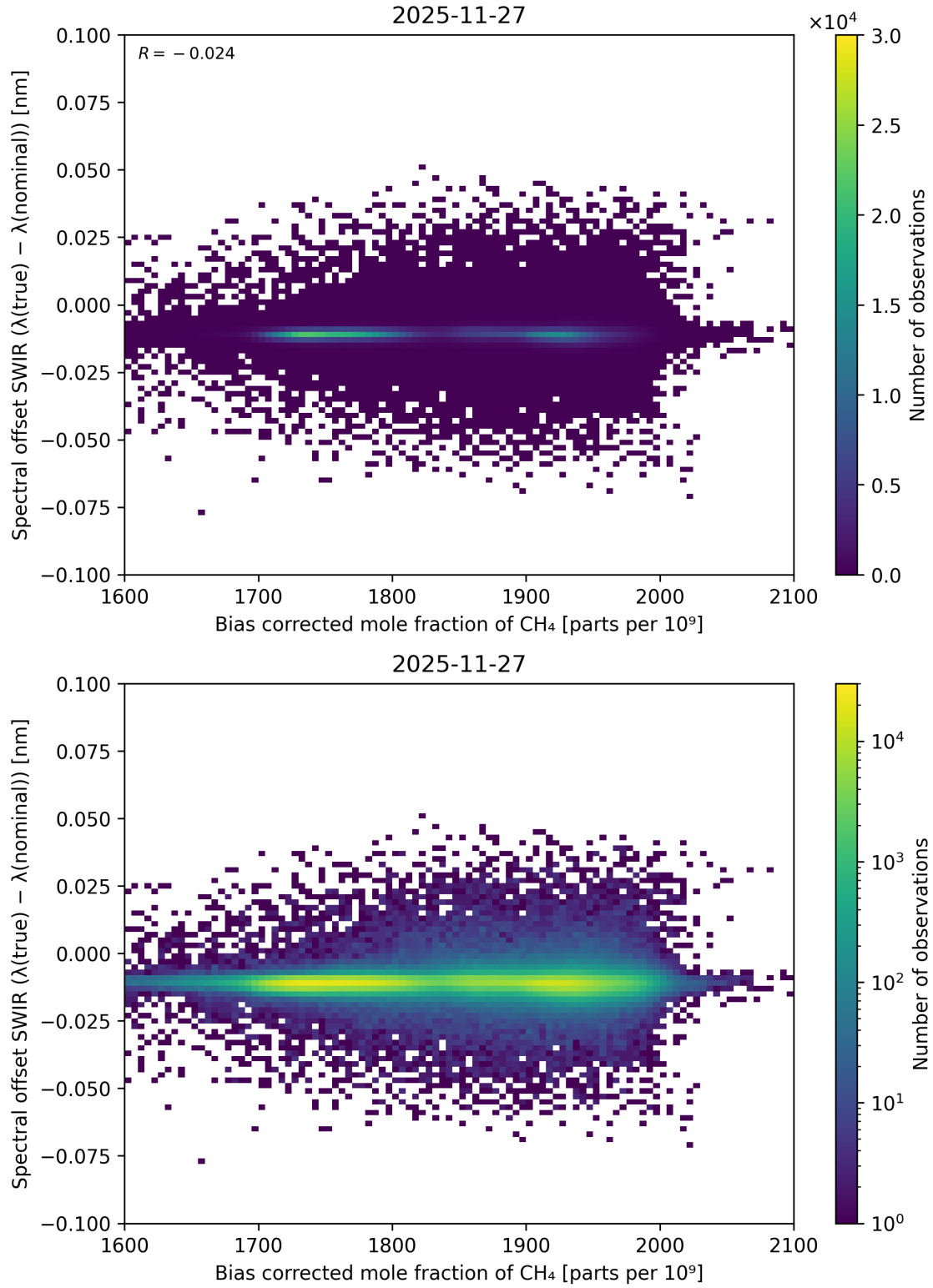
Figure 79: Scatter density plot of “Bias corrected mole fraction of \text{CH}_4 ” against “Spectral offset SWIR ( \lambda_{\text{true}} - \lambda_{\text{nominal}} )” for 2025-11-26 to 2025-11-28.
