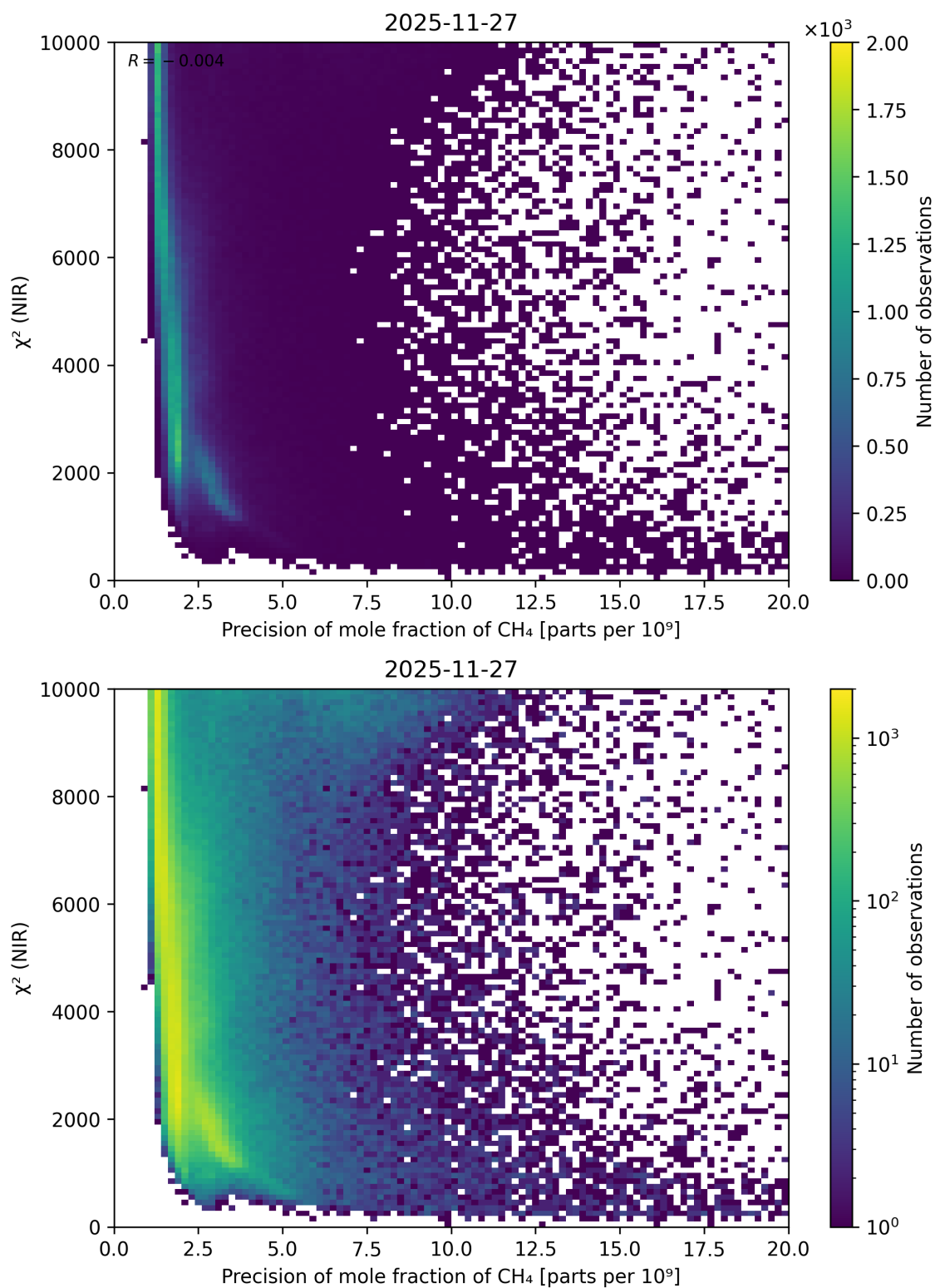
Figure 89: Scatter density plot of “Precision of mole fraction of CH 4 ” against “ \chi^2 (NIR)” for 2025-11-26 to 2025-11-28.
