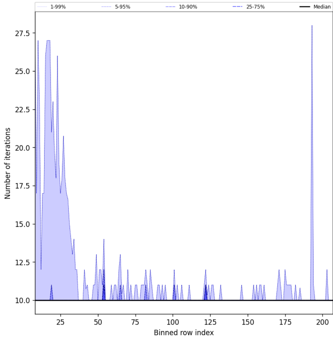
Figure 45: Along track statistics of “Number of iterations” for 2025-11-26 to 2025-11-28
