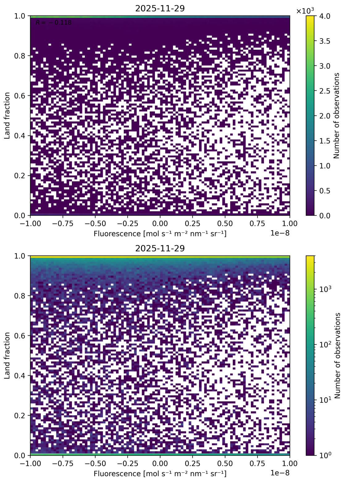
Figure 60: Scatter density plot of “Fluorescence” against “Land fraction” for 2025-11-28 to 2025-11-30.
