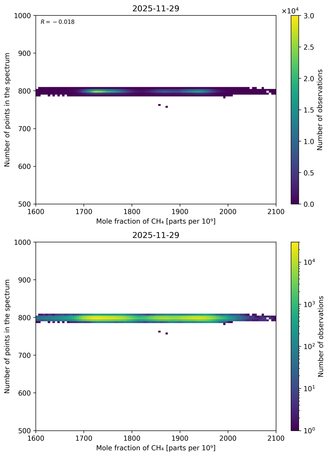
Figure 88: Scatter density plot of “Mole fraction of CH 4 ” against “Number of points in the spectrum” for 2025-11-28 to 2025-11-30.
