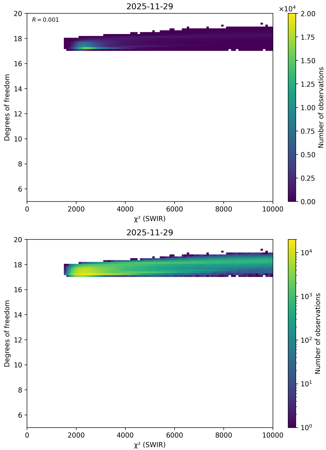
Figure 53: Scatter density plot of “ \chi^2 (SWIR)” against “Degrees of freedom” for 2025-11-28 to 2025-11-30.
