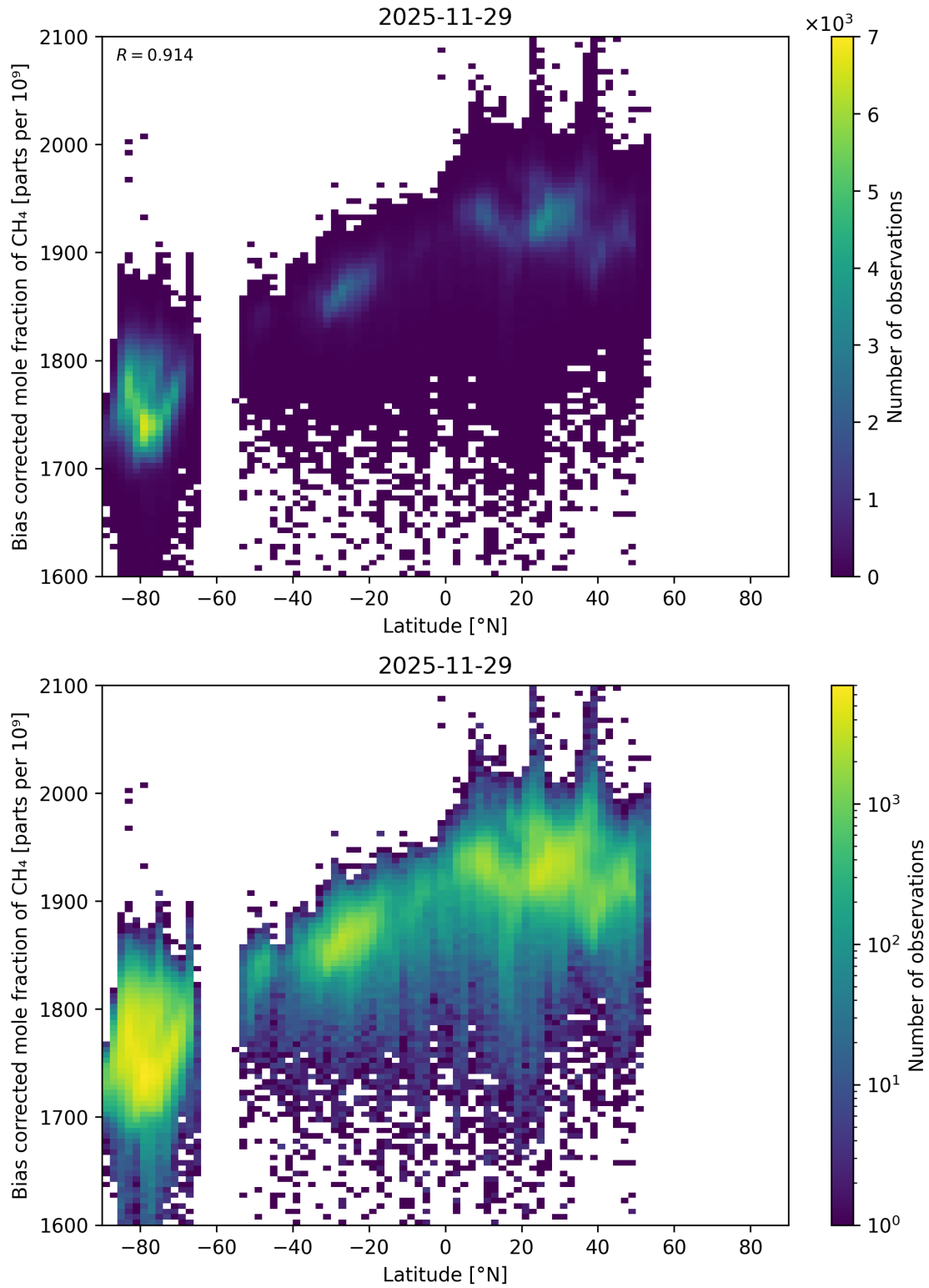
Figure 67: Scatter density plot of “Latitude” against “Bias corrected mole fraction of CH 4 ” for 2025-11-28 to 2025-11-30.
