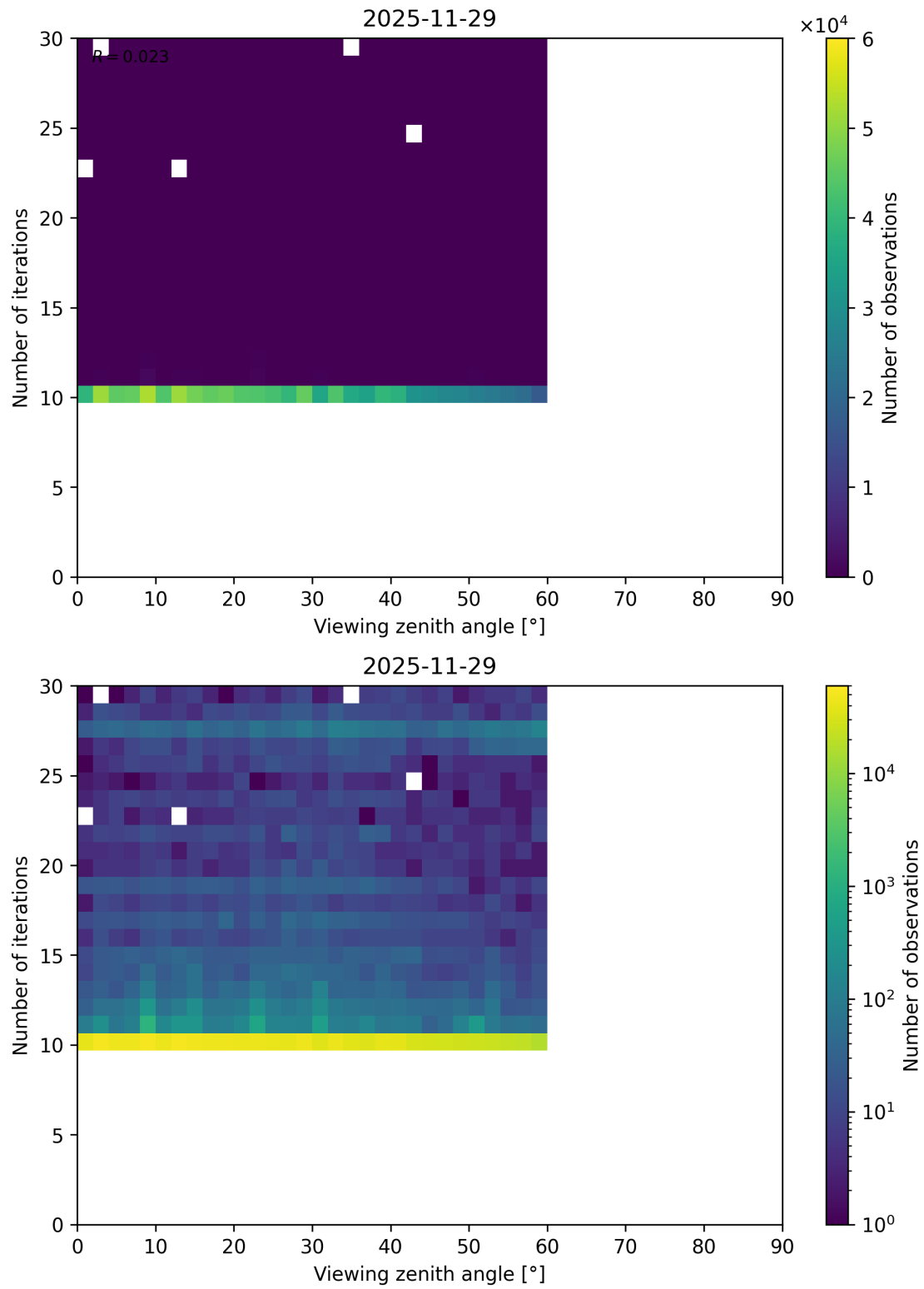
Figure 129: Scatter density plot of “Viewing zenith angle” against “Number of iterations” for 2025-11-28 to 2025-11-30.
