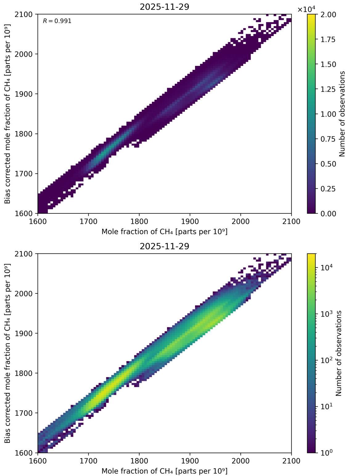
Figure 85: Scatter density plot of “Mole fraction of CH 4 ” against “Bias corrected mole fraction of CH 4 ” for 2025-11-28 to 2025-11-30.
