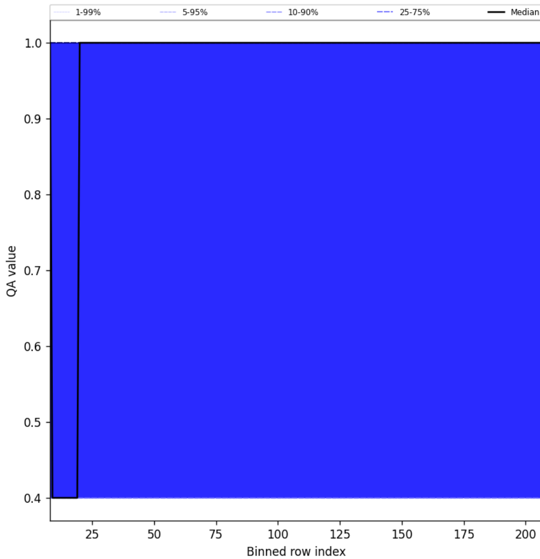
Figure 36: Along track statistics of “QA value” for 2025-11-28 to 2025-11-30
