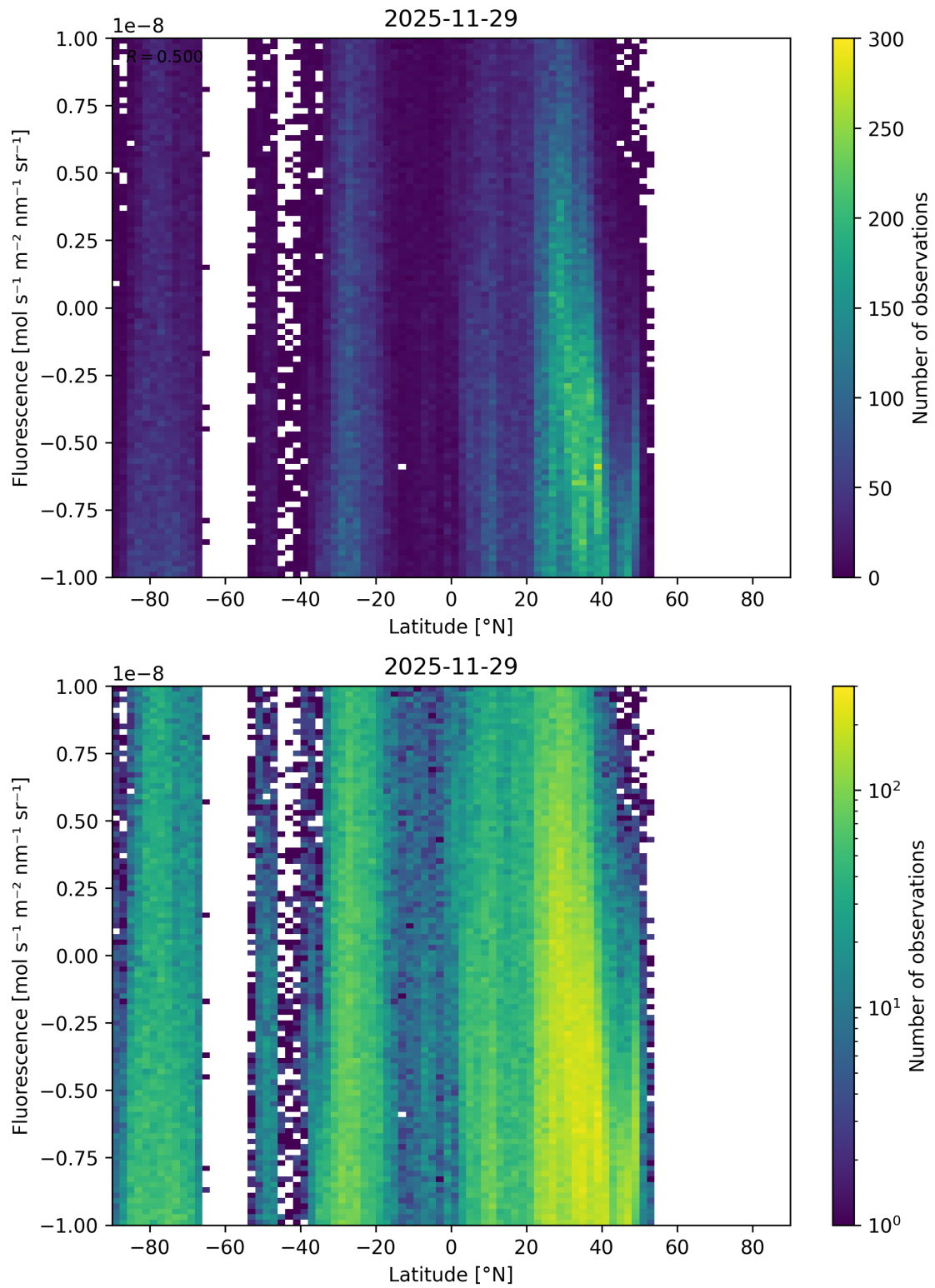
Figure 64: Scatter density plot of “Latitude” against “Fluorescence” for 2025-11-28 to 2025-11-30.
