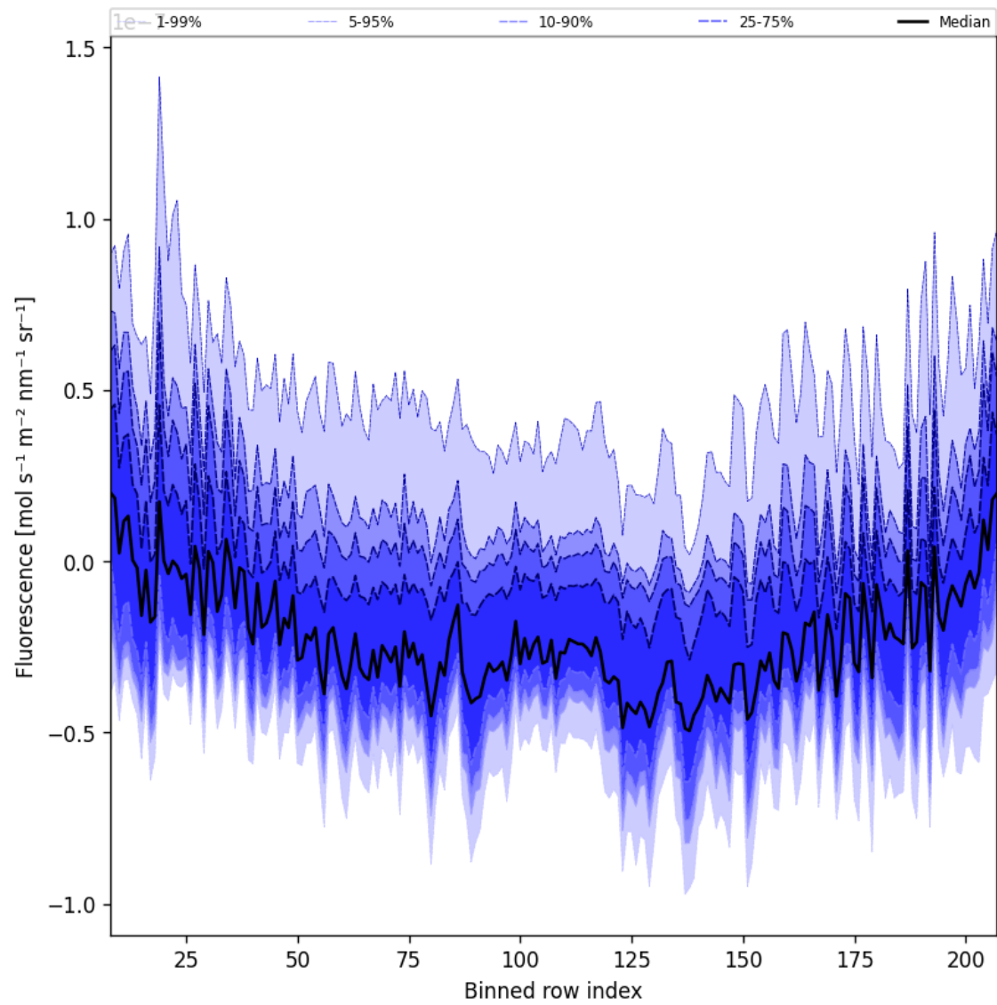
Figure 46: Along track statistics of “Fluorescence” for 2025-11-28 to 2025-11-30
