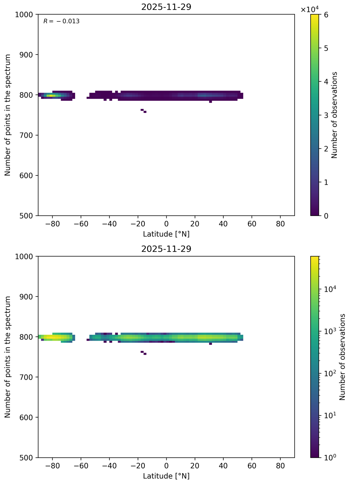
Figure 70: Scatter density plot of “Latitude” against “Number of points in the spectrum” for 2025-11-28 to 2025-11-30.
