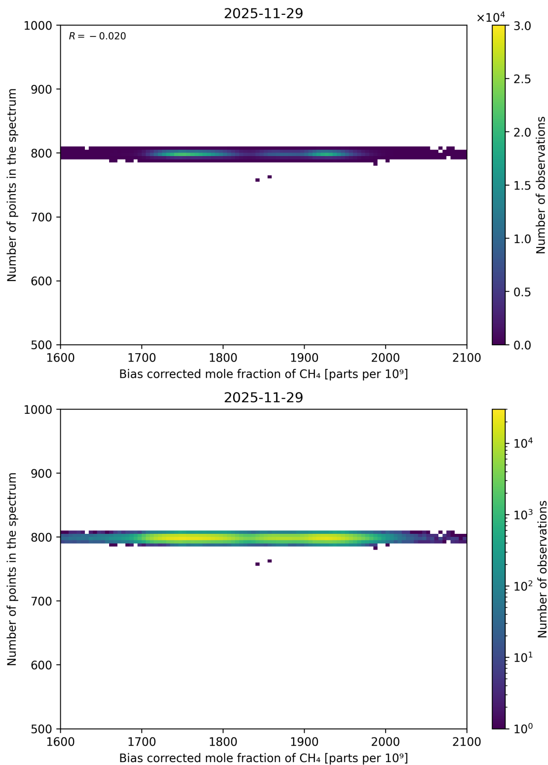
Figure 78: Scatter density plot of “Bias corrected mole fraction of CH 4 ” against “Number of points in the spectrum” for 2025-11-28 to 2025-11-30.
