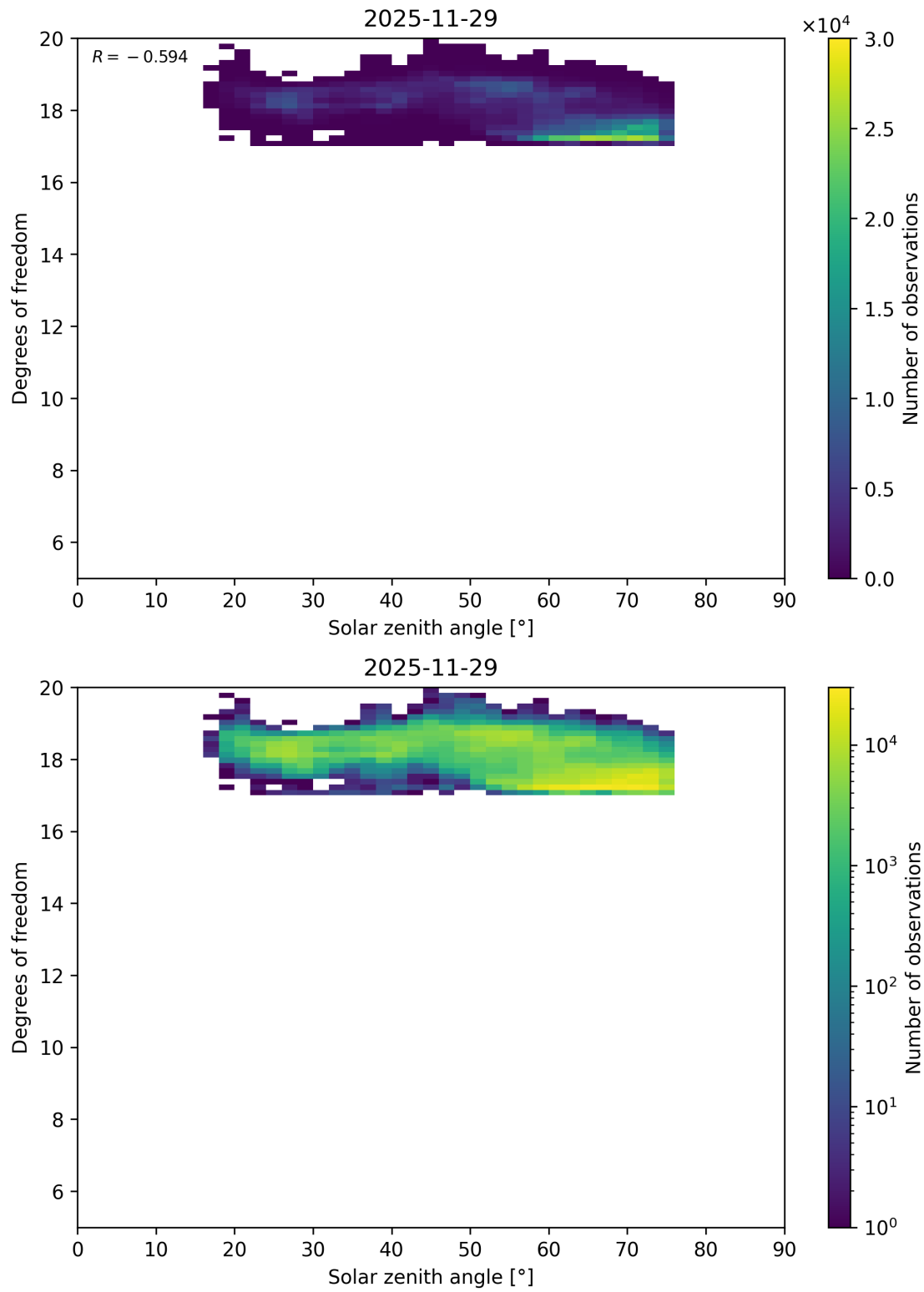
Figure 110: Scatter density plot of “Solar zenith angle” against “Degrees of freedom” for 2025-11-28 to 2025-11-30.
