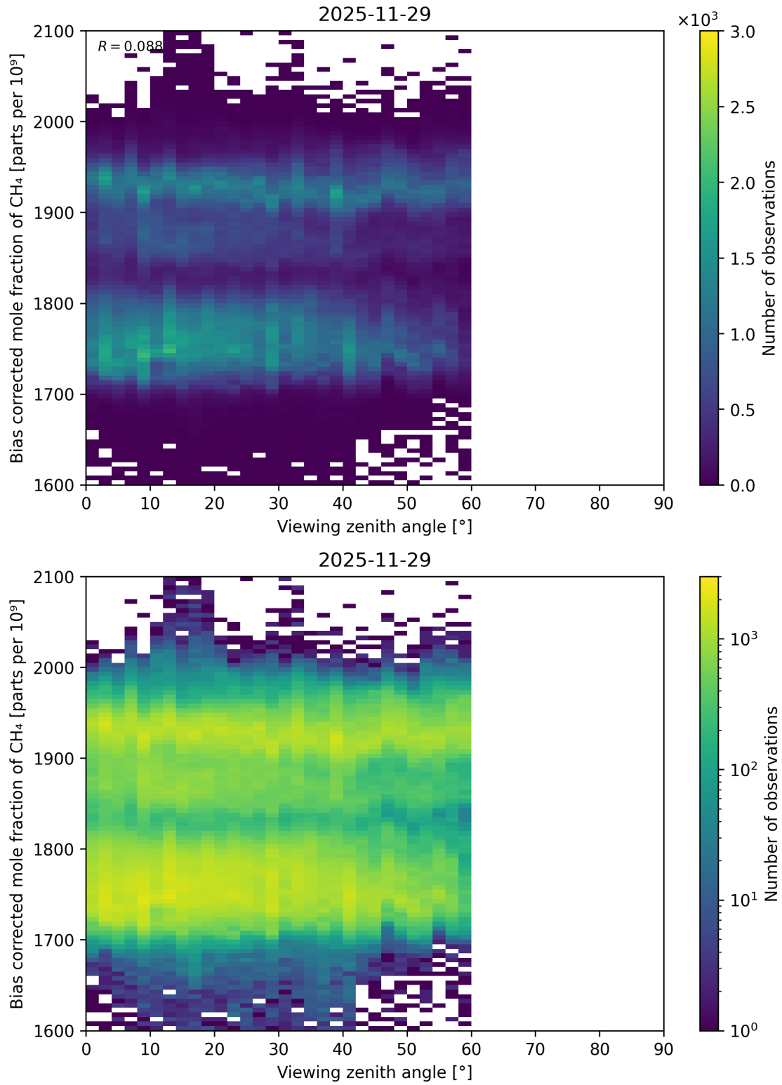
Figure 127: Scatter density plot of “Viewing zenith angle” against “Bias corrected mole fraction of CH 4 ” for 2025-11-28 to 2025-11-30.
