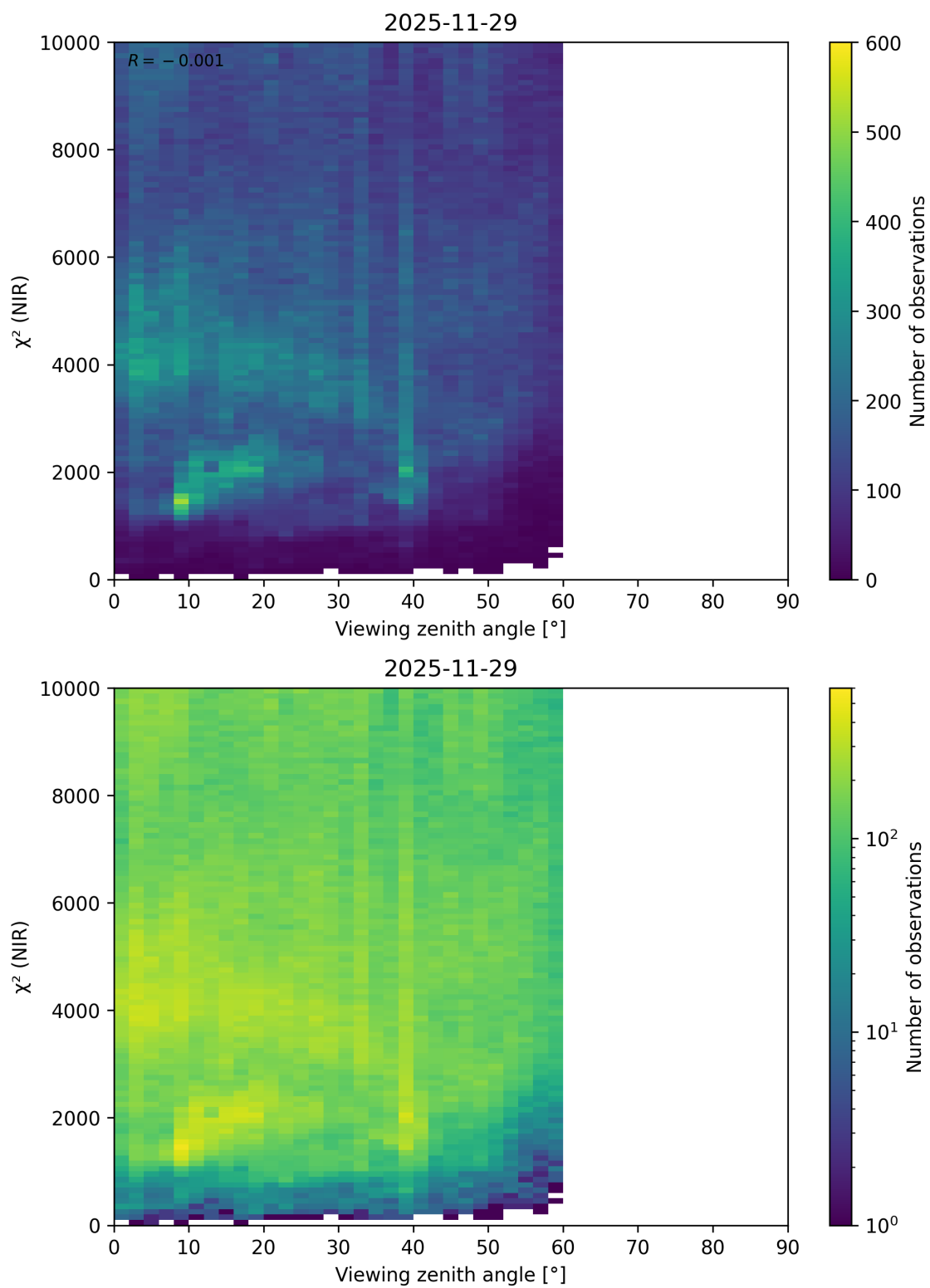
Figure 120: Scatter density plot of “Viewing zenith angle” against “ \chi^2 (NIR)” for 2025-11-28 to 2025-11-30.
