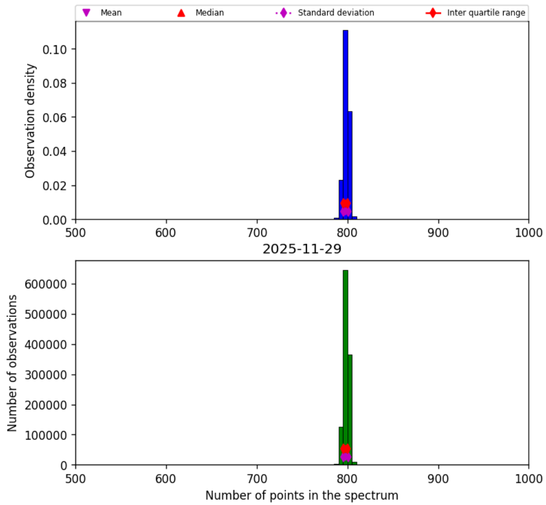
Figure 28: Histogram of “Number of points in the spectrum” for 2025-11-28 to 2025-11-30
