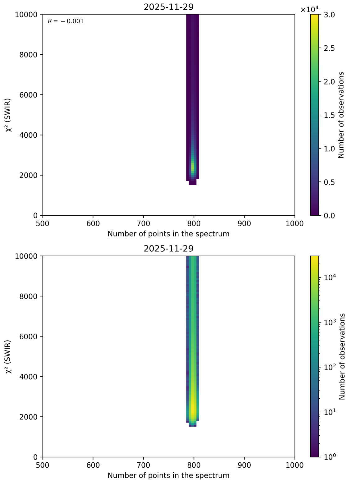
Figure 102: Scatter density plot of “Number of points in the spectrum” against “ \chi^2 (SWIR)” for 2025-11-28 to 2025-11-30.
