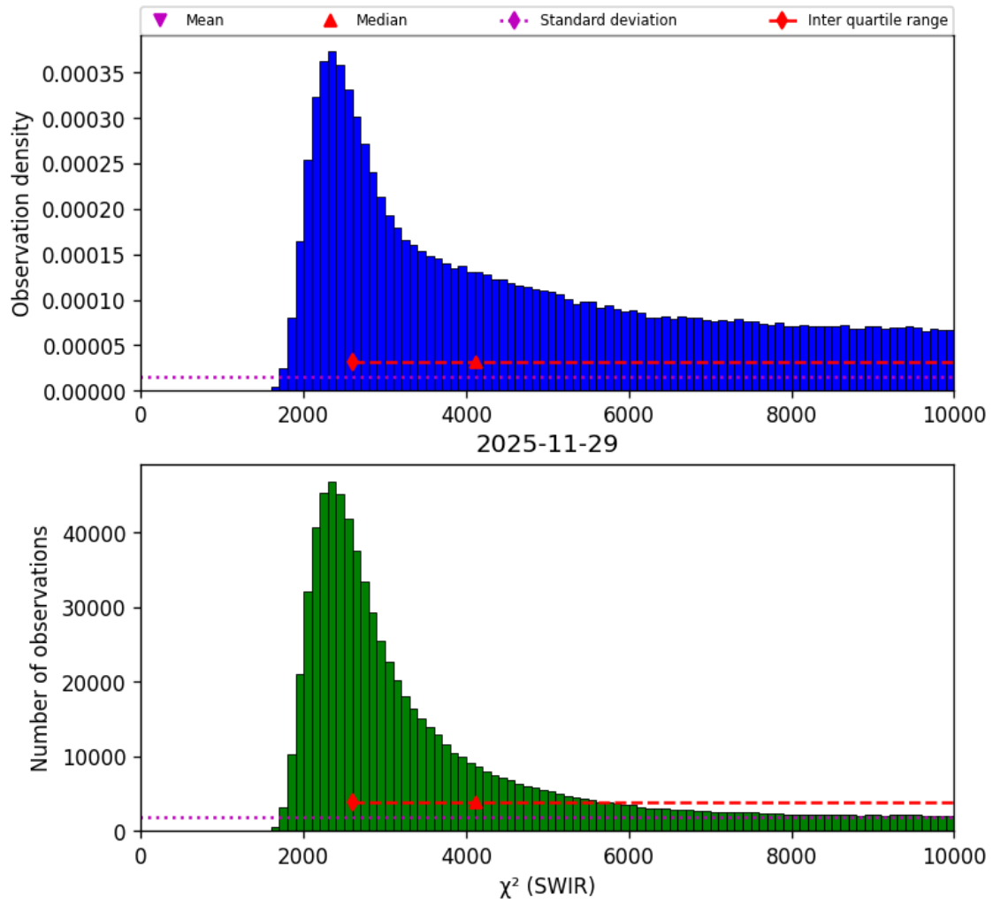
Figure 30: Histogram of " \chi^2 (SWIR)" for 2025-11-28 to 2025-11-30
