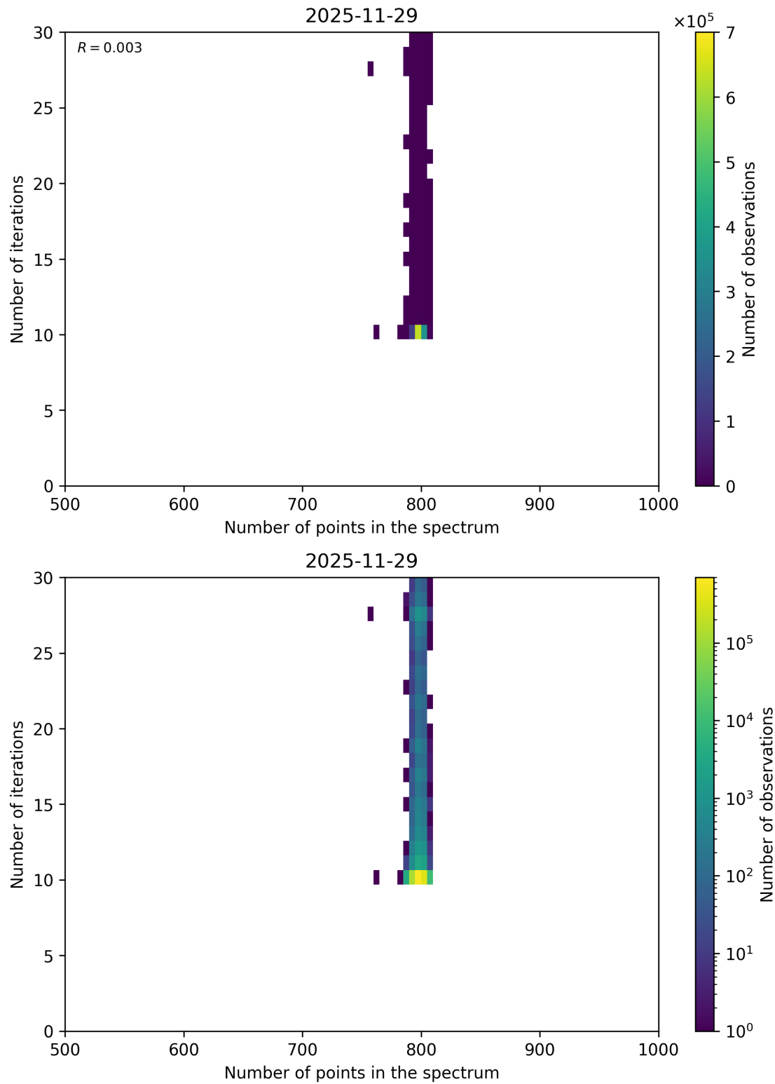
Figure 106: Scatter density plot of “Number of points in the spectrum” against “Number of iterations” for 2025-11-28 to 2025-11-30.
