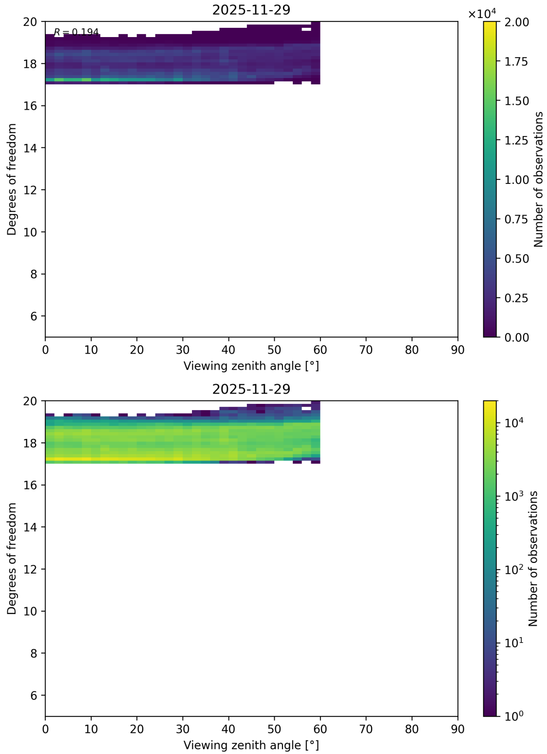
Figure 122: Scatter density plot of “Viewing zenith angle” against “Degrees of freedom” for 2025-11-28 to 2025-11-30.
