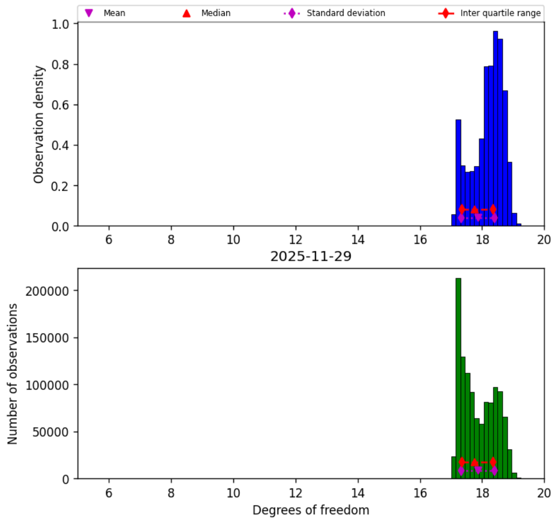
Figure 32: Histogram of “Degrees of freedom” for 2025-11-28 to 2025-11-30
