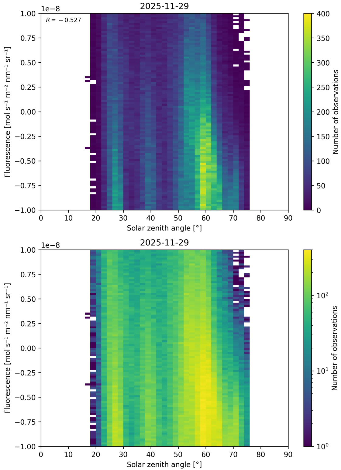
Figure 111: Scatter density plot of “Solar zenith angle” against “Fluorescence” for 2025-11-28 to 2025-11-30.
