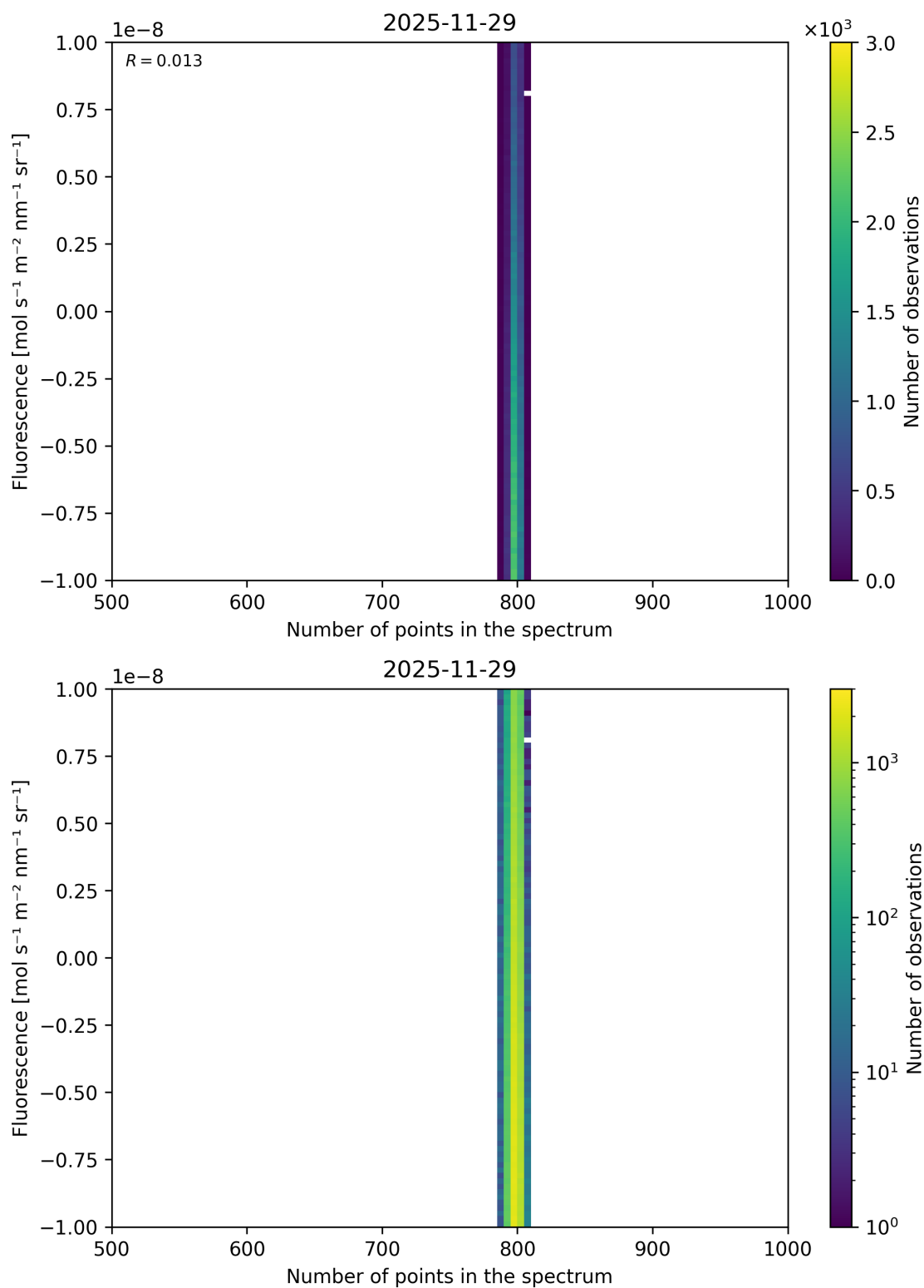
Figure 104: Scatter density plot of “Number of points in the spectrum” against “Fluorescence” for 2025-11-28 to 2025-11-30.
