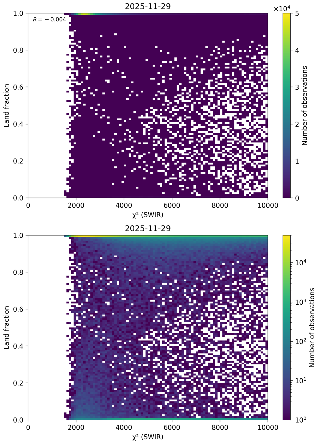
Figure 55: Scatter density plot of “ \chi^2 (SWIR)” against “Land fraction” for 2025-11-28 to 2025-11-30.
