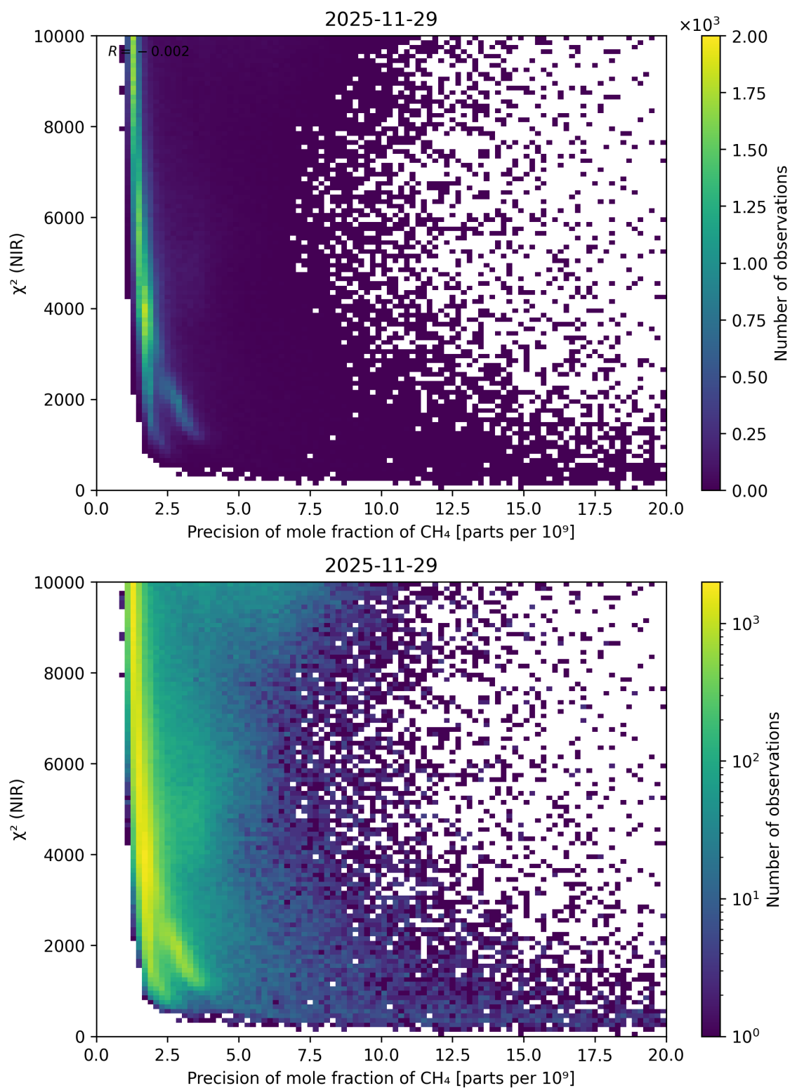
Figure 89: Scatter density plot of “Precision of mole fraction of \text{CH}_4 ” against “ \chi^2 (NIR)” for 2025-11-28 to 2025-11-30.
