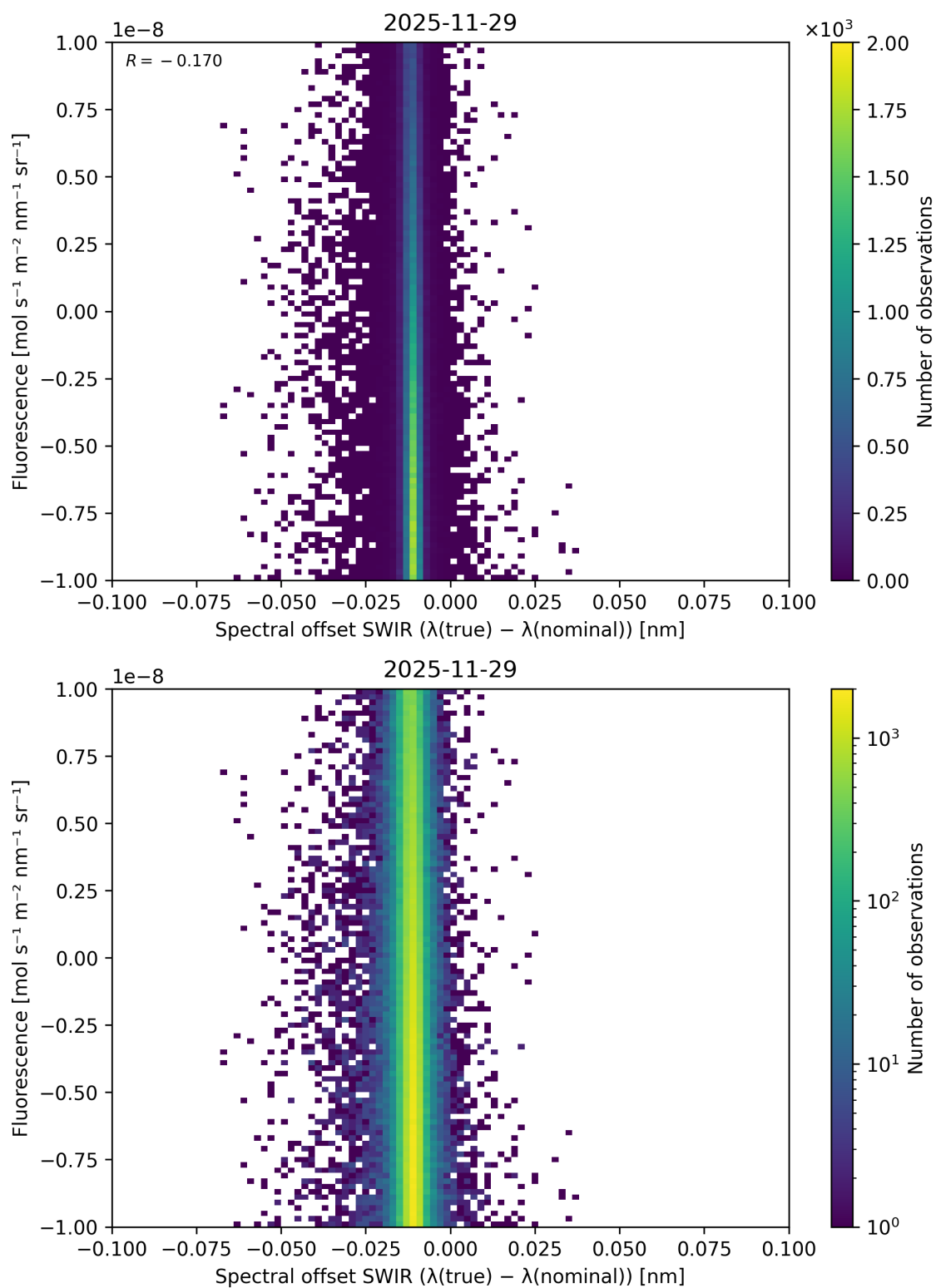
Figure 136: Scatter density plot of “Spectral offset SWIR ( \lambda_{\text{true}} - \lambda_{\text{nominal}} )” against “Fluorescence” for 2025-11-28 to 2025-11-30.
