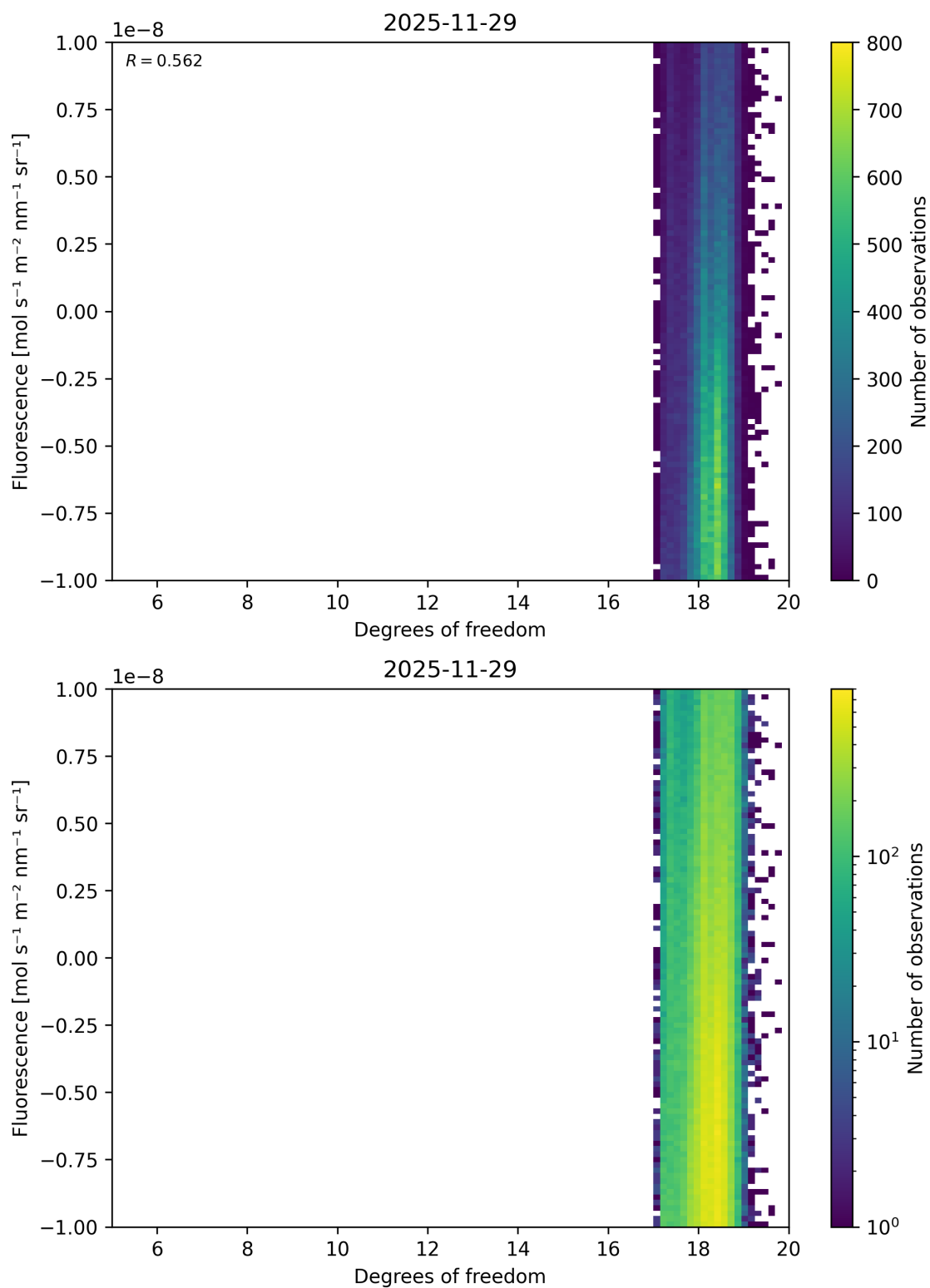
Figure 57: Scatter density plot of “Degrees of freedom” against “Fluorescence” for 2025-11-28 to 2025-11-30.
