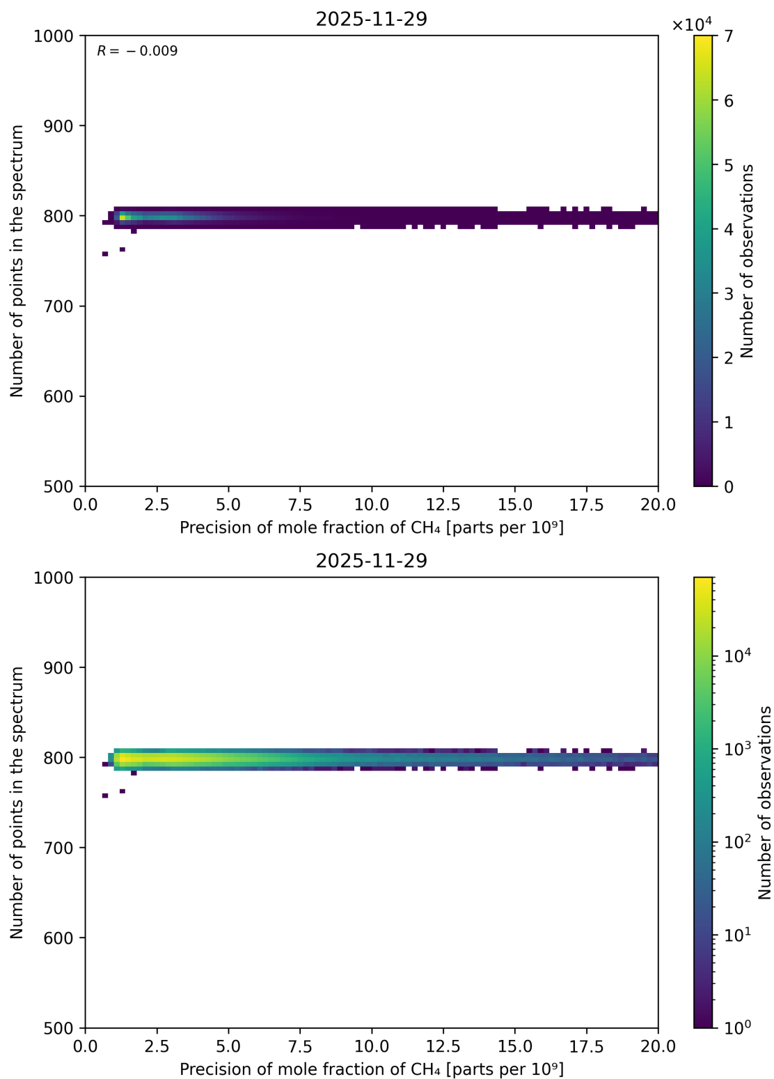
Figure 96: Scatter density plot of “Precision of mole fraction of CH 4 ” against “Number of points in the spectrum” for 2025-11-28 to 2025-11-30.
