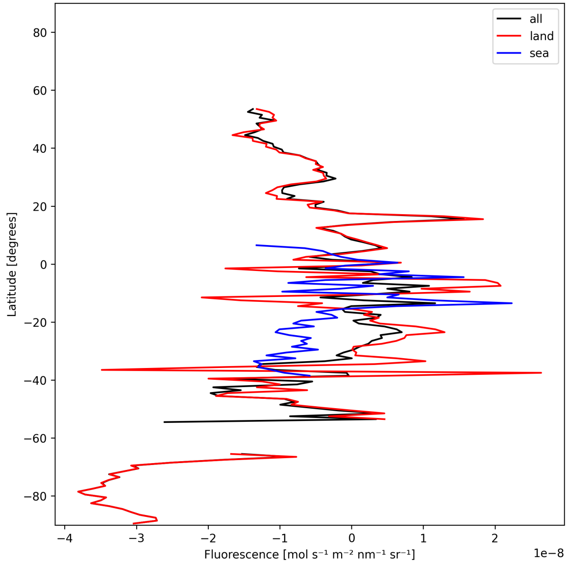
Figure 22: Zonal average of “Fluorescence” for 2025-11-28 to 2025-11-30.
