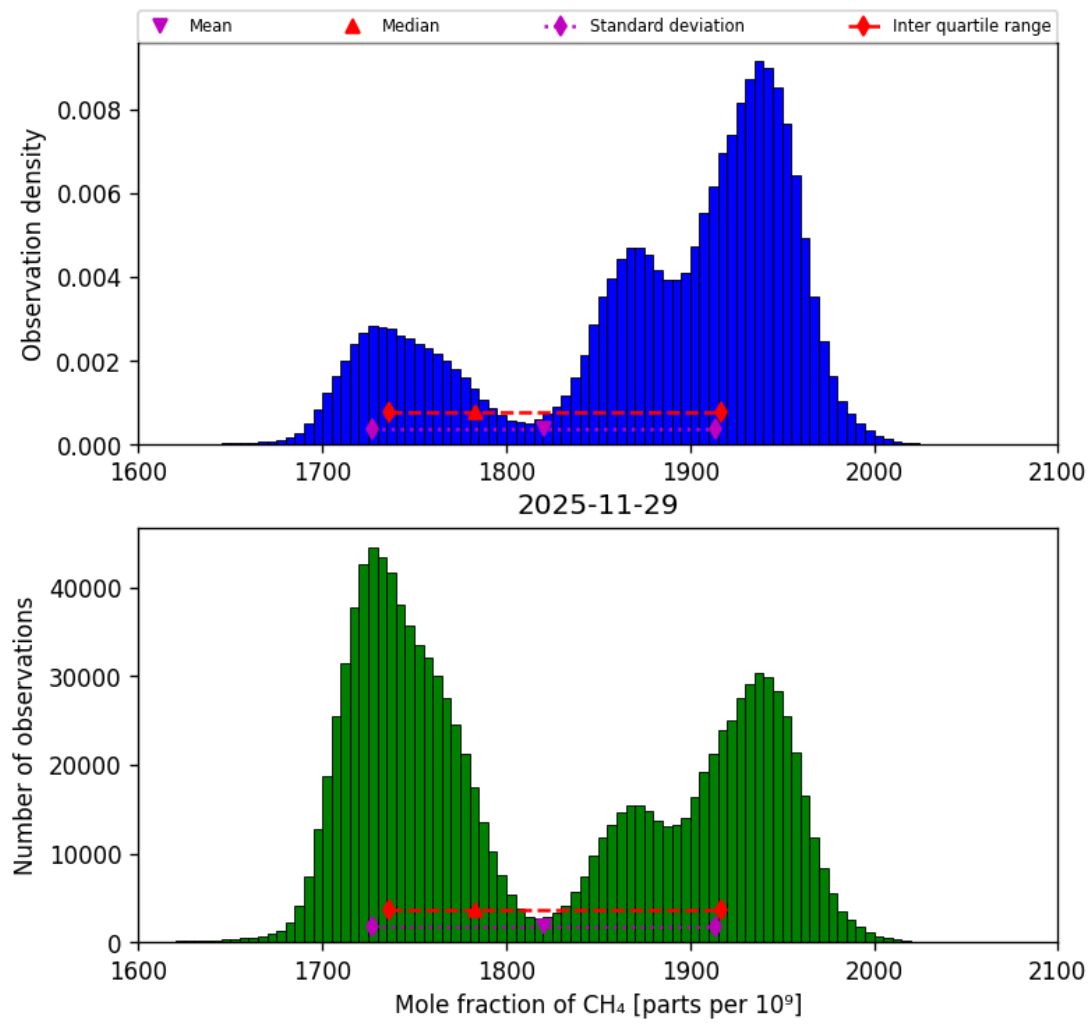
Figure 25: Histogram of “Mole fraction of CH 4 ” for 2025-11-28 to 2025-11-30
