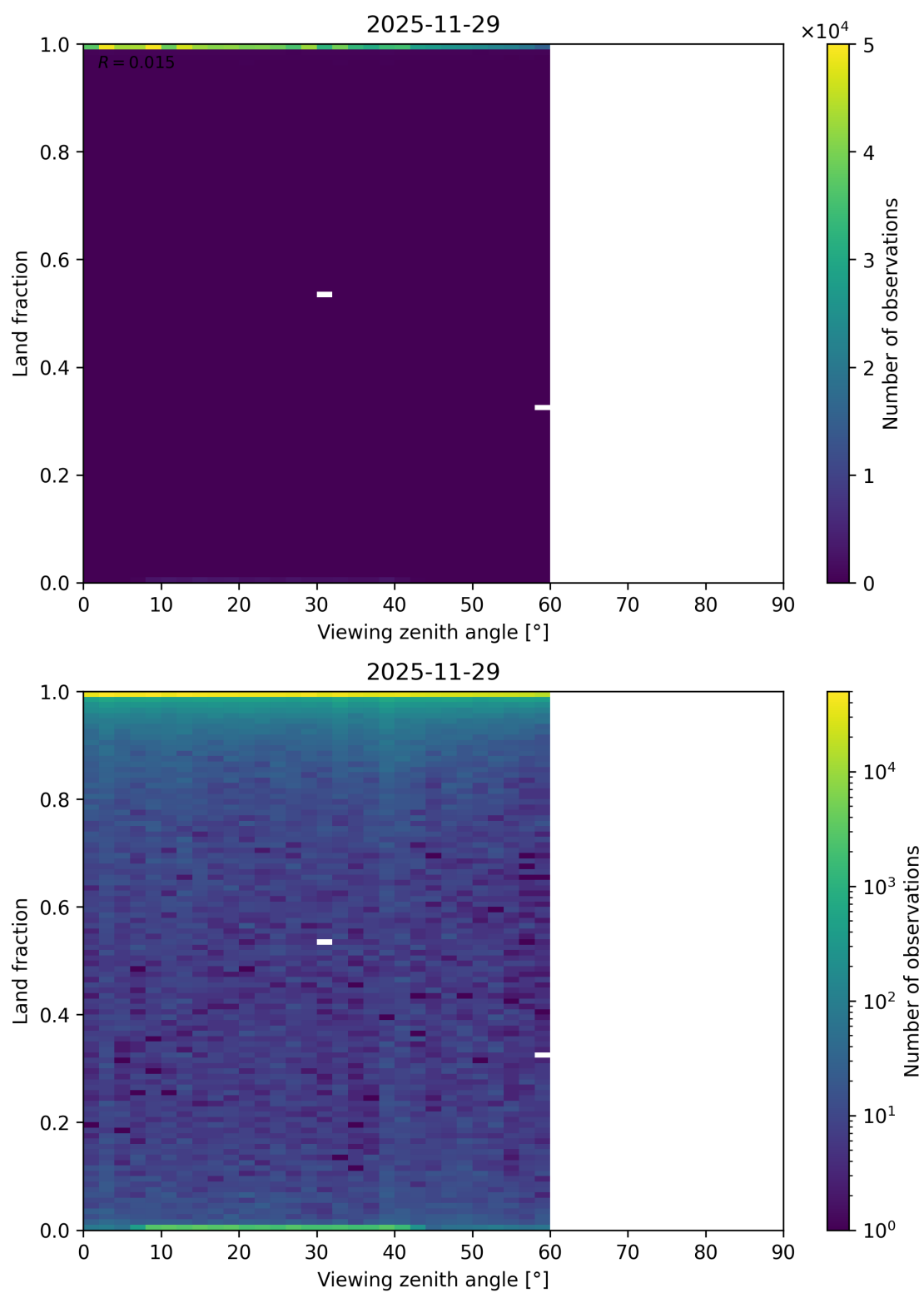
Figure 124: Scatter density plot of “Viewing zenith angle” against “Land fraction” for 2025-11-28 to 2025-11-30.
