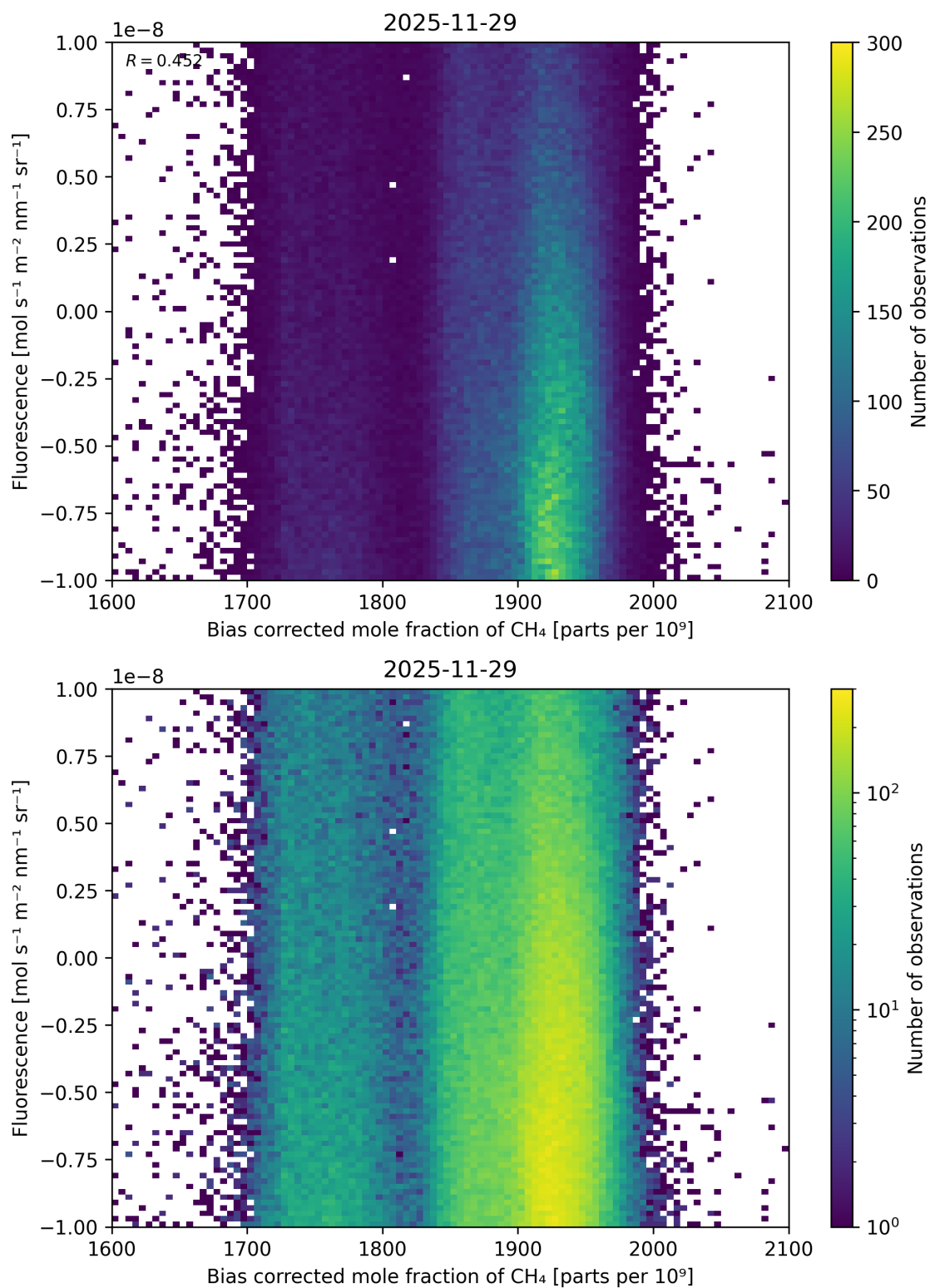
Figure 75: Scatter density plot of “Bias corrected mole fraction of \text{CH}_4 ” against “Fluorescence” for 2025-11-28 to 2025-11-30.
