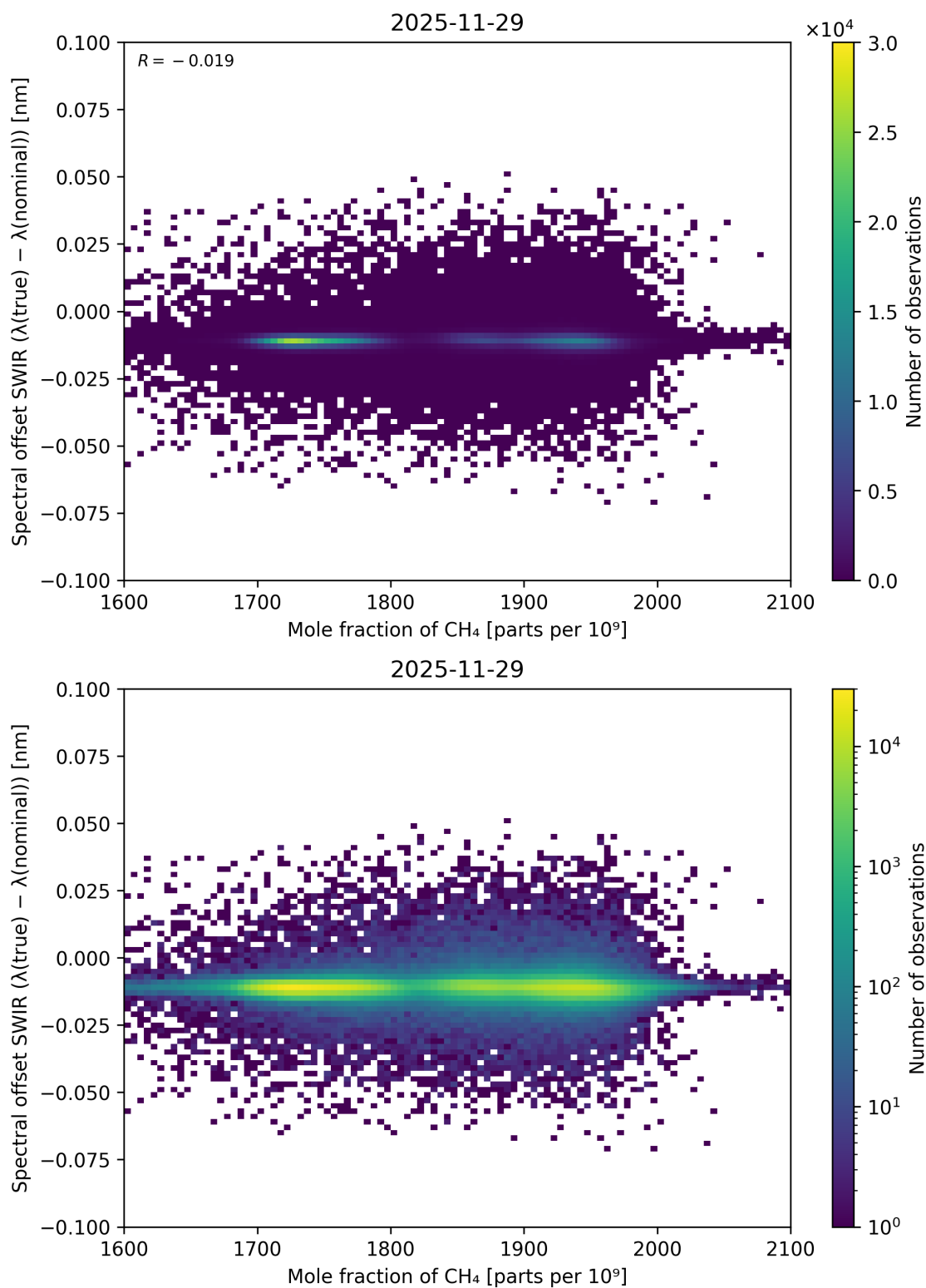
Figure 98: Scatter density plot of “Mole fraction of CH 4 ” against “Spectral offset SWIR ( \lambda_{\text{true}} - \lambda_{\text{nominal}} )” for 2025-11-28 to 2025-11-30.
