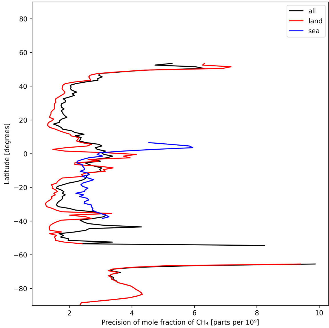
Figure 14: Zonal average of “Precision of mole fraction of CH 4 ” for 2025-11-28 to 2025-11-30.
