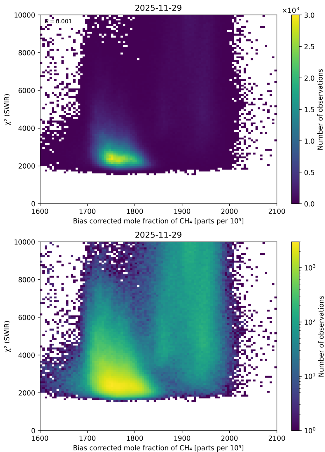
Figure 73: Scatter density plot of “Bias corrected mole fraction of \text{CH}_4 ” against “ \chi^2 (SWIR)” for 2025-11-28 to 2025-11-30.
