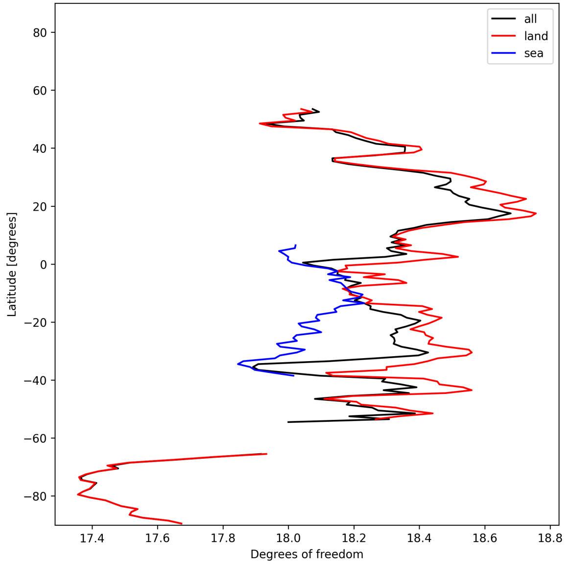
Figure 20: Zonal average of “Degrees of freedom” for 2025-11-28 to 2025-11-30.
