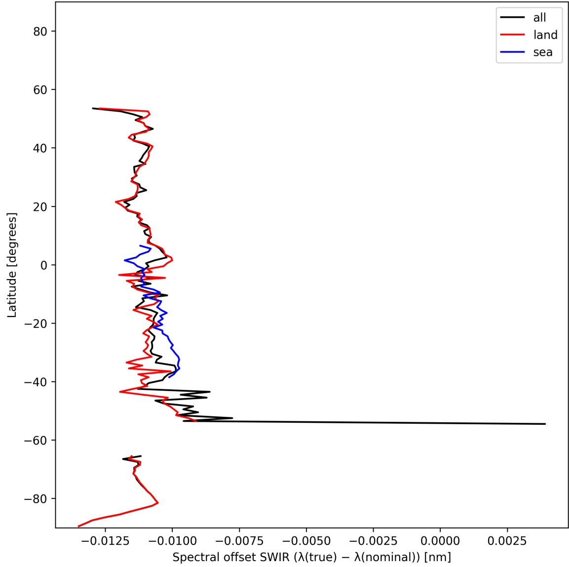
Figure 17: Zonal average of “Spectral offset SWIR ( \lambda_{\text{true}} - \lambda_{\text{nominal}} )” for 2025-11-28 to 2025-11-30.
