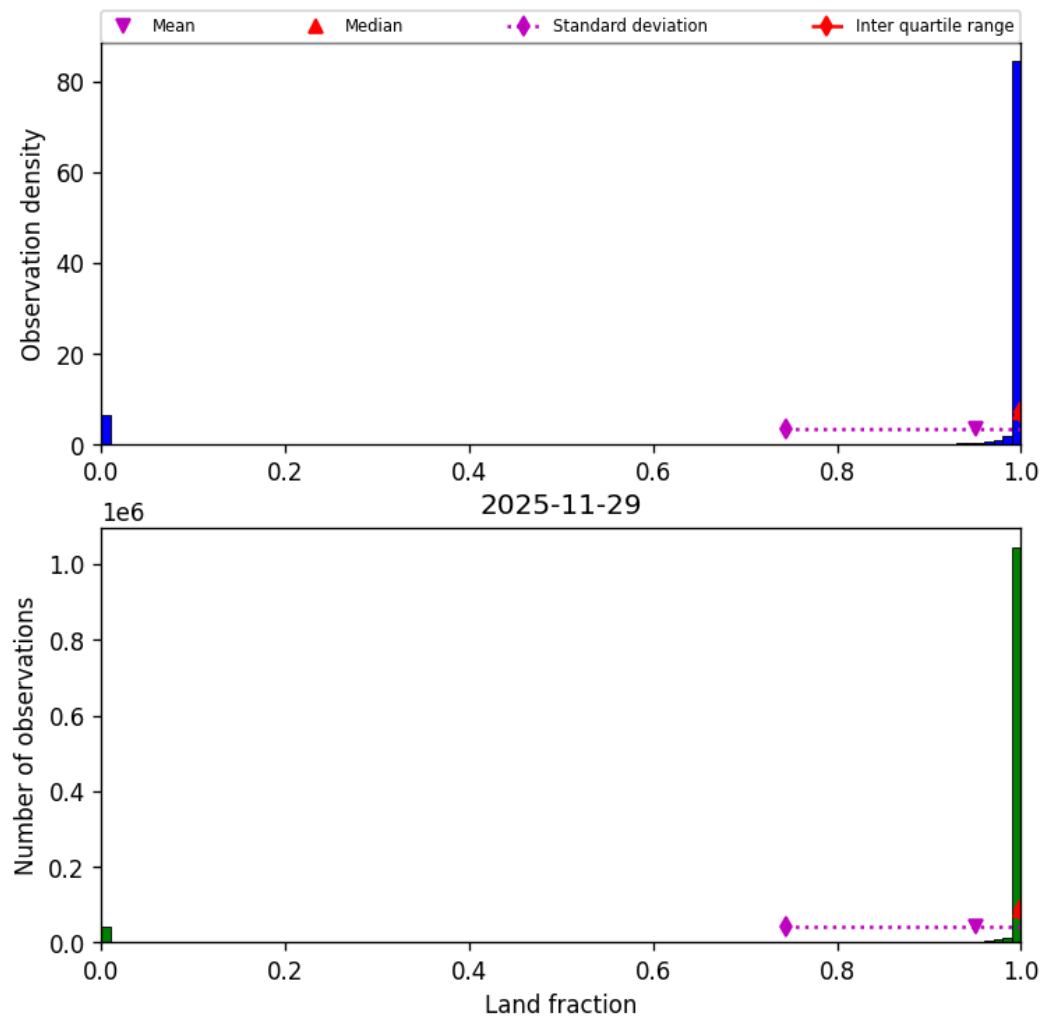
Figure 35: Histogram of “Land fraction” for 2025-11-28 to 2025-11-30
