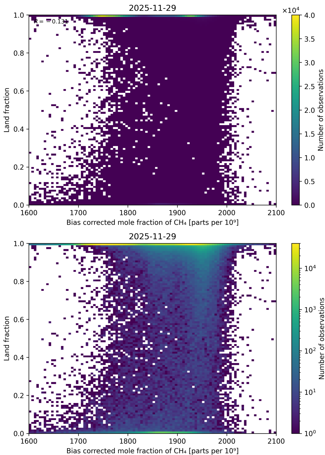
Figure 76: Scatter density plot of “Bias corrected mole fraction of CH 4 ” against “Land fraction” for 2025-11-28 to 2025-11-30.
