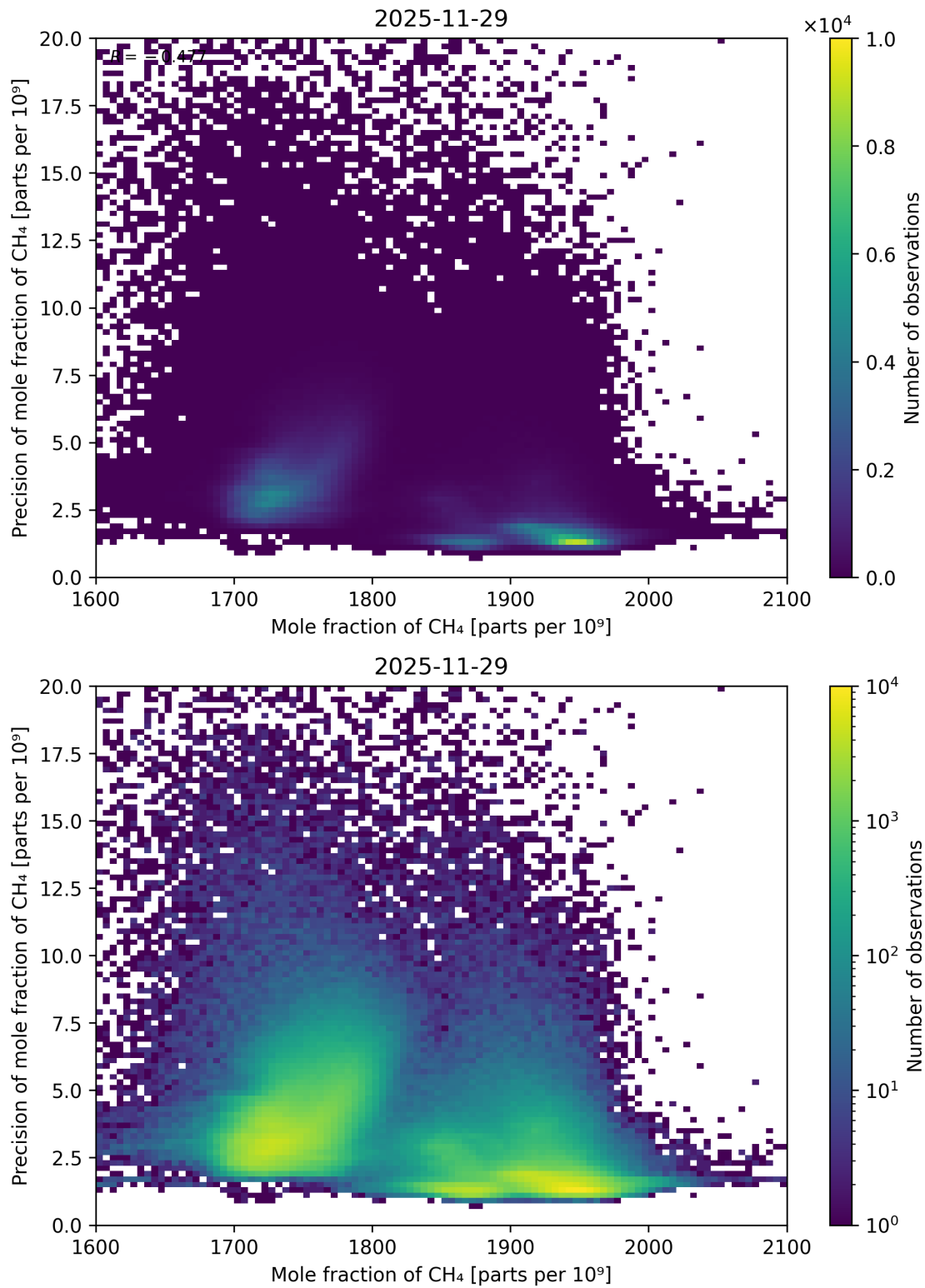
Figure 86: Scatter density plot of “Mole fraction of CH 4 ” against “Precision of mole fraction of CH 4 ” for 2025-11-28 to 2025-11-30.
