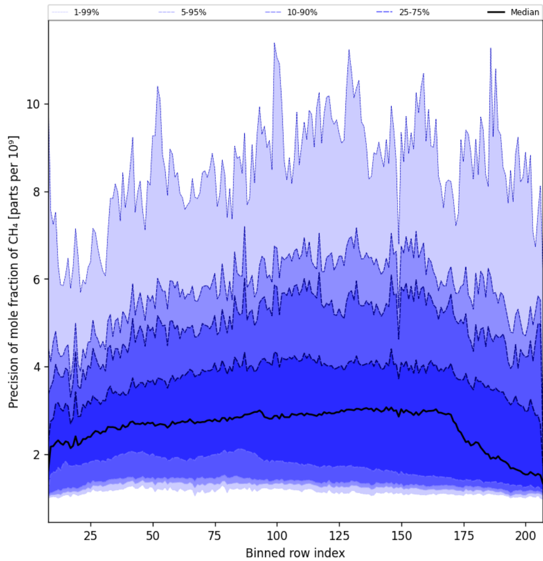
Figure 38: Along track statistics of “Precision of mole fraction of CH 4 ” for 2025-11-28 to 2025-11-30
