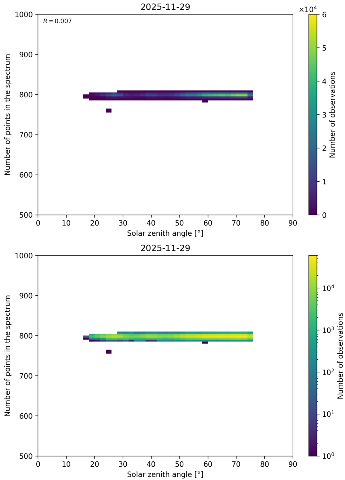
Figure 118: Scatter density plot of “Solar zenith angle” against “Number of points in the spectrum” for 2025-11-28 to 2025-11-30.
