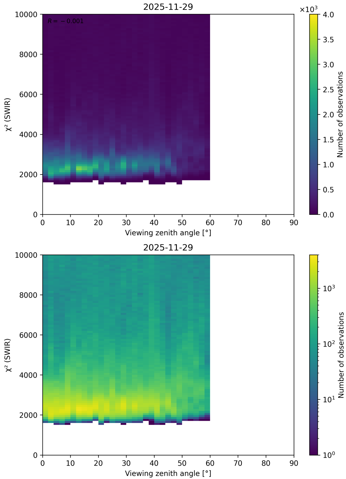
Figure 121: Scatter density plot of “Viewing zenith angle” against “ \chi^2 (SWIR)” for 2025-11-28 to 2025-11-30.
