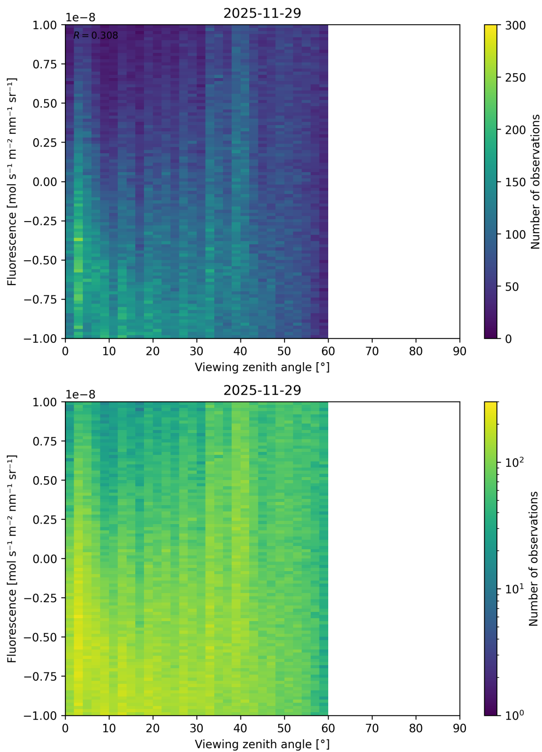
Figure 123: Scatter density plot of “Viewing zenith angle” against “Fluorescence” for 2025-11-28 to 2025-11-30.
