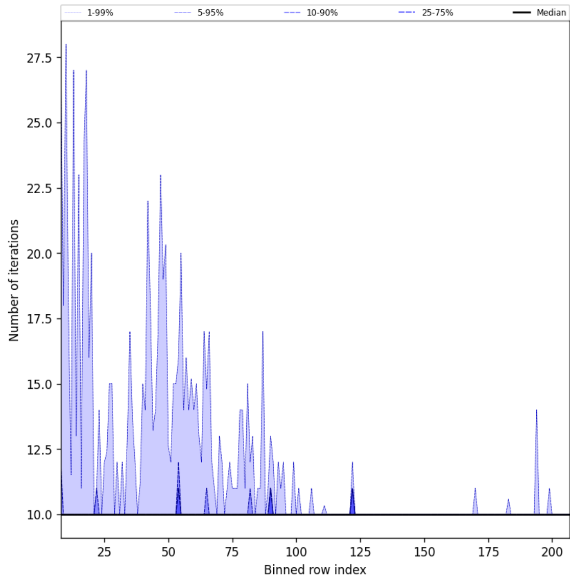
Figure 45: Along track statistics of “Number of iterations” for 2025-11-28 to 2025-11-30
