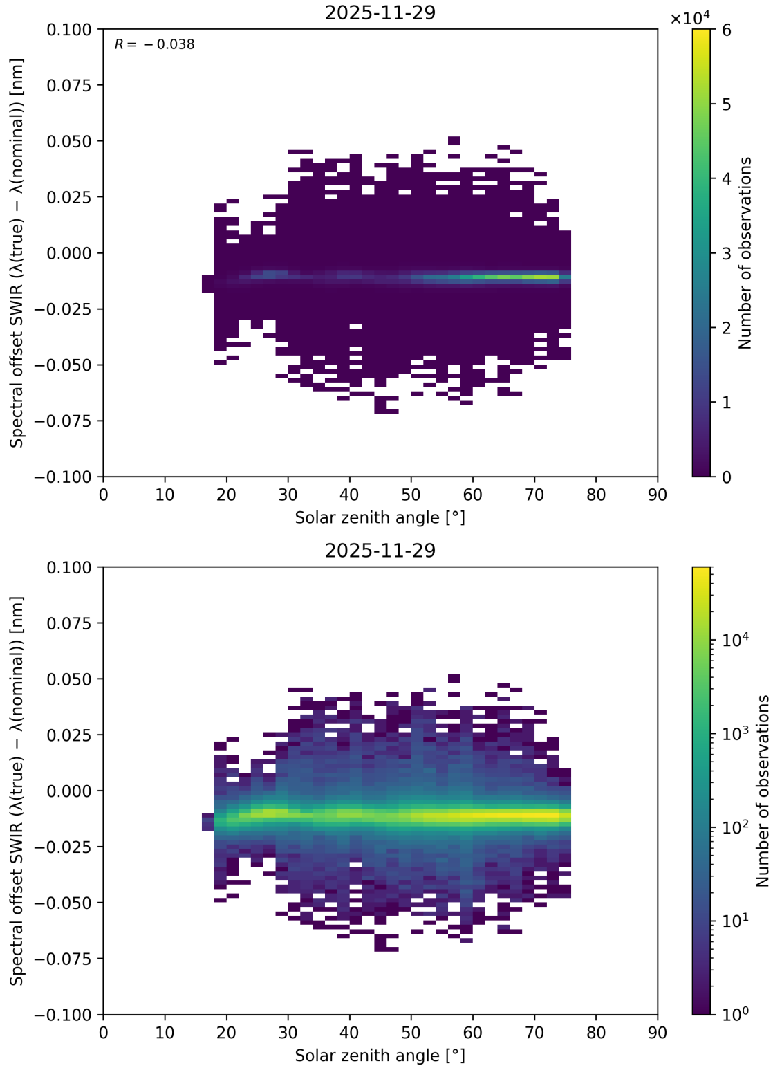
Figure 119: Scatter density plot of “Solar zenith angle” against “Spectral offset SWIR ( \lambda_{\text{true}} - \lambda_{\text{nominal}} )” for 2025-11-28 to 2025-11-30.
