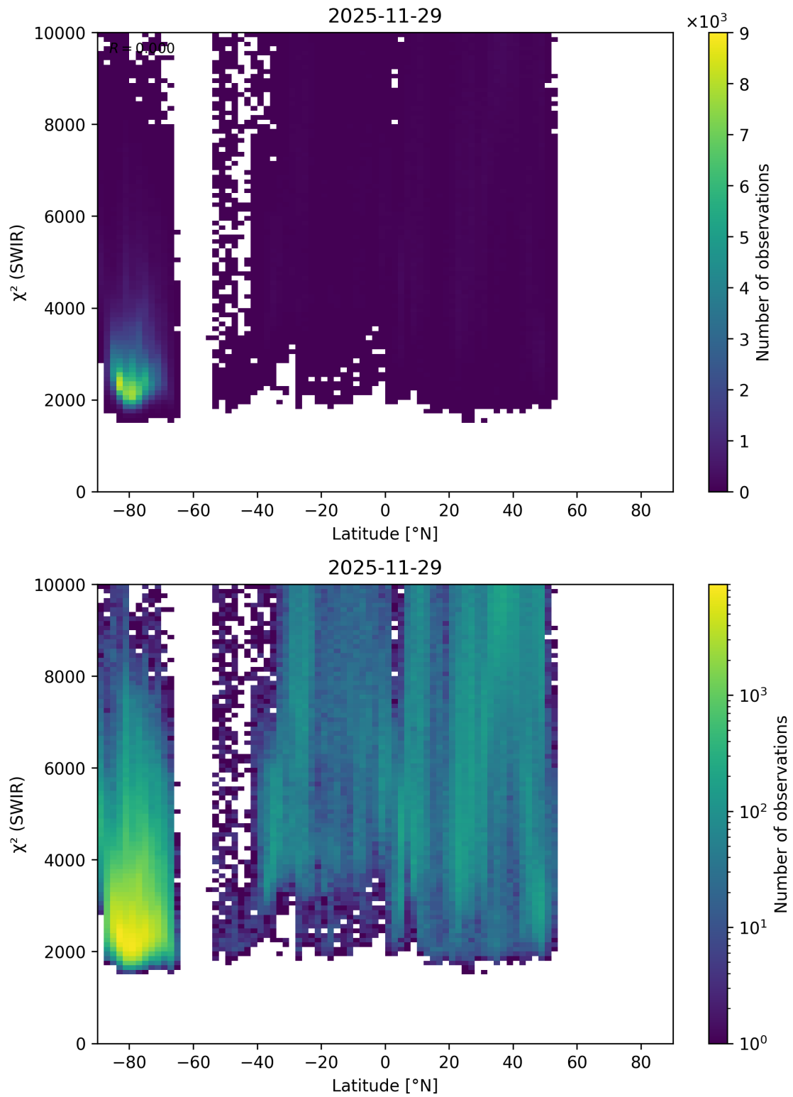
Figure 62: Scatter density plot of “Latitude” against “ \chi^2 (SWIR)” for 2025-11-28 to 2025-11-30.
