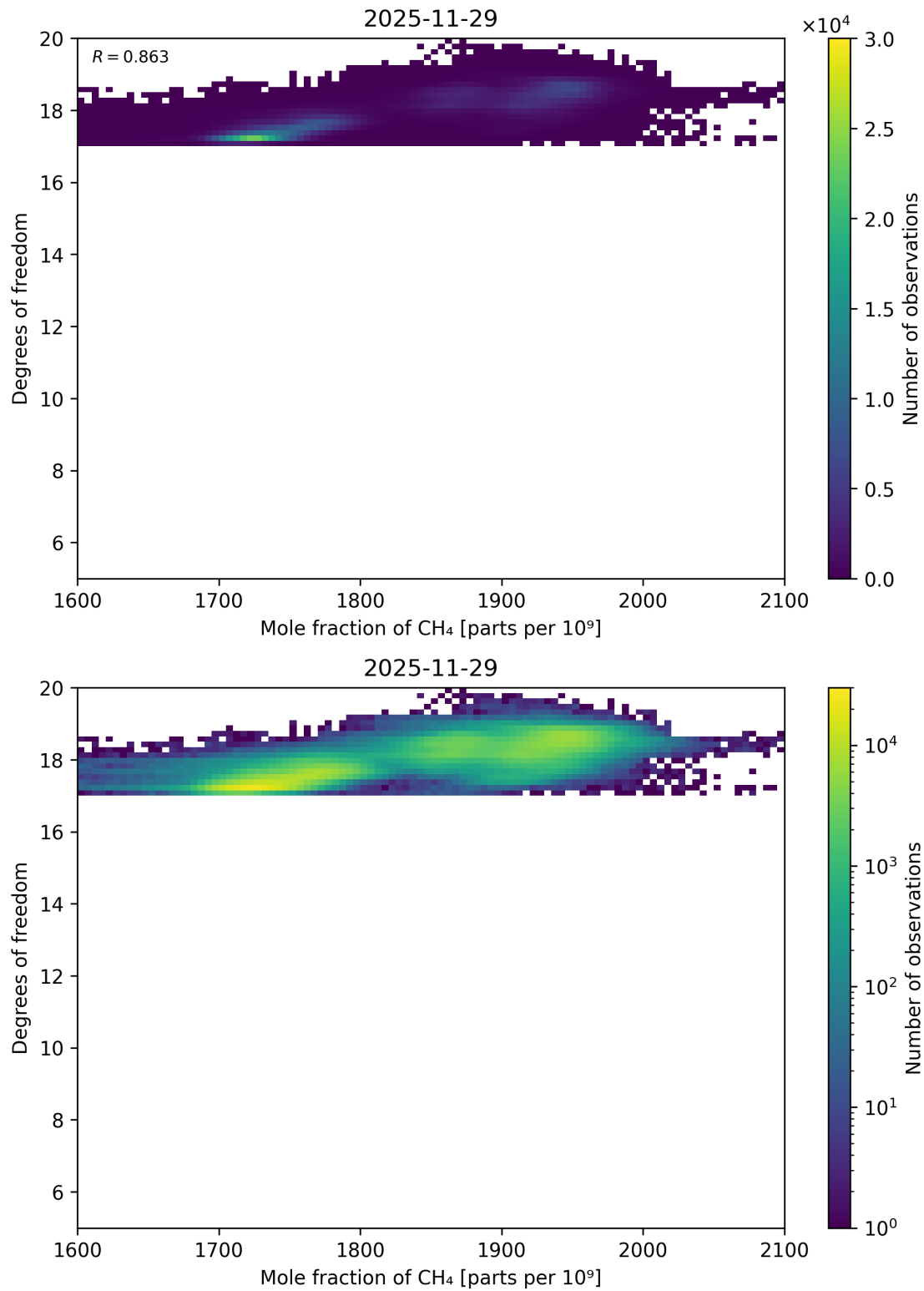
Figure 82: Scatter density plot of “Mole fraction of CH 4 ” against “Degrees of freedom” for 2025-11-28 to 2025-11-30.
