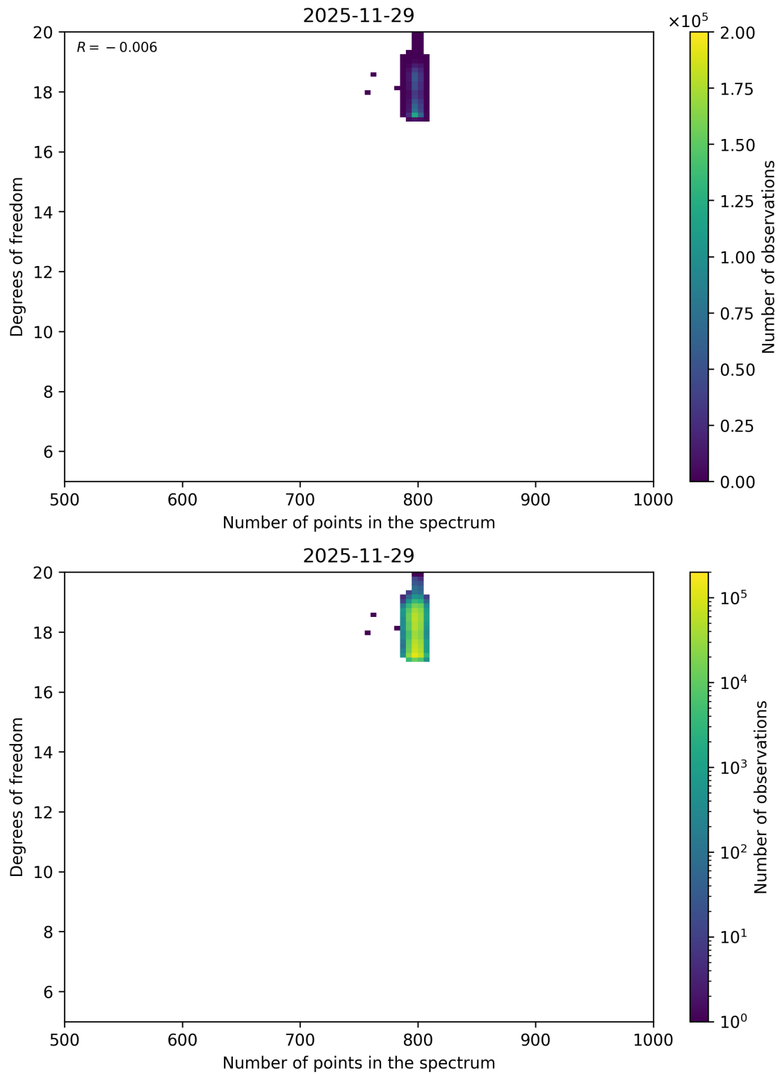
Figure 103: Scatter density plot of “Number of points in the spectrum” against “Degrees of freedom” for 2025-11-28 to 2025-11-30.
