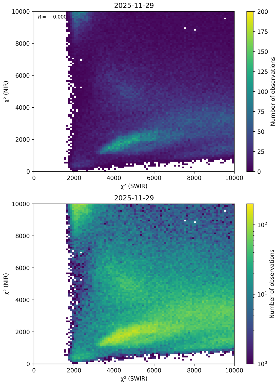
Figure 52: Scatter density plot of “ \chi^2 (SWIR)” against “ \chi^2 (NIR)” for 2025-11-28 to 2025-11-30.
