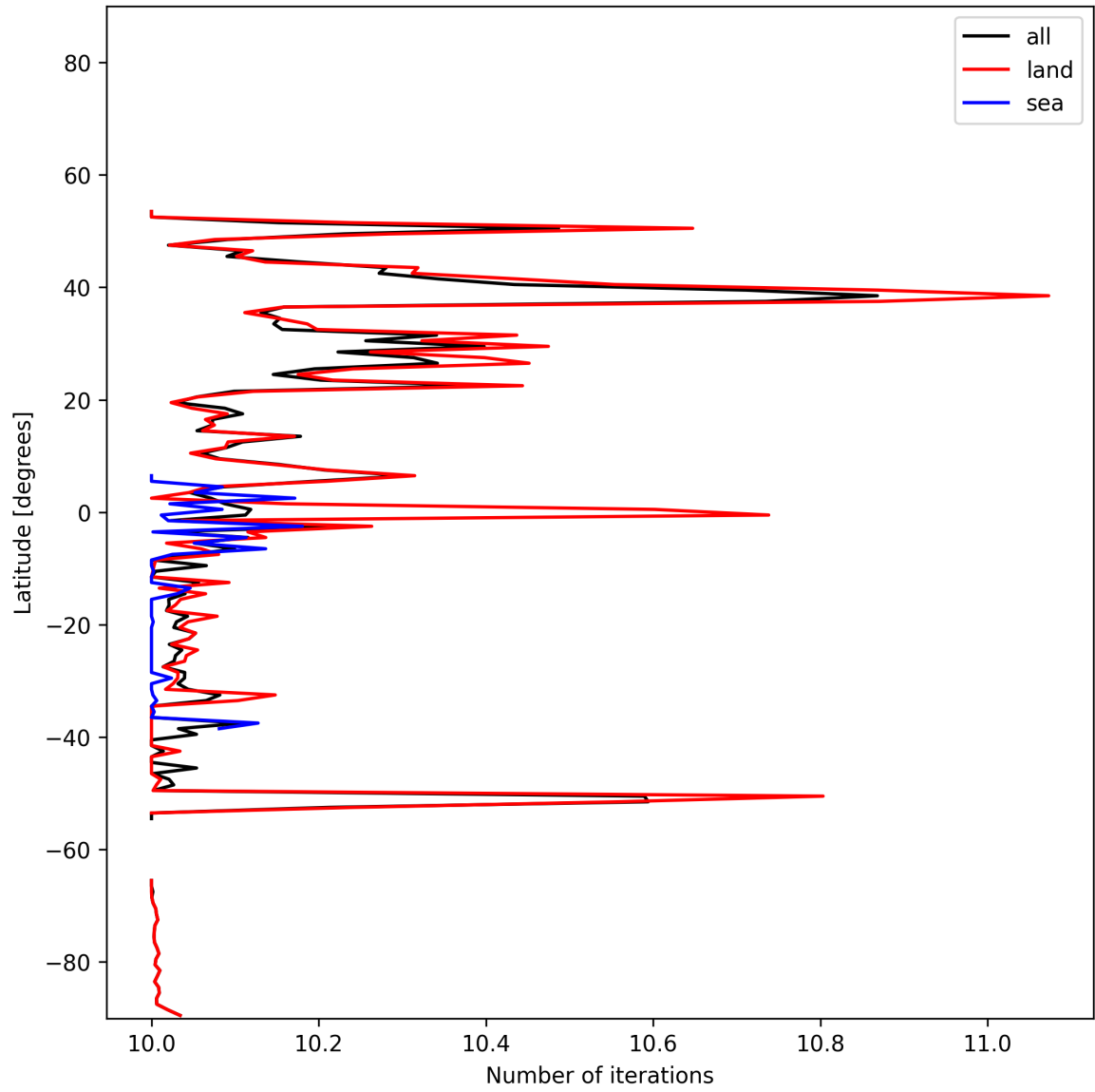
Figure 21: Zonal average of “Number of iterations” for 2025-11-28 to 2025-11-30.
