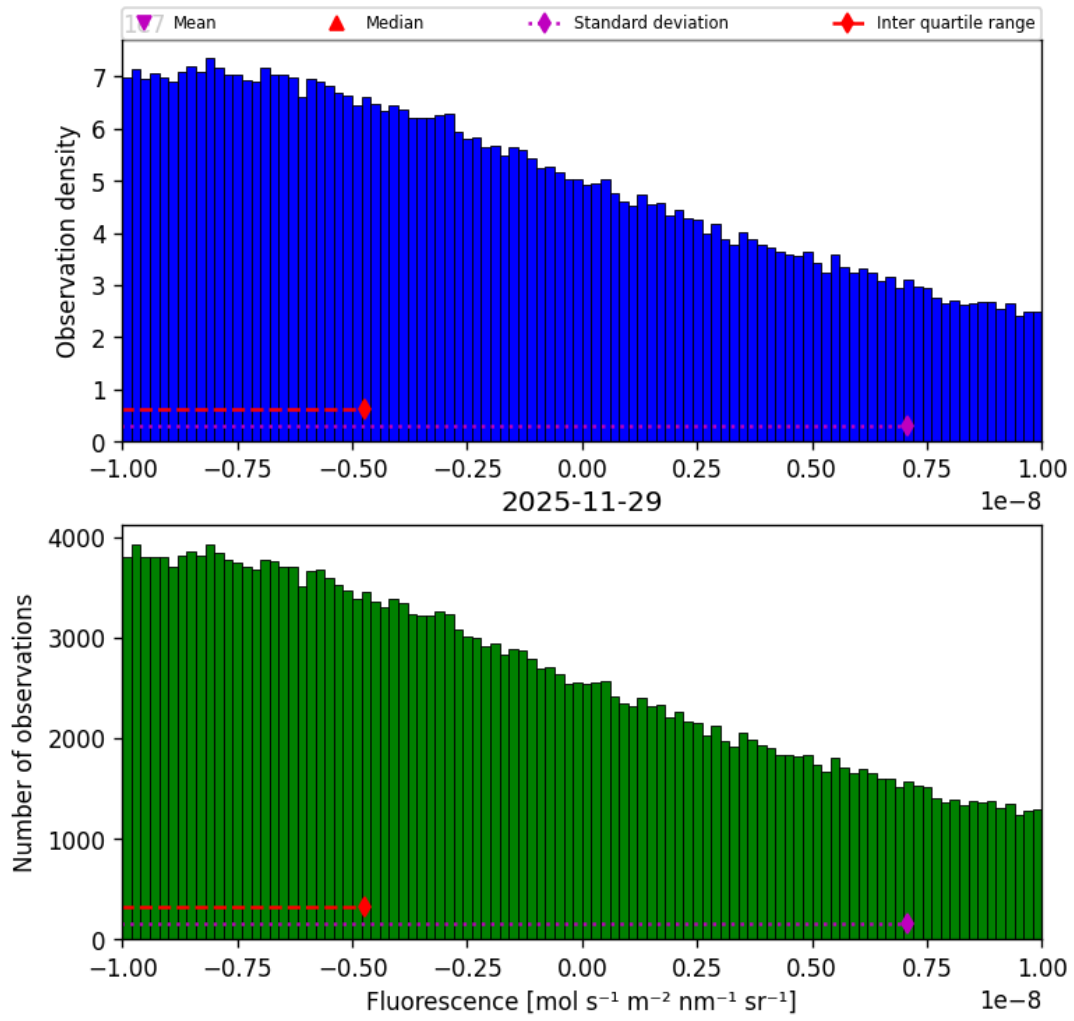
Figure 34: Histogram of “Fluorescence” for 2025-11-28 to 2025-11-30
