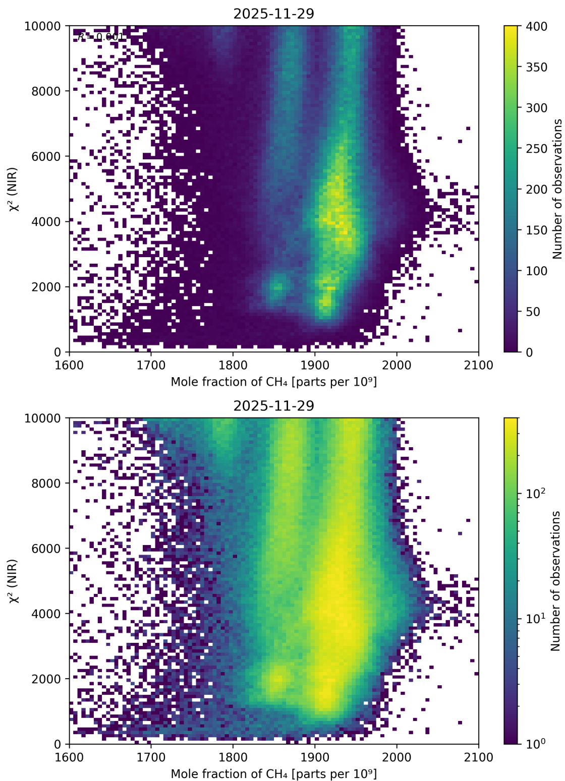
Figure 80: Scatter density plot of “Mole fraction of \text{CH}_4 ” against “ \chi^2 (NIR)” for 2025-11-28 to 2025-11-30.
