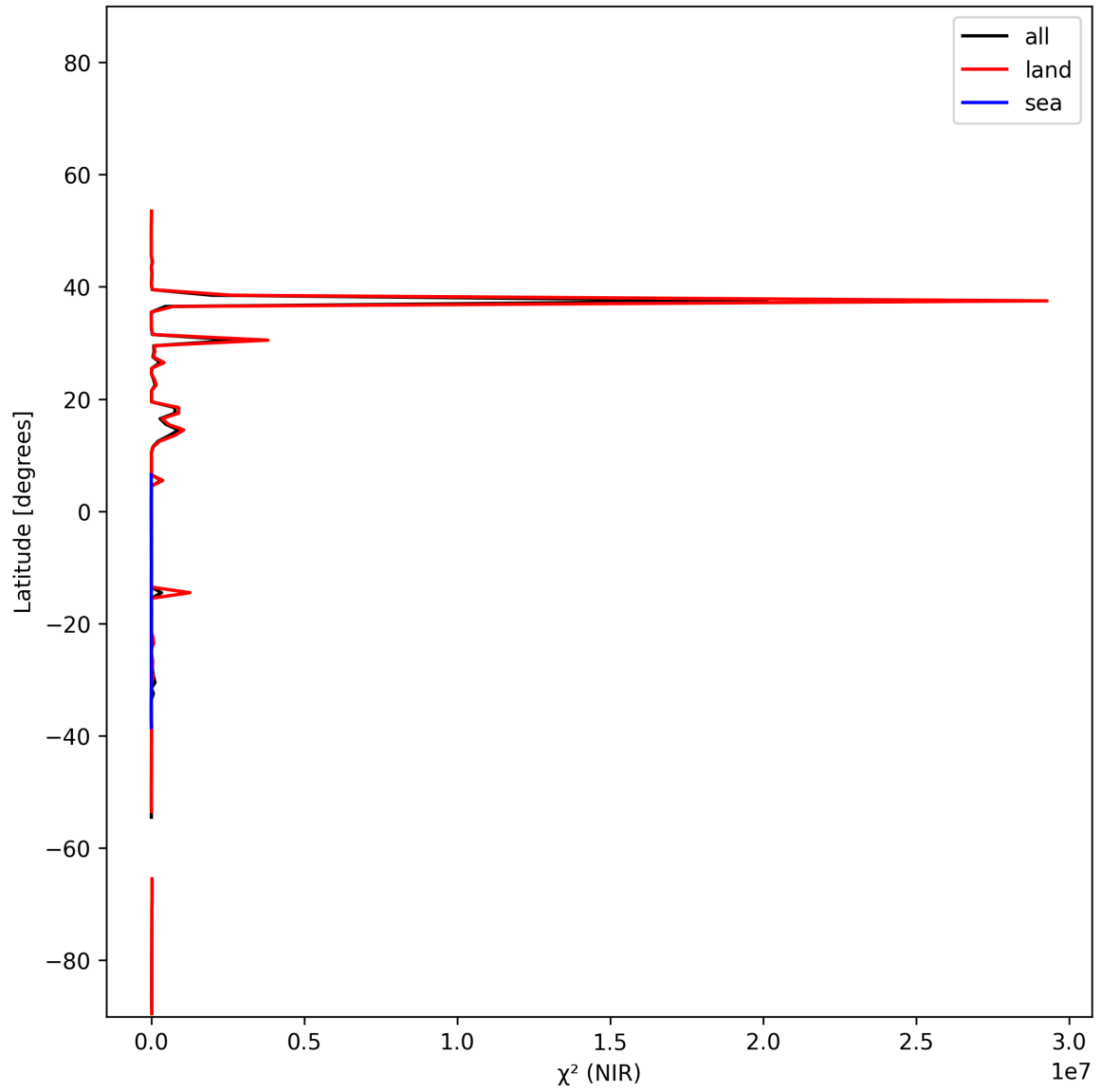
Figure 19: Zonal average of “ \chi^2 (NIR)” for 2025-11-28 to 2025-11-30.
