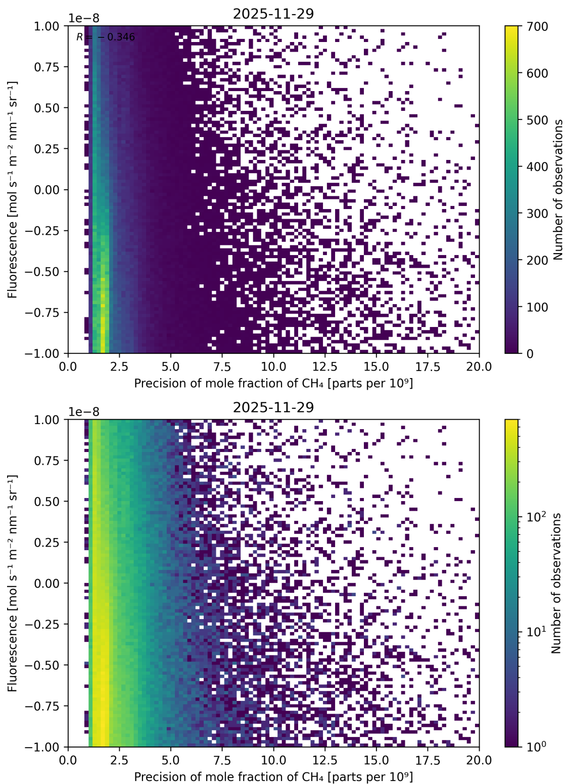
Figure 92: Scatter density plot of “Precision of mole fraction of CH 4 ” against “Fluorescence” for 2025-11-28 to 2025-11-30.
