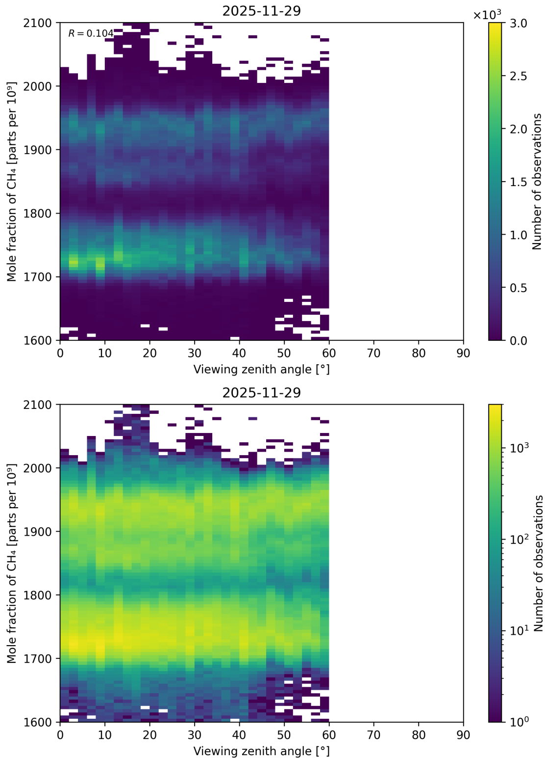
Figure 126: Scatter density plot of “Viewing zenith angle” against “Mole fraction of CH 4 ” for 2025-11-28 to 2025-11-30.
