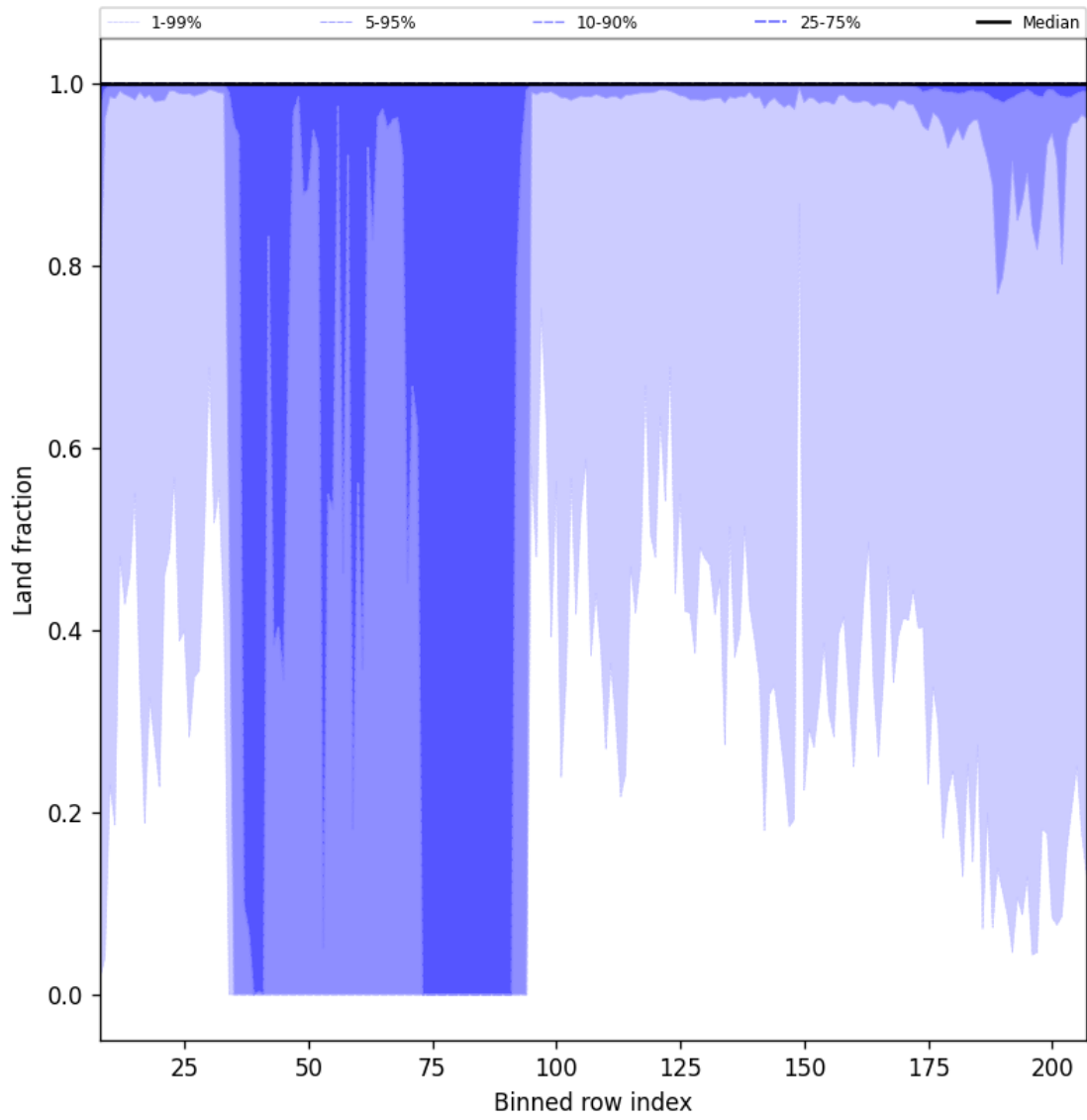
Figure 47: Along track statistics of "Land fraction" for 2025-11-28 to 2025-11-30
