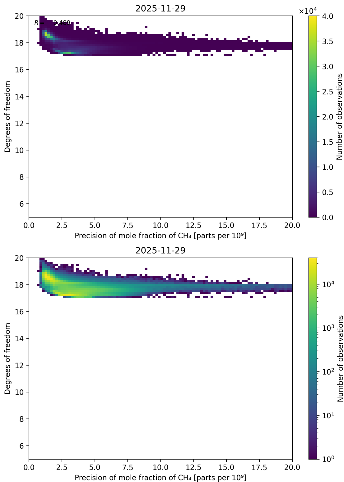
Figure 91: Scatter density plot of “Precision of mole fraction of CH 4 ” against “Degrees of freedom” for 2025-11-28 to 2025-11-30.
