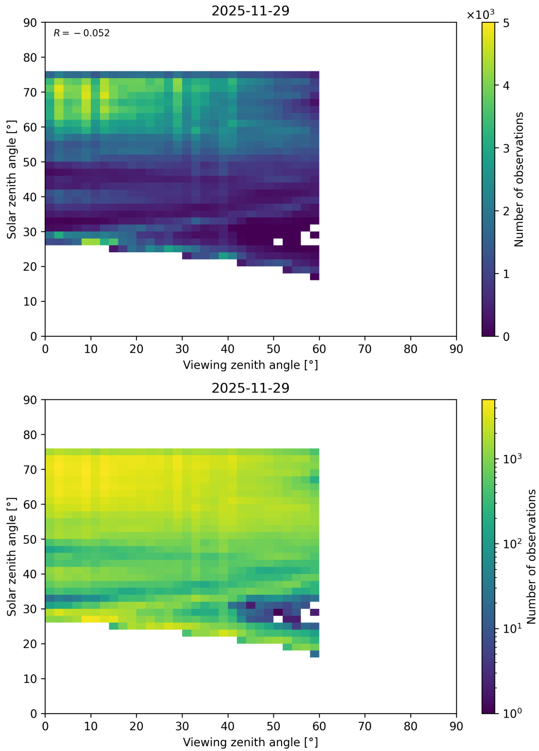
Figure 131: Scatter density plot of “Viewing zenith angle” against “Solar zenith angle” for 2025-11-28 to 2025-11-30.
