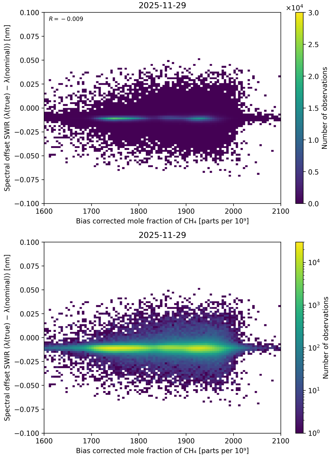
Figure 79: Scatter density plot of “Bias corrected mole fraction of \text{CH}_4 ” against “Spectral offset SWIR ( \lambda_{\text{true}} - \lambda_{\text{nominal}} )” for 2025-11-28 to 2025-11-30.
