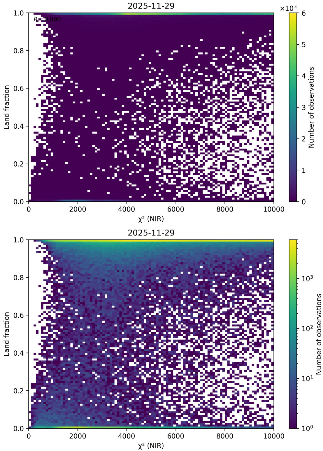
Figure 50: Scatter density plot of “ \chi^2 (NIR)” against “Land fraction” for 2025-11-28 to 2025-11-30.
