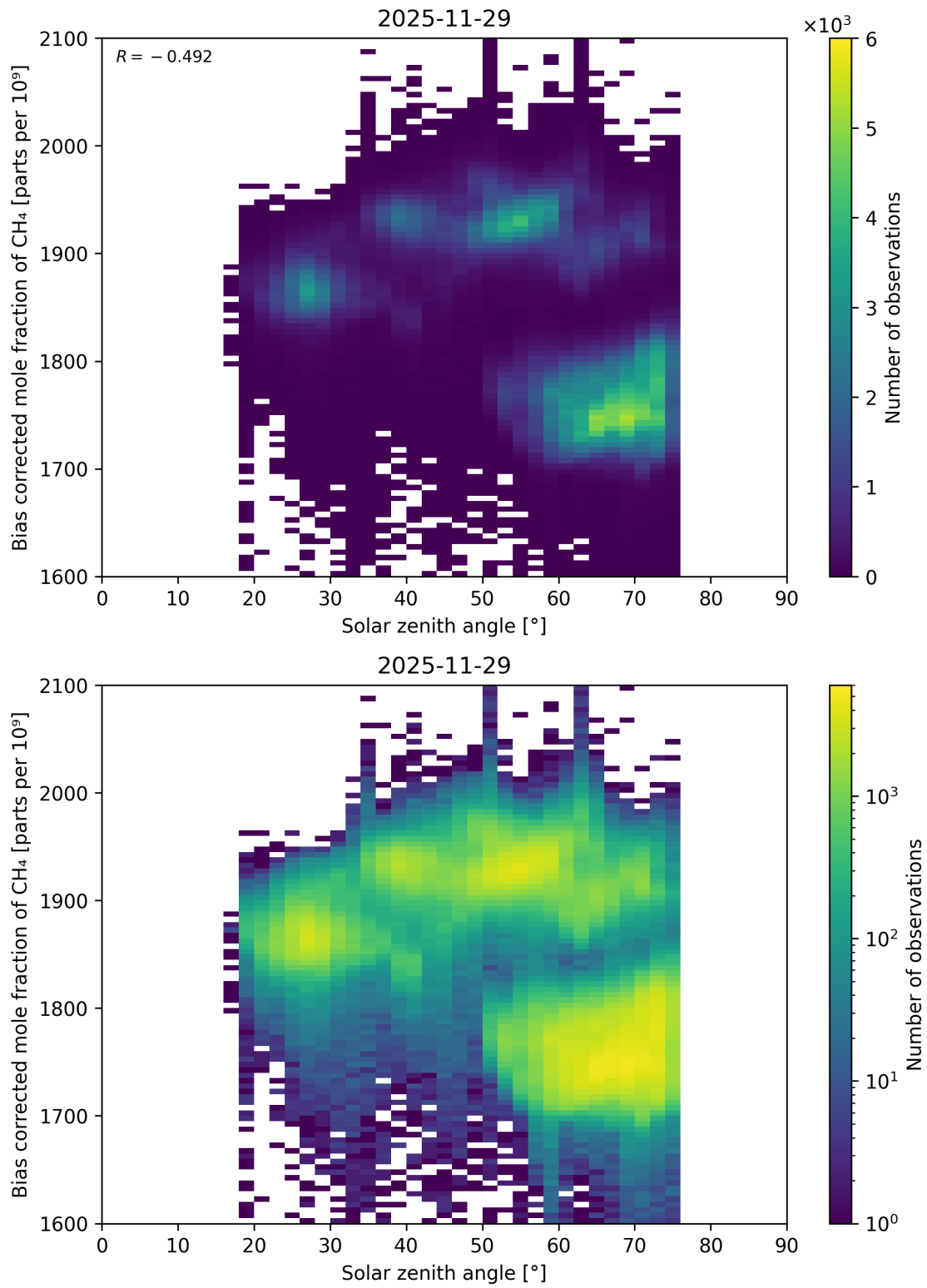
Figure 115: Scatter density plot of “Solar zenith angle” against “Bias corrected mole fraction of CH 4 ” for 2025-11-28 to 2025-11-30.
