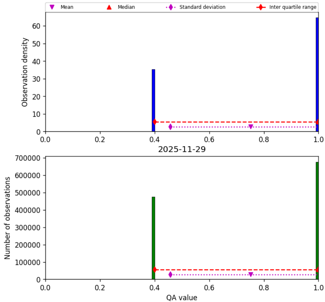
Figure 24: Histogram of “QA value” for 2025-11-28 to 2025-11-30
