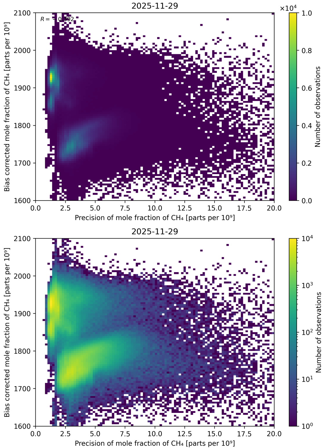
Figure 94: Scatter density plot of “Precision of mole fraction of CH 4 ” against “Bias corrected mole fraction of CH 4 ” for 2025-11-28 to 2025-11-30.
