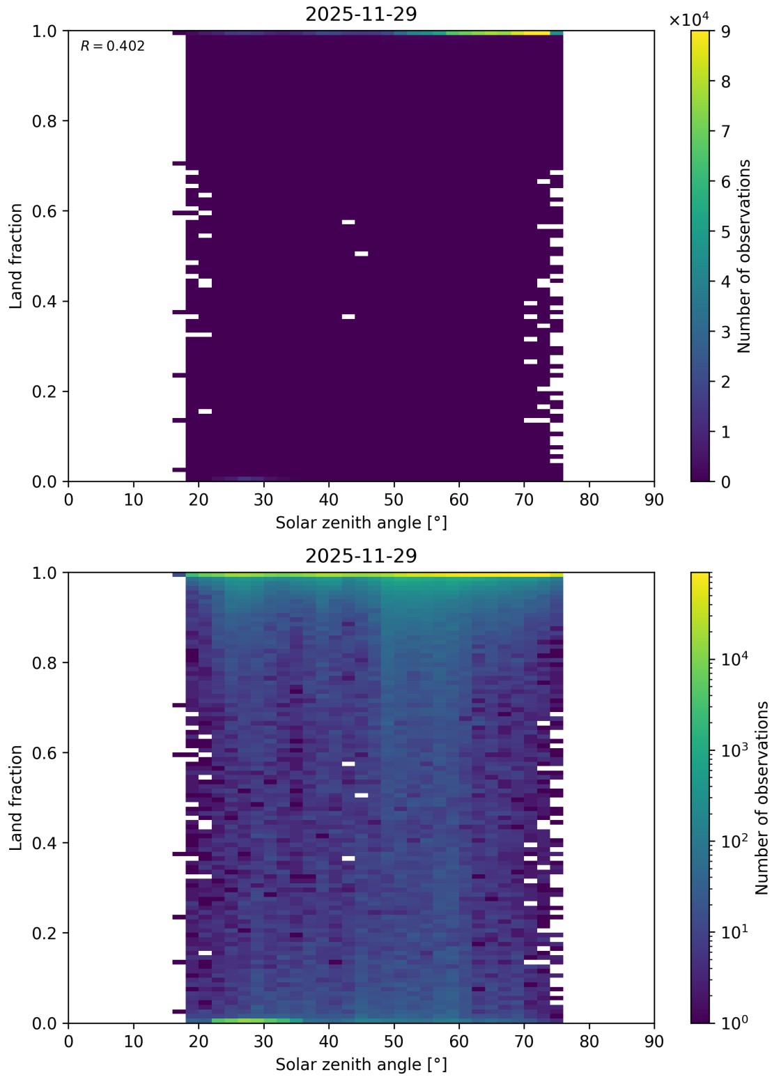
Figure 112: Scatter density plot of “Solar zenith angle” against “Land fraction” for 2025-11-28 to 2025-11-30.
