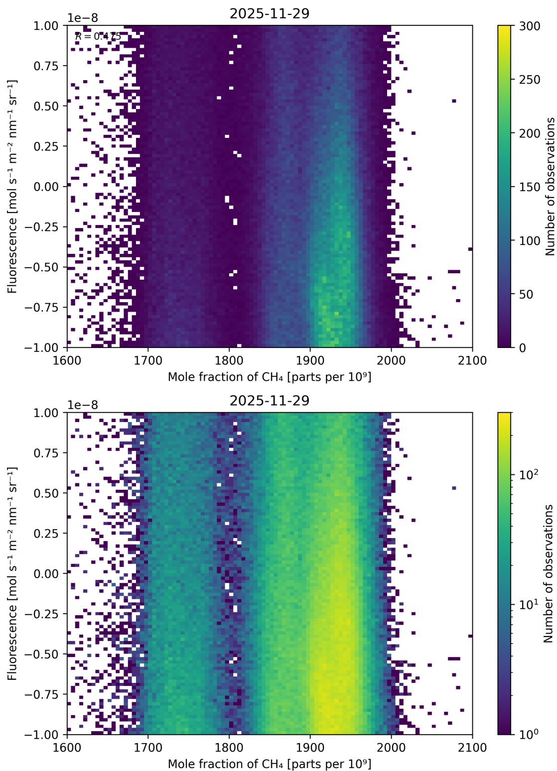
Figure 83: Scatter density plot of “Mole fraction of \text{CH}_4 ” against “Fluorescence” for 2025-11-28 to 2025-11-30.
