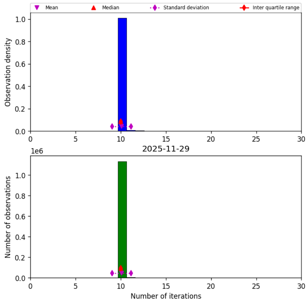
Figure 33: Histogram of “Number of iterations” for 2025-11-28 to 2025-11-30
