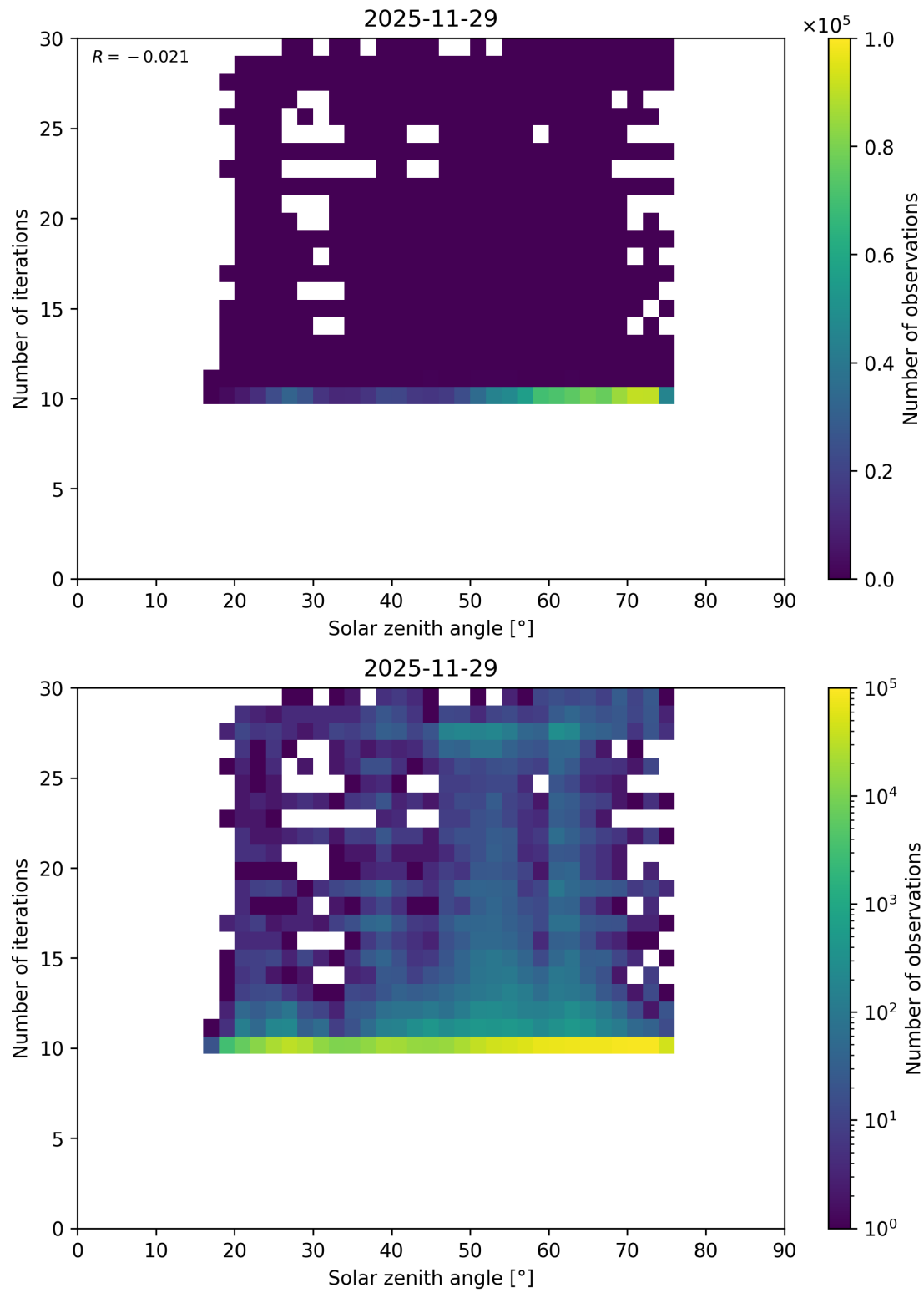
Figure 117: Scatter density plot of “Solar zenith angle” against “Number of iterations” for 2025-11-28 to 2025-11-30.
