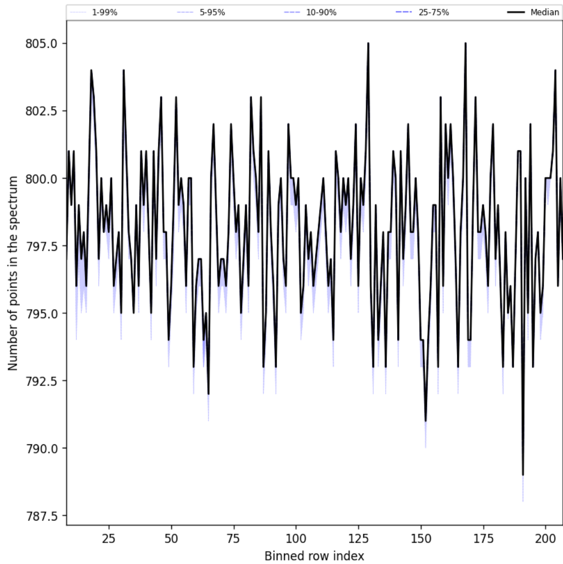
Figure 40: Along track statistics of “Number of points in the spectrum” for 2025-11-28 to 2025-11-30
