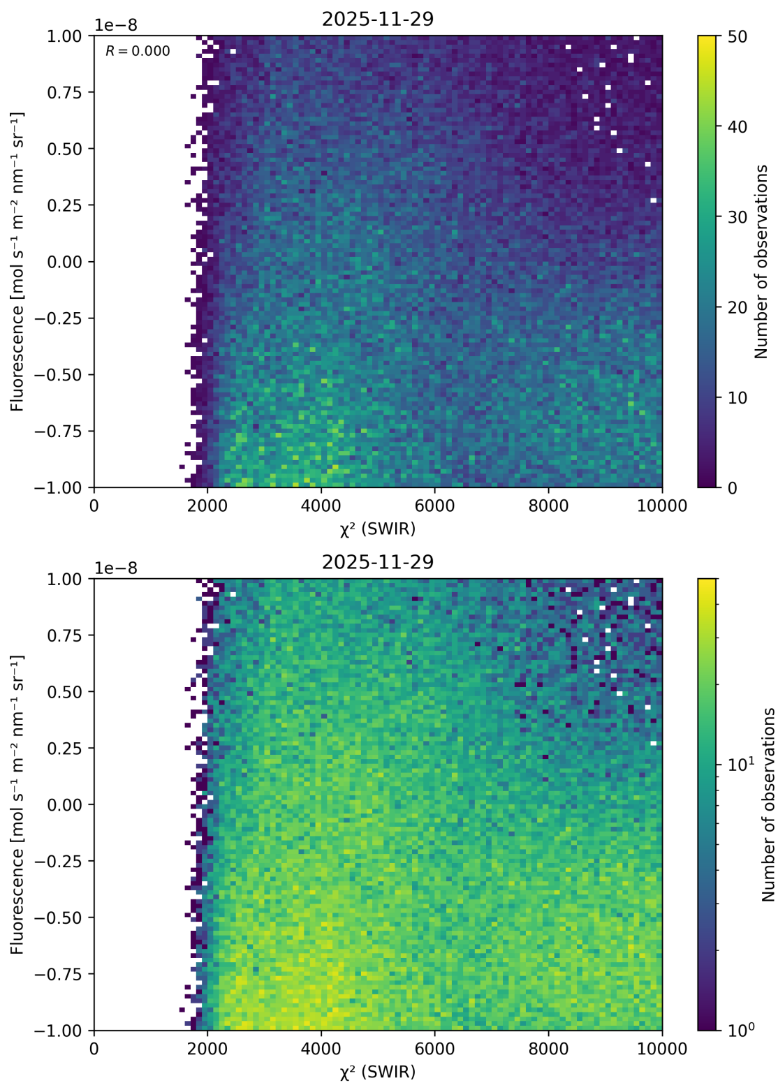
Figure 54: Scatter density plot of “ \chi^2 (SWIR)” against “Fluorescence” for 2025-11-28 to 2025-11-30.
