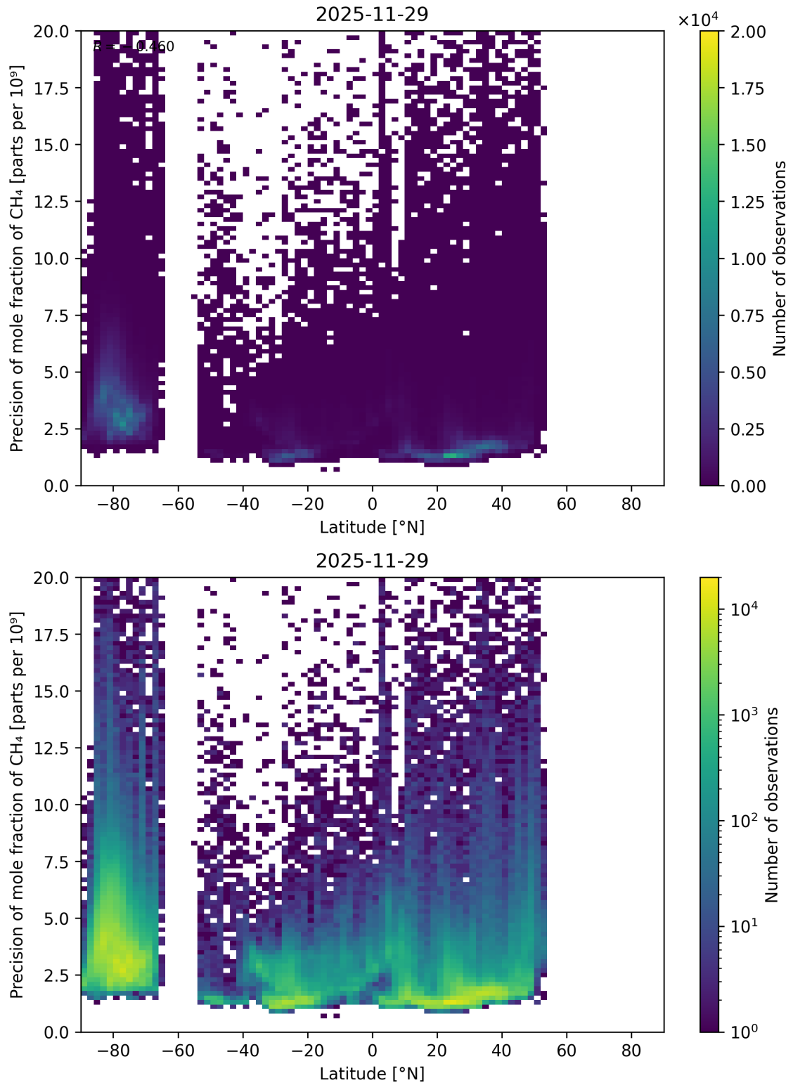
Figure 68: Scatter density plot of “Latitude” against “Precision of mole fraction of CH 4 ” for 2025-11-28 to 2025-11-30.
