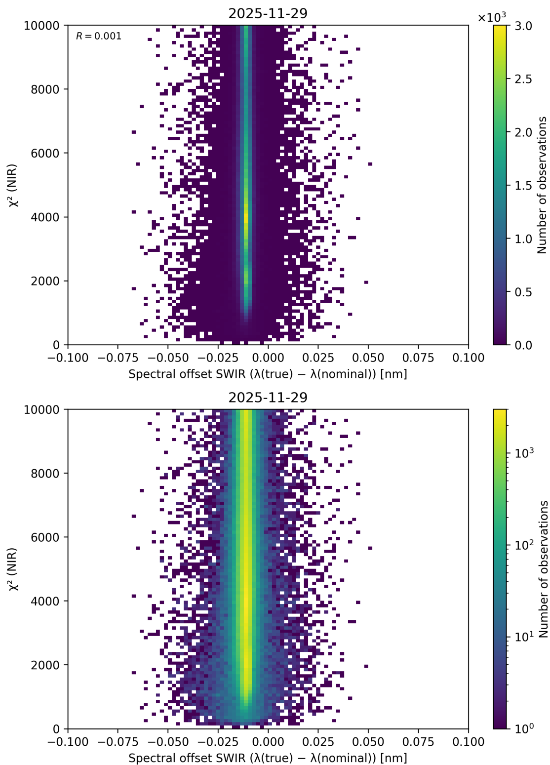
Figure 133: Scatter density plot of “Spectral offset SWIR ( \lambda_{\text{true}} - \lambda_{\text{nominal}} )” against “ \chi^2 (NIR)” for 2025-11-28 to 2025-11-30.
