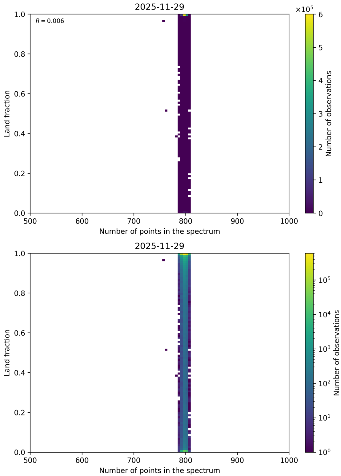
Figure 105: Scatter density plot of “Number of points in the spectrum” against “Land fraction” for 2025-11-28 to 2025-11-30.
