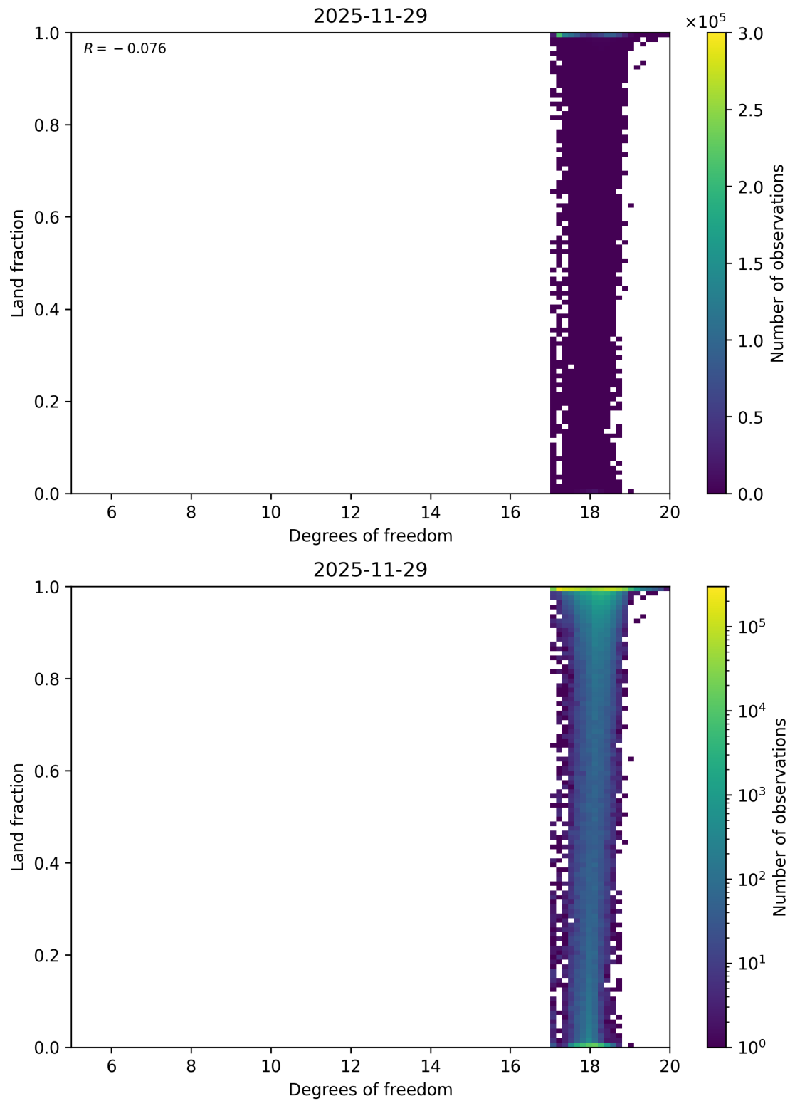
Figure 58: Scatter density plot of “Degrees of freedom” against “Land fraction” for 2025-11-28 to 2025-11-30.
