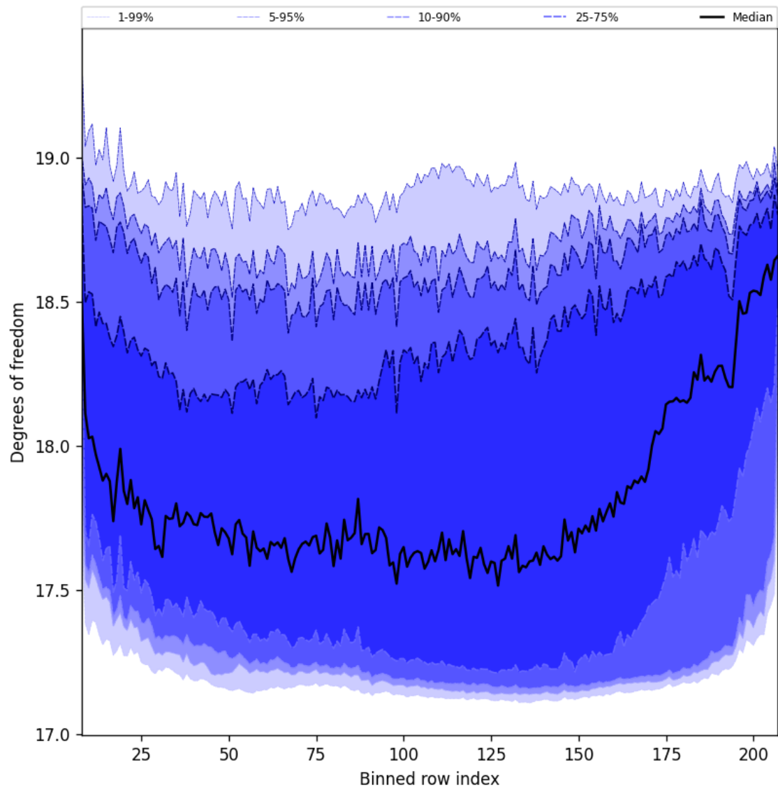
Figure 44: Along track statistics of “Degrees of freedom” for 2025-11-28 to 2025-11-30
