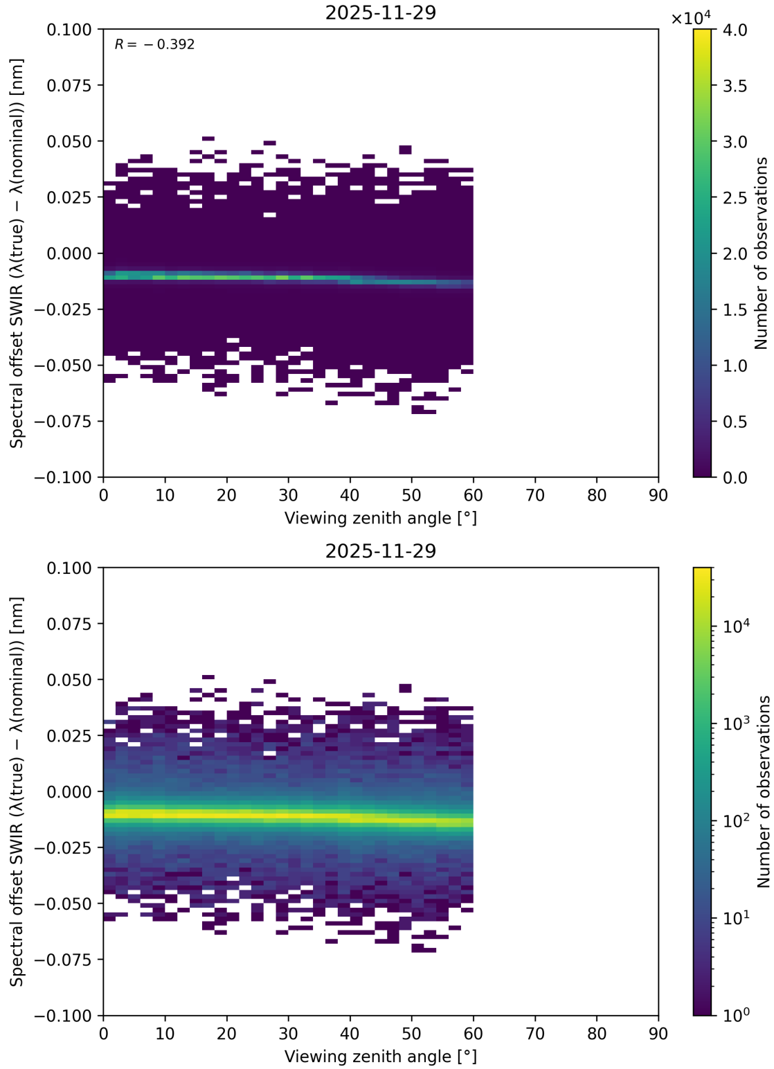
Figure 132: Scatter density plot of “Viewing zenith angle” against “Spectral offset SWIR ( \lambda_{\text{true}} - \lambda_{\text{nominal}} )” for 2025-11-28 to 2025-11-30.
