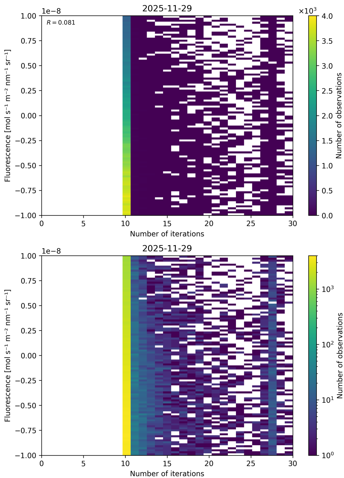
Figure 99: Scatter density plot of “Number of iterations” against “Fluorescence” for 2025-11-28 to 2025-11-30.
