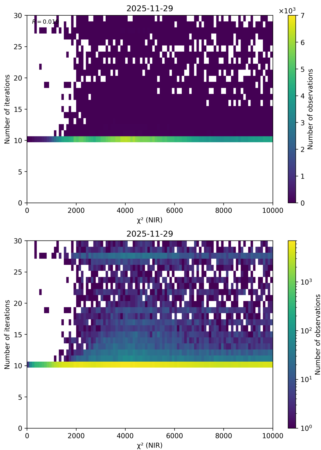
Figure 51: Scatter density plot of “ \chi^2 (NIR)” against “Number of iterations” for 2025-11-28 to 2025-11-30.
