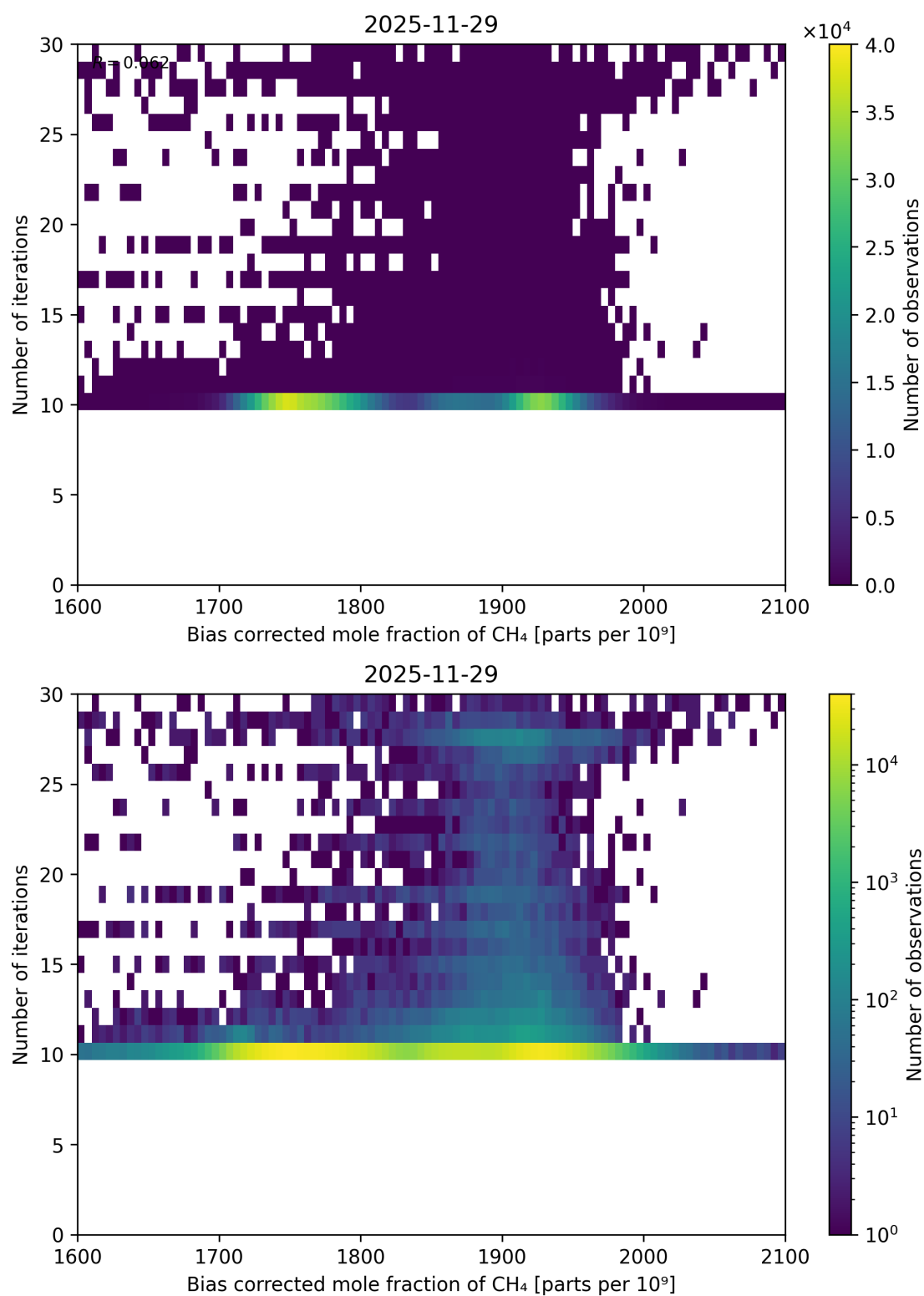
Figure 77: Scatter density plot of “Bias corrected mole fraction of CH 4 ” against “Number of iterations” for 2025-11-28 to 2025-11-30.
