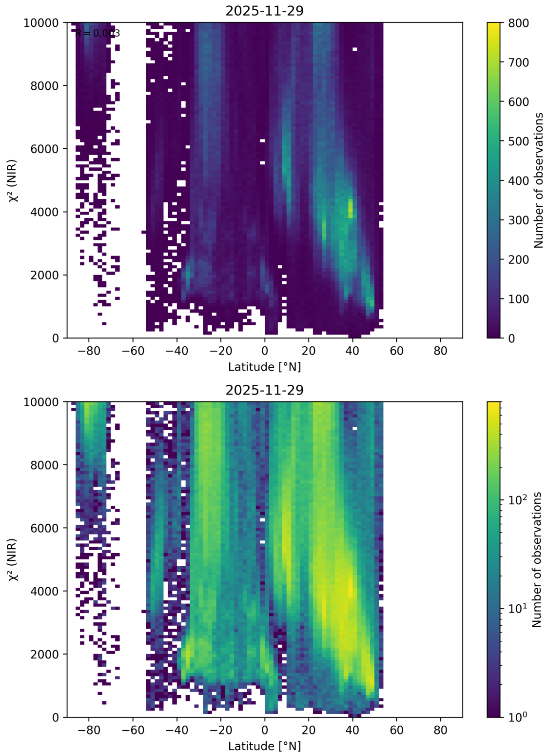
Figure 61: Scatter density plot of “Latitude” against “ \chi^2 (NIR)” for 2025-11-28 to 2025-11-30.
