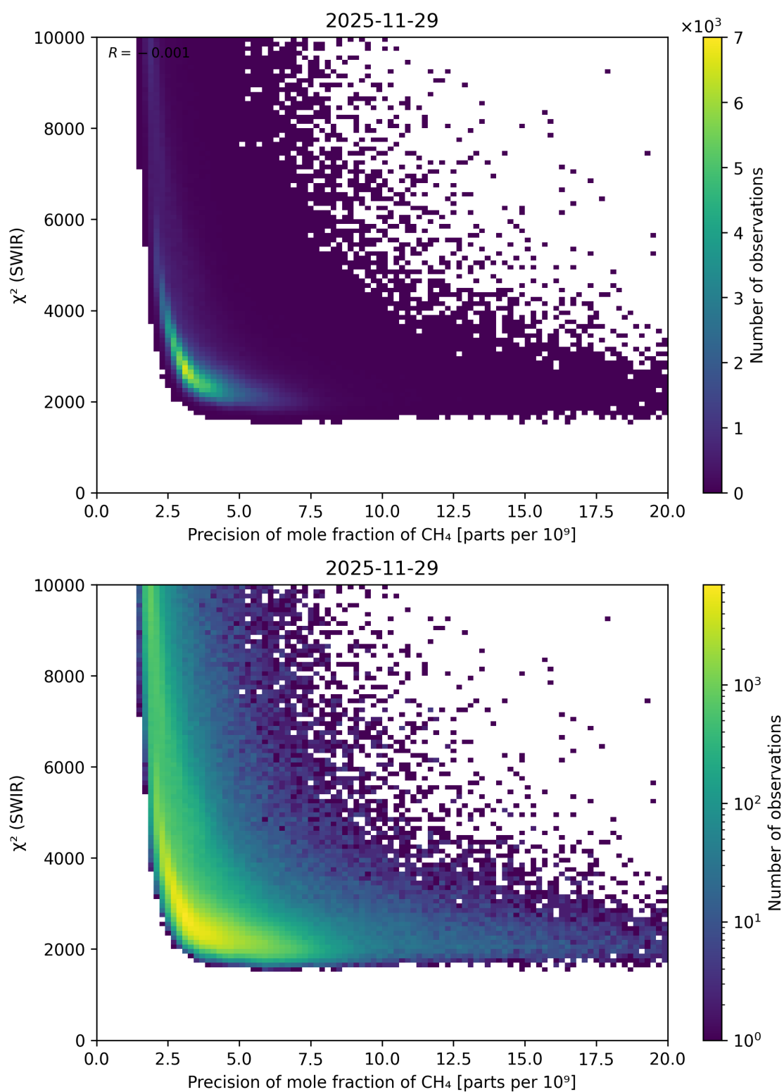
Figure 90: Scatter density plot of “Precision of mole fraction of CH 4 ” against “ \chi^2 (SWIR)” for 2025-11-28 to 2025-11-30.
