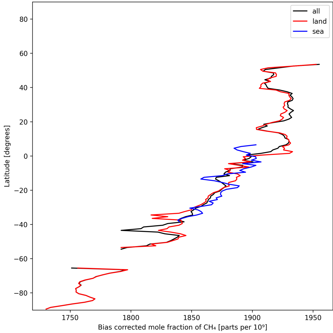
Figure 15: Zonal average of “Bias corrected mole fraction of CH 4 ” for 2025-11-28 to 2025-11-30.
