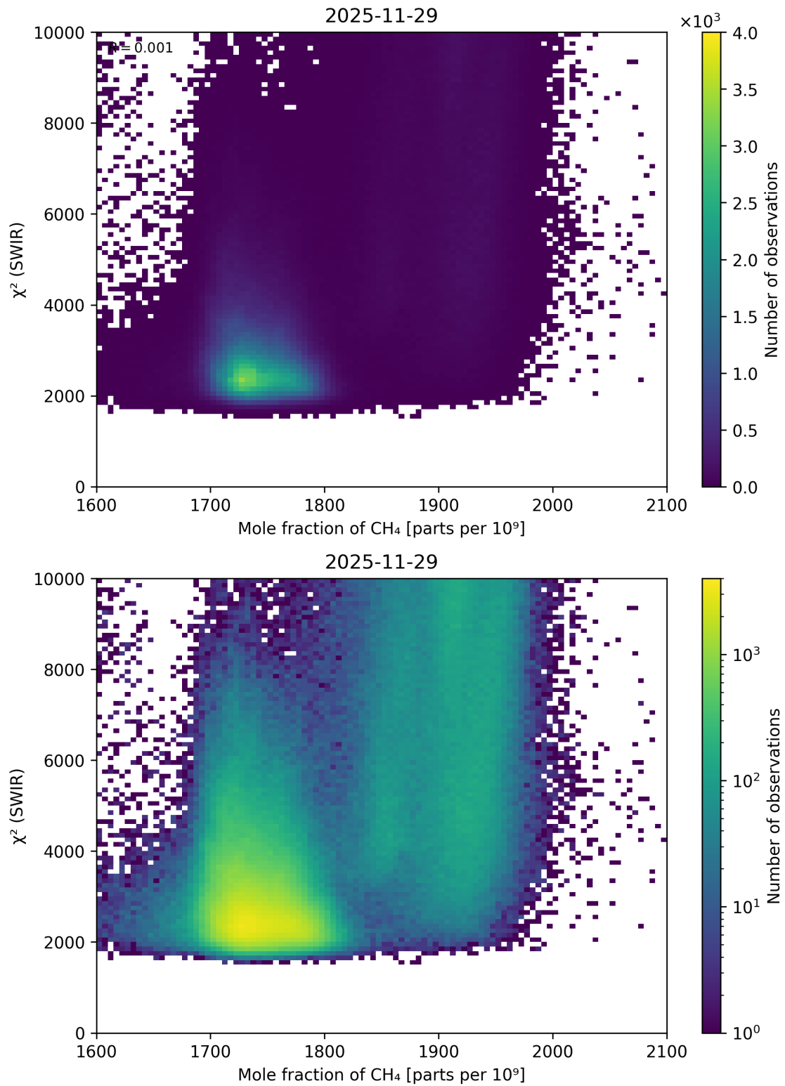
Figure 81: Scatter density plot of “Mole fraction of \text{CH}_4 ” against “ \chi^2 (SWIR)” for 2025-11-28 to 2025-11-30.
