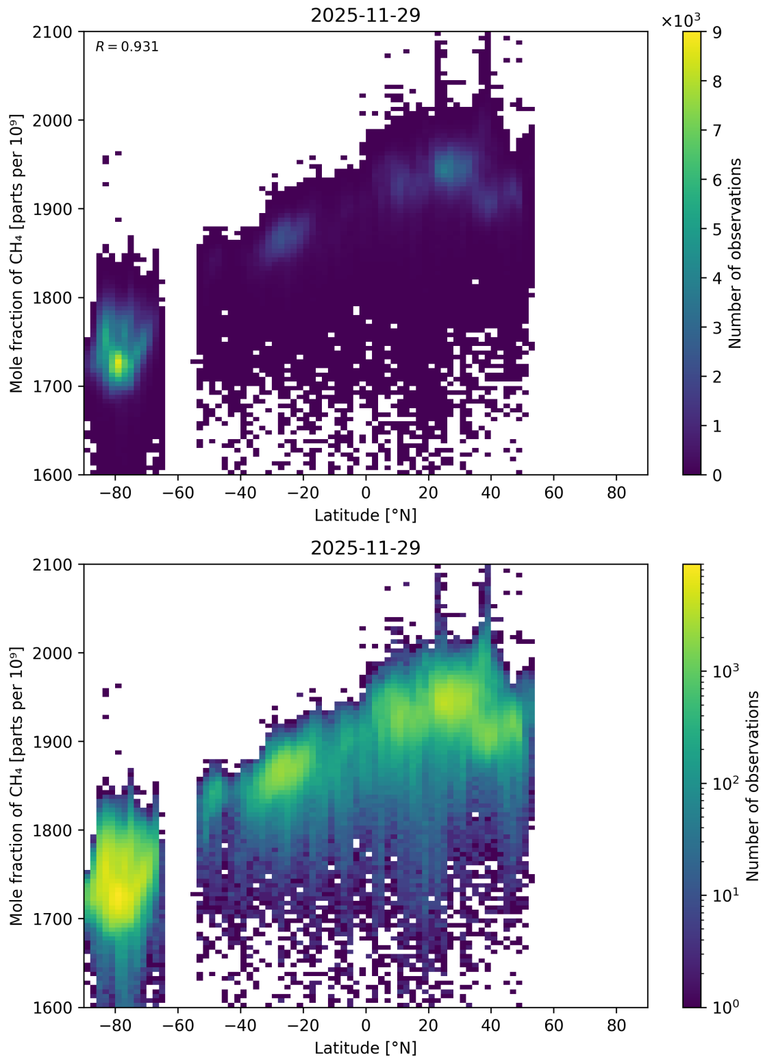
Figure 66: Scatter density plot of “Latitude” against “Mole fraction of CH 4 ” for 2025-11-28 to 2025-11-30.
