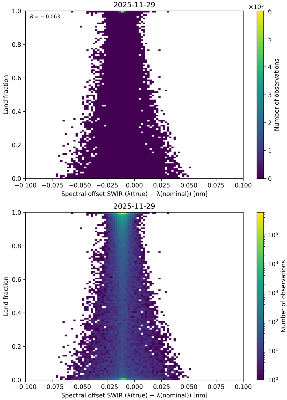
Figure 137: Scatter density plot of “Spectral offset SWIR ( \lambda_{\text{true}} - \lambda_{\text{nominal}} )” against “Land fraction” for 2025-11-28 to 2025-11-30.
