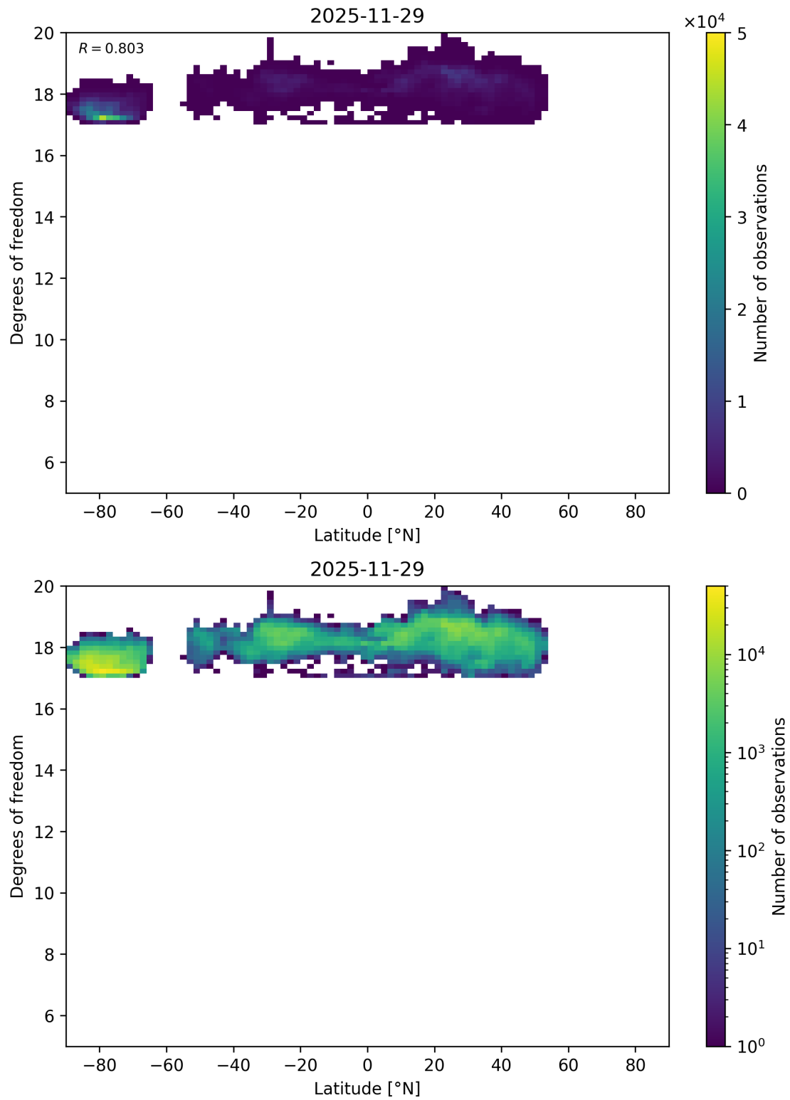
Figure 63: Scatter density plot of “Latitude” against “Degrees of freedom” for 2025-11-28 to 2025-11-30.
