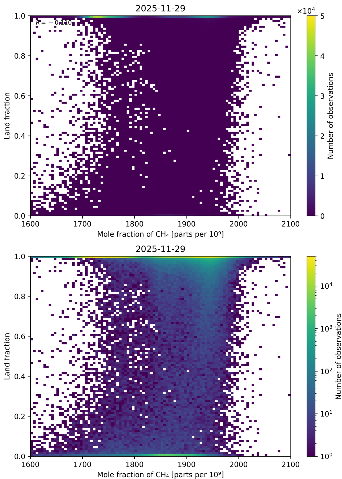
Figure 84: Scatter density plot of “Mole fraction of CH 4 ” against “Land fraction” for 2025-11-28 to 2025-11-30.
