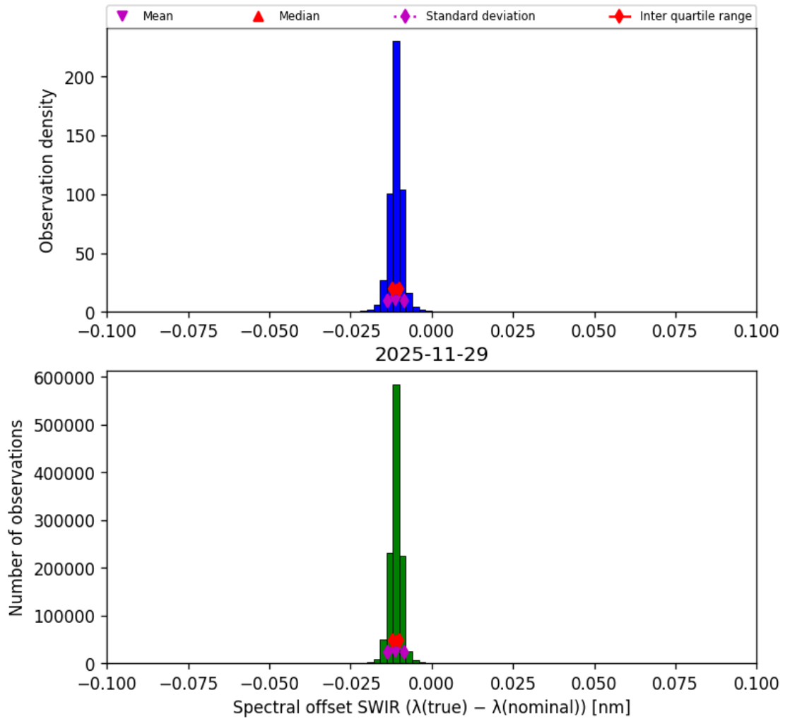
Figure 29: Histogram of “Spectral offset SWIR ( \lambda_{\text{true}} - \lambda_{\text{nominal}} )” for 2025-11-28 to 2025-11-30
