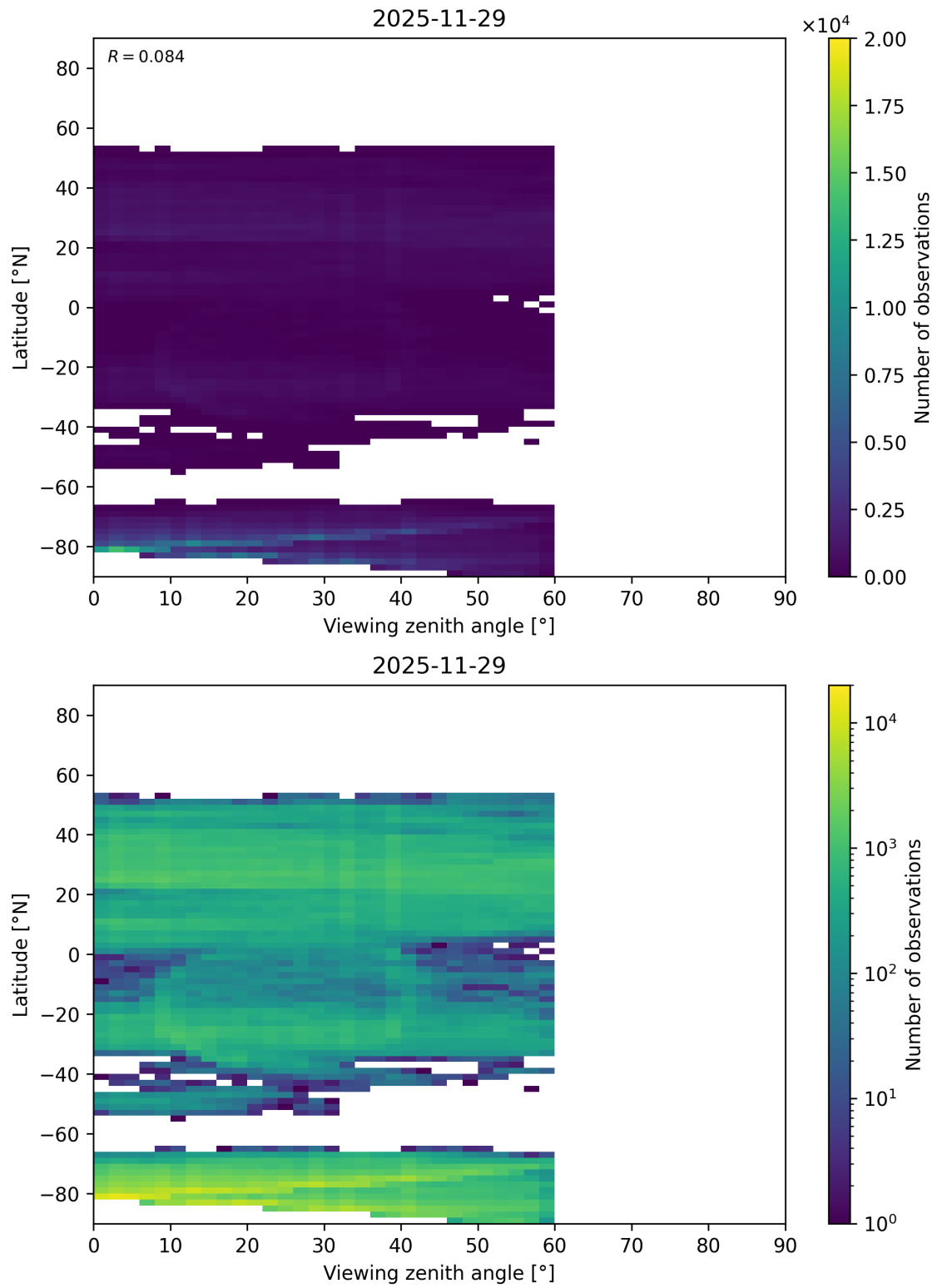
Figure 125: Scatter density plot of “Viewing zenith angle” against “Latitude” for 2025-11-28 to 2025-11-30.
