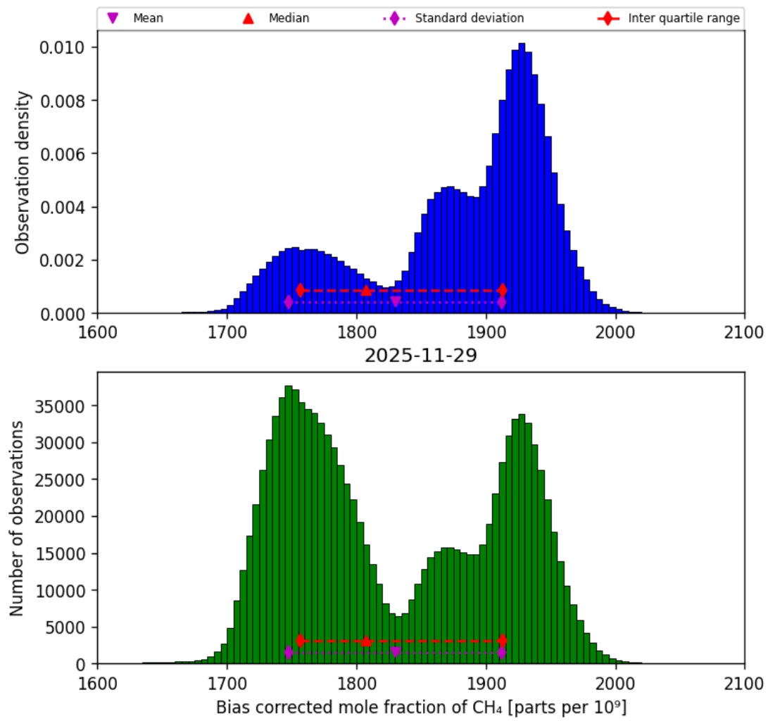
Figure 27: Histogram of “Bias corrected mole fraction of CH 4 ” for 2025-11-28 to 2025-11-30
