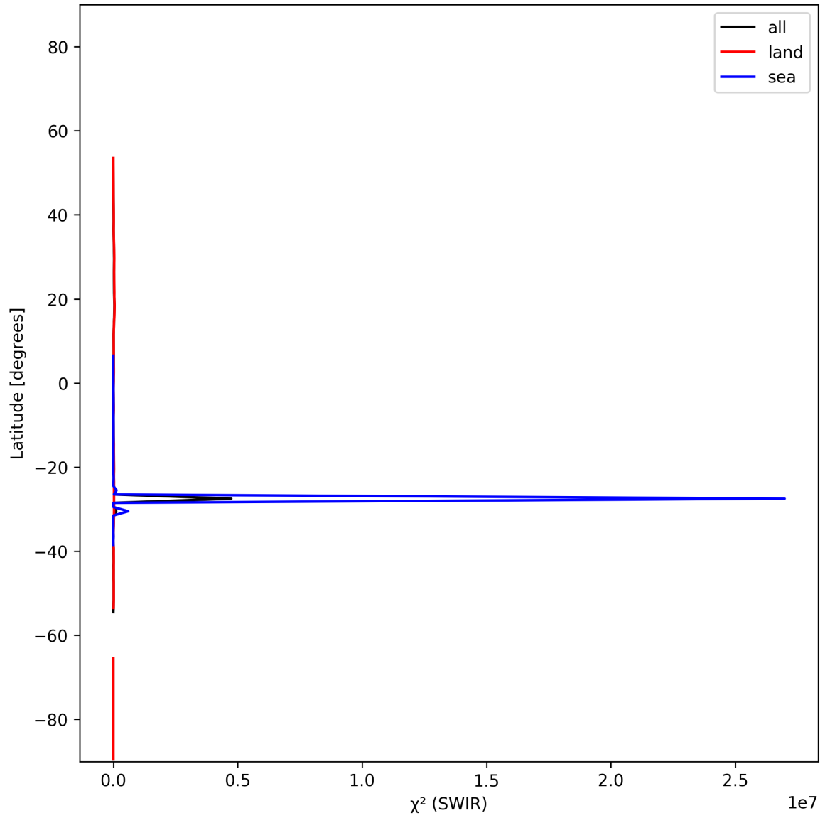
Figure 18: Zonal average of “ \chi^2 (SWIR)” for 2025-11-28 to 2025-11-30.
