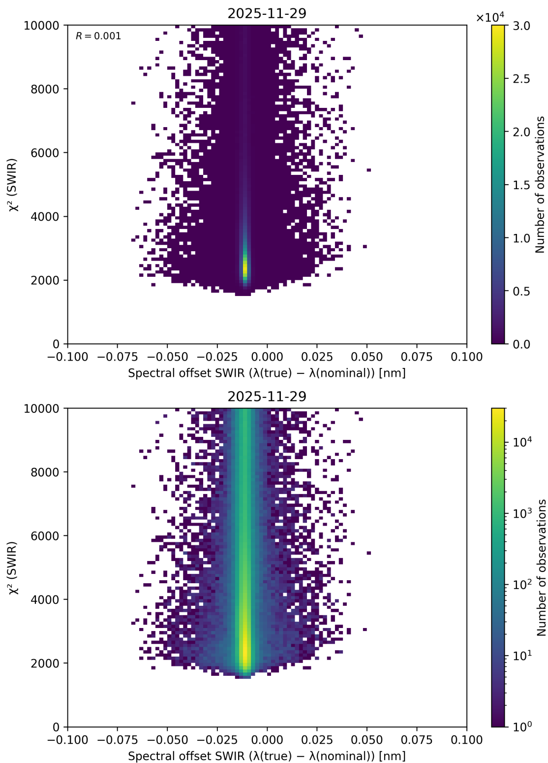
Figure 134: Scatter density plot of “Spectral offset SWIR ( \lambda_{\text{true}} - \lambda_{\text{nominal}} )” against “ \chi^2 (SWIR)” for 2025-11-28 to 2025-11-30.
