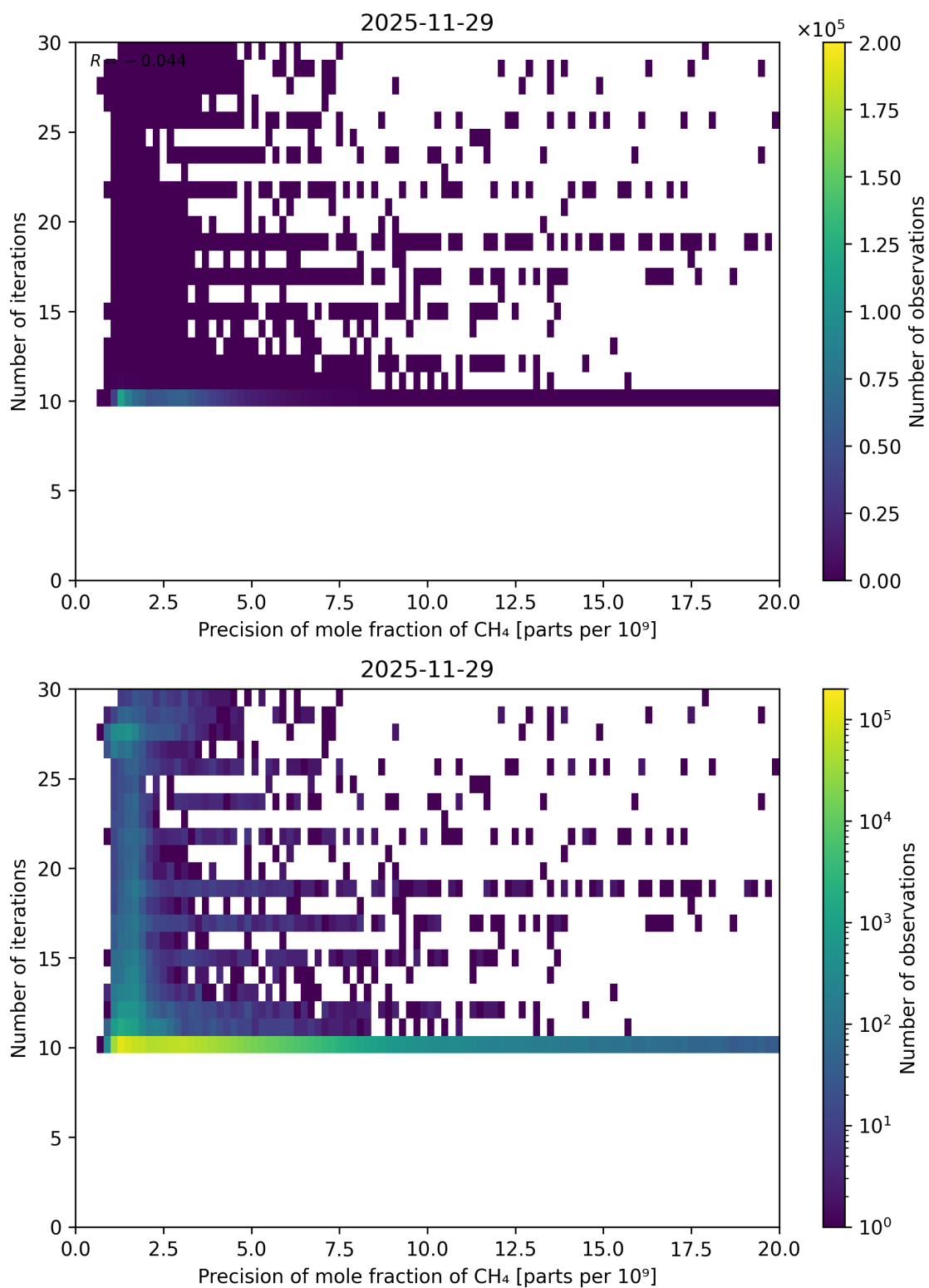
Figure 95: Scatter density plot of “Precision of mole fraction of CH 4 ” against “Number of iterations” for 2025-11-28 to 2025-11-30.
