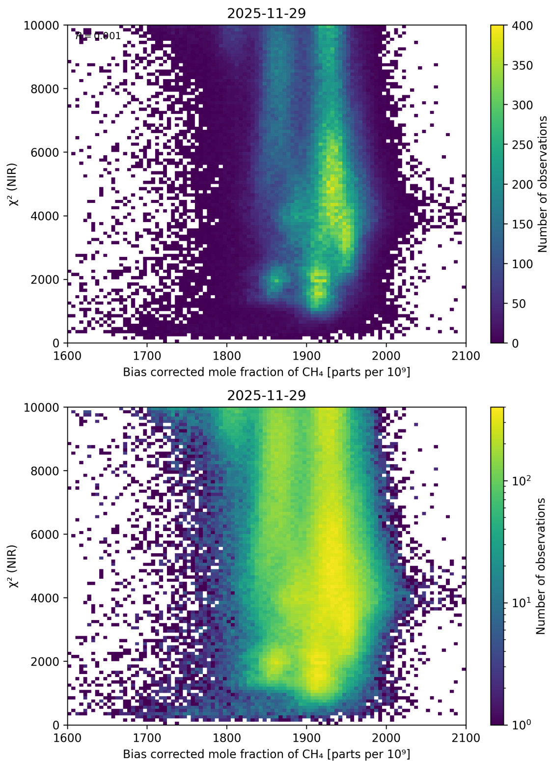
Figure 72: Scatter density plot of “Bias corrected mole fraction of CH 4 ” against “ \chi^2 (NIR)” for 2025-11-28 to 2025-11-30.
