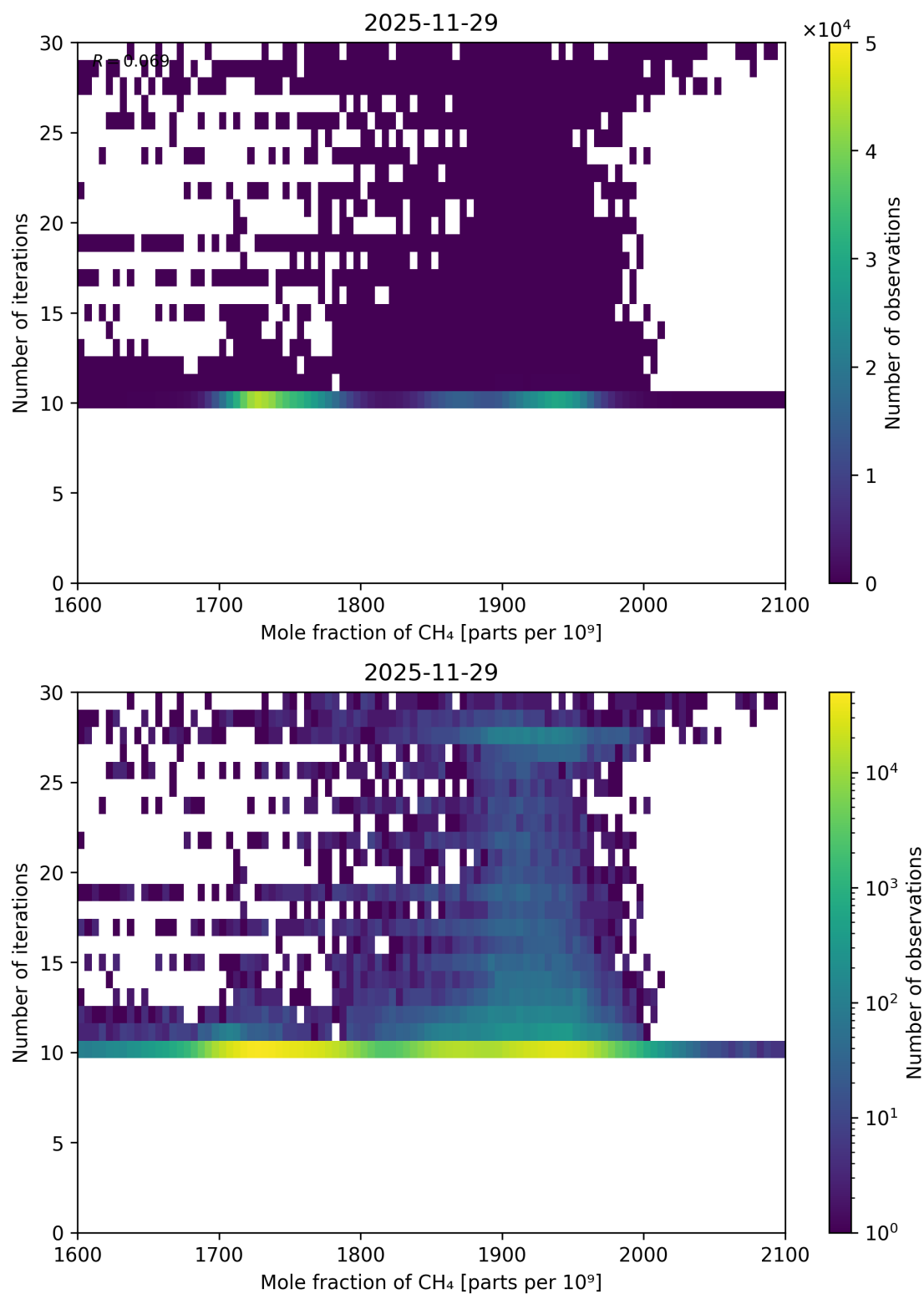
Figure 87: Scatter density plot of “Mole fraction of CH 4 ” against “Number of iterations” for 2025-11-28 to 2025-11-30.
