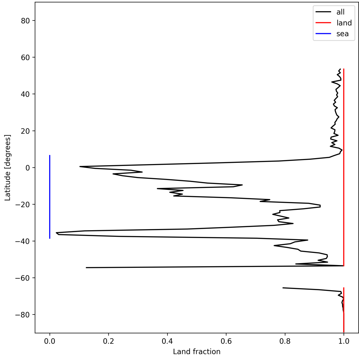
Figure 23: Zonal average of “Land fraction” for 2025-11-28 to 2025-11-30.
