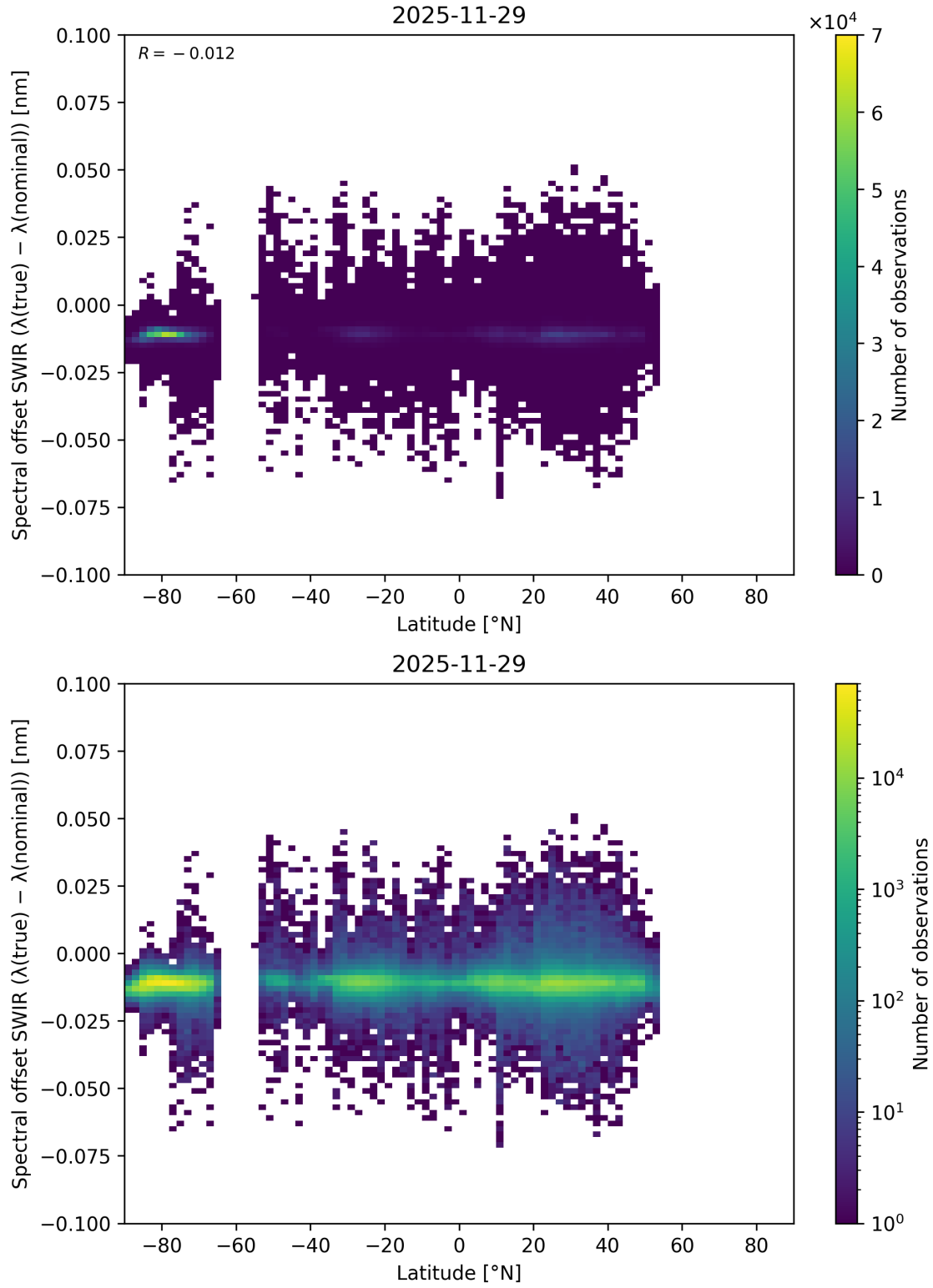
Figure 71: Scatter density plot of “Latitude” against “Spectral offset SWIR ( \lambda_{\text{true}} - \lambda_{\text{nominal}} )” for 2025-11-28 to 2025-11-30.
