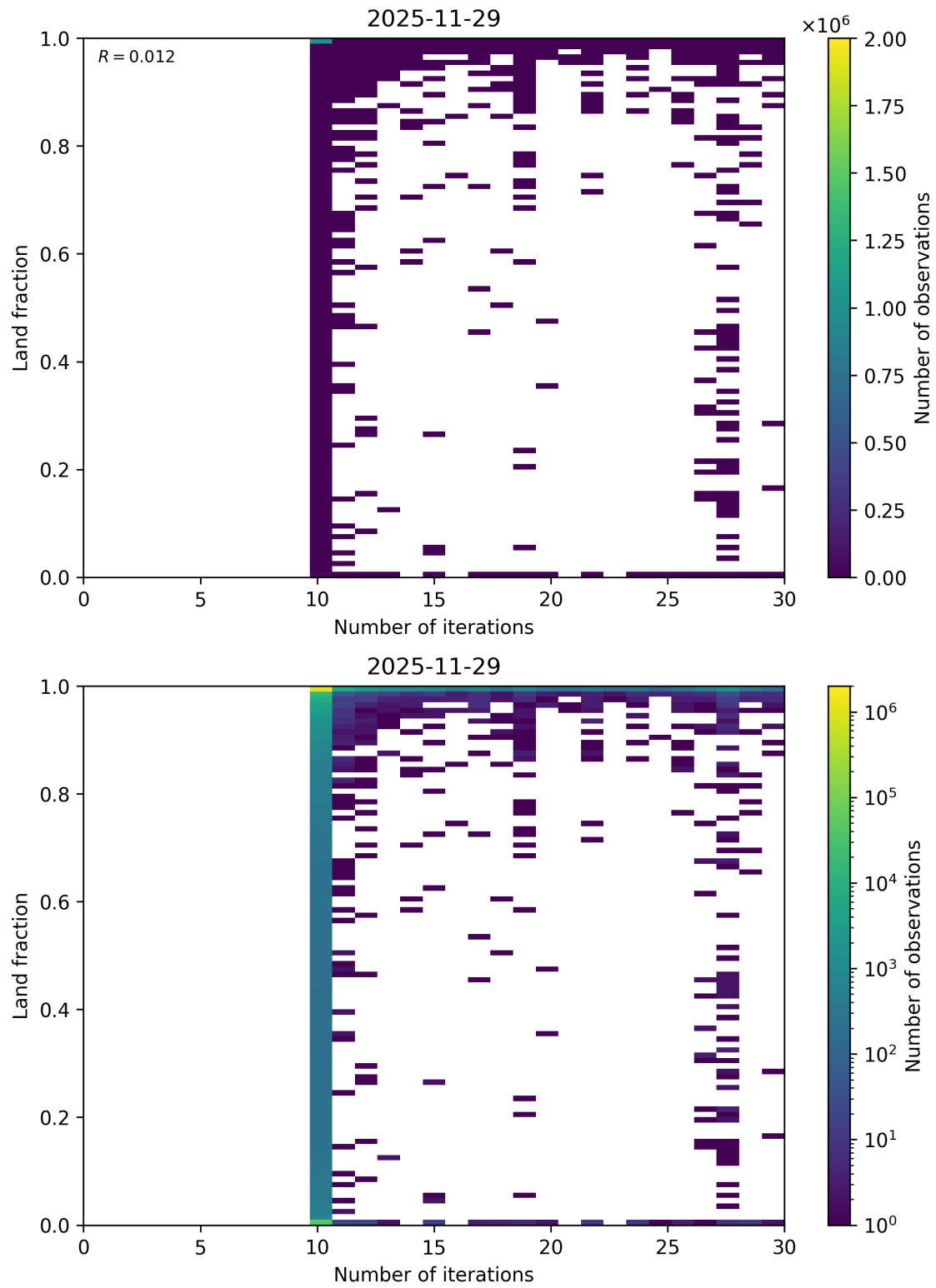
Figure 100: Scatter density plot of “Number of iterations” against “Land fraction” for 2025-11-28 to 2025-11-30.
