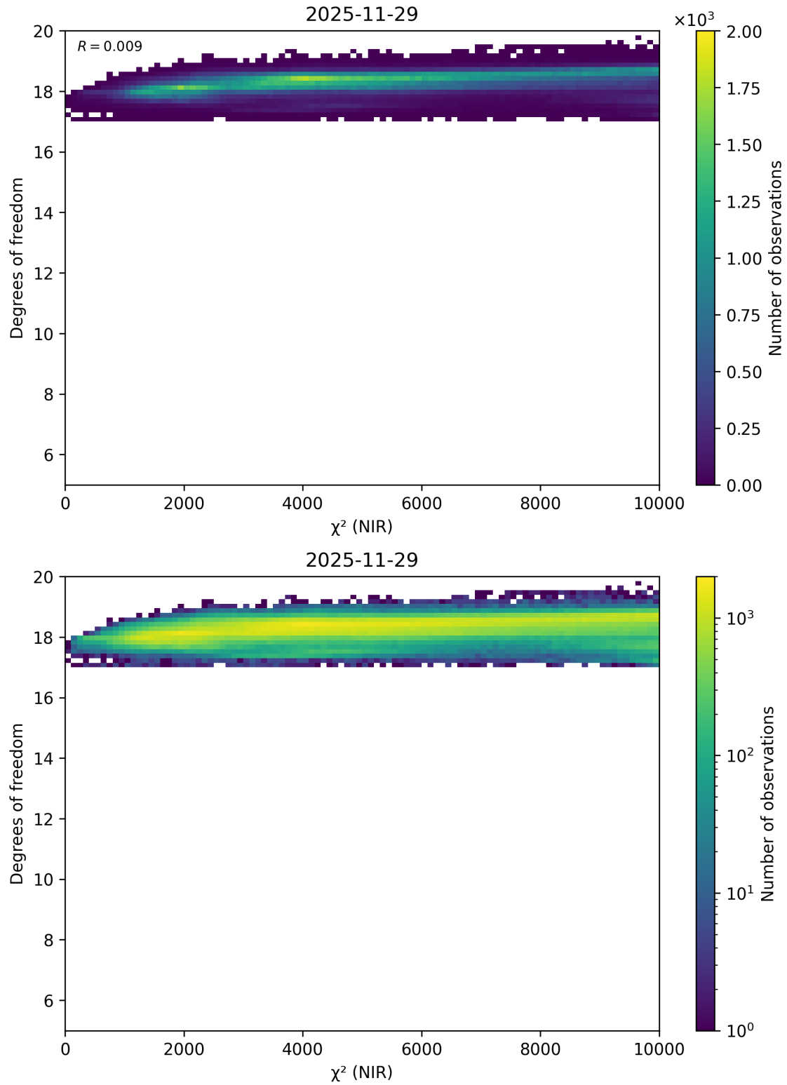
Figure 48: Scatter density plot of “ \chi^2 (NIR)” against “Degrees of freedom” for 2025-11-28 to 2025-11-30.
