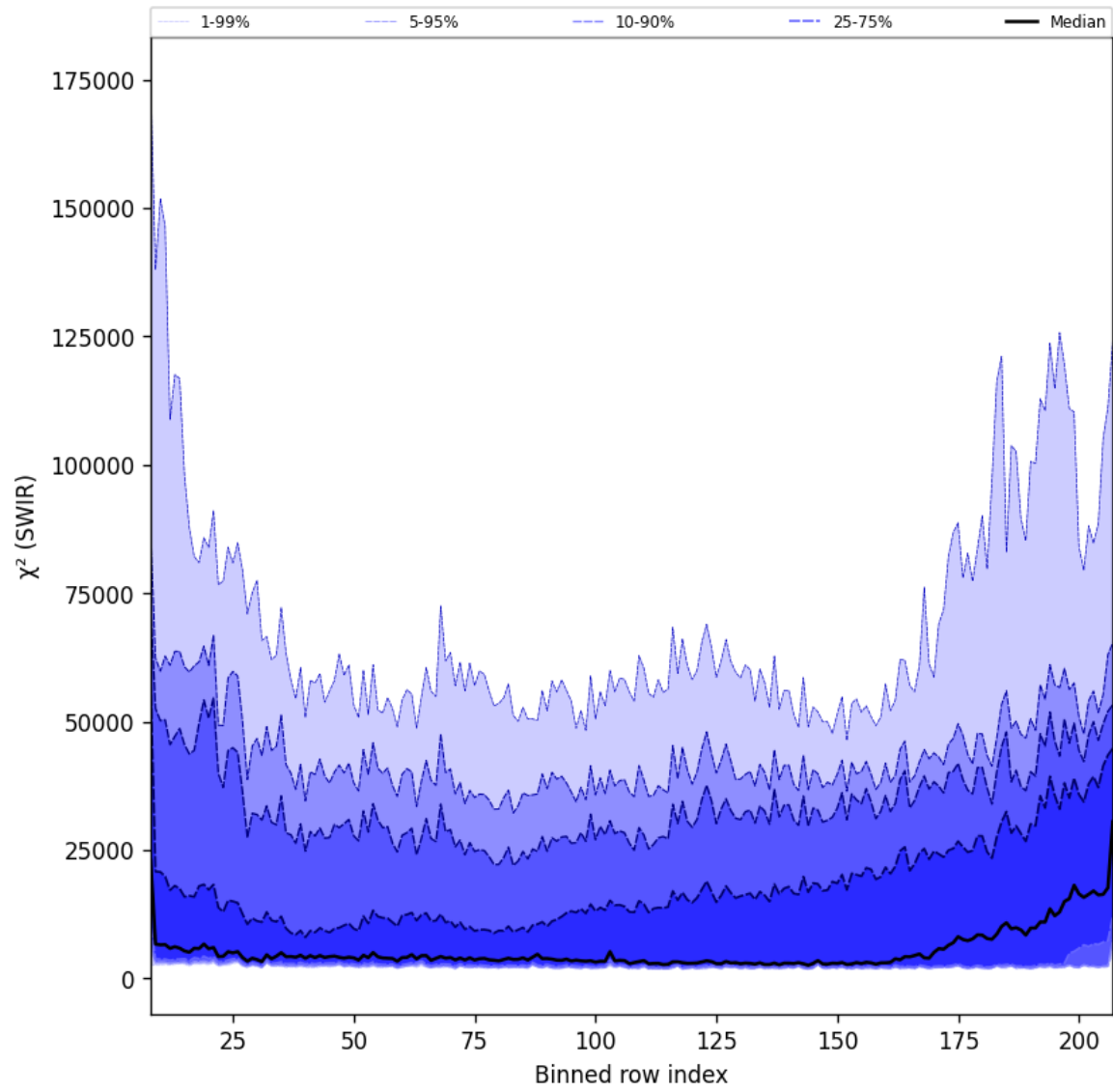
Figure 42: Along track statistics of “ \chi^2 (SWIR)” for 2025-11-28 to 2025-11-30
