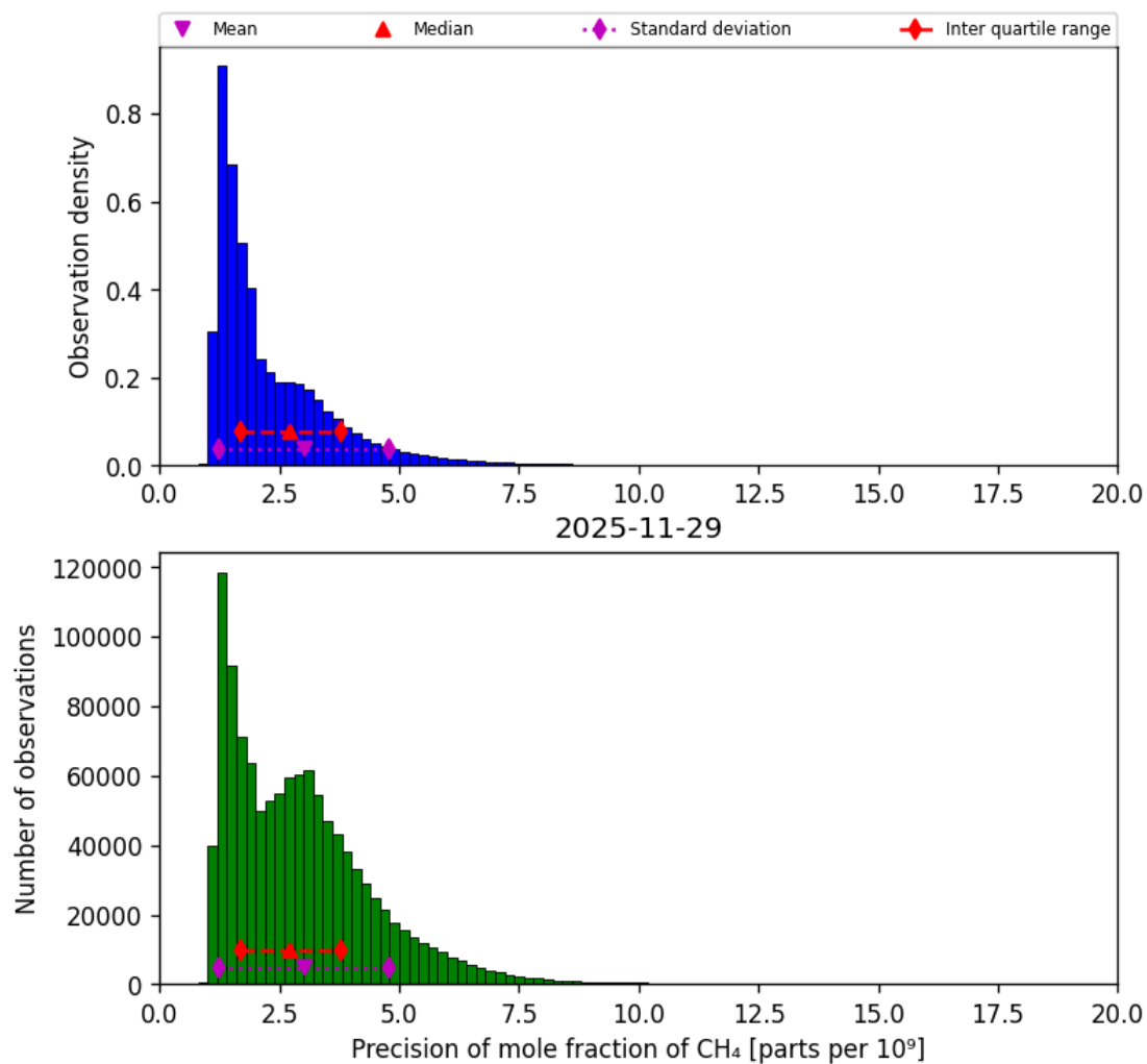
Figure 26: Histogram of “Precision of mole fraction of CH 4 ” for 2025-11-28 to 2025-11-30
