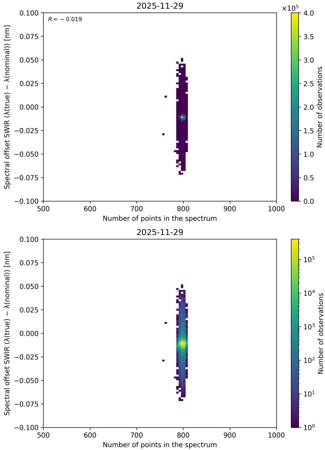
Figure 107: Scatter density plot of “Number of points in the spectrum” against “Spectral offset SWIR ( \lambda_{\text{true}} - \lambda_{\text{nominal}} )” for 2025-11-28 to 2025-11-30.
