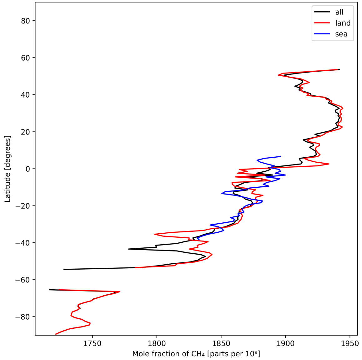
Figure 13: Zonal average of “Mole fraction of CH 4 ” for 2025-11-28 to 2025-11-30.
