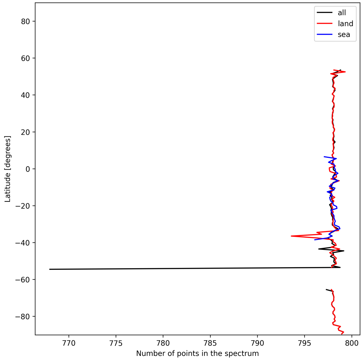
Figure 16: Zonal average of “Number of points in the spectrum” for 2025-11-28 to 2025-11-30.
