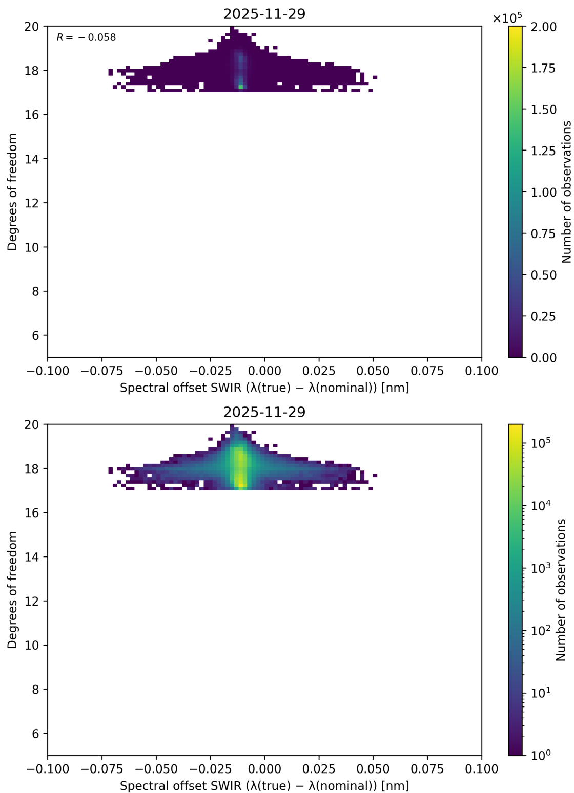
Figure 135: Scatter density plot of “Spectral offset SWIR ( \lambda_{\text{true}} - \lambda_{\text{nominal}} )” against “Degrees of freedom” for 2025-11-28 to 2025-11-30.
