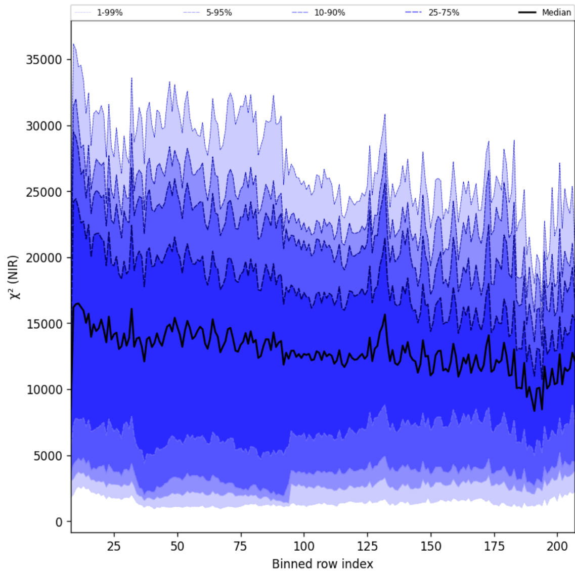
Figure 43: Along track statistics of “ \chi^2 (NIR)” for 2025-11-28 to 2025-11-30
