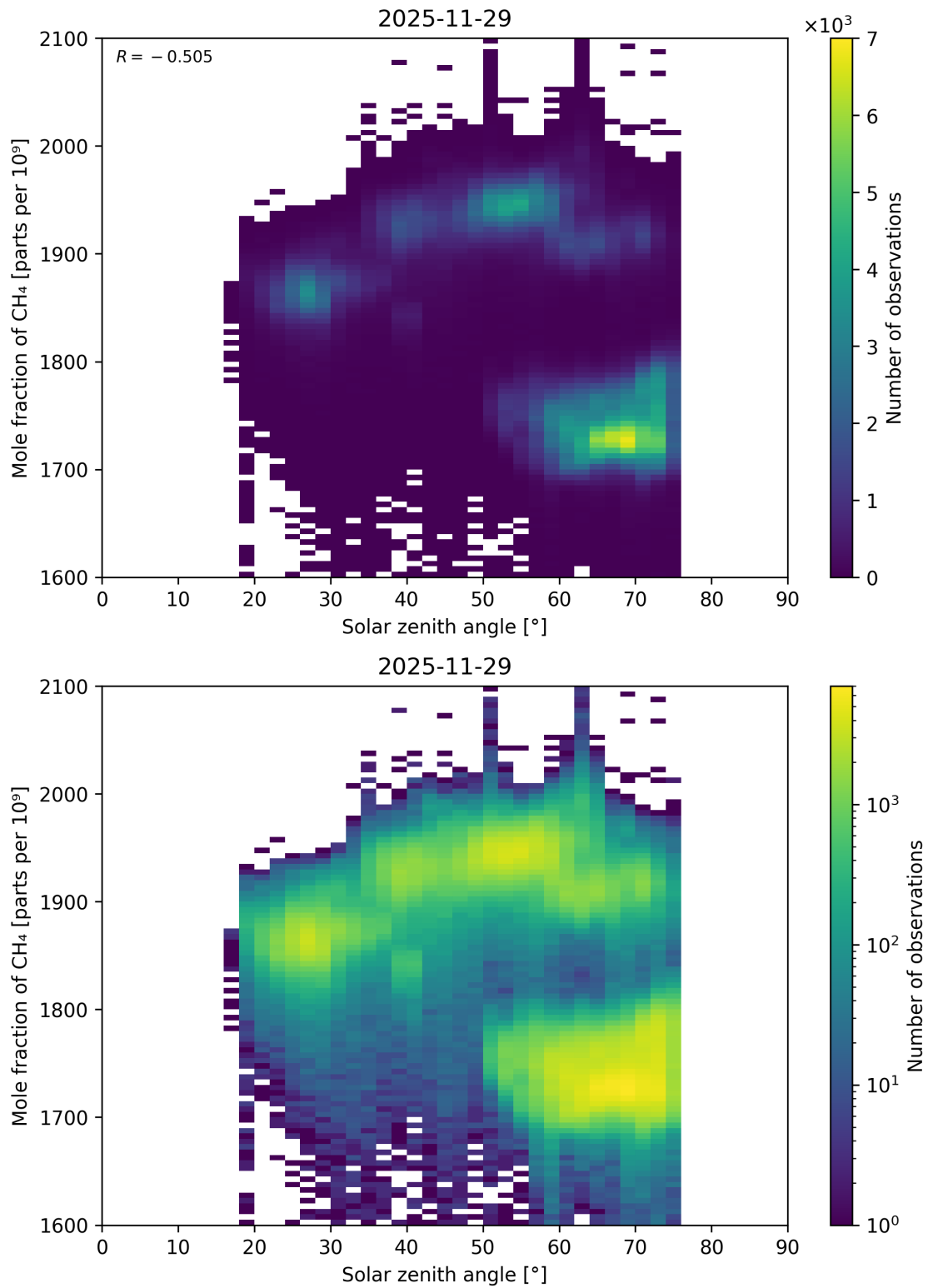
Figure 114: Scatter density plot of “Solar zenith angle” against “Mole fraction of CH 4 ” for 2025-11-28 to 2025-11-30.
