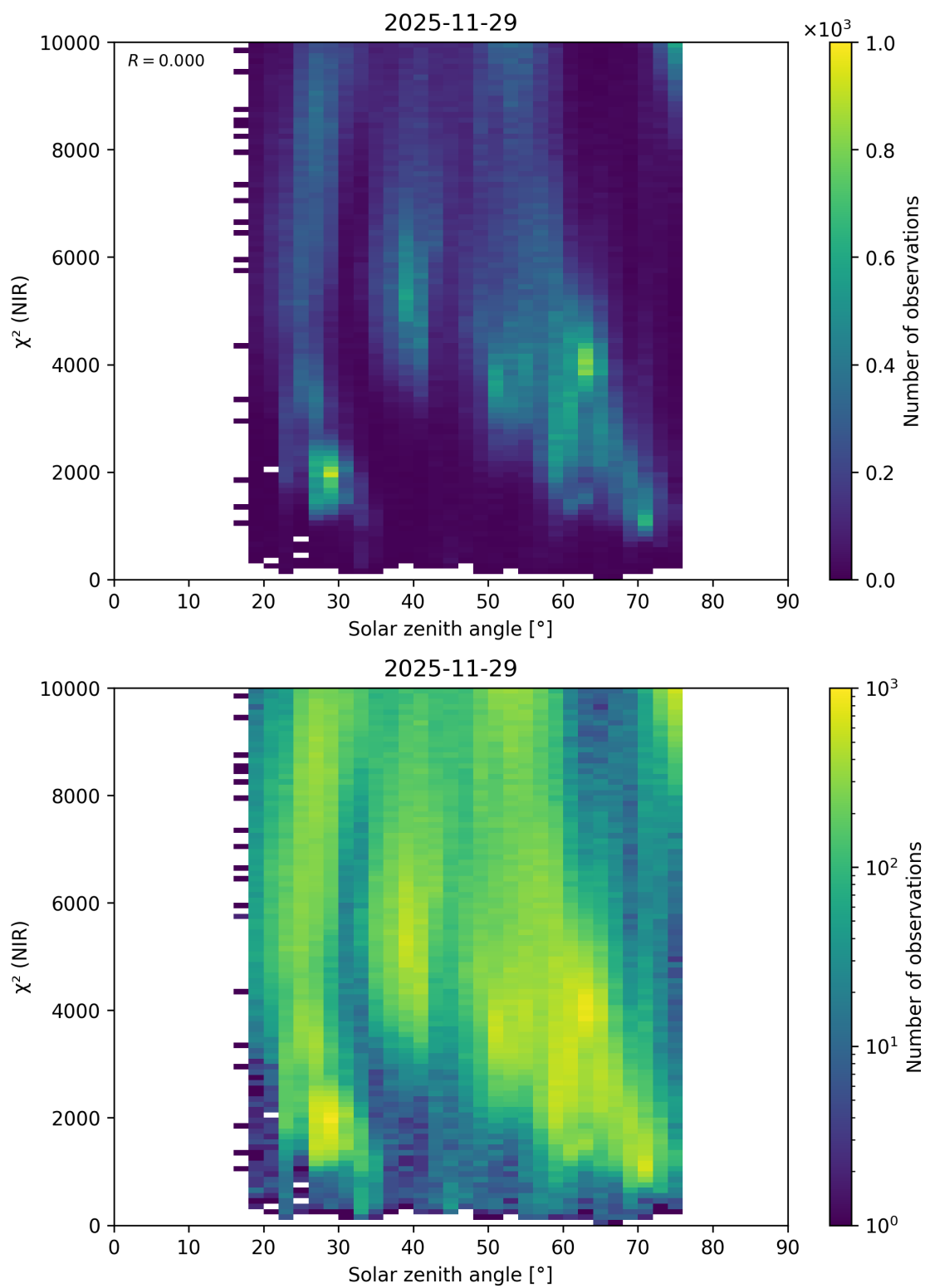
Figure 108: Scatter density plot of “Solar zenith angle” against “ \chi^2 (NIR)” for 2025-11-28 to 2025-11-30.
