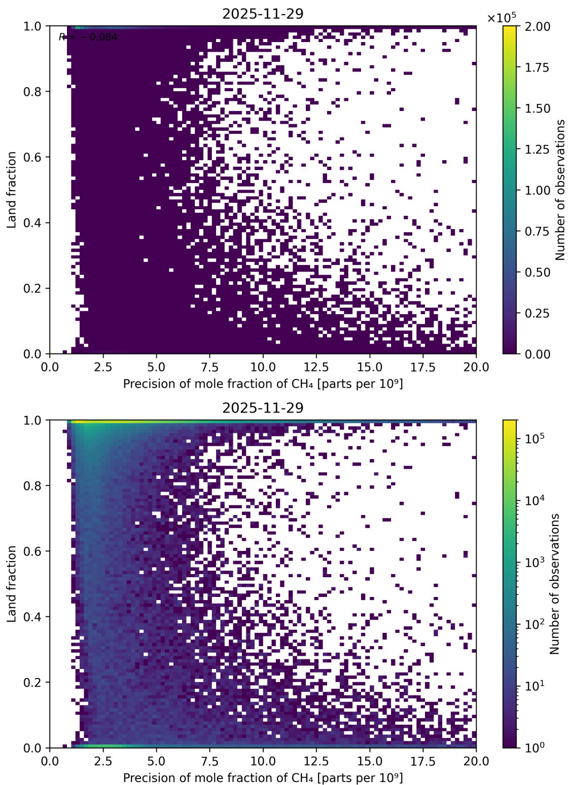
Figure 93: Scatter density plot of “Precision of mole fraction of CH 4 ” against “Land fraction” for 2025-11-28 to 2025-11-30.
