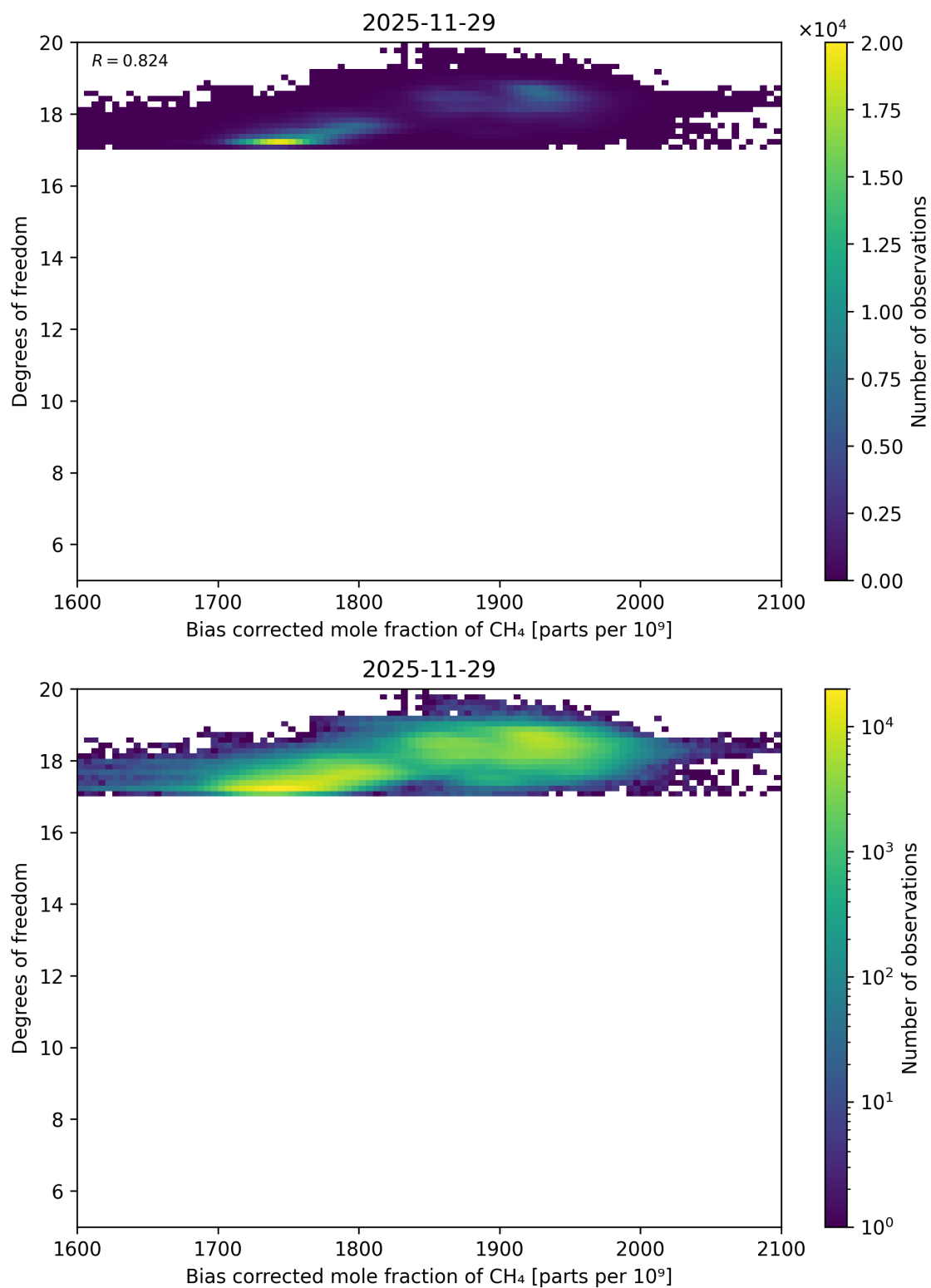
Figure 74: Scatter density plot of “Bias corrected mole fraction of CH 4 ” against “Degrees of freedom” for 2025-11-28 to 2025-11-30.
