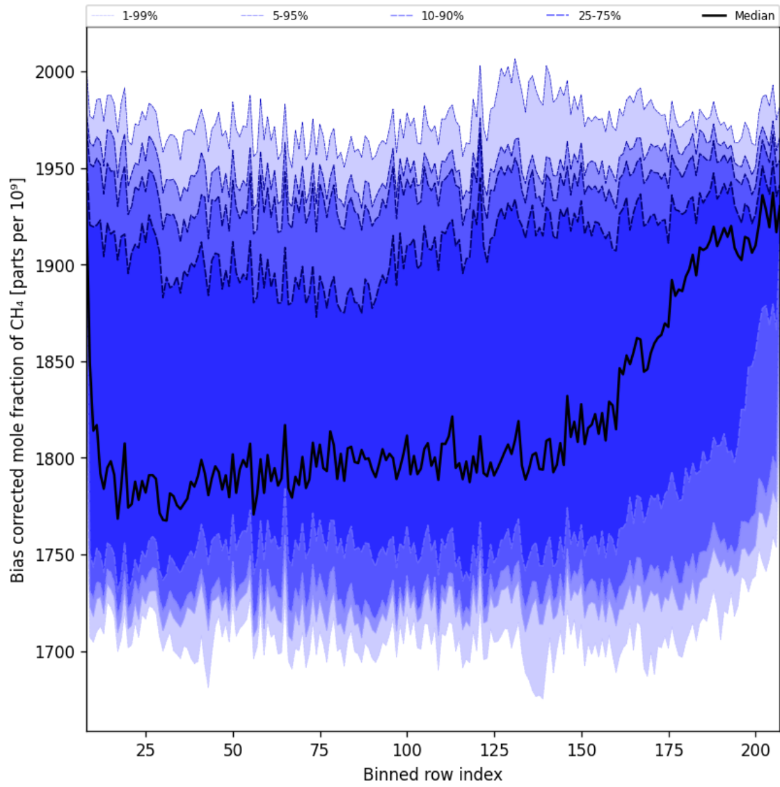
Figure 39: Along track statistics of “Bias corrected mole fraction of CH 4 ” for 2025-11-28 to 2025-11-30
