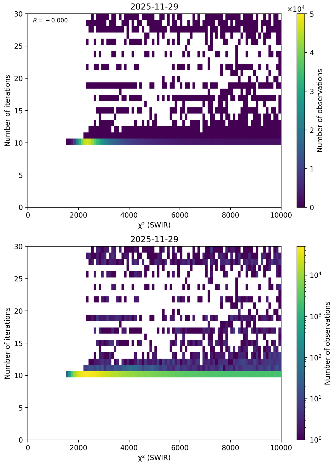
Figure 56: Scatter density plot of “ \chi^2 (SWIR)” against “Number of iterations” for 2025-11-28 to 2025-11-30.
