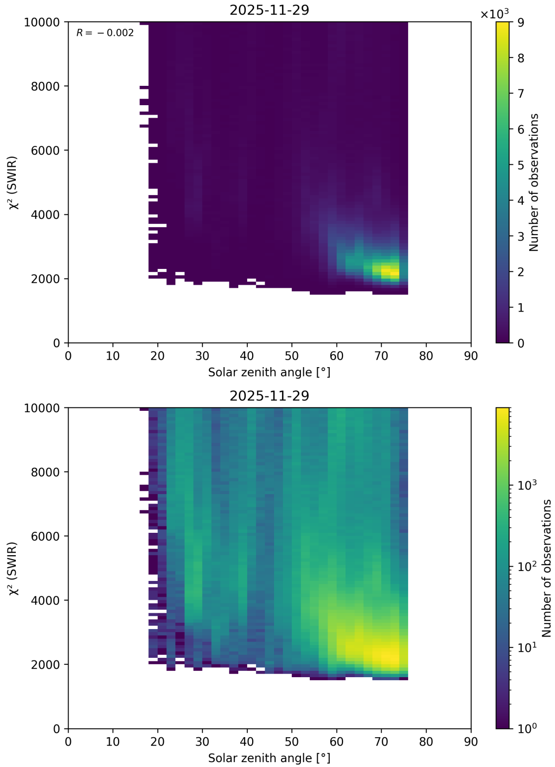
Figure 109: Scatter density plot of “Solar zenith angle” against “ \chi^2 (SWIR)” for 2025-11-28 to 2025-11-30.
