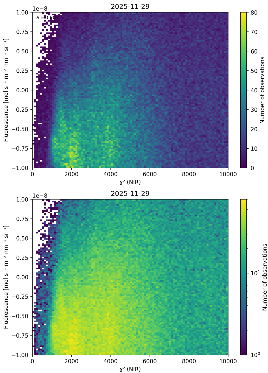
Figure 49: Scatter density plot of “ \chi^2 (NIR)” against “Fluorescence” for 2025-11-28 to 2025-11-30.
