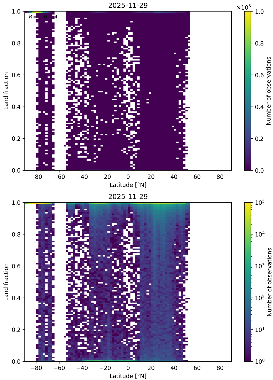
Figure 65: Scatter density plot of “Latitude” against “Land fraction” for 2025-11-28 to 2025-11-30.
