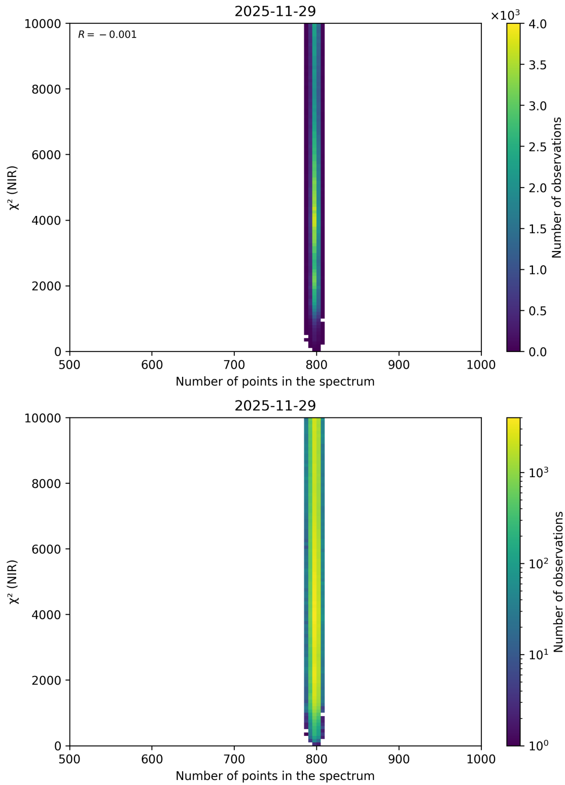
Figure 101: Scatter density plot of “Number of points in the spectrum” against “ \chi^2 (NIR)” for 2025-11-28 to 2025-11-30.
