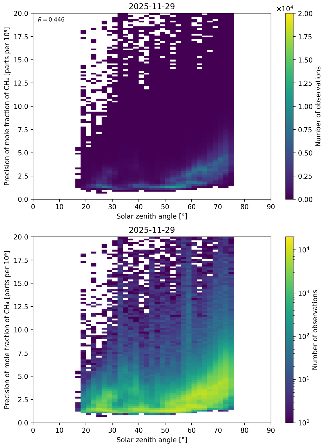
Figure 116: Scatter density plot of “Solar zenith angle” against “Precision of mole fraction of \text{CH}_4 ” for 2025-11-28 to 2025-11-30.
