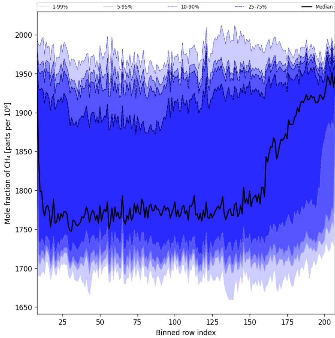
Figure 37: Along track statistics of “Mole fraction of CH 4 ” for 2025-11-28 to 2025-11-30
