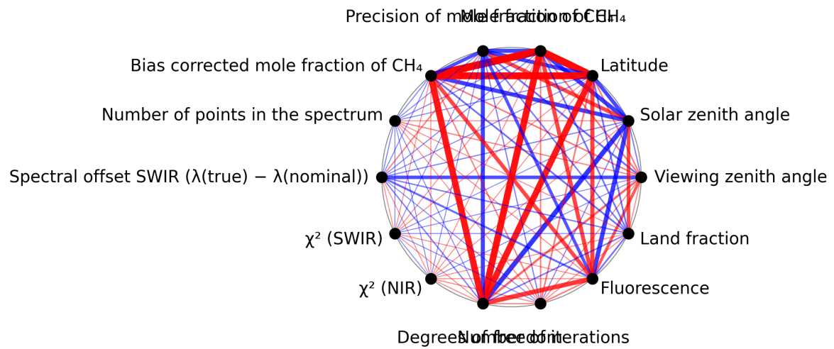
Figure 1: Map of correlation graph for 2025-11-28 to 2025-11-30.
