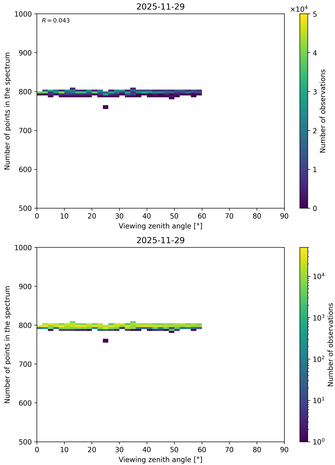
Figure 130: Scatter density plot of “Viewing zenith angle” against “Number of points in the spectrum” for 2025-11-28 to 2025-11-30.
