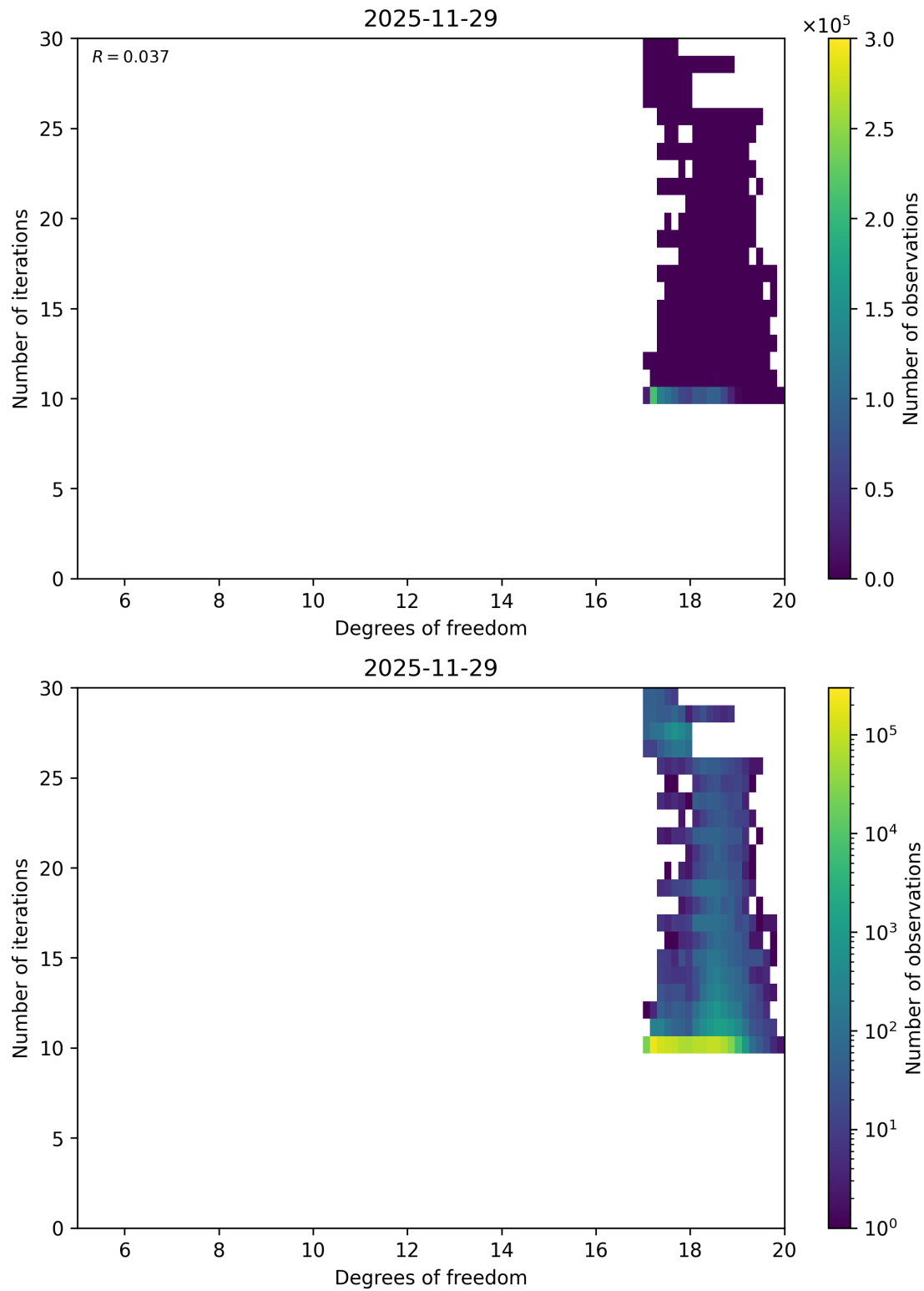
Figure 59: Scatter density plot of “Degrees of freedom” against “Number of iterations” for 2025-11-28 to 2025-11-30.
