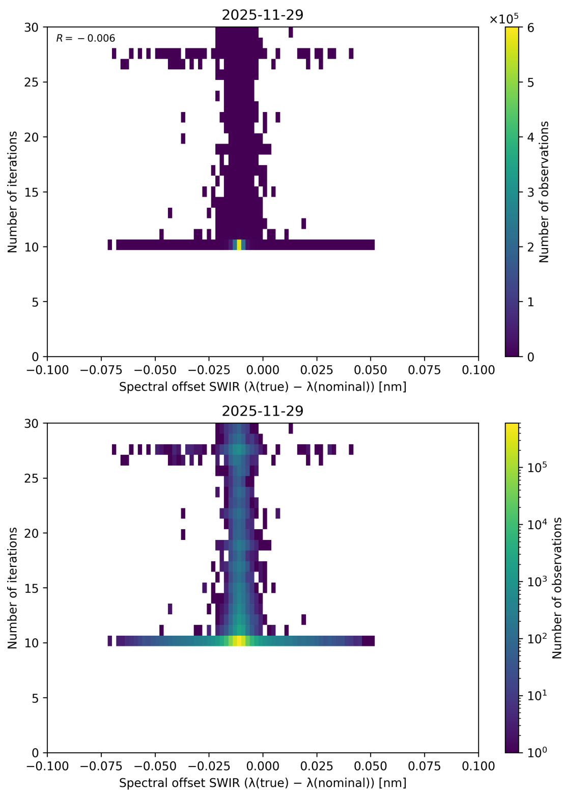
Figure 138: Scatter density plot of “Spectral offset SWIR ( \lambda_{\text{true}} - \lambda_{\text{nominal}} )” against “Number of iterations” for 2025-11-28 to 2025-11-30.
