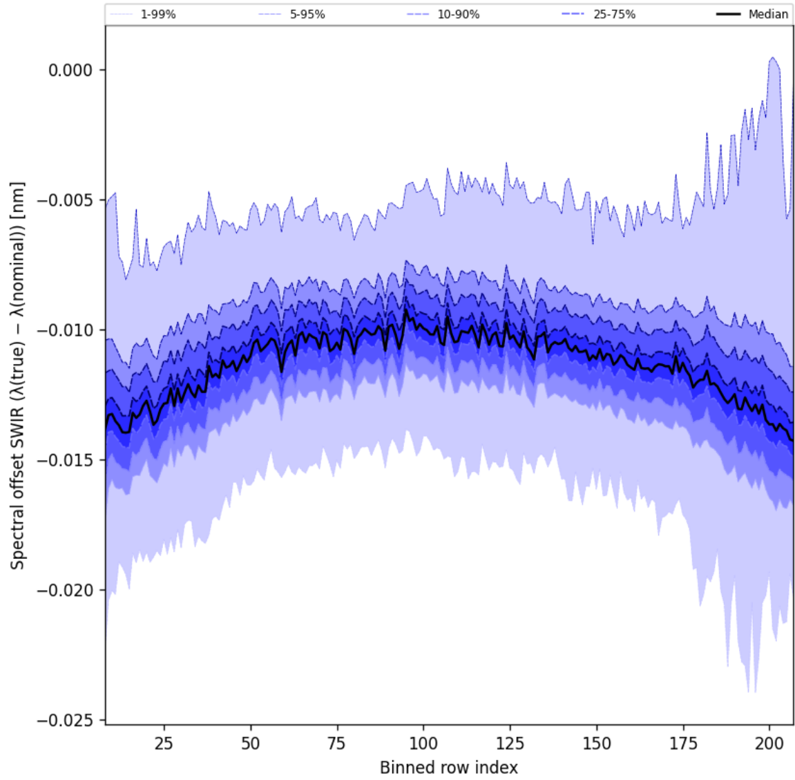
Figure 41: Along track statistics of “Spectral offset SWIR ( \lambda_{\text{true}} - \lambda_{\text{nominal}} )” for 2025-11-28 to 2025-11-30
