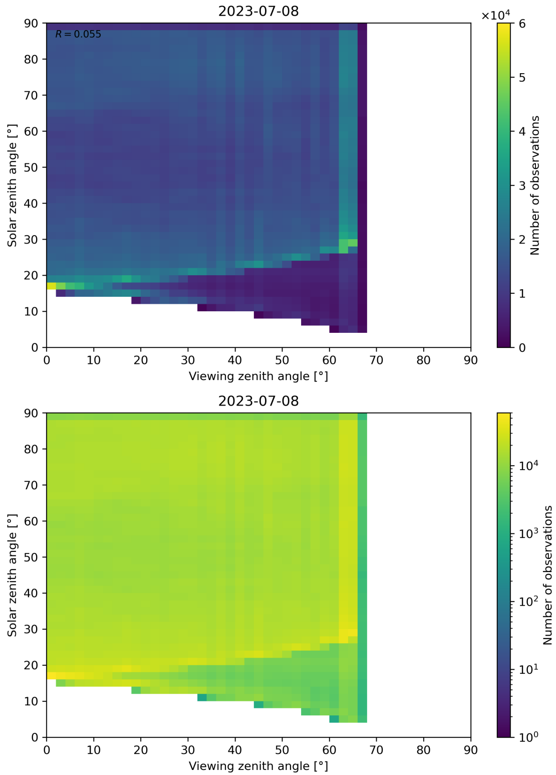
Figure 114: Scatter density plot of “Viewing zenith angle” against “Solar zenith angle” for 2023-07-08 to 2023-07-09.
