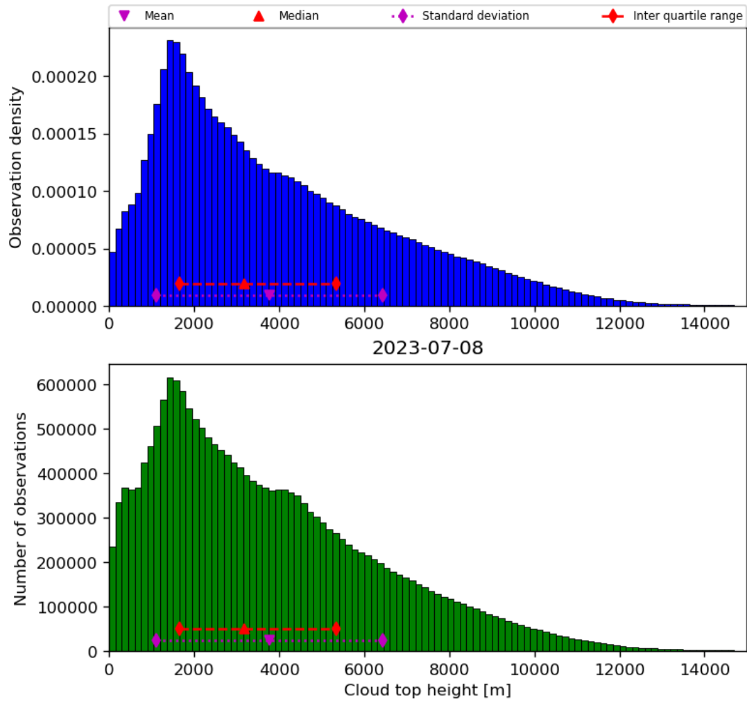
Figure 40: Histogram of “Cloud top height” for 2023-07-08 to 2023-07-09
