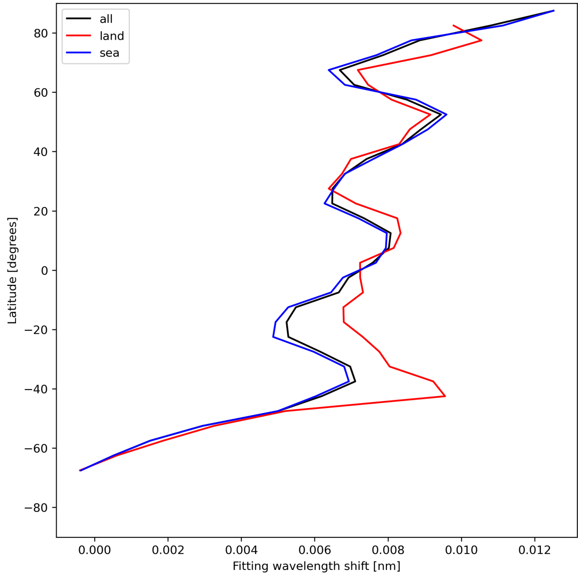
Figure 33: Zonal average of “Fitting wavelength shift” for 2023-07-08 to 2023-07-09.
