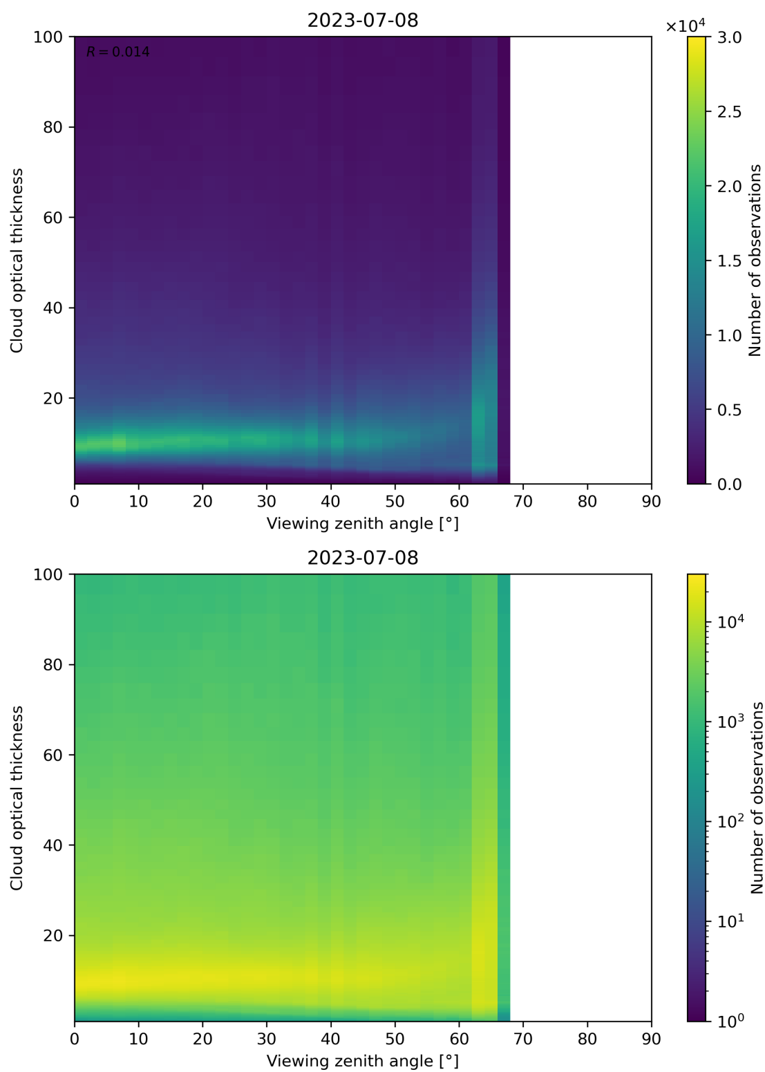
Figure 111: Scatter density plot of “Viewing zenith angle” against “Cloud optical thickness” for 2023-07-08 to 2023-07-09.
