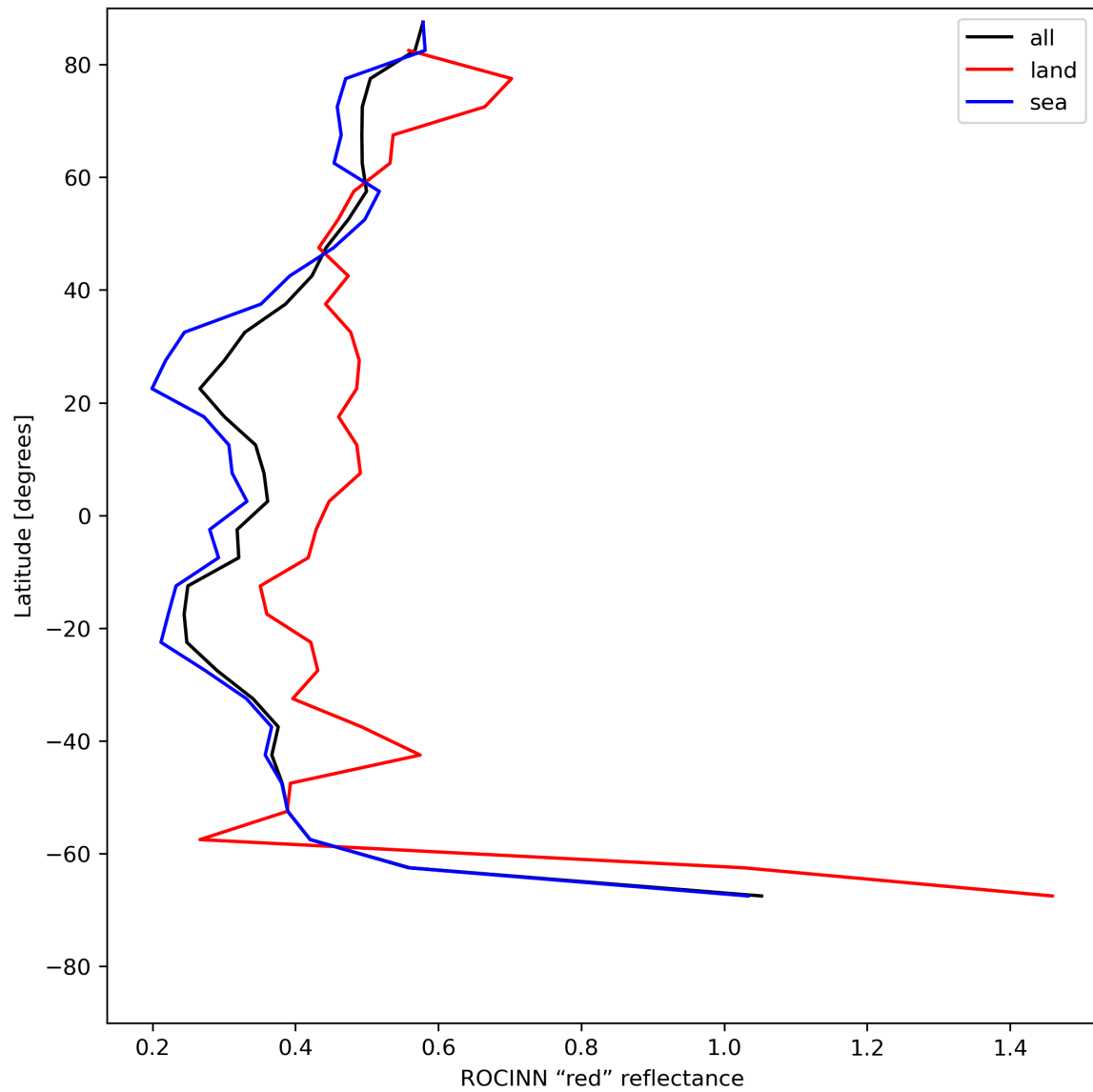
Figure 37: Zonal average of “ROCINN “red” reflectance” for 2023-07-08 to 2023-07-09.
