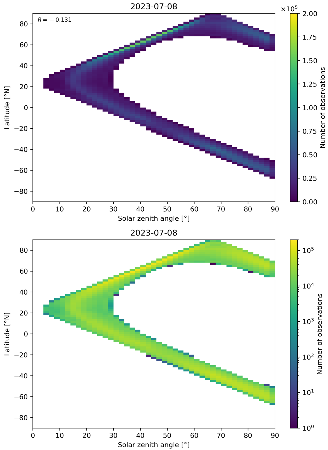
Figure 105: Scatter density plot of “Solar zenith angle” against “Latitude” for 2023-07-08 to 2023-07-09.
