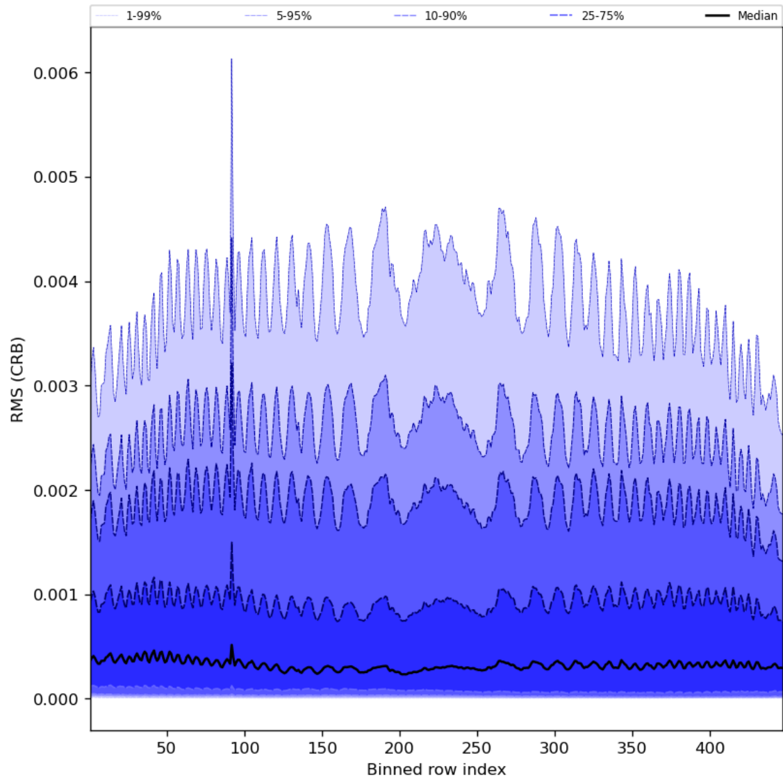
Figure 64: Along track statistics of “RMS (CRB)” for 2023-07-08 to 2023-07-09
