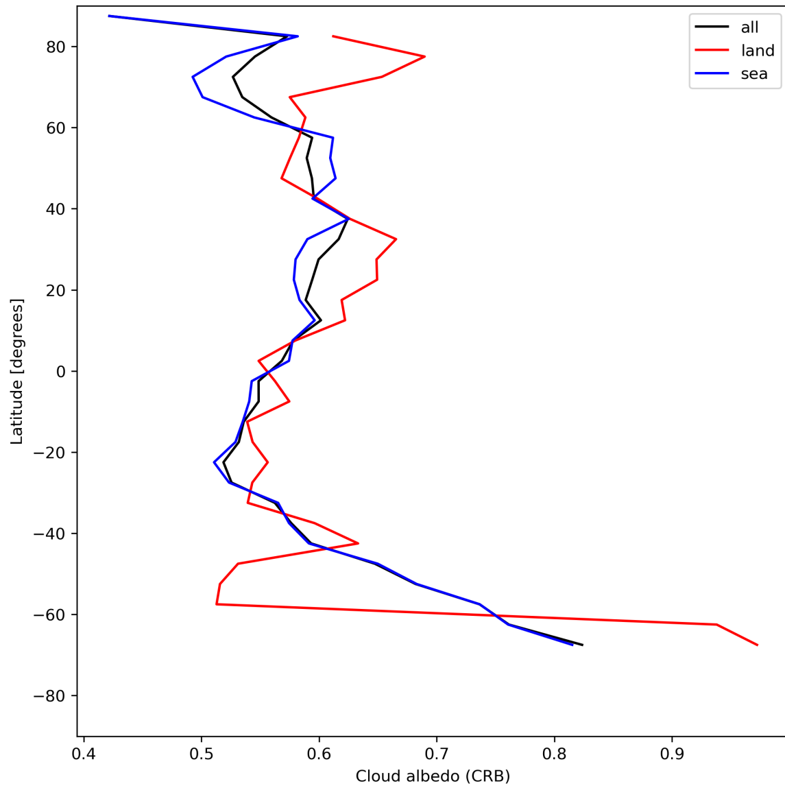
Figure 28: Zonal average of “Cloud albedo (CRB)” for 2023-07-08 to 2023-07-09.
