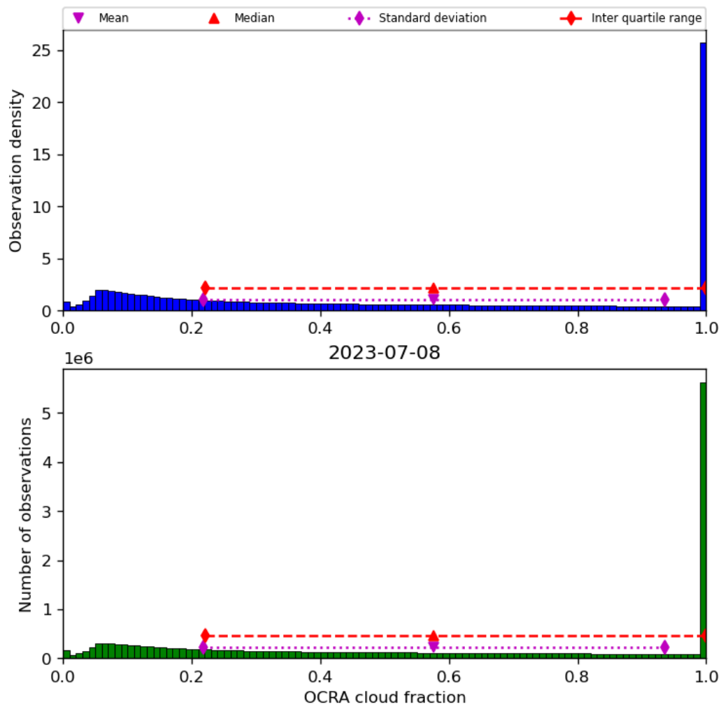
Figure 50: Histogram of “OCRA cloud fraction” for 2023-07-08 to 2023-07-09
