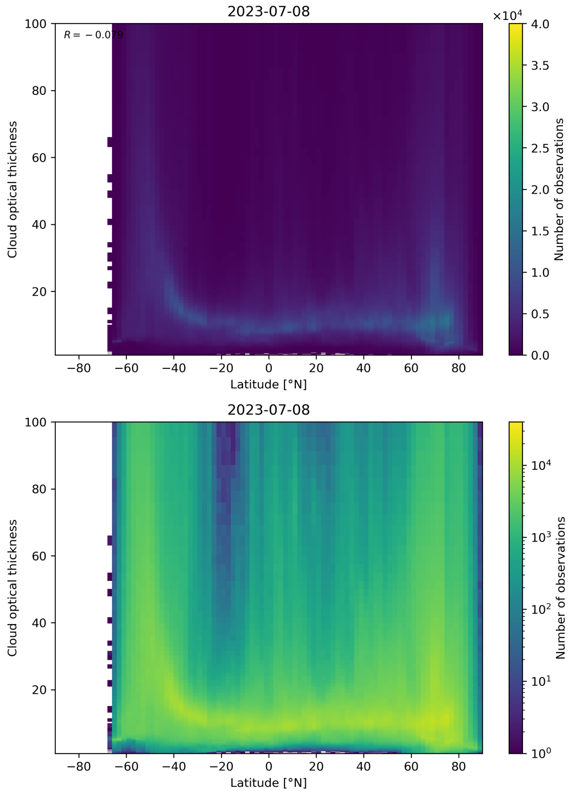
Figure 96: Scatter density plot of “Latitude” against “Cloud optical thickness” for 2023-07-08 to 2023-07-09.
