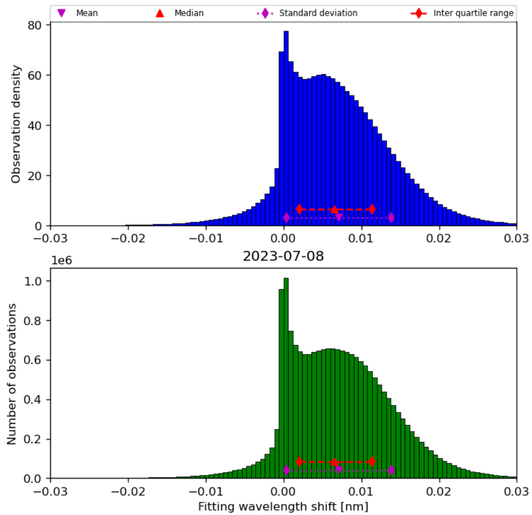
Figure 49: Histogram of “Fitting wavelength shift” for 2023-07-08 to 2023-07-09
