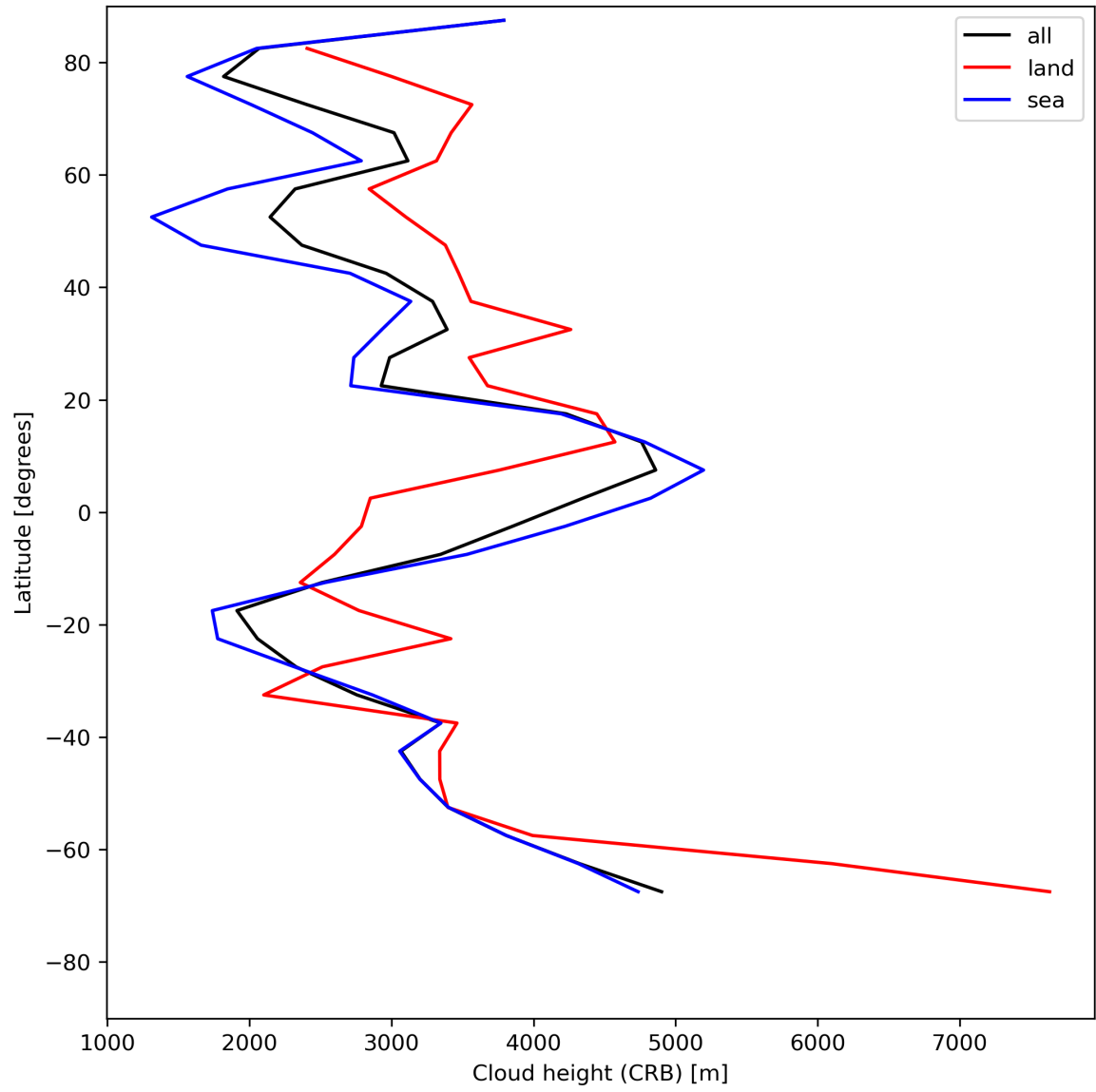
Figure 27: Zonal average of “Cloud height (CRB)” for 2023-07-08 to 2023-07-09.
