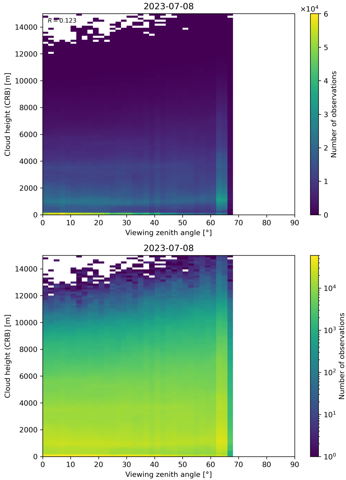
Figure 110: Scatter density plot of “Viewing zenith angle” against “Cloud height (CRB)” for 2023-07-08 to 2023-07-09.
