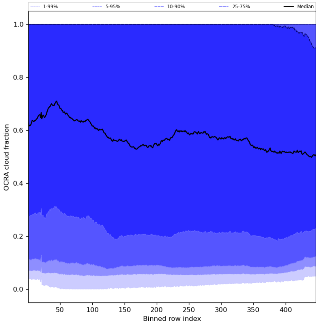
Figure 66: Along track statistics of “OCRA cloud fraction” for 2023-07-08 to 2023-07-09
