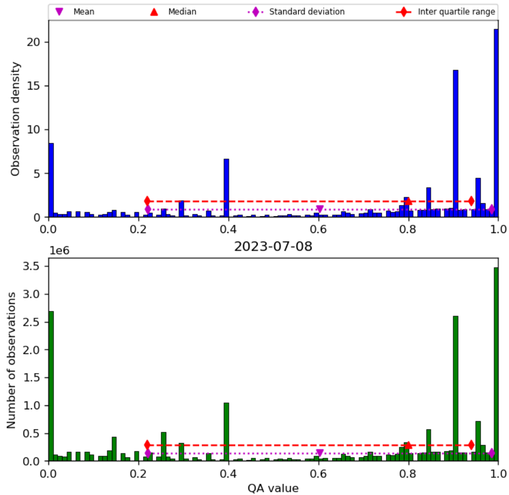
Figure 38: Histogram of “QA value” for 2023-07-08 to 2023-07-09
