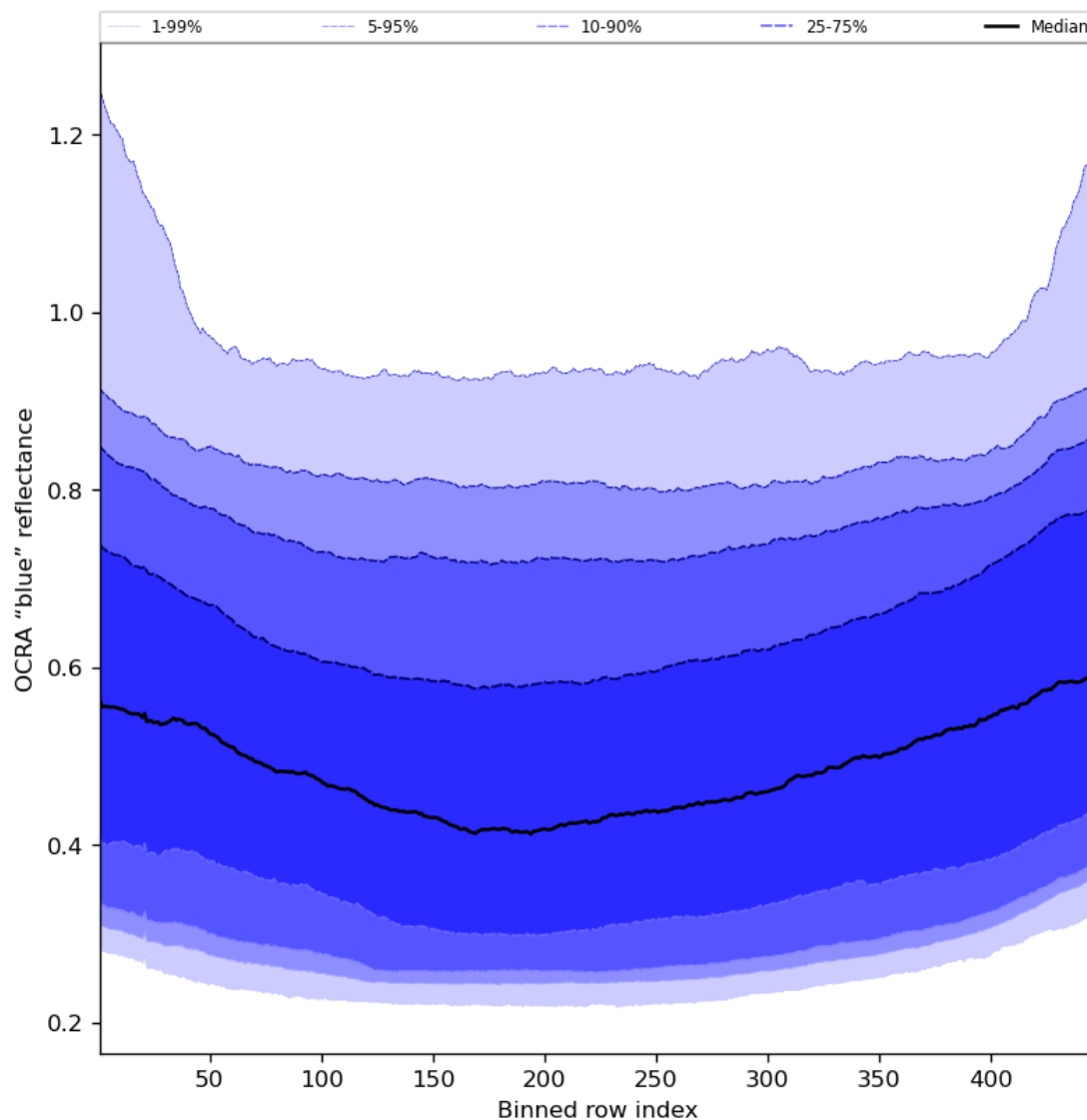
Figure 67: Along track statistics of “OCRA “blue” reflectance” for 2023-07-08 to 2023-07-09
