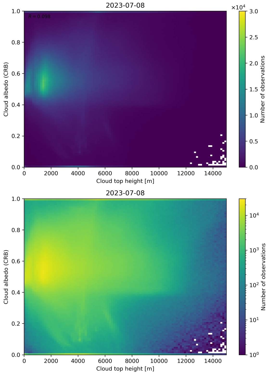
Figure 86: Scatter density plot of “Cloud top height” against “Cloud albedo (CRB)” for 2023-07-08 to 2023-07-09.
