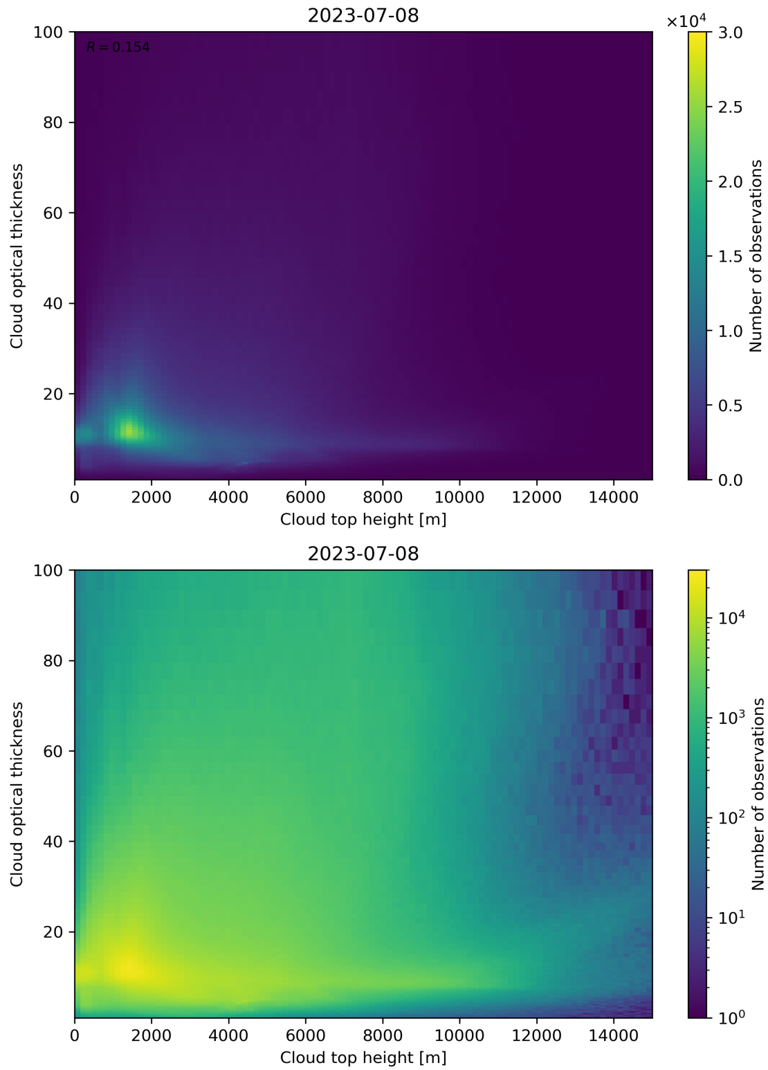
Figure 90: Scatter density plot of “Cloud top height” against “Cloud optical thickness” for 2023-07-08 to 2023-07-09.
