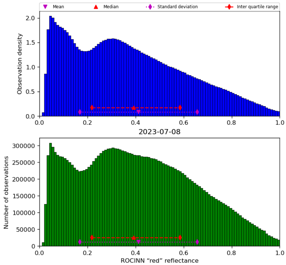
Figure 53: Histogram of “ROCINN “red” reflectance” for 2023-07-08 to 2023-07-09
