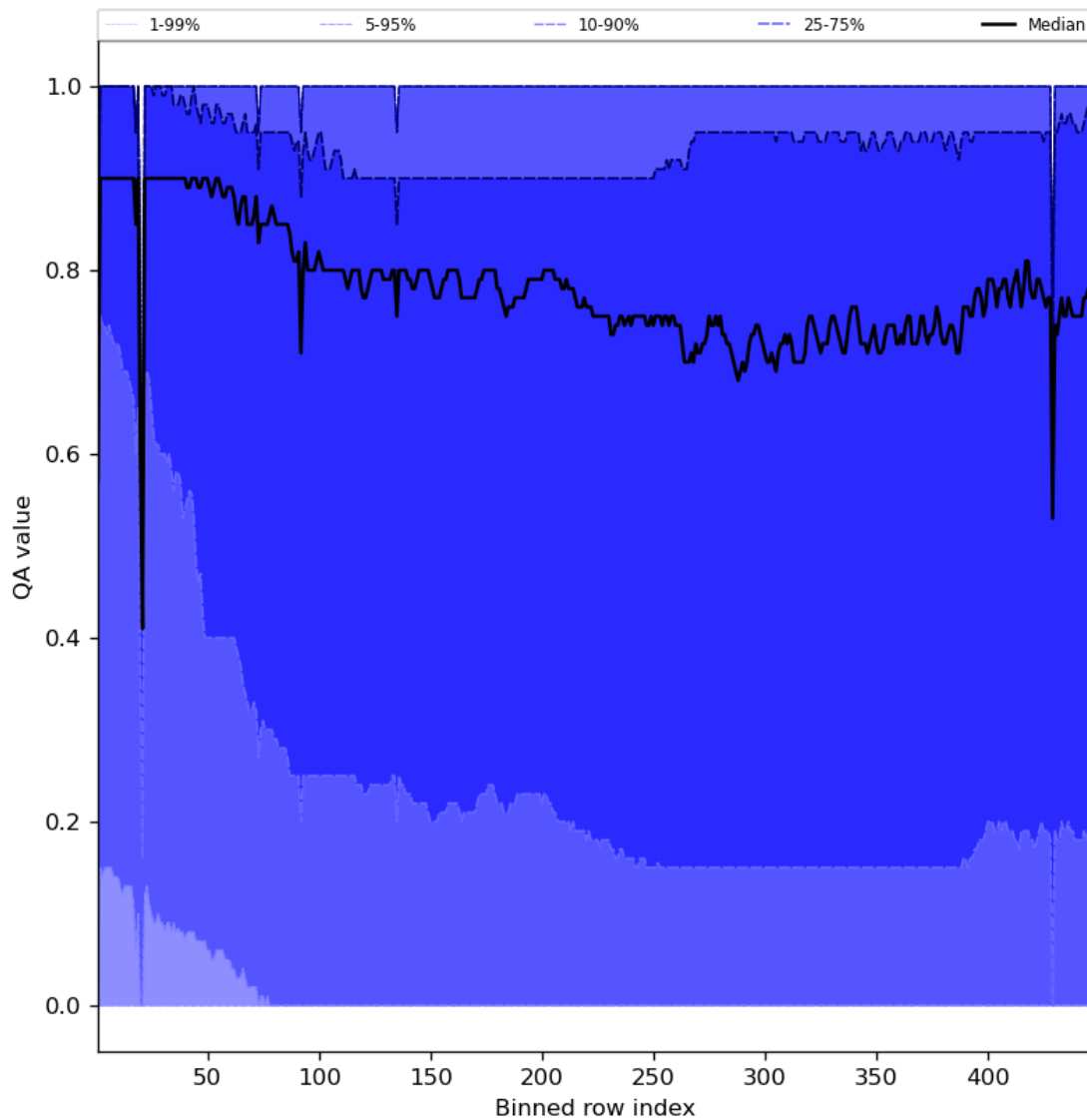
Figure 54: Along track statistics of “QA value” for 2023-07-08 to 2023-07-09
