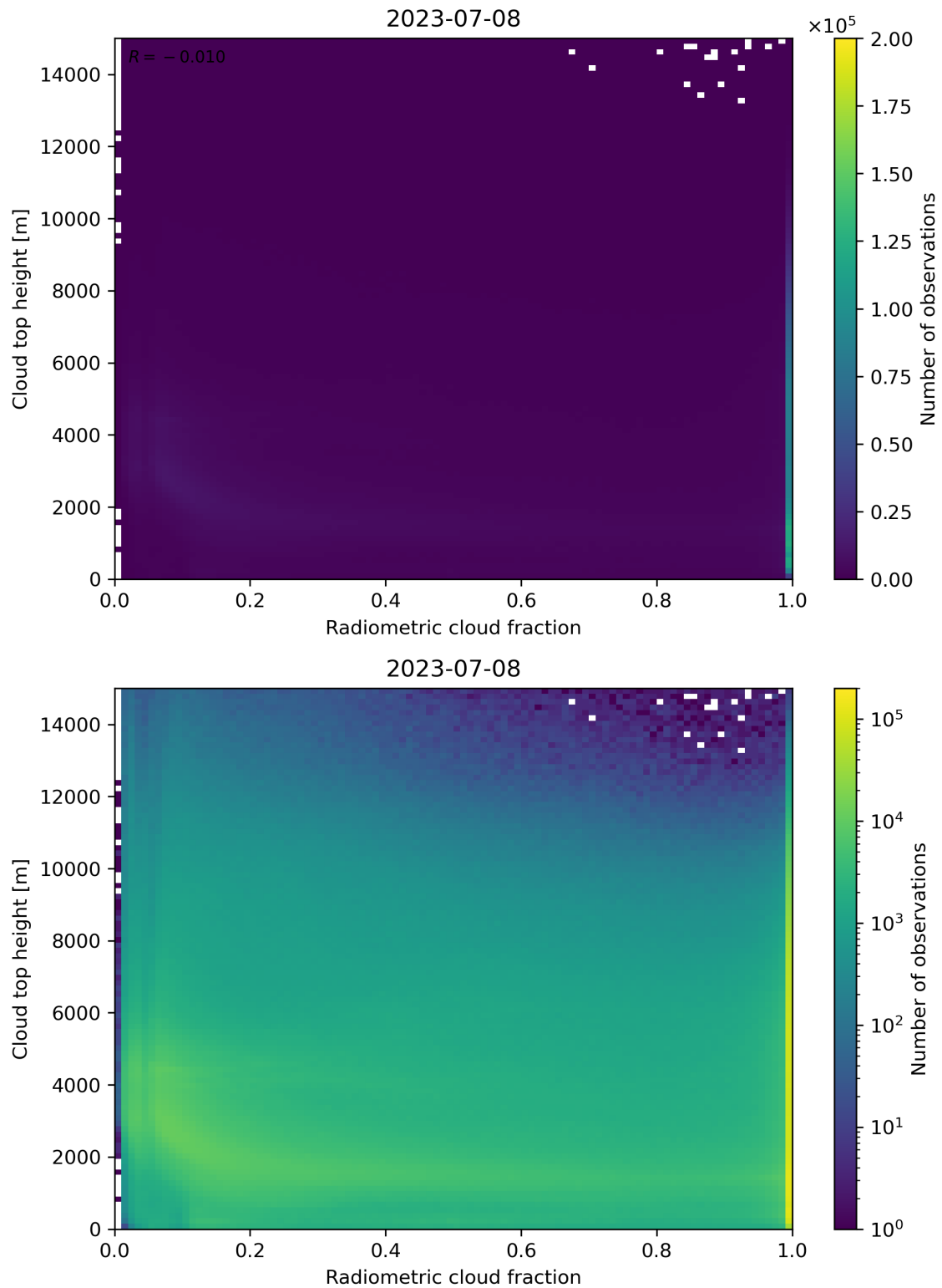
Figure 76: Scatter density plot of “Radiometric cloud fraction” against “Cloud top height” for 2023-07-08 to 2023-07-09.
