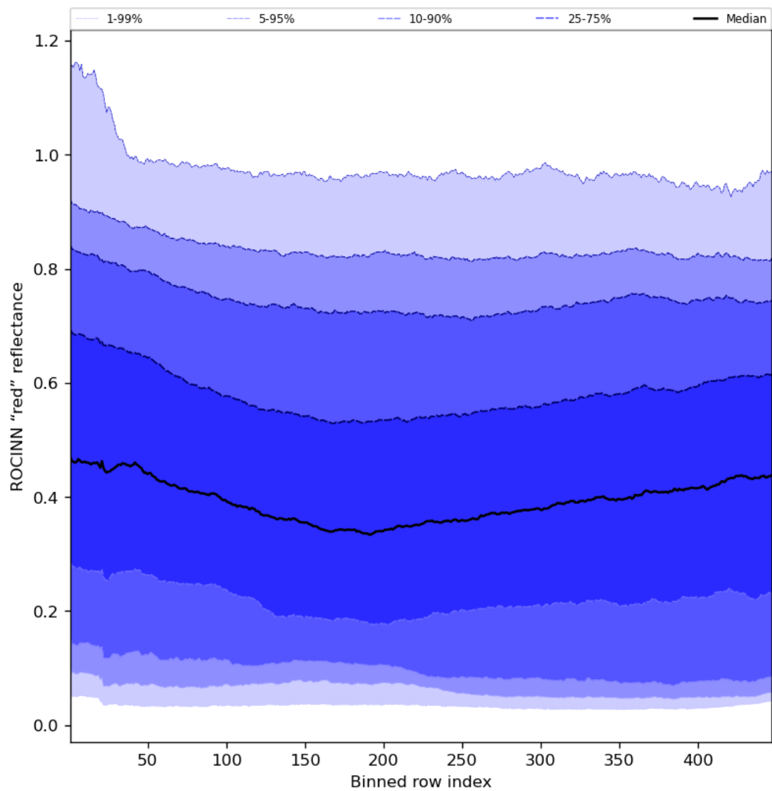
Figure 69: Along track statistics of "ROCINN "red" reflectance" for 2023-07-08 to 2023-07-09
