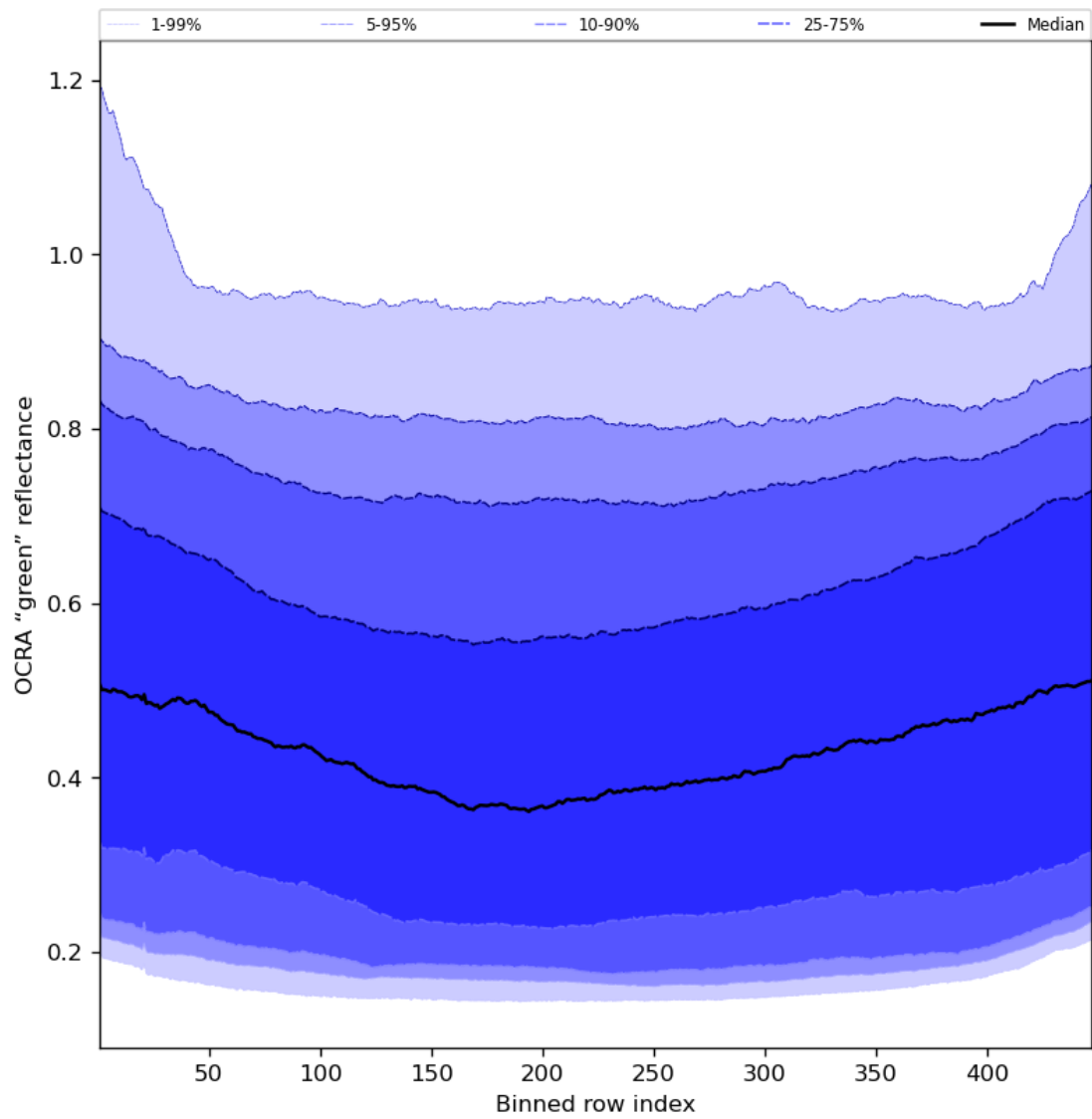
Figure 68: Along track statistics of “OCRA “green” reflectance” for 2023-07-08 to 2023-07-09
