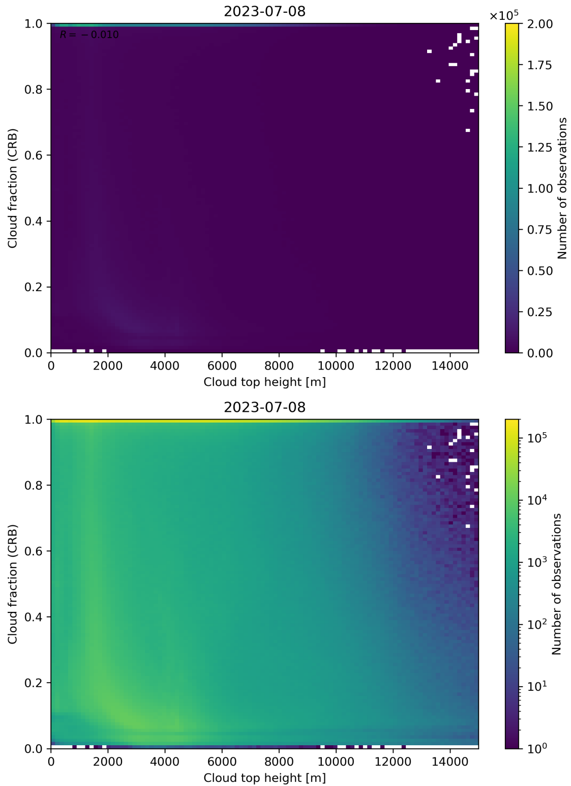
Figure 88: Scatter density plot of “Cloud top height” against “Cloud fraction (CRB)” for 2023-07-08 to 2023-07-09.
