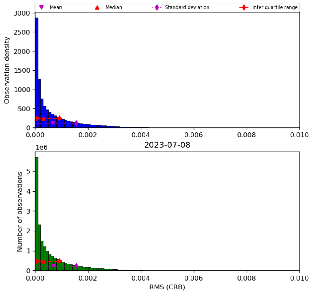
Figure 48: Histogram of “RMS (CRB)” for 2023-07-08 to 2023-07-09
