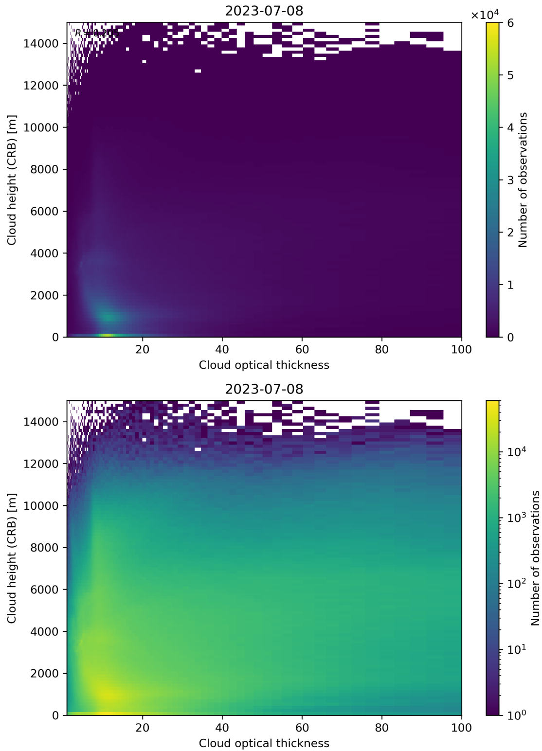
Figure 85: Scatter density plot of “Cloud optical thickness” against “Cloud height (CRB)” for 2023-07-08 to 2023-07-09.
