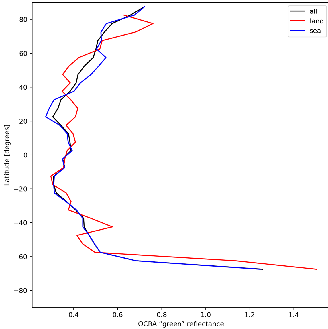
Figure 36: Zonal average of “OCRA “green” reflectance” for 2023-07-08 to 2023-07-09.
