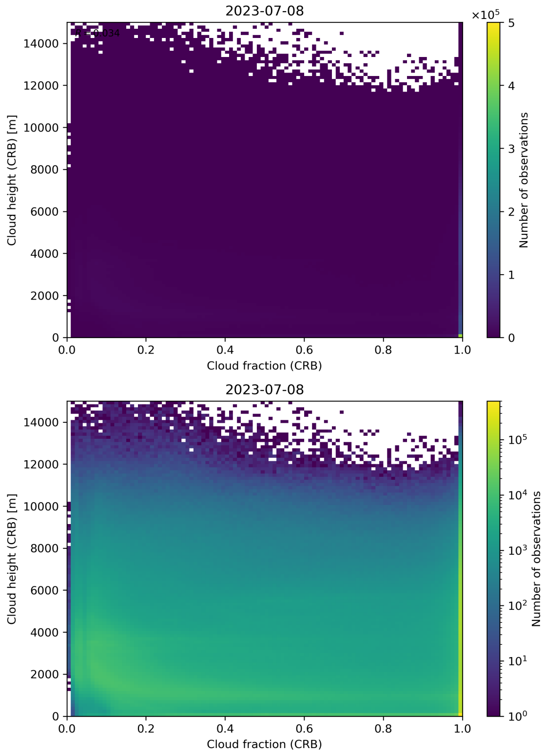
Figure 79: Scatter density plot of “Cloud fraction (CRB)” against “Cloud height (CRB)” for 2023-07-08 to 2023-07-09.
