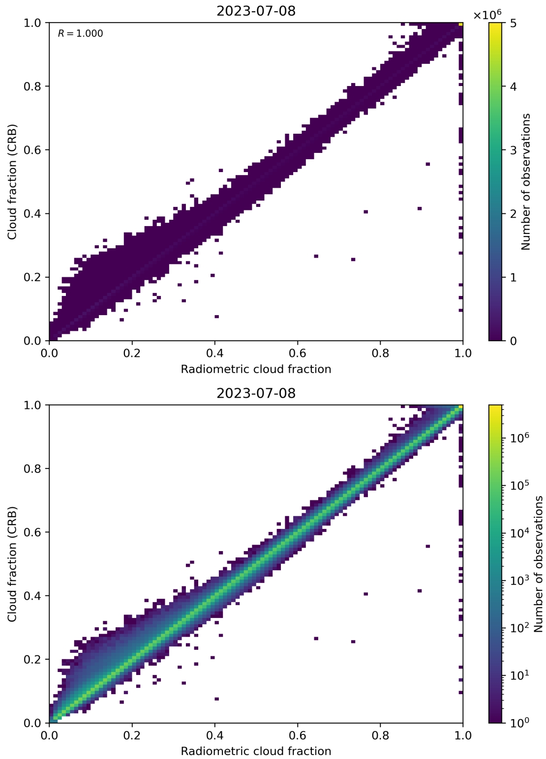
Figure 73: Scatter density plot of “Radiometric cloud fraction” against “Cloud fraction (CRB)” for 2023-07-08 to 2023-07-09.
