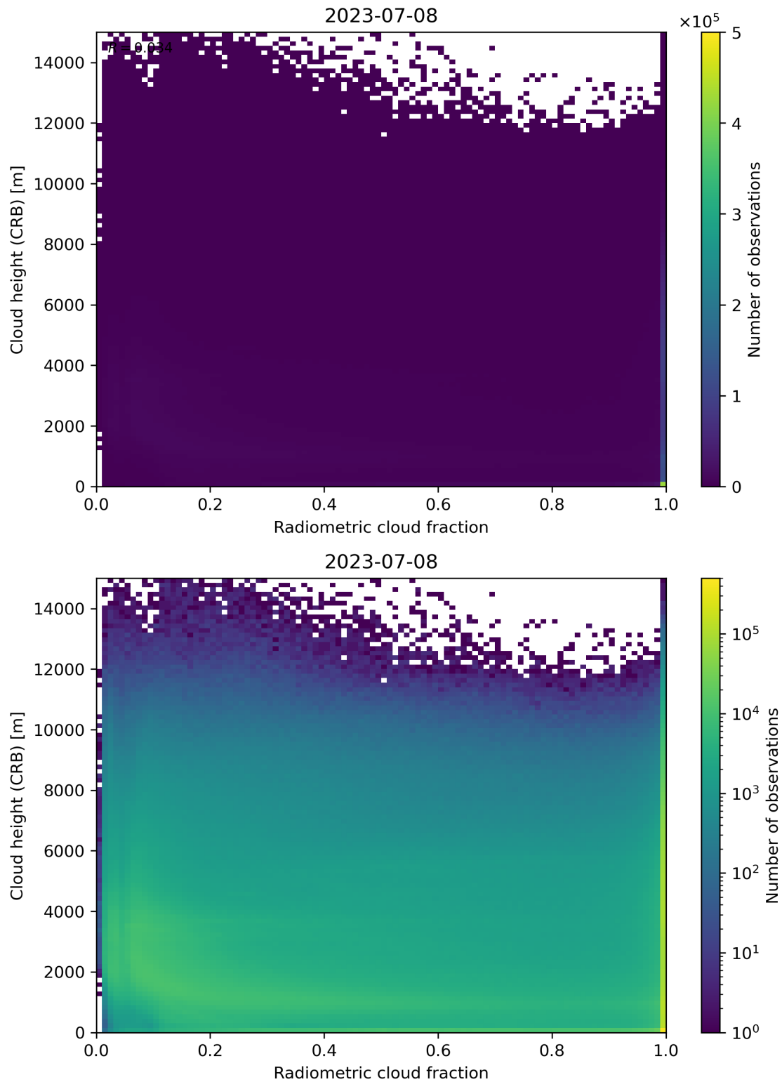
Figure 74: Scatter density plot of “Radiometric cloud fraction” against “Cloud height (CRB)” for 2023-07-08 to 2023-07-09.
