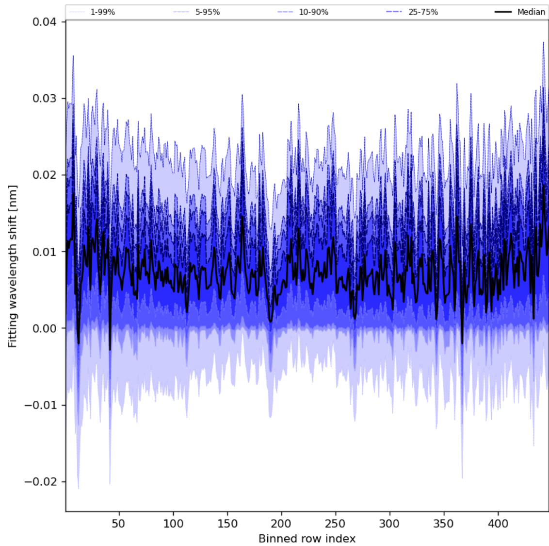
Figure 65: Along track statistics of “Fitting wavelength shift” for 2023-07-08 to 2023-07-09
