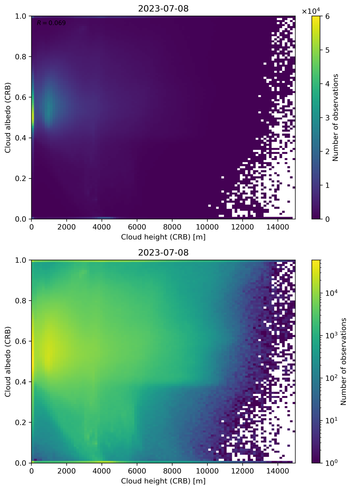
Figure 80: Scatter density plot of “Cloud height (CRB)” against “Cloud albedo (CRB)” for 2023-07-08 to 2023-07-09.
