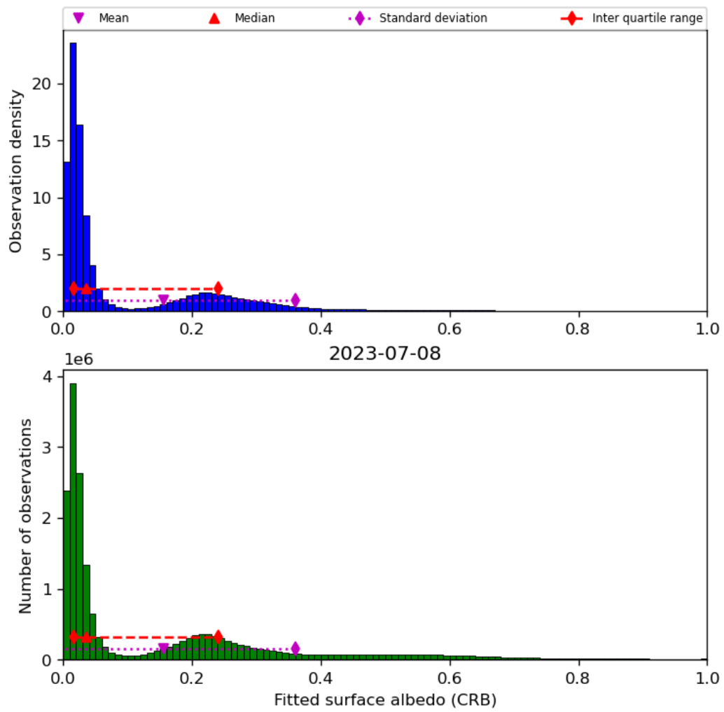
Figure 46: Histogram of “Fitted surface albedo (CRB)” for 2023-07-08 to 2023-07-09
