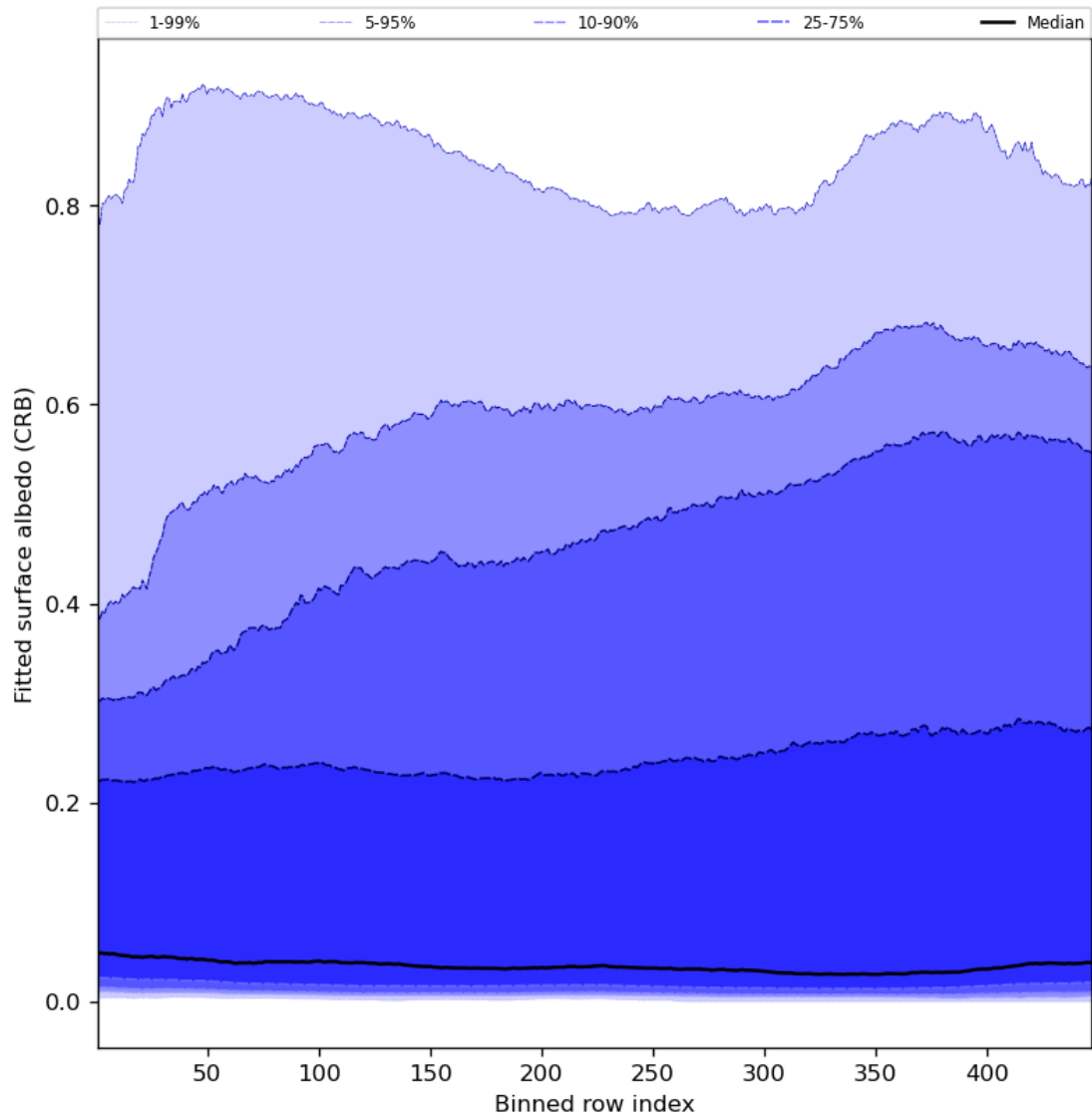
Figure 62: Along track statistics of “Fitted surface albedo (CRB)” for 2023-07-08 to 2023-07-09
