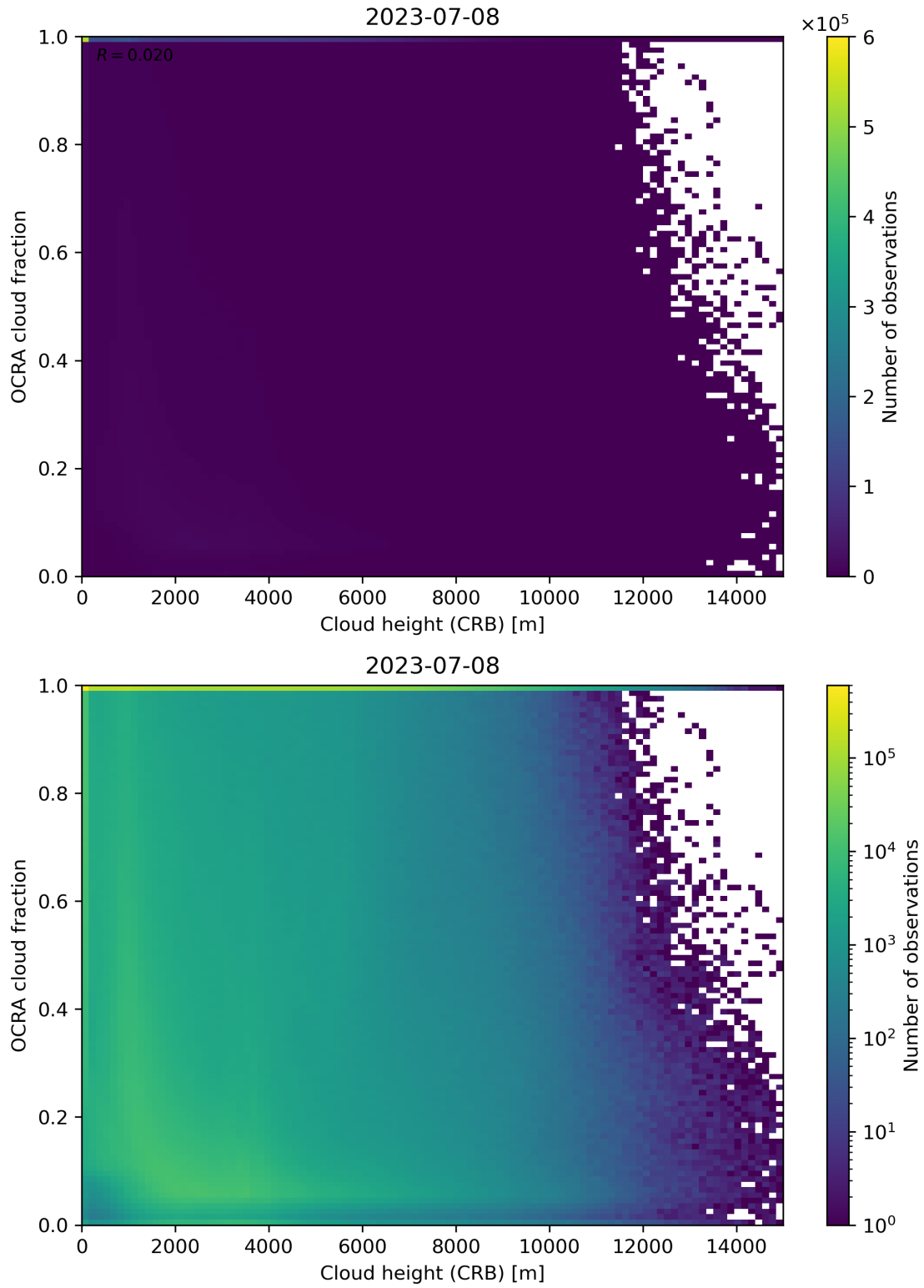
Figure 81: Scatter density plot of “Cloud height (CRB)” against “OCRA cloud fraction” for 2023-07-08 to 2023-07-09.
