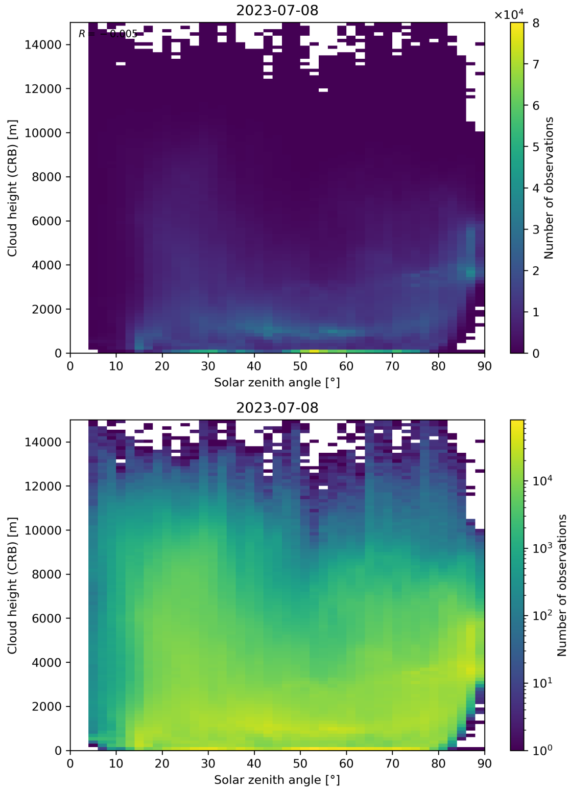
Figure 102: Scatter density plot of “Solar zenith angle” against “Cloud height (CRB)” for 2023-07-08 to 2023-07-09.
