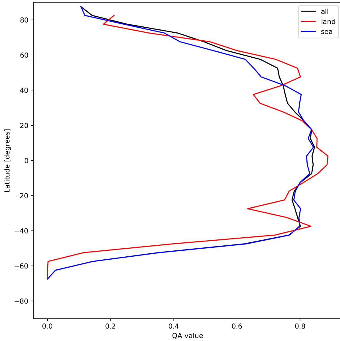
Figure 22: Zonal average of “QA value” for 2023-07-08 to 2023-07-09.
