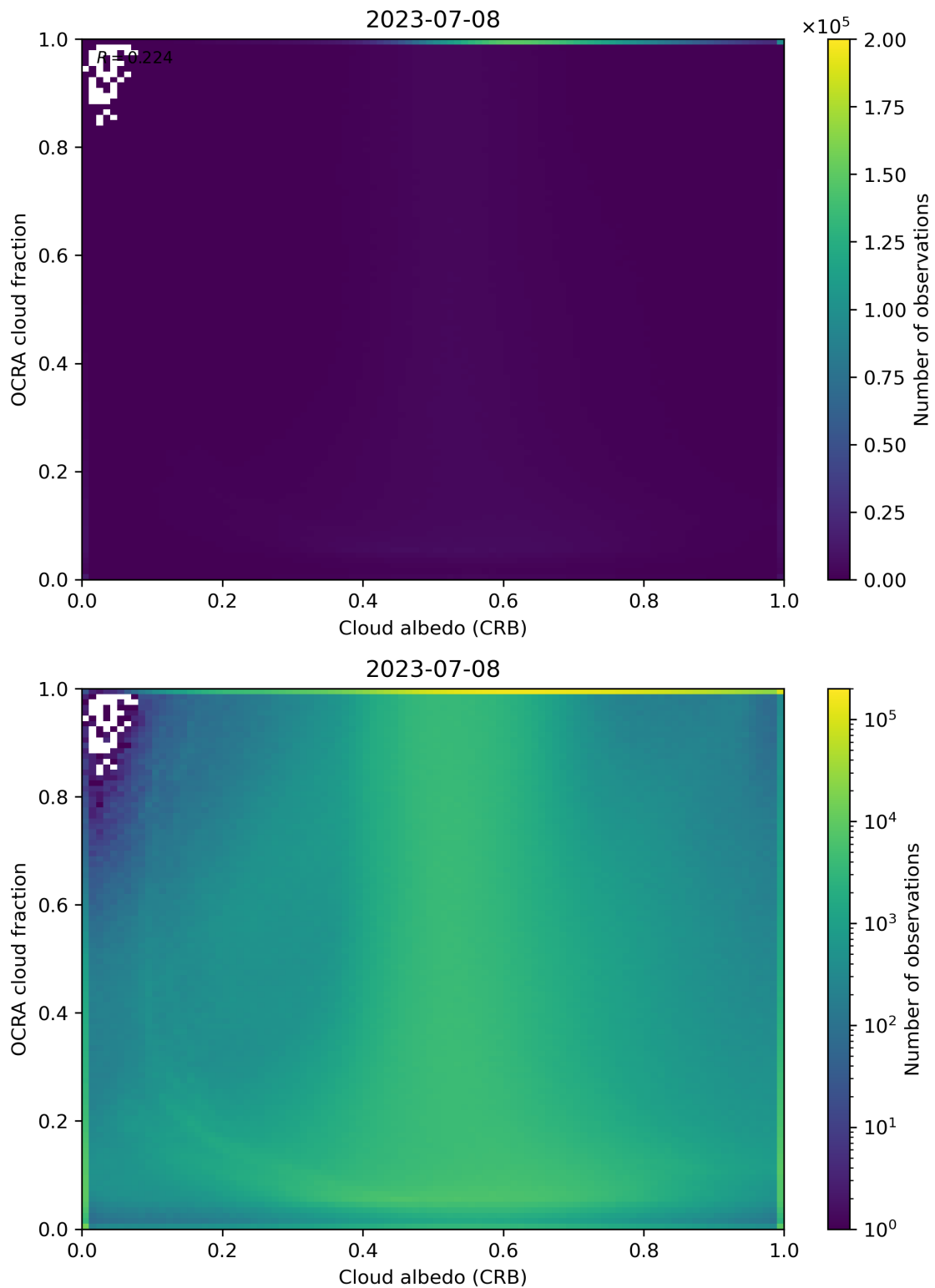
Figure 70: Scatter density plot of “Cloud albedo (CRB)” against “OCRA cloud fraction” for 2023-07-08 to 2023-07-09.
