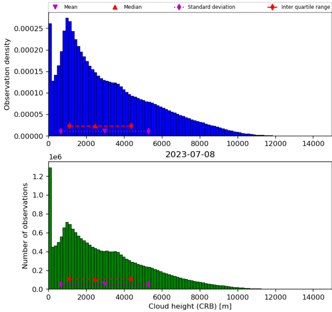
Figure 43: Histogram of “Cloud height (CRB)” for 2023-07-08 to 2023-07-09
