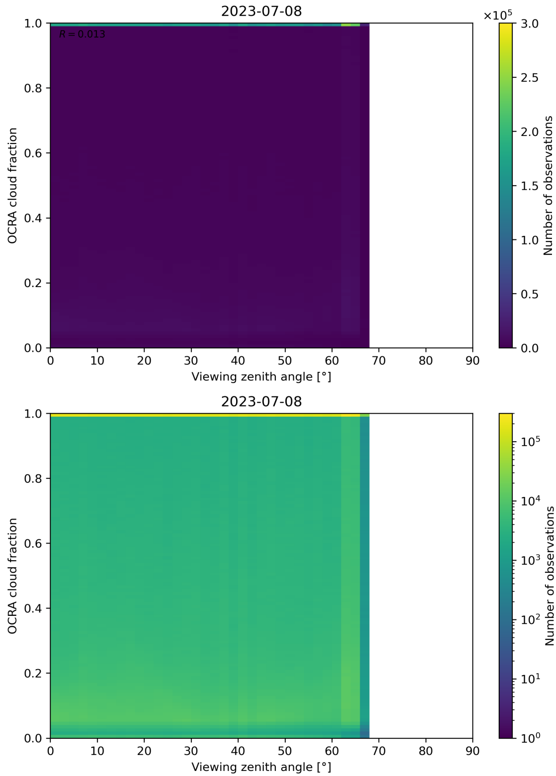
Figure 108: Scatter density plot of “Viewing zenith angle” against “OCRA cloud fraction” for 2023-07-08 to 2023-07-09.
