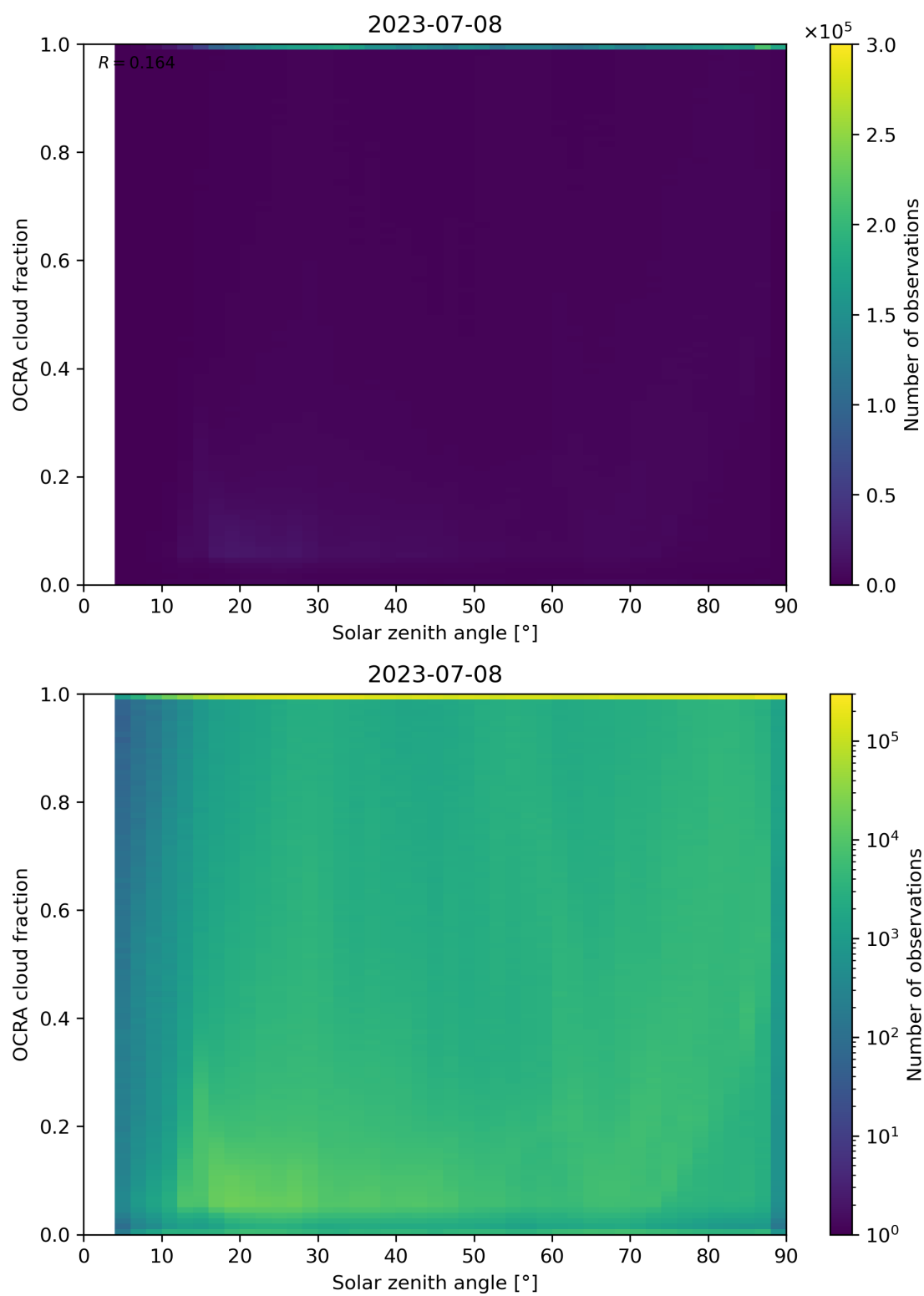
Figure 100: Scatter density plot of “Solar zenith angle” against “OCRA cloud fraction” for 2023-07-08 to 2023-07-09.
