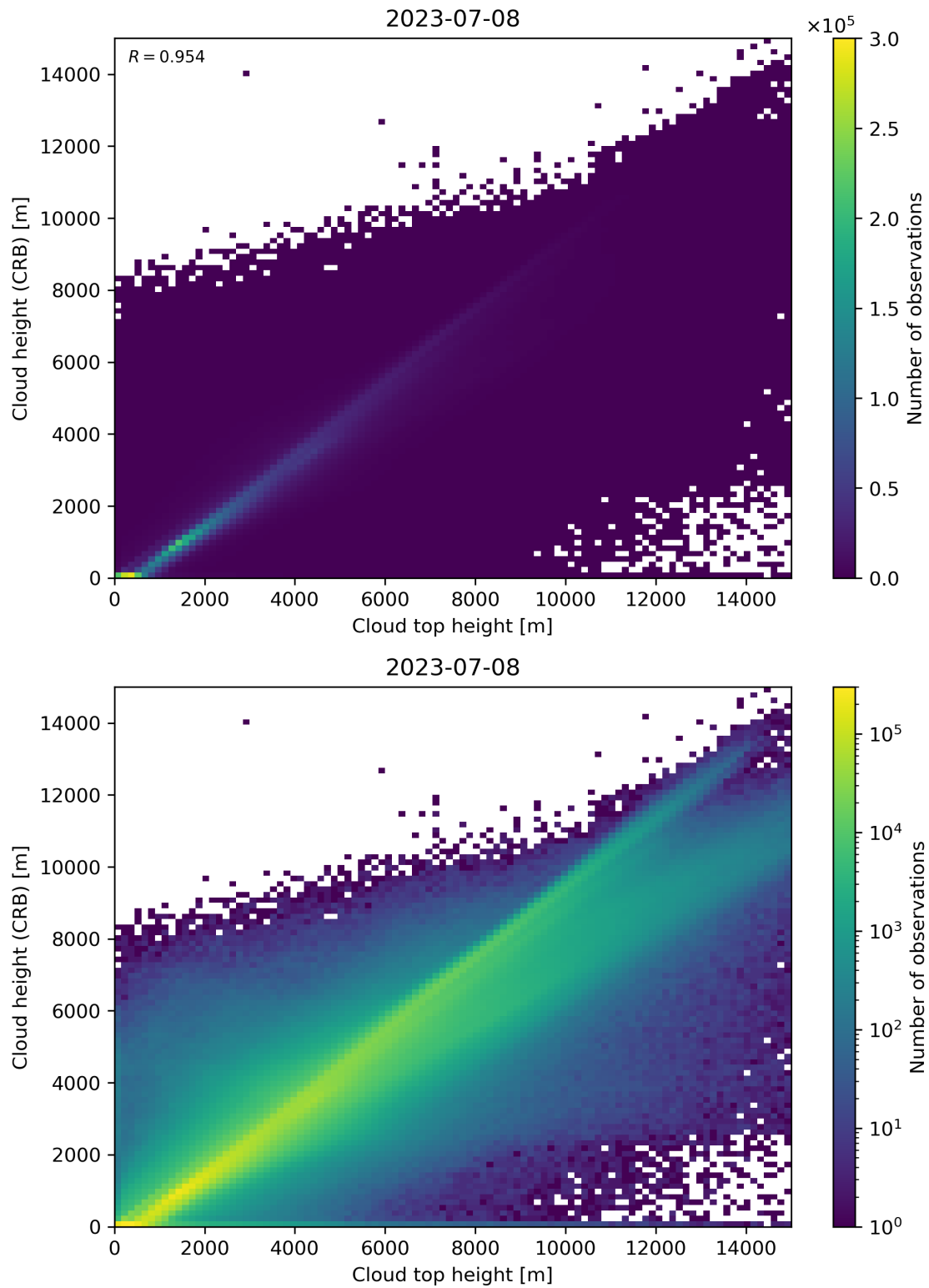
Figure 89: Scatter density plot of “Cloud top height” against “Cloud height (CRB)” for 2023-07-08 to 2023-07-09.
