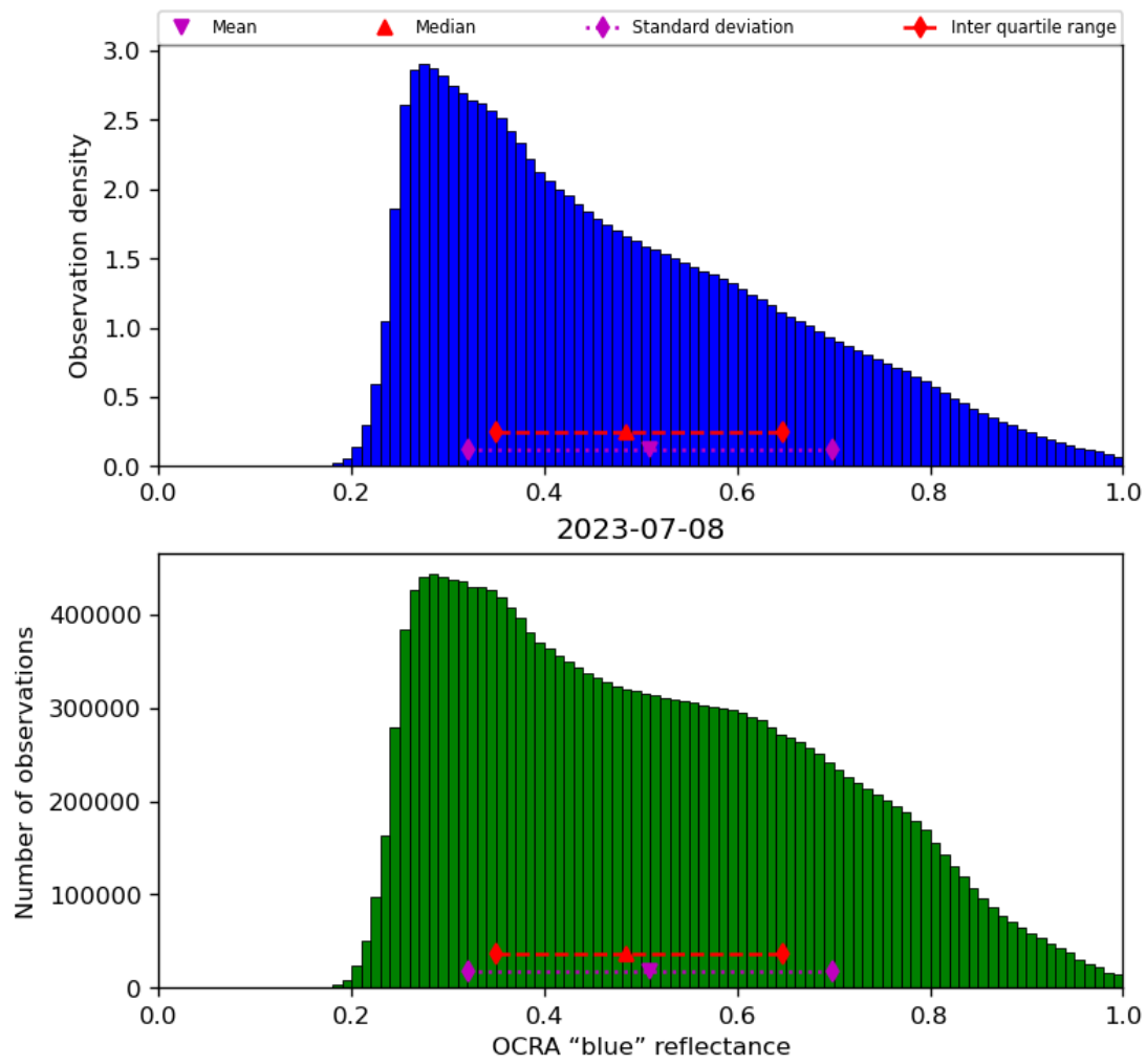
Figure 51: Histogram of “OCRA “blue” reflectance” for 2023-07-08 to 2023-07-09
