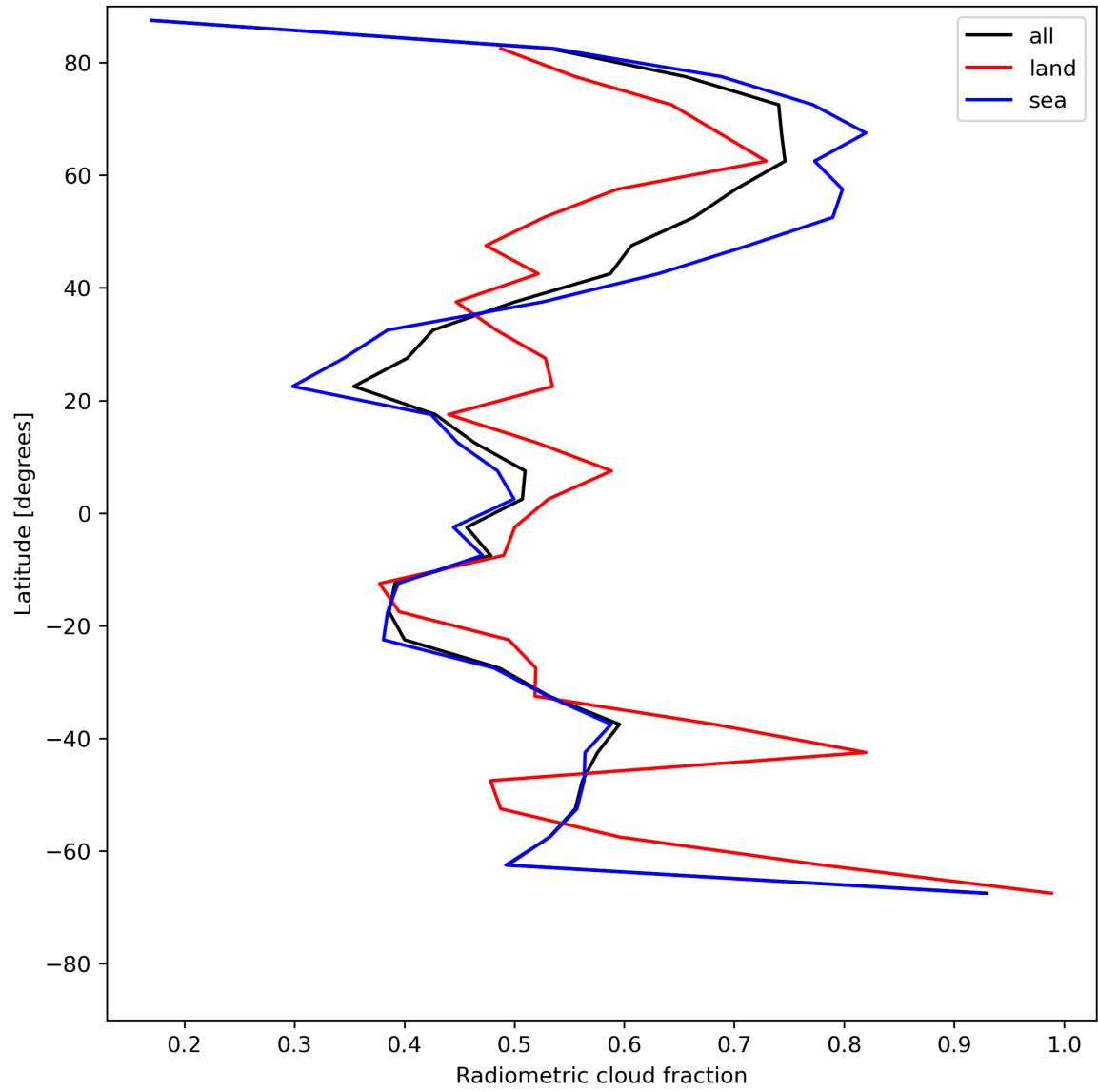
Figure 23: Zonal average of “Radiometric cloud fraction” for 2023-07-08 to 2023-07-09.
