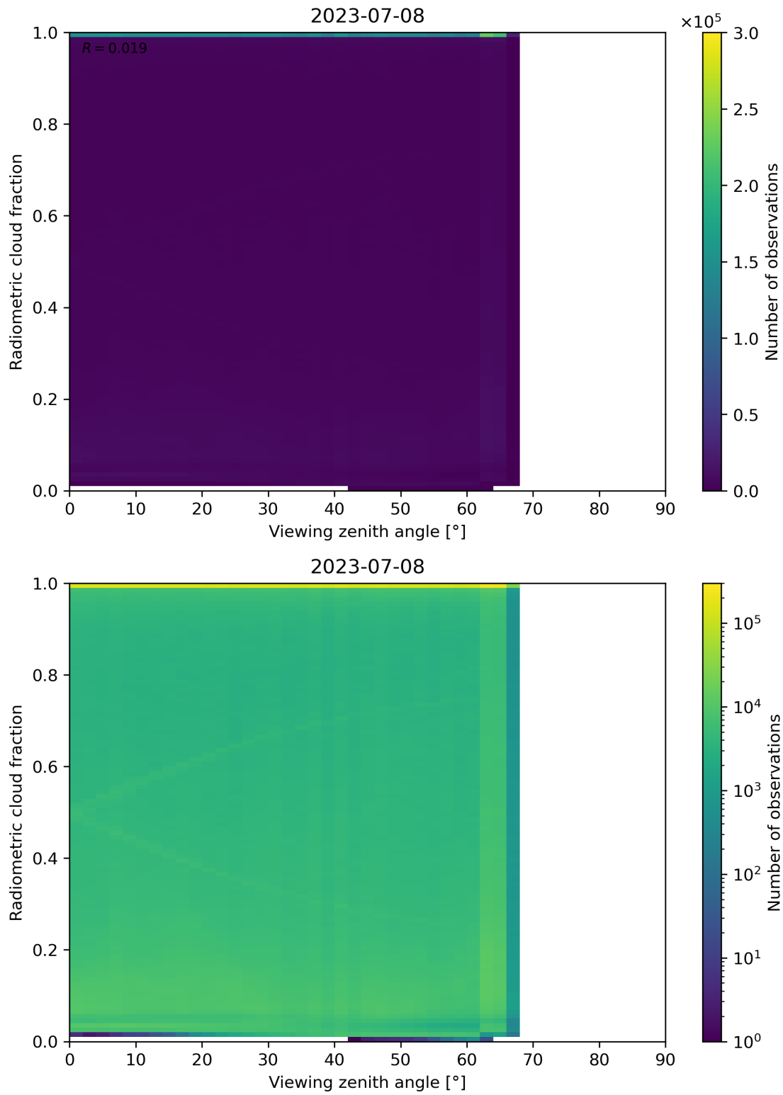
Figure 107: Scatter density plot of “Viewing zenith angle” against “Radiometric cloud fraction” for 2023-07-08 to 2023-07-09.
