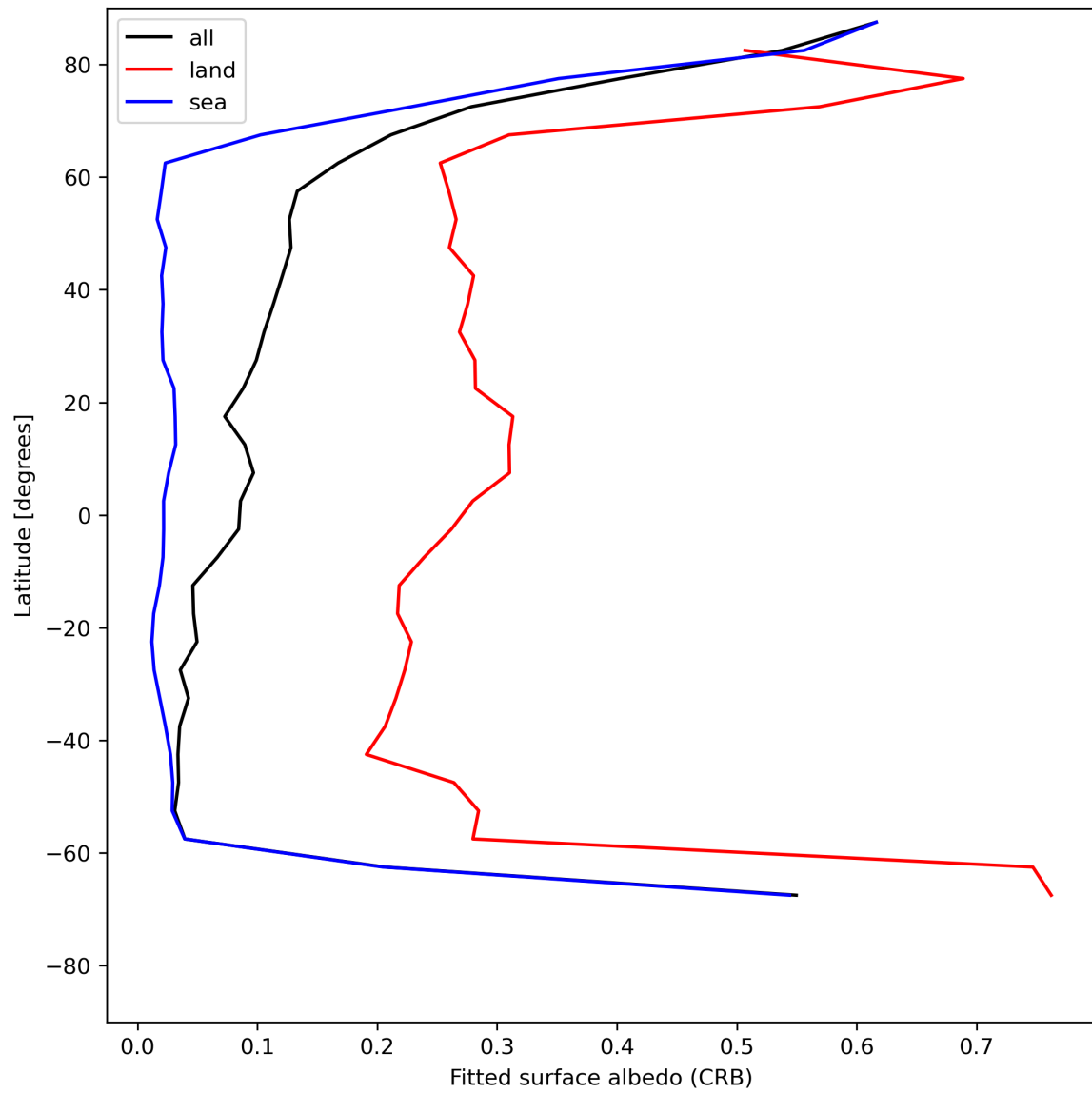
Figure 30: Zonal average of “Fitted surface albedo (CRB)” for 2023-07-08 to 2023-07-09.
