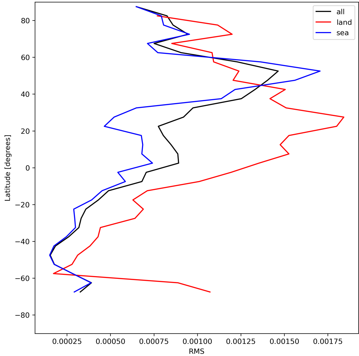
Figure 31: Zonal average of “RMS” for 2023-07-08 to 2023-07-09.
