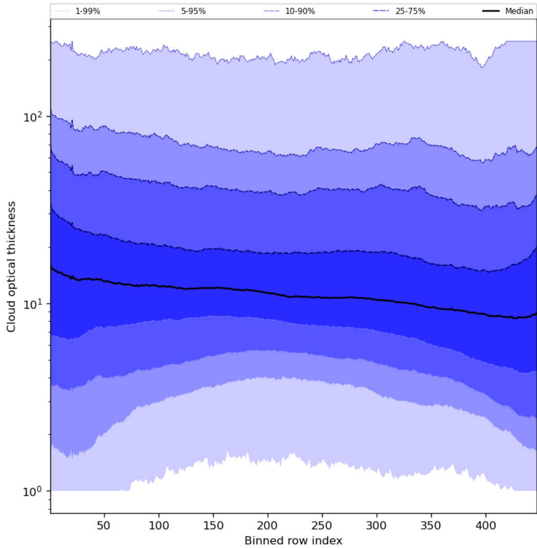
Figure 57: Along track statistics of “Cloud optical thickness” for 2023-07-08 to 2023-07-09
