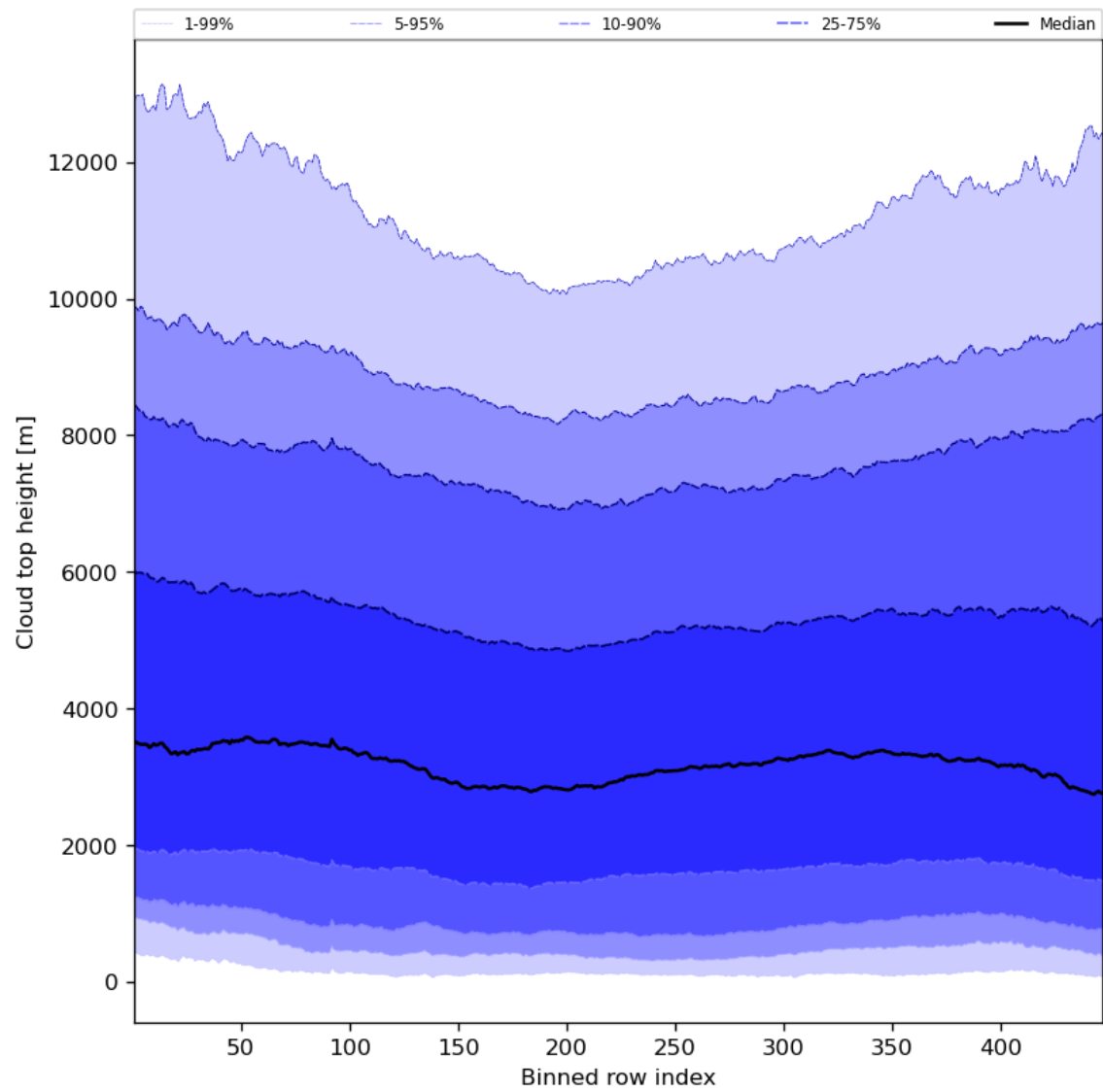
Figure 56: Along track statistics of “Cloud top height” for 2023-07-08 to 2023-07-09
