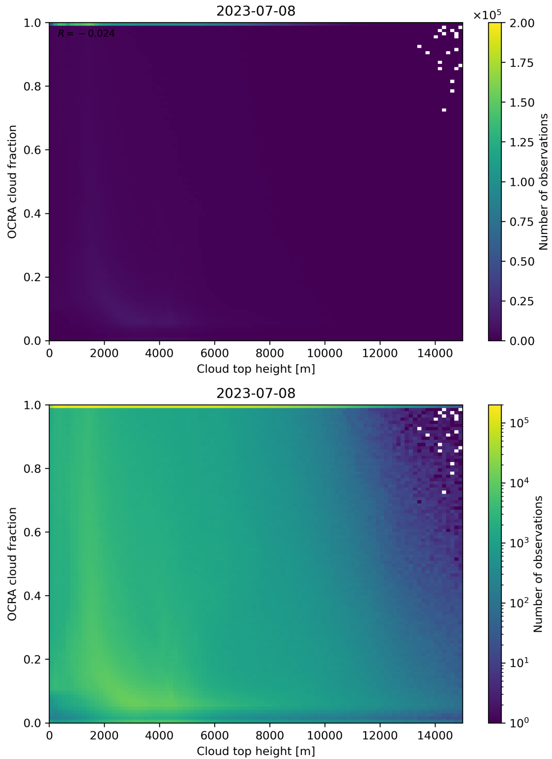
Figure 87: Scatter density plot of “Cloud top height” against “OCRA cloud fraction” for 2023-07-08 to 2023-07-09.
