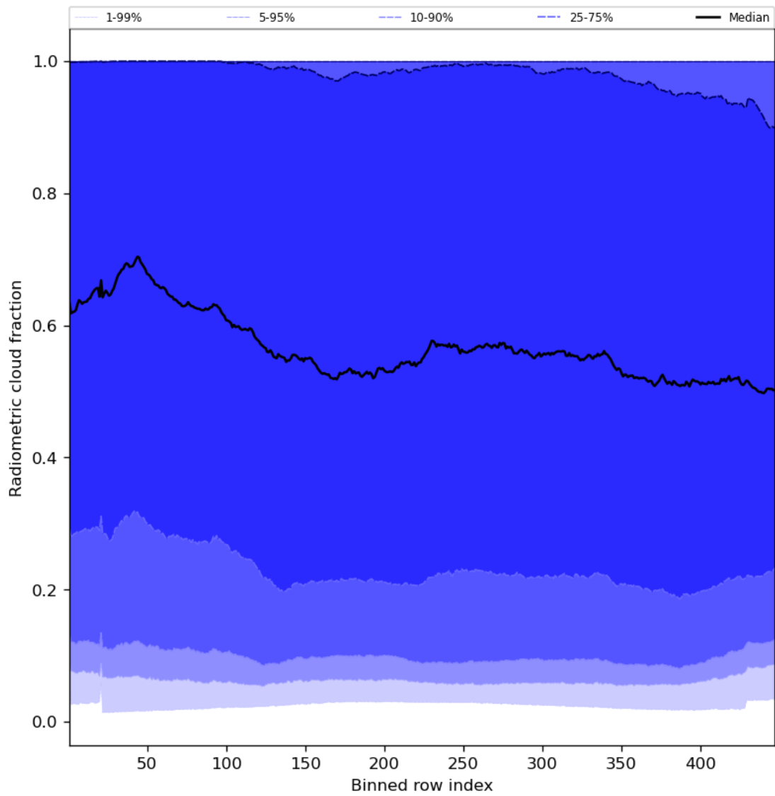
Figure 55: Along track statistics of “Radiometric cloud fraction” for 2023-07-08 to 2023-07-09
