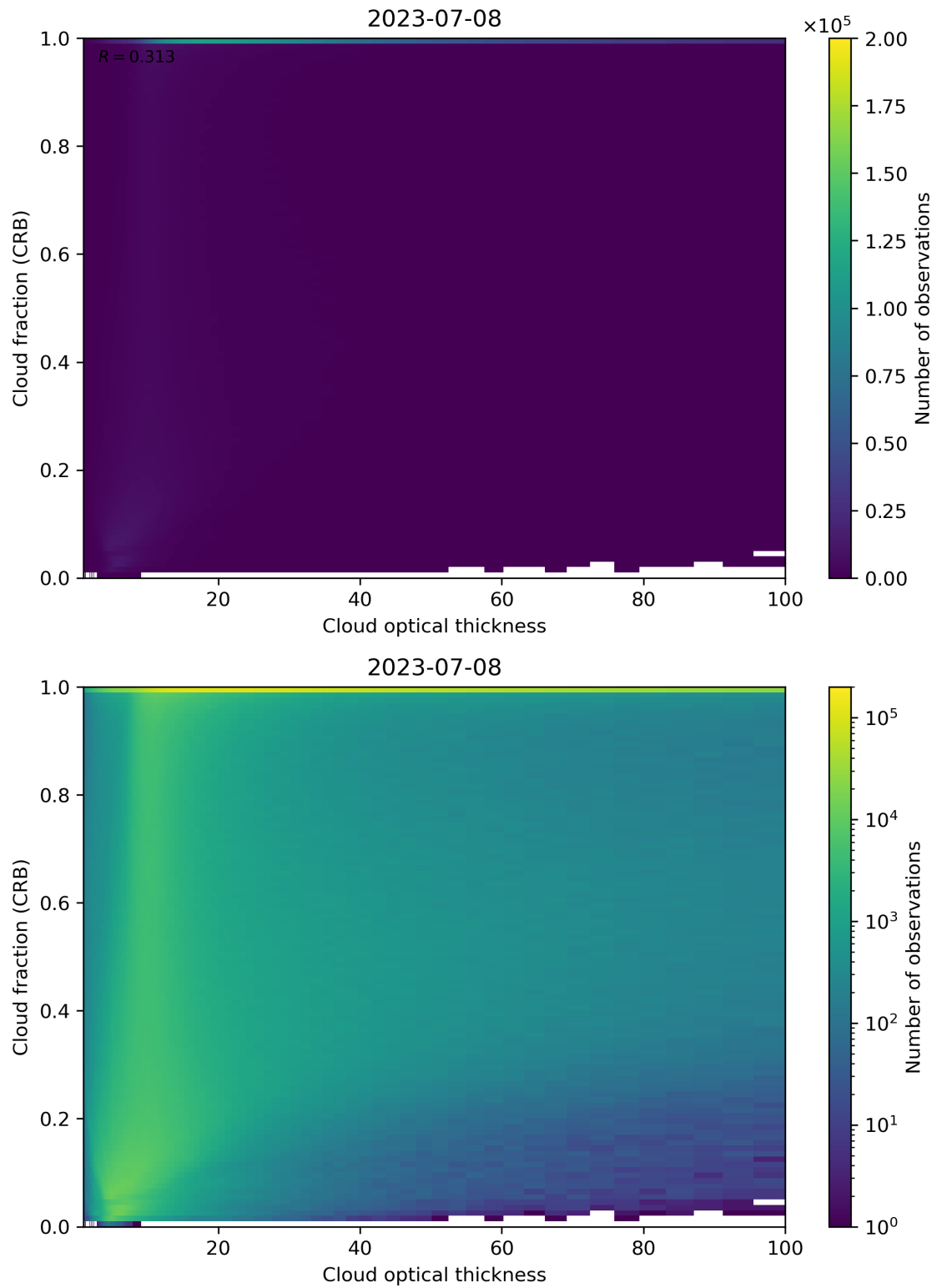
Figure 84: Scatter density plot of “Cloud optical thickness” against “Cloud fraction (CRB)” for 2023-07-08 to 2023-07-09.
