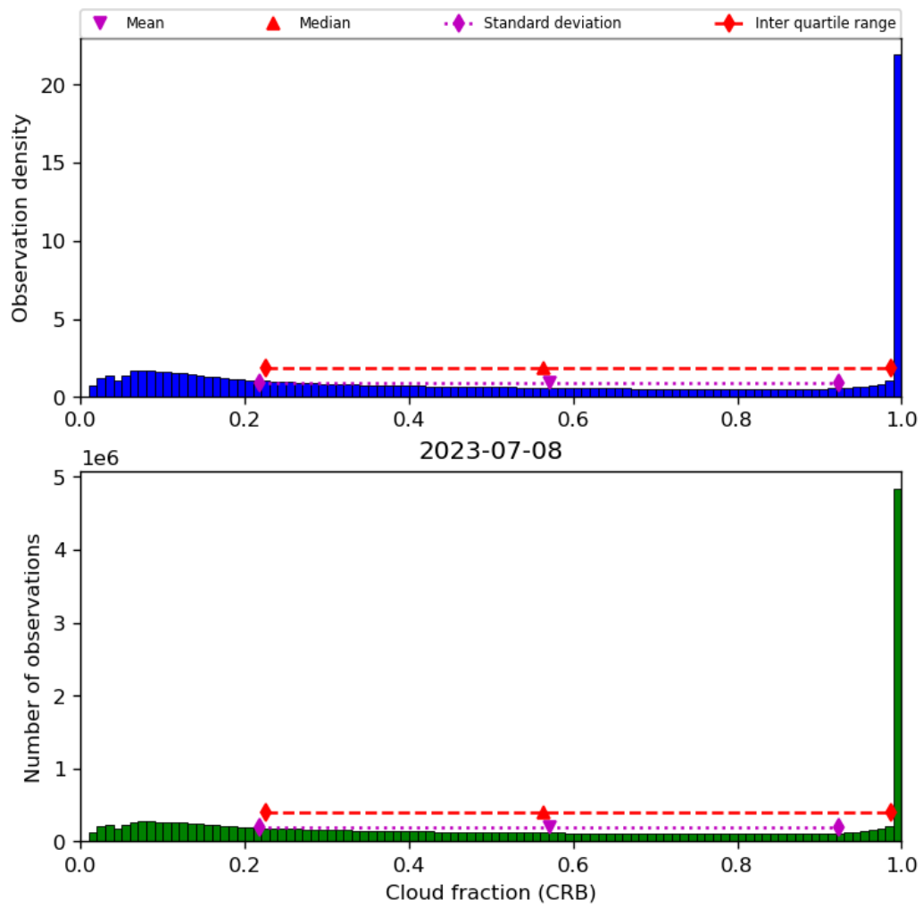
Figure 42: Histogram of “Cloud fraction (CRB)” for 2023-07-08 to 2023-07-09
