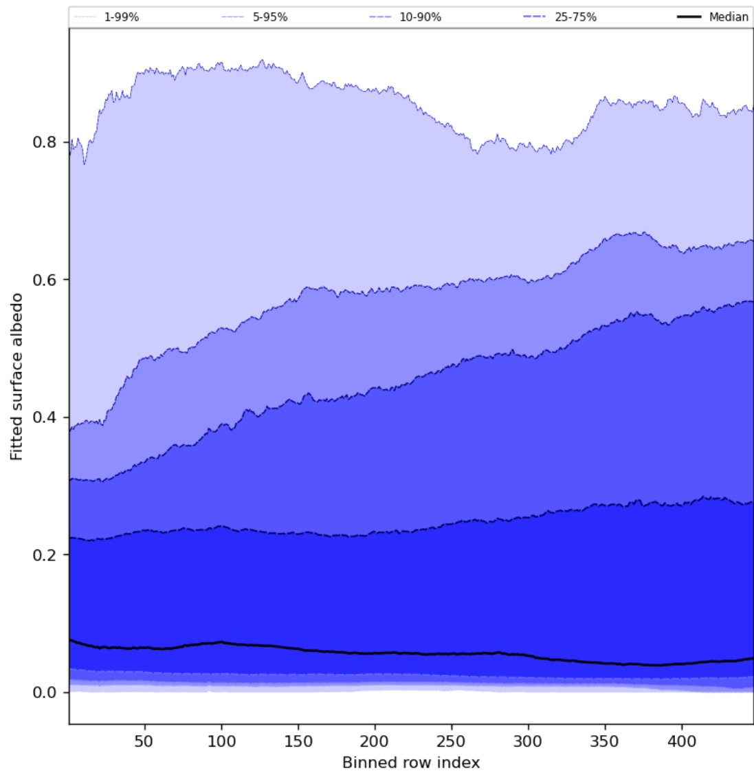
Figure 61: Along track statistics of “Fitted surface albedo” for 2023-07-08 to 2023-07-09
