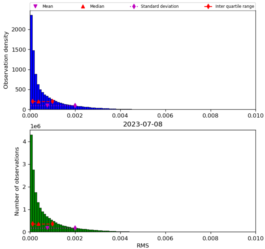
Figure 47: Histogram of “RMS” for 2023-07-08 to 2023-07-09
