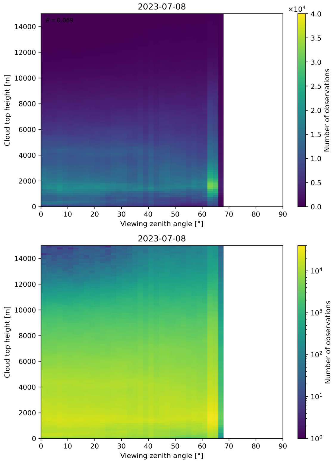
Figure 112: Scatter density plot of “Viewing zenith angle” against “Cloud top height” for 2023-07-08 to 2023-07-09.
