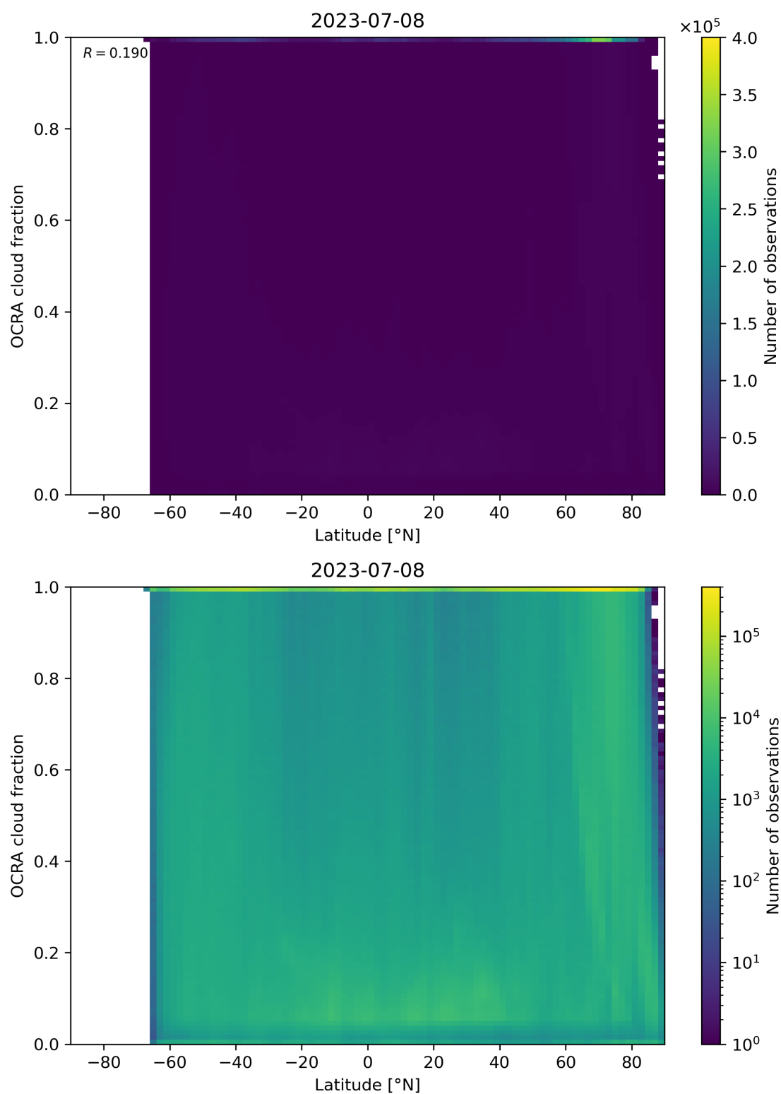
Figure 93: Scatter density plot of “Latitude” against “OCRA cloud fraction” for 2023-07-08 to 2023-07-09.
