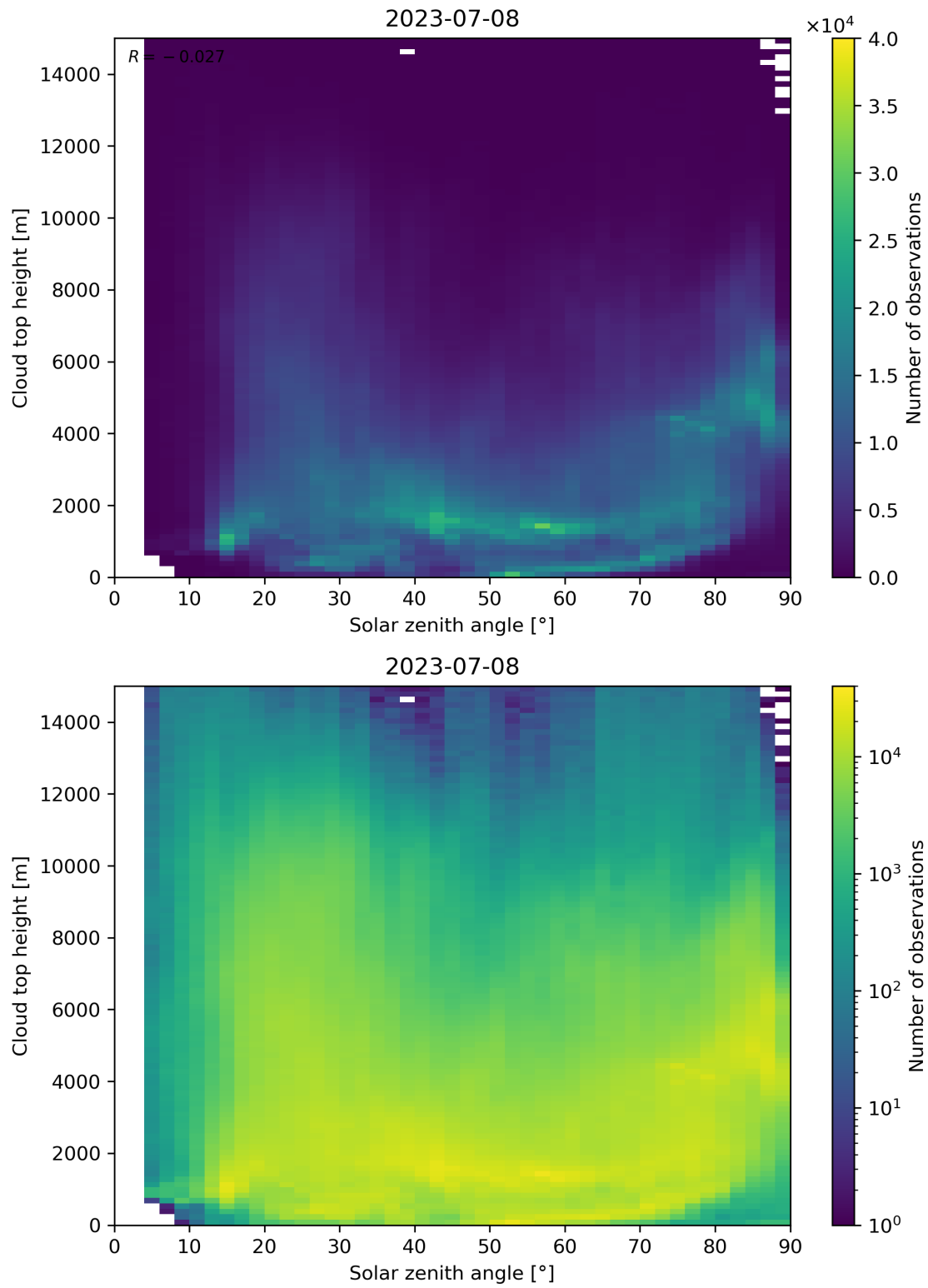
Figure 104: Scatter density plot of “Solar zenith angle” against “Cloud top height” for 2023-07-08 to 2023-07-09.
