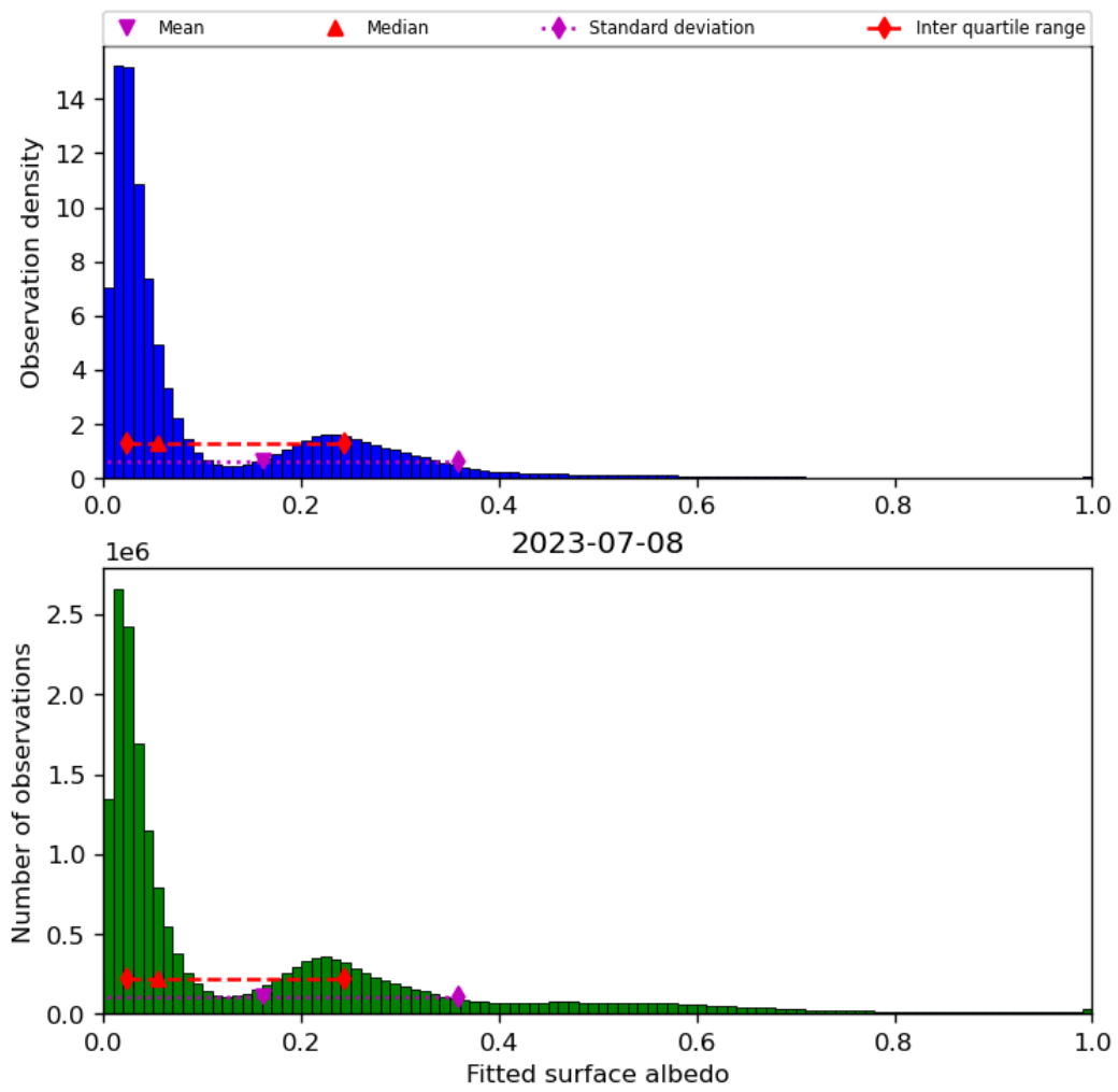
Figure 45: Histogram of “Fitted surface albedo” for 2023-07-08 to 2023-07-09
