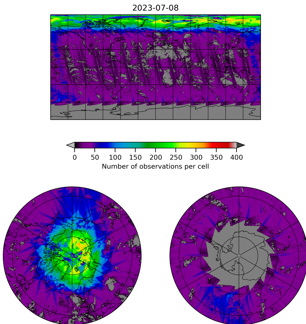
Figure 21: Map of the number of observations for 2023-07-08 to 2023-07-09
