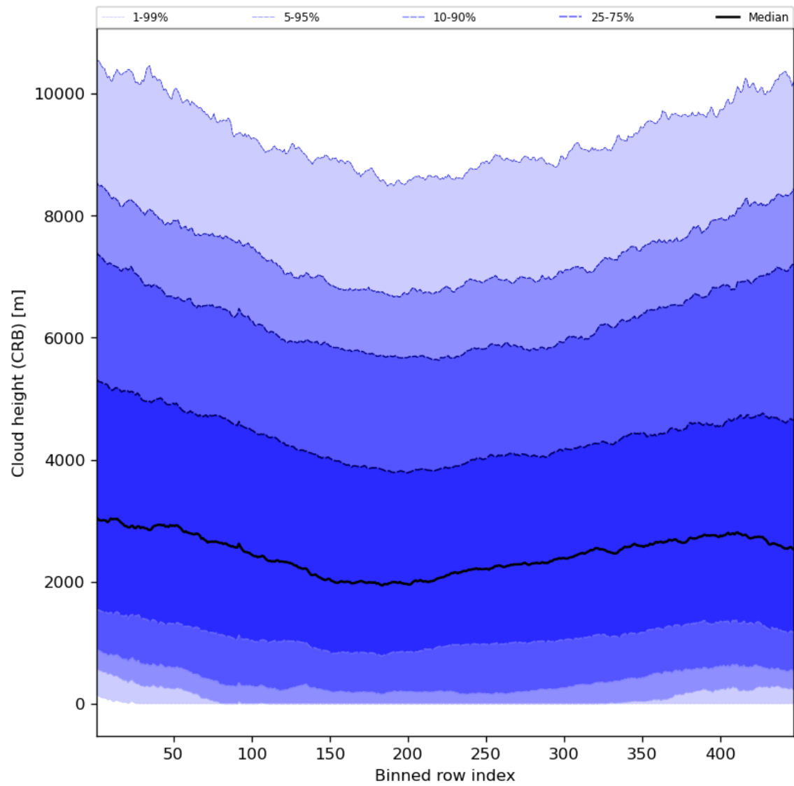
Figure 59: Along track statistics of “Cloud height (CRB)” for 2023-07-08 to 2023-07-09
