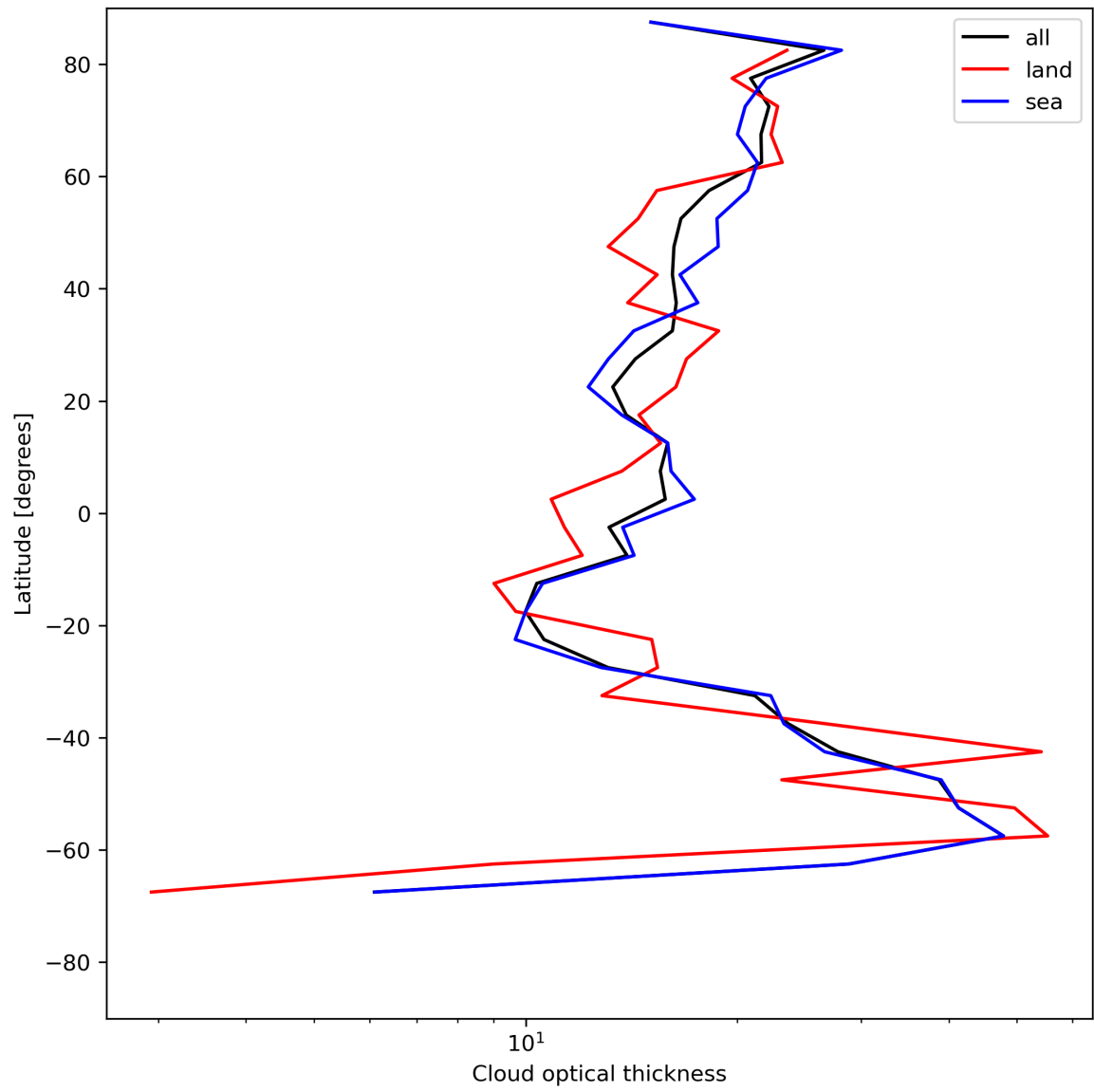
Figure 25: Zonal average of “Cloud optical thickness” for 2023-07-08 to 2023-07-09.
