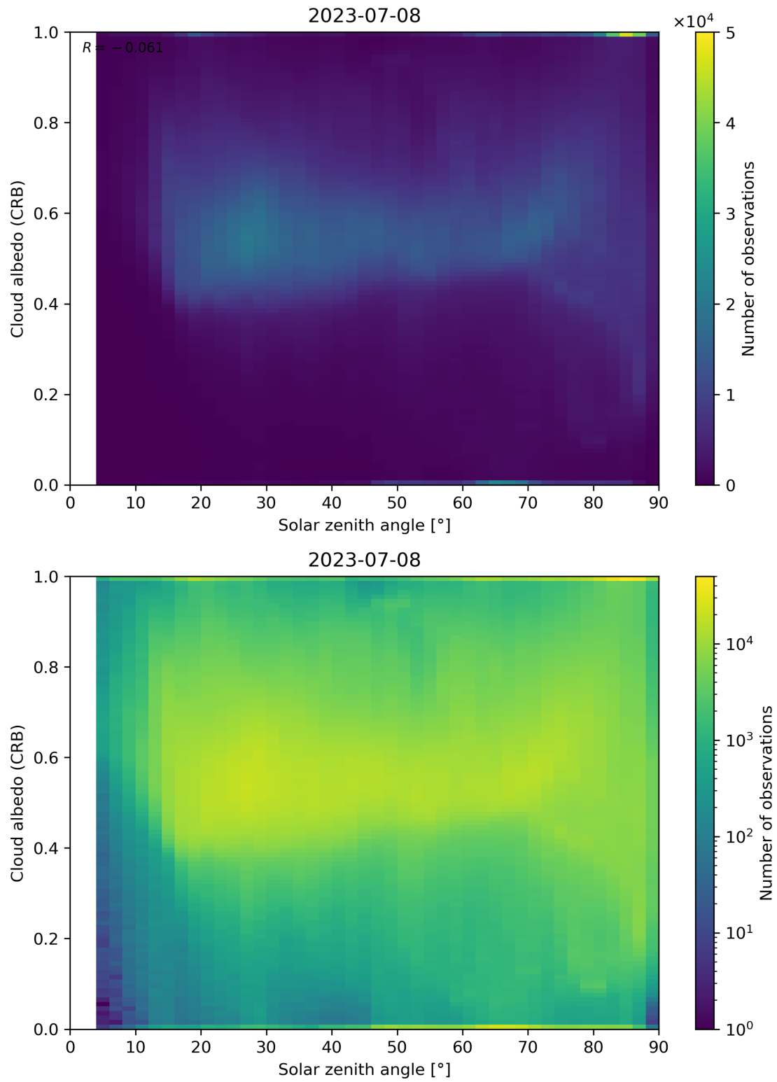
Figure 98: Scatter density plot of “Solar zenith angle” against “Cloud albedo (CRB)” for 2023-07-08 to 2023-07-09.
