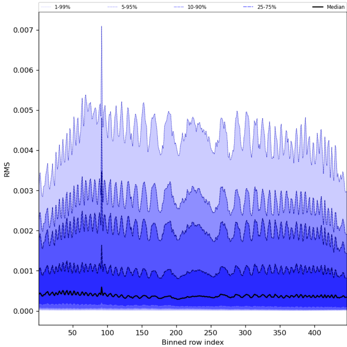
Figure 63: Along track statistics of “RMS” for 2023-07-08 to 2023-07-09
