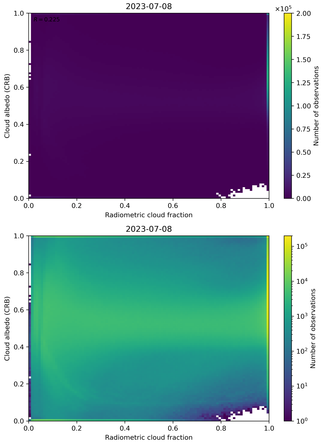
Figure 71: Scatter density plot of “Radiometric cloud fraction” against “Cloud albedo (CRB)” for 2023-07-08 to 2023-07-09.
