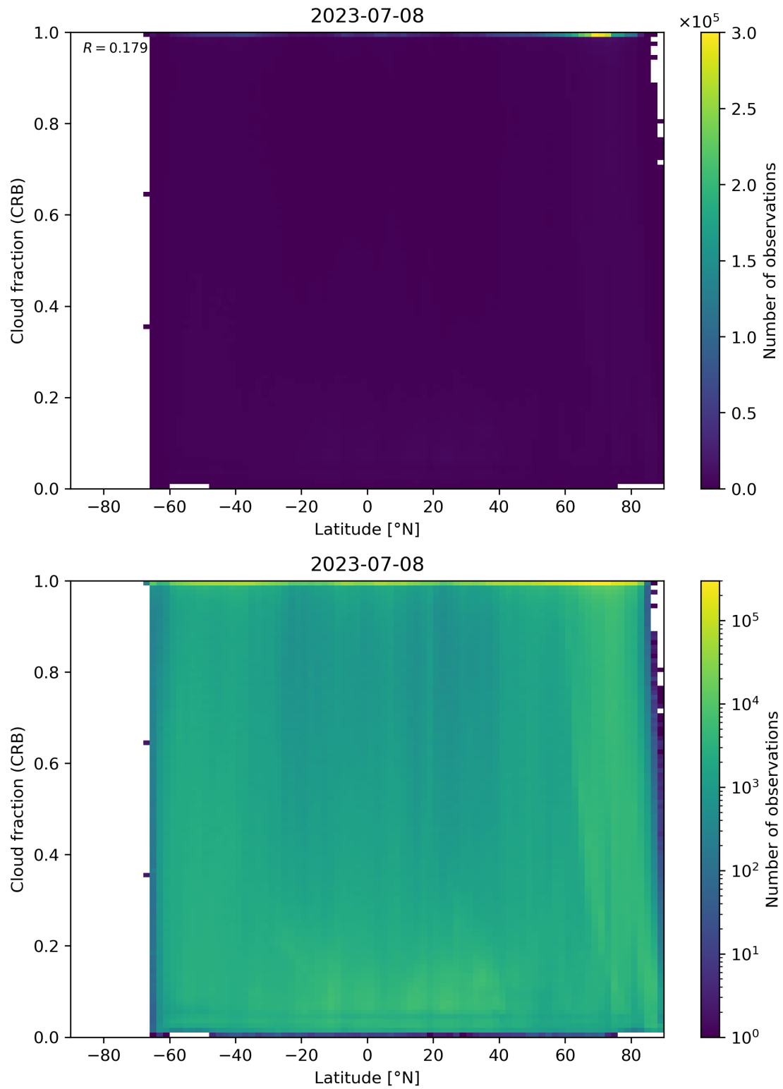
Figure 94: Scatter density plot of “Latitude” against “Cloud fraction (CRB)” for 2023-07-08 to 2023-07-09.
