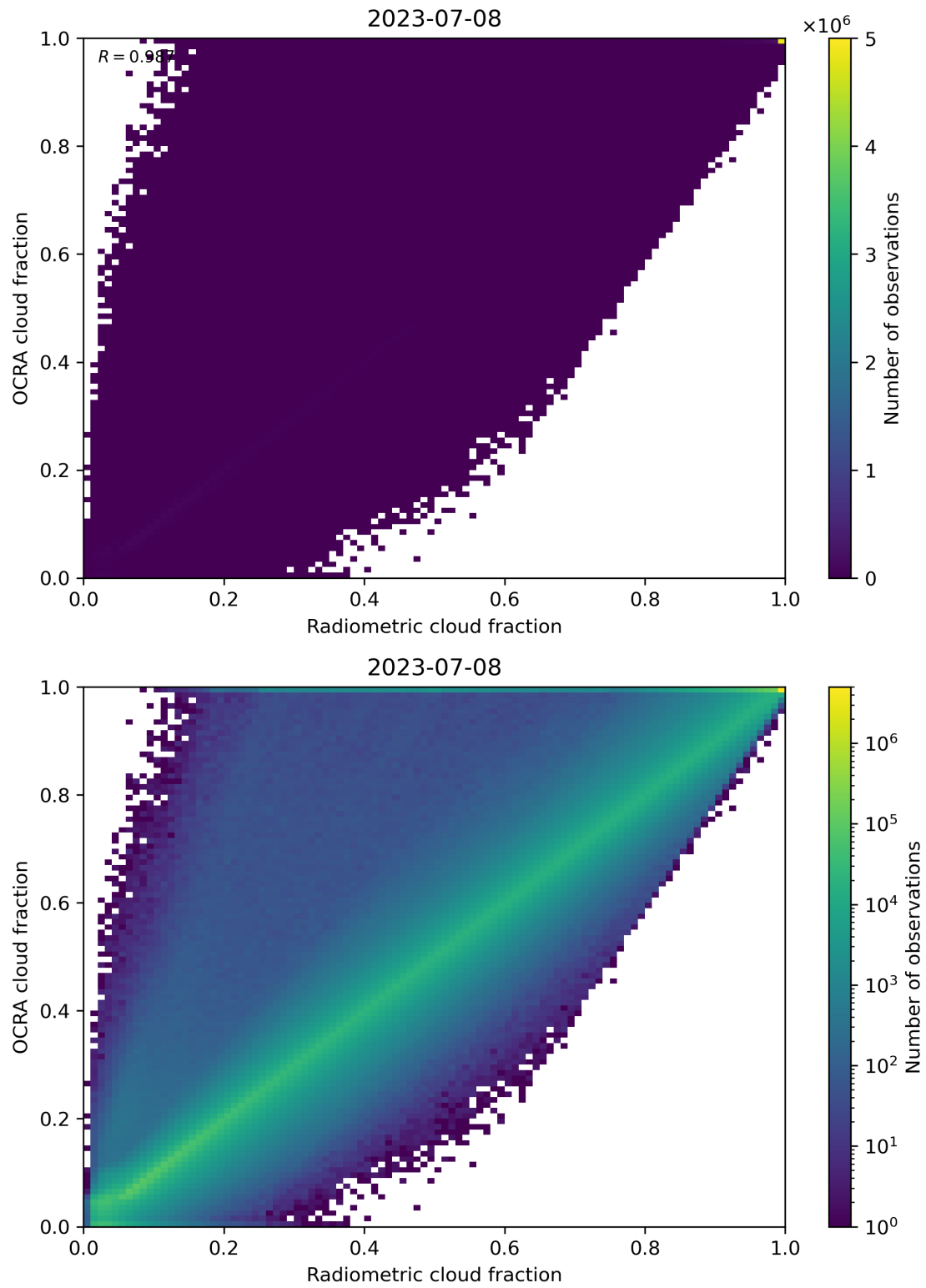
Figure 72: Scatter density plot of “Radiometric cloud fraction” against “OCRA cloud fraction” for 2023-07-08 to 2023-07-09.
