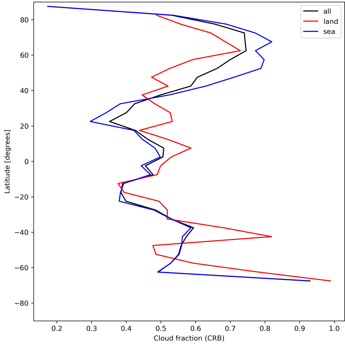
Figure 26: Zonal average of “Cloud fraction (CRB)” for 2023-07-08 to 2023-07-09.
