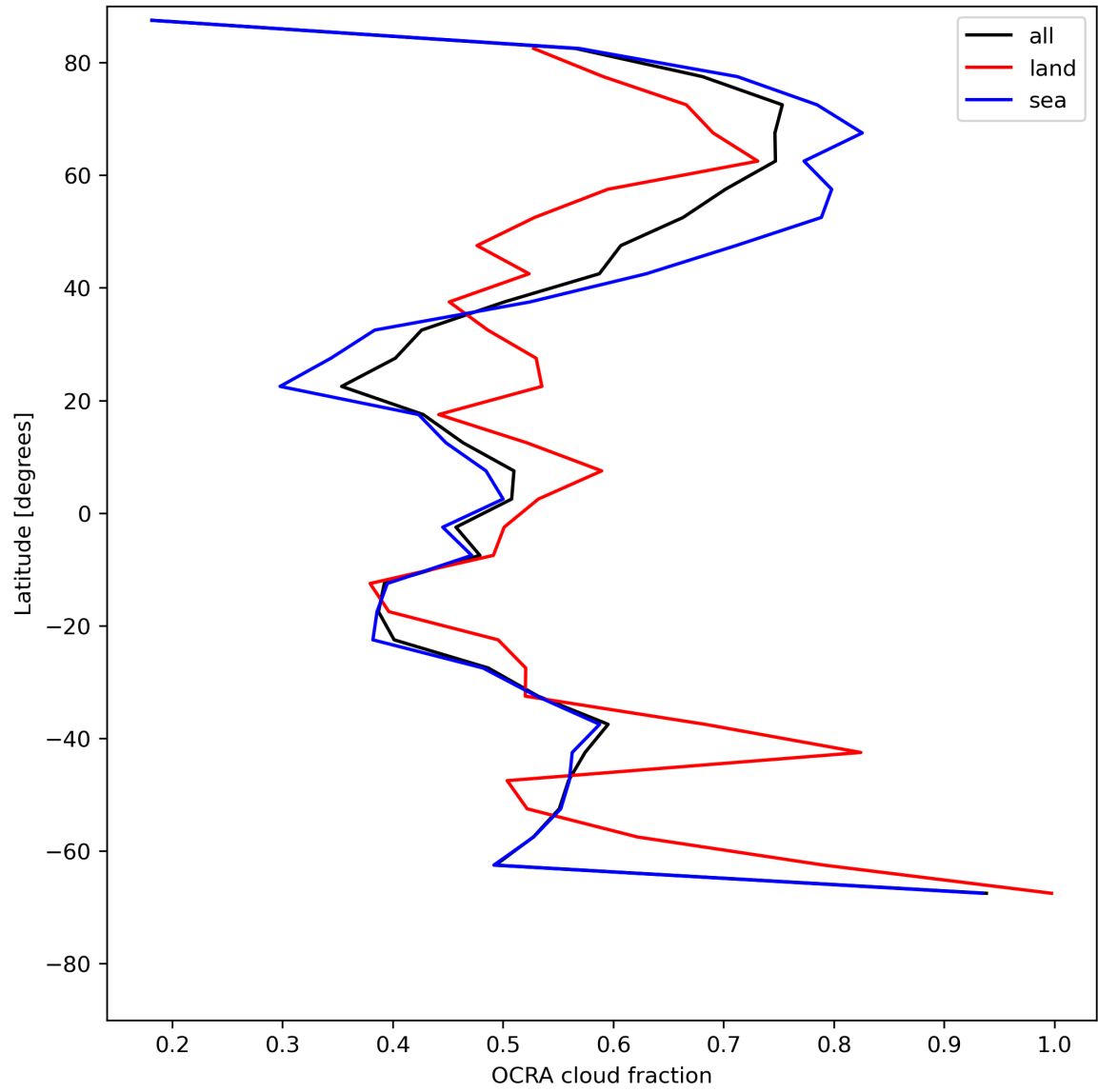
Figure 34: Zonal average of “OCRA cloud fraction” for 2023-07-08 to 2023-07-09.
