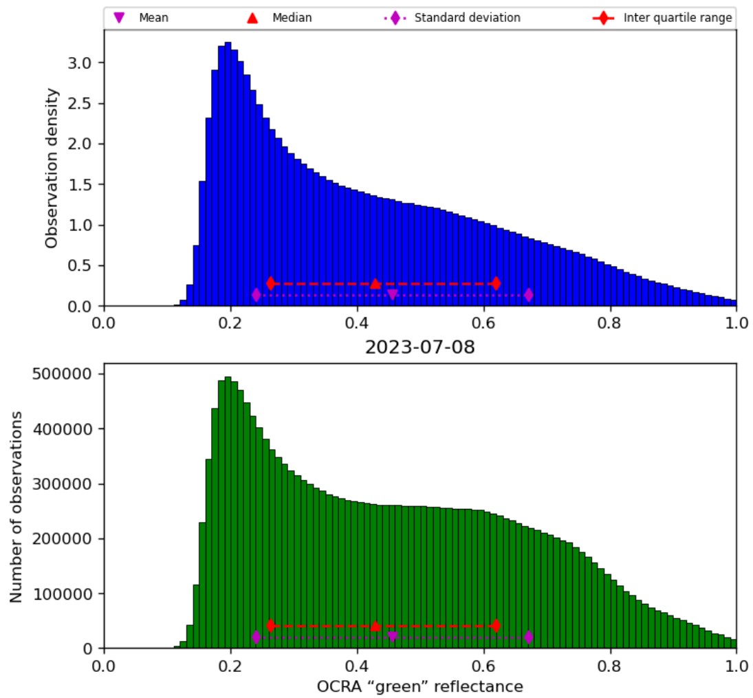
Figure 52: Histogram of “OCRA “green” reflectance” for 2023-07-08 to 2023-07-09
