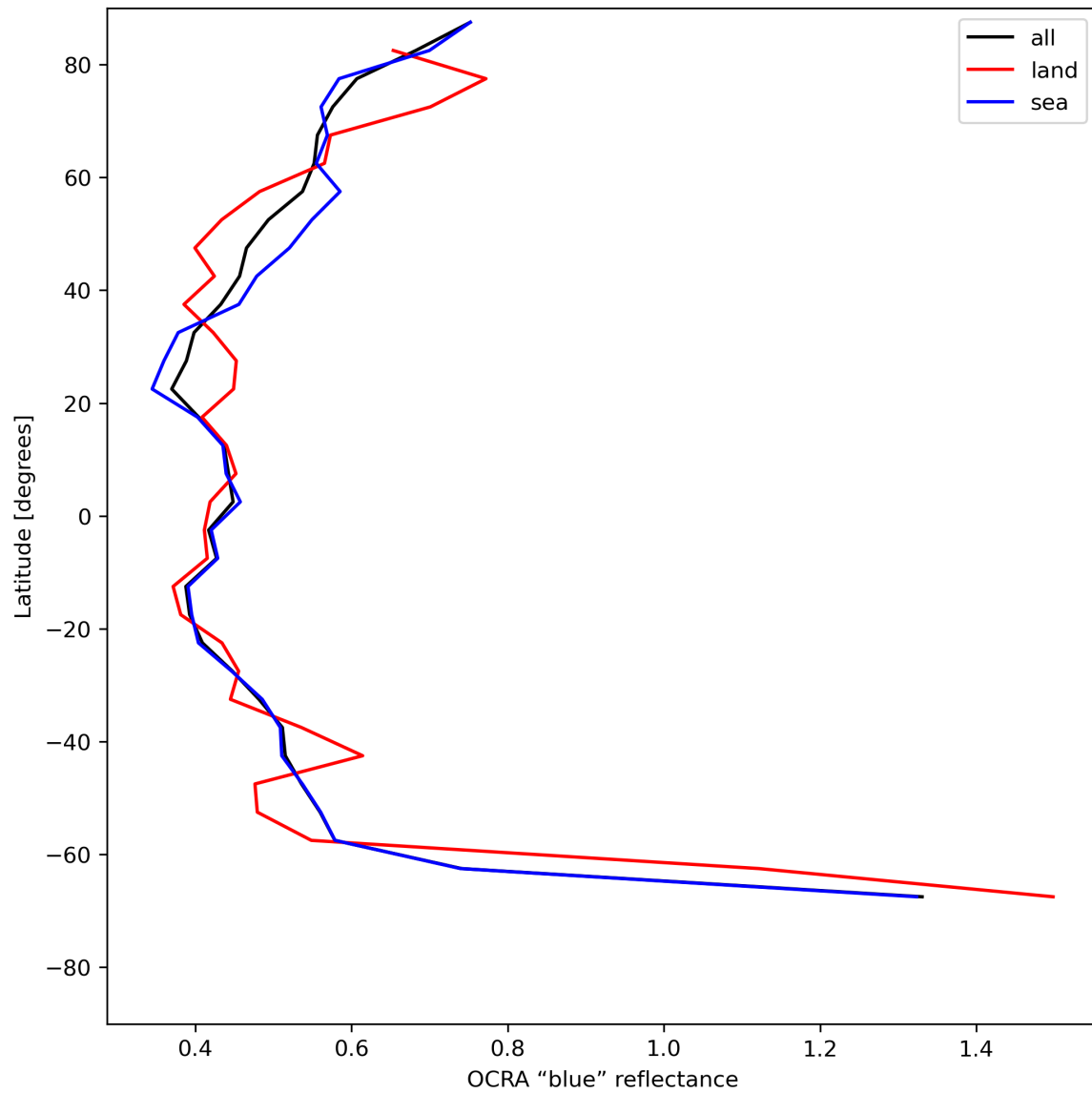
Figure 35: Zonal average of “OCRA “blue” reflectance” for 2023-07-08 to 2023-07-09.
