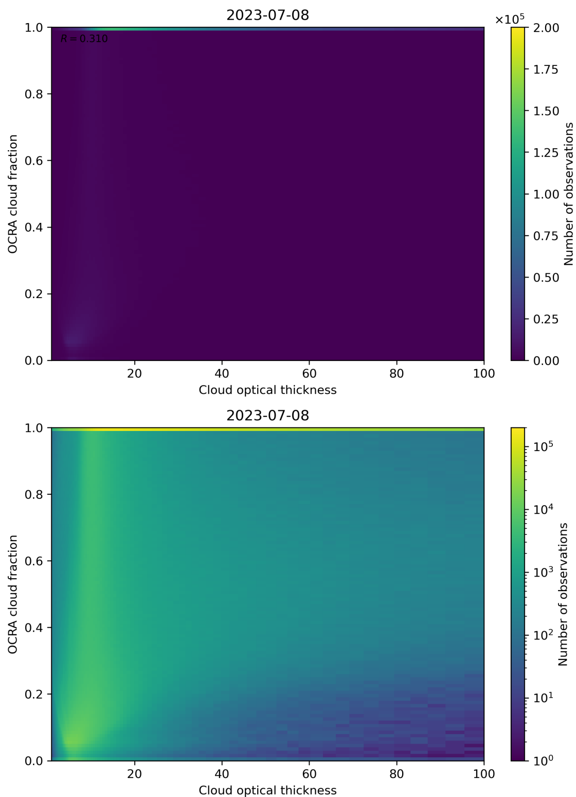
Figure 83: Scatter density plot of “Cloud optical thickness” against “OCRA cloud fraction” for 2023-07-08 to 2023-07-09.
