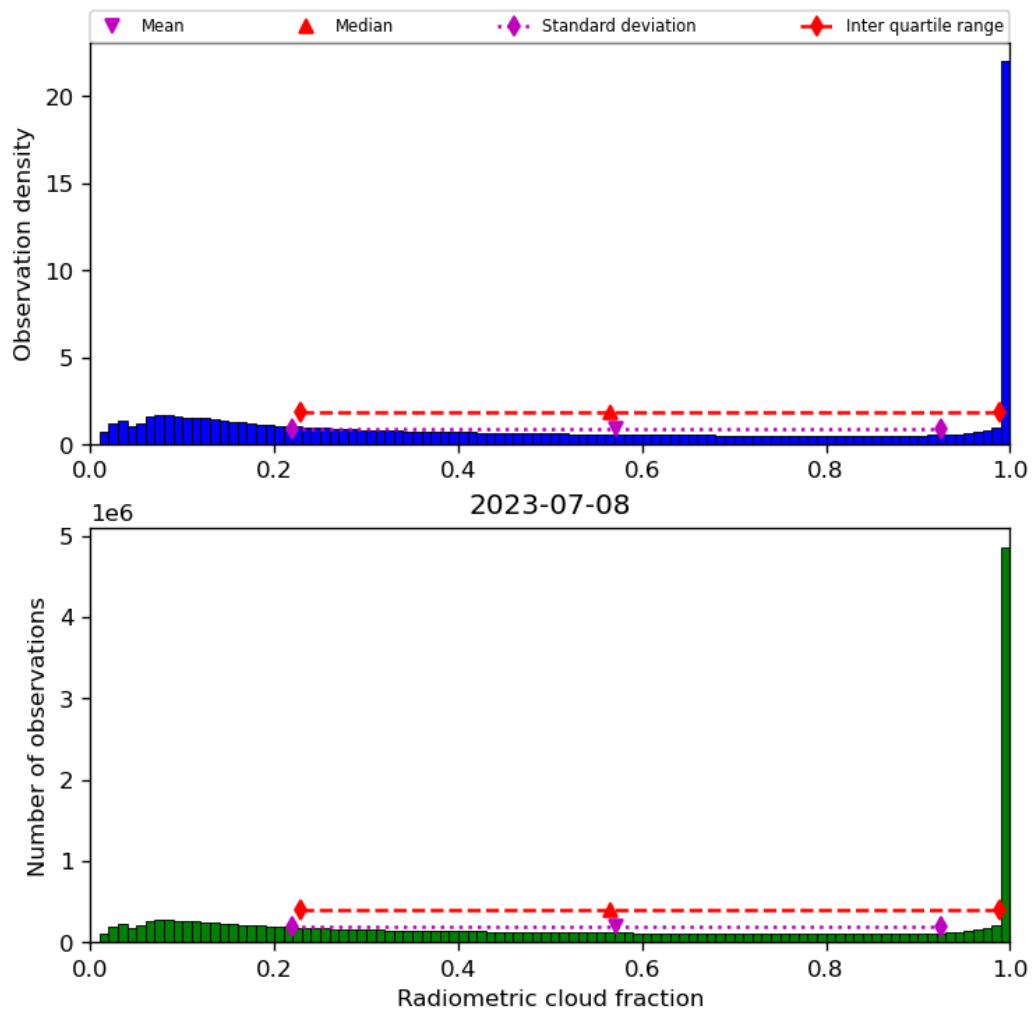
Figure 39: Histogram of “Radiometric cloud fraction” for 2023-07-08 to 2023-07-09
