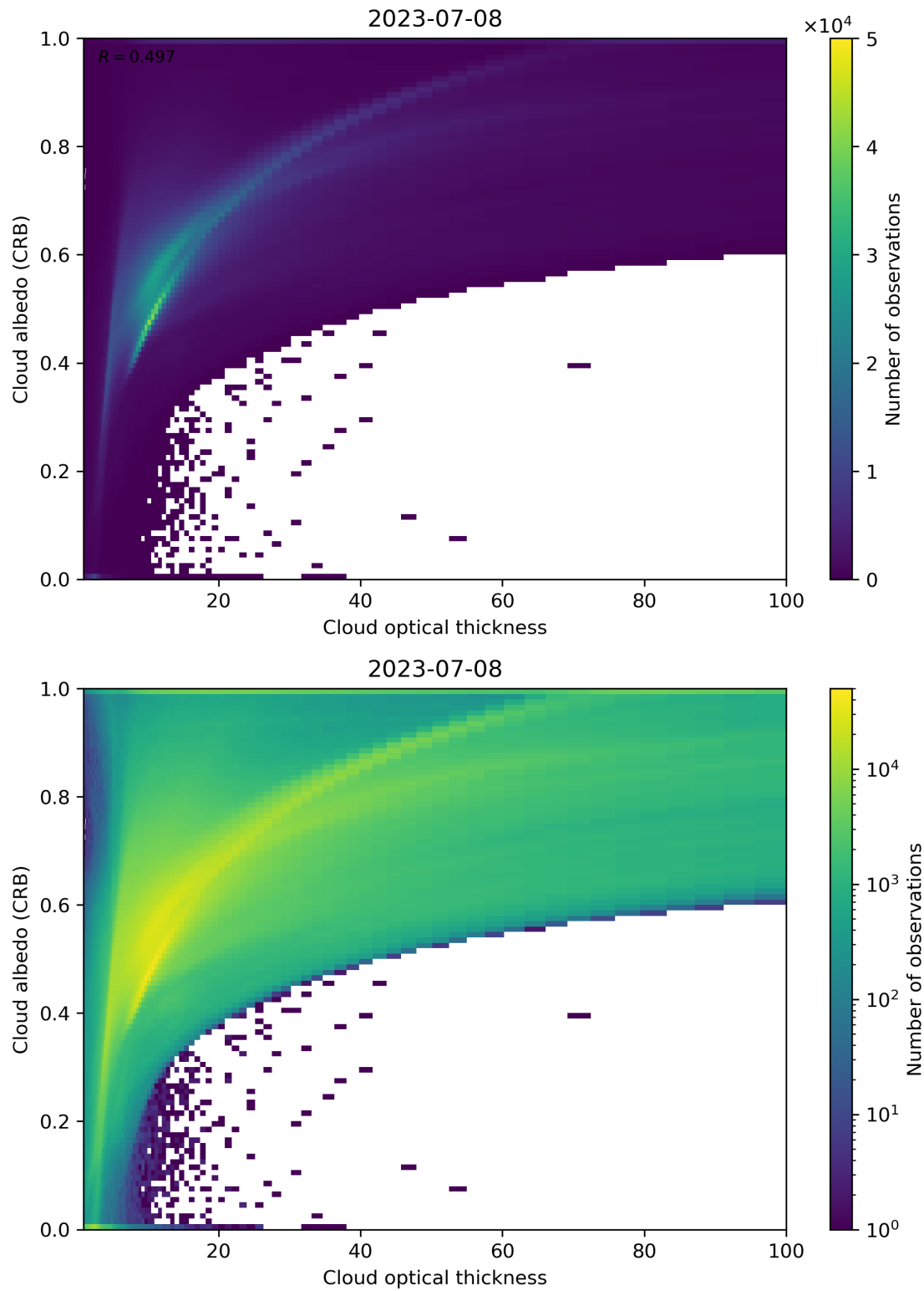
Figure 82: Scatter density plot of “Cloud optical thickness” against “Cloud albedo (CRB)” for 2023-07-08 to 2023-07-09.
