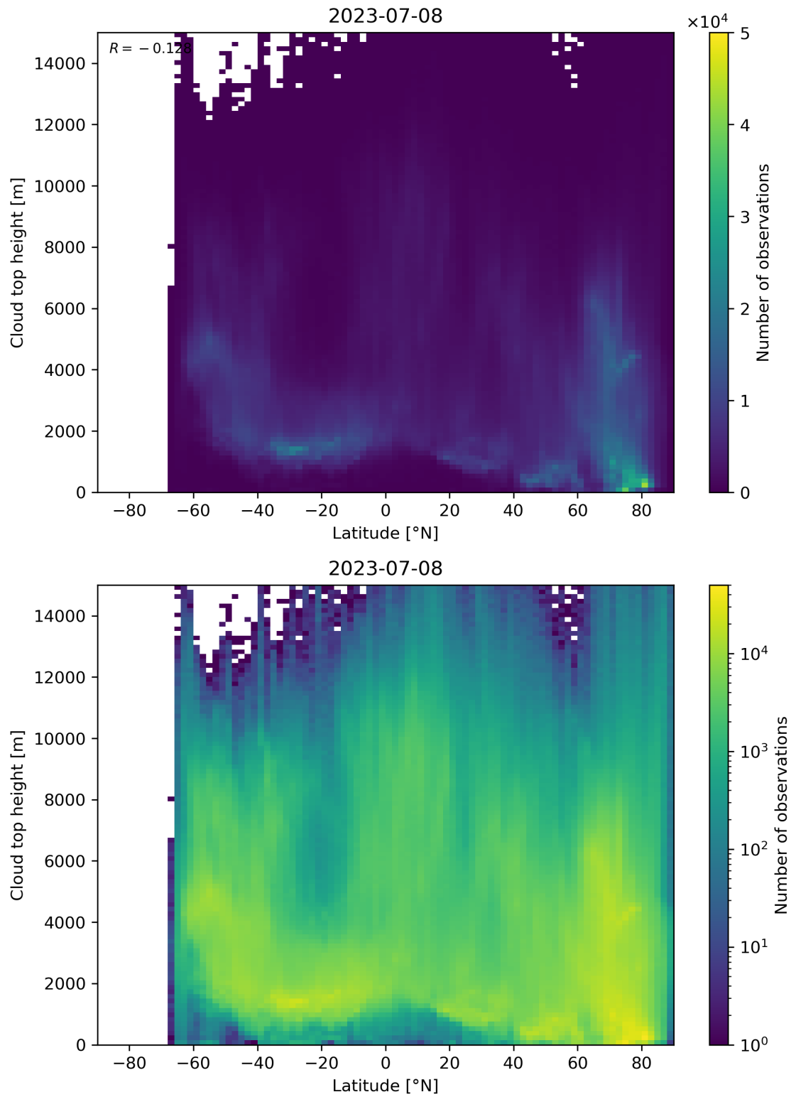
Figure 97: Scatter density plot of “Latitude” against “Cloud top height” for 2023-07-08 to 2023-07-09.
