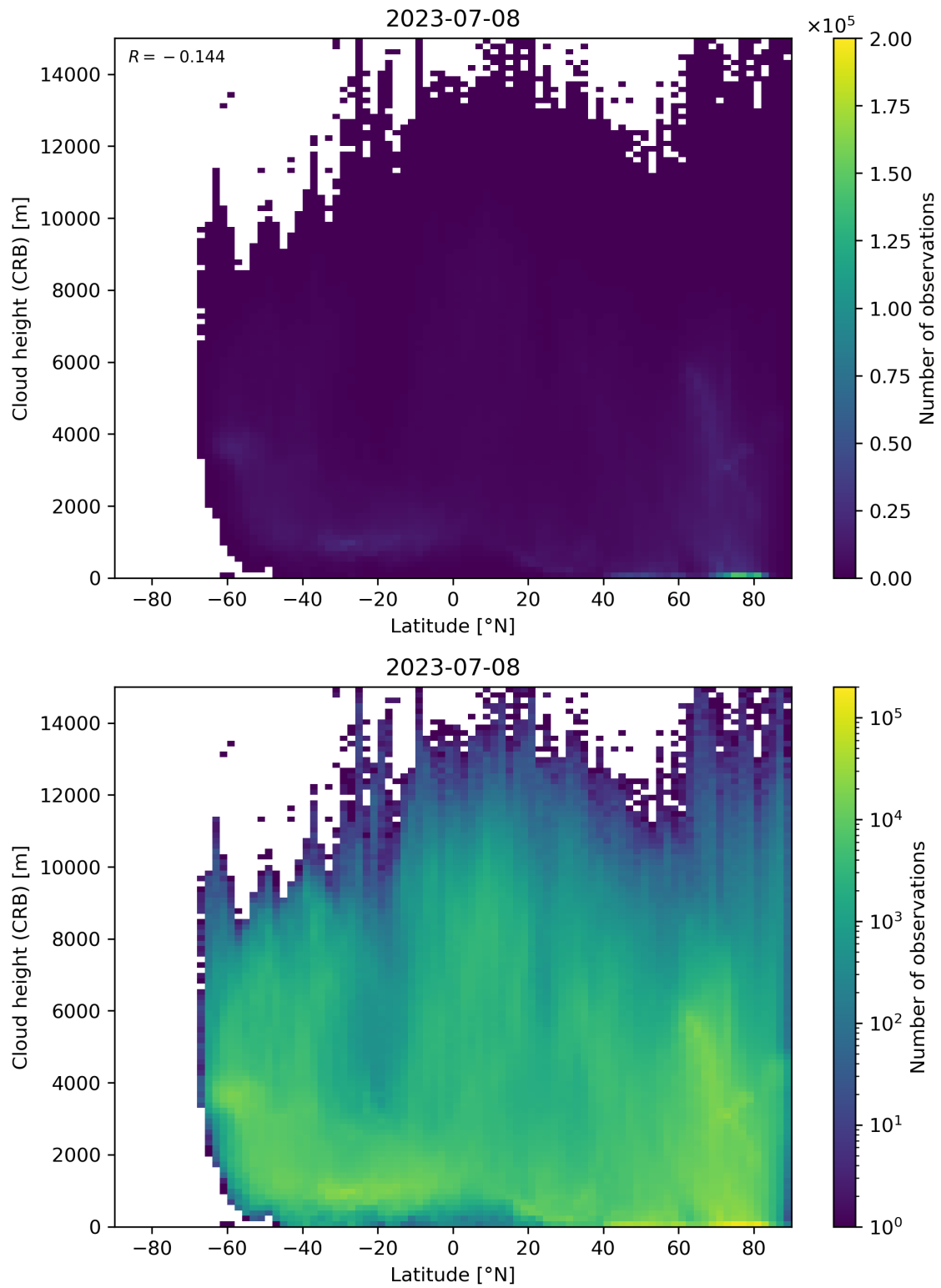
Figure 95: Scatter density plot of “Latitude” against “Cloud height (CRB)” for 2023-07-08 to 2023-07-09.
