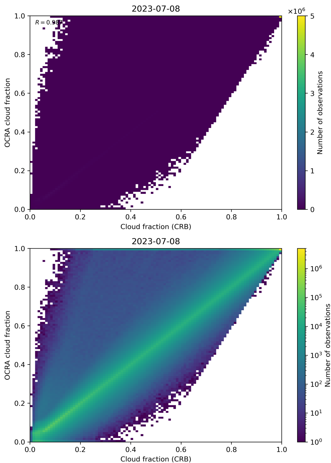
Figure 78: Scatter density plot of “Cloud fraction (CRB)” against “OCRA cloud fraction” for 2023-07-08 to 2023-07-09.
