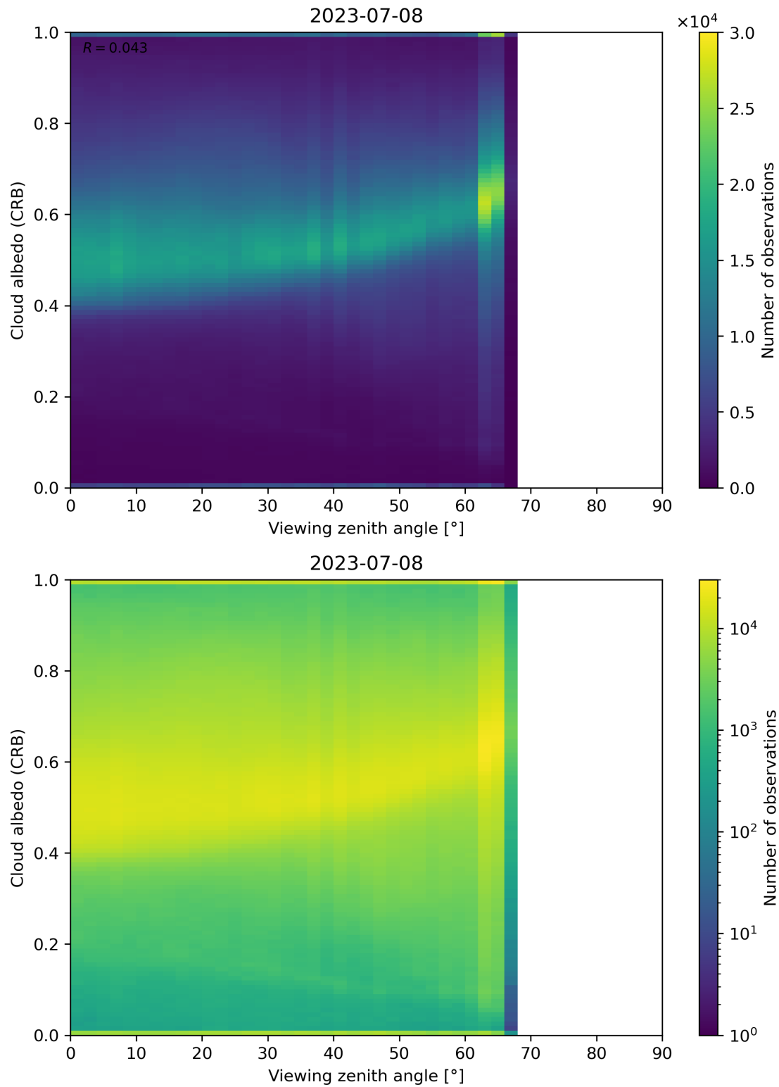
Figure 106: Scatter density plot of “Viewing zenith angle” against “Cloud albedo (CRB)” for 2023-07-08 to 2023-07-09.
