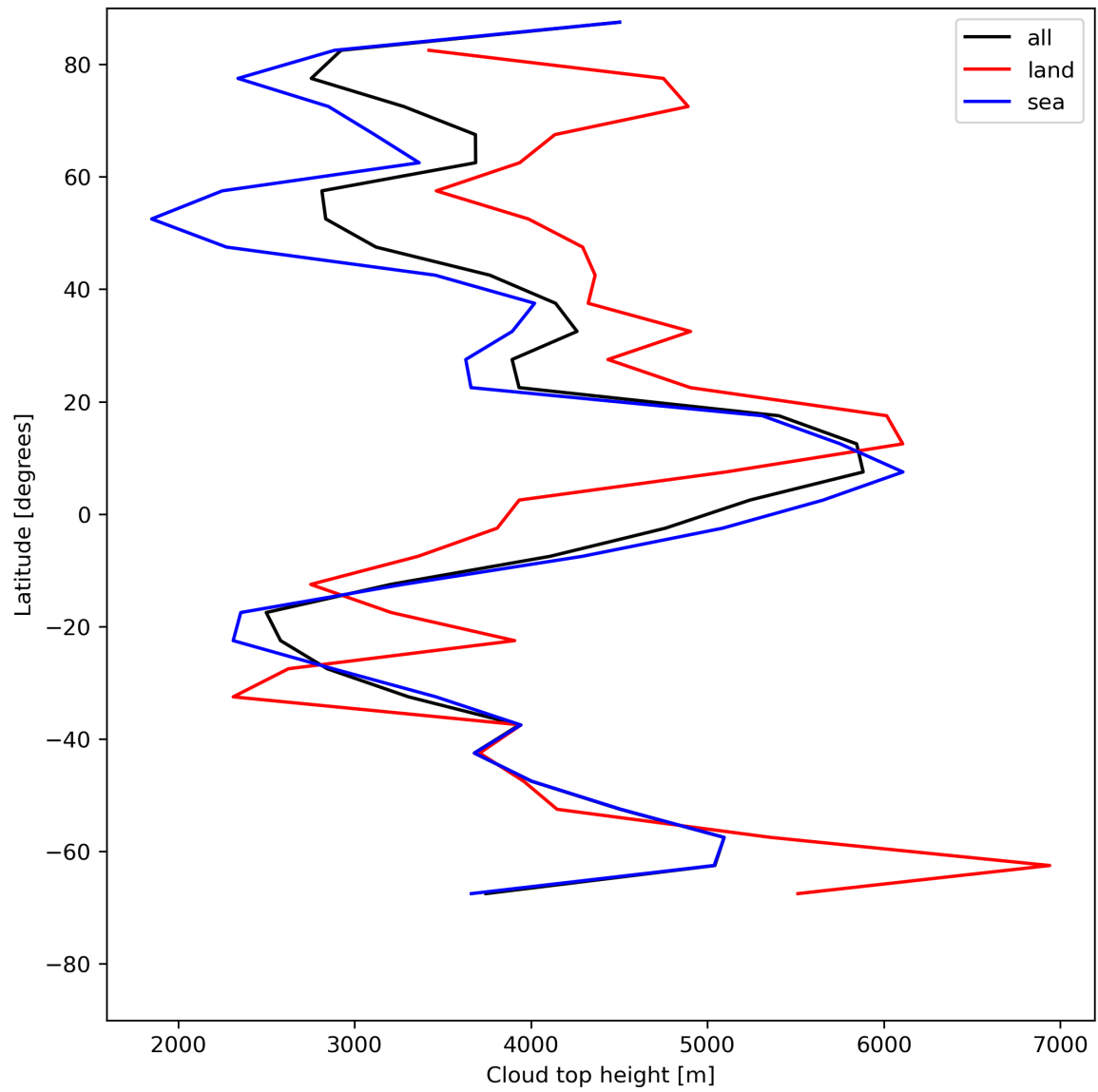
Figure 24: Zonal average of “Cloud top height” for 2023-07-08 to 2023-07-09.
