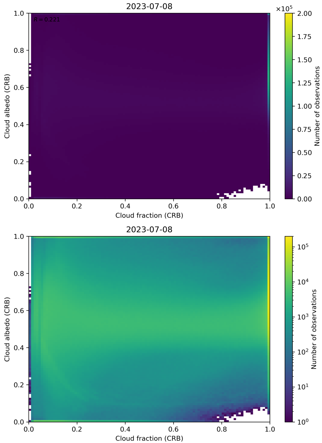
Figure 77: Scatter density plot of “Cloud fraction (CRB)” against “Cloud albedo (CRB)” for 2023-07-08 to 2023-07-09.
