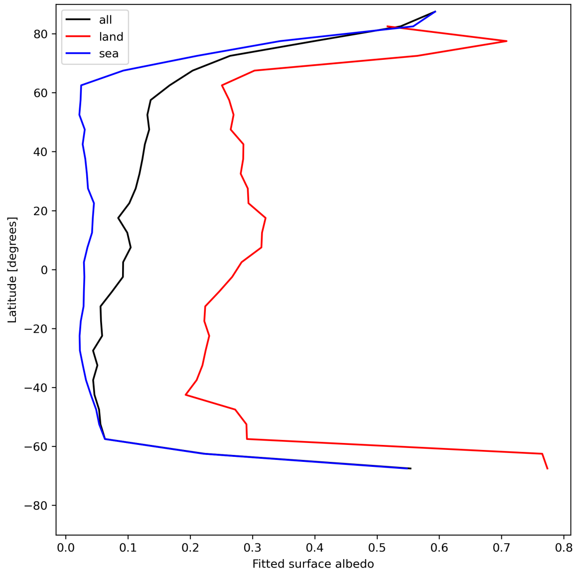
Figure 29: Zonal average of “Fitted surface albedo” for 2023-07-08 to 2023-07-09.
