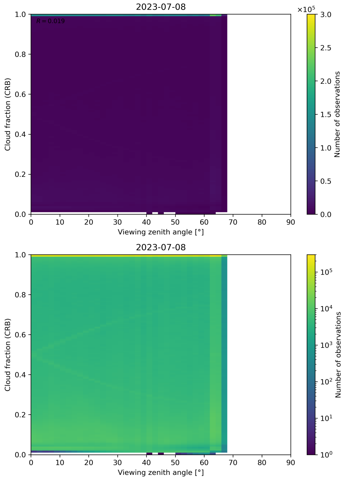
Figure 109: Scatter density plot of “Viewing zenith angle” against “Cloud fraction (CRB)” for 2023-07-08 to 2023-07-09.
