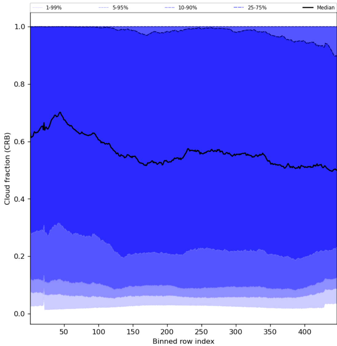
Figure 58: Along track statistics of “Cloud fraction (CRB)” for 2023-07-08 to 2023-07-09
