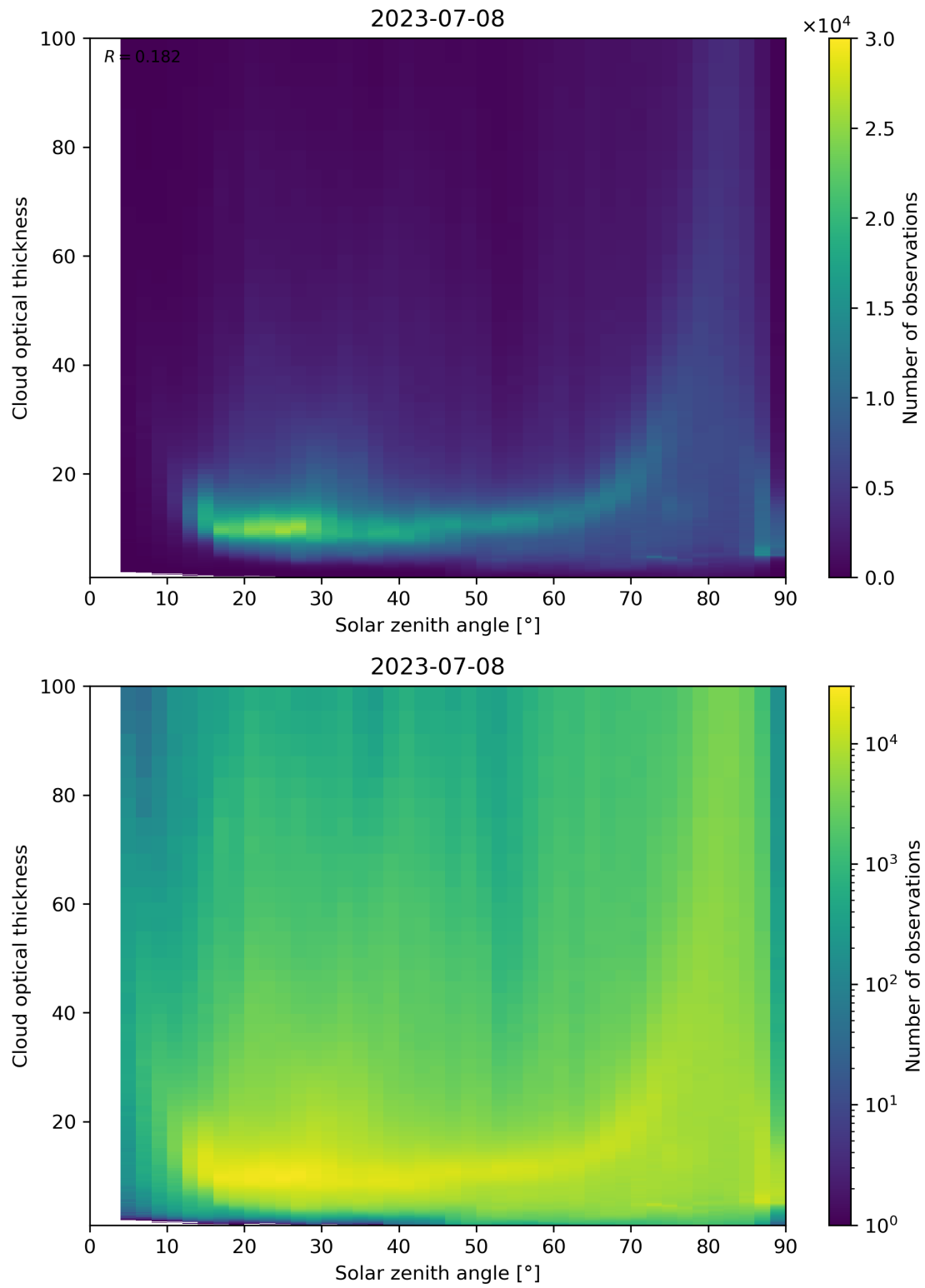
Figure 103: Scatter density plot of “Solar zenith angle” against “Cloud optical thickness” for 2023-07-08 to 2023-07-09.
