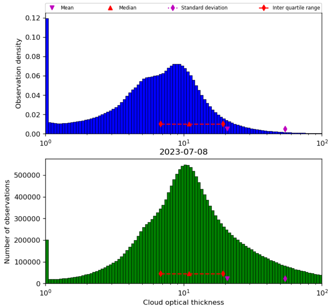
Figure 41: Histogram of “Cloud optical thickness” for 2023-07-08 to 2023-07-09
