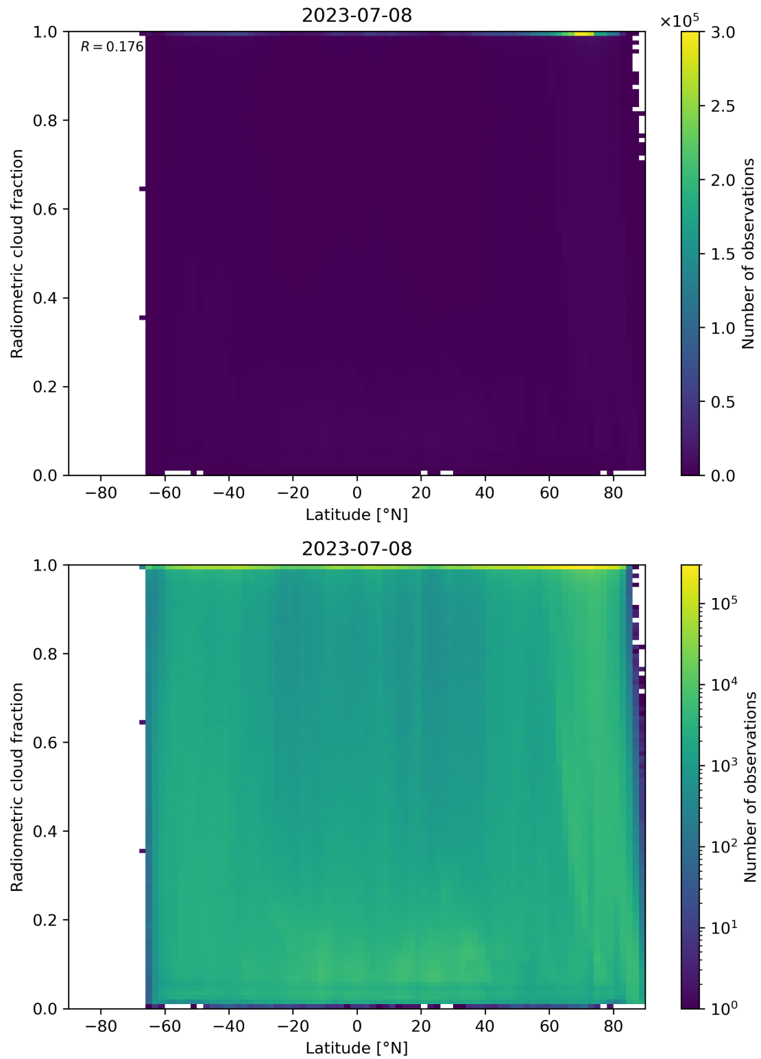
Figure 92: Scatter density plot of “Latitude” against “Radiometric cloud fraction” for 2023-07-08 to 2023-07-09.
