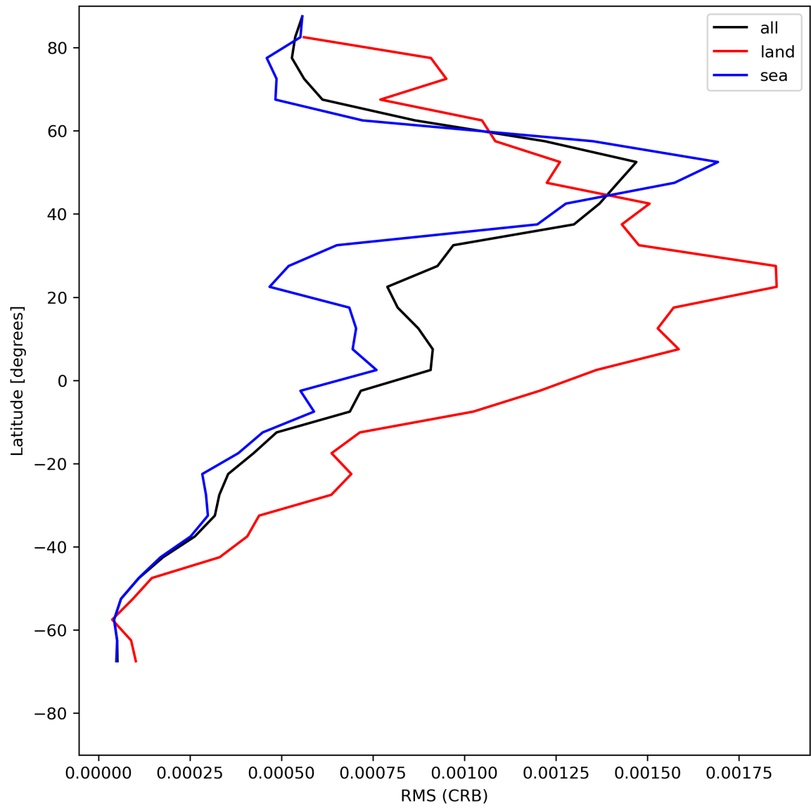
Figure 32: Zonal average of “RMS (CRB)” for 2023-07-08 to 2023-07-09.
