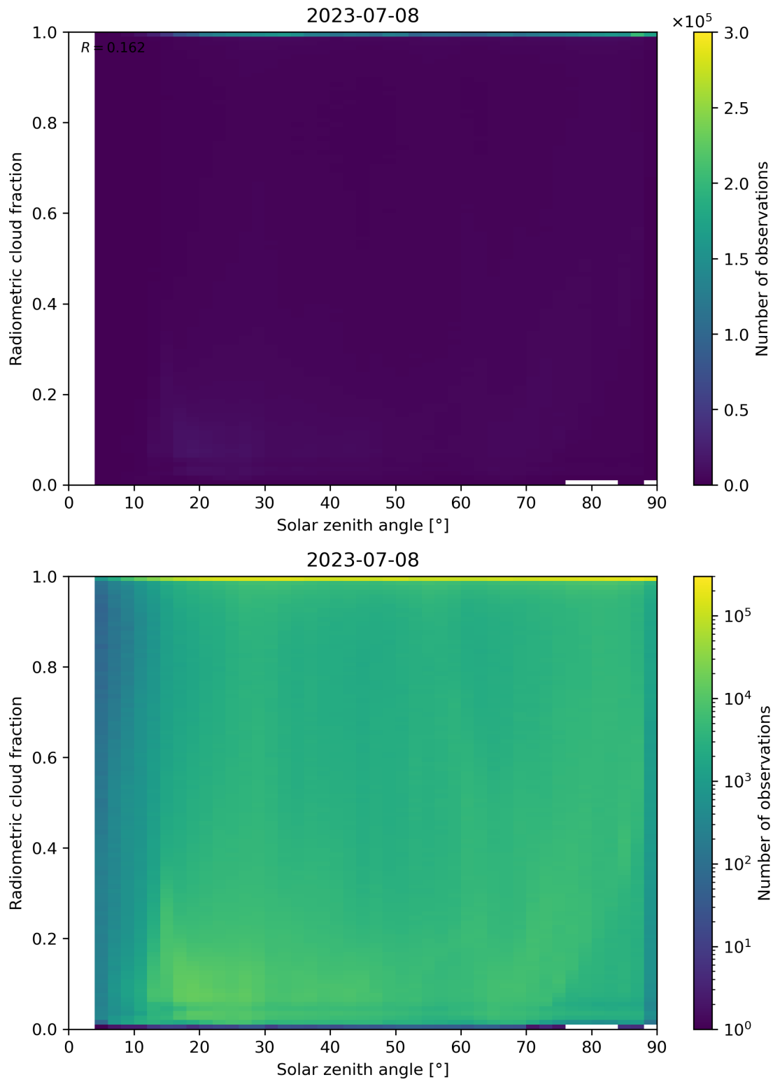
Figure 99: Scatter density plot of “Solar zenith angle” against “Radiometric cloud fraction” for 2023-07-08 to 2023-07-09.
