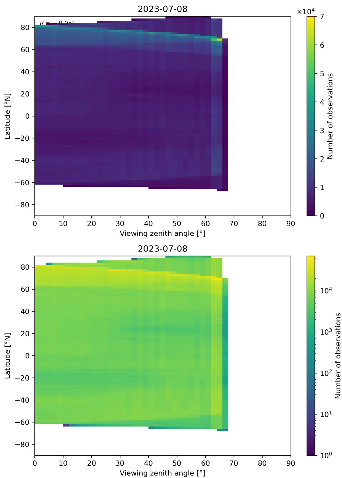
Figure 113: Scatter density plot of “Viewing zenith angle” against “Latitude” for 2023-07-08 to 2023-07-09.
