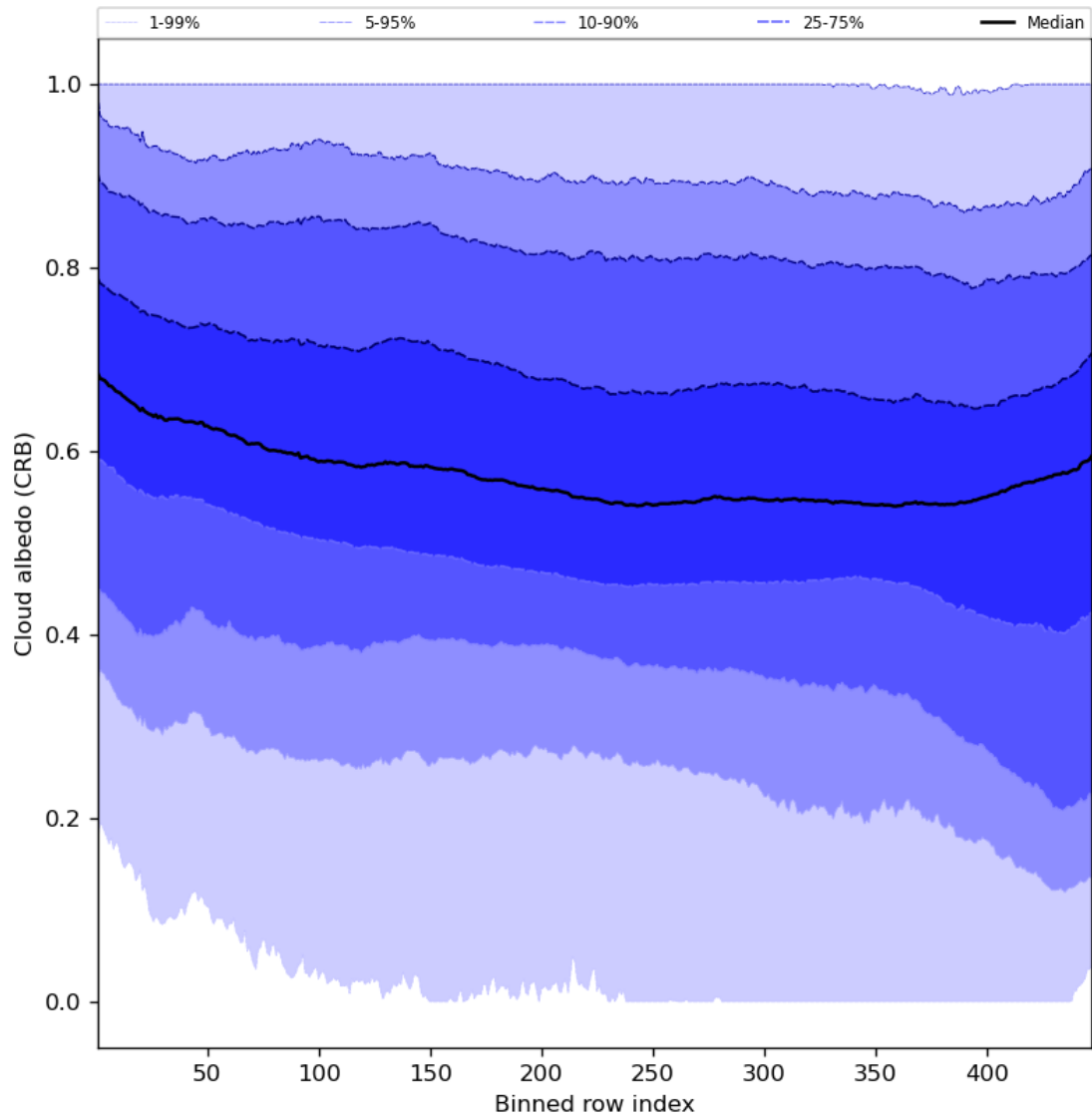
Figure 60: Along track statistics of “Cloud albedo (CRB)” for 2023-07-08 to 2023-07-09
