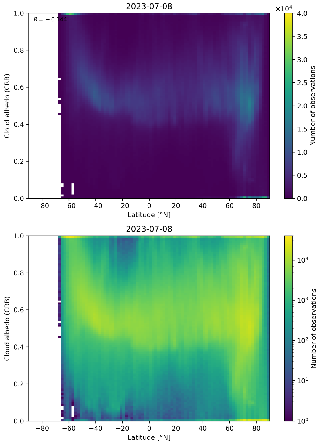
Figure 91: Scatter density plot of “Latitude” against “Cloud albedo (CRB)” for 2023-07-08 to 2023-07-09.
