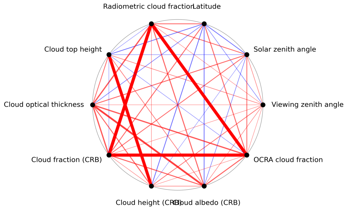
Figure 1: Map of correlation graph for 2023-07-08 to 2023-07-09.
