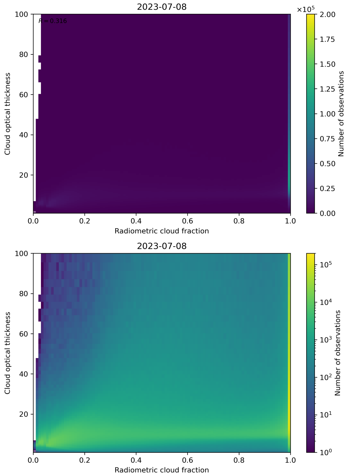
Figure 75: Scatter density plot of “Radiometric cloud fraction” against “Cloud optical thickness” for 2023-07-08 to 2023-07-09.
