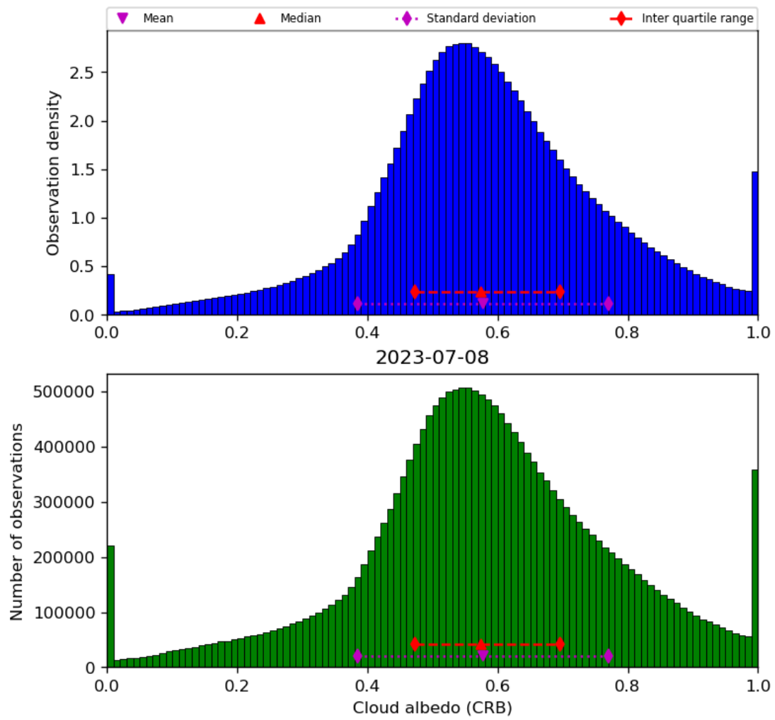
Figure 44: Histogram of “Cloud albedo (CRB)” for 2023-07-08 to 2023-07-09
