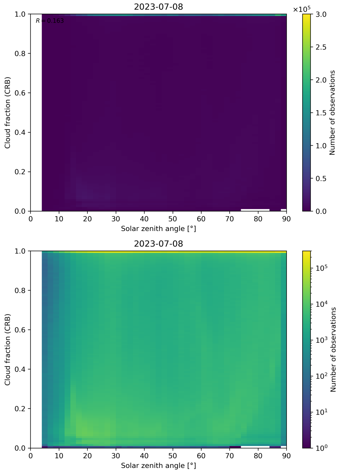
Figure 101: Scatter density plot of “Solar zenith angle” against “Cloud fraction (CRB)” for 2023-07-08 to 2023-07-09.
