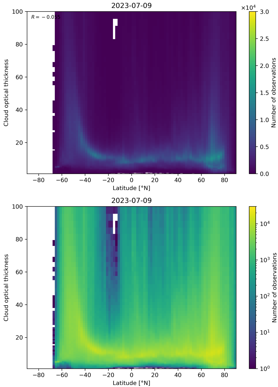
Figure 96: Scatter density plot of “Latitude” against “Cloud optical thickness” for 2023-07-08 to 2023-07-10.
