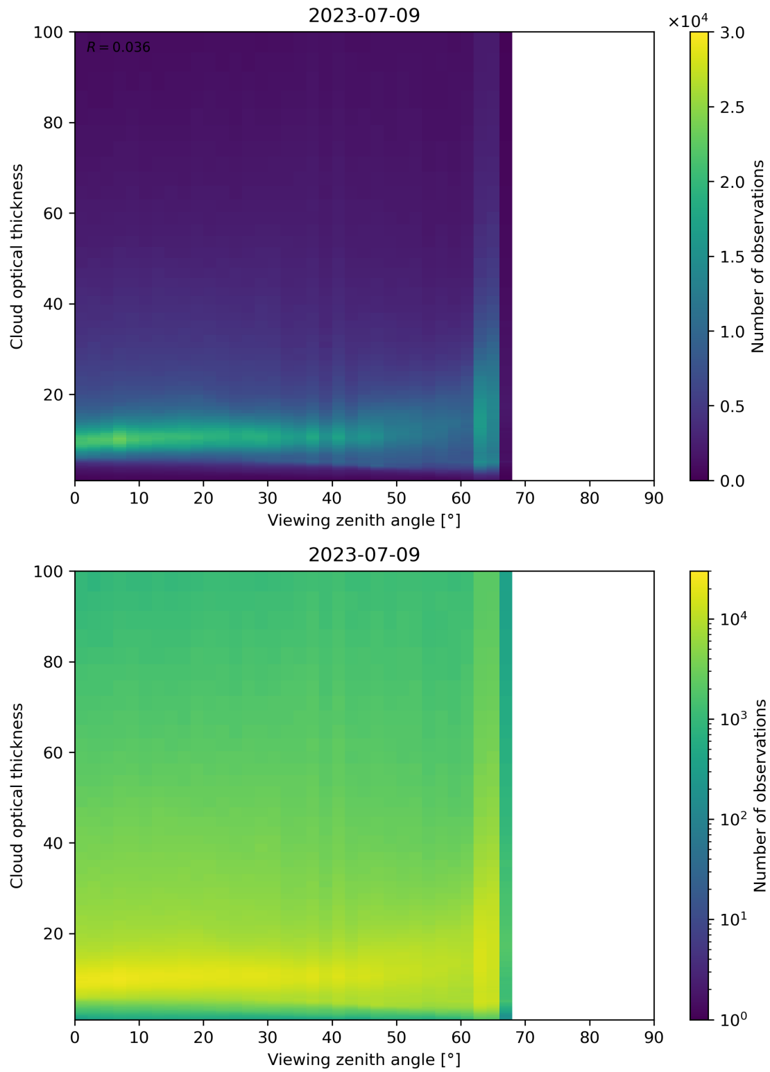
Figure 111: Scatter density plot of “Viewing zenith angle” against “Cloud optical thickness” for 2023-07-08 to 2023-07-10.
