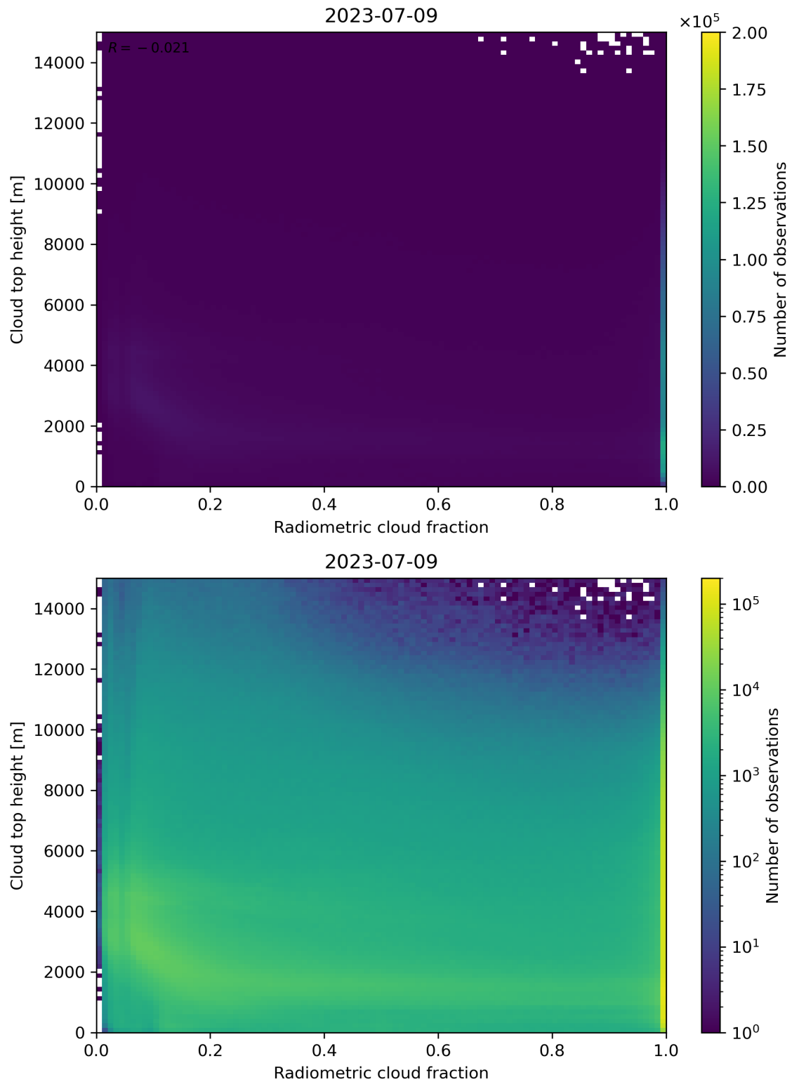
Figure 76: Scatter density plot of “Radiometric cloud fraction” against “Cloud top height” for 2023-07-08 to 2023-07-10.
