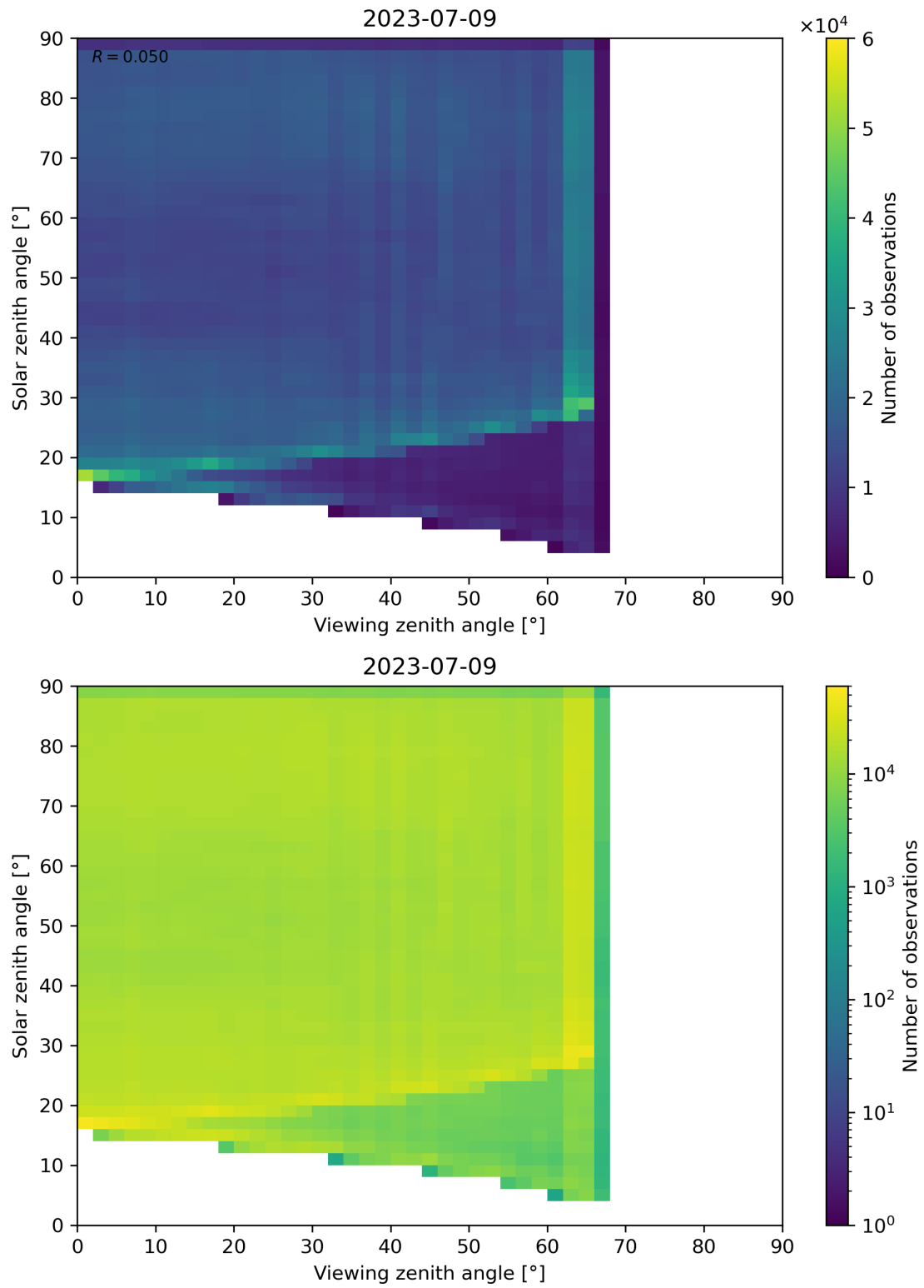
Figure 114: Scatter density plot of “Viewing zenith angle” against “Solar zenith angle” for 2023-07-08 to 2023-07-10.
