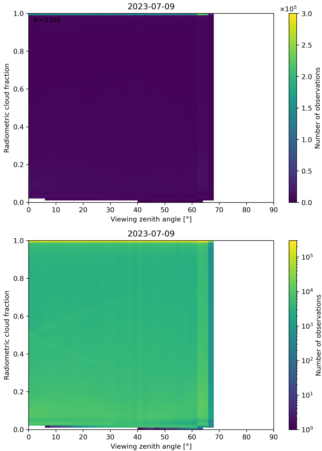
Figure 107: Scatter density plot of “Viewing zenith angle” against “Radiometric cloud fraction” for 2023-07-08 to 2023-07-10.
