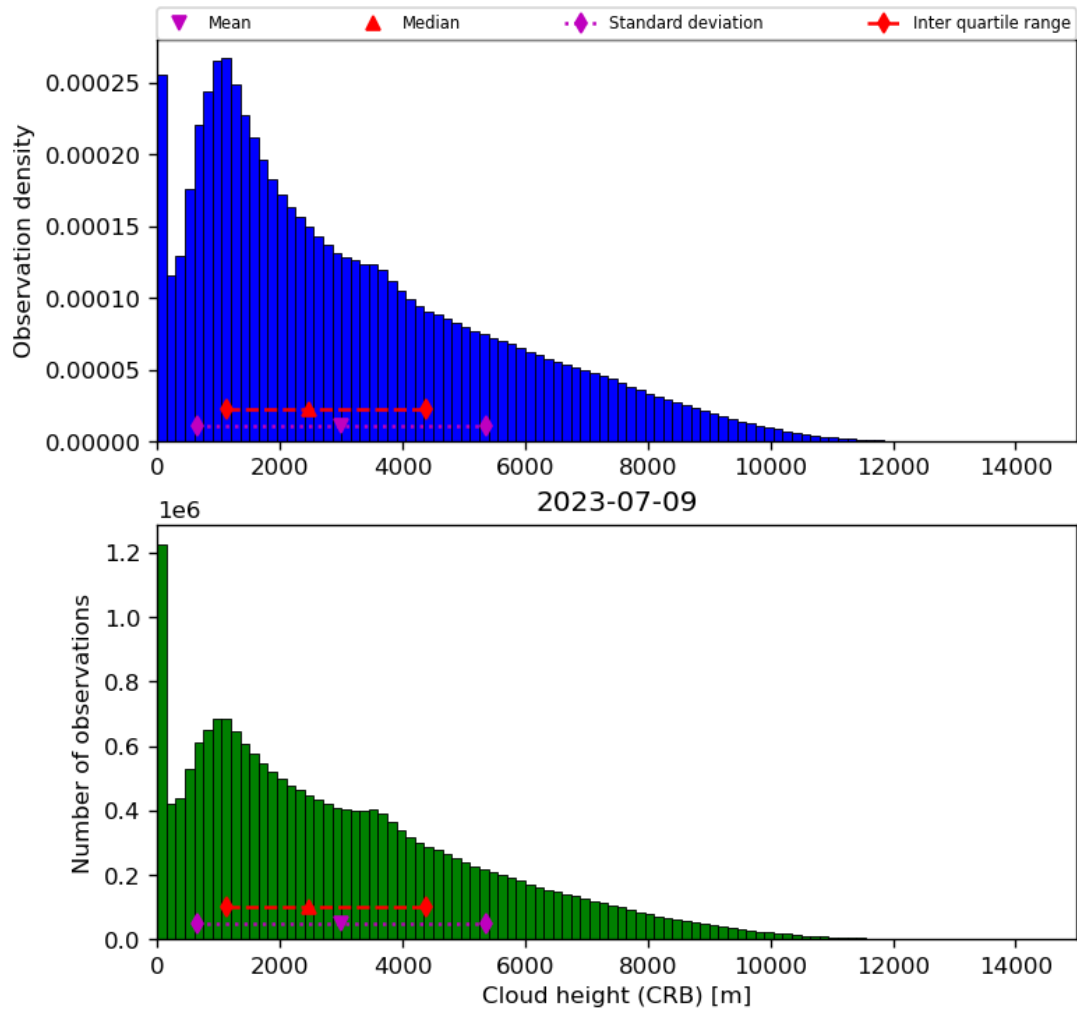
Figure 43: Histogram of “Cloud height (CRB)” for 2023-07-08 to 2023-07-10
