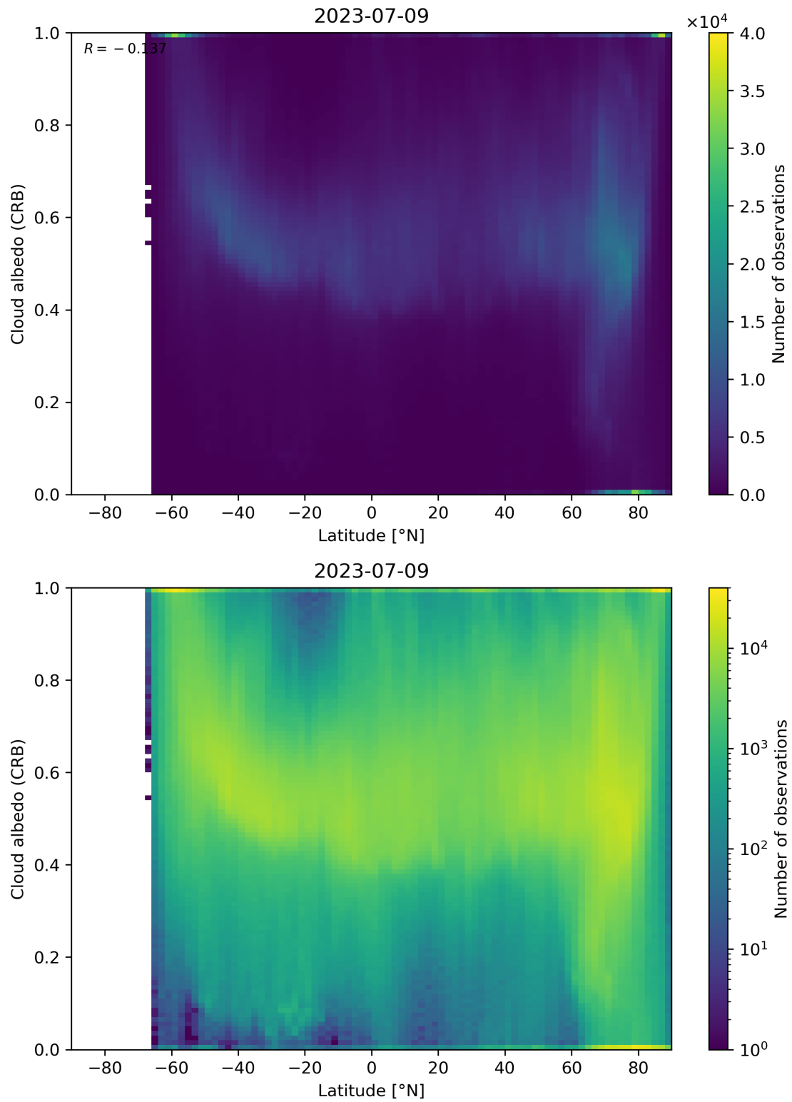
Figure 91: Scatter density plot of “Latitude” against “Cloud albedo (CRB)” for 2023-07-08 to 2023-07-10.
