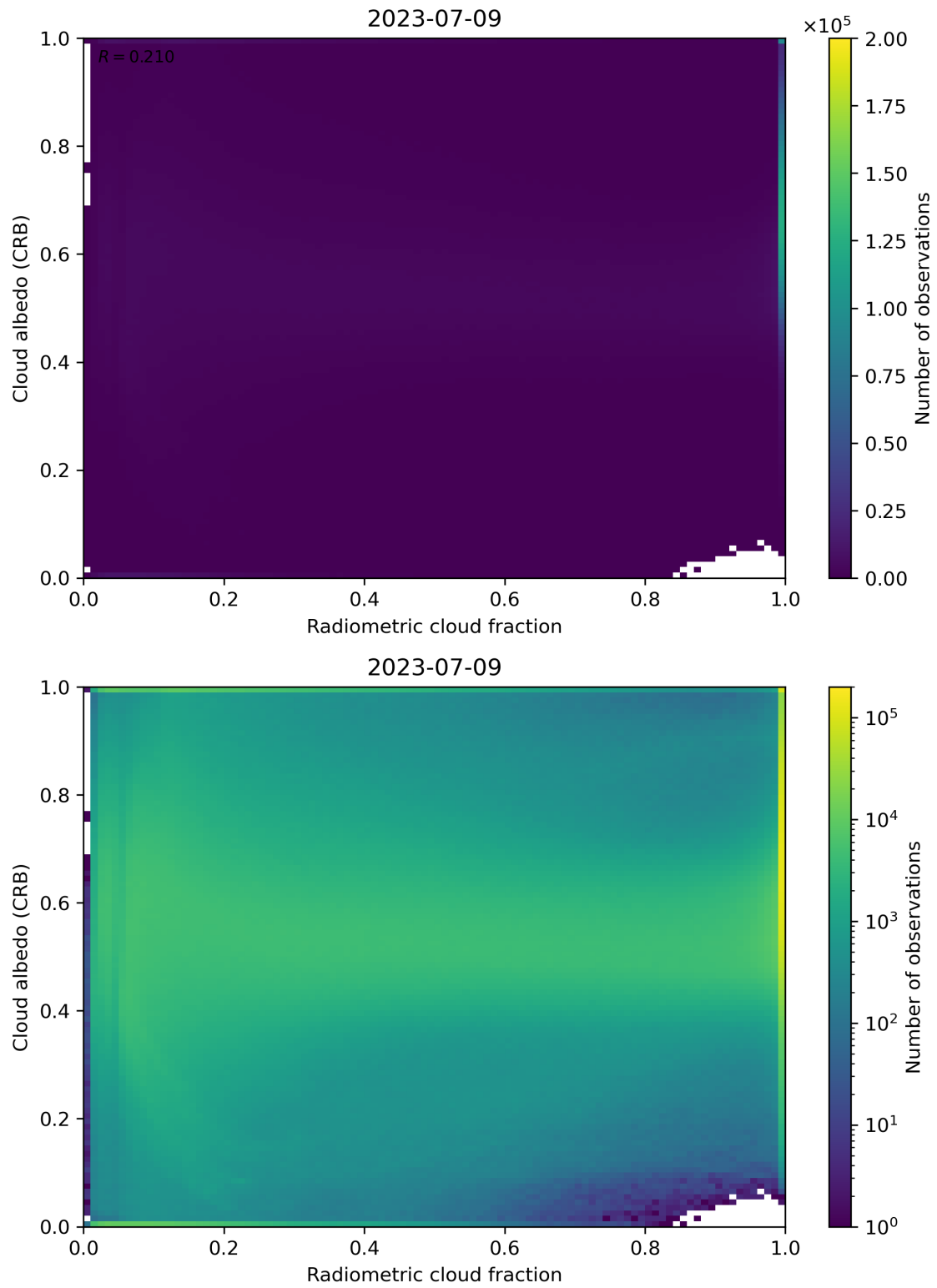
Figure 71: Scatter density plot of “Radiometric cloud fraction” against “Cloud albedo (CRB)” for 2023-07-08 to 2023-07-10.
