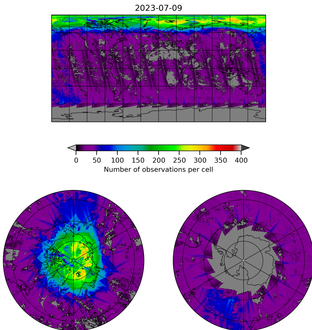
Figure 21: Map of the number of observations for 2023-07-08 to 2023-07-10
