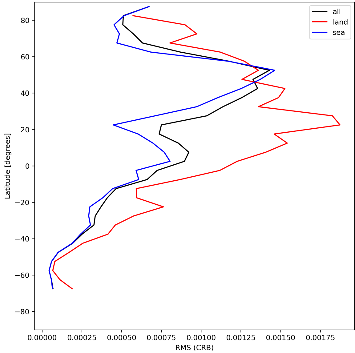
Figure 32: Zonal average of “RMS (CRB)” for 2023-07-08 to 2023-07-10.
