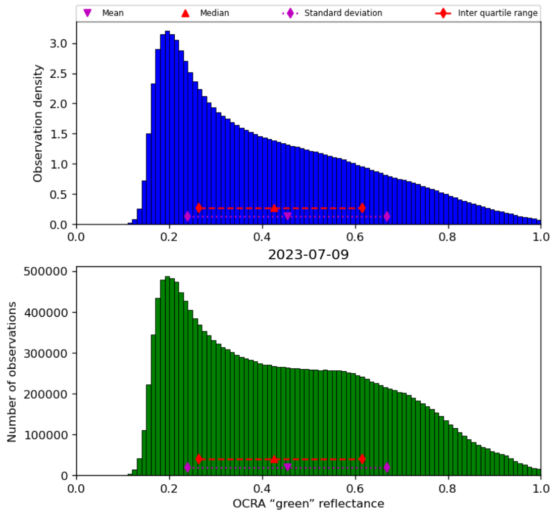
Figure 52: Histogram of “OCRA “green” reflectance” for 2023-07-08 to 2023-07-10
