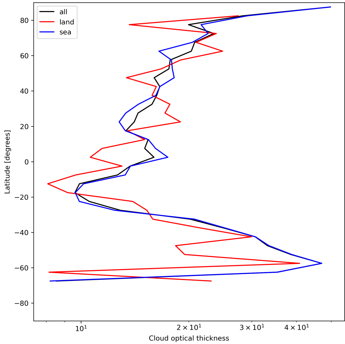
Figure 25: Zonal average of “Cloud optical thickness” for 2023-07-08 to 2023-07-10.
