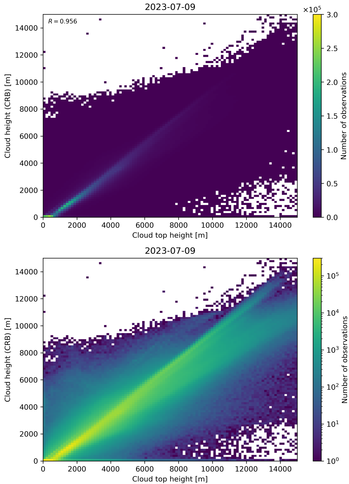
Figure 89: Scatter density plot of “Cloud top height” against “Cloud height (CRB)” for 2023-07-08 to 2023-07-10.
