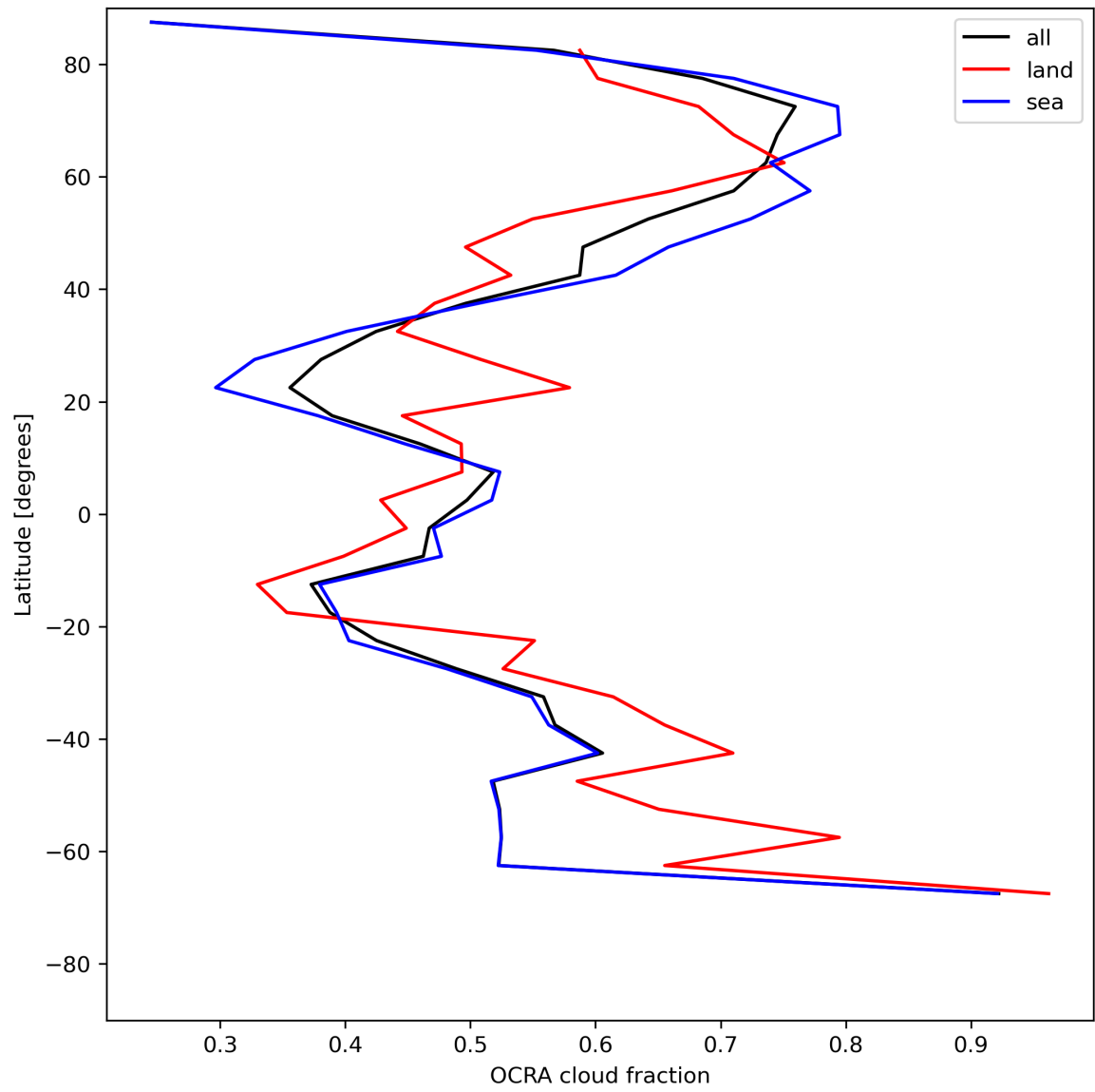
Figure 34: Zonal average of “OCRA cloud fraction” for 2023-07-08 to 2023-07-10.
