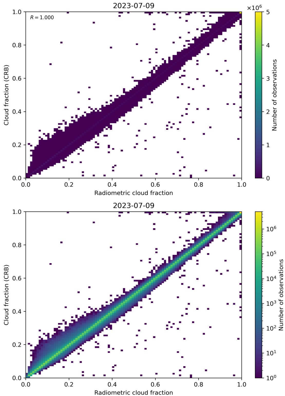
Figure 73: Scatter density plot of “Radiometric cloud fraction” against “Cloud fraction (CRB)” for 2023-07-08 to 2023-07-10.
