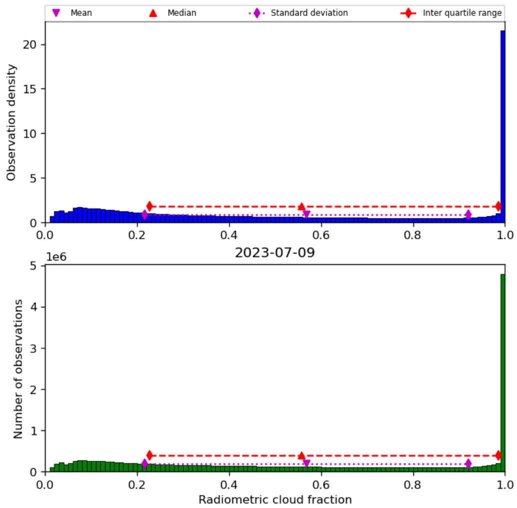
Figure 39: Histogram of “Radiometric cloud fraction” for 2023-07-08 to 2023-07-10
