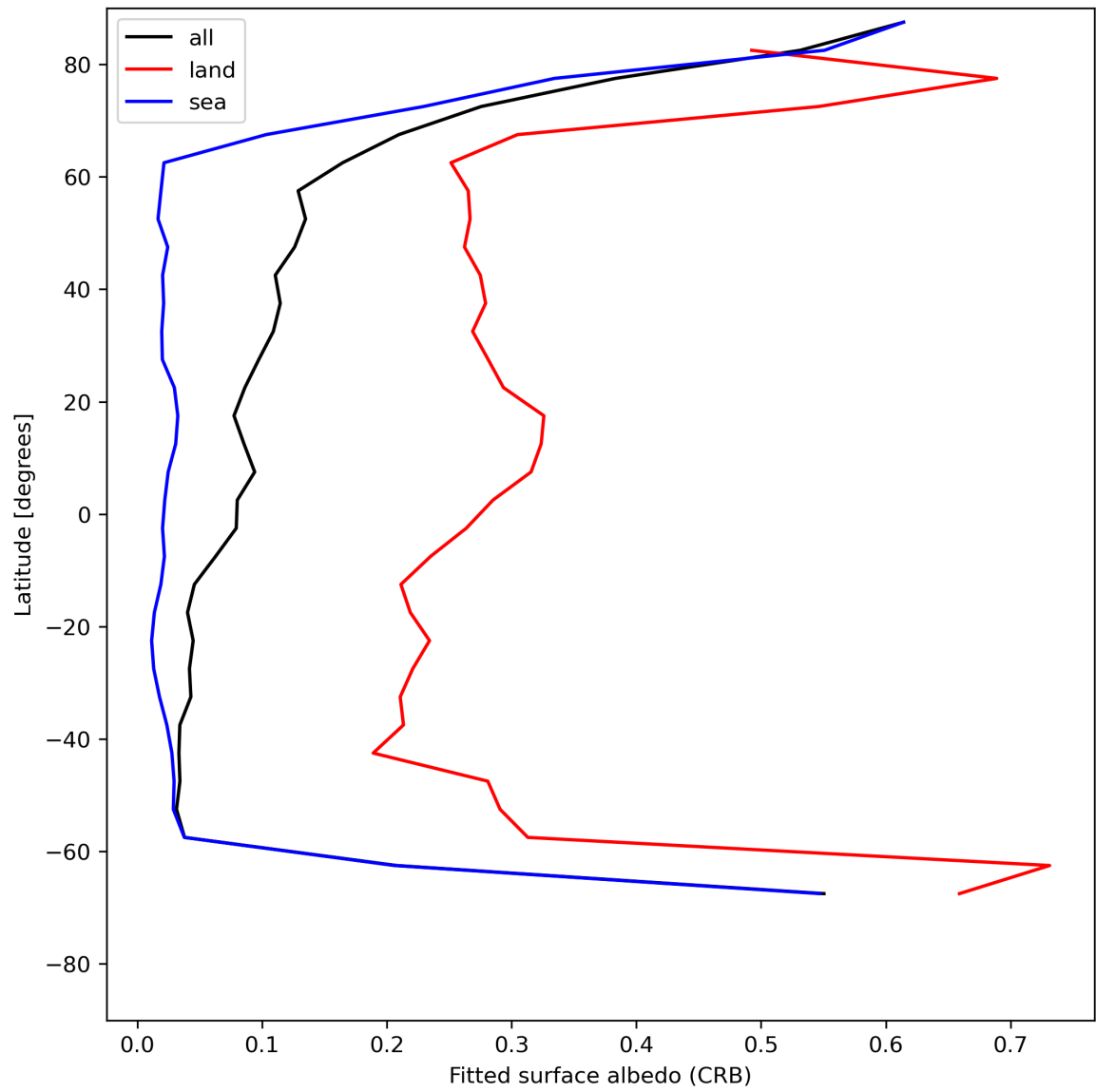
Figure 30: Zonal average of “Fitted surface albedo (CRB)” for 2023-07-08 to 2023-07-10.
