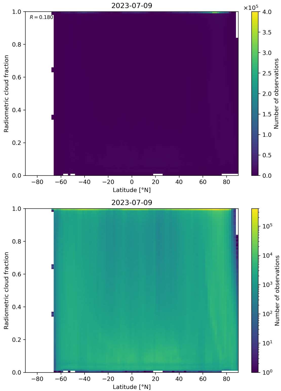
Figure 92: Scatter density plot of “Latitude” against “Radiometric cloud fraction” for 2023-07-08 to 2023-07-10.
