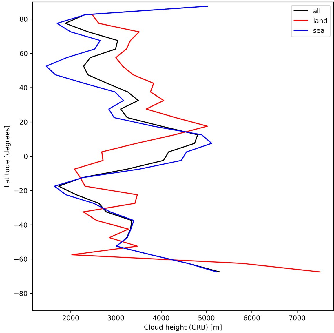
Figure 27: Zonal average of “Cloud height (CRB)” for 2023-07-08 to 2023-07-10.
