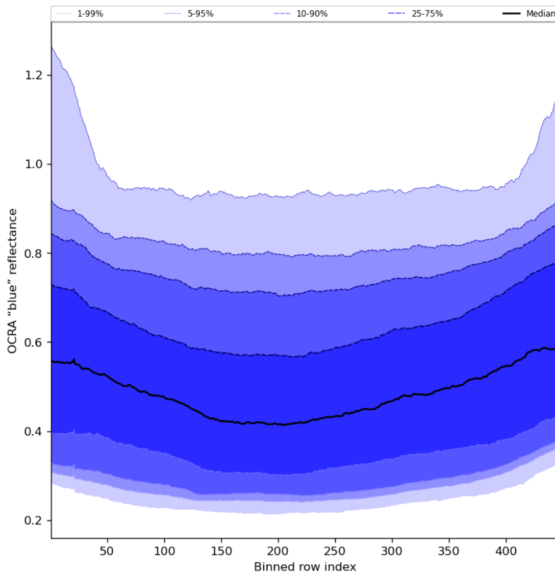
Figure 67: Along track statistics of “OCRA “blue” reflectance” for 2023-07-08 to 2023-07-10
