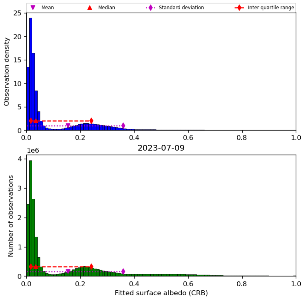
Figure 46: Histogram of “Fitted surface albedo (CRB)” for 2023-07-08 to 2023-07-10
