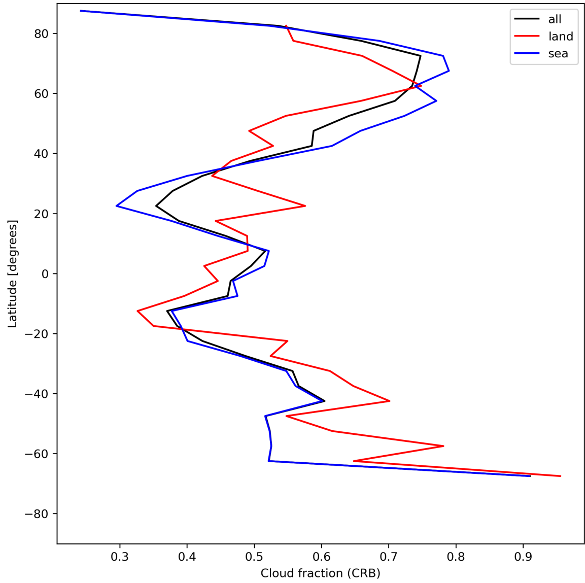
Figure 26: Zonal average of “Cloud fraction (CRB)” for 2023-07-08 to 2023-07-10.
