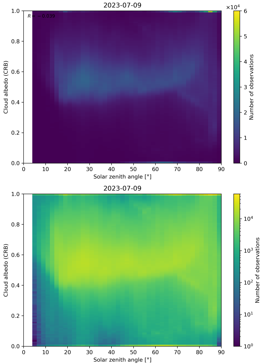
Figure 98: Scatter density plot of “Solar zenith angle” against “Cloud albedo (CRB)” for 2023-07-08 to 2023-07-10.
