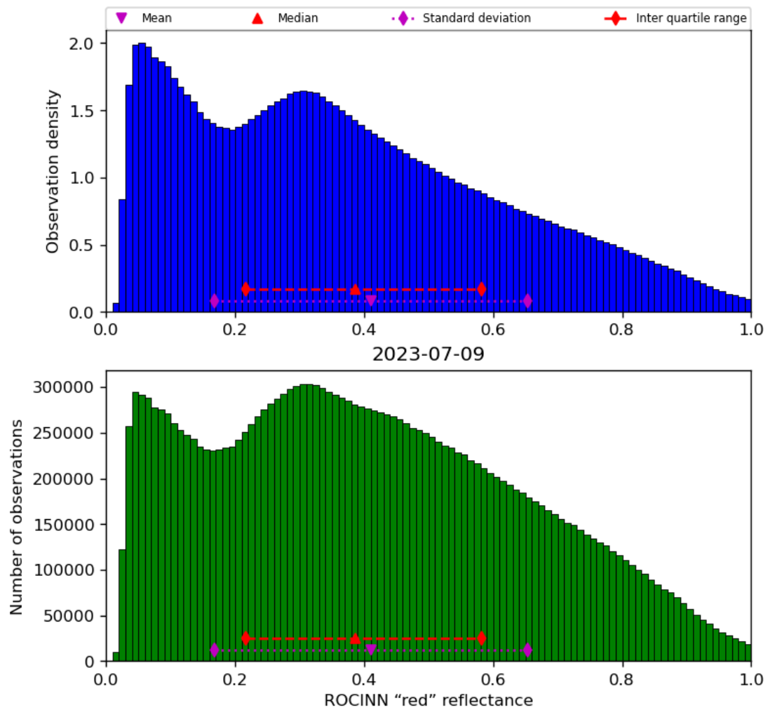
Figure 53: Histogram of “ROCINN “red” reflectance” for 2023-07-08 to 2023-07-10
