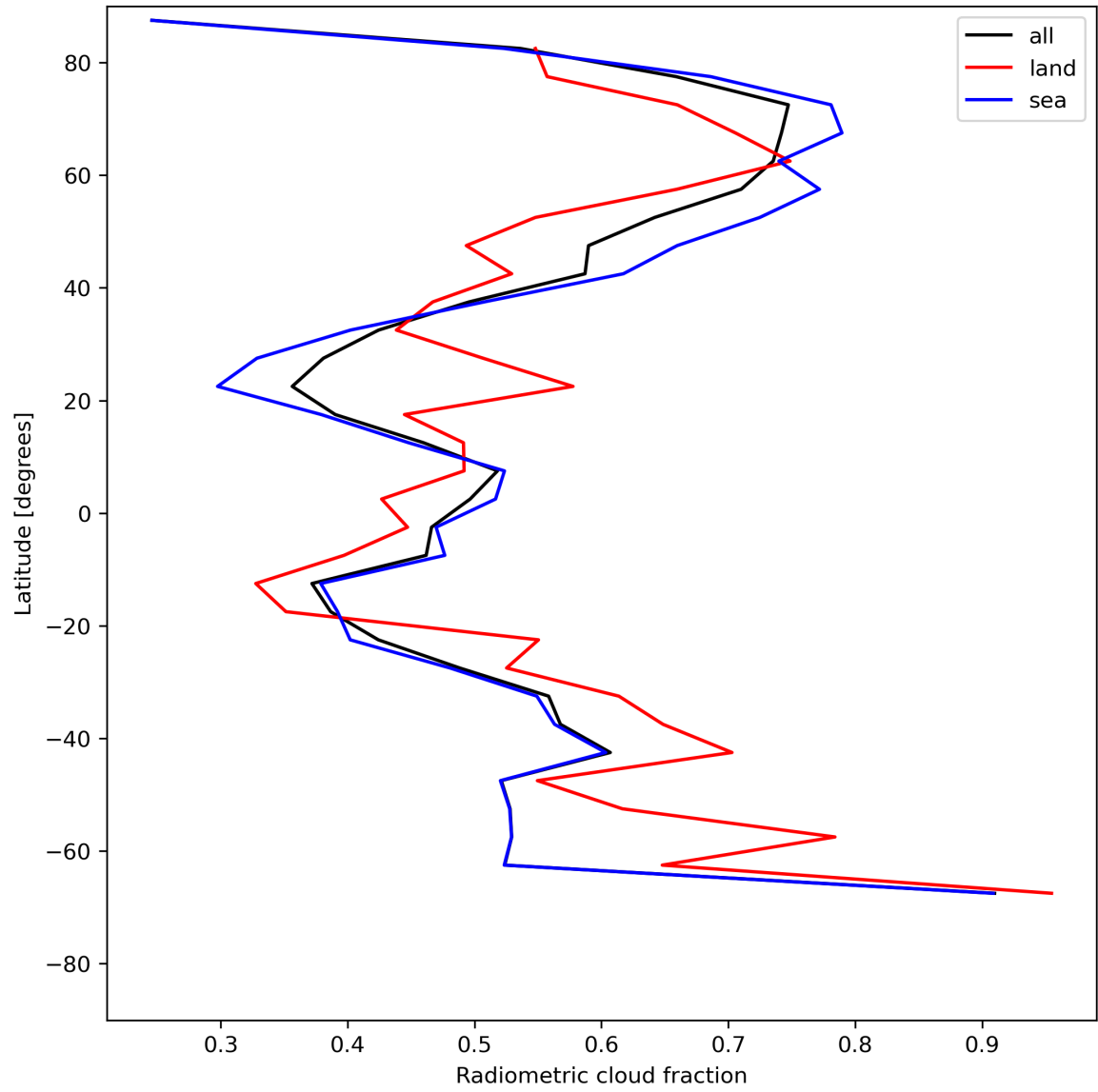
Figure 23: Zonal average of “Radiometric cloud fraction” for 2023-07-08 to 2023-07-10.
