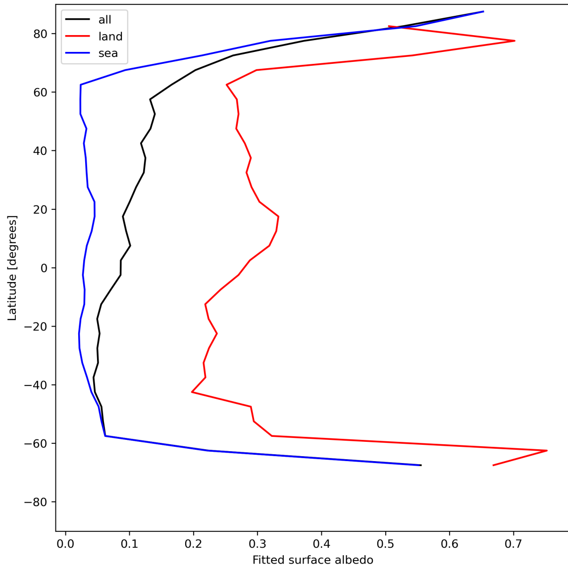
Figure 29: Zonal average of “Fitted surface albedo” for 2023-07-08 to 2023-07-10.
