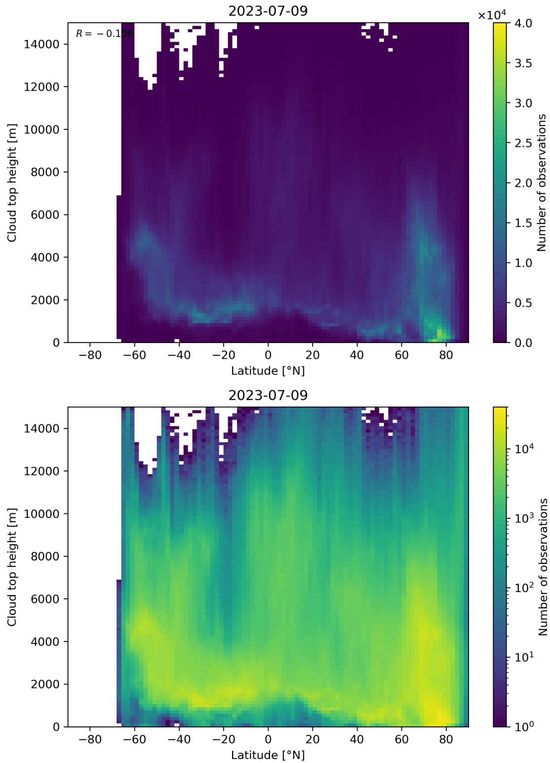
Figure 97: Scatter density plot of “Latitude” against “Cloud top height” for 2023-07-08 to 2023-07-10.
