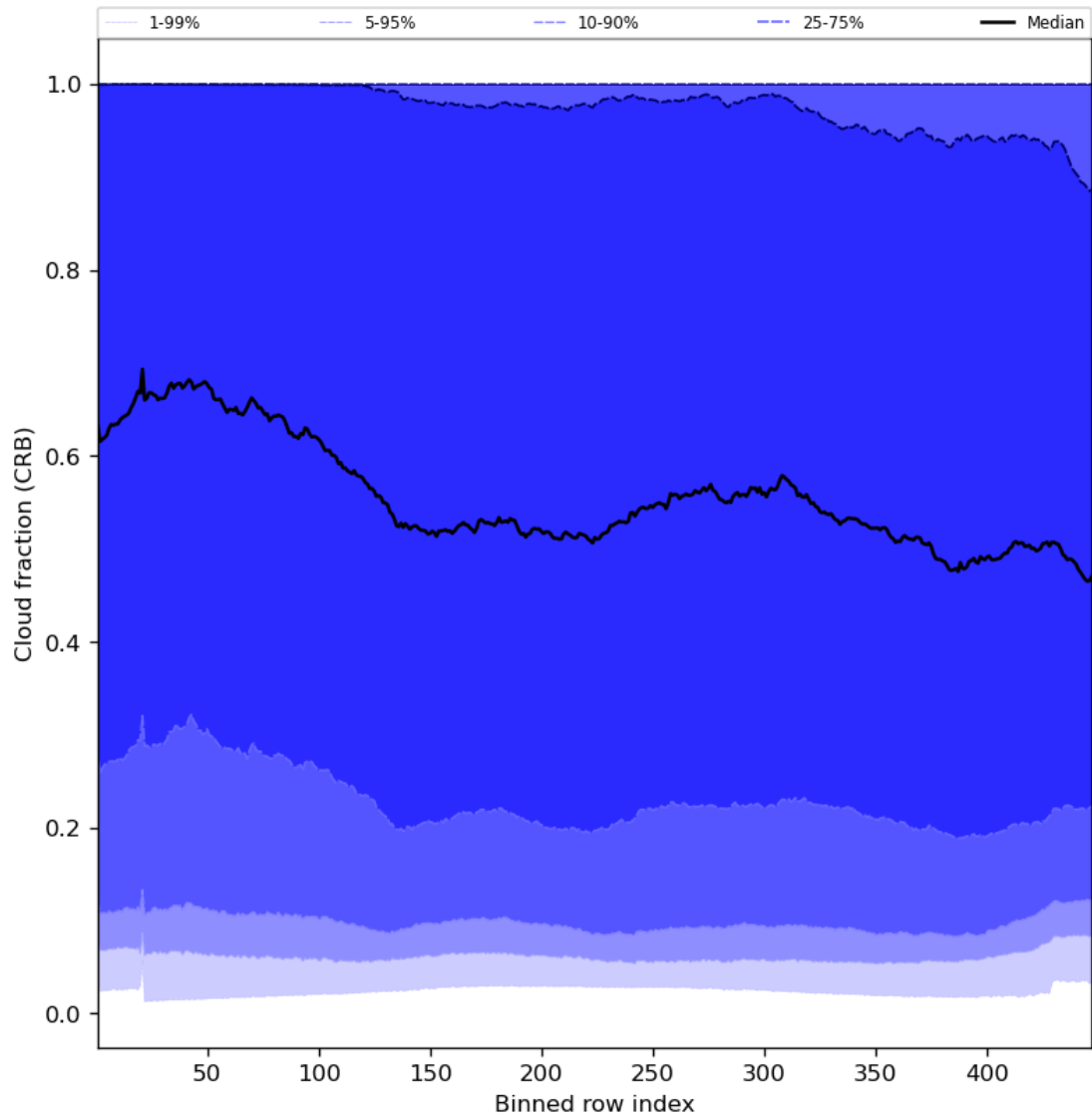
Figure 58: Along track statistics of “Cloud fraction (CRB)” for 2023-07-08 to 2023-07-10
