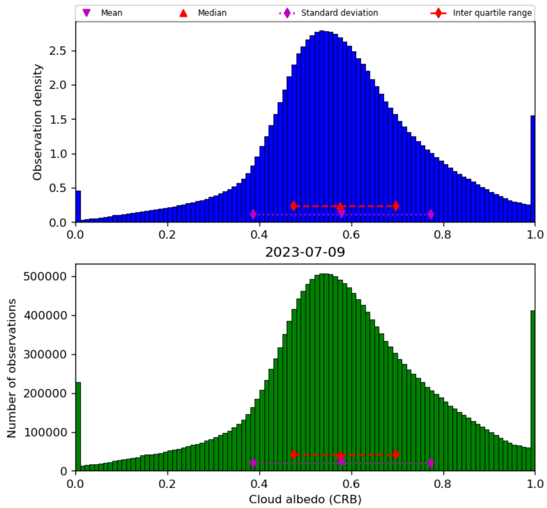
Figure 44: Histogram of “Cloud albedo (CRB)” for 2023-07-08 to 2023-07-10
