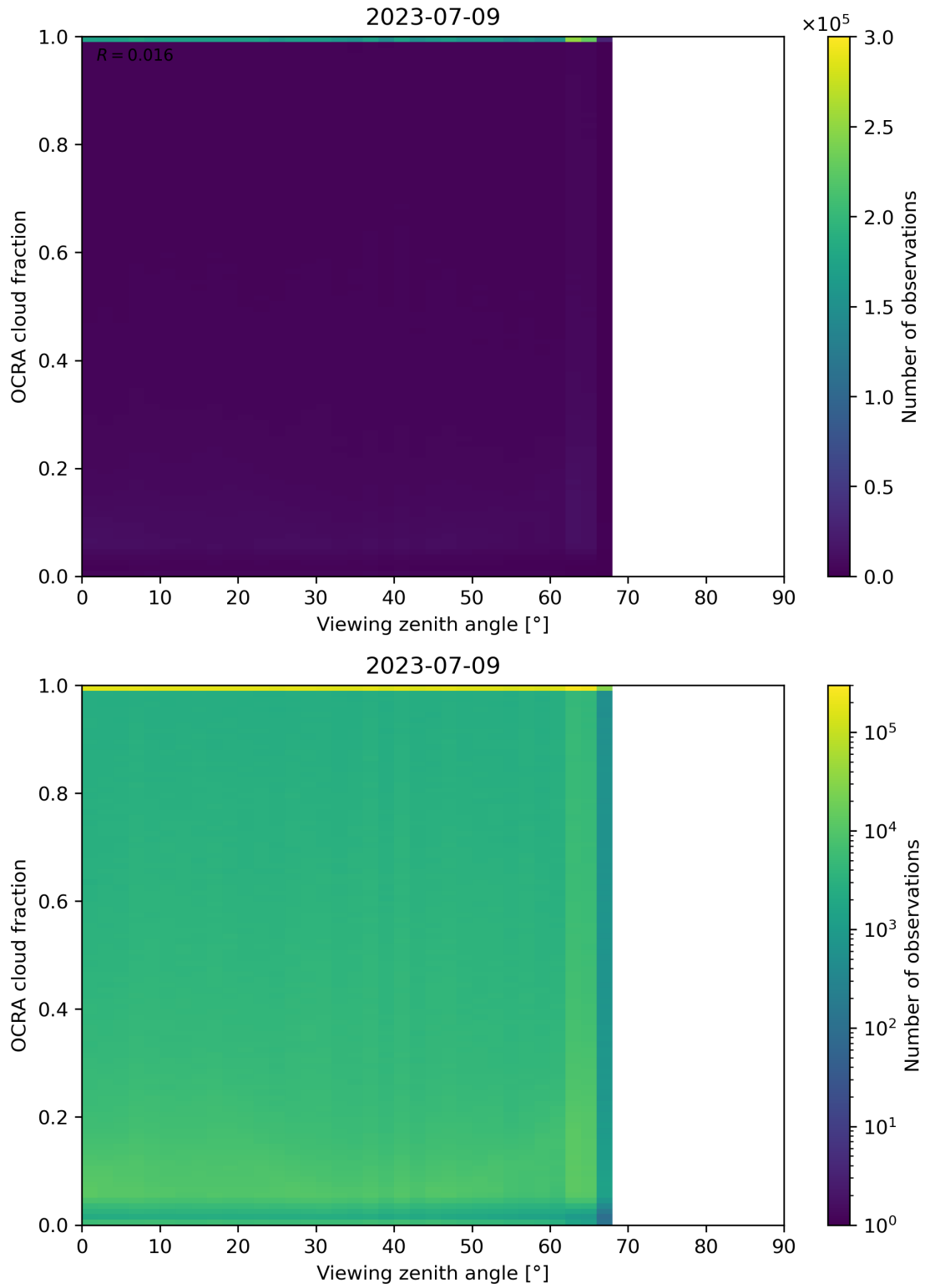
Figure 108: Scatter density plot of “Viewing zenith angle” against “OCRA cloud fraction” for 2023-07-08 to 2023-07-10.
