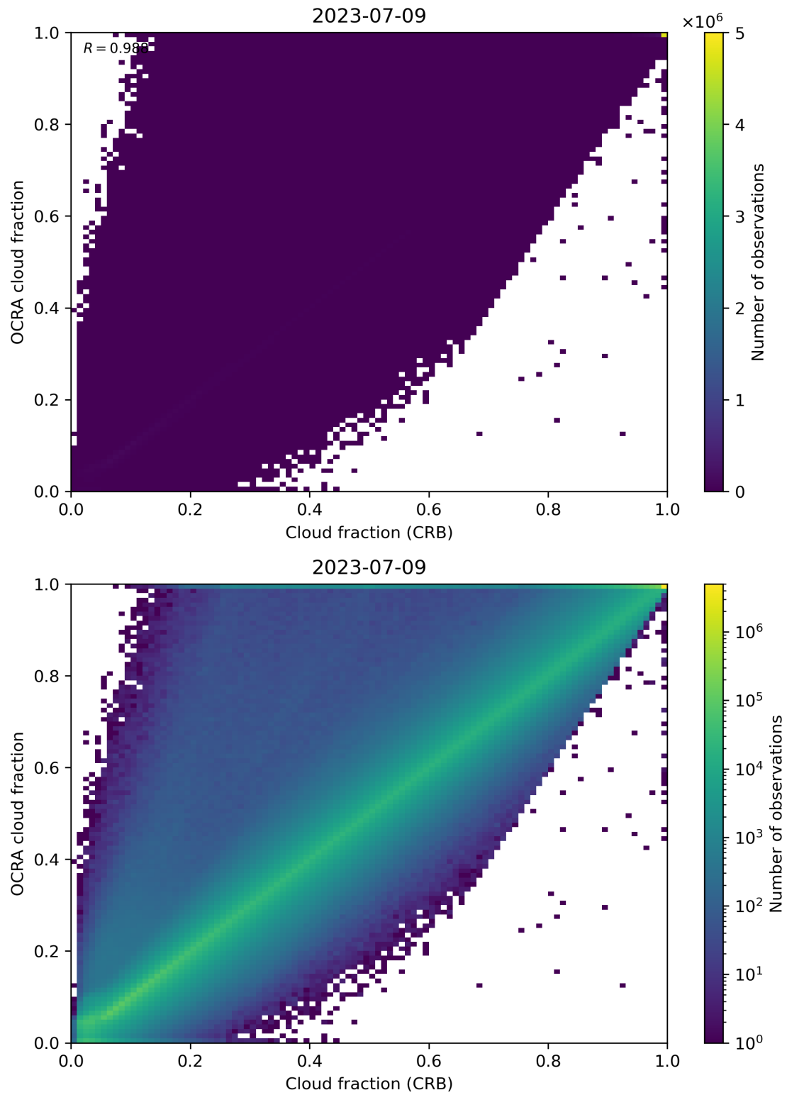
Figure 78: Scatter density plot of “Cloud fraction (CRB)” against “OCRA cloud fraction” for 2023-07-08 to 2023-07-10.
