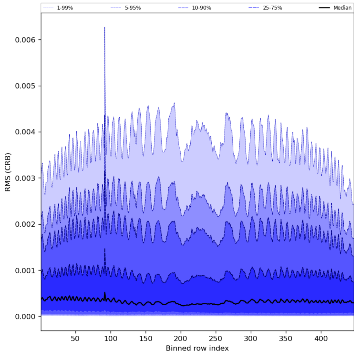
Figure 64: Along track statistics of “RMS (CRB)” for 2023-07-08 to 2023-07-10
