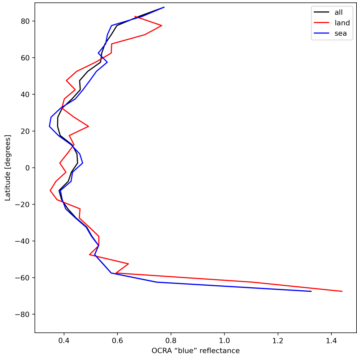
Figure 35: Zonal average of “OCRA “blue” reflectance” for 2023-07-08 to 2023-07-10.
