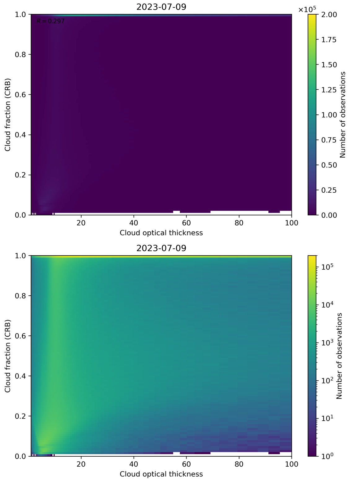
Figure 84: Scatter density plot of “Cloud optical thickness” against “Cloud fraction (CRB)” for 2023-07-08 to 2023-07-10.
