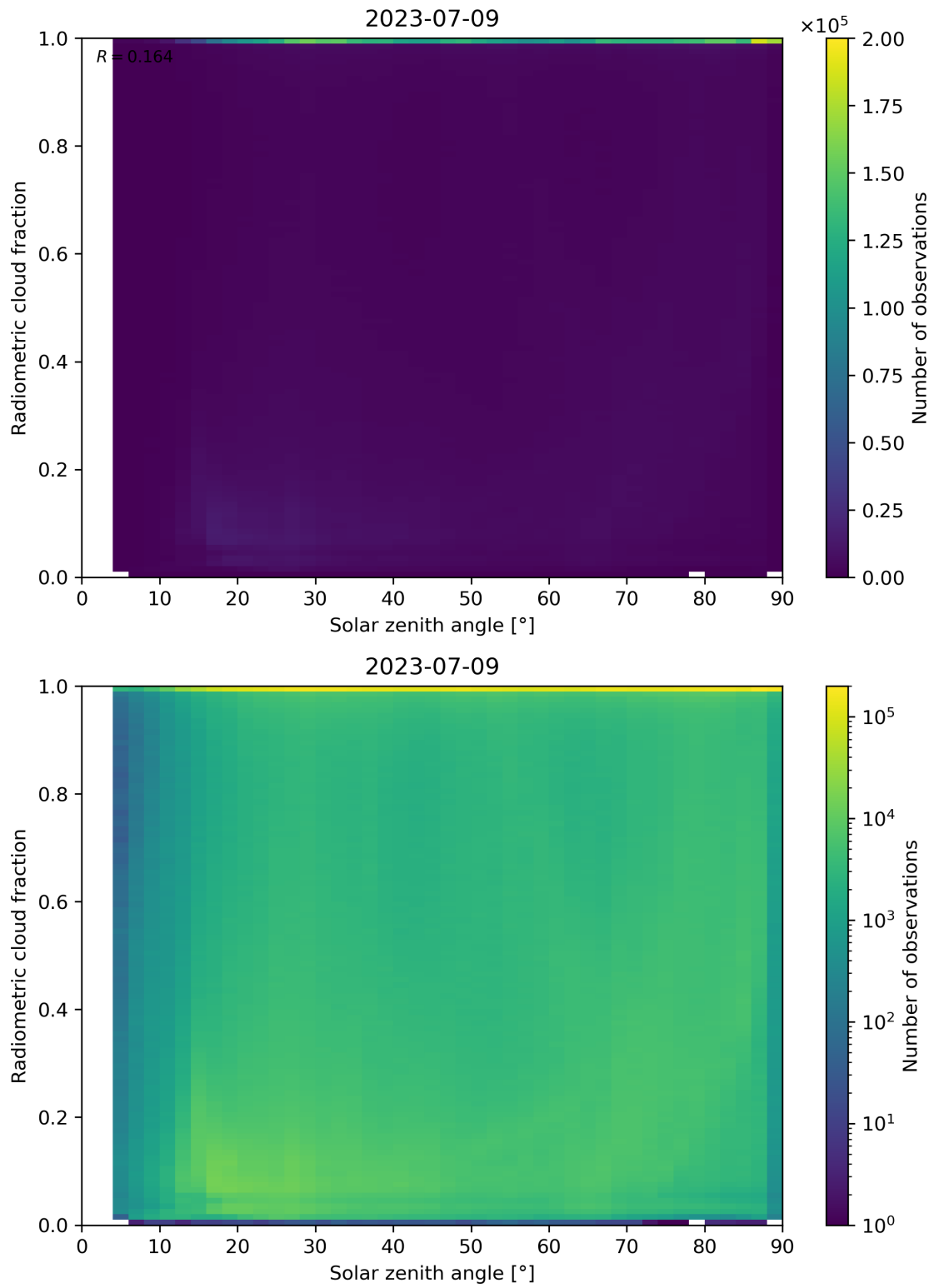
Figure 99: Scatter density plot of “Solar zenith angle” against “Radiometric cloud fraction” for 2023-07-08 to 2023-07-10.
