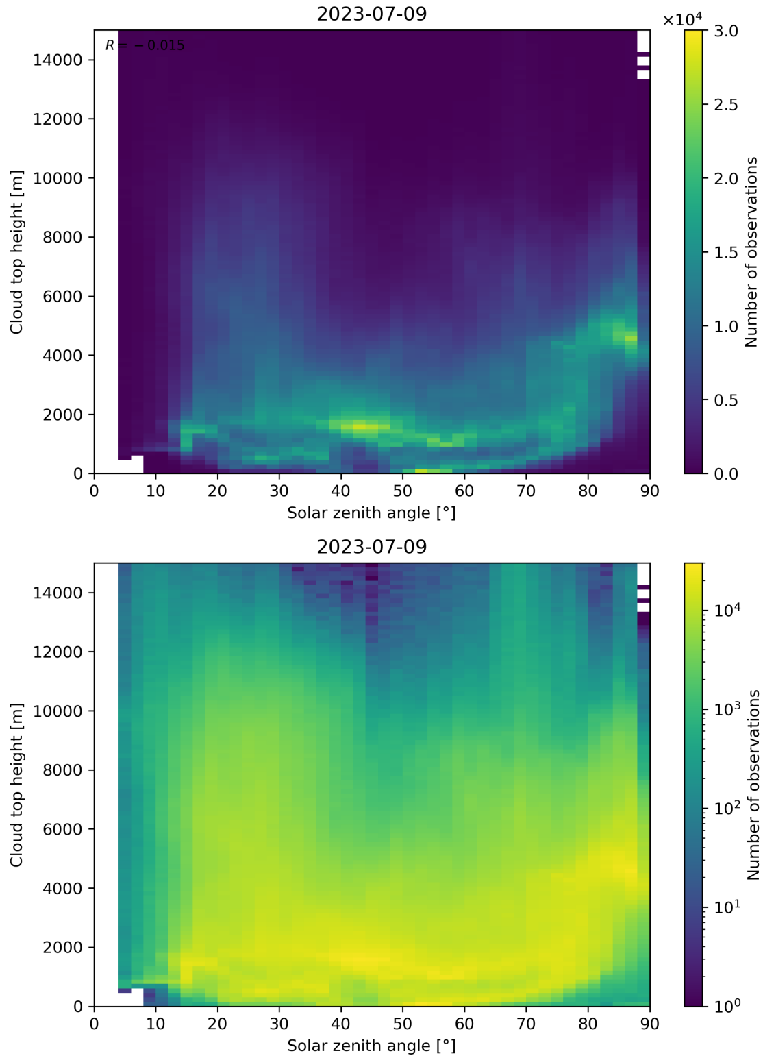
Figure 104: Scatter density plot of “Solar zenith angle” against “Cloud top height” for 2023-07-08 to 2023-07-10.
