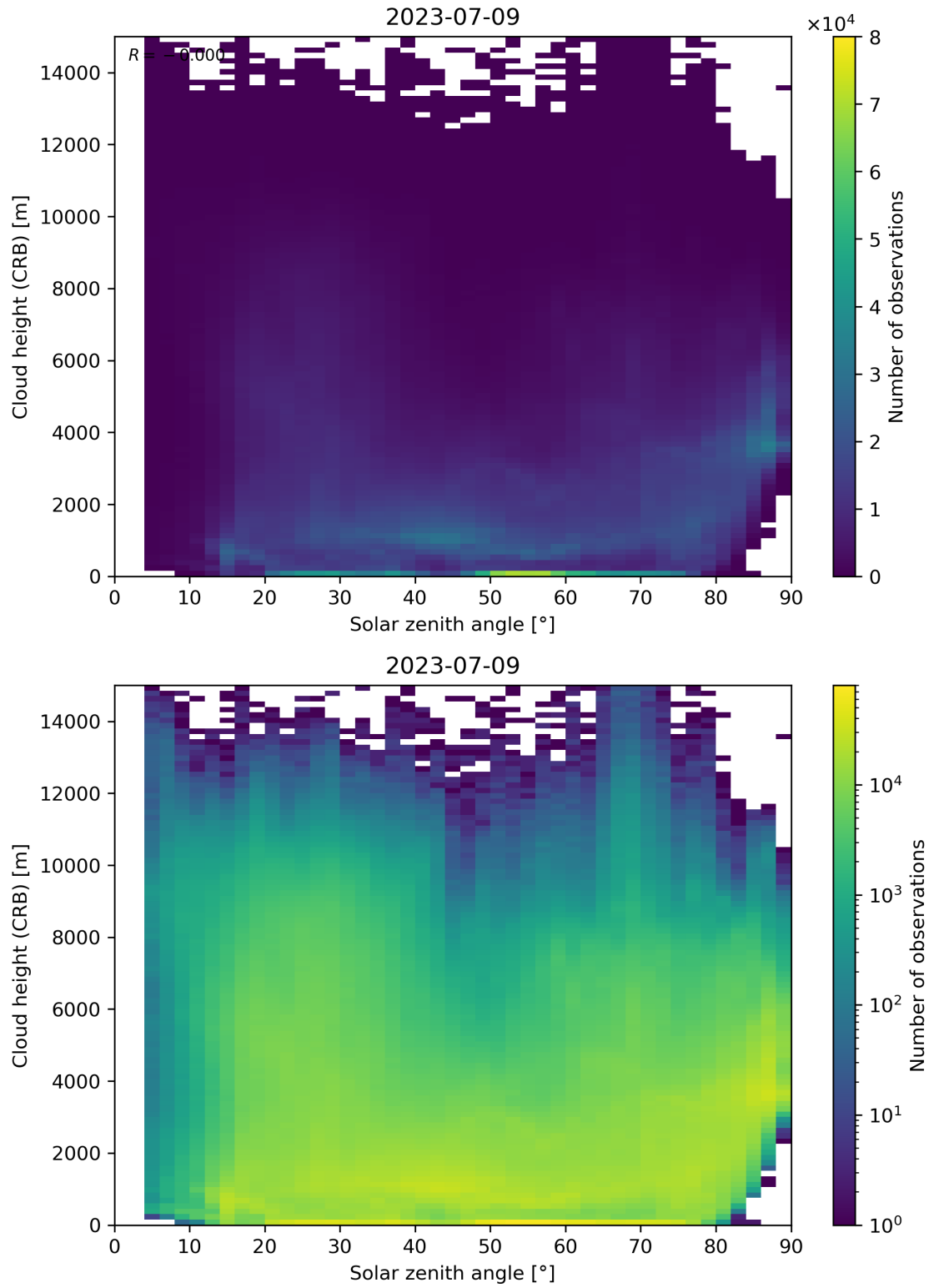
Figure 102: Scatter density plot of “Solar zenith angle” against “Cloud height (CRB)” for 2023-07-08 to 2023-07-10.
