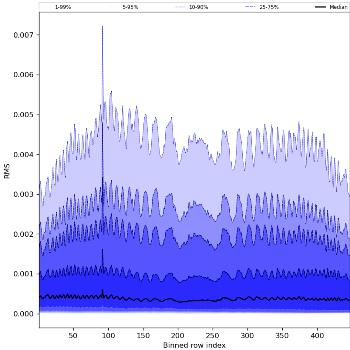
Figure 63: Along track statistics of “RMS” for 2023-07-08 to 2023-07-10
