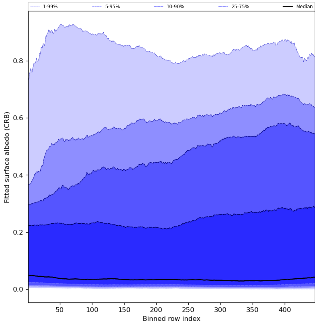
Figure 62: Along track statistics of “Fitted surface albedo (CRB)” for 2023-07-08 to 2023-07-10
