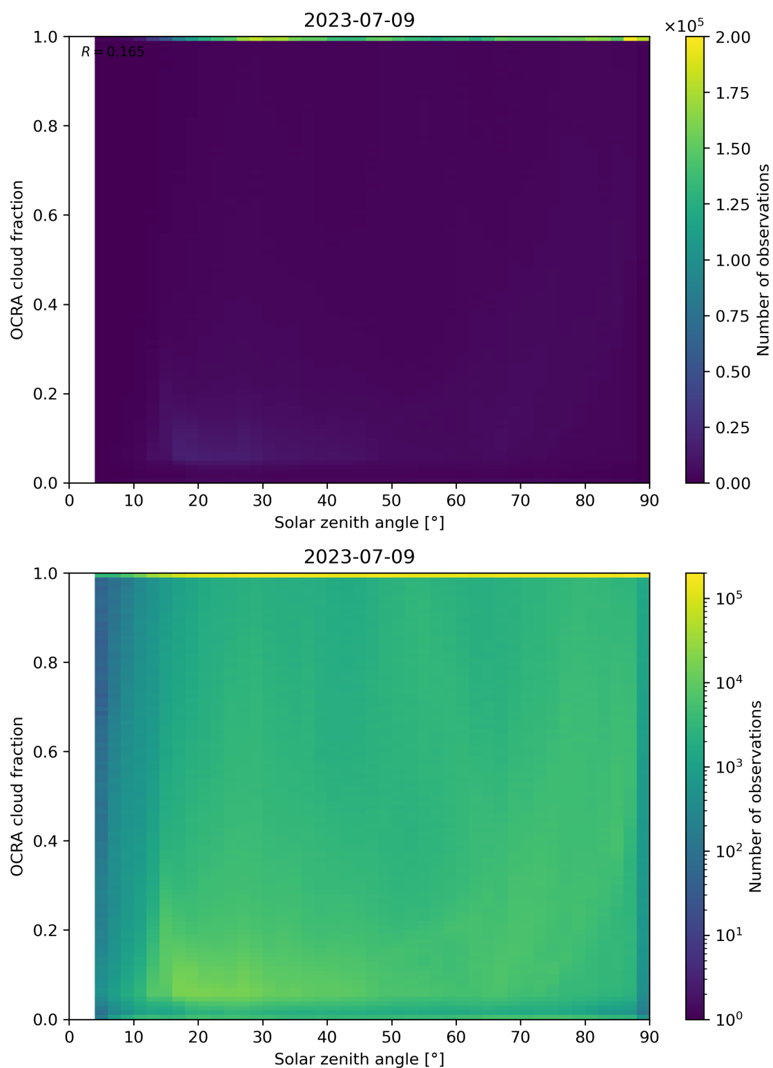
Figure 100: Scatter density plot of “Solar zenith angle” against “OCRA cloud fraction” for 2023-07-08 to 2023-07-10.
