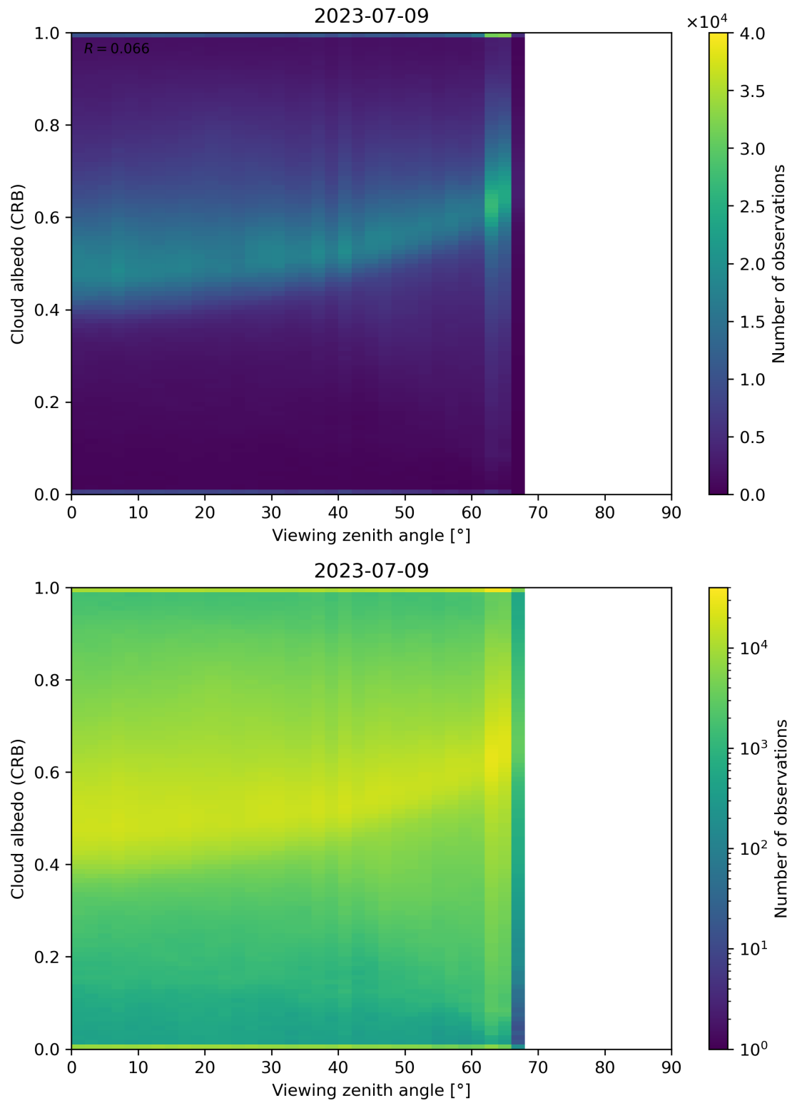
Figure 106: Scatter density plot of “Viewing zenith angle” against “Cloud albedo (CRB)” for 2023-07-08 to 2023-07-10.
