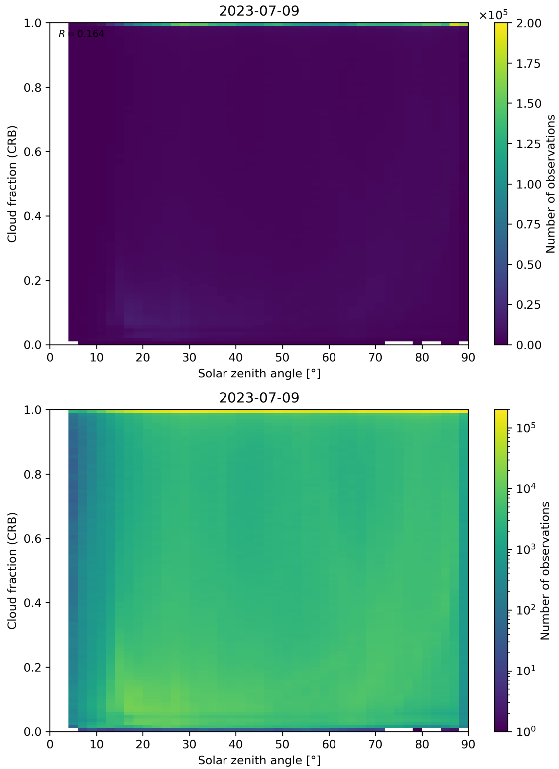
Figure 101: Scatter density plot of “Solar zenith angle” against “Cloud fraction (CRB)” for 2023-07-08 to 2023-07-10.
