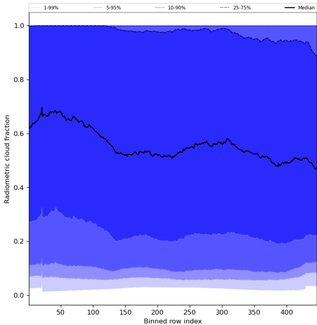
Figure 55: Along track statistics of “Radiometric cloud fraction” for 2023-07-08 to 2023-07-10
