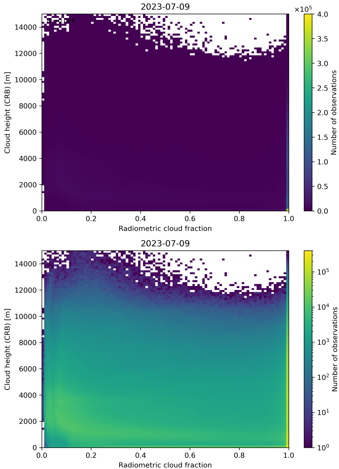
Figure 74: Scatter density plot of “Radiometric cloud fraction” against “Cloud height (CRB)” for 2023-07-08 to 2023-07-10.
