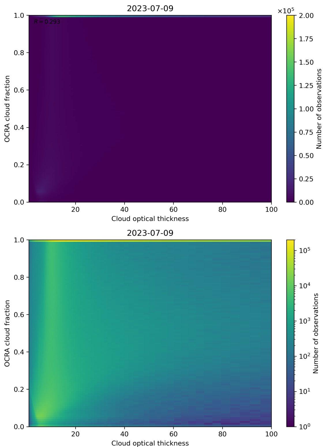
Figure 83: Scatter density plot of “Cloud optical thickness” against “OCRA cloud fraction” for 2023-07-08 to 2023-07-10.
