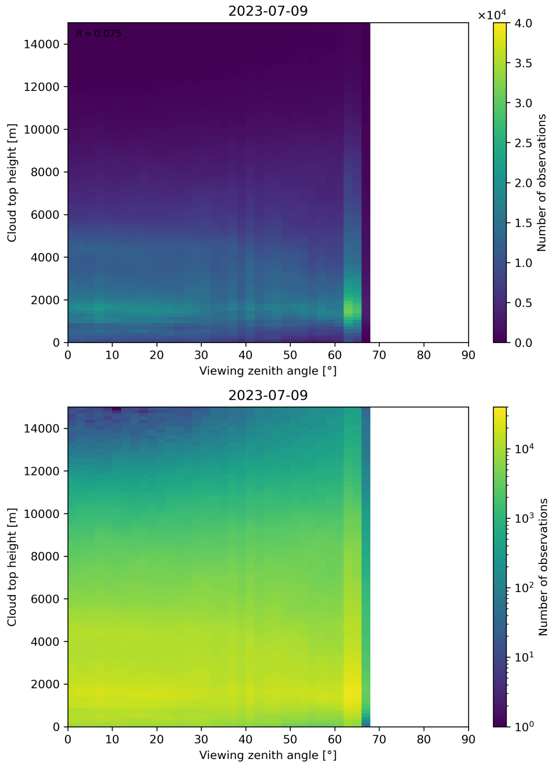
Figure 112: Scatter density plot of “Viewing zenith angle” against “Cloud top height” for 2023-07-08 to 2023-07-10.
