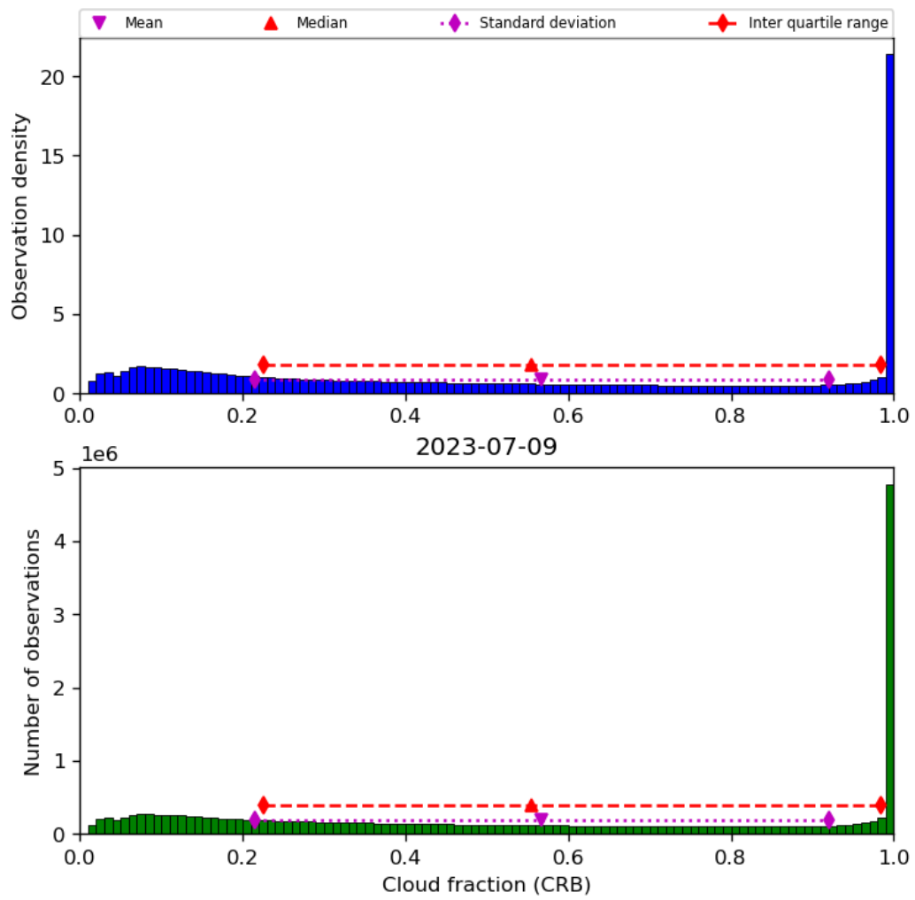
Figure 42: Histogram of “Cloud fraction (CRB)” for 2023-07-08 to 2023-07-10
