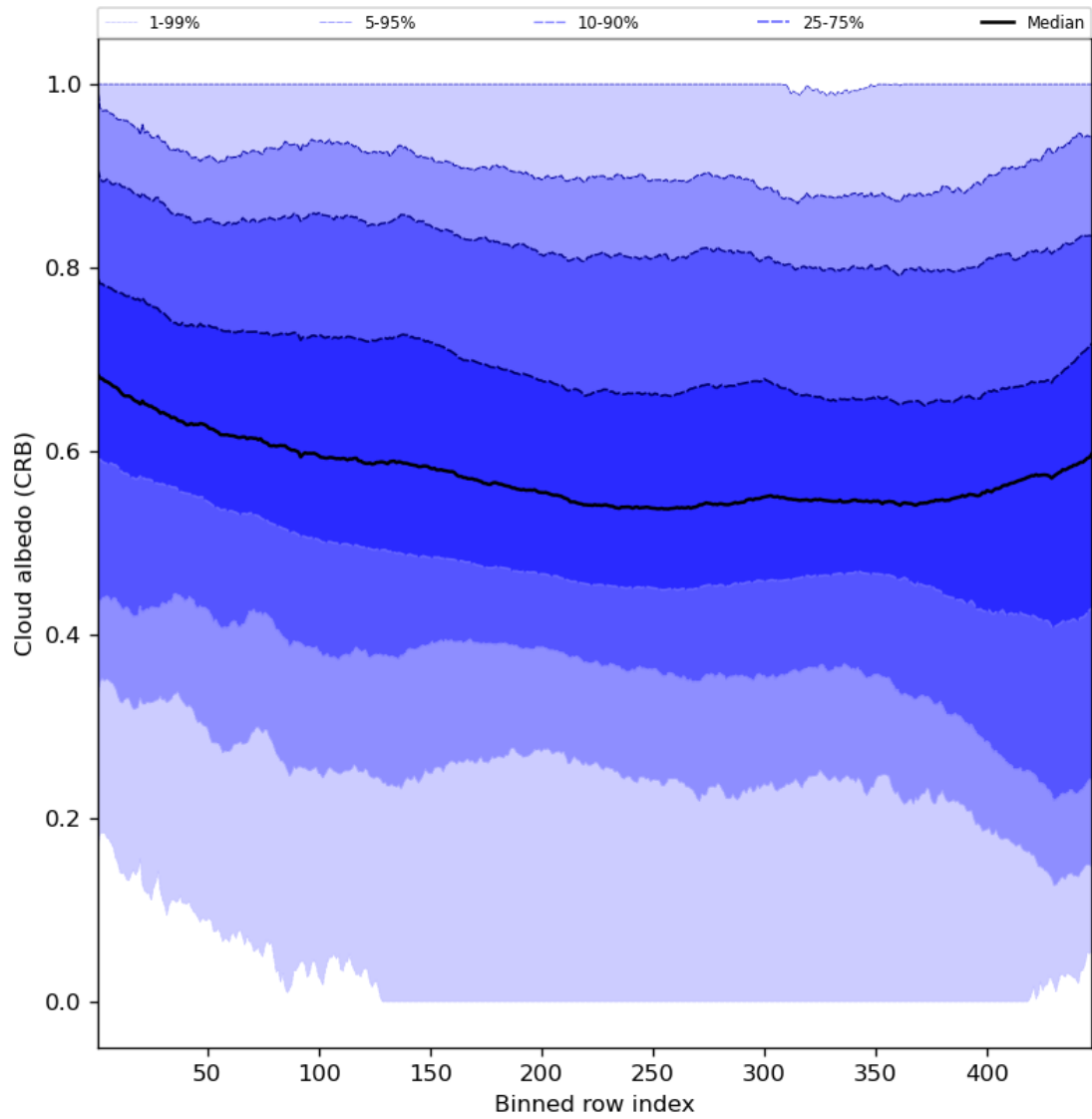
Figure 60: Along track statistics of “Cloud albedo (CRB)” for 2023-07-08 to 2023-07-10
