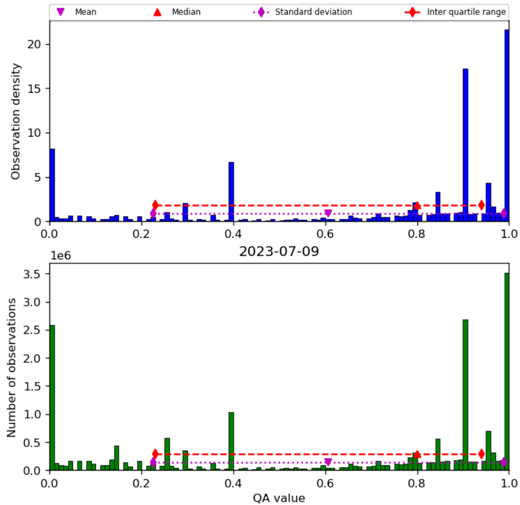
Figure 38: Histogram of “QA value” for 2023-07-08 to 2023-07-10
