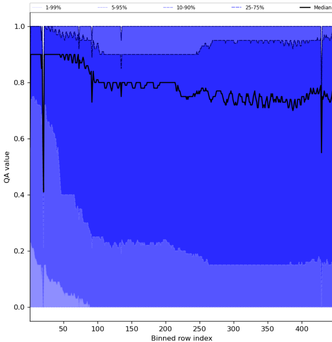
Figure 54: Along track statistics of “QA value” for 2023-07-08 to 2023-07-10
