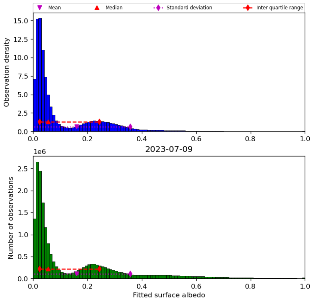
Figure 45: Histogram of “Fitted surface albedo” for 2023-07-08 to 2023-07-10
