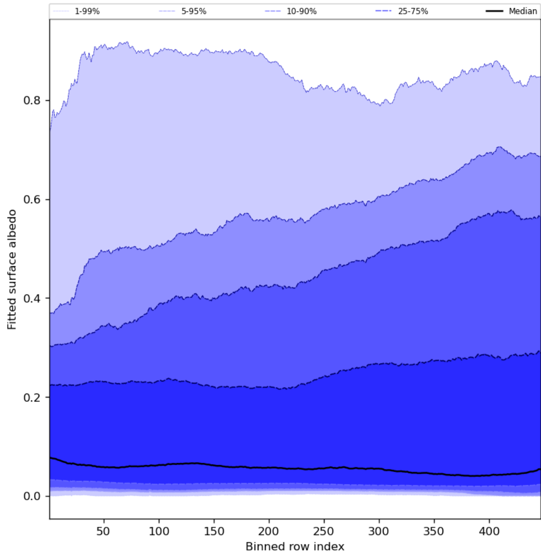
Figure 61: Along track statistics of “Fitted surface albedo” for 2023-07-08 to 2023-07-10
