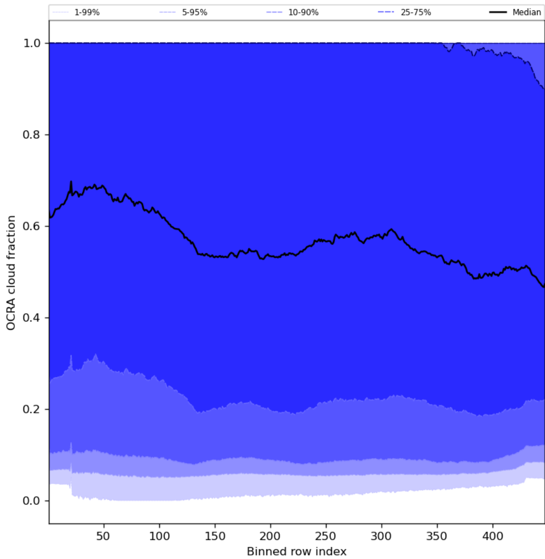
Figure 66: Along track statistics of “OCRA cloud fraction” for 2023-07-08 to 2023-07-10
