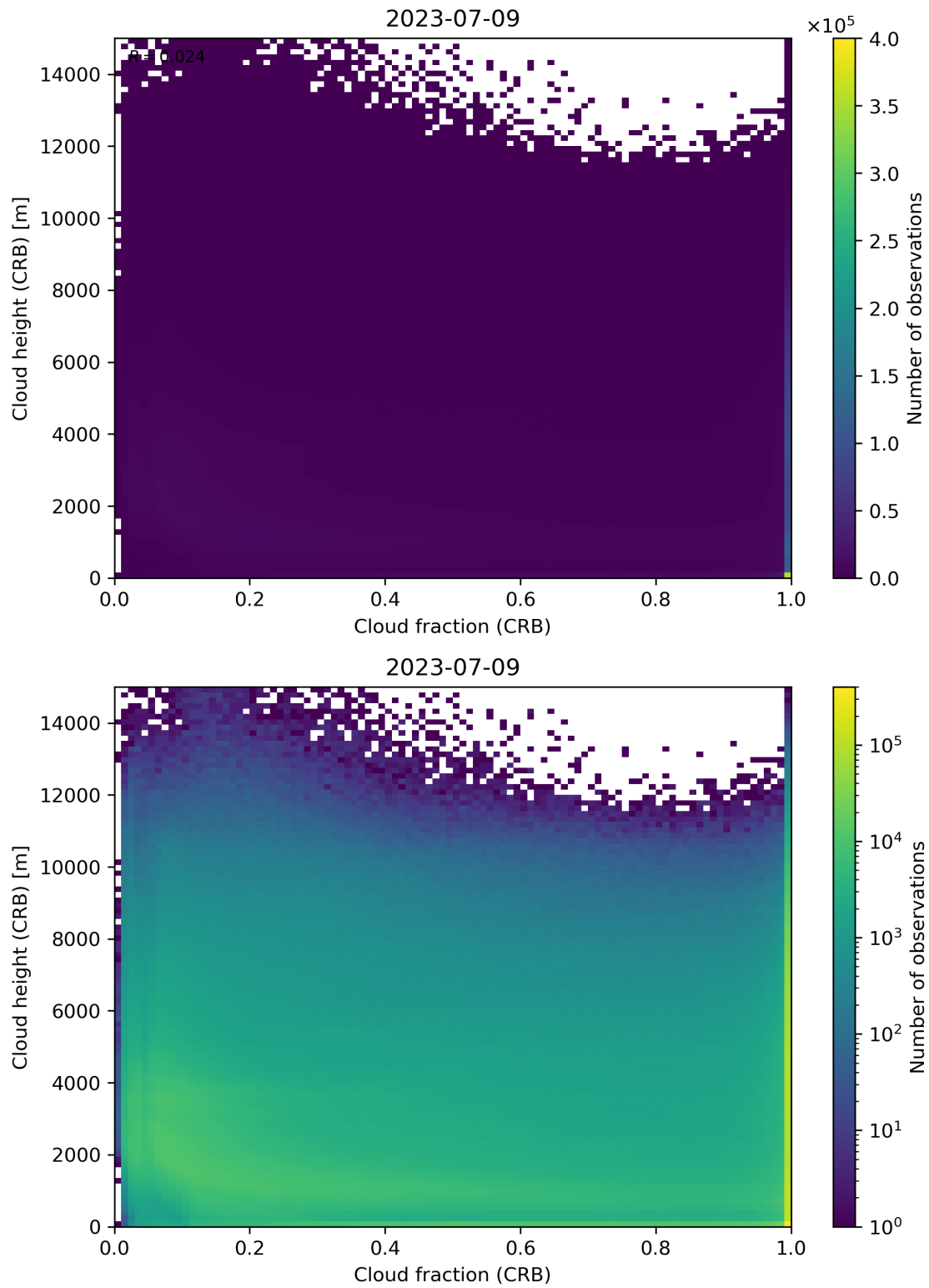
Figure 79: Scatter density plot of “Cloud fraction (CRB)” against “Cloud height (CRB)” for 2023-07-08 to 2023-07-10.
