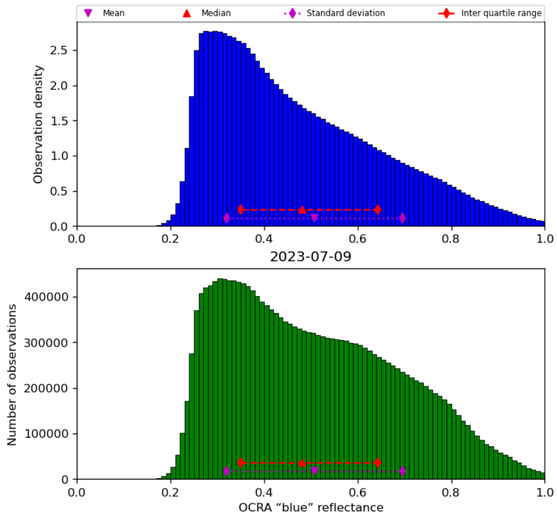
Figure 51: Histogram of “OCRA “blue” reflectance” for 2023-07-08 to 2023-07-10
