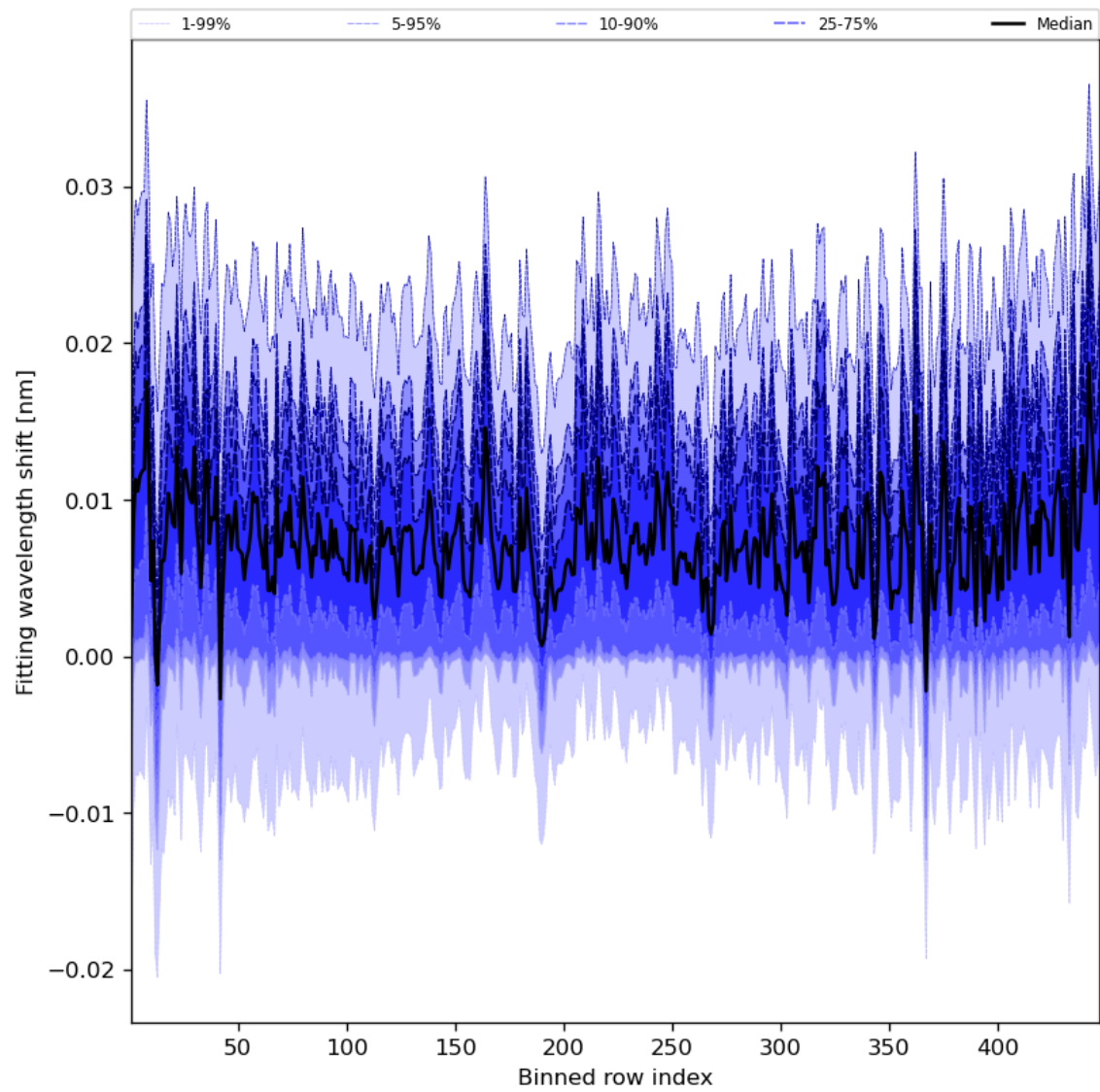
Figure 65: Along track statistics of “Fitting wavelength shift” for 2023-07-08 to 2023-07-10
