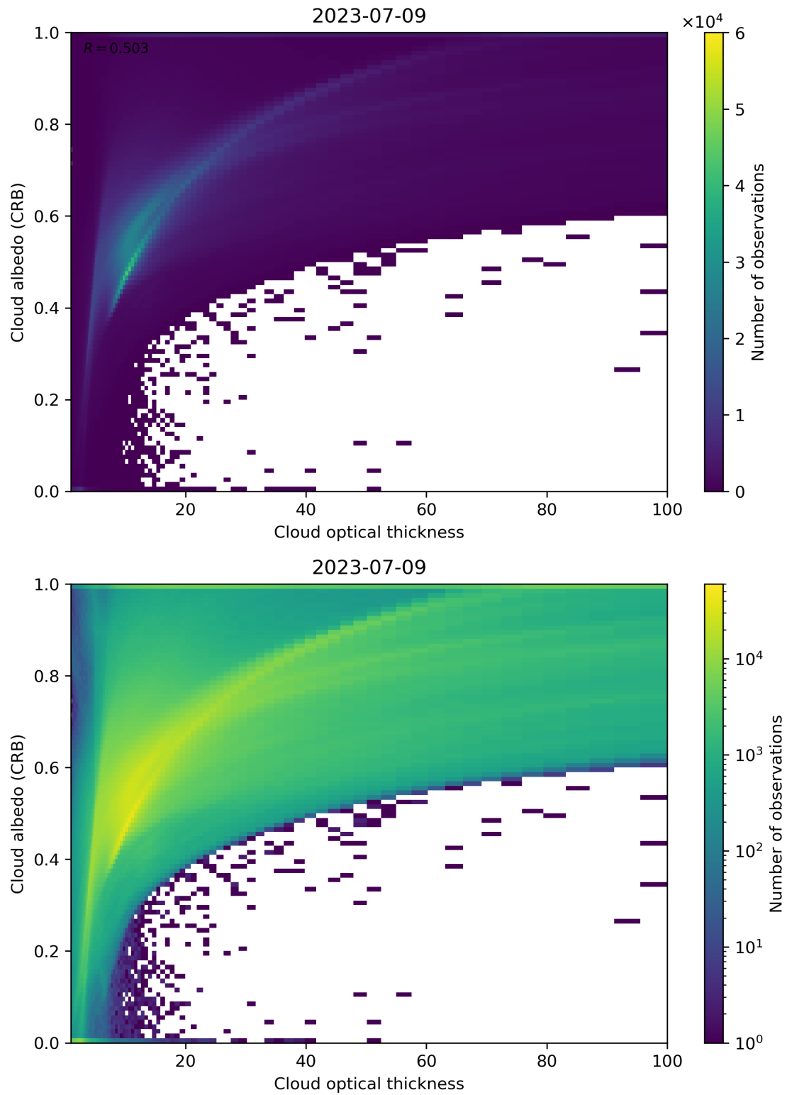
Figure 82: Scatter density plot of “Cloud optical thickness” against “Cloud albedo (CRB)” for 2023-07-08 to 2023-07-10.
