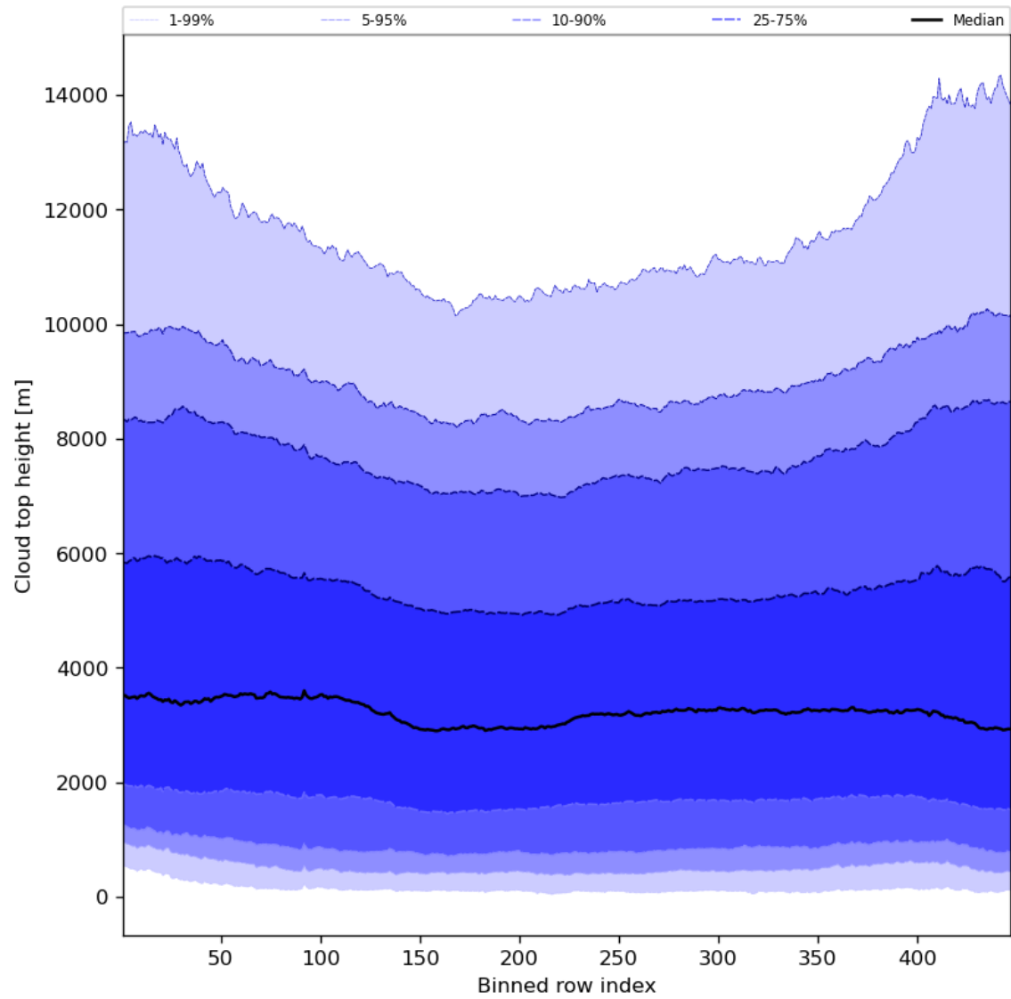
Figure 56: Along track statistics of “Cloud top height” for 2023-07-08 to 2023-07-10
