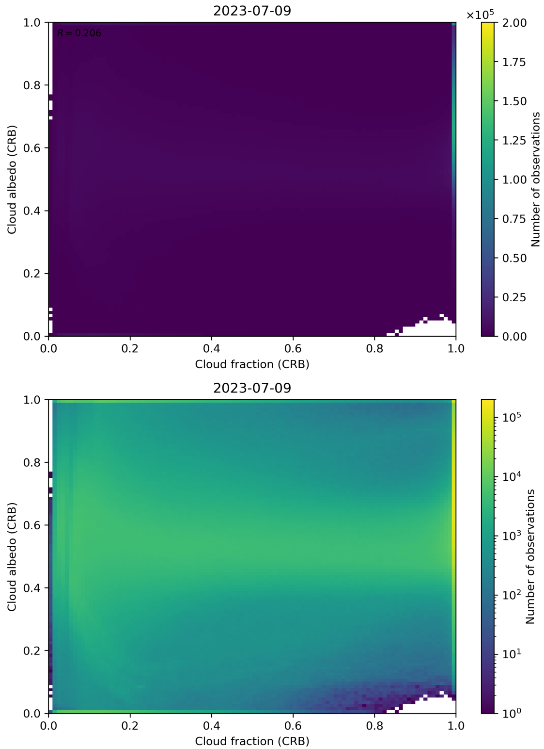
Figure 77: Scatter density plot of “Cloud fraction (CRB)” against “Cloud albedo (CRB)” for 2023-07-08 to 2023-07-10.
