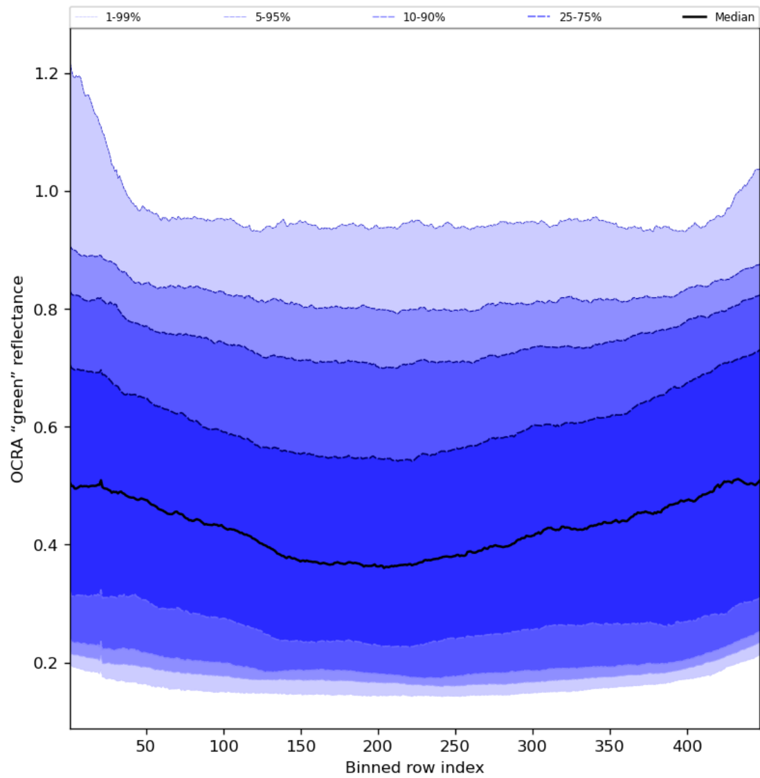
Figure 68: Along track statistics of “OCRA “green” reflectance” for 2023-07-08 to 2023-07-10
