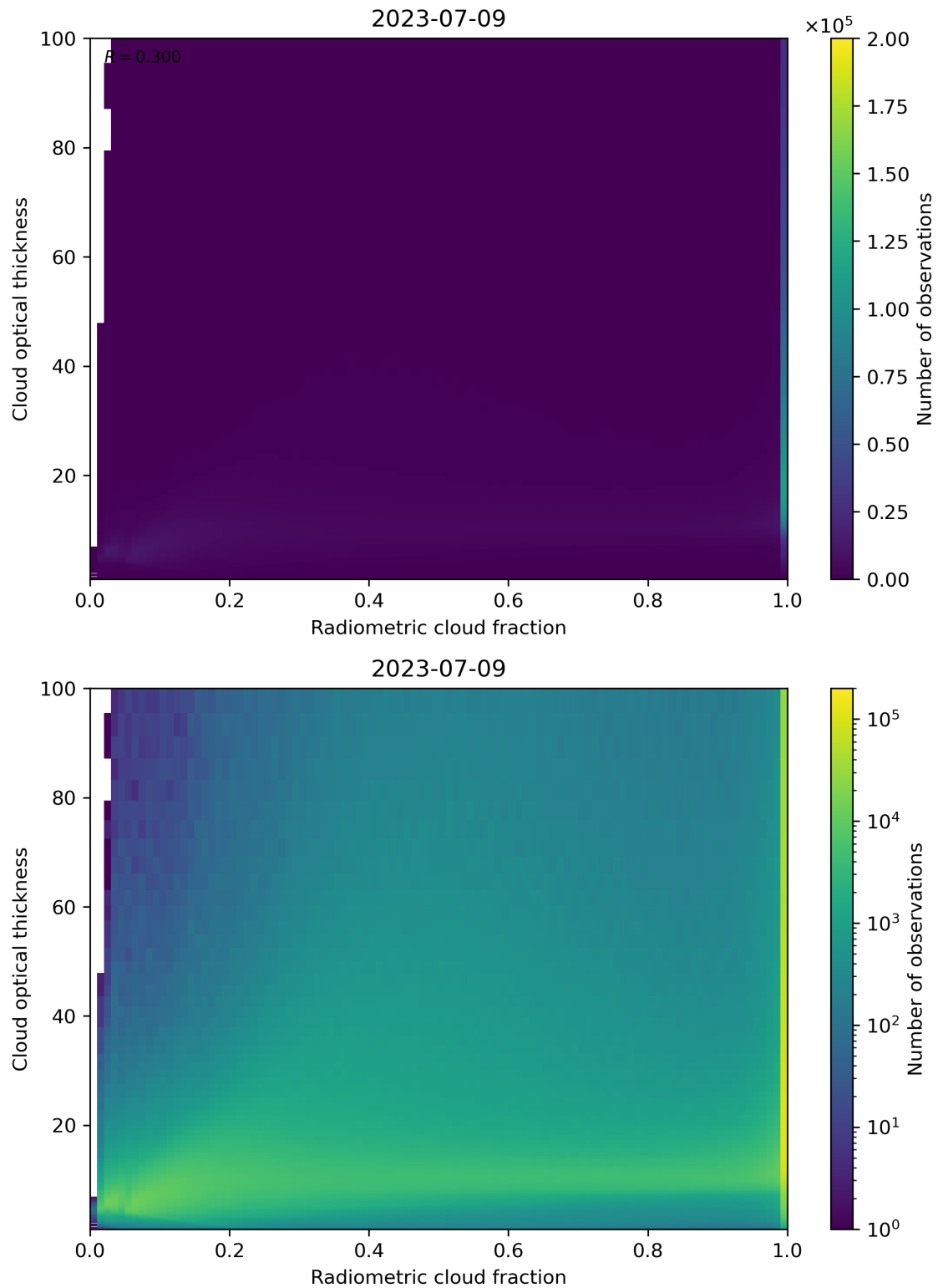
Figure 75: Scatter density plot of “Radiometric cloud fraction” against “Cloud optical thickness” for 2023-07-08 to 2023-07-10.
