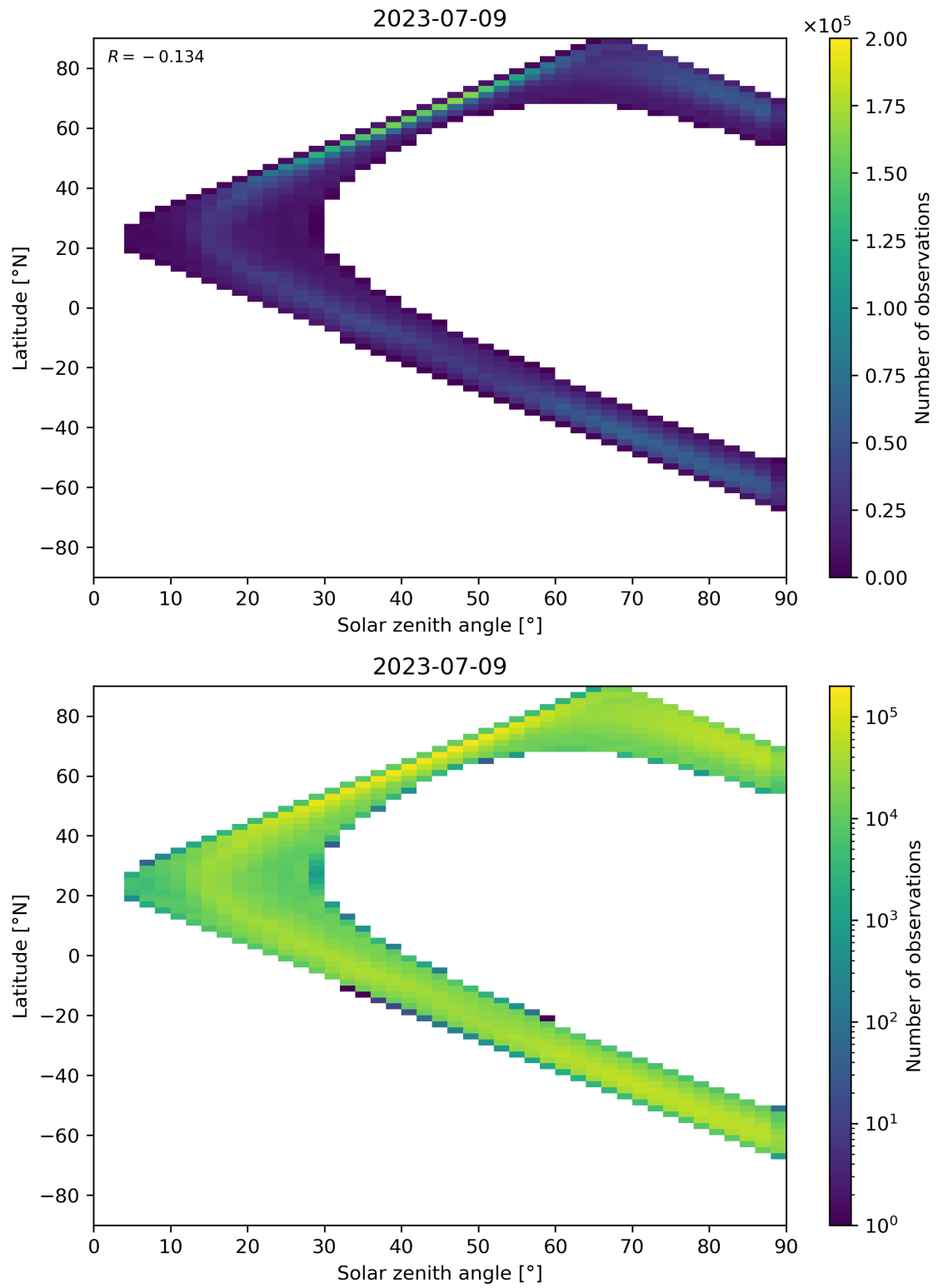
Figure 105: Scatter density plot of “Solar zenith angle” against “Latitude” for 2023-07-08 to 2023-07-10.
