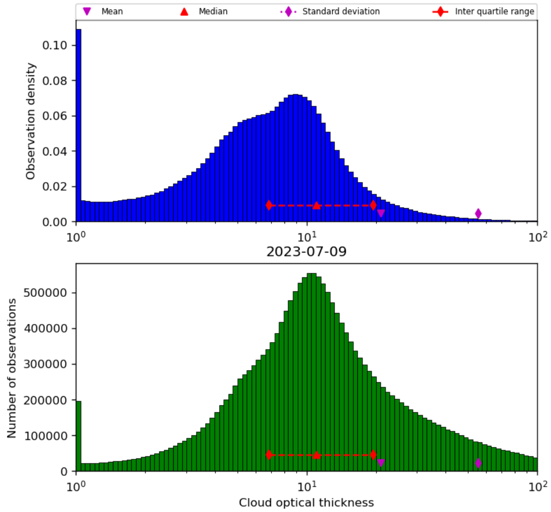
Figure 41: Histogram of “Cloud optical thickness” for 2023-07-08 to 2023-07-10
