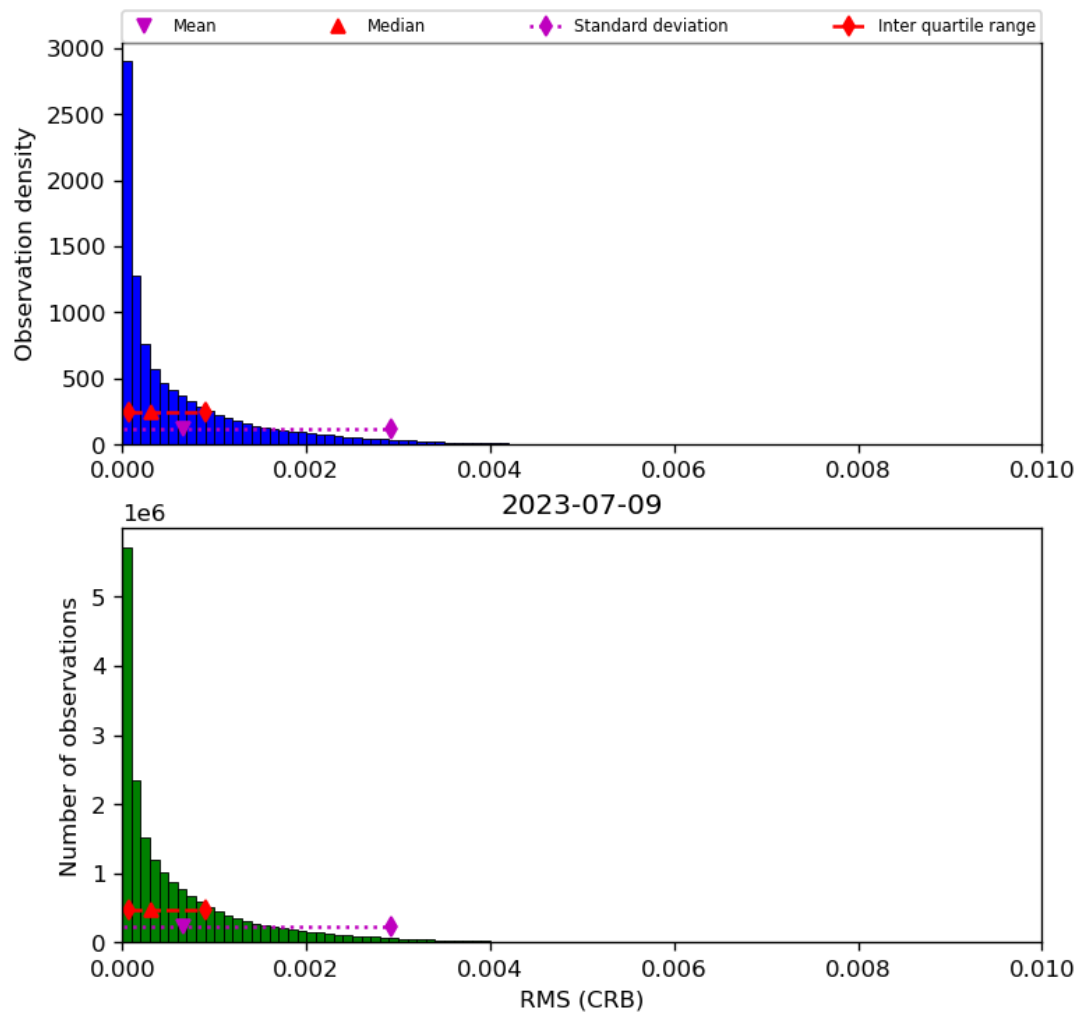
Figure 48: Histogram of “RMS (CRB)” for 2023-07-08 to 2023-07-10
