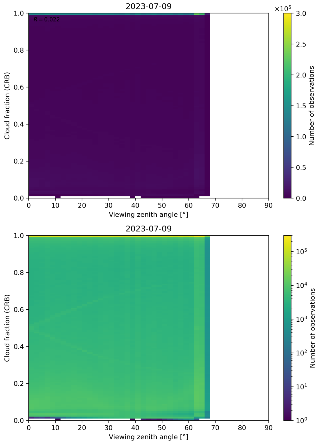
Figure 109: Scatter density plot of “Viewing zenith angle” against “Cloud fraction (CRB)” for 2023-07-08 to 2023-07-10.
