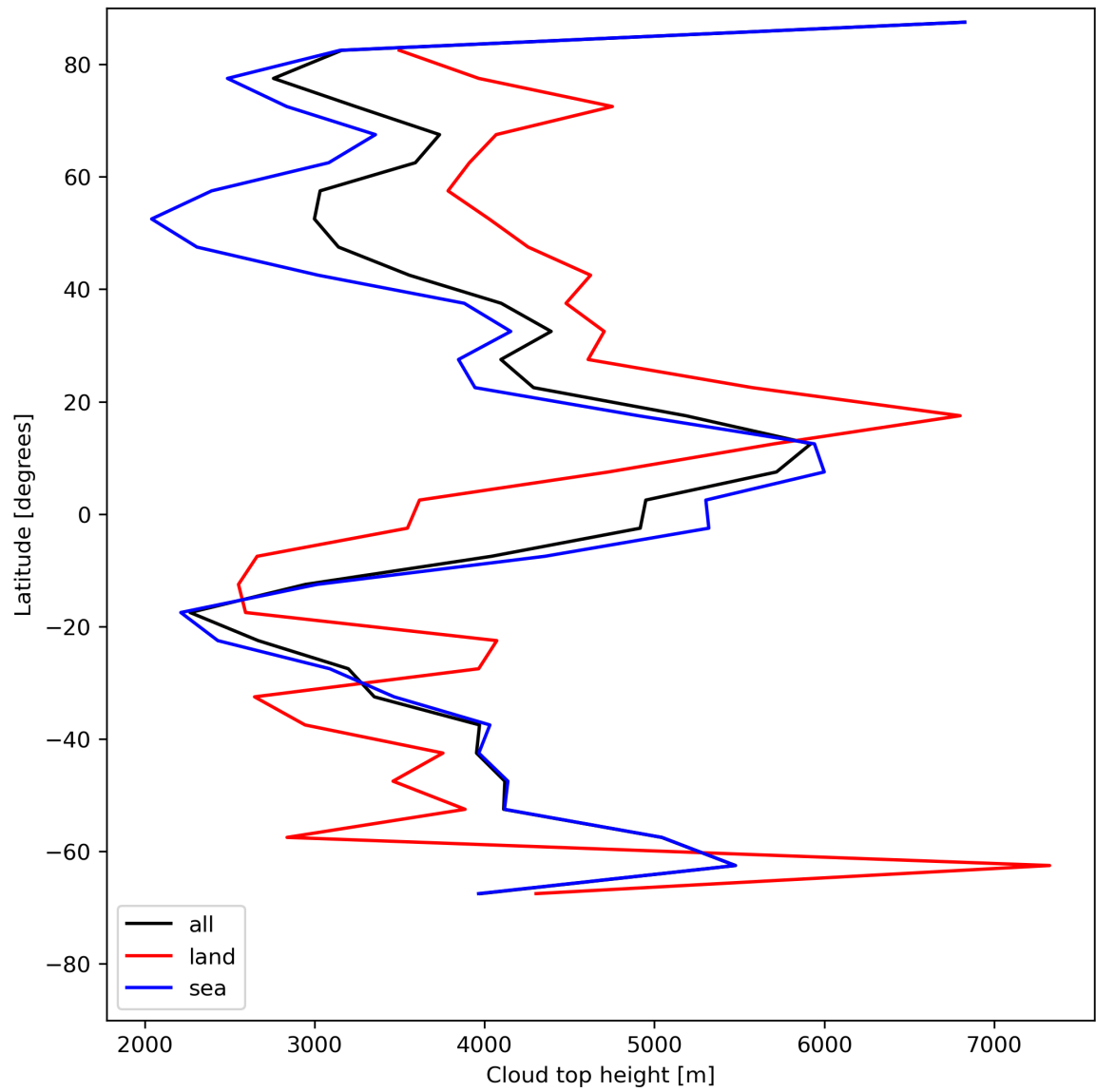
Figure 24: Zonal average of “Cloud top height” for 2023-07-08 to 2023-07-10.
