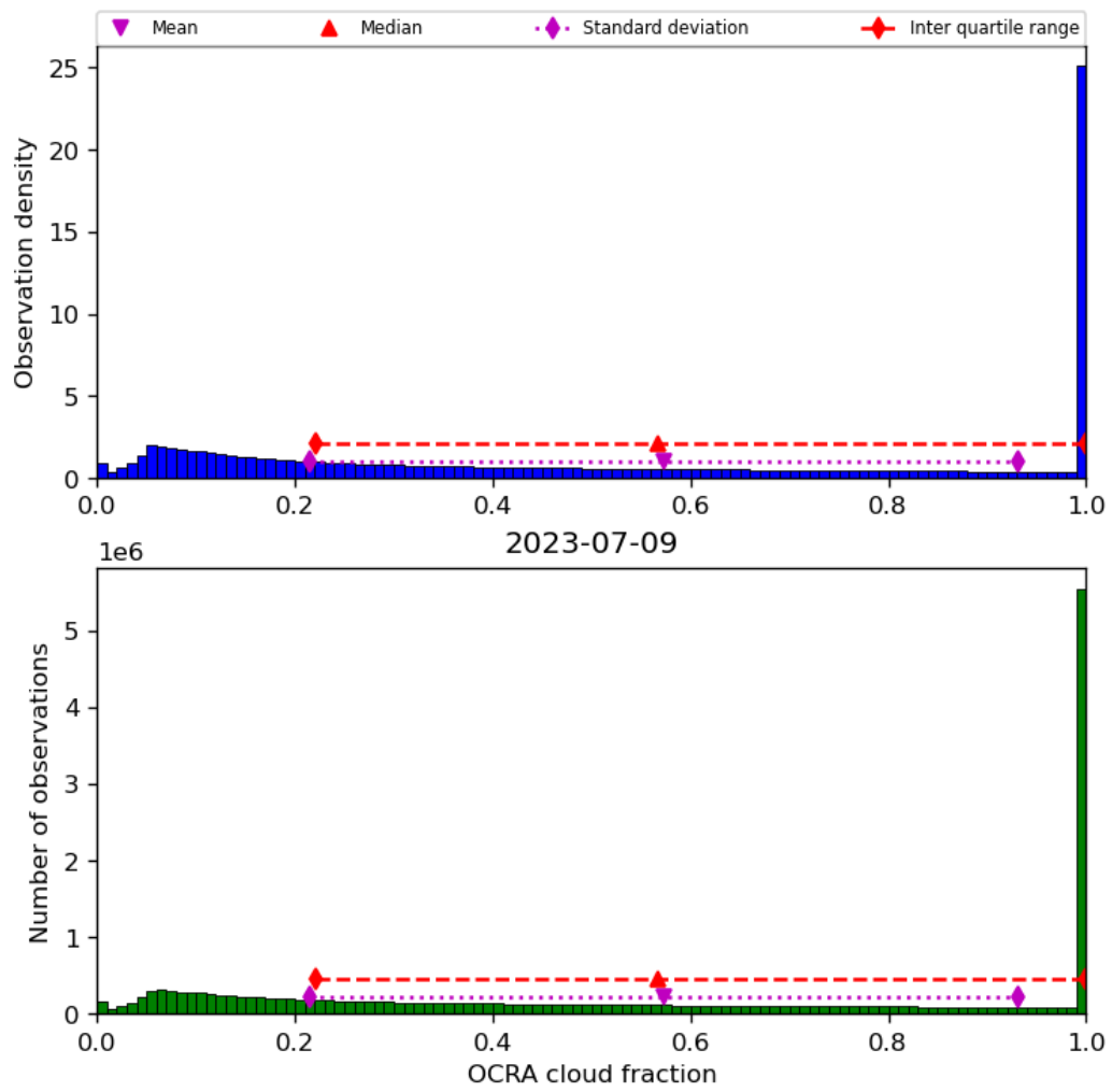
Figure 50: Histogram of “OCRA cloud fraction” for 2023-07-08 to 2023-07-10
