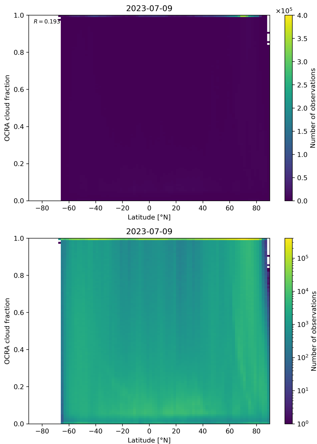
Figure 93: Scatter density plot of “Latitude” against “OCRA cloud fraction” for 2023-07-08 to 2023-07-10.
