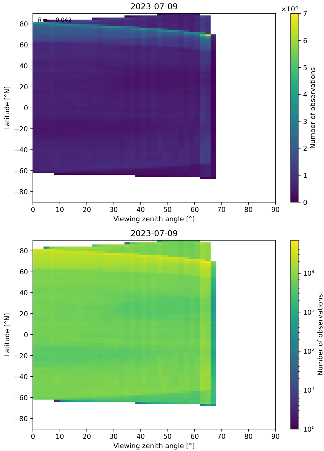
Figure 113: Scatter density plot of “Viewing zenith angle” against “Latitude” for 2023-07-08 to 2023-07-10.
