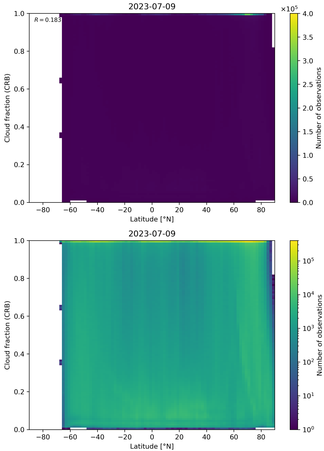
Figure 94: Scatter density plot of “Latitude” against “Cloud fraction (CRB)” for 2023-07-08 to 2023-07-10.
