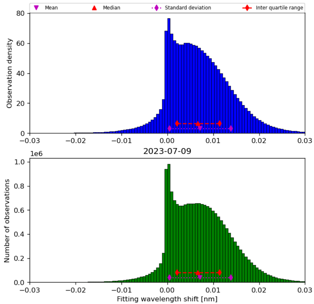
Figure 49: Histogram of “Fitting wavelength shift” for 2023-07-08 to 2023-07-10
