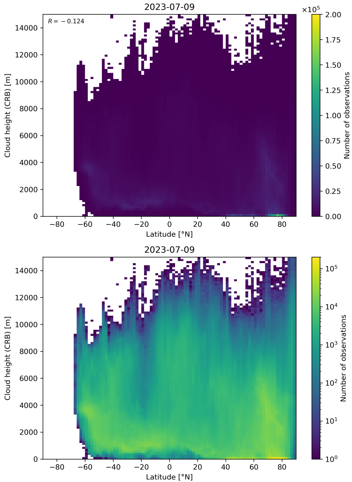
Figure 95: Scatter density plot of “Latitude” against “Cloud height (CRB)” for 2023-07-08 to 2023-07-10.
