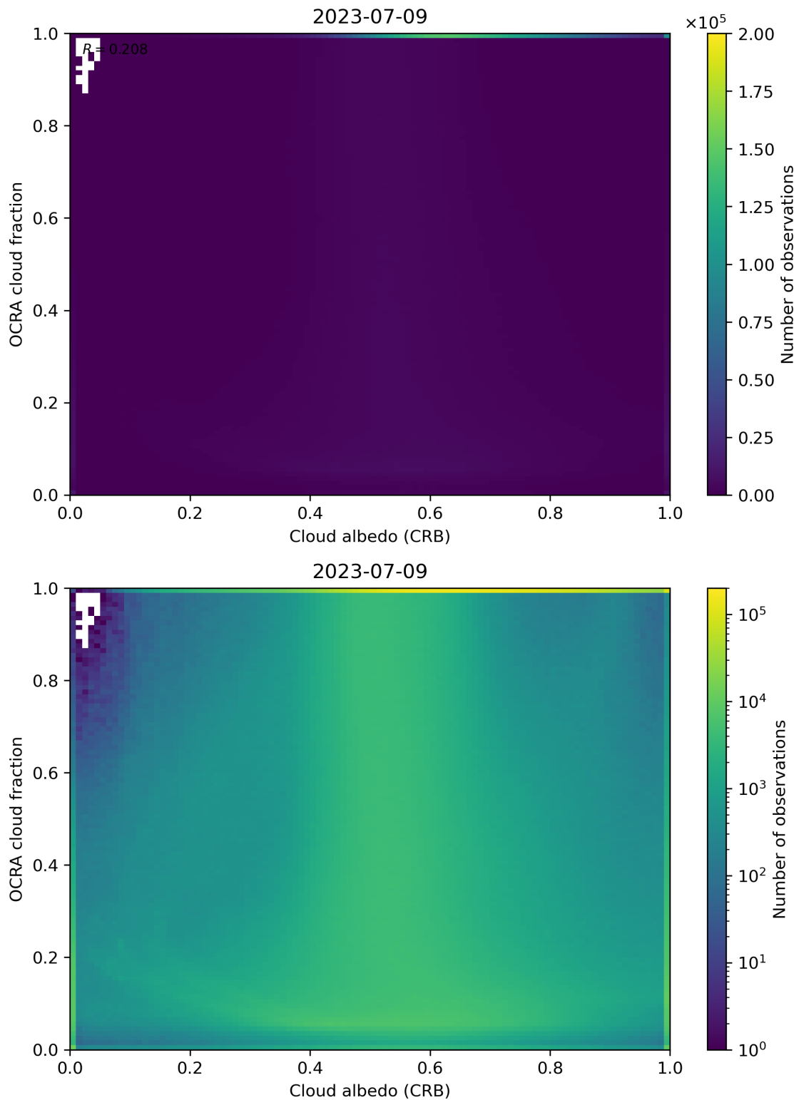
Figure 70: Scatter density plot of “Cloud albedo (CRB)” against “OCRA cloud fraction” for 2023-07-08 to 2023-07-10.
