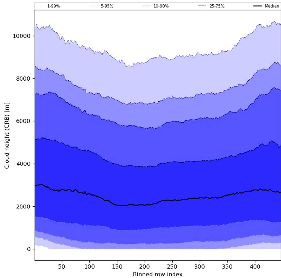
Figure 59: Along track statistics of “Cloud height (CRB)” for 2023-07-08 to 2023-07-10
