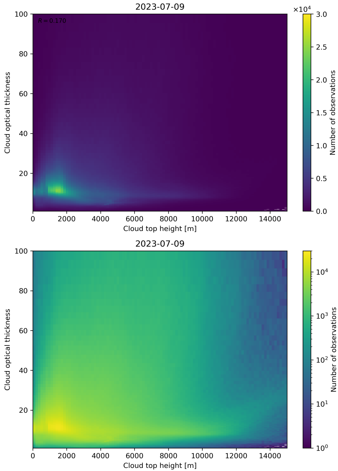
Figure 90: Scatter density plot of “Cloud top height” against “Cloud optical thickness” for 2023-07-08 to 2023-07-10.
