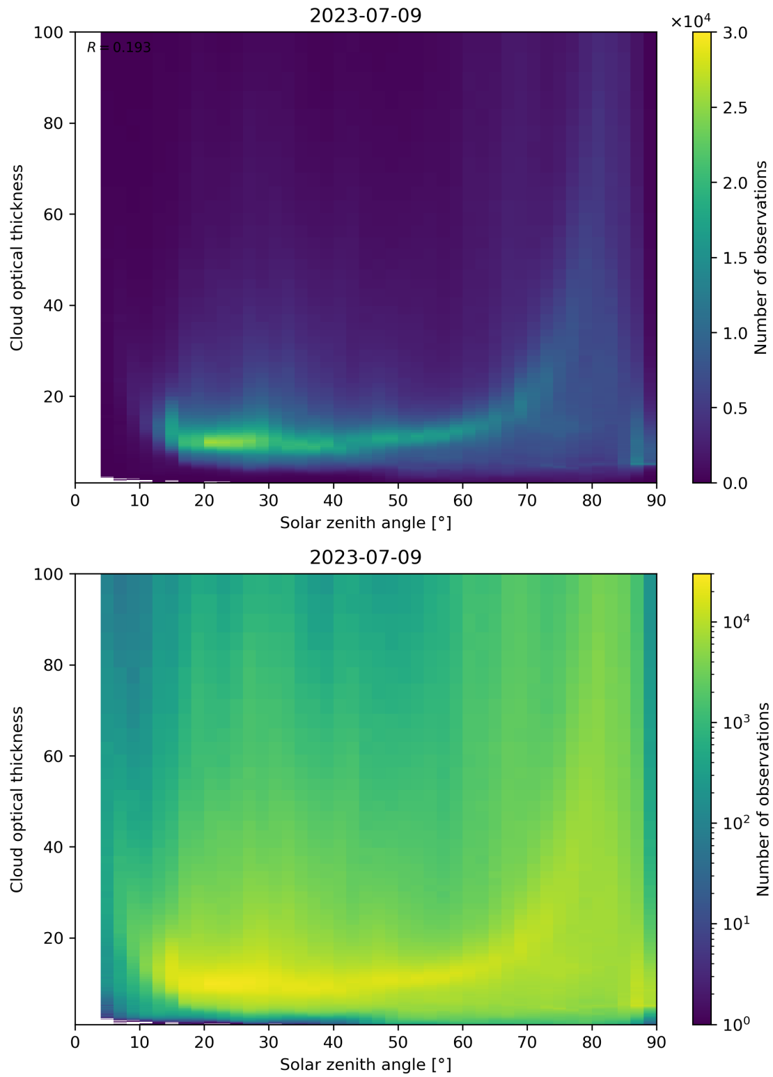
Figure 103: Scatter density plot of “Solar zenith angle” against “Cloud optical thickness” for 2023-07-08 to 2023-07-10.
