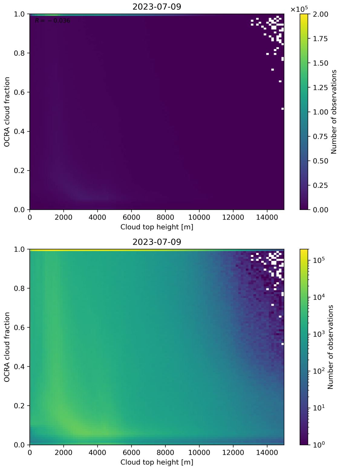
Figure 87: Scatter density plot of “Cloud top height” against “OCRA cloud fraction” for 2023-07-08 to 2023-07-10.
