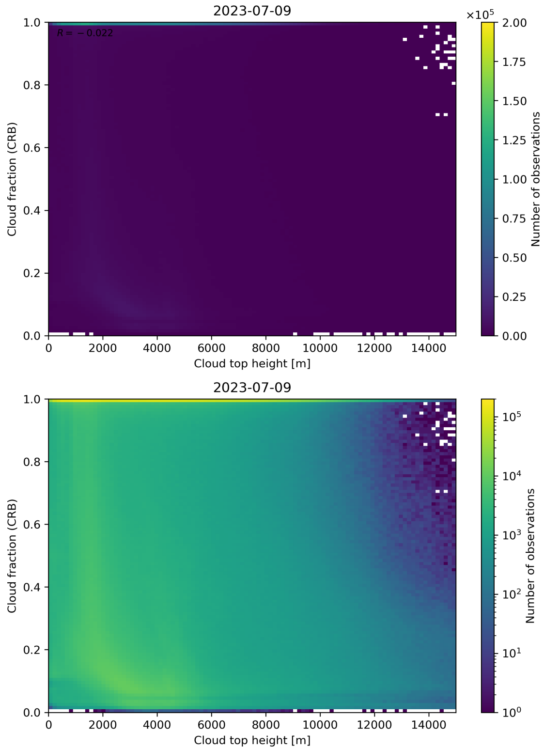
Figure 88: Scatter density plot of “Cloud top height” against “Cloud fraction (CRB)” for 2023-07-08 to 2023-07-10.
