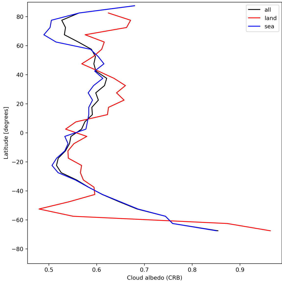
Figure 28: Zonal average of “Cloud albedo (CRB)” for 2023-07-08 to 2023-07-10.
