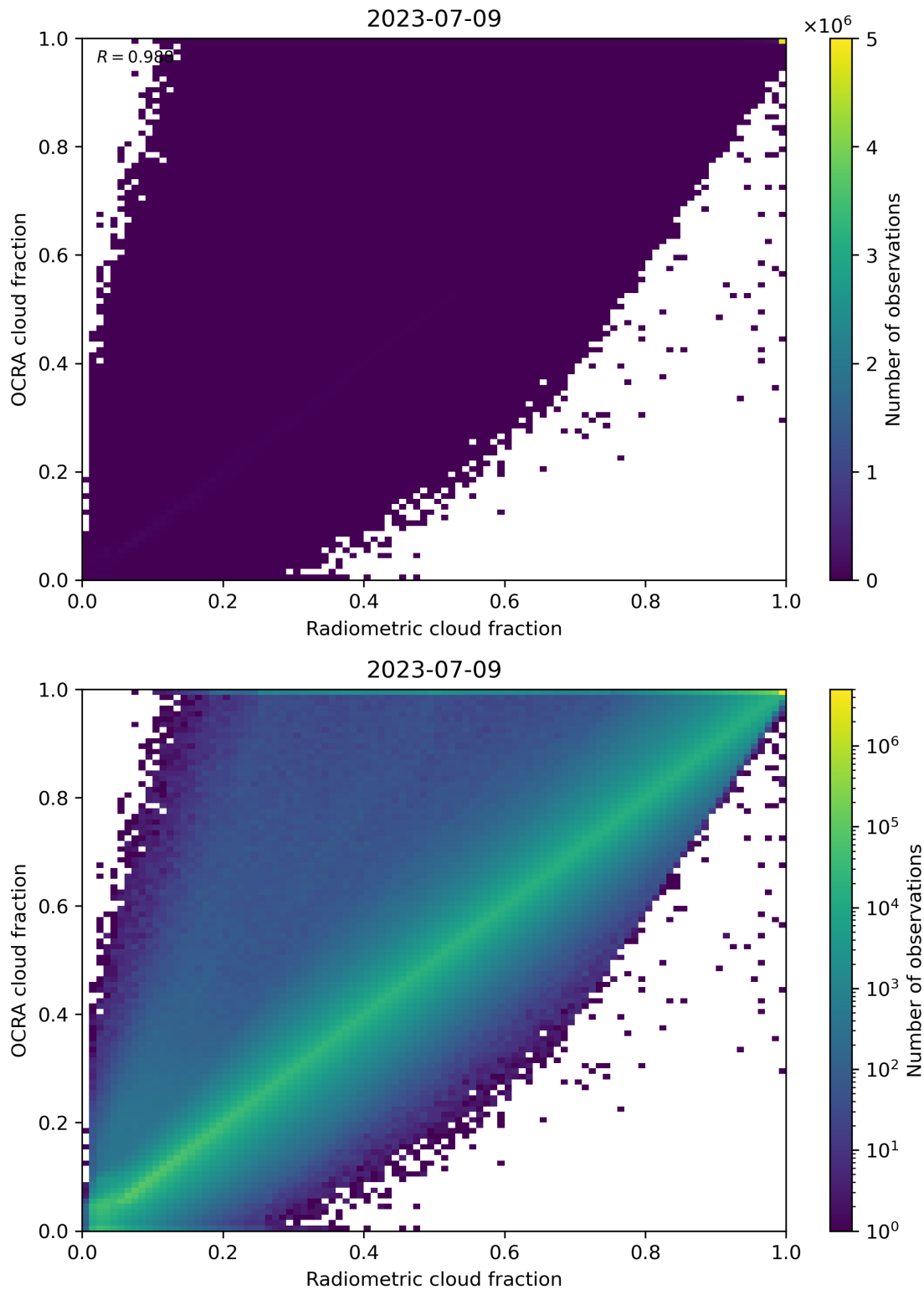
Figure 72: Scatter density plot of “Radiometric cloud fraction” against “OCRA cloud fraction” for 2023-07-08 to 2023-07-10.
