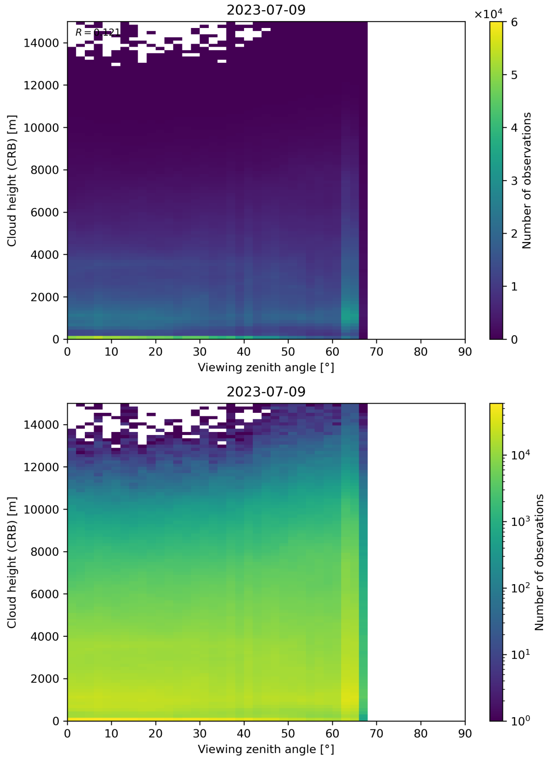
Figure 110: Scatter density plot of “Viewing zenith angle” against “Cloud height (CRB)” for 2023-07-08 to 2023-07-10.
