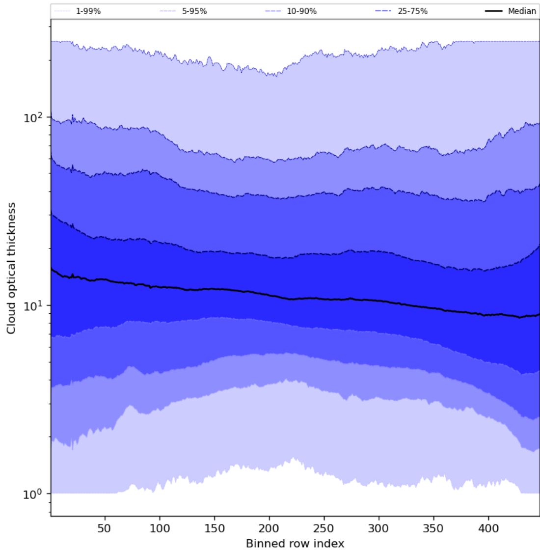
Figure 57: Along track statistics of “Cloud optical thickness” for 2023-07-08 to 2023-07-10
