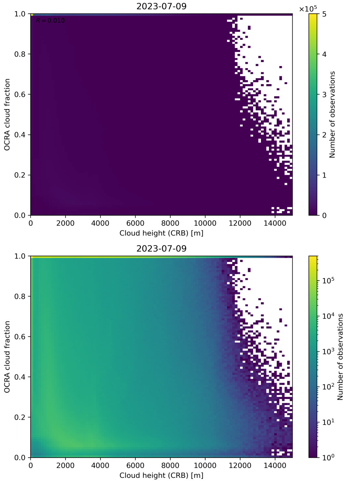
Figure 81: Scatter density plot of “Cloud height (CRB)” against “OCRA cloud fraction” for 2023-07-08 to 2023-07-10.
