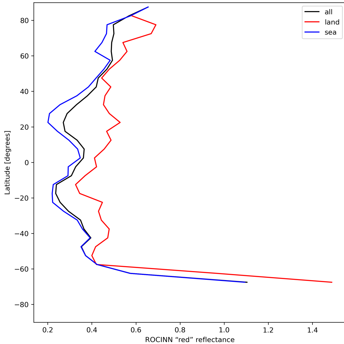
Figure 37: Zonal average of “ROCINN “red” reflectance” for 2023-07-08 to 2023-07-10.
