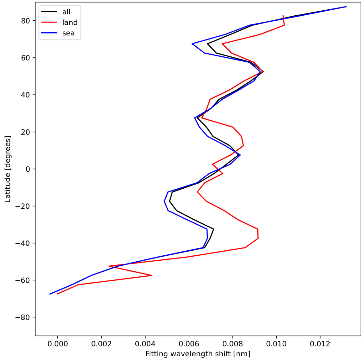
Figure 33: Zonal average of “Fitting wavelength shift” for 2023-07-08 to 2023-07-10.
