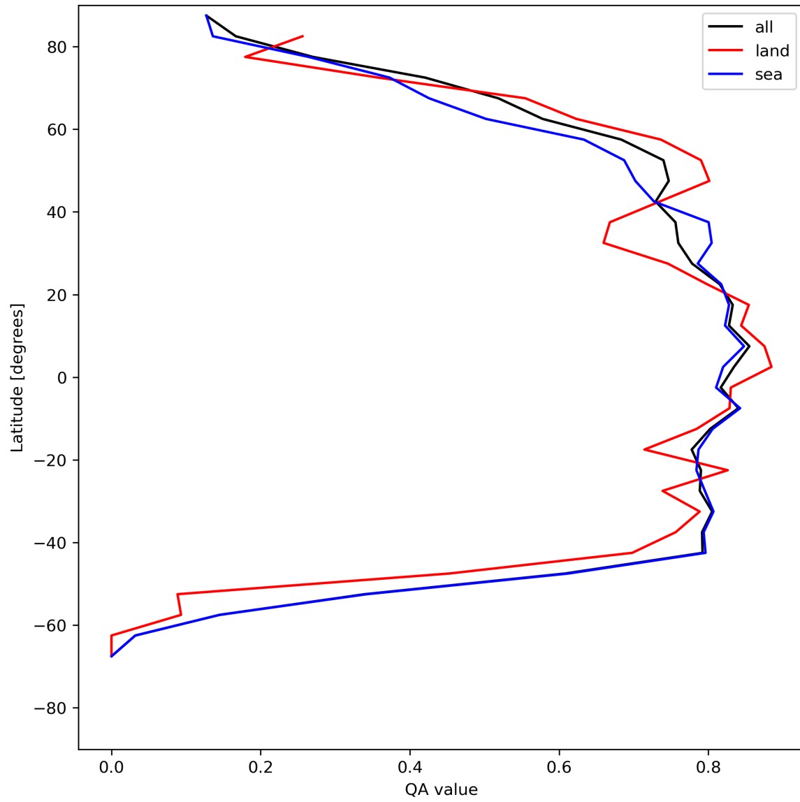
Figure 22: Zonal average of “QA value” for 2023-07-08 to 2023-07-10.
