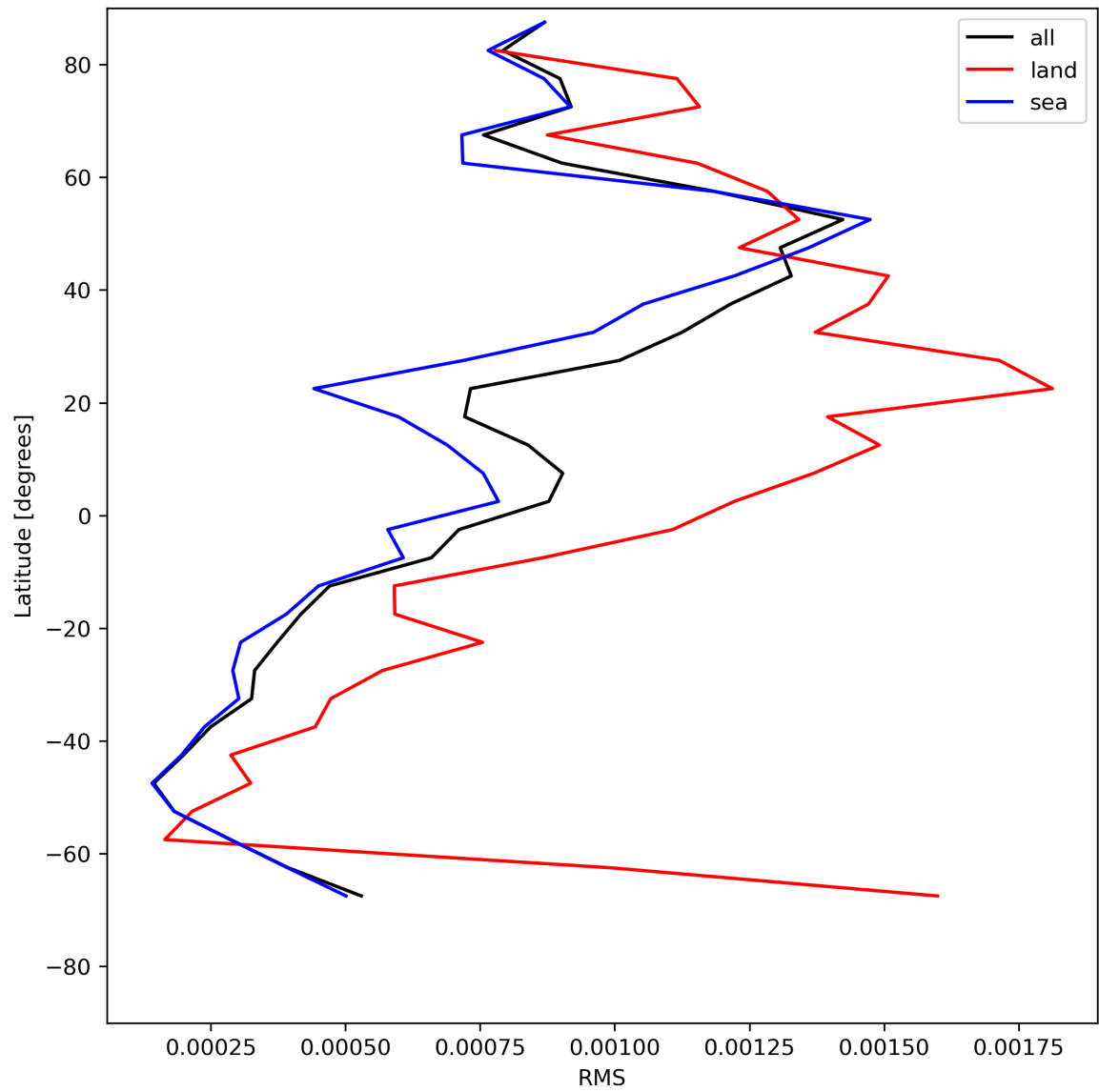
Figure 31: Zonal average of “RMS” for 2023-07-08 to 2023-07-10.
