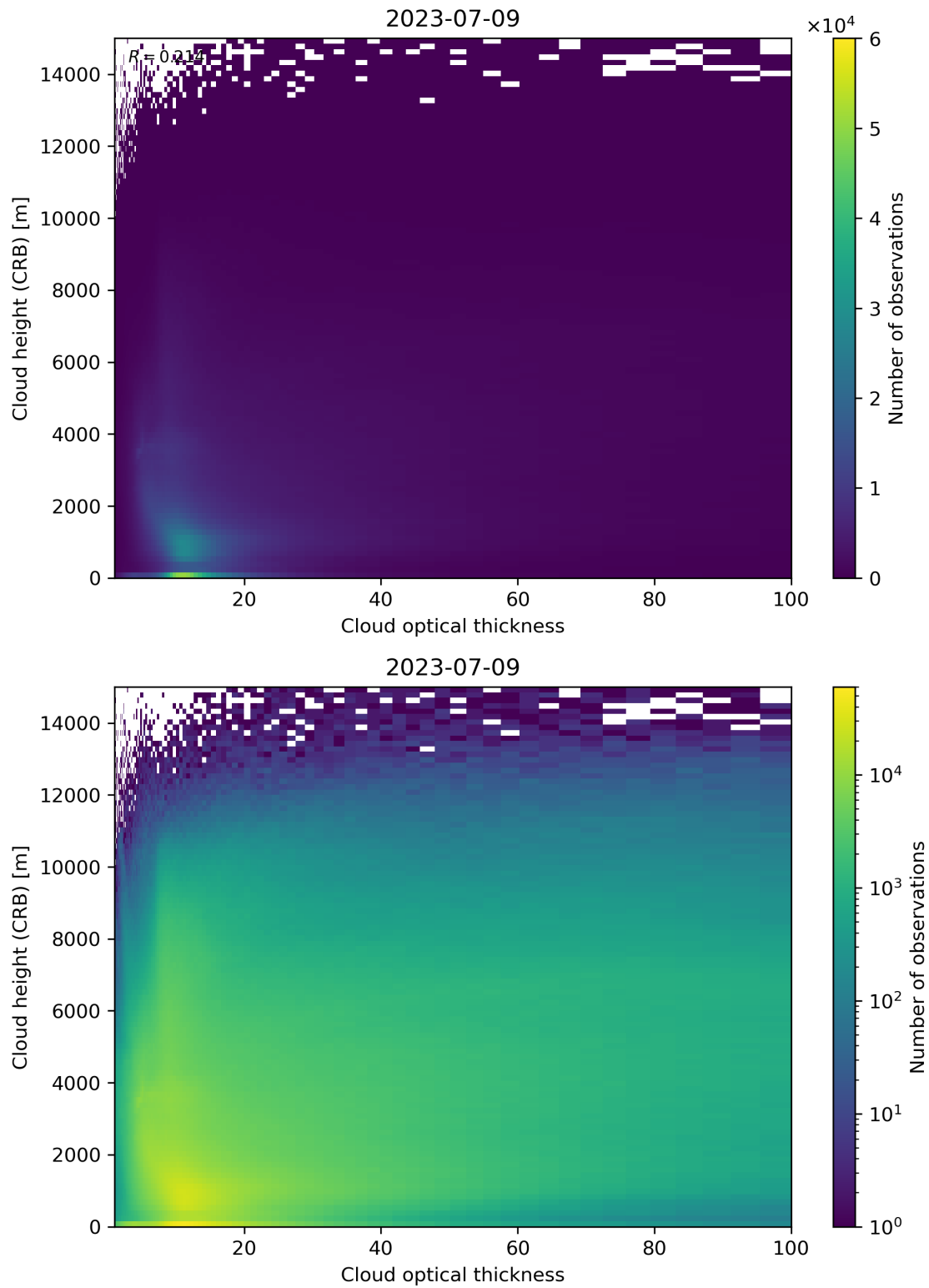
Figure 85: Scatter density plot of “Cloud optical thickness” against “Cloud height (CRB)” for 2023-07-08 to 2023-07-10.
