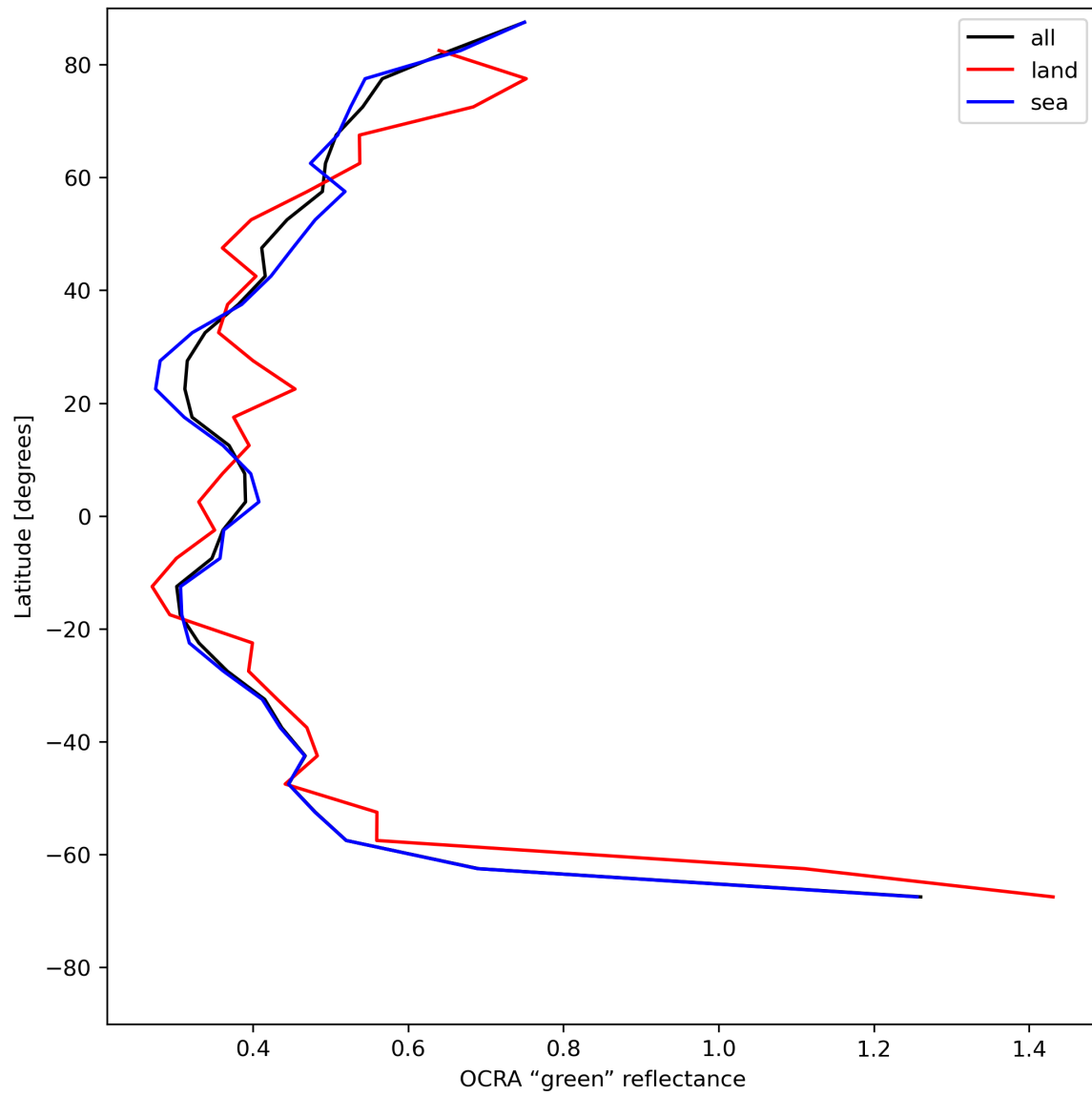
Figure 36: Zonal average of “OCRA “green” reflectance” for 2023-07-08 to 2023-07-10.
