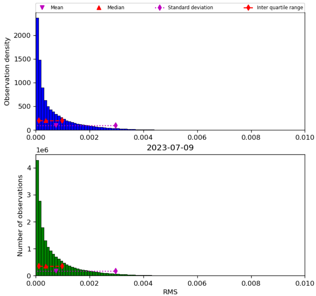
Figure 47: Histogram of “RMS” for 2023-07-08 to 2023-07-10
