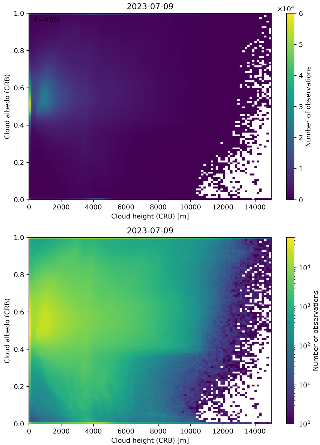
Figure 80: Scatter density plot of “Cloud height (CRB)” against “Cloud albedo (CRB)” for 2023-07-08 to 2023-07-10.
