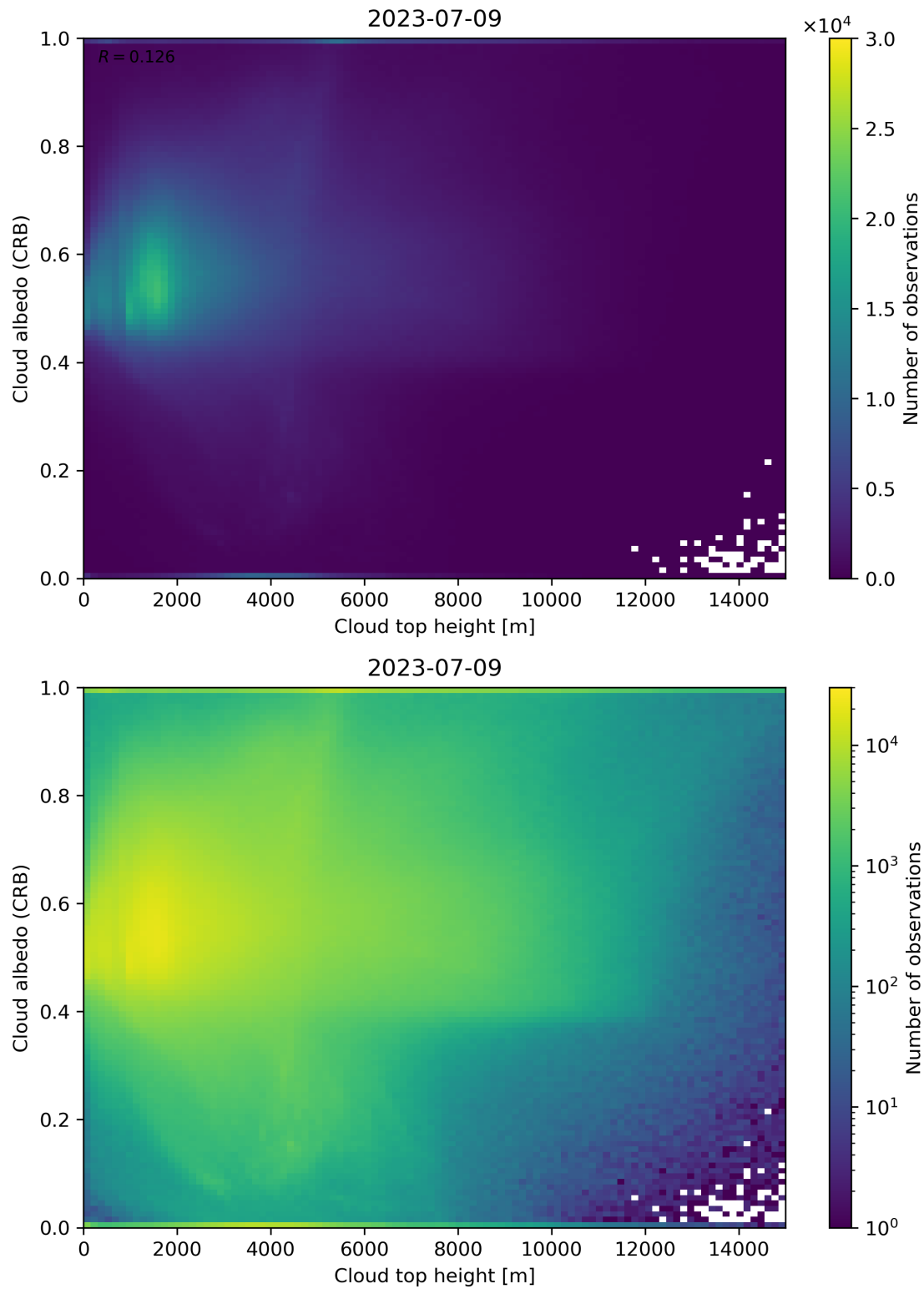
Figure 86: Scatter density plot of “Cloud top height” against “Cloud albedo (CRB)” for 2023-07-08 to 2023-07-10.
