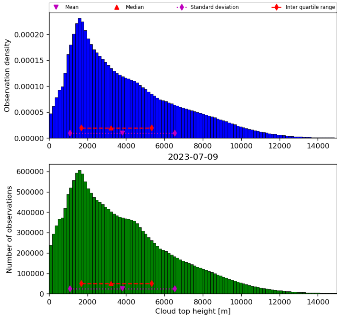
Figure 40: Histogram of “Cloud top height” for 2023-07-08 to 2023-07-10
