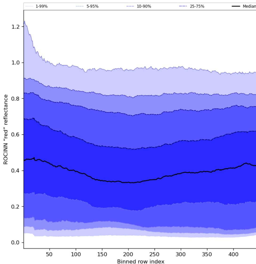
Figure 69: Along track statistics of “ROCINN “red” reflectance” for 2023-07-08 to 2023-07-10
