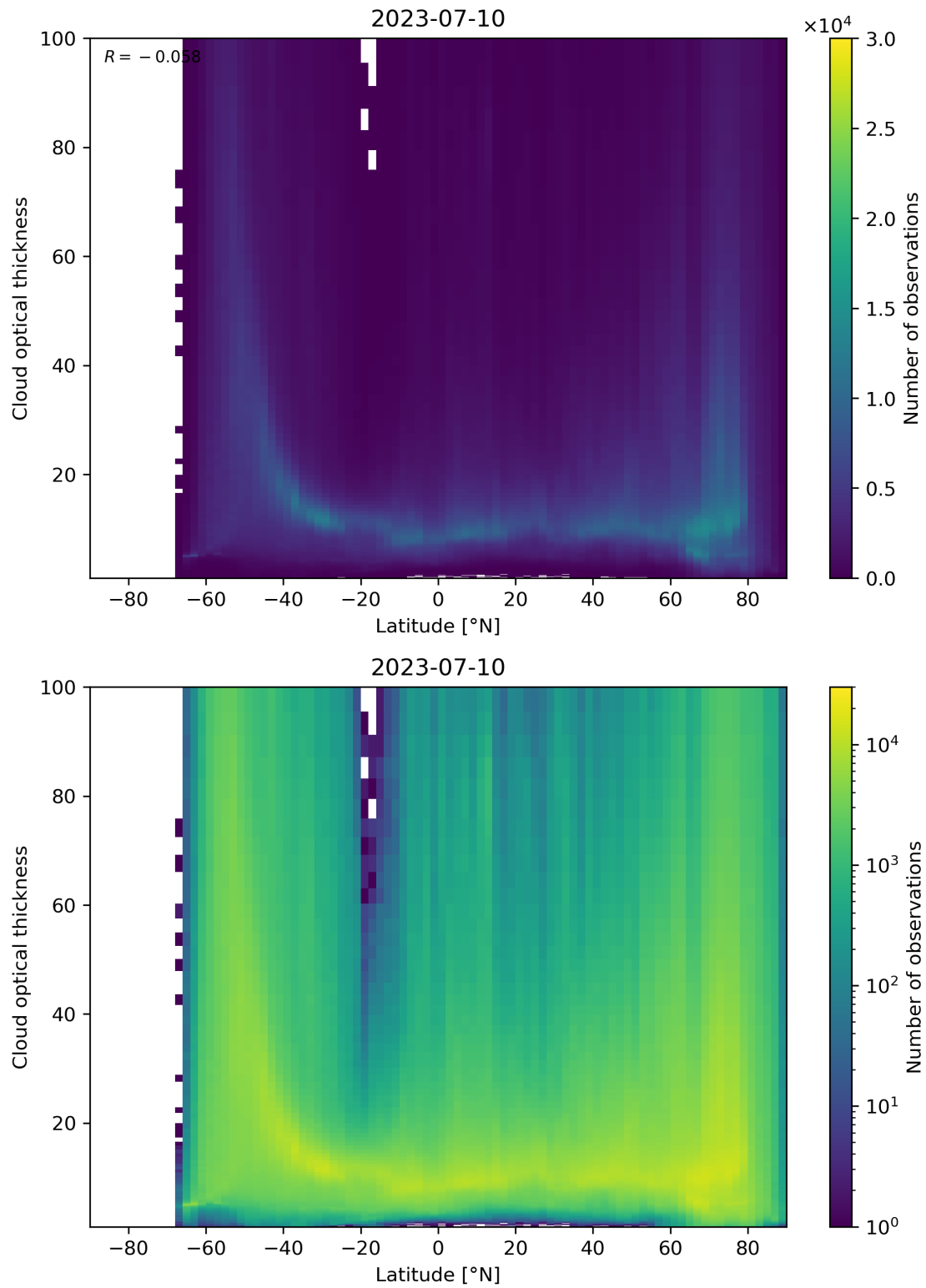
Figure 96: Scatter density plot of “Latitude” against “Cloud optical thickness” for 2023-07-09 to 2023-07-11.
