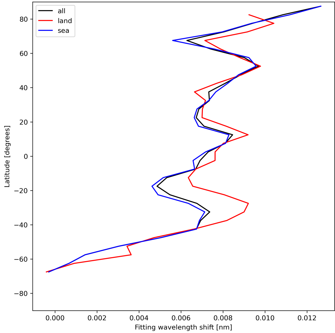
Figure 33: Zonal average of “Fitting wavelength shift” for 2023-07-09 to 2023-07-11.
