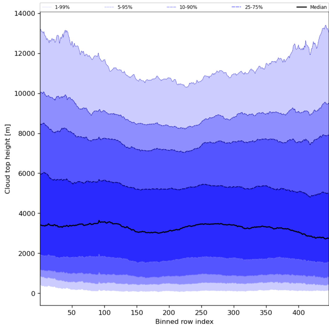
Figure 56: Along track statistics of “Cloud top height” for 2023-07-09 to 2023-07-11
