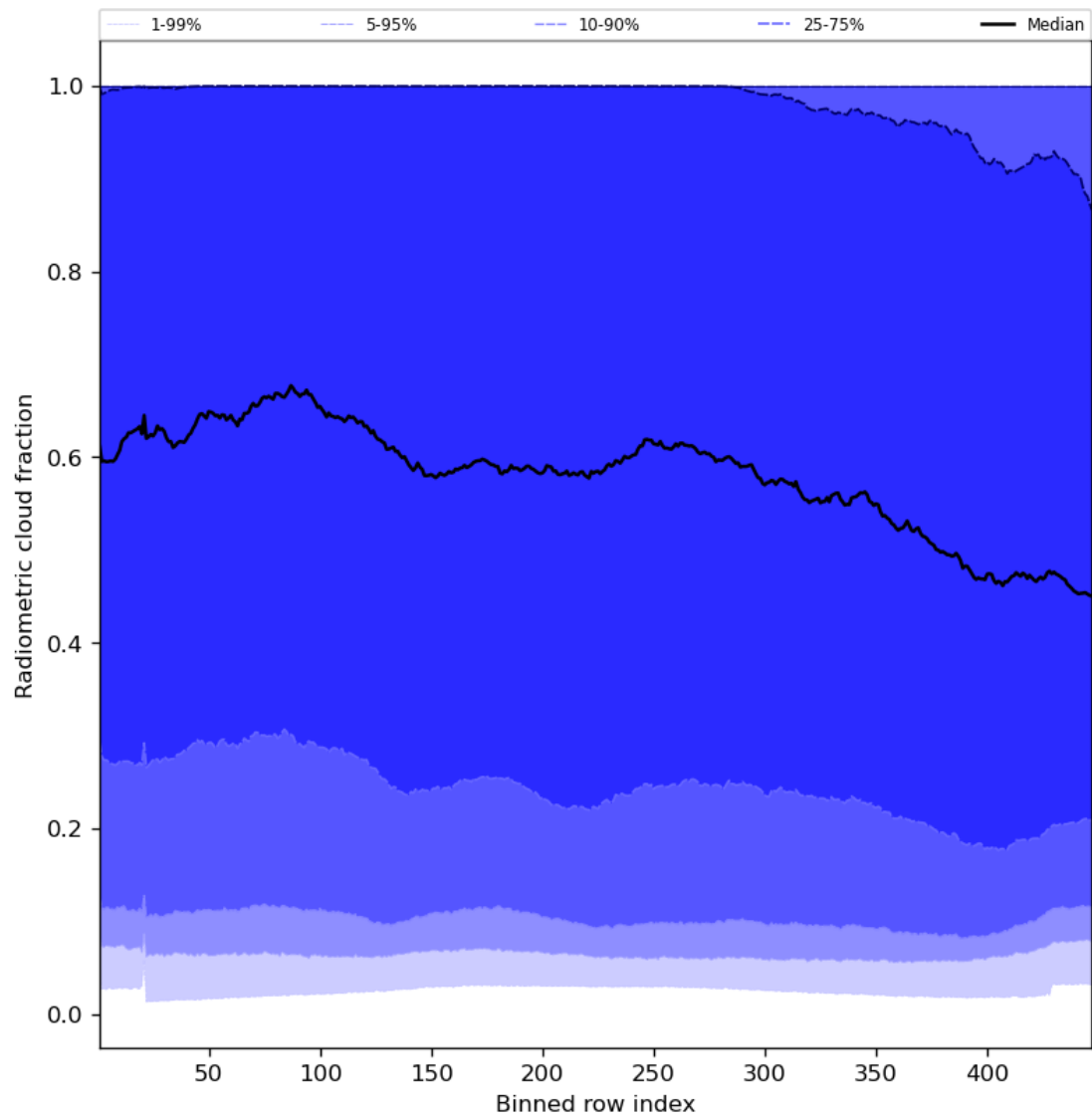
Figure 55: Along track statistics of “Radiometric cloud fraction” for 2023-07-09 to 2023-07-11
