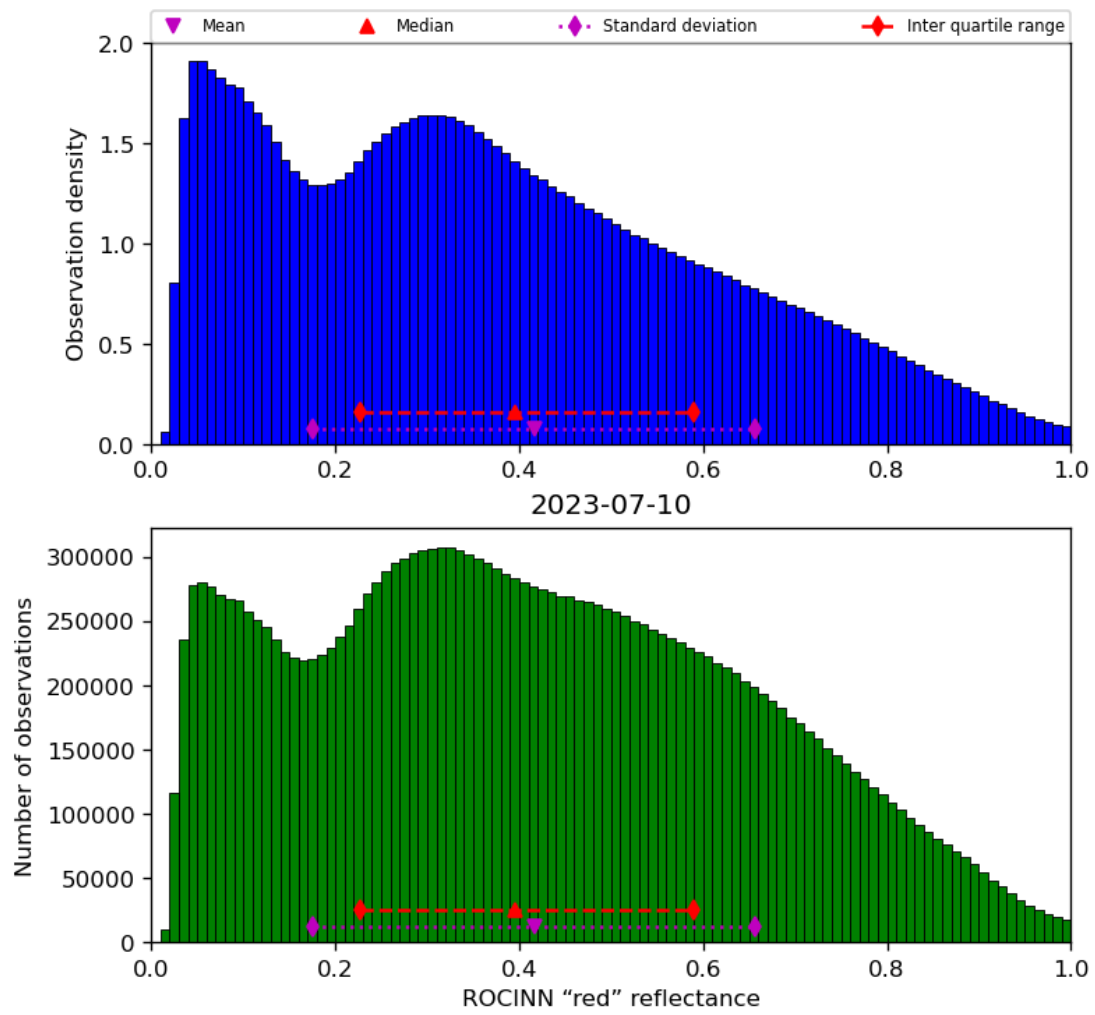
Figure 53: Histogram of “ROCINN “red” reflectance” for 2023-07-09 to 2023-07-11
