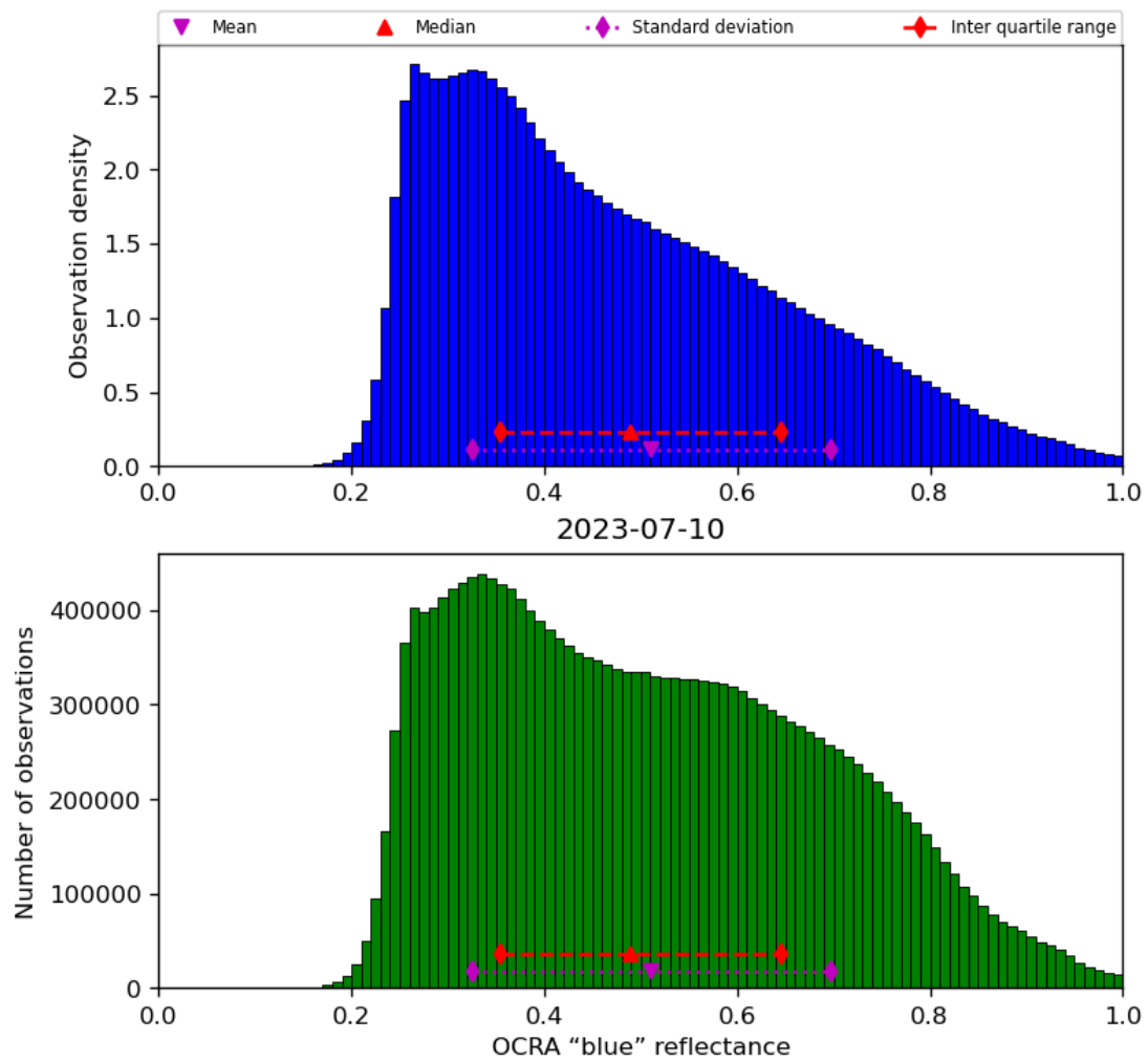
Figure 51: Histogram of “OCRA “blue” reflectance” for 2023-07-09 to 2023-07-11
