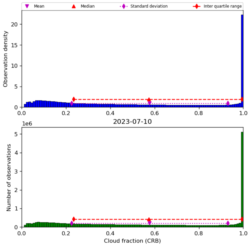
Figure 42: Histogram of “Cloud fraction (CRB)” for 2023-07-09 to 2023-07-11
