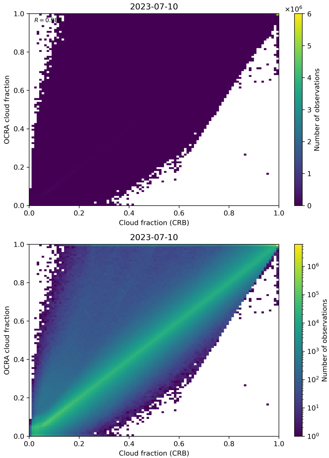
Figure 78: Scatter density plot of “Cloud fraction (CRB)” against “OCRA cloud fraction” for 2023-07-09 to 2023-07-11.
