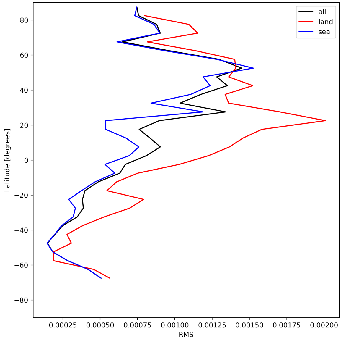
Figure 31: Zonal average of “RMS” for 2023-07-09 to 2023-07-11.
