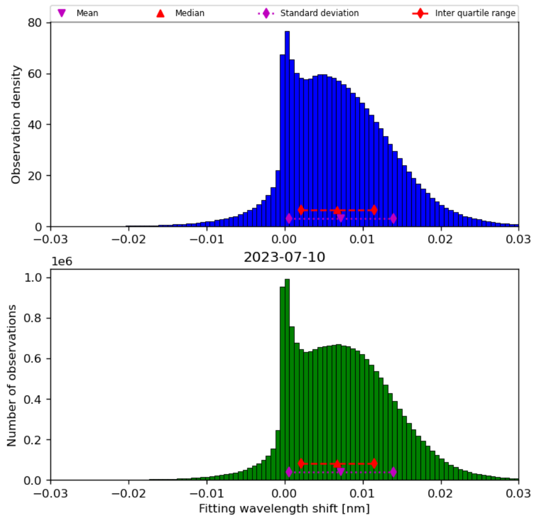
Figure 49: Histogram of “Fitting wavelength shift” for 2023-07-09 to 2023-07-11
