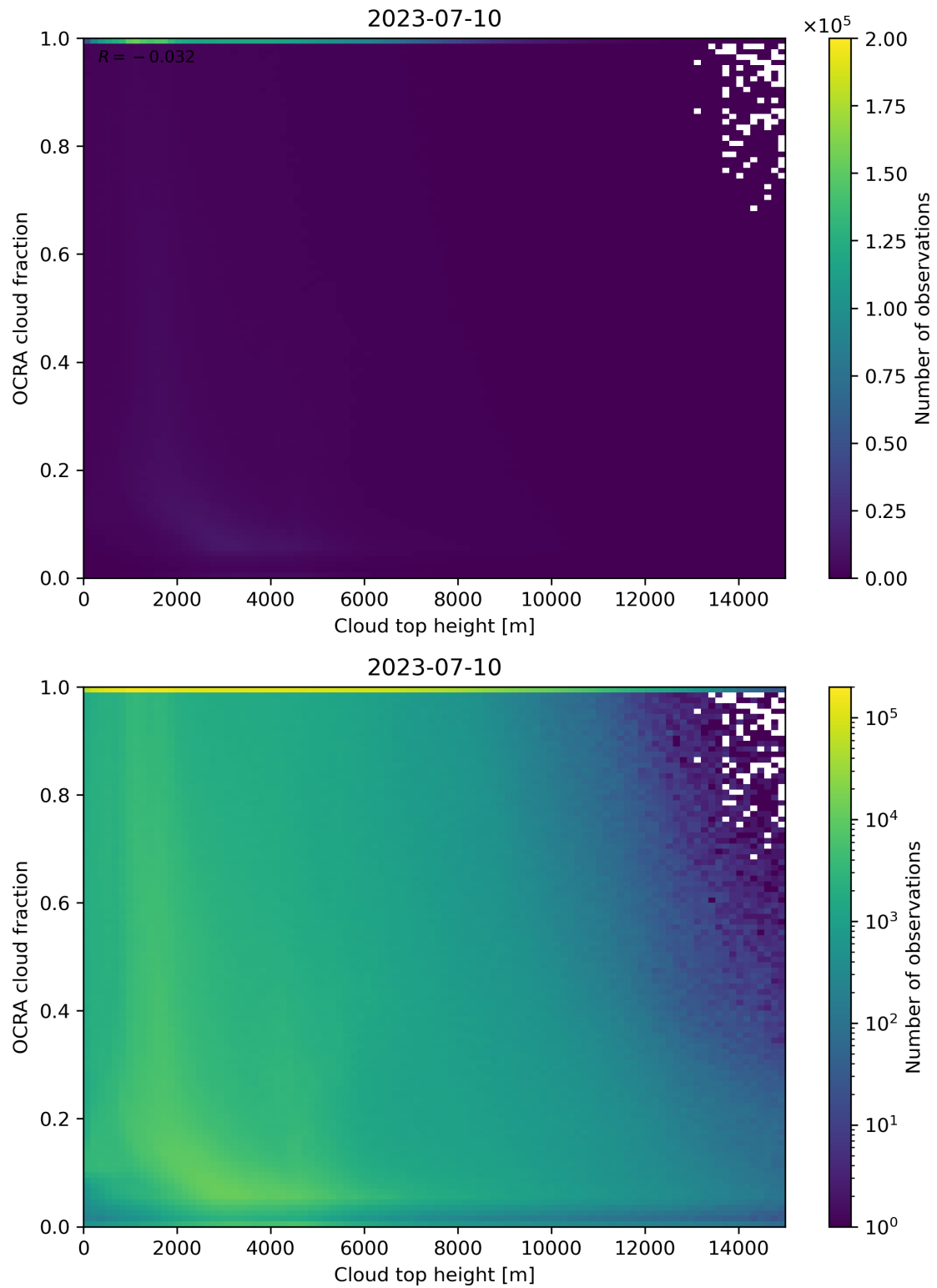
Figure 87: Scatter density plot of “Cloud top height” against “OCRA cloud fraction” for 2023-07-09 to 2023-07-11.
