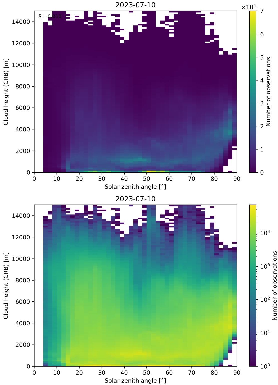
Figure 102: Scatter density plot of “Solar zenith angle” against “Cloud height (CRB)” for 2023-07-09 to 2023-07-11.
