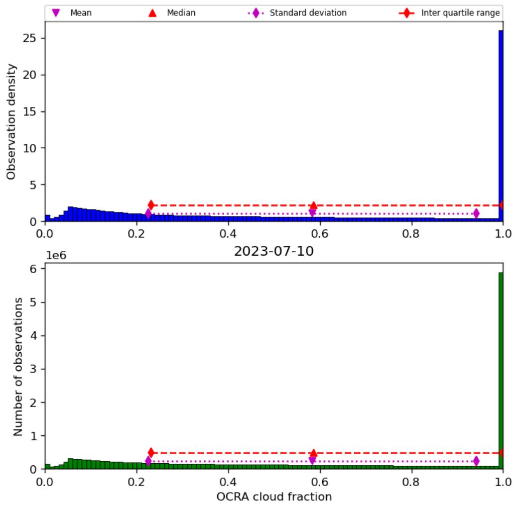
Figure 50: Histogram of “OCRA cloud fraction” for 2023-07-09 to 2023-07-11
