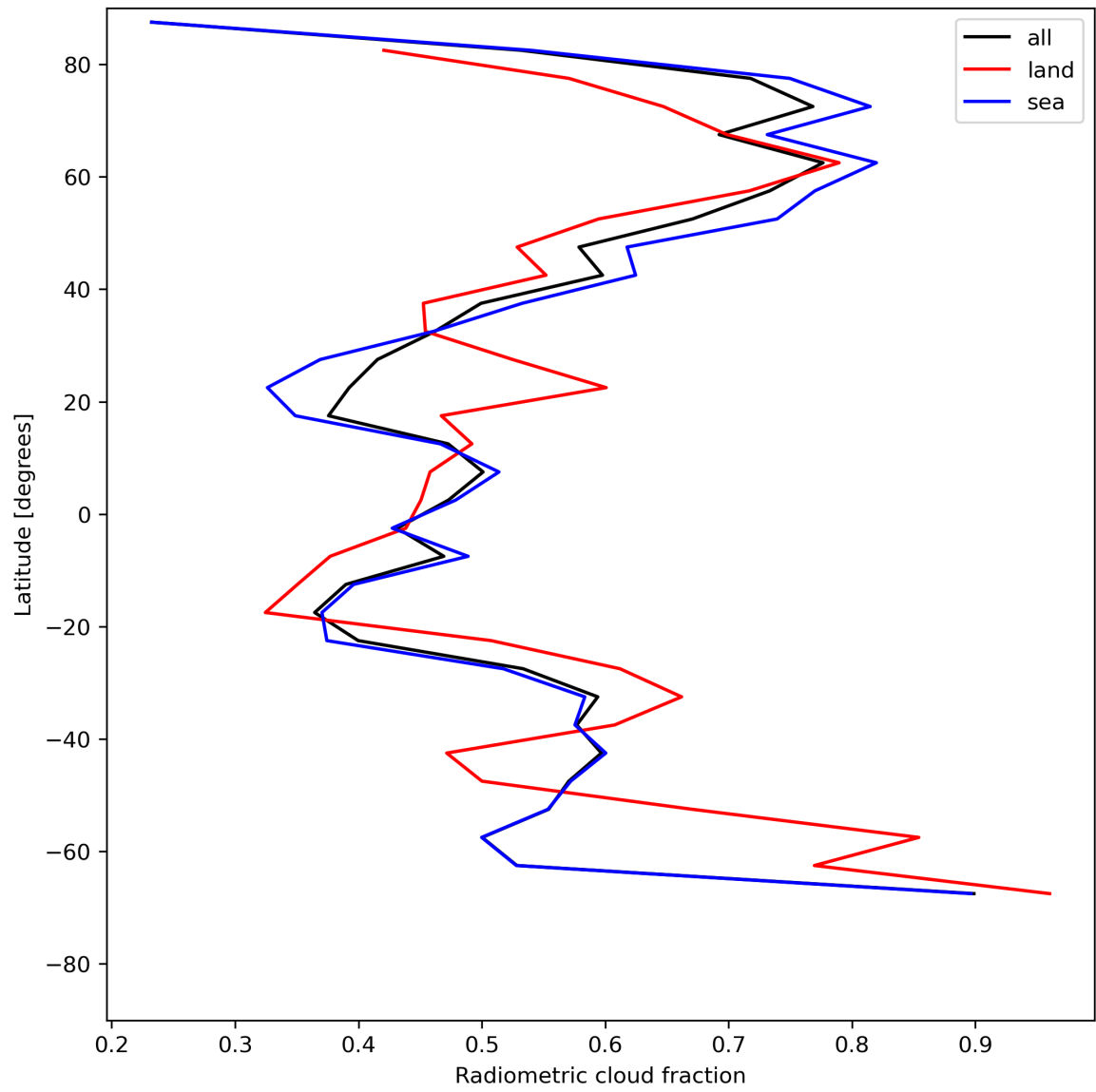
Figure 23: Zonal average of “Radiometric cloud fraction” for 2023-07-09 to 2023-07-11.
