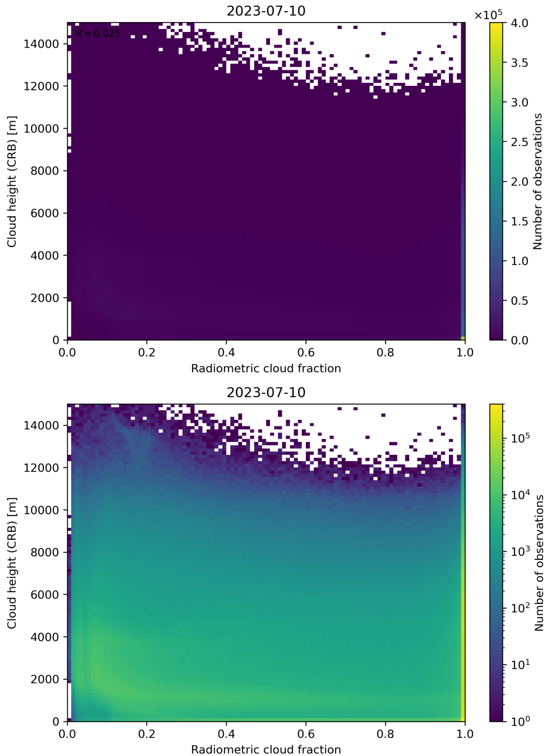
Figure 74: Scatter density plot of “Radiometric cloud fraction” against “Cloud height (CRB)” for 2023-07-09 to 2023-07-11.
