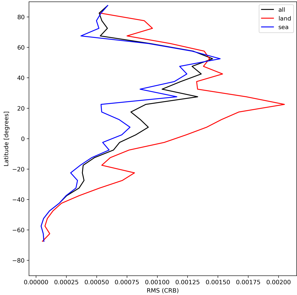
Figure 32: Zonal average of “RMS (CRB)” for 2023-07-09 to 2023-07-11.
