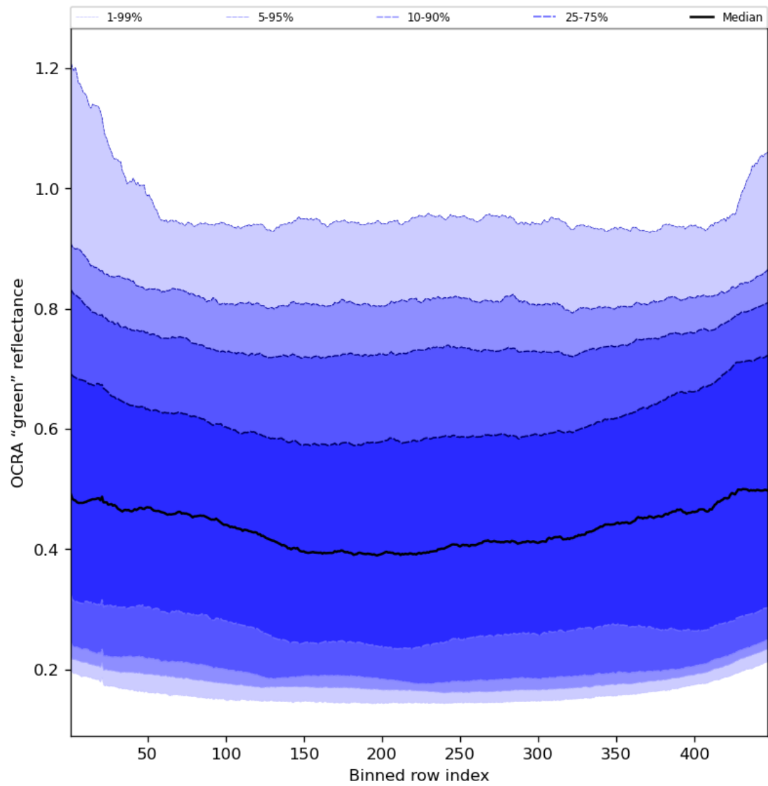
Figure 68: Along track statistics of “OCRA “green” reflectance” for 2023-07-09 to 2023-07-11
