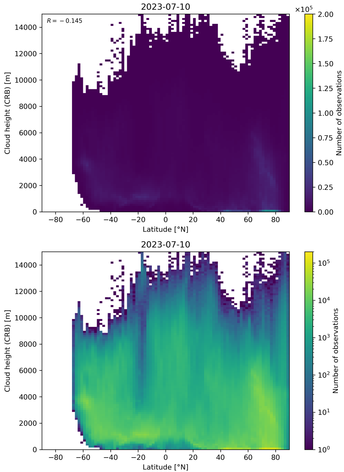
Figure 95: Scatter density plot of “Latitude” against “Cloud height (CRB)” for 2023-07-09 to 2023-07-11.
