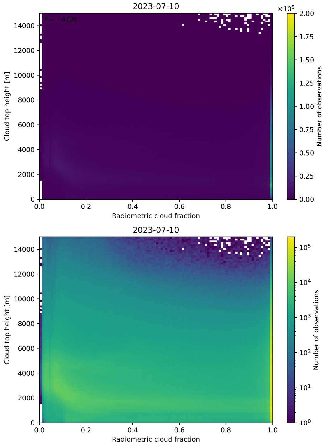
Figure 76: Scatter density plot of “Radiometric cloud fraction” against “Cloud top height” for 2023-07-09 to 2023-07-11.
