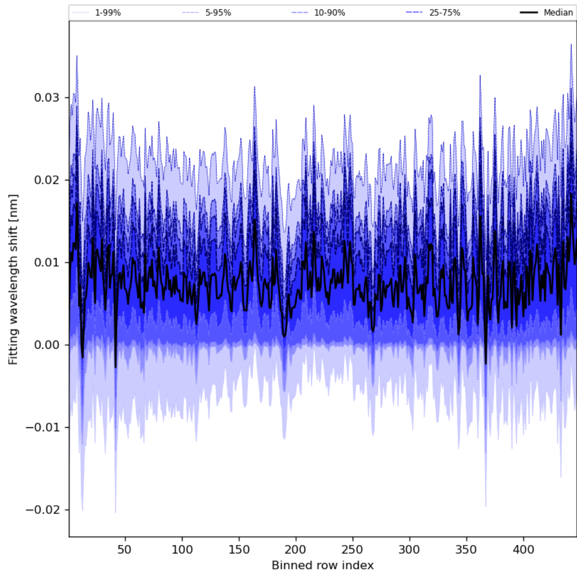
Figure 65: Along track statistics of “Fitting wavelength shift” for 2023-07-09 to 2023-07-11
