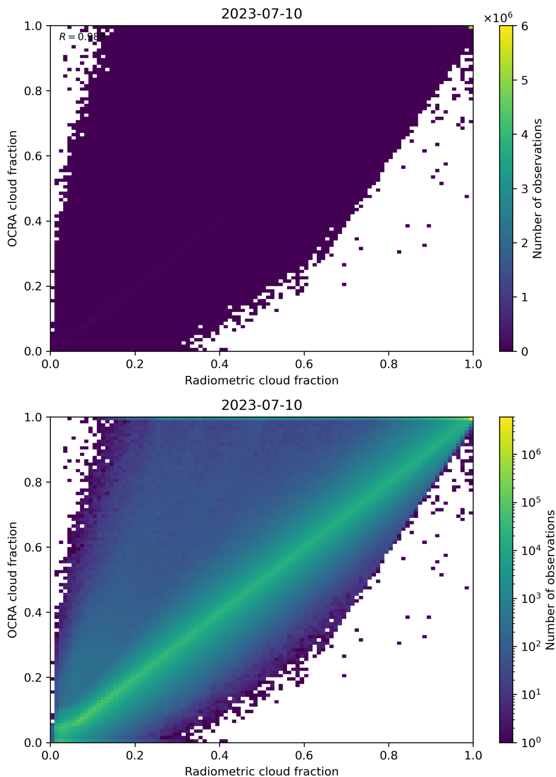
Figure 72: Scatter density plot of “Radiometric cloud fraction” against “OCRA cloud fraction” for 2023-07-09 to 2023-07-11.
