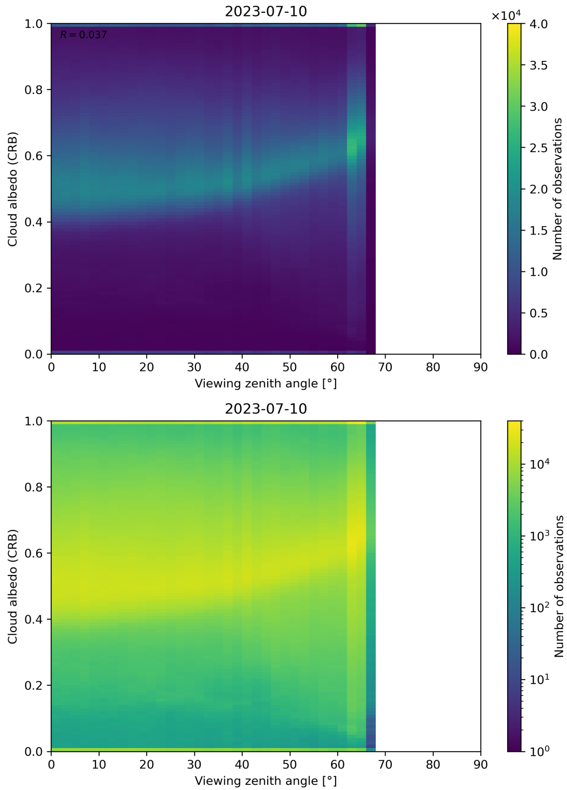
Figure 106: Scatter density plot of “Viewing zenith angle” against “Cloud albedo (CRB)” for 2023-07-09 to 2023-07-11.
