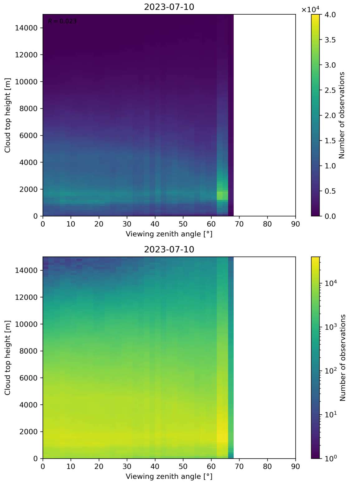
Figure 112: Scatter density plot of “Viewing zenith angle” against “Cloud top height” for 2023-07-09 to 2023-07-11.
