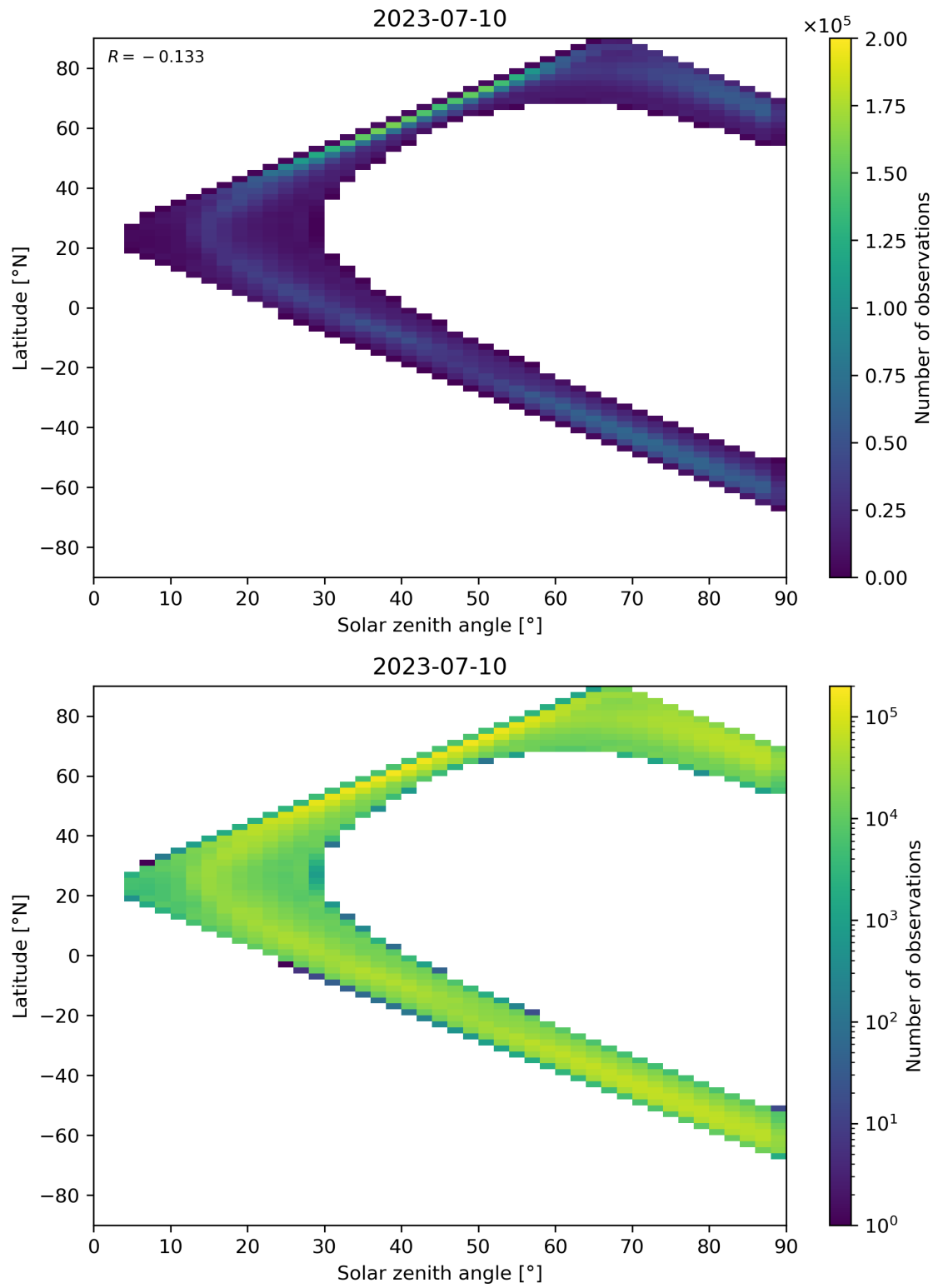
Figure 105: Scatter density plot of “Solar zenith angle” against “Latitude” for 2023-07-09 to 2023-07-11.
