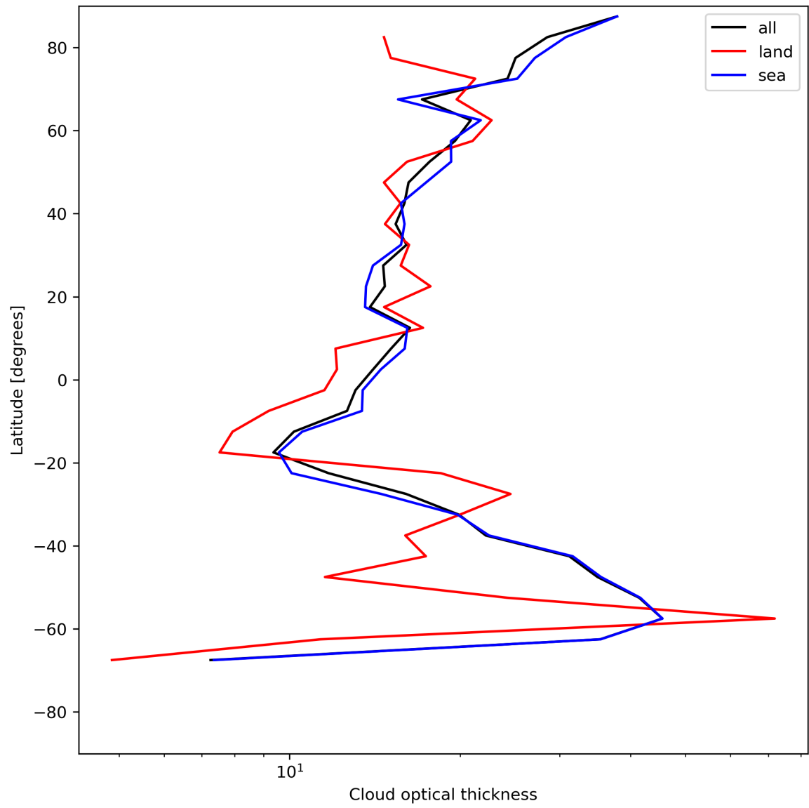
Figure 25: Zonal average of “Cloud optical thickness” for 2023-07-09 to 2023-07-11.
