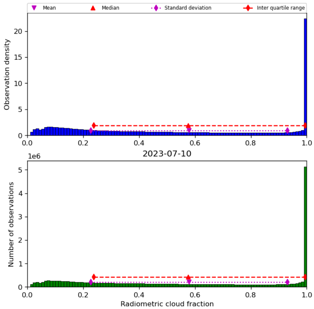
Figure 39: Histogram of “Radiometric cloud fraction” for 2023-07-09 to 2023-07-11
