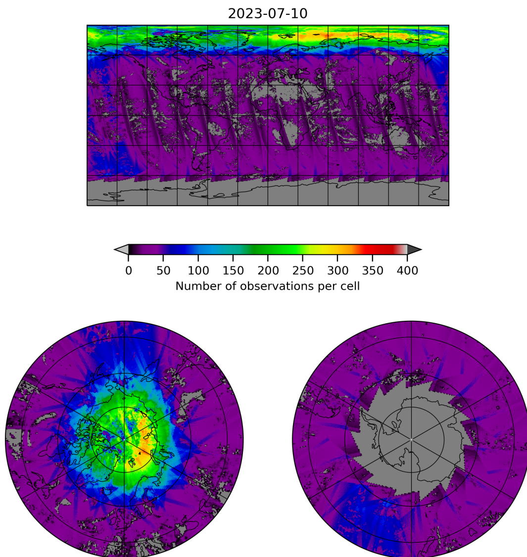
Figure 21: Map of the number of observations for 2023-07-09 to 2023-07-11
