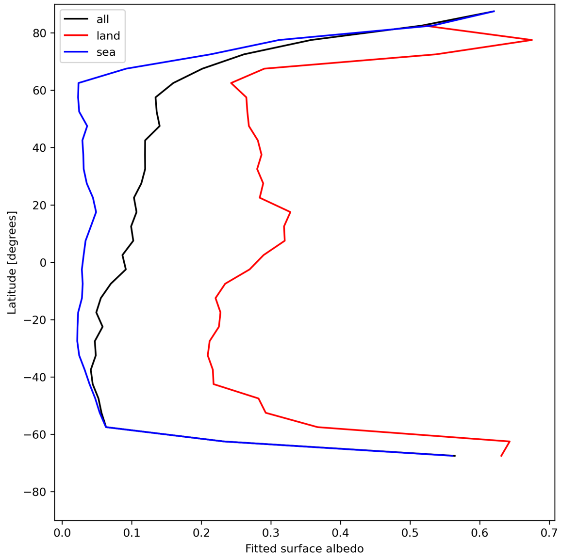
Figure 29: Zonal average of “Fitted surface albedo” for 2023-07-09 to 2023-07-11.
