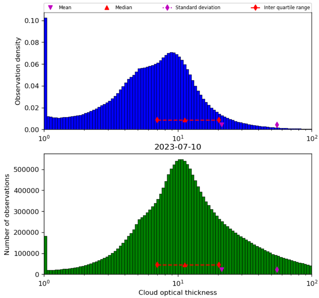
Figure 41: Histogram of “Cloud optical thickness” for 2023-07-09 to 2023-07-11
