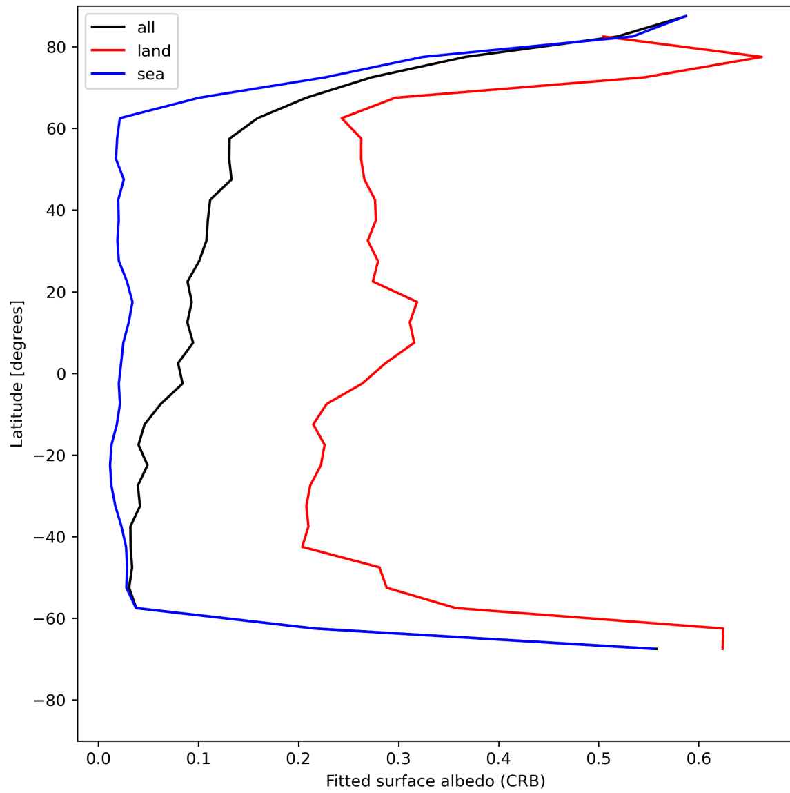
Figure 30: Zonal average of “Fitted surface albedo (CRB)” for 2023-07-09 to 2023-07-11.
