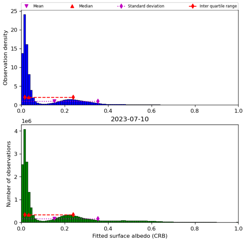
Figure 46: Histogram of “Fitted surface albedo (CRB)” for 2023-07-09 to 2023-07-11
