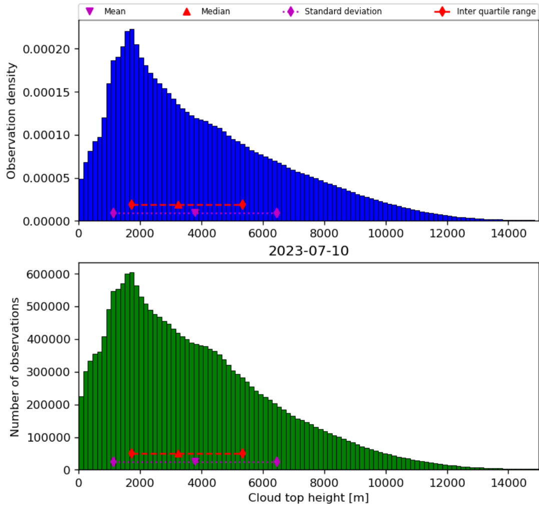
Figure 40: Histogram of “Cloud top height” for 2023-07-09 to 2023-07-11
