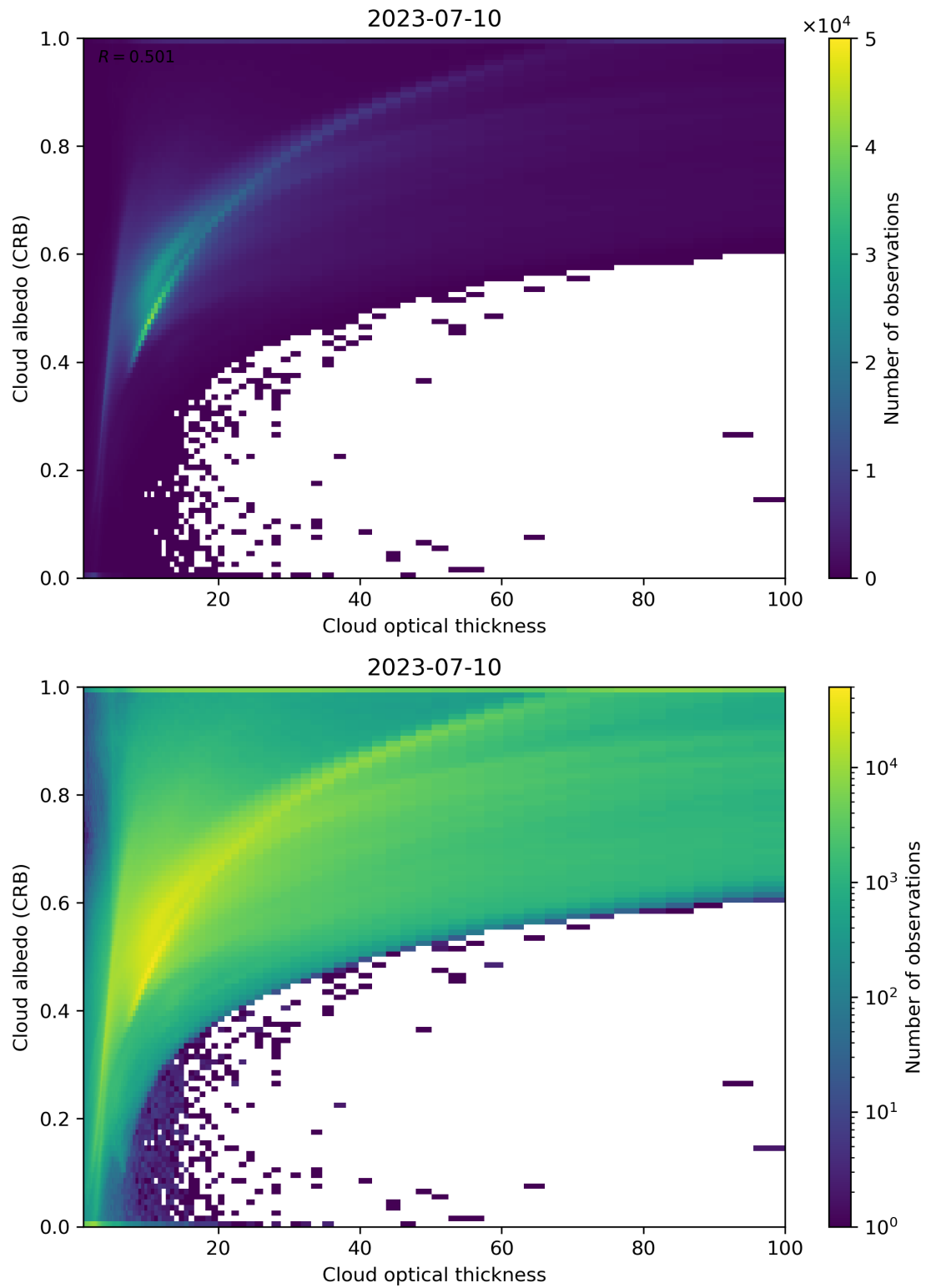
Figure 82: Scatter density plot of “Cloud optical thickness” against “Cloud albedo (CRB)” for 2023-07-09 to 2023-07-11.
