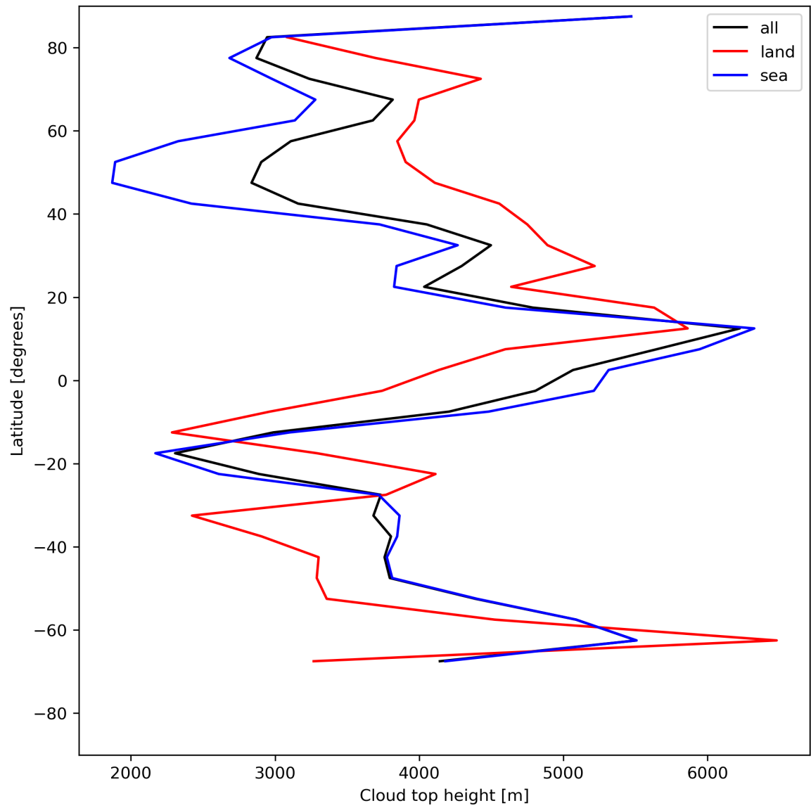
Figure 24: Zonal average of “Cloud top height” for 2023-07-09 to 2023-07-11.
