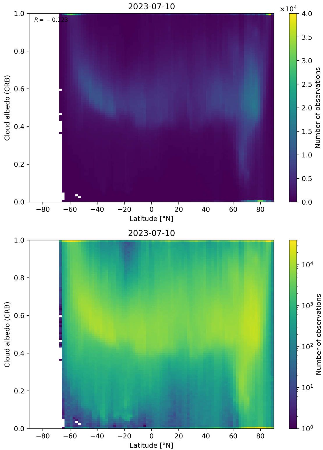
Figure 91: Scatter density plot of “Latitude” against “Cloud albedo (CRB)” for 2023-07-09 to 2023-07-11.
