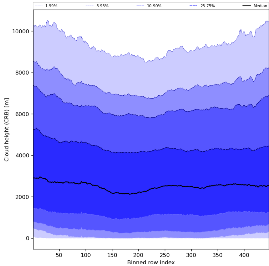
Figure 59: Along track statistics of “Cloud height (CRB)” for 2023-07-09 to 2023-07-11
