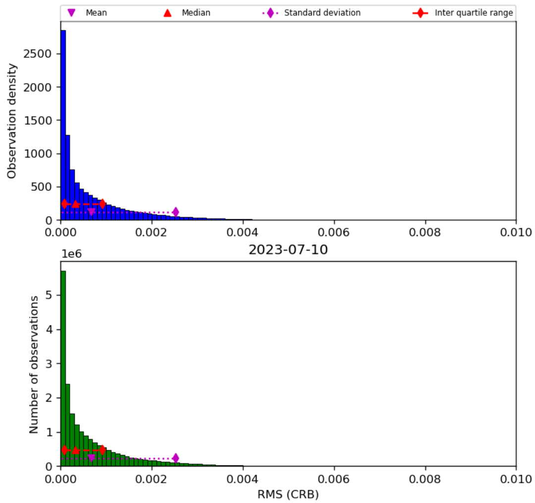
Figure 48: Histogram of “RMS (CRB)” for 2023-07-09 to 2023-07-11
