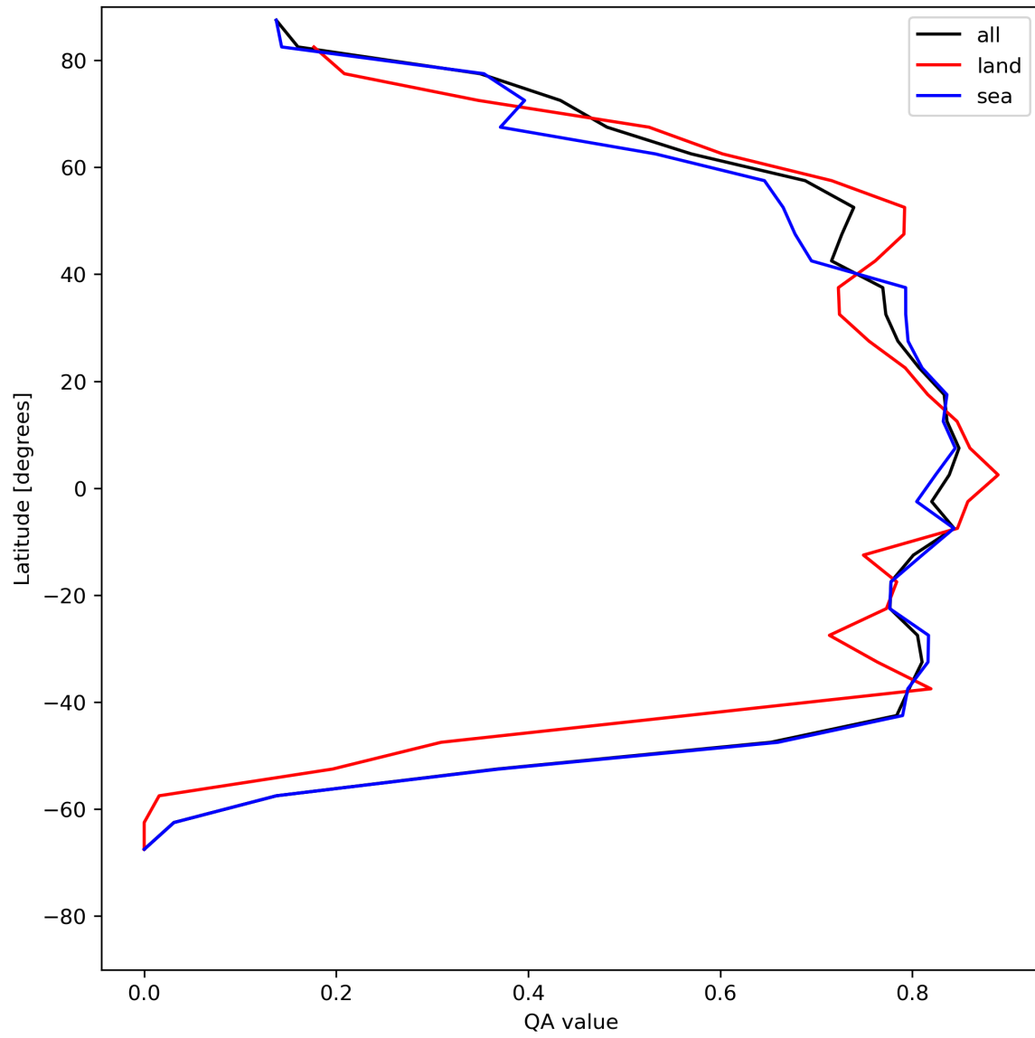
Figure 22: Zonal average of “QA value” for 2023-07-09 to 2023-07-11.
