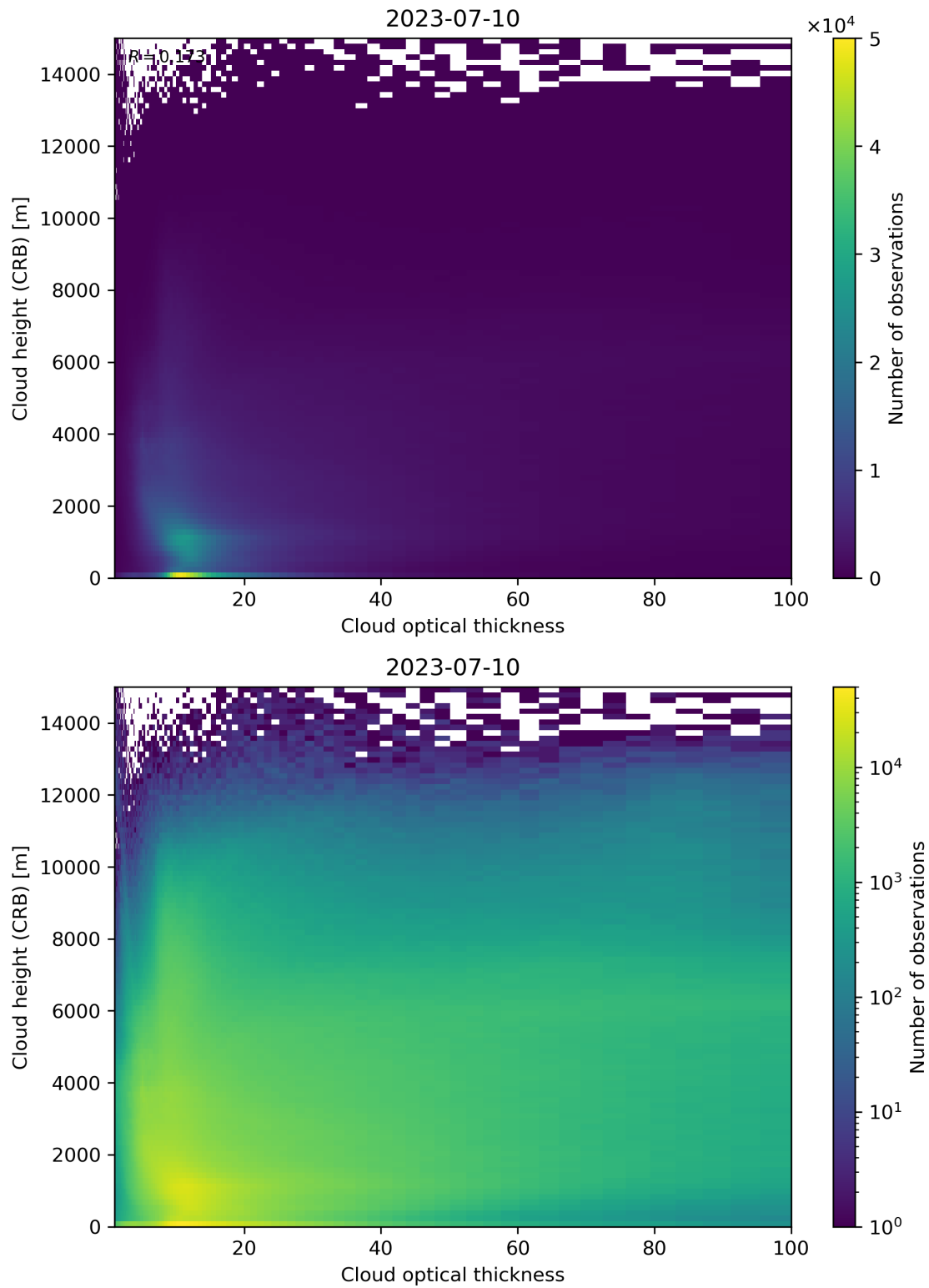
Figure 85: Scatter density plot of “Cloud optical thickness” against “Cloud height (CRB)” for 2023-07-09 to 2023-07-11.
