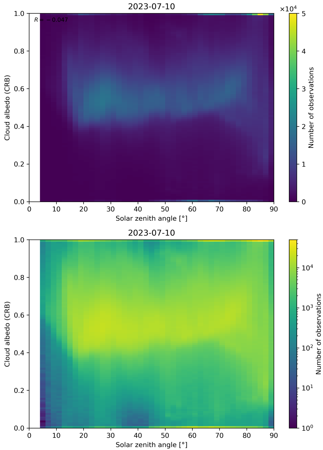
Figure 98: Scatter density plot of “Solar zenith angle” against “Cloud albedo (CRB)” for 2023-07-09 to 2023-07-11.
