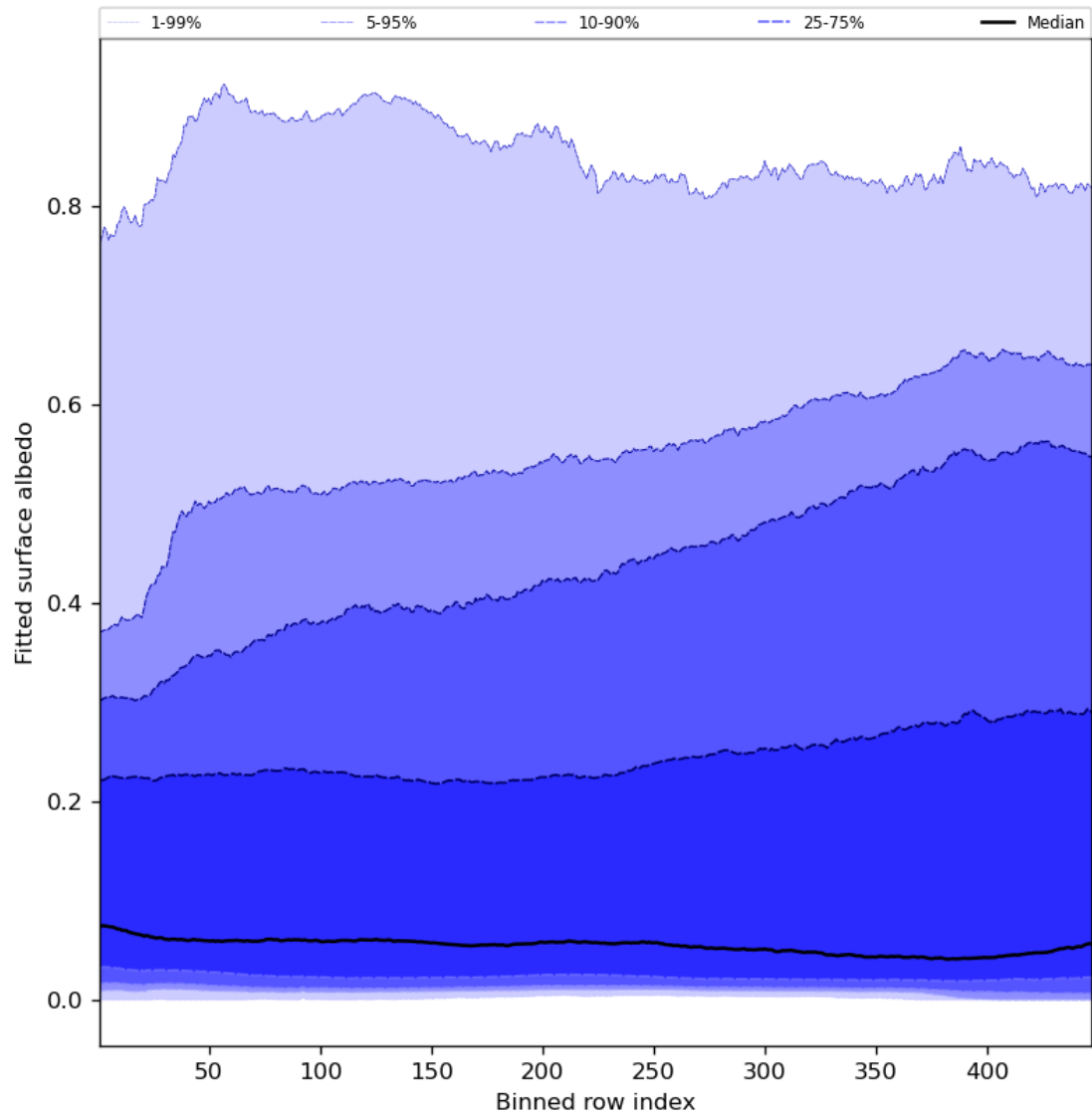
Figure 61: Along track statistics of “Fitted surface albedo” for 2023-07-09 to 2023-07-11
