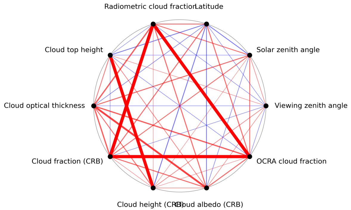
Figure 1: Map of correlation graph for 2023-07-09 to 2023-07-11.
