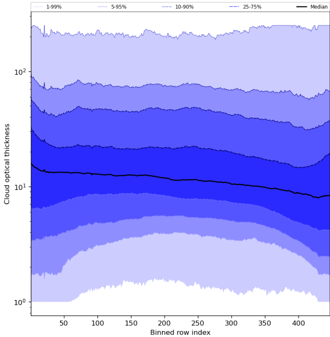
Figure 57: Along track statistics of “Cloud optical thickness” for 2023-07-09 to 2023-07-11
