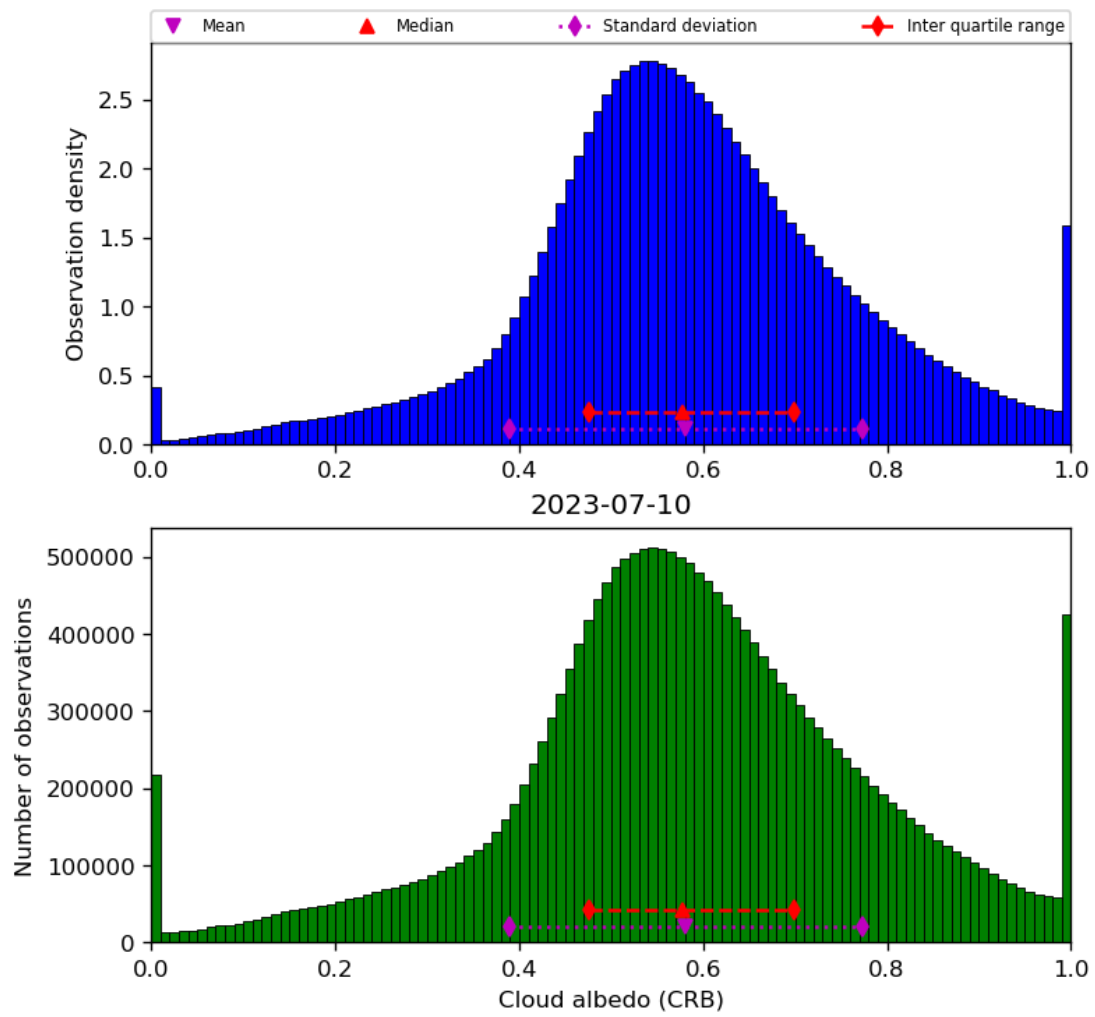
Figure 44: Histogram of “Cloud albedo (CRB)” for 2023-07-09 to 2023-07-11
