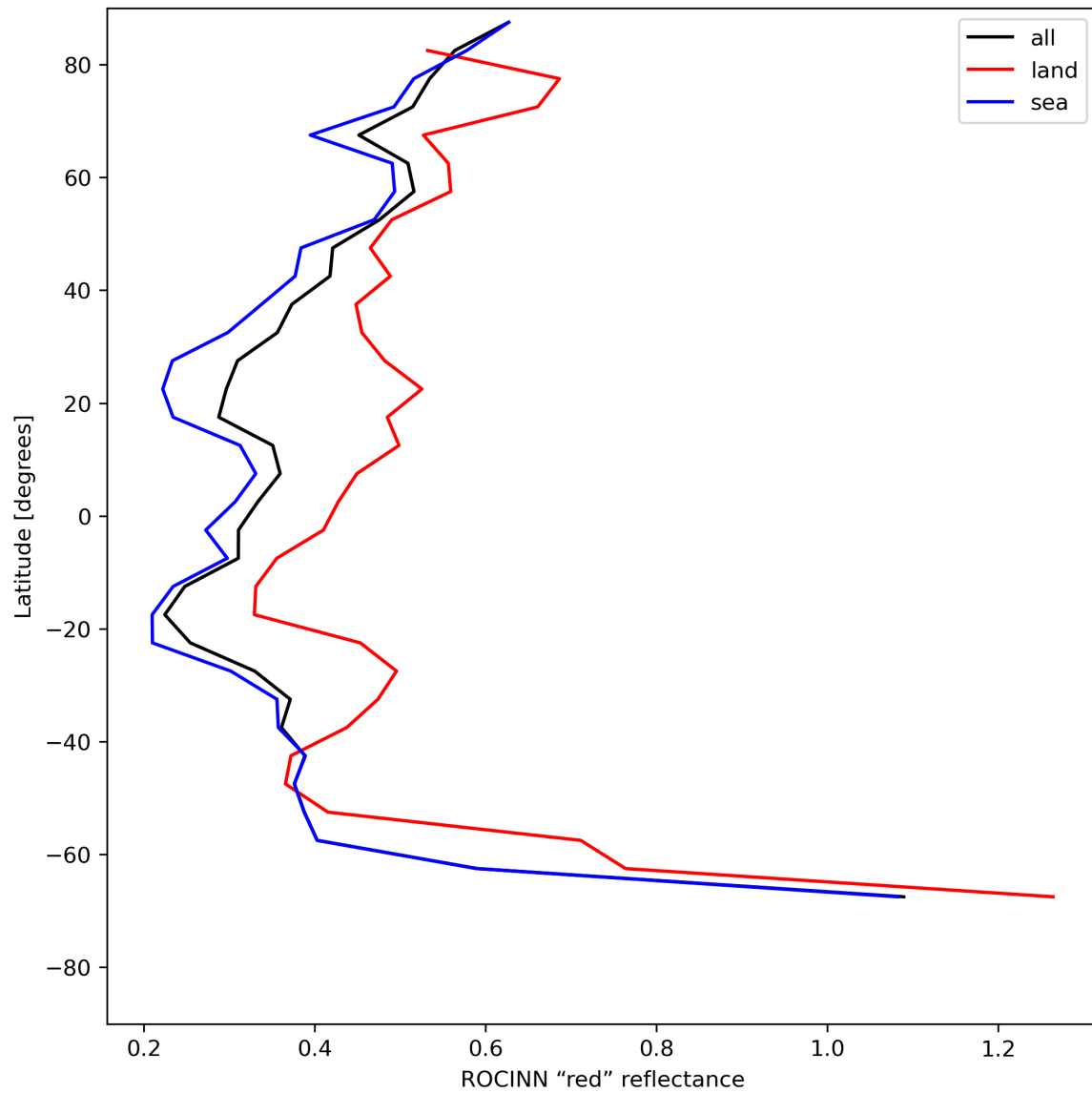
Figure 37: Zonal average of “ROCINN “red” reflectance” for 2023-07-09 to 2023-07-11.
