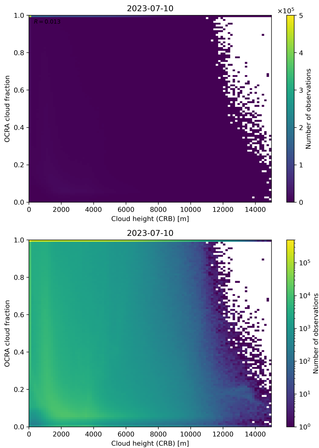
Figure 81: Scatter density plot of “Cloud height (CRB)” against “OCRA cloud fraction” for 2023-07-09 to 2023-07-11.
