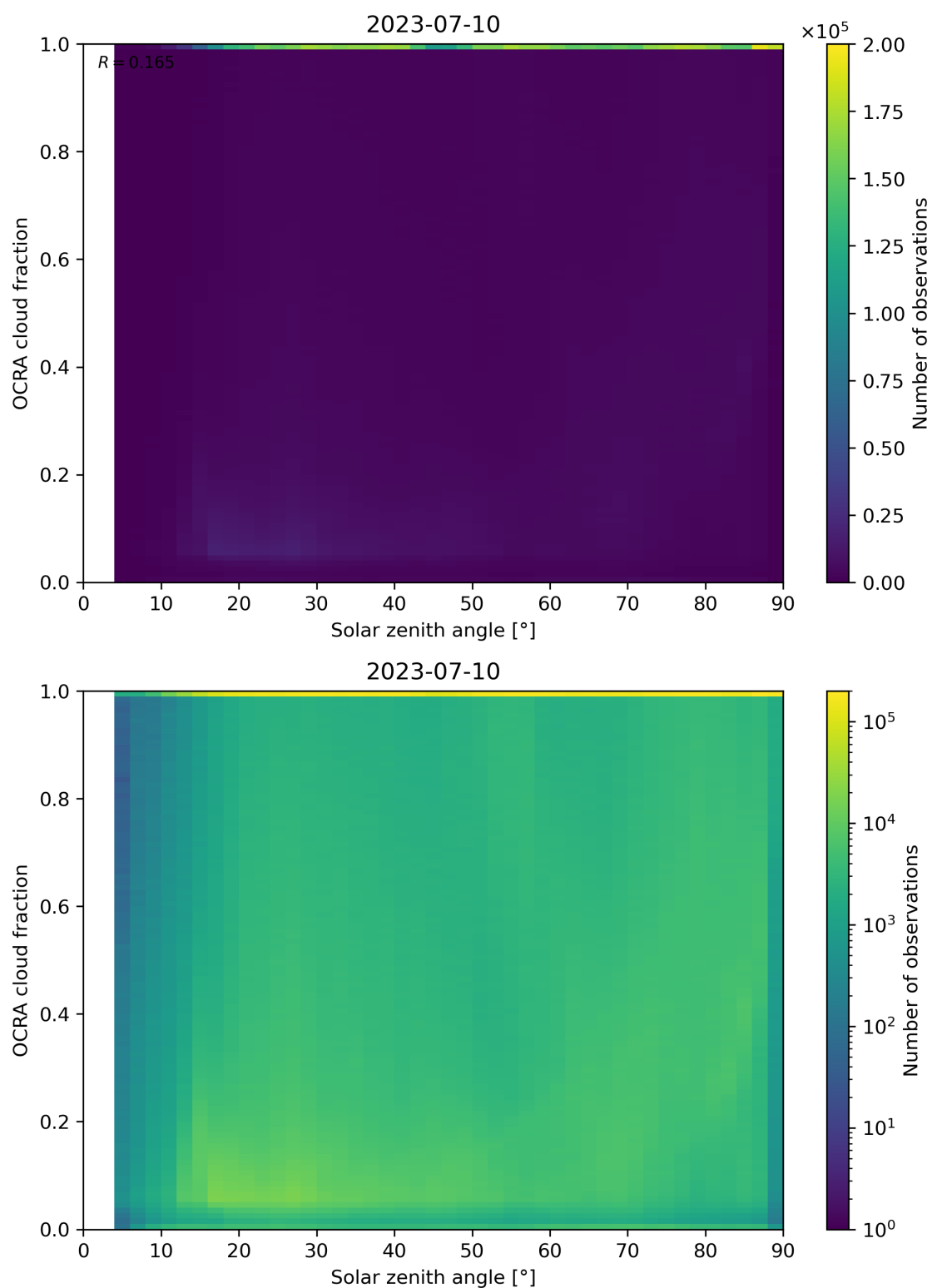
Figure 100: Scatter density plot of “Solar zenith angle” against “OCRA cloud fraction” for 2023-07-09 to 2023-07-11.
