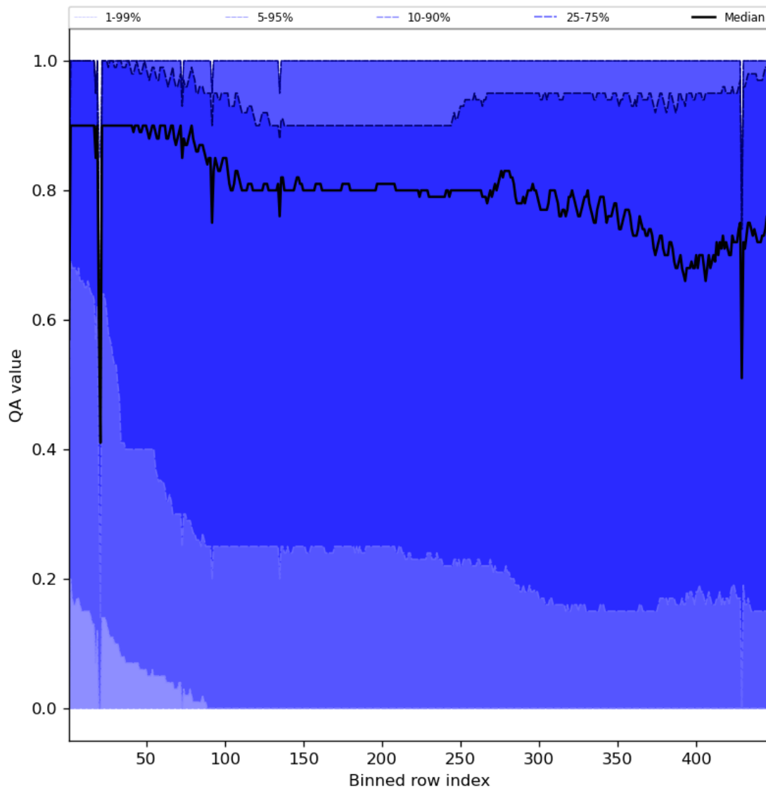
Figure 54: Along track statistics of “QA value” for 2023-07-09 to 2023-07-11
