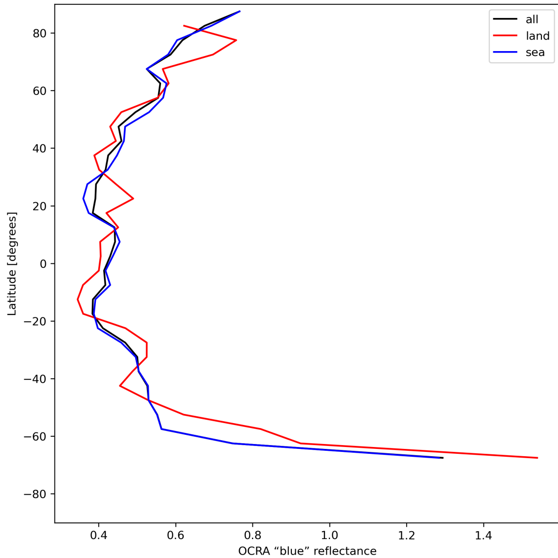
Figure 35: Zonal average of “OCRA “blue” reflectance” for 2023-07-09 to 2023-07-11.
