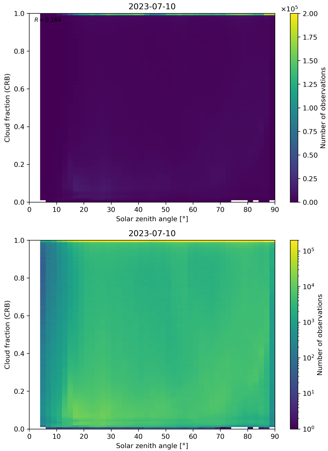
Figure 101: Scatter density plot of “Solar zenith angle” against “Cloud fraction (CRB)” for 2023-07-09 to 2023-07-11.
