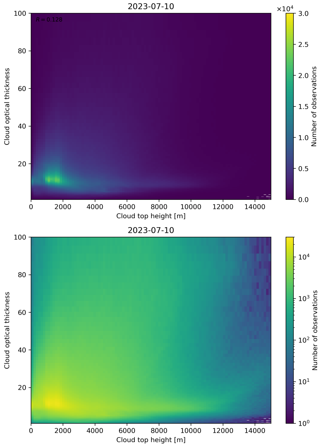
Figure 90: Scatter density plot of “Cloud top height” against “Cloud optical thickness” for 2023-07-09 to 2023-07-11.
