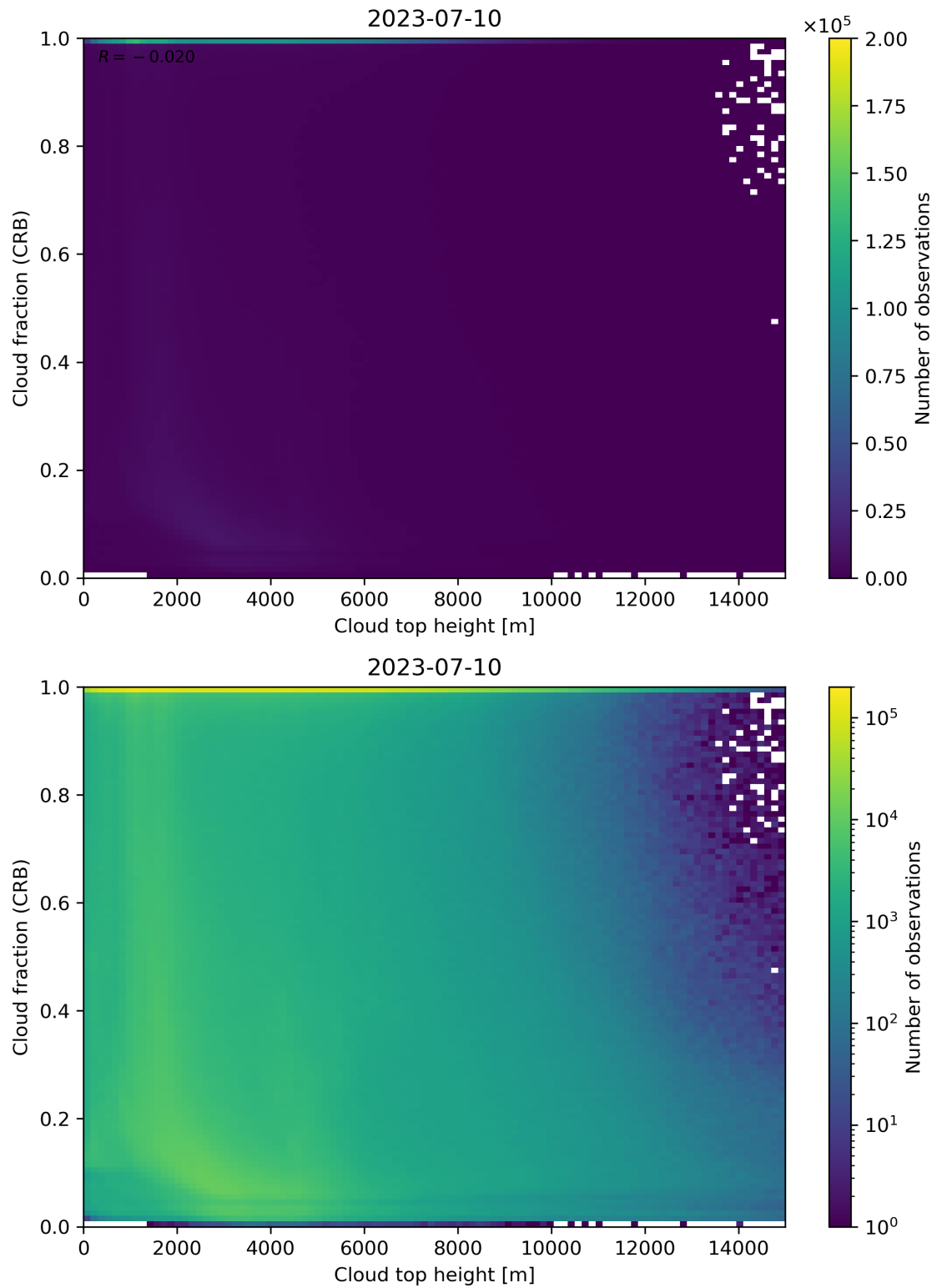
Figure 88: Scatter density plot of “Cloud top height” against “Cloud fraction (CRB)” for 2023-07-09 to 2023-07-11.
