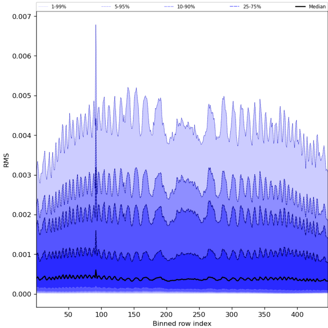
Figure 63: Along track statistics of “RMS” for 2023-07-09 to 2023-07-11
