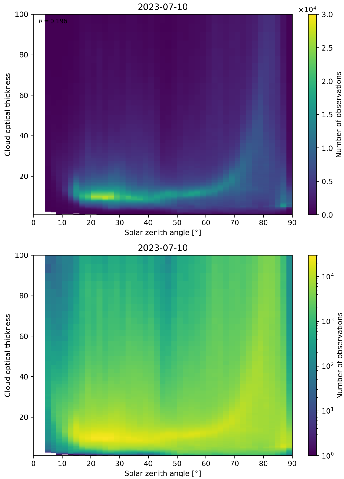
Figure 103: Scatter density plot of “Solar zenith angle” against “Cloud optical thickness” for 2023-07-09 to 2023-07-11.
