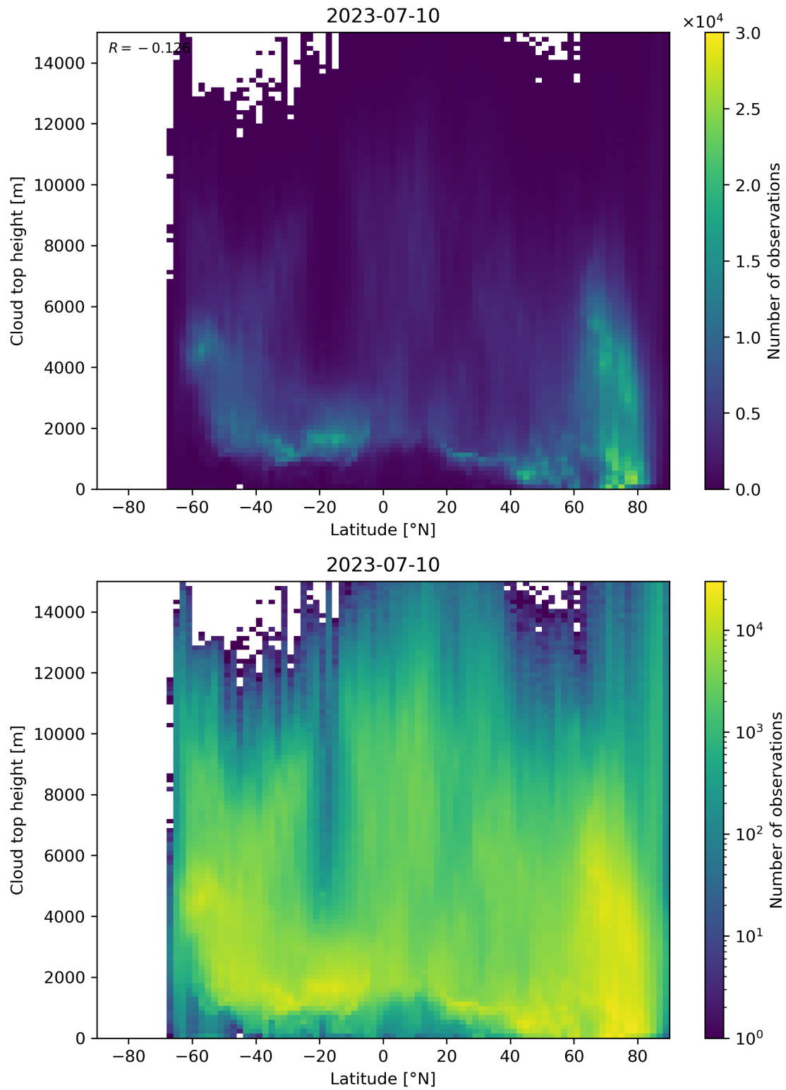
Figure 97: Scatter density plot of “Latitude” against “Cloud top height” for 2023-07-09 to 2023-07-11.
