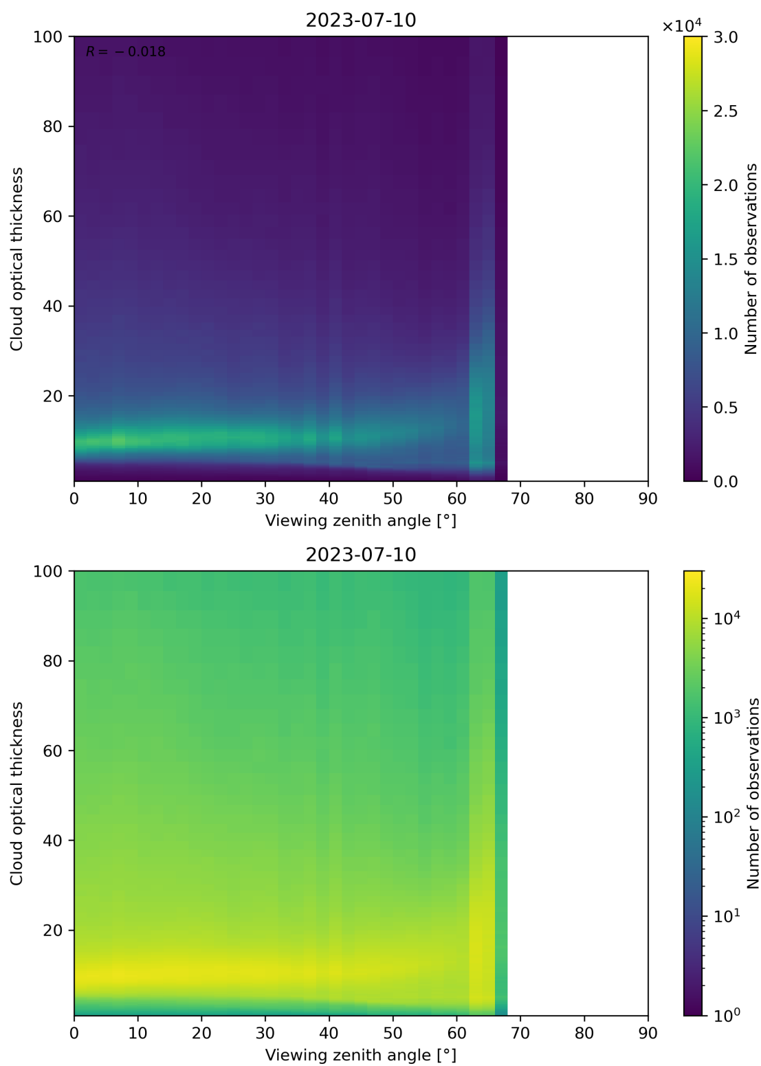
Figure 111: Scatter density plot of “Viewing zenith angle” against “Cloud optical thickness” for 2023-07-09 to 2023-07-11.
