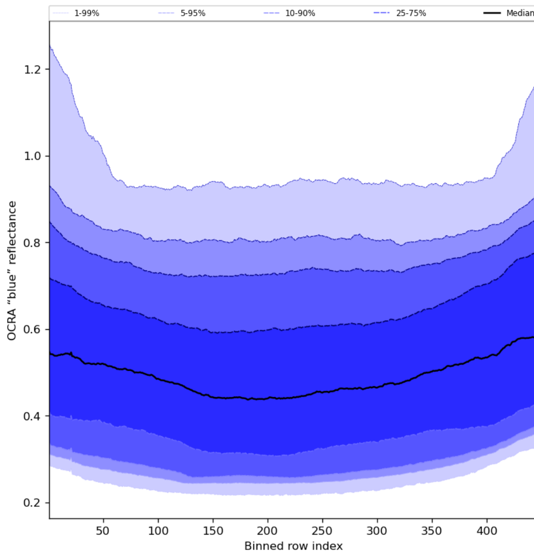
Figure 67: Along track statistics of “OCRA “blue” reflectance” for 2023-07-09 to 2023-07-11
