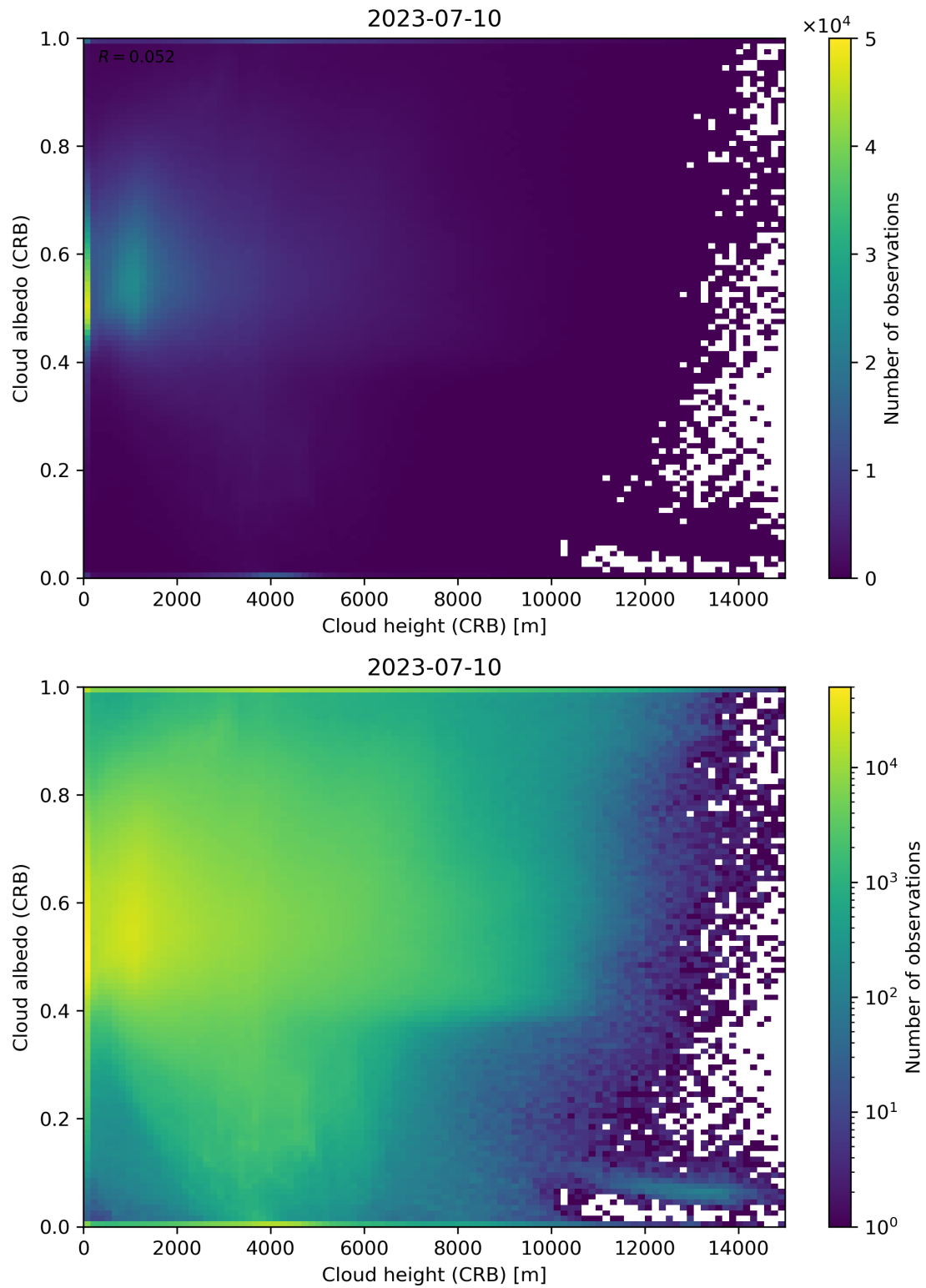
Figure 80: Scatter density plot of “Cloud height (CRB)” against “Cloud albedo (CRB)” for 2023-07-09 to 2023-07-11.
