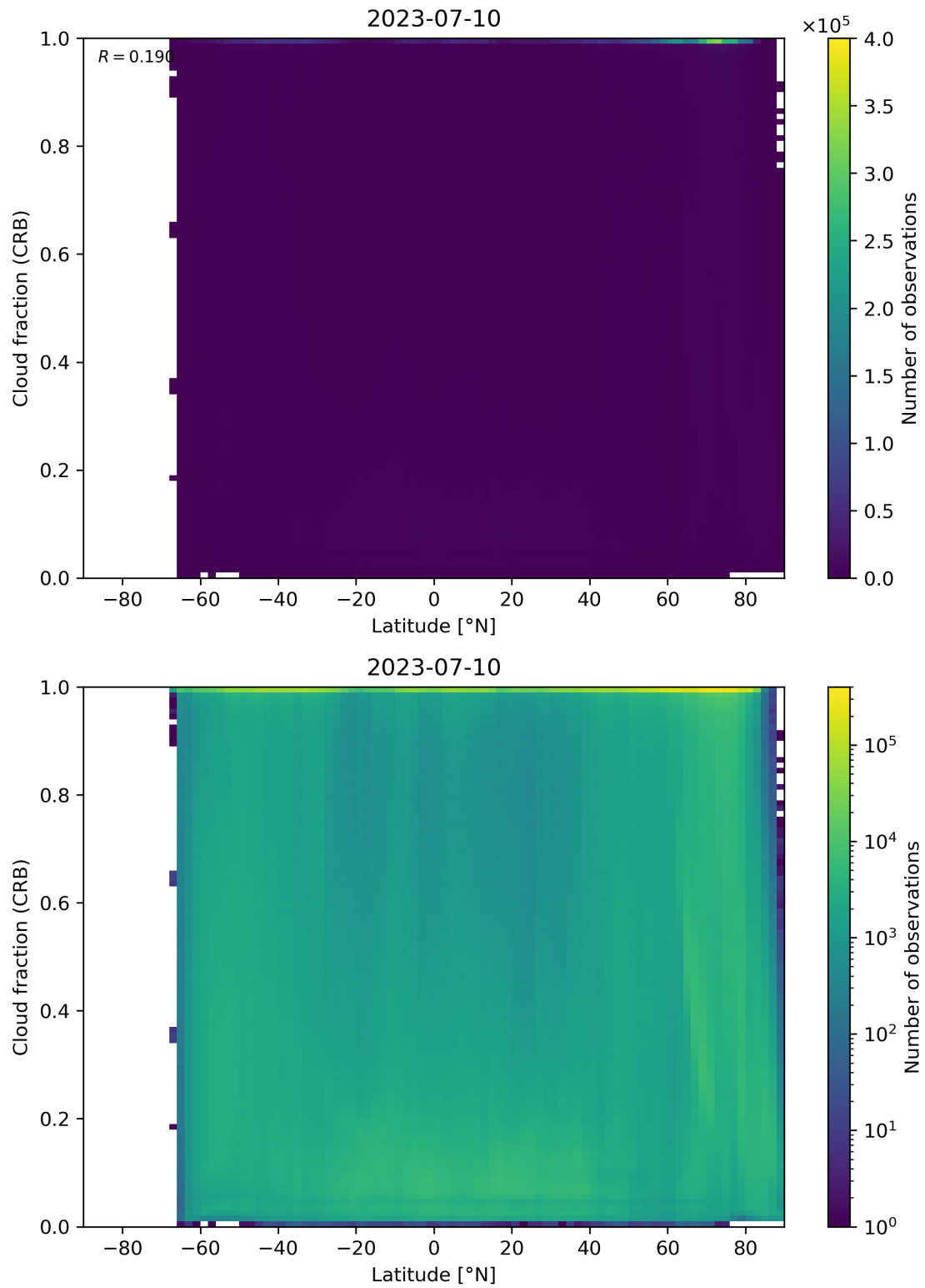
Figure 94: Scatter density plot of “Latitude” against “Cloud fraction (CRB)” for 2023-07-09 to 2023-07-11.
