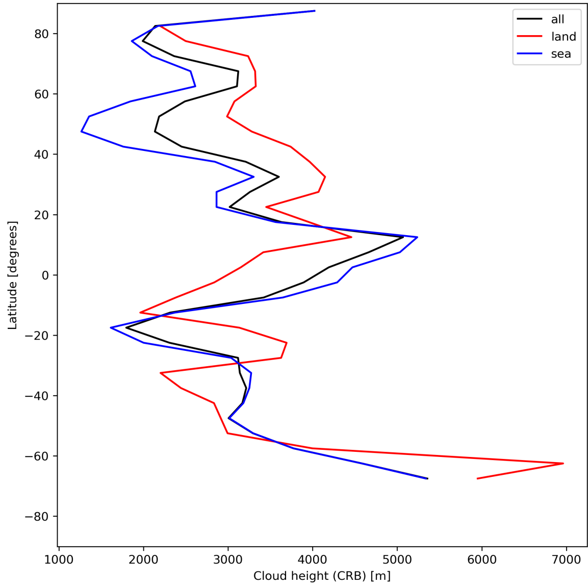
Figure 27: Zonal average of “Cloud height (CRB)” for 2023-07-09 to 2023-07-11.
