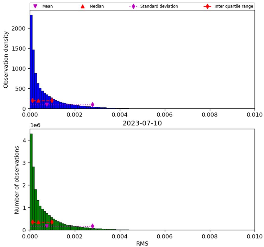
Figure 47: Histogram of “RMS” for 2023-07-09 to 2023-07-11
