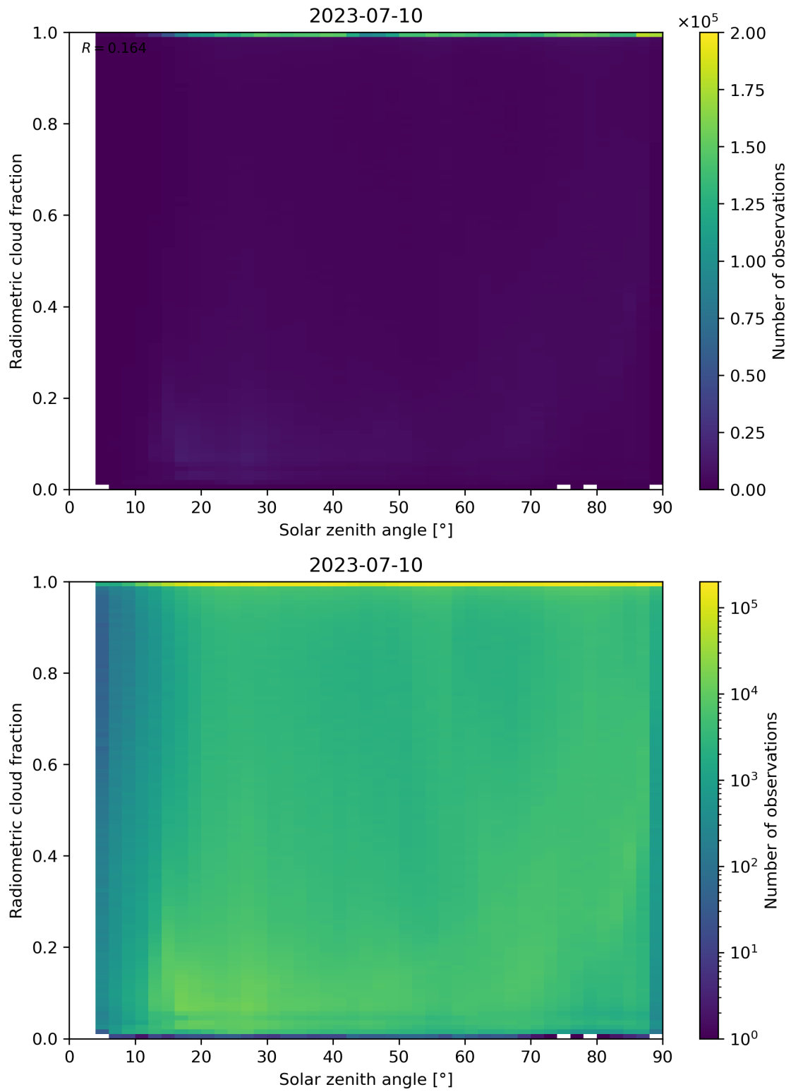
Figure 99: Scatter density plot of “Solar zenith angle” against “Radiometric cloud fraction” for 2023-07-09 to 2023-07-11.
