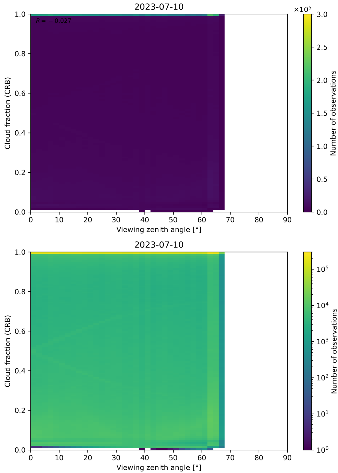
Figure 109: Scatter density plot of “Viewing zenith angle” against “Cloud fraction (CRB)” for 2023-07-09 to 2023-07-11.
