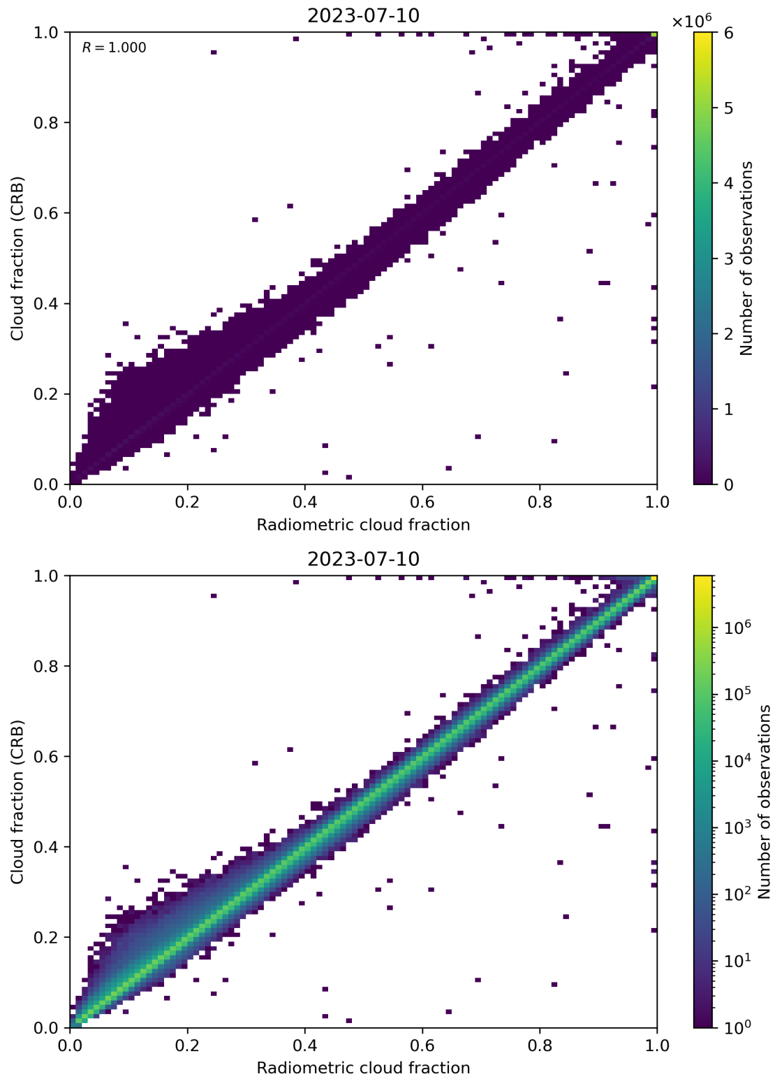
Figure 73: Scatter density plot of “Radiometric cloud fraction” against “Cloud fraction (CRB)” for 2023-07-09 to 2023-07-11.
