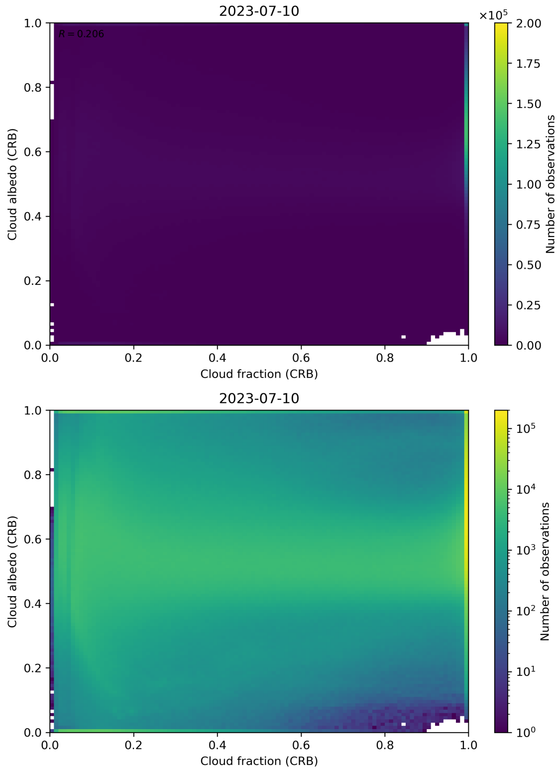
Figure 77: Scatter density plot of “Cloud fraction (CRB)” against “Cloud albedo (CRB)” for 2023-07-09 to 2023-07-11.
