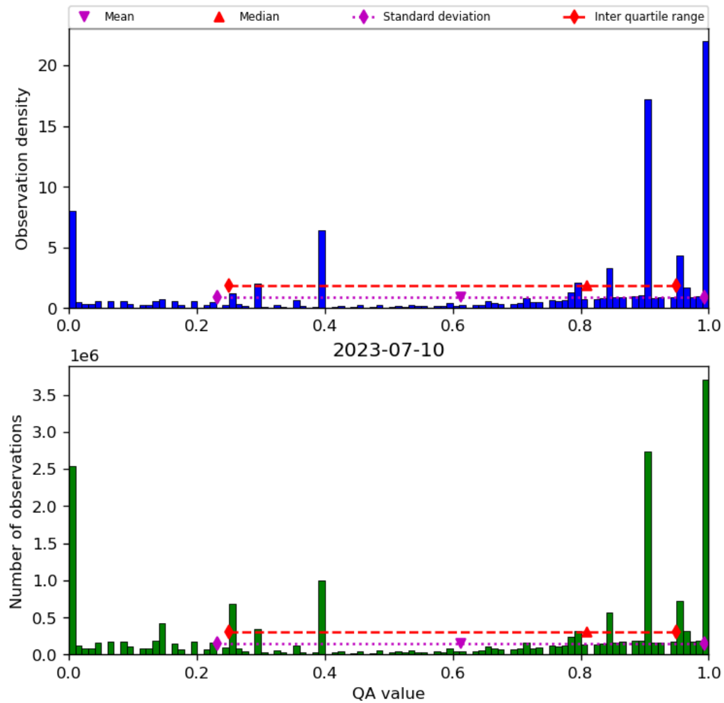
Figure 38: Histogram of “QA value” for 2023-07-09 to 2023-07-11
