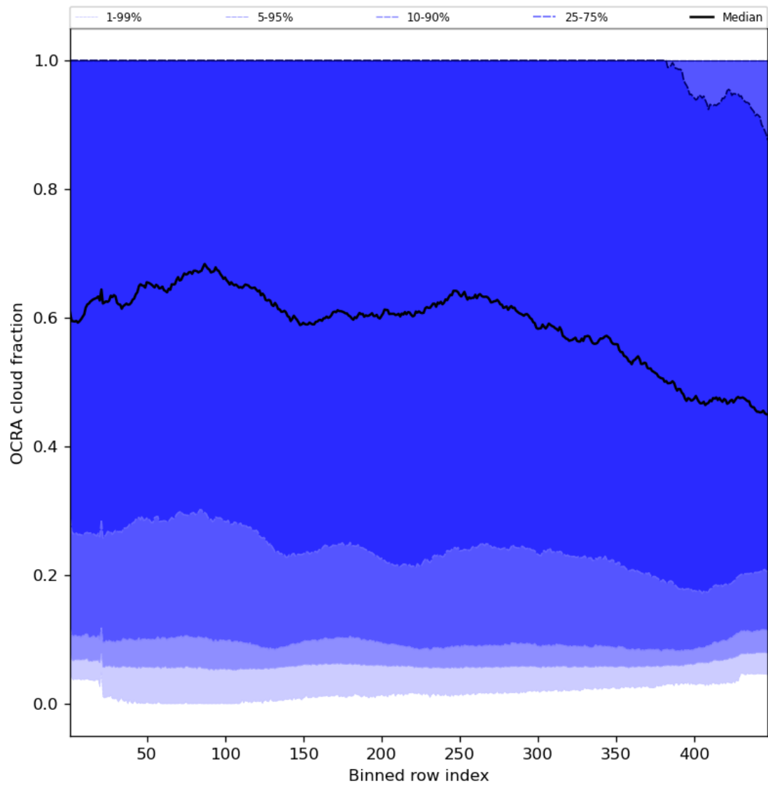
Figure 66: Along track statistics of “OCRA cloud fraction” for 2023-07-09 to 2023-07-11
