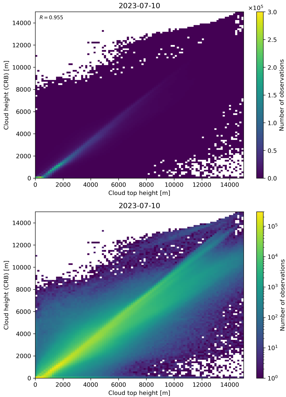
Figure 89: Scatter density plot of “Cloud top height” against “Cloud height (CRB)” for 2023-07-09 to 2023-07-11.
