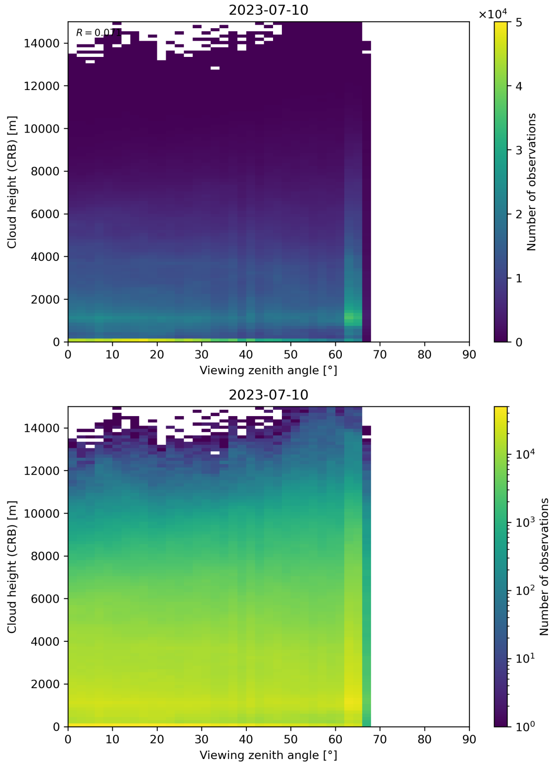
Figure 110: Scatter density plot of “Viewing zenith angle” against “Cloud height (CRB)” for 2023-07-09 to 2023-07-11.
