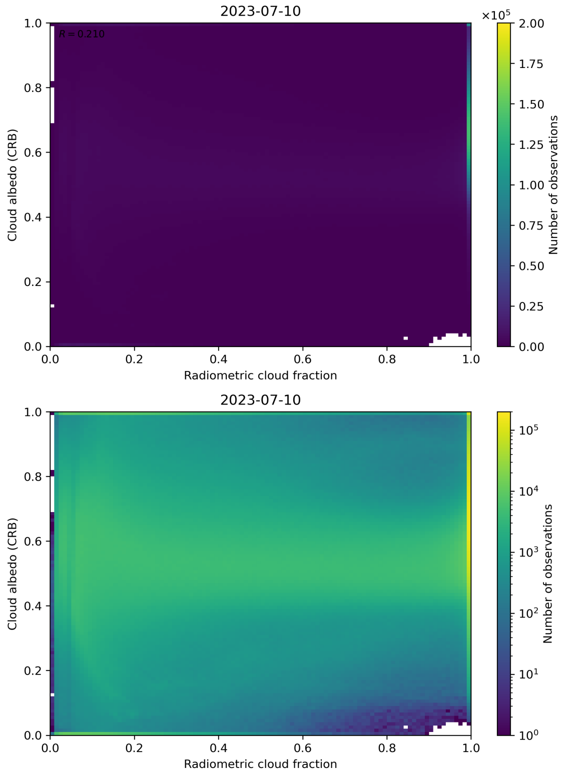
Figure 71: Scatter density plot of “Radiometric cloud fraction” against “Cloud albedo (CRB)” for 2023-07-09 to 2023-07-11.
