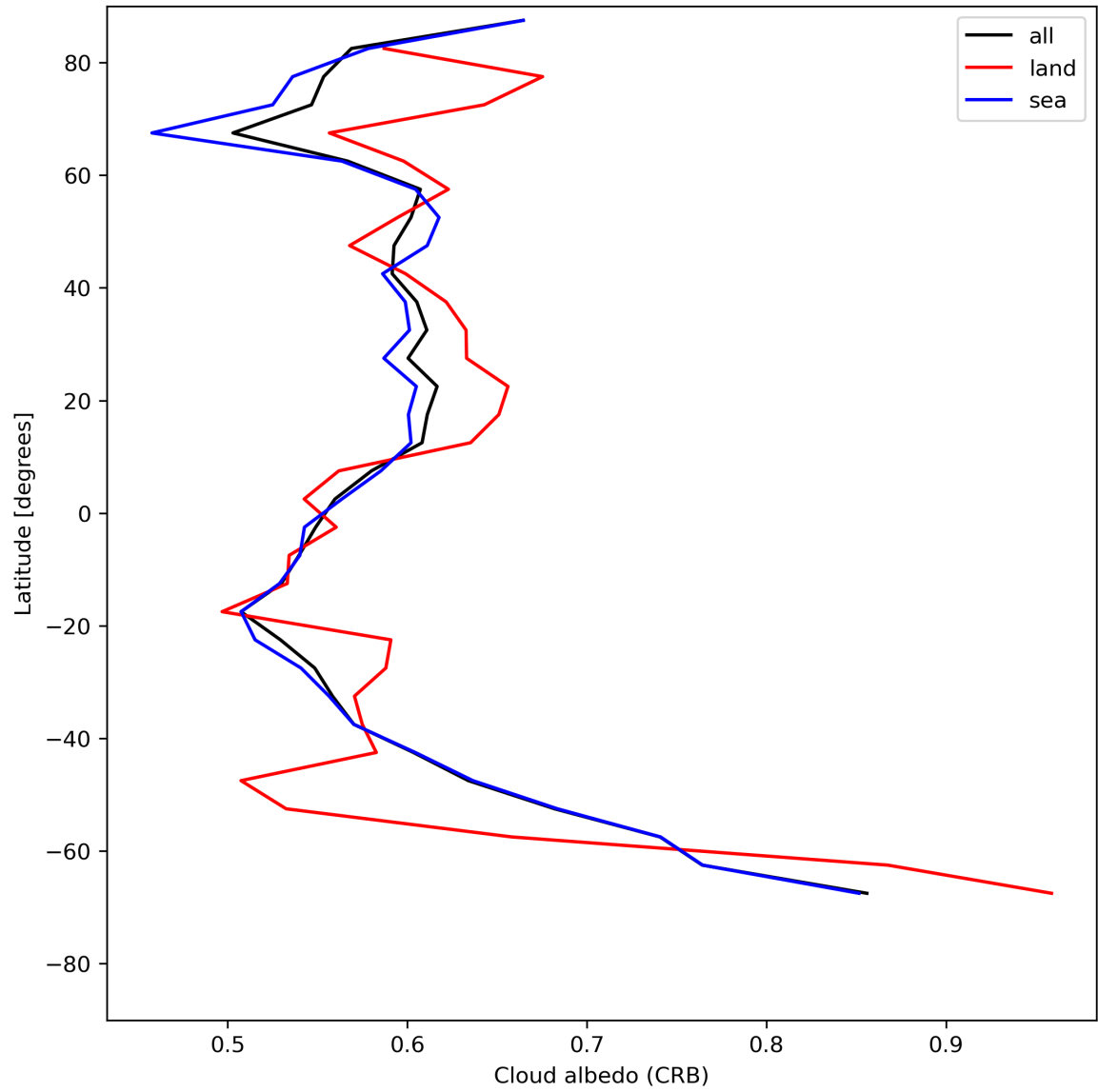
Figure 28: Zonal average of “Cloud albedo (CRB)” for 2023-07-09 to 2023-07-11.
