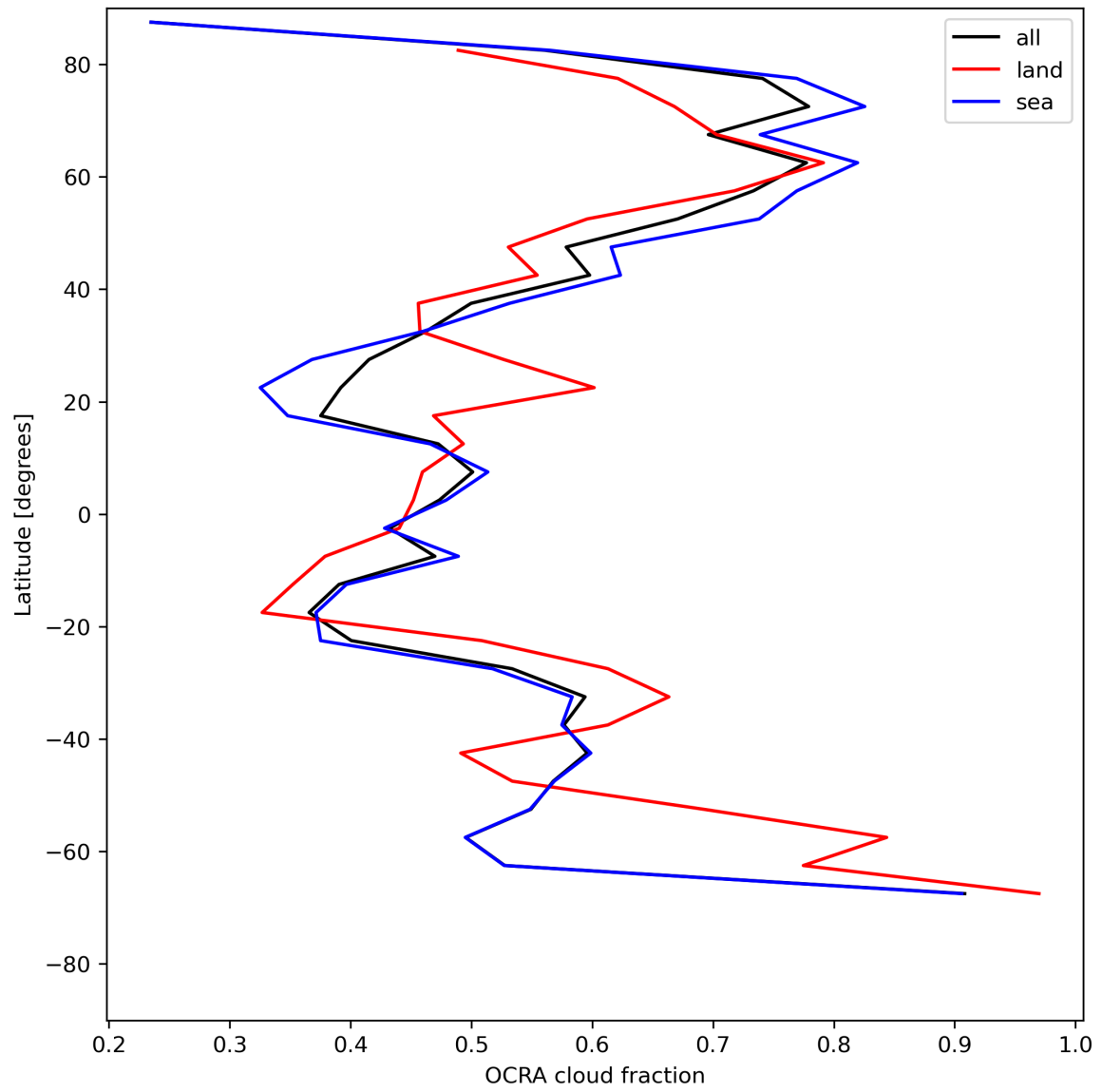
Figure 34: Zonal average of “OCRA cloud fraction” for 2023-07-09 to 2023-07-11.
