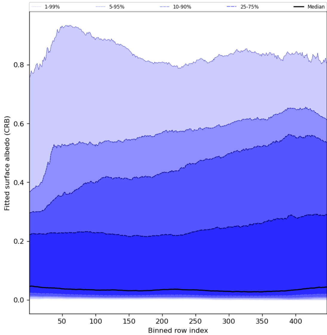
Figure 62: Along track statistics of “Fitted surface albedo (CRB)” for 2023-07-09 to 2023-07-11
