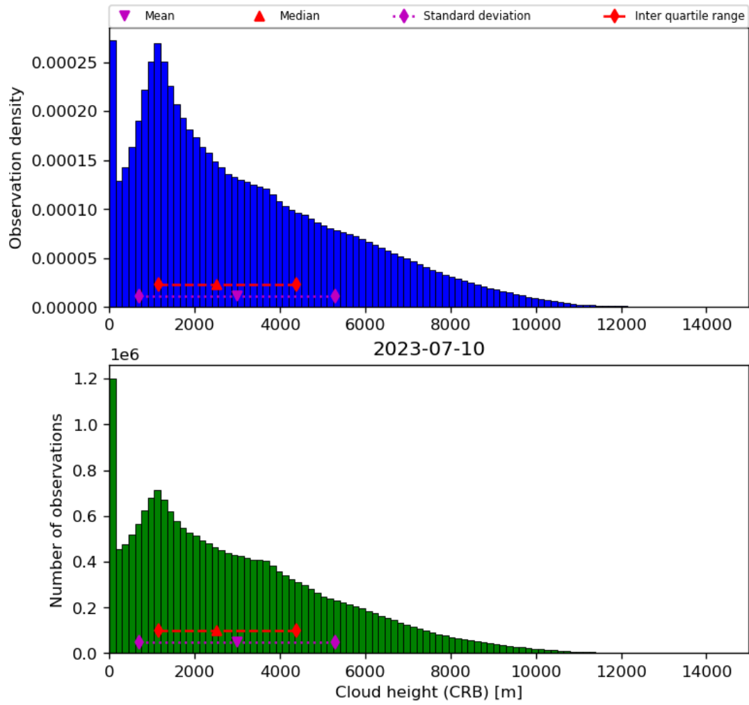
Figure 43: Histogram of “Cloud height (CRB)” for 2023-07-09 to 2023-07-11
