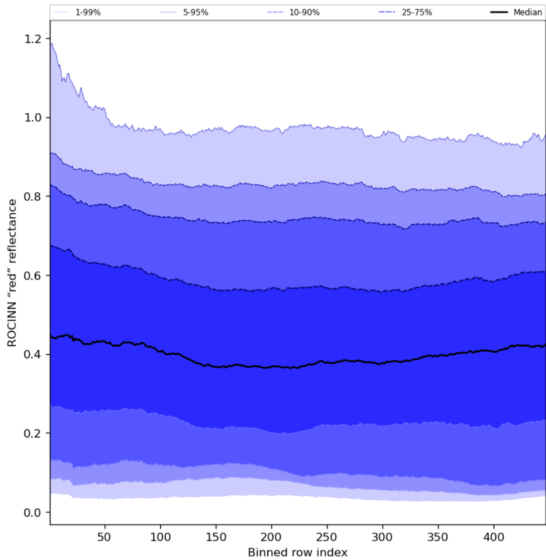
Figure 69: Along track statistics of “ROCINN “red” reflectance” for 2023-07-09 to 2023-07-11
