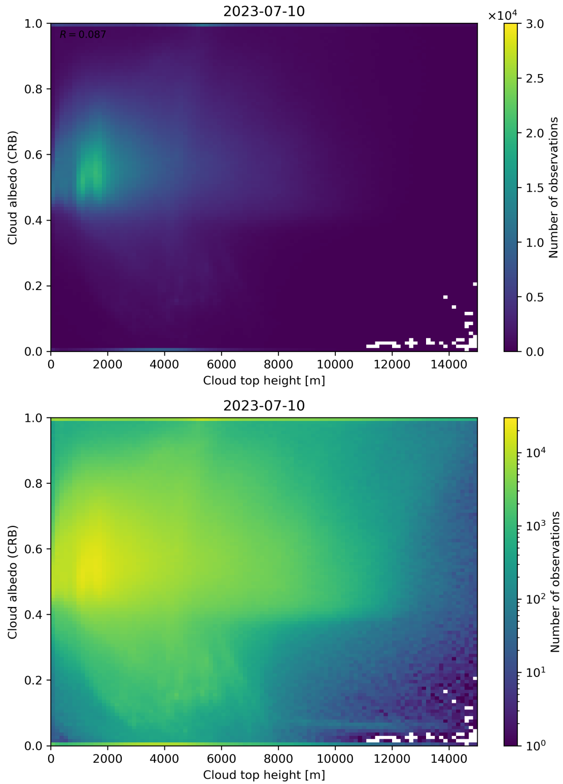
Figure 86: Scatter density plot of “Cloud top height” against “Cloud albedo (CRB)” for 2023-07-09 to 2023-07-11.
