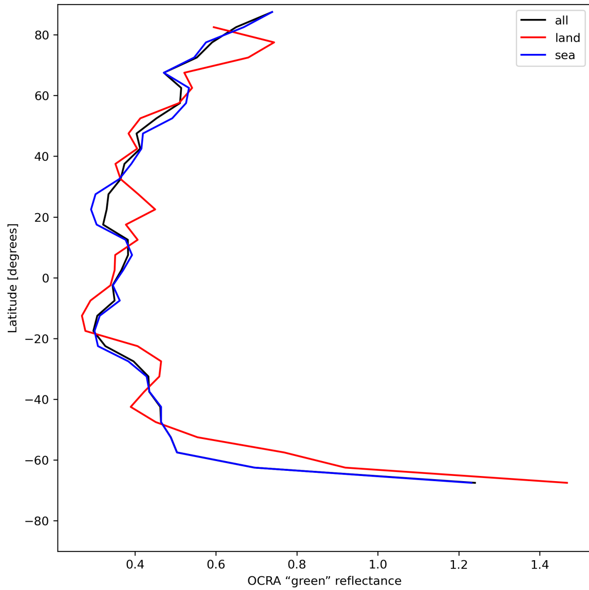
Figure 36: Zonal average of “OCRA “green” reflectance” for 2023-07-09 to 2023-07-11.
