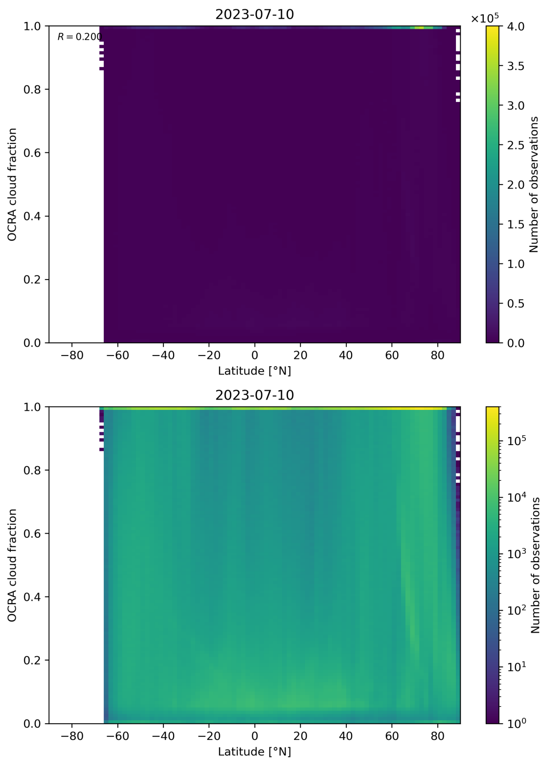
Figure 93: Scatter density plot of “Latitude” against “OCRA cloud fraction” for 2023-07-09 to 2023-07-11.
