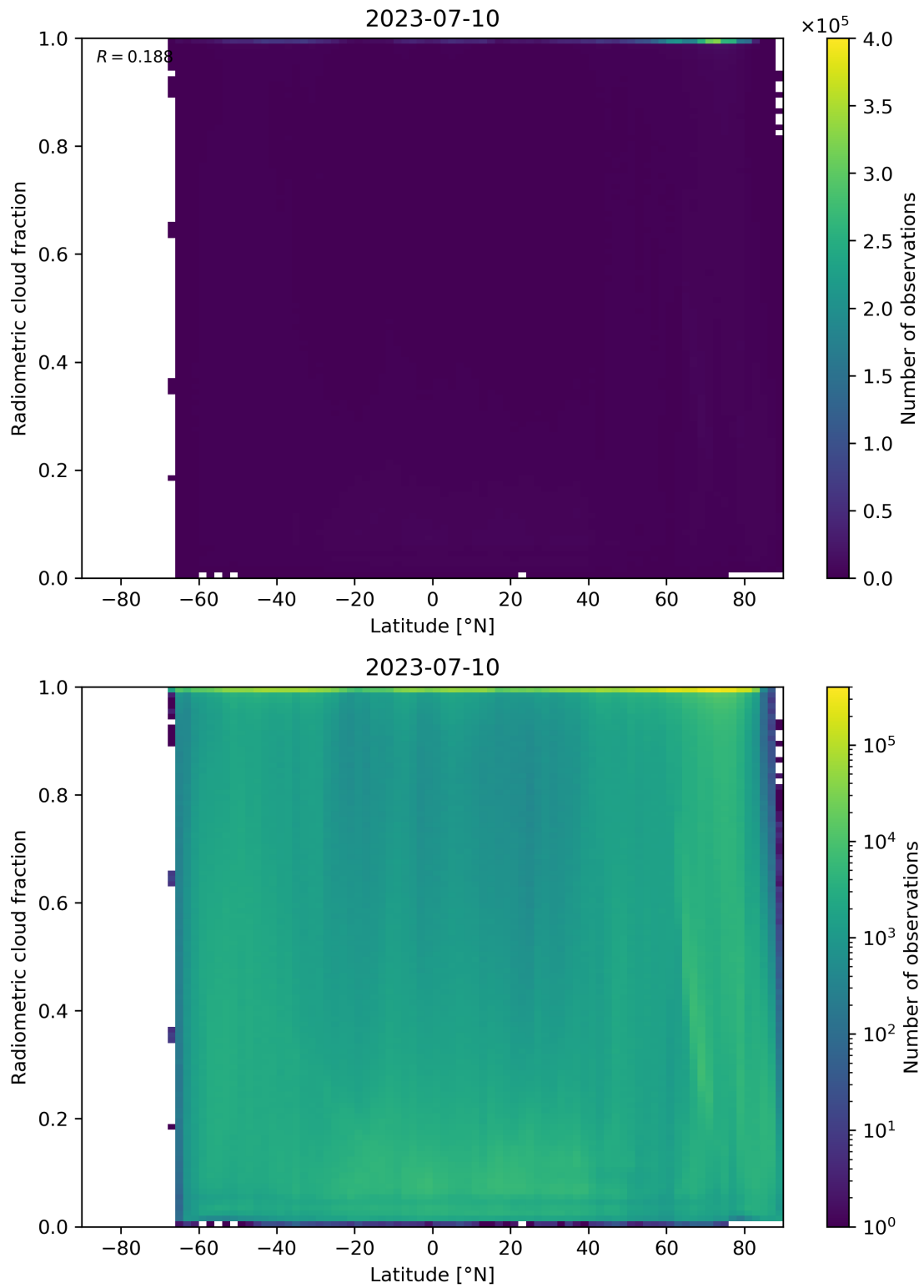
Figure 92: Scatter density plot of “Latitude” against “Radiometric cloud fraction” for 2023-07-09 to 2023-07-11.
