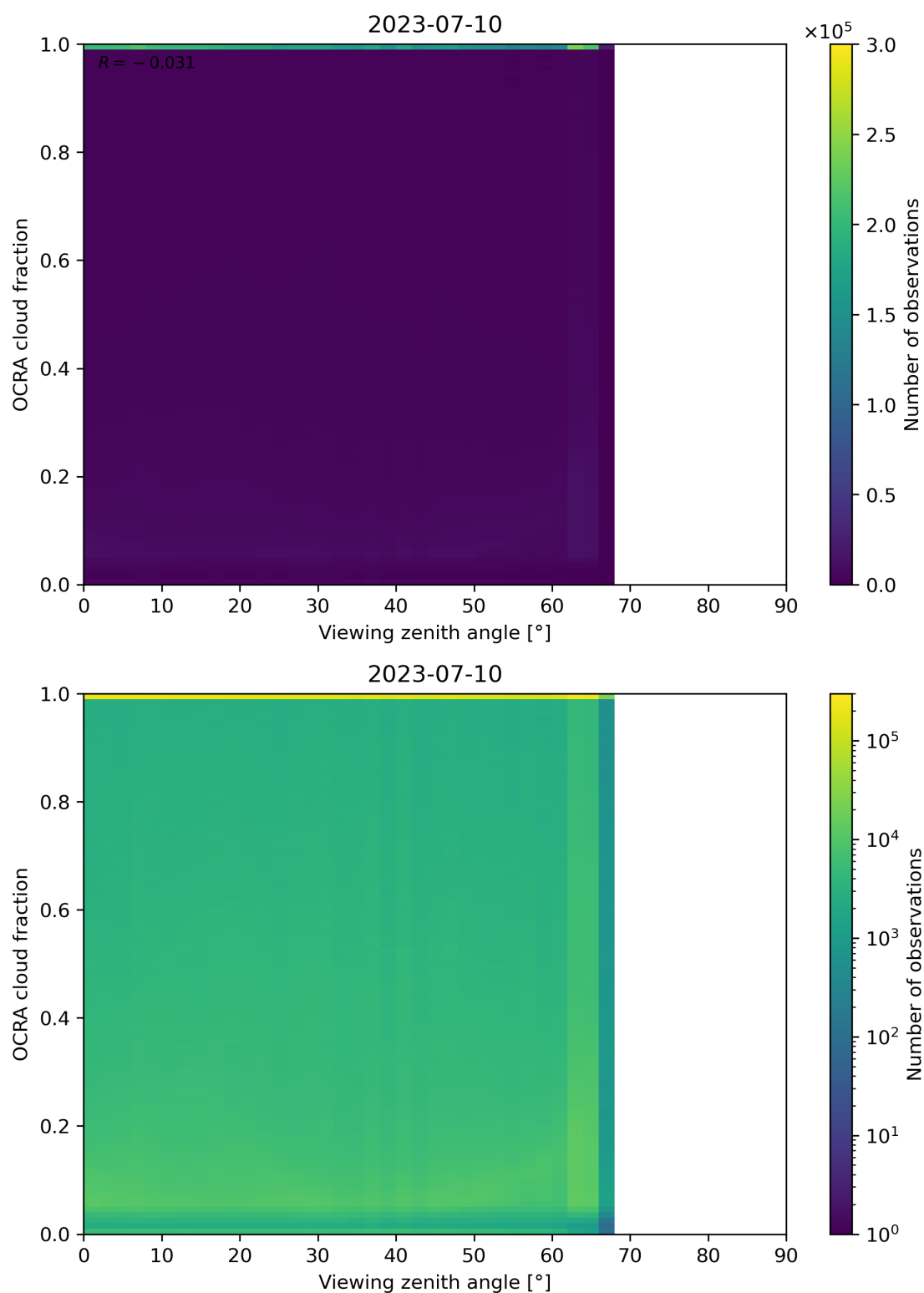
Figure 108: Scatter density plot of “Viewing zenith angle” against “OCRA cloud fraction” for 2023-07-09 to 2023-07-11.
