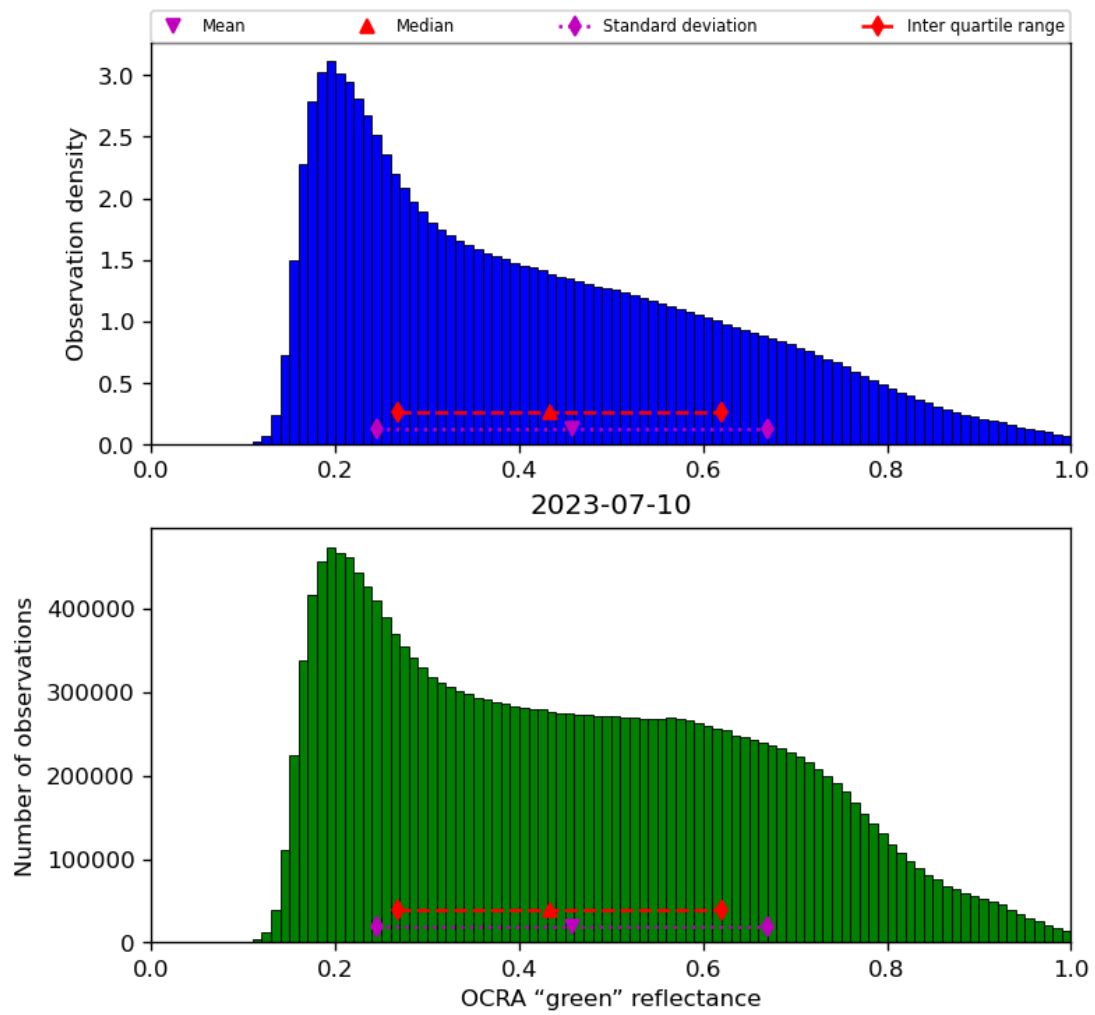
Figure 52: Histogram of “OCRA “green” reflectance” for 2023-07-09 to 2023-07-11
