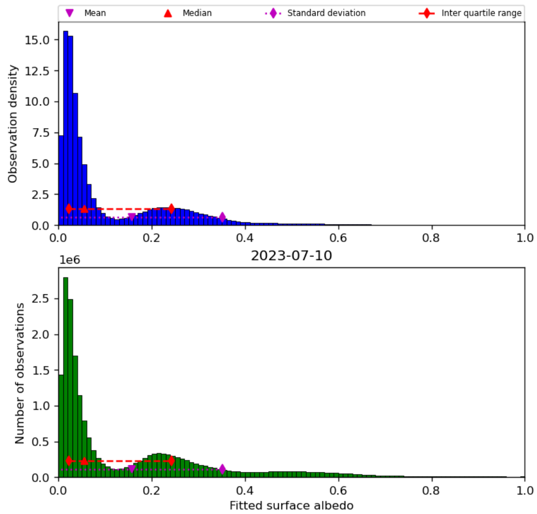
Figure 45: Histogram of “Fitted surface albedo” for 2023-07-09 to 2023-07-11
