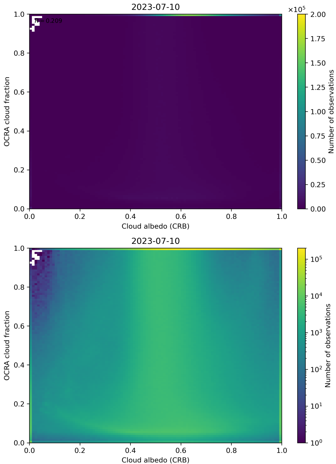
Figure 70: Scatter density plot of “Cloud albedo (CRB)” against “OCRA cloud fraction” for 2023-07-09 to 2023-07-11.
