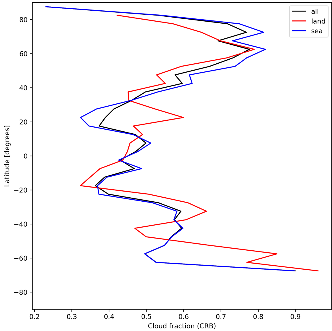
Figure 26: Zonal average of “Cloud fraction (CRB)” for 2023-07-09 to 2023-07-11.
