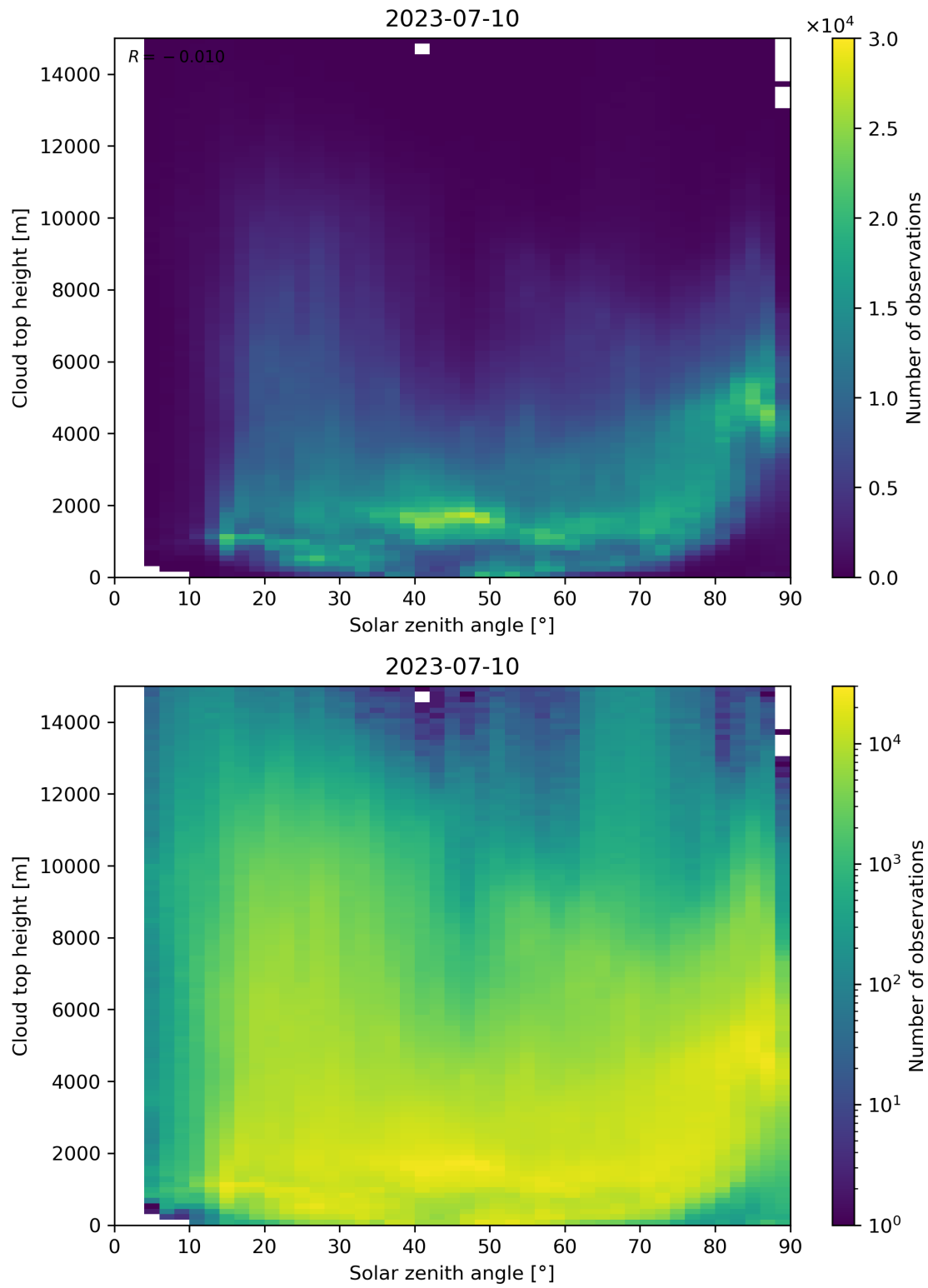
Figure 104: Scatter density plot of “Solar zenith angle” against “Cloud top height” for 2023-07-09 to 2023-07-11.
