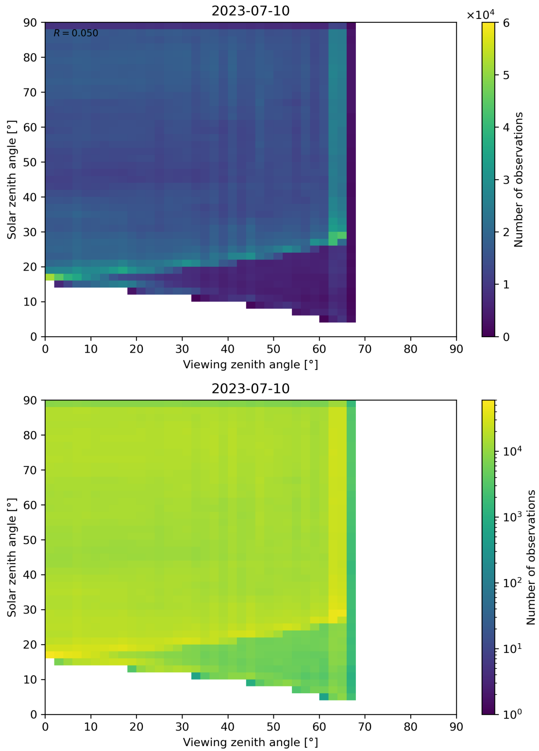
Figure 114: Scatter density plot of “Viewing zenith angle” against “Solar zenith angle” for 2023-07-09 to 2023-07-11.
