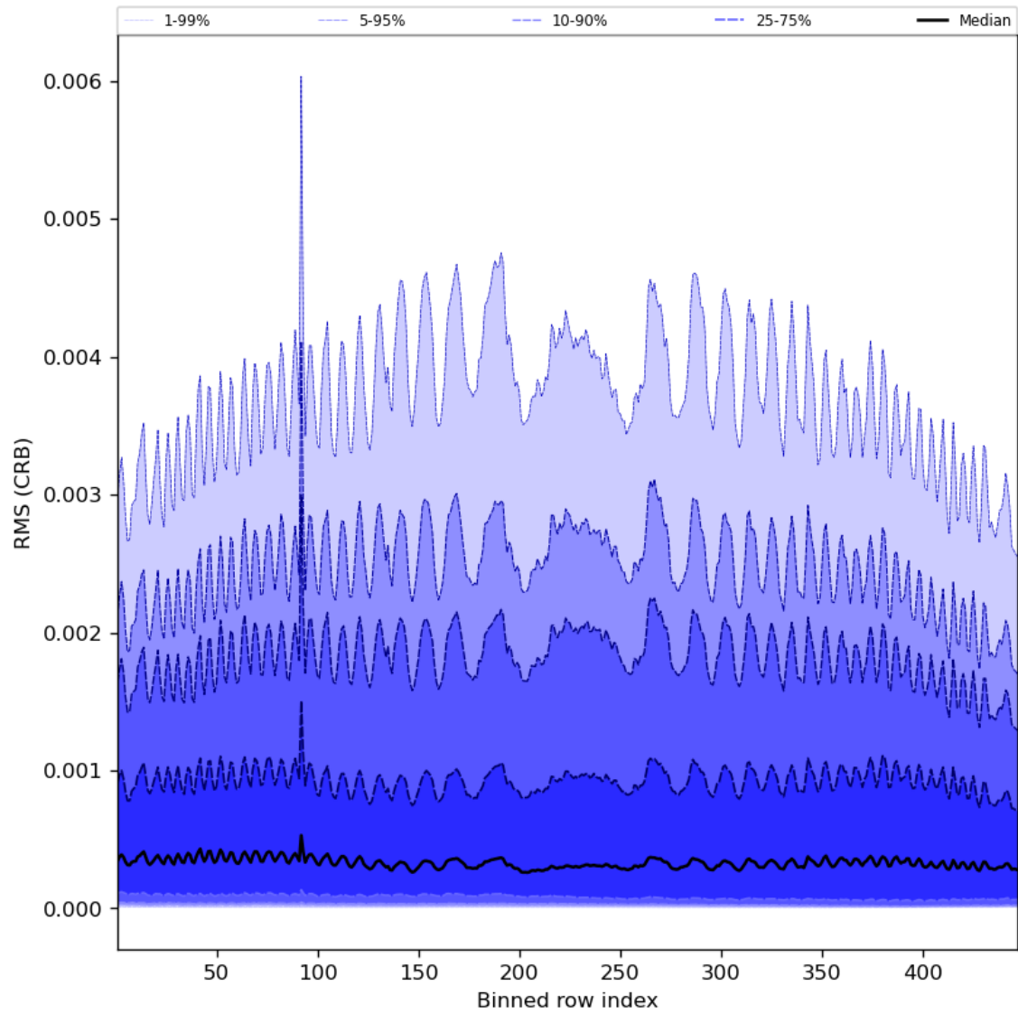
Figure 64: Along track statistics of “RMS (CRB)” for 2023-07-09 to 2023-07-11
