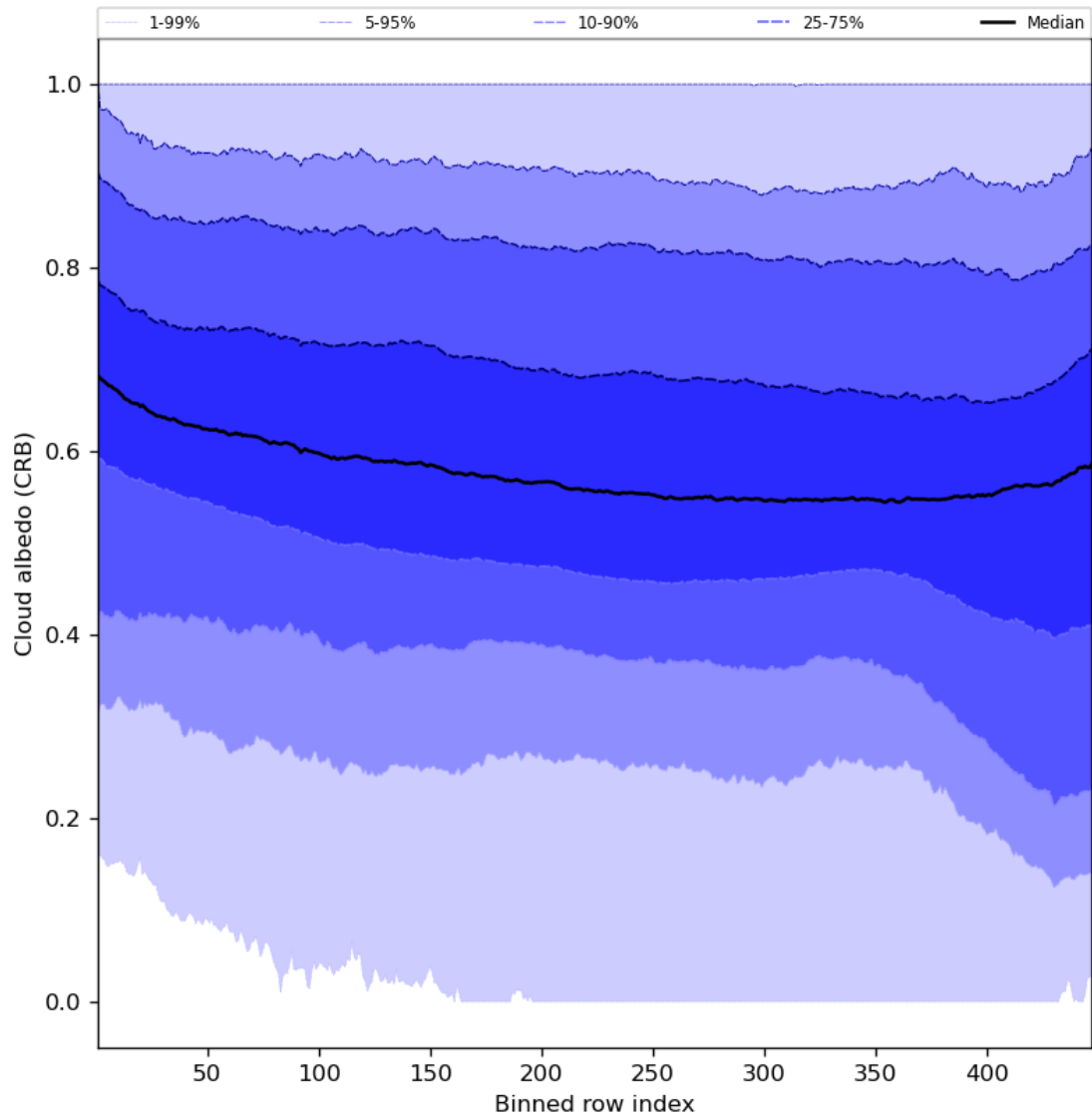
Figure 60: Along track statistics of “Cloud albedo (CRB)” for 2023-07-09 to 2023-07-11
