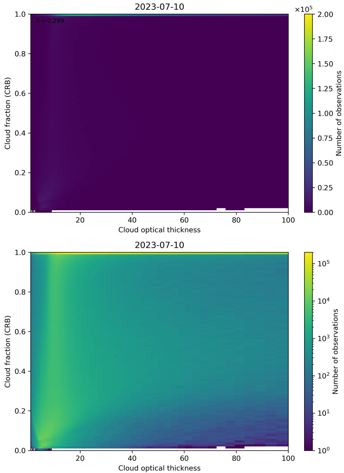
Figure 84: Scatter density plot of “Cloud optical thickness” against “Cloud fraction (CRB)” for 2023-07-09 to 2023-07-11.
