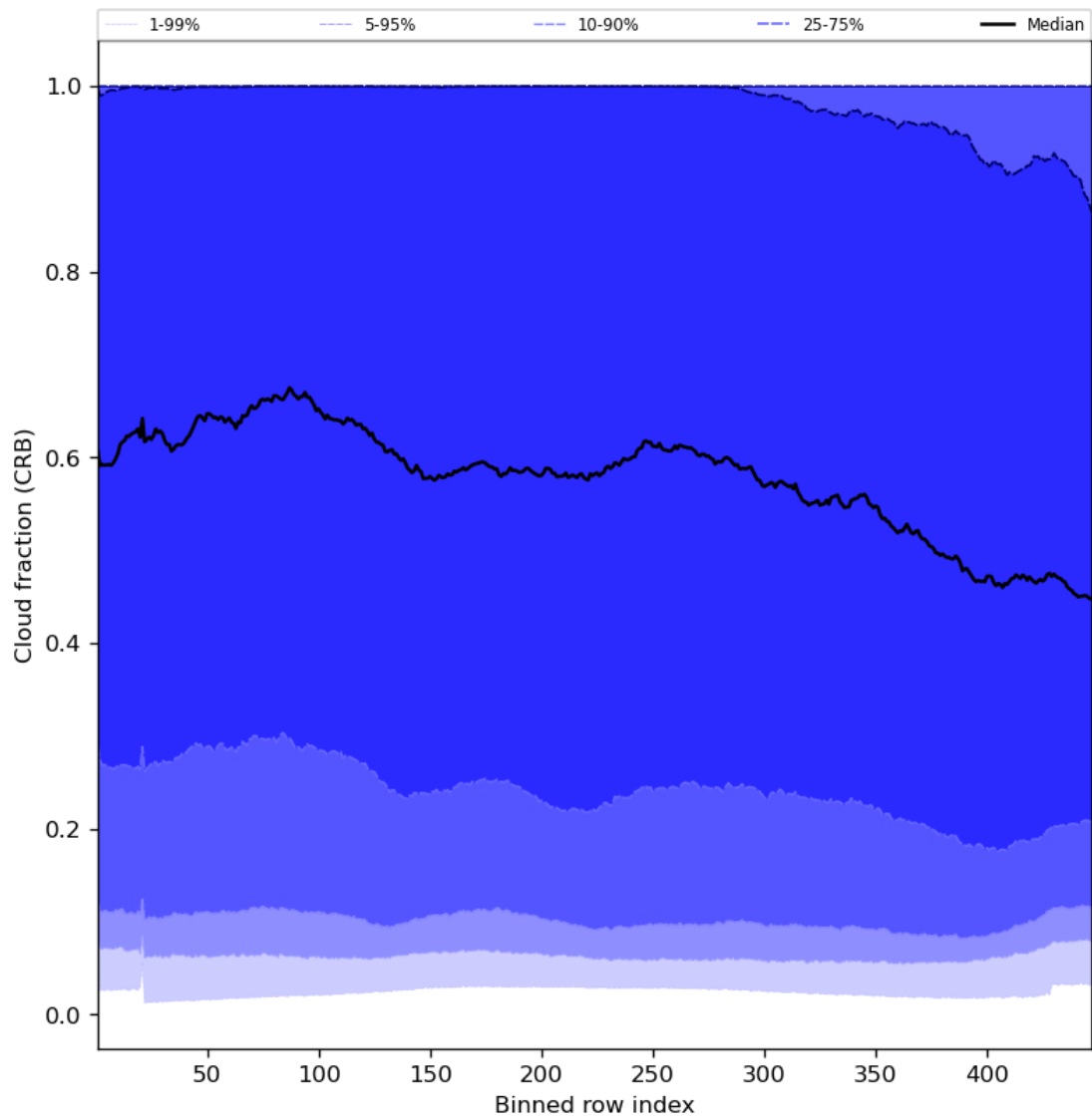
Figure 58: Along track statistics of “Cloud fraction (CRB)” for 2023-07-09 to 2023-07-11
