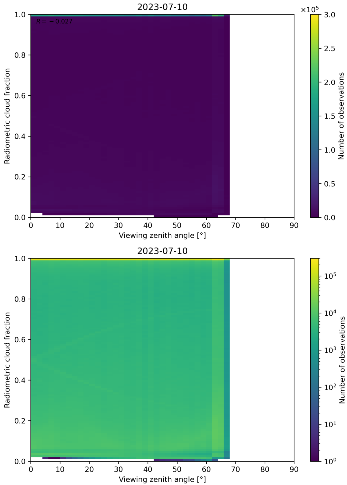
Figure 107: Scatter density plot of “Viewing zenith angle” against “Radiometric cloud fraction” for 2023-07-09 to 2023-07-11.
