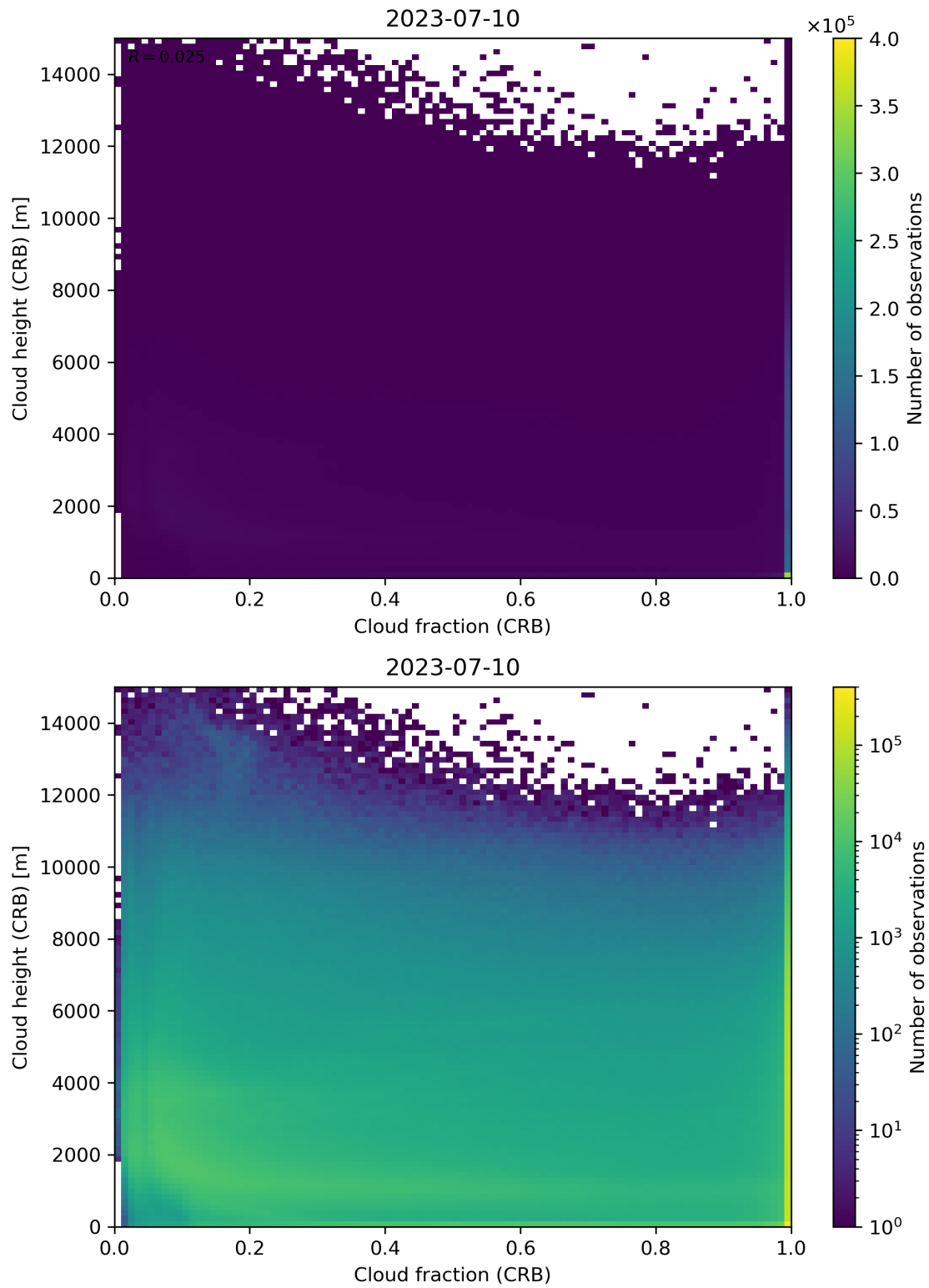
Figure 79: Scatter density plot of “Cloud fraction (CRB)” against “Cloud height (CRB)” for 2023-07-09 to 2023-07-11.
