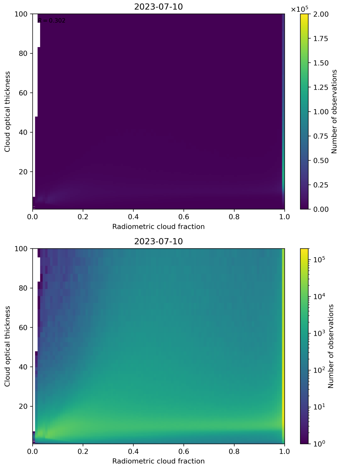
Figure 75: Scatter density plot of “Radiometric cloud fraction” against “Cloud optical thickness” for 2023-07-09 to 2023-07-11.
