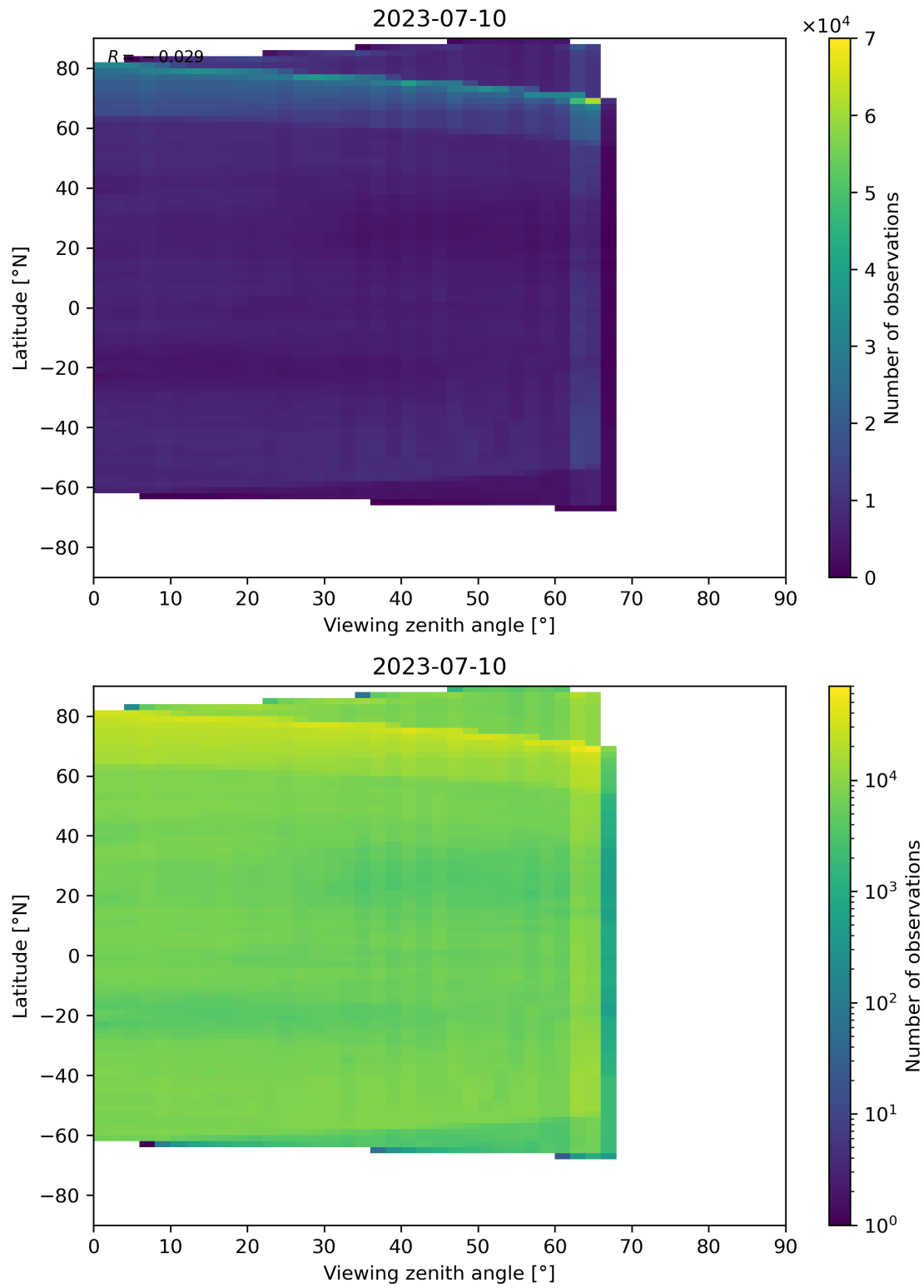
Figure 113: Scatter density plot of “Viewing zenith angle” against “Latitude” for 2023-07-09 to 2023-07-11.
