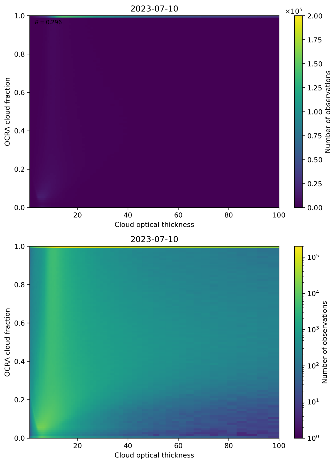
Figure 83: Scatter density plot of “Cloud optical thickness” against “OCRA cloud fraction” for 2023-07-09 to 2023-07-11.
