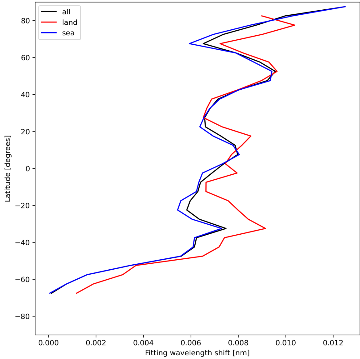
Figure 33: Zonal average of “Fitting wavelength shift” for 2023-07-13 to 2023-07-14.
