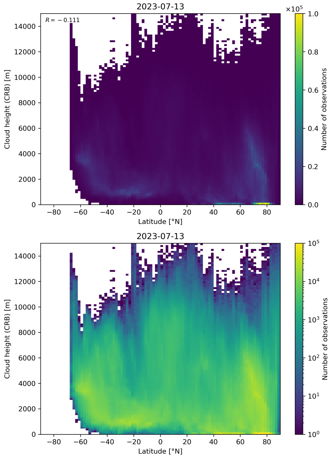
Figure 95: Scatter density plot of “Latitude” against “Cloud height (CRB)” for 2023-07-13 to 2023-07-14.
