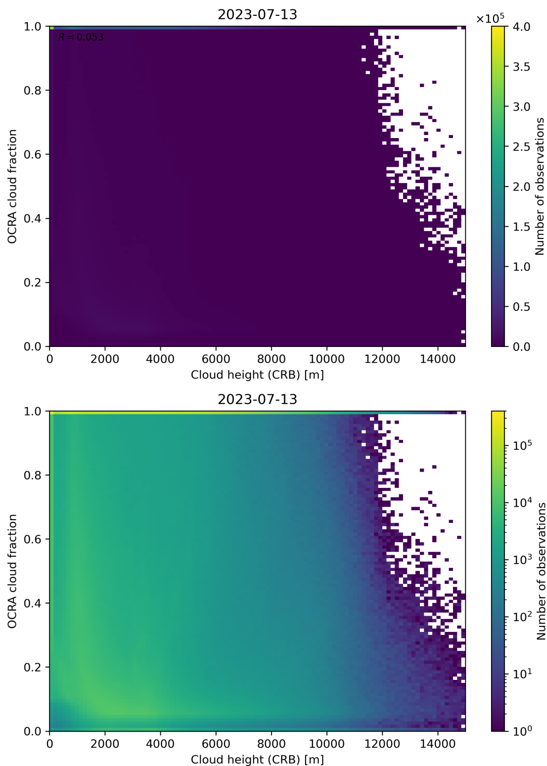
Figure 81: Scatter density plot of “Cloud height (CRB)” against “OCRA cloud fraction” for 2023-07-13 to 2023-07-14.
