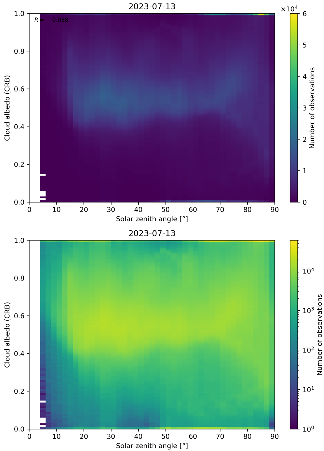
Figure 98: Scatter density plot of “Solar zenith angle” against “Cloud albedo (CRB)” for 2023-07-13 to 2023-07-14.
