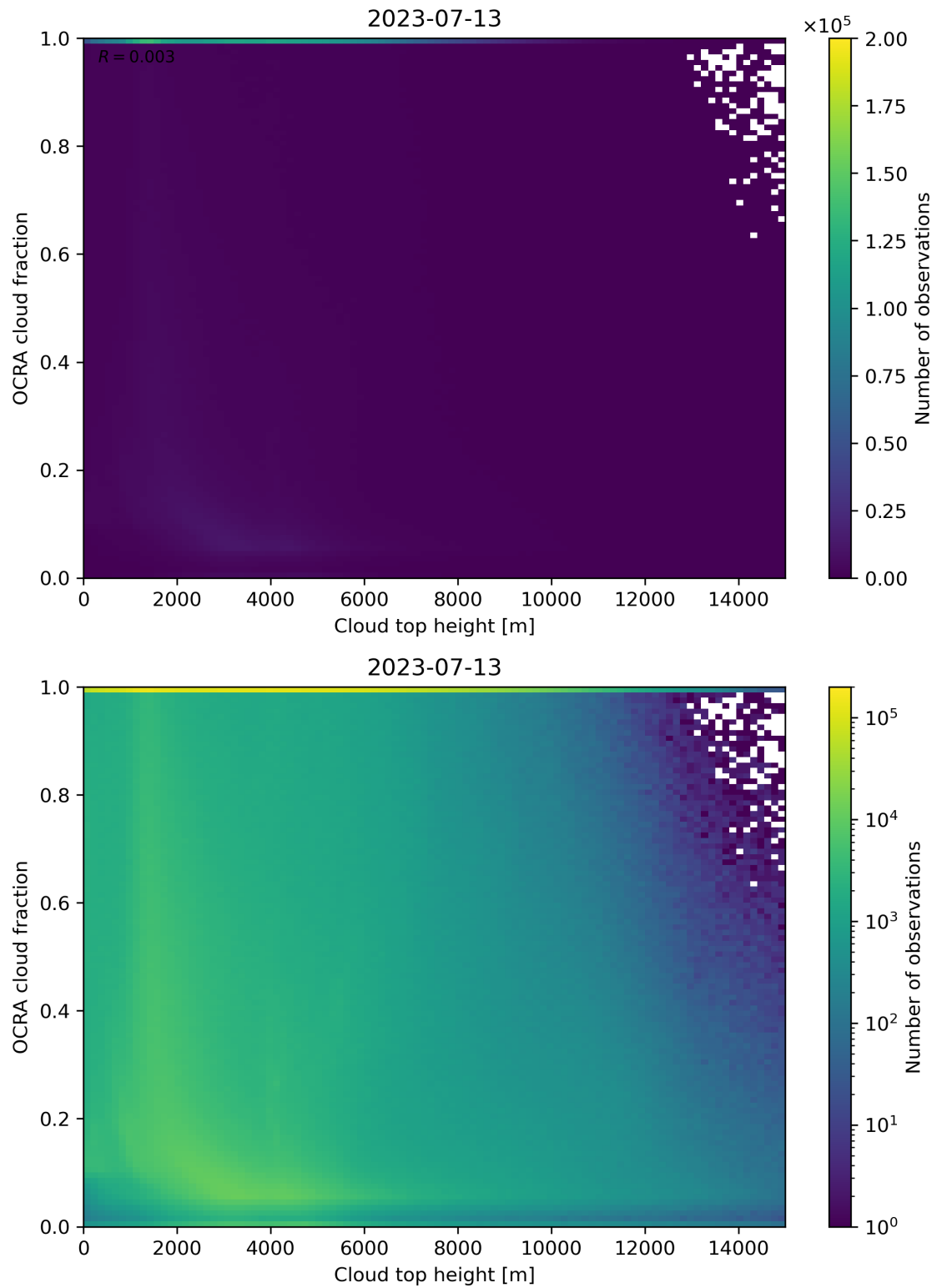
Figure 87: Scatter density plot of “Cloud top height” against “OCRA cloud fraction” for 2023-07-13 to 2023-07-14.
