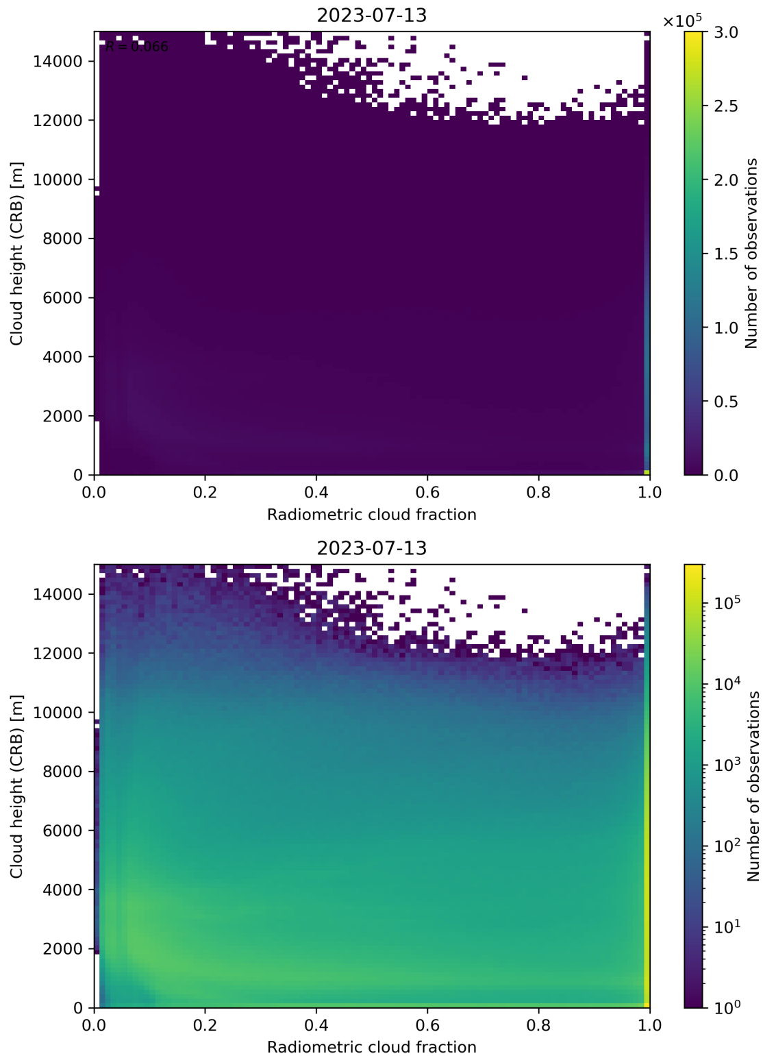
Figure 74: Scatter density plot of “Radiometric cloud fraction” against “Cloud height (CRB)” for 2023-07-13 to 2023-07-14.
