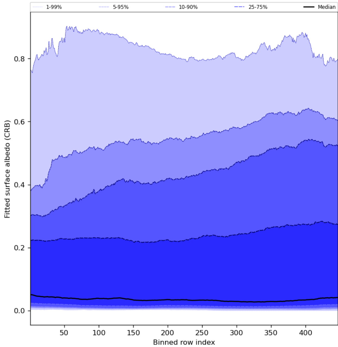
Figure 62: Along track statistics of “Fitted surface albedo (CRB)” for 2023-07-13 to 2023-07-14
