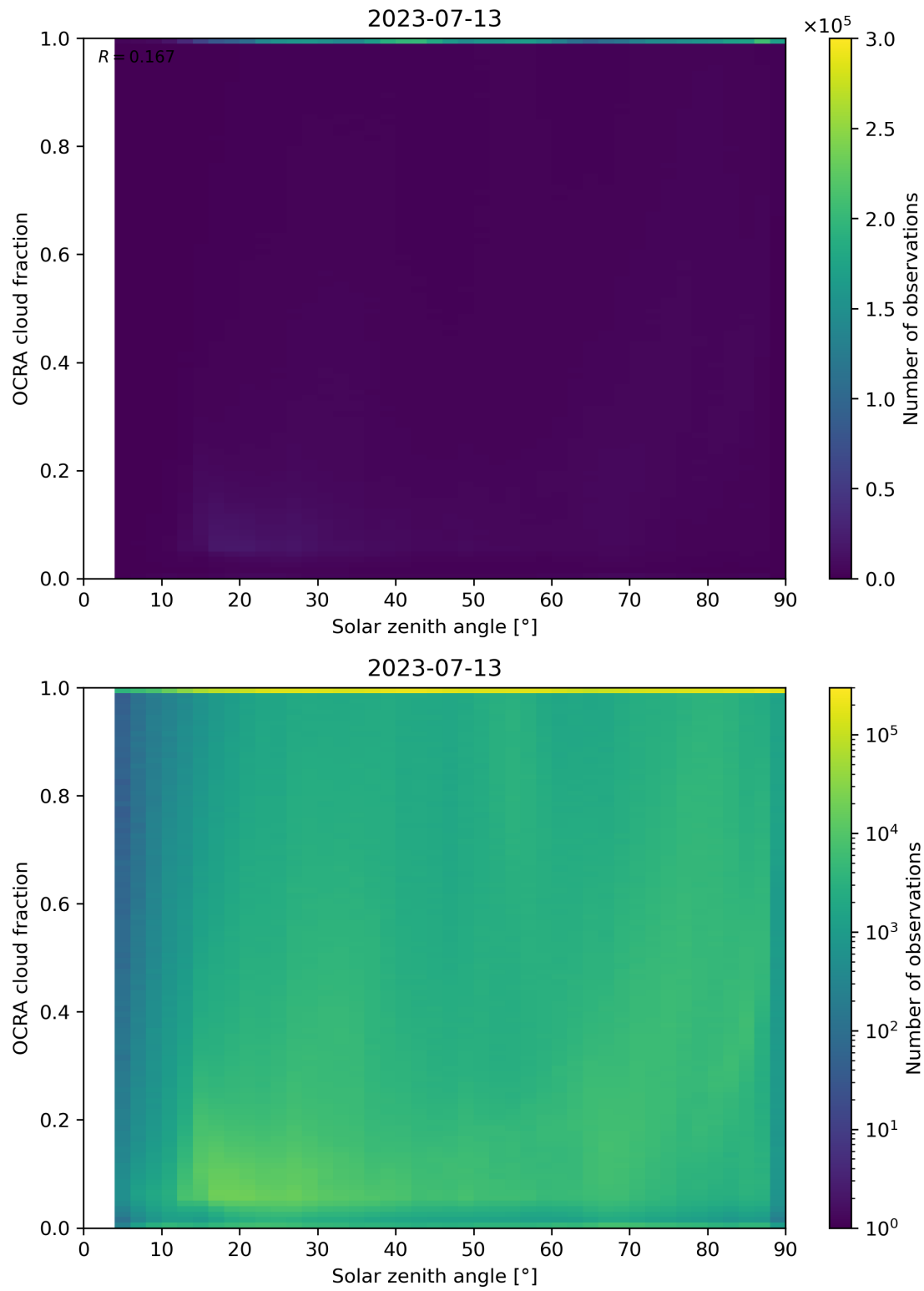
Figure 100: Scatter density plot of “Solar zenith angle” against “OCRA cloud fraction” for 2023-07-13 to 2023-07-14.
