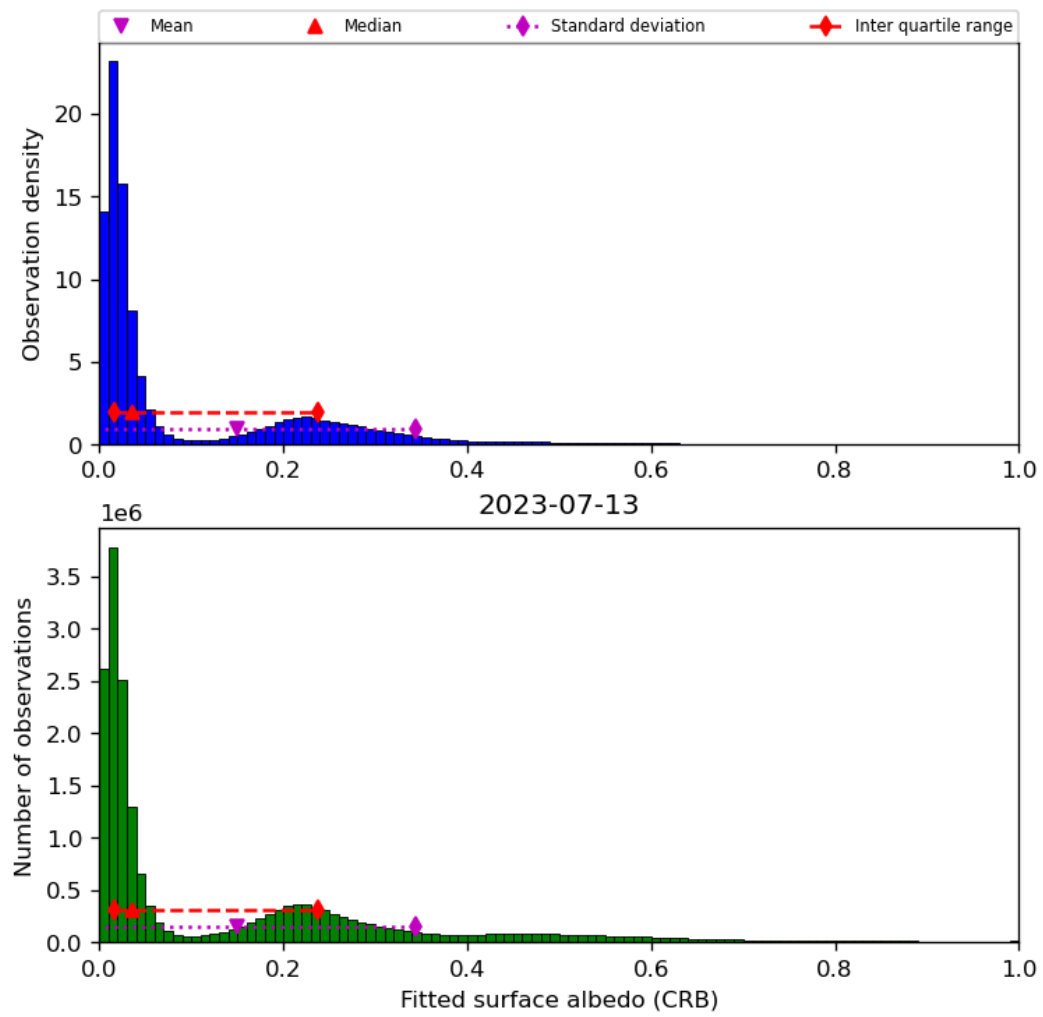
Figure 46: Histogram of “Fitted surface albedo (CRB)” for 2023-07-13 to 2023-07-14
