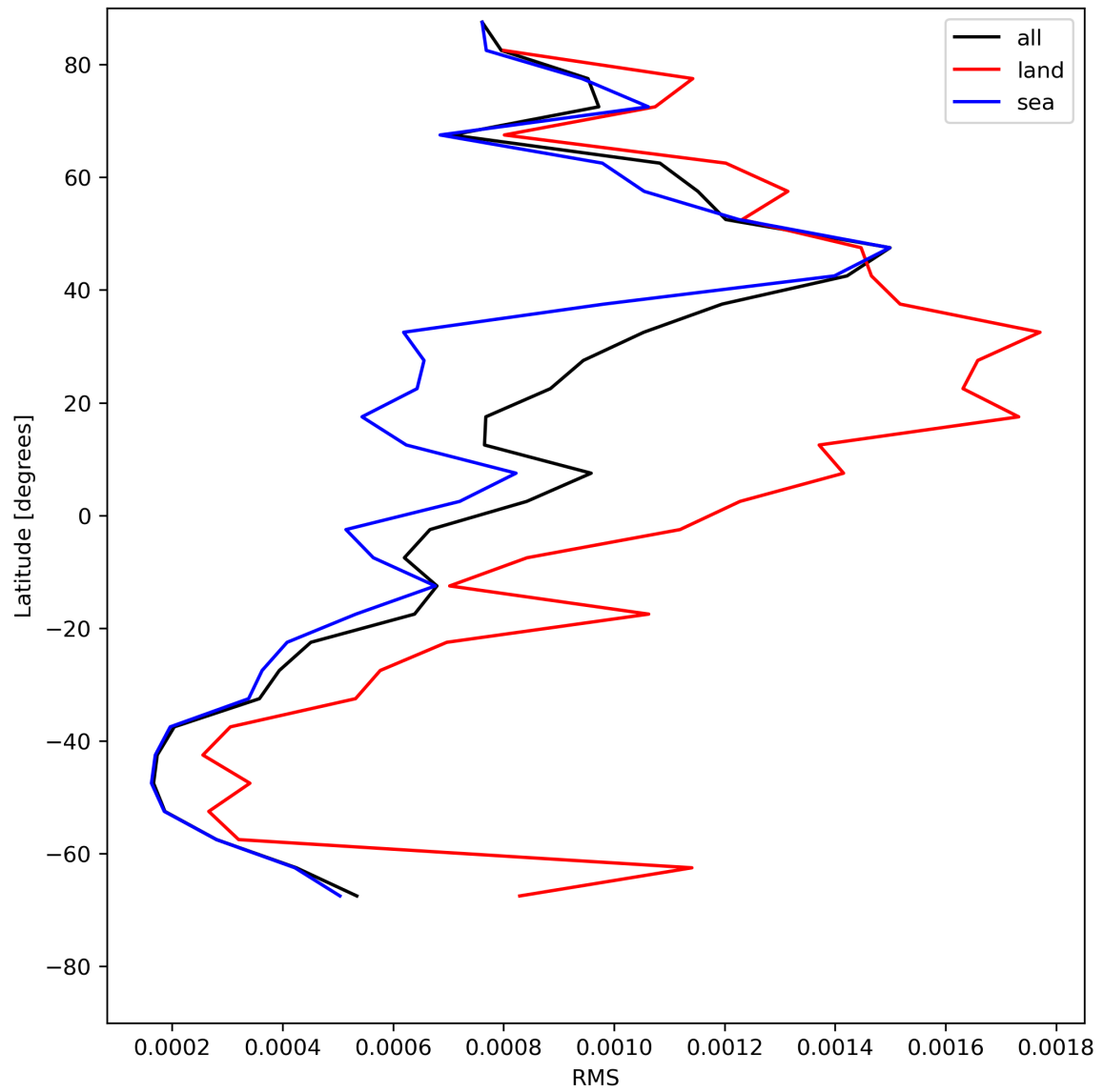
Figure 31: Zonal average of “RMS” for 2023-07-13 to 2023-07-14.
