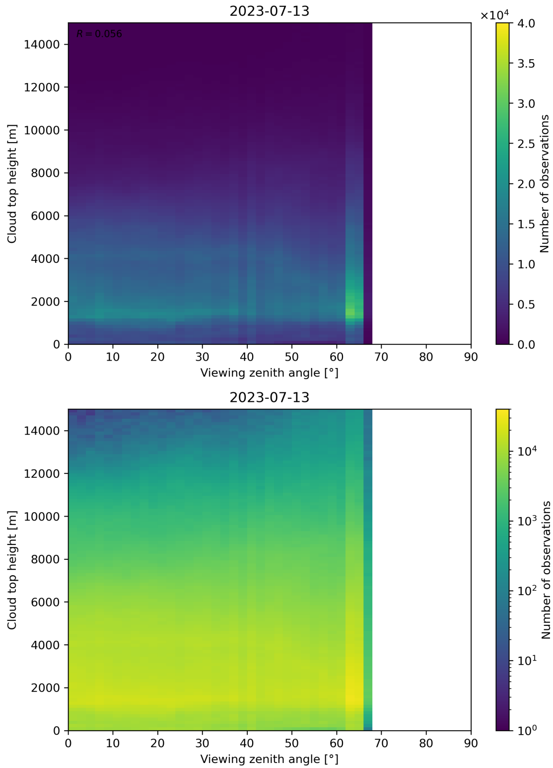
Figure 112: Scatter density plot of “Viewing zenith angle” against “Cloud top height” for 2023-07-13 to 2023-07-14.
