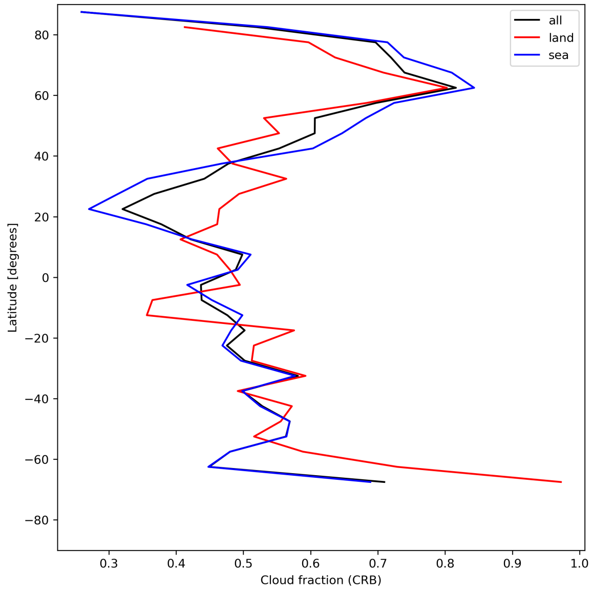
Figure 26: Zonal average of “Cloud fraction (CRB)” for 2023-07-13 to 2023-07-14.
