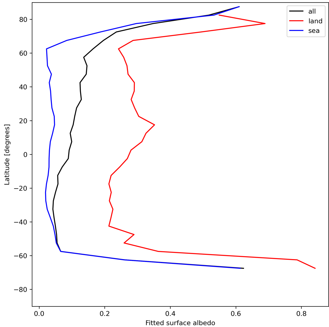
Figure 29: Zonal average of “Fitted surface albedo” for 2023-07-13 to 2023-07-14.
