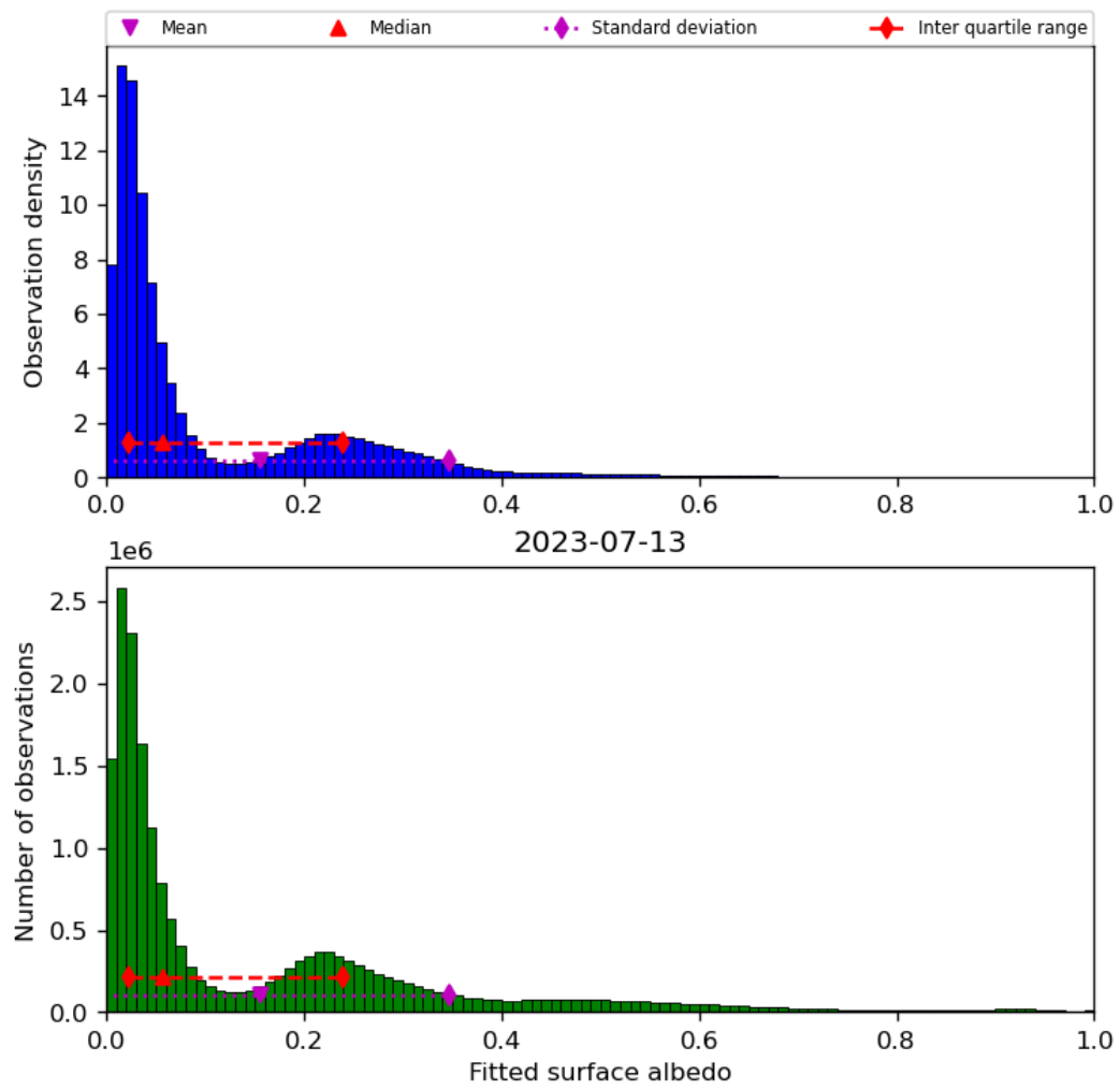
Figure 45: Histogram of “Fitted surface albedo” for 2023-07-13 to 2023-07-14
