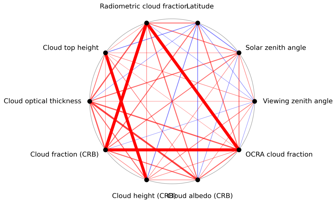
Figure 1: Map of correlation graph for 2023-07-13 to 2023-07-14.
