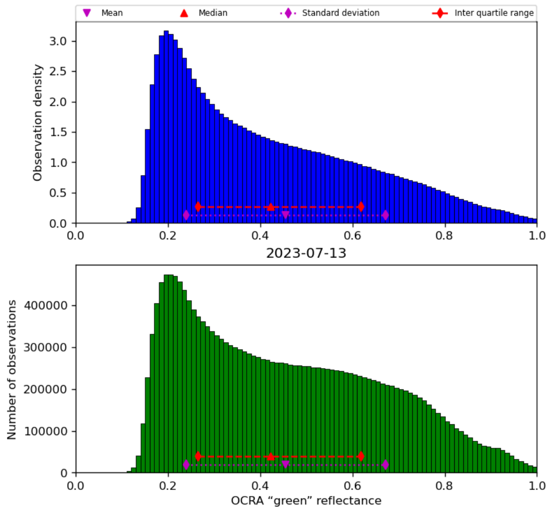
Figure 52: Histogram of “OCRA “green” reflectance” for 2023-07-13 to 2023-07-14
