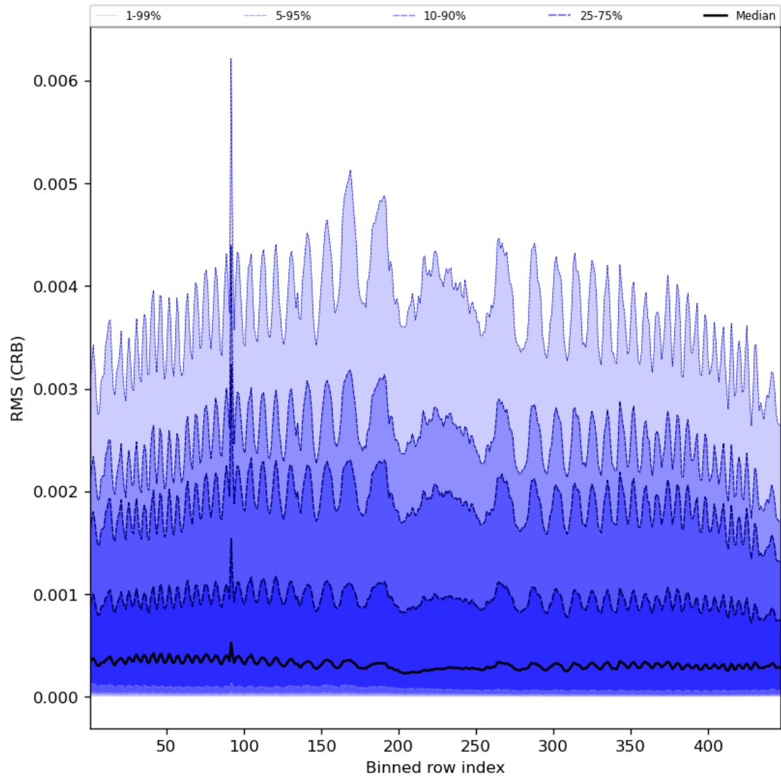
Figure 64: Along track statistics of “RMS (CRB)” for 2023-07-13 to 2023-07-14
