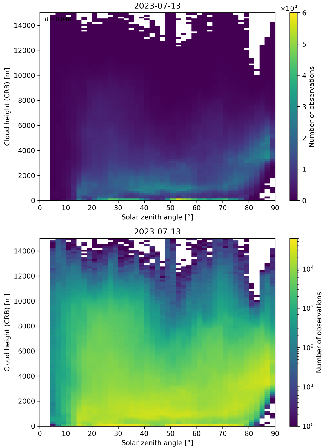
Figure 102: Scatter density plot of “Solar zenith angle” against “Cloud height (CRB)” for 2023-07-13 to 2023-07-14.
