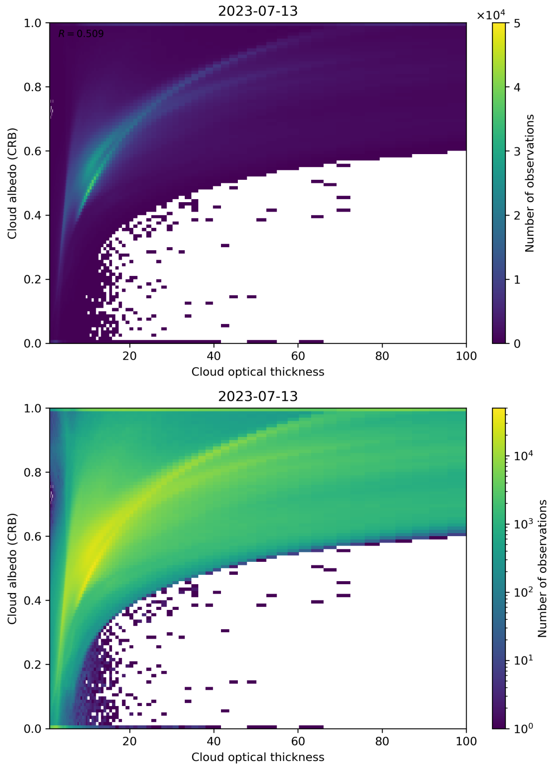
Figure 82: Scatter density plot of “Cloud optical thickness” against “Cloud albedo (CRB)” for 2023-07-13 to 2023-07-14.
