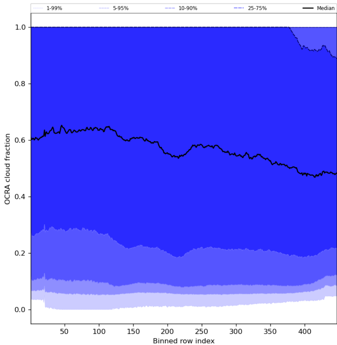
Figure 66: Along track statistics of “OCRA cloud fraction” for 2023-07-13 to 2023-07-14
