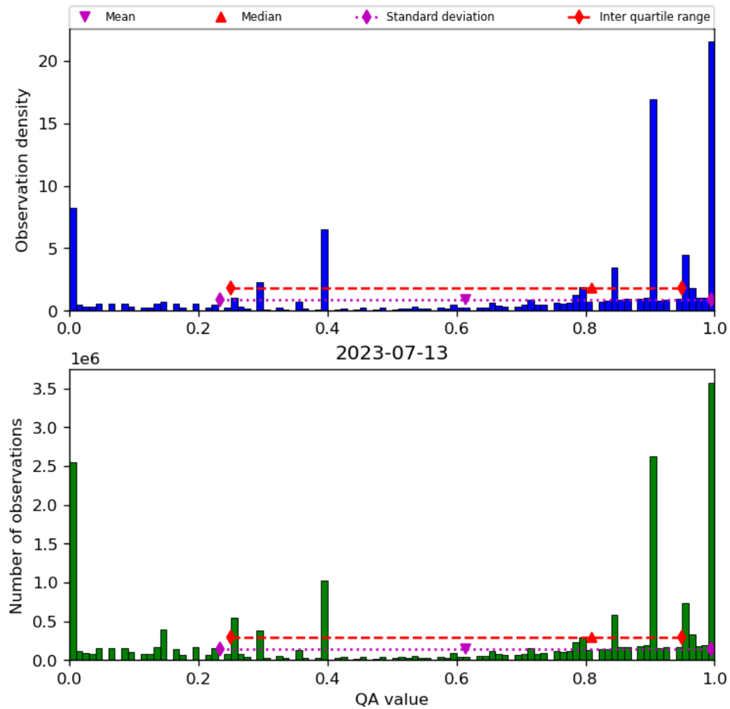
Figure 38: Histogram of “QA value” for 2023-07-13 to 2023-07-14
