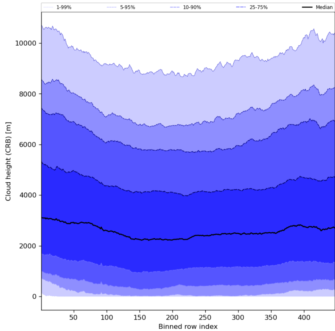
Figure 59: Along track statistics of “Cloud height (CRB)” for 2023-07-13 to 2023-07-14
