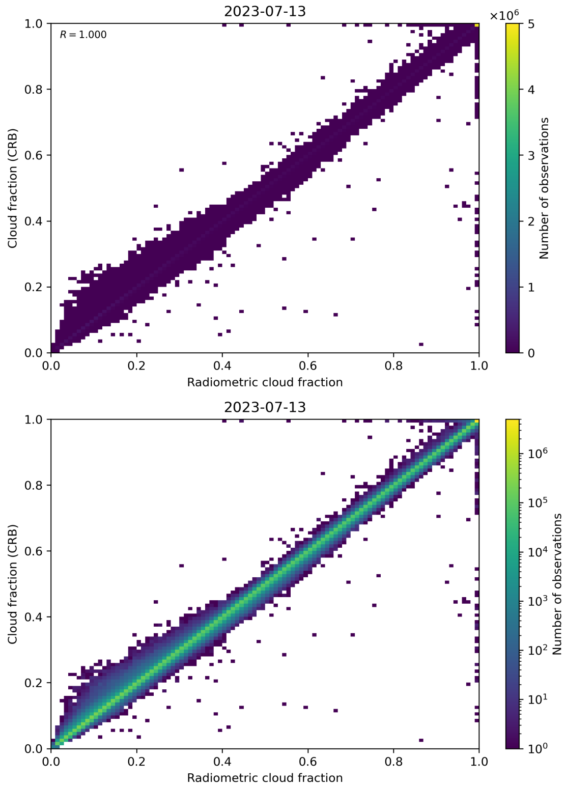
Figure 73: Scatter density plot of “Radiometric cloud fraction” against “Cloud fraction (CRB)” for 2023-07-13 to 2023-07-14.
