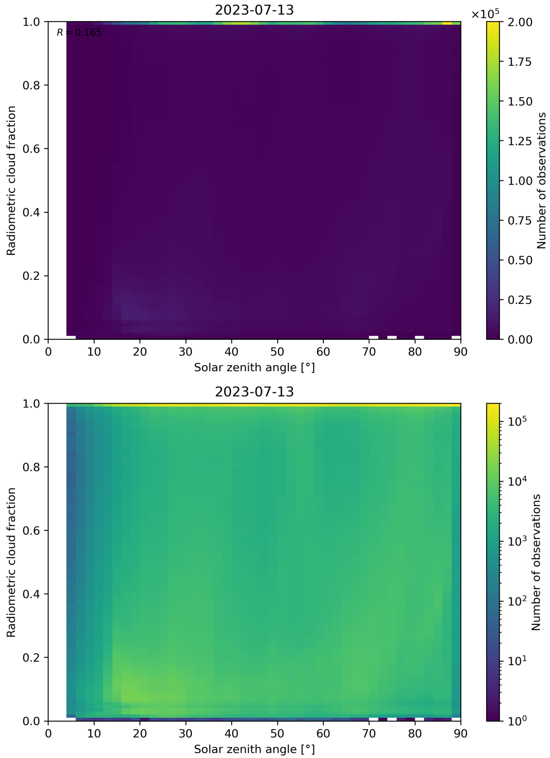
Figure 99: Scatter density plot of “Solar zenith angle” against “Radiometric cloud fraction” for 2023-07-13 to 2023-07-14.
