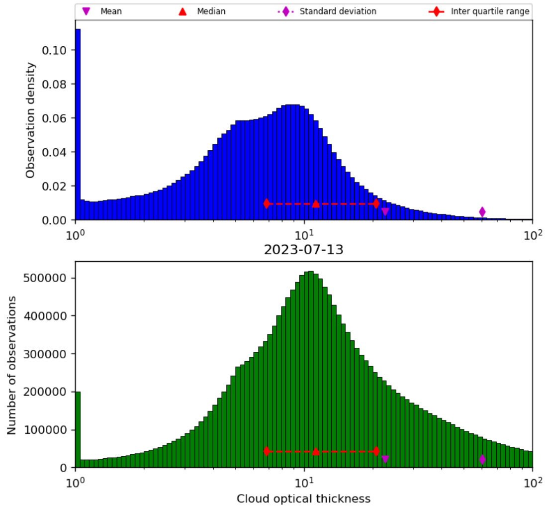
Figure 41: Histogram of “Cloud optical thickness” for 2023-07-13 to 2023-07-14
