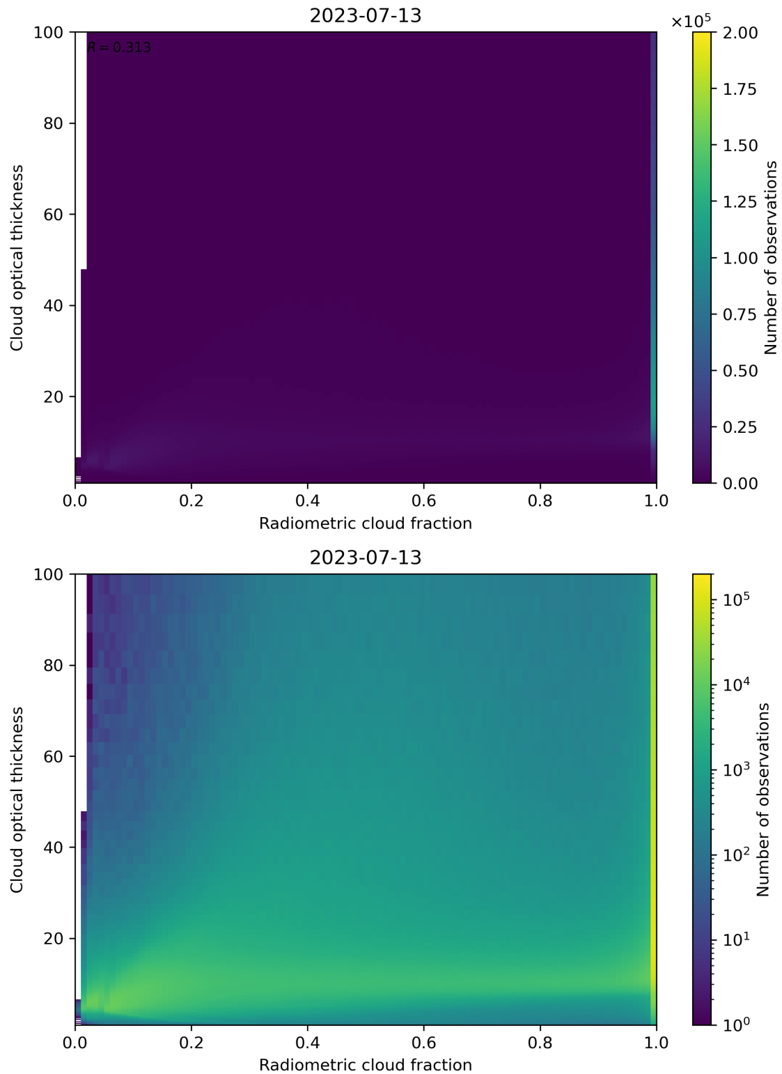
Figure 75: Scatter density plot of “Radiometric cloud fraction” against “Cloud optical thickness” for 2023-07-13 to 2023-07-14.
