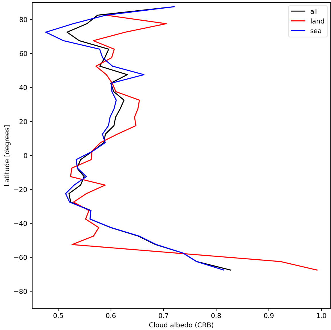
Figure 28: Zonal average of “Cloud albedo (CRB)” for 2023-07-13 to 2023-07-14.
