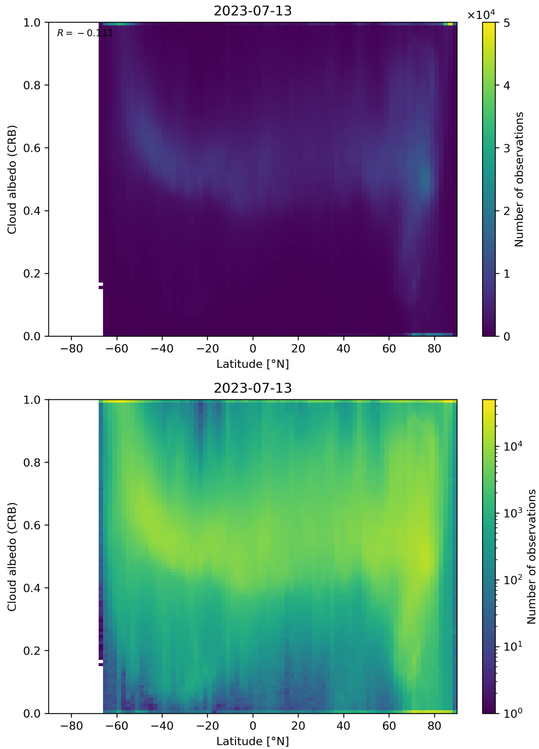
Figure 91: Scatter density plot of “Latitude” against “Cloud albedo (CRB)” for 2023-07-13 to 2023-07-14.
