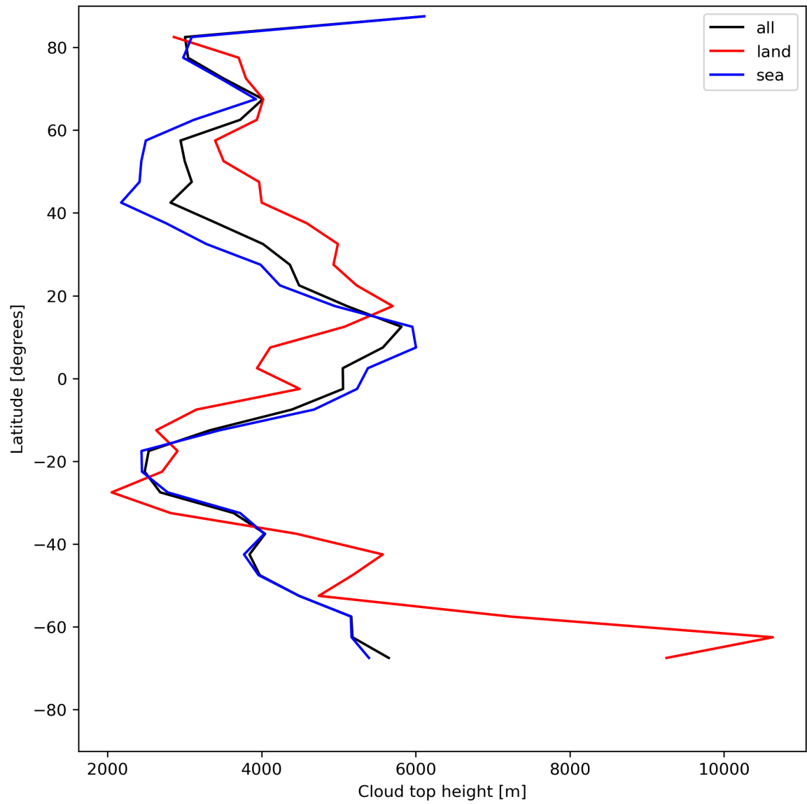
Figure 24: Zonal average of “Cloud top height” for 2023-07-13 to 2023-07-14.
