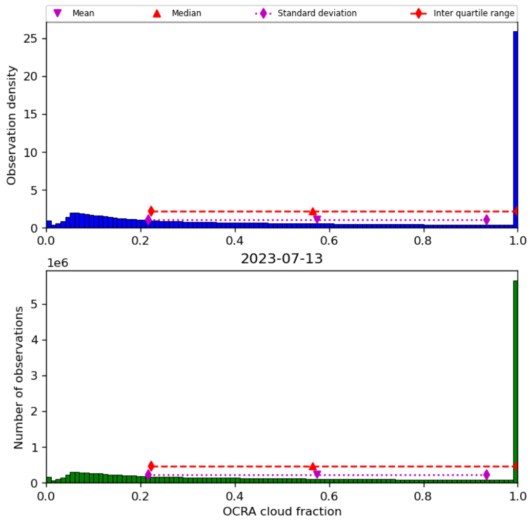
Figure 50: Histogram of “OCRA cloud fraction” for 2023-07-13 to 2023-07-14
