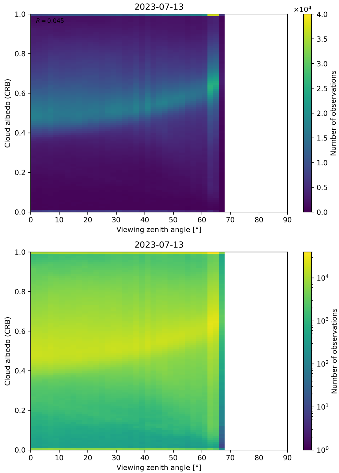
Figure 106: Scatter density plot of “Viewing zenith angle” against “Cloud albedo (CRB)” for 2023-07-13 to 2023-07-14.
