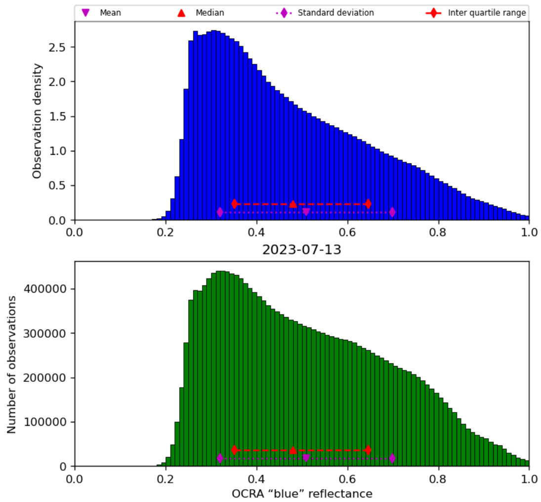
Figure 51: Histogram of “OCRA “blue” reflectance” for 2023-07-13 to 2023-07-14
