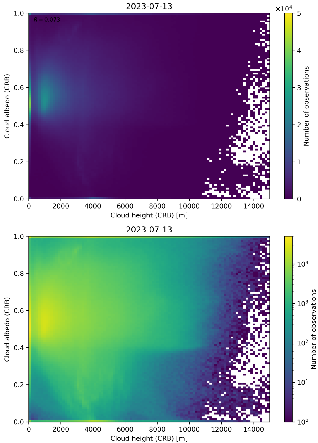
Figure 80: Scatter density plot of “Cloud height (CRB)” against “Cloud albedo (CRB)” for 2023-07-13 to 2023-07-14.
