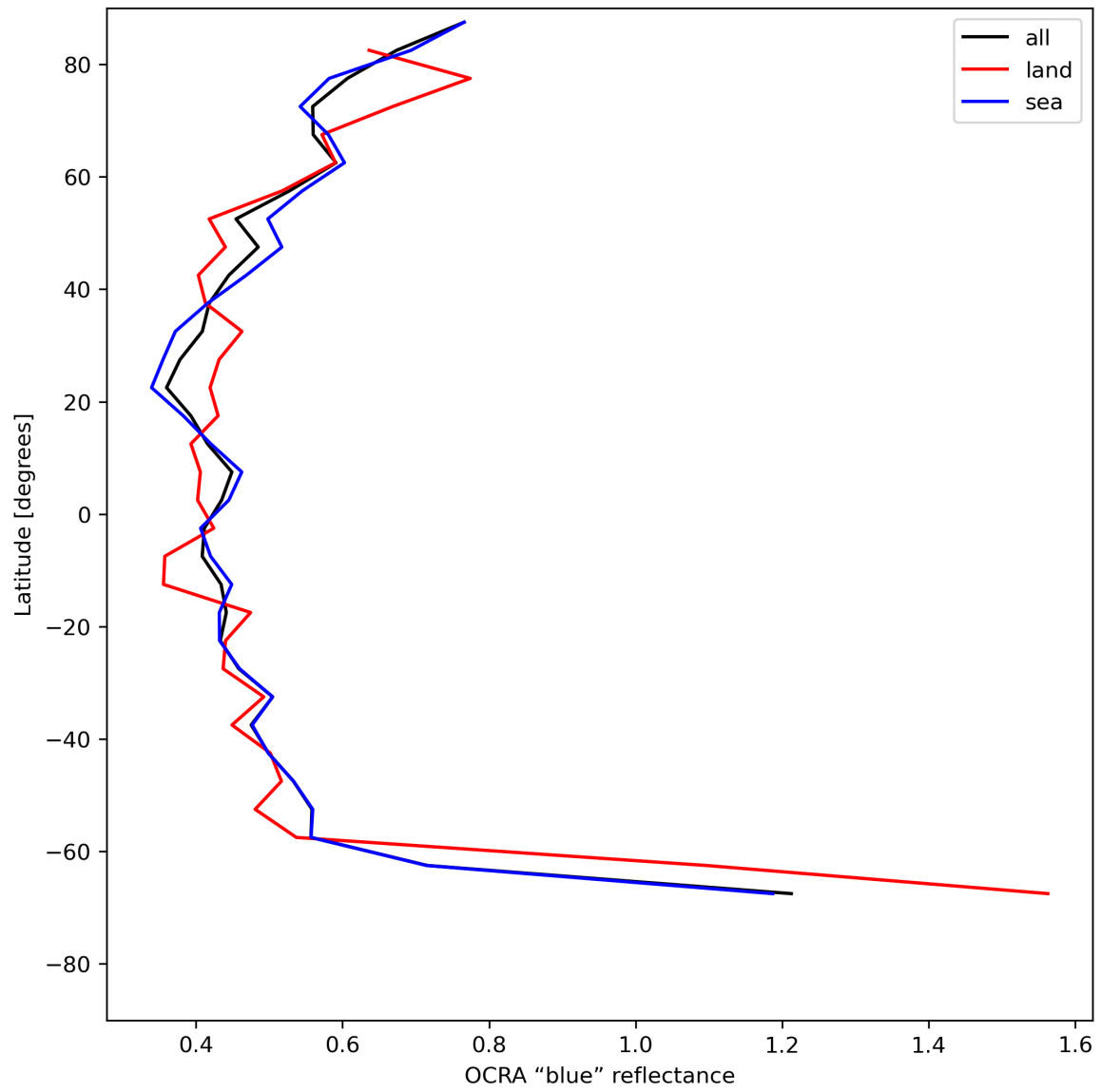
Figure 35: Zonal average of “OCRA “blue” reflectance” for 2023-07-13 to 2023-07-14.
