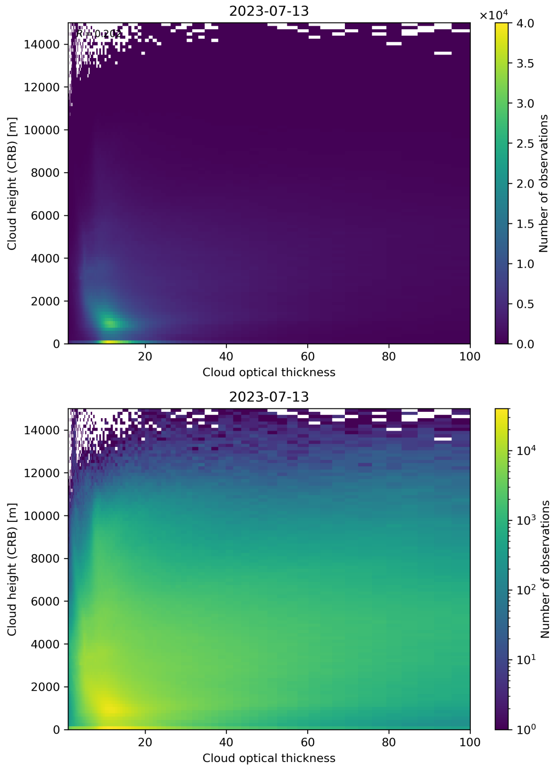
Figure 85: Scatter density plot of “Cloud optical thickness” against “Cloud height (CRB)” for 2023-07-13 to 2023-07-14.
