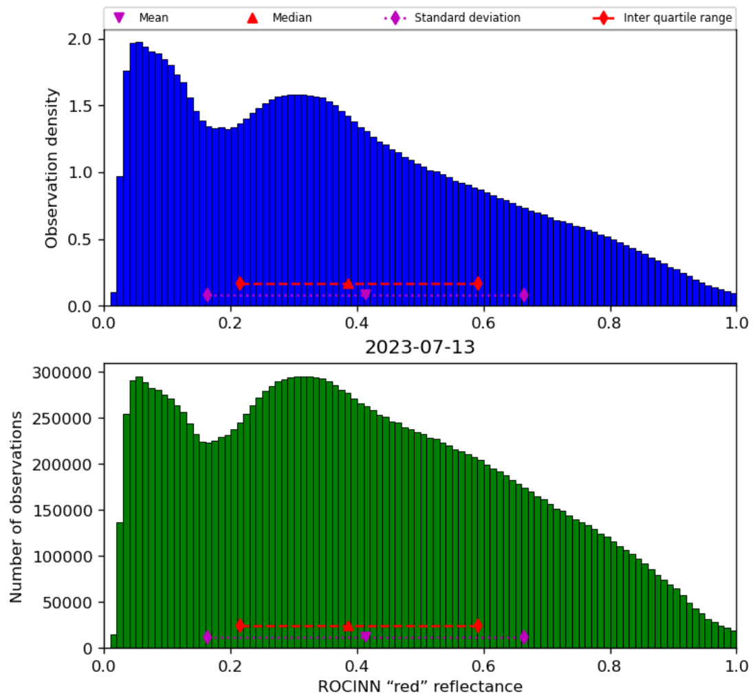
Figure 53: Histogram of “ROCINN “red” reflectance” for 2023-07-13 to 2023-07-14
