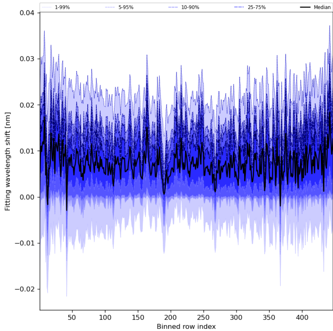
Figure 65: Along track statistics of “Fitting wavelength shift” for 2023-07-13 to 2023-07-14
