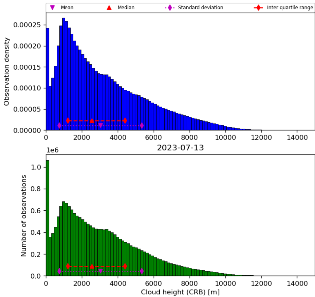
Figure 43: Histogram of “Cloud height (CRB)” for 2023-07-13 to 2023-07-14
