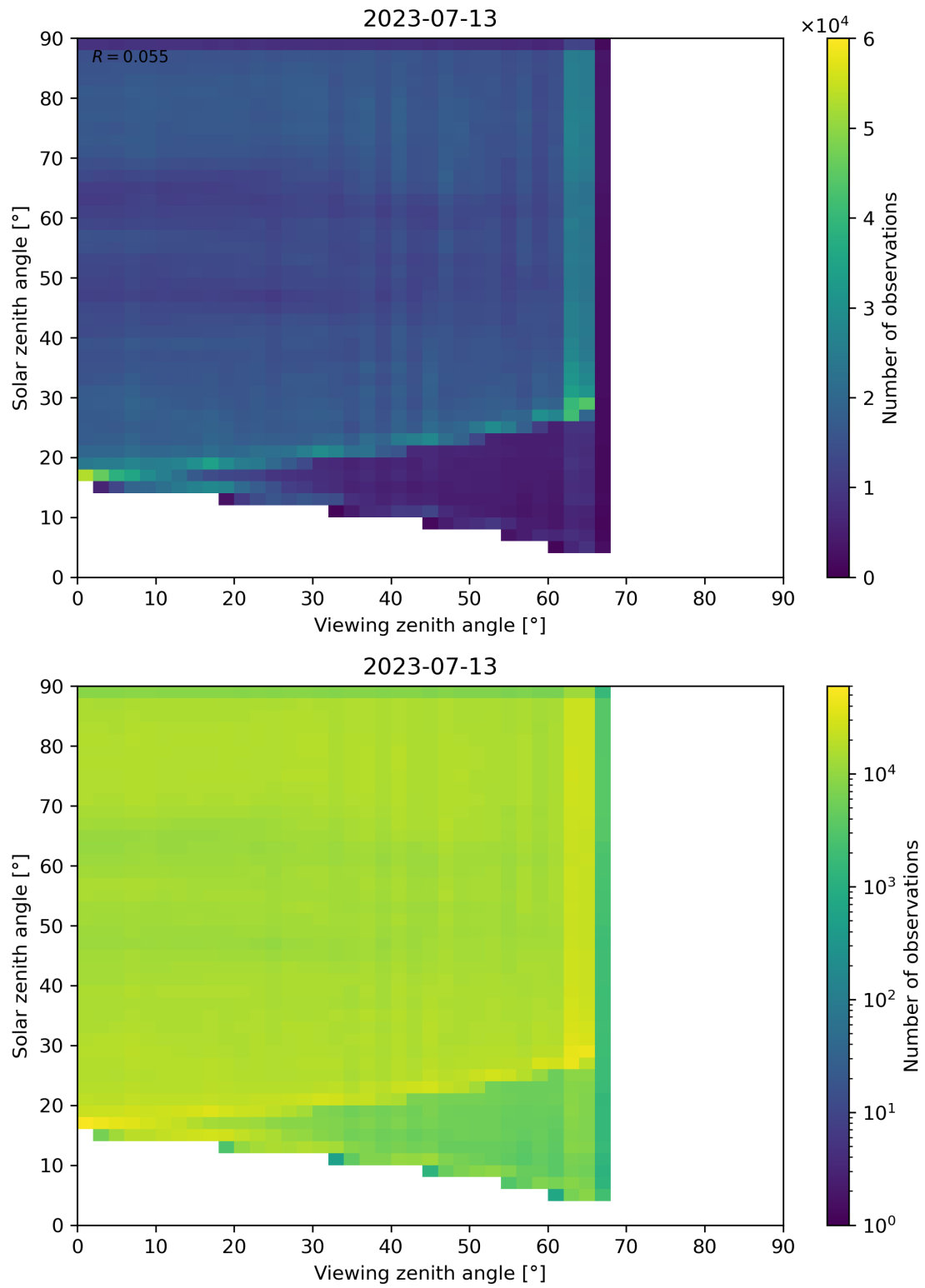
Figure 114: Scatter density plot of “Viewing zenith angle” against “Solar zenith angle” for 2023-07-13 to 2023-07-14.
