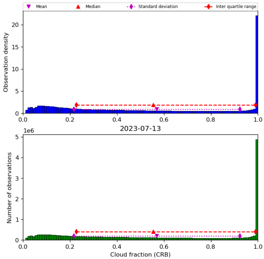
Figure 42: Histogram of “Cloud fraction (CRB)” for 2023-07-13 to 2023-07-14
