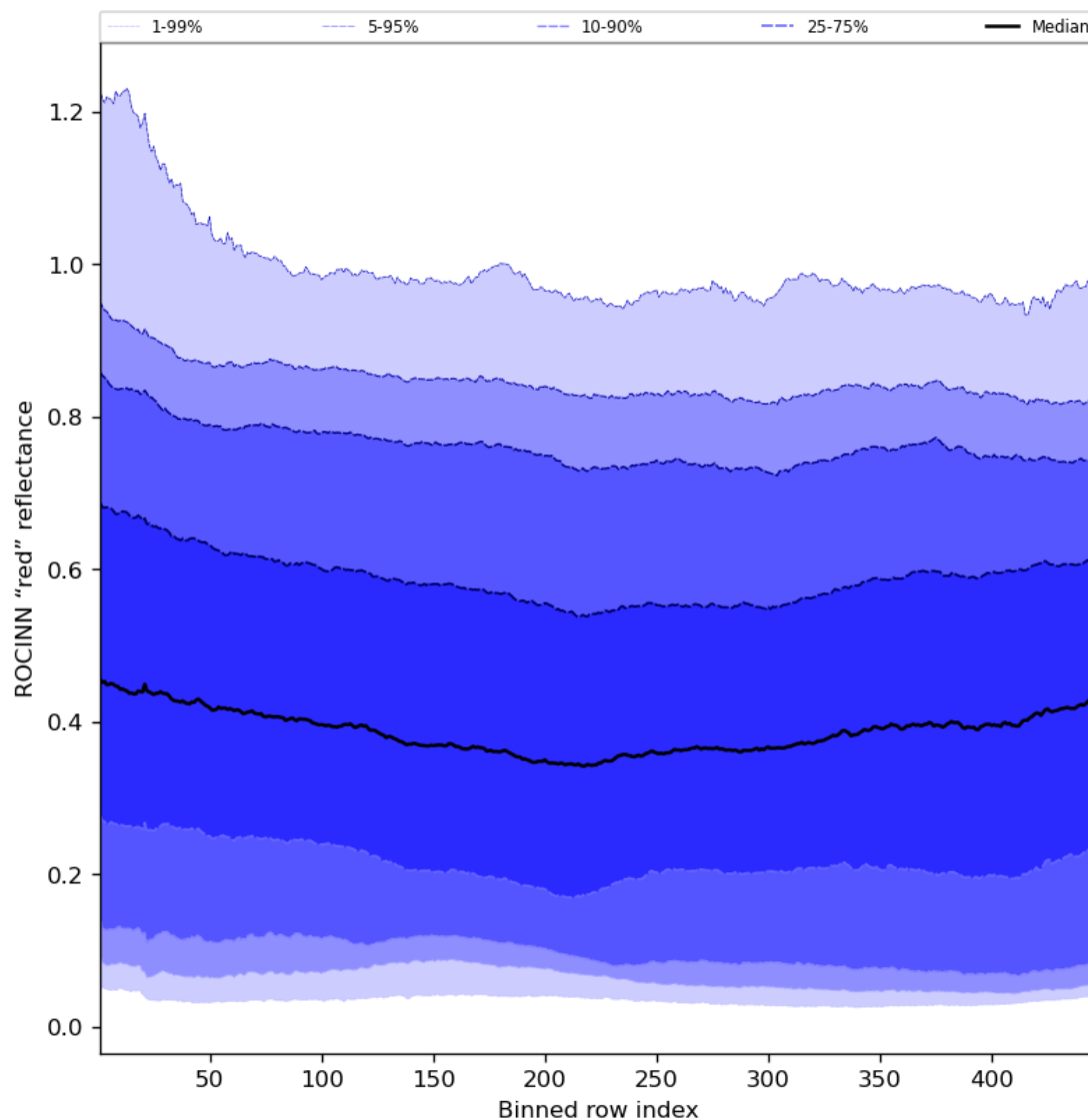
Figure 69: Along track statistics of “ROCINN “red” reflectance” for 2023-07-13 to 2023-07-14
