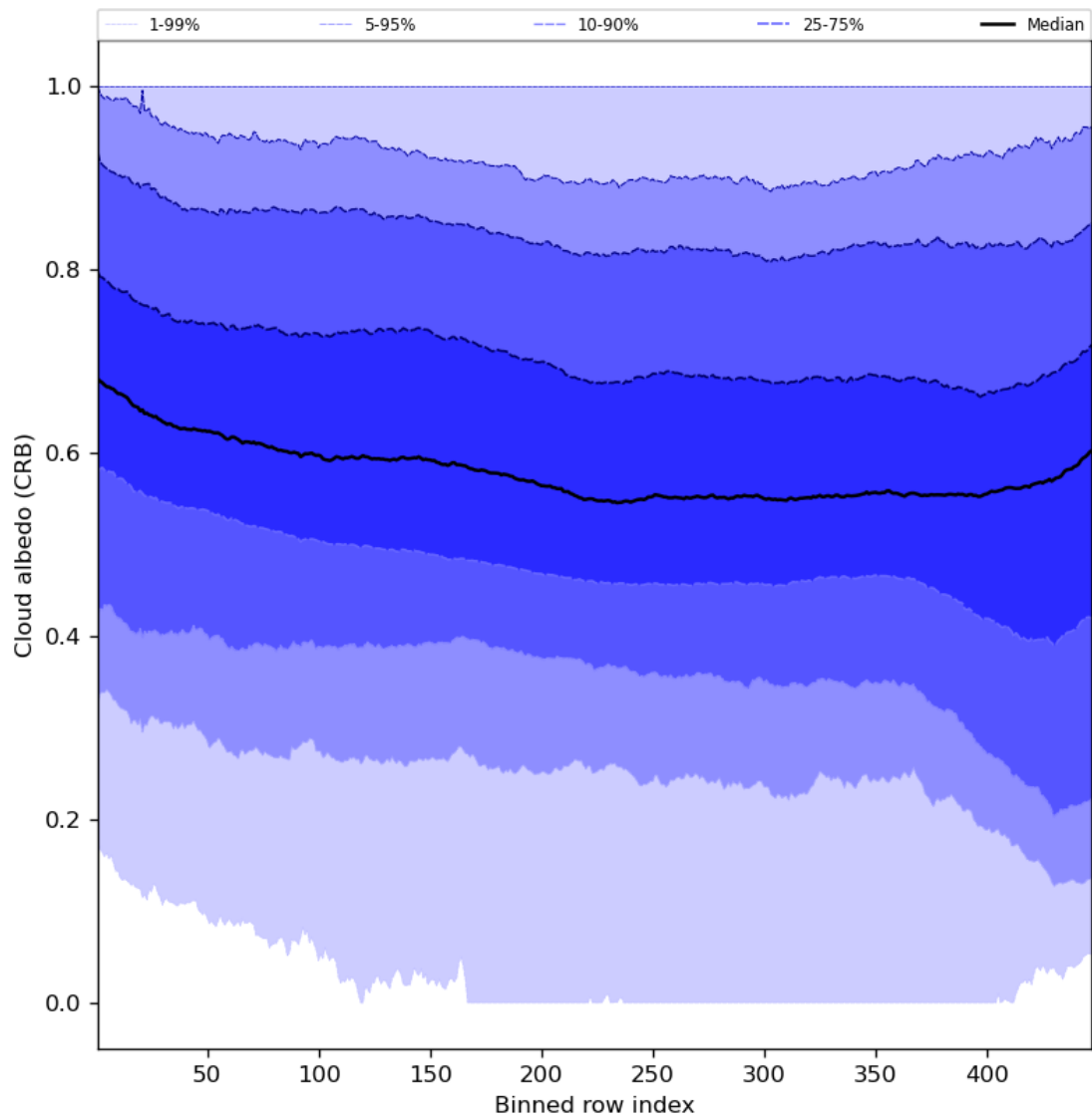
Figure 60: Along track statistics of “Cloud albedo (CRB)” for 2023-07-13 to 2023-07-14
