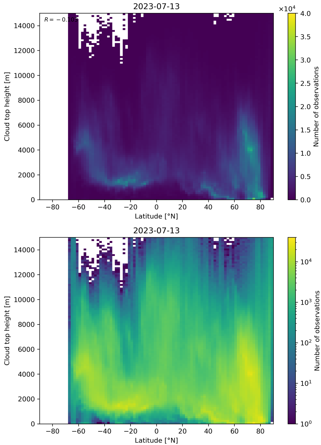
Figure 97: Scatter density plot of “Latitude” against “Cloud top height” for 2023-07-13 to 2023-07-14.
