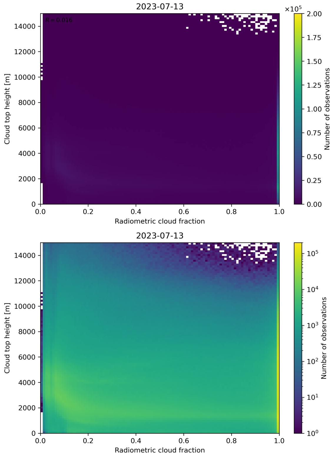
Figure 76: Scatter density plot of “Radiometric cloud fraction” against “Cloud top height” for 2023-07-13 to 2023-07-14.
