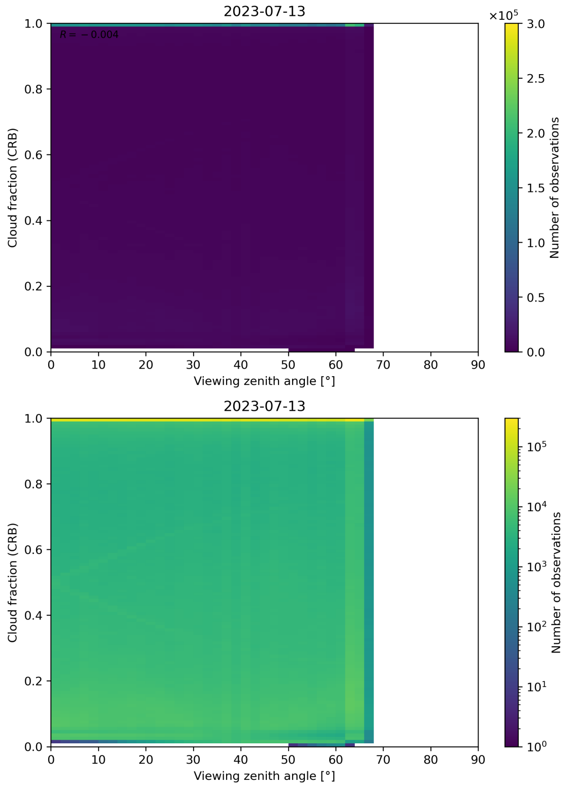
Figure 109: Scatter density plot of “Viewing zenith angle” against “Cloud fraction (CRB)” for 2023-07-13 to 2023-07-14.
