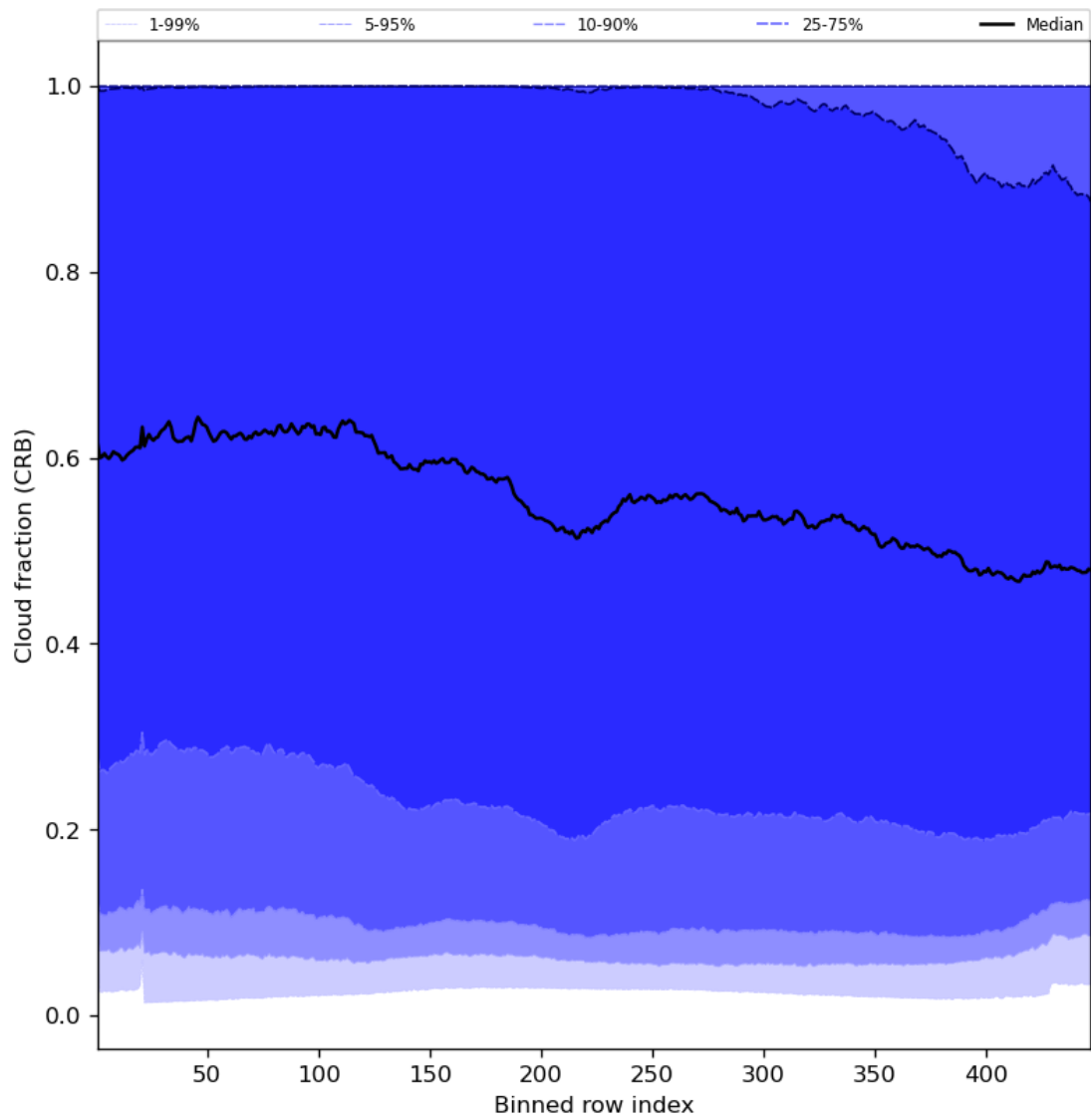
Figure 58: Along track statistics of “Cloud fraction (CRB)” for 2023-07-13 to 2023-07-14
