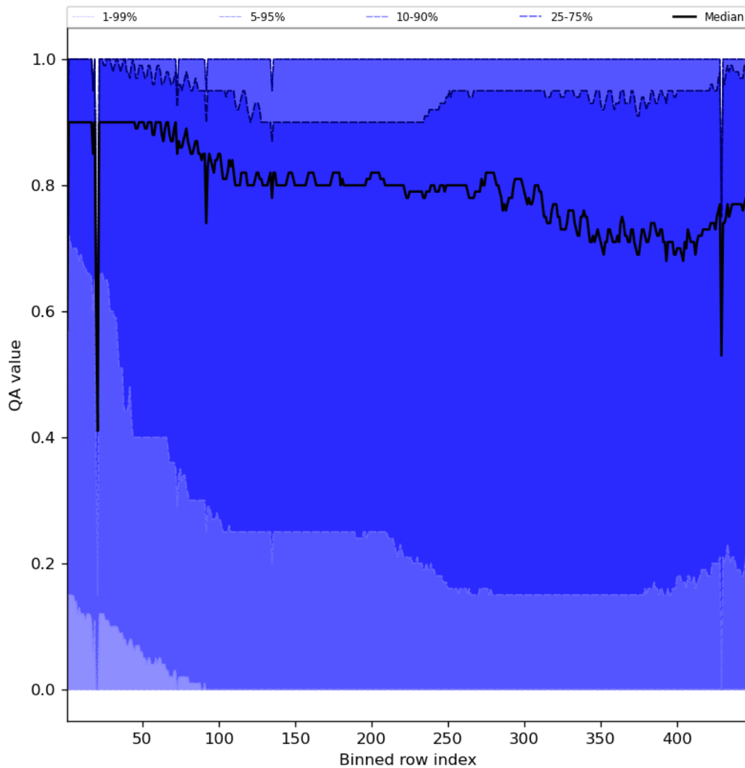
Figure 54: Along track statistics of “QA value” for 2023-07-13 to 2023-07-14
