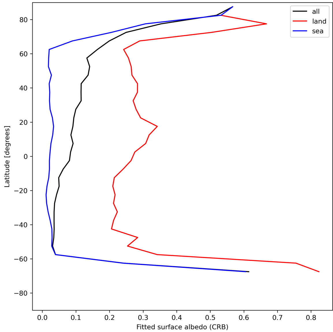
Figure 30: Zonal average of “Fitted surface albedo (CRB)” for 2023-07-13 to 2023-07-14.
