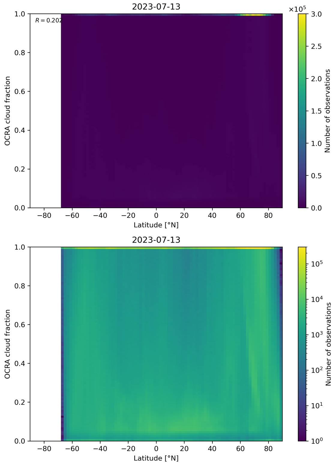
Figure 93: Scatter density plot of “Latitude” against “OCRA cloud fraction” for 2023-07-13 to 2023-07-14.
