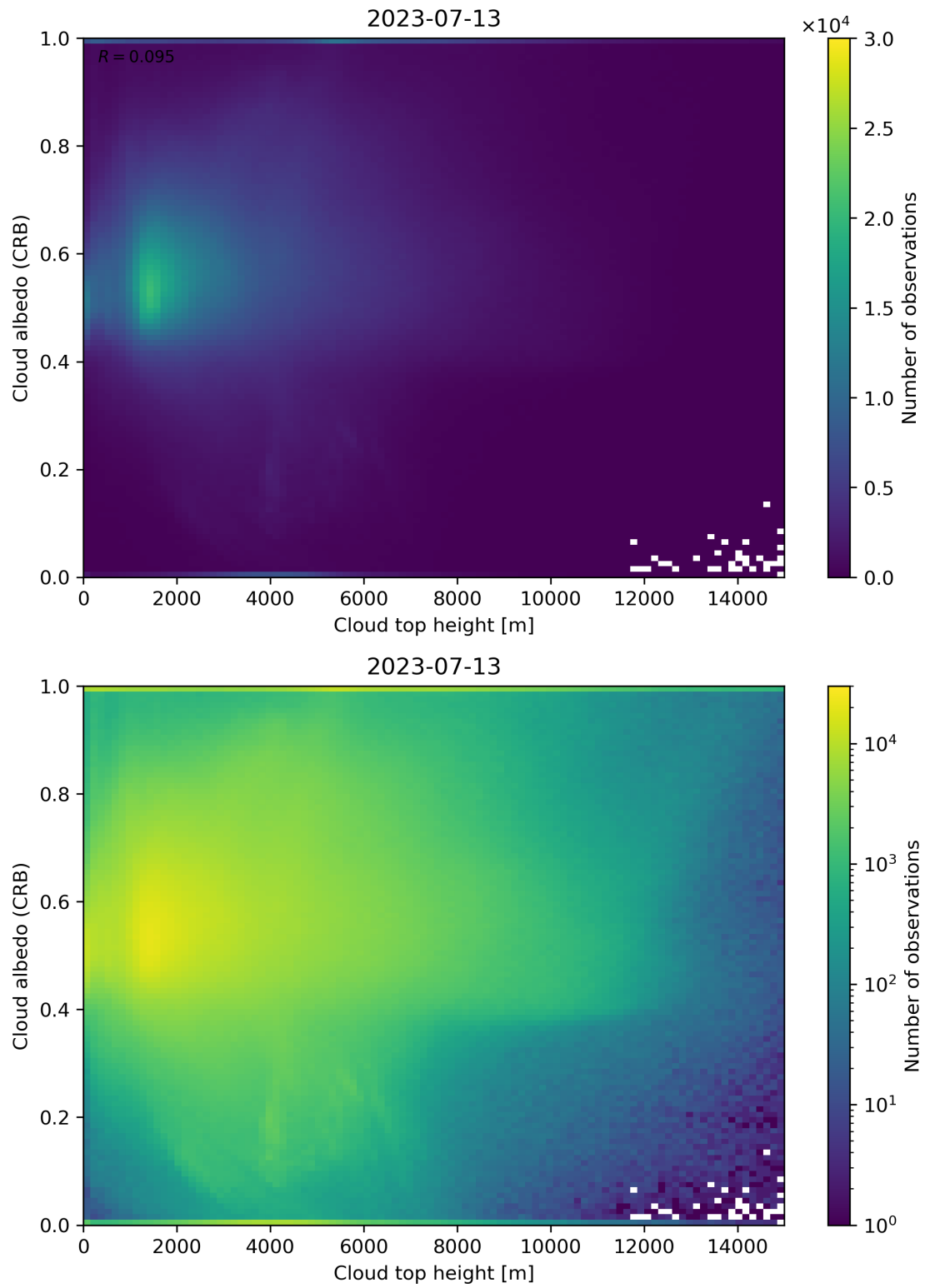
Figure 86: Scatter density plot of “Cloud top height” against “Cloud albedo (CRB)” for 2023-07-13 to 2023-07-14.
