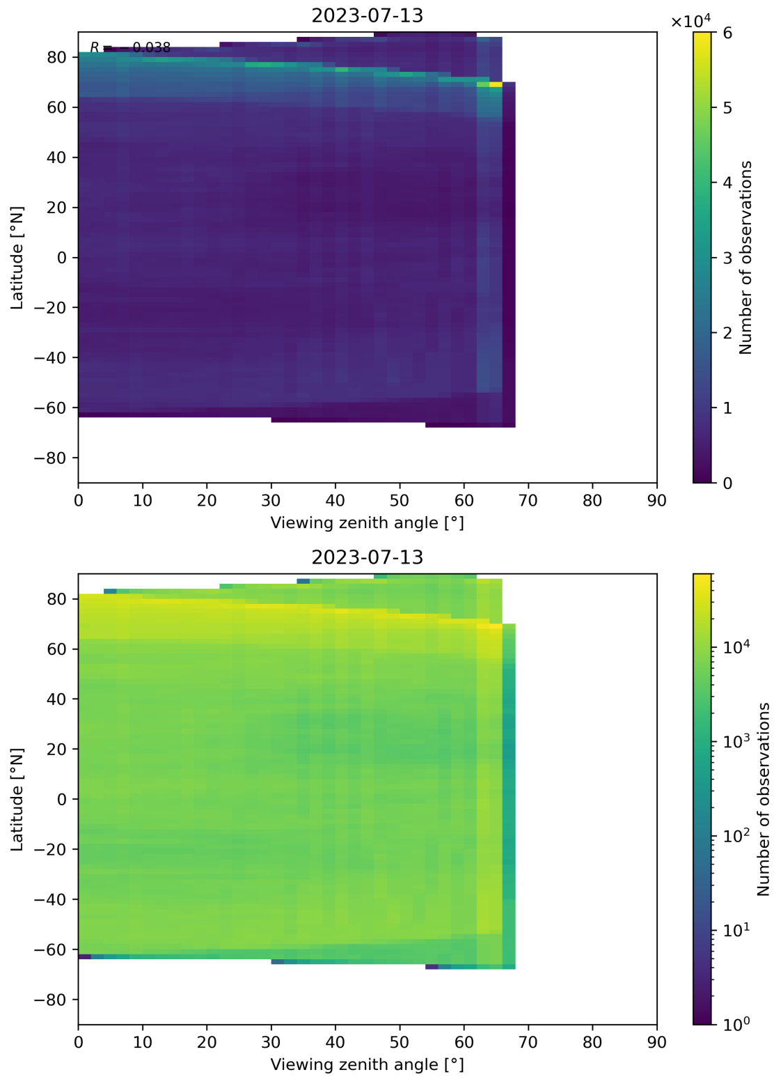
Figure 113: Scatter density plot of “Viewing zenith angle” against “Latitude” for 2023-07-13 to 2023-07-14.
