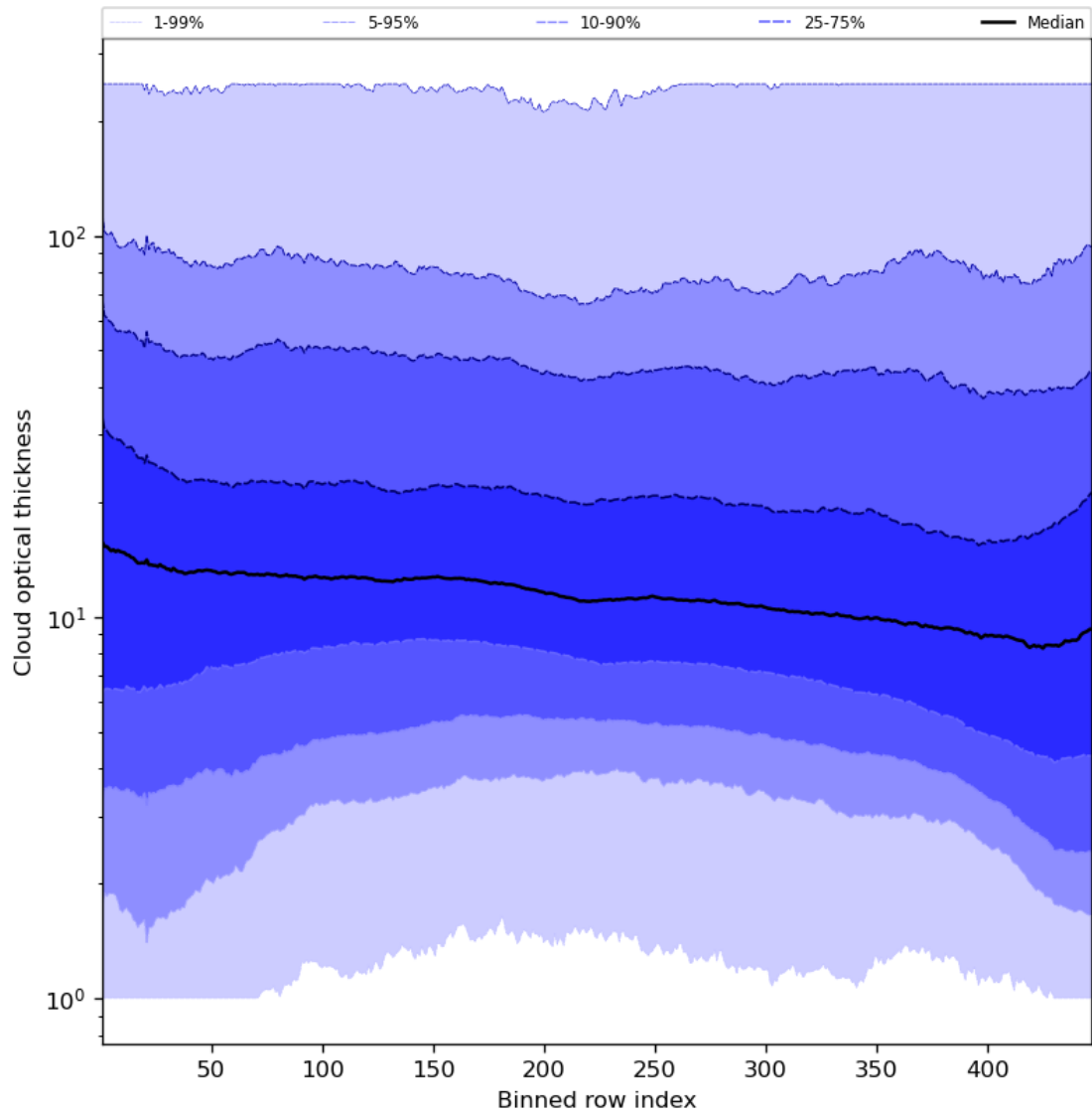
Figure 57: Along track statistics of “Cloud optical thickness” for 2023-07-13 to 2023-07-14
