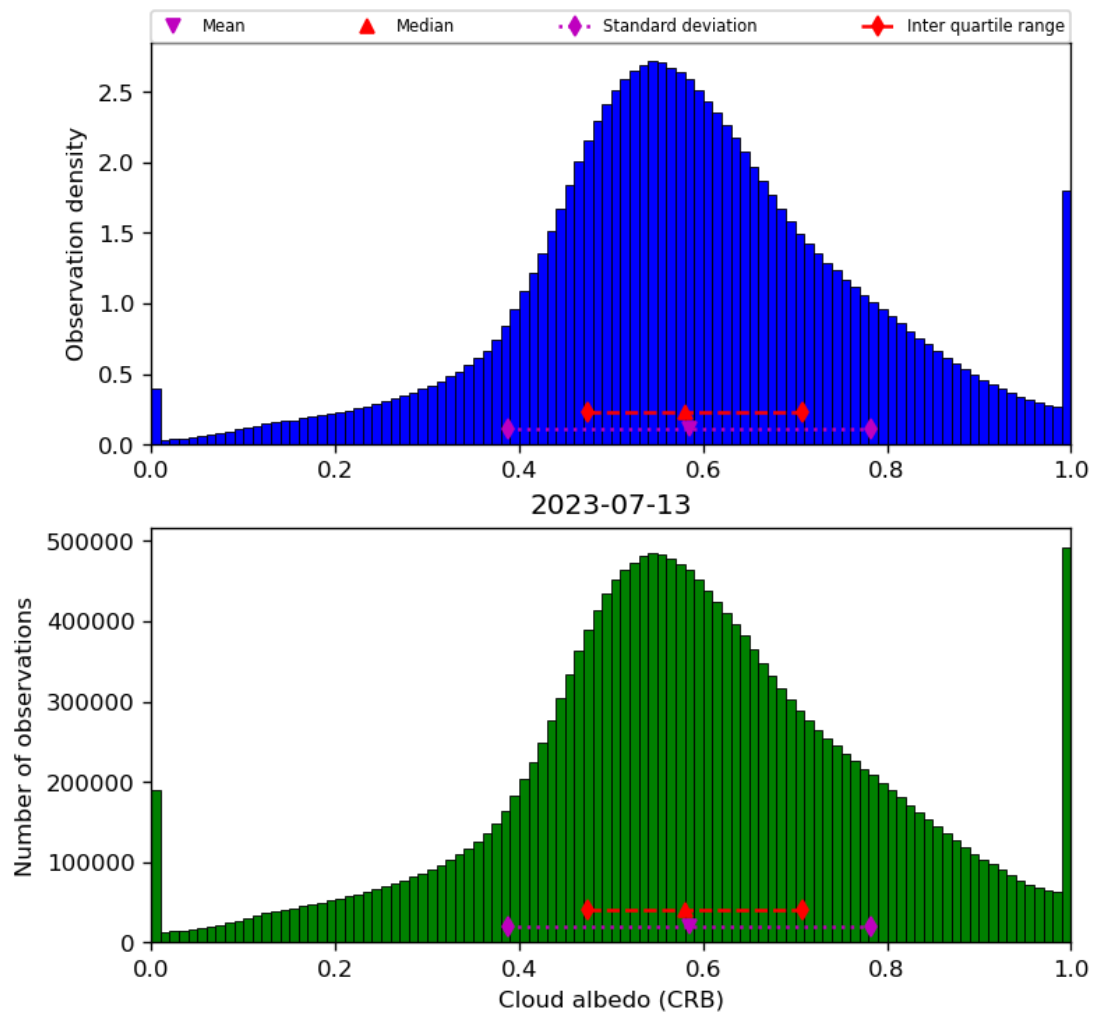
Figure 44: Histogram of “Cloud albedo (CRB)” for 2023-07-13 to 2023-07-14
