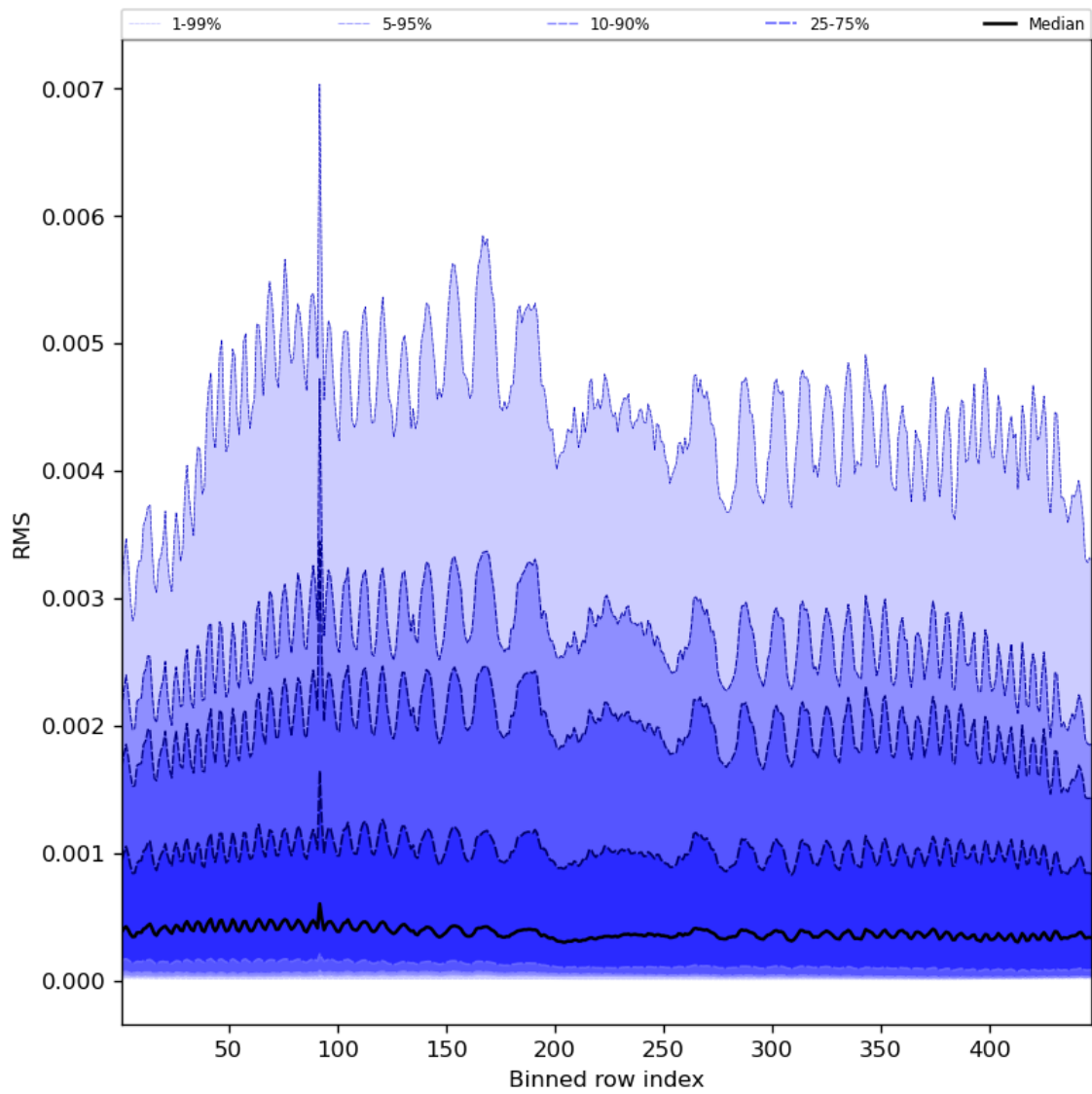
Figure 63: Along track statistics of “RMS” for 2023-07-13 to 2023-07-14
