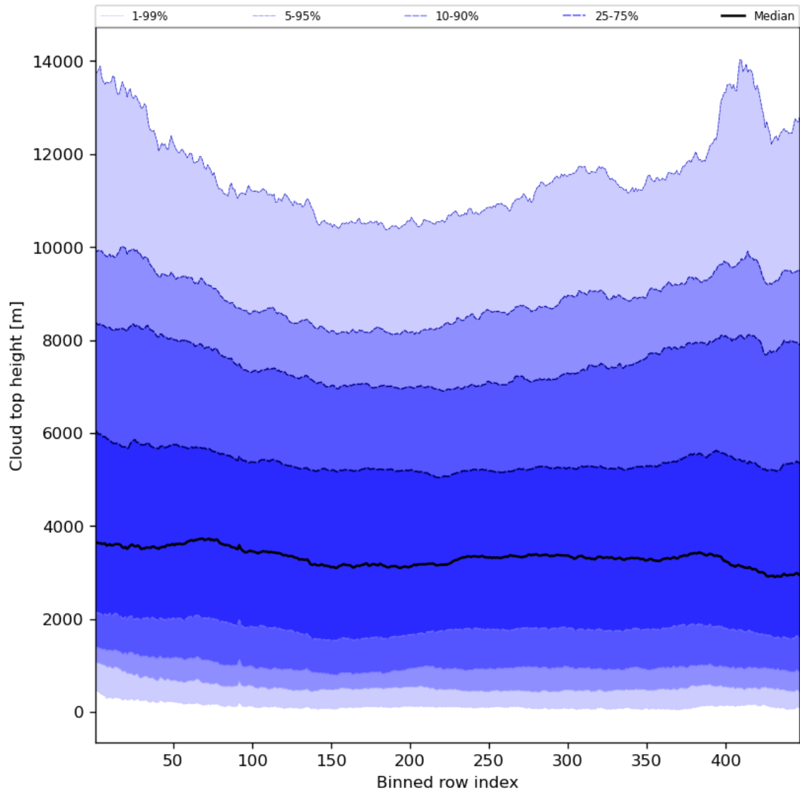
Figure 56: Along track statistics of “Cloud top height” for 2023-07-13 to 2023-07-14
