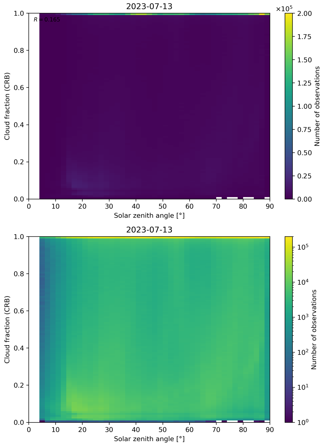
Figure 101: Scatter density plot of “Solar zenith angle” against “Cloud fraction (CRB)” for 2023-07-13 to 2023-07-14.
