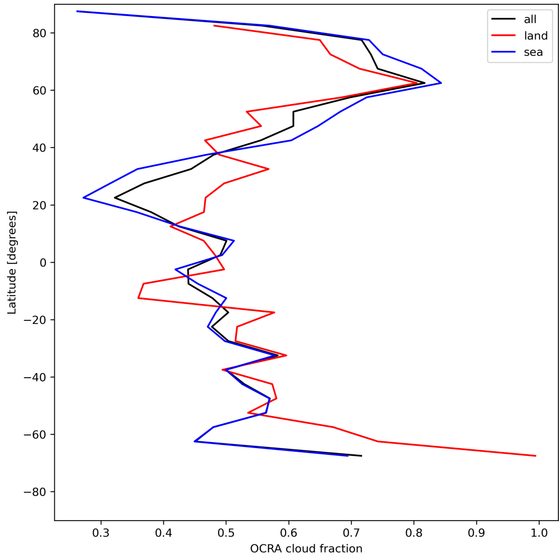
Figure 34: Zonal average of “OCRA cloud fraction” for 2023-07-13 to 2023-07-14.
