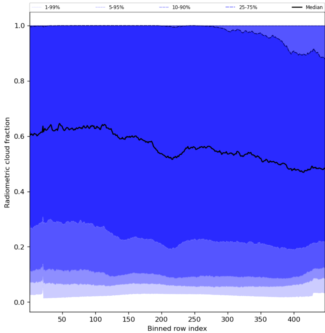
Figure 55: Along track statistics of “Radiometric cloud fraction” for 2023-07-13 to 2023-07-14
