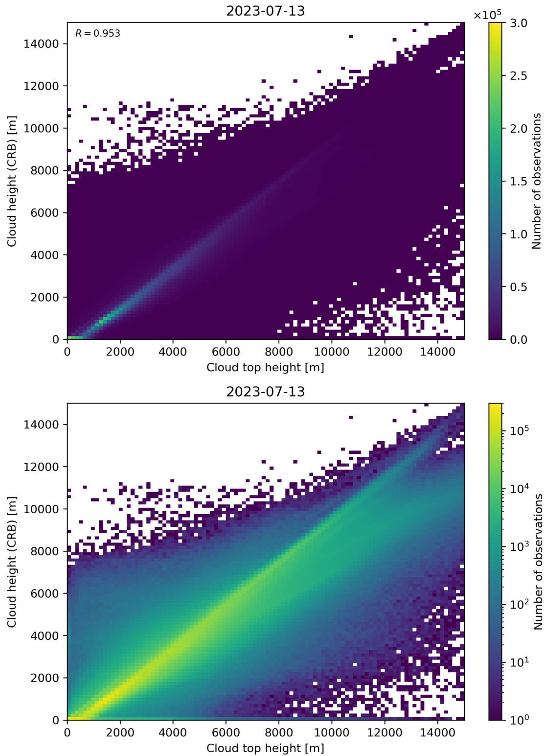
Figure 89: Scatter density plot of “Cloud top height” against “Cloud height (CRB)” for 2023-07-13 to 2023-07-14.
