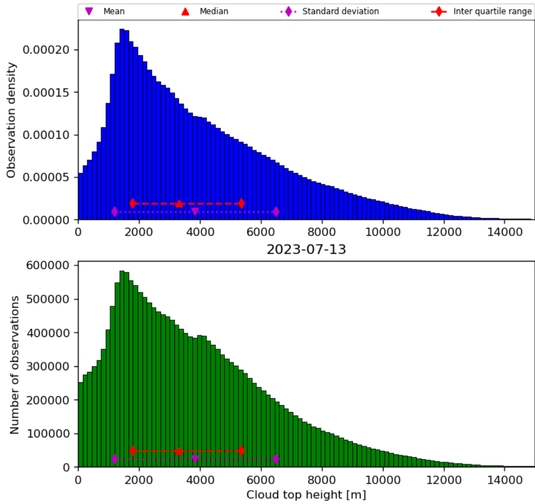
Figure 40: Histogram of “Cloud top height” for 2023-07-13 to 2023-07-14
