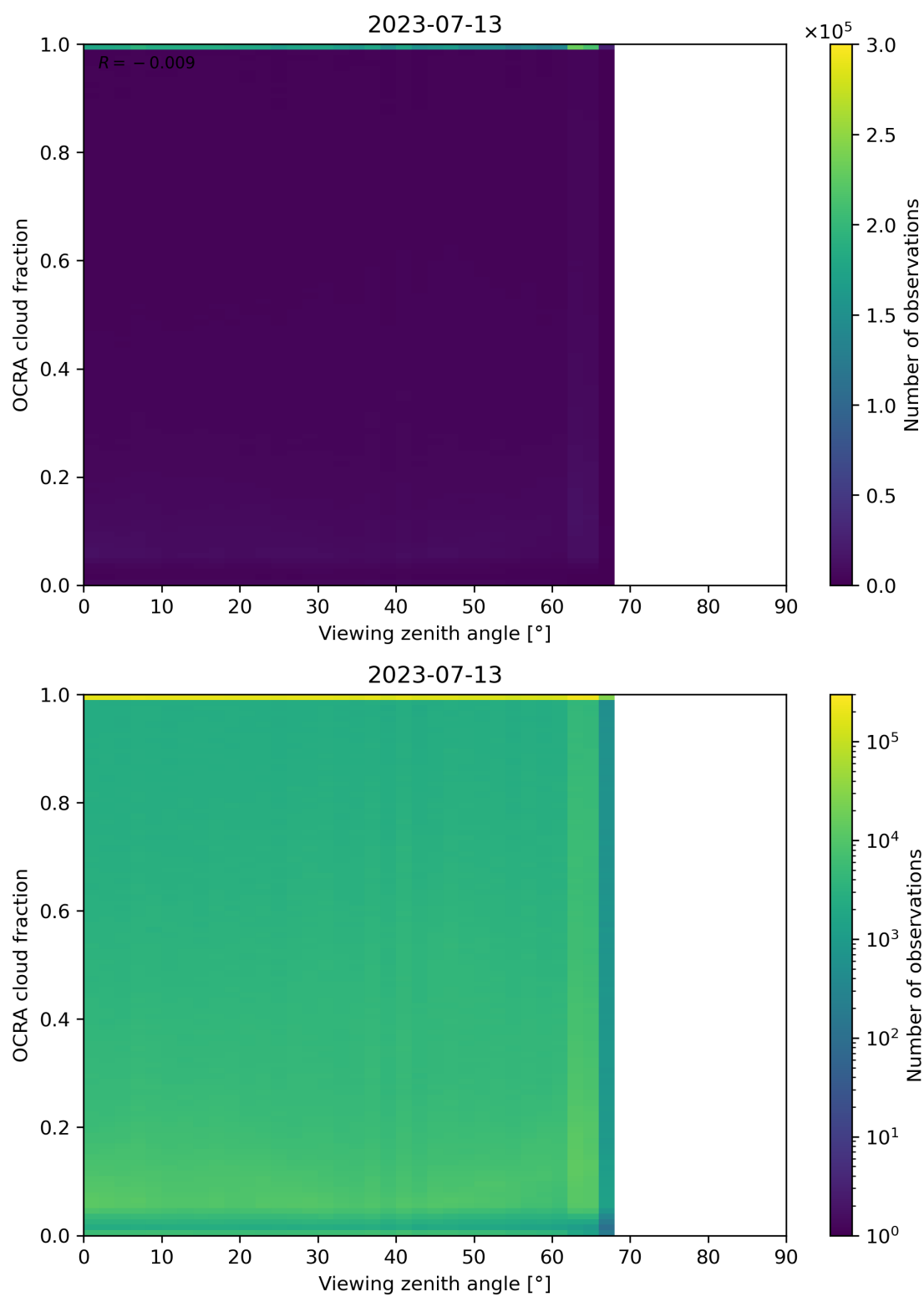
Figure 108: Scatter density plot of “Viewing zenith angle” against “OCRA cloud fraction” for 2023-07-13 to 2023-07-14.
