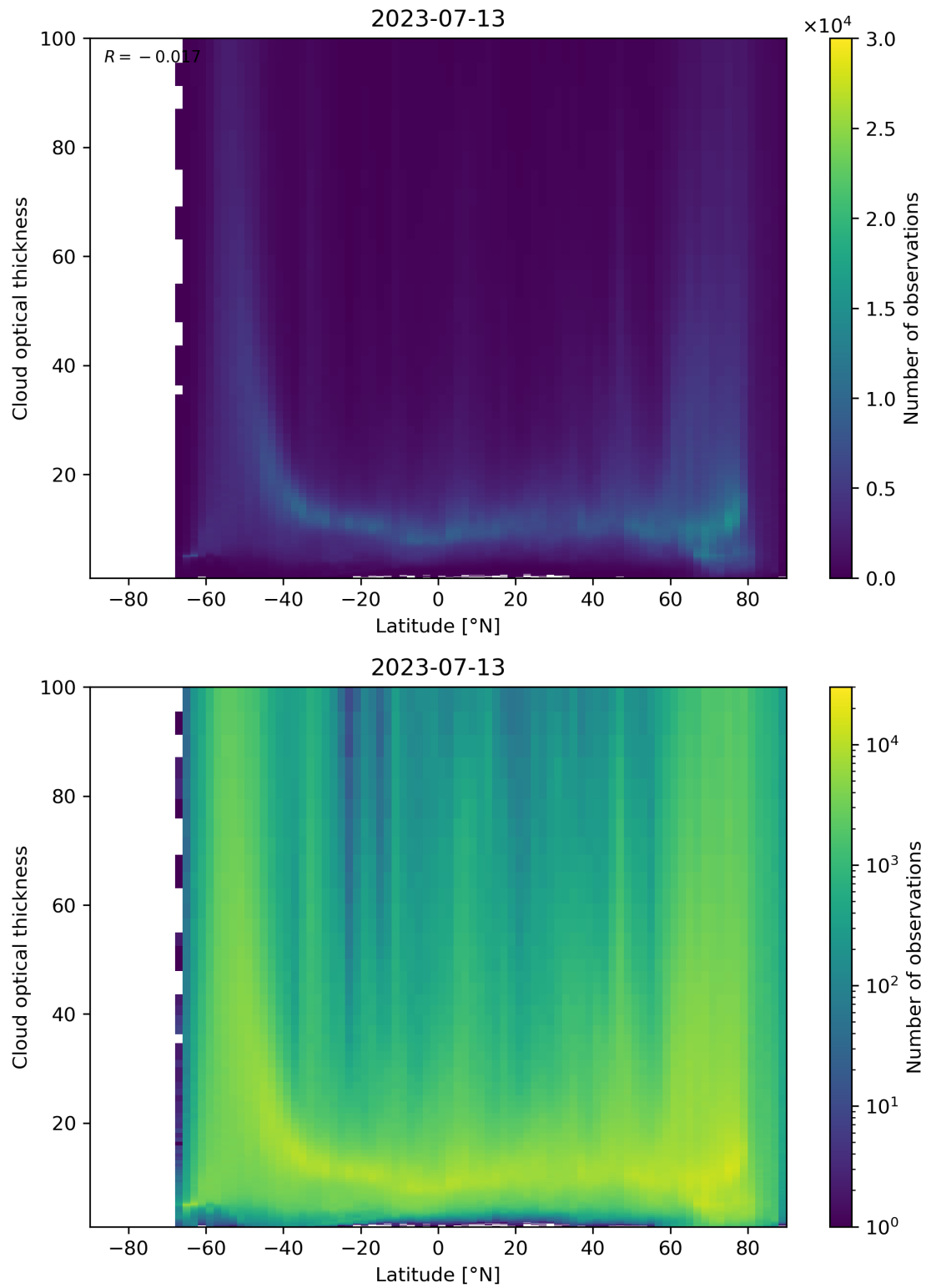
Figure 96: Scatter density plot of “Latitude” against “Cloud optical thickness” for 2023-07-13 to 2023-07-14.
