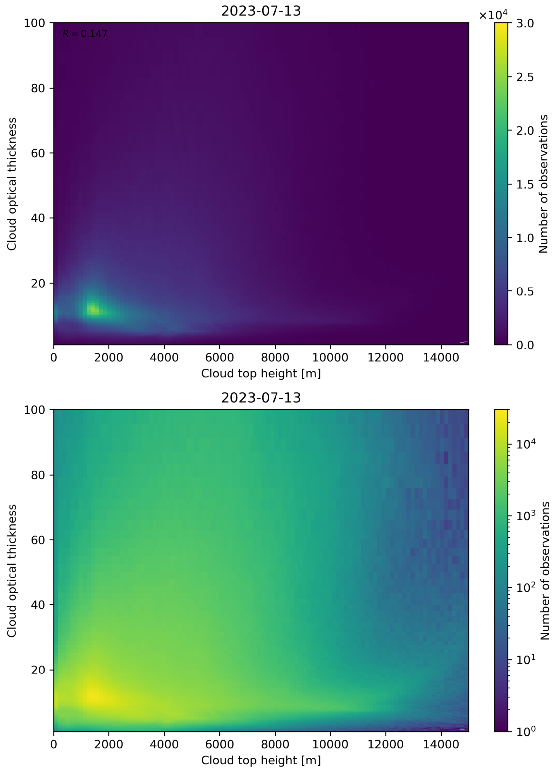
Figure 90: Scatter density plot of “Cloud top height” against “Cloud optical thickness” for 2023-07-13 to 2023-07-14.
