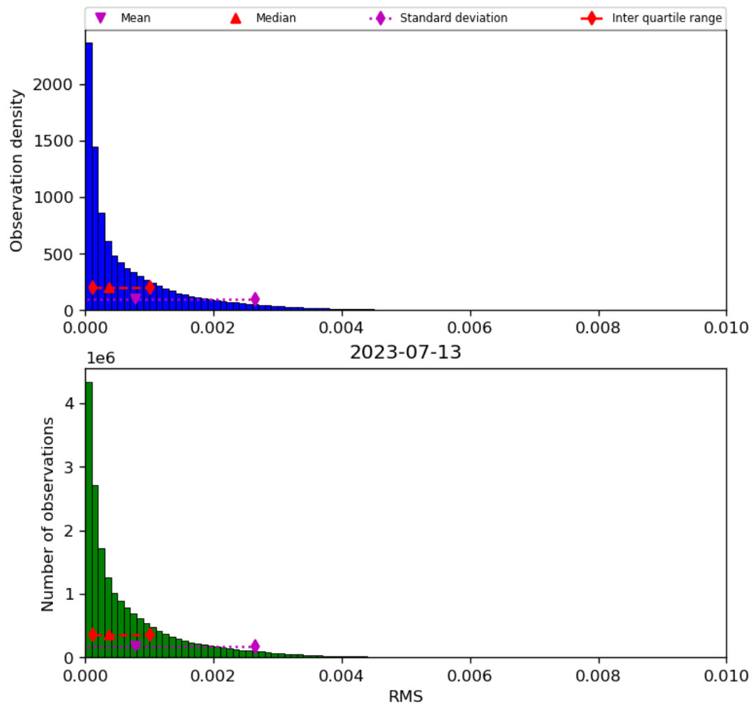
Figure 47: Histogram of “RMS” for 2023-07-13 to 2023-07-14
