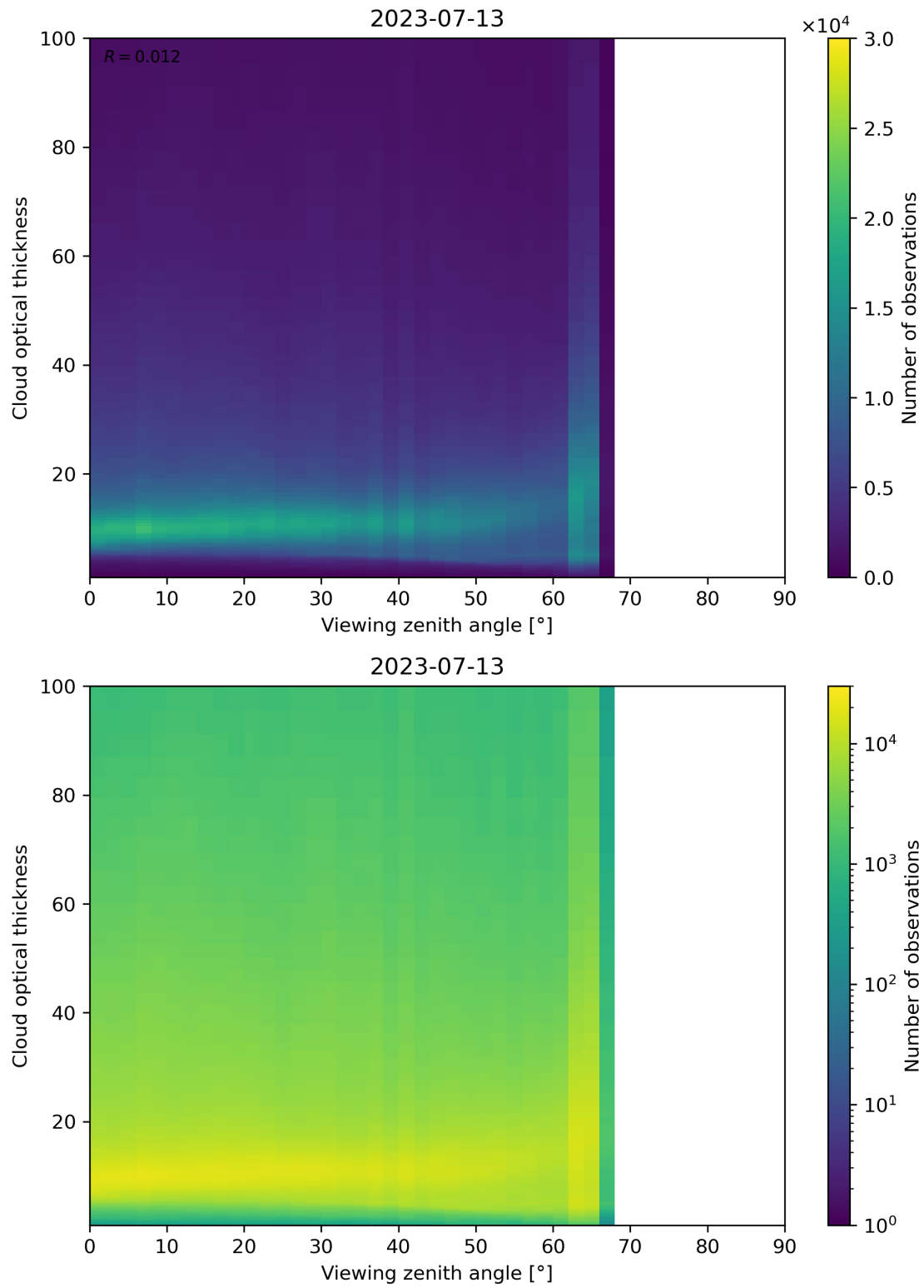
Figure 111: Scatter density plot of “Viewing zenith angle” against “Cloud optical thickness” for 2023-07-13 to 2023-07-14.
