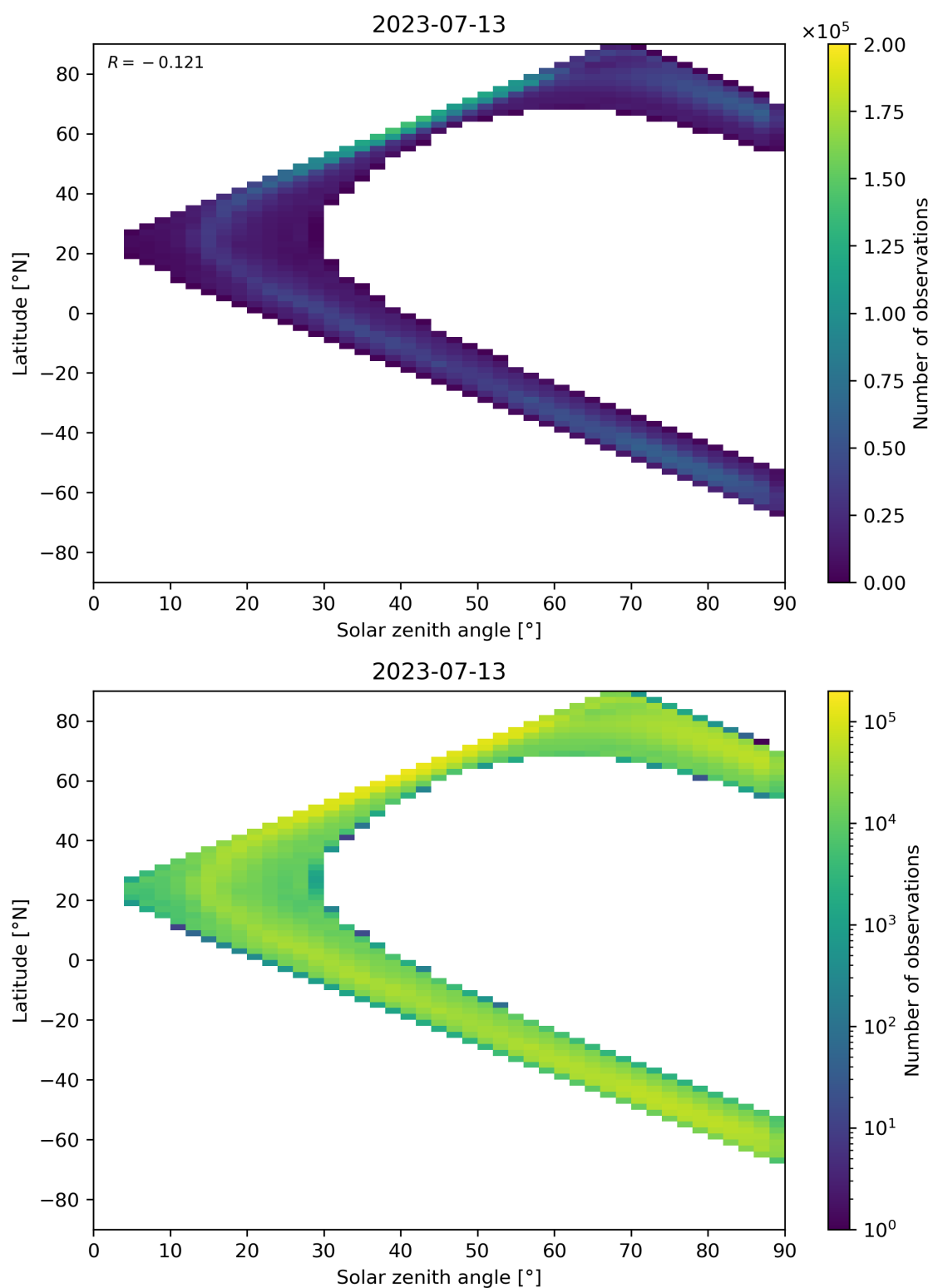
Figure 105: Scatter density plot of “Solar zenith angle” against “Latitude” for 2023-07-13 to 2023-07-14.
