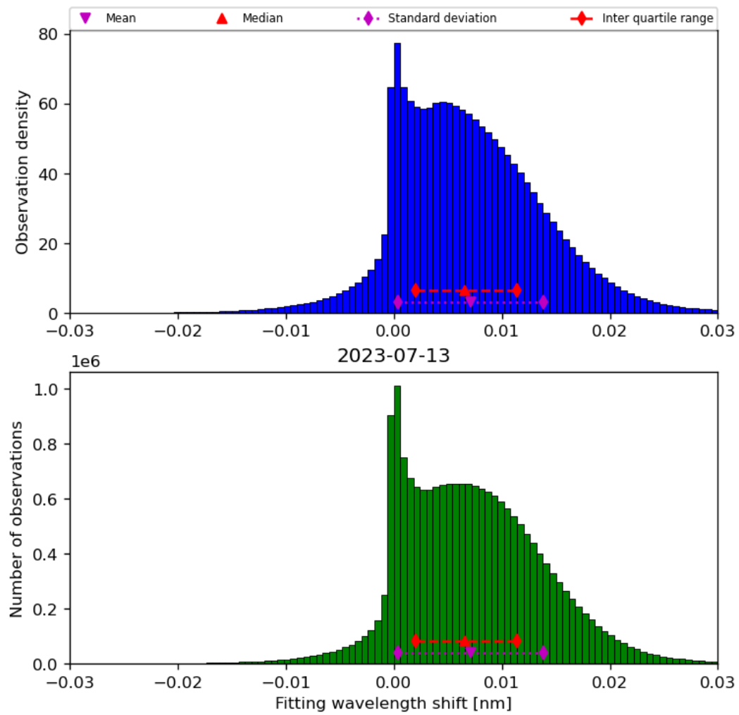
Figure 49: Histogram of “Fitting wavelength shift” for 2023-07-13 to 2023-07-14
