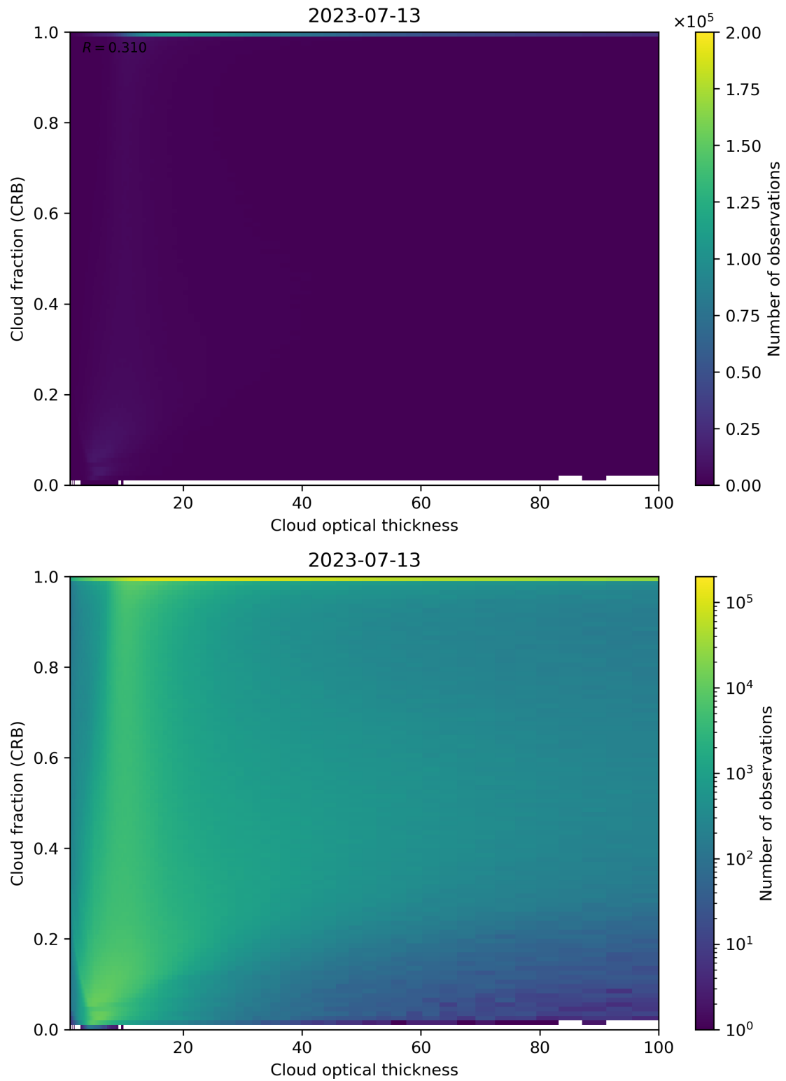
Figure 84: Scatter density plot of “Cloud optical thickness” against “Cloud fraction (CRB)” for 2023-07-13 to 2023-07-14.
