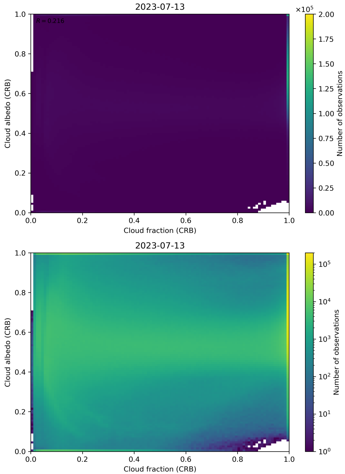
Figure 77: Scatter density plot of “Cloud fraction (CRB)” against “Cloud albedo (CRB)” for 2023-07-13 to 2023-07-14.
