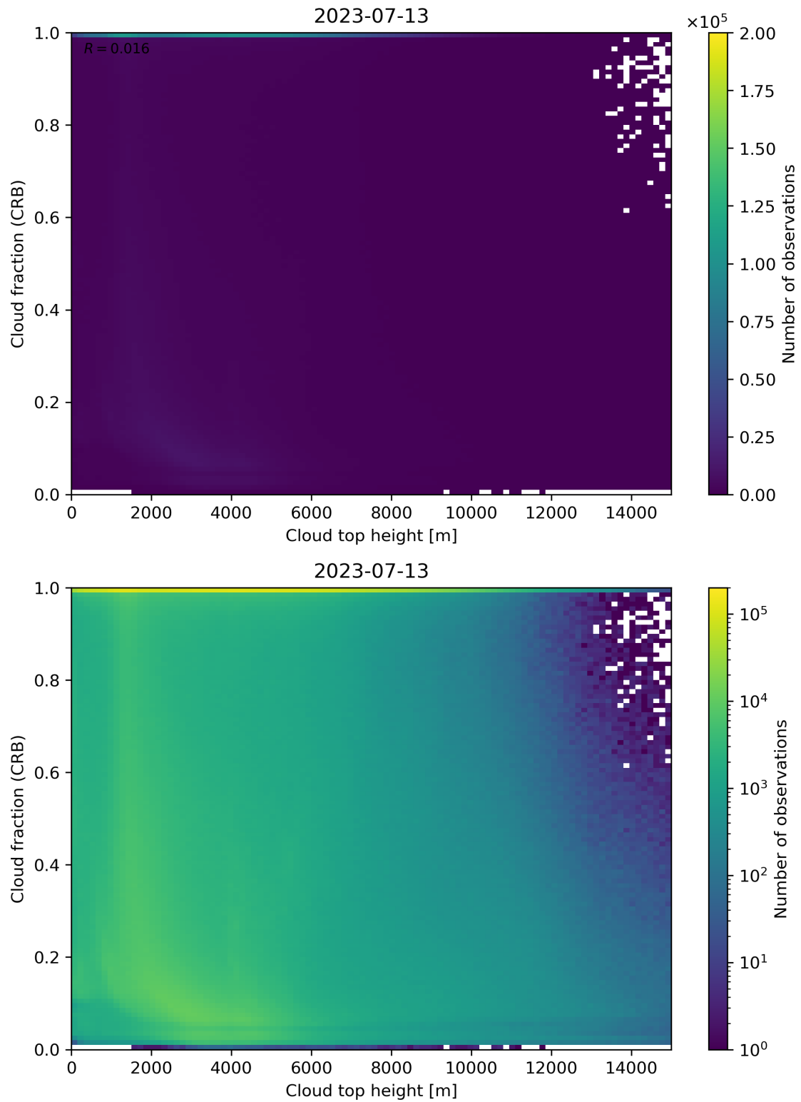
Figure 88: Scatter density plot of “Cloud top height” against “Cloud fraction (CRB)” for 2023-07-13 to 2023-07-14.
