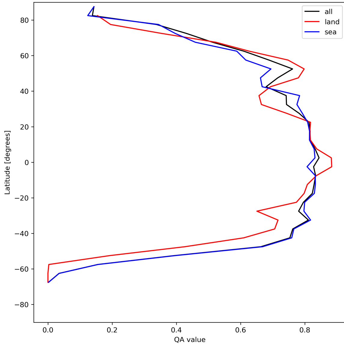
Figure 22: Zonal average of “QA value” for 2023-07-13 to 2023-07-14.
