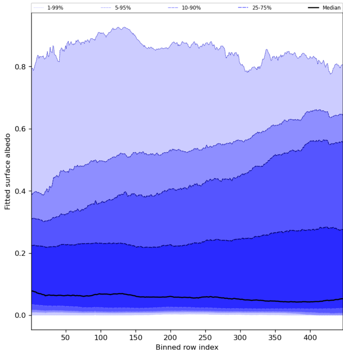
Figure 61: Along track statistics of “Fitted surface albedo” for 2023-07-13 to 2023-07-14
