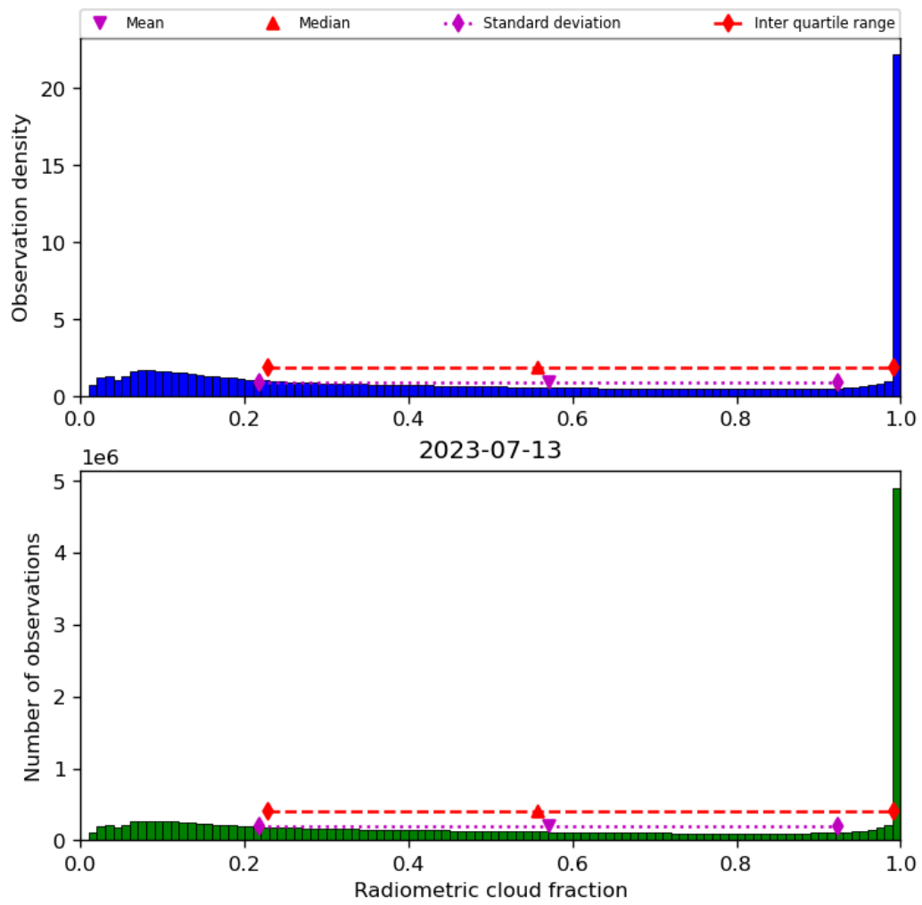
Figure 39: Histogram of “Radiometric cloud fraction” for 2023-07-13 to 2023-07-14
