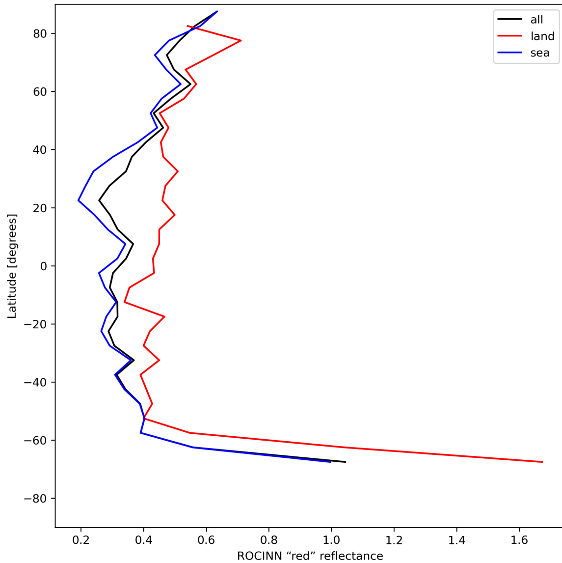
Figure 37: Zonal average of “ROCINN “red” reflectance” for 2023-07-13 to 2023-07-14.
