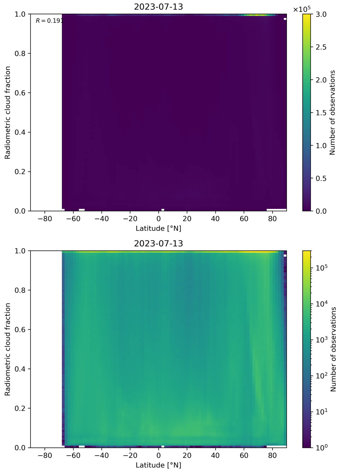
Figure 92: Scatter density plot of “Latitude” against “Radiometric cloud fraction” for 2023-07-13 to 2023-07-14.
