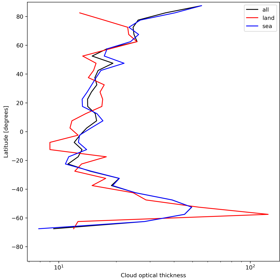
Figure 25: Zonal average of “Cloud optical thickness” for 2023-07-13 to 2023-07-14.
