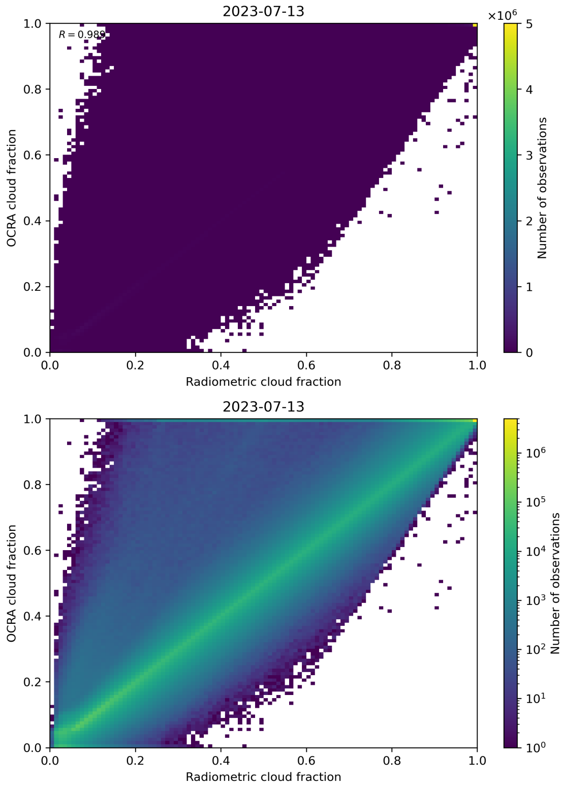
Figure 72: Scatter density plot of “Radiometric cloud fraction” against “OCRA cloud fraction” for 2023-07-13 to 2023-07-14.
