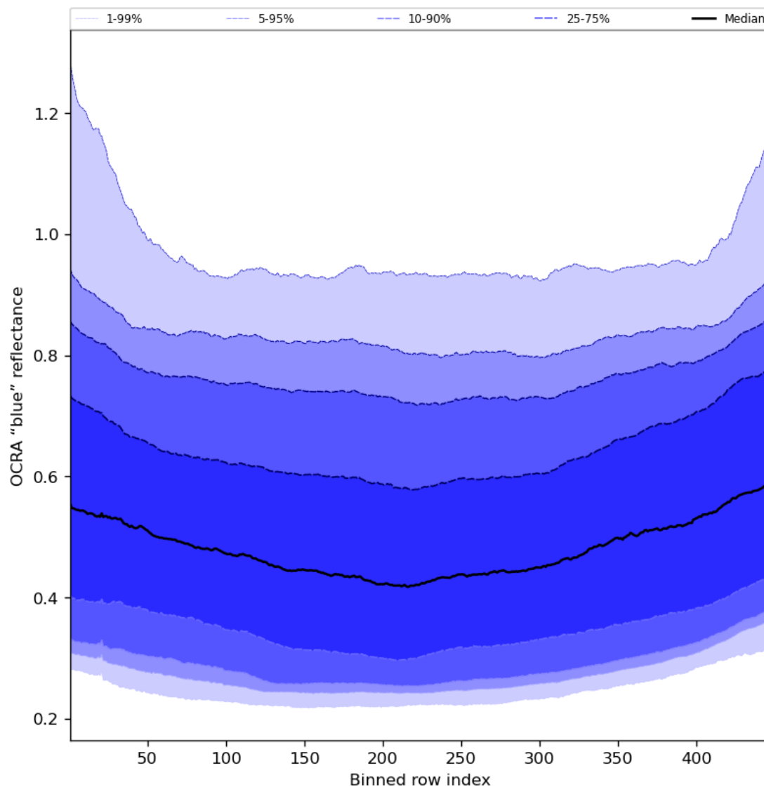
Figure 67: Along track statistics of “OCRA “blue” reflectance” for 2023-07-13 to 2023-07-14
