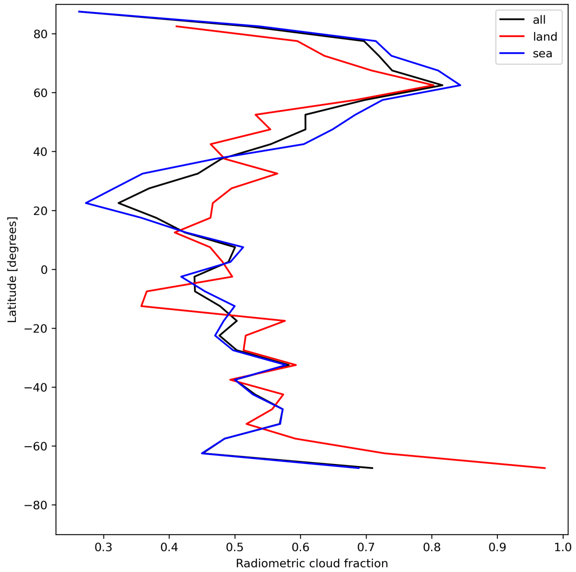
Figure 23: Zonal average of “Radiometric cloud fraction” for 2023-07-13 to 2023-07-14.
