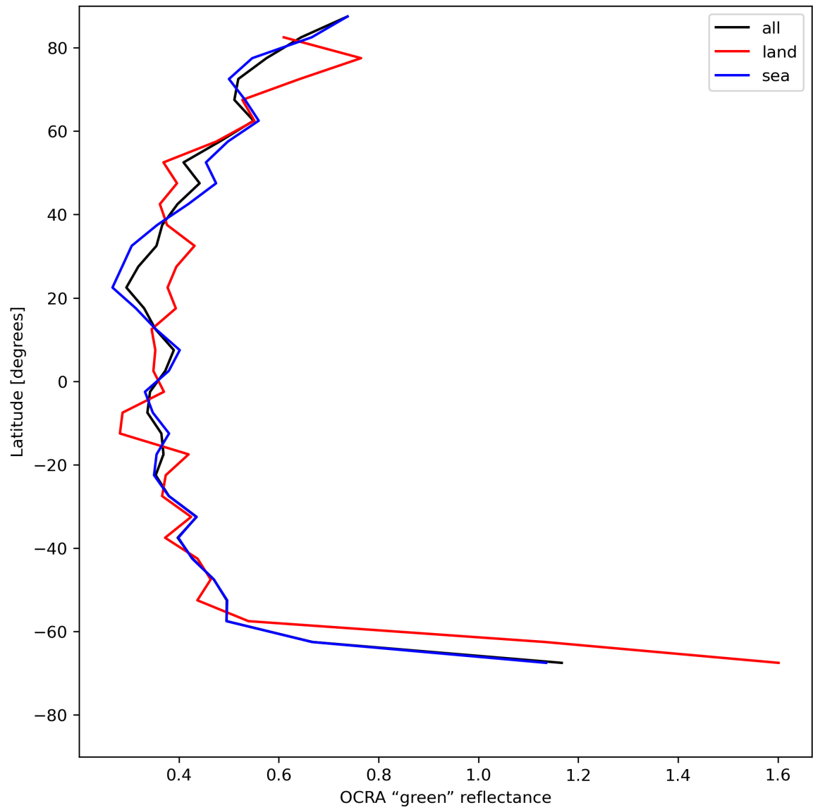
Figure 36: Zonal average of “OCRA “green” reflectance” for 2023-07-13 to 2023-07-14.
