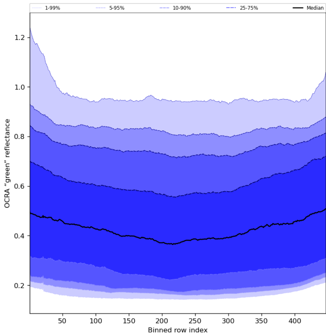
Figure 68: Along track statistics of “OCRA “green” reflectance” for 2023-07-13 to 2023-07-14
