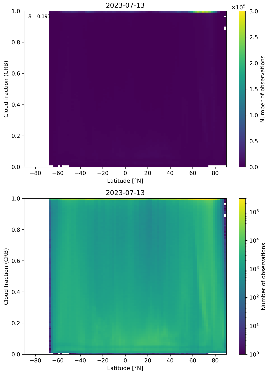
Figure 94: Scatter density plot of “Latitude” against “Cloud fraction (CRB)” for 2023-07-13 to 2023-07-14.
