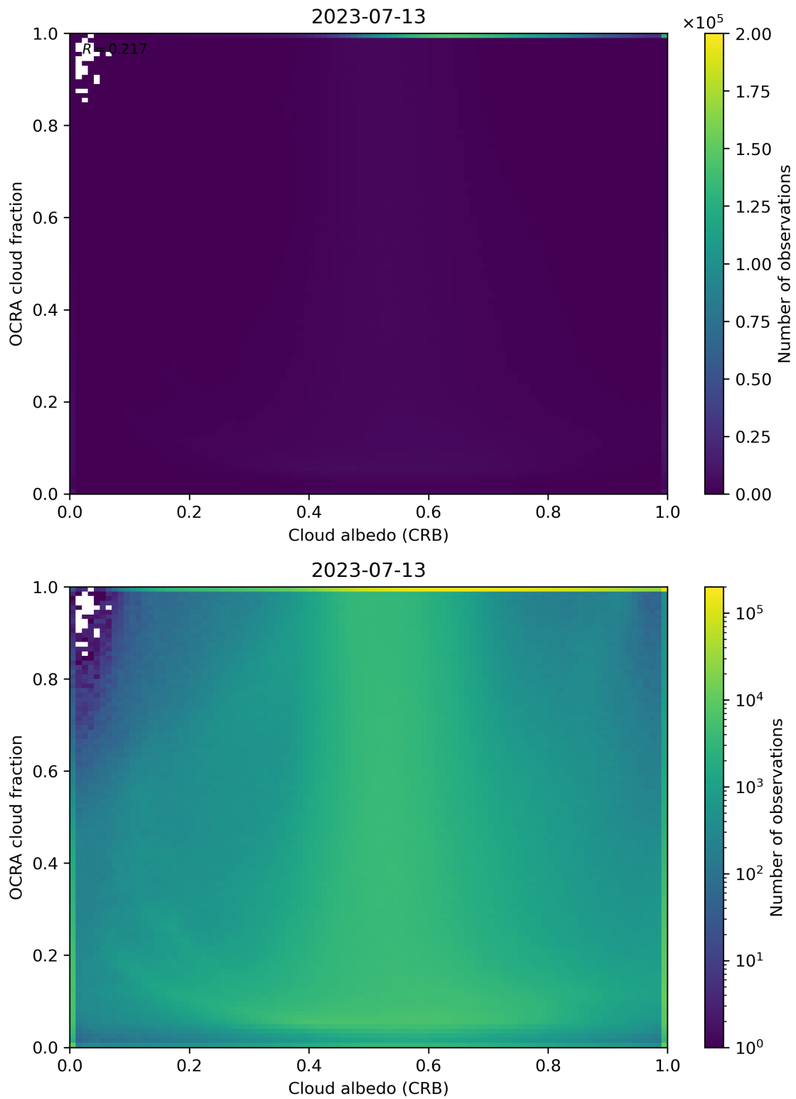
Figure 70: Scatter density plot of “Cloud albedo (CRB)” against “OCRA cloud fraction” for 2023-07-13 to 2023-07-14.
