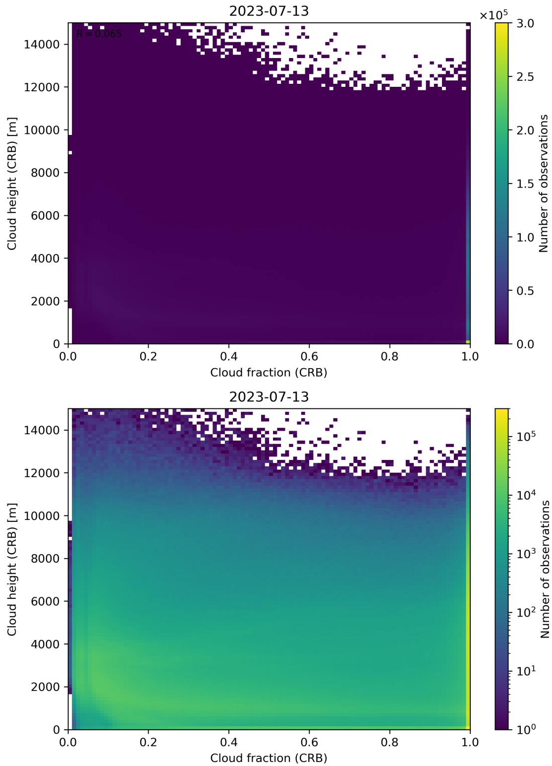
Figure 79: Scatter density plot of “Cloud fraction (CRB)” against “Cloud height (CRB)” for 2023-07-13 to 2023-07-14.
