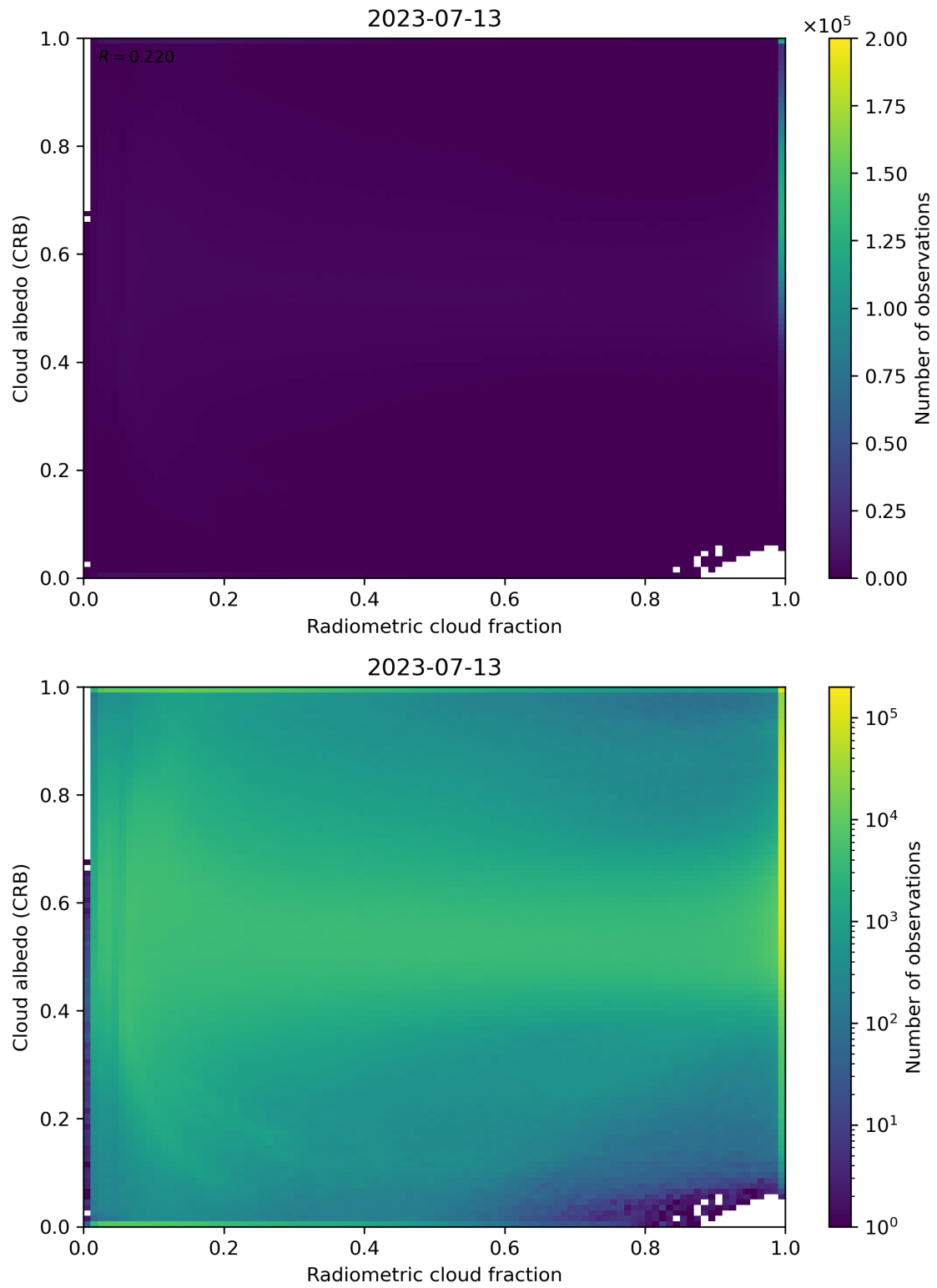
Figure 71: Scatter density plot of “Radiometric cloud fraction” against “Cloud albedo (CRB)” for 2023-07-13 to 2023-07-14.
