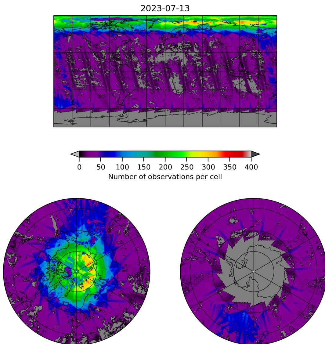
Figure 21: Map of the number of observations for 2023-07-13 to 2023-07-14
