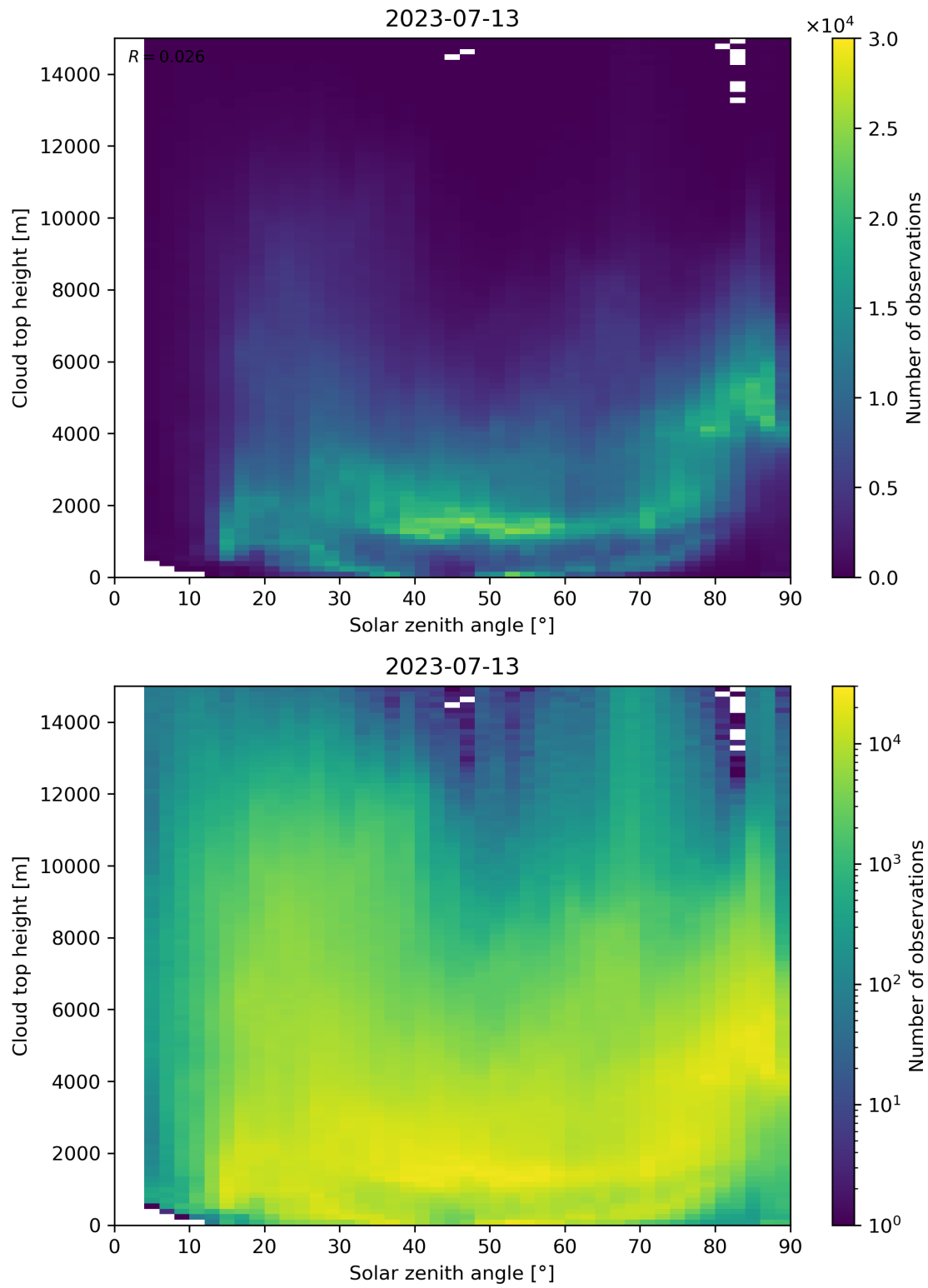
Figure 104: Scatter density plot of “Solar zenith angle” against “Cloud top height” for 2023-07-13 to 2023-07-14.
