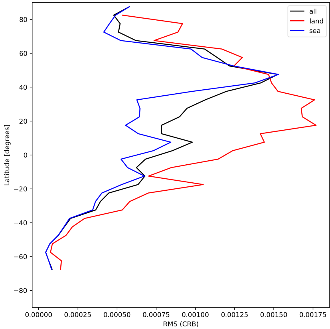
Figure 32: Zonal average of “RMS (CRB)” for 2023-07-13 to 2023-07-14.
