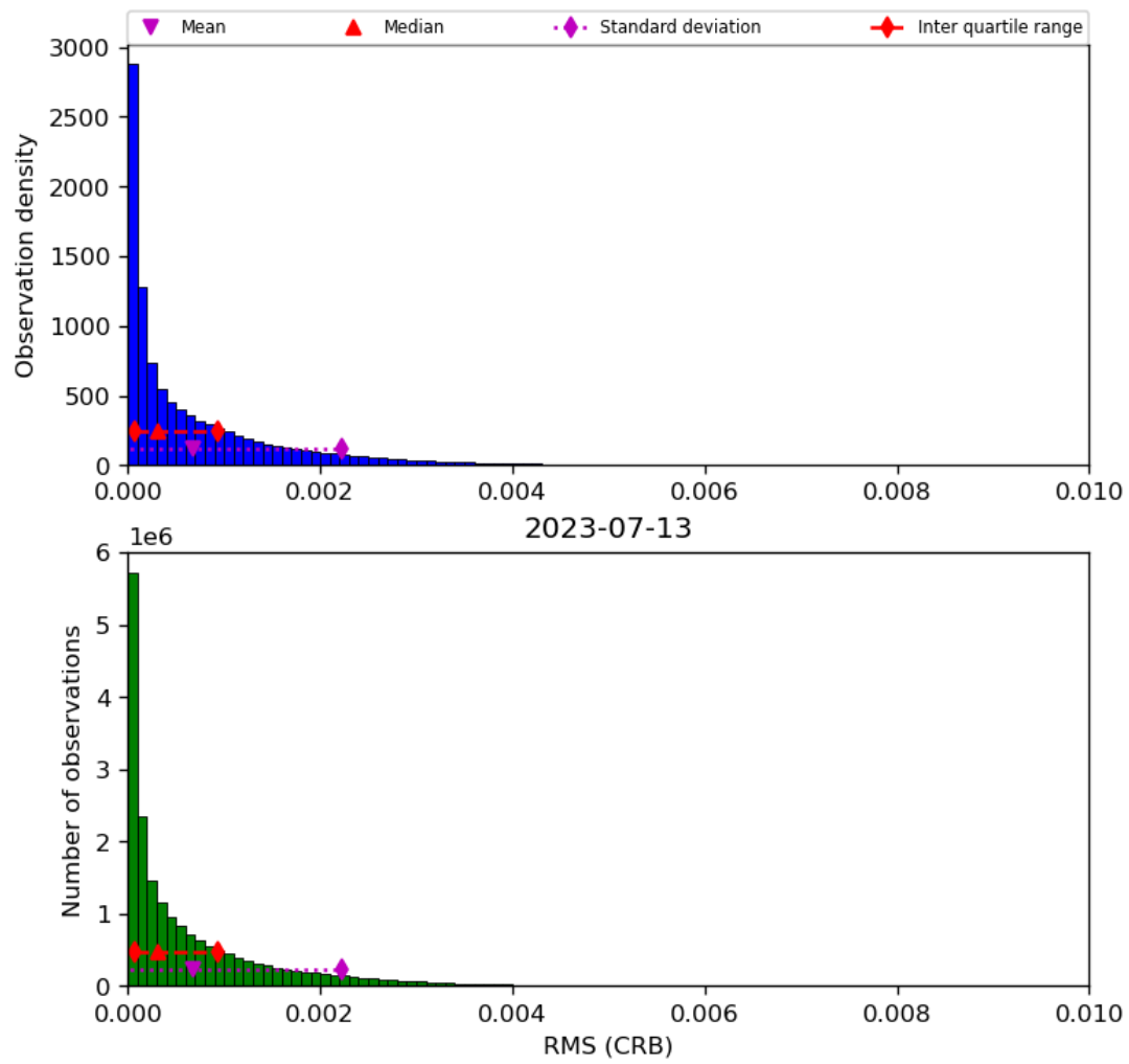
Figure 48: Histogram of “RMS (CRB)” for 2023-07-13 to 2023-07-14
