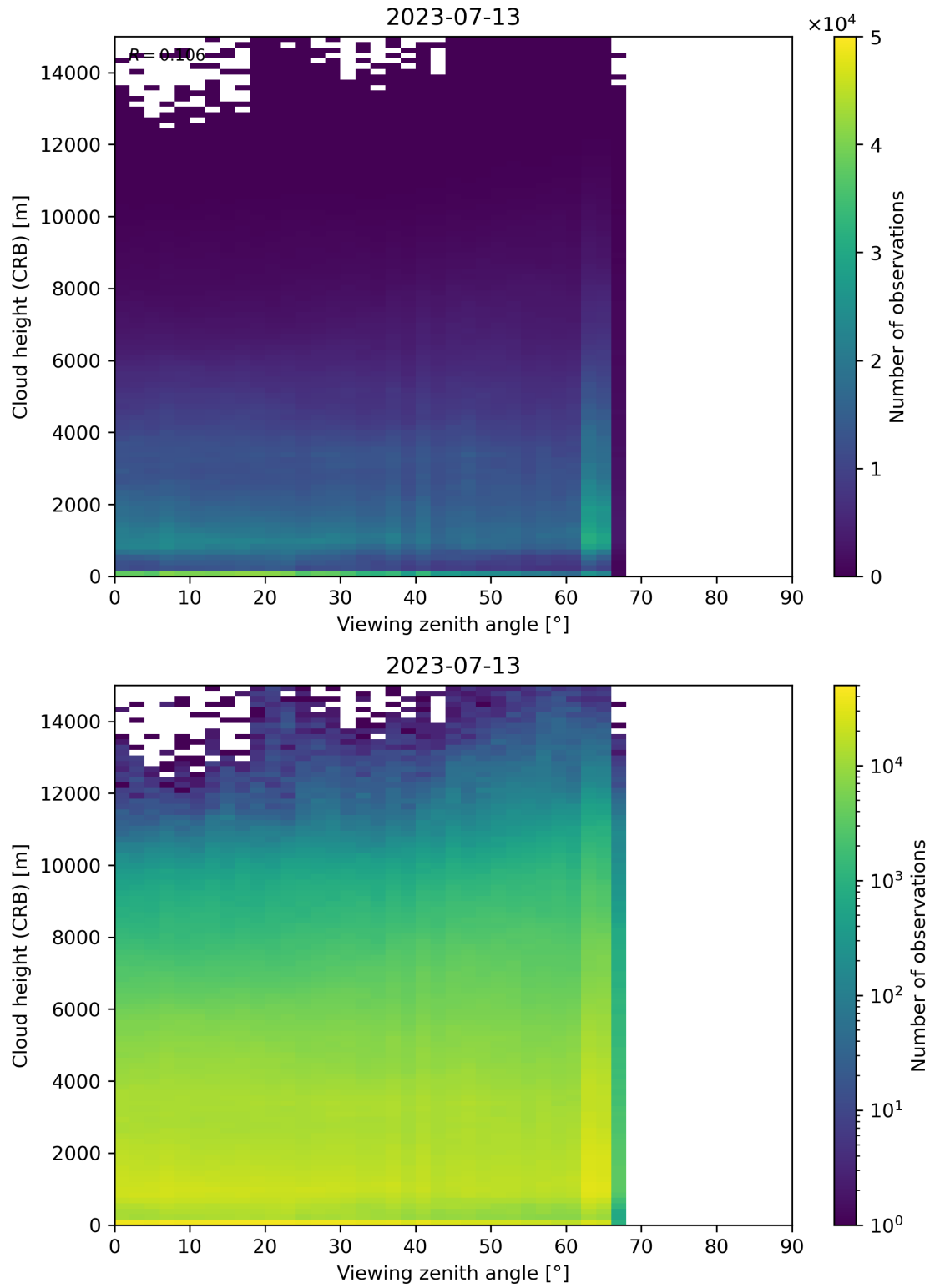
Figure 110: Scatter density plot of “Viewing zenith angle” against “Cloud height (CRB)” for 2023-07-13 to 2023-07-14.
