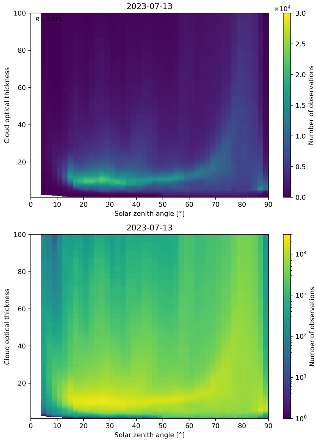
Figure 103: Scatter density plot of “Solar zenith angle” against “Cloud optical thickness” for 2023-07-13 to 2023-07-14.
