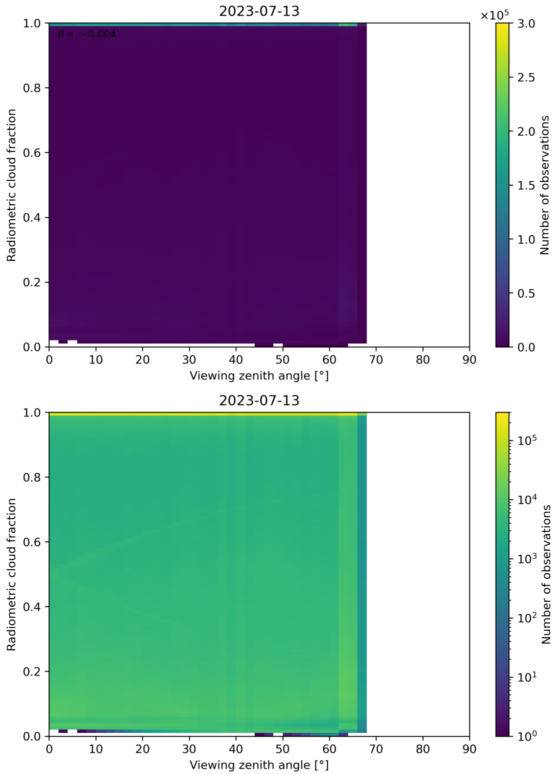
Figure 107: Scatter density plot of “Viewing zenith angle” against “Radiometric cloud fraction” for 2023-07-13 to 2023-07-14.
