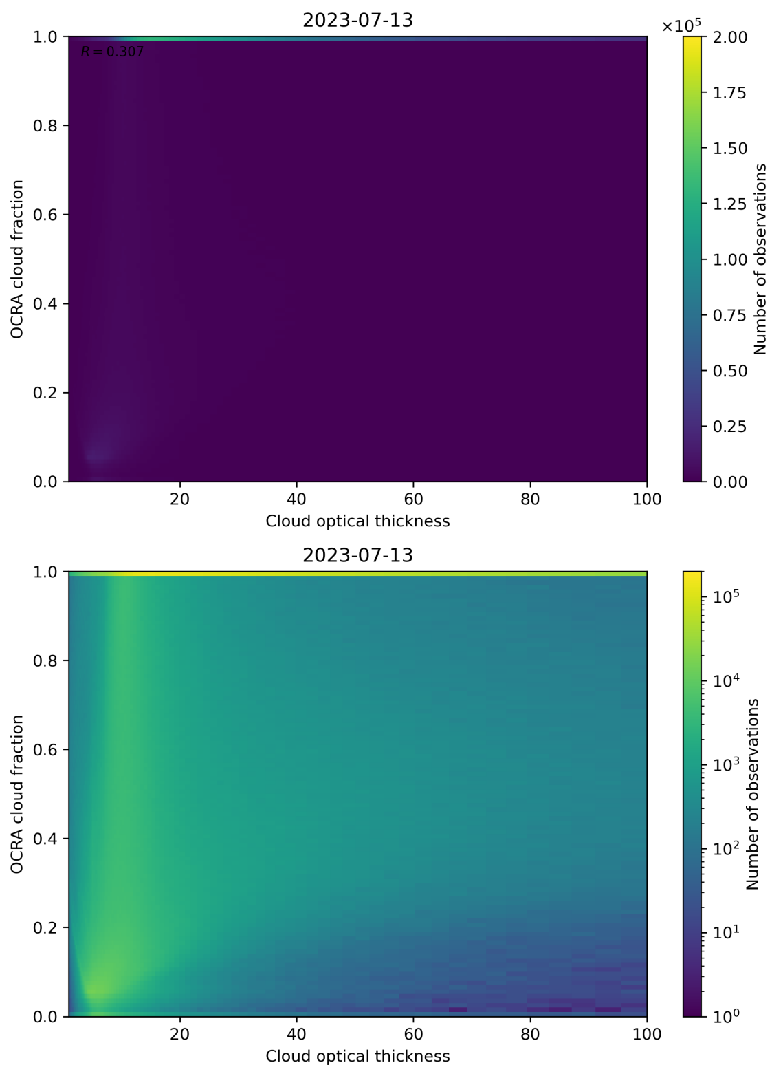
Figure 83: Scatter density plot of “Cloud optical thickness” against “OCRA cloud fraction” for 2023-07-13 to 2023-07-14.
