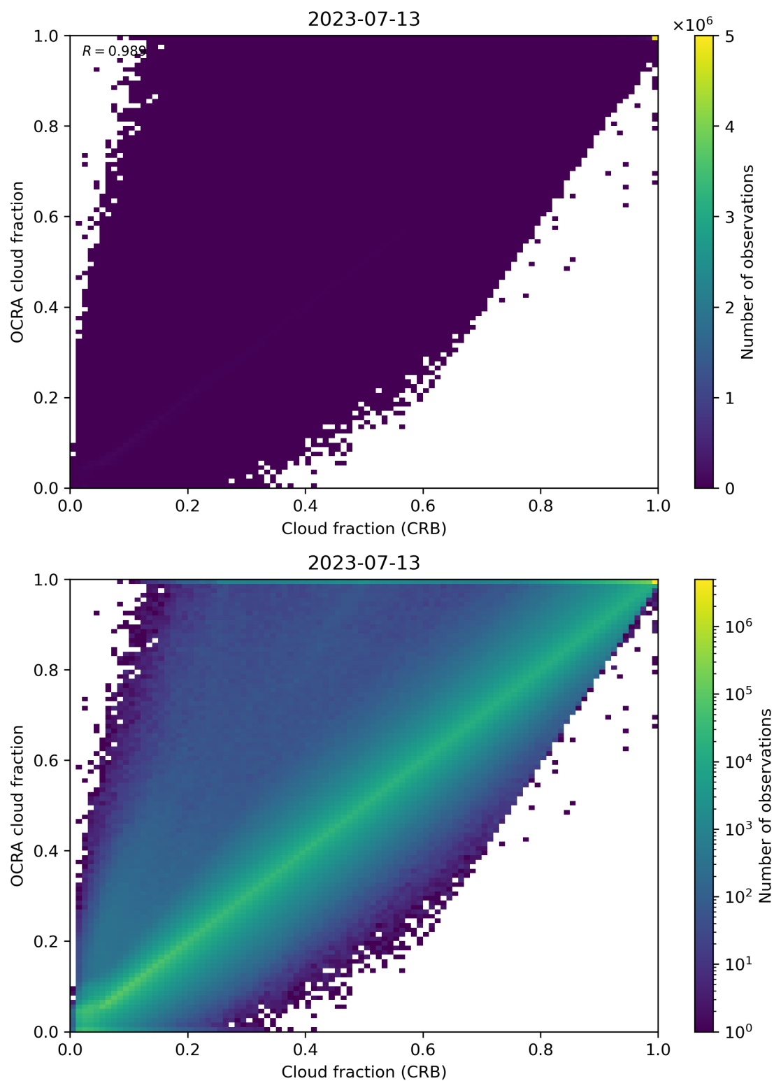
Figure 78: Scatter density plot of “Cloud fraction (CRB)” against “OCRA cloud fraction” for 2023-07-13 to 2023-07-14.
