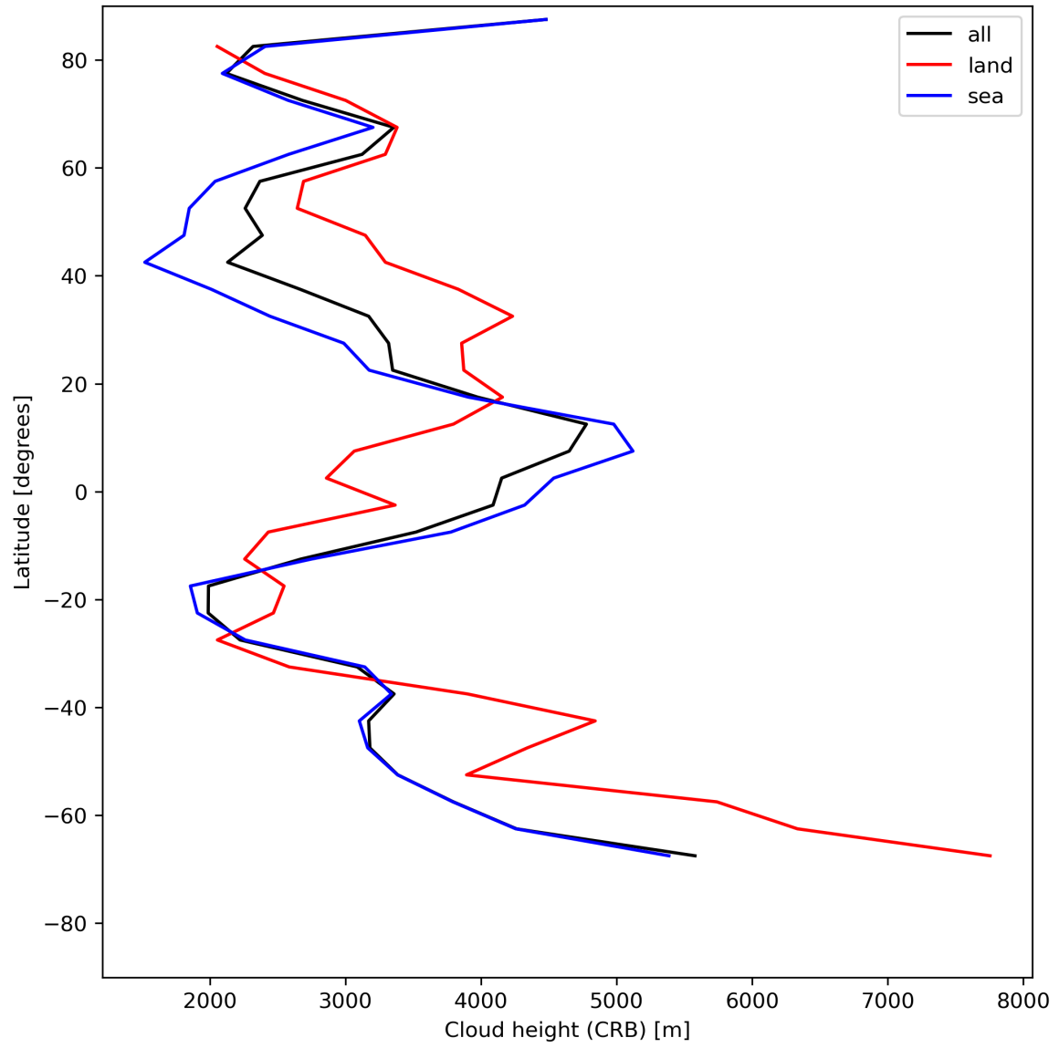
Figure 27: Zonal average of “Cloud height (CRB)” for 2023-07-13 to 2023-07-14.
