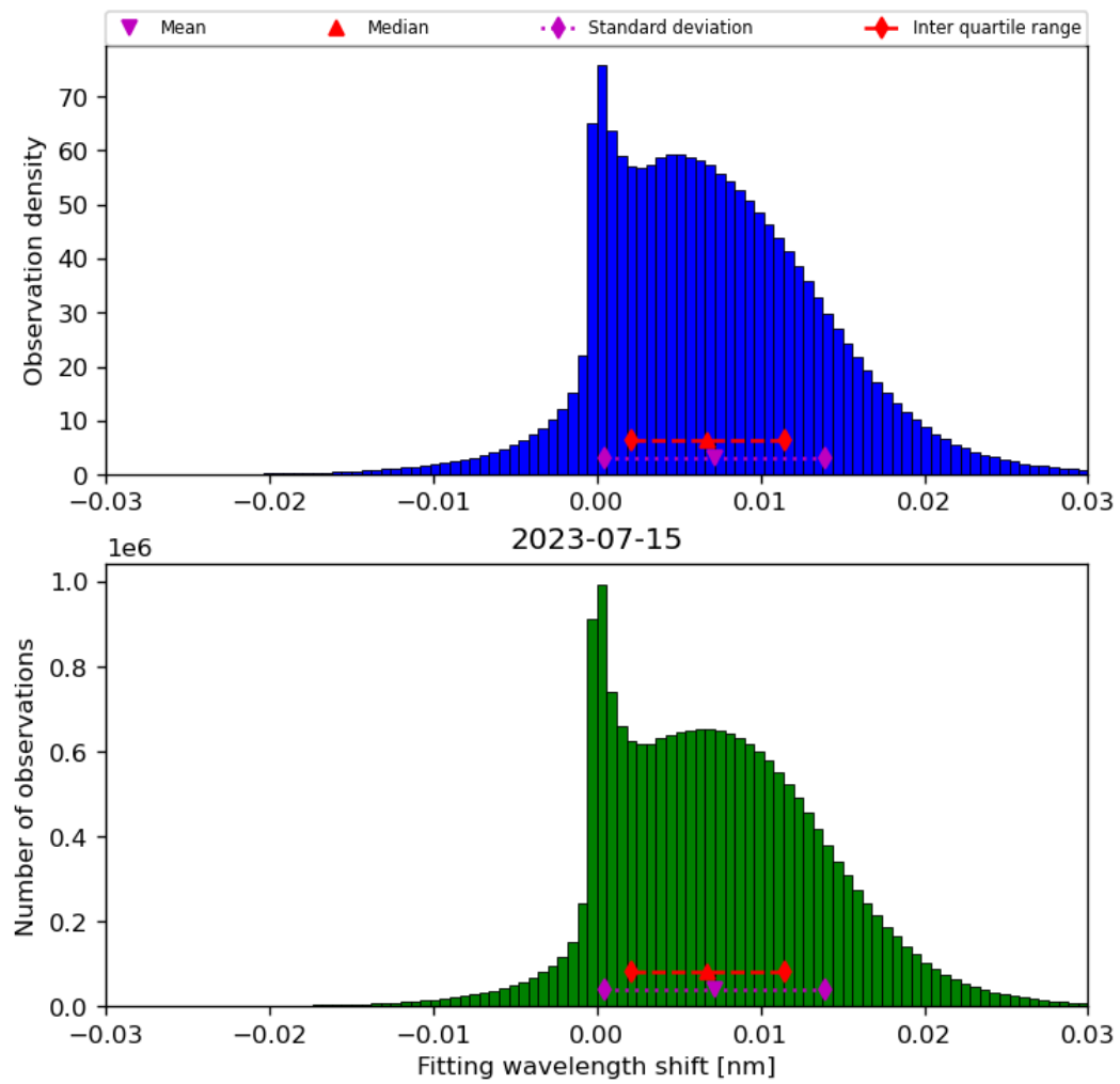
Figure 49: Histogram of “Fitting wavelength shift” for 2023-07-14 to 2023-07-16
