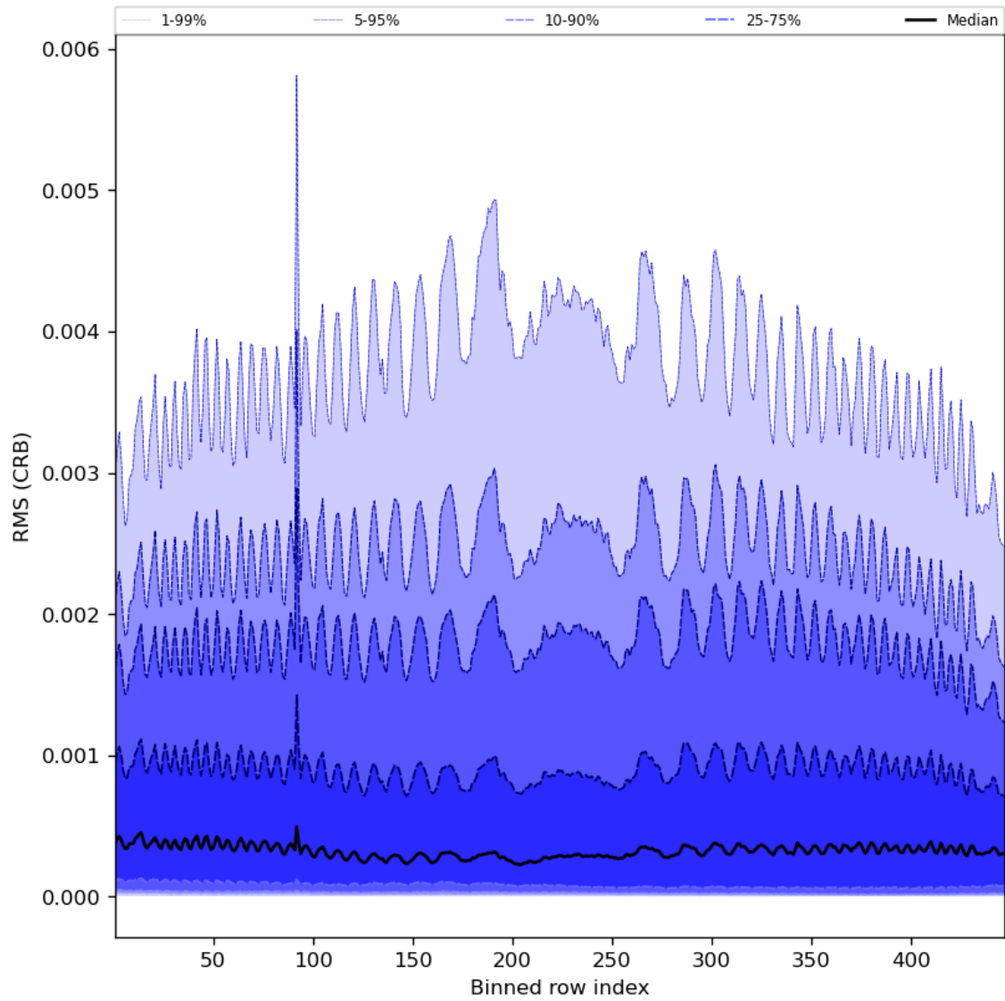
Figure 64: Along track statistics of “RMS (CRB)” for 2023-07-14 to 2023-07-16
