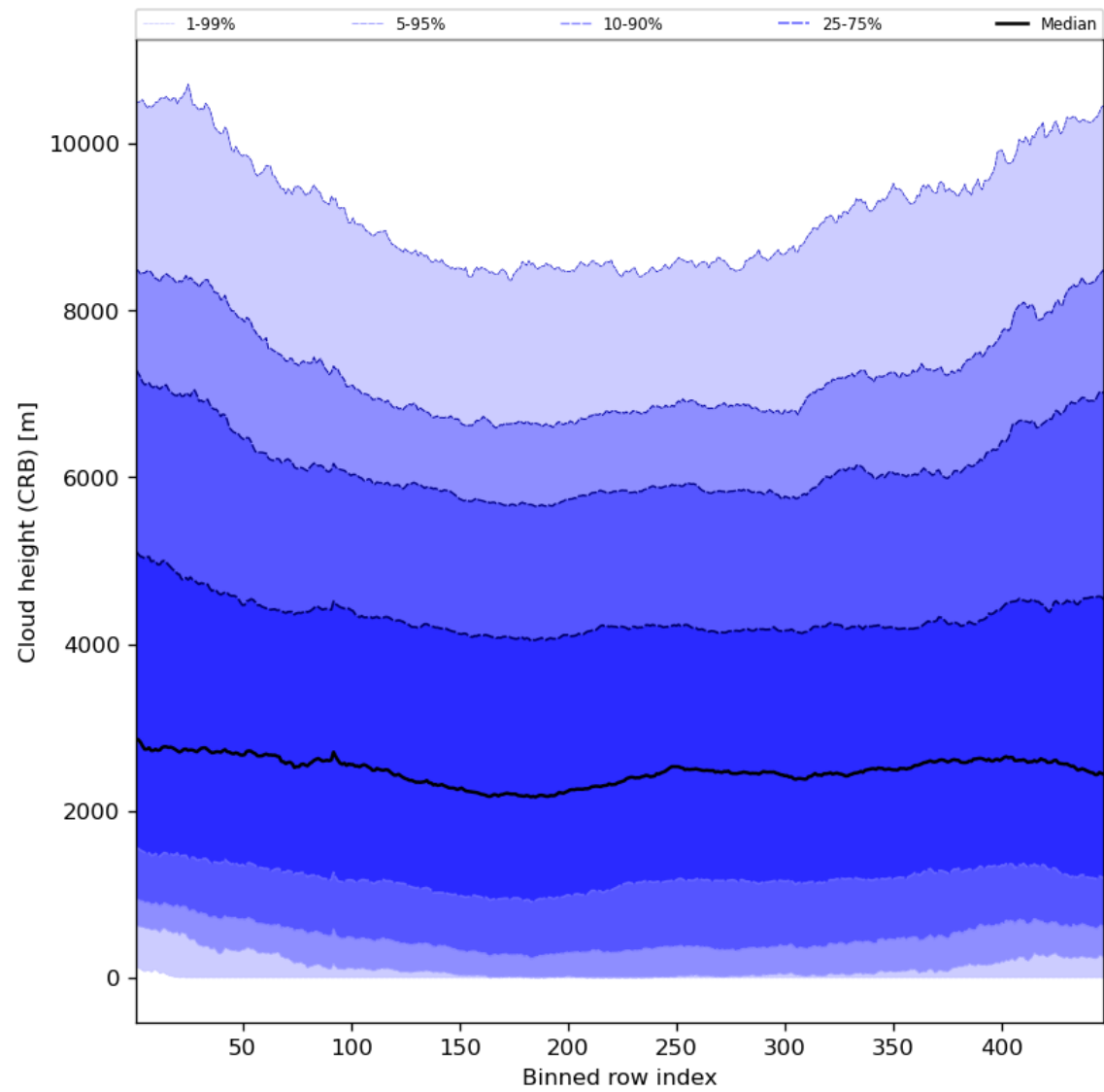
Figure 59: Along track statistics of “Cloud height (CRB)” for 2023-07-14 to 2023-07-16
