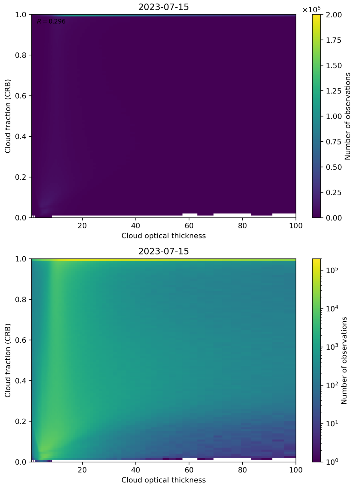
Figure 84: Scatter density plot of “Cloud optical thickness” against “Cloud fraction (CRB)” for 2023-07-14 to 2023-07-16.
