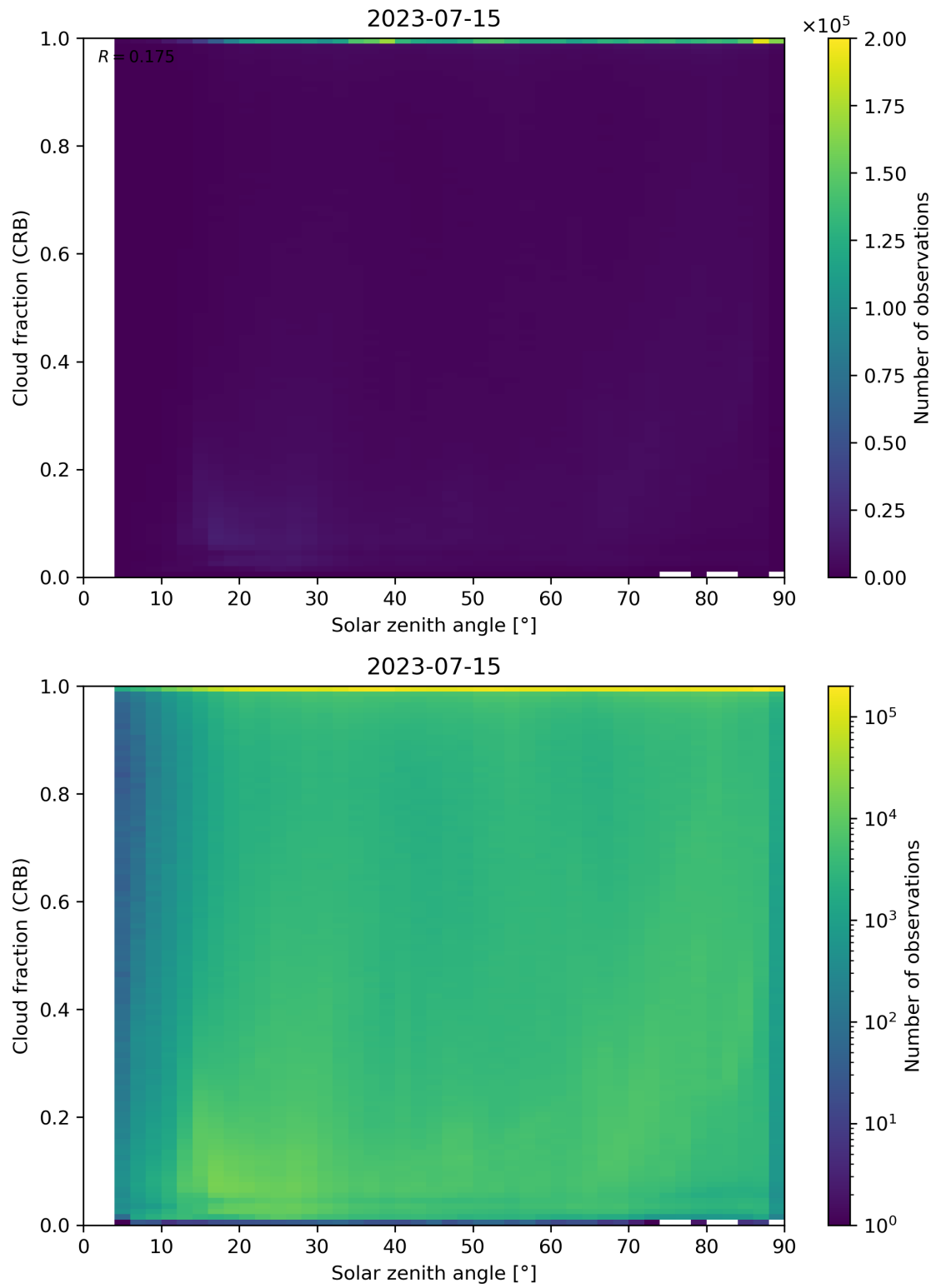
Figure 101: Scatter density plot of “Solar zenith angle” against “Cloud fraction (CRB)” for 2023-07-14 to 2023-07-16.
