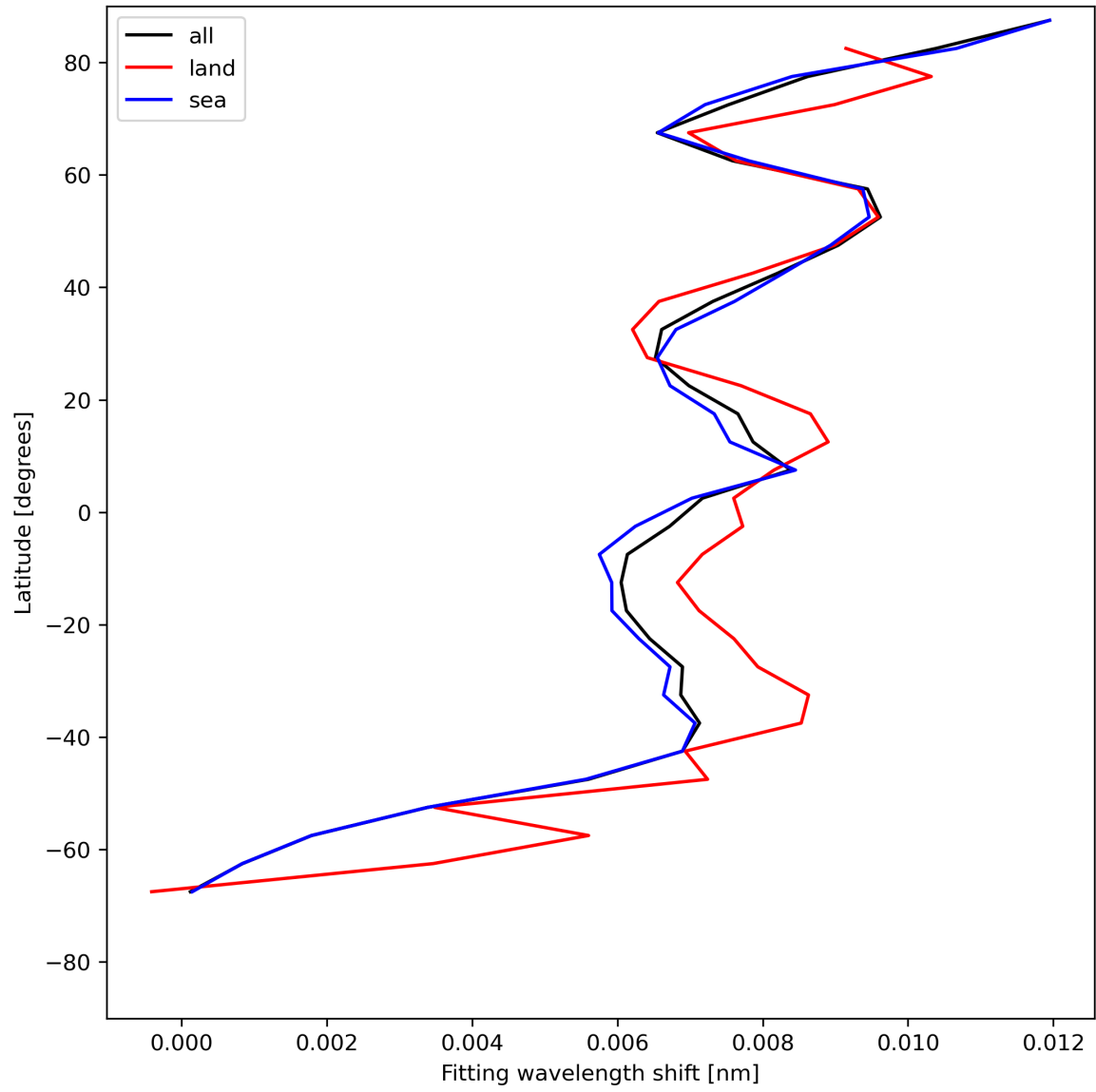
Figure 33: Zonal average of “Fitting wavelength shift” for 2023-07-14 to 2023-07-16.
