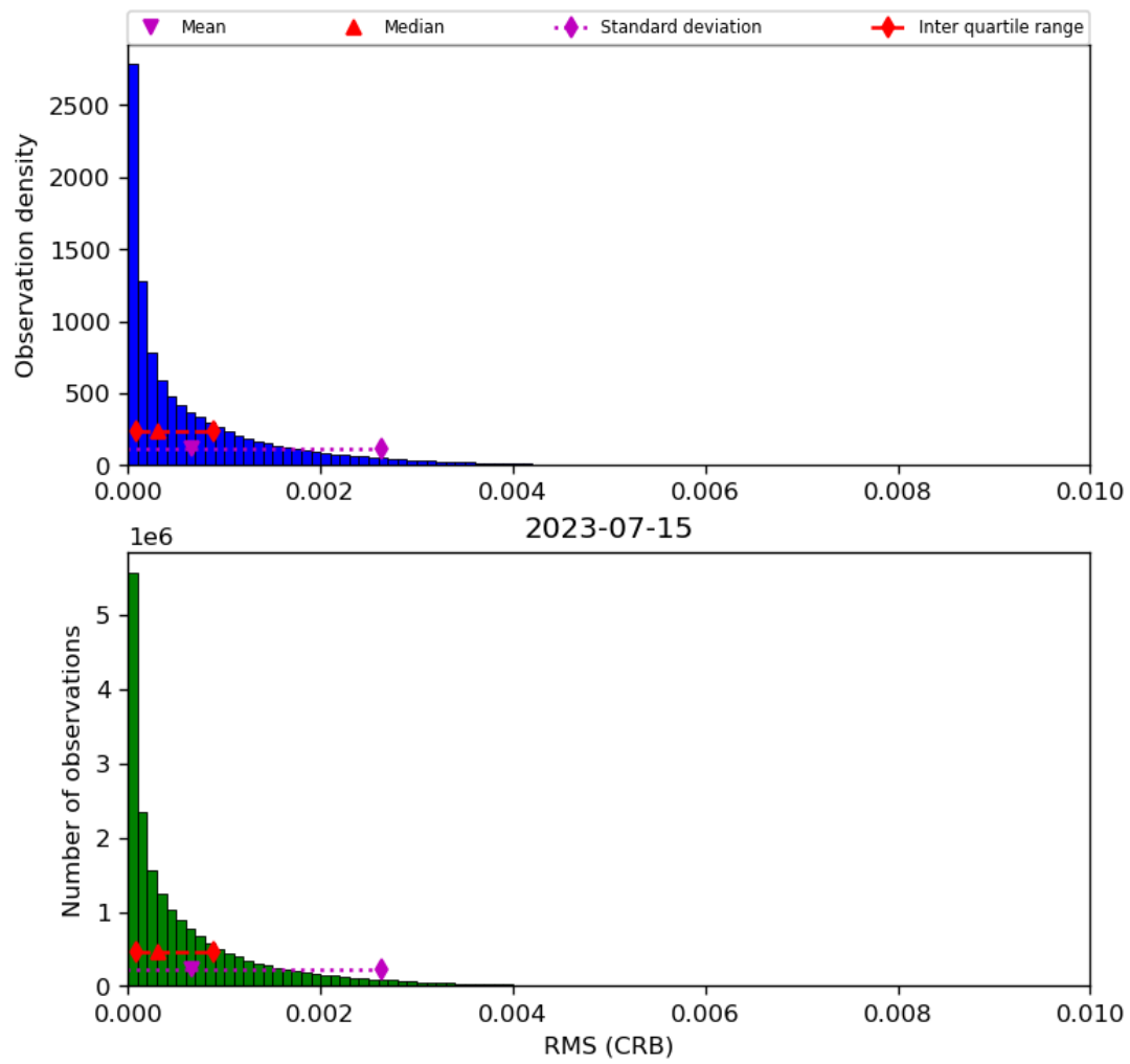
Figure 48: Histogram of “RMS (CRB)” for 2023-07-14 to 2023-07-16
