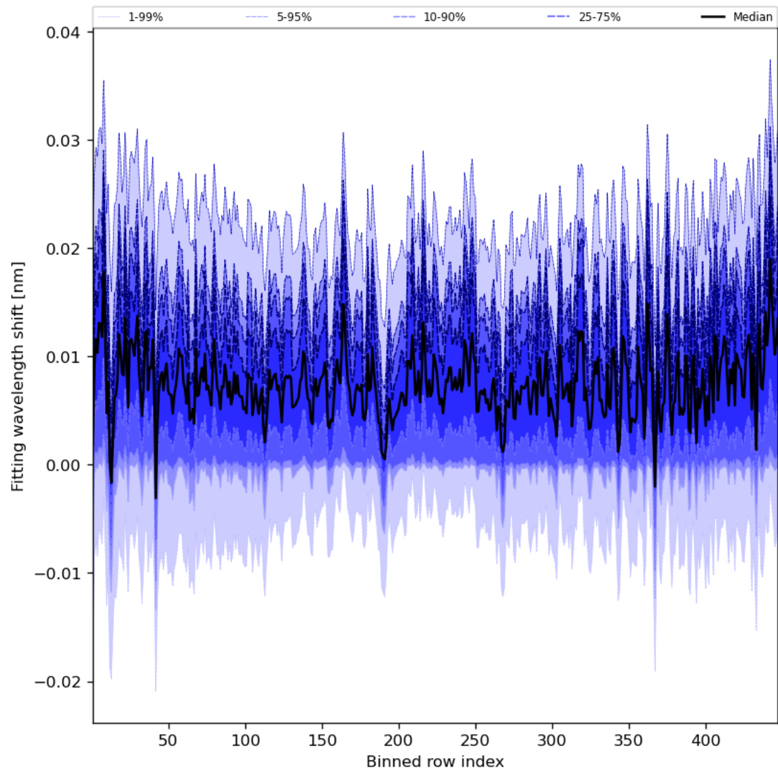
Figure 65: Along track statistics of “Fitting wavelength shift” for 2023-07-14 to 2023-07-16
