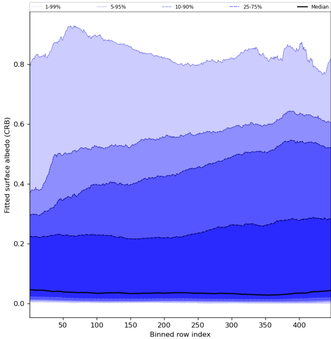
Figure 62: Along track statistics of “Fitted surface albedo (CRB)” for 2023-07-14 to 2023-07-16
