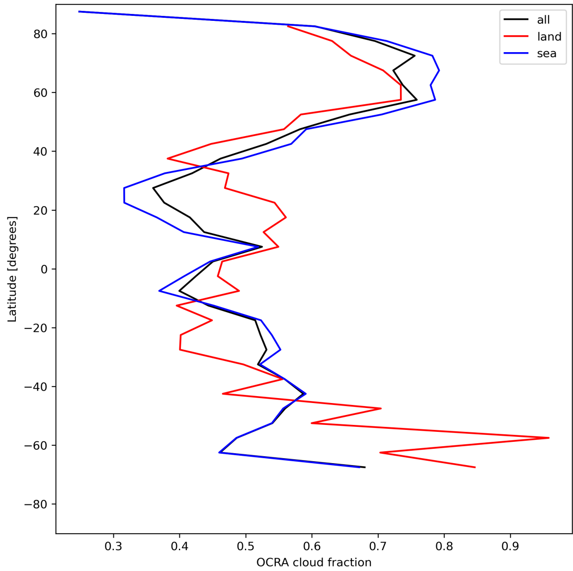
Figure 34: Zonal average of “OCRA cloud fraction” for 2023-07-14 to 2023-07-16.
