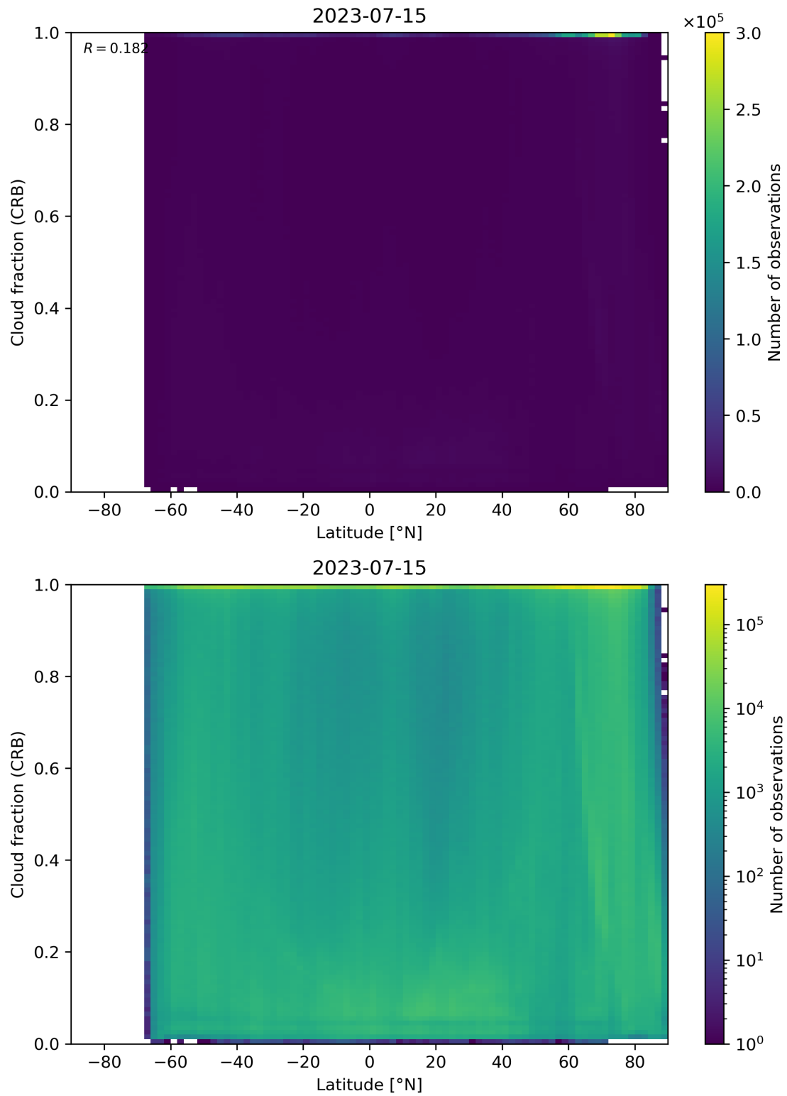
Figure 94: Scatter density plot of “Latitude” against “Cloud fraction (CRB)” for 2023-07-14 to 2023-07-16.
