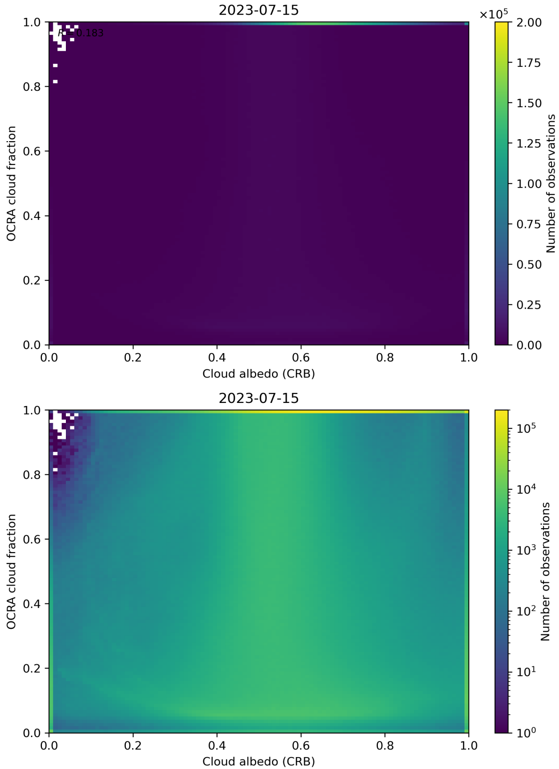
Figure 70: Scatter density plot of “Cloud albedo (CRB)” against “OCRA cloud fraction” for 2023-07-14 to 2023-07-16.
