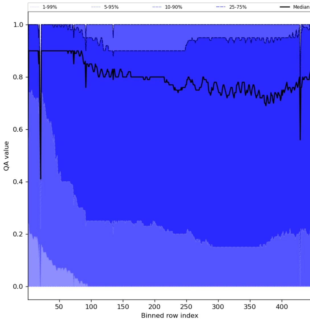
Figure 54: Along track statistics of “QA value” for 2023-07-14 to 2023-07-16
