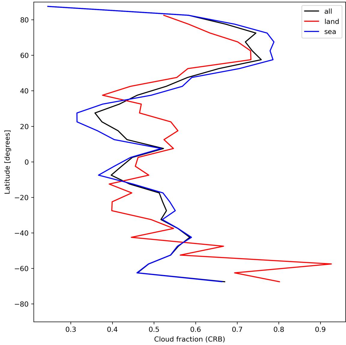
Figure 26: Zonal average of “Cloud fraction (CRB)” for 2023-07-14 to 2023-07-16.
