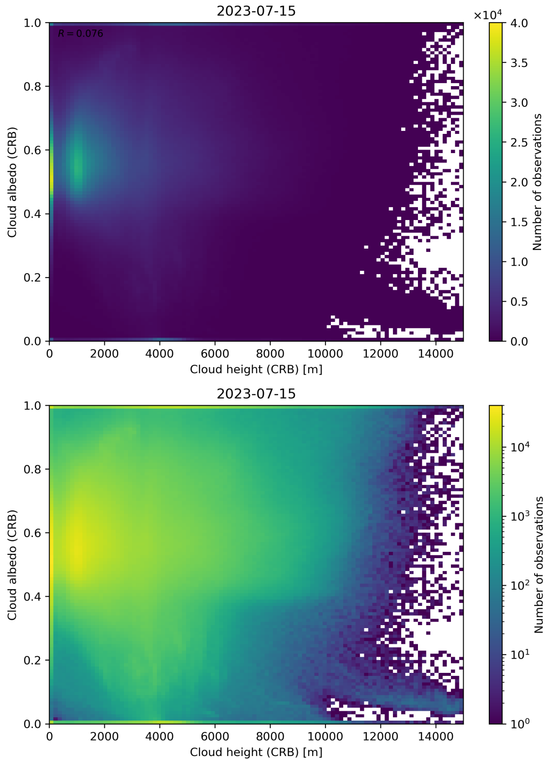
Figure 80: Scatter density plot of “Cloud height (CRB)” against “Cloud albedo (CRB)” for 2023-07-14 to 2023-07-16.
