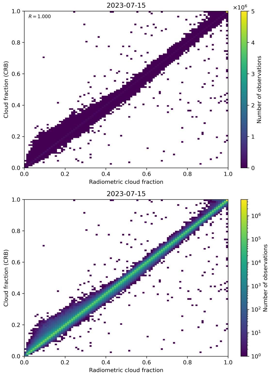
Figure 73: Scatter density plot of “Radiometric cloud fraction” against “Cloud fraction (CRB)” for 2023-07-14 to 2023-07-16.
