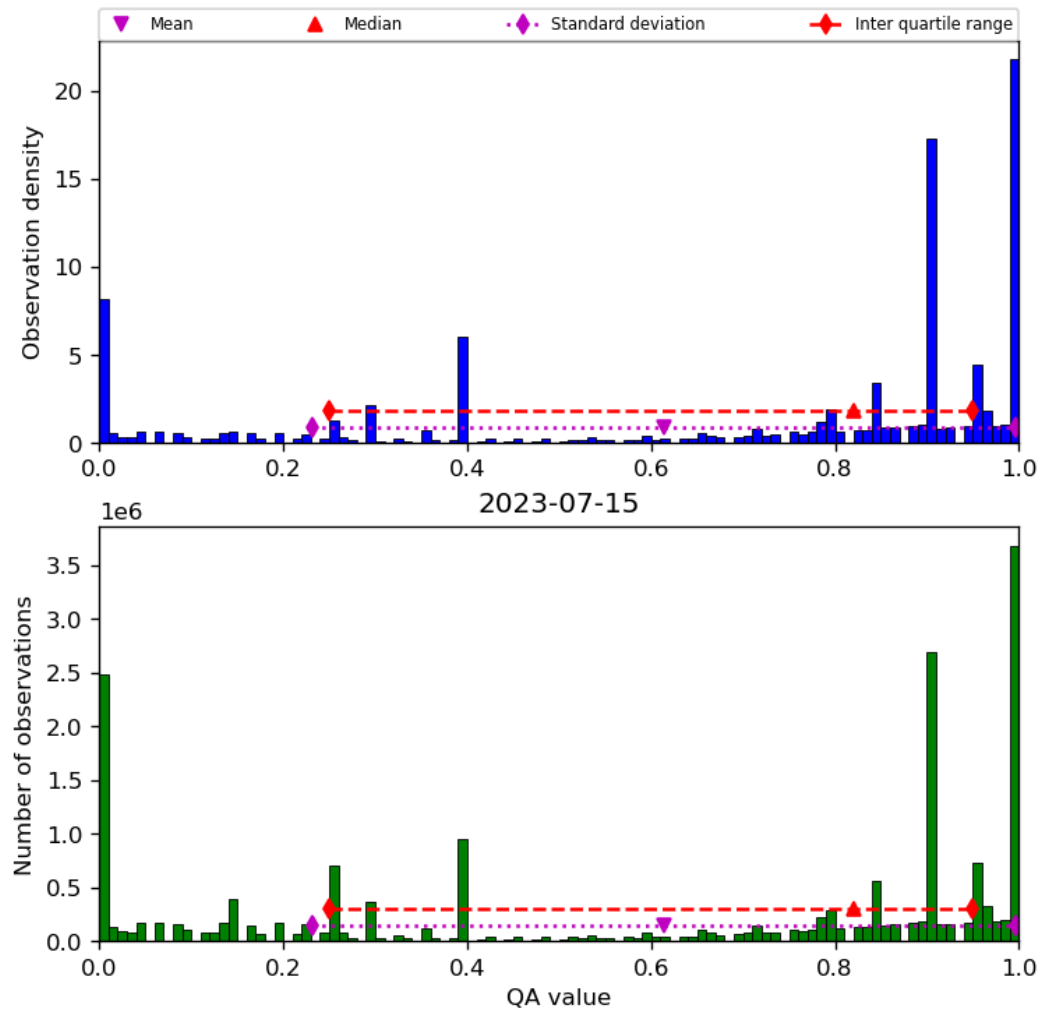
Figure 38: Histogram of “QA value” for 2023-07-14 to 2023-07-16
