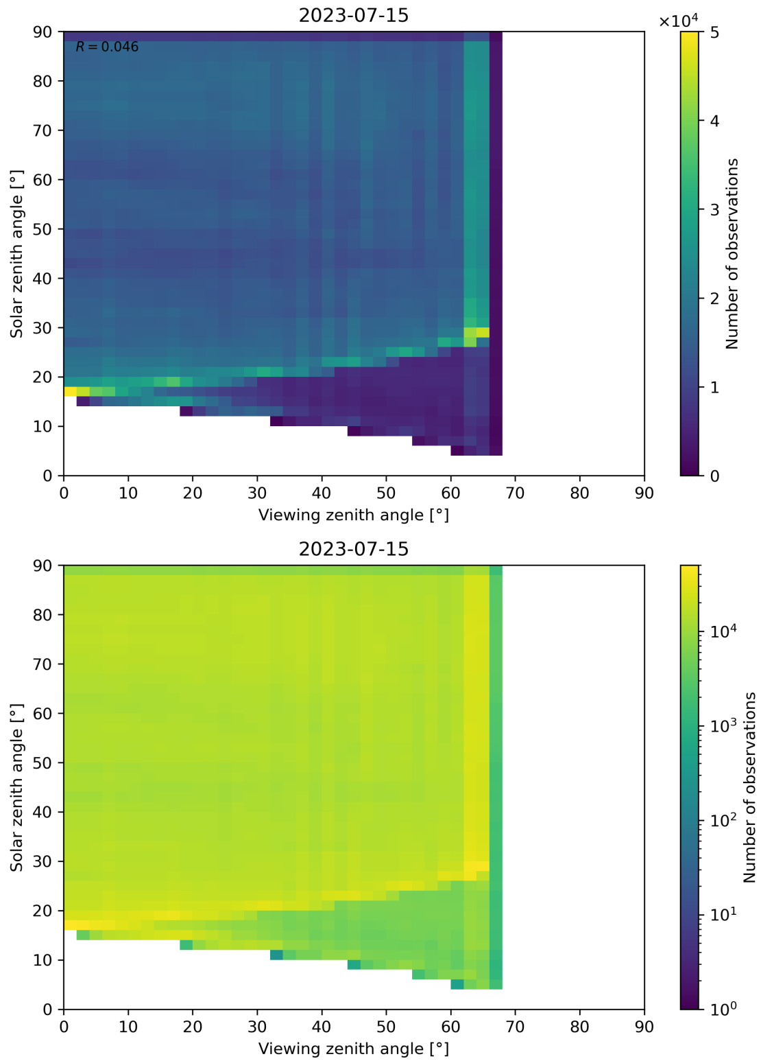
Figure 114: Scatter density plot of “Viewing zenith angle” against “Solar zenith angle” for 2023-07-14 to 2023-07-16.
