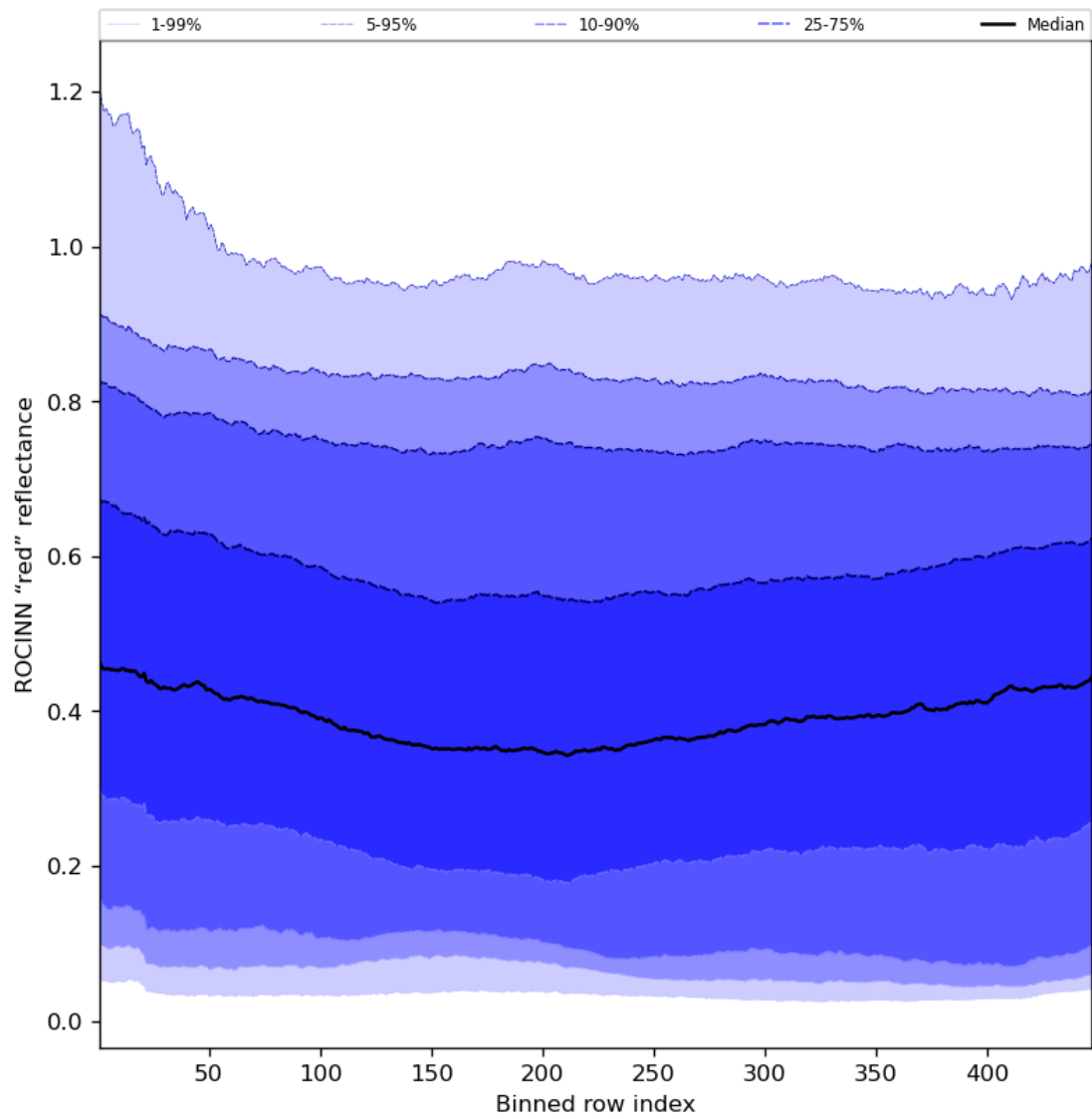
Figure 69: Along track statistics of “ROCINN “red” reflectance” for 2023-07-14 to 2023-07-16
