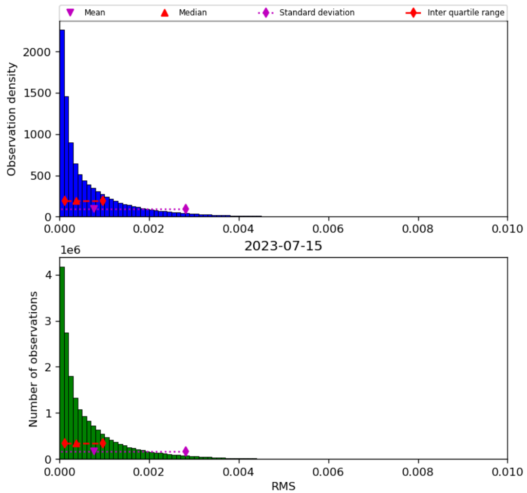
Figure 47: Histogram of “RMS” for 2023-07-14 to 2023-07-16
