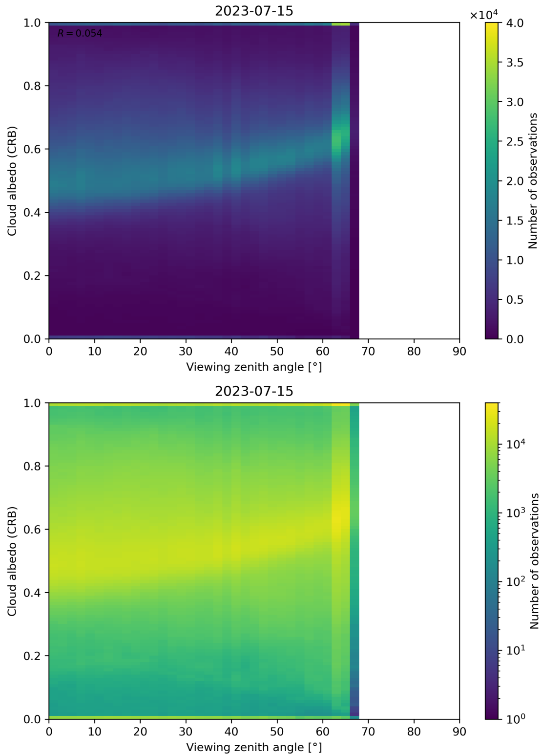
Figure 106: Scatter density plot of “Viewing zenith angle” against “Cloud albedo (CRB)” for 2023-07-14 to 2023-07-16.
