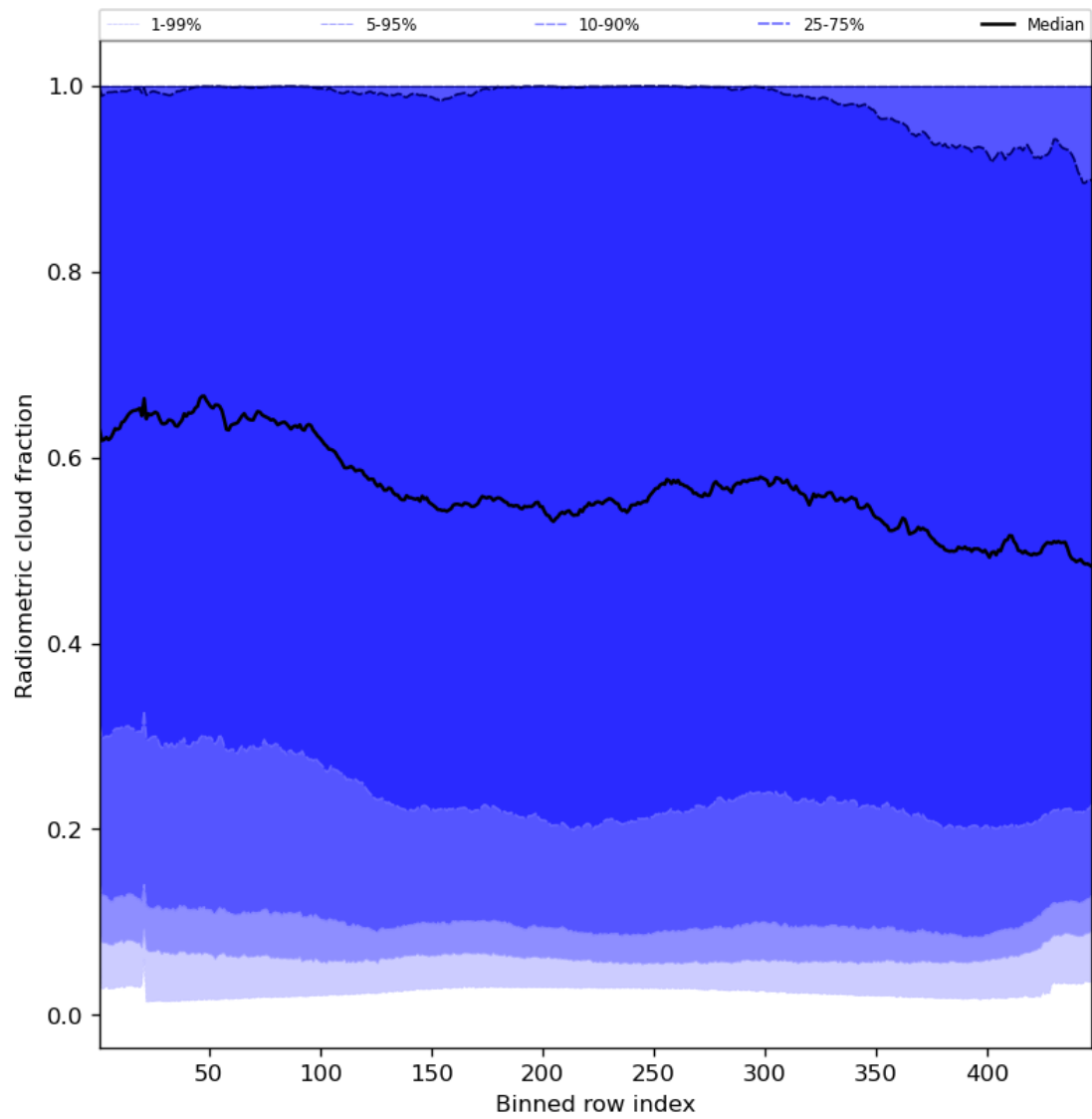
Figure 55: Along track statistics of “Radiometric cloud fraction” for 2023-07-14 to 2023-07-16
