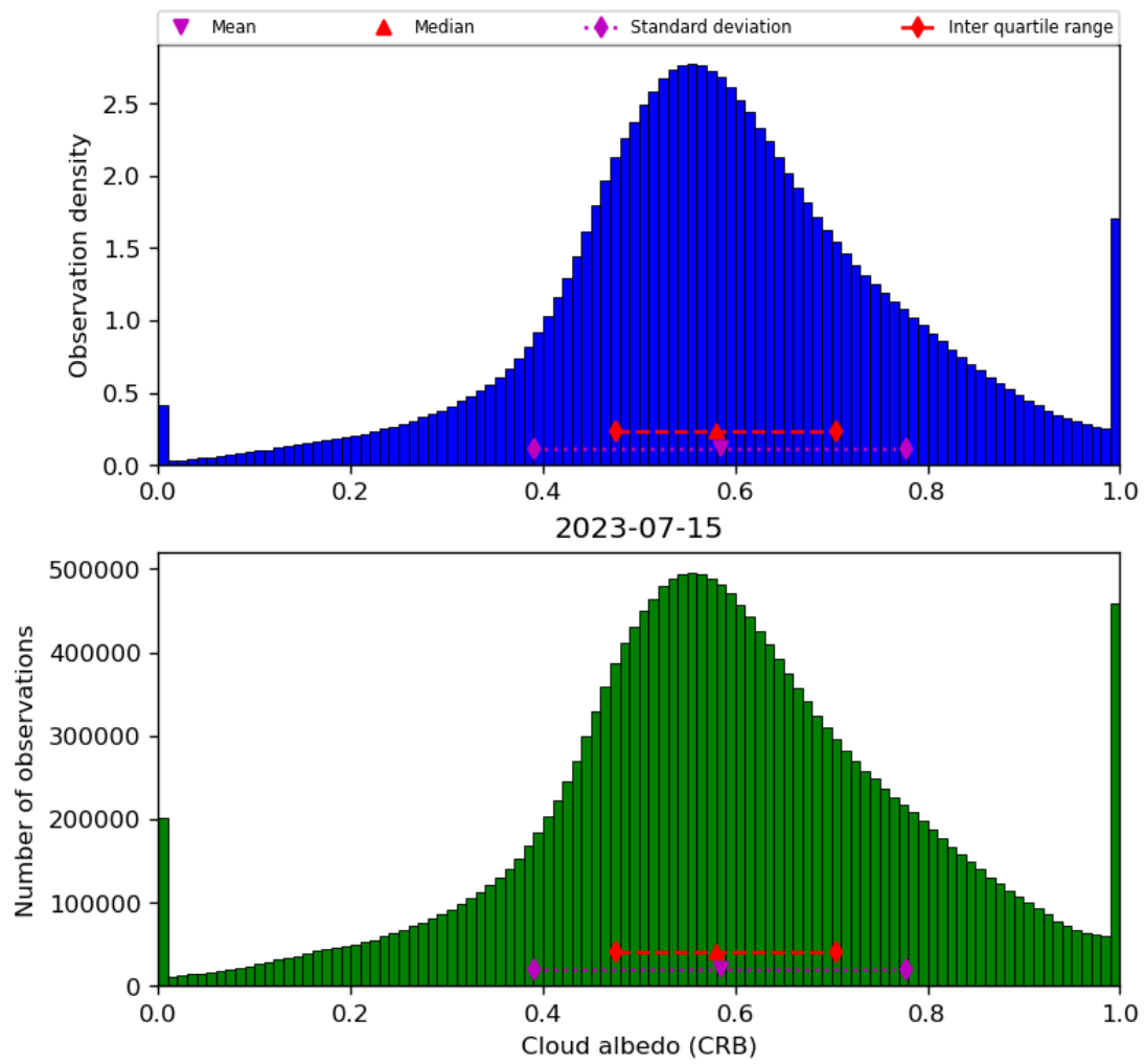
Figure 44: Histogram of “Cloud albedo (CRB)” for 2023-07-14 to 2023-07-16
