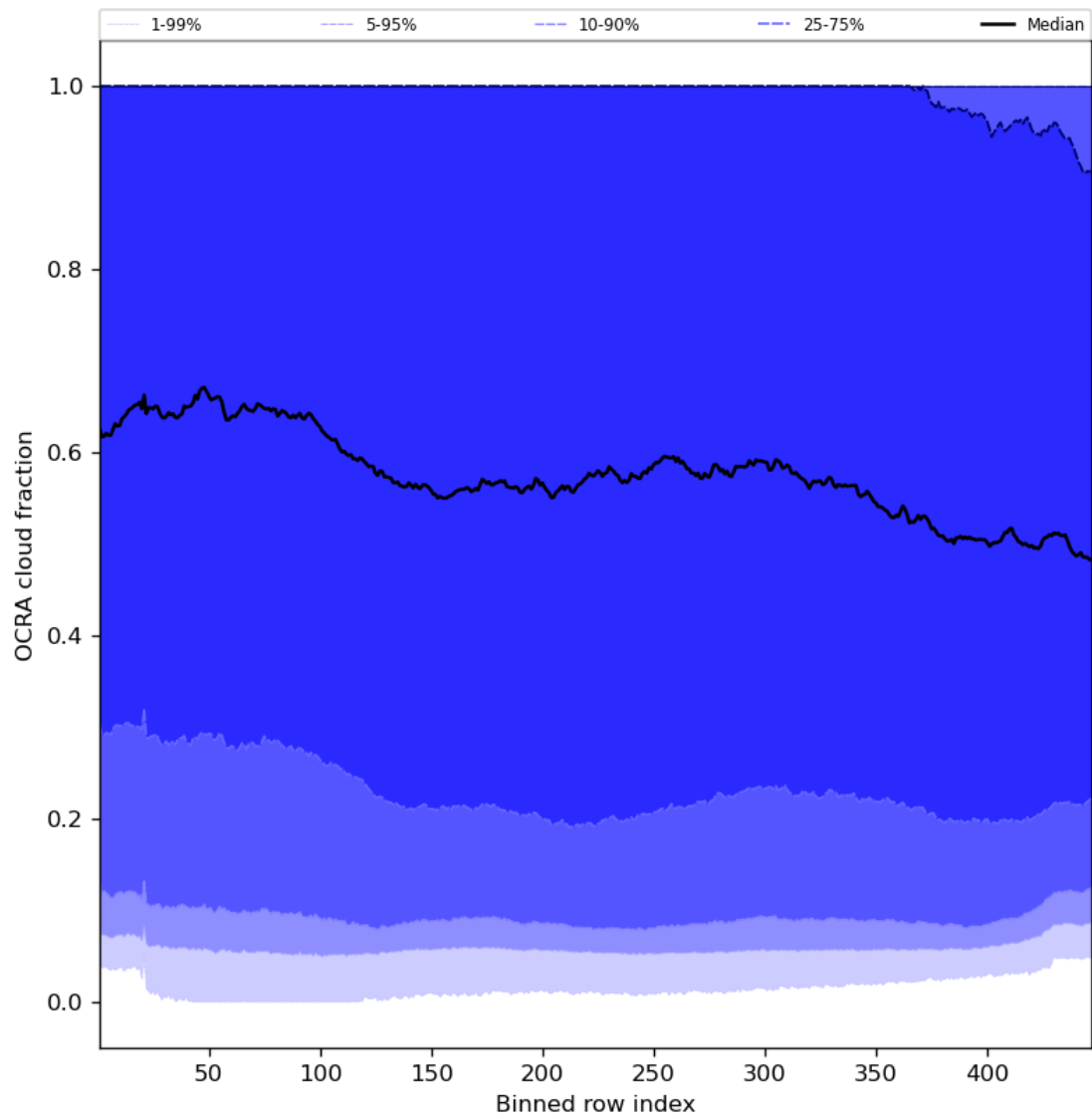
Figure 66: Along track statistics of “OCRA cloud fraction” for 2023-07-14 to 2023-07-16
