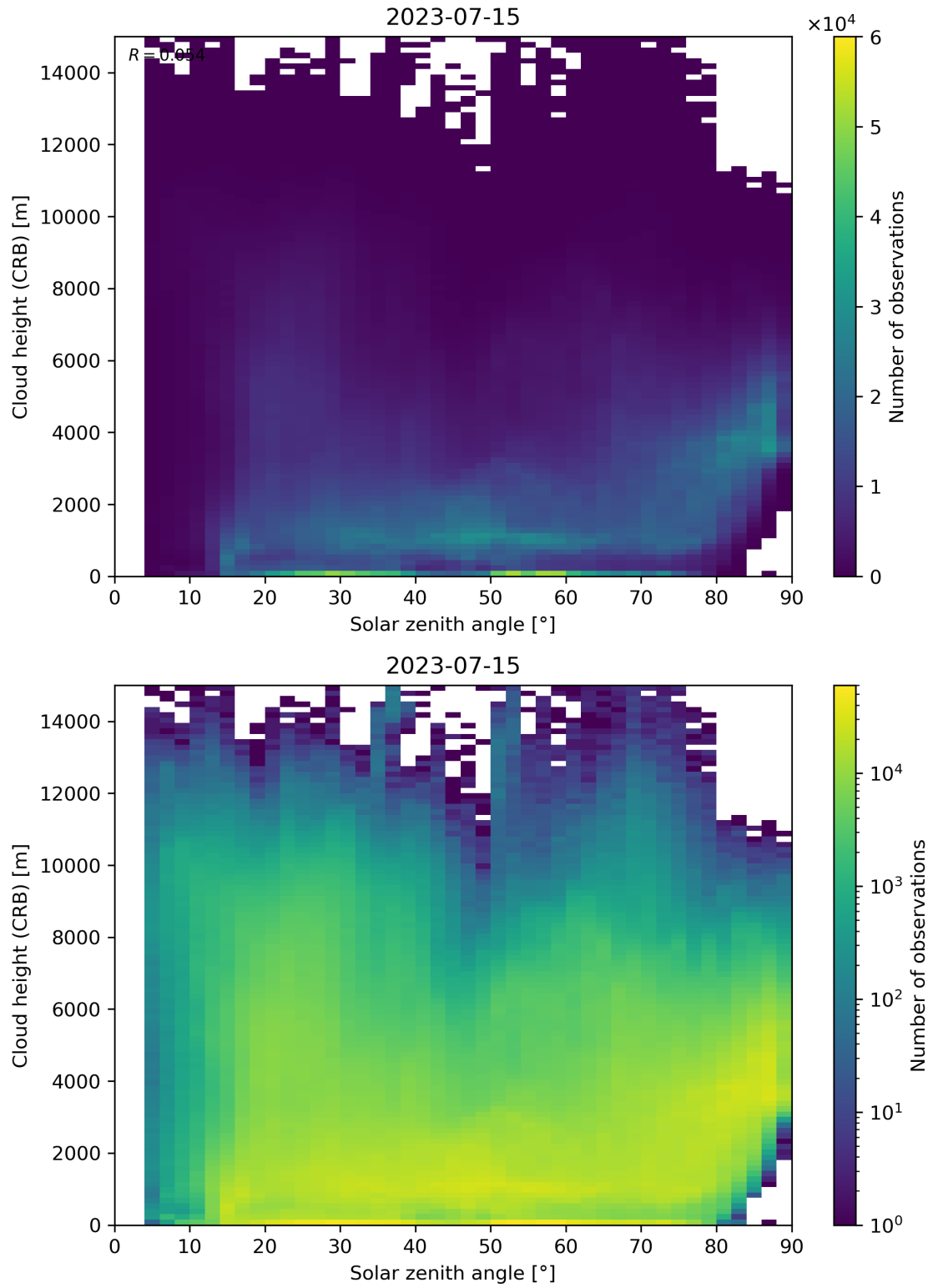
Figure 102: Scatter density plot of “Solar zenith angle” against “Cloud height (CRB)” for 2023-07-14 to 2023-07-16.
