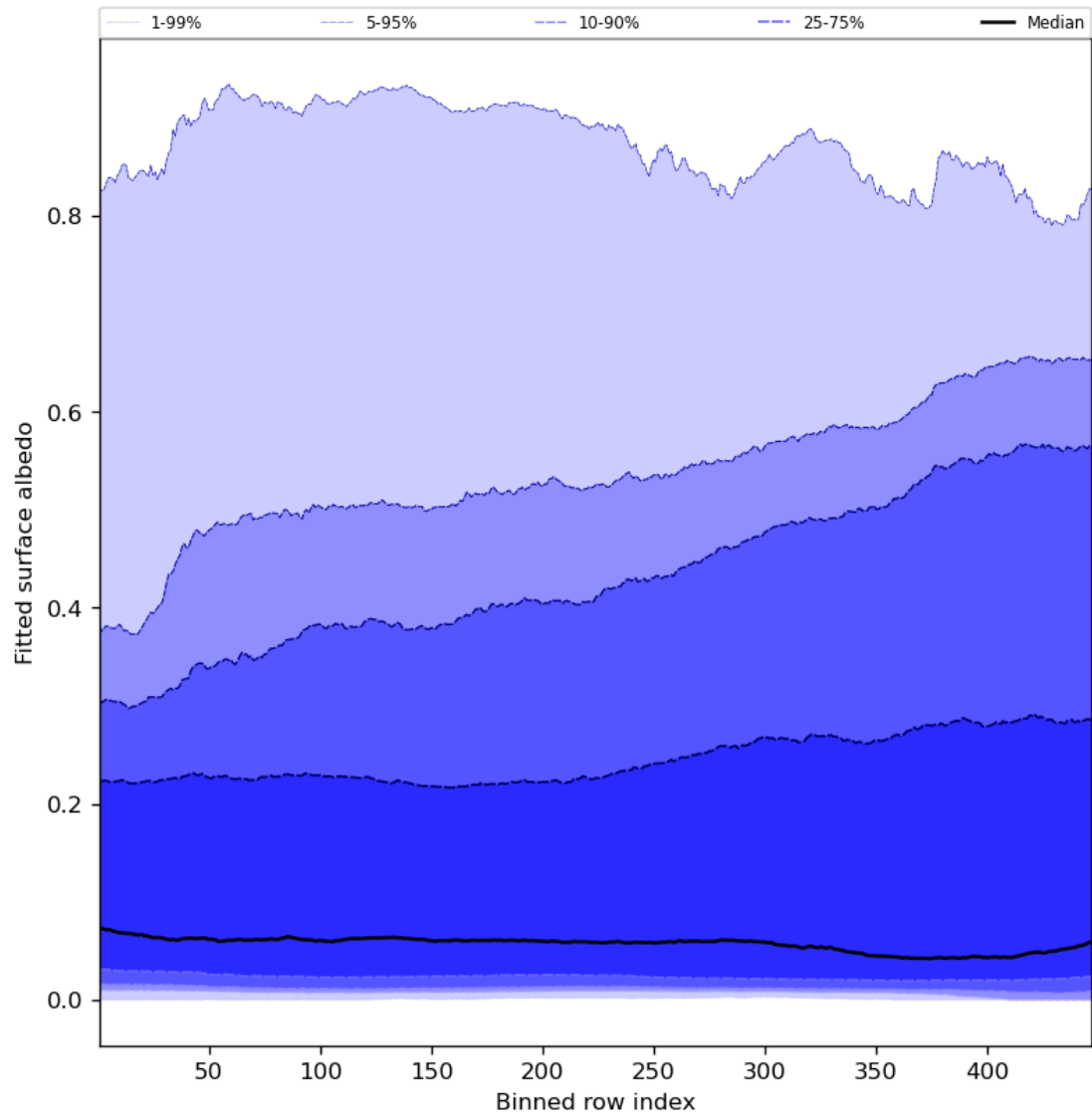
Figure 61: Along track statistics of “Fitted surface albedo” for 2023-07-14 to 2023-07-16
