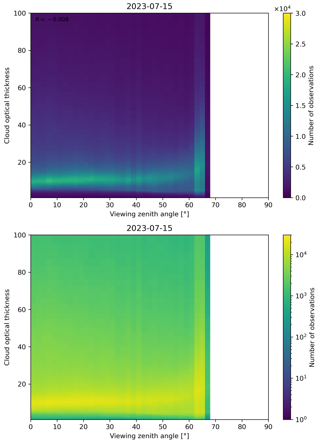
Figure 111: Scatter density plot of “Viewing zenith angle” against “Cloud optical thickness” for 2023-07-14 to 2023-07-16.
