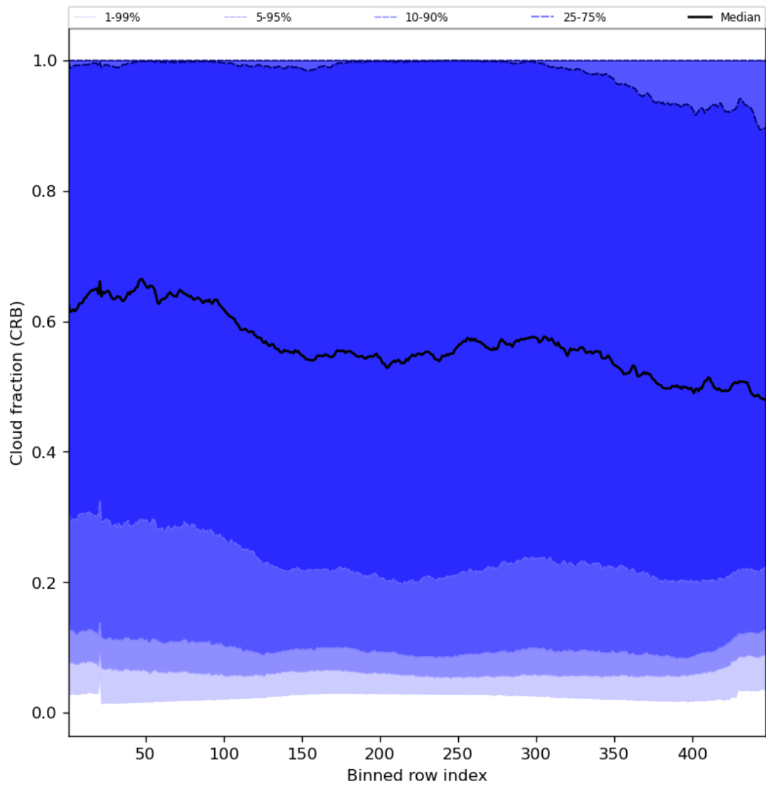
Figure 58: Along track statistics of “Cloud fraction (CRB)” for 2023-07-14 to 2023-07-16
