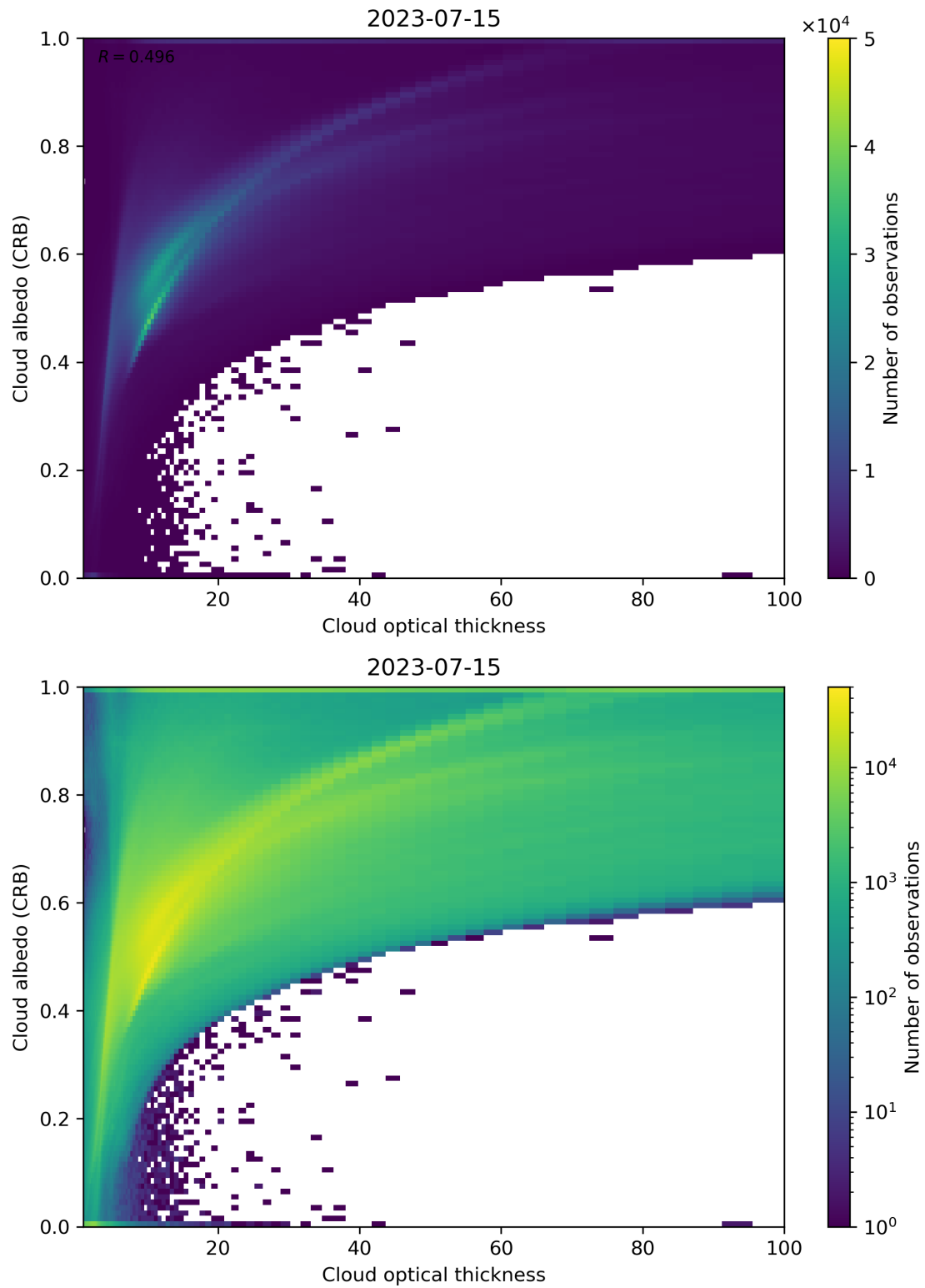
Figure 82: Scatter density plot of “Cloud optical thickness” against “Cloud albedo (CRB)” for 2023-07-14 to 2023-07-16.
