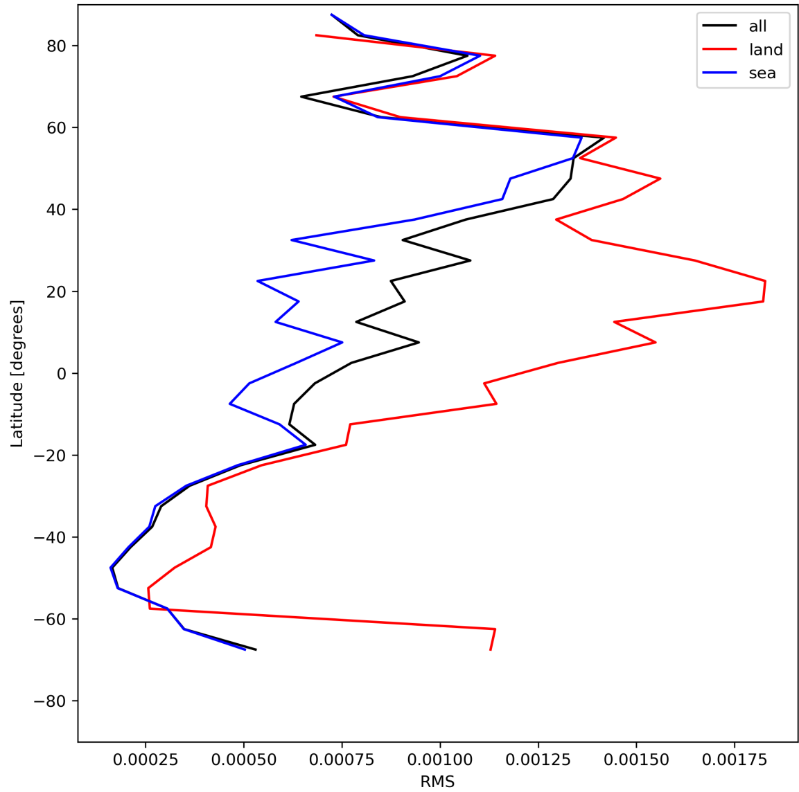
Figure 31: Zonal average of “RMS” for 2023-07-14 to 2023-07-16.
