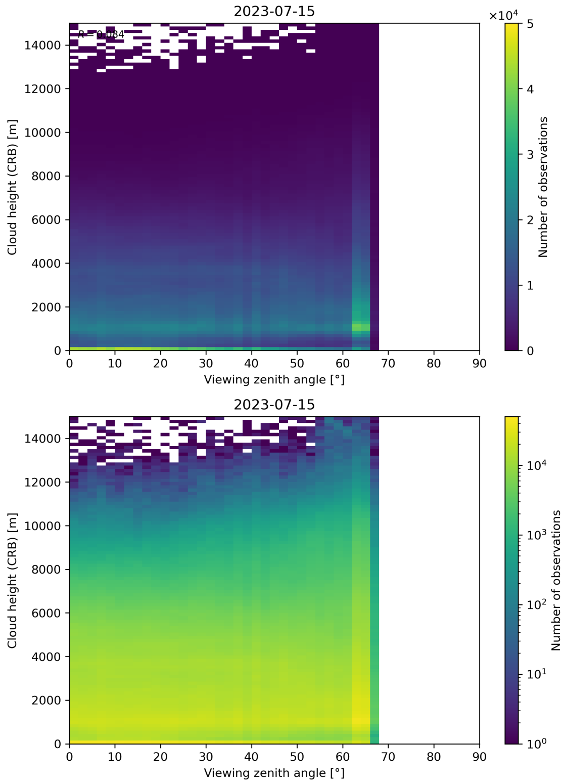
Figure 110: Scatter density plot of “Viewing zenith angle” against “Cloud height (CRB)” for 2023-07-14 to 2023-07-16.
