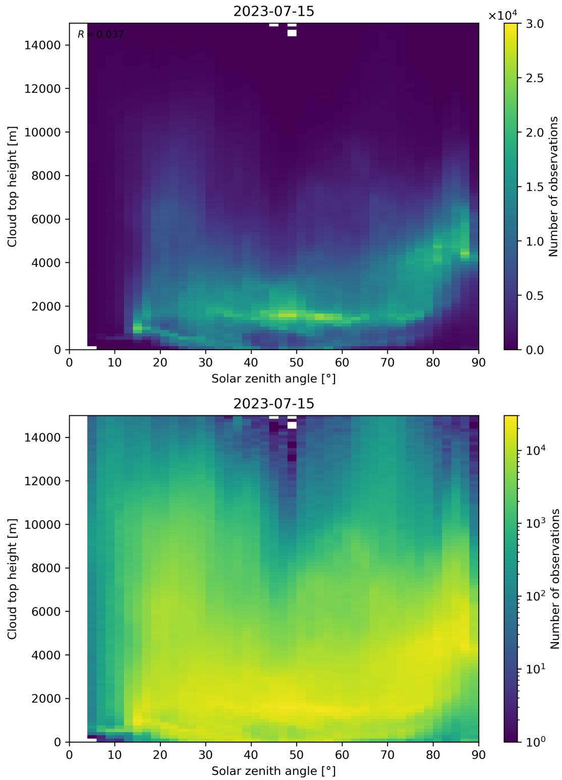
Figure 104: Scatter density plot of “Solar zenith angle” against “Cloud top height” for 2023-07-14 to 2023-07-16.
