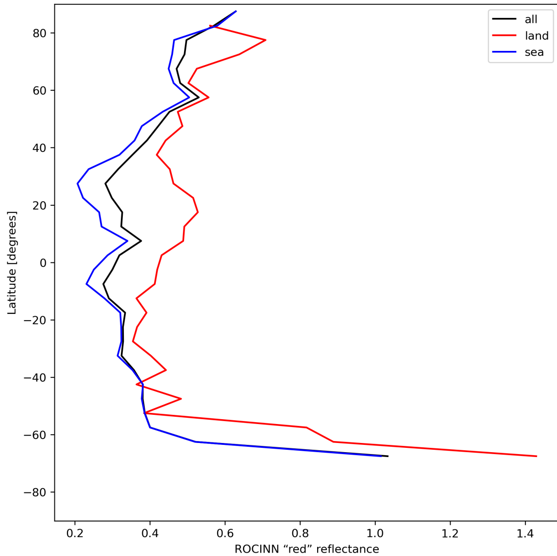
Figure 37: Zonal average of “ROCINN “red” reflectance” for 2023-07-14 to 2023-07-16.
