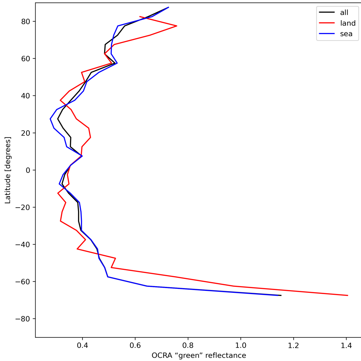
Figure 36: Zonal average of “OCRA “green” reflectance” for 2023-07-14 to 2023-07-16.
