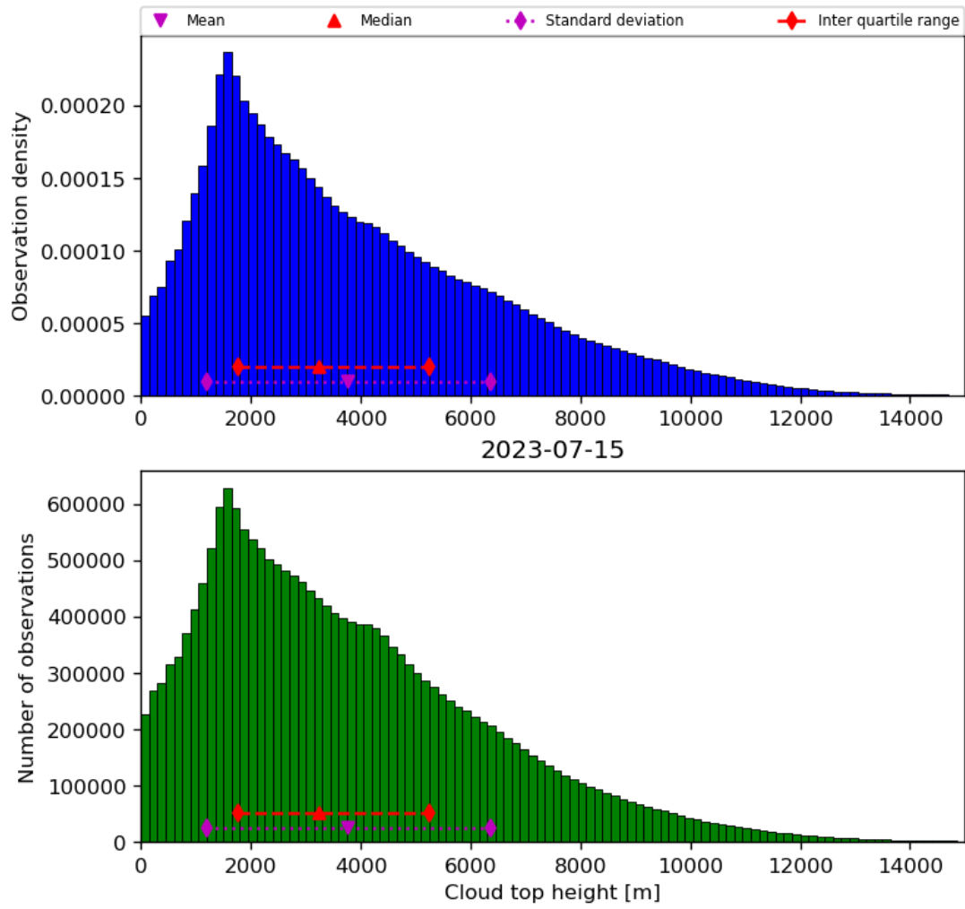
Figure 40: Histogram of “Cloud top height” for 2023-07-14 to 2023-07-16
