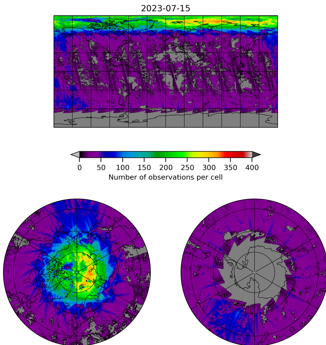
Figure 21: Map of the number of observations for 2023-07-14 to 2023-07-16
