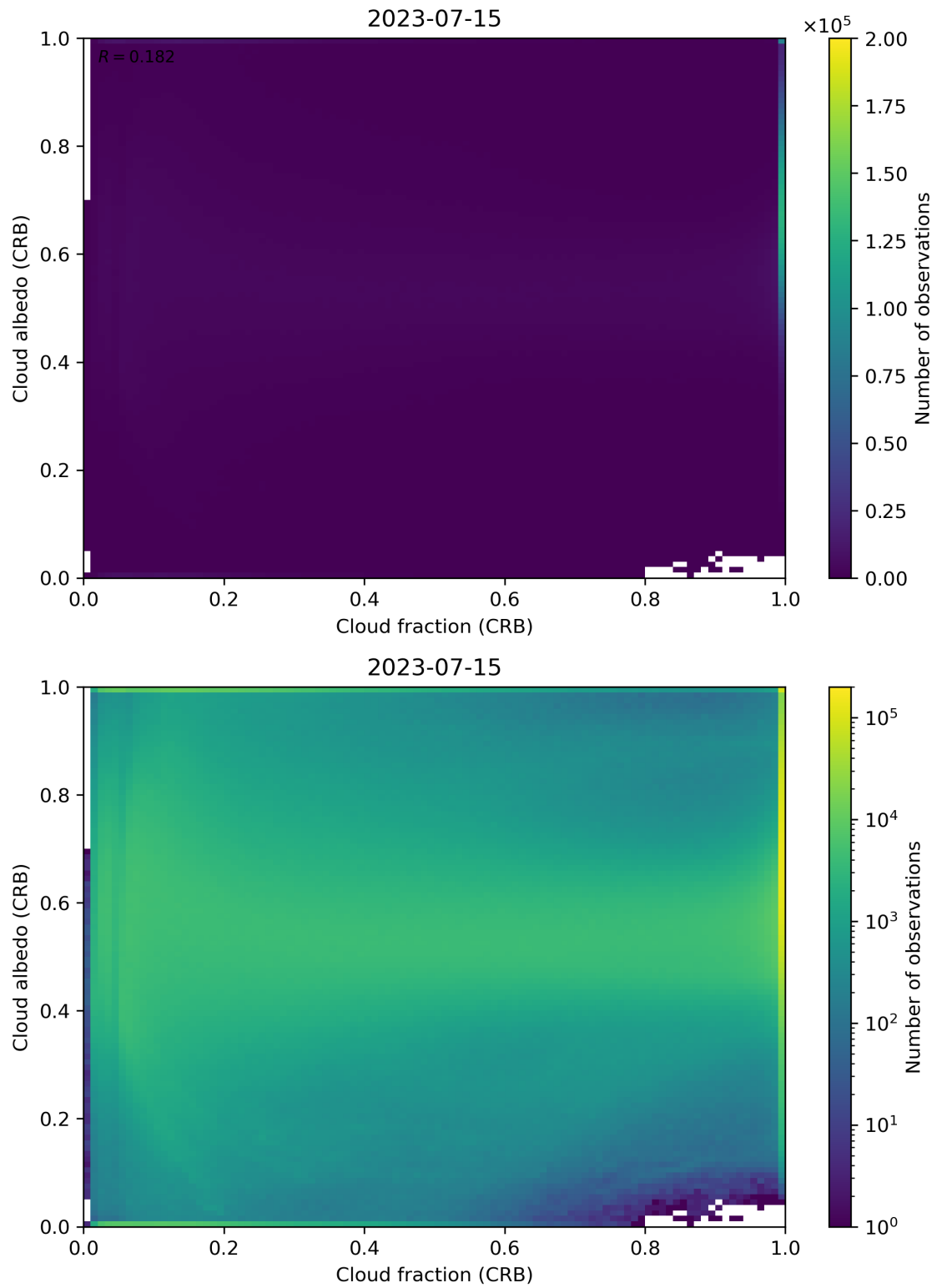
Figure 77: Scatter density plot of “Cloud fraction (CRB)” against “Cloud albedo (CRB)” for 2023-07-14 to 2023-07-16.
