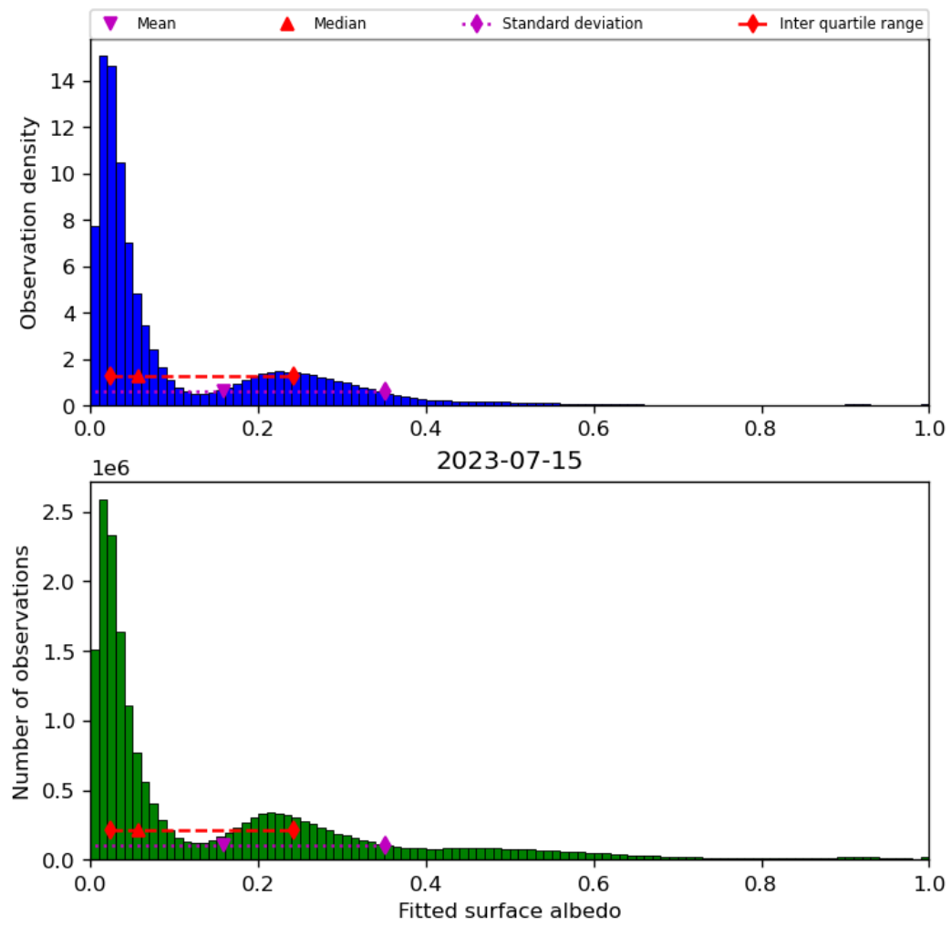
Figure 45: Histogram of “Fitted surface albedo” for 2023-07-14 to 2023-07-16
