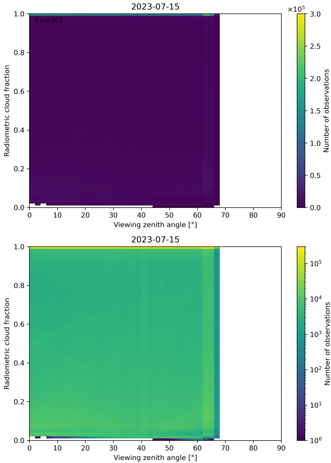
Figure 107: Scatter density plot of “Viewing zenith angle” against “Radiometric cloud fraction” for 2023-07-14 to 2023-07-16.
