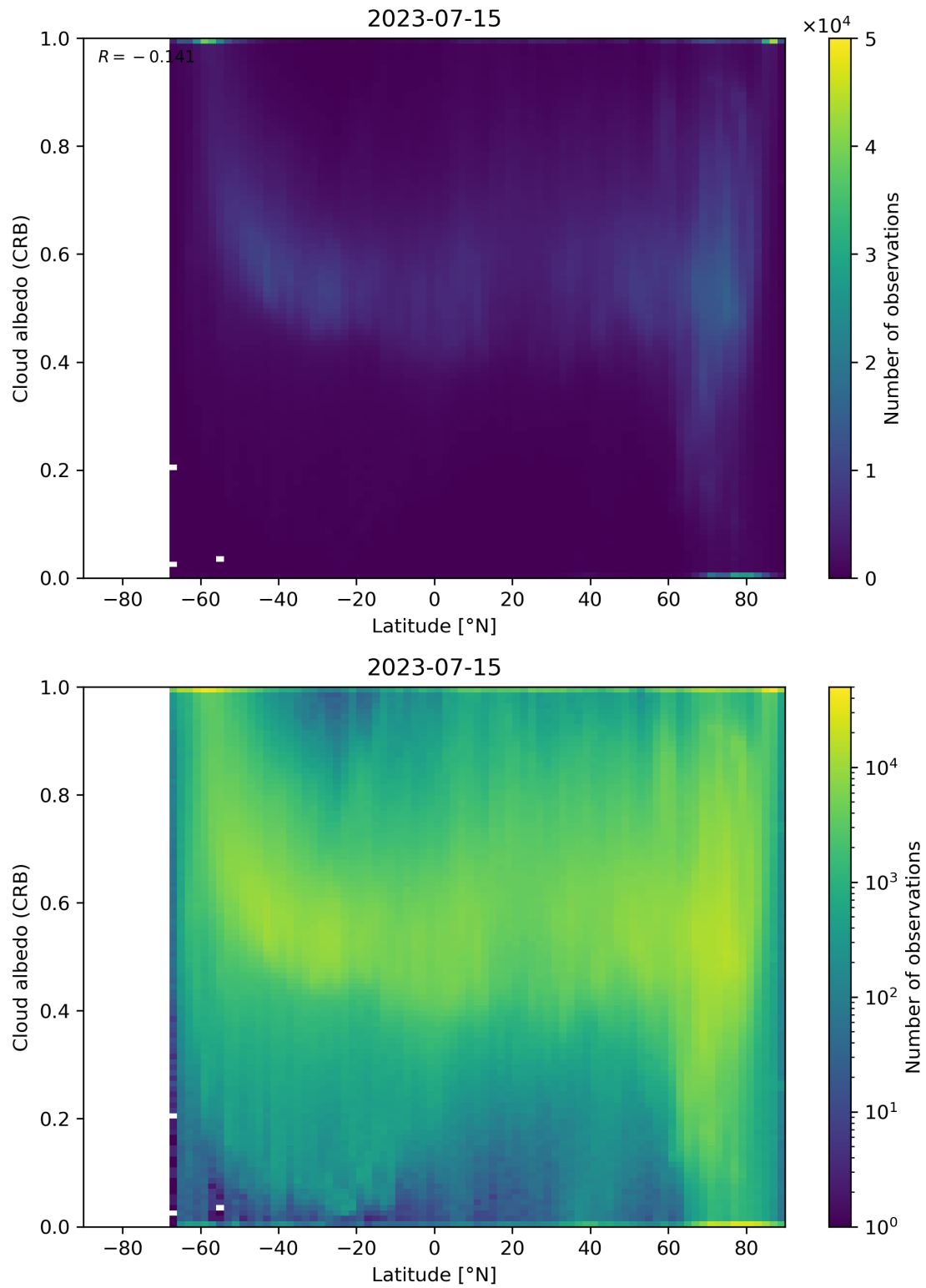
Figure 91: Scatter density plot of “Latitude” against “Cloud albedo (CRB)” for 2023-07-14 to 2023-07-16.
