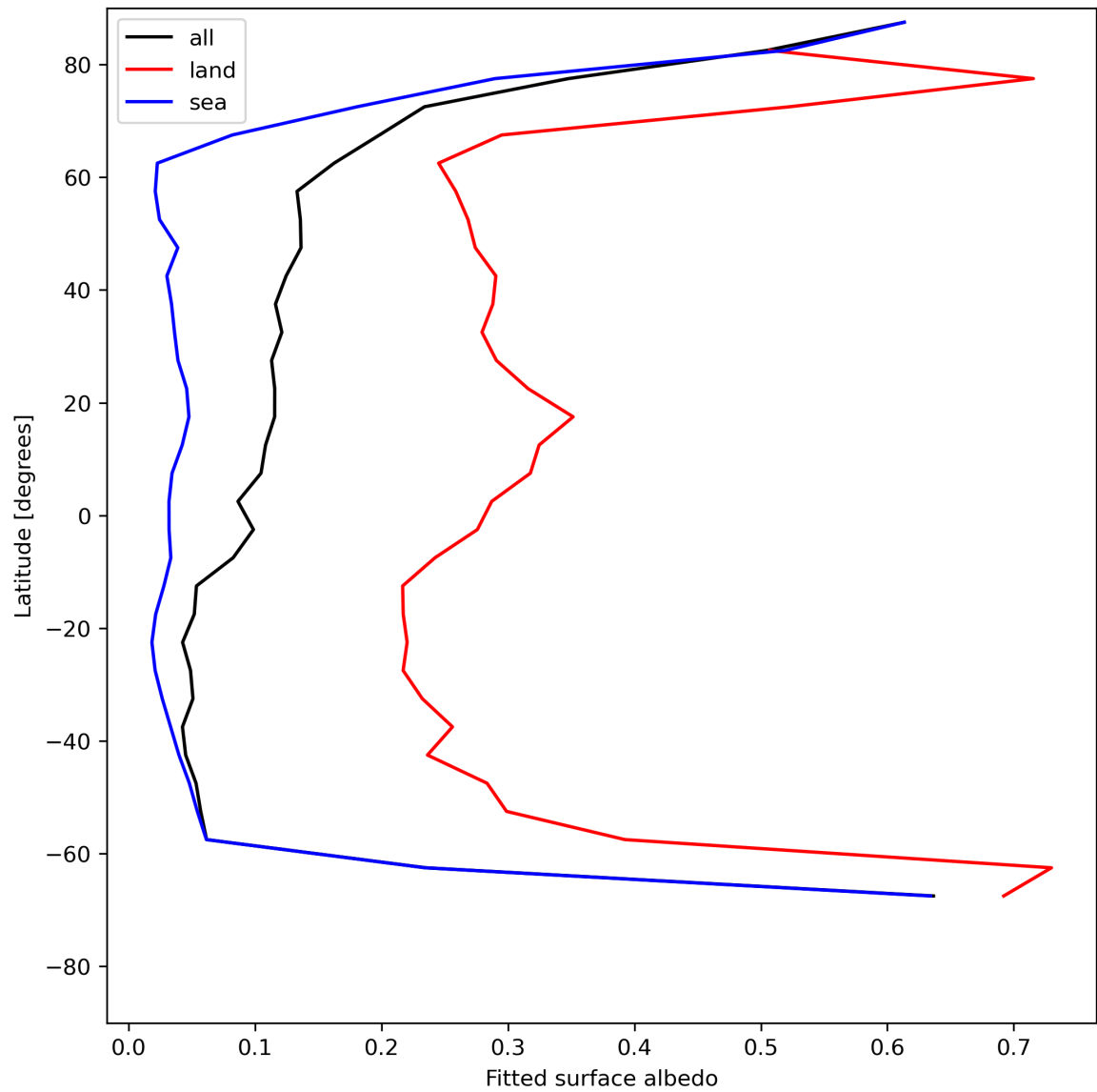
Figure 29: Zonal average of “Fitted surface albedo” for 2023-07-14 to 2023-07-16.
