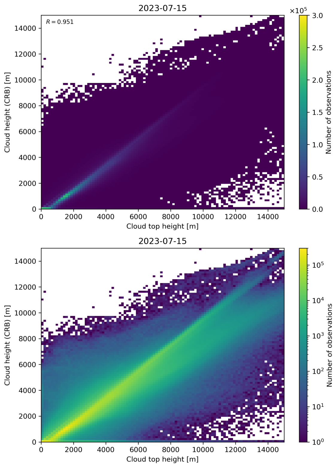
Figure 89: Scatter density plot of “Cloud top height” against “Cloud height (CRB)” for 2023-07-14 to 2023-07-16.
