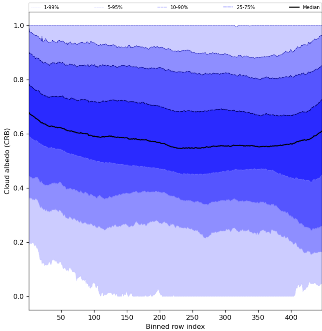
Figure 60: Along track statistics of “Cloud albedo (CRB)” for 2023-07-14 to 2023-07-16
