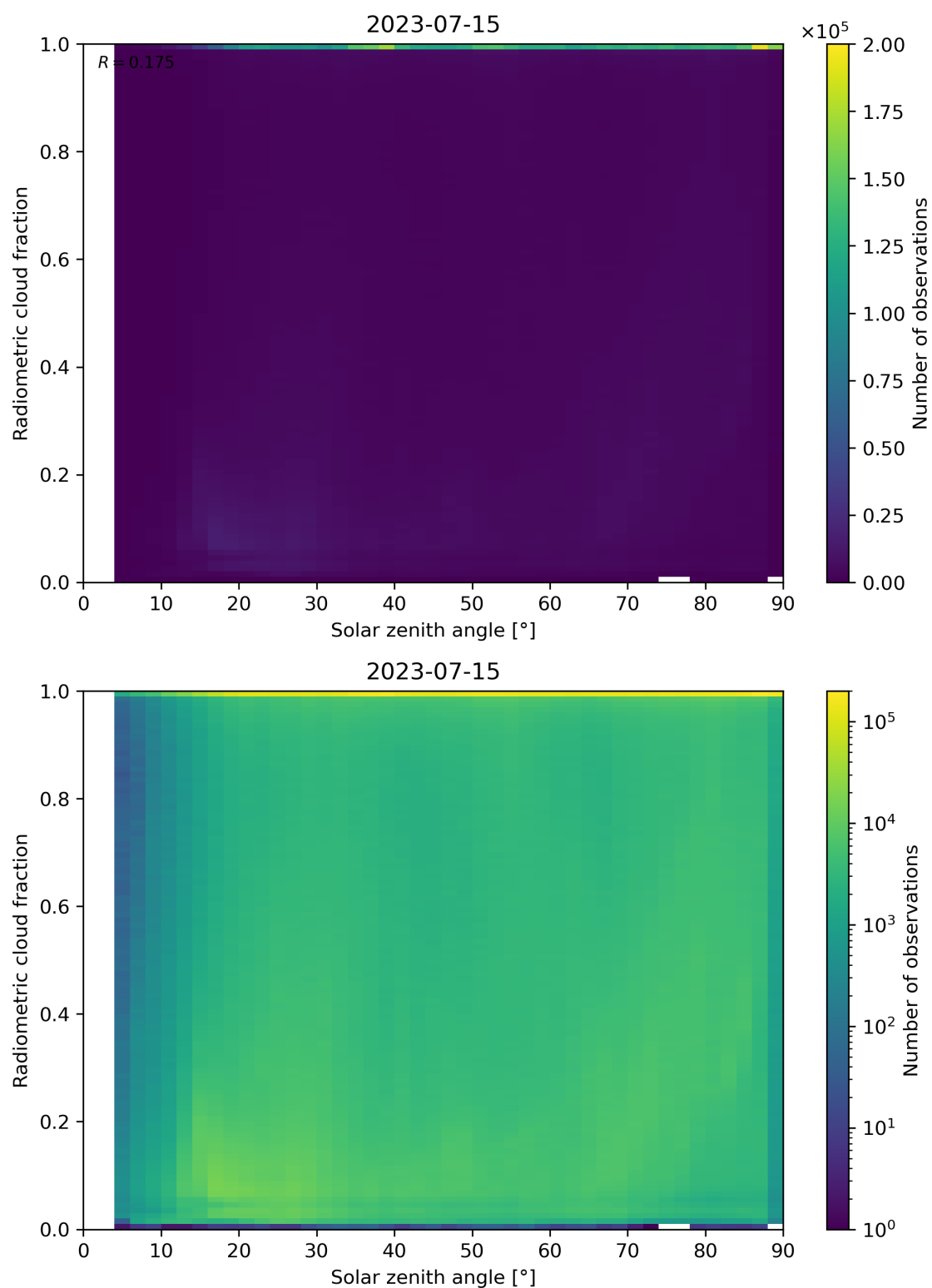
Figure 99: Scatter density plot of “Solar zenith angle” against “Radiometric cloud fraction” for 2023-07-14 to 2023-07-16.
