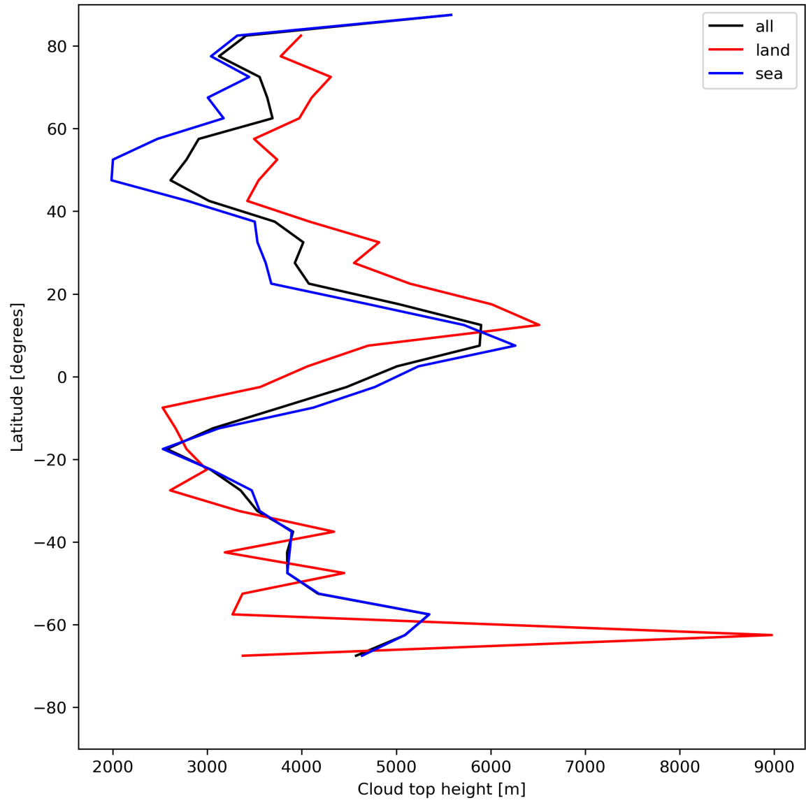
Figure 24: Zonal average of “Cloud top height” for 2023-07-14 to 2023-07-16.
