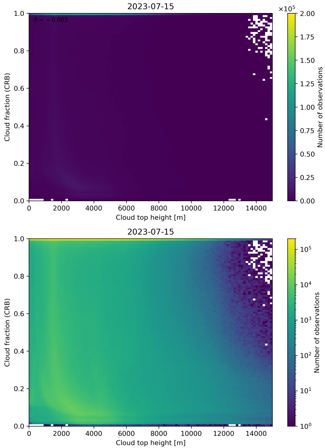
Figure 88: Scatter density plot of “Cloud top height” against “Cloud fraction (CRB)” for 2023-07-14 to 2023-07-16.
