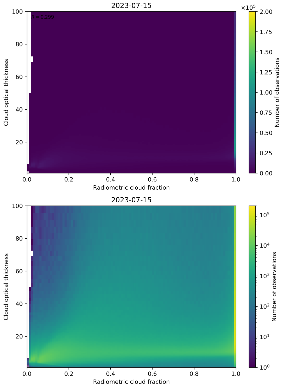
Figure 75: Scatter density plot of “Radiometric cloud fraction” against “Cloud optical thickness” for 2023-07-14 to 2023-07-16.
