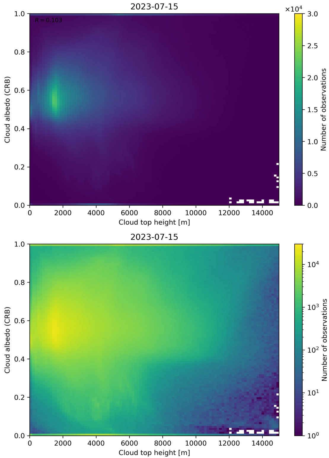
Figure 86: Scatter density plot of “Cloud top height” against “Cloud albedo (CRB)” for 2023-07-14 to 2023-07-16.
