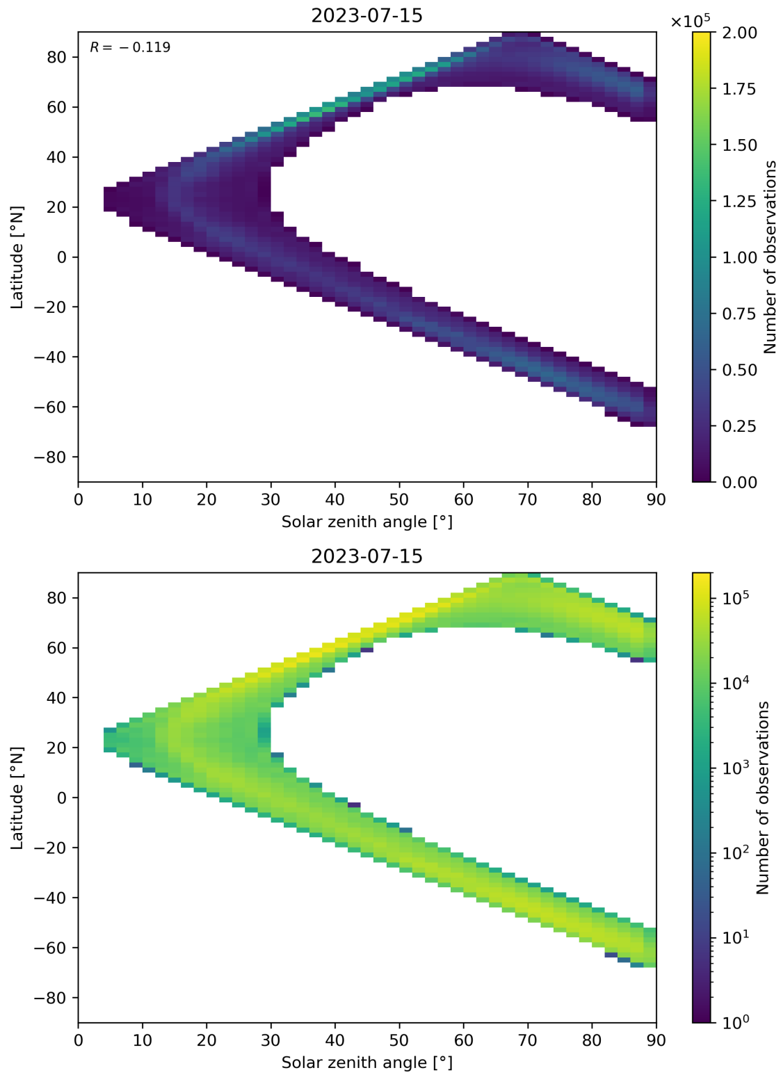
Figure 105: Scatter density plot of “Solar zenith angle” against “Latitude” for 2023-07-14 to 2023-07-16.
