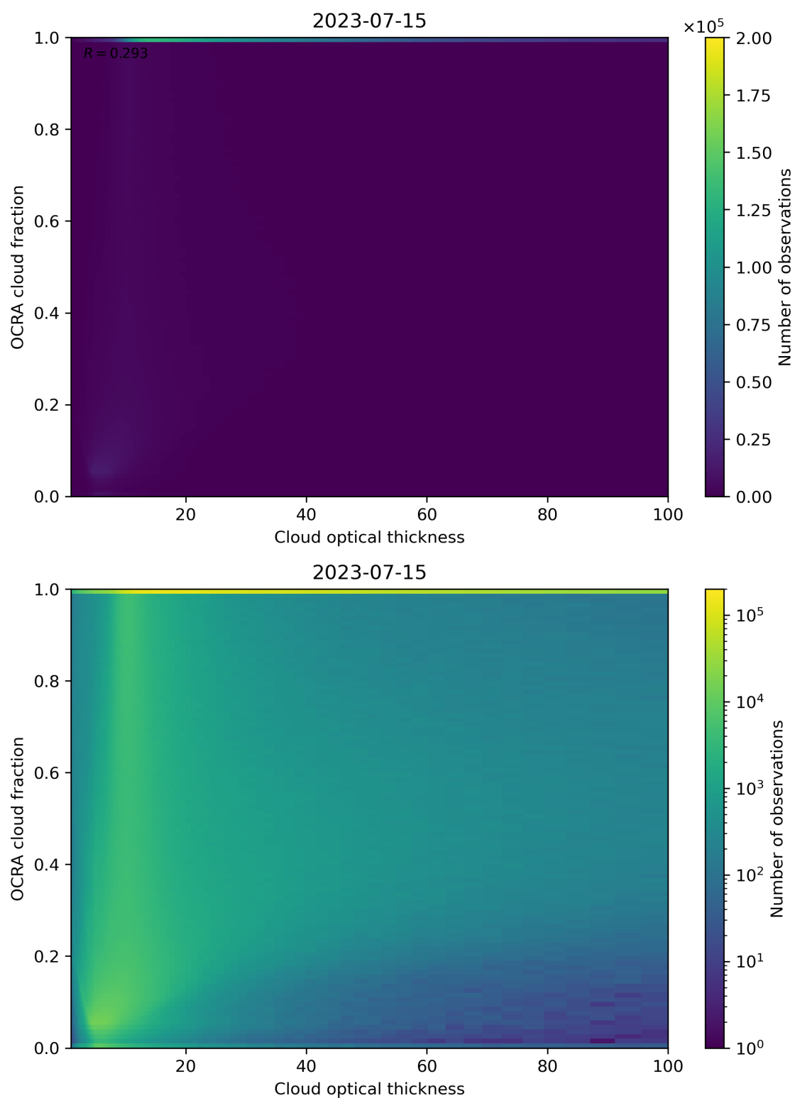
Figure 83: Scatter density plot of “Cloud optical thickness” against “OCRA cloud fraction” for 2023-07-14 to 2023-07-16.
