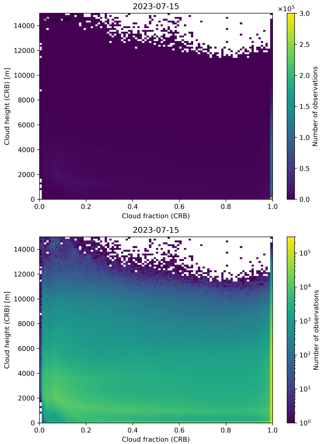
Figure 79: Scatter density plot of “Cloud fraction (CRB)” against “Cloud height (CRB)” for 2023-07-14 to 2023-07-16.
