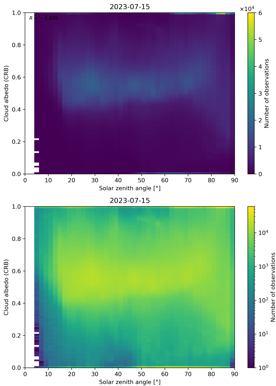
Figure 98: Scatter density plot of “Solar zenith angle” against “Cloud albedo (CRB)” for 2023-07-14 to 2023-07-16.
