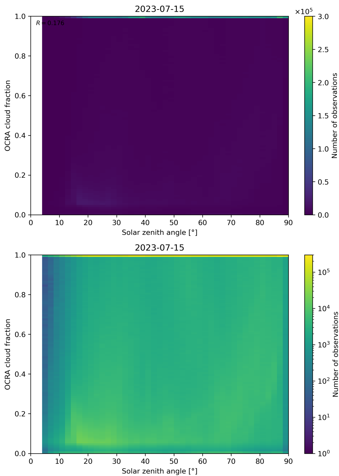
Figure 100: Scatter density plot of “Solar zenith angle” against “OCRA cloud fraction” for 2023-07-14 to 2023-07-16.
