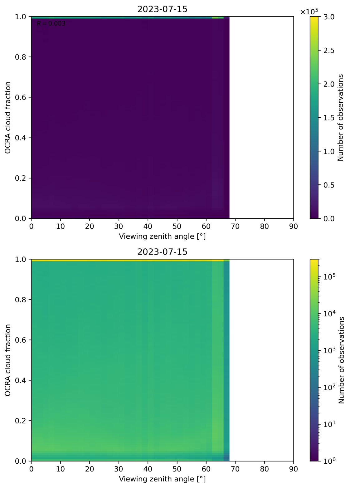
Figure 108: Scatter density plot of “Viewing zenith angle” against “OCRA cloud fraction” for 2023-07-14 to 2023-07-16.
