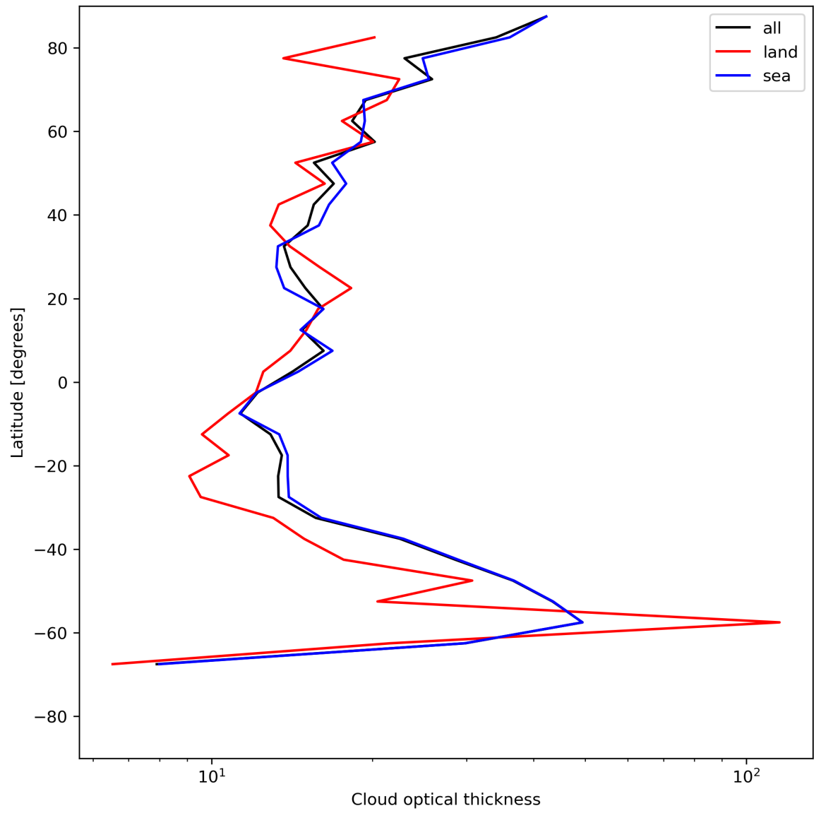
Figure 25: Zonal average of “Cloud optical thickness” for 2023-07-14 to 2023-07-16.
