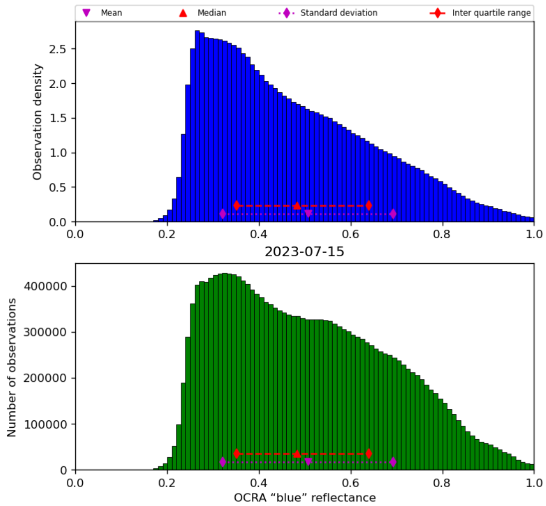
Figure 51: Histogram of “OCRA “blue” reflectance” for 2023-07-14 to 2023-07-16
