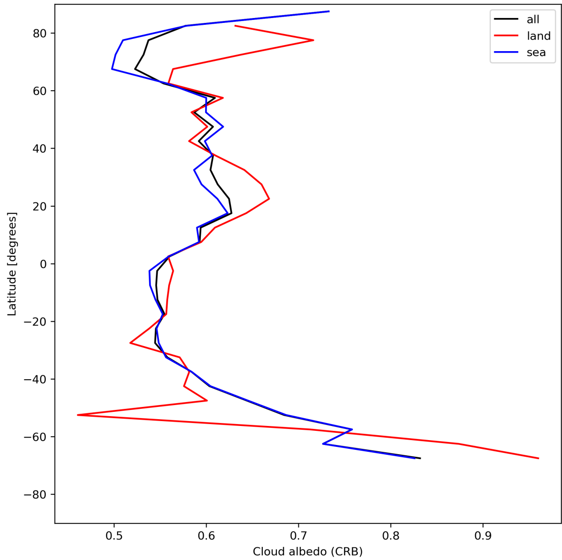
Figure 28: Zonal average of “Cloud albedo (CRB)” for 2023-07-14 to 2023-07-16.
