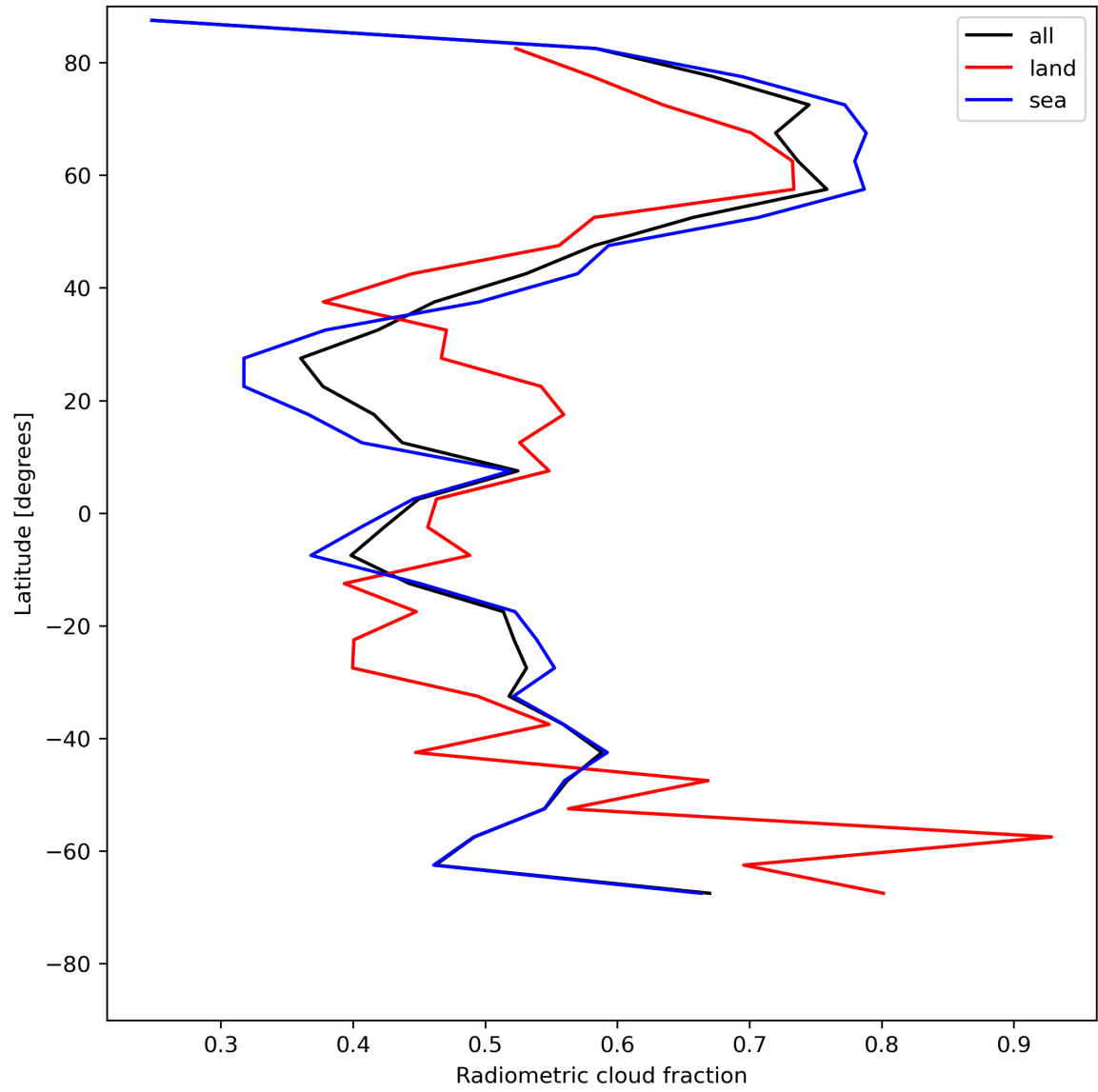
Figure 23: Zonal average of “Radiometric cloud fraction” for 2023-07-14 to 2023-07-16.
