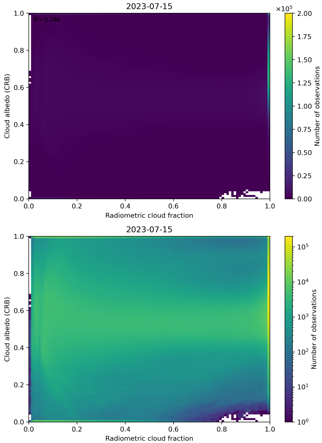
Figure 71: Scatter density plot of “Radiometric cloud fraction” against “Cloud albedo (CRB)” for 2023-07-14 to 2023-07-16.
