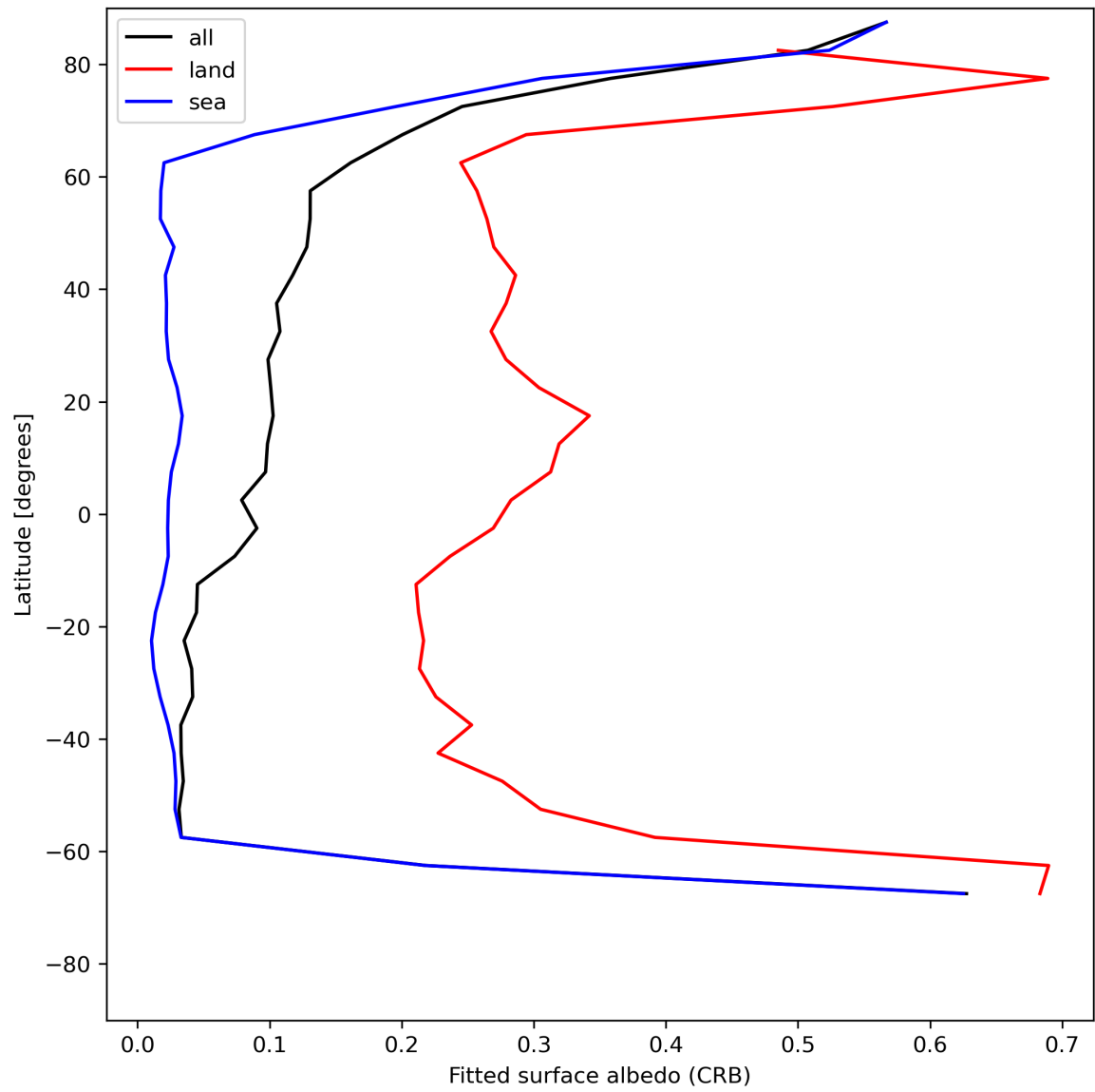
Figure 30: Zonal average of “Fitted surface albedo (CRB)” for 2023-07-14 to 2023-07-16.
