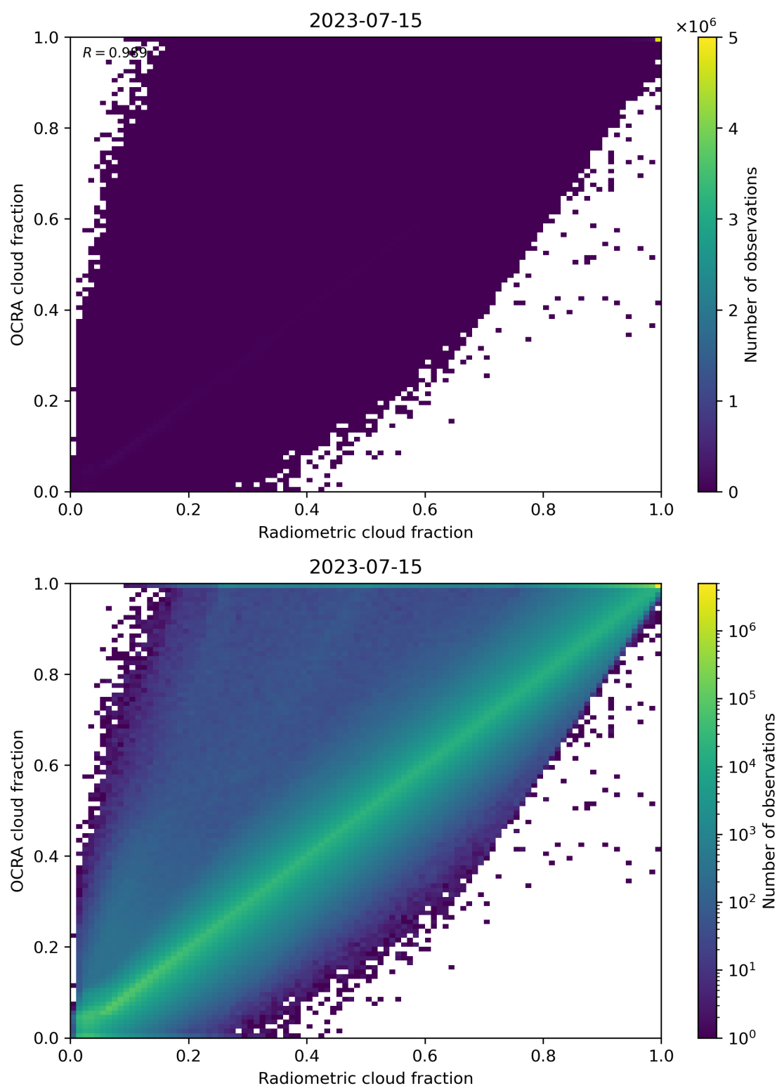
Figure 72: Scatter density plot of “Radiometric cloud fraction” against “OCRA cloud fraction” for 2023-07-14 to 2023-07-16.
