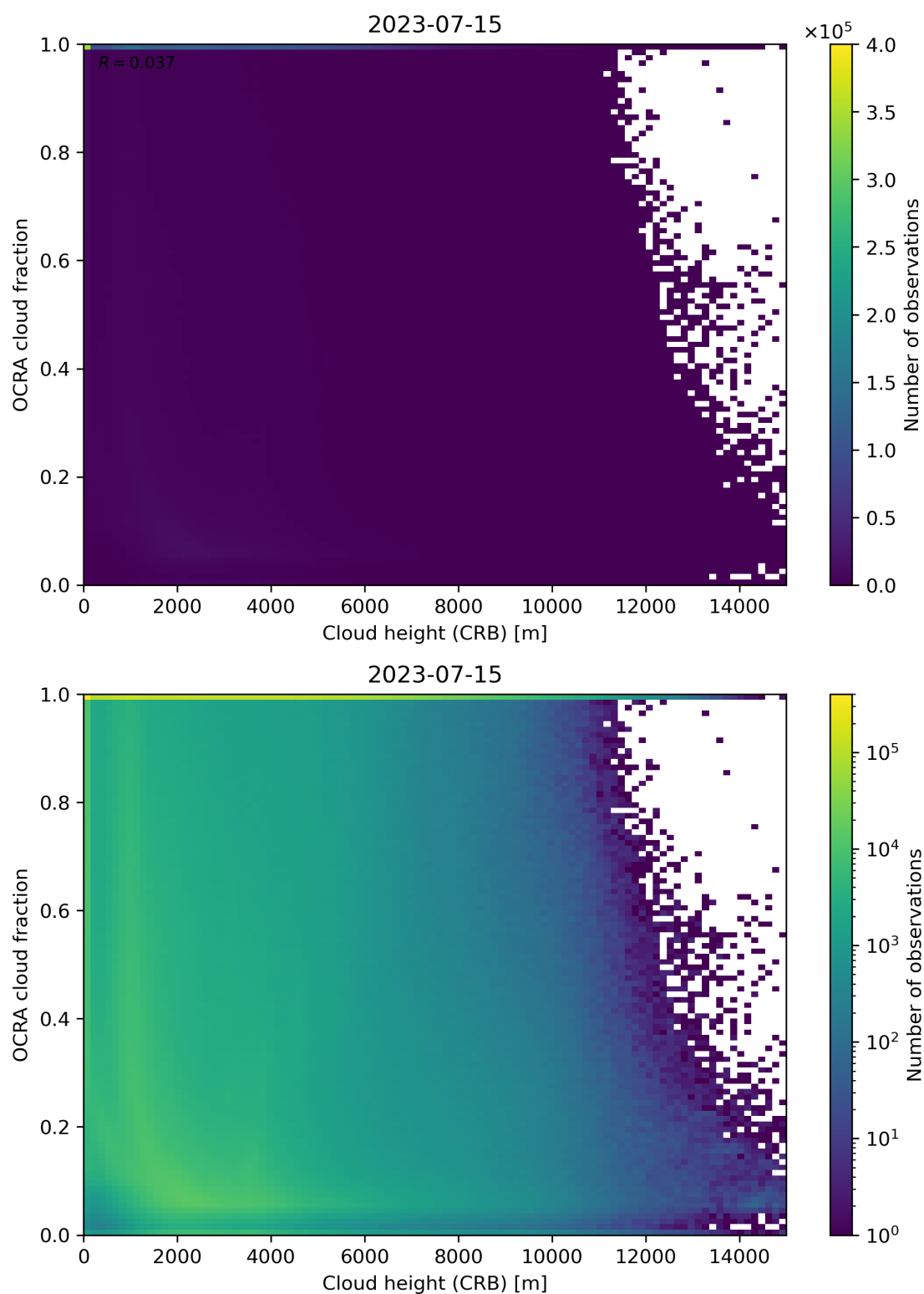
Figure 81: Scatter density plot of “Cloud height (CRB)” against “OCRA cloud fraction” for 2023-07-14 to 2023-07-16.
