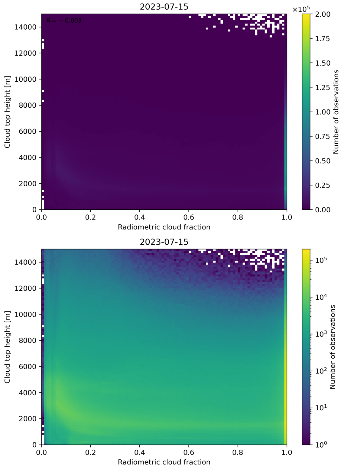
Figure 76: Scatter density plot of “Radiometric cloud fraction” against “Cloud top height” for 2023-07-14 to 2023-07-16.
