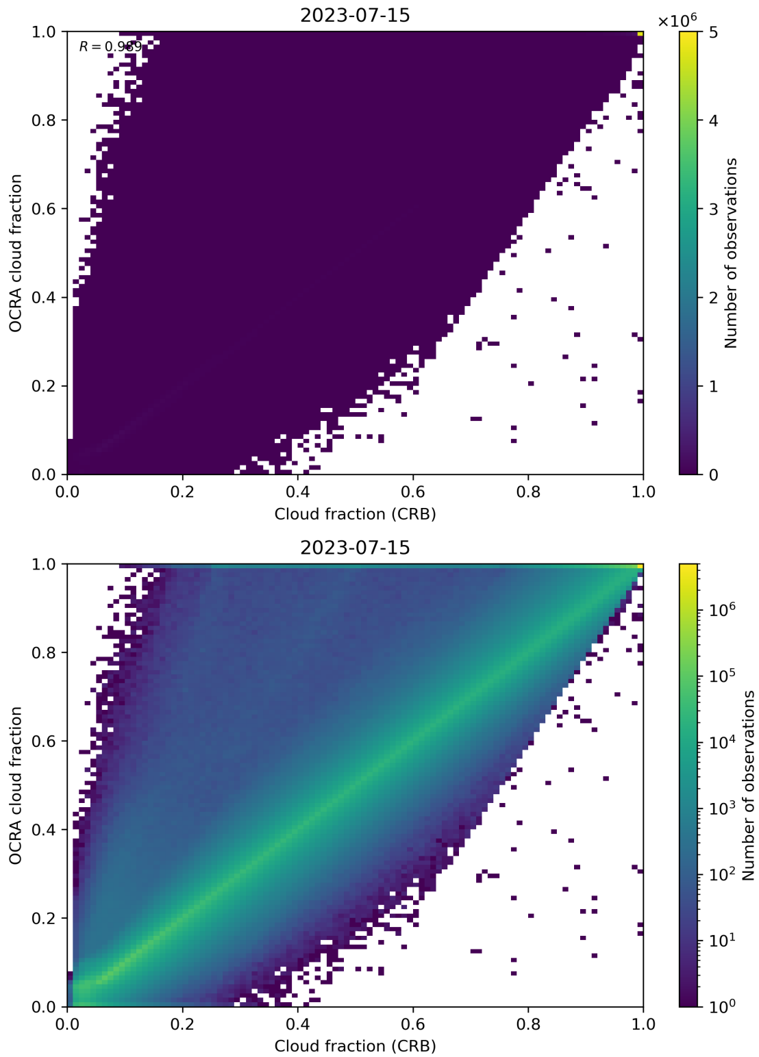
Figure 78: Scatter density plot of “Cloud fraction (CRB)” against “OCRA cloud fraction” for 2023-07-14 to 2023-07-16.
