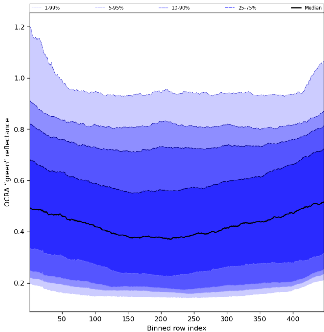
Figure 68: Along track statistics of “OCRA “green” reflectance” for 2023-07-14 to 2023-07-16
