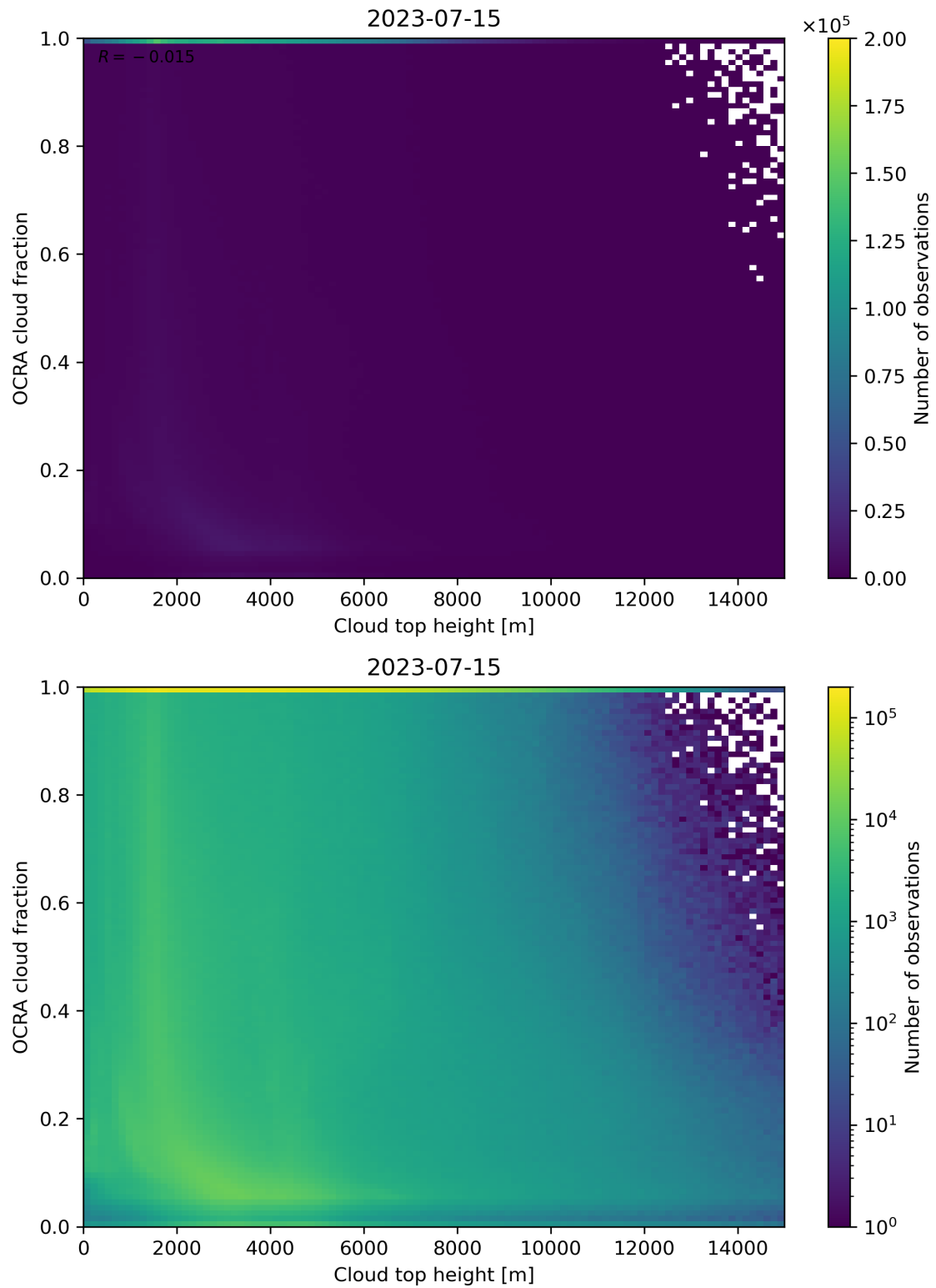
Figure 87: Scatter density plot of “Cloud top height” against “OCRA cloud fraction” for 2023-07-14 to 2023-07-16.
