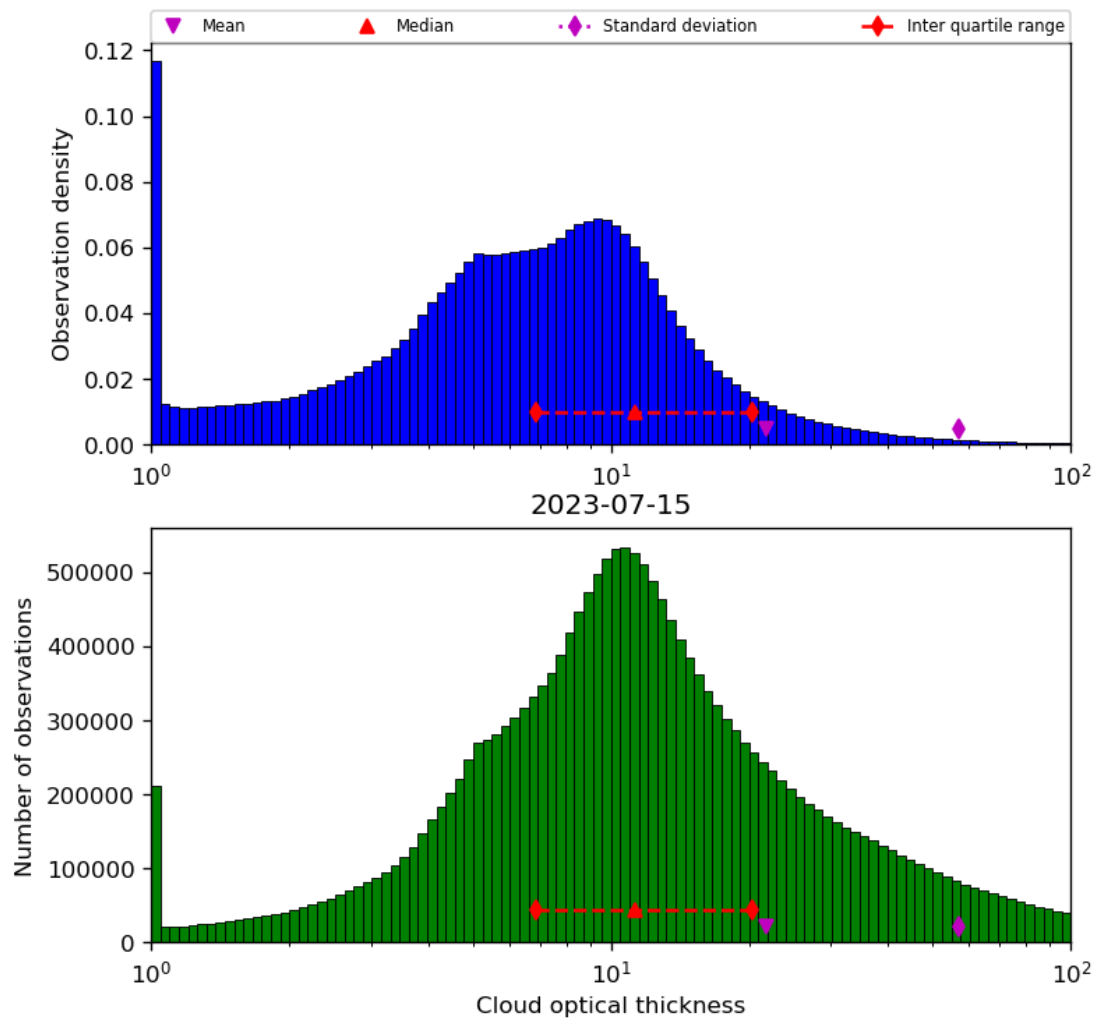
Figure 41: Histogram of “Cloud optical thickness” for 2023-07-14 to 2023-07-16
