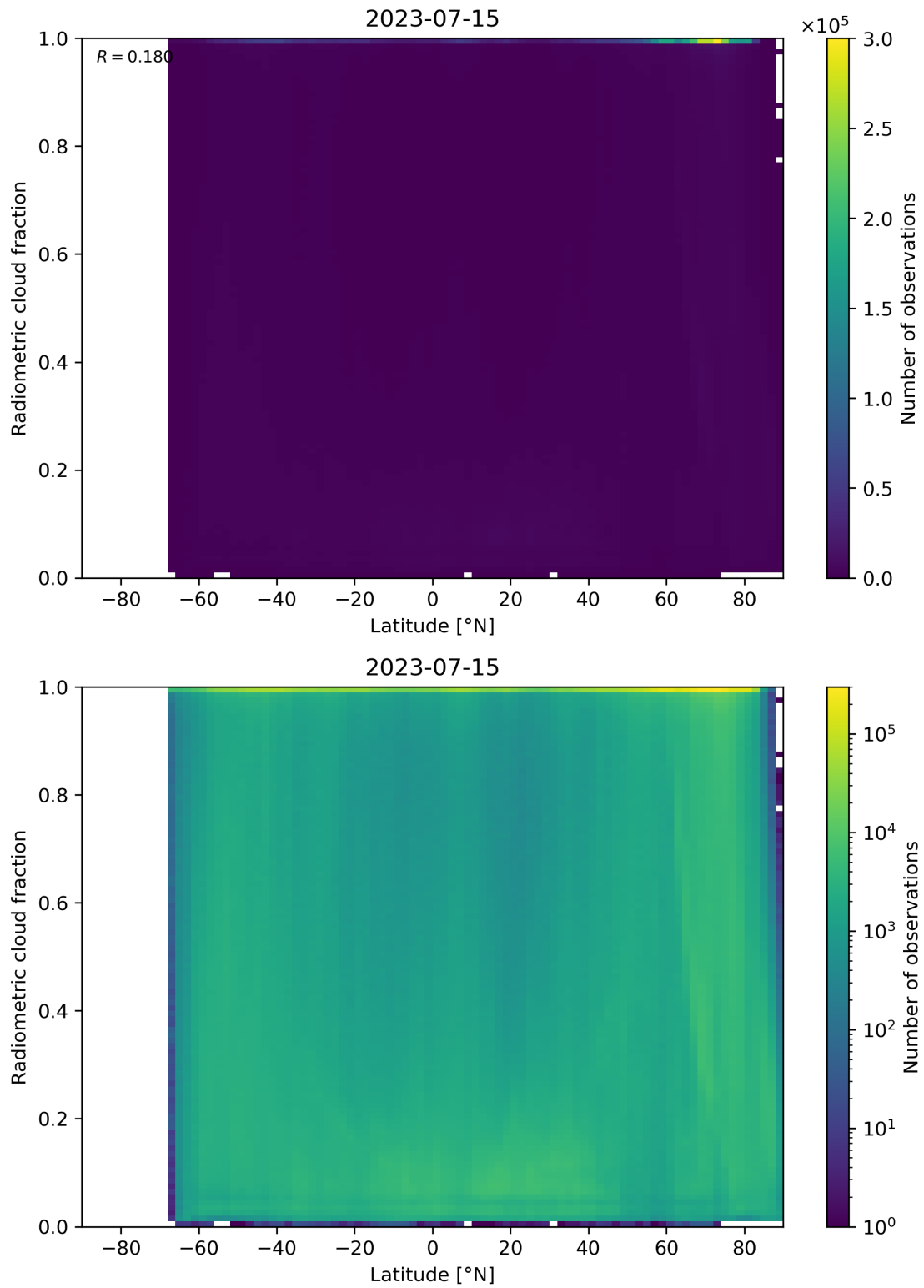
Figure 92: Scatter density plot of “Latitude” against “Radiometric cloud fraction” for 2023-07-14 to 2023-07-16.
