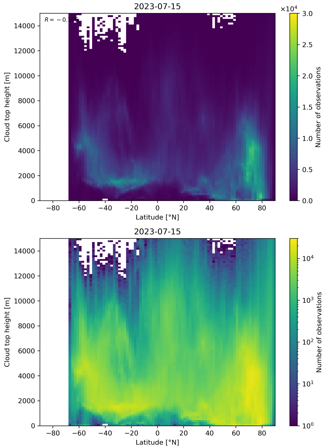
Figure 97: Scatter density plot of “Latitude” against “Cloud top height” for 2023-07-14 to 2023-07-16.
