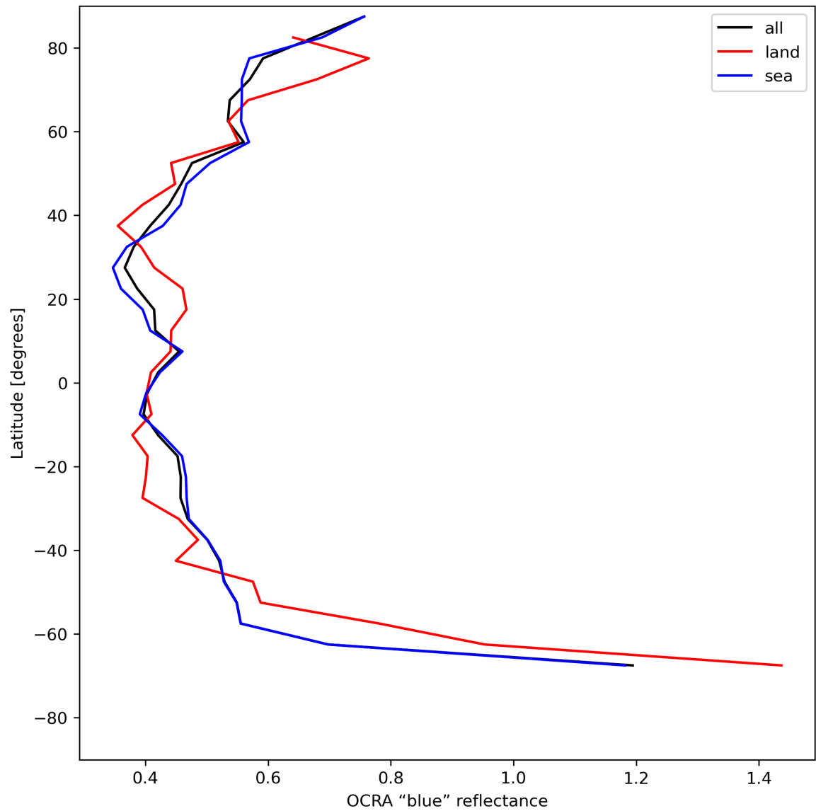
Figure 35: Zonal average of “OCRA “blue” reflectance” for 2023-07-14 to 2023-07-16.
