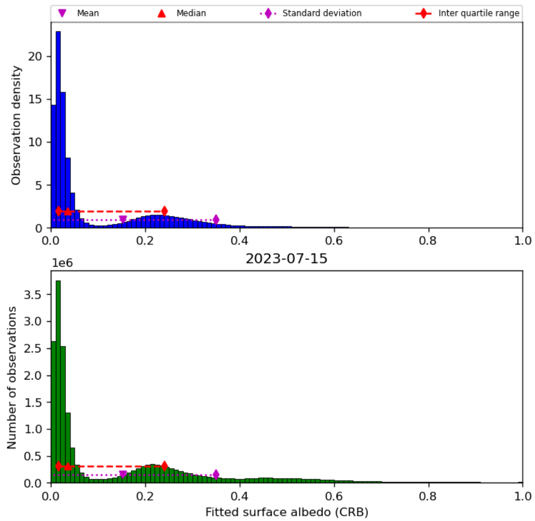
Figure 46: Histogram of “Fitted surface albedo (CRB)” for 2023-07-14 to 2023-07-16
