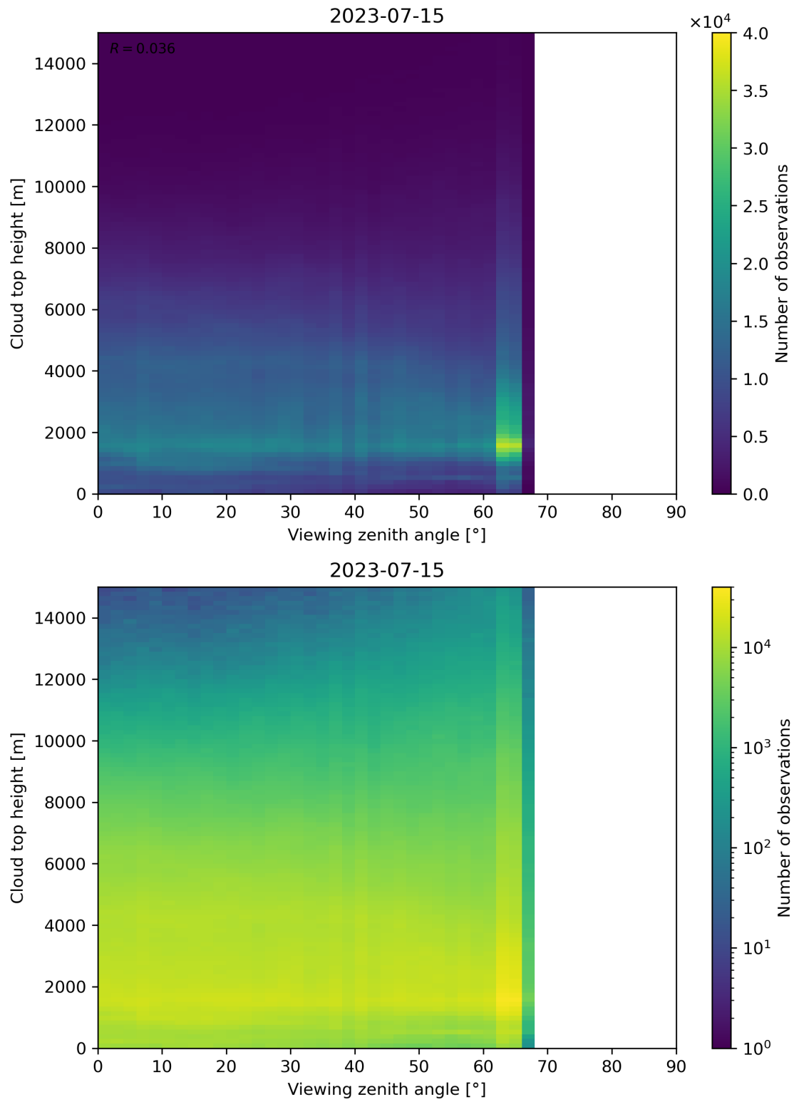
Figure 112: Scatter density plot of “Viewing zenith angle” against “Cloud top height” for 2023-07-14 to 2023-07-16.
