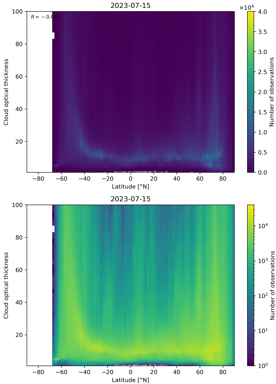
Figure 96: Scatter density plot of “Latitude” against “Cloud optical thickness” for 2023-07-14 to 2023-07-16.
