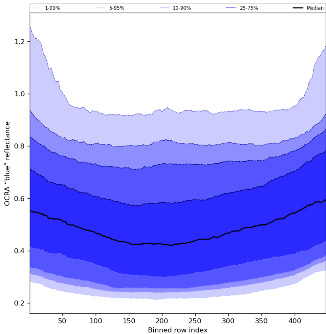
Figure 67: Along track statistics of “OCRA “blue” reflectance” for 2023-07-14 to 2023-07-16
