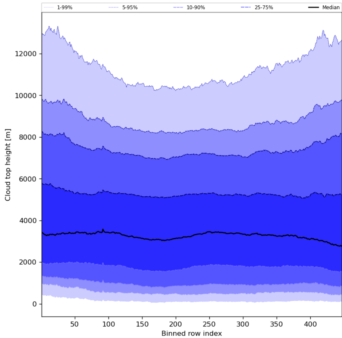
Figure 56: Along track statistics of “Cloud top height” for 2023-07-14 to 2023-07-16
