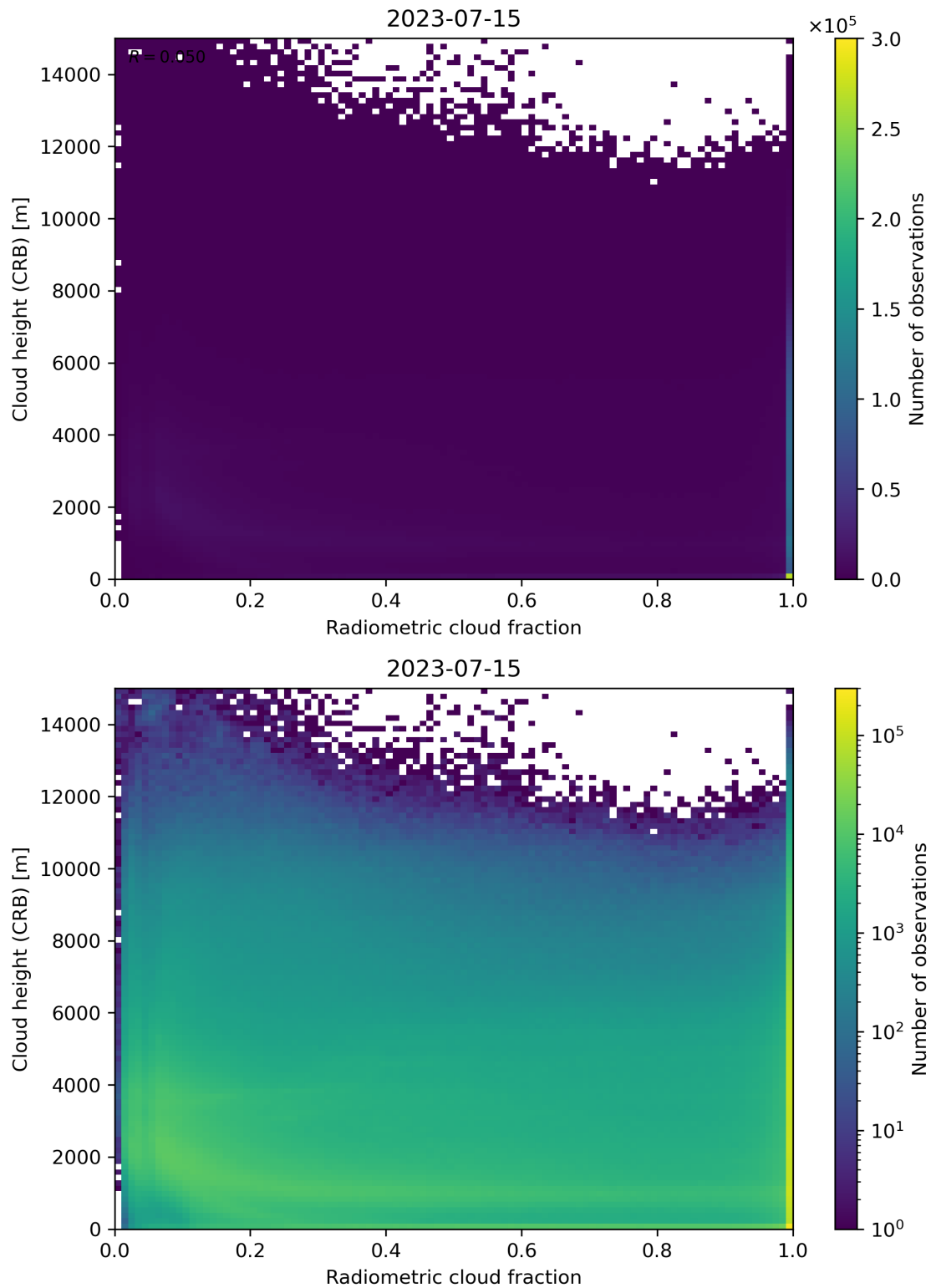
Figure 74: Scatter density plot of “Radiometric cloud fraction” against “Cloud height (CRB)” for 2023-07-14 to 2023-07-16.
