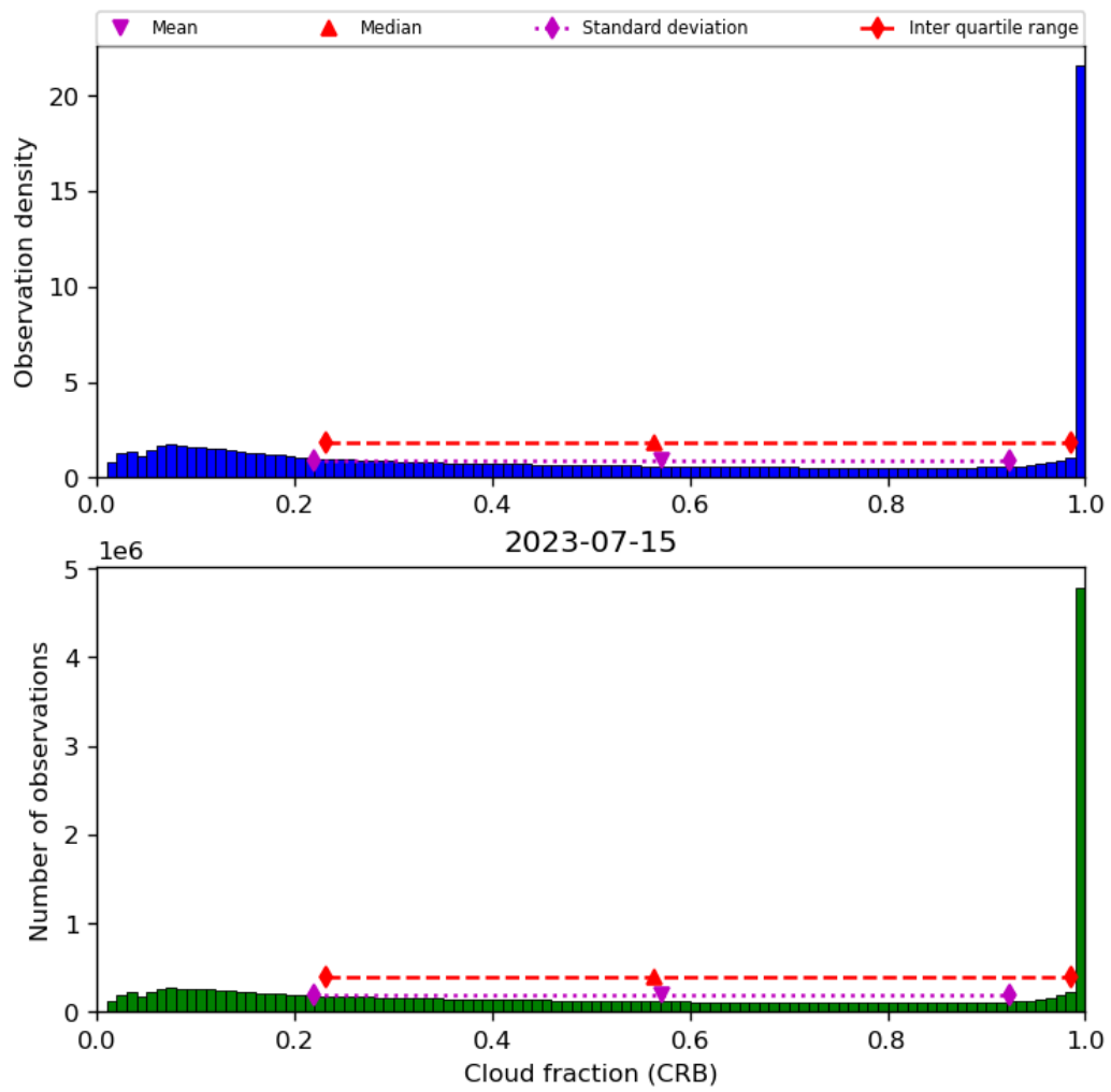
Figure 42: Histogram of “Cloud fraction (CRB)” for 2023-07-14 to 2023-07-16
