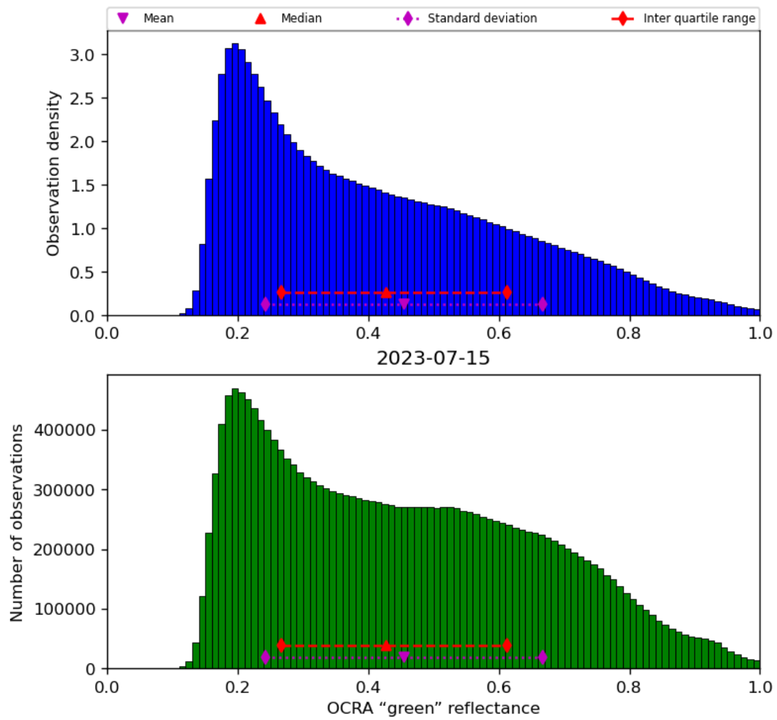
Figure 52: Histogram of “OCRA “green” reflectance” for 2023-07-14 to 2023-07-16
