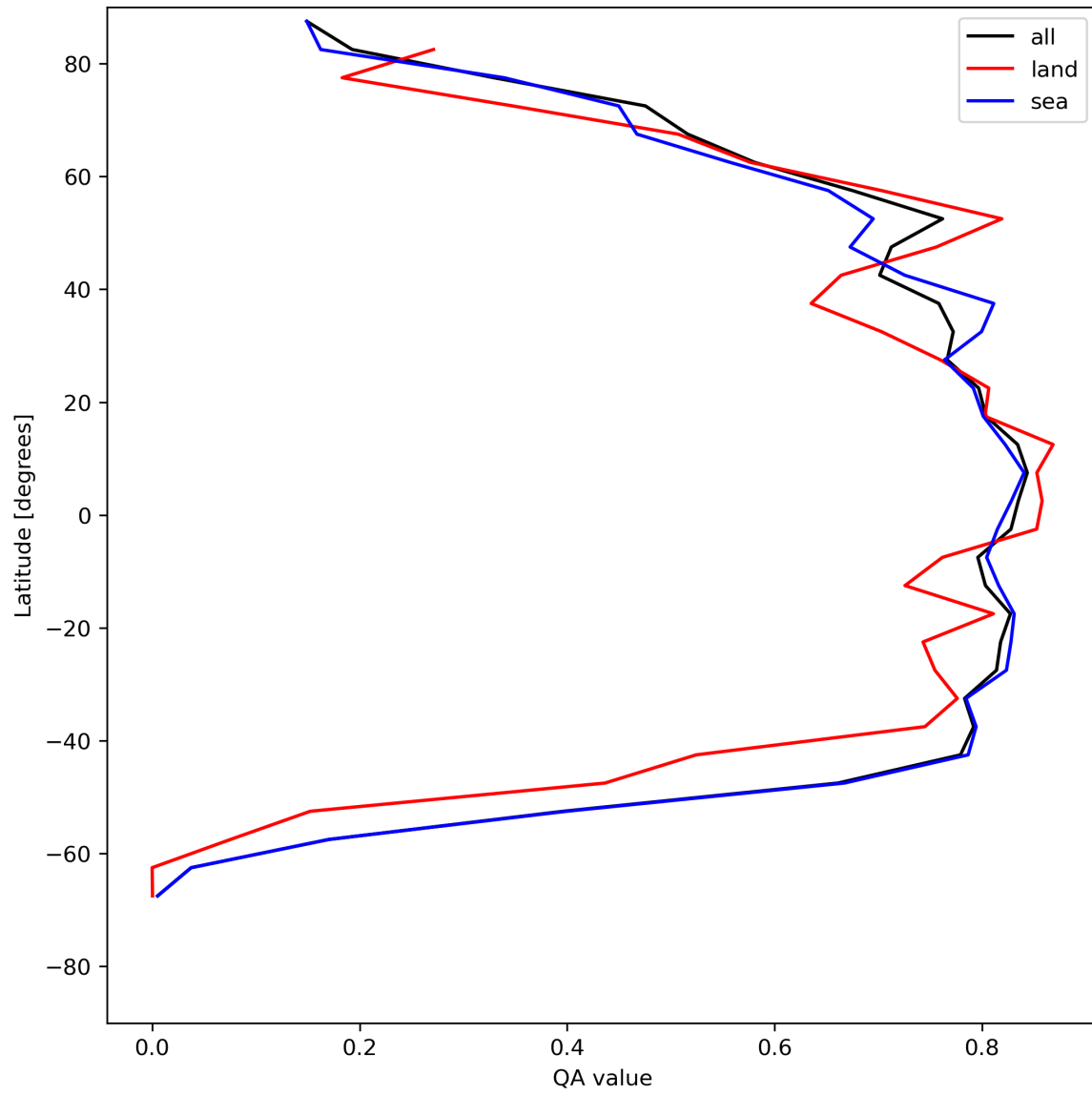
Figure 22: Zonal average of “QA value” for 2023-07-14 to 2023-07-16.
