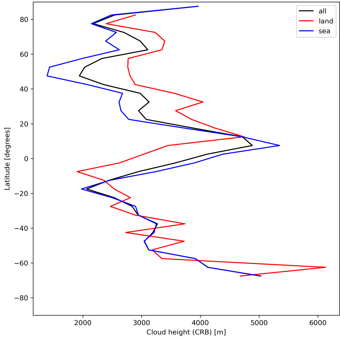
Figure 27: Zonal average of “Cloud height (CRB)” for 2023-07-14 to 2023-07-16.
