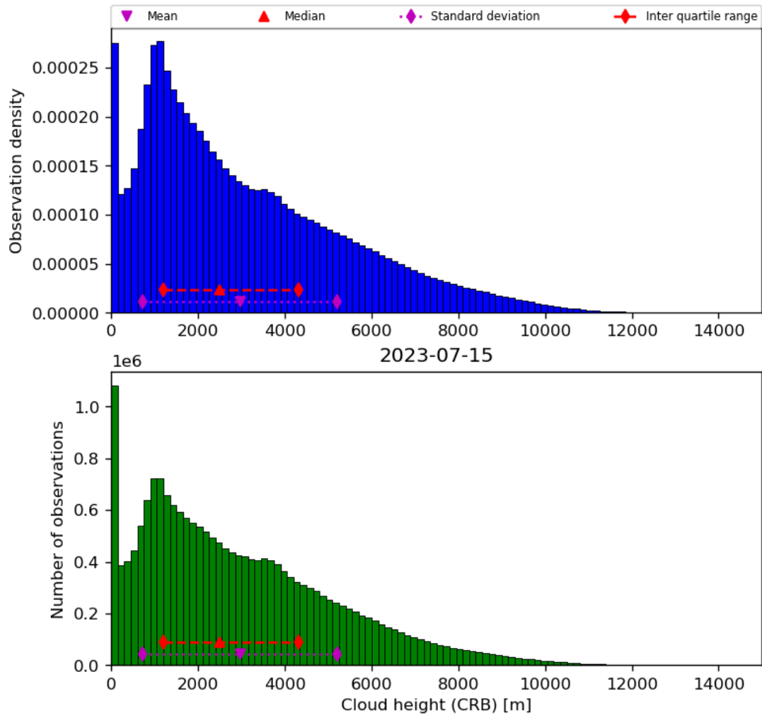
Figure 43: Histogram of “Cloud height (CRB)” for 2023-07-14 to 2023-07-16
