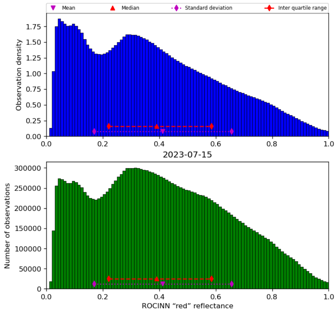
Figure 53: Histogram of “ROCINN “red” reflectance” for 2023-07-14 to 2023-07-16
