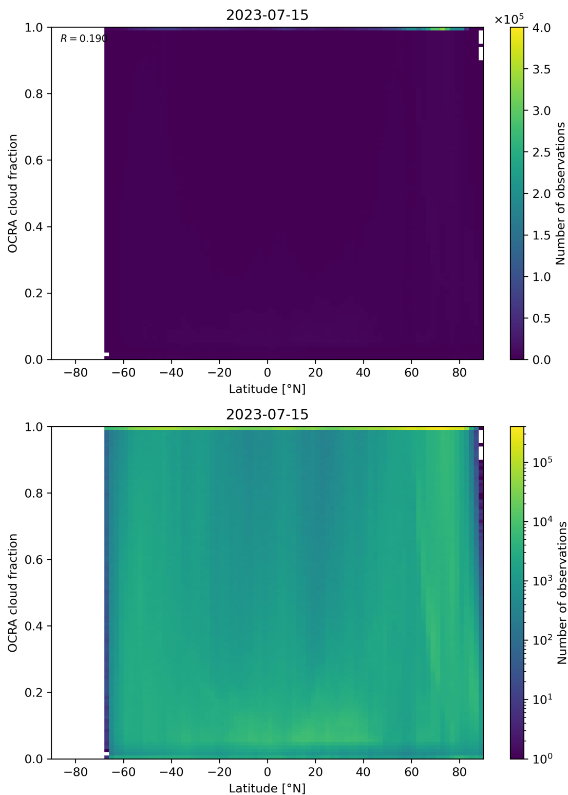
Figure 93: Scatter density plot of “Latitude” against “OCRA cloud fraction” for 2023-07-14 to 2023-07-16.
