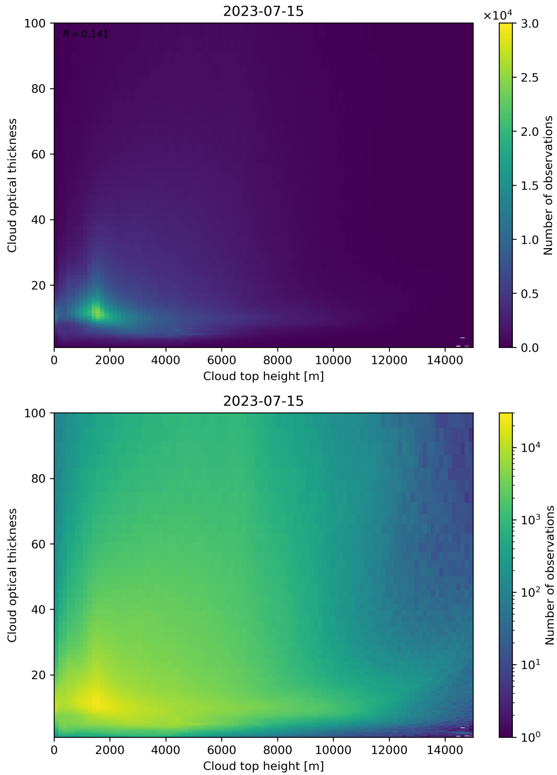
Figure 90: Scatter density plot of “Cloud top height” against “Cloud optical thickness” for 2023-07-14 to 2023-07-16.
