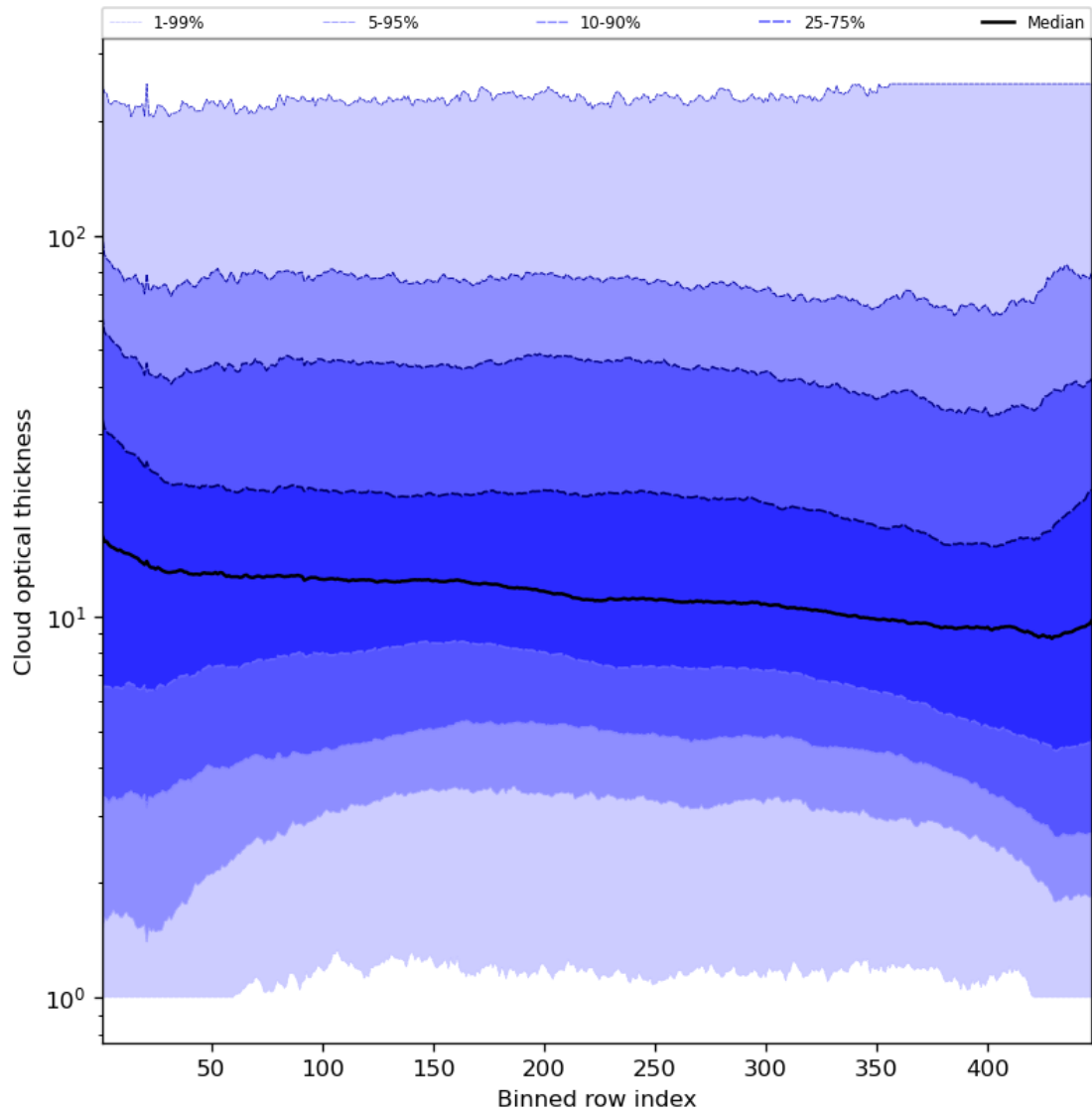
Figure 57: Along track statistics of “Cloud optical thickness” for 2023-07-14 to 2023-07-16
