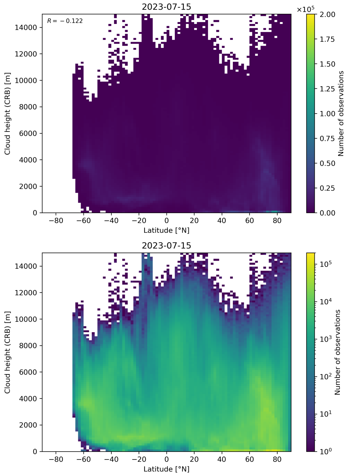
Figure 95: Scatter density plot of “Latitude” against “Cloud height (CRB)” for 2023-07-14 to 2023-07-16.
