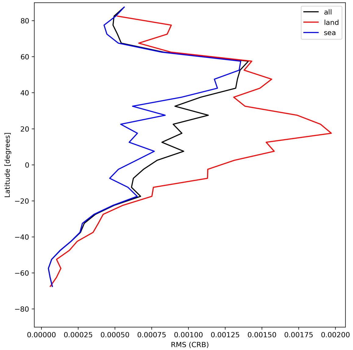
Figure 32: Zonal average of “RMS (CRB)” for 2023-07-14 to 2023-07-16.
