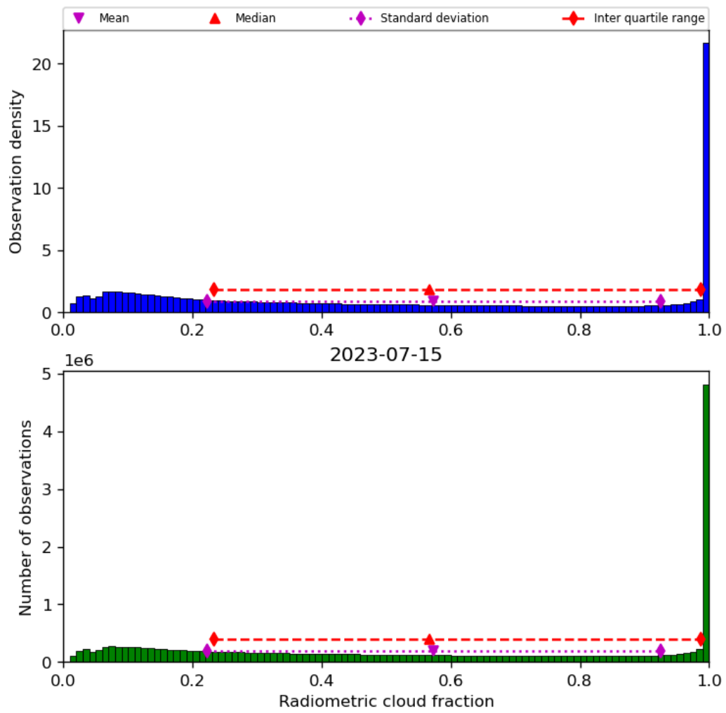
Figure 39: Histogram of “Radiometric cloud fraction” for 2023-07-14 to 2023-07-16
