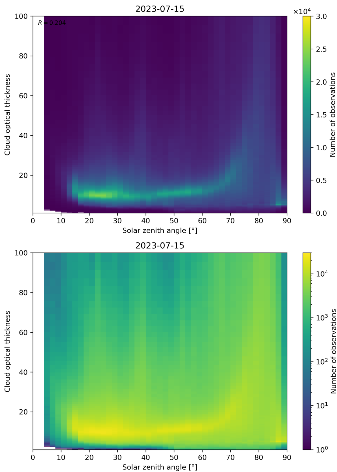
Figure 103: Scatter density plot of “Solar zenith angle” against “Cloud optical thickness” for 2023-07-14 to 2023-07-16.
