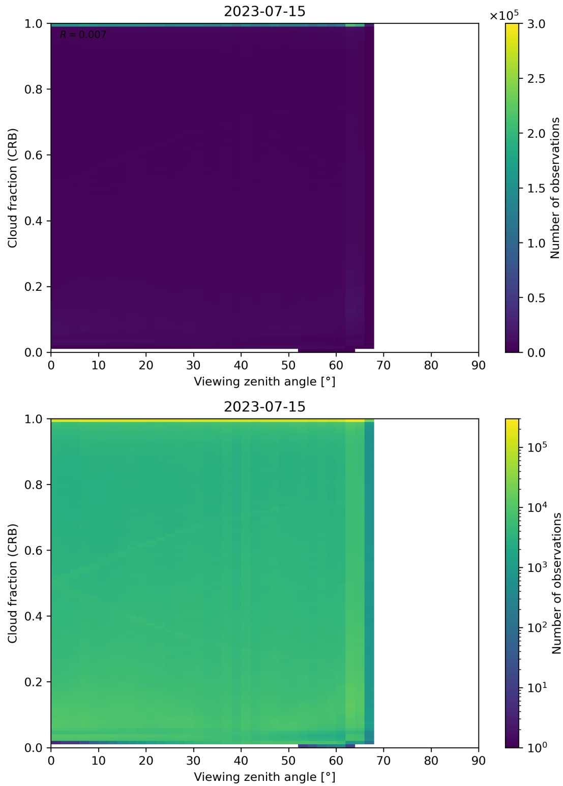
Figure 109: Scatter density plot of “Viewing zenith angle” against “Cloud fraction (CRB)” for 2023-07-14 to 2023-07-16.
