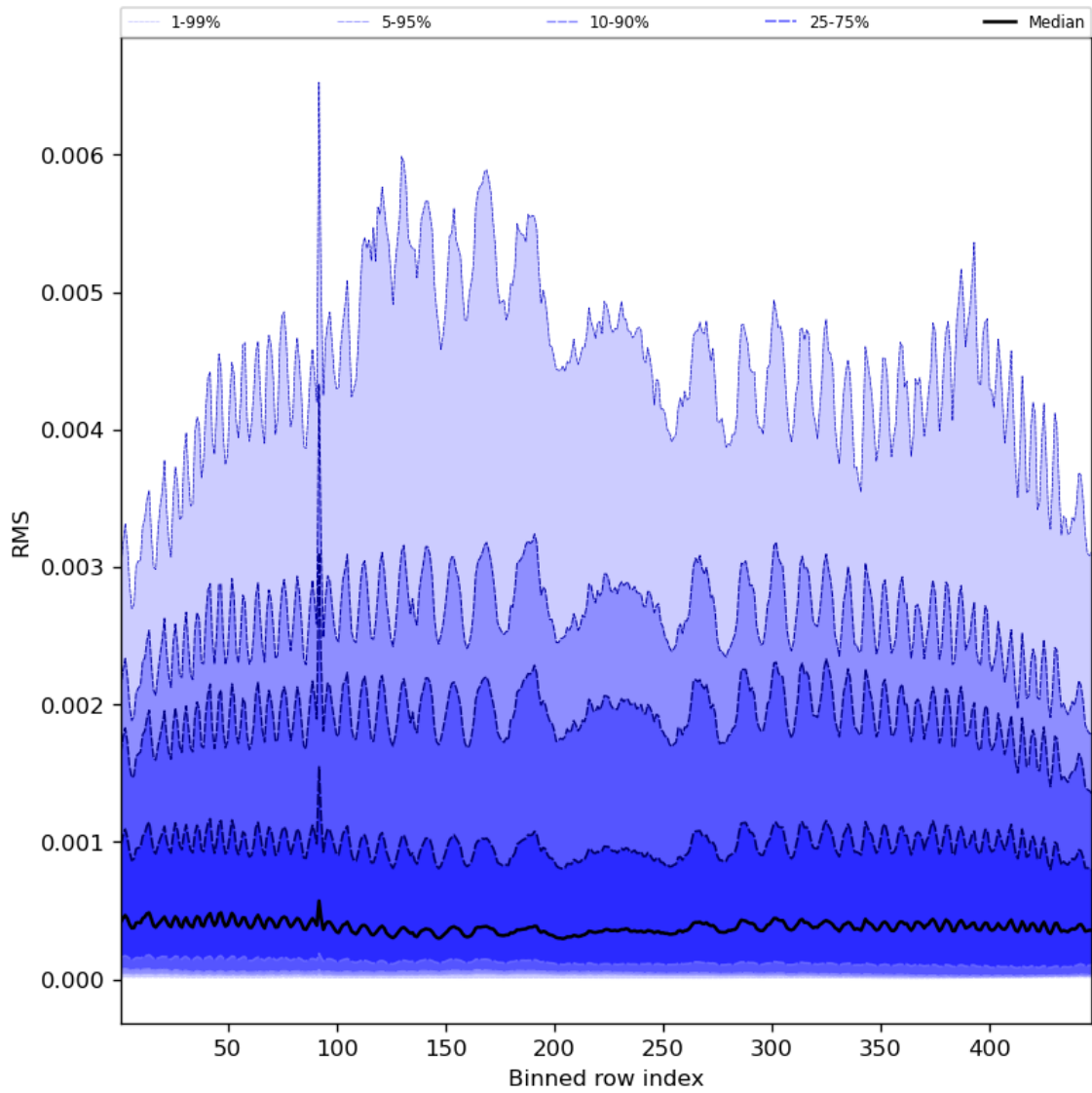
Figure 63: Along track statistics of “RMS” for 2023-07-14 to 2023-07-16
