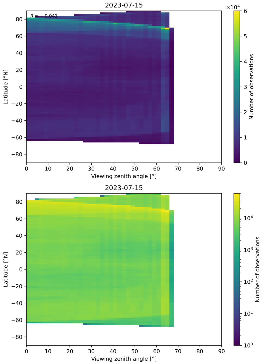
Figure 113: Scatter density plot of “Viewing zenith angle” against “Latitude” for 2023-07-14 to 2023-07-16.
