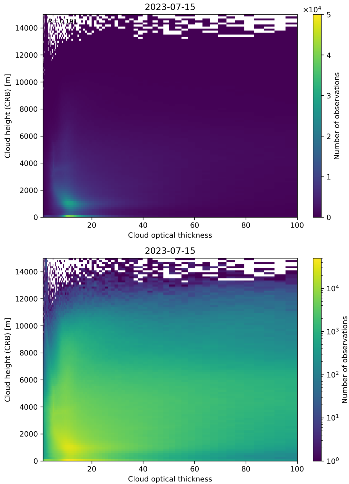
Figure 85: Scatter density plot of “Cloud optical thickness” against “Cloud height (CRB)” for 2023-07-14 to 2023-07-16.
