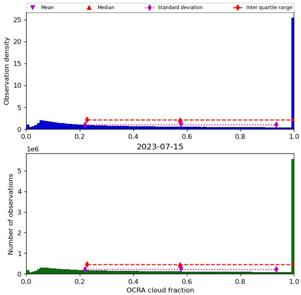
Figure 50: Histogram of “OCRA cloud fraction” for 2023-07-14 to 2023-07-16
