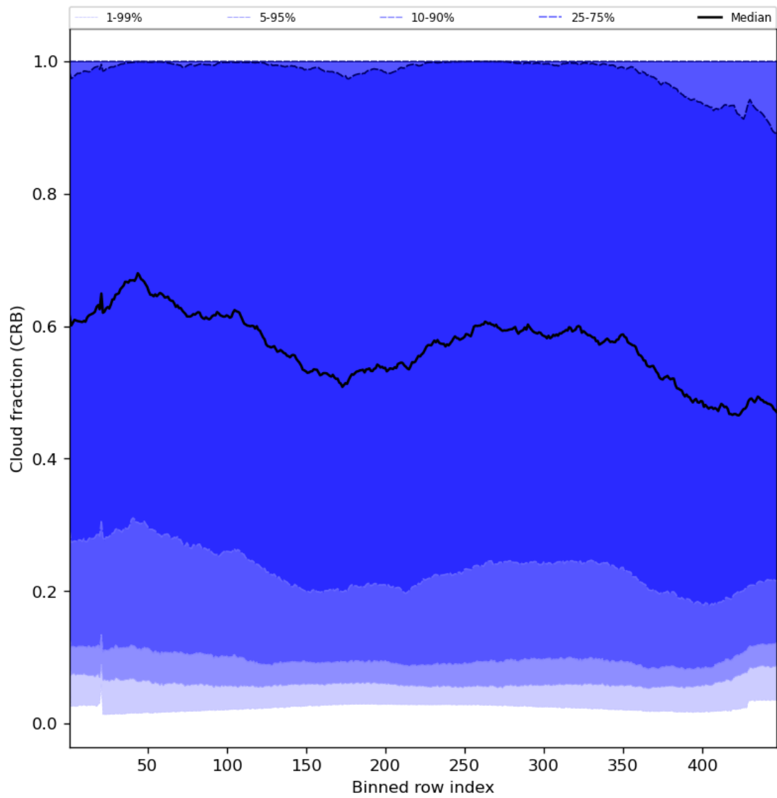
Figure 58: Along track statistics of “Cloud fraction (CRB)” for 2023-07-15 to 2023-07-17
