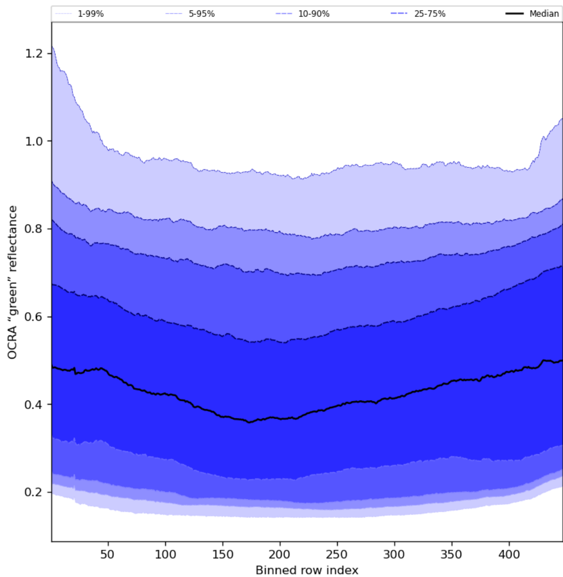
Figure 68: Along track statistics of “OCRA “green” reflectance” for 2023-07-15 to 2023-07-17
