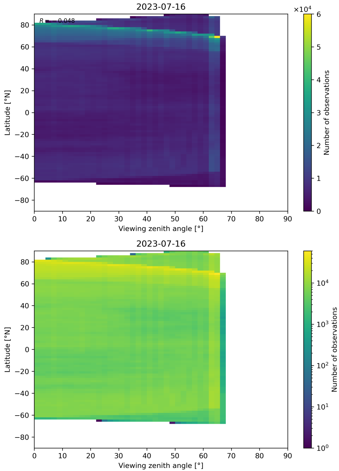
Figure 113: Scatter density plot of “Viewing zenith angle” against “Latitude” for 2023-07-15 to 2023-07-17.
