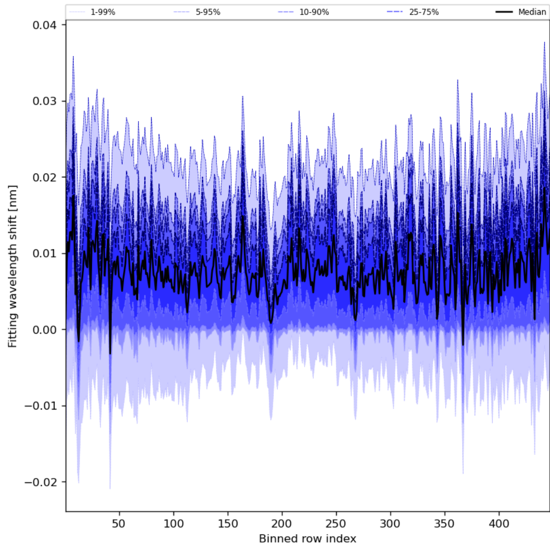
Figure 65: Along track statistics of “Fitting wavelength shift” for 2023-07-15 to 2023-07-17
