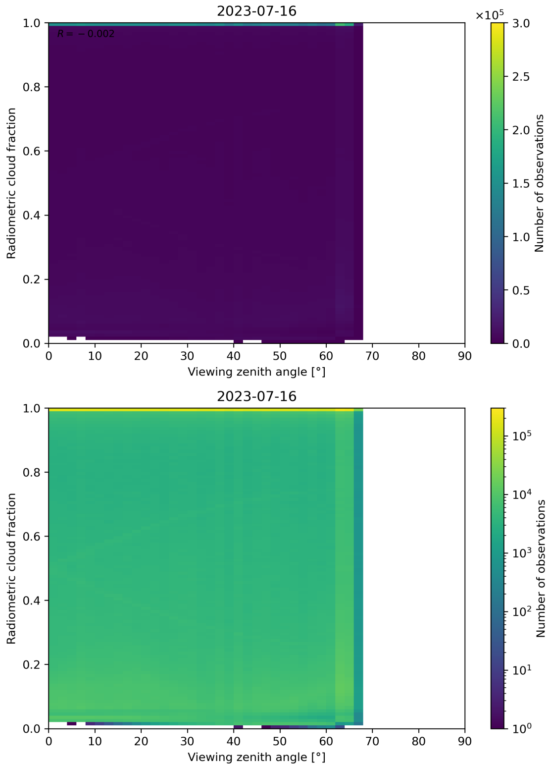
Figure 107: Scatter density plot of “Viewing zenith angle” against “Radiometric cloud fraction” for 2023-07-15 to 2023-07-17.
