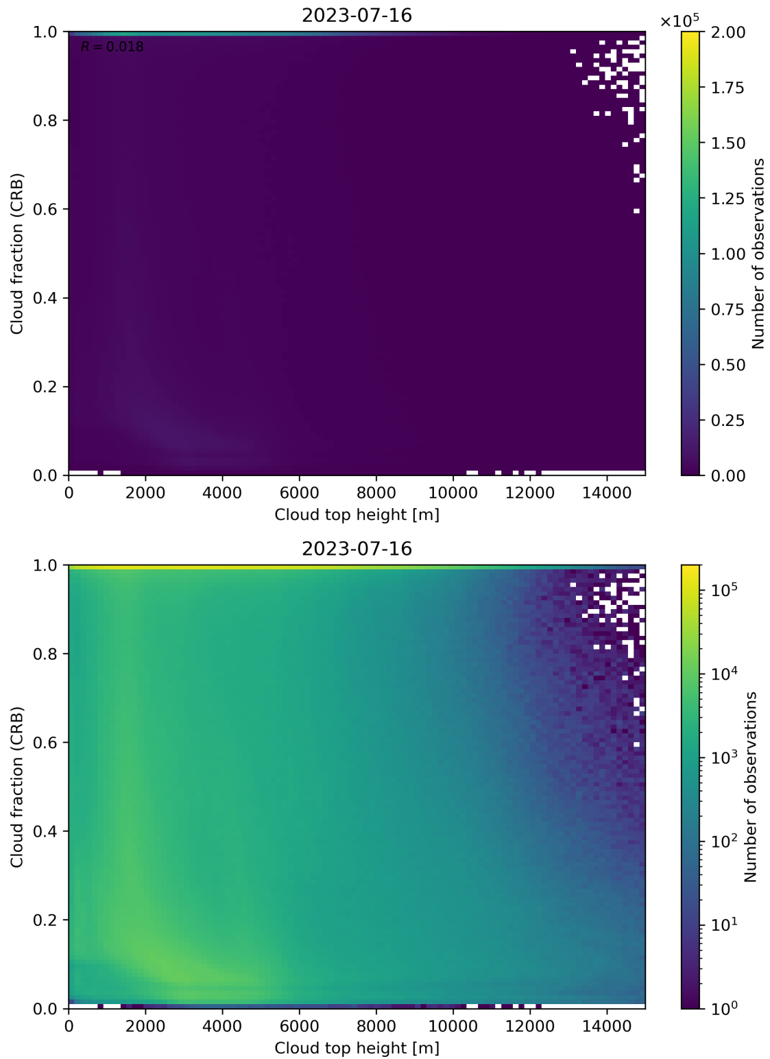
Figure 88: Scatter density plot of “Cloud top height” against “Cloud fraction (CRB)” for 2023-07-15 to 2023-07-17.
