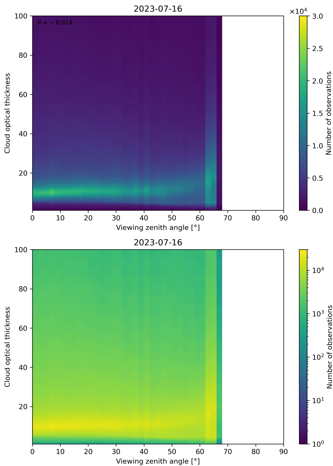
Figure 111: Scatter density plot of “Viewing zenith angle” against “Cloud optical thickness” for 2023-07-15 to 2023-07-17.
