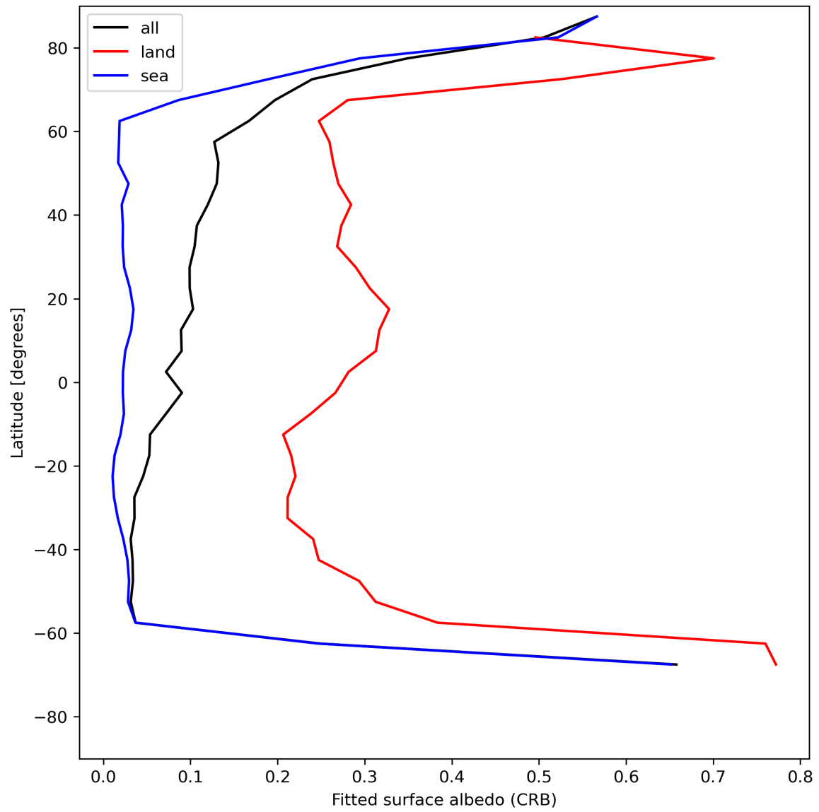
Figure 30: Zonal average of “Fitted surface albedo (CRB)” for 2023-07-15 to 2023-07-17.
