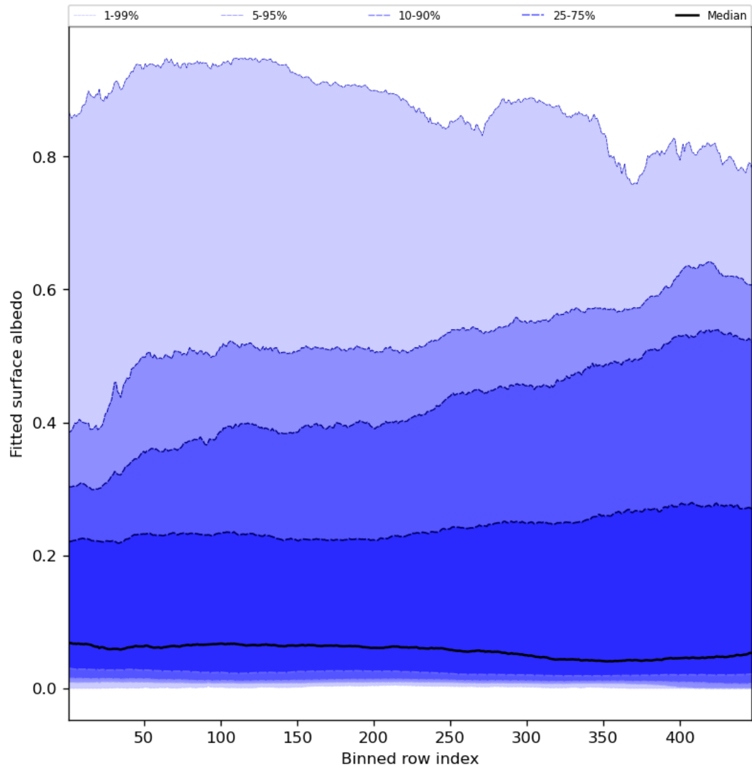
Figure 61: Along track statistics of “Fitted surface albedo” for 2023-07-15 to 2023-07-17
