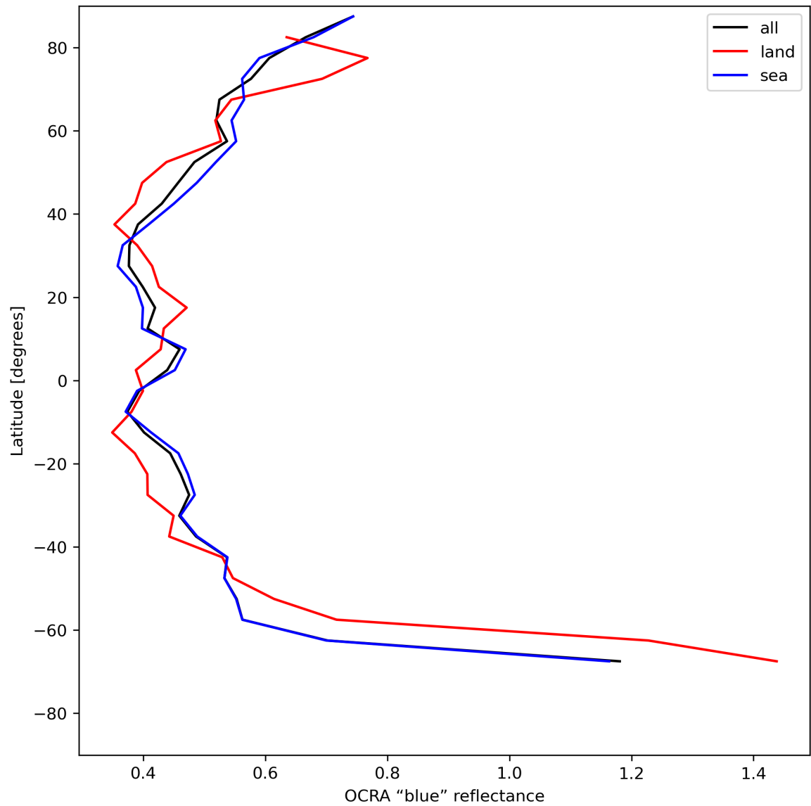
Figure 35: Zonal average of “OCRA “blue” reflectance” for 2023-07-15 to 2023-07-17.
