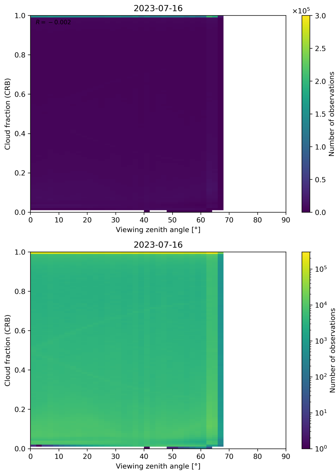
Figure 109: Scatter density plot of “Viewing zenith angle” against “Cloud fraction (CRB)” for 2023-07-15 to 2023-07-17.
