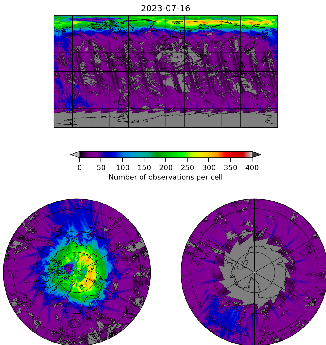
Figure 21: Map of the number of observations for 2023-07-15 to 2023-07-17
