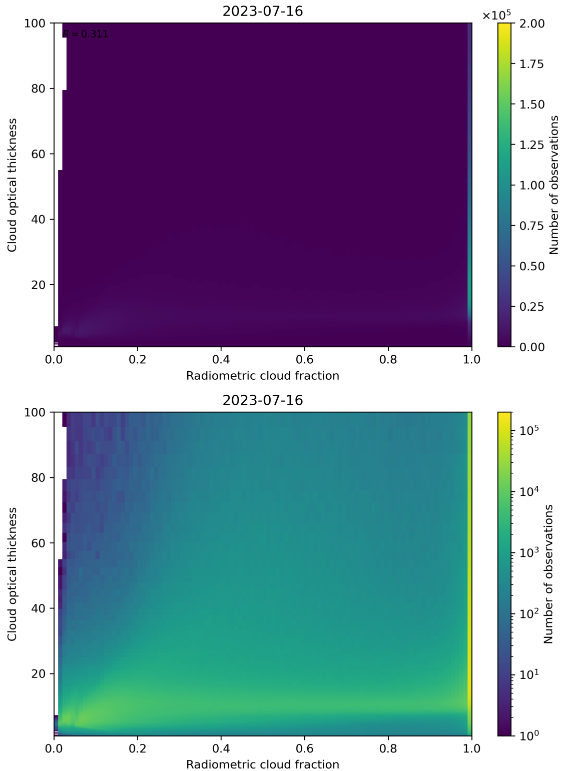
Figure 75: Scatter density plot of “Radiometric cloud fraction” against “Cloud optical thickness” for 2023-07-15 to 2023-07-17.
