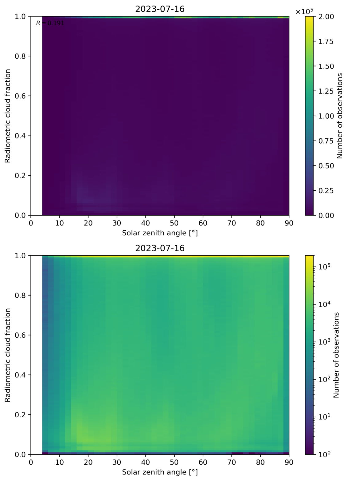
Figure 99: Scatter density plot of “Solar zenith angle” against “Radiometric cloud fraction” for 2023-07-15 to 2023-07-17.
