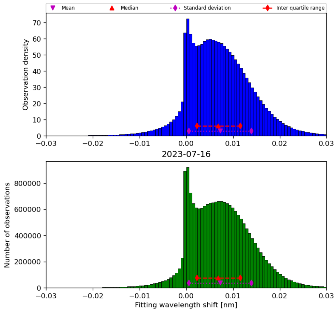
Figure 49: Histogram of “Fitting wavelength shift” for 2023-07-15 to 2023-07-17
