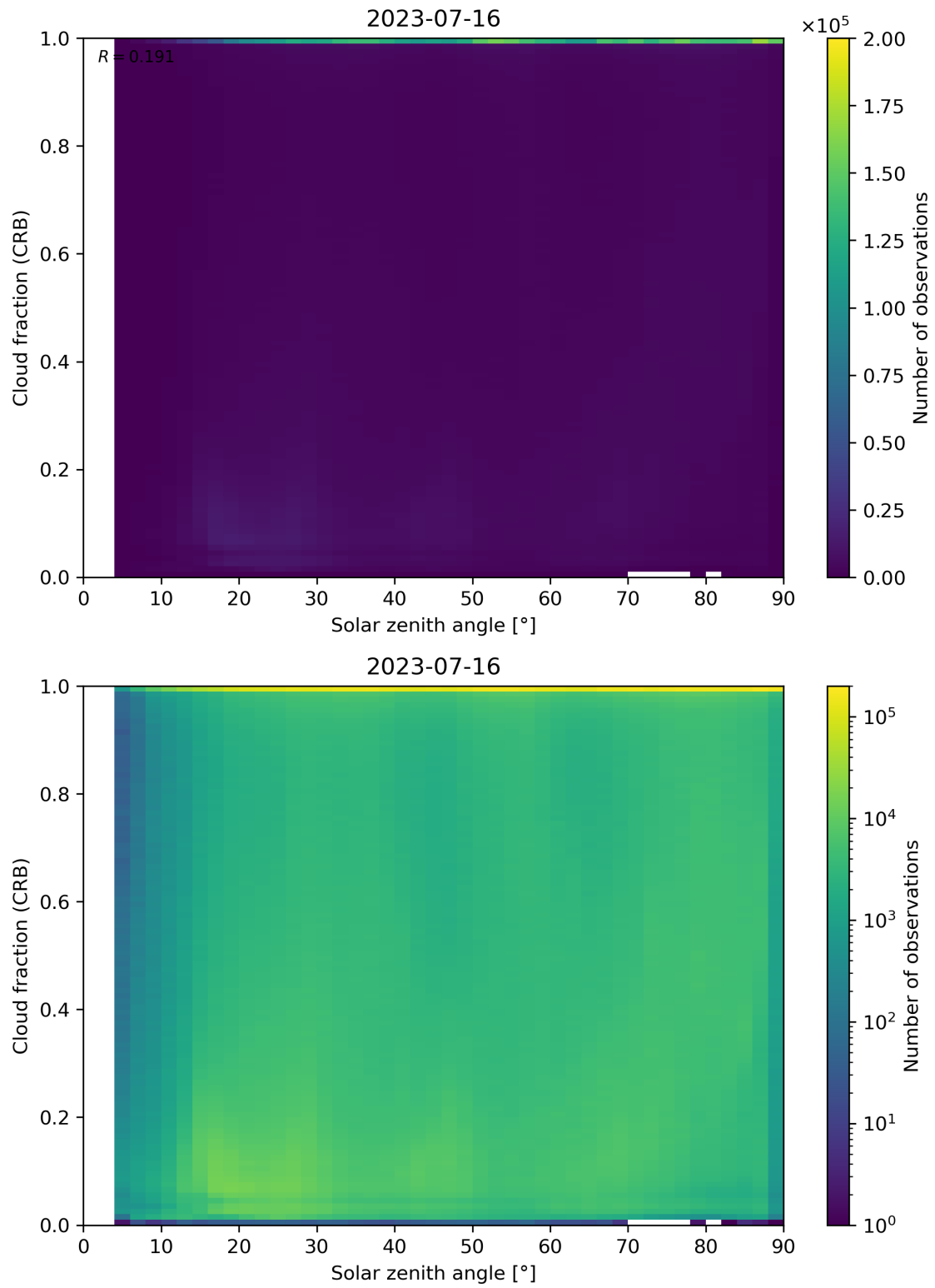
Figure 101: Scatter density plot of “Solar zenith angle” against “Cloud fraction (CRB)” for 2023-07-15 to 2023-07-17.
