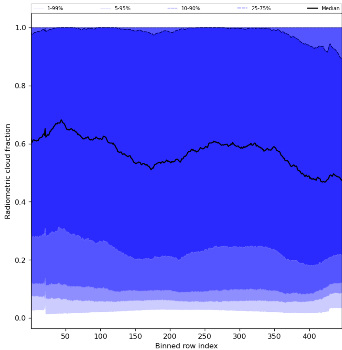
Figure 55: Along track statistics of “Radiometric cloud fraction” for 2023-07-15 to 2023-07-17
