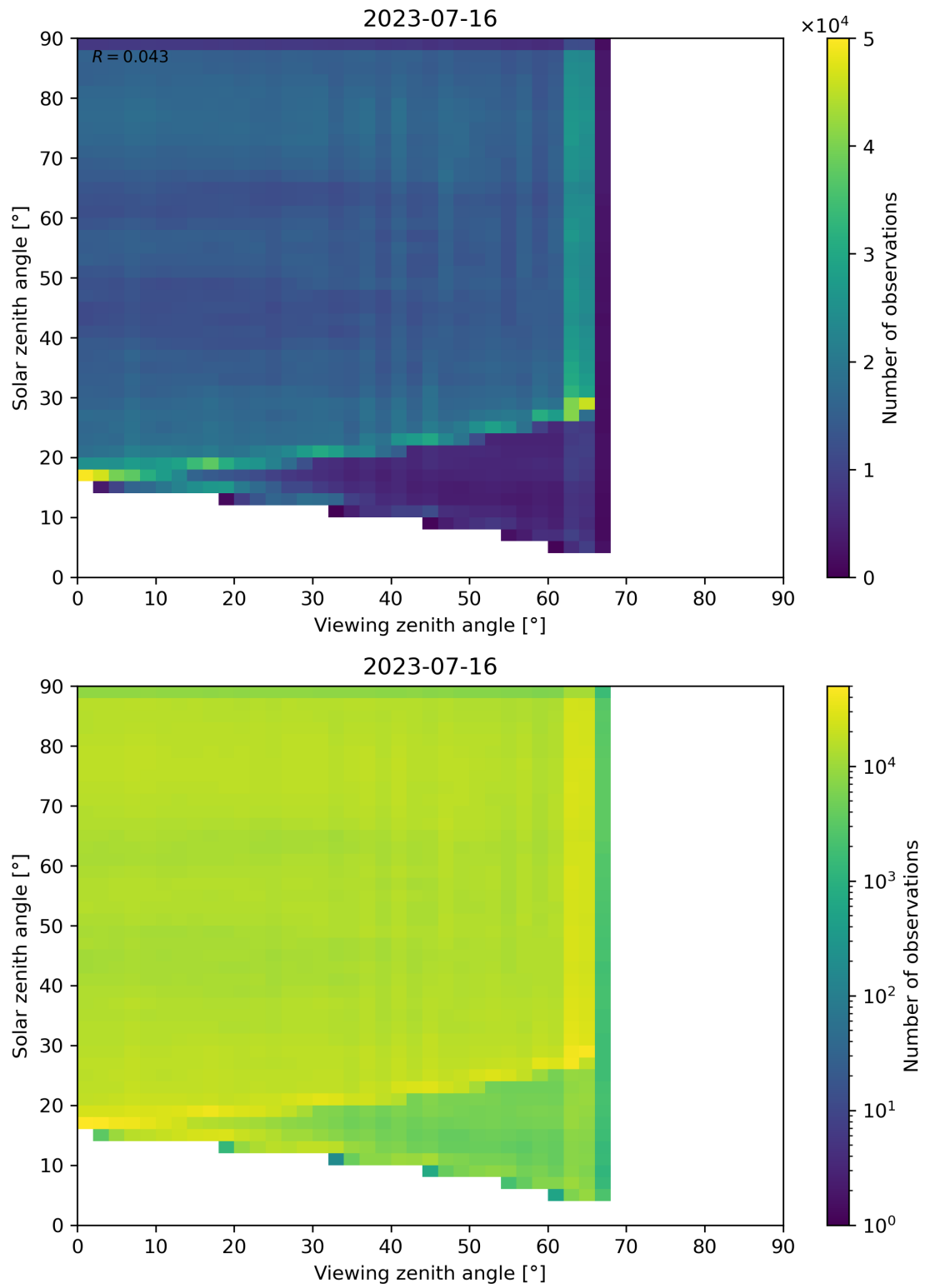
Figure 114: Scatter density plot of “Viewing zenith angle” against “Solar zenith angle” for 2023-07-15 to 2023-07-17.
