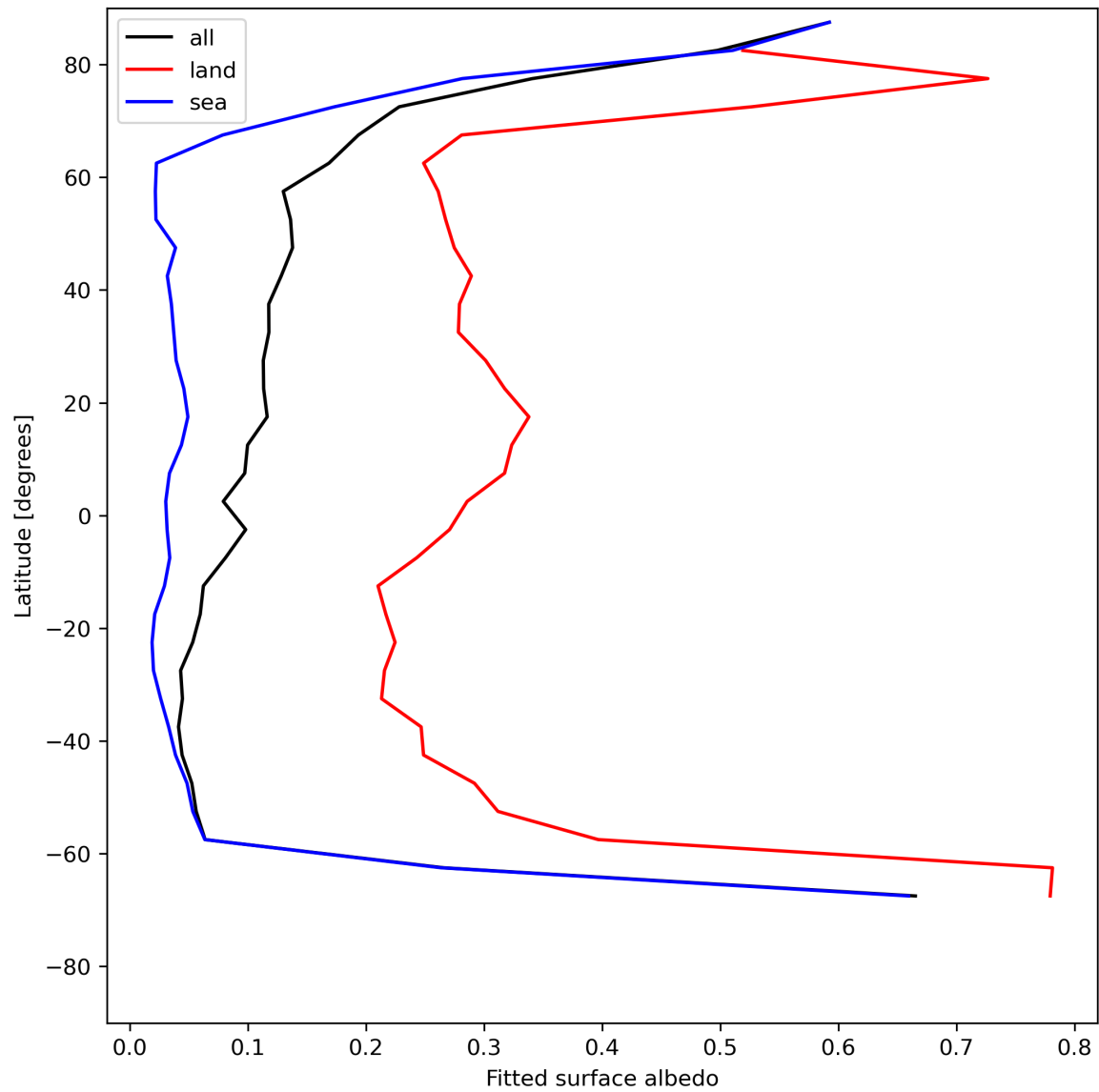
Figure 29: Zonal average of “Fitted surface albedo” for 2023-07-15 to 2023-07-17.
