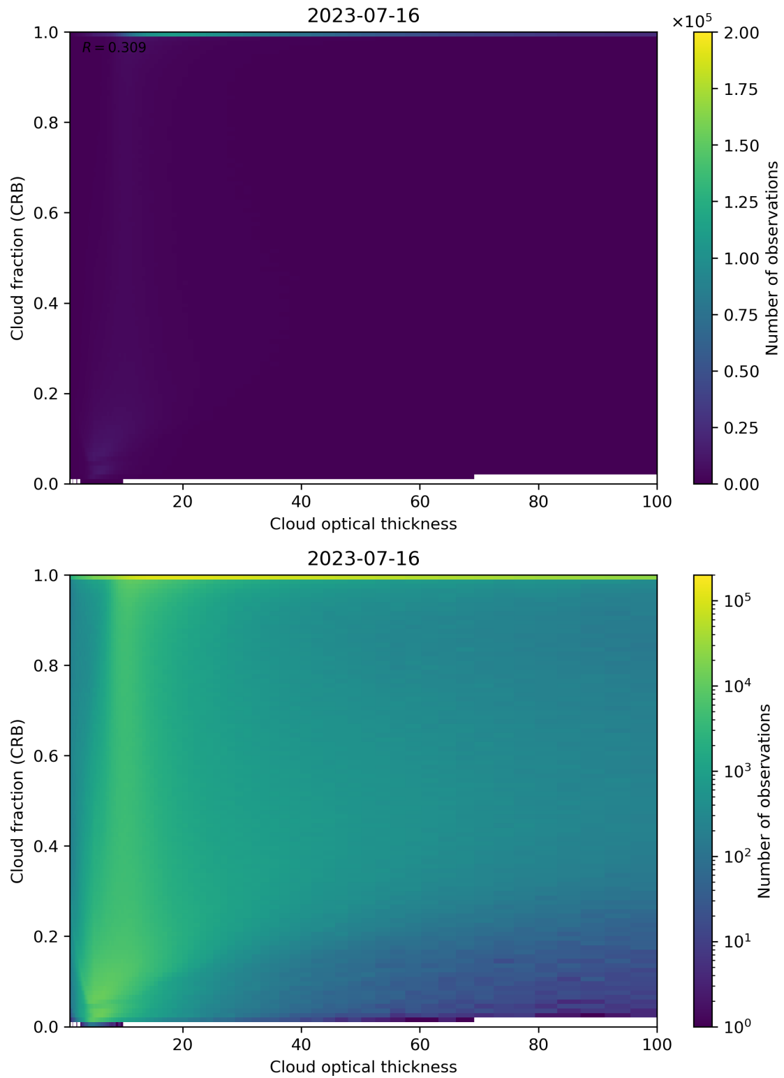
Figure 84: Scatter density plot of “Cloud optical thickness” against “Cloud fraction (CRB)” for 2023-07-15 to 2023-07-17.
