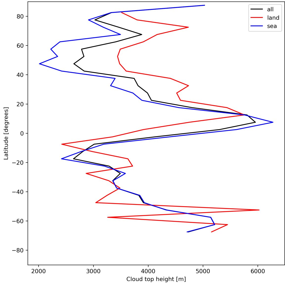
Figure 24: Zonal average of “Cloud top height” for 2023-07-15 to 2023-07-17.
