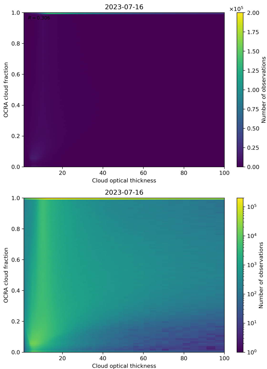
Figure 83: Scatter density plot of “Cloud optical thickness” against “OCRA cloud fraction” for 2023-07-15 to 2023-07-17.
