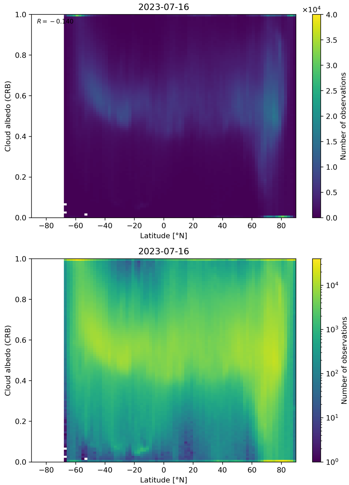
Figure 91: Scatter density plot of “Latitude” against “Cloud albedo (CRB)” for 2023-07-15 to 2023-07-17.
