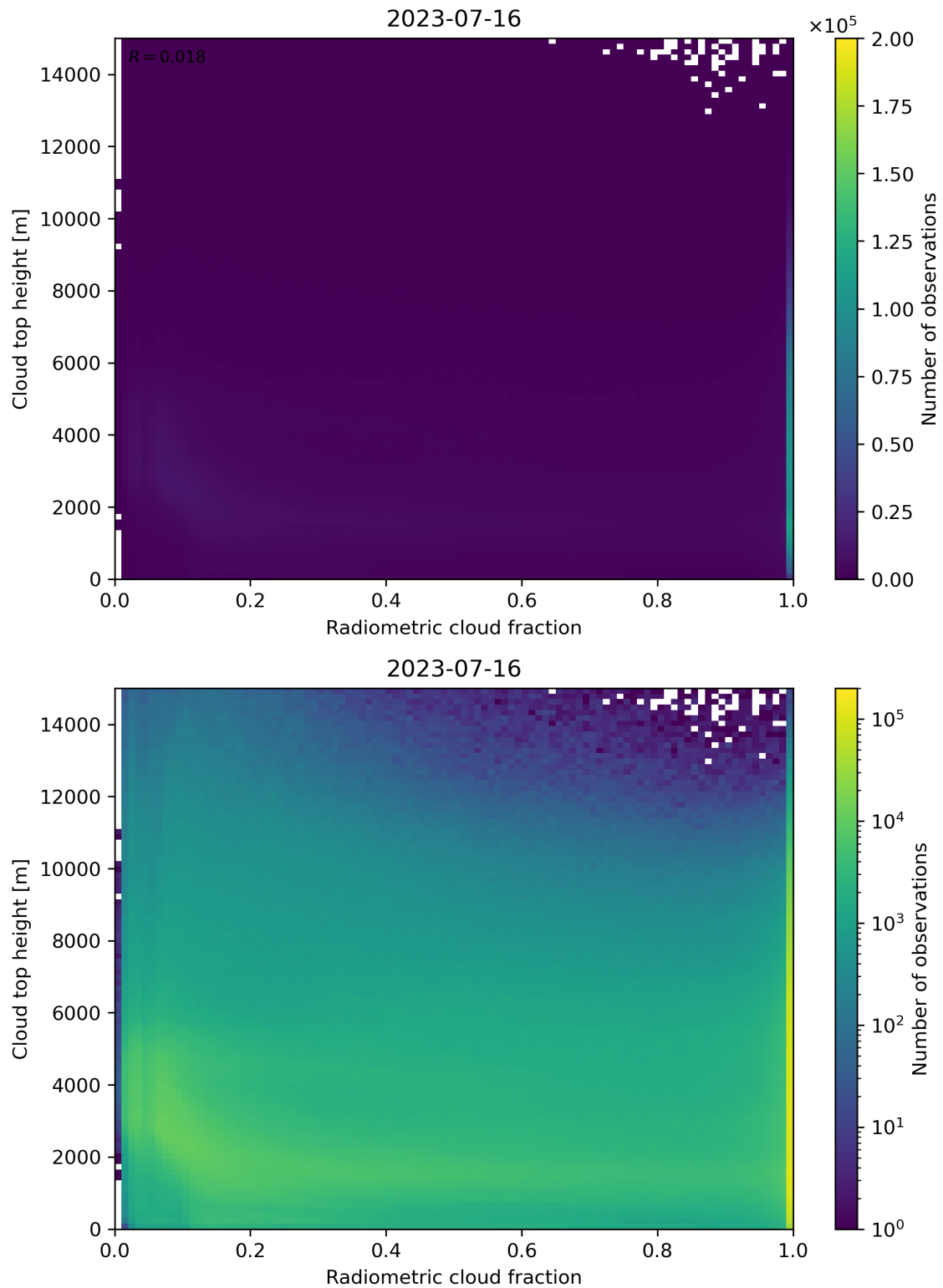
Figure 76: Scatter density plot of “Radiometric cloud fraction” against “Cloud top height” for 2023-07-15 to 2023-07-17.
