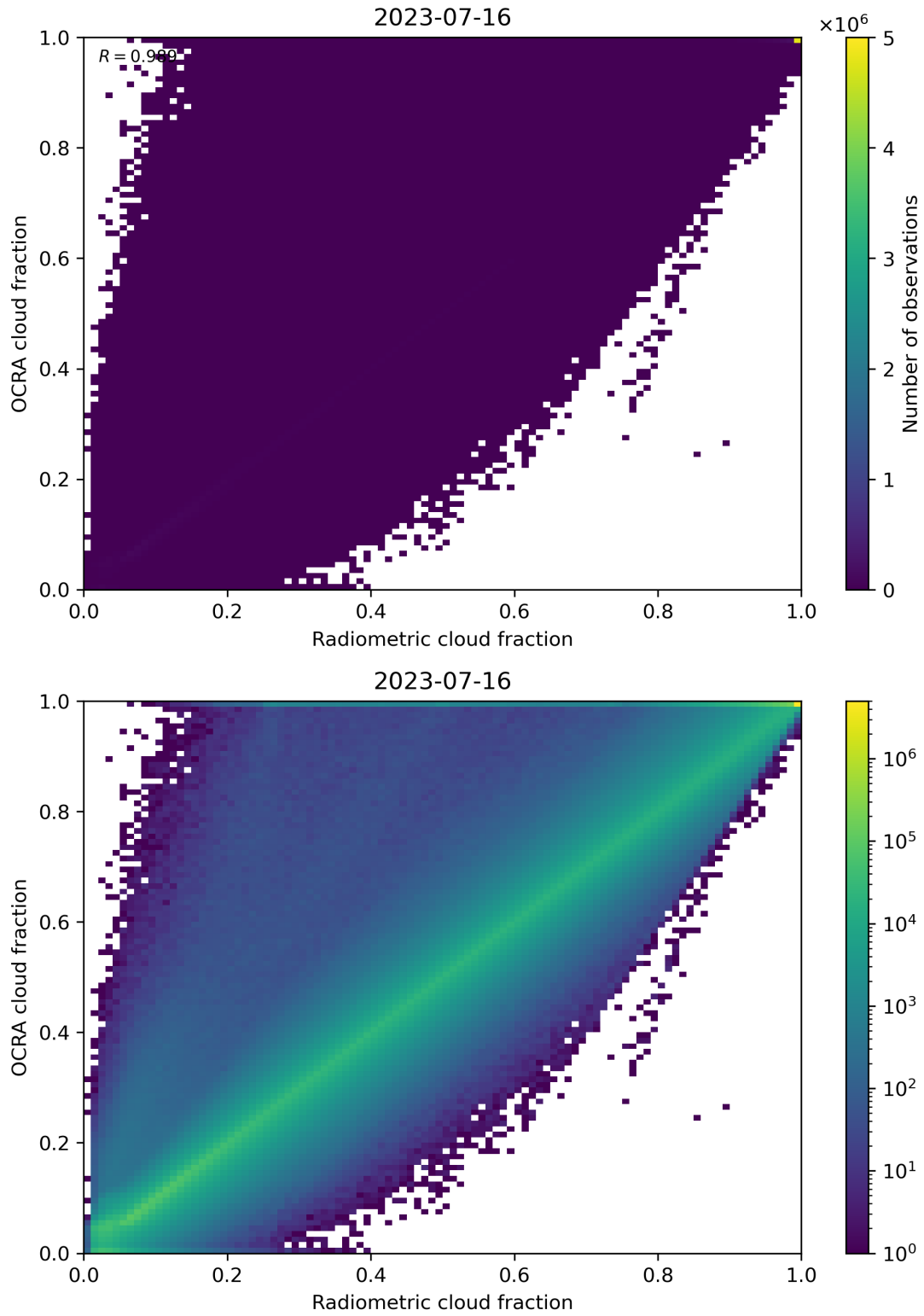
Figure 72: Scatter density plot of “Radiometric cloud fraction” against “OCRA cloud fraction” for 2023-07-15 to 2023-07-17.
