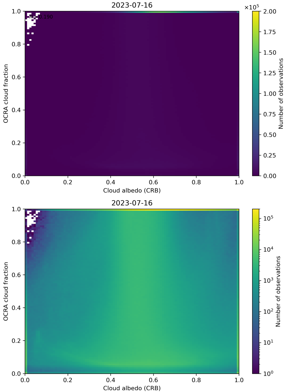
Figure 70: Scatter density plot of “Cloud albedo (CRB)” against “OCRA cloud fraction” for 2023-07-15 to 2023-07-17.
