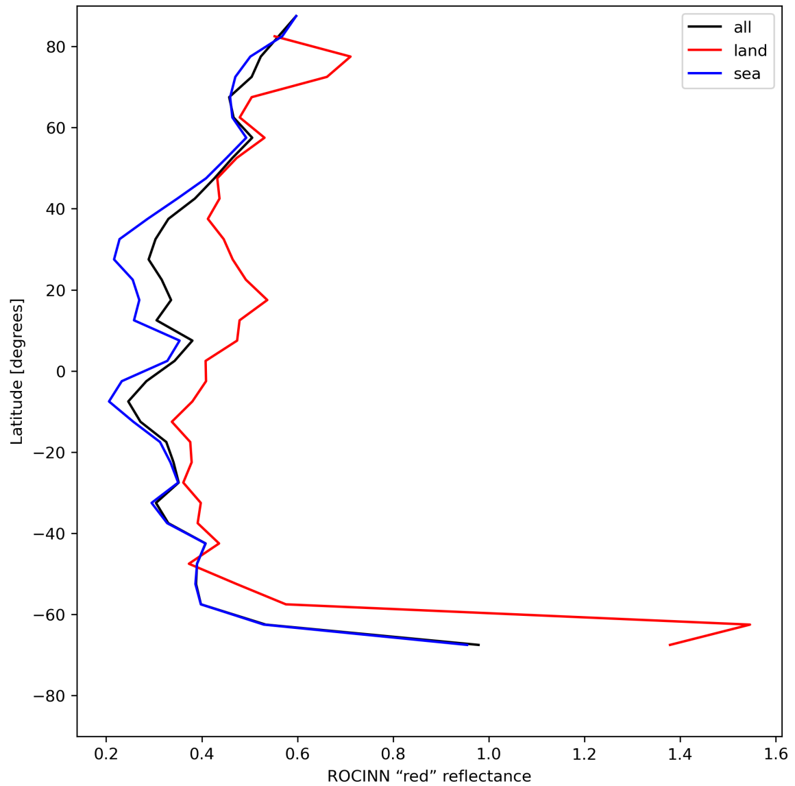
Figure 37: Zonal average of “ROCINN “red” reflectance” for 2023-07-15 to 2023-07-17.
