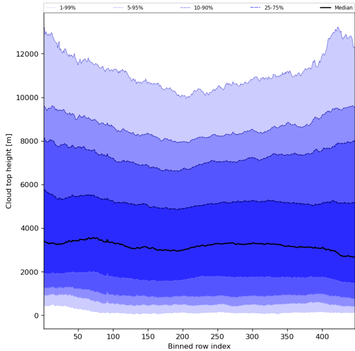
Figure 56: Along track statistics of “Cloud top height” for 2023-07-15 to 2023-07-17
