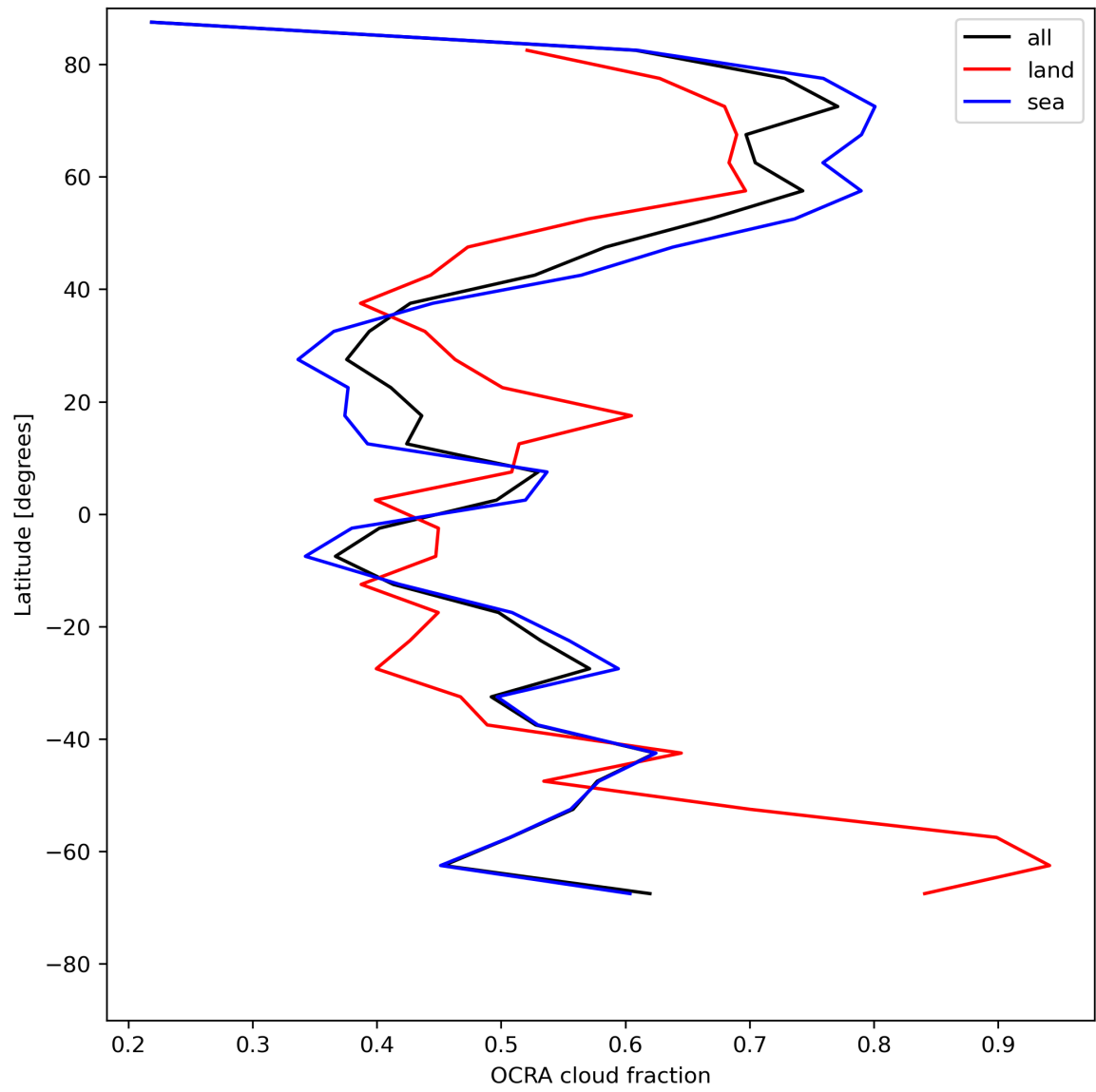
Figure 34: Zonal average of “OCRA cloud fraction” for 2023-07-15 to 2023-07-17.
