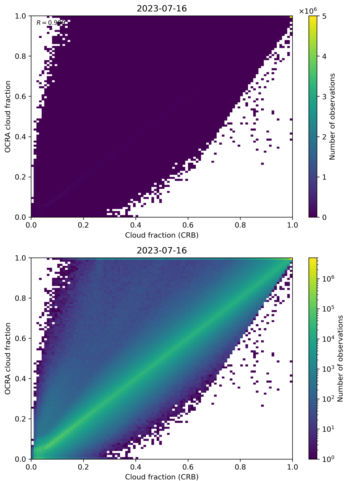
Figure 78: Scatter density plot of “Cloud fraction (CRB)” against “OCRA cloud fraction” for 2023-07-15 to 2023-07-17.
