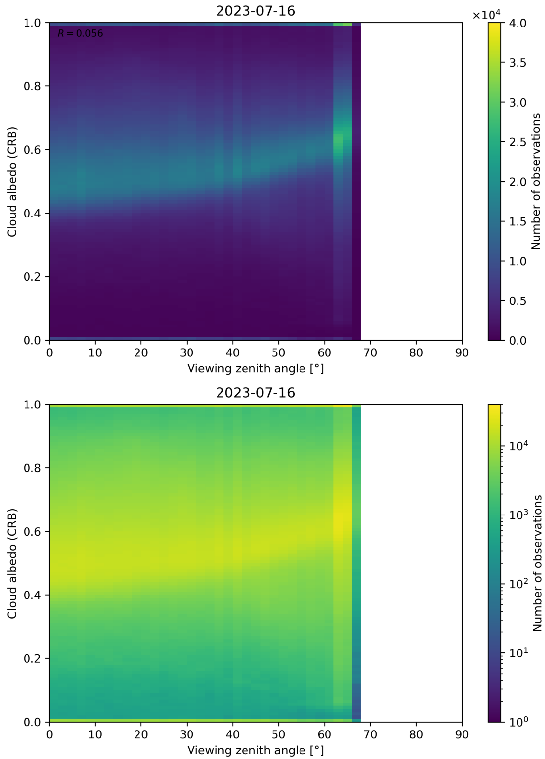
Figure 106: Scatter density plot of “Viewing zenith angle” against “Cloud albedo (CRB)” for 2023-07-15 to 2023-07-17.
