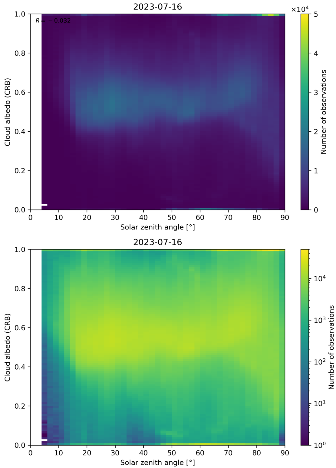
Figure 98: Scatter density plot of “Solar zenith angle” against “Cloud albedo (CRB)” for 2023-07-15 to 2023-07-17.
