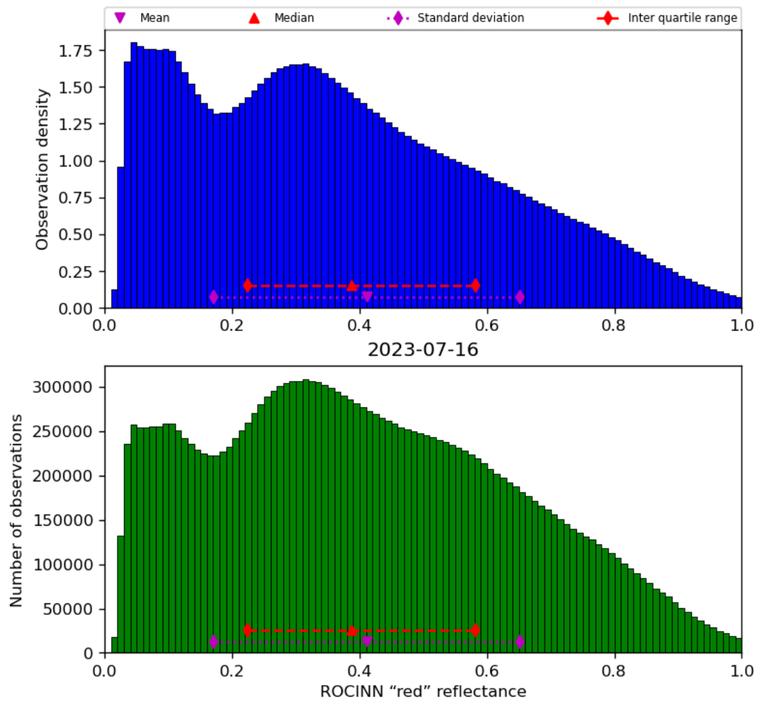
Figure 53: Histogram of “ROCINN “red” reflectance” for 2023-07-15 to 2023-07-17
