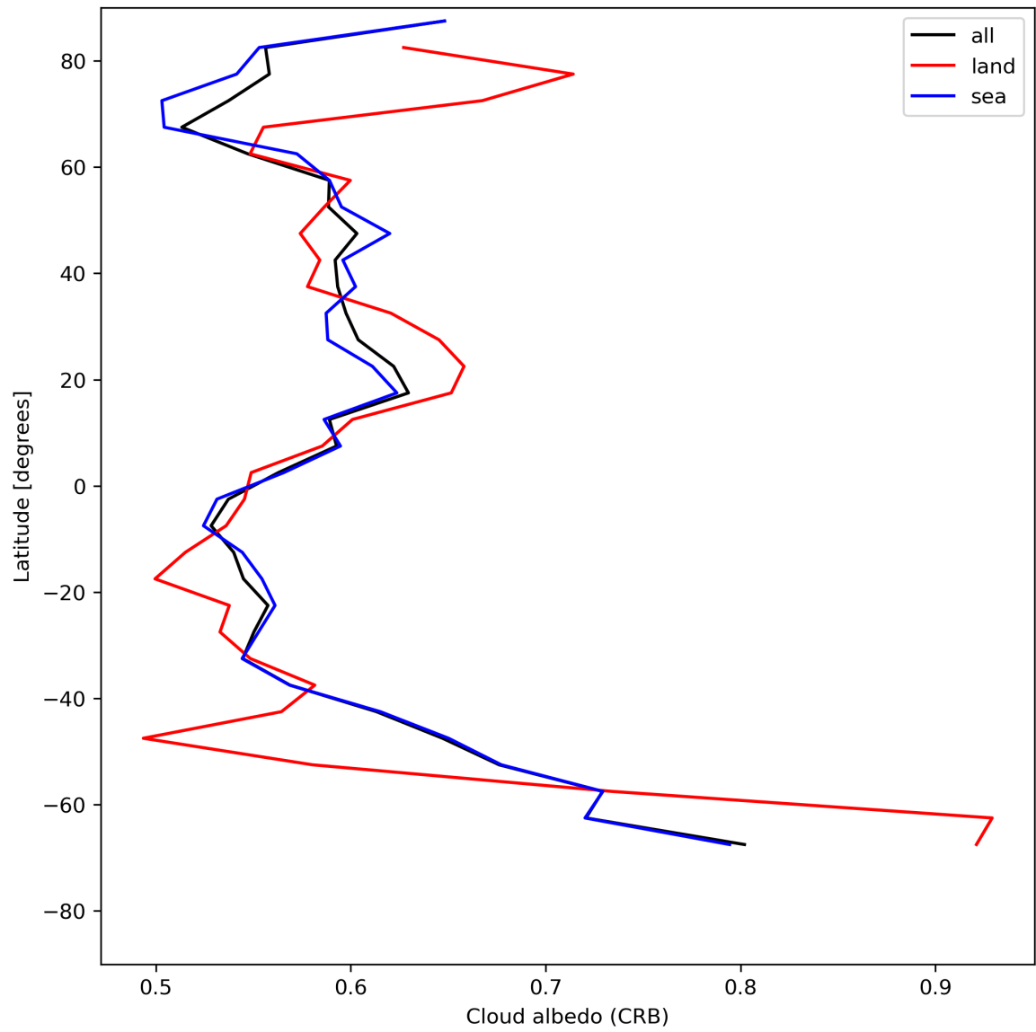
Figure 28: Zonal average of “Cloud albedo (CRB)” for 2023-07-15 to 2023-07-17.
