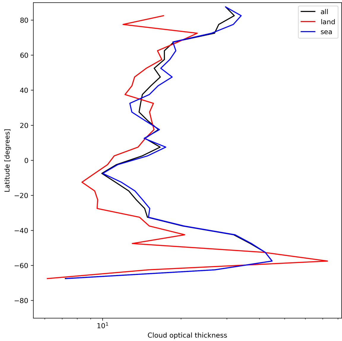
Figure 25: Zonal average of “Cloud optical thickness” for 2023-07-15 to 2023-07-17.
