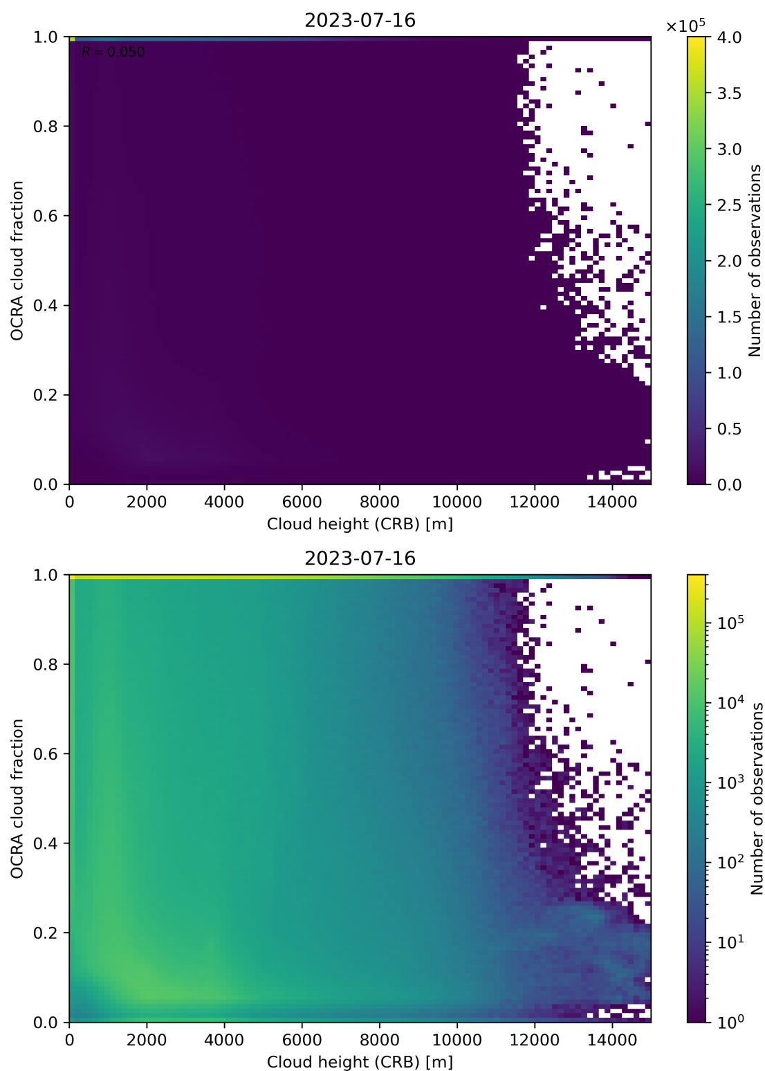
Figure 81: Scatter density plot of “Cloud height (CRB)” against “OCRA cloud fraction” for 2023-07-15 to 2023-07-17.
