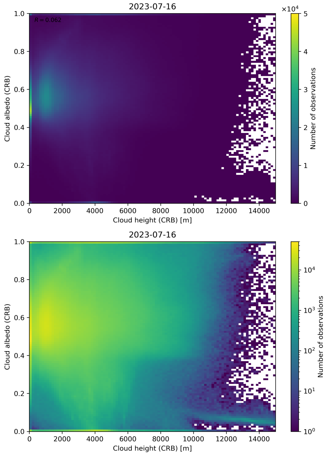
Figure 80: Scatter density plot of “Cloud height (CRB)” against “Cloud albedo (CRB)” for 2023-07-15 to 2023-07-17.
