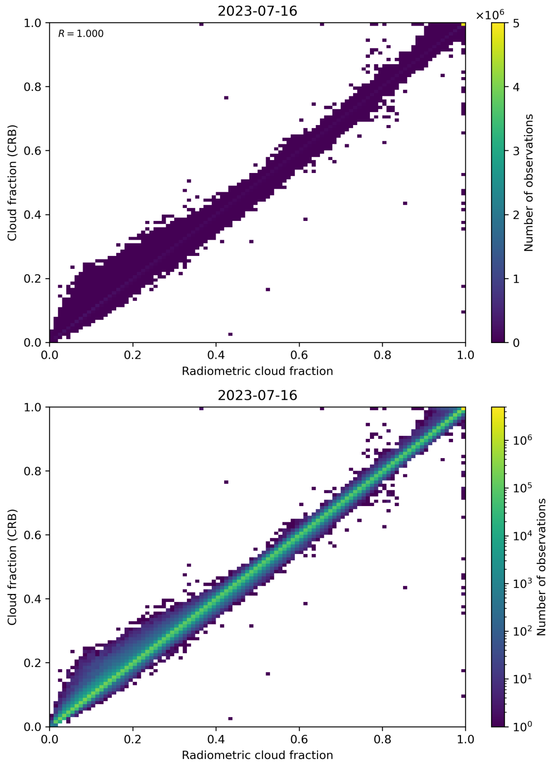
Figure 73: Scatter density plot of “Radiometric cloud fraction” against “Cloud fraction (CRB)” for 2023-07-15 to 2023-07-17.
