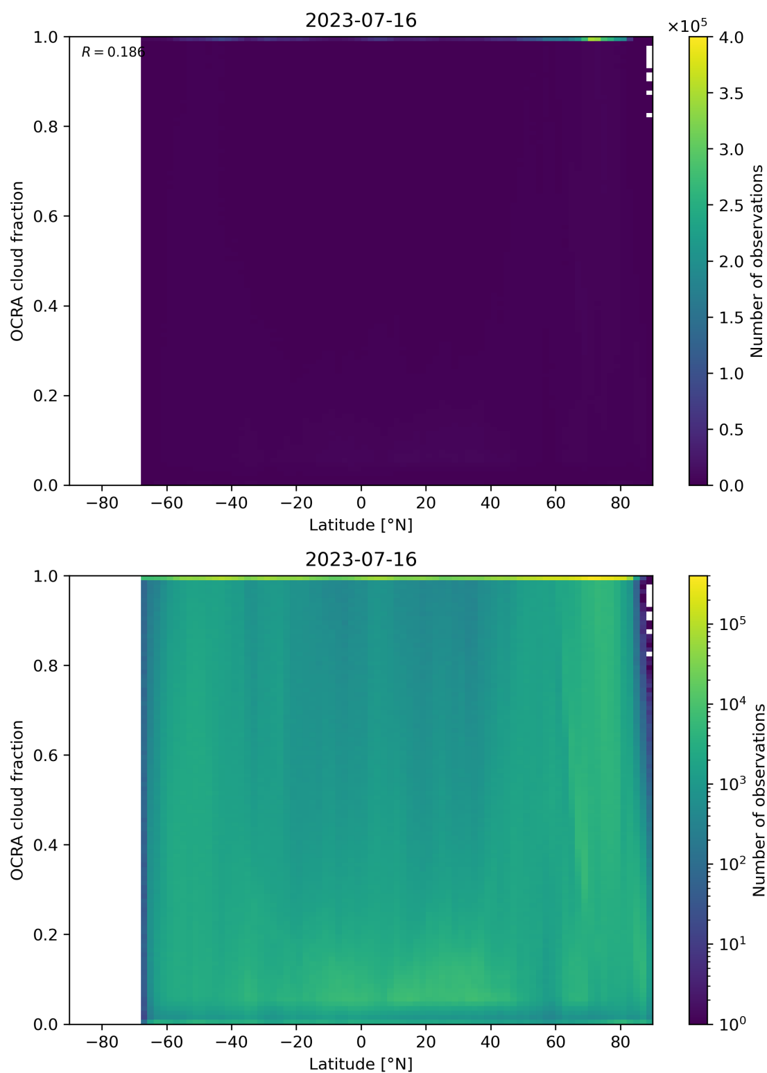
Figure 93: Scatter density plot of “Latitude” against “OCRA cloud fraction” for 2023-07-15 to 2023-07-17.
