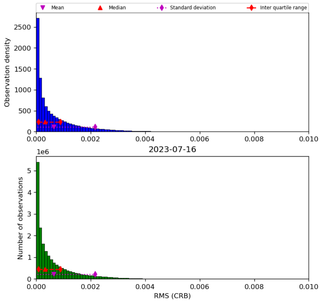
Figure 48: Histogram of “RMS (CRB)” for 2023-07-15 to 2023-07-17
