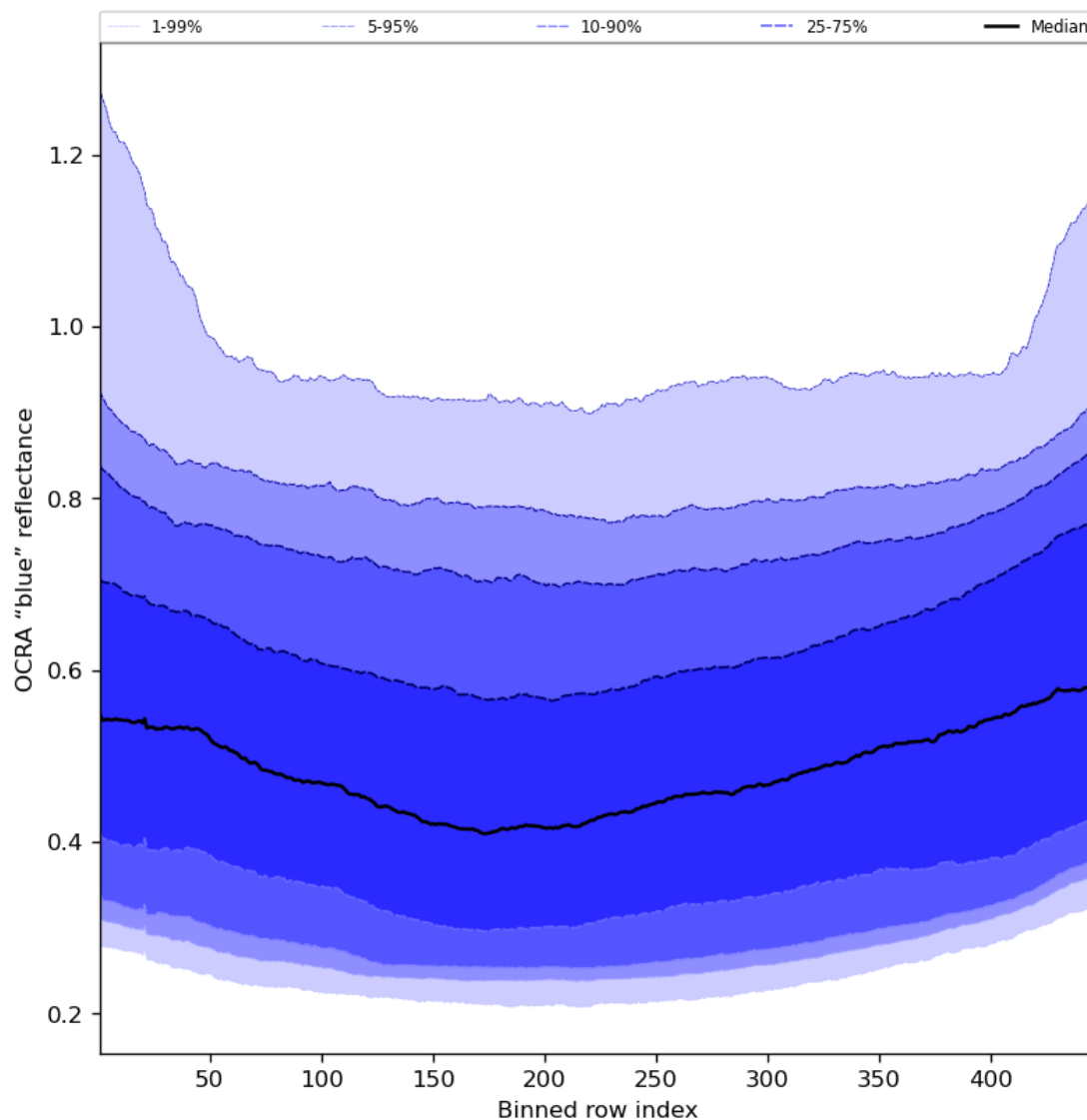
Figure 67: Along track statistics of “OCRA “blue” reflectance” for 2023-07-15 to 2023-07-17
