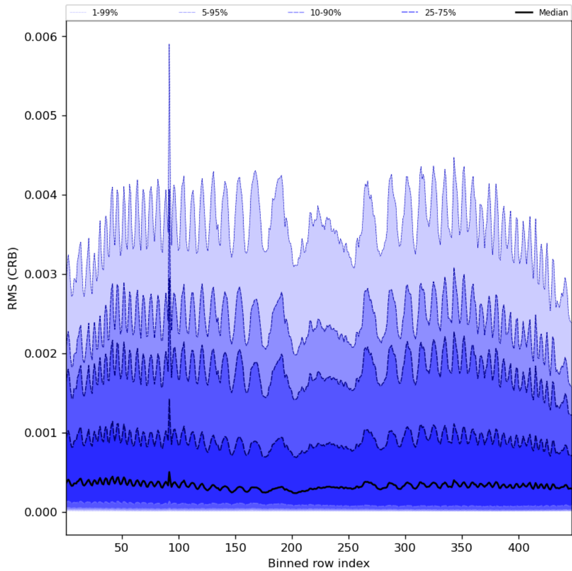
Figure 64: Along track statistics of “RMS (CRB)” for 2023-07-15 to 2023-07-17
