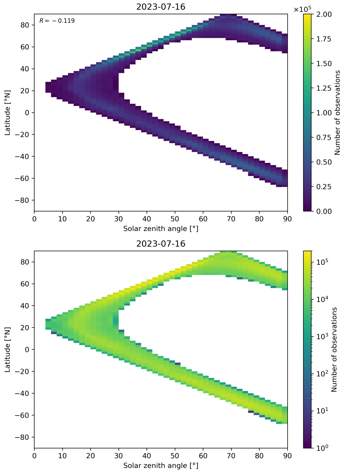
Figure 105: Scatter density plot of “Solar zenith angle” against “Latitude” for 2023-07-15 to 2023-07-17.
