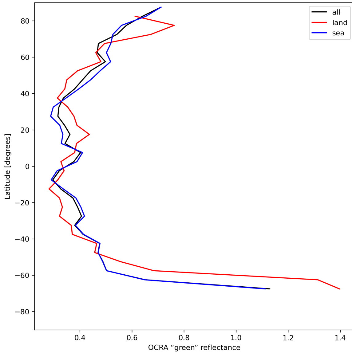
Figure 36: Zonal average of “OCRA “green” reflectance” for 2023-07-15 to 2023-07-17.
