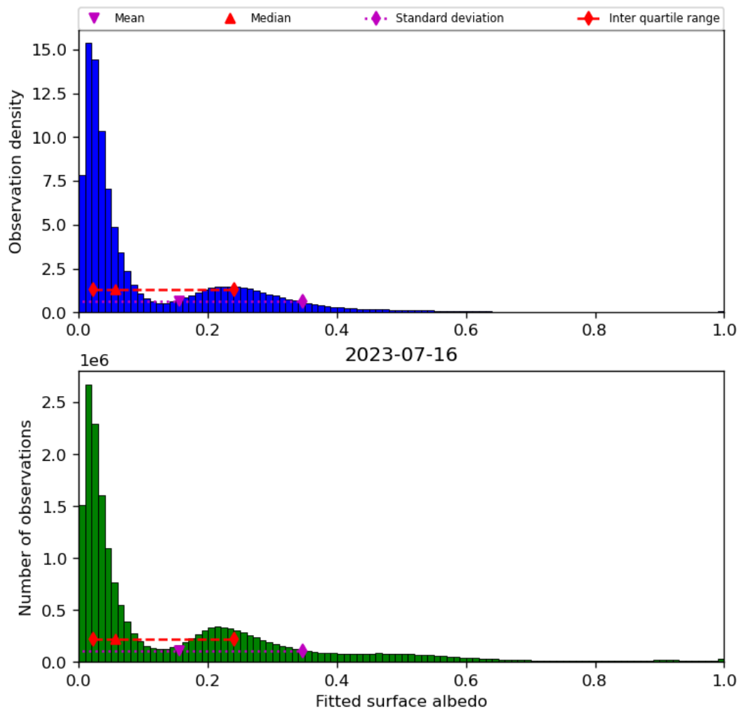
Figure 45: Histogram of “Fitted surface albedo” for 2023-07-15 to 2023-07-17
