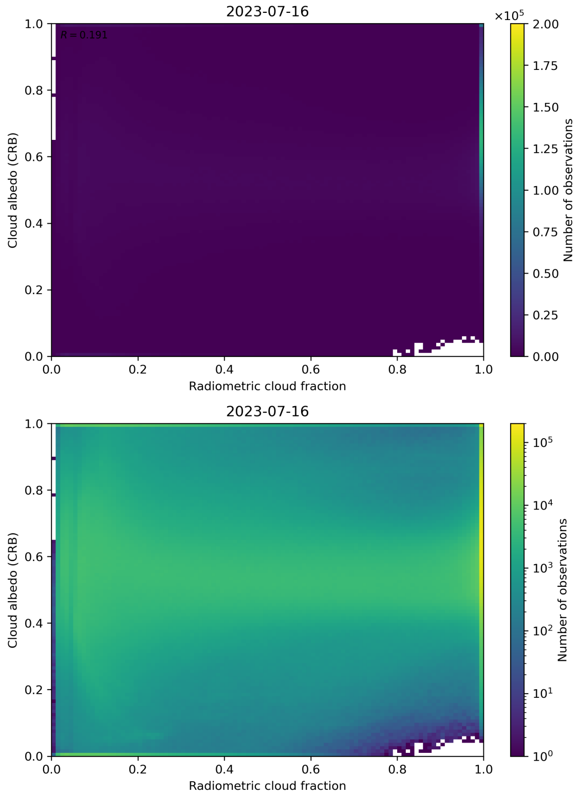
Figure 71: Scatter density plot of “Radiometric cloud fraction” against “Cloud albedo (CRB)” for 2023-07-15 to 2023-07-17.
