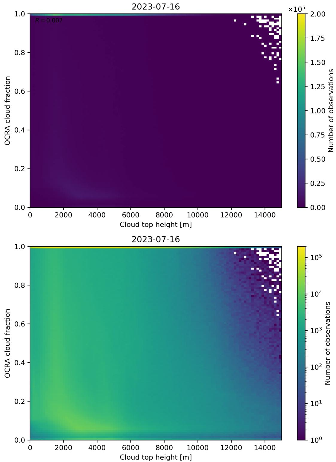
Figure 87: Scatter density plot of “Cloud top height” against “OCRA cloud fraction” for 2023-07-15 to 2023-07-17.
