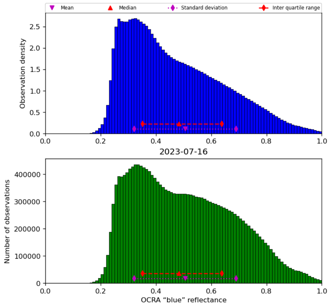
Figure 51: Histogram of “OCRA “blue” reflectance” for 2023-07-15 to 2023-07-17
