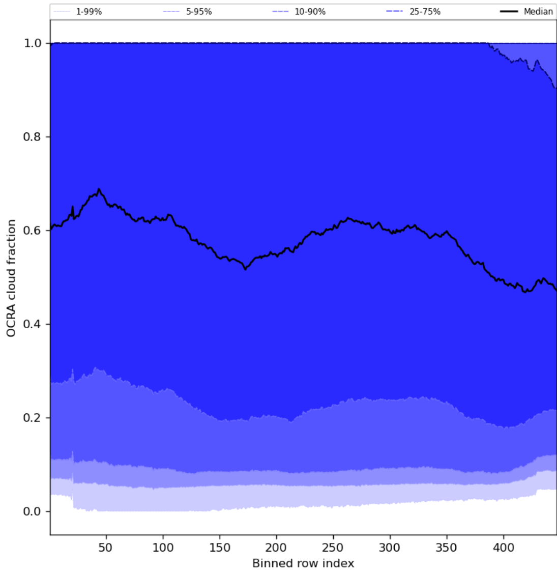
Figure 66: Along track statistics of “OCRA cloud fraction” for 2023-07-15 to 2023-07-17
