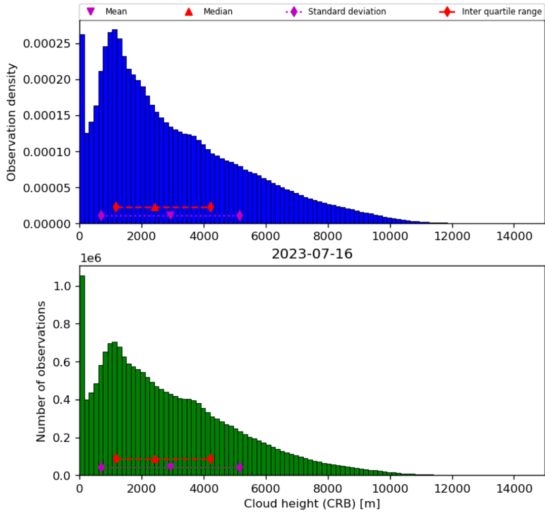
Figure 43: Histogram of “Cloud height (CRB)” for 2023-07-15 to 2023-07-17
