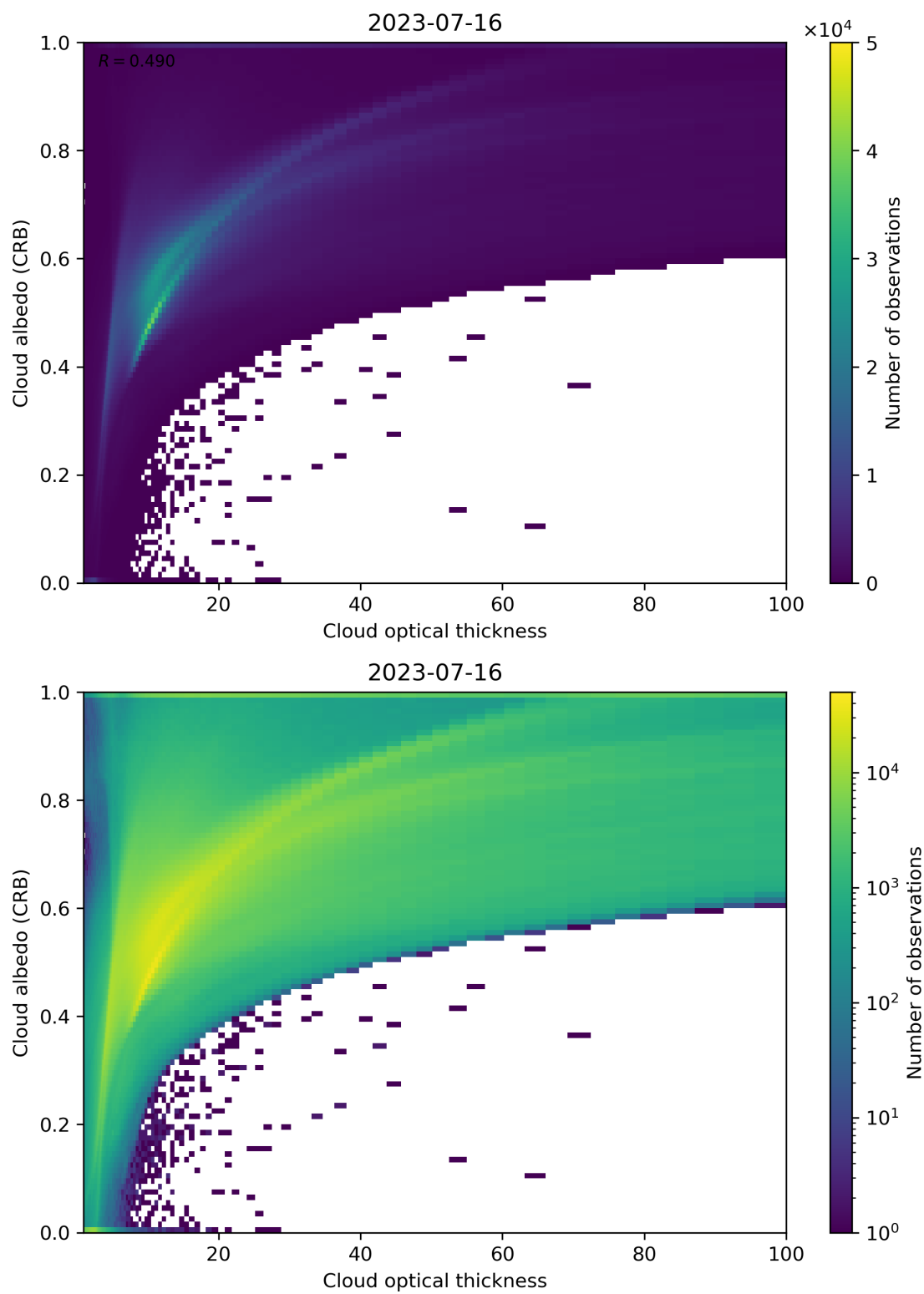
Figure 82: Scatter density plot of “Cloud optical thickness” against “Cloud albedo (CRB)” for 2023-07-15 to 2023-07-17.
