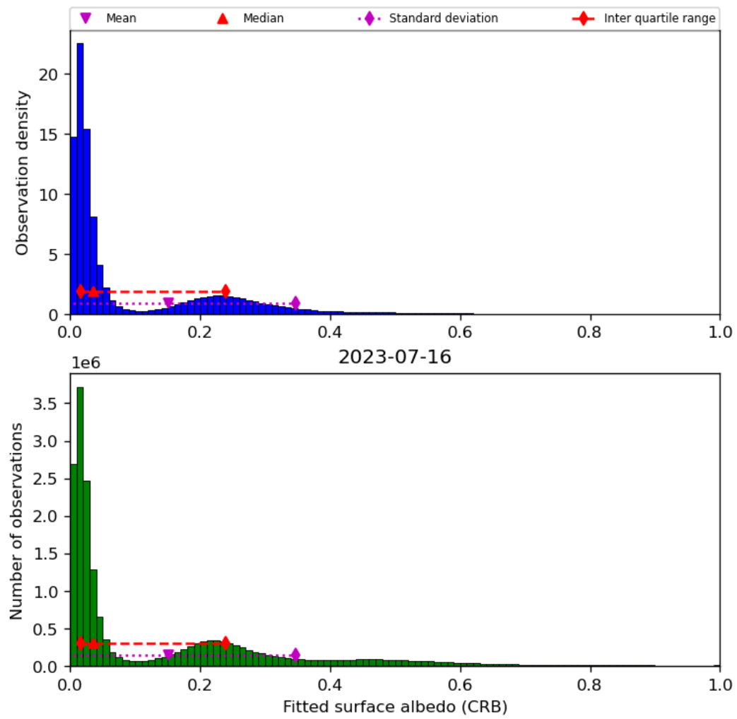
Figure 46: Histogram of “Fitted surface albedo (CRB)” for 2023-07-15 to 2023-07-17
