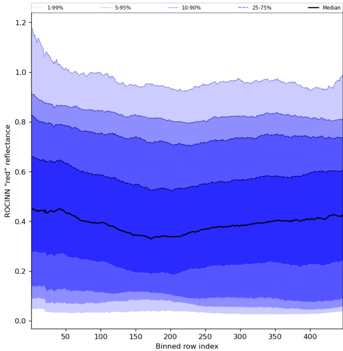
Figure 69: Along track statistics of "ROCINN "red" reflectance" for 2023-07-15 to 2023-07-17
