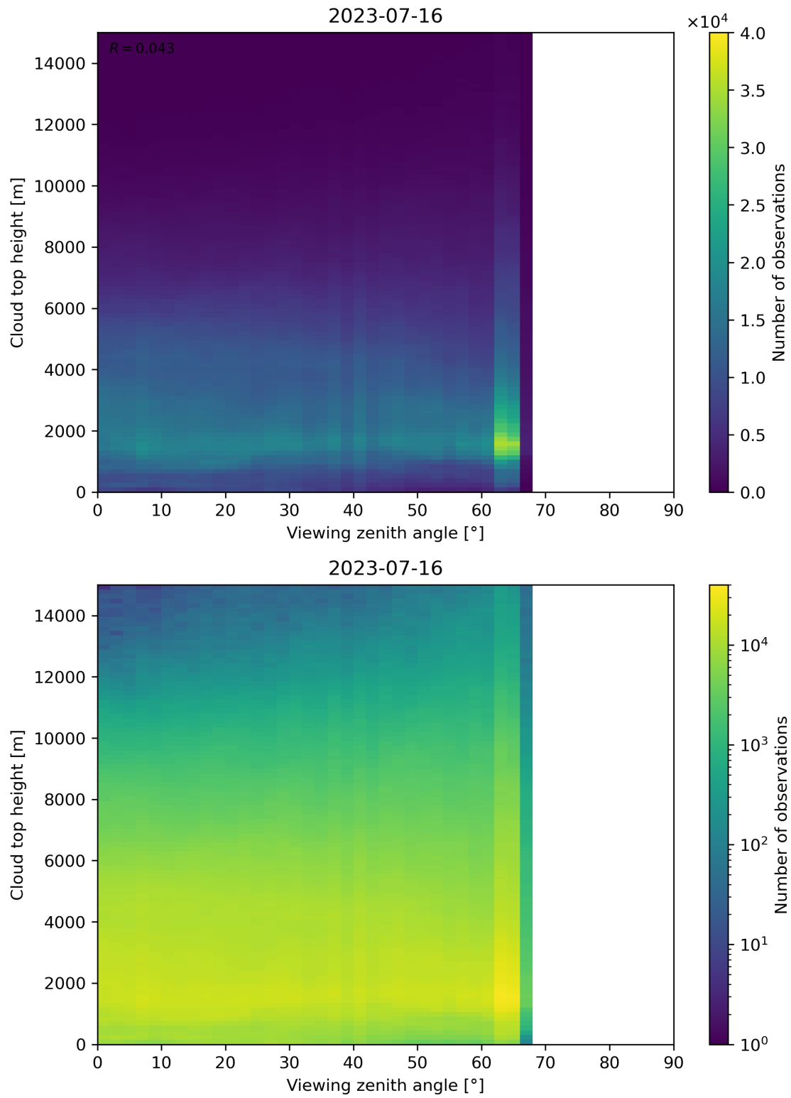
Figure 112: Scatter density plot of “Viewing zenith angle” against “Cloud top height” for 2023-07-15 to 2023-07-17.
