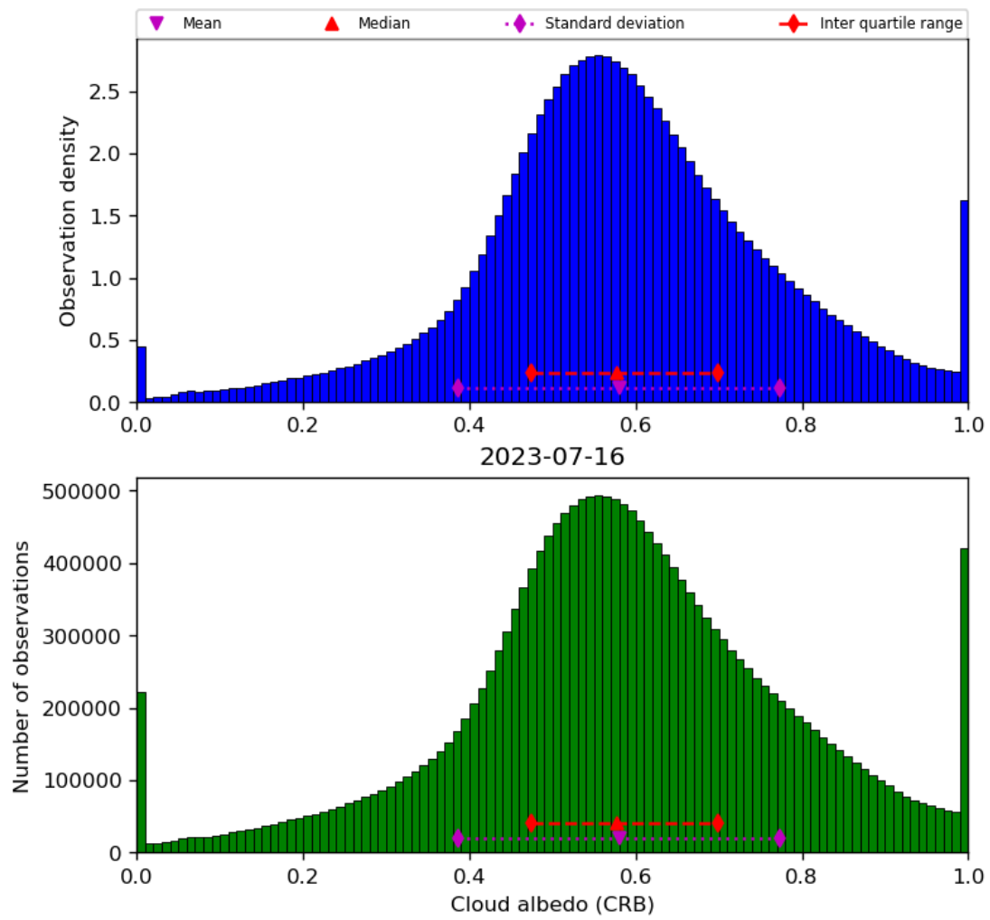
Figure 44: Histogram of “Cloud albedo (CRB)” for 2023-07-15 to 2023-07-17
