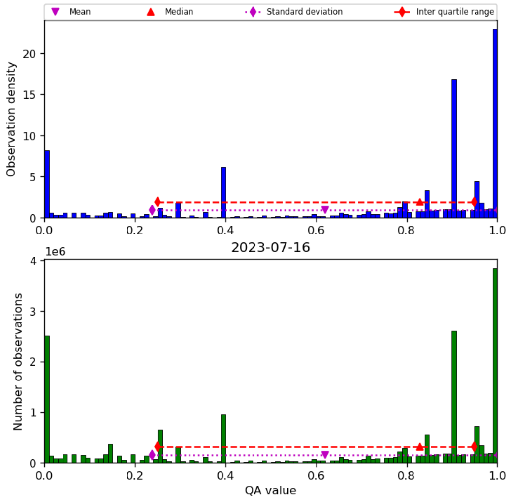
Figure 38: Histogram of “QA value” for 2023-07-15 to 2023-07-17
