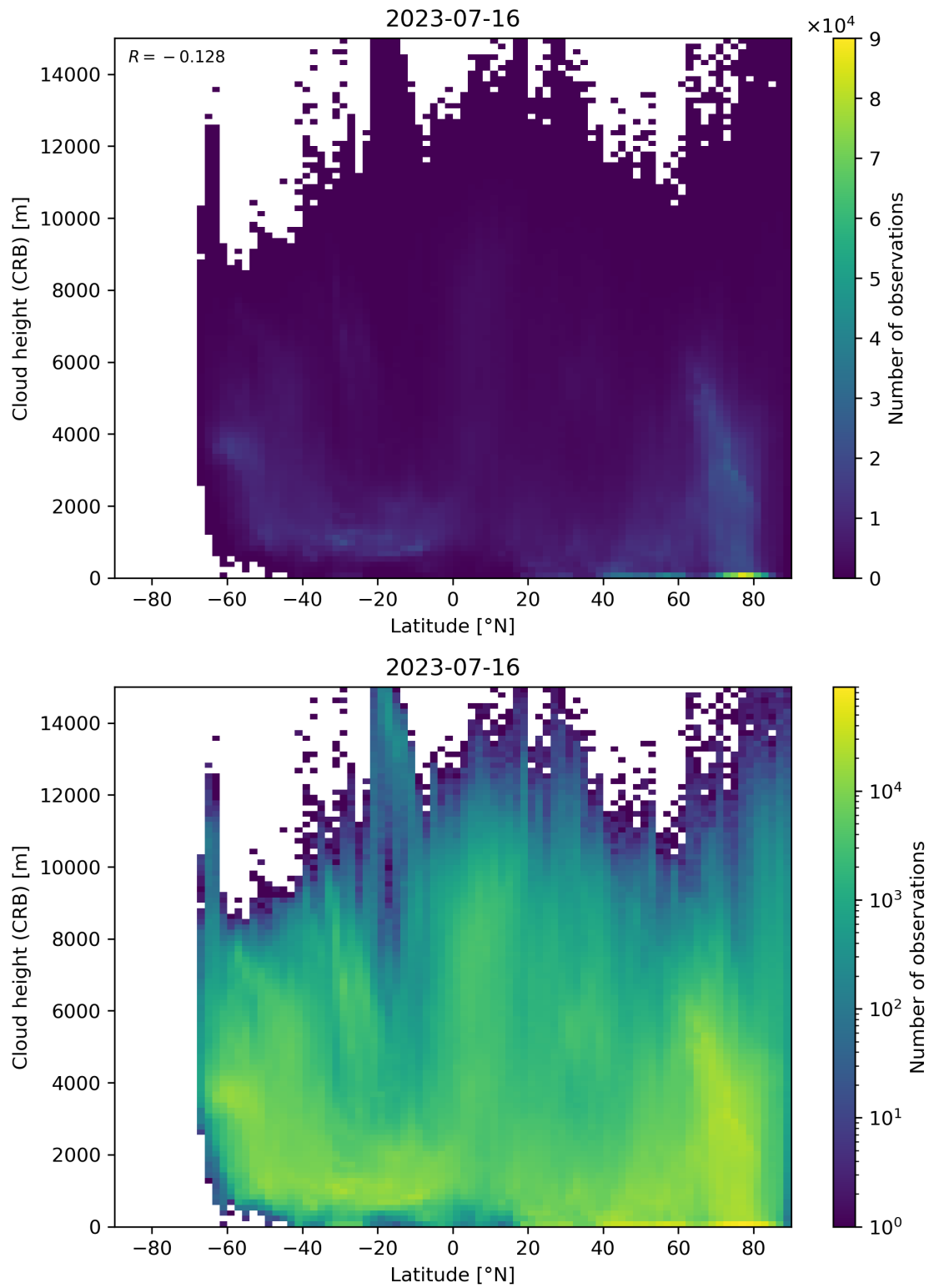
Figure 95: Scatter density plot of “Latitude” against “Cloud height (CRB)” for 2023-07-15 to 2023-07-17.
