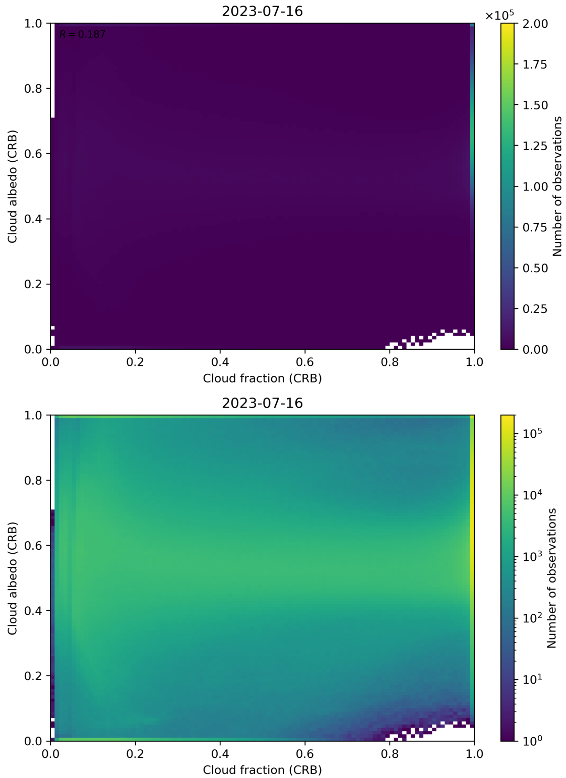
Figure 77: Scatter density plot of “Cloud fraction (CRB)” against “Cloud albedo (CRB)” for 2023-07-15 to 2023-07-17.
