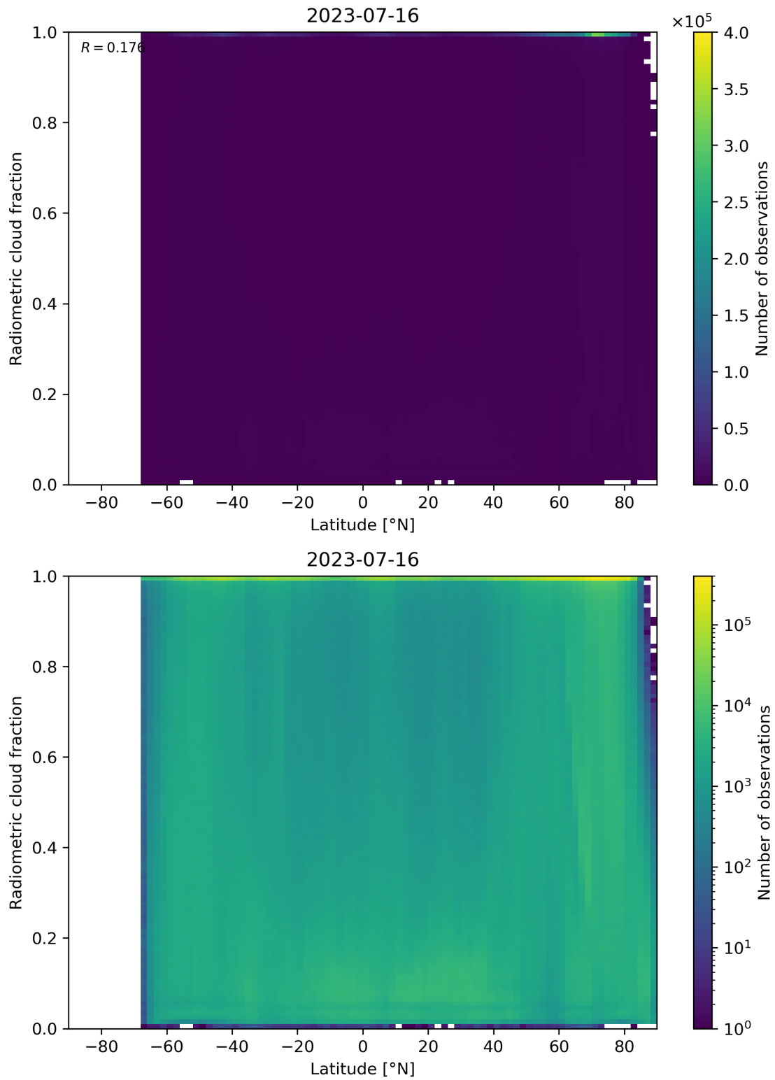
Figure 92: Scatter density plot of “Latitude” against “Radiometric cloud fraction” for 2023-07-15 to 2023-07-17.
