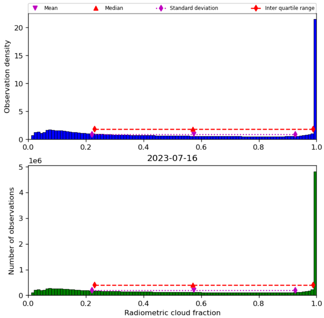
Figure 39: Histogram of “Radiometric cloud fraction” for 2023-07-15 to 2023-07-17
