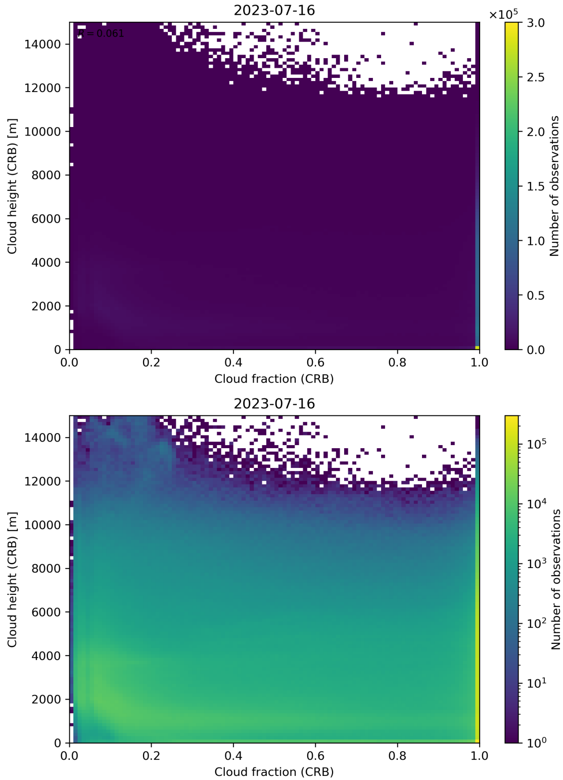
Figure 79: Scatter density plot of “Cloud fraction (CRB)” against “Cloud height (CRB)” for 2023-07-15 to 2023-07-17.
