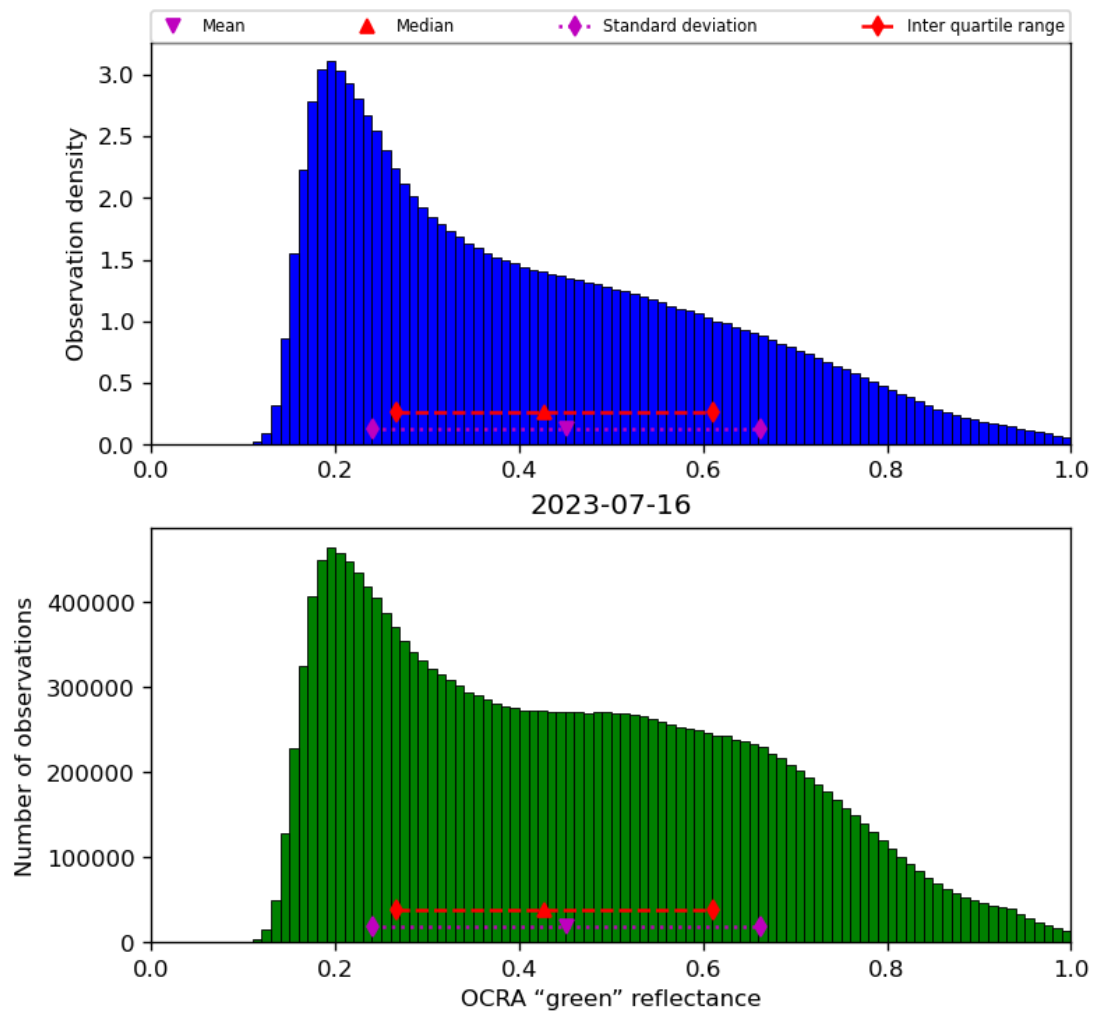
Figure 52: Histogram of “OCRA “green” reflectance” for 2023-07-15 to 2023-07-17
