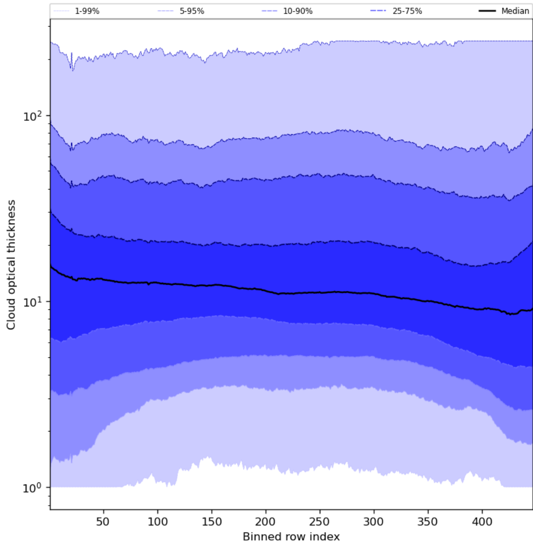
Figure 57: Along track statistics of “Cloud optical thickness” for 2023-07-15 to 2023-07-17
