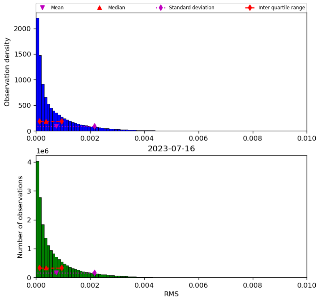
Figure 47: Histogram of “RMS” for 2023-07-15 to 2023-07-17
