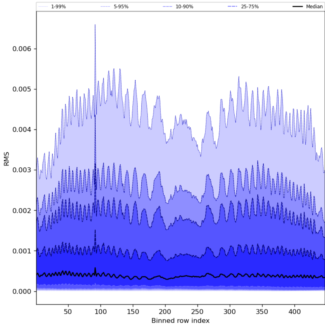
Figure 63: Along track statistics of “RMS” for 2023-07-15 to 2023-07-17
