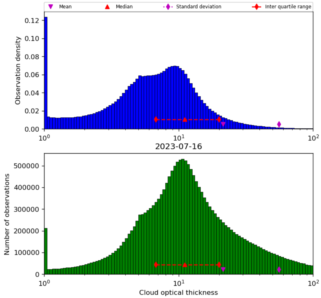
Figure 41: Histogram of “Cloud optical thickness” for 2023-07-15 to 2023-07-17
