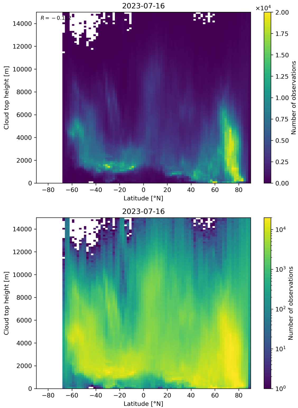
Figure 97: Scatter density plot of “Latitude” against “Cloud top height” for 2023-07-15 to 2023-07-17.
