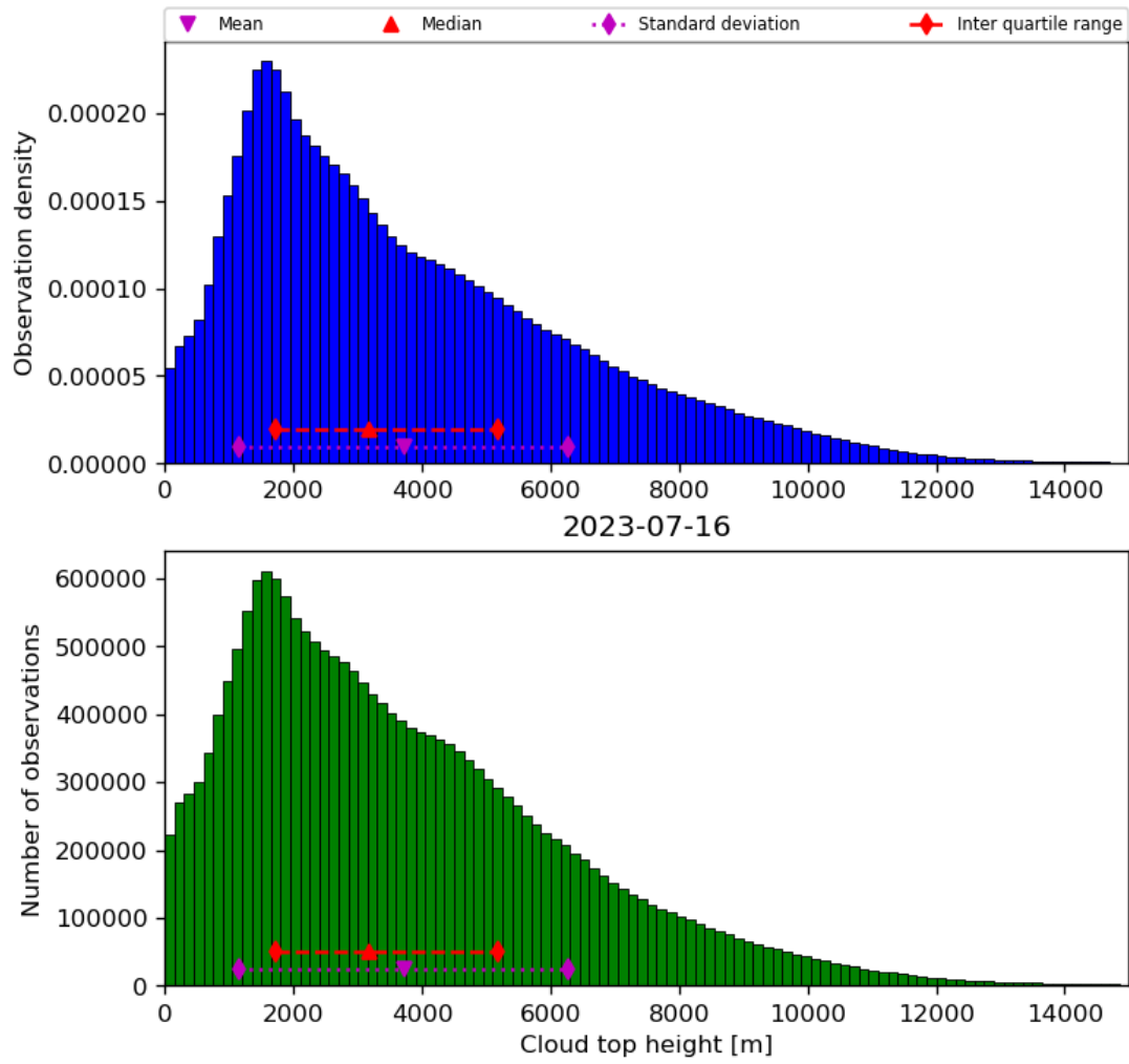
Figure 40: Histogram of “Cloud top height” for 2023-07-15 to 2023-07-17
