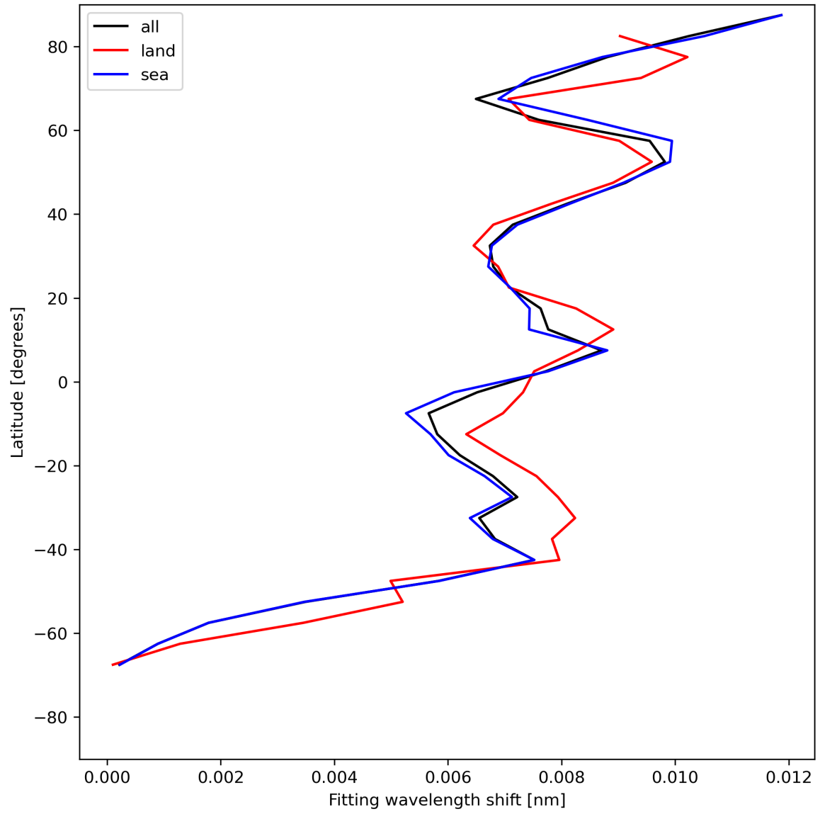
Figure 33: Zonal average of “Fitting wavelength shift” for 2023-07-15 to 2023-07-17.
