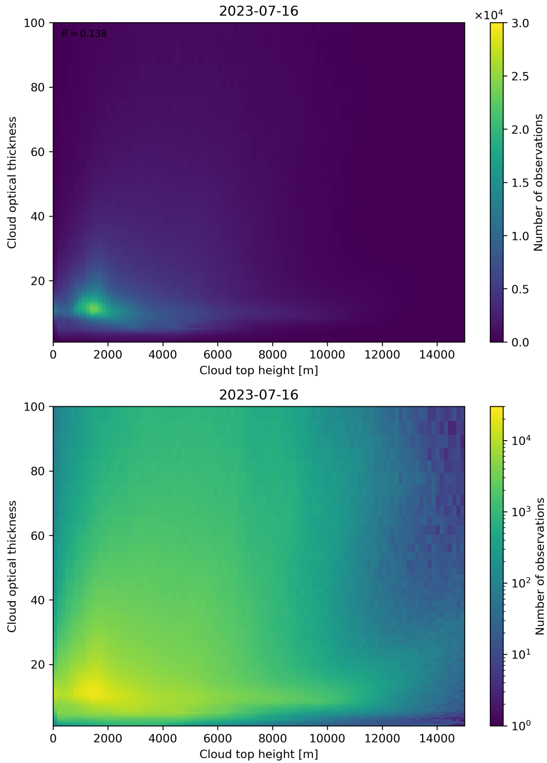
Figure 90: Scatter density plot of “Cloud top height” against “Cloud optical thickness” for 2023-07-15 to 2023-07-17.
