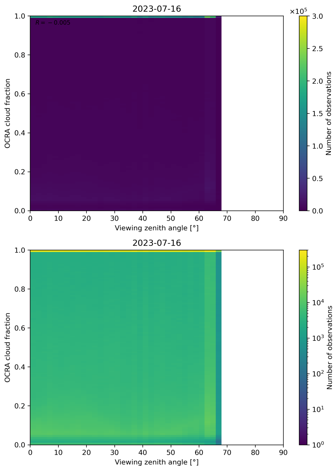
Figure 108: Scatter density plot of “Viewing zenith angle” against “OCRA cloud fraction” for 2023-07-15 to 2023-07-17.
