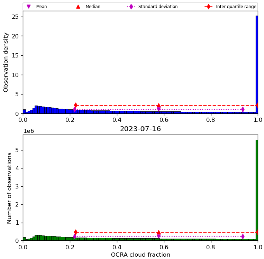
Figure 50: Histogram of “OCRA cloud fraction” for 2023-07-15 to 2023-07-17
