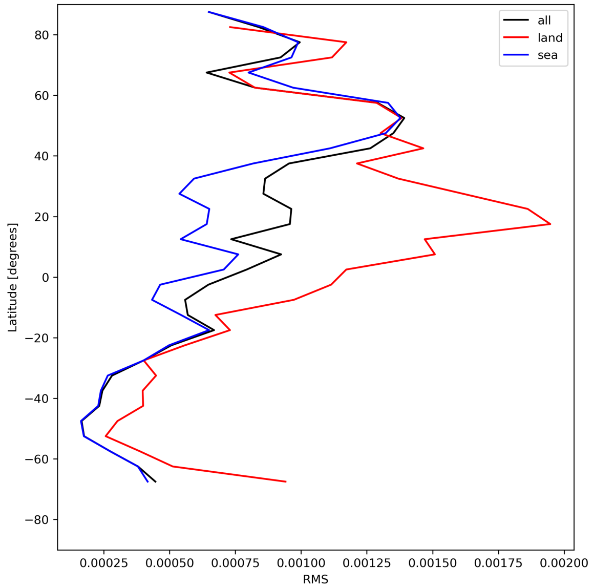
Figure 31: Zonal average of “RMS” for 2023-07-15 to 2023-07-17.
