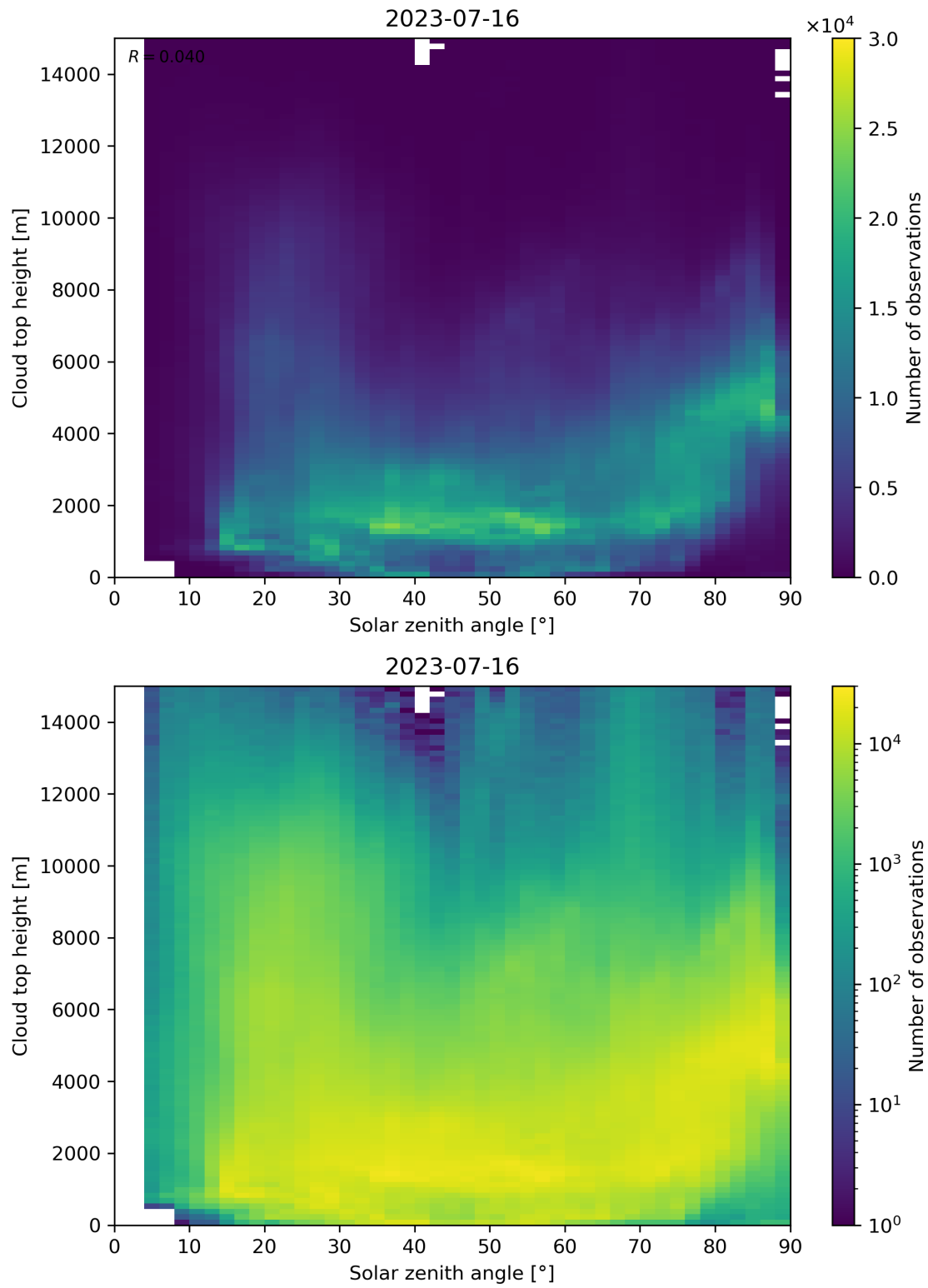
Figure 104: Scatter density plot of “Solar zenith angle” against “Cloud top height” for 2023-07-15 to 2023-07-17.
