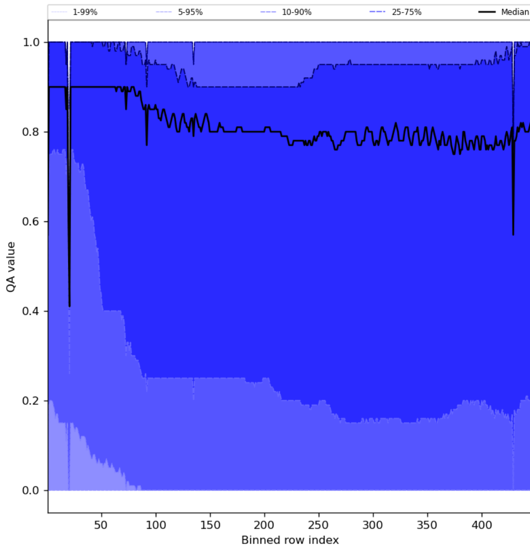
Figure 54: Along track statistics of “QA value” for 2023-07-15 to 2023-07-17
