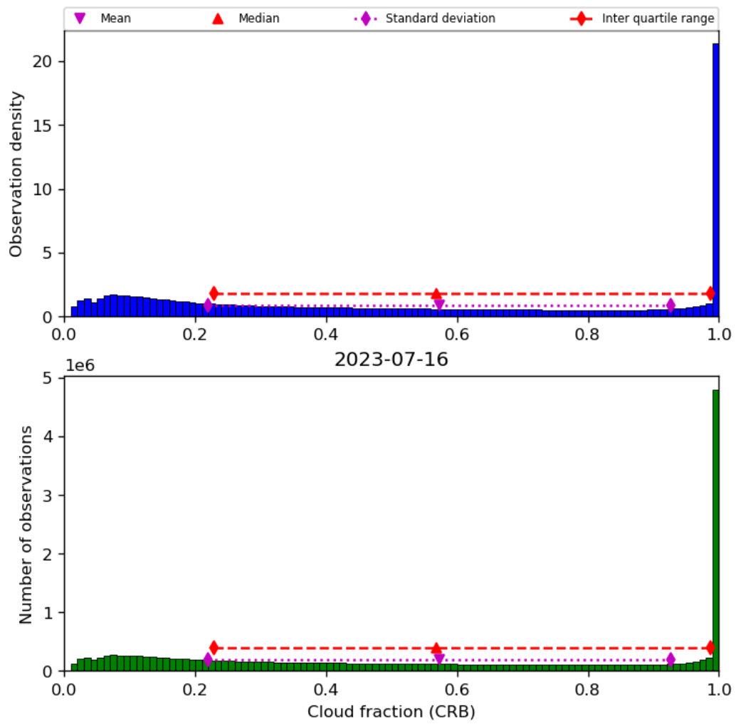
Figure 42: Histogram of “Cloud fraction (CRB)” for 2023-07-15 to 2023-07-17
