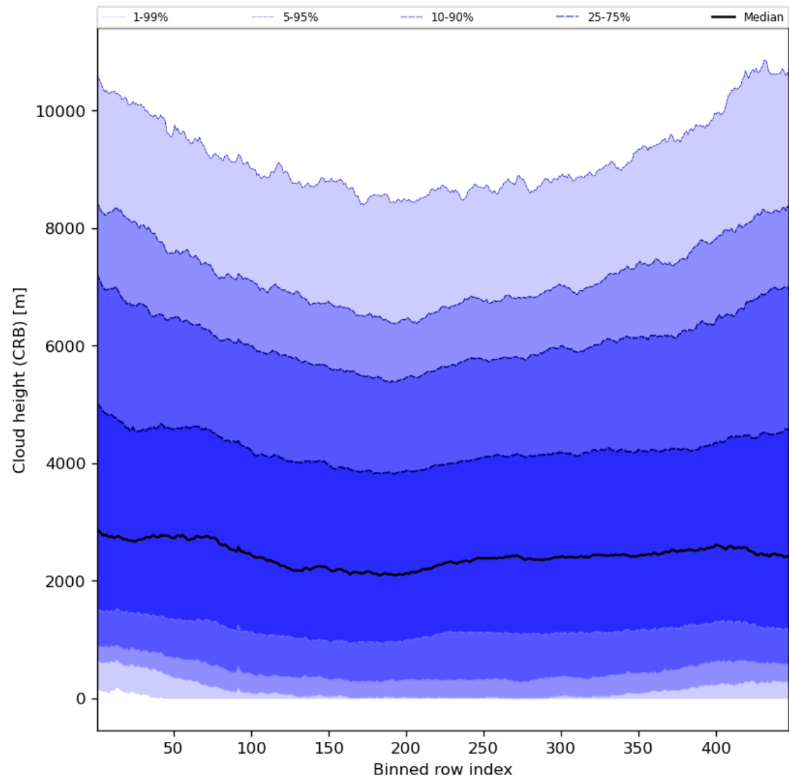
Figure 59: Along track statistics of “Cloud height (CRB)” for 2023-07-15 to 2023-07-17
