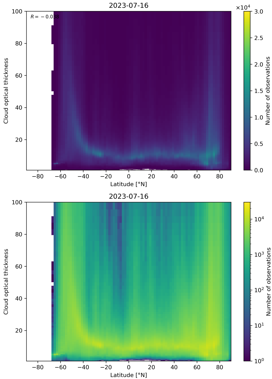
Figure 96: Scatter density plot of “Latitude” against “Cloud optical thickness” for 2023-07-15 to 2023-07-17.
