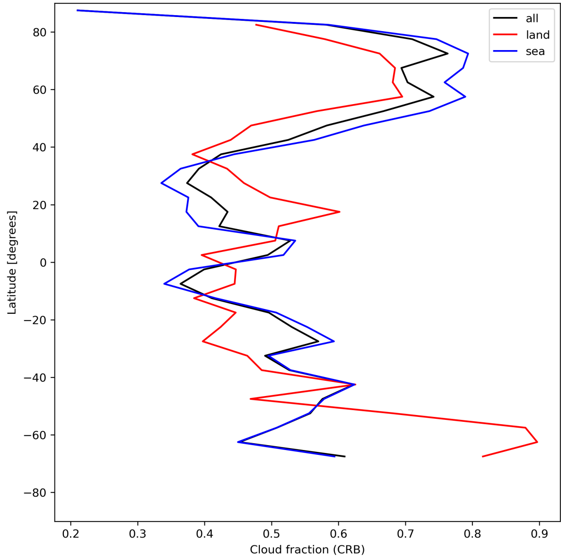
Figure 26: Zonal average of “Cloud fraction (CRB)” for 2023-07-15 to 2023-07-17.
