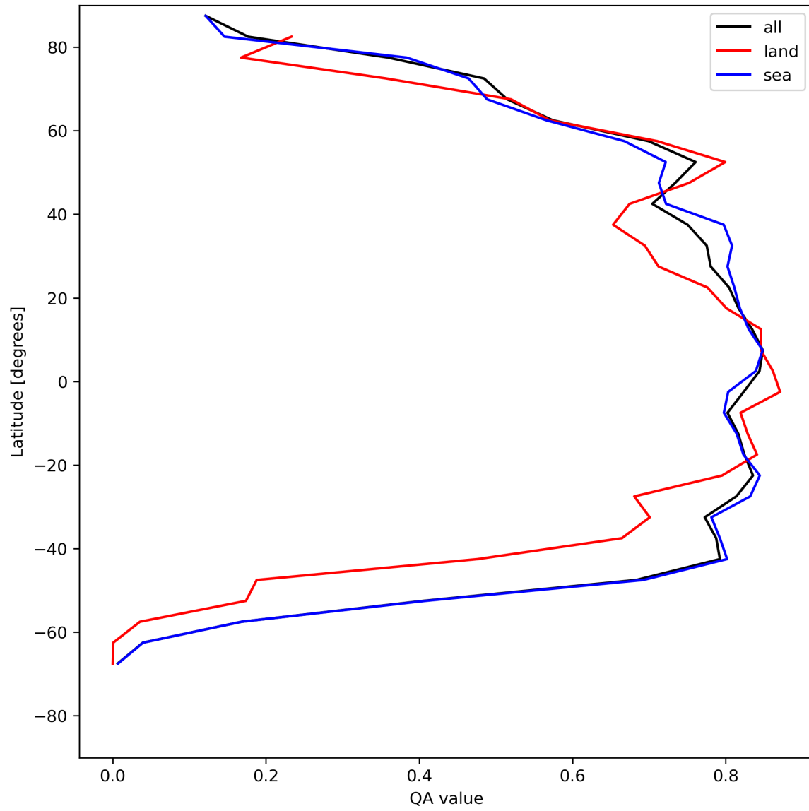
Figure 22: Zonal average of “QA value” for 2023-07-15 to 2023-07-17.
