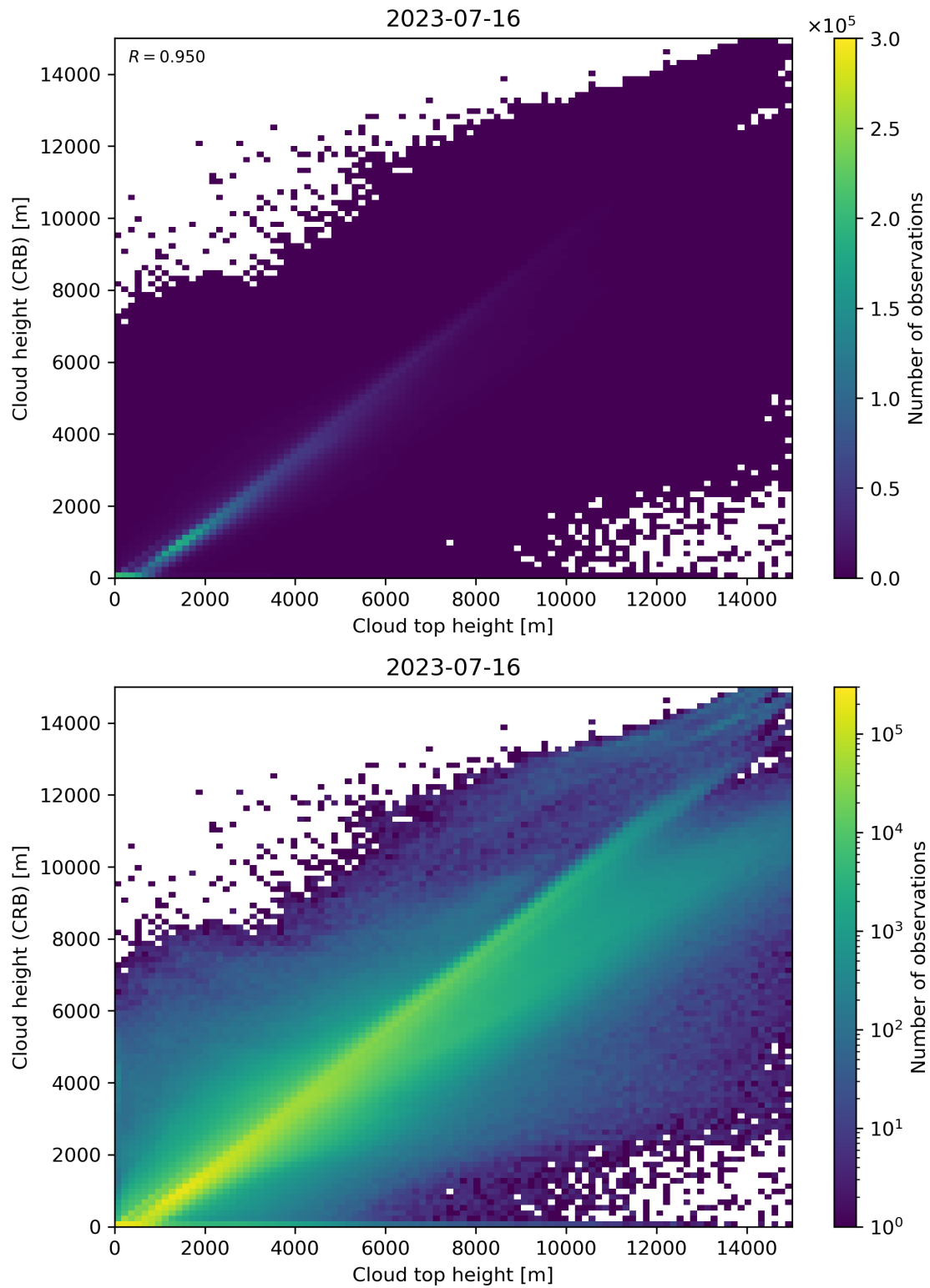
Figure 89: Scatter density plot of “Cloud top height” against “Cloud height (CRB)” for 2023-07-15 to 2023-07-17.
