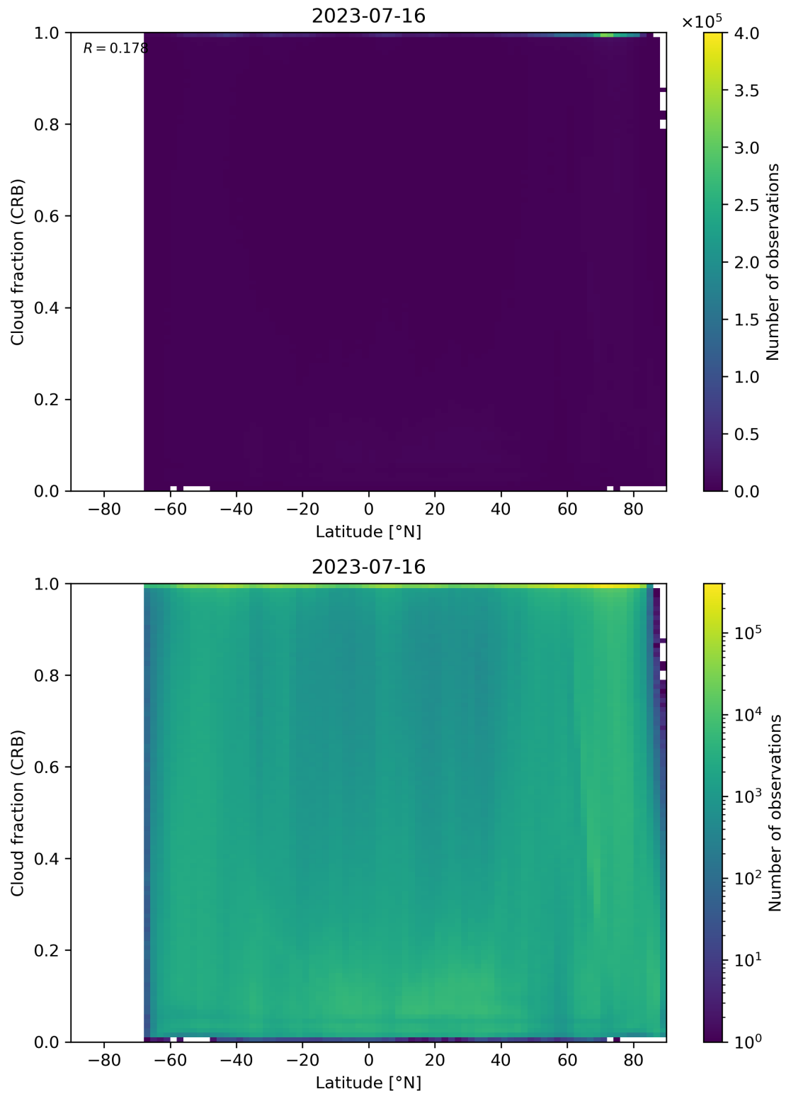
Figure 94: Scatter density plot of “Latitude” against “Cloud fraction (CRB)” for 2023-07-15 to 2023-07-17.
