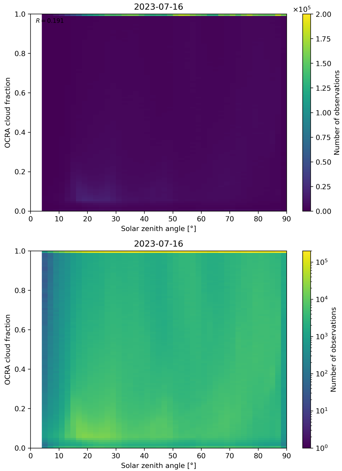
Figure 100: Scatter density plot of “Solar zenith angle” against “OCRA cloud fraction” for 2023-07-15 to 2023-07-17.
