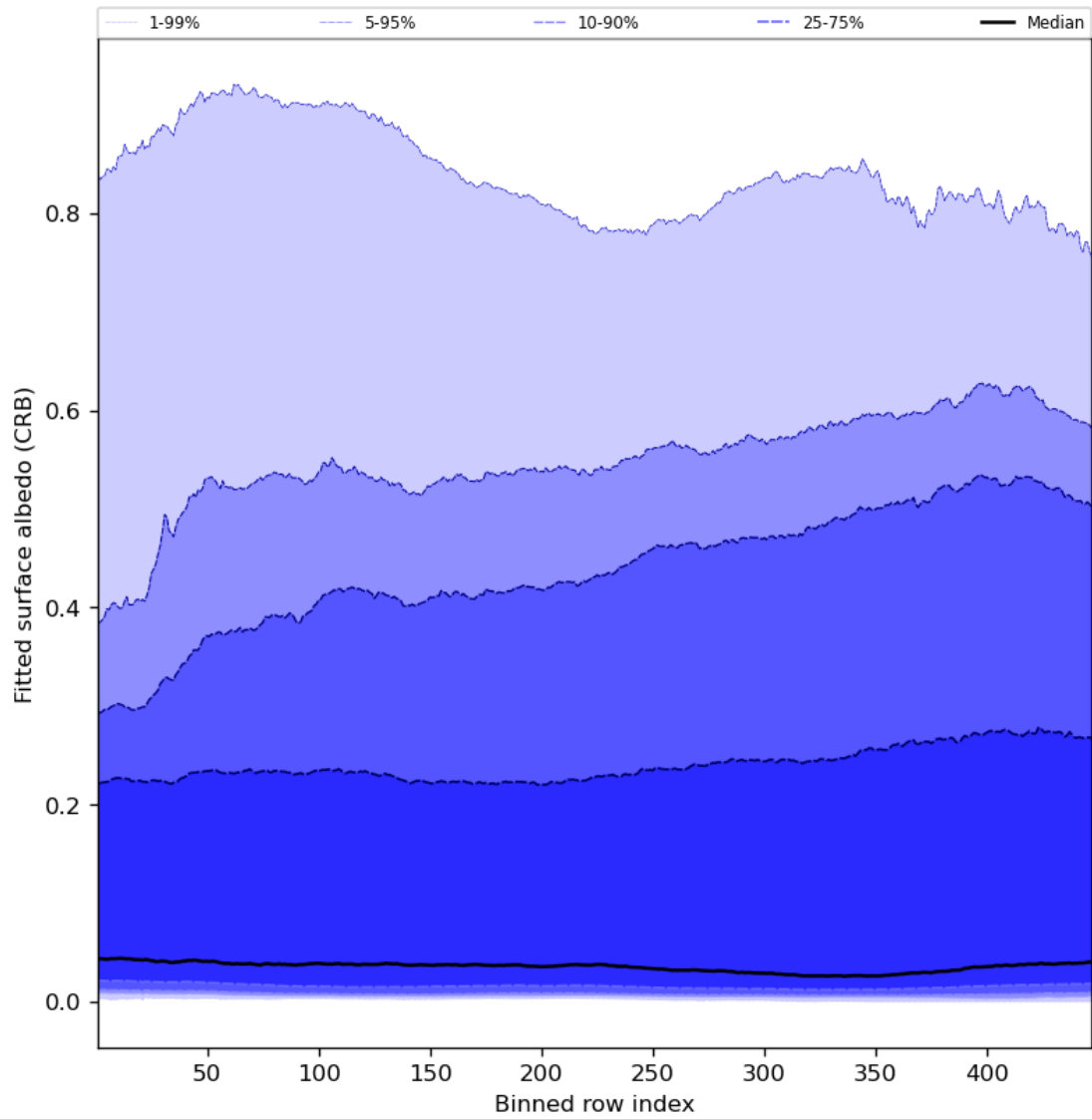
Figure 62: Along track statistics of “Fitted surface albedo (CRB)” for 2023-07-15 to 2023-07-17
