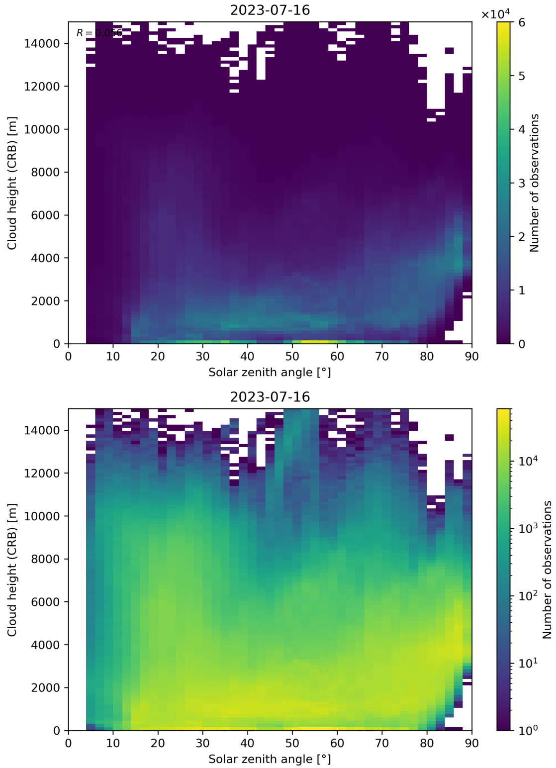
Figure 102: Scatter density plot of “Solar zenith angle” against “Cloud height (CRB)” for 2023-07-15 to 2023-07-17.
