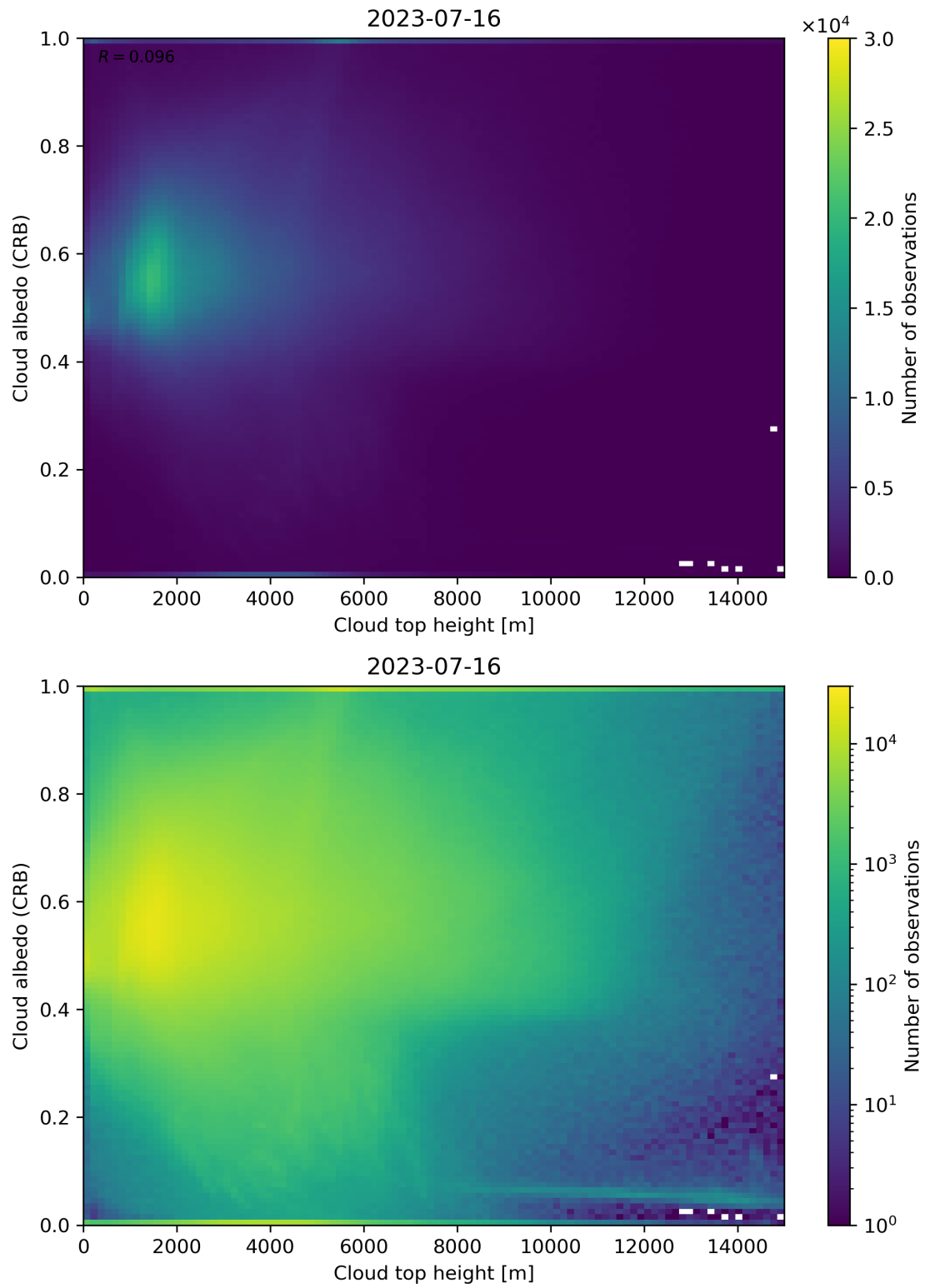
Figure 86: Scatter density plot of “Cloud top height” against “Cloud albedo (CRB)” for 2023-07-15 to 2023-07-17.
