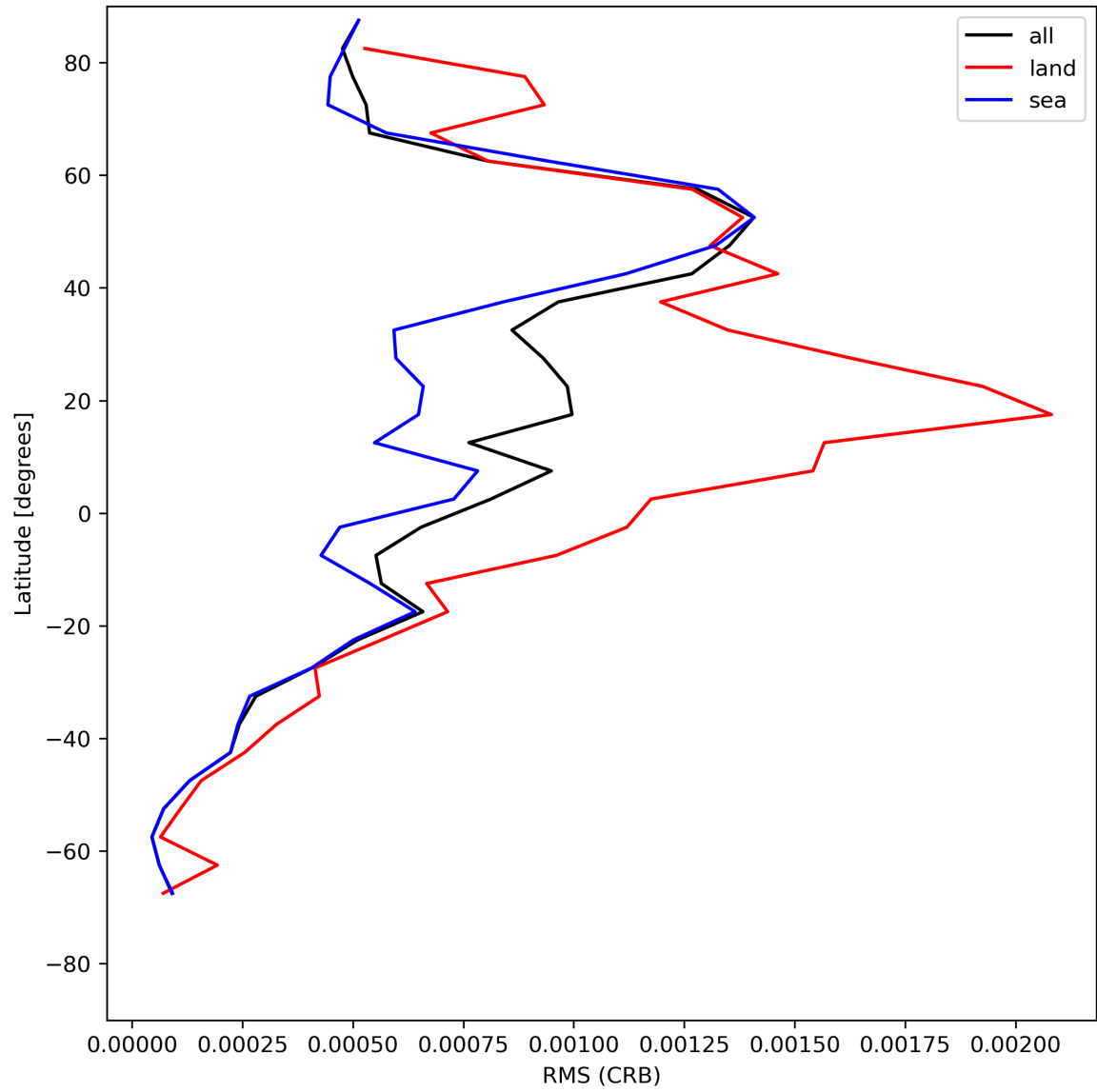
Figure 32: Zonal average of “RMS (CRB)” for 2023-07-15 to 2023-07-17.
