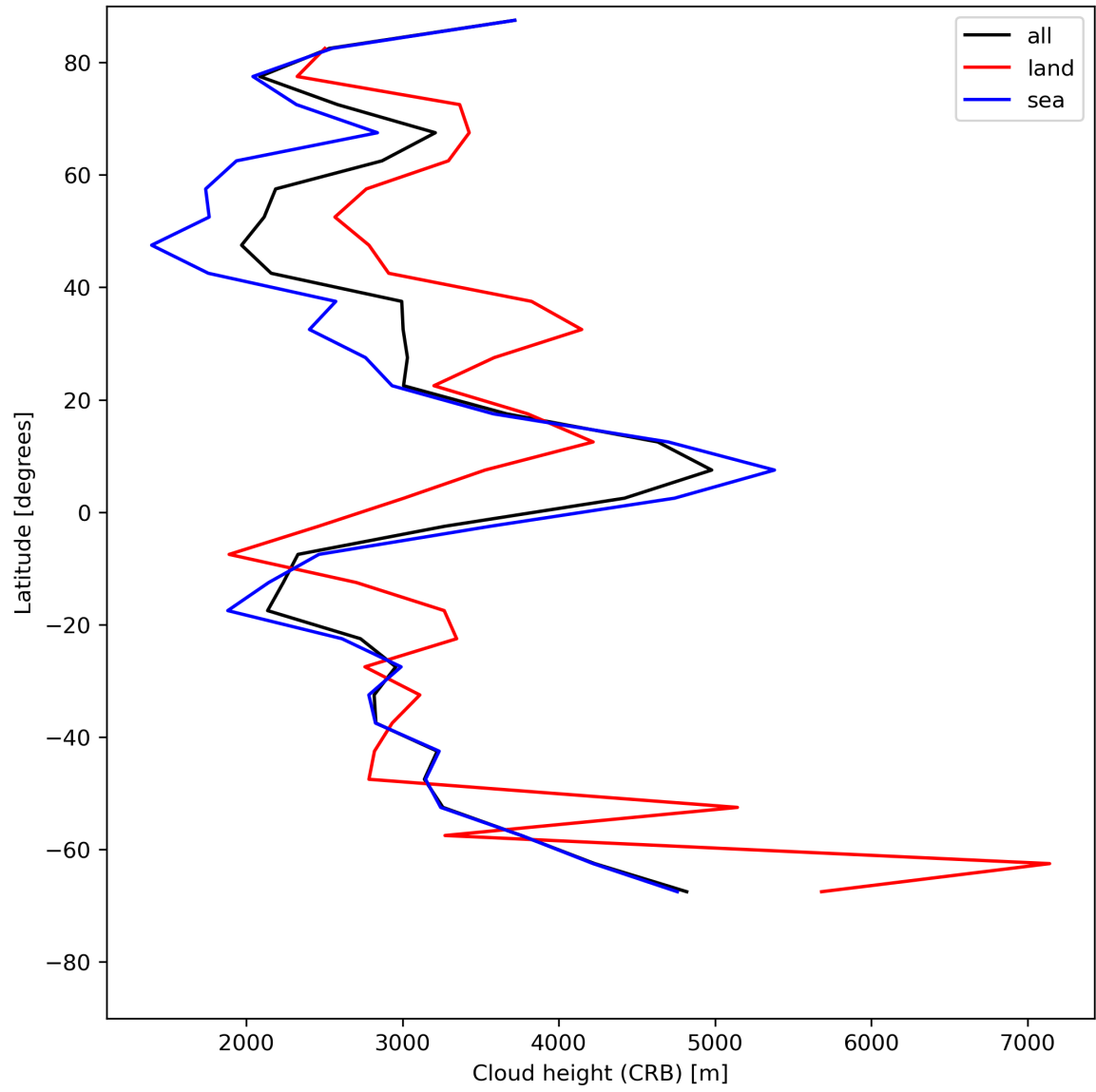
Figure 27: Zonal average of “Cloud height (CRB)” for 2023-07-15 to 2023-07-17.
