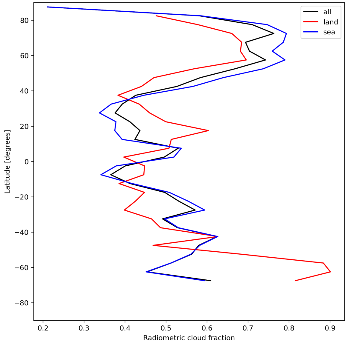
Figure 23: Zonal average of “Radiometric cloud fraction” for 2023-07-15 to 2023-07-17.
