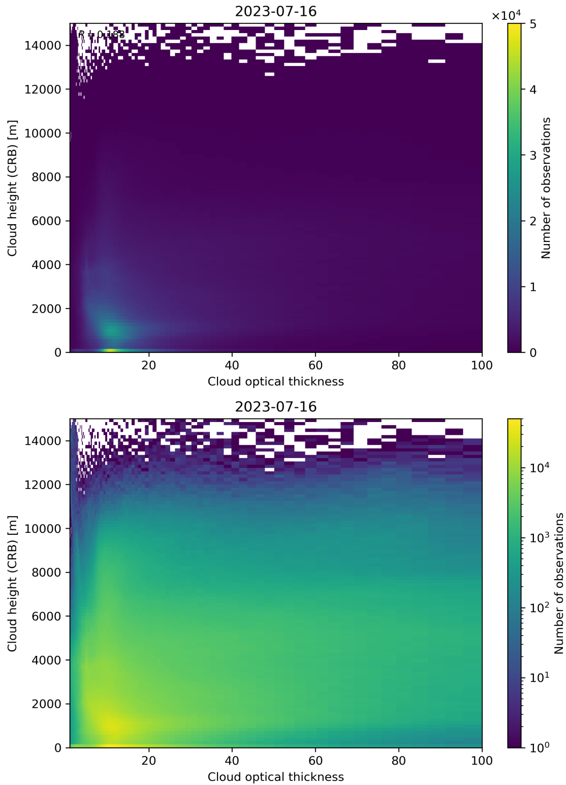
Figure 85: Scatter density plot of “Cloud optical thickness” against “Cloud height (CRB)” for 2023-07-15 to 2023-07-17.
