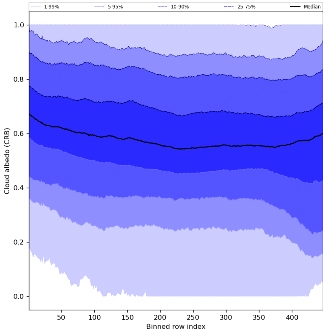
Figure 60: Along track statistics of “Cloud albedo (CRB)” for 2023-07-15 to 2023-07-17
