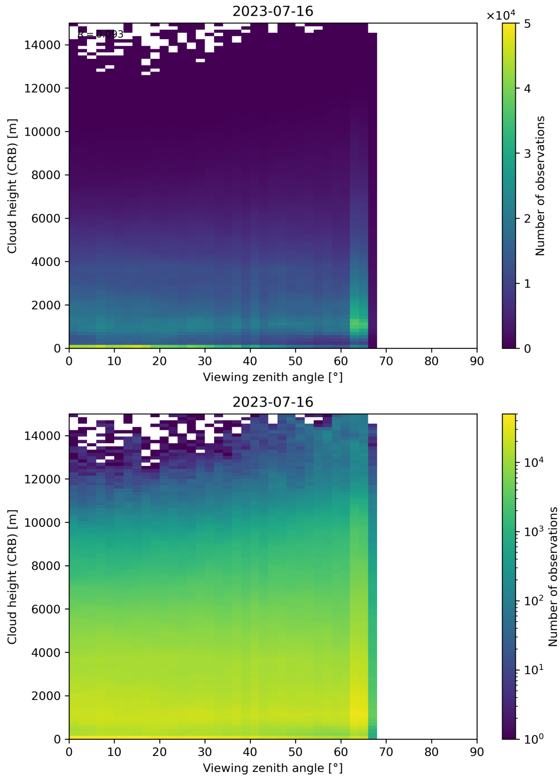
Figure 110: Scatter density plot of “Viewing zenith angle” against “Cloud height (CRB)” for 2023-07-15 to 2023-07-17.
