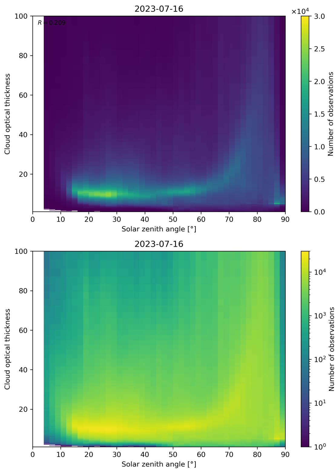
Figure 103: Scatter density plot of “Solar zenith angle” against “Cloud optical thickness” for 2023-07-15 to 2023-07-17.
