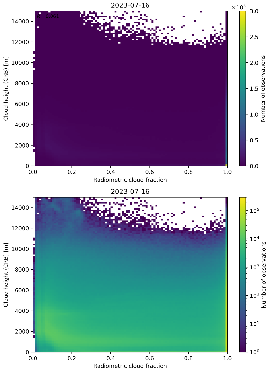
Figure 74: Scatter density plot of “Radiometric cloud fraction” against “Cloud height (CRB)” for 2023-07-15 to 2023-07-17.
