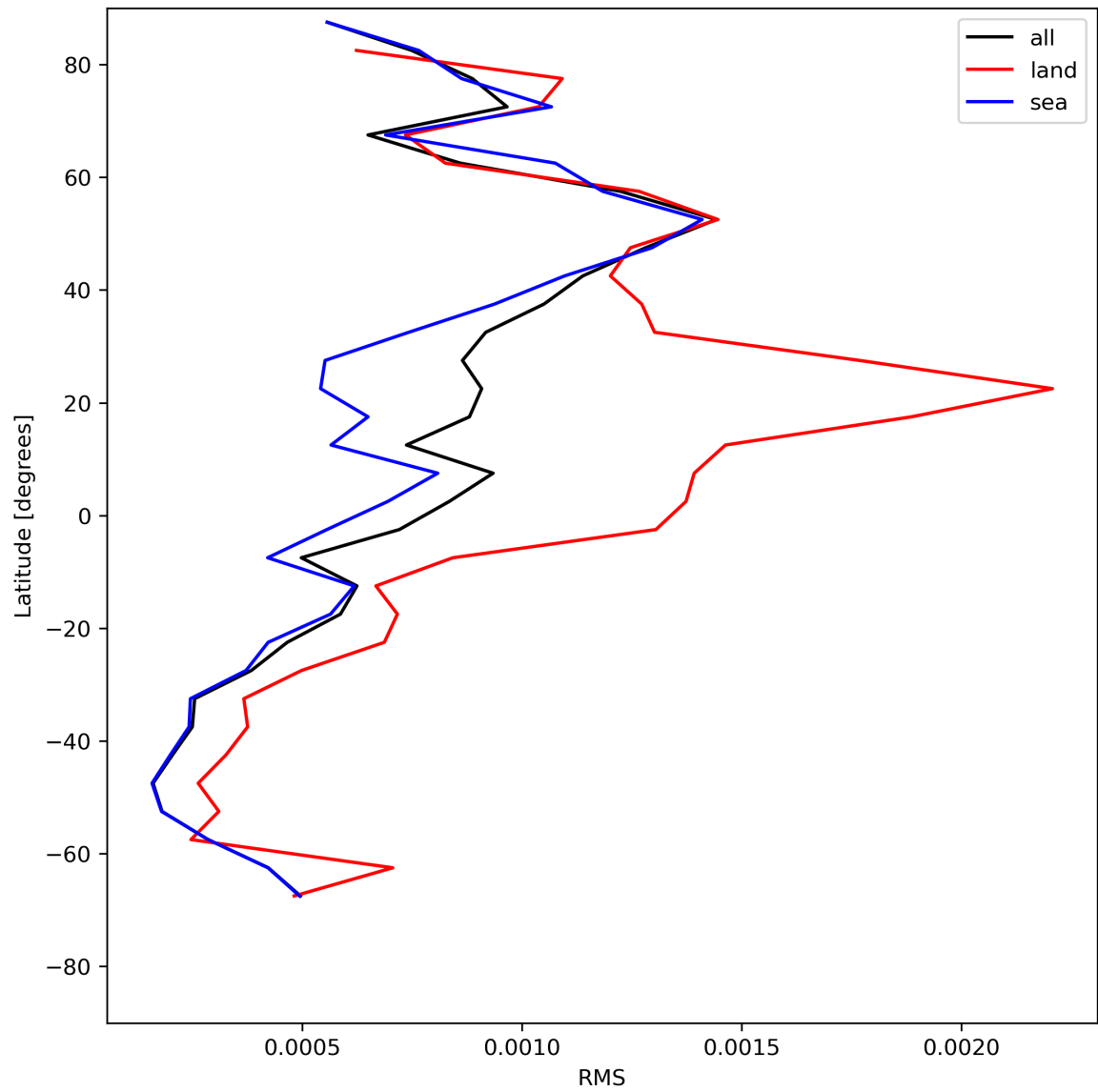
Figure 31: Zonal average of “RMS” for 2023-07-17 to 2023-07-19.
