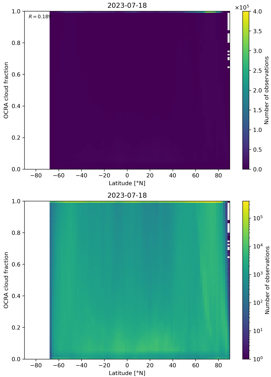
Figure 93: Scatter density plot of “Latitude” against “OCRA cloud fraction” for 2023-07-17 to 2023-07-19.
