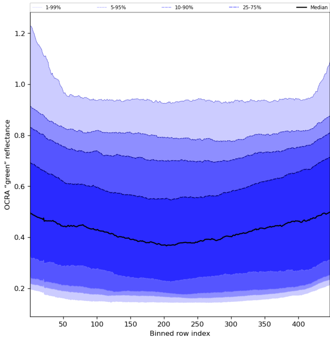
Figure 68: Along track statistics of "OCRA "green" reflectance" for 2023-07-17 to 2023-07-19
