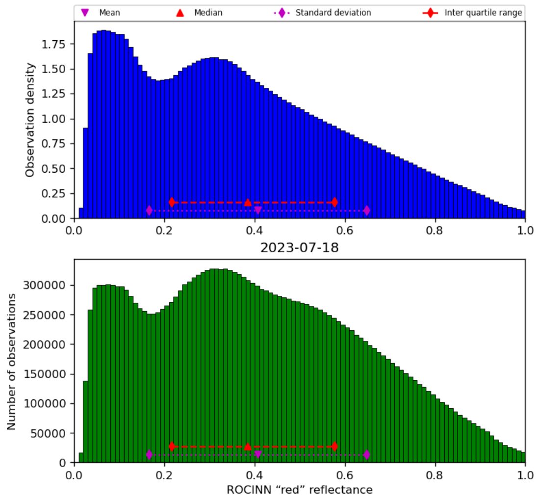
Figure 53: Histogram of “ROCINN “red” reflectance” for 2023-07-17 to 2023-07-19
