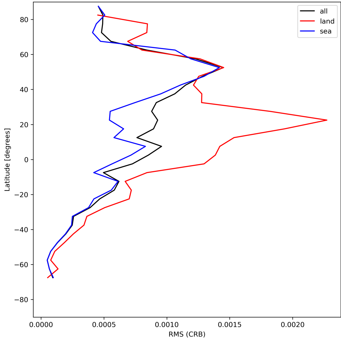
Figure 32: Zonal average of “RMS (CRB)” for 2023-07-17 to 2023-07-19.
