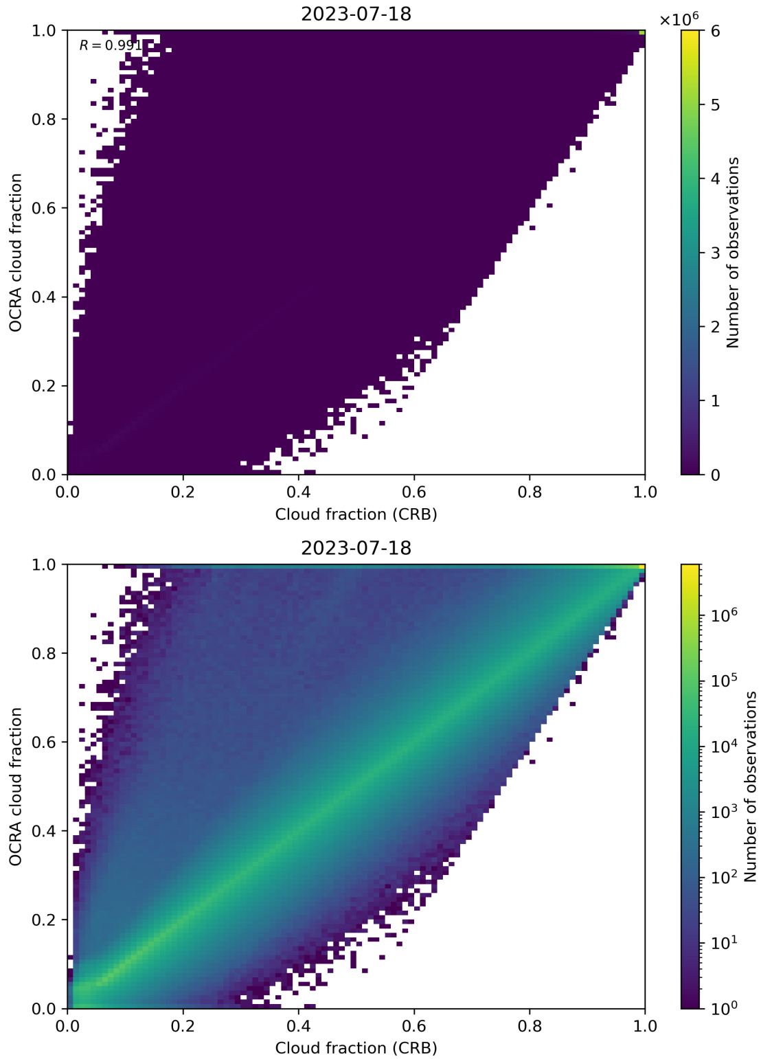
Figure 78: Scatter density plot of “Cloud fraction (CRB)” against “OCRA cloud fraction” for 2023-07-17 to 2023-07-19.
