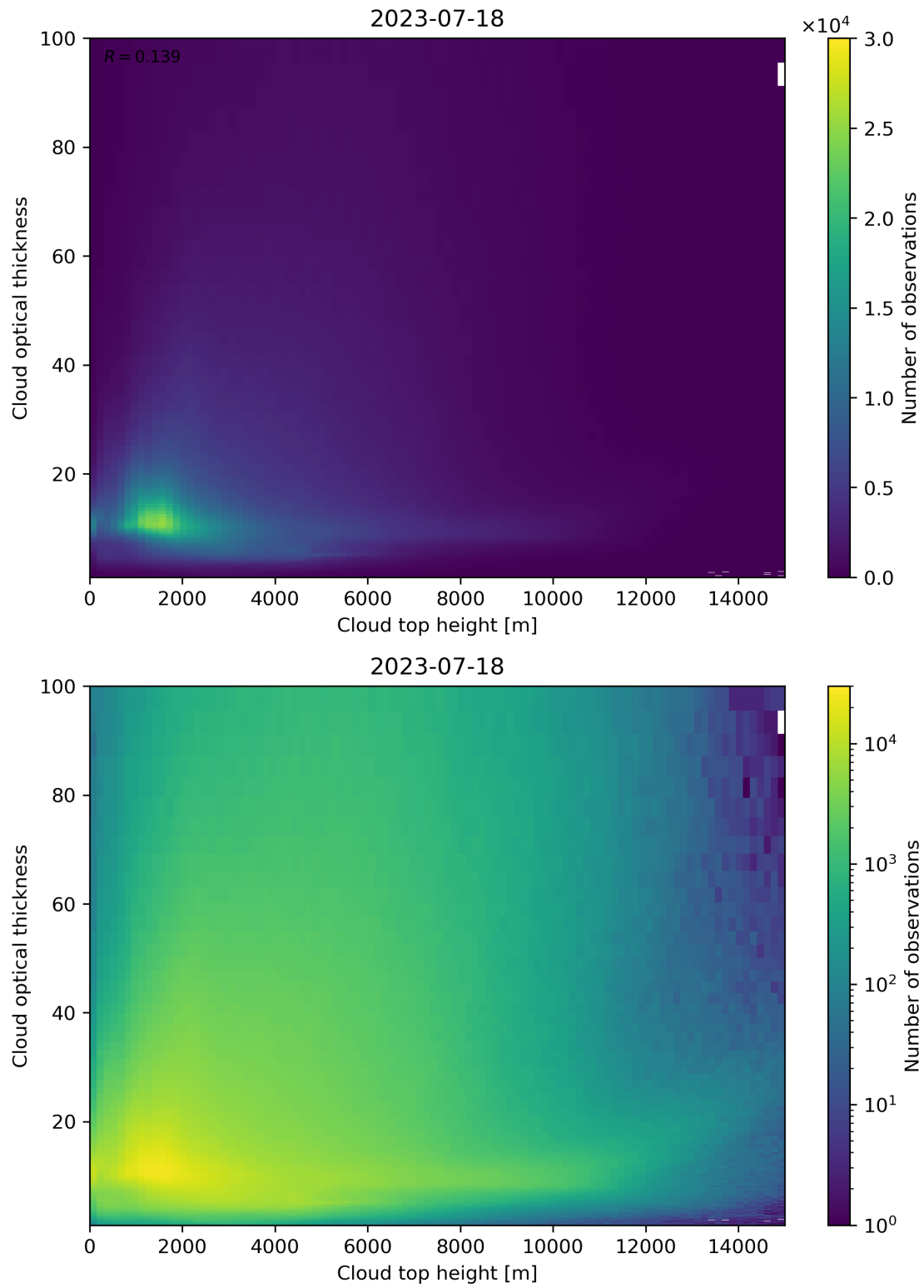
Figure 90: Scatter density plot of “Cloud top height” against “Cloud optical thickness” for 2023-07-17 to 2023-07-19.
