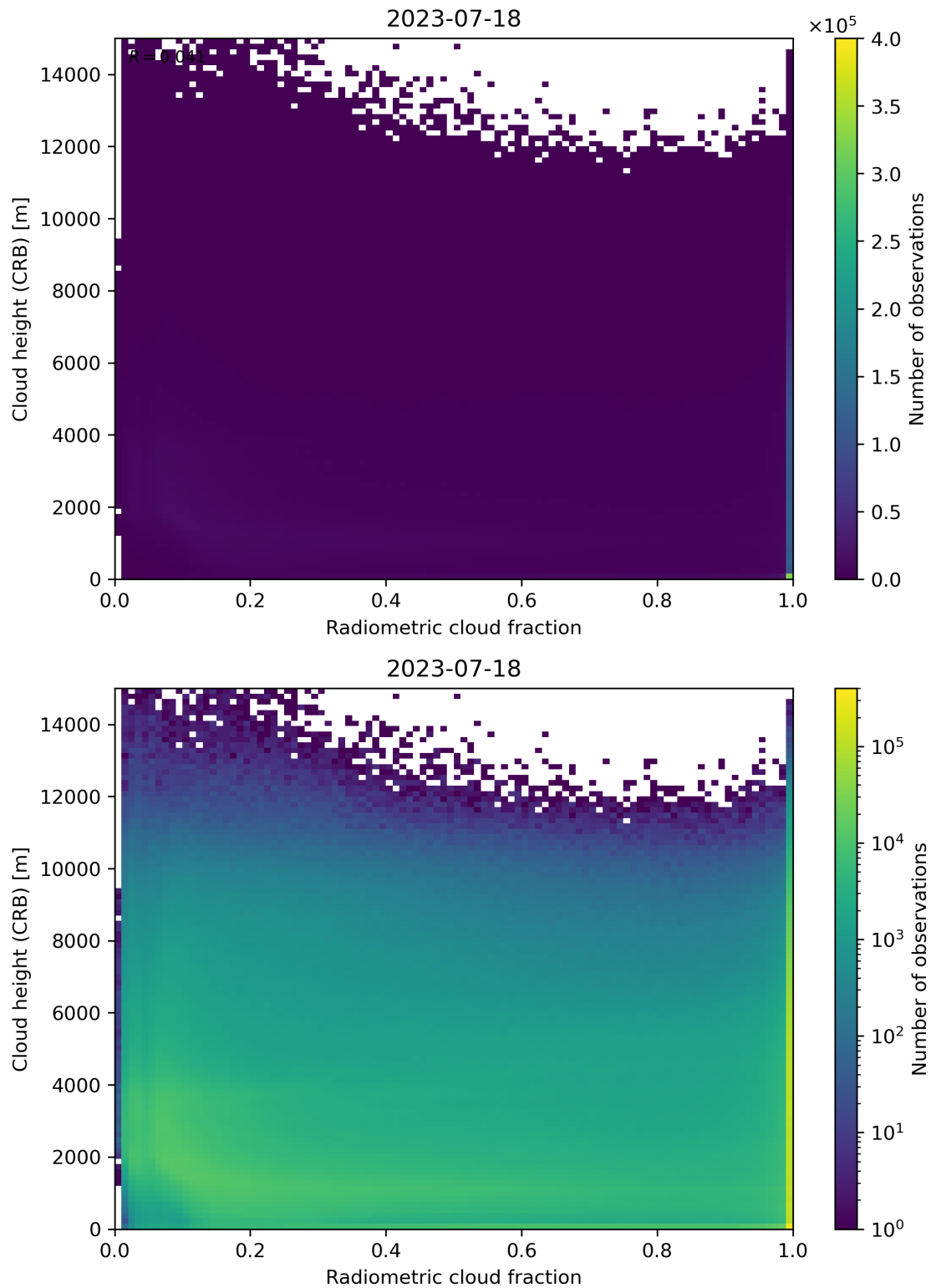
Figure 74: Scatter density plot of “Radiometric cloud fraction” against “Cloud height (CRB)” for 2023-07-17 to 2023-07-19.
