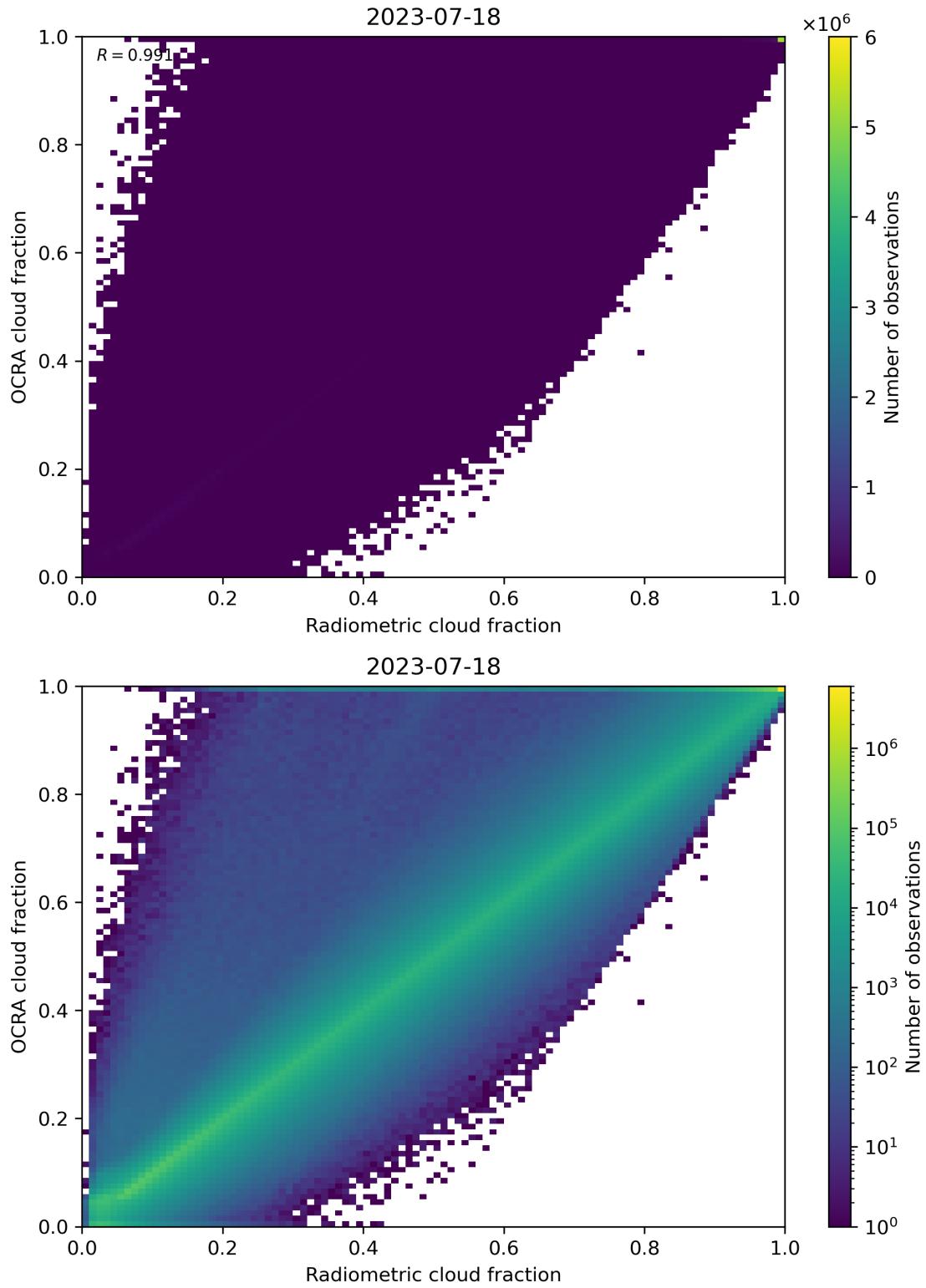
Figure 72: Scatter density plot of “Radiometric cloud fraction” against “OCRA cloud fraction” for 2023-07-17 to 2023-07-19.
