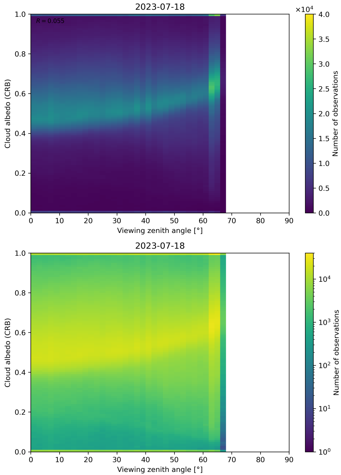
Figure 106: Scatter density plot of “Viewing zenith angle” against “Cloud albedo (CRB)” for 2023-07-17 to 2023-07-19.
