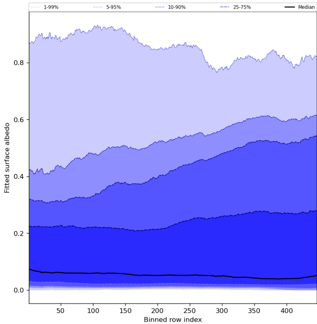
Figure 61: Along track statistics of “Fitted surface albedo” for 2023-07-17 to 2023-07-19
