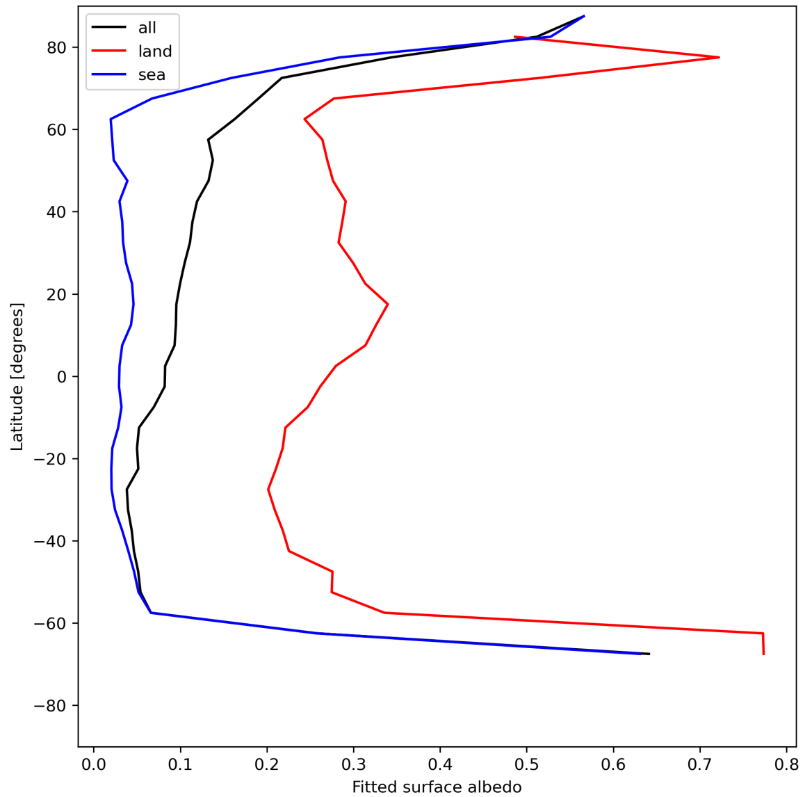
Figure 29: Zonal average of “Fitted surface albedo” for 2023-07-17 to 2023-07-19.
