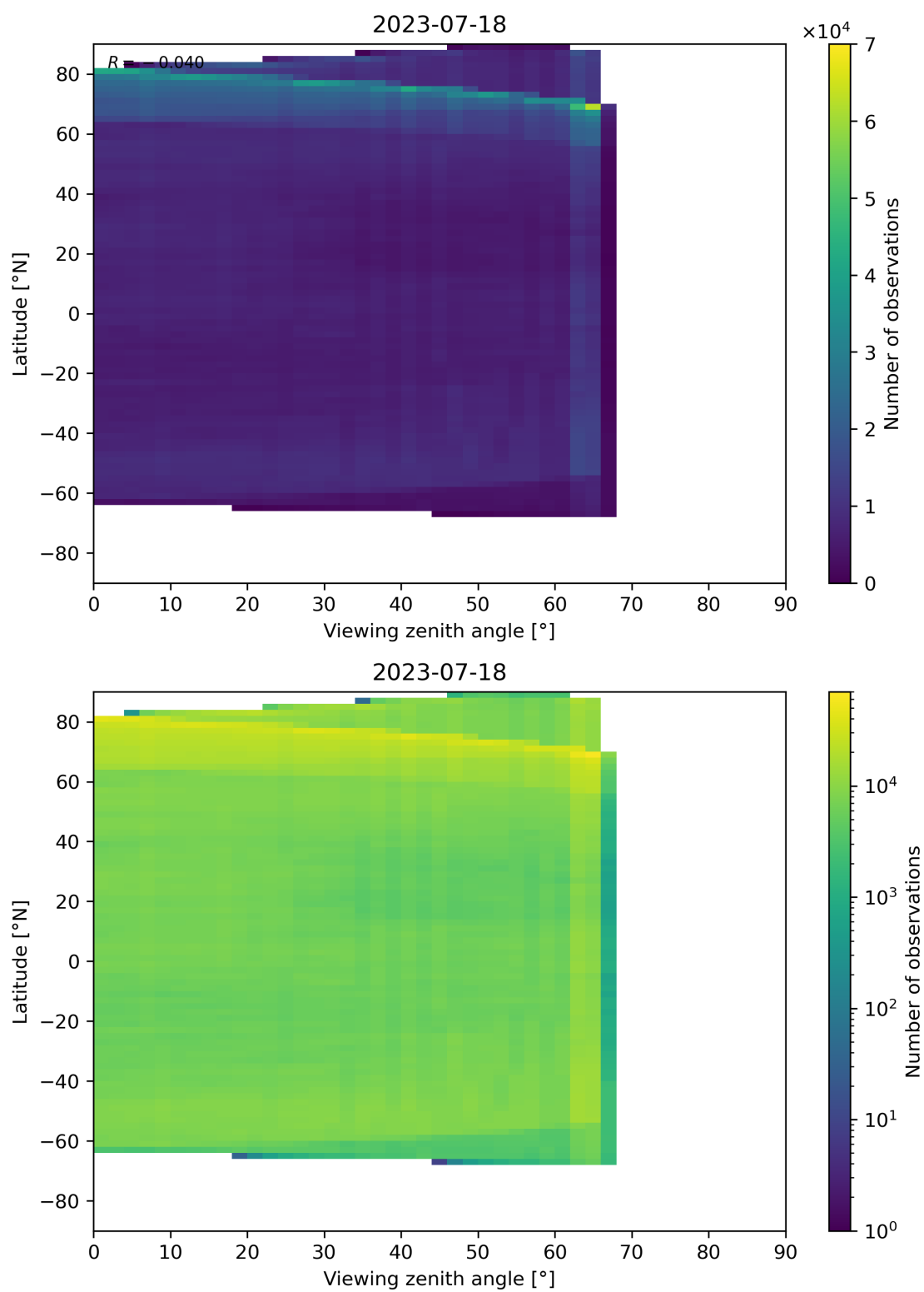
Figure 113: Scatter density plot of “Viewing zenith angle” against “Latitude” for 2023-07-17 to 2023-07-19.
