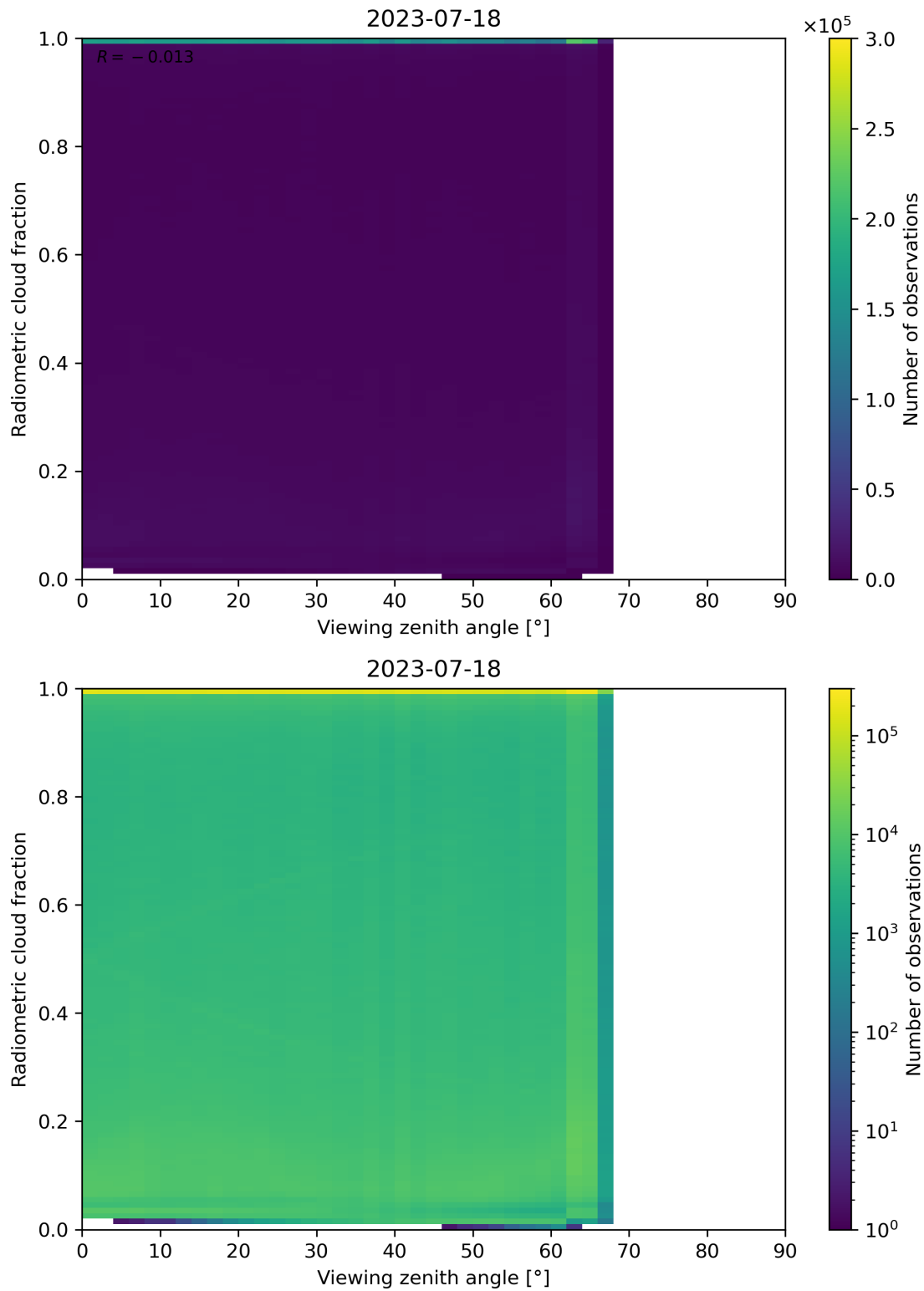
Figure 107: Scatter density plot of “Viewing zenith angle” against “Radiometric cloud fraction” for 2023-07-17 to 2023-07-19.
