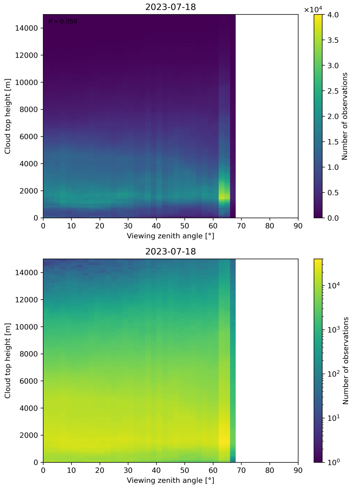
Figure 112: Scatter density plot of “Viewing zenith angle” against “Cloud top height” for 2023-07-17 to 2023-07-19.
