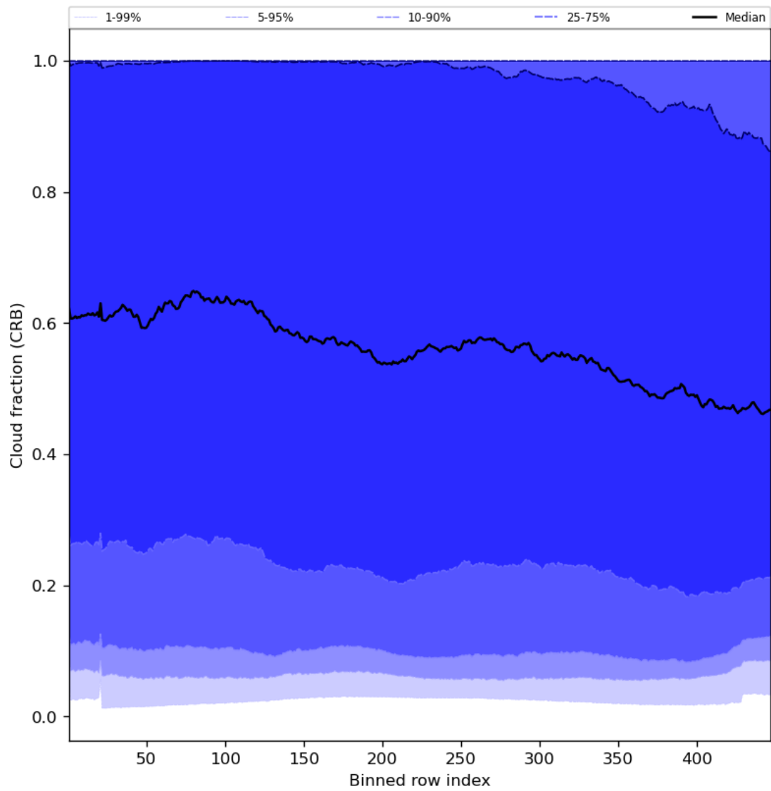
Figure 58: Along track statistics of “Cloud fraction (CRB)” for 2023-07-17 to 2023-07-19
