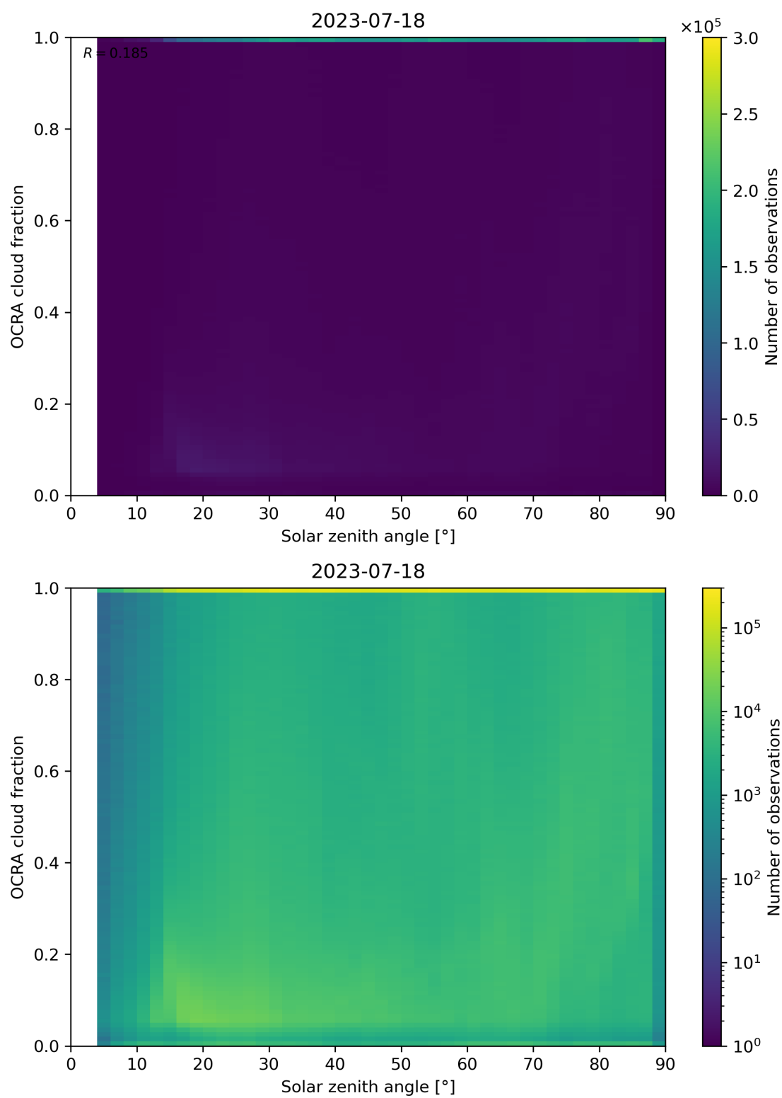
Figure 100: Scatter density plot of “Solar zenith angle” against “OCRA cloud fraction” for 2023-07-17 to 2023-07-19.
