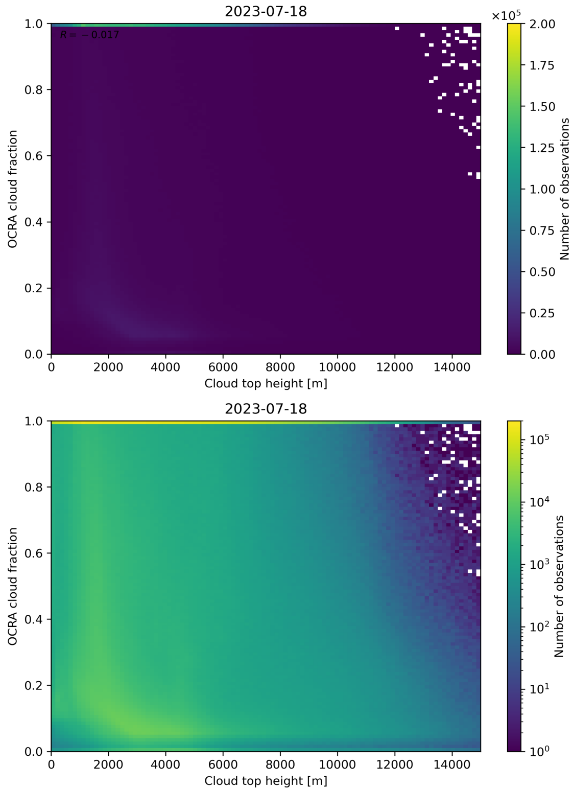
Figure 87: Scatter density plot of “Cloud top height” against “OCRA cloud fraction” for 2023-07-17 to 2023-07-19.
