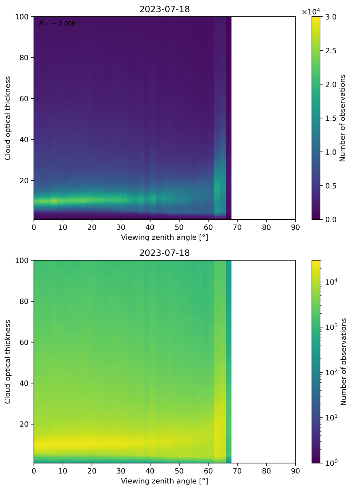
Figure 111: Scatter density plot of “Viewing zenith angle” against “Cloud optical thickness” for 2023-07-17 to 2023-07-19.
