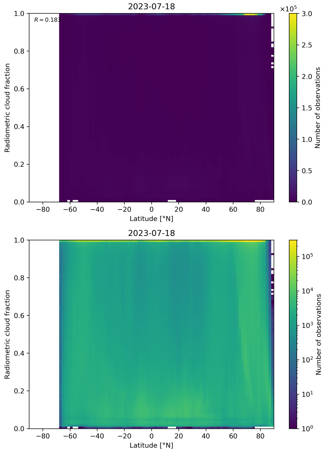
Figure 92: Scatter density plot of “Latitude” against “Radiometric cloud fraction” for 2023-07-17 to 2023-07-19.
