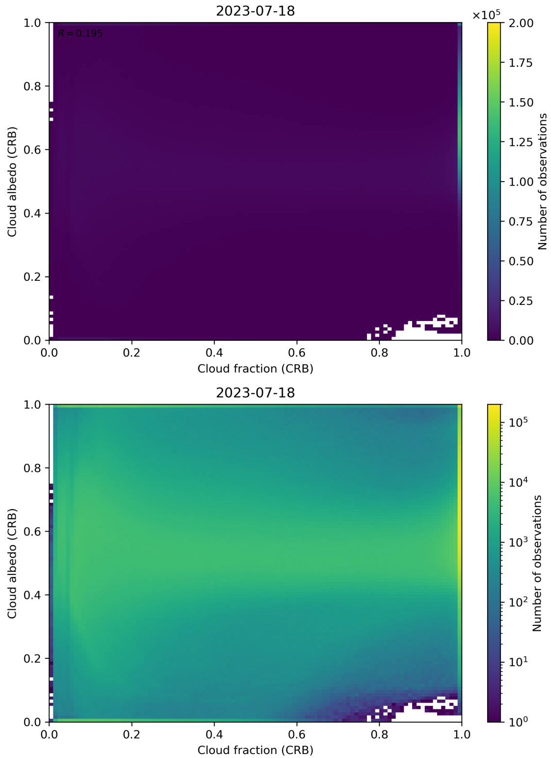
Figure 77: Scatter density plot of “Cloud fraction (CRB)” against “Cloud albedo (CRB)” for 2023-07-17 to 2023-07-19.
