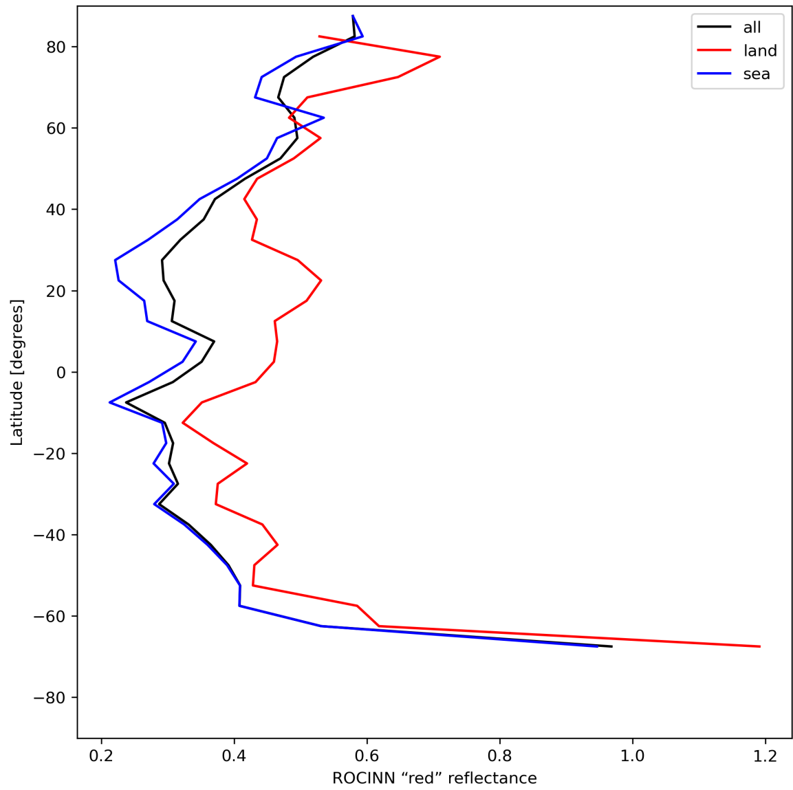
Figure 37: Zonal average of “ROCINN “red” reflectance” for 2023-07-17 to 2023-07-19.
