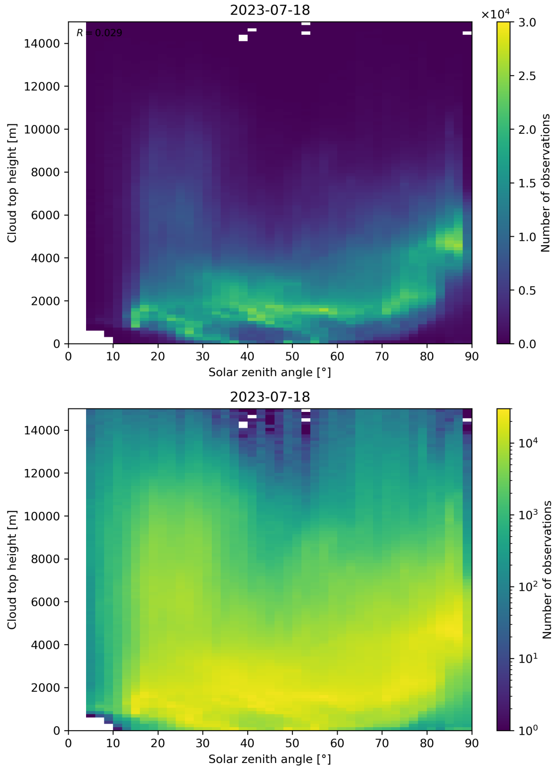
Figure 104: Scatter density plot of “Solar zenith angle” against “Cloud top height” for 2023-07-17 to 2023-07-19.
