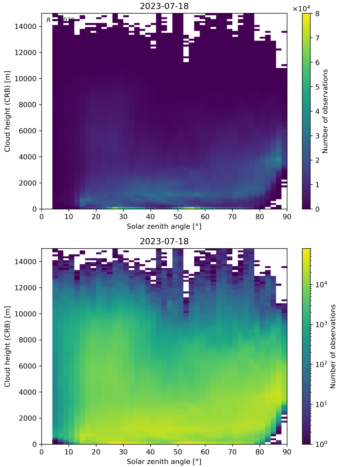
Figure 102: Scatter density plot of “Solar zenith angle” against “Cloud height (CRB)” for 2023-07-17 to 2023-07-19.
