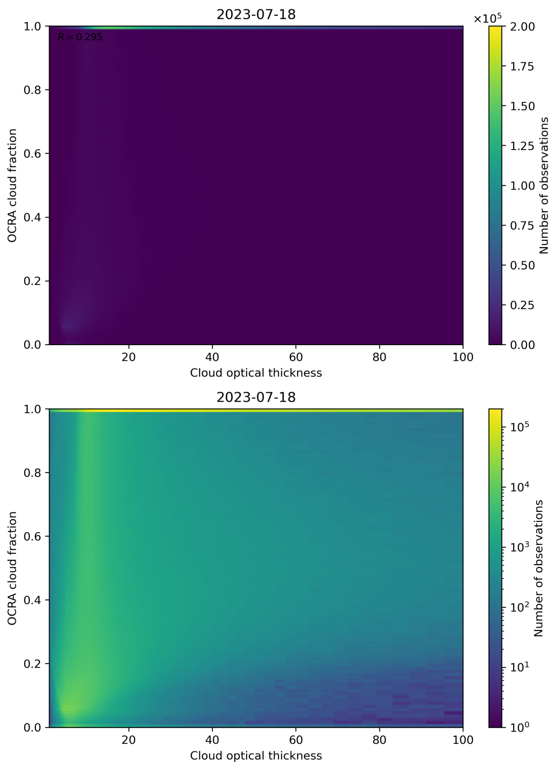
Figure 83: Scatter density plot of “Cloud optical thickness” against “OCRA cloud fraction” for 2023-07-17 to 2023-07-19.
