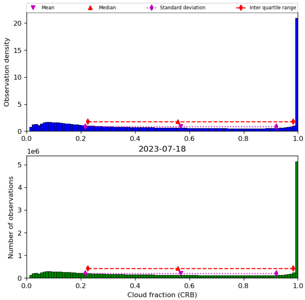
Figure 42: Histogram of “Cloud fraction (CRB)” for 2023-07-17 to 2023-07-19
