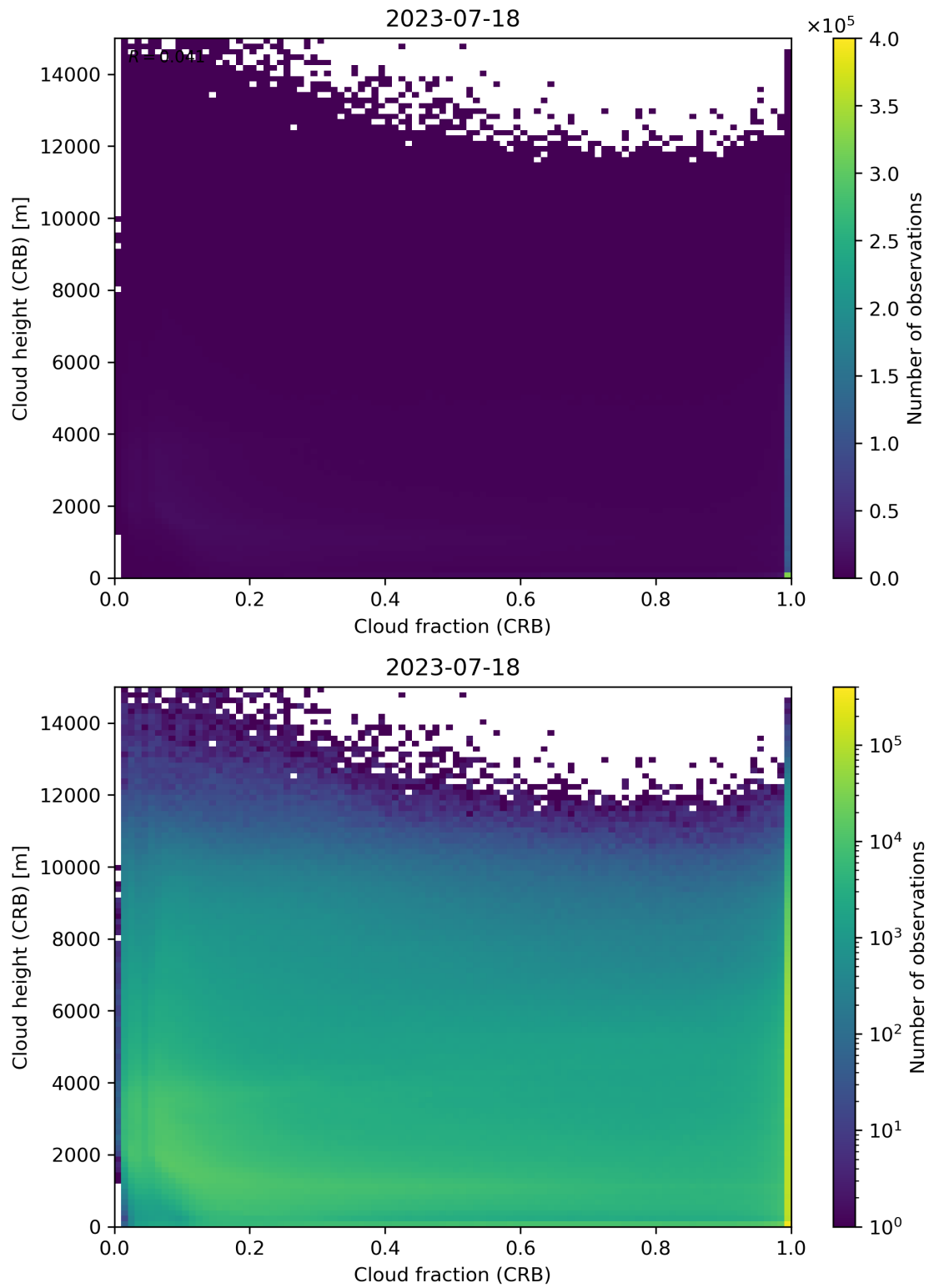
Figure 79: Scatter density plot of “Cloud fraction (CRB)” against “Cloud height (CRB)” for 2023-07-17 to 2023-07-19.
