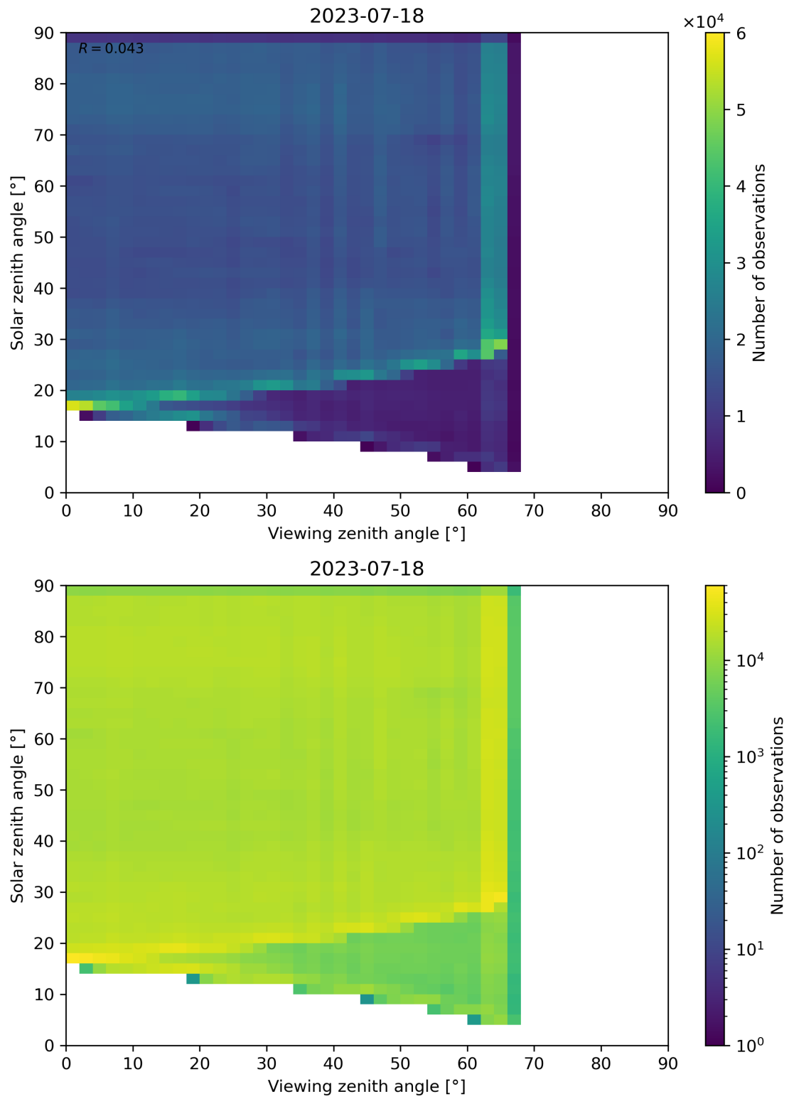
Figure 114: Scatter density plot of “Viewing zenith angle” against “Solar zenith angle” for 2023-07-17 to 2023-07-19.
