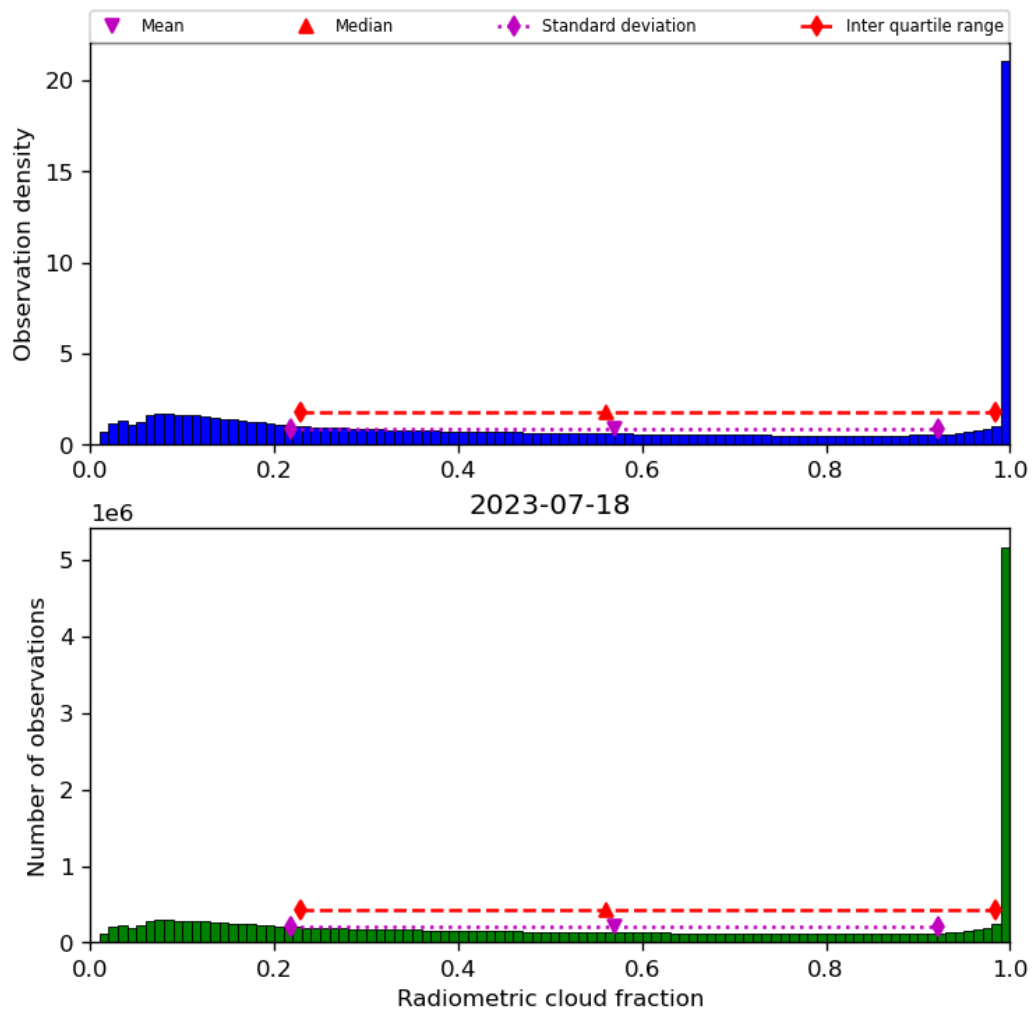
Figure 39: Histogram of “Radiometric cloud fraction” for 2023-07-17 to 2023-07-19
