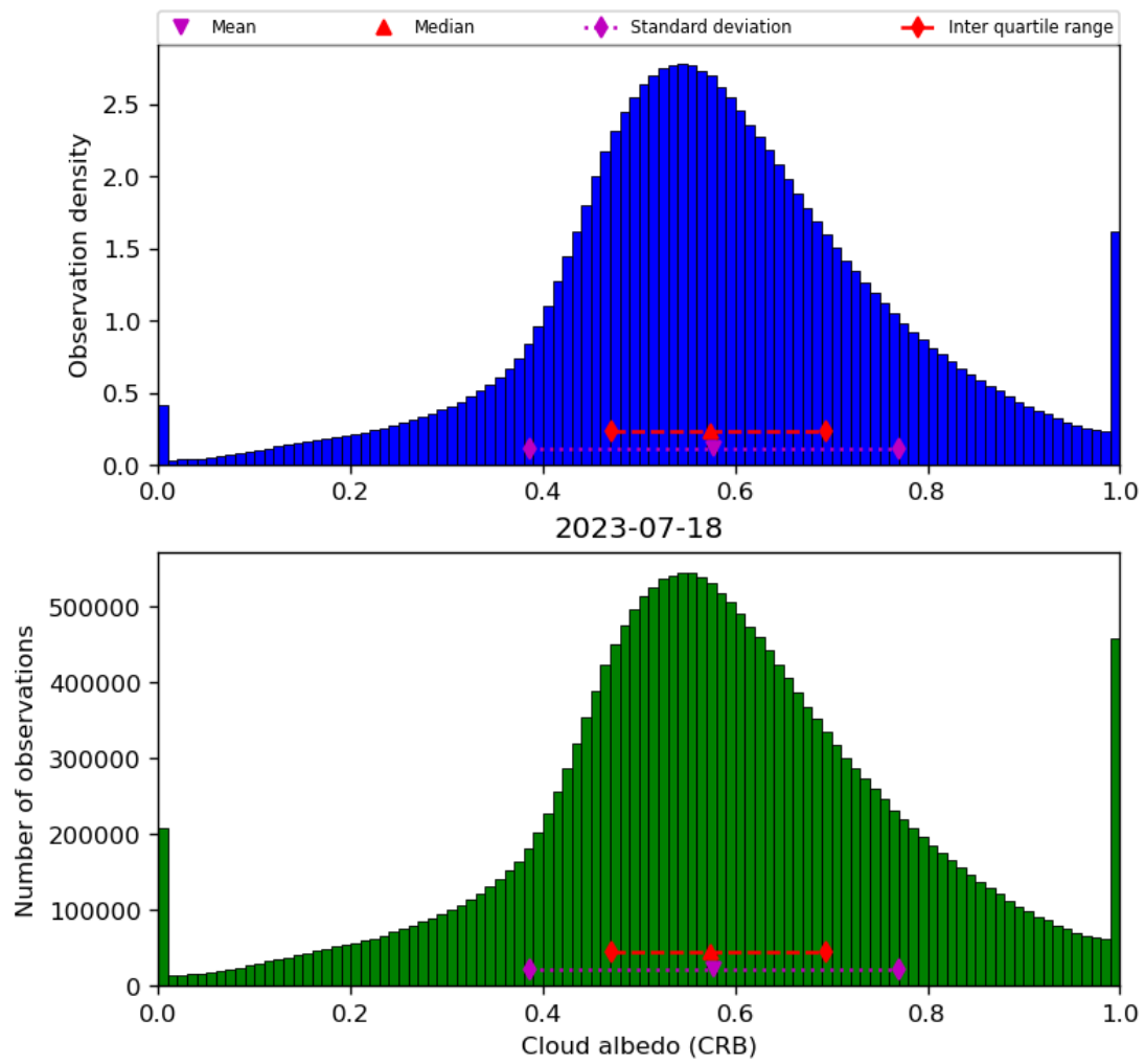
Figure 44: Histogram of “Cloud albedo (CRB)” for 2023-07-17 to 2023-07-19
