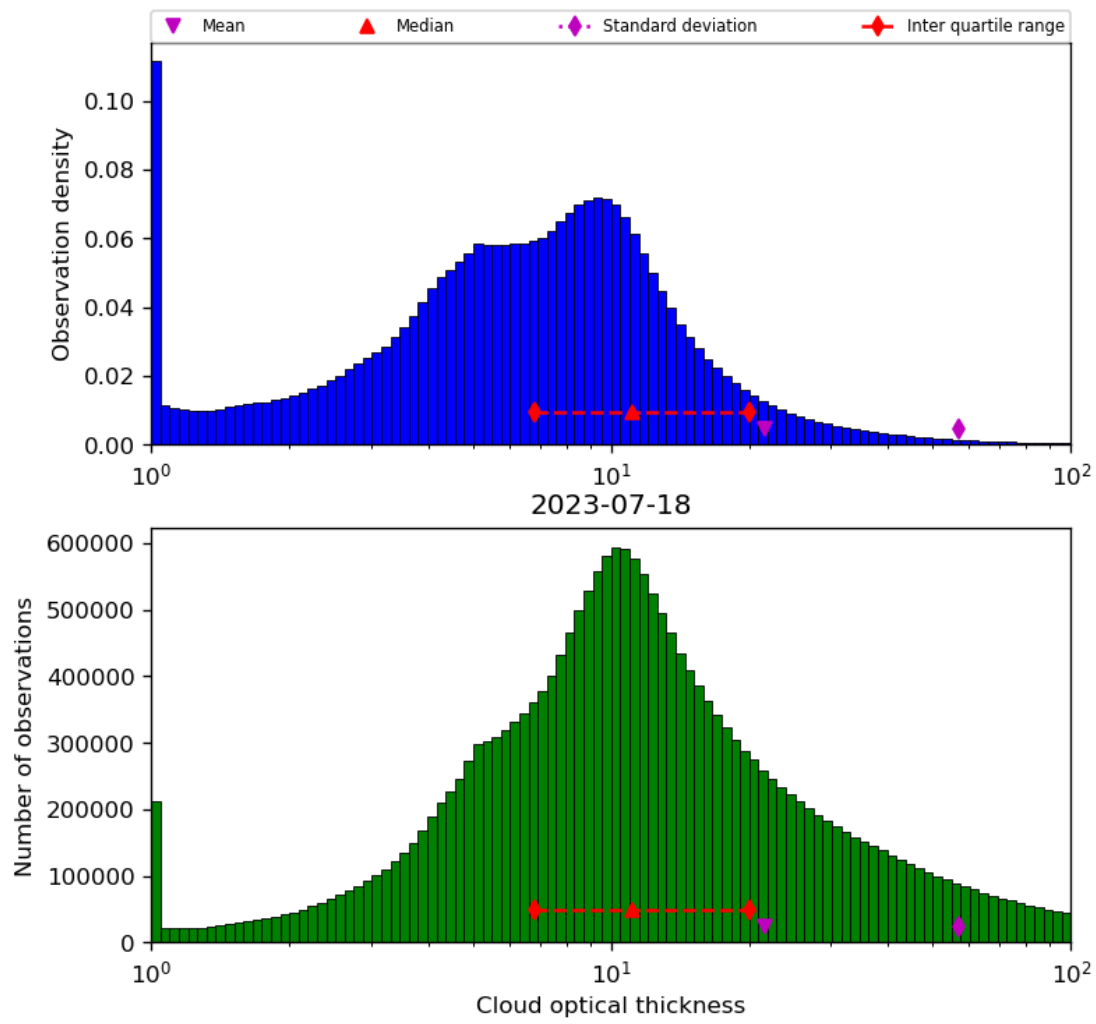
Figure 41: Histogram of “Cloud optical thickness” for 2023-07-17 to 2023-07-19
