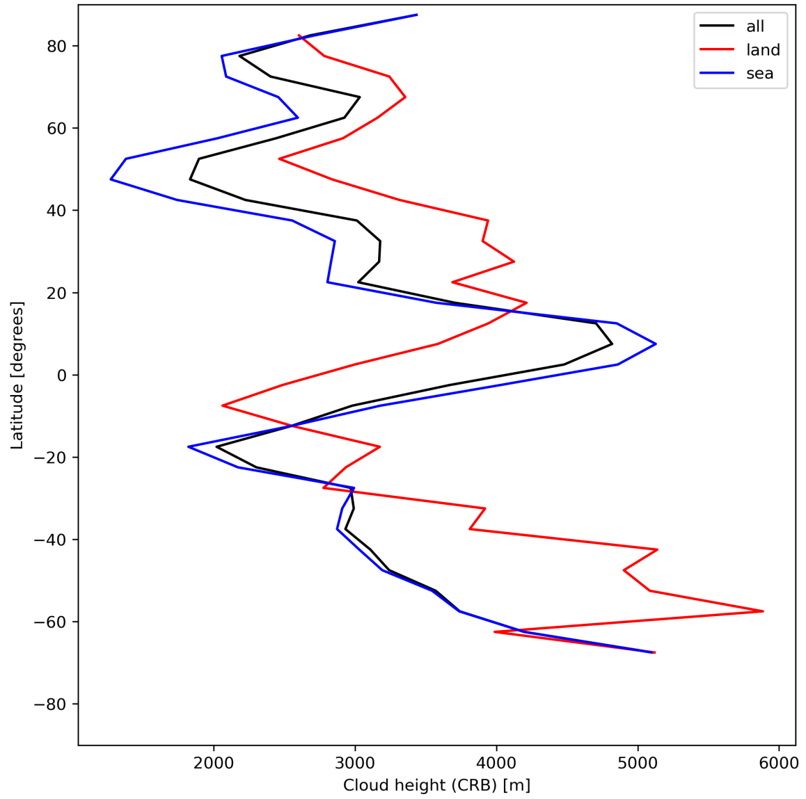
Figure 27: Zonal average of “Cloud height (CRB)” for 2023-07-17 to 2023-07-19.
