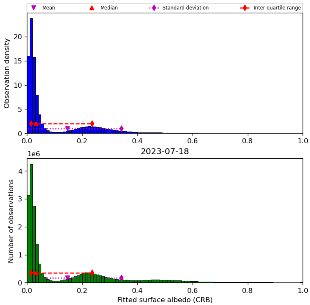
Figure 46: Histogram of “Fitted surface albedo (CRB)” for 2023-07-17 to 2023-07-19
