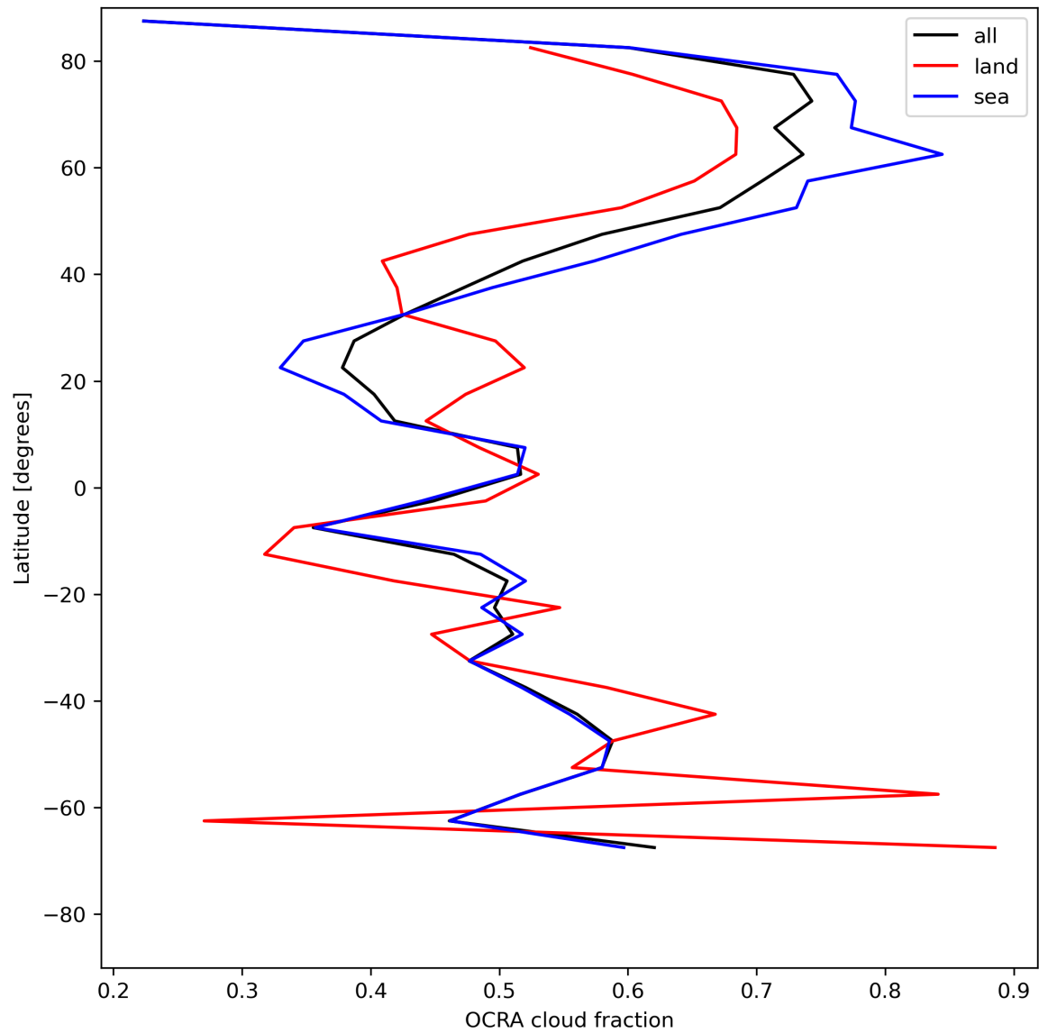
Figure 34: Zonal average of “OCRA cloud fraction” for 2023-07-17 to 2023-07-19.
