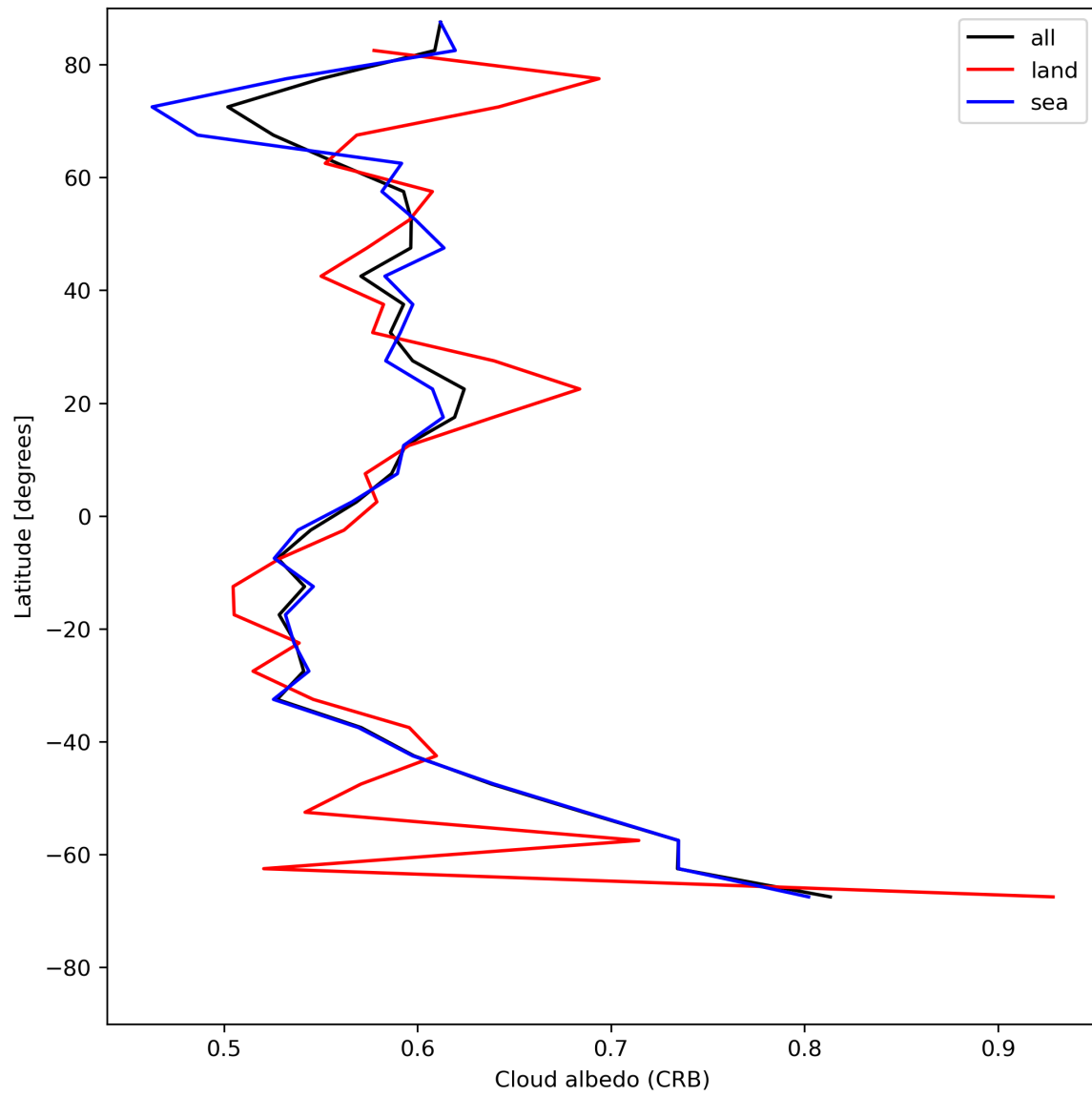
Figure 28: Zonal average of “Cloud albedo (CRB)” for 2023-07-17 to 2023-07-19.
