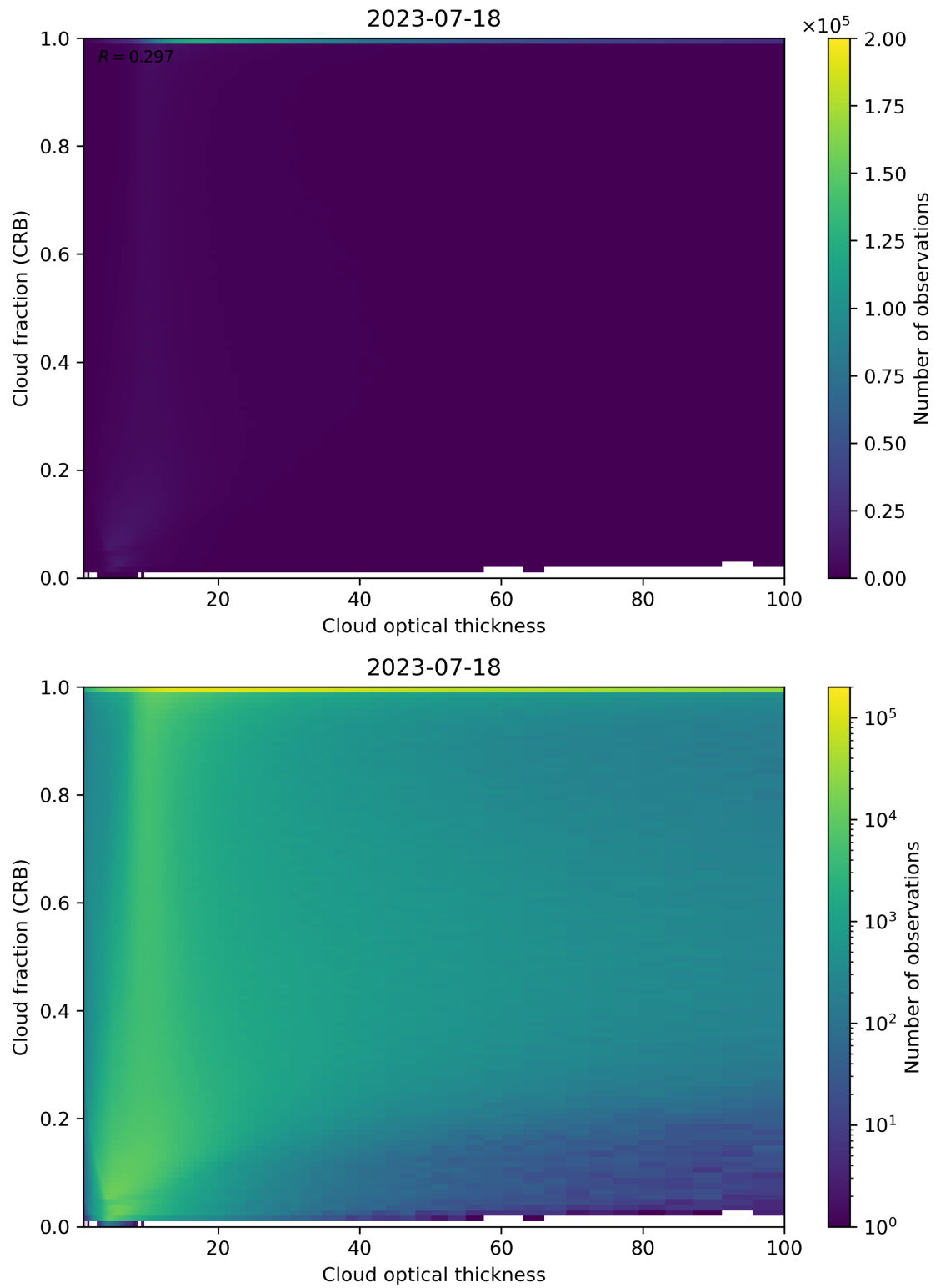
Figure 84: Scatter density plot of “Cloud optical thickness” against “Cloud fraction (CRB)” for 2023-07-17 to 2023-07-19.
