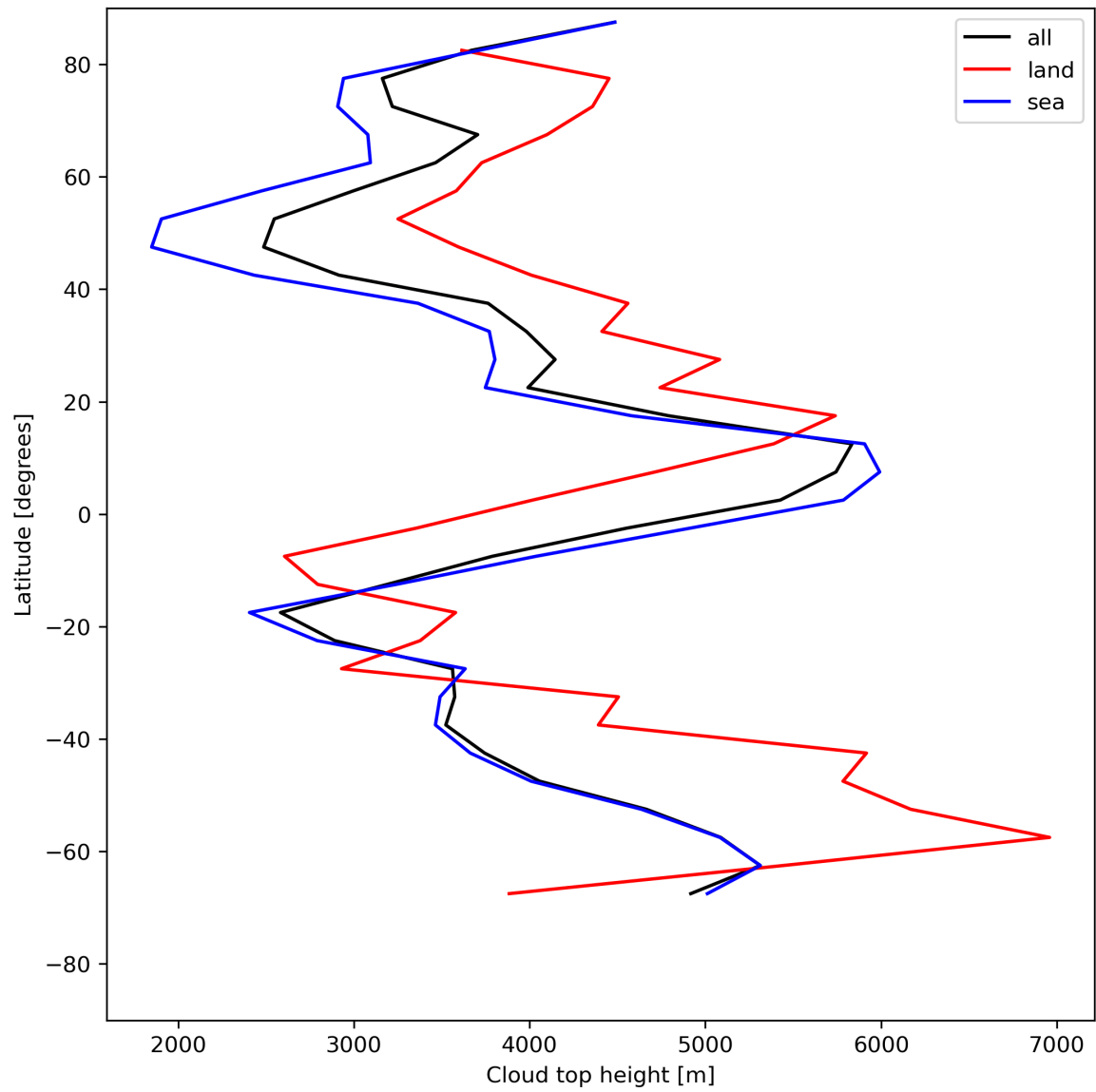
Figure 24: Zonal average of “Cloud top height” for 2023-07-17 to 2023-07-19.
