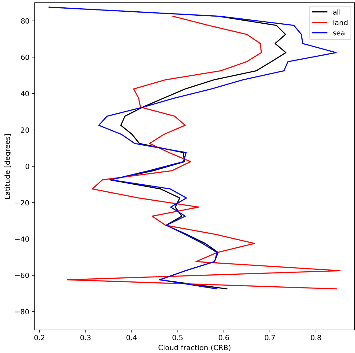
Figure 26: Zonal average of “Cloud fraction (CRB)” for 2023-07-17 to 2023-07-19.
