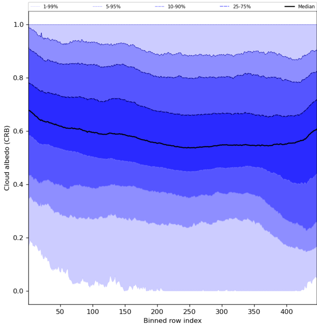
Figure 60: Along track statistics of “Cloud albedo (CRB)” for 2023-07-17 to 2023-07-19
