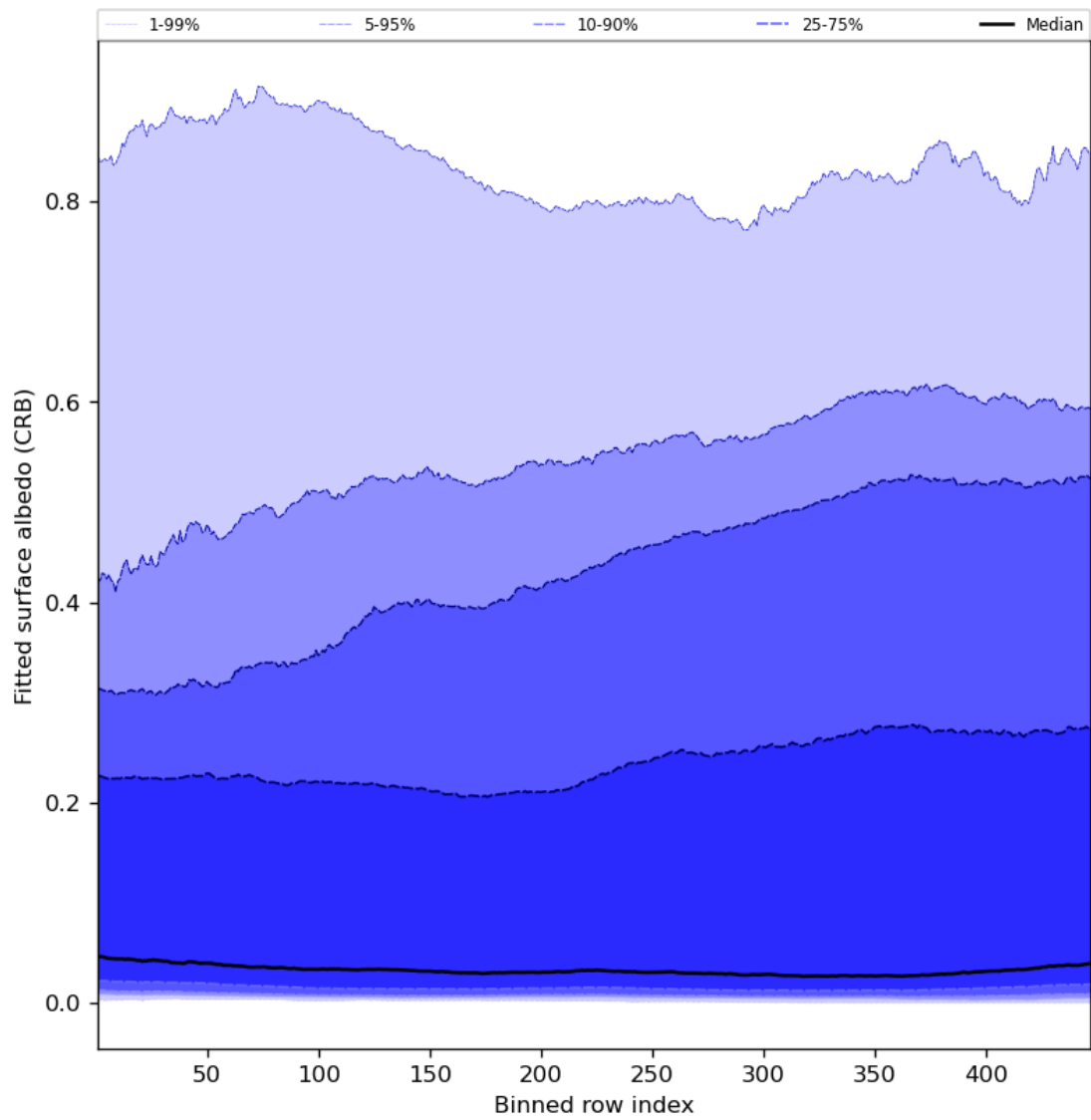
Figure 62: Along track statistics of “Fitted surface albedo (CRB)” for 2023-07-17 to 2023-07-19
