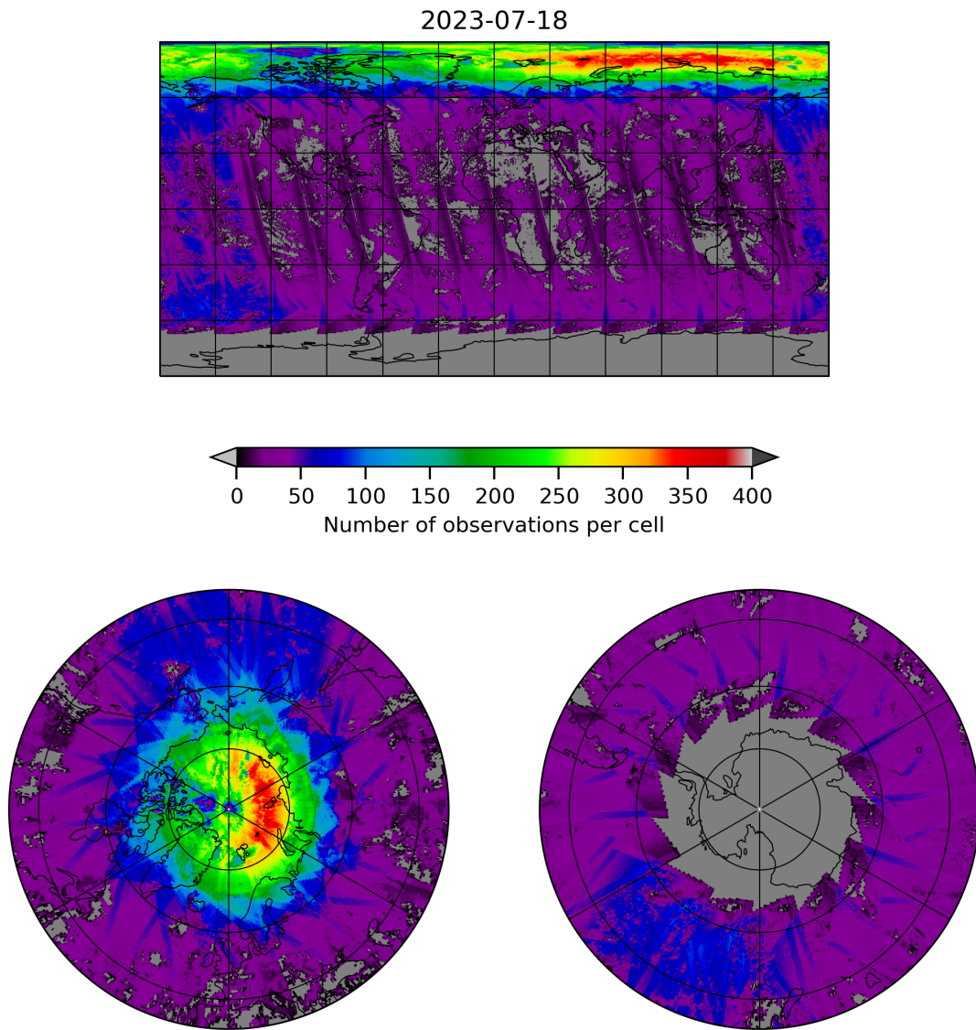
Figure 21: Map of the number of observations for 2023-07-17 to 2023-07-19
