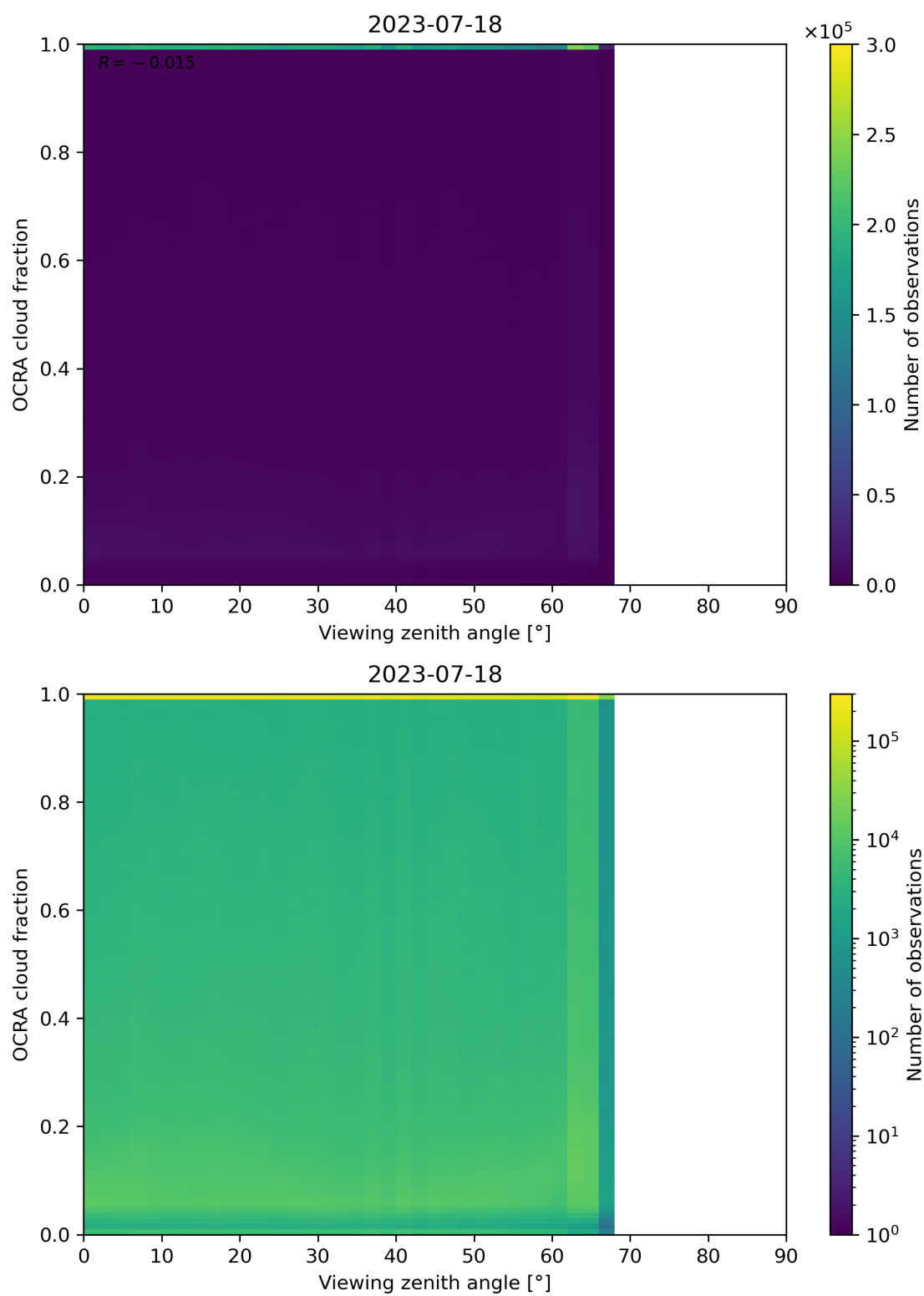
Figure 108: Scatter density plot of “Viewing zenith angle” against “OCRA cloud fraction” for 2023-07-17 to 2023-07-19.
