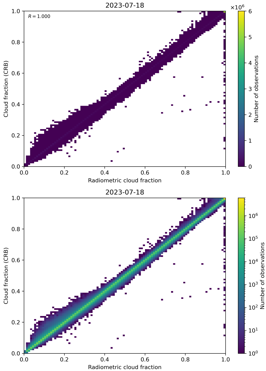
Figure 73: Scatter density plot of “Radiometric cloud fraction” against “Cloud fraction (CRB)” for 2023-07-17 to 2023-07-19.
