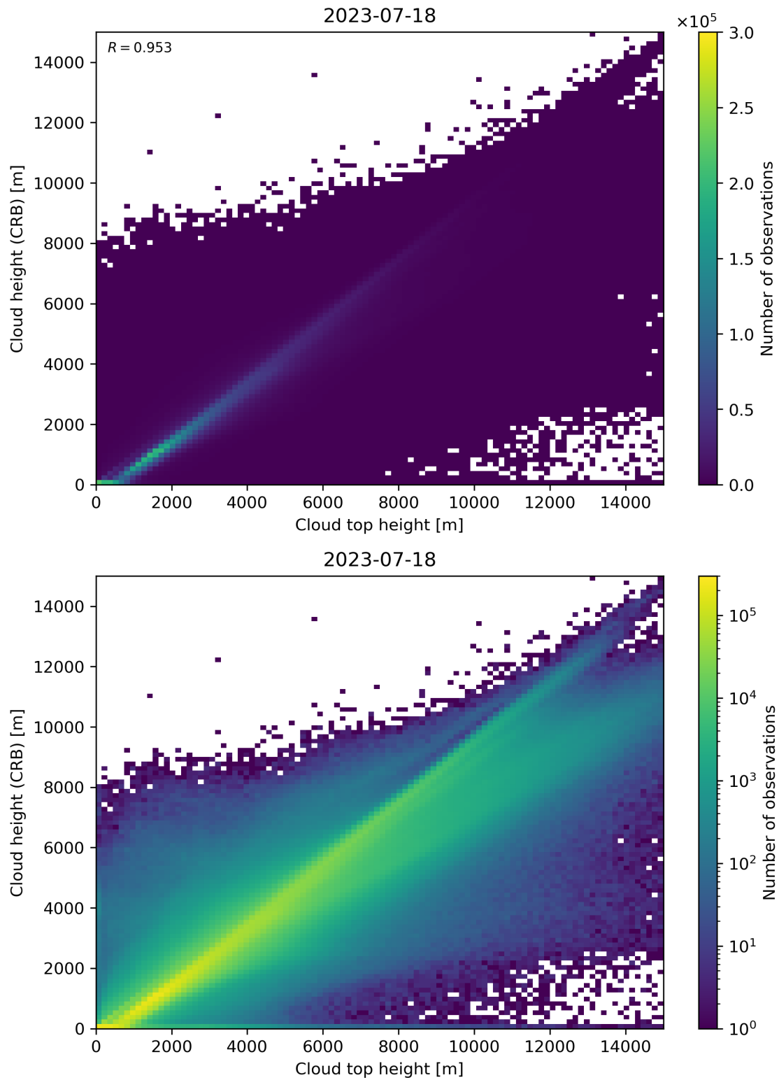
Figure 89: Scatter density plot of “Cloud top height” against “Cloud height (CRB)” for 2023-07-17 to 2023-07-19.
