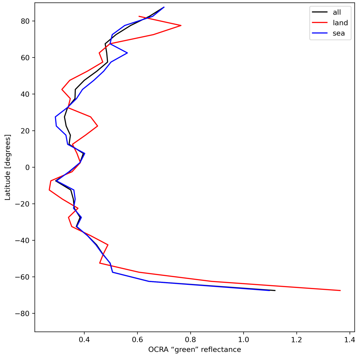
Figure 36: Zonal average of “OCRA “green” reflectance” for 2023-07-17 to 2023-07-19.
