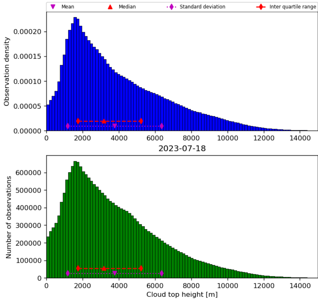
Figure 40: Histogram of “Cloud top height” for 2023-07-17 to 2023-07-19
