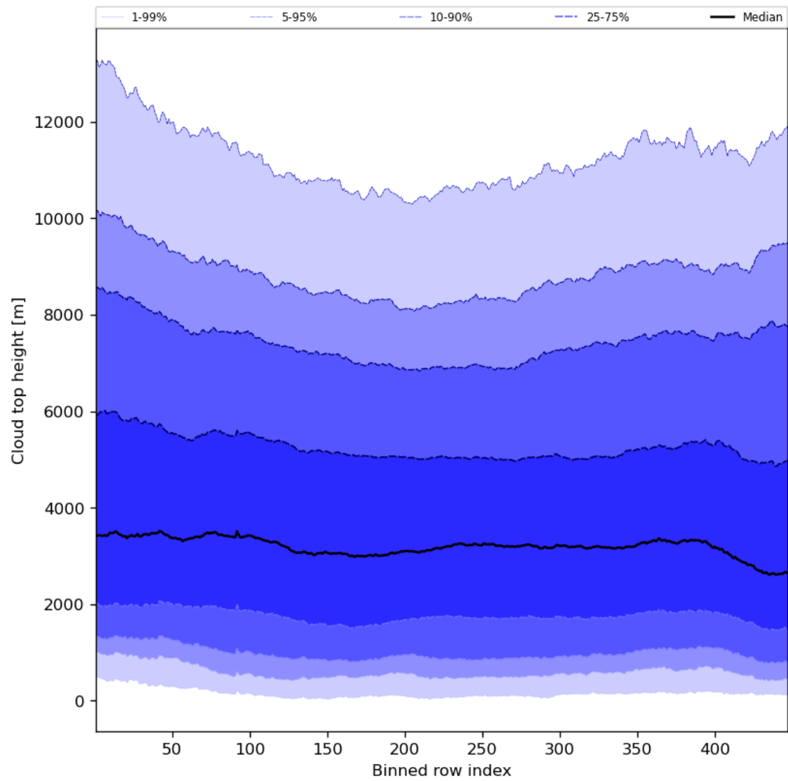
Figure 56: Along track statistics of “Cloud top height” for 2023-07-17 to 2023-07-19
