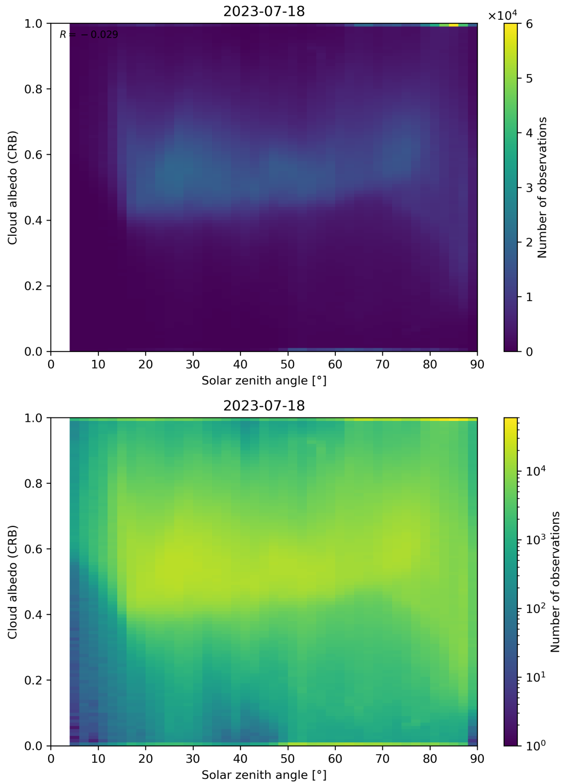
Figure 98: Scatter density plot of “Solar zenith angle” against “Cloud albedo (CRB)” for 2023-07-17 to 2023-07-19.
