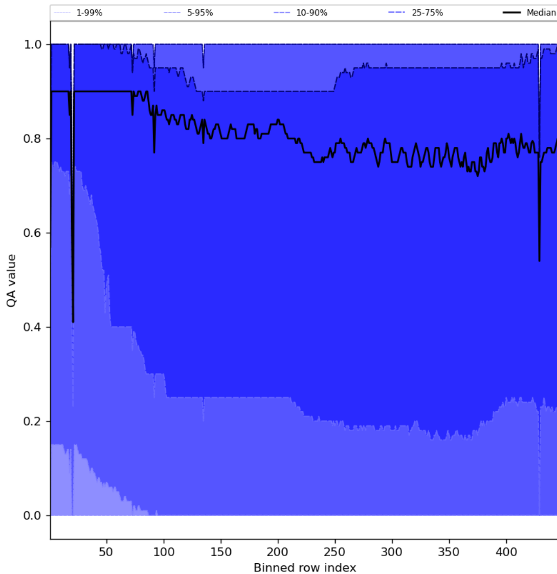
Figure 54: Along track statistics of “QA value” for 2023-07-17 to 2023-07-19
