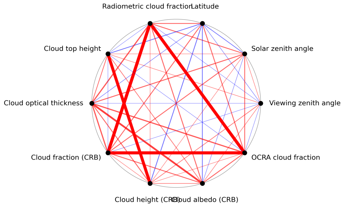
Figure 1: Map of correlation graph for 2023-07-17 to 2023-07-19.
