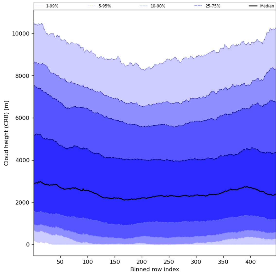
Figure 59: Along track statistics of “Cloud height (CRB)” for 2023-07-17 to 2023-07-19
