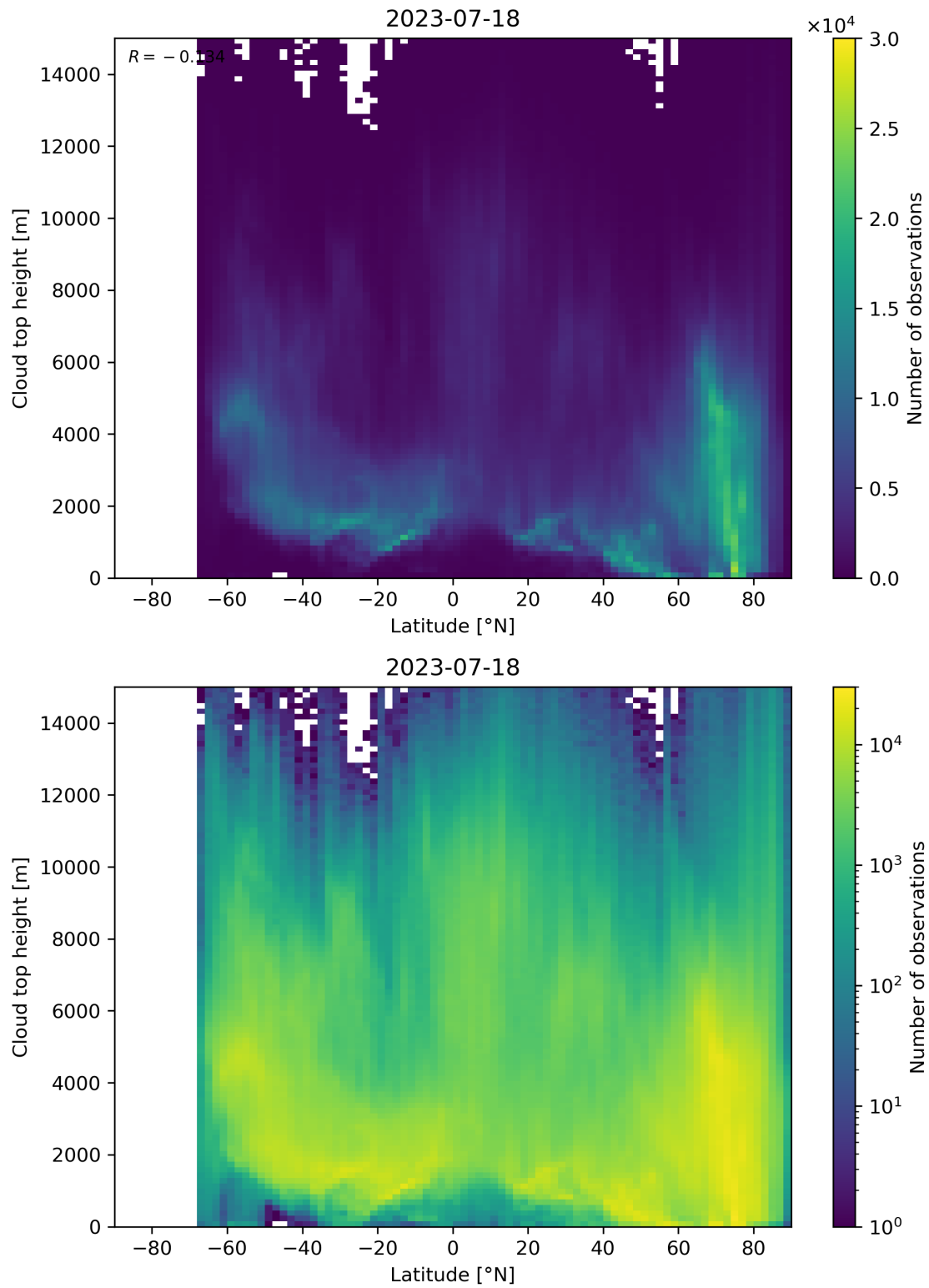
Figure 97: Scatter density plot of “Latitude” against “Cloud top height” for 2023-07-17 to 2023-07-19.
