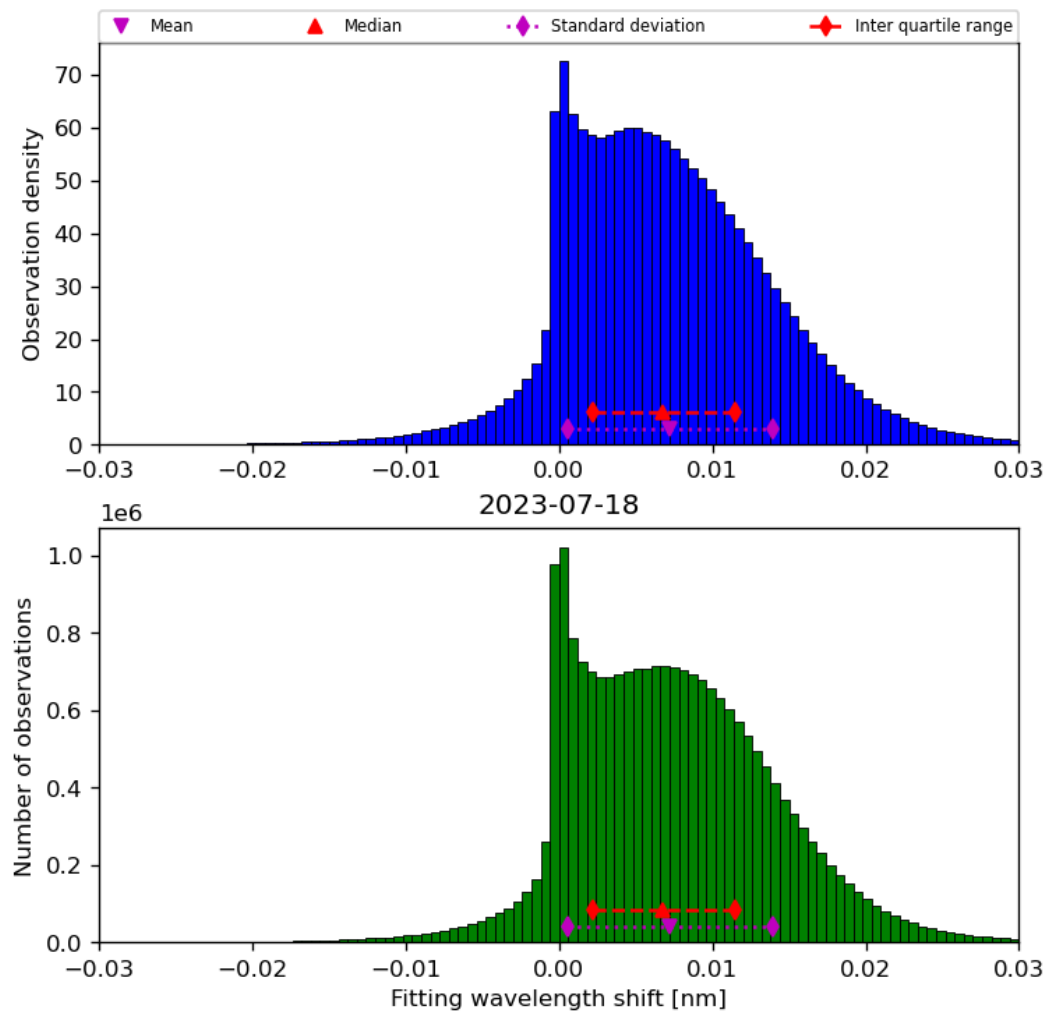
Figure 49: Histogram of “Fitting wavelength shift” for 2023-07-17 to 2023-07-19
