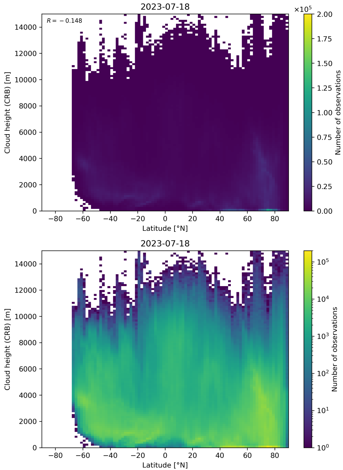
Figure 95: Scatter density plot of “Latitude” against “Cloud height (CRB)” for 2023-07-17 to 2023-07-19.
