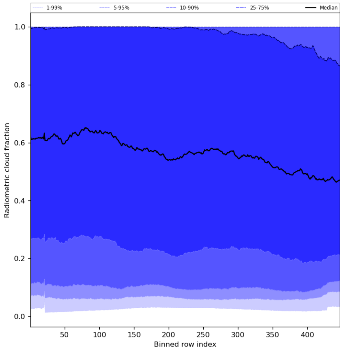
Figure 55: Along track statistics of “Radiometric cloud fraction” for 2023-07-17 to 2023-07-19
