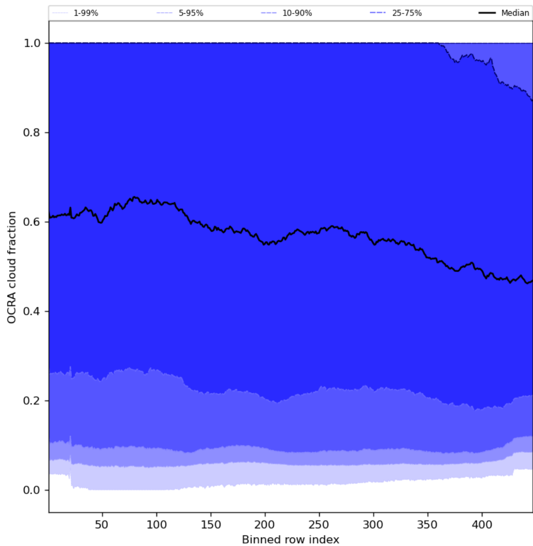
Figure 66: Along track statistics of “OCRA cloud fraction” for 2023-07-17 to 2023-07-19
