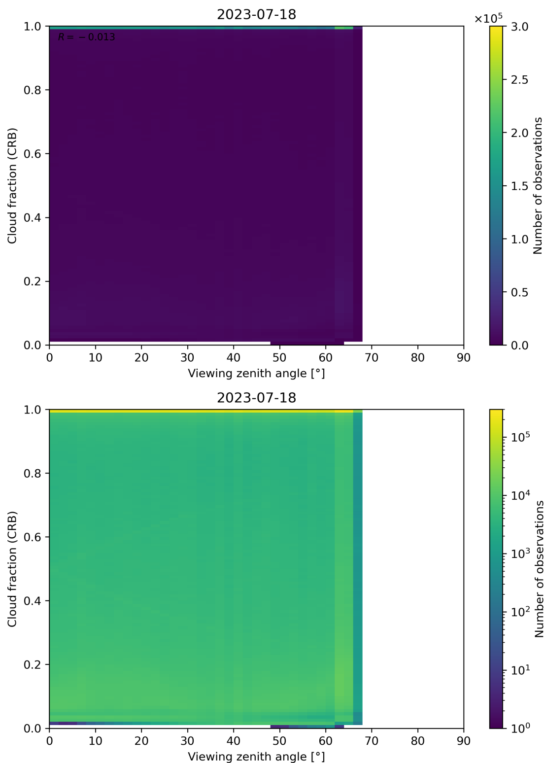
Figure 109: Scatter density plot of “Viewing zenith angle” against “Cloud fraction (CRB)” for 2023-07-17 to 2023-07-19.
