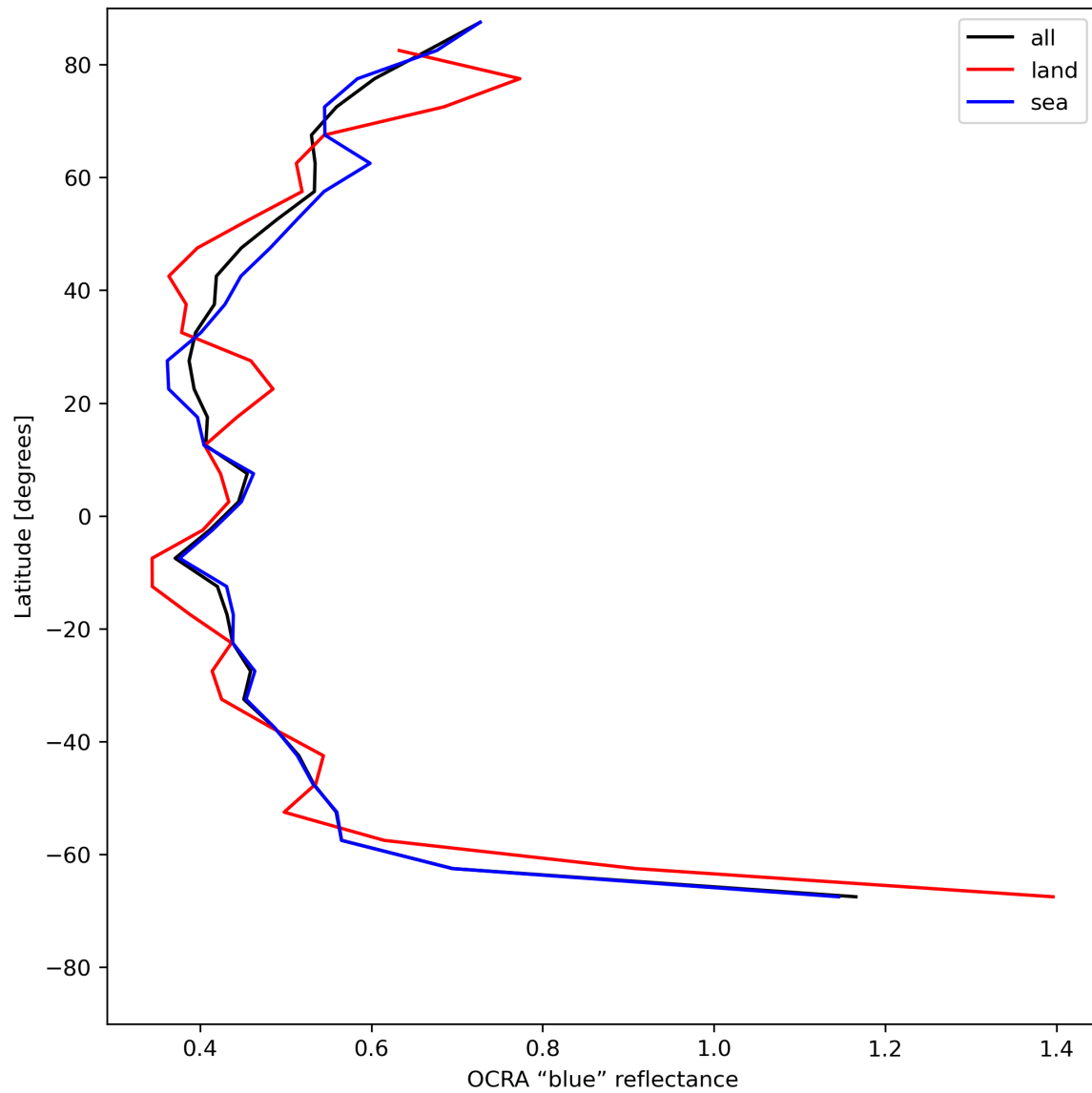
Figure 35: Zonal average of “OCRA “blue” reflectance” for 2023-07-17 to 2023-07-19.
