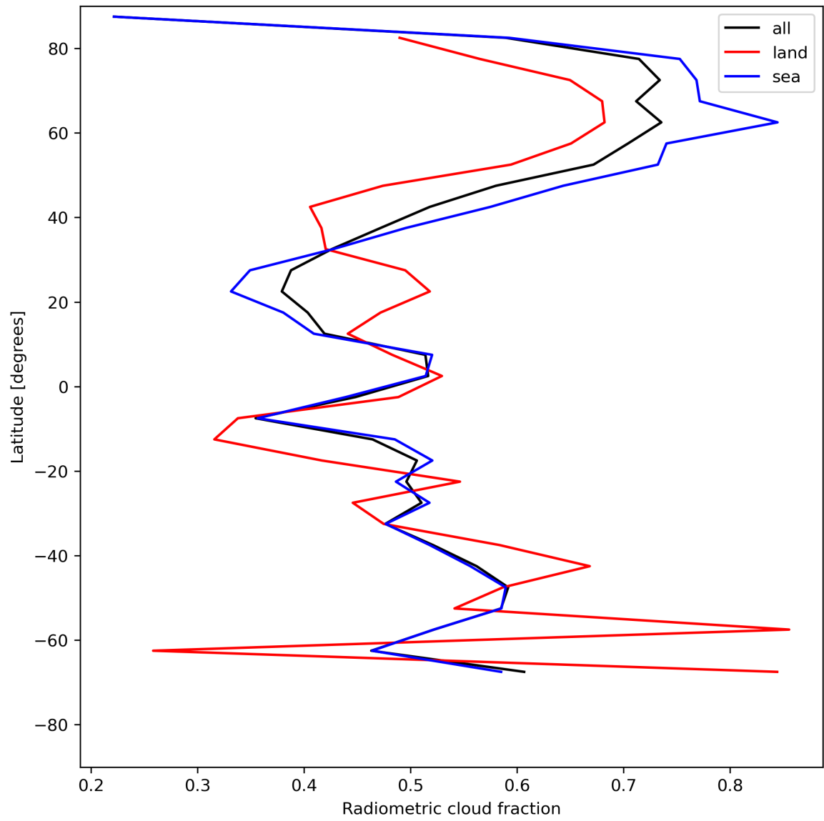
Figure 23: Zonal average of “Radiometric cloud fraction” for 2023-07-17 to 2023-07-19.
