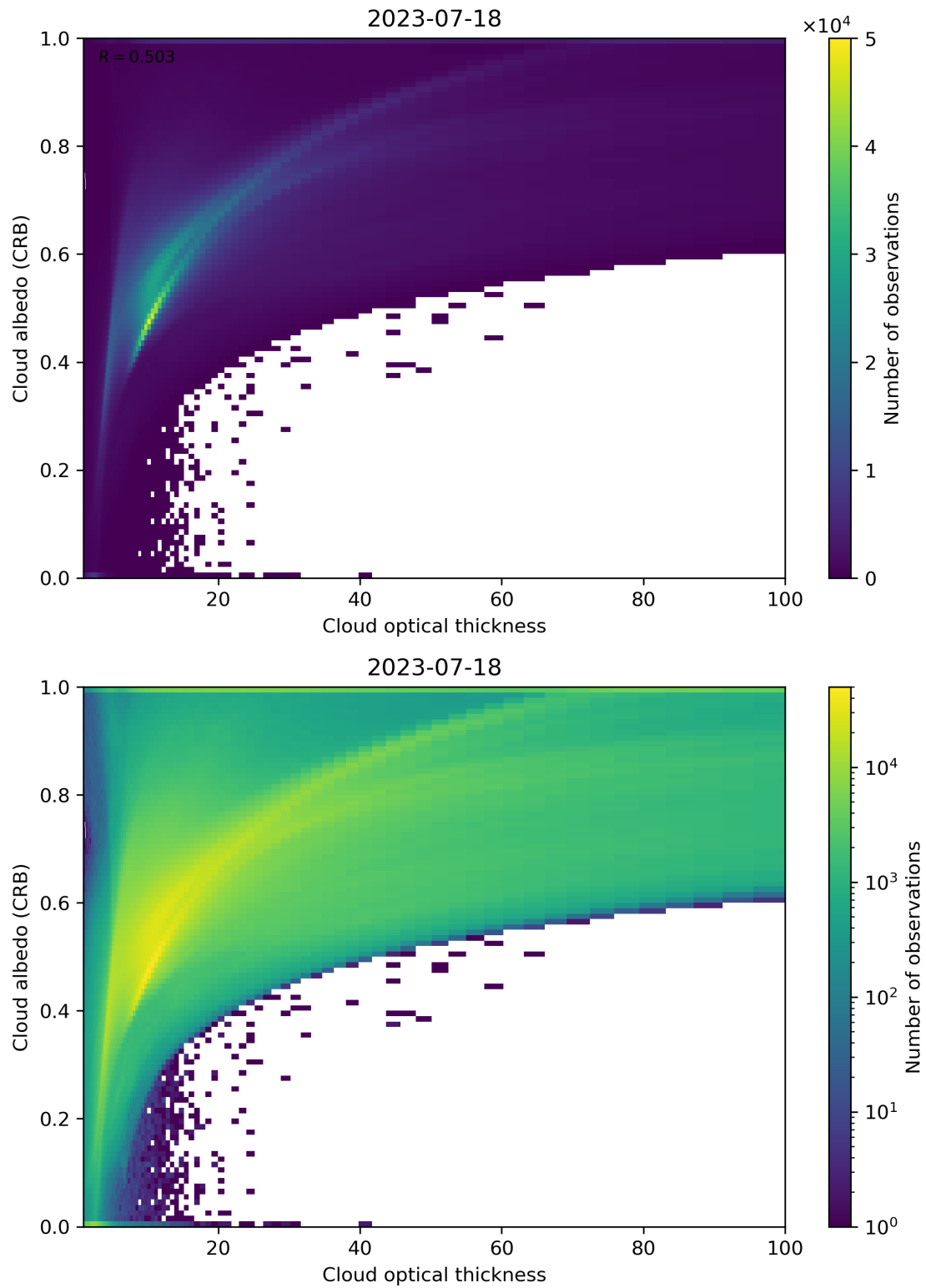
Figure 82: Scatter density plot of “Cloud optical thickness” against “Cloud albedo (CRB)” for 2023-07-17 to 2023-07-19.
