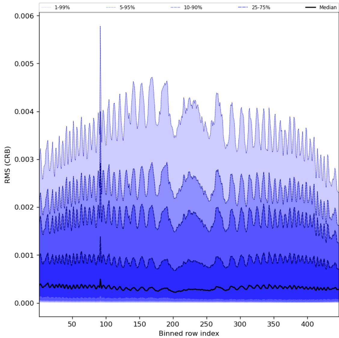
Figure 64: Along track statistics of “RMS (CRB)” for 2023-07-17 to 2023-07-19
