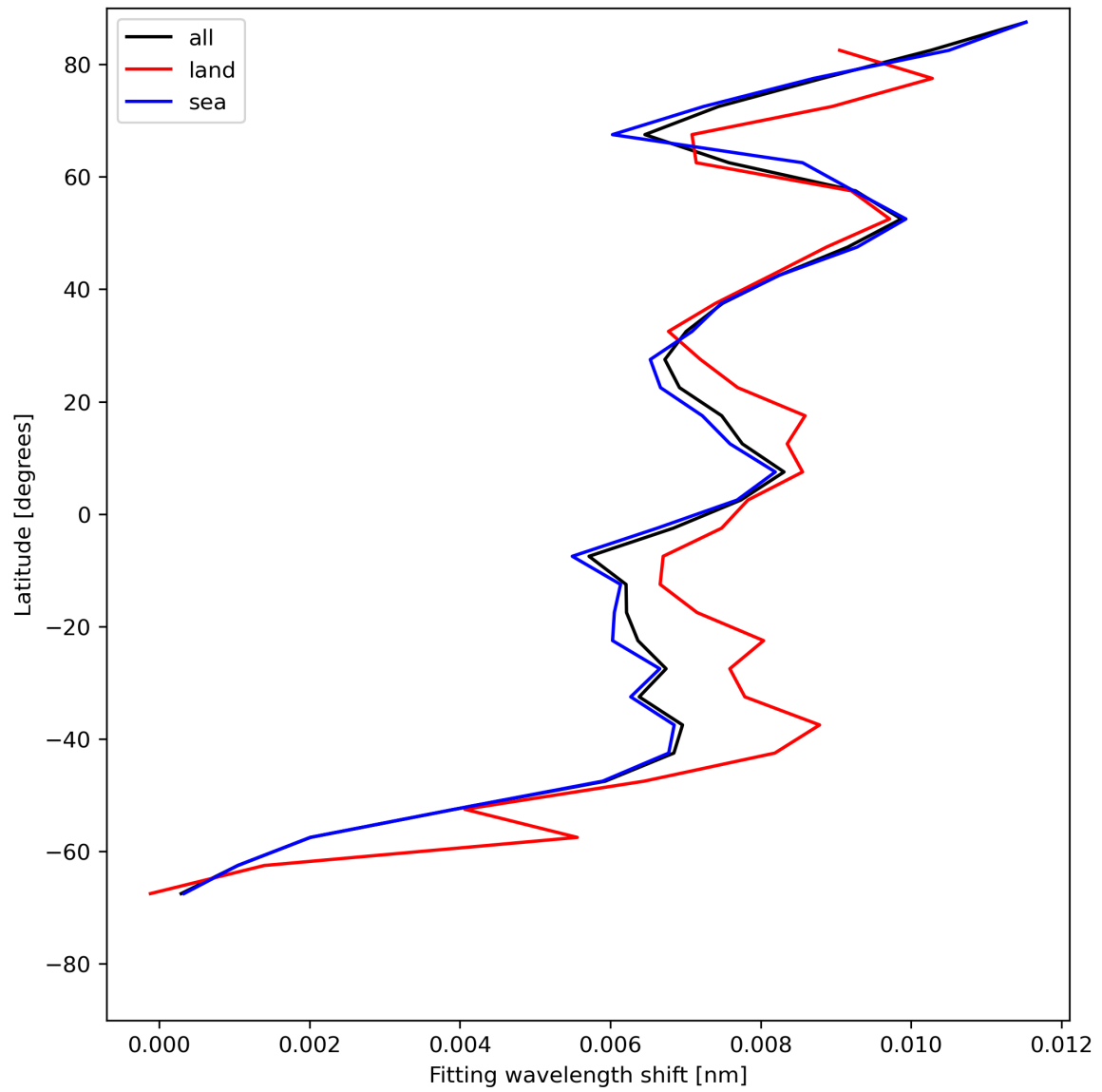
Figure 33: Zonal average of “Fitting wavelength shift” for 2023-07-17 to 2023-07-19.
