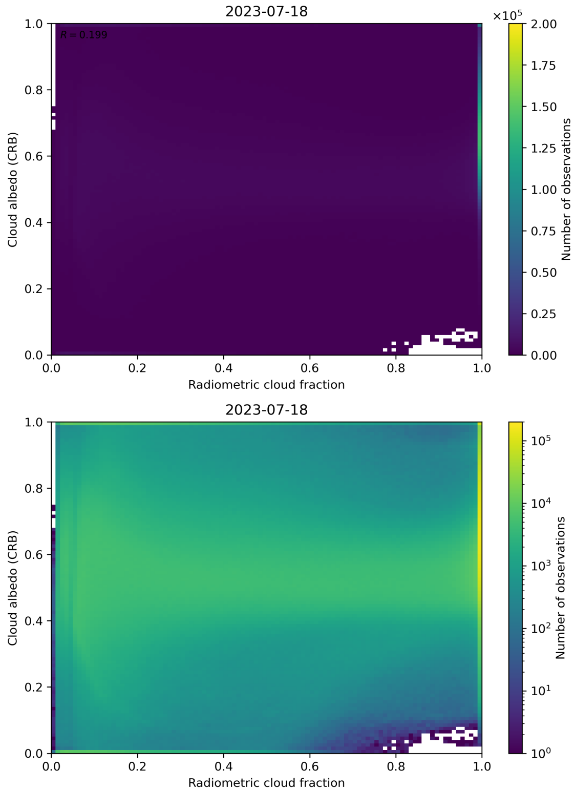
Figure 71: Scatter density plot of “Radiometric cloud fraction” against “Cloud albedo (CRB)” for 2023-07-17 to 2023-07-19.
