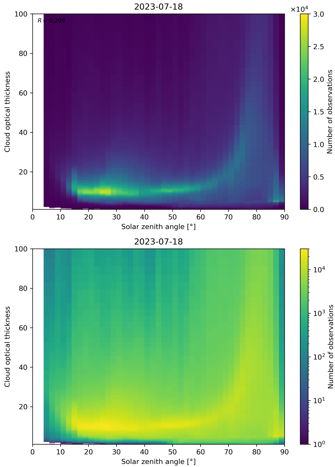
Figure 103: Scatter density plot of “Solar zenith angle” against “Cloud optical thickness” for 2023-07-17 to 2023-07-19.
