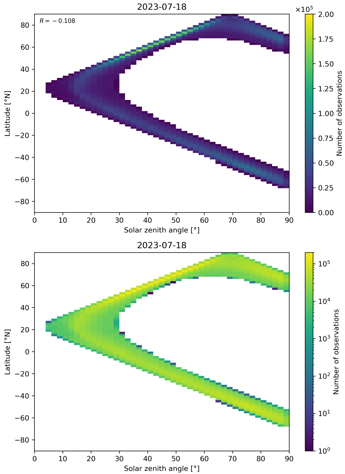
Figure 105: Scatter density plot of “Solar zenith angle” against “Latitude” for 2023-07-17 to 2023-07-19.
