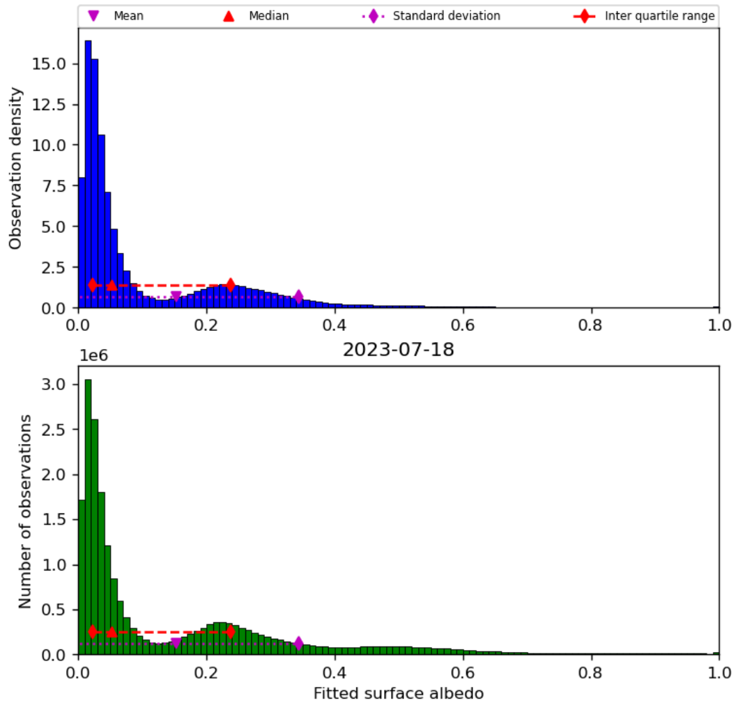
Figure 45: Histogram of “Fitted surface albedo” for 2023-07-17 to 2023-07-19
