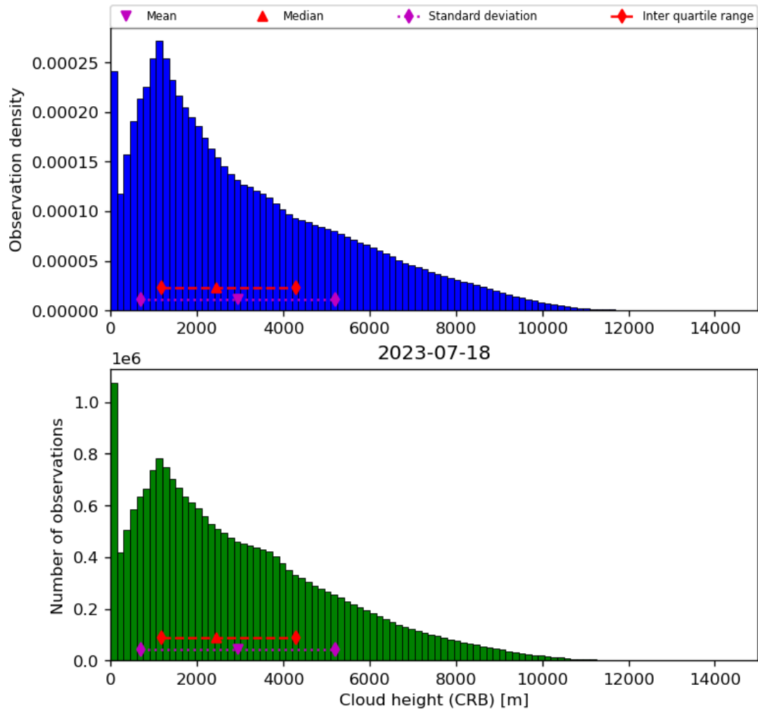
Figure 43: Histogram of “Cloud height (CRB)” for 2023-07-17 to 2023-07-19
