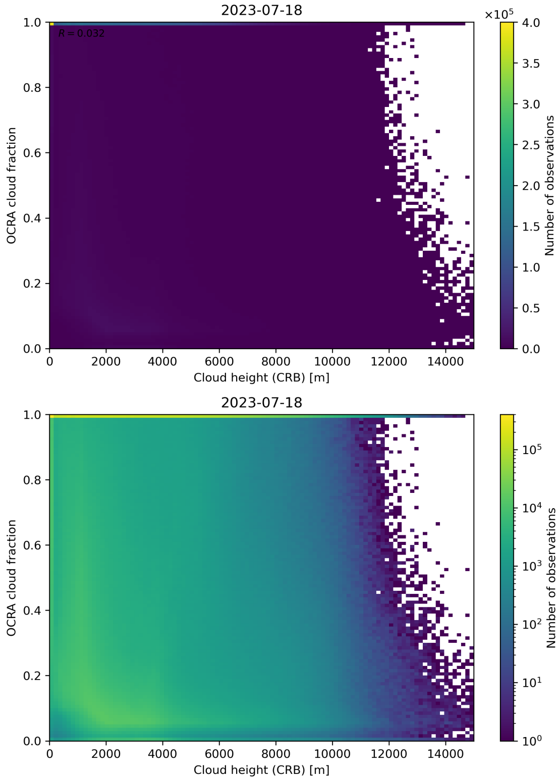
Figure 81: Scatter density plot of “Cloud height (CRB)” against “OCRA cloud fraction” for 2023-07-17 to 2023-07-19.
