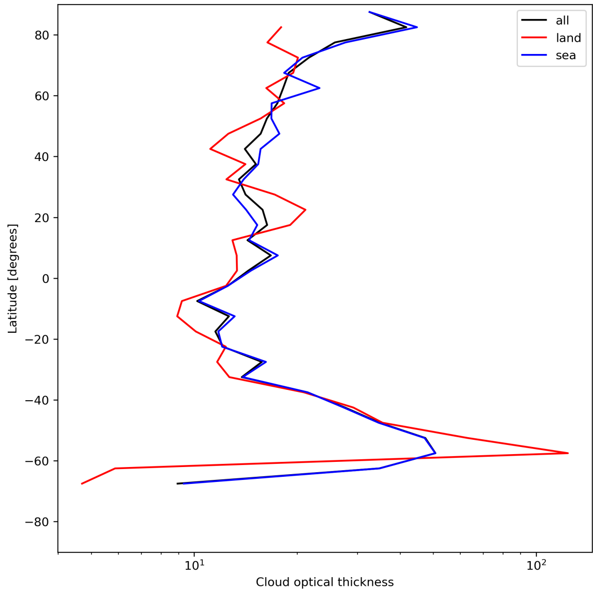
Figure 25: Zonal average of “Cloud optical thickness” for 2023-07-17 to 2023-07-19.
