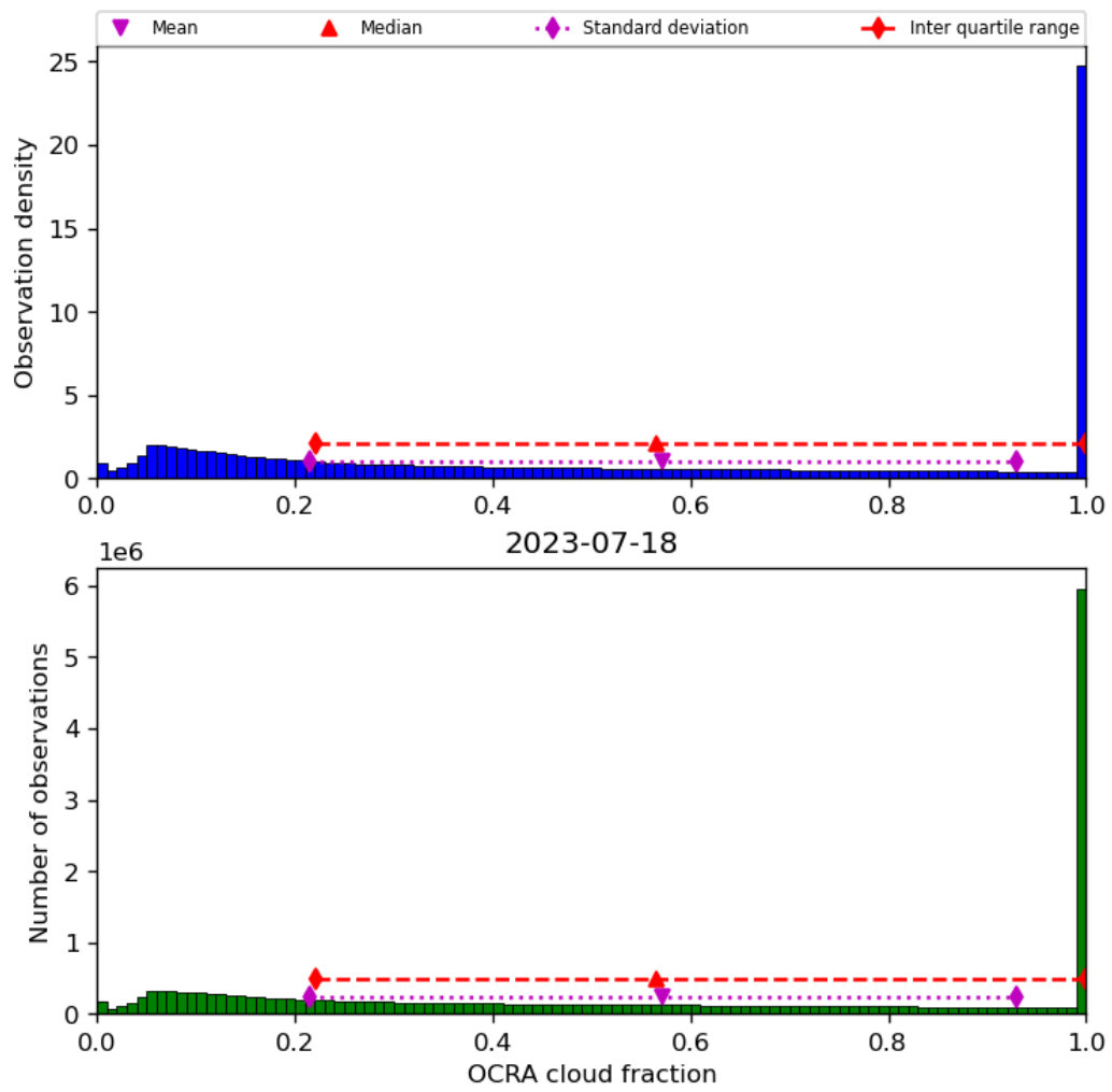
Figure 50: Histogram of “OCRA cloud fraction” for 2023-07-17 to 2023-07-19
