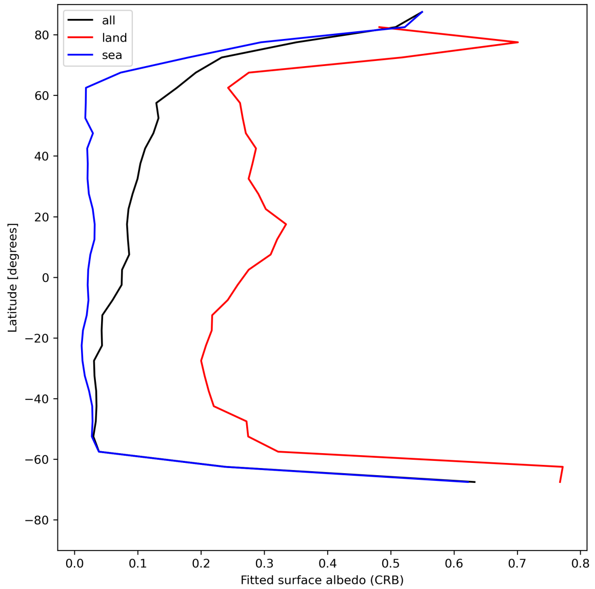
Figure 30: Zonal average of “Fitted surface albedo (CRB)” for 2023-07-17 to 2023-07-19.
