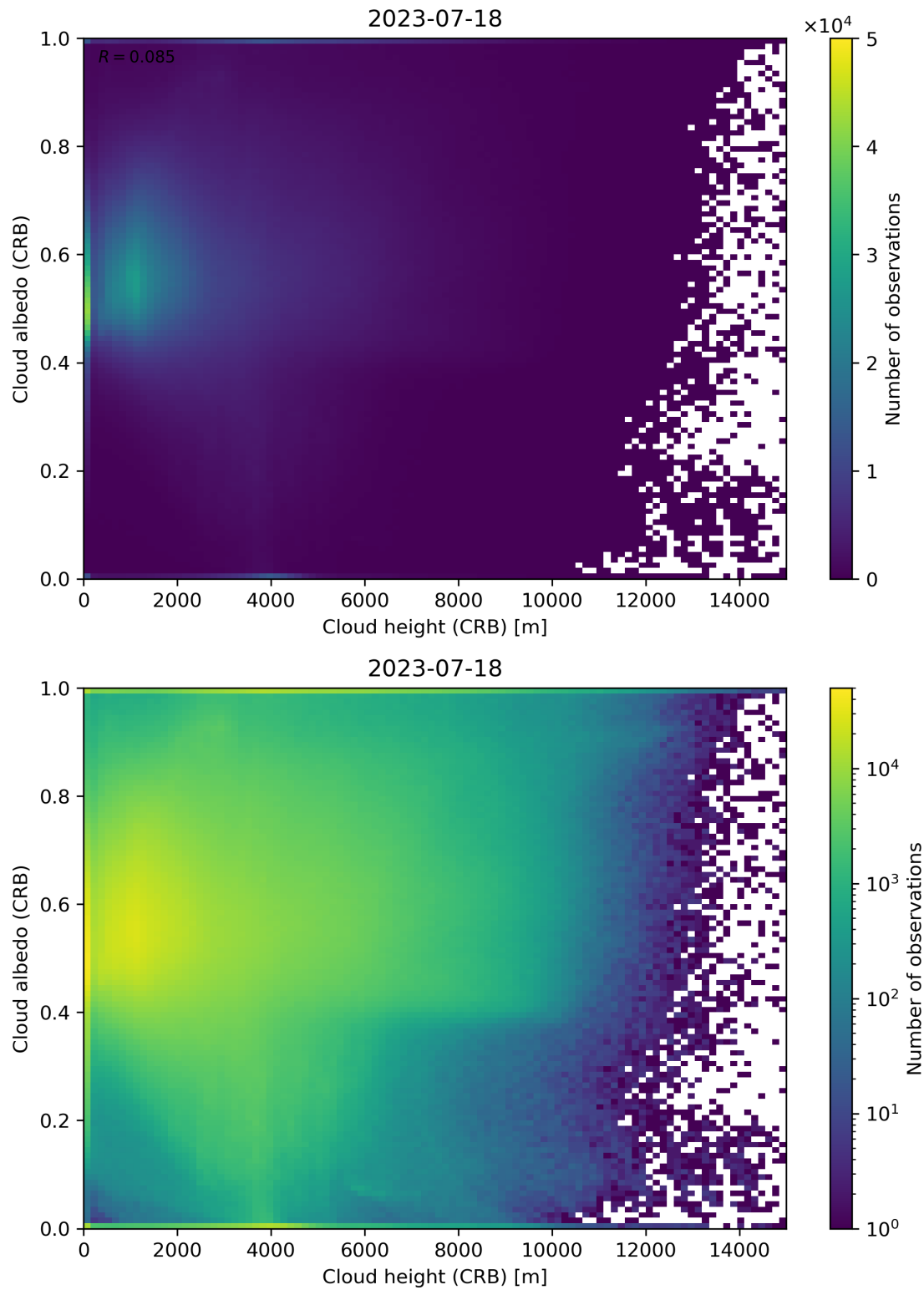
Figure 80: Scatter density plot of “Cloud height (CRB)” against “Cloud albedo (CRB)” for 2023-07-17 to 2023-07-19.
