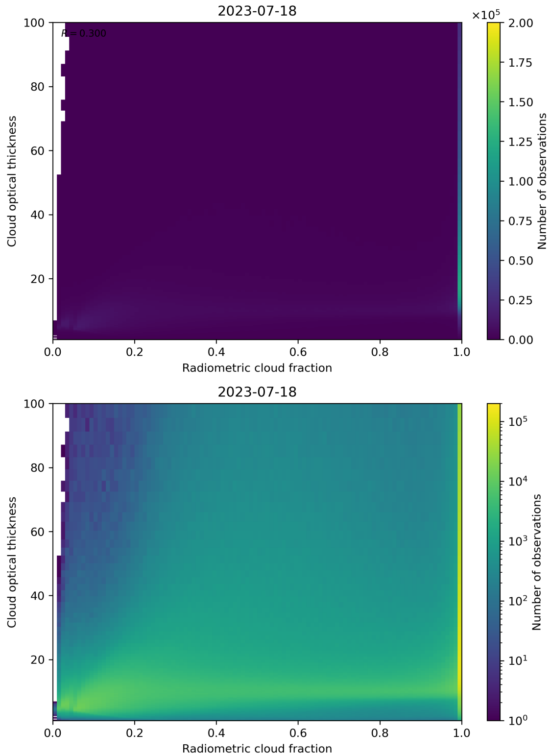
Figure 75: Scatter density plot of “Radiometric cloud fraction” against “Cloud optical thickness” for 2023-07-17 to 2023-07-19.
