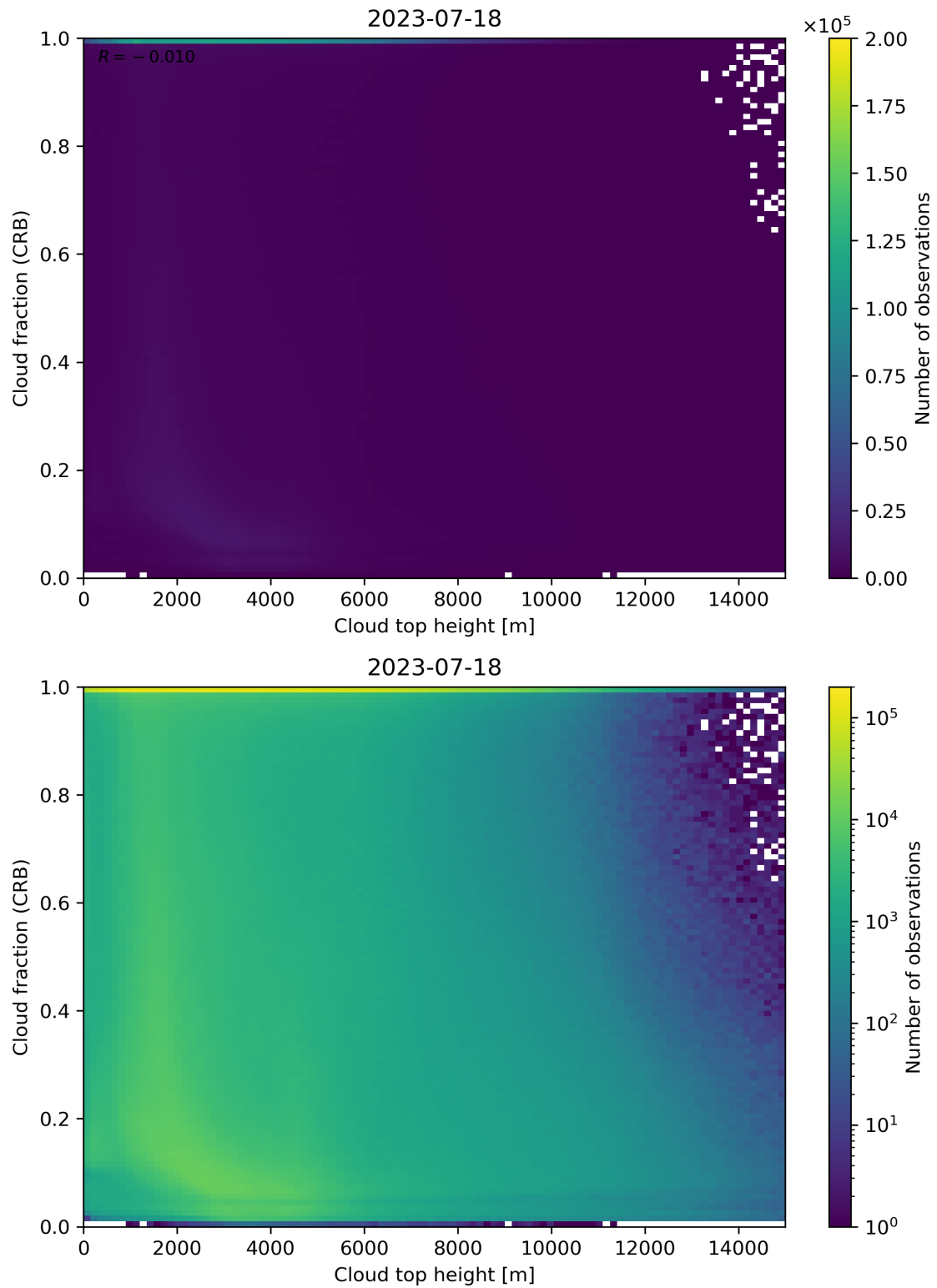
Figure 88: Scatter density plot of “Cloud top height” against “Cloud fraction (CRB)” for 2023-07-17 to 2023-07-19.
