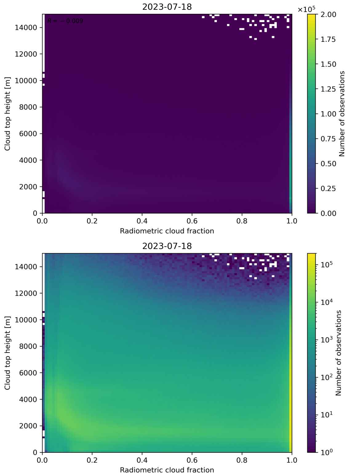
Figure 76: Scatter density plot of “Radiometric cloud fraction” against “Cloud top height” for 2023-07-17 to 2023-07-19.
