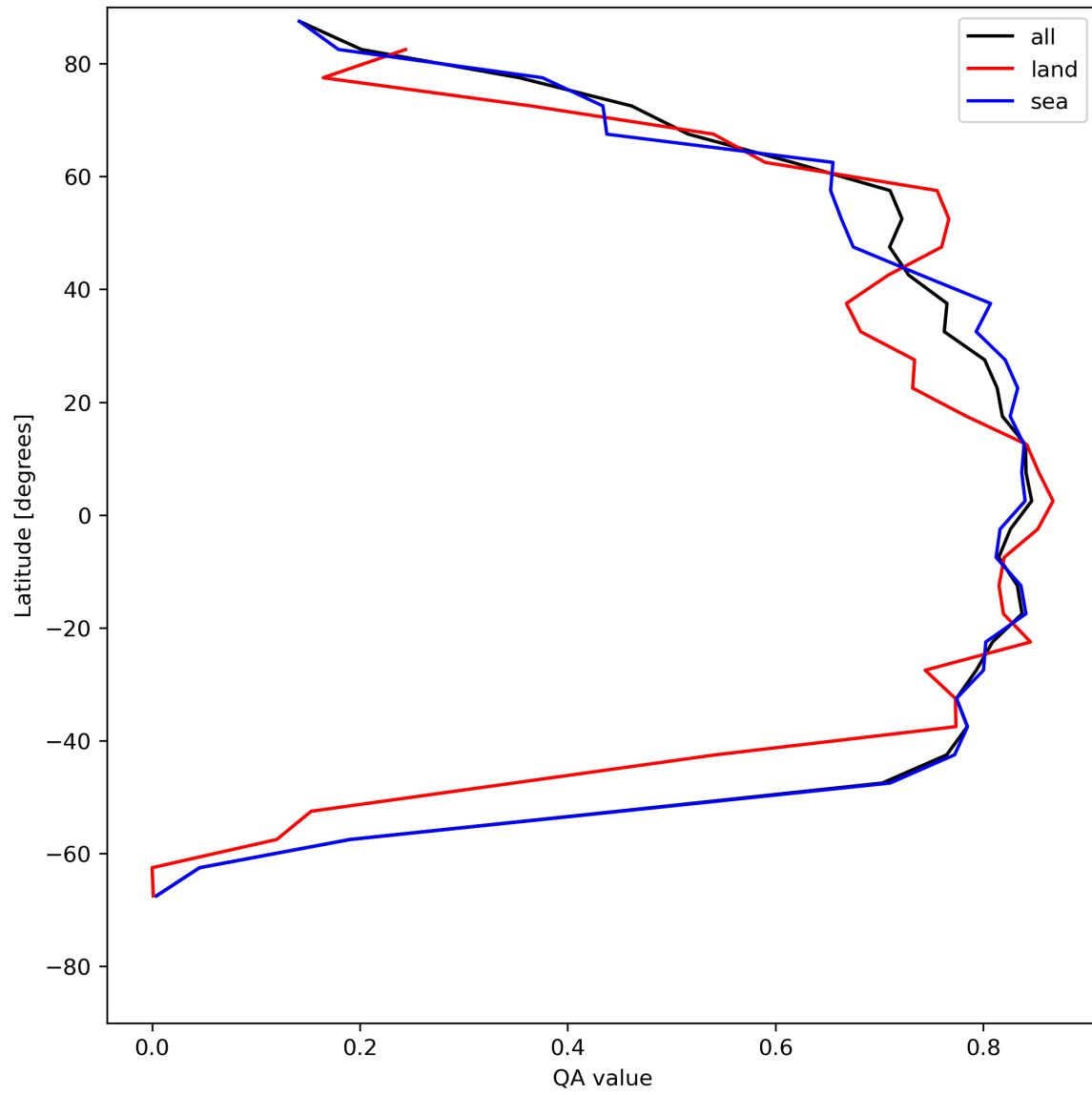
Figure 22: Zonal average of “QA value” for 2023-07-17 to 2023-07-19.
