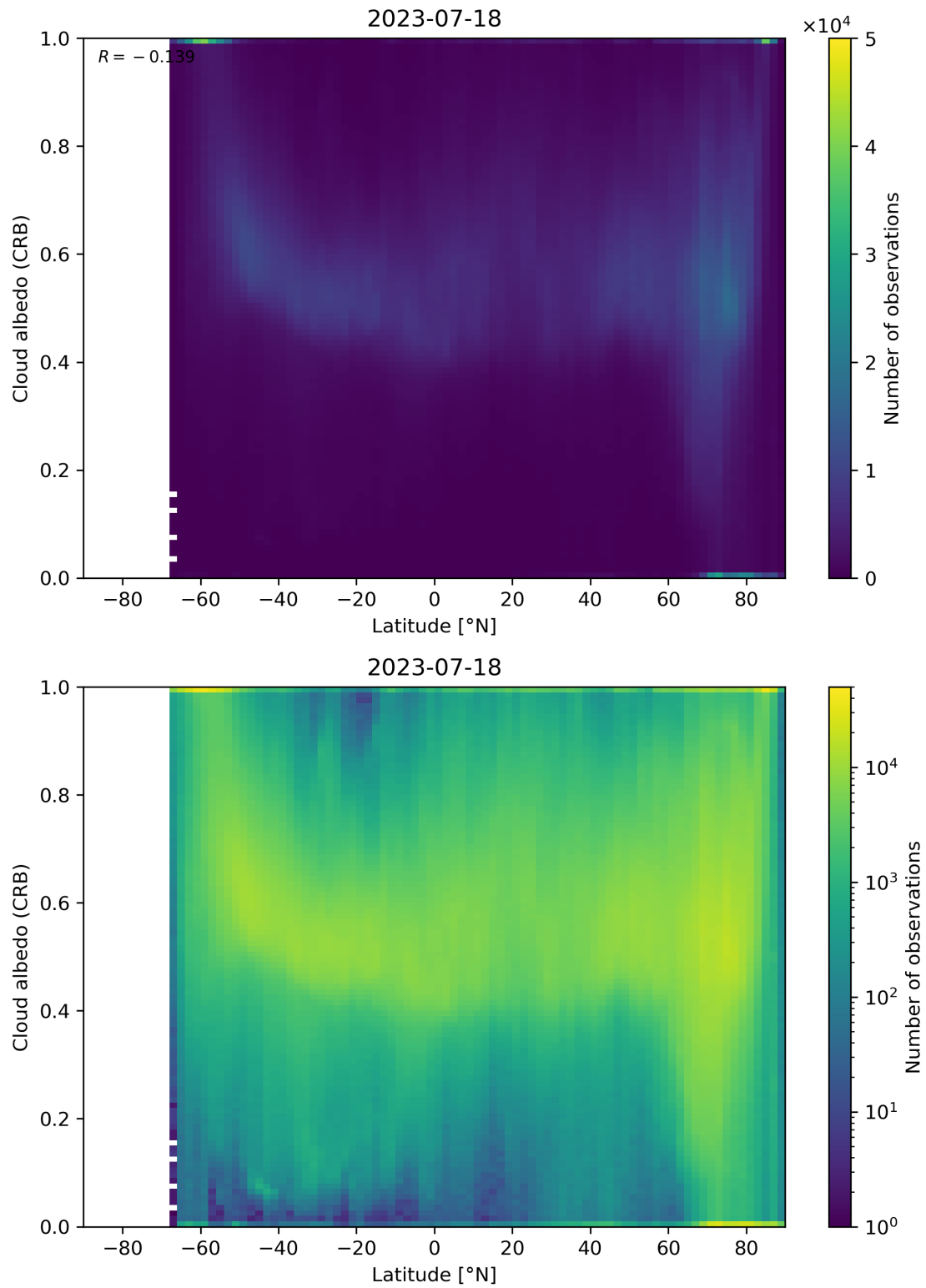
Figure 91: Scatter density plot of “Latitude” against “Cloud albedo (CRB)” for 2023-07-17 to 2023-07-19.
