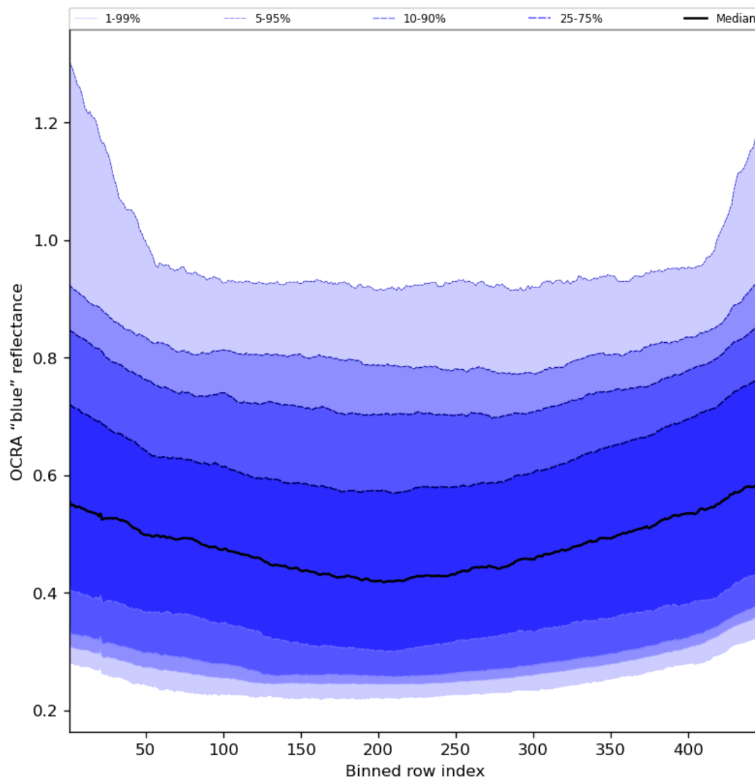
Figure 67: Along track statistics of “OCRA “blue” reflectance” for 2023-07-17 to 2023-07-19
