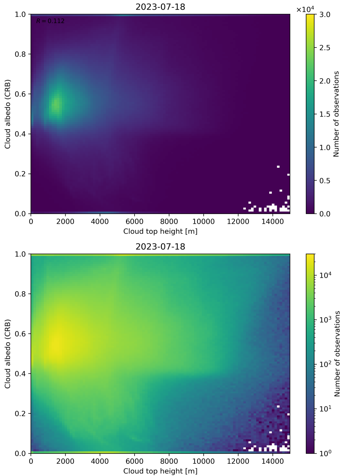
Figure 86: Scatter density plot of “Cloud top height” against “Cloud albedo (CRB)” for 2023-07-17 to 2023-07-19.
