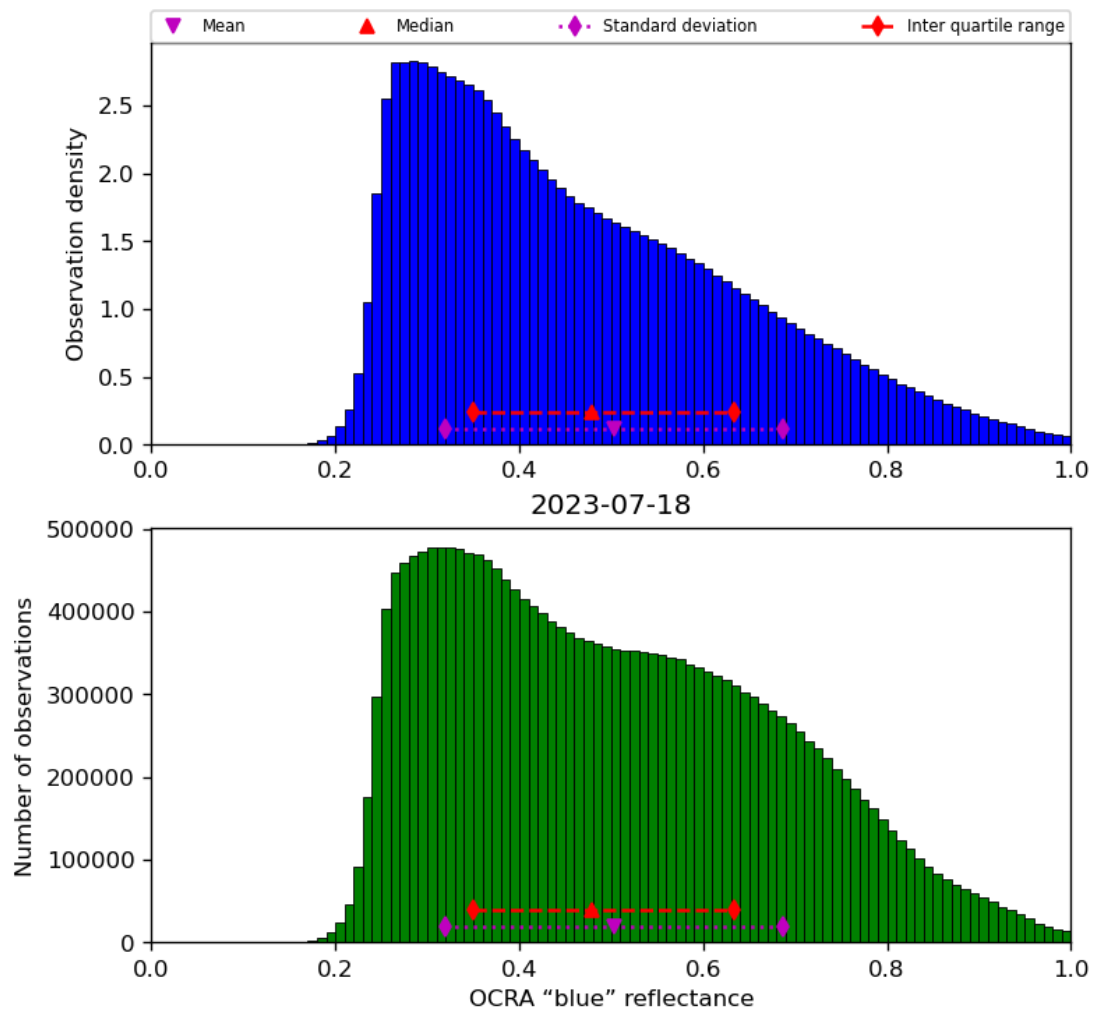
Figure 51: Histogram of “OCRA “blue” reflectance” for 2023-07-17 to 2023-07-19
