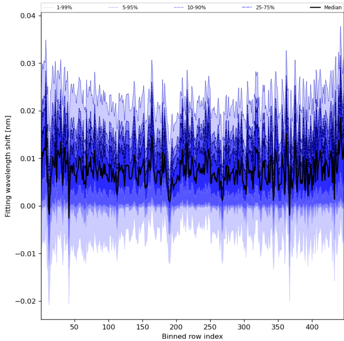
Figure 65: Along track statistics of “Fitting wavelength shift” for 2023-07-17 to 2023-07-19
