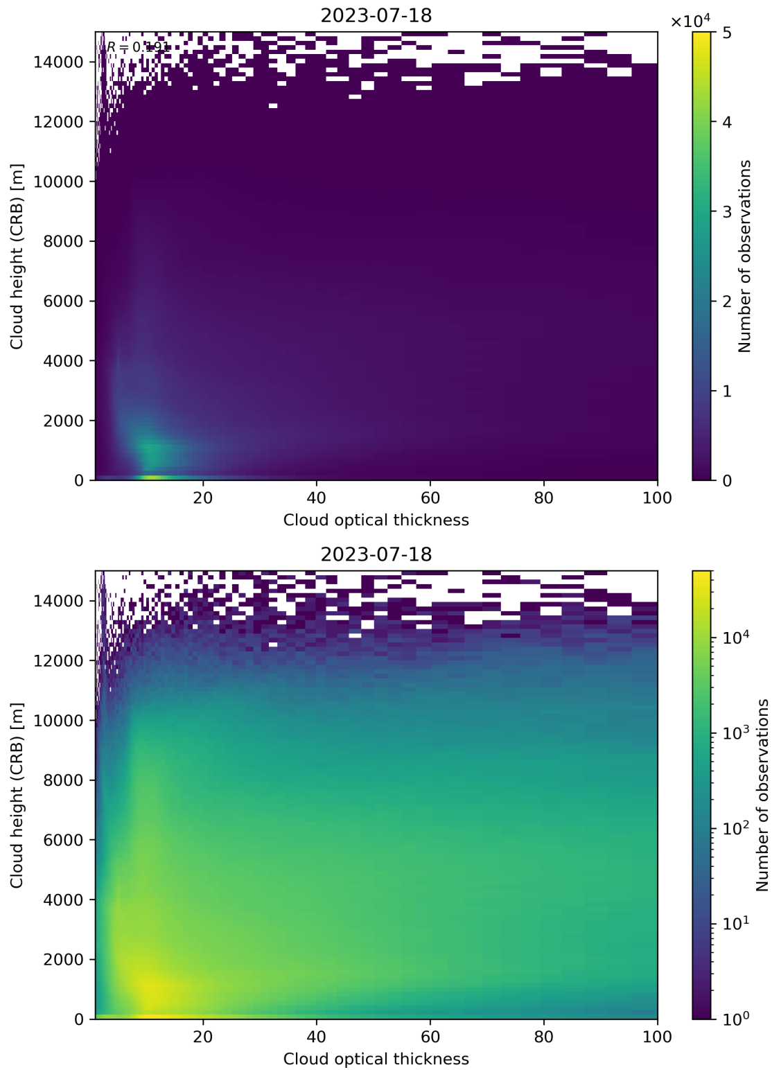
Figure 85: Scatter density plot of “Cloud optical thickness” against “Cloud height (CRB)” for 2023-07-17 to 2023-07-19.
