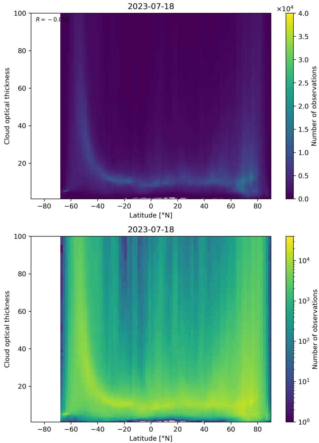
Figure 96: Scatter density plot of “Latitude” against “Cloud optical thickness” for 2023-07-17 to 2023-07-19.
