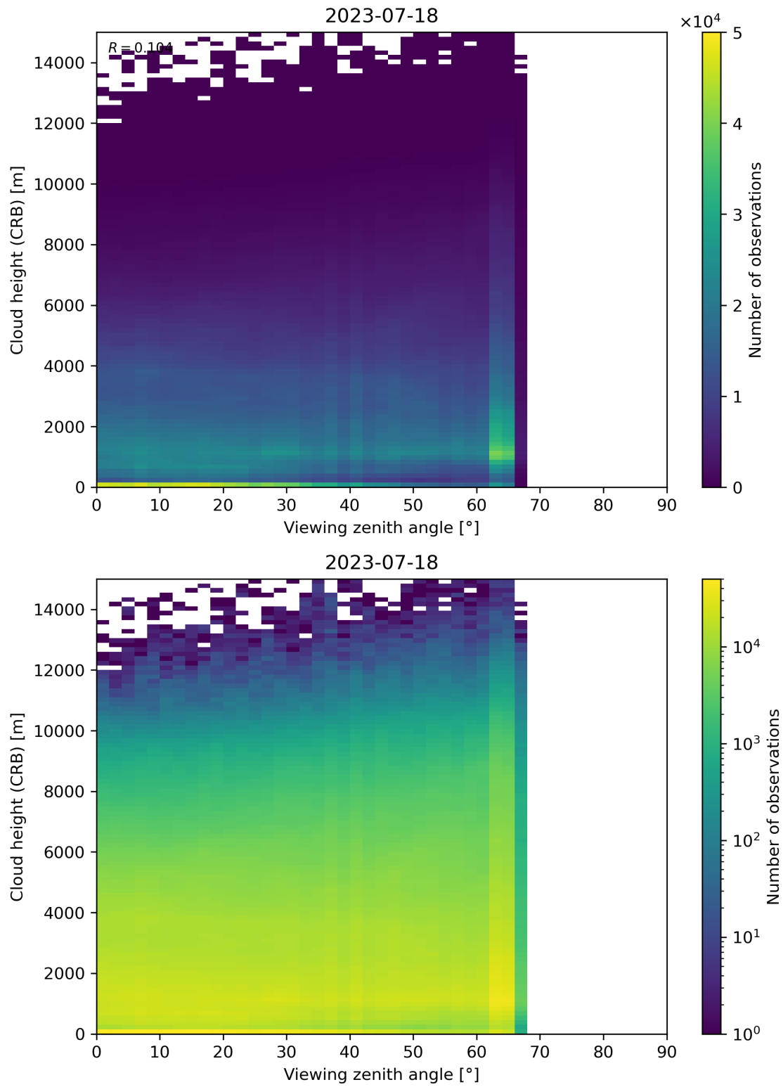
Figure 110: Scatter density plot of “Viewing zenith angle” against “Cloud height (CRB)” for 2023-07-17 to 2023-07-19.
