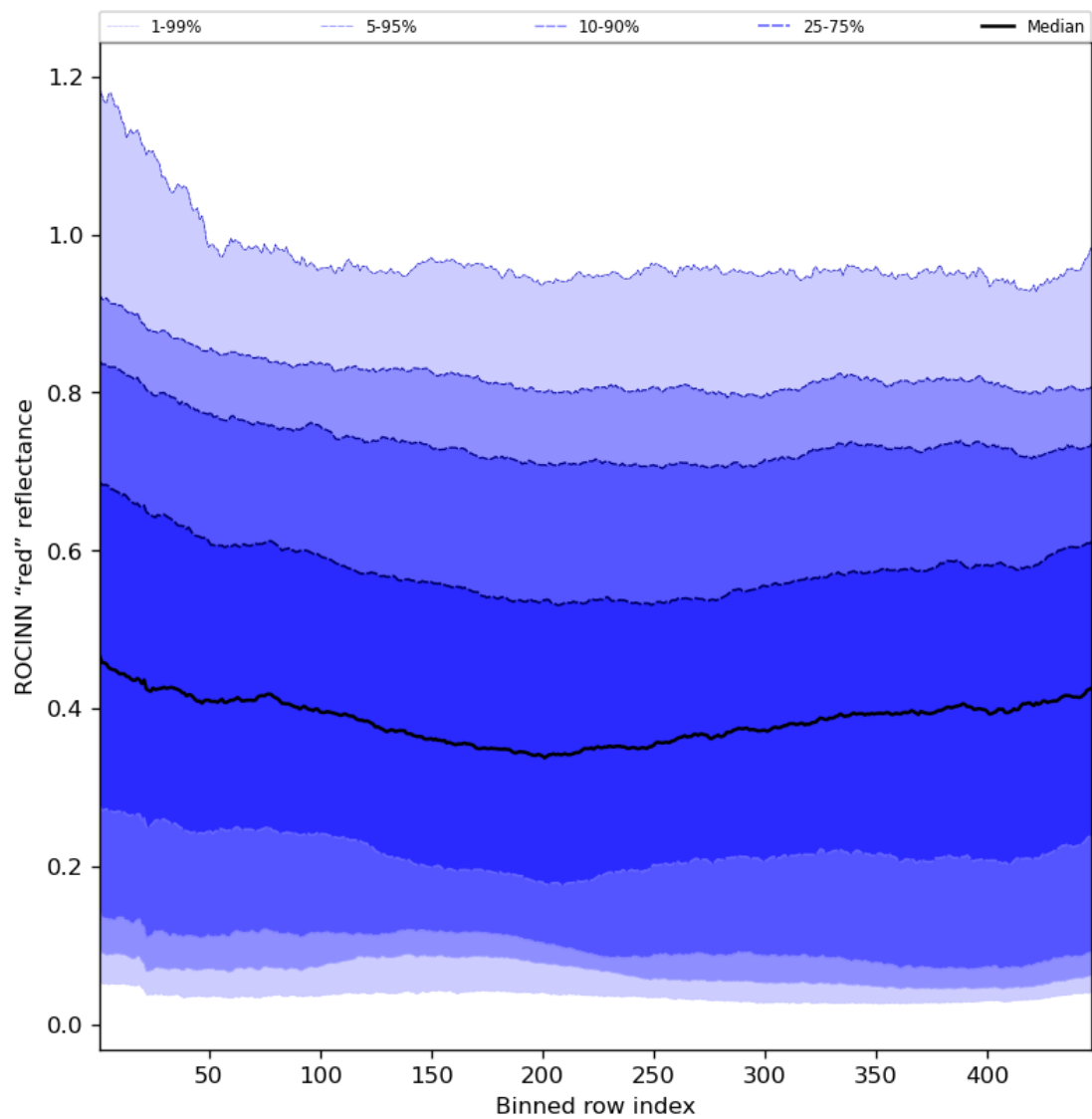
Figure 69: Along track statistics of “ROCINN “red” reflectance” for 2023-07-17 to 2023-07-19
