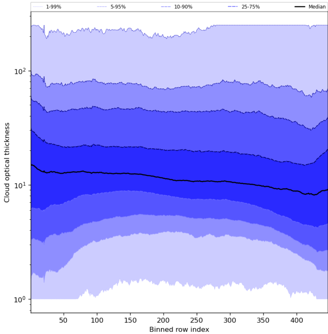
Figure 57: Along track statistics of “Cloud optical thickness” for 2023-07-17 to 2023-07-19
