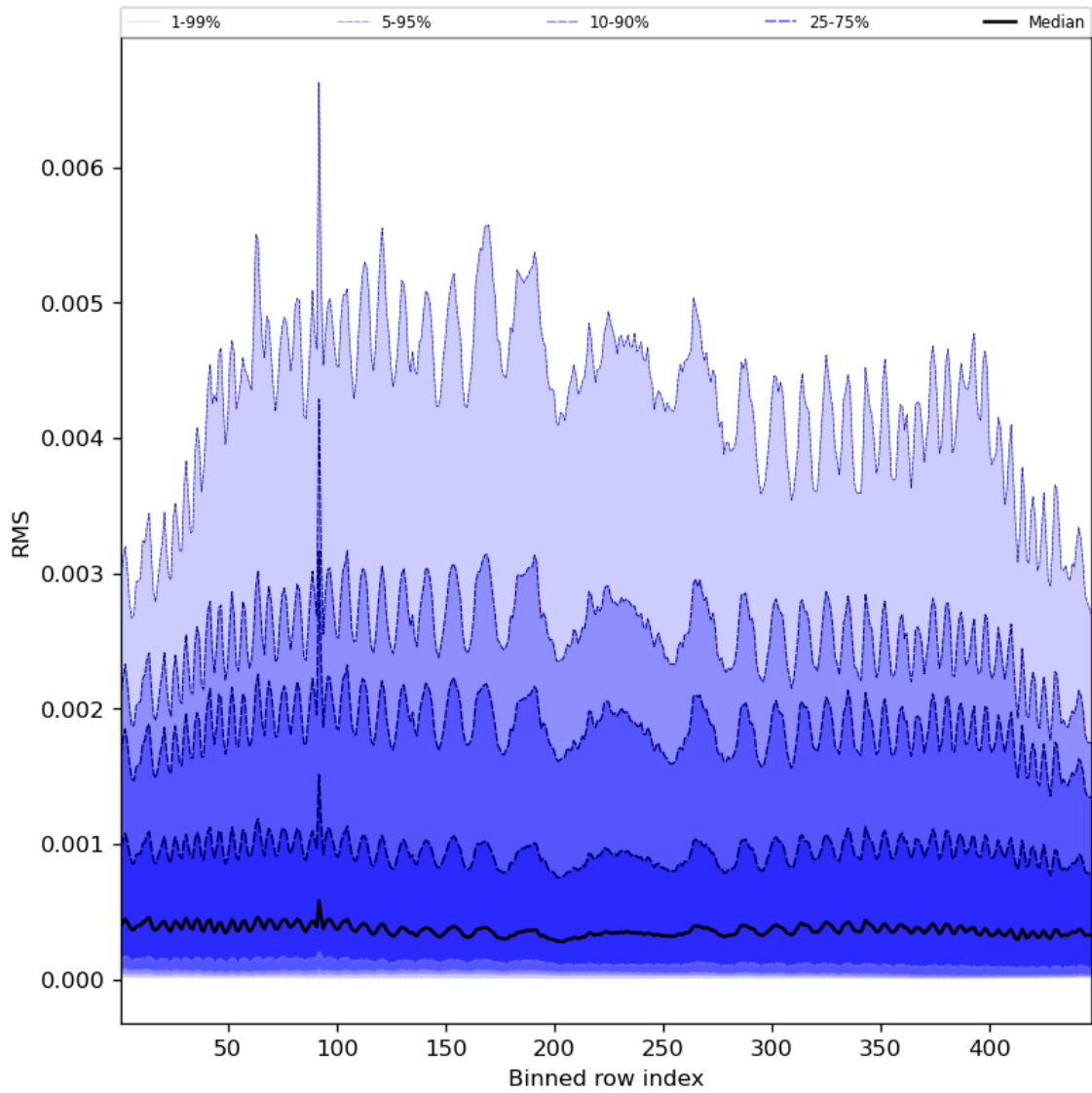
Figure 63: Along track statistics of “RMS” for 2023-07-17 to 2023-07-19
