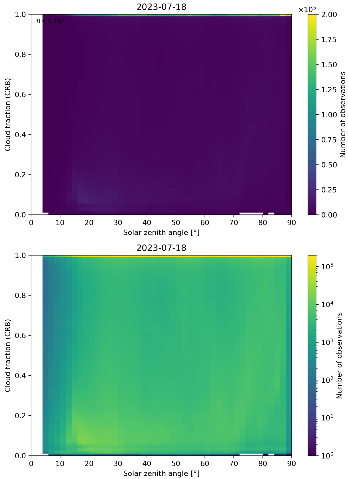
Figure 101: Scatter density plot of “Solar zenith angle” against “Cloud fraction (CRB)” for 2023-07-17 to 2023-07-19.
