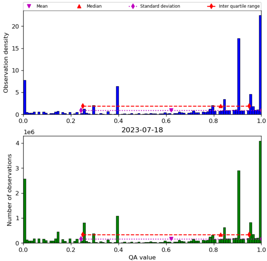
Figure 38: Histogram of “QA value” for 2023-07-17 to 2023-07-19
