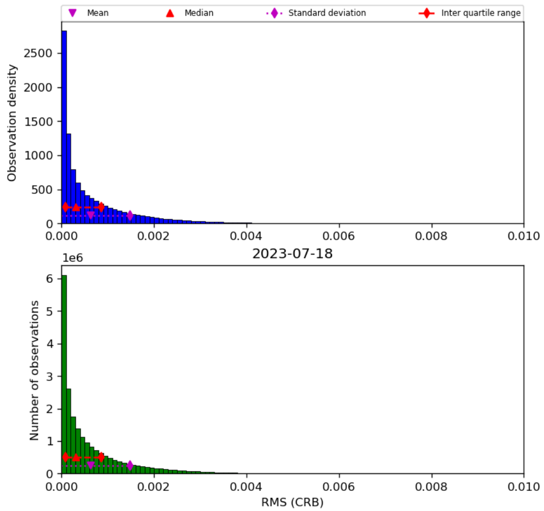
Figure 48: Histogram of “RMS (CRB)” for 2023-07-17 to 2023-07-19
