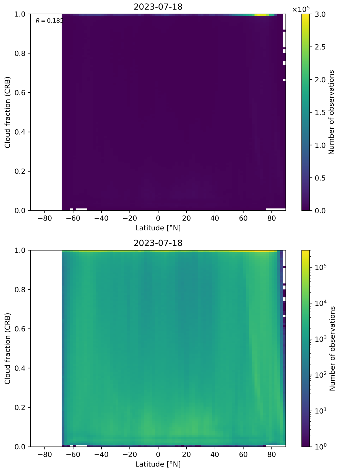
Figure 94: Scatter density plot of “Latitude” against “Cloud fraction (CRB)” for 2023-07-17 to 2023-07-19.
