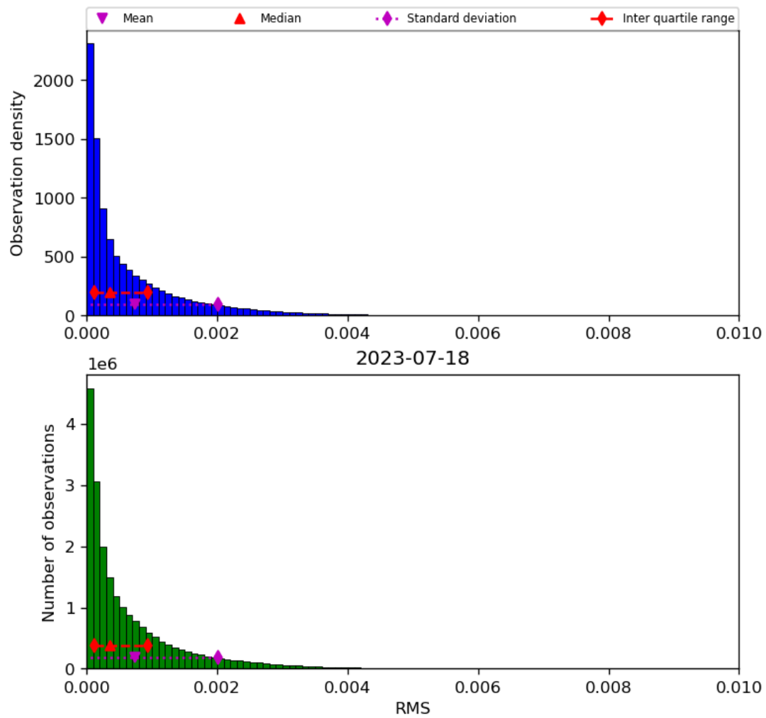
Figure 47: Histogram of “RMS” for 2023-07-17 to 2023-07-19
