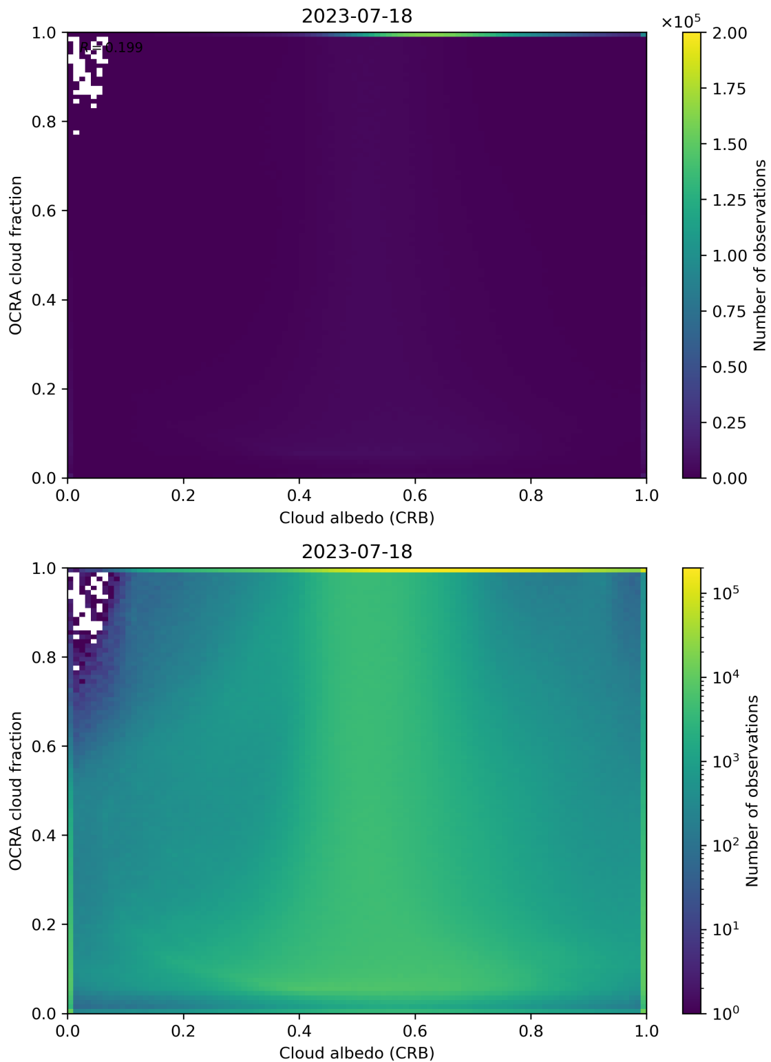
Figure 70: Scatter density plot of “Cloud albedo (CRB)” against “OCRA cloud fraction” for 2023-07-17 to 2023-07-19.
