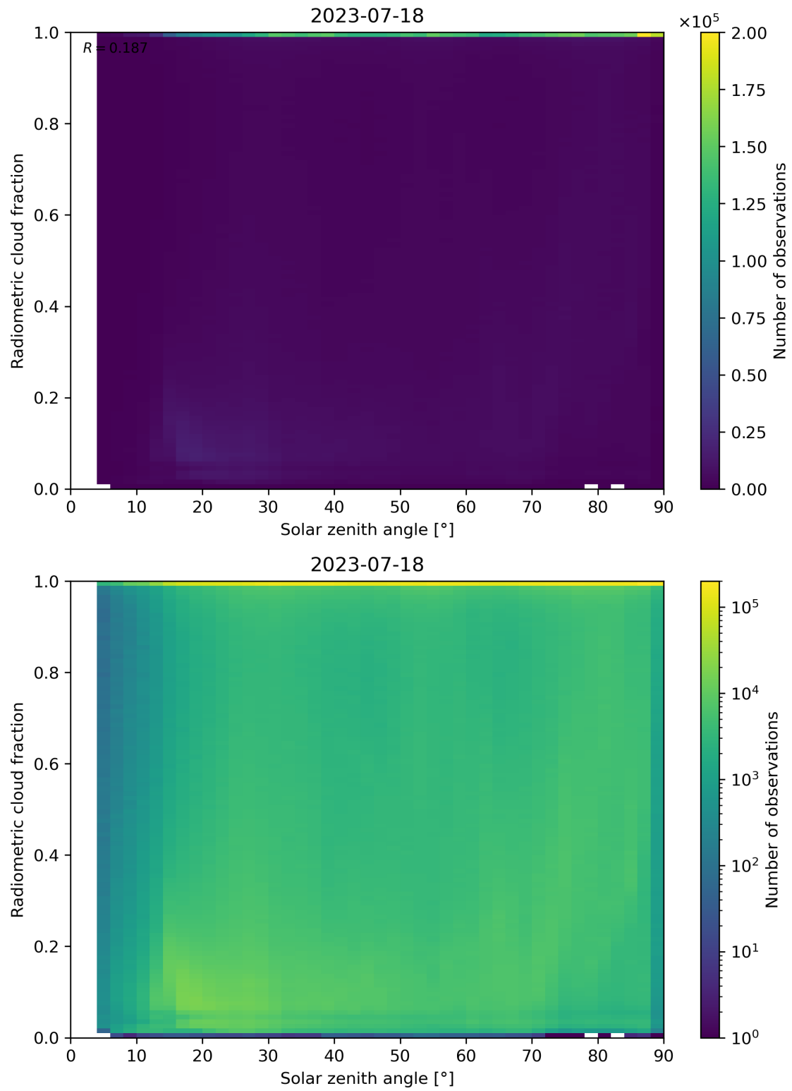
Figure 99: Scatter density plot of “Solar zenith angle” against “Radiometric cloud fraction” for 2023-07-17 to 2023-07-19.
