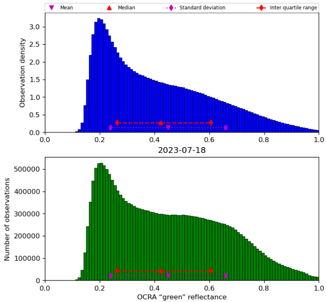
Figure 52: Histogram of “OCRA “green” reflectance” for 2023-07-17 to 2023-07-19
