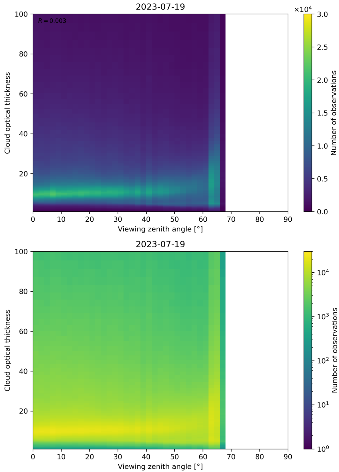
Figure 111: Scatter density plot of “Viewing zenith angle” against “Cloud optical thickness” for 2023-07-19 to 2023-07-20.
