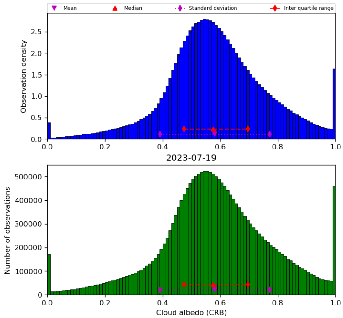
Figure 44: Histogram of “Cloud albedo (CRB)” for 2023-07-19 to 2023-07-20
