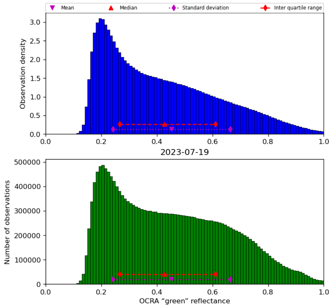
Figure 52: Histogram of “OCRA “green” reflectance” for 2023-07-19 to 2023-07-20
