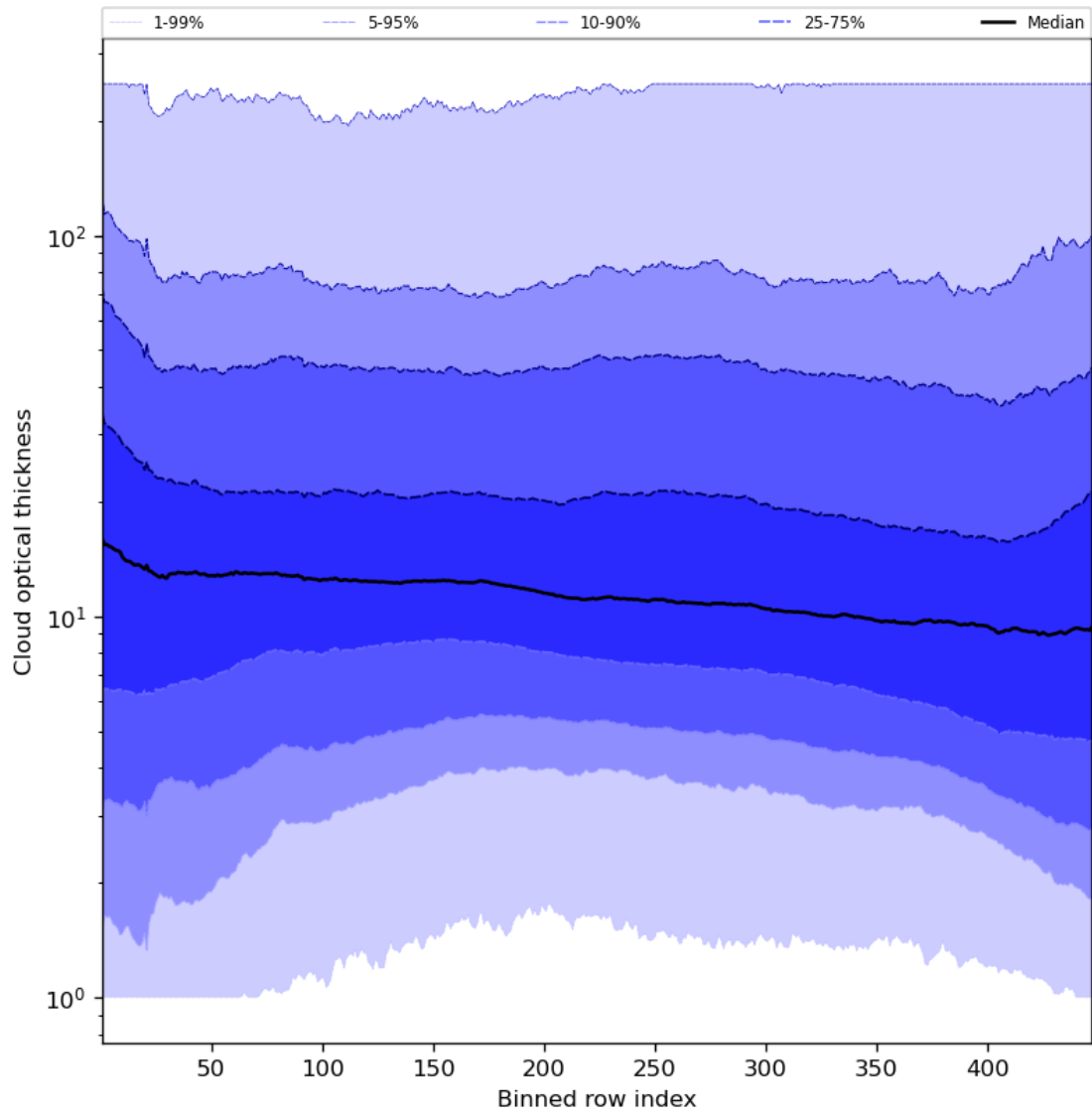
Figure 57: Along track statistics of “Cloud optical thickness” for 2023-07-19 to 2023-07-20
