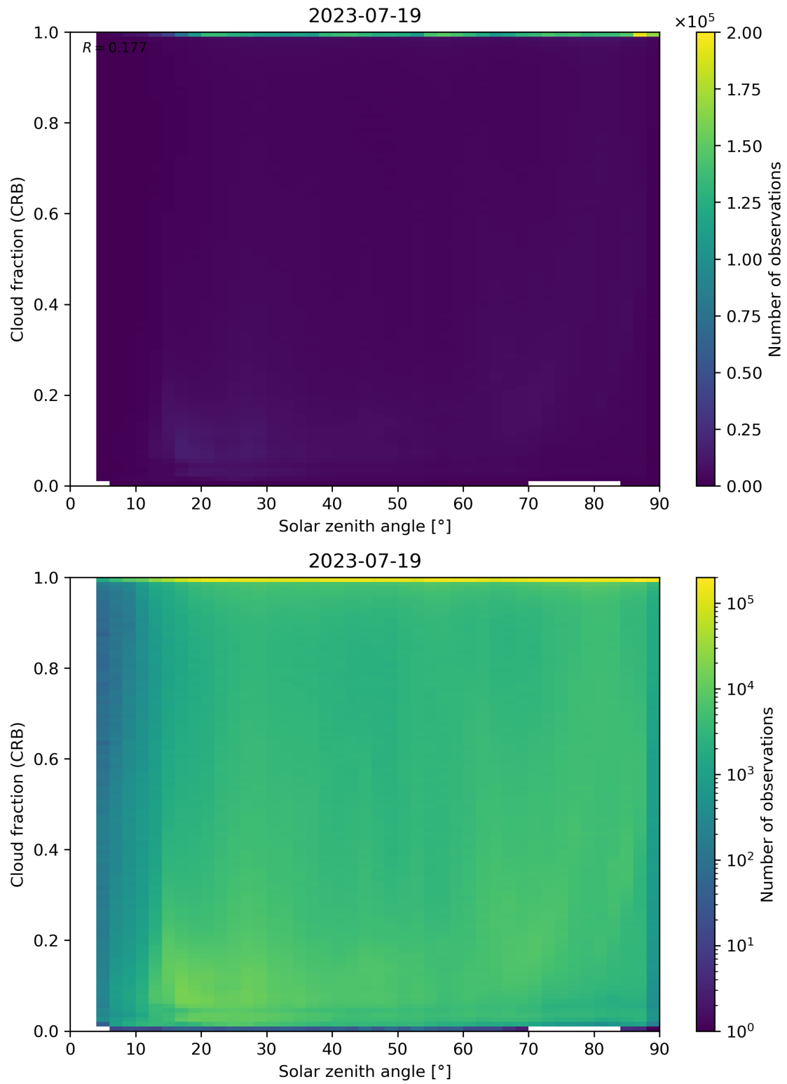
Figure 101: Scatter density plot of “Solar zenith angle” against “Cloud fraction (CRB)” for 2023-07-19 to 2023-07-20.
