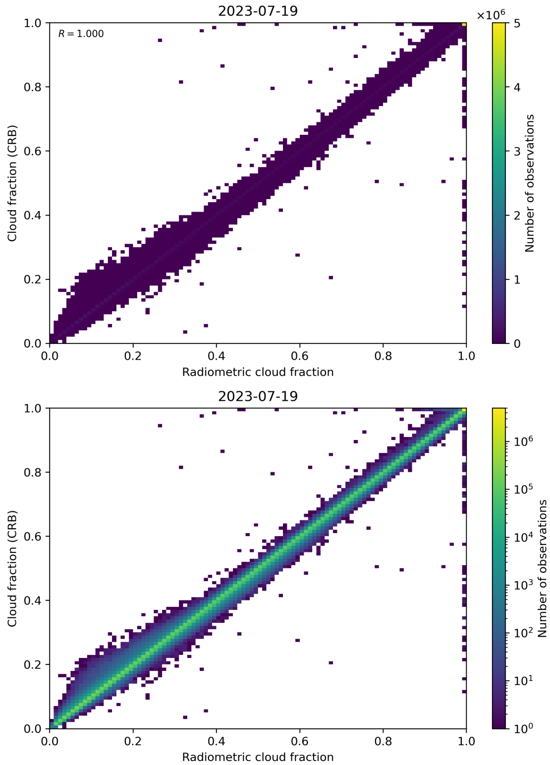
Figure 73: Scatter density plot of “Radiometric cloud fraction” against “Cloud fraction (CRB)” for 2023-07-19 to 2023-07-20.
