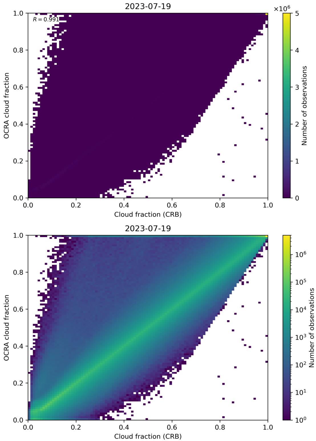
Figure 78: Scatter density plot of “Cloud fraction (CRB)” against “OCRA cloud fraction” for 2023-07-19 to 2023-07-20.
