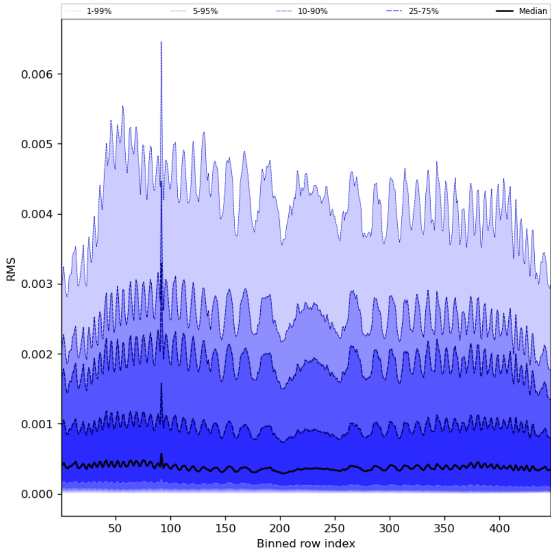
Figure 63: Along track statistics of “RMS” for 2023-07-19 to 2023-07-20
