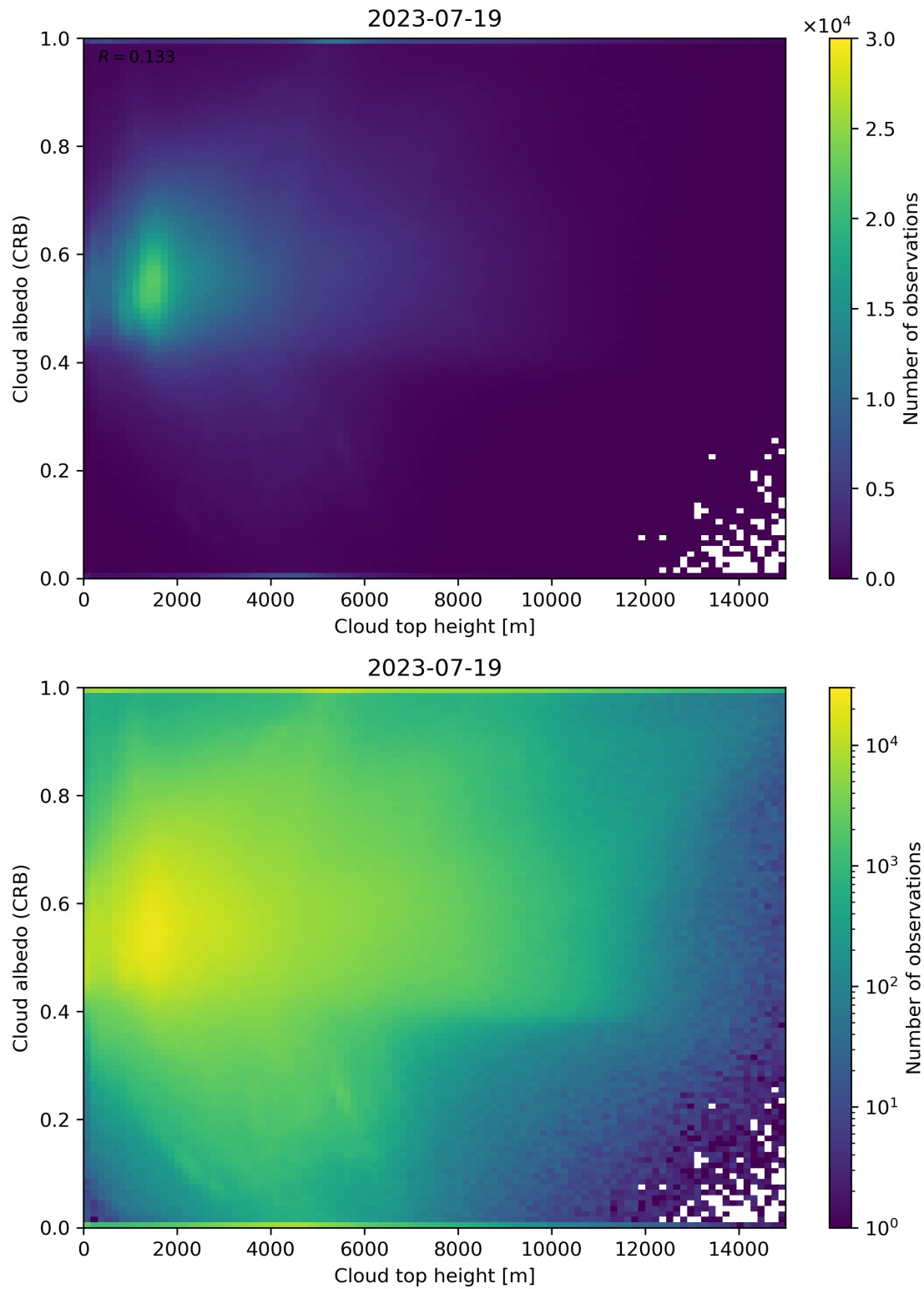
Figure 86: Scatter density plot of “Cloud top height” against “Cloud albedo (CRB)” for 2023-07-19 to 2023-07-20.
