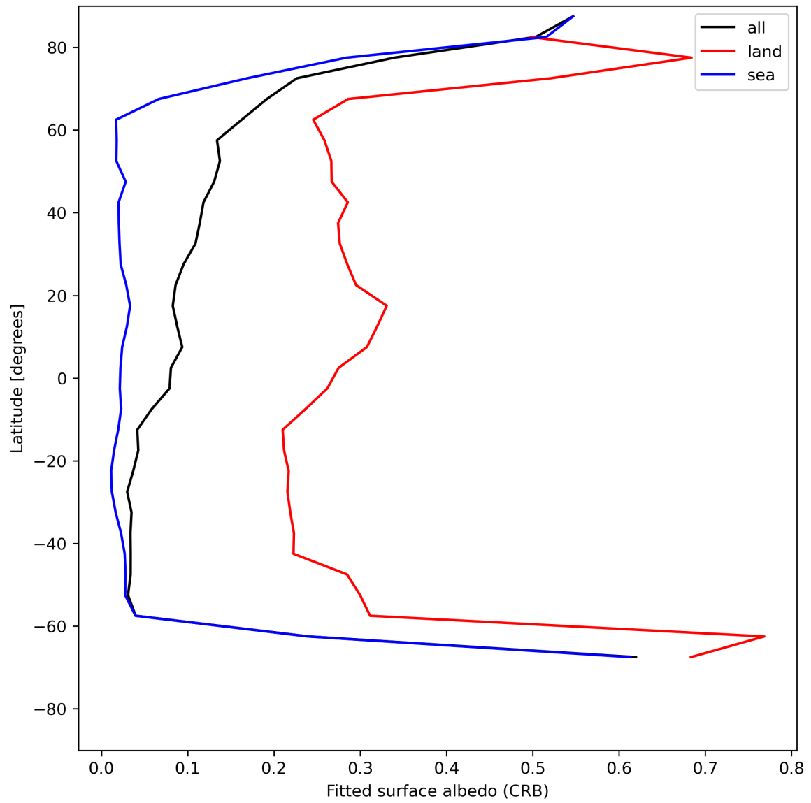
Figure 30: Zonal average of “Fitted surface albedo (CRB)” for 2023-07-19 to 2023-07-20.
