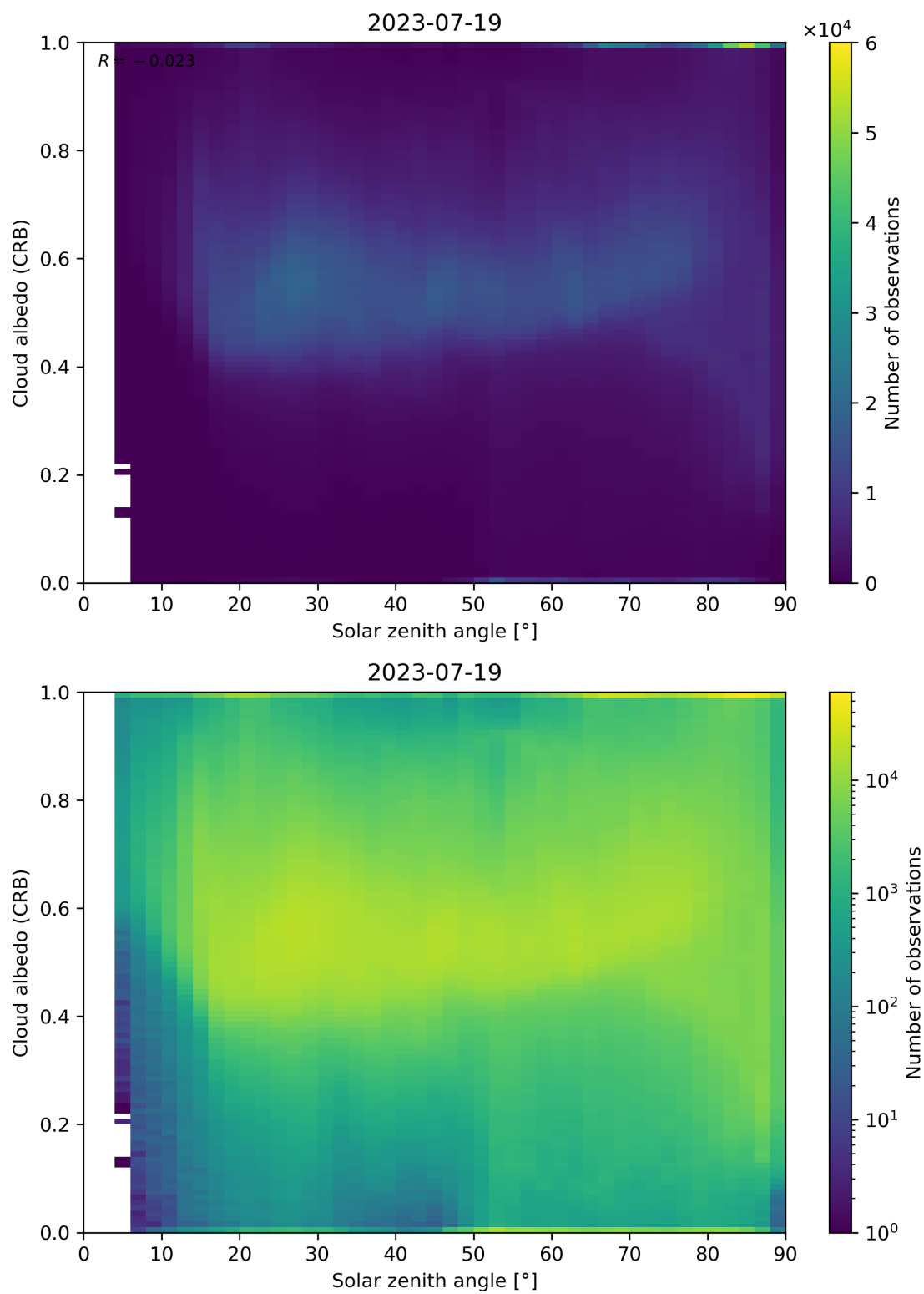
Figure 98: Scatter density plot of “Solar zenith angle” against “Cloud albedo (CRB)” for 2023-07-19 to 2023-07-20.
