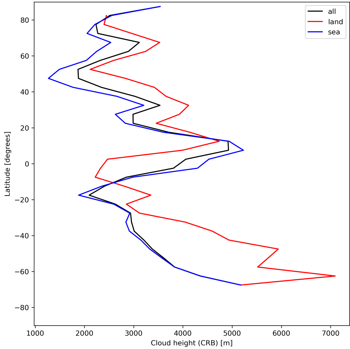
Figure 27: Zonal average of “Cloud height (CRB)” for 2023-07-19 to 2023-07-20.
