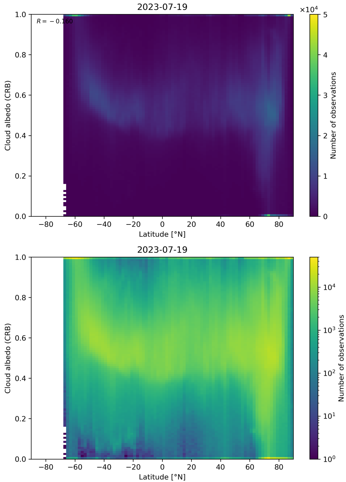
Figure 91: Scatter density plot of “Latitude” against “Cloud albedo (CRB)” for 2023-07-19 to 2023-07-20.
