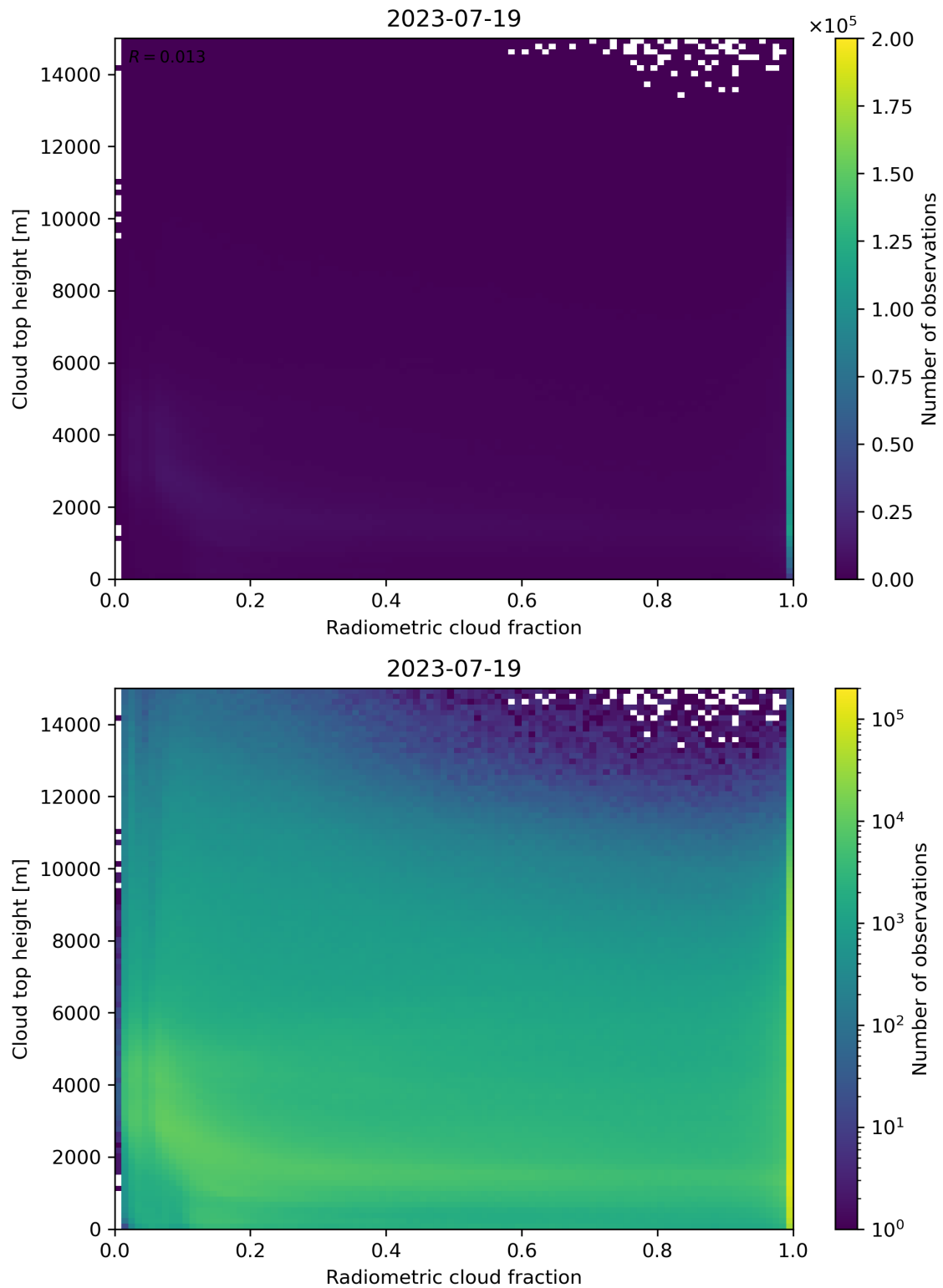
Figure 76: Scatter density plot of “Radiometric cloud fraction” against “Cloud top height” for 2023-07-19 to 2023-07-20.
