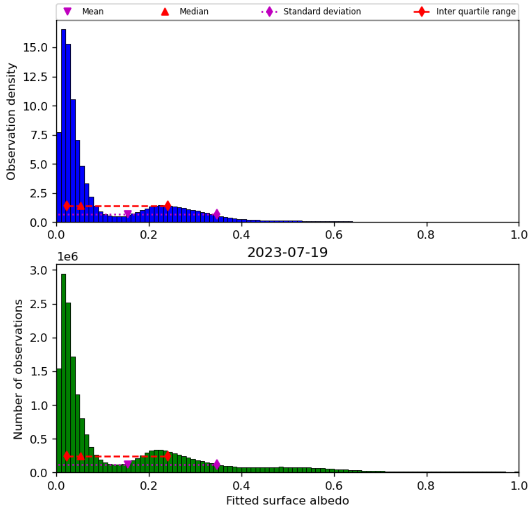
Figure 45: Histogram of “Fitted surface albedo” for 2023-07-19 to 2023-07-20
