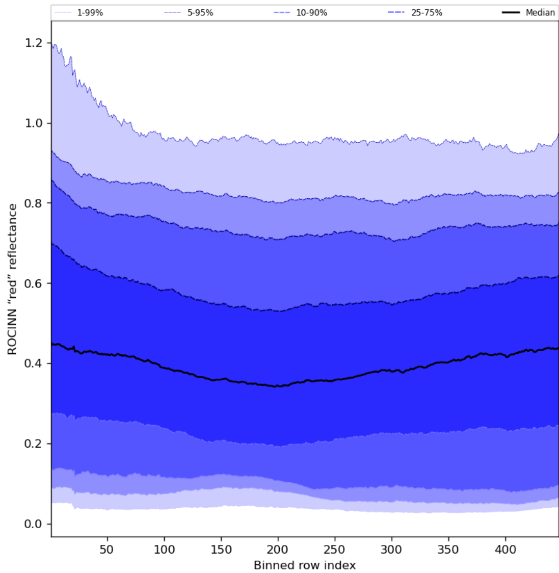
Figure 69: Along track statistics of “ROCINN “red” reflectance” for 2023-07-19 to 2023-07-20
