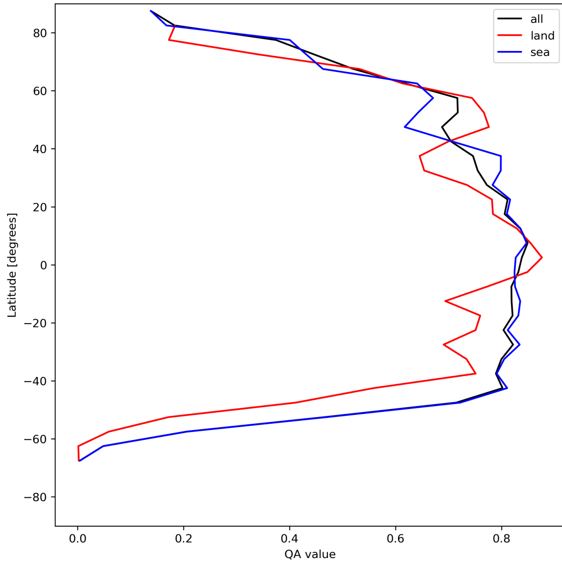
Figure 22: Zonal average of “QA value” for 2023-07-19 to 2023-07-20.
