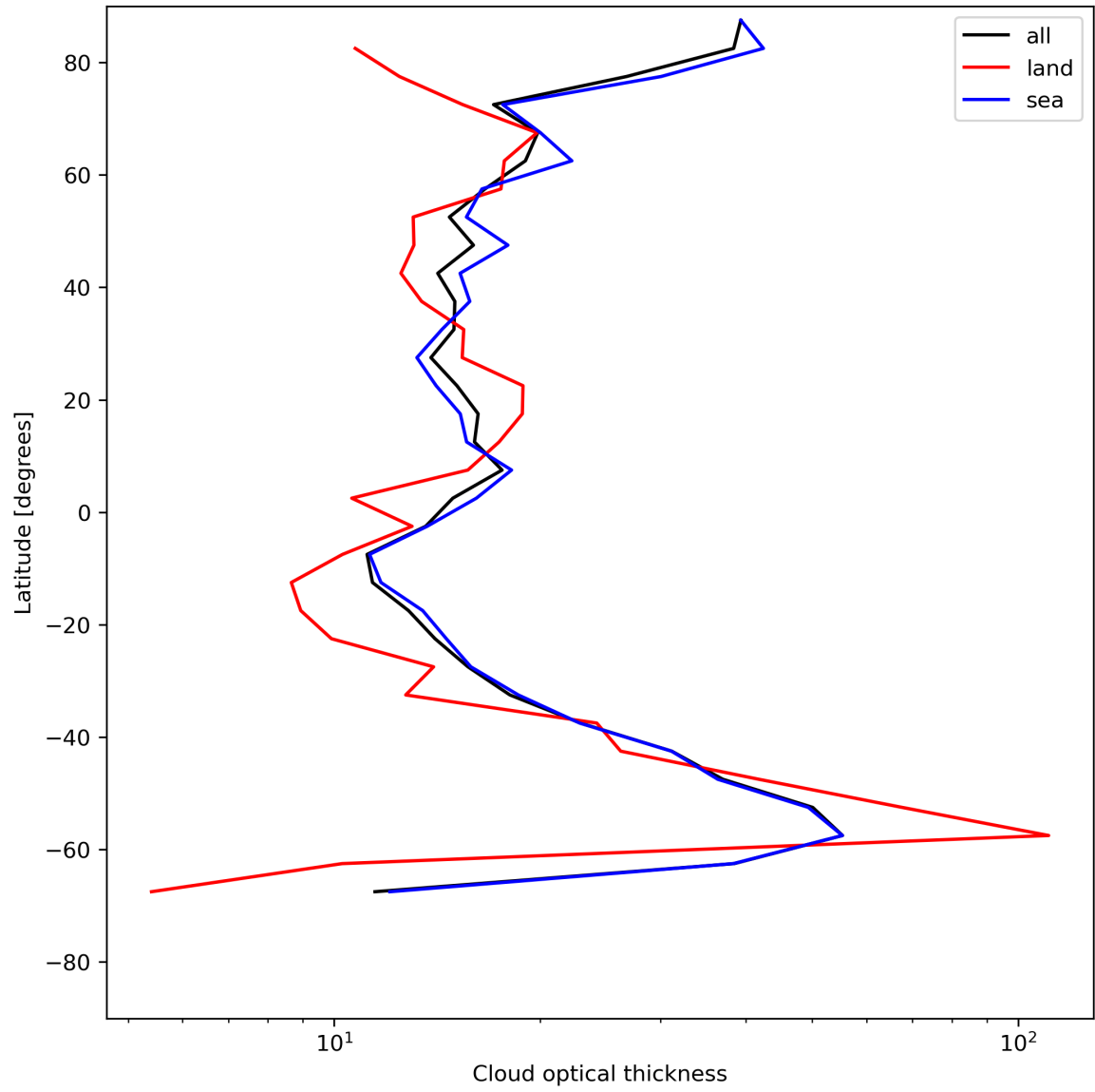
Figure 25: Zonal average of “Cloud optical thickness” for 2023-07-19 to 2023-07-20.
