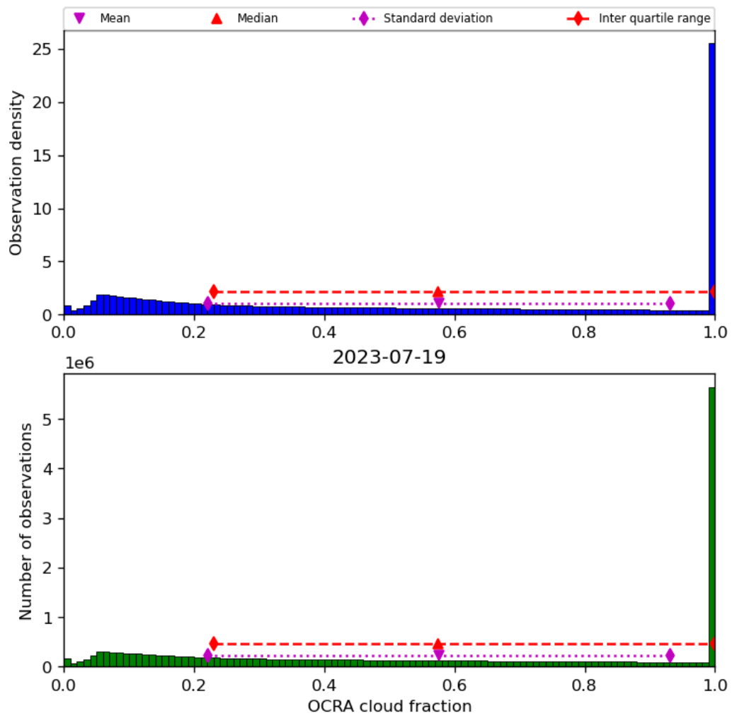
Figure 50: Histogram of “OCRA cloud fraction” for 2023-07-19 to 2023-07-20
