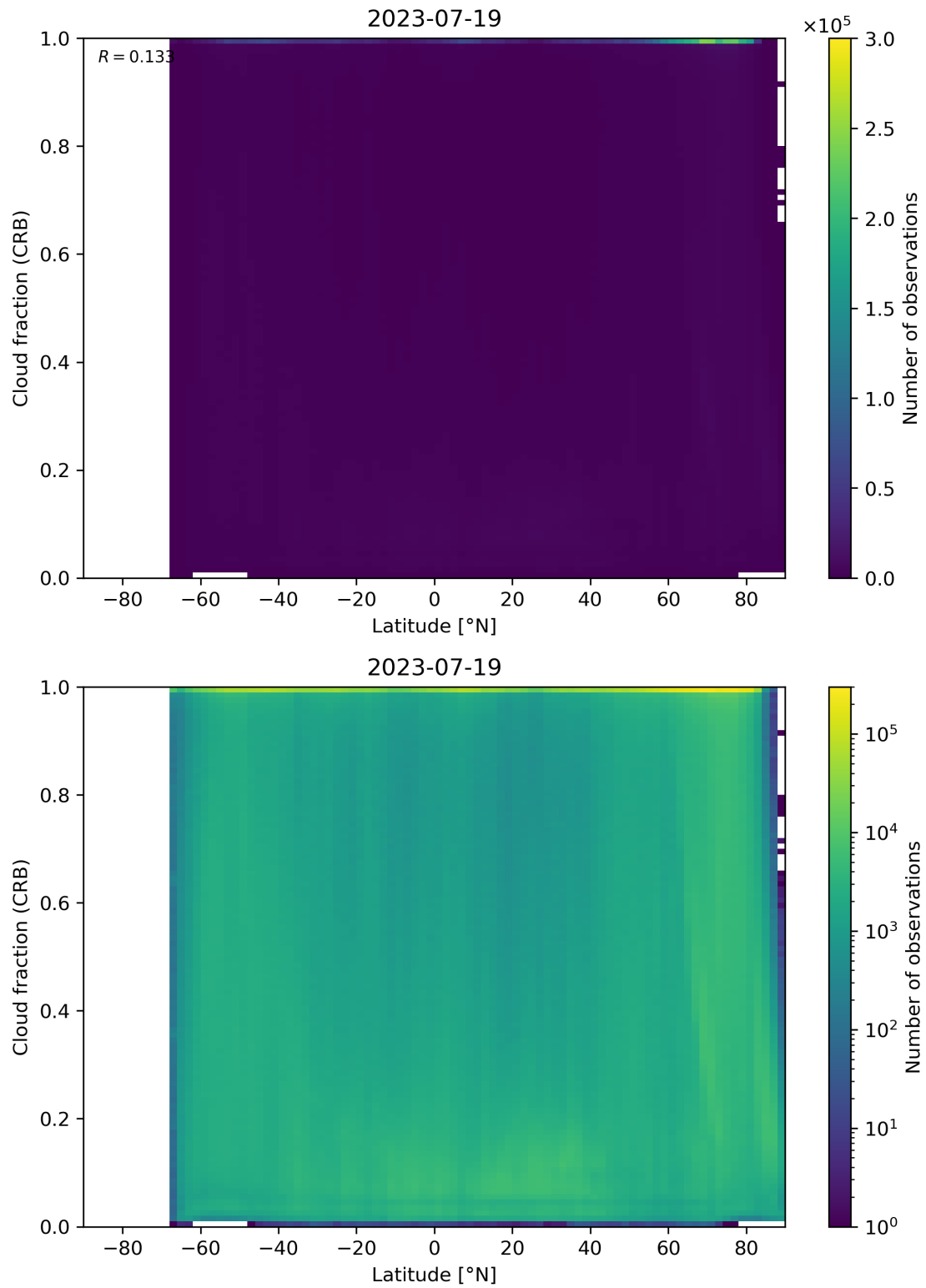
Figure 94: Scatter density plot of “Latitude” against “Cloud fraction (CRB)” for 2023-07-19 to 2023-07-20.
