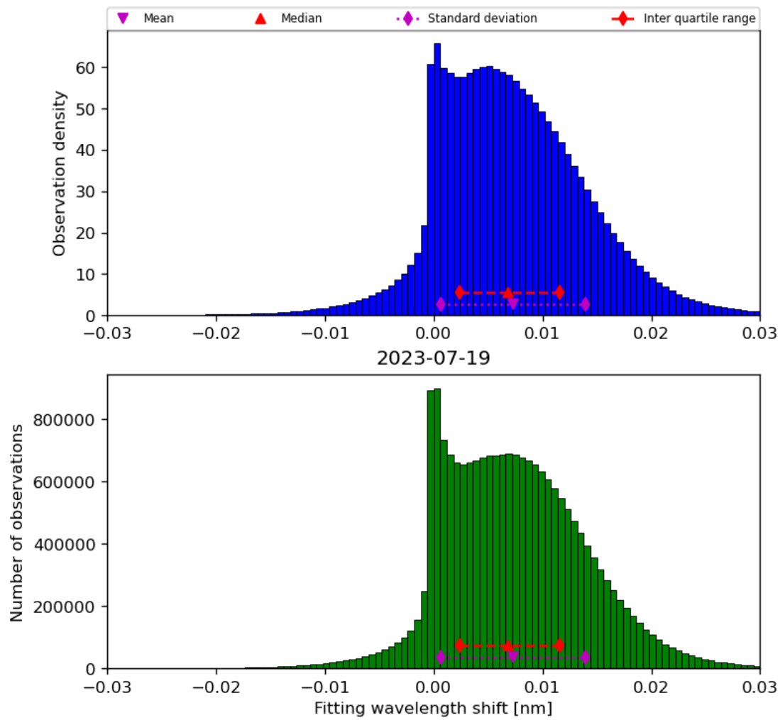
Figure 49: Histogram of “Fitting wavelength shift” for 2023-07-19 to 2023-07-20
