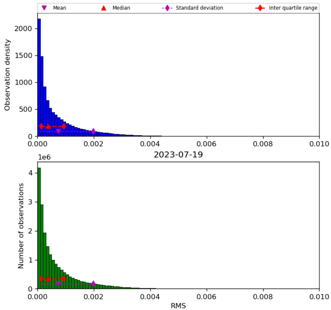
Figure 47: Histogram of “RMS” for 2023-07-19 to 2023-07-20
