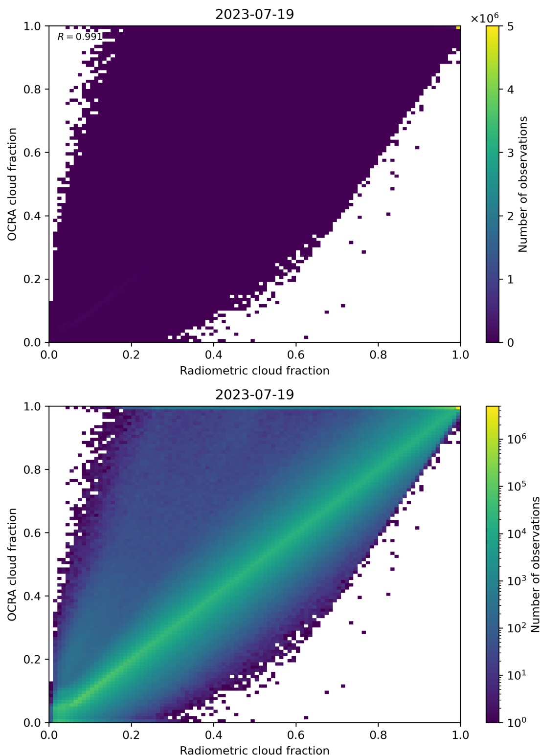
Figure 72: Scatter density plot of “Radiometric cloud fraction” against “OCRA cloud fraction” for 2023-07-19 to 2023-07-20.
