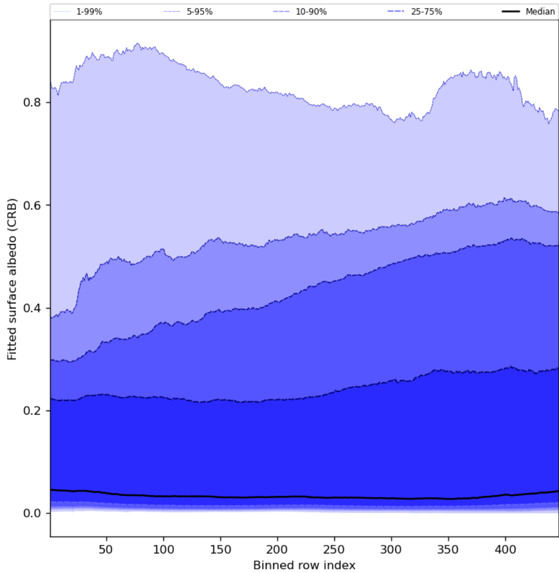
Figure 62: Along track statistics of “Fitted surface albedo (CRB)” for 2023-07-19 to 2023-07-20
