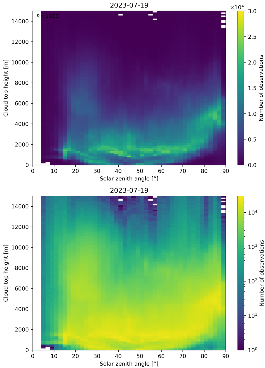
Figure 104: Scatter density plot of “Solar zenith angle” against “Cloud top height” for 2023-07-19 to 2023-07-20.
