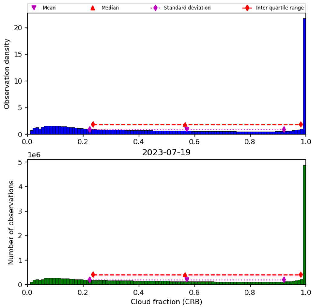
Figure 42: Histogram of “Cloud fraction (CRB)” for 2023-07-19 to 2023-07-20
