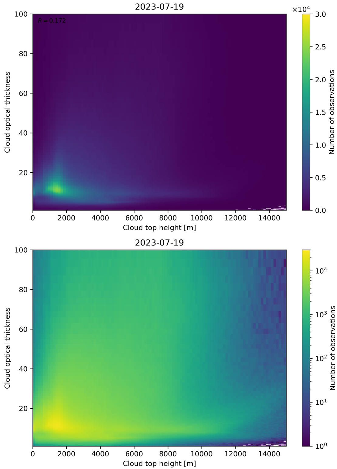
Figure 90: Scatter density plot of “Cloud top height” against “Cloud optical thickness” for 2023-07-19 to 2023-07-20.
