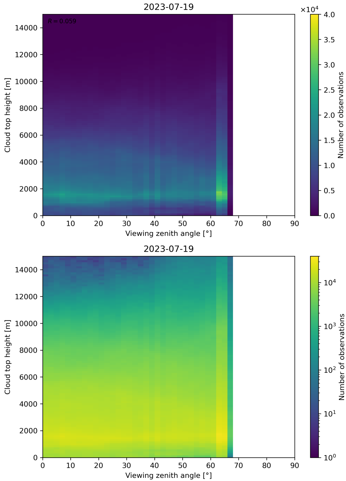
Figure 112: Scatter density plot of “Viewing zenith angle” against “Cloud top height” for 2023-07-19 to 2023-07-20.
