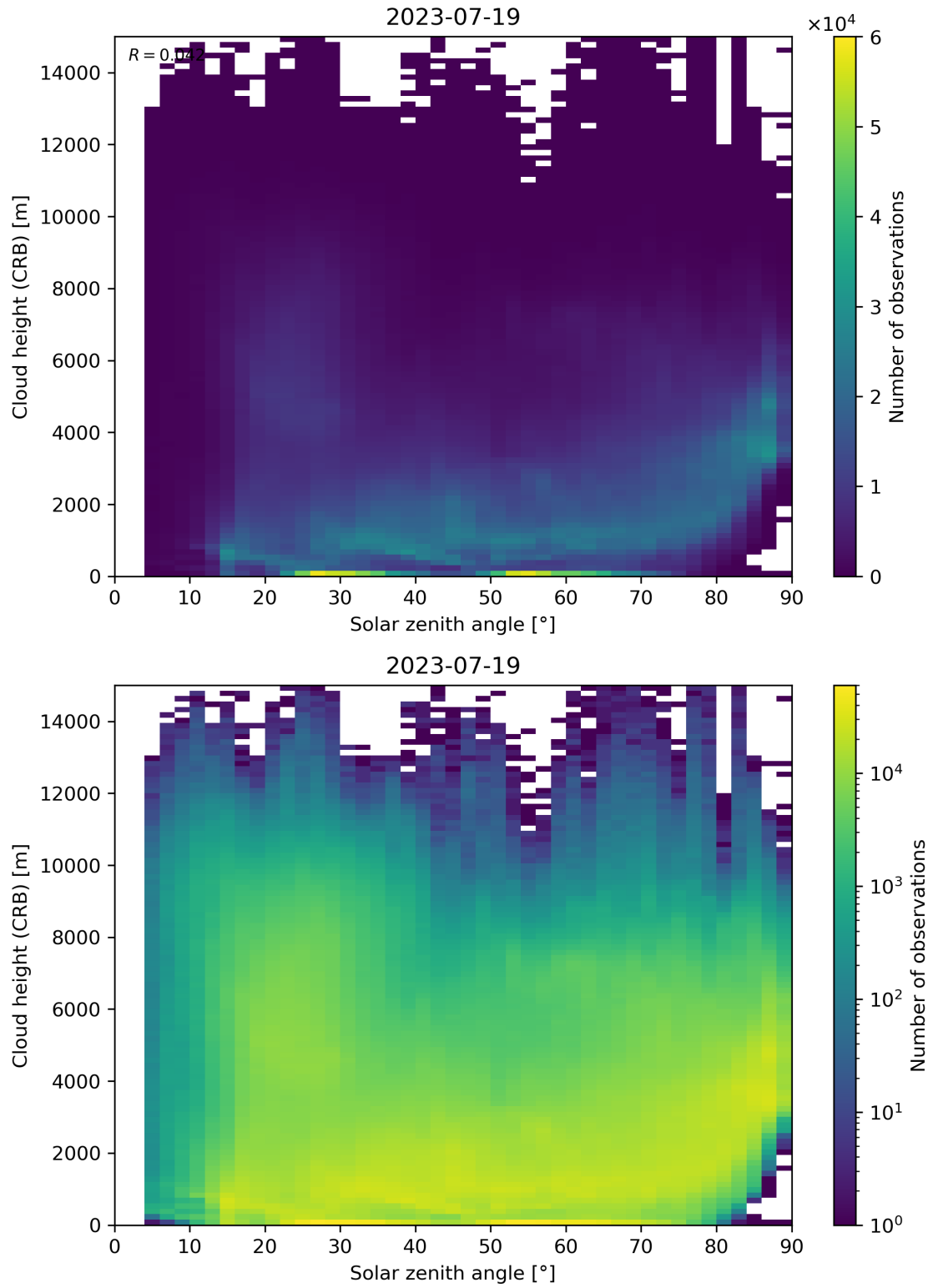
Figure 102: Scatter density plot of “Solar zenith angle” against “Cloud height (CRB)” for 2023-07-19 to 2023-07-20.
