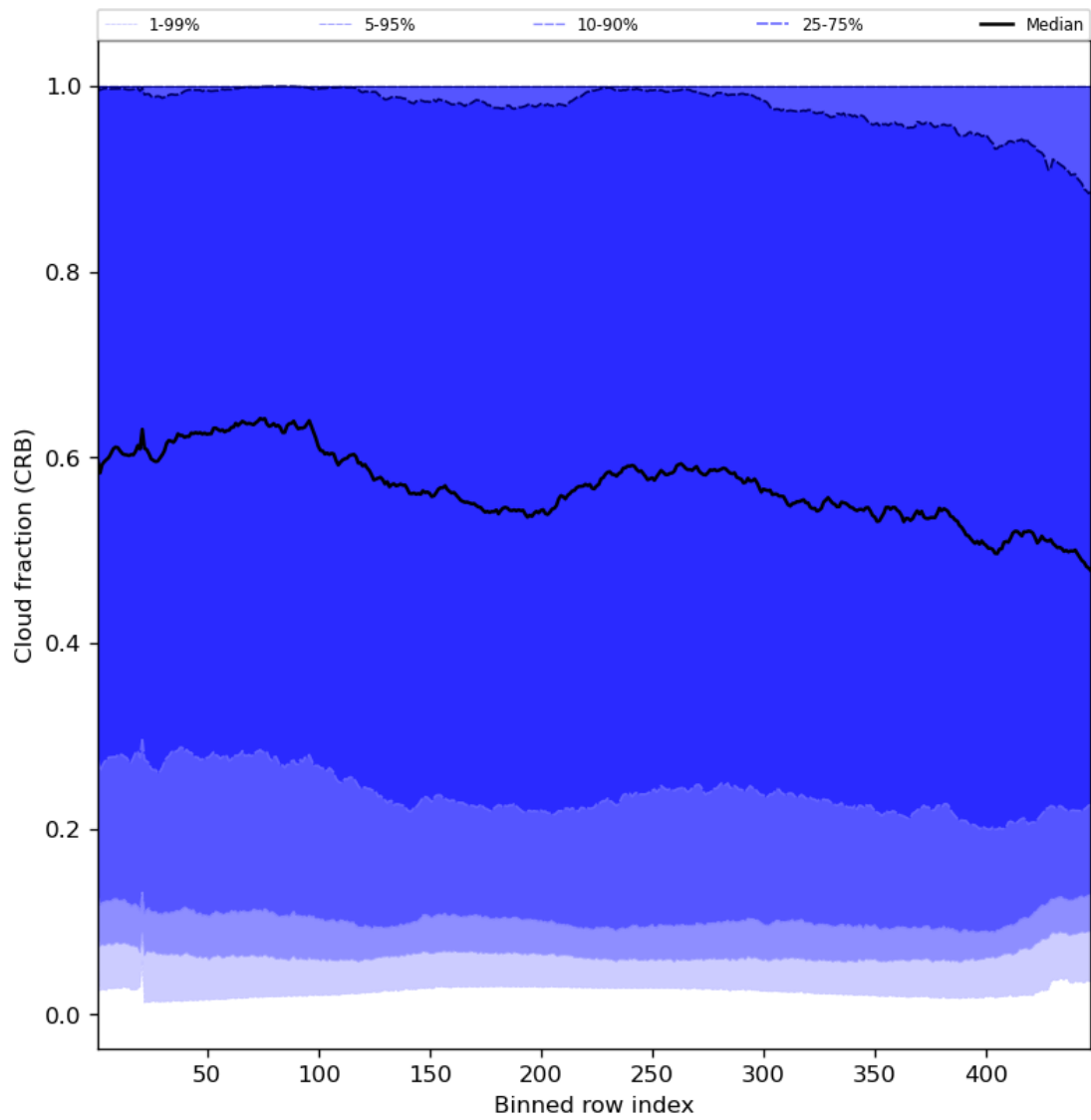
Figure 58: Along track statistics of “Cloud fraction (CRB)” for 2023-07-19 to 2023-07-20
