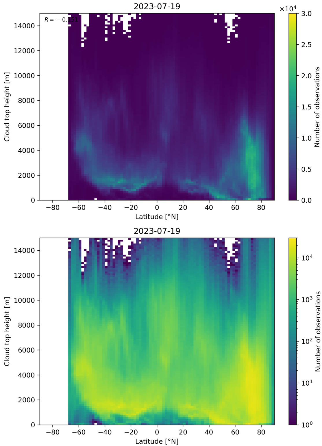
Figure 97: Scatter density plot of “Latitude” against “Cloud top height” for 2023-07-19 to 2023-07-20.
