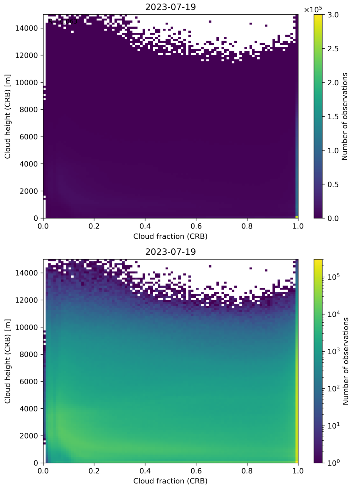
Figure 79: Scatter density plot of “Cloud fraction (CRB)” against “Cloud height (CRB)” for 2023-07-19 to 2023-07-20.
