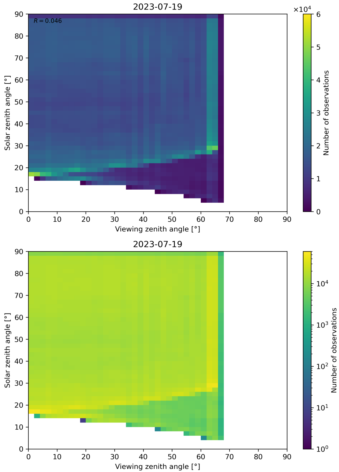
Figure 114: Scatter density plot of “Viewing zenith angle” against “Solar zenith angle” for 2023-07-19 to 2023-07-20.
