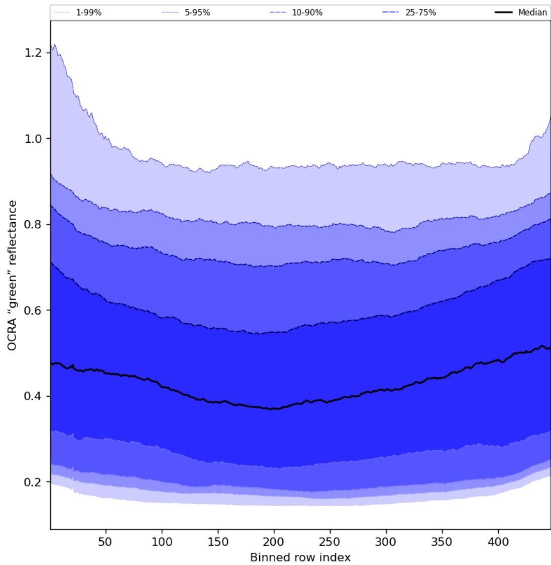
Figure 68: Along track statistics of “OCRA “green” reflectance” for 2023-07-19 to 2023-07-20
