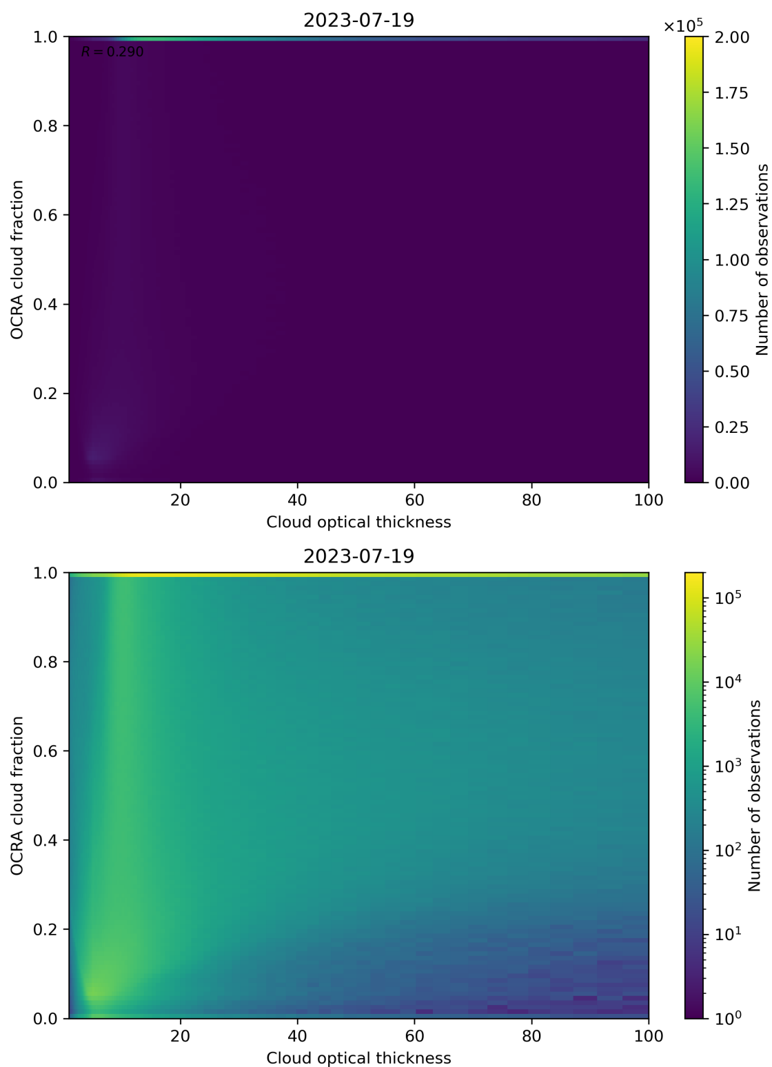
Figure 83: Scatter density plot of “Cloud optical thickness” against “OCRA cloud fraction” for 2023-07-19 to 2023-07-20.
