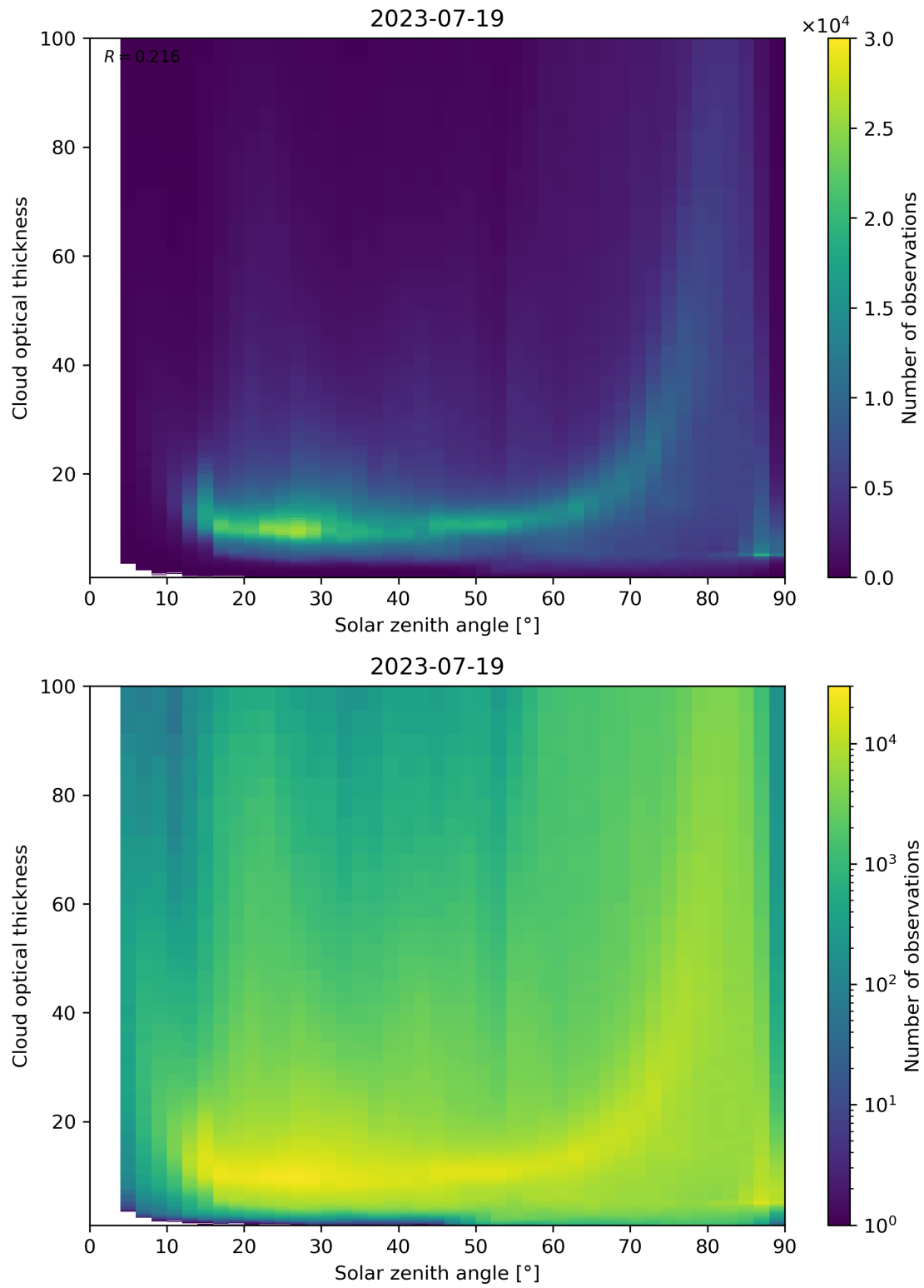
Figure 103: Scatter density plot of “Solar zenith angle” against “Cloud optical thickness” for 2023-07-19 to 2023-07-20.
