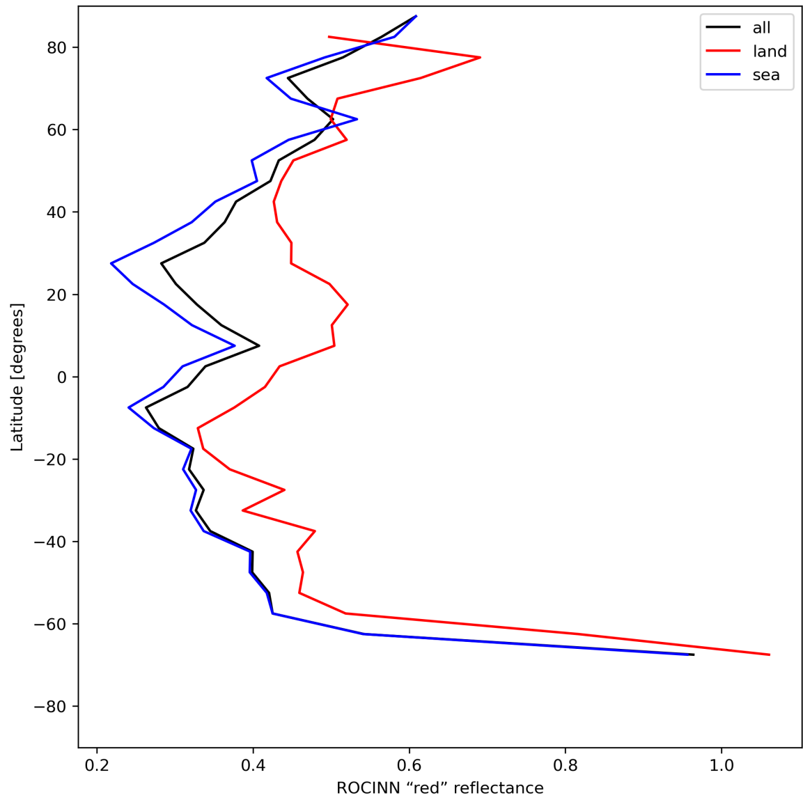
Figure 37: Zonal average of “ROCINN “red” reflectance” for 2023-07-19 to 2023-07-20.
