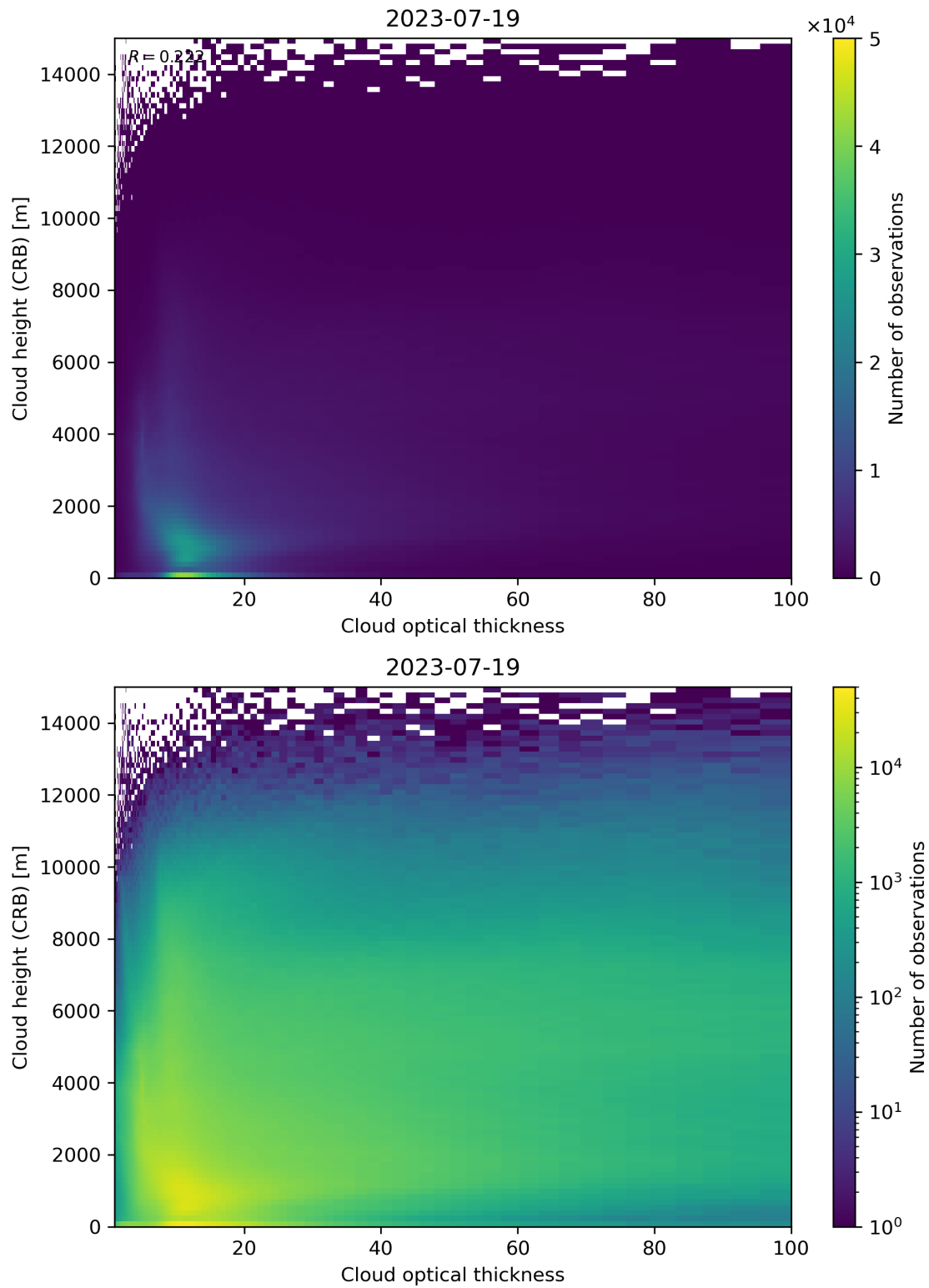
Figure 85: Scatter density plot of “Cloud optical thickness” against “Cloud height (CRB)” for 2023-07-19 to 2023-07-20.
