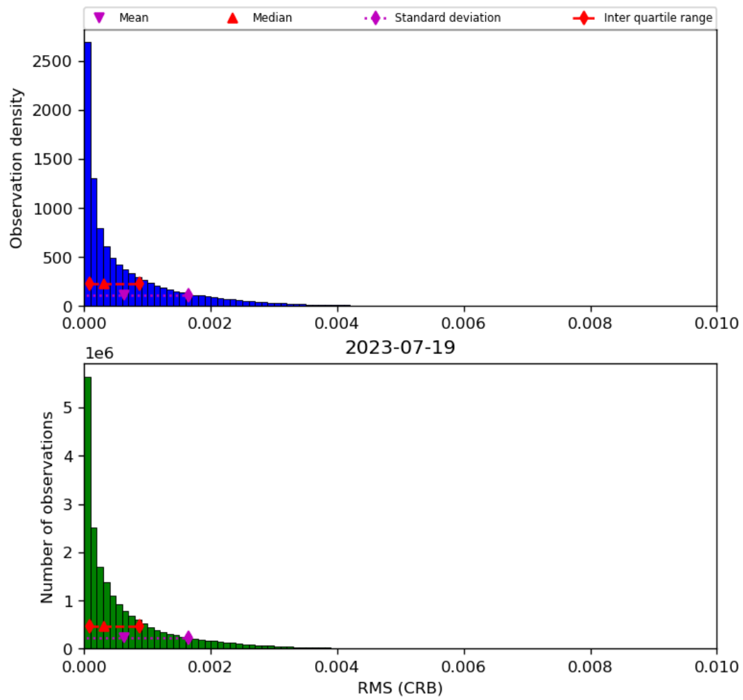
Figure 48: Histogram of “RMS (CRB)” for 2023-07-19 to 2023-07-20
