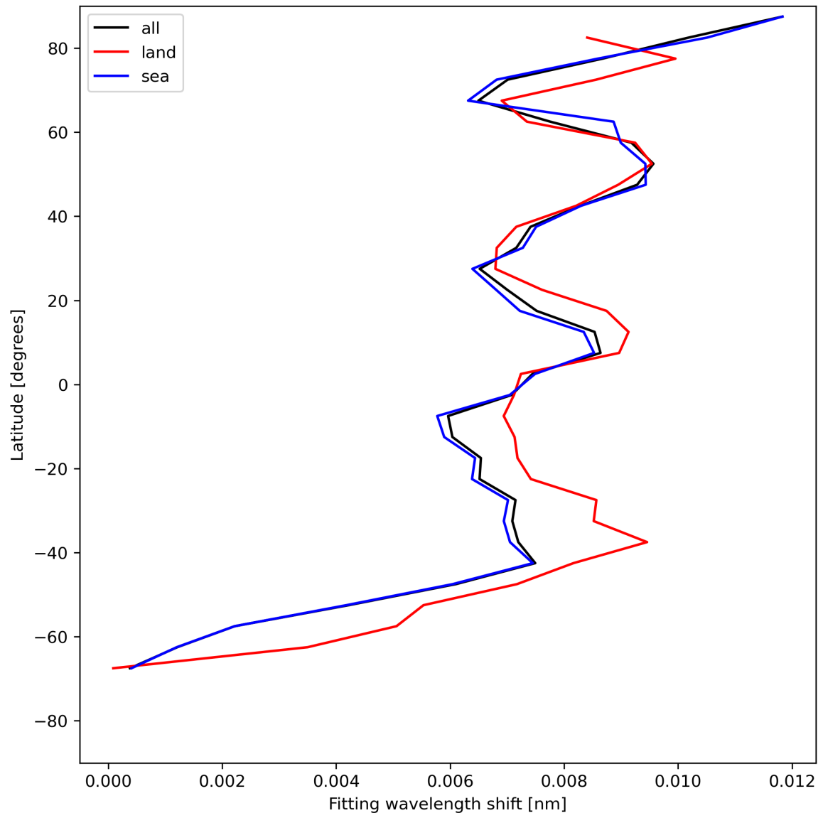
Figure 33: Zonal average of “Fitting wavelength shift” for 2023-07-19 to 2023-07-20.
