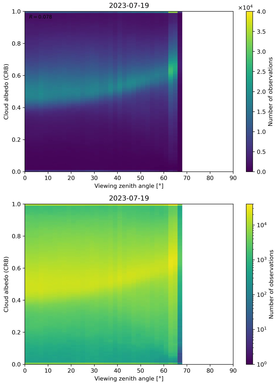
Figure 106: Scatter density plot of “Viewing zenith angle” against “Cloud albedo (CRB)” for 2023-07-19 to 2023-07-20.
