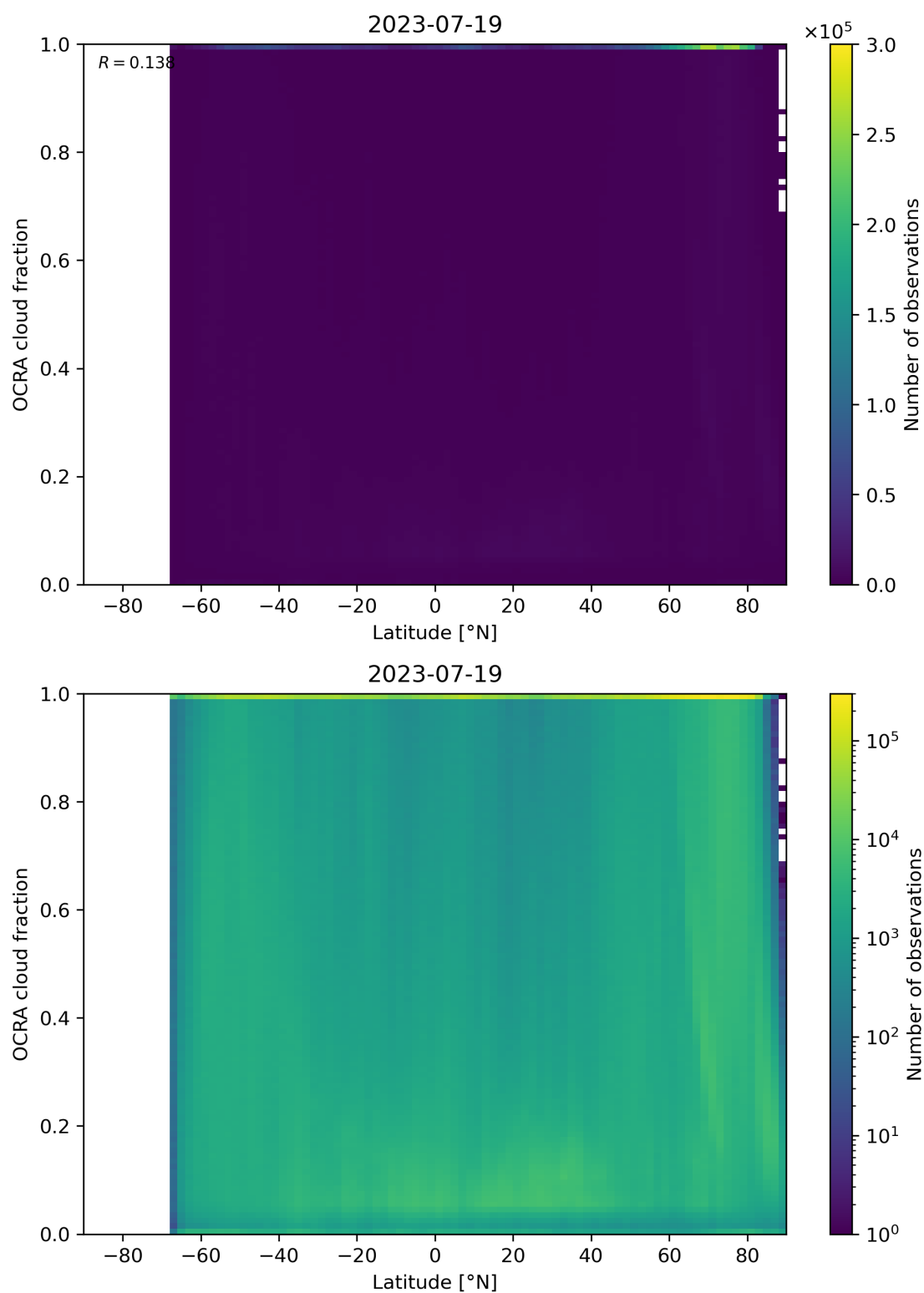
Figure 93: Scatter density plot of “Latitude” against “OCRA cloud fraction” for 2023-07-19 to 2023-07-20.
