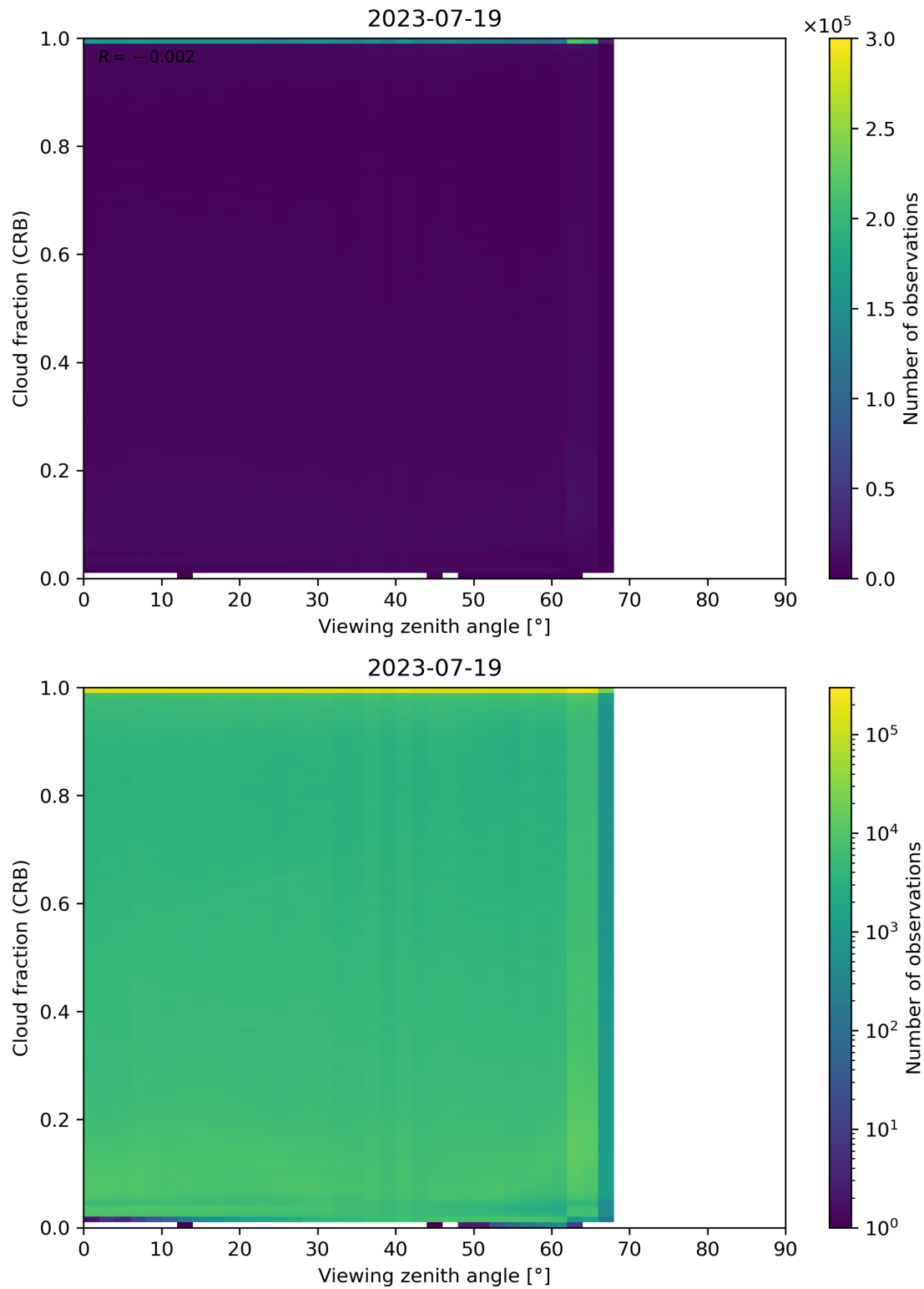
Figure 109: Scatter density plot of “Viewing zenith angle” against “Cloud fraction (CRB)” for 2023-07-19 to 2023-07-20.
