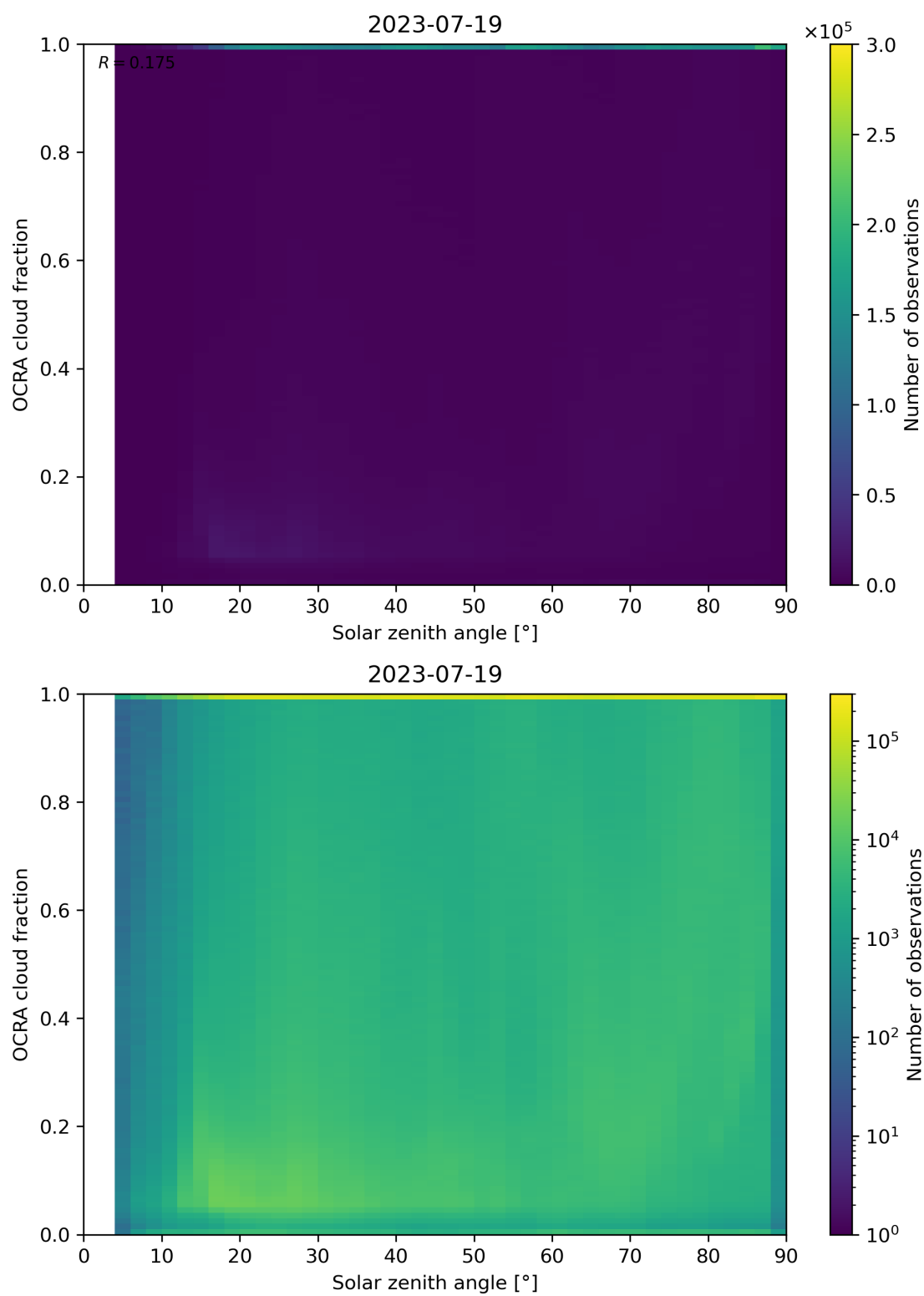
Figure 100: Scatter density plot of “Solar zenith angle” against “OCRA cloud fraction” for 2023-07-19 to 2023-07-20.
