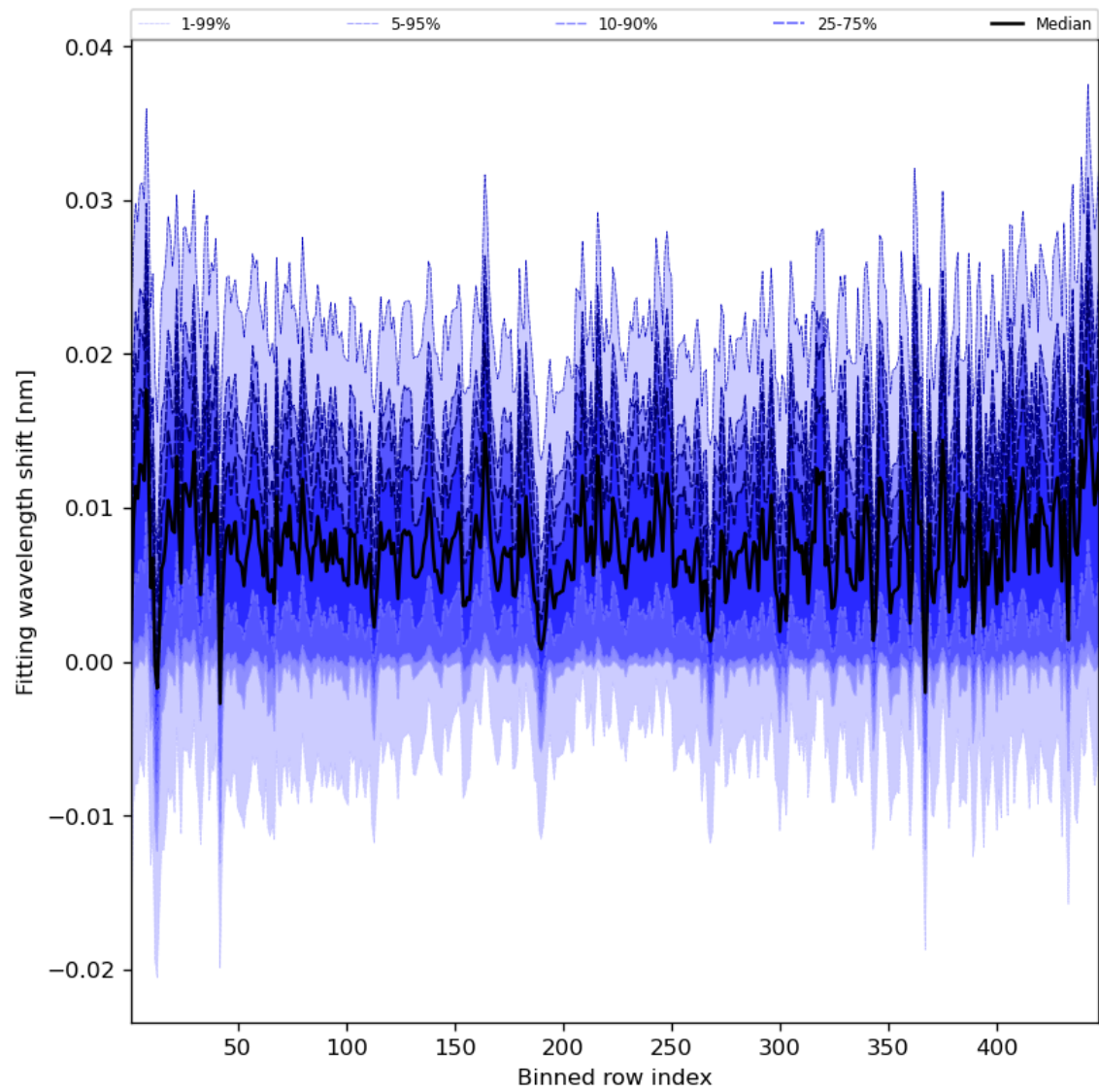
Figure 65: Along track statistics of “Fitting wavelength shift” for 2023-07-19 to 2023-07-20
