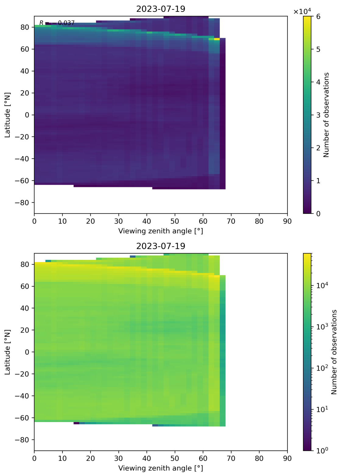
Figure 113: Scatter density plot of “Viewing zenith angle” against “Latitude” for 2023-07-19 to 2023-07-20.
