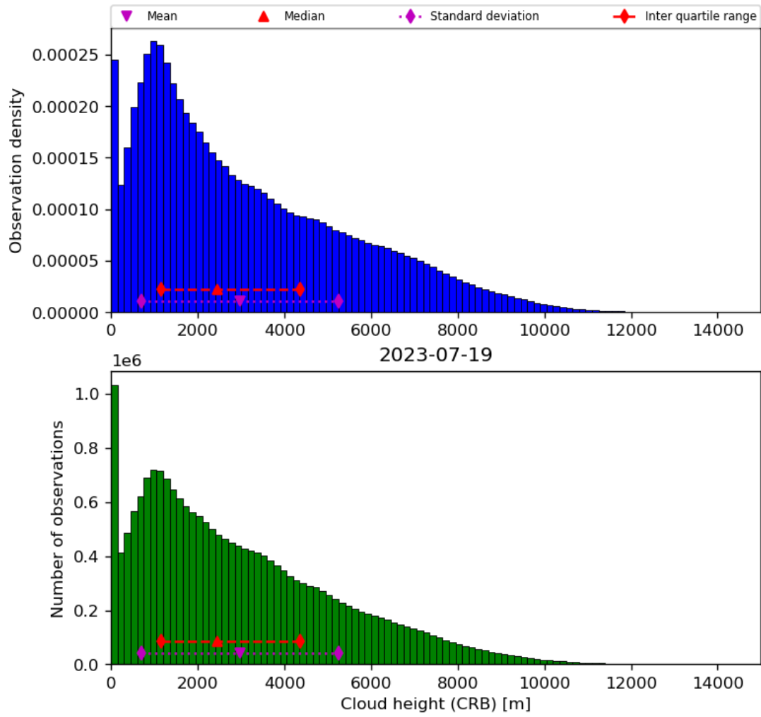
Figure 43: Histogram of “Cloud height (CRB)” for 2023-07-19 to 2023-07-20
