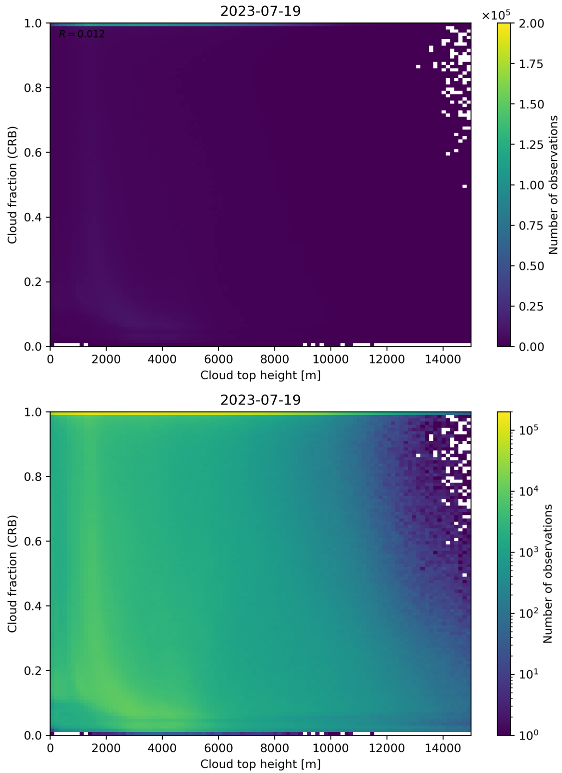
Figure 88: Scatter density plot of “Cloud top height” against “Cloud fraction (CRB)” for 2023-07-19 to 2023-07-20.
