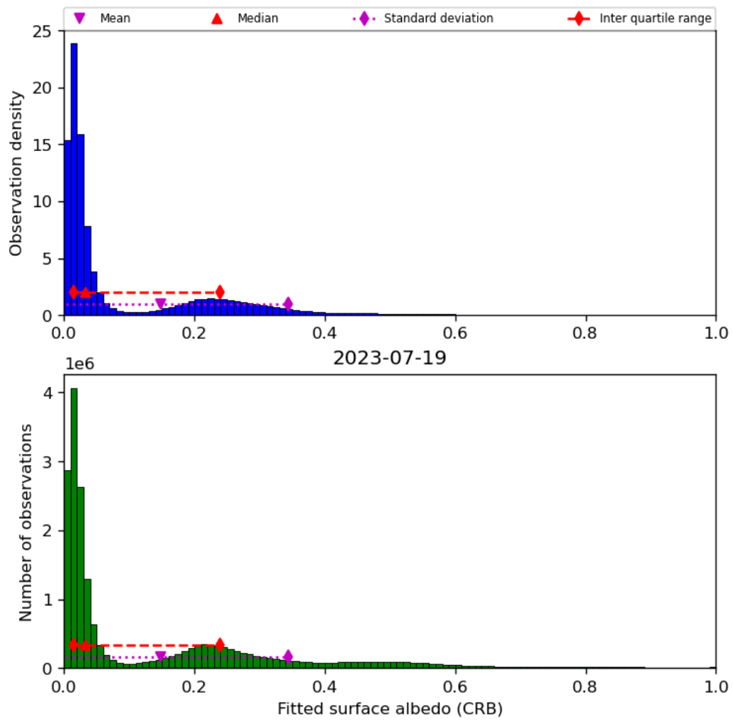
Figure 46: Histogram of “Fitted surface albedo (CRB)” for 2023-07-19 to 2023-07-20
