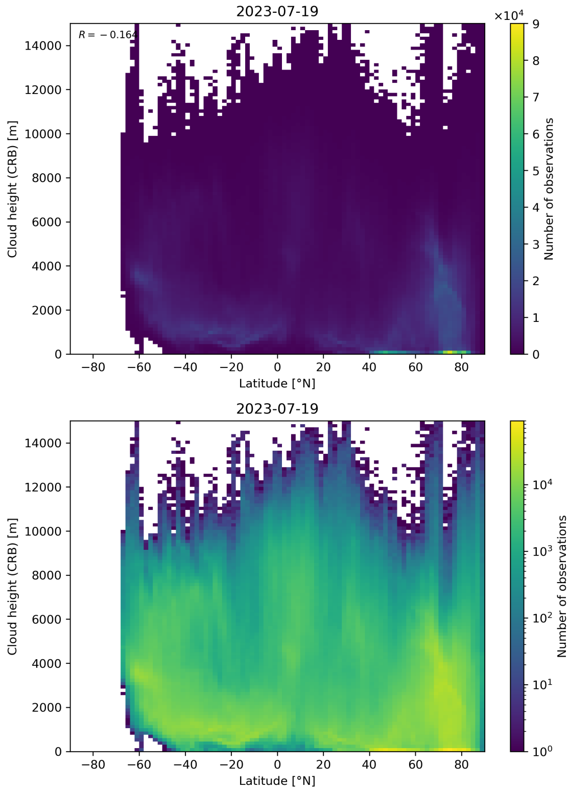
Figure 95: Scatter density plot of “Latitude” against “Cloud height (CRB)” for 2023-07-19 to 2023-07-20.
