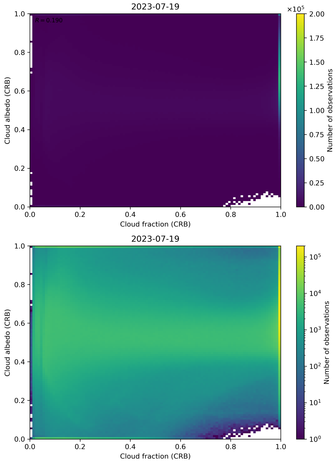
Figure 77: Scatter density plot of “Cloud fraction (CRB)” against “Cloud albedo (CRB)” for 2023-07-19 to 2023-07-20.
