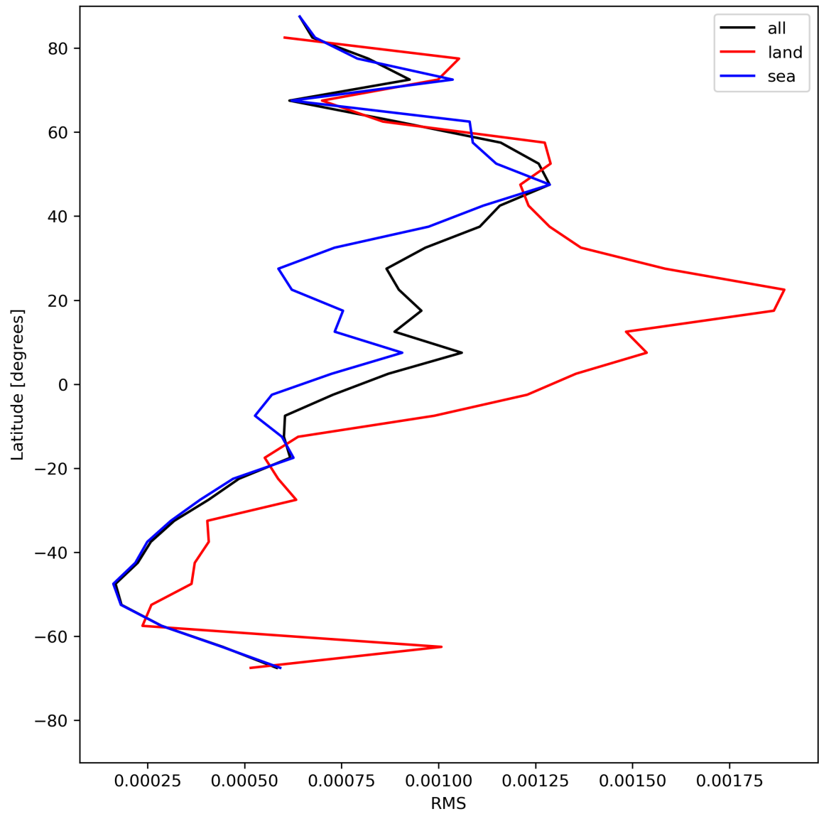
Figure 31: Zonal average of “RMS” for 2023-07-19 to 2023-07-20.
