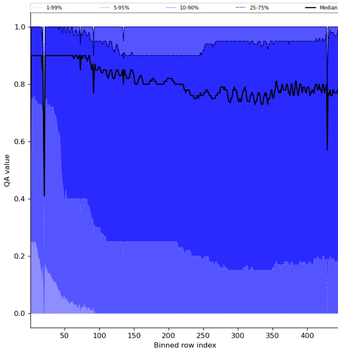
Figure 54: Along track statistics of “QA value” for 2023-07-19 to 2023-07-20
