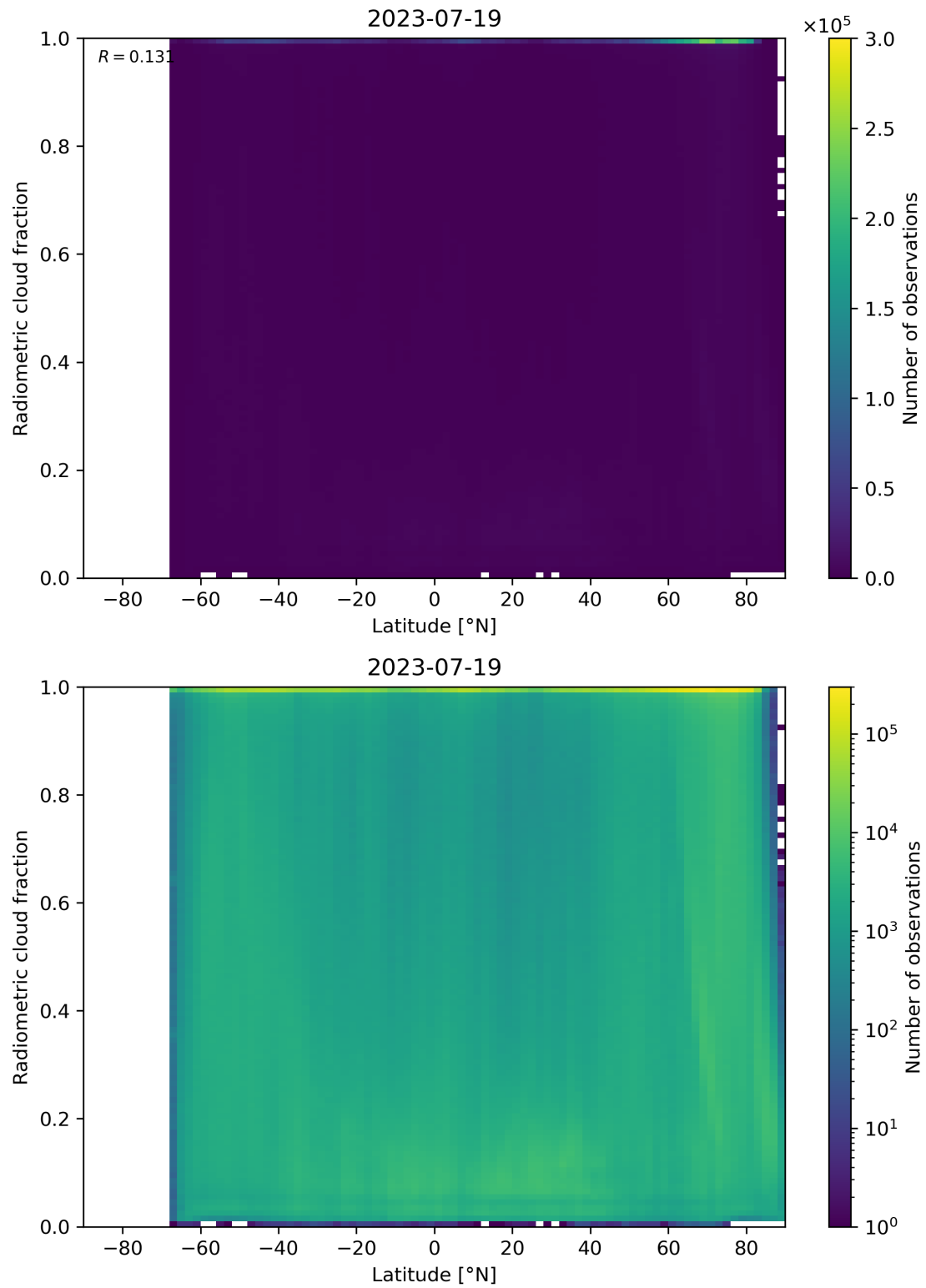
Figure 92: Scatter density plot of “Latitude” against “Radiometric cloud fraction” for 2023-07-19 to 2023-07-20.
