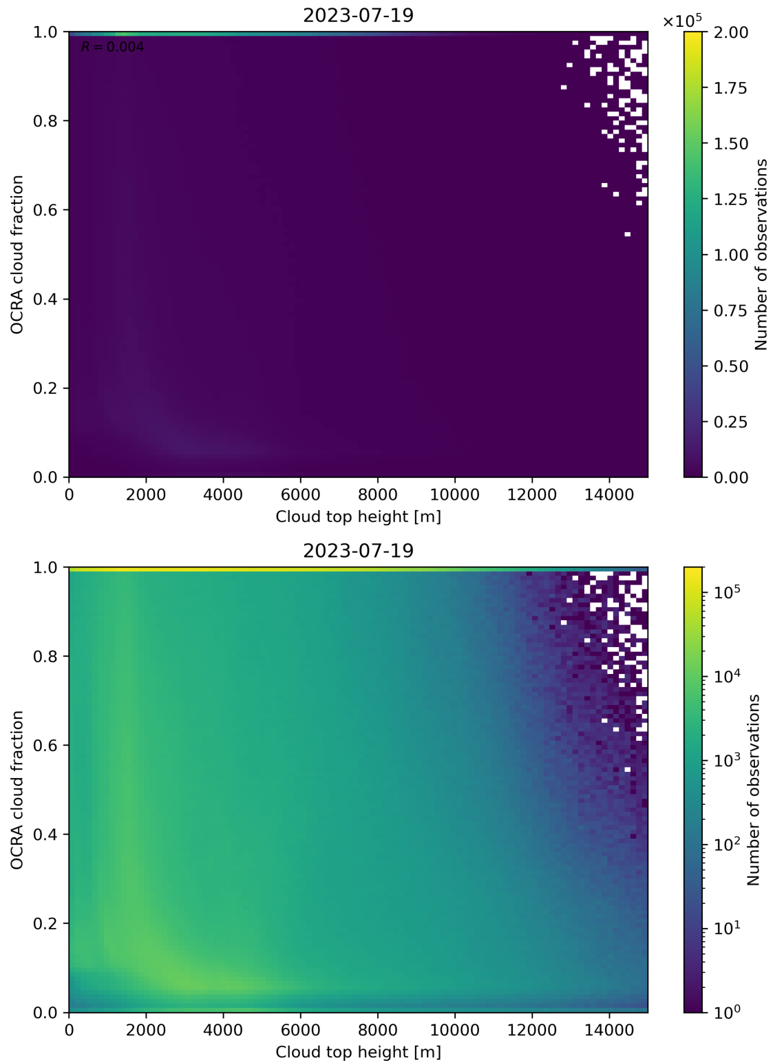
Figure 87: Scatter density plot of “Cloud top height” against “OCRA cloud fraction” for 2023-07-19 to 2023-07-20.
