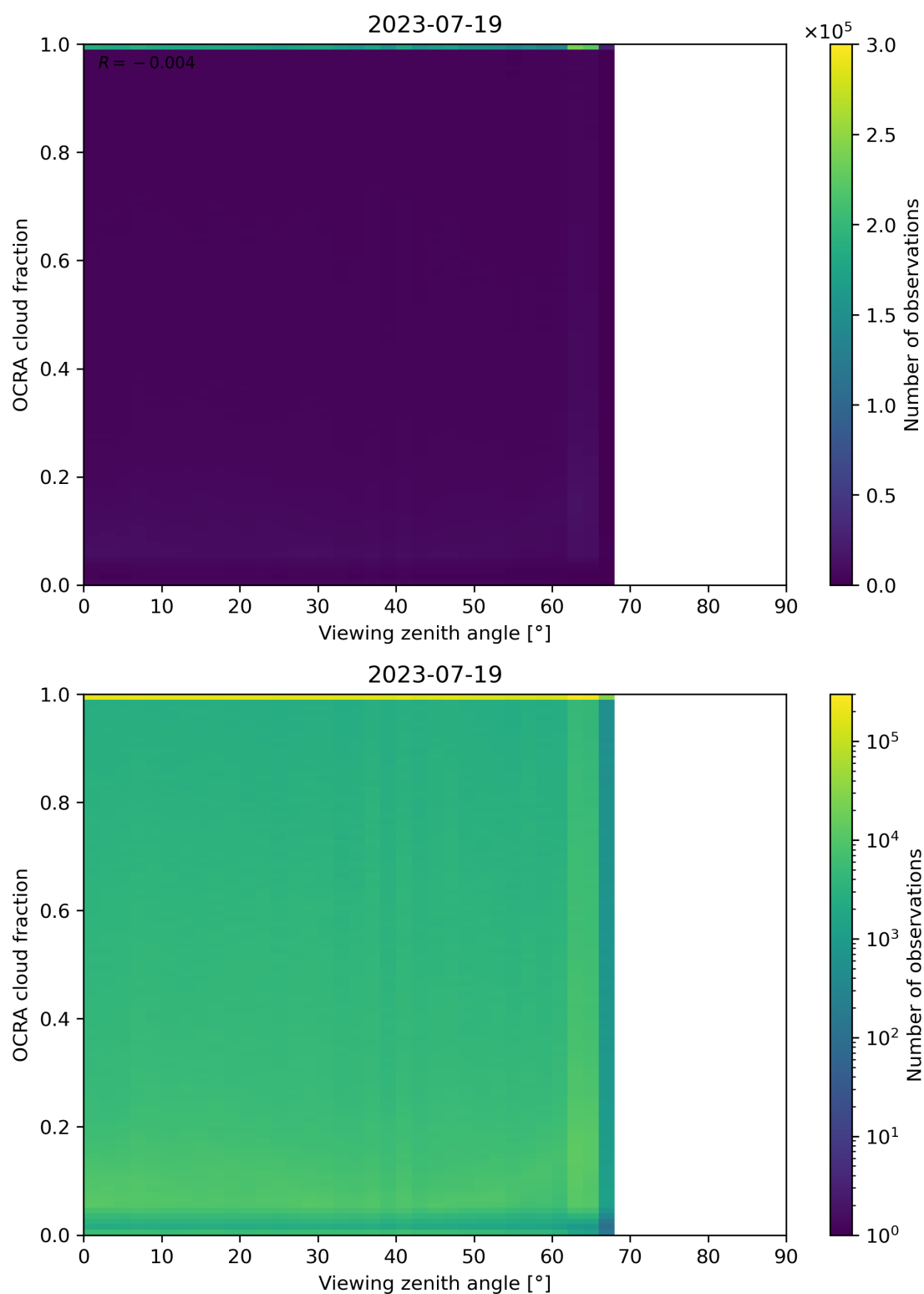
Figure 108: Scatter density plot of “Viewing zenith angle” against “OCRA cloud fraction” for 2023-07-19 to 2023-07-20.
