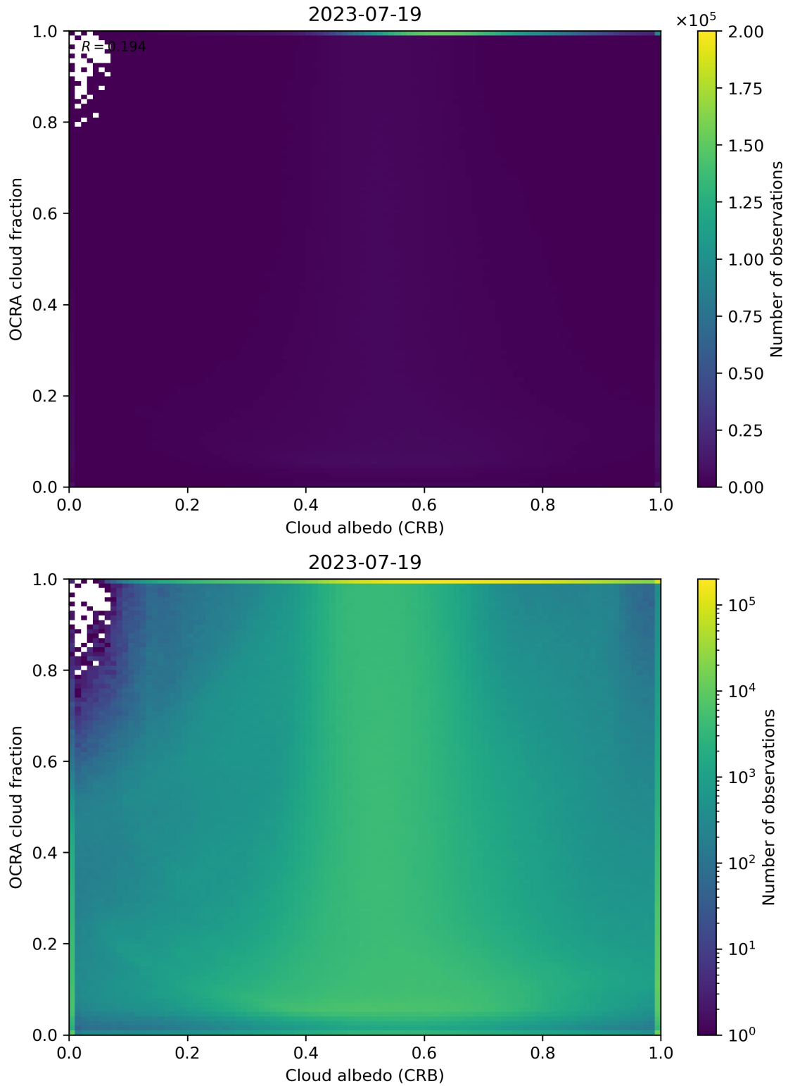
Figure 70: Scatter density plot of “Cloud albedo (CRB)” against “OCRA cloud fraction” for 2023-07-19 to 2023-07-20.
