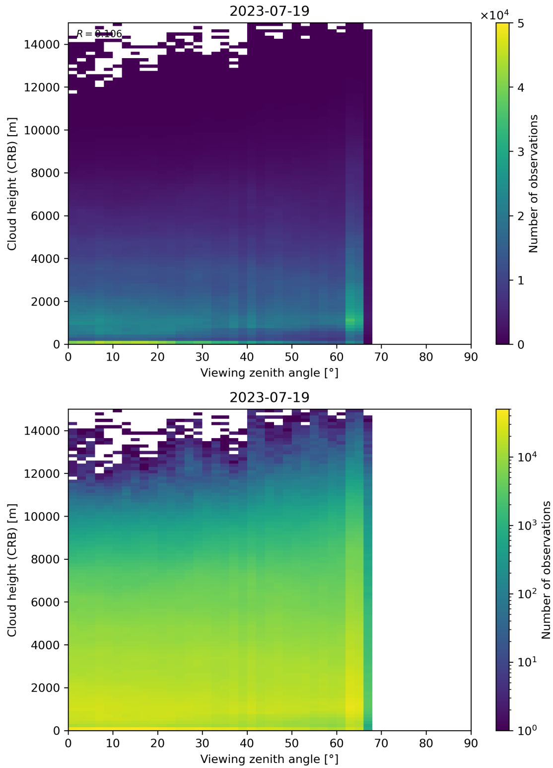
Figure 110: Scatter density plot of “Viewing zenith angle” against “Cloud height (CRB)” for 2023-07-19 to 2023-07-20.
