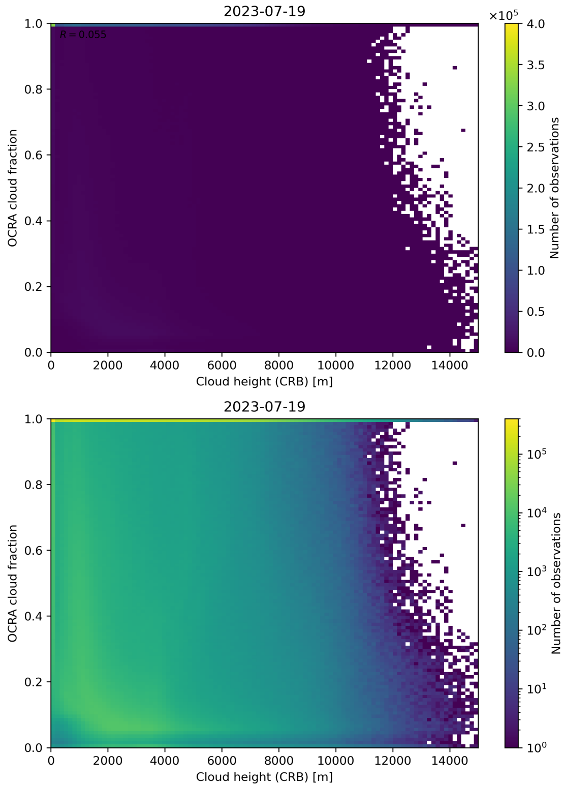
Figure 81: Scatter density plot of “Cloud height (CRB)” against “OCRA cloud fraction” for 2023-07-19 to 2023-07-20.
