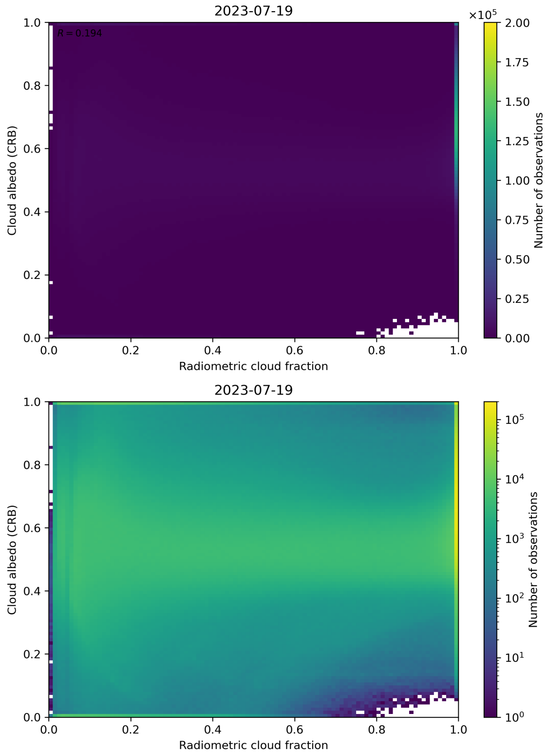
Figure 71: Scatter density plot of “Radiometric cloud fraction” against “Cloud albedo (CRB)” for 2023-07-19 to 2023-07-20.
