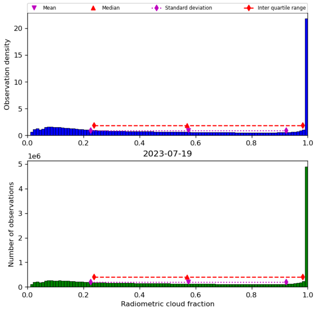
Figure 39: Histogram of “Radiometric cloud fraction” for 2023-07-19 to 2023-07-20
