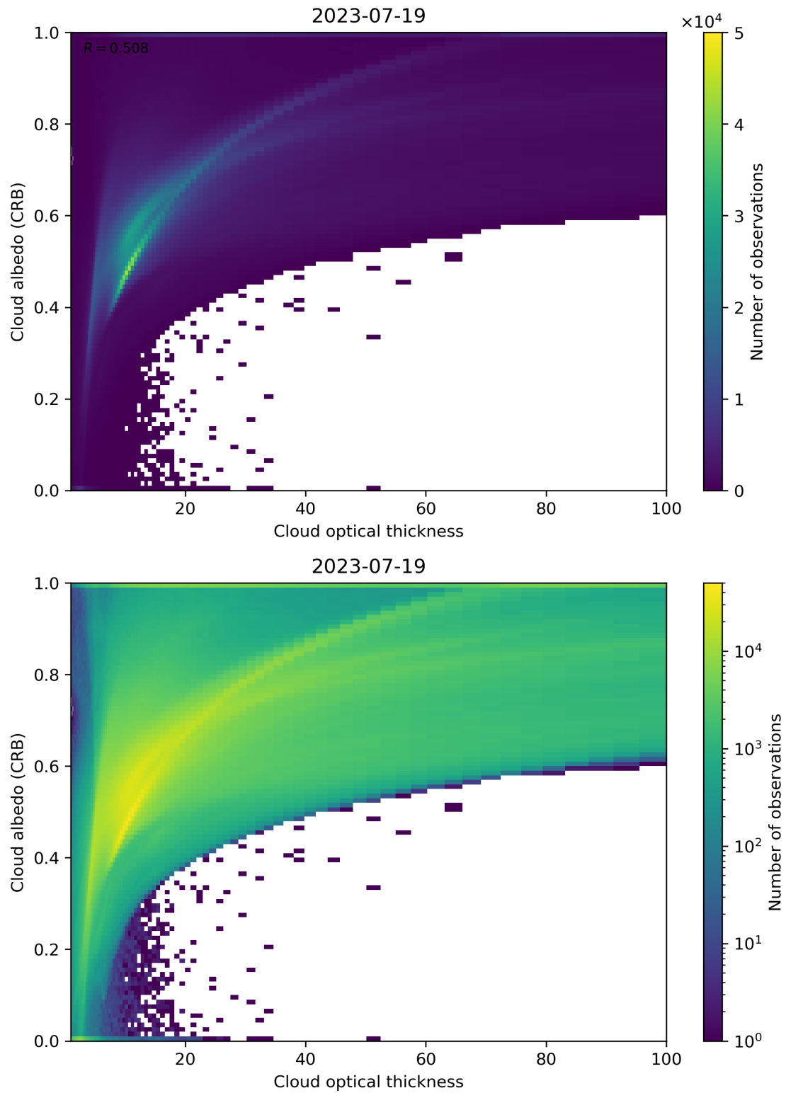
Figure 82: Scatter density plot of “Cloud optical thickness” against “Cloud albedo (CRB)” for 2023-07-19 to 2023-07-20.
