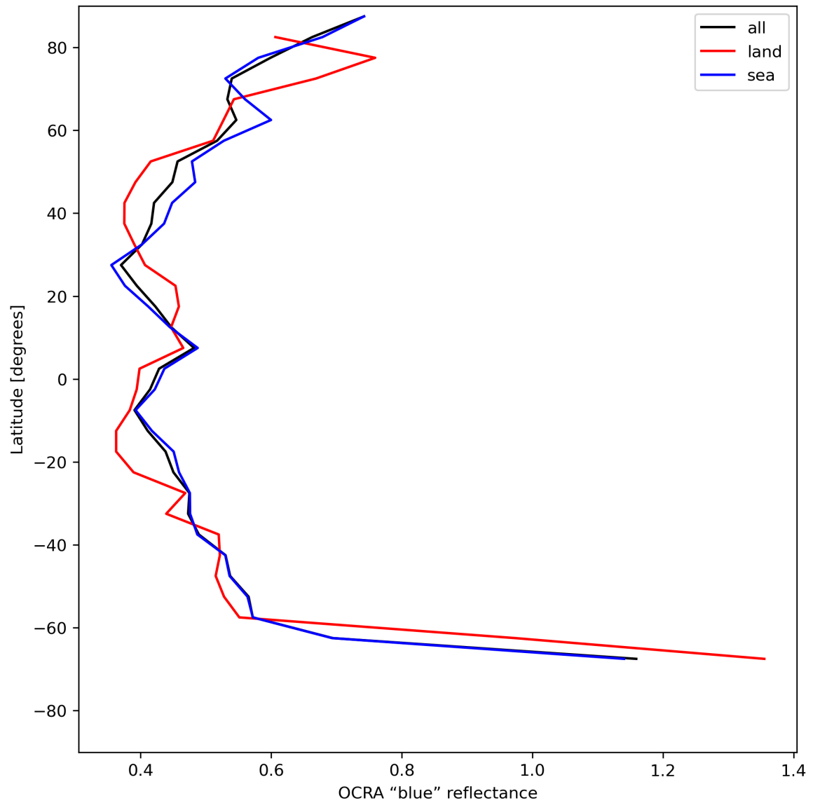
Figure 35: Zonal average of “OCRA “blue” reflectance” for 2023-07-19 to 2023-07-20.
