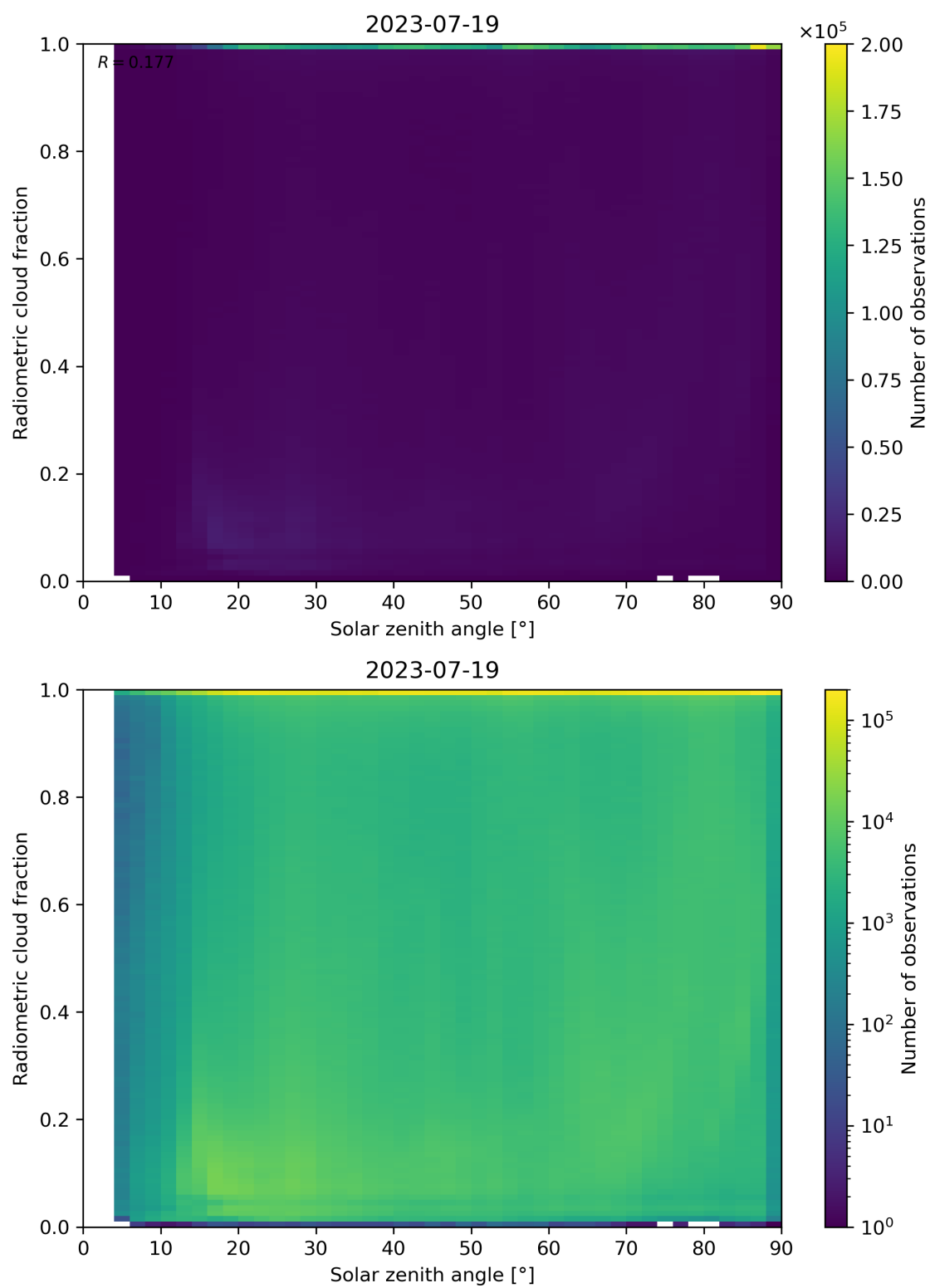
Figure 99: Scatter density plot of “Solar zenith angle” against “Radiometric cloud fraction” for 2023-07-19 to 2023-07-20.
