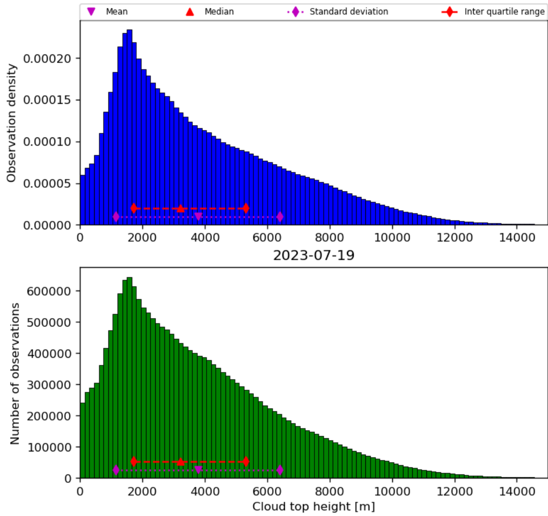
Figure 40: Histogram of “Cloud top height” for 2023-07-19 to 2023-07-20
