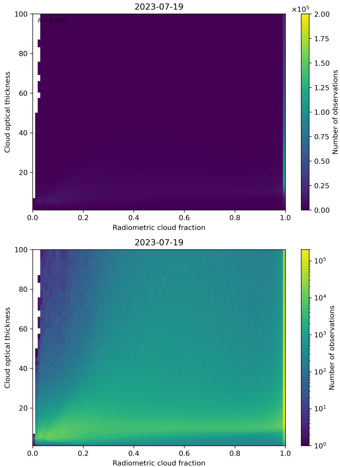
Figure 75: Scatter density plot of “Radiometric cloud fraction” against “Cloud optical thickness” for 2023-07-19 to 2023-07-20.
