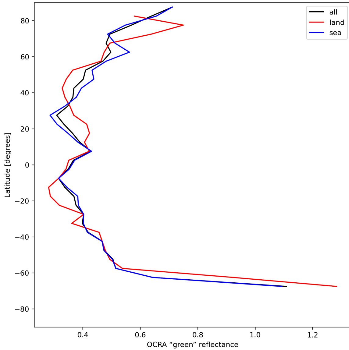
Figure 36: Zonal average of “OCRA “green” reflectance” for 2023-07-19 to 2023-07-20.
