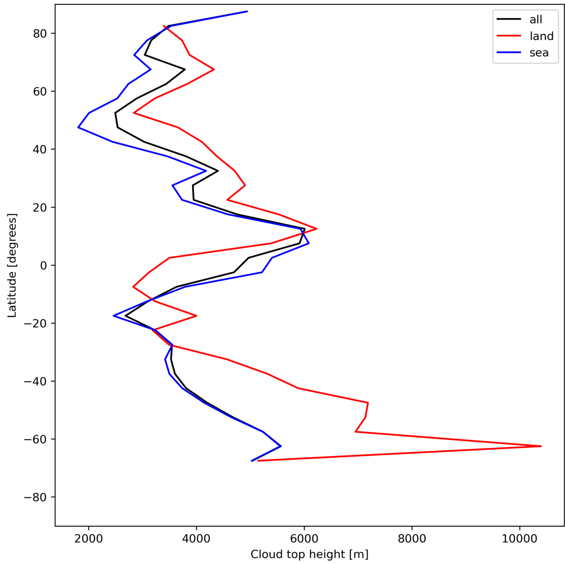
Figure 24: Zonal average of “Cloud top height” for 2023-07-19 to 2023-07-20.
