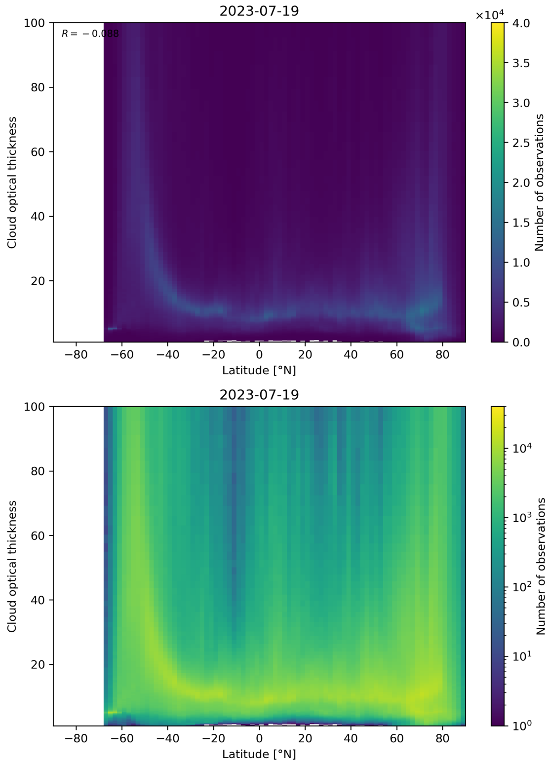
Figure 96: Scatter density plot of “Latitude” against “Cloud optical thickness” for 2023-07-19 to 2023-07-20.
