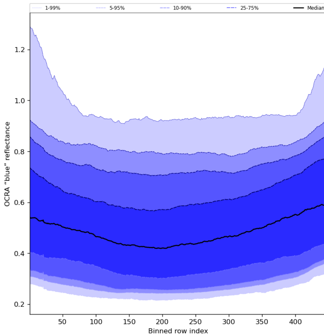
Figure 67: Along track statistics of “OCRA “blue” reflectance” for 2023-07-19 to 2023-07-20
