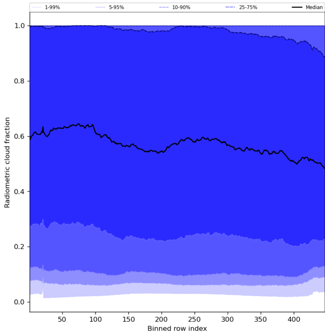
Figure 55: Along track statistics of “Radiometric cloud fraction” for 2023-07-19 to 2023-07-20
