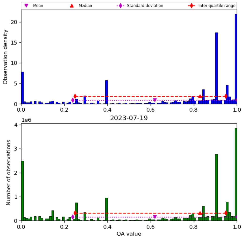
Figure 38: Histogram of “QA value” for 2023-07-19 to 2023-07-20
