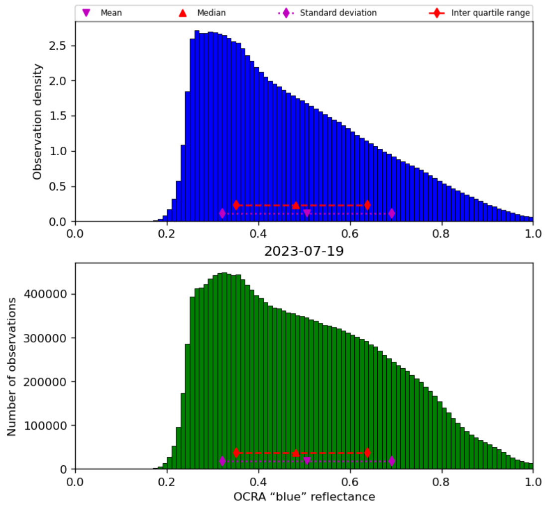
Figure 51: Histogram of “OCRA “blue” reflectance” for 2023-07-19 to 2023-07-20
