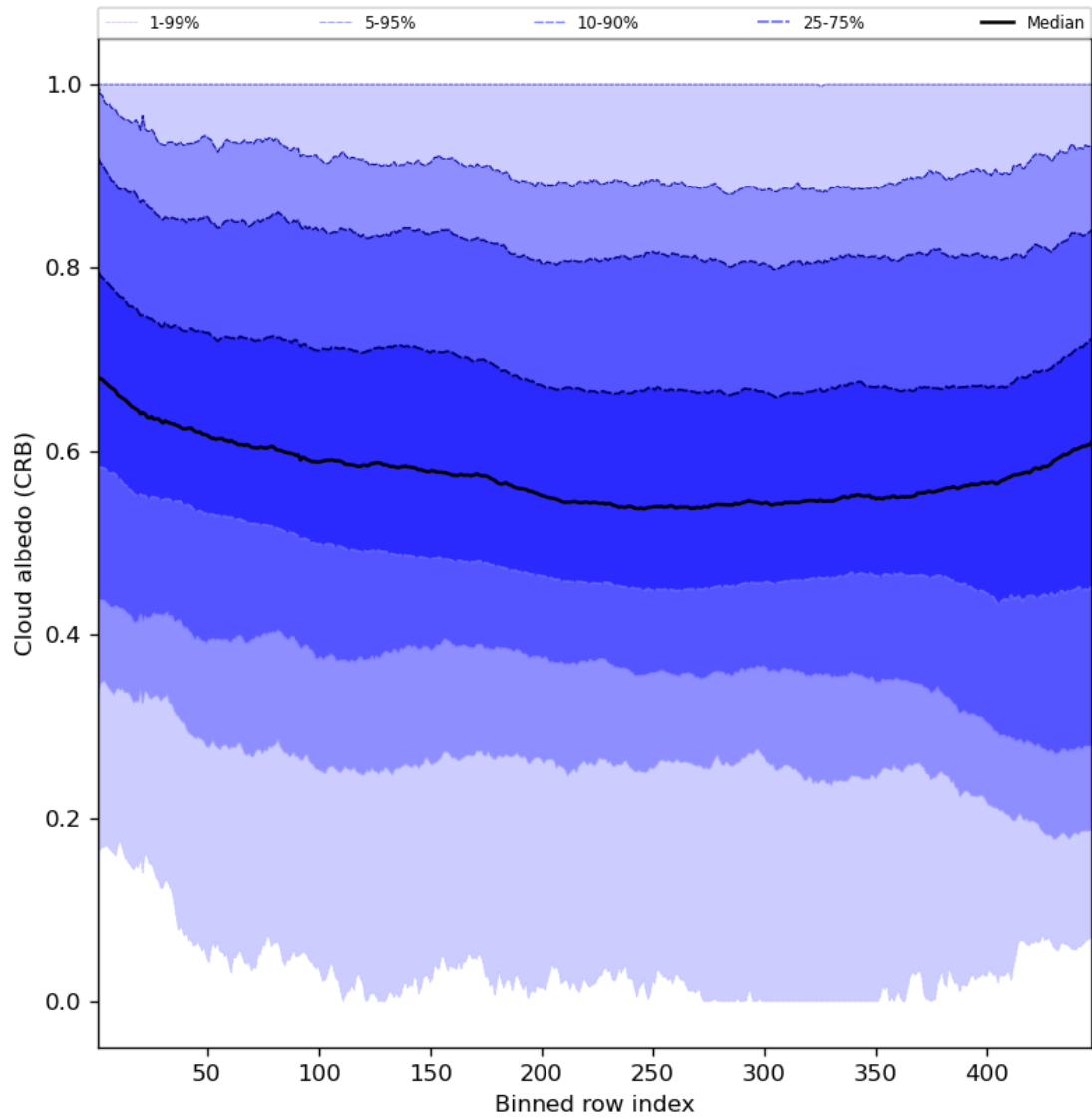
Figure 60: Along track statistics of “Cloud albedo (CRB)” for 2023-07-19 to 2023-07-20
