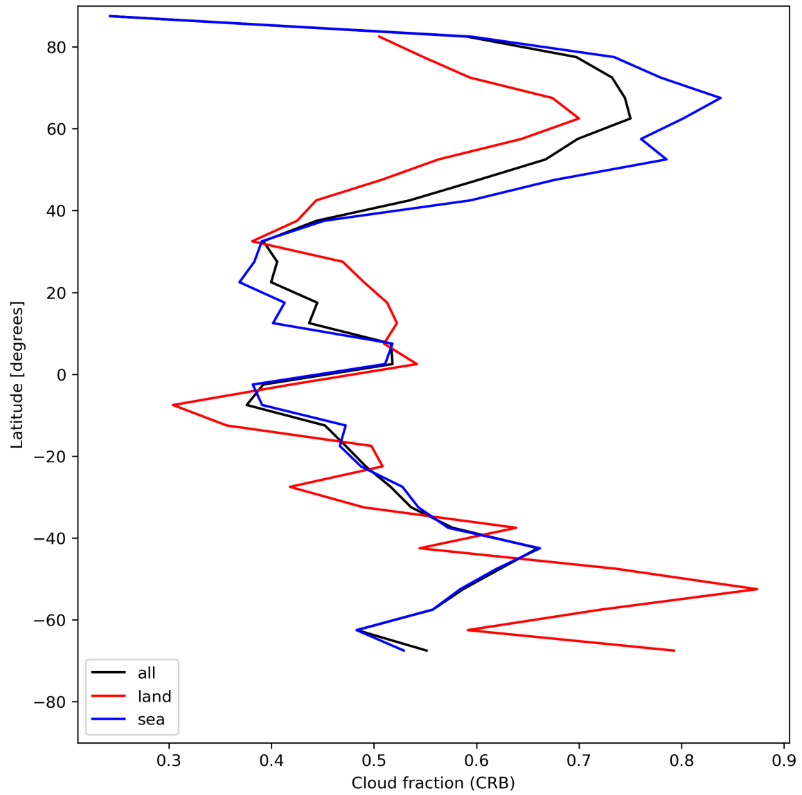
Figure 26: Zonal average of “Cloud fraction (CRB)” for 2023-07-20 to 2023-07-22.
