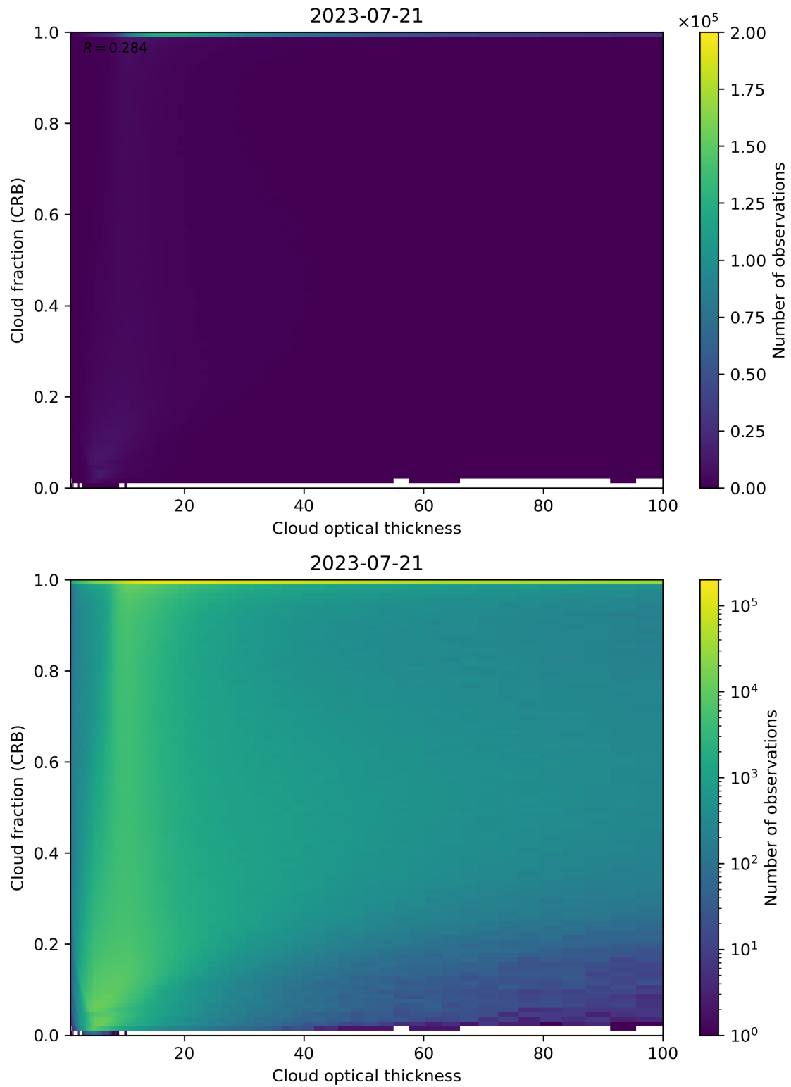
Figure 84: Scatter density plot of “Cloud optical thickness” against “Cloud fraction (CRB)” for 2023-07-20 to 2023-07-22.
