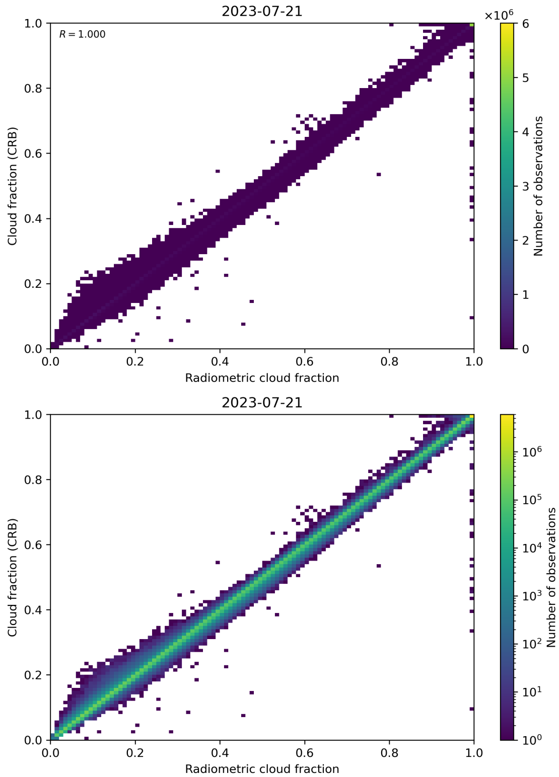
Figure 73: Scatter density plot of “Radiometric cloud fraction” against “Cloud fraction (CRB)” for 2023-07-20 to 2023-07-22.
