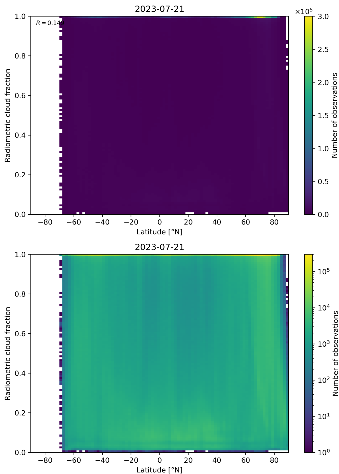
Figure 92: Scatter density plot of “Latitude” against “Radiometric cloud fraction” for 2023-07-20 to 2023-07-22.
