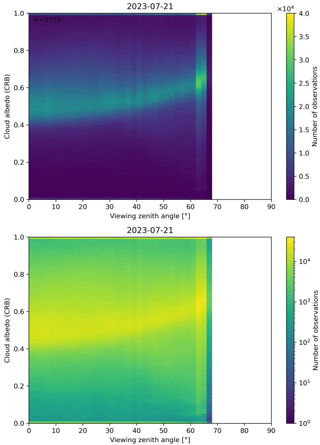
Figure 106: Scatter density plot of “Viewing zenith angle” against “Cloud albedo (CRB)” for 2023-07-20 to 2023-07-22.
