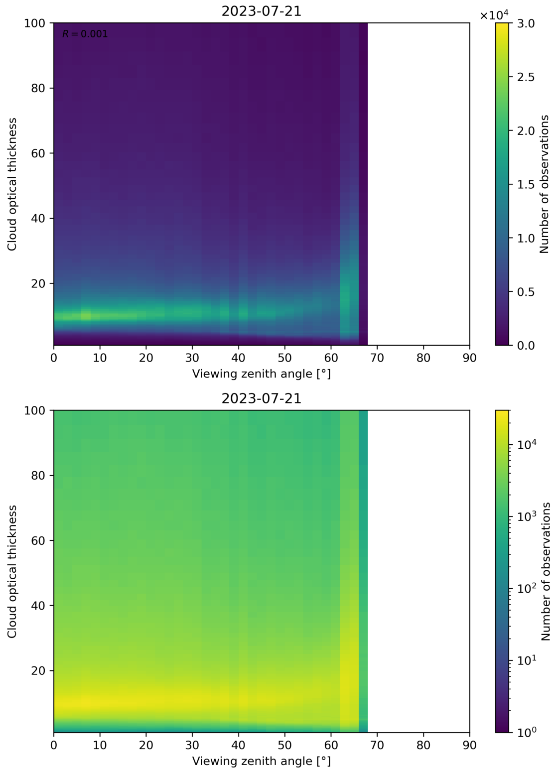
Figure 111: Scatter density plot of “Viewing zenith angle” against “Cloud optical thickness” for 2023-07-20 to 2023-07-22.
