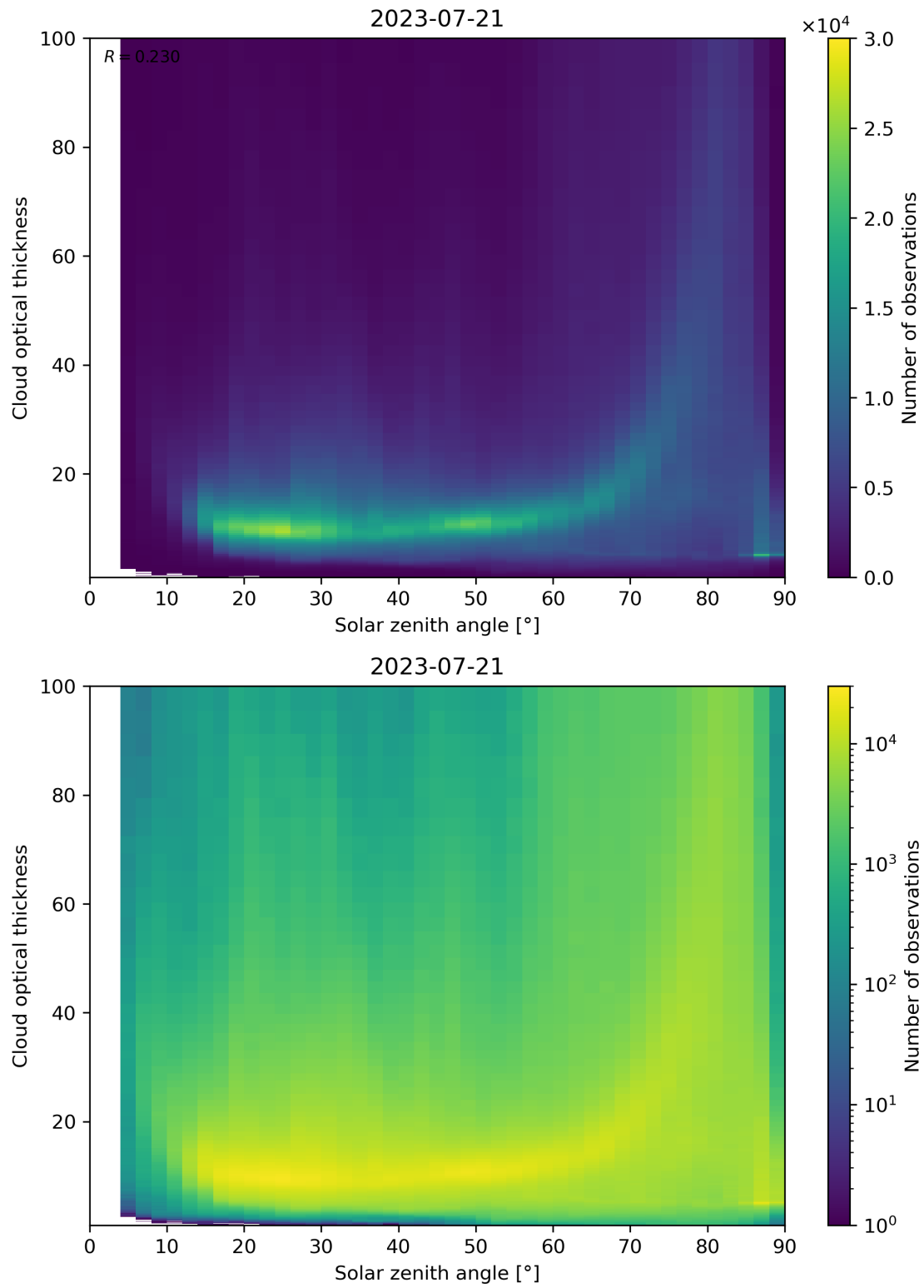
Figure 103: Scatter density plot of “Solar zenith angle” against “Cloud optical thickness” for 2023-07-20 to 2023-07-22.
