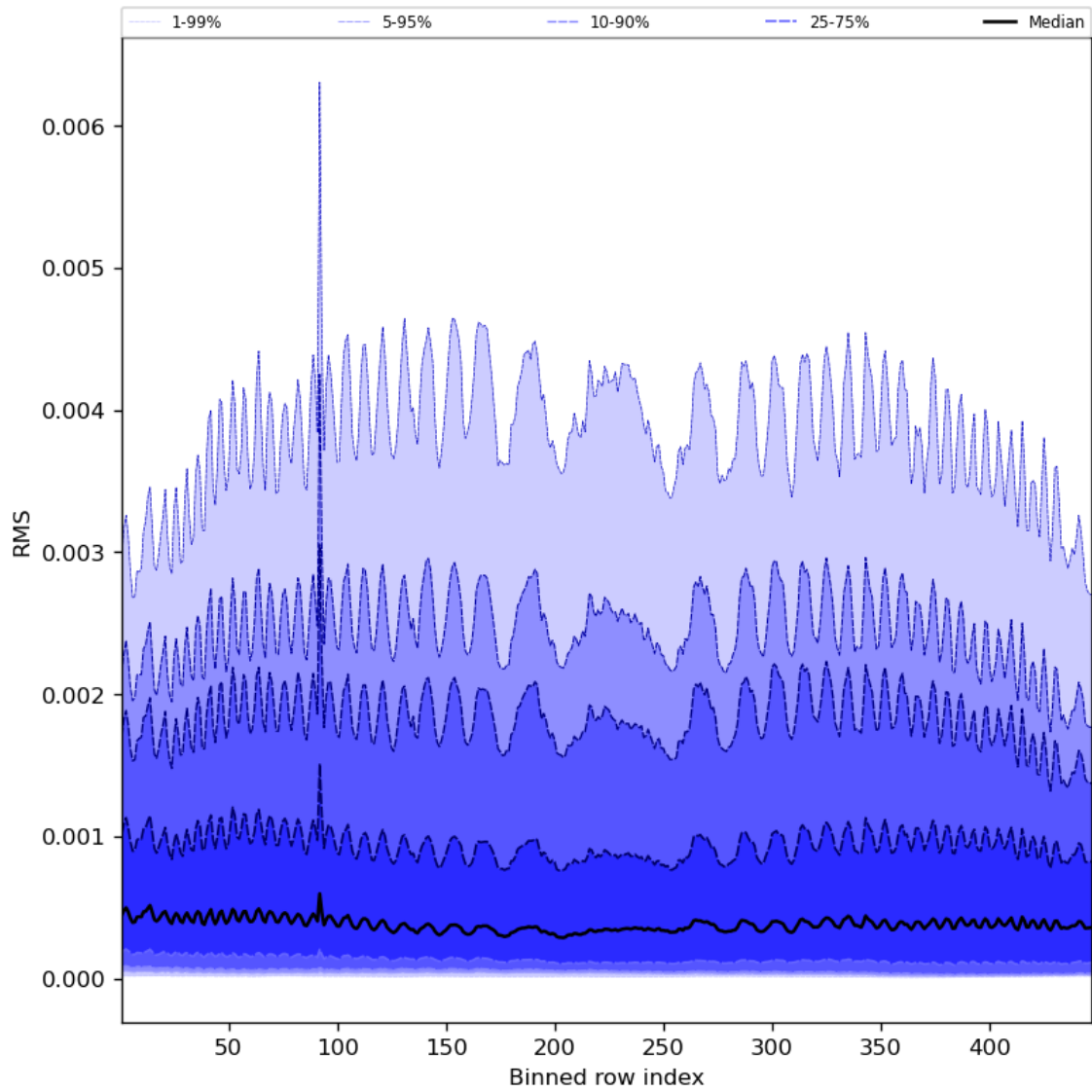
Figure 63: Along track statistics of “RMS” for 2023-07-20 to 2023-07-22
