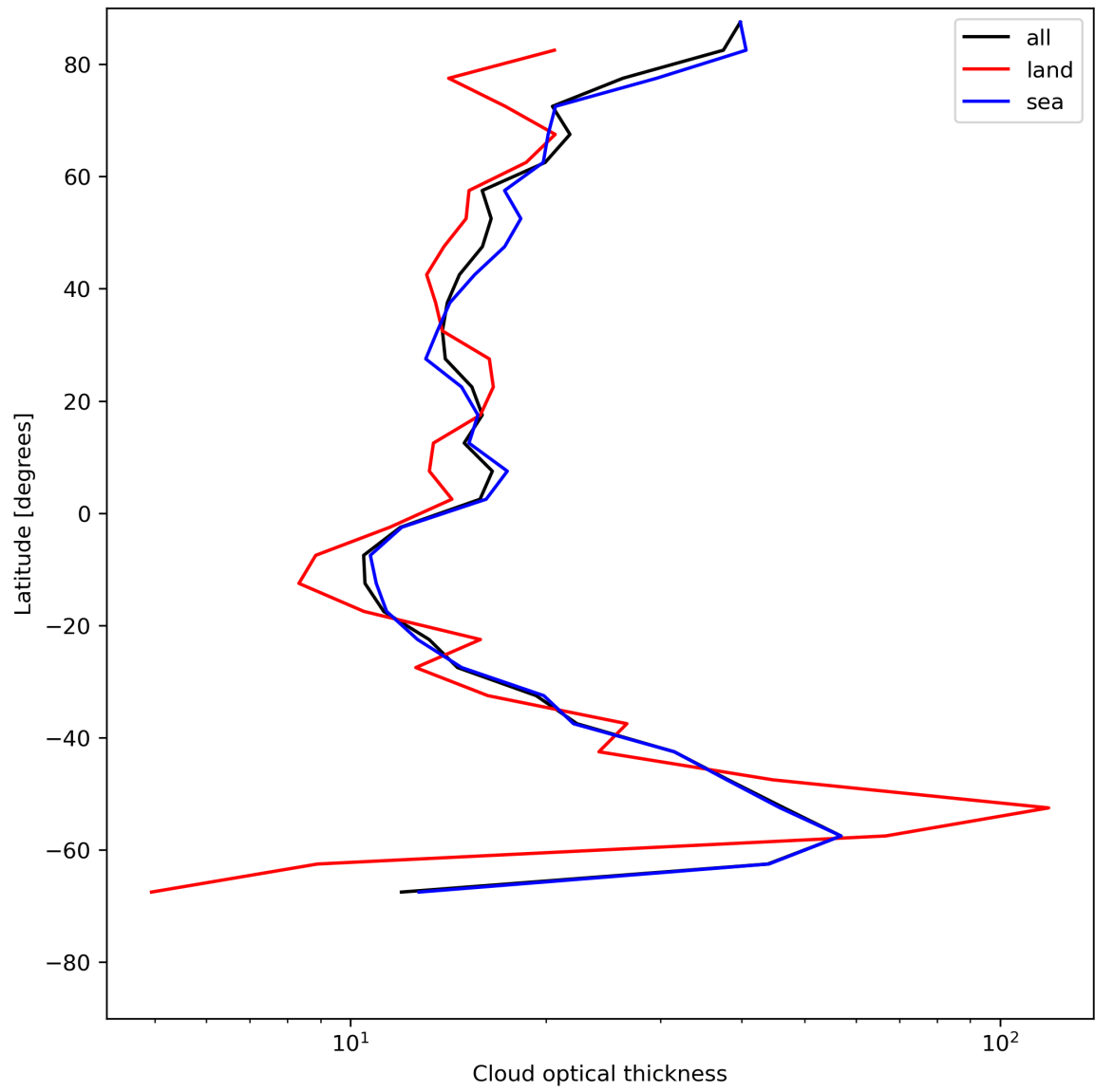
Figure 25: Zonal average of “Cloud optical thickness” for 2023-07-20 to 2023-07-22.
