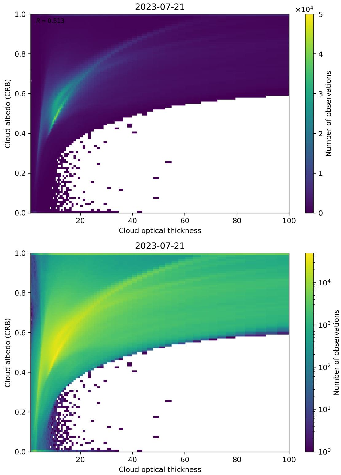
Figure 82: Scatter density plot of “Cloud optical thickness” against “Cloud albedo (CRB)” for 2023-07-20 to 2023-07-22.
