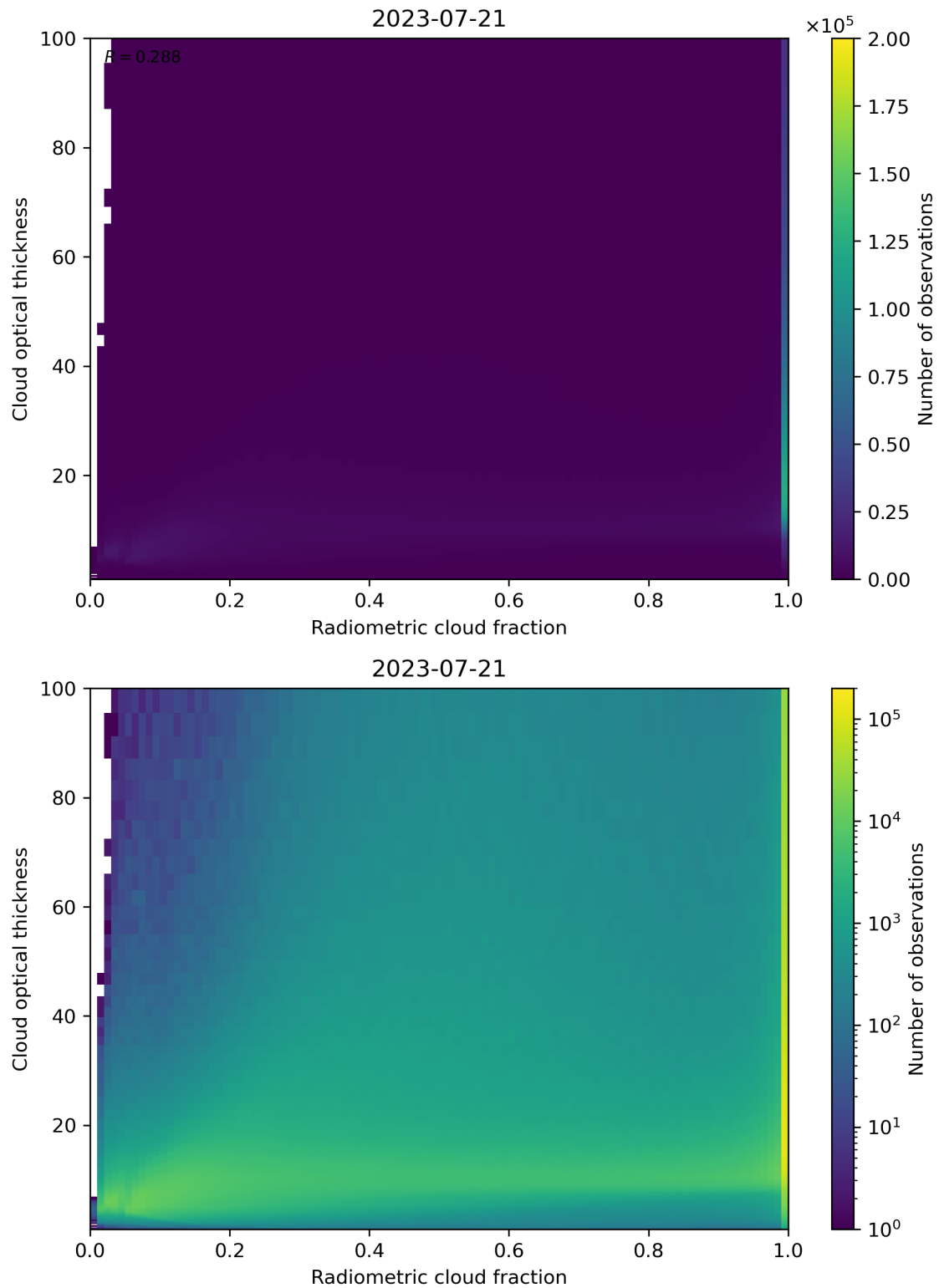
Figure 75: Scatter density plot of “Radiometric cloud fraction” against “Cloud optical thickness” for 2023-07-20 to 2023-07-22.
