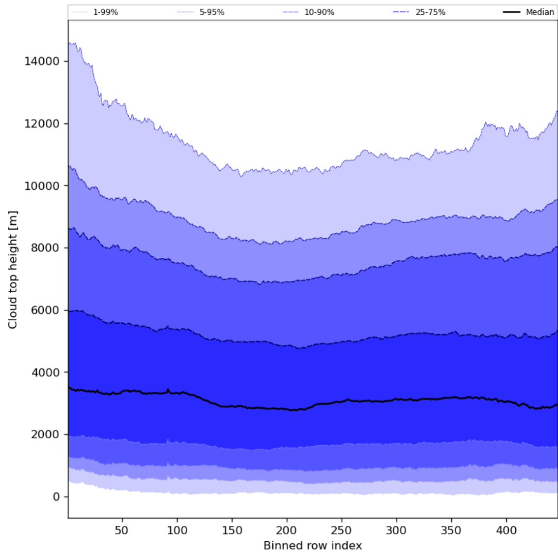
Figure 56: Along track statistics of “Cloud top height” for 2023-07-20 to 2023-07-22
