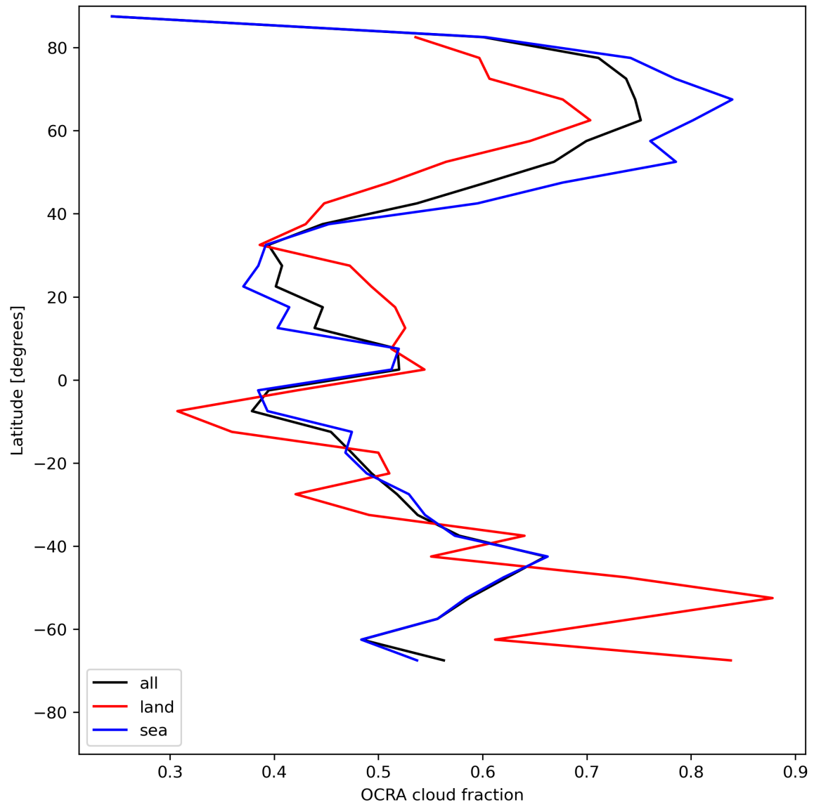
Figure 34: Zonal average of “OCRA cloud fraction” for 2023-07-20 to 2023-07-22.
