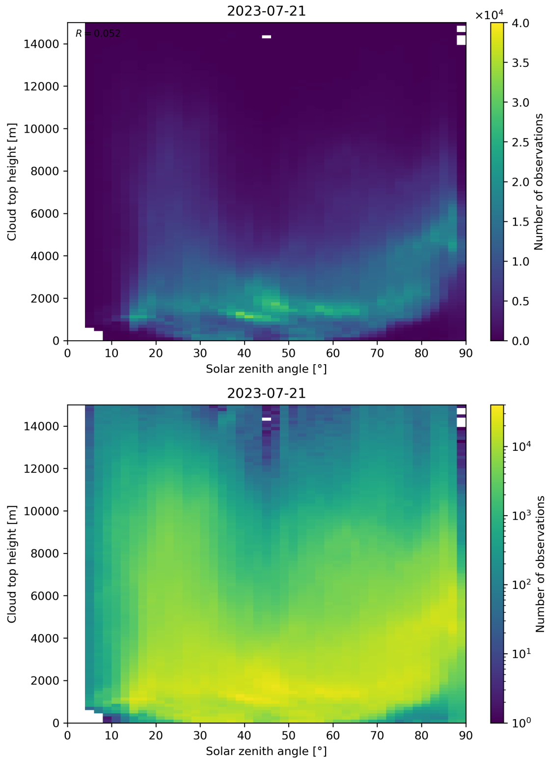
Figure 104: Scatter density plot of “Solar zenith angle” against “Cloud top height” for 2023-07-20 to 2023-07-22.
