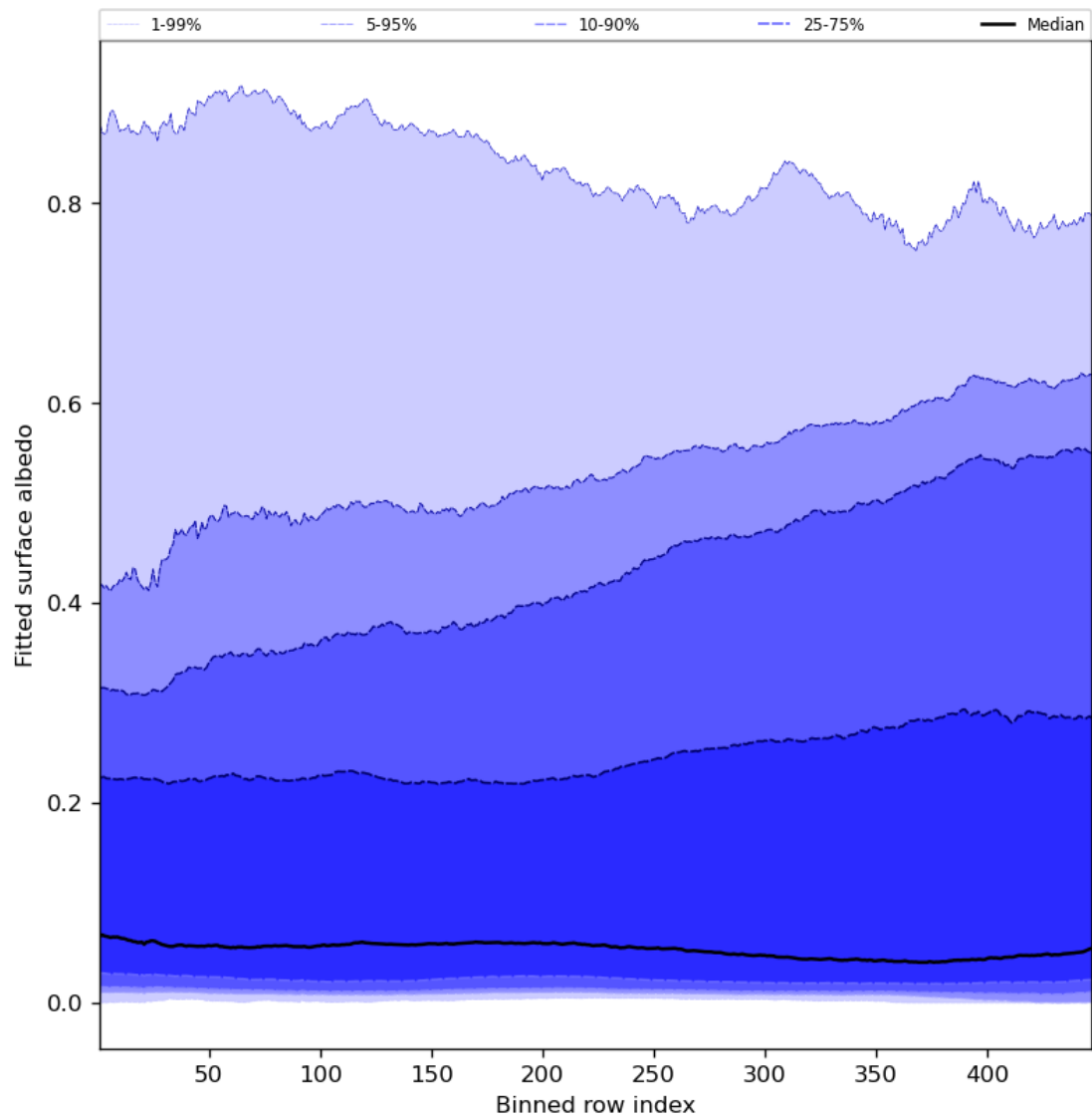
Figure 61: Along track statistics of “Fitted surface albedo” for 2023-07-20 to 2023-07-22
