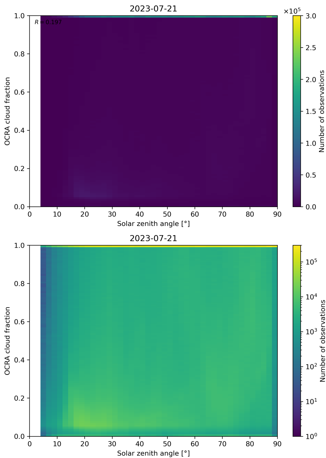
Figure 100: Scatter density plot of “Solar zenith angle” against “OCRA cloud fraction” for 2023-07-20 to 2023-07-22.
