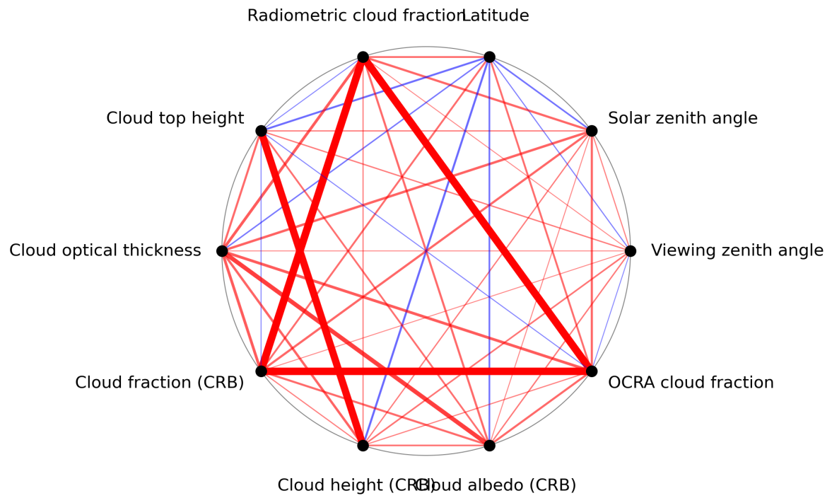
Figure 1: Map of correlation graph for 2023-07-20 to 2023-07-22.
