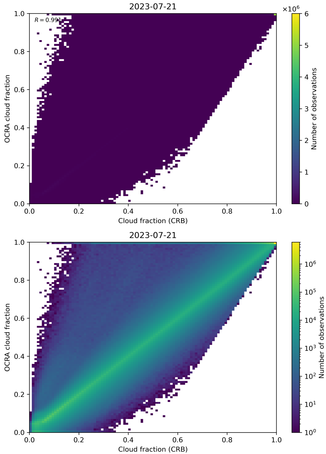
Figure 78: Scatter density plot of “Cloud fraction (CRB)” against “OCRA cloud fraction” for 2023-07-20 to 2023-07-22.
