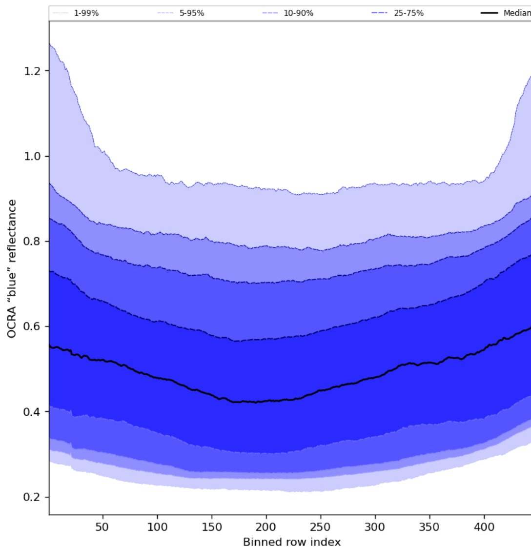
Figure 67: Along track statistics of “OCRA “blue” reflectance” for 2023-07-20 to 2023-07-22
