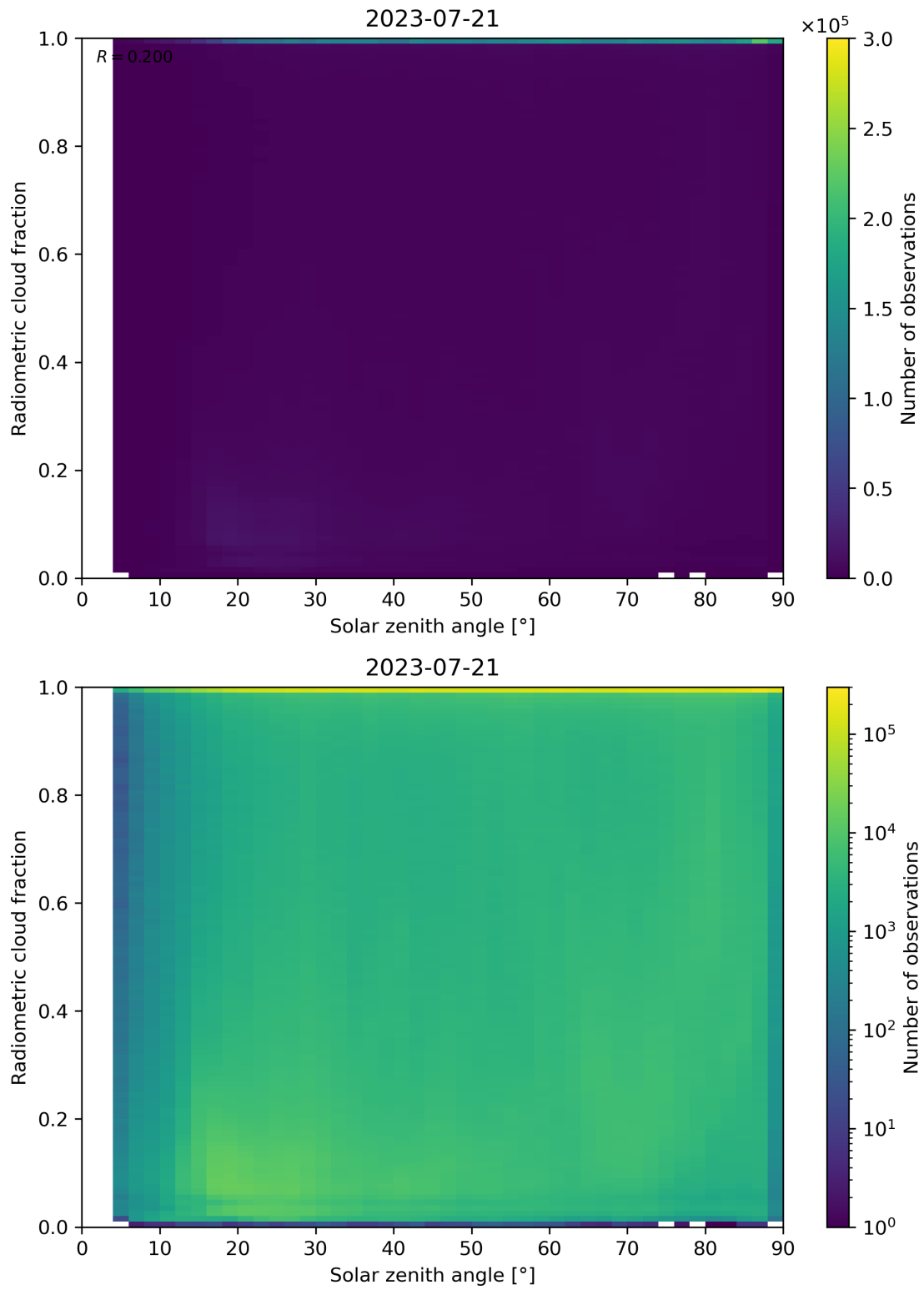
Figure 99: Scatter density plot of “Solar zenith angle” against “Radiometric cloud fraction” for 2023-07-20 to 2023-07-22.
