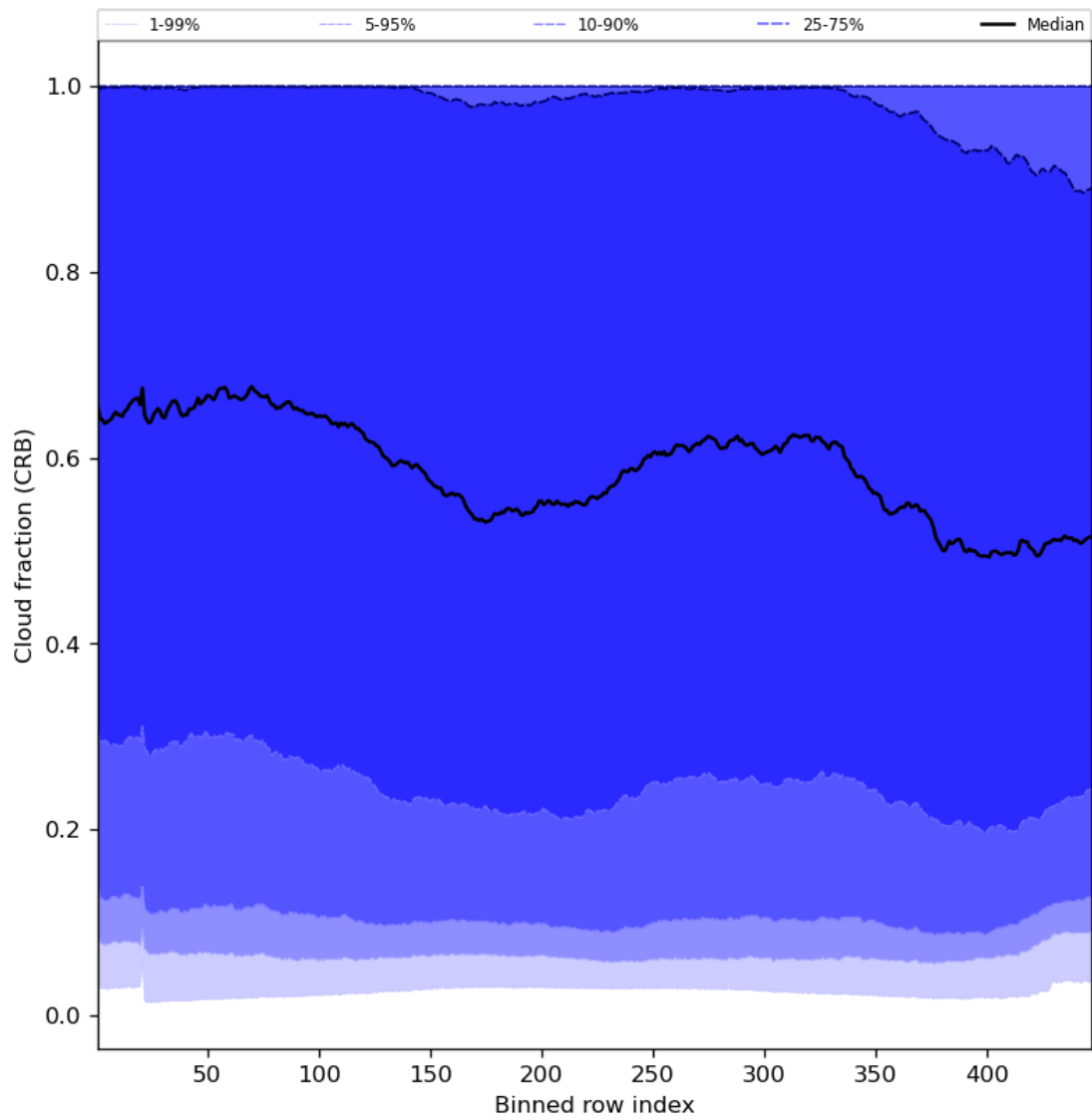
Figure 58: Along track statistics of “Cloud fraction (CRB)” for 2023-07-20 to 2023-07-22
