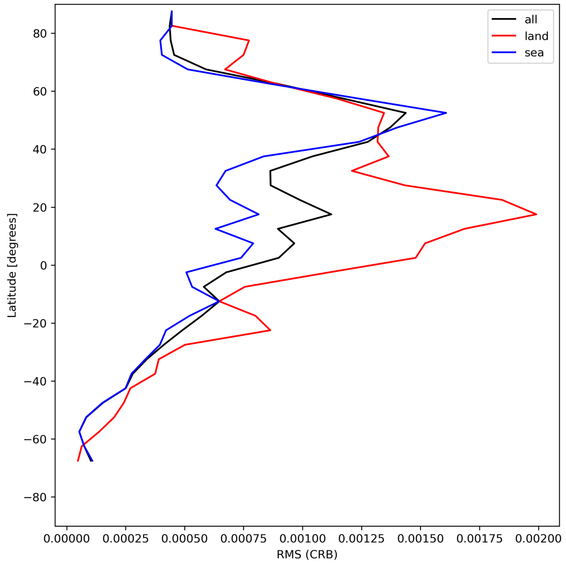
Figure 32: Zonal average of “RMS (CRB)” for 2023-07-20 to 2023-07-22.
