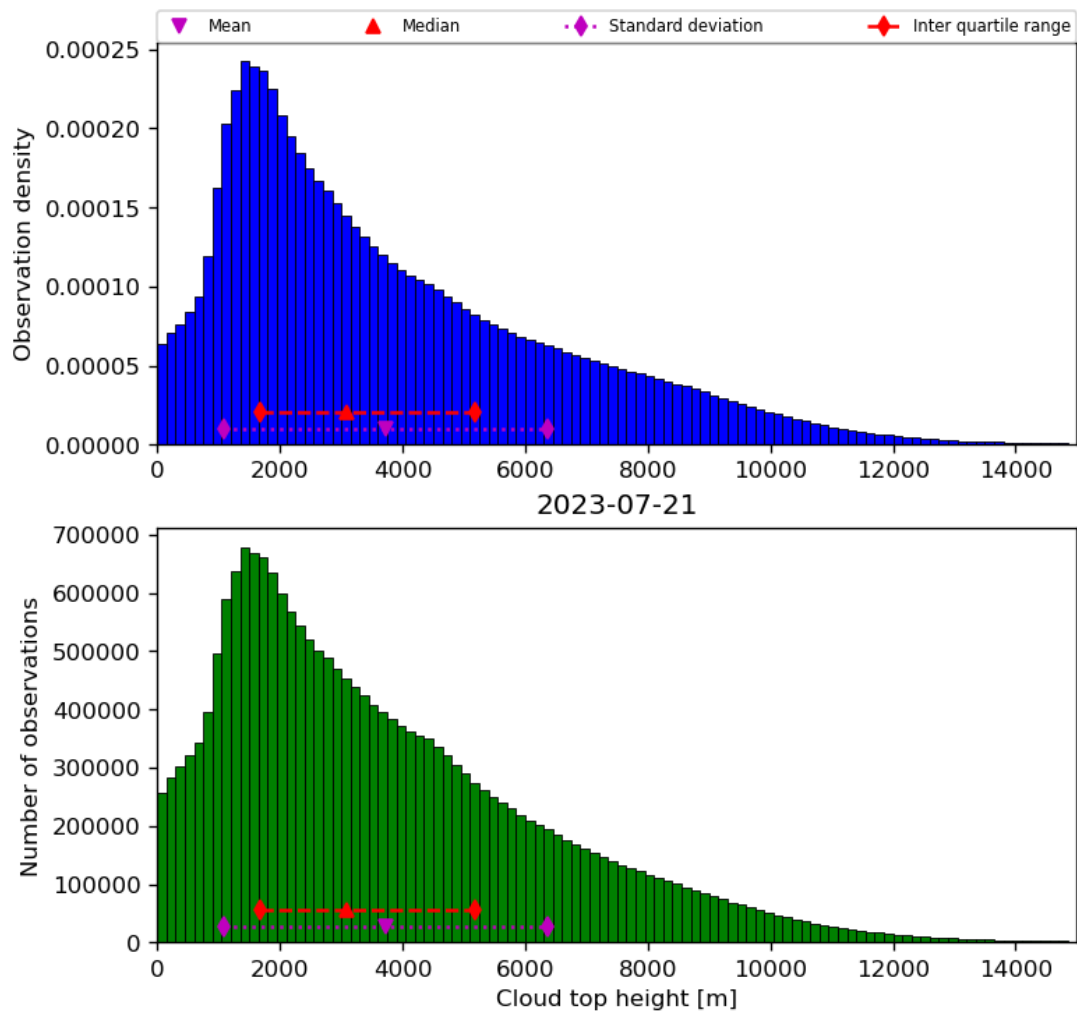
Figure 40: Histogram of “Cloud top height” for 2023-07-20 to 2023-07-22
