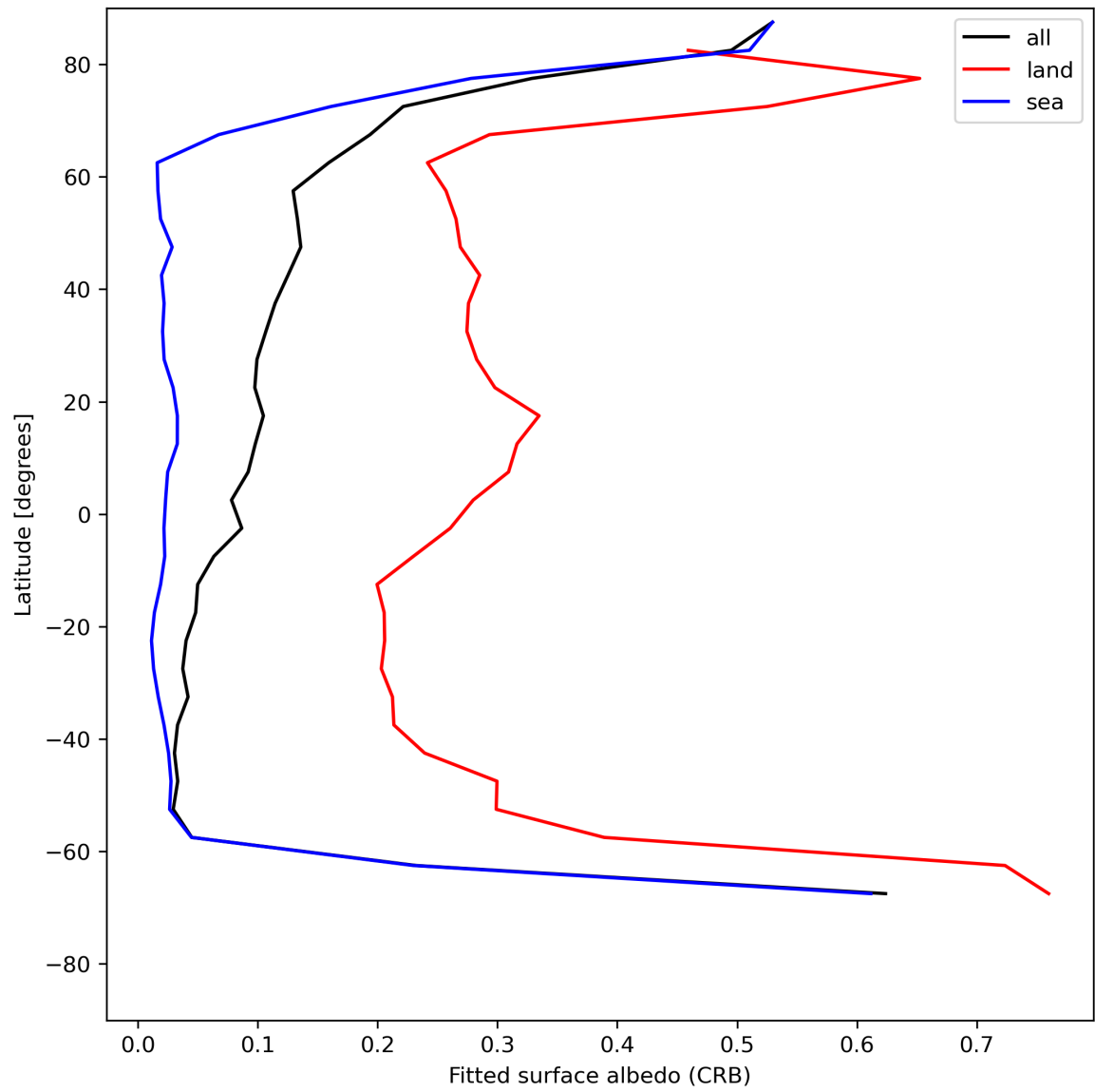
Figure 30: Zonal average of “Fitted surface albedo (CRB)” for 2023-07-20 to 2023-07-22.
