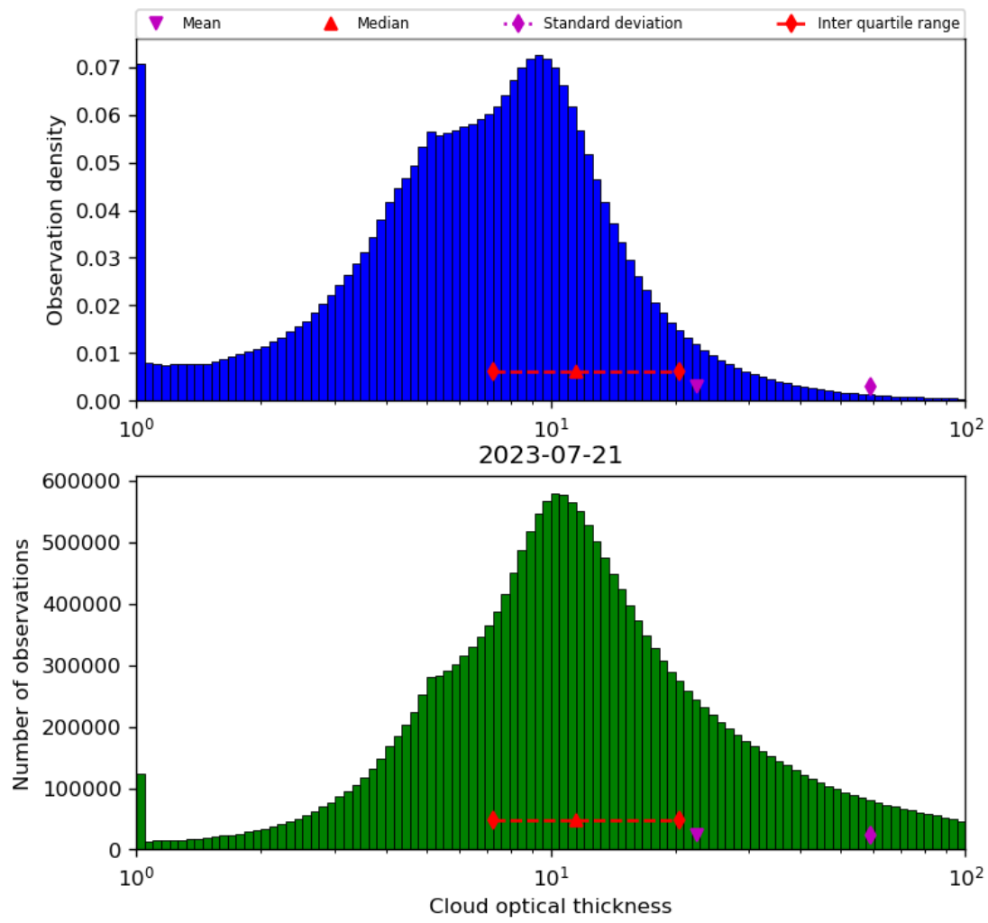
Figure 41: Histogram of “Cloud optical thickness” for 2023-07-20 to 2023-07-22
