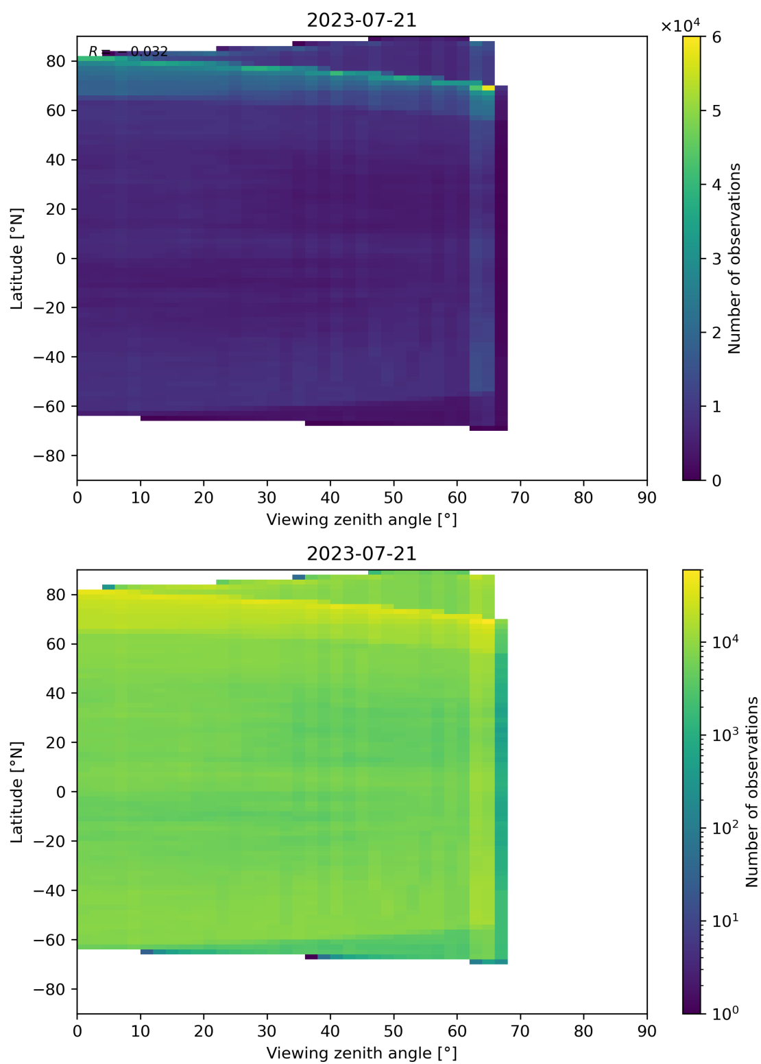
Figure 113: Scatter density plot of “Viewing zenith angle” against “Latitude” for 2023-07-20 to 2023-07-22.
