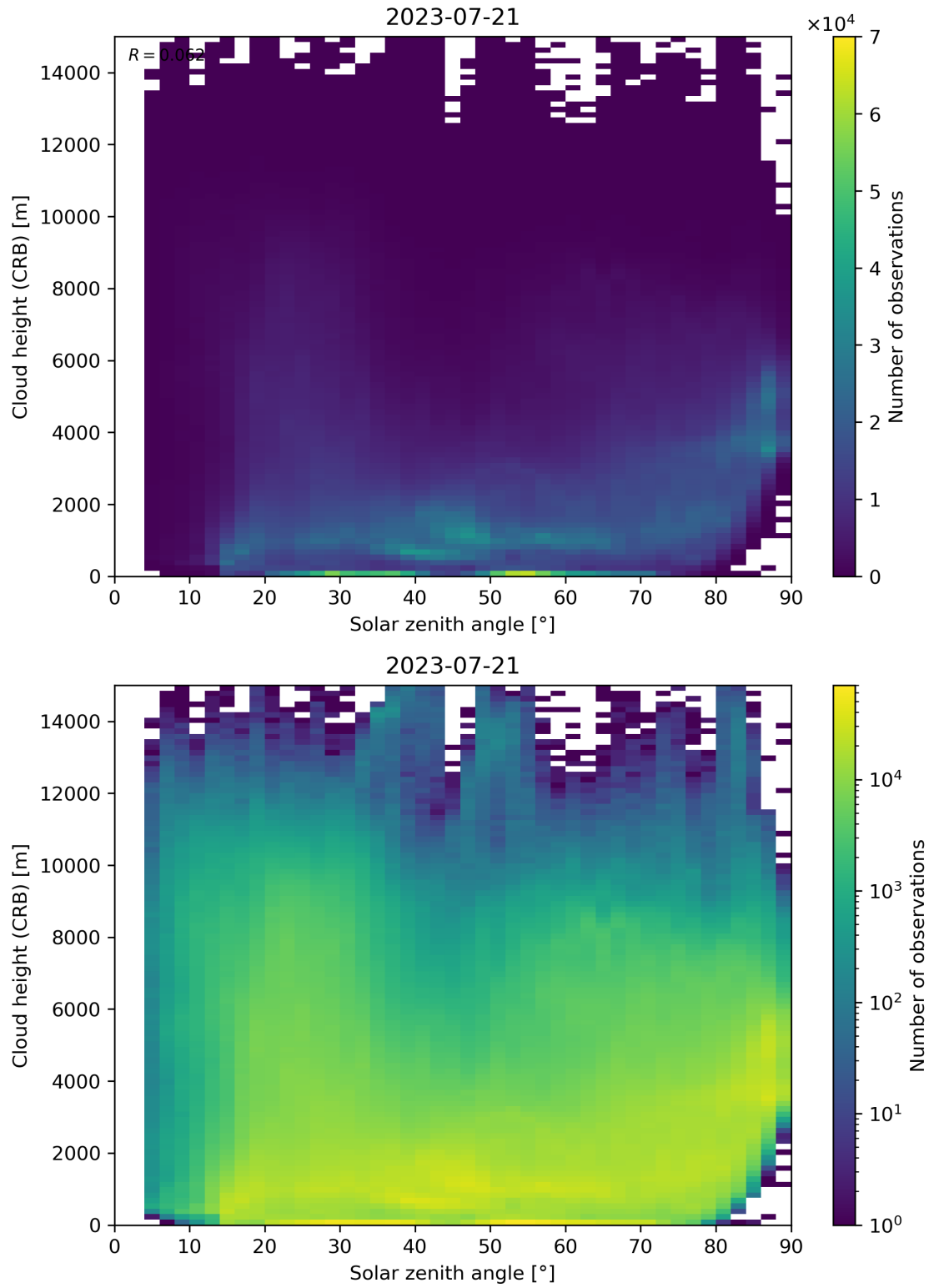
Figure 102: Scatter density plot of “Solar zenith angle” against “Cloud height (CRB)” for 2023-07-20 to 2023-07-22.
