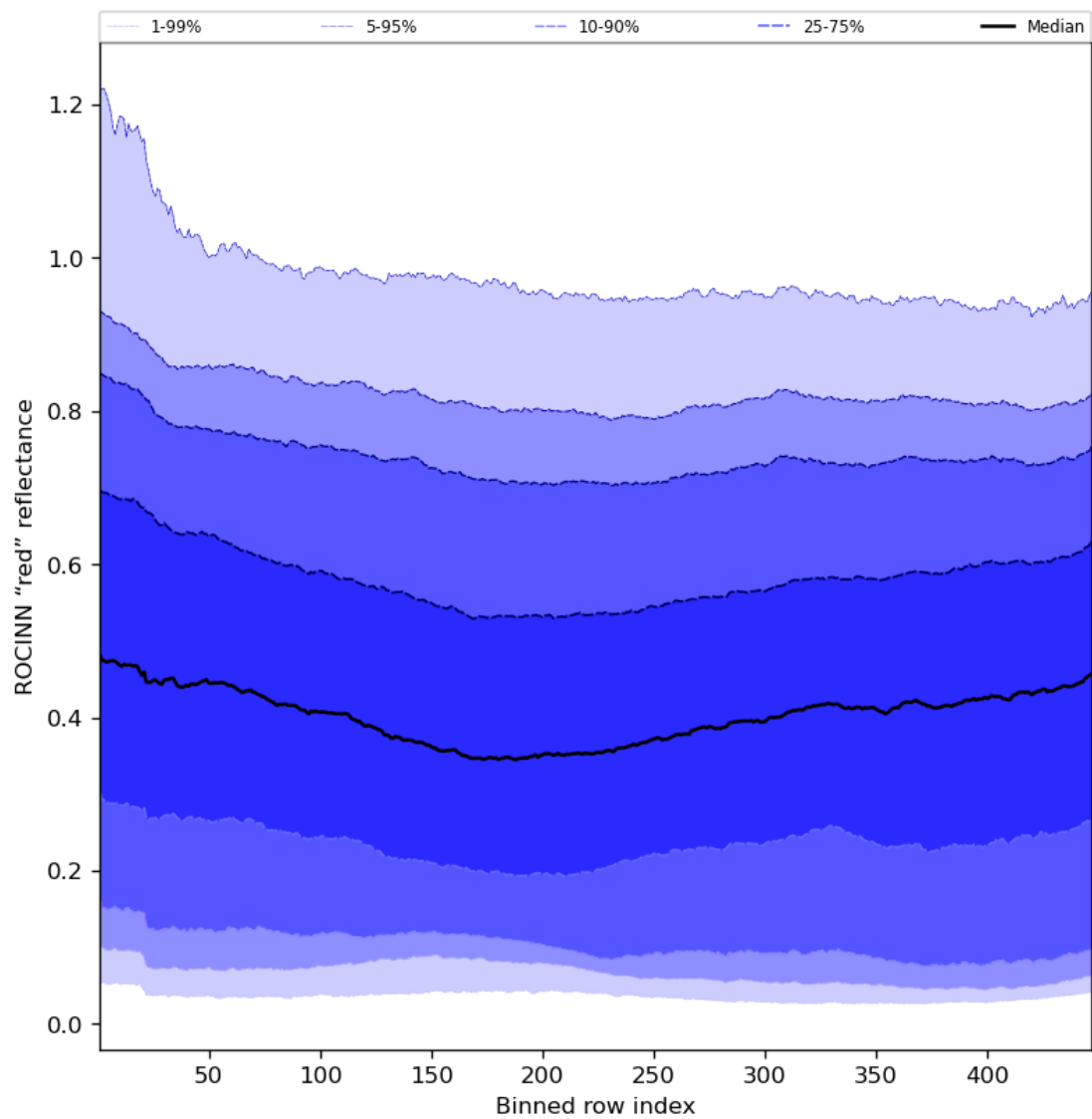
Figure 69: Along track statistics of “ROCINN “red” reflectance” for 2023-07-20 to 2023-07-22
