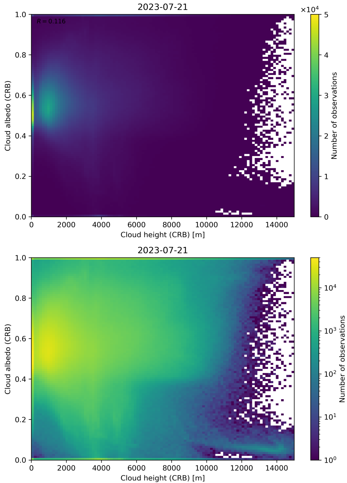
Figure 80: Scatter density plot of “Cloud height (CRB)” against “Cloud albedo (CRB)” for 2023-07-20 to 2023-07-22.
