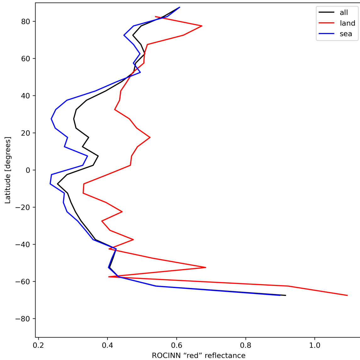
Figure 37: Zonal average of “ROCINN “red” reflectance” for 2023-07-20 to 2023-07-22.
