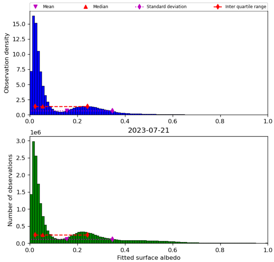
Figure 45: Histogram of “Fitted surface albedo” for 2023-07-20 to 2023-07-22
