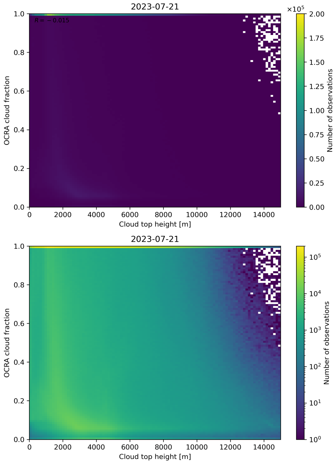
Figure 87: Scatter density plot of “Cloud top height” against “OCRA cloud fraction” for 2023-07-20 to 2023-07-22.
