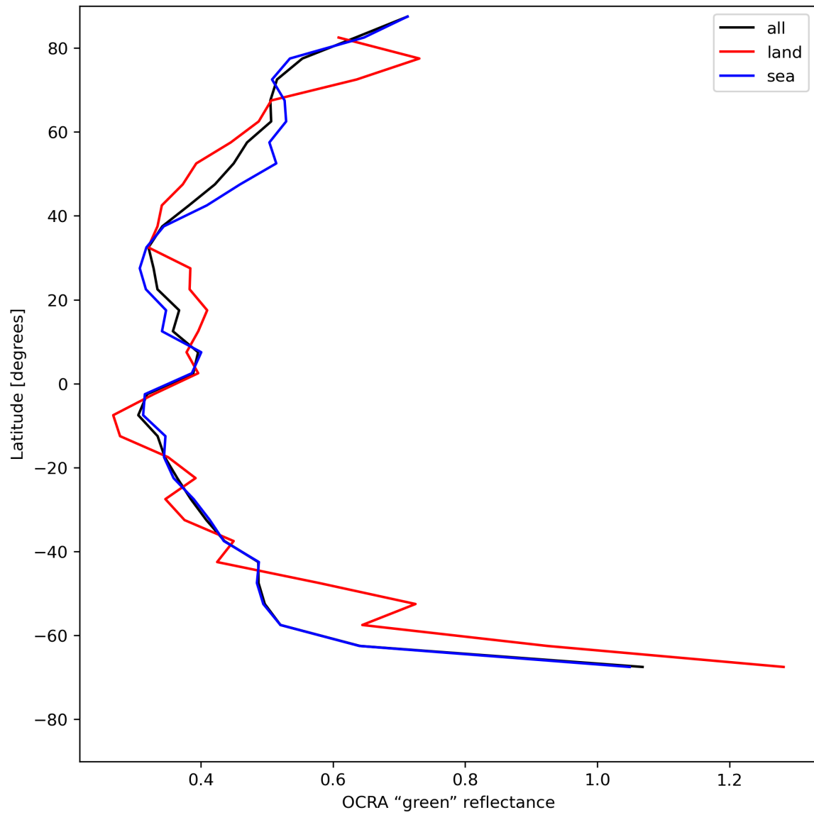
Figure 36: Zonal average of “OCRA “green” reflectance” for 2023-07-20 to 2023-07-22.
