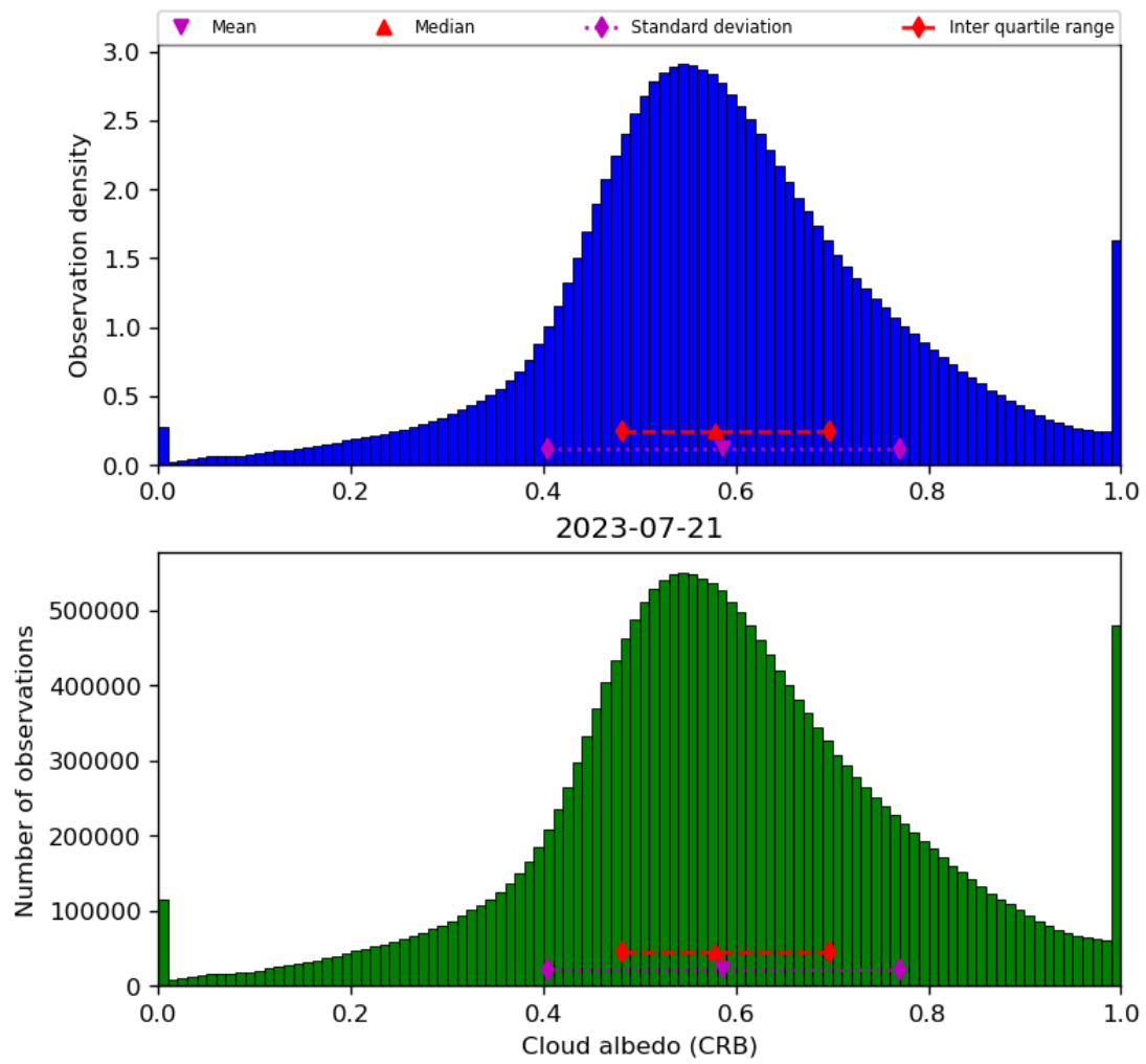
Figure 44: Histogram of “Cloud albedo (CRB)” for 2023-07-20 to 2023-07-22
