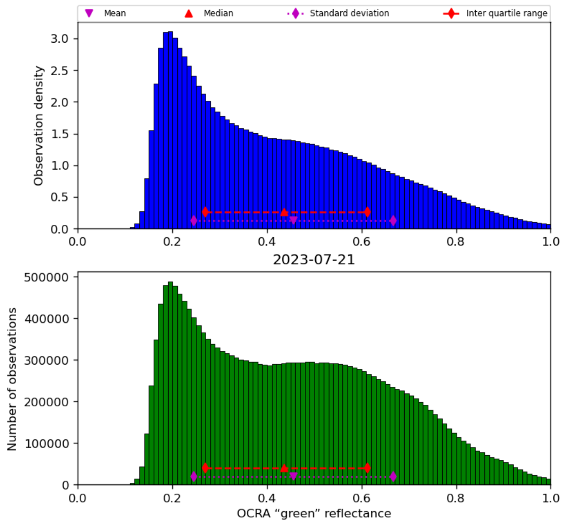
Figure 52: Histogram of “OCRA “green” reflectance” for 2023-07-20 to 2023-07-22
