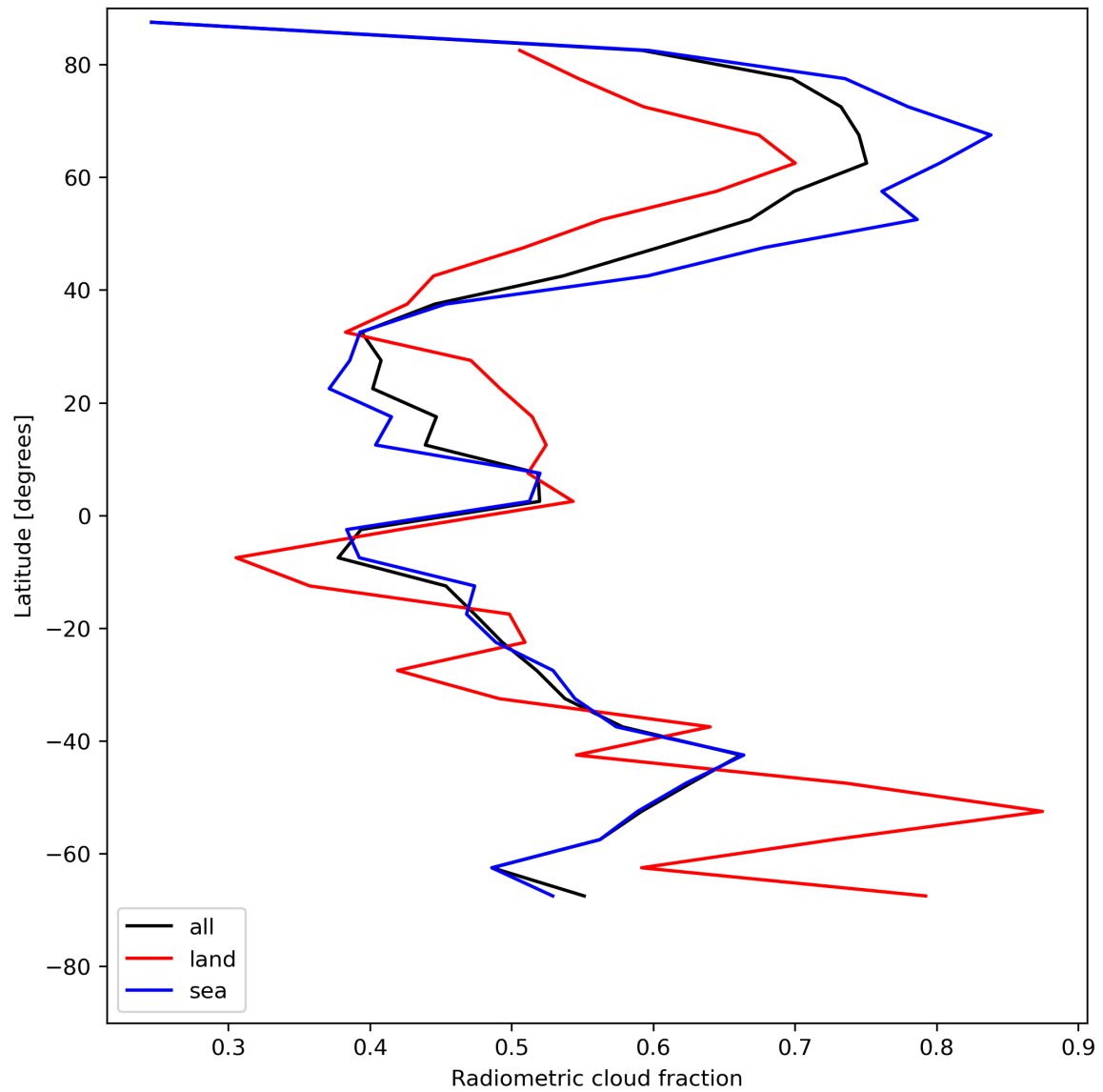
Figure 23: Zonal average of “Radiometric cloud fraction” for 2023-07-20 to 2023-07-22.
