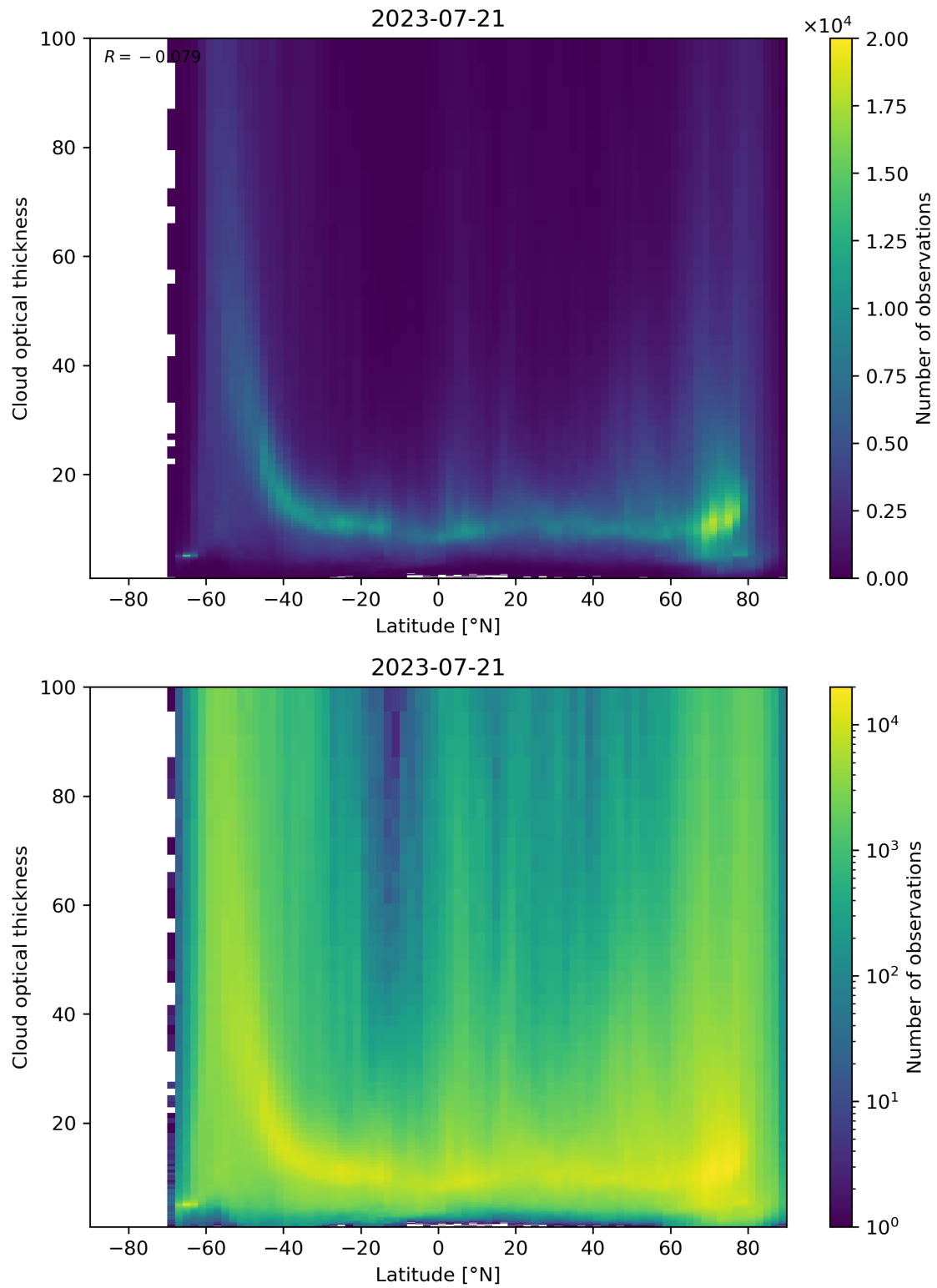
Figure 96: Scatter density plot of “Latitude” against “Cloud optical thickness” for 2023-07-20 to 2023-07-22.
