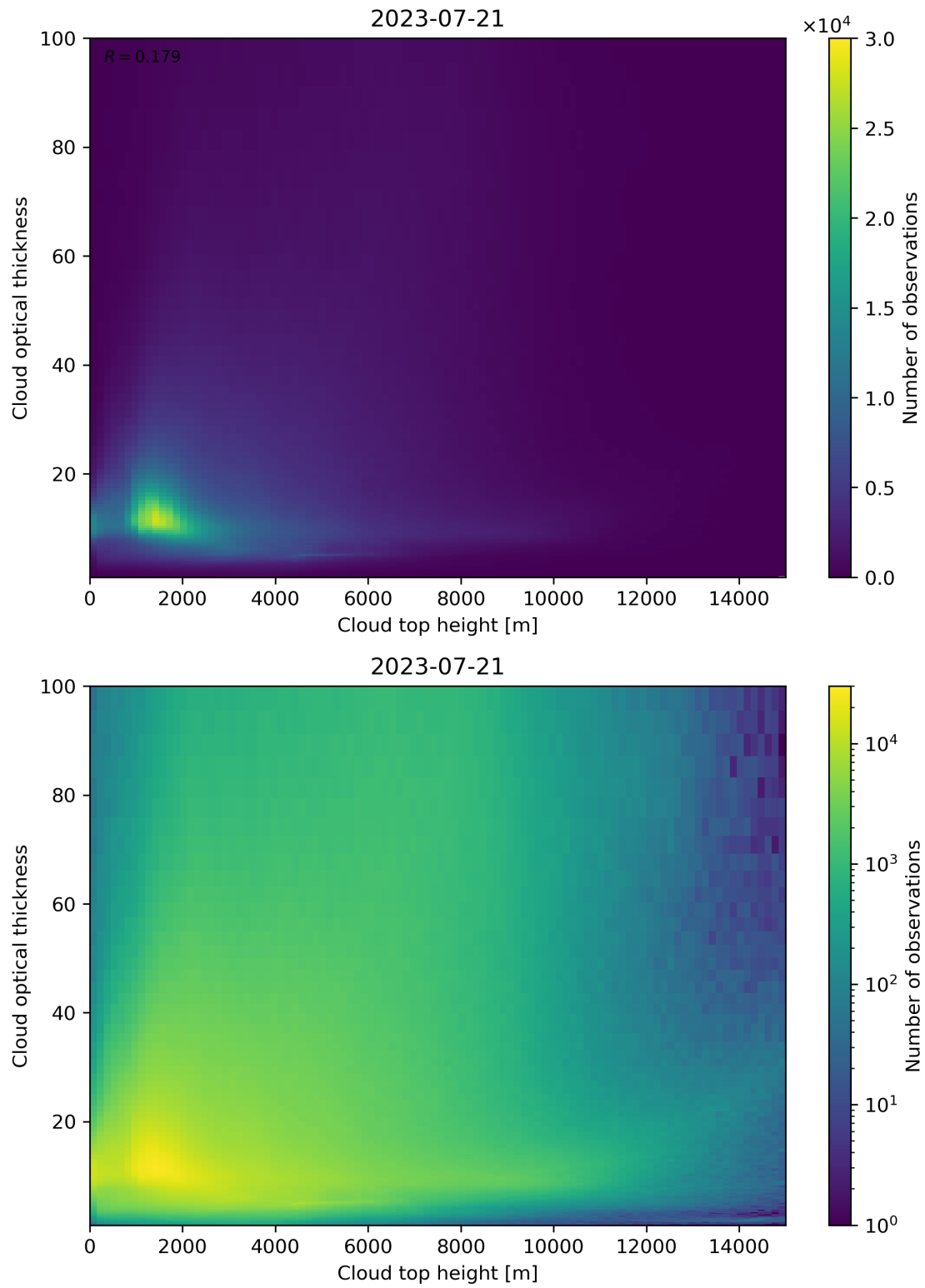
Figure 90: Scatter density plot of “Cloud top height” against “Cloud optical thickness” for 2023-07-20 to 2023-07-22.
