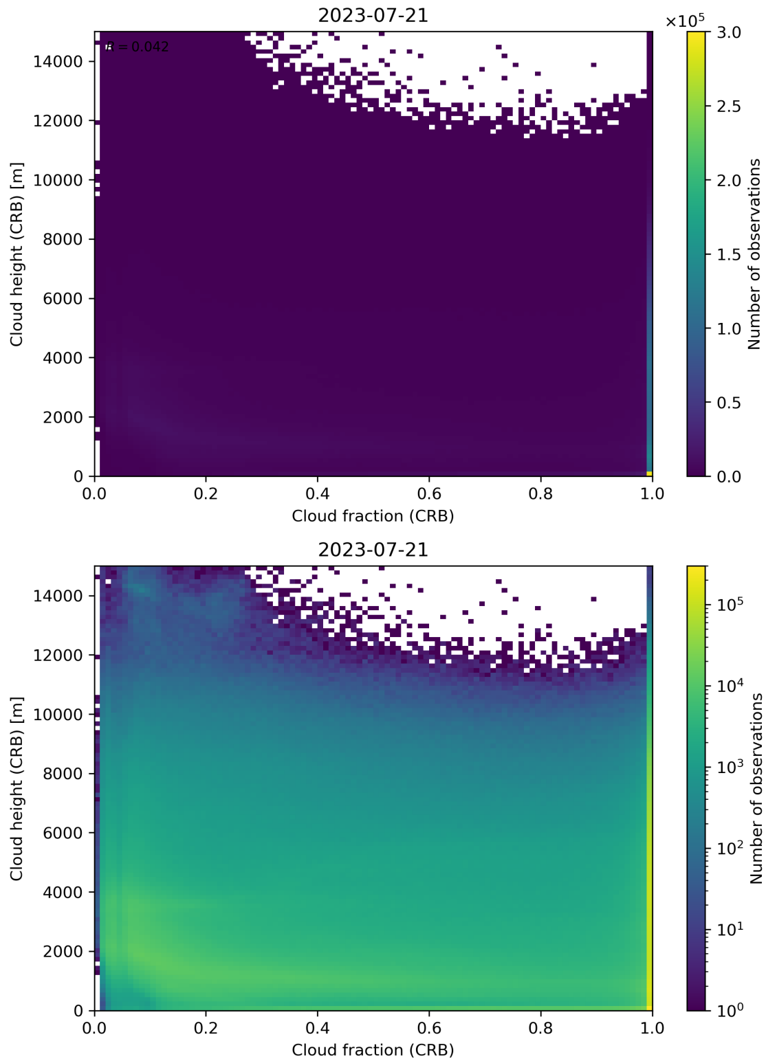
Figure 79: Scatter density plot of “Cloud fraction (CRB)” against “Cloud height (CRB)” for 2023-07-20 to 2023-07-22.
