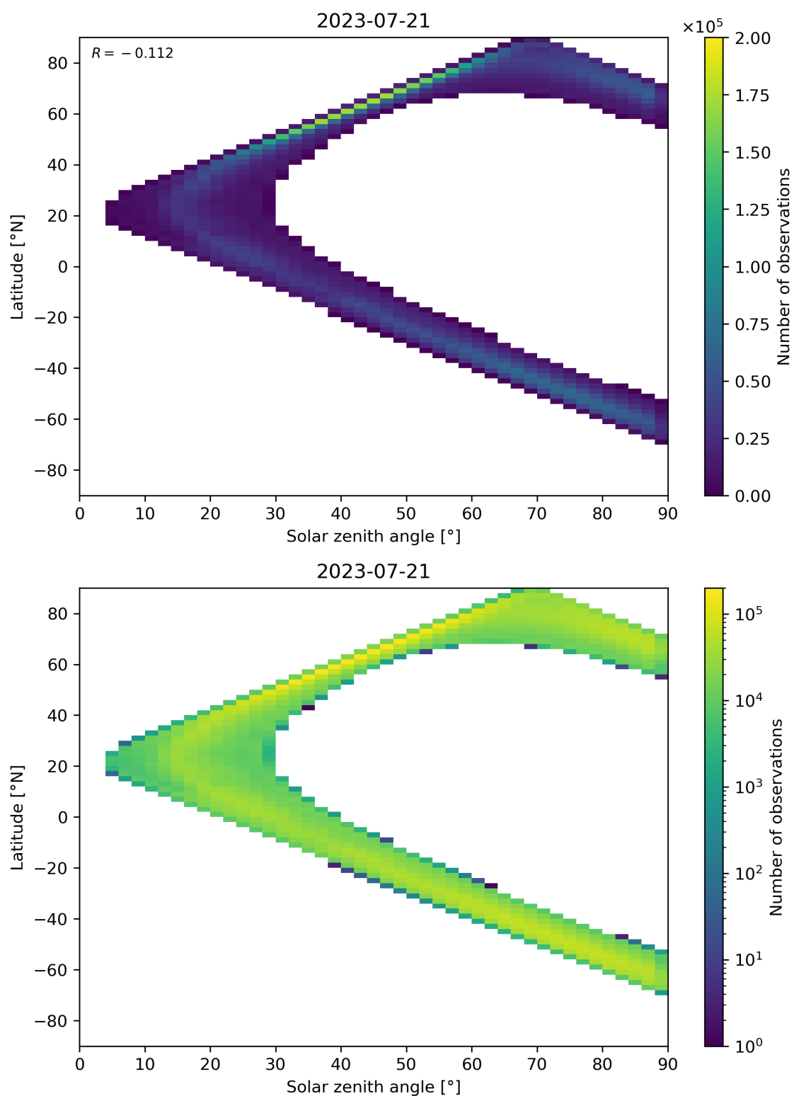
Figure 105: Scatter density plot of “Solar zenith angle” against “Latitude” for 2023-07-20 to 2023-07-22.
