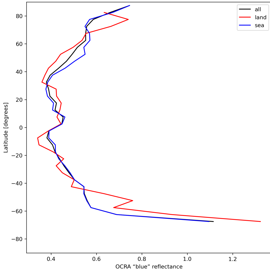
Figure 35: Zonal average of “OCRA “blue” reflectance” for 2023-07-20 to 2023-07-22.
