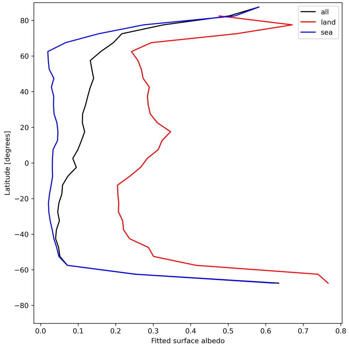
Figure 29: Zonal average of “Fitted surface albedo” for 2023-07-20 to 2023-07-22.
