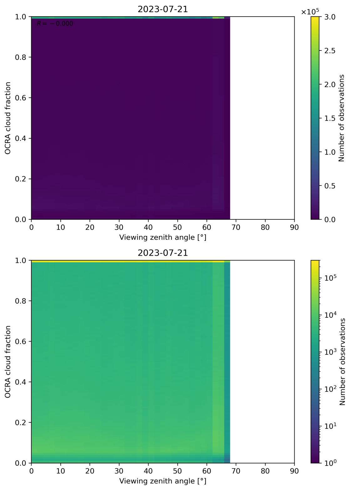
Figure 108: Scatter density plot of “Viewing zenith angle” against “OCRA cloud fraction” for 2023-07-20 to 2023-07-22.
