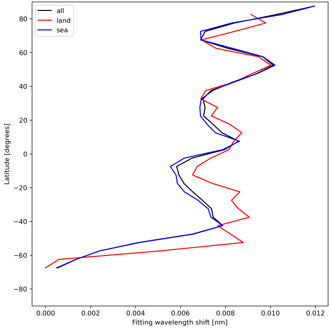
Figure 33: Zonal average of “Fitting wavelength shift” for 2023-07-20 to 2023-07-22.
