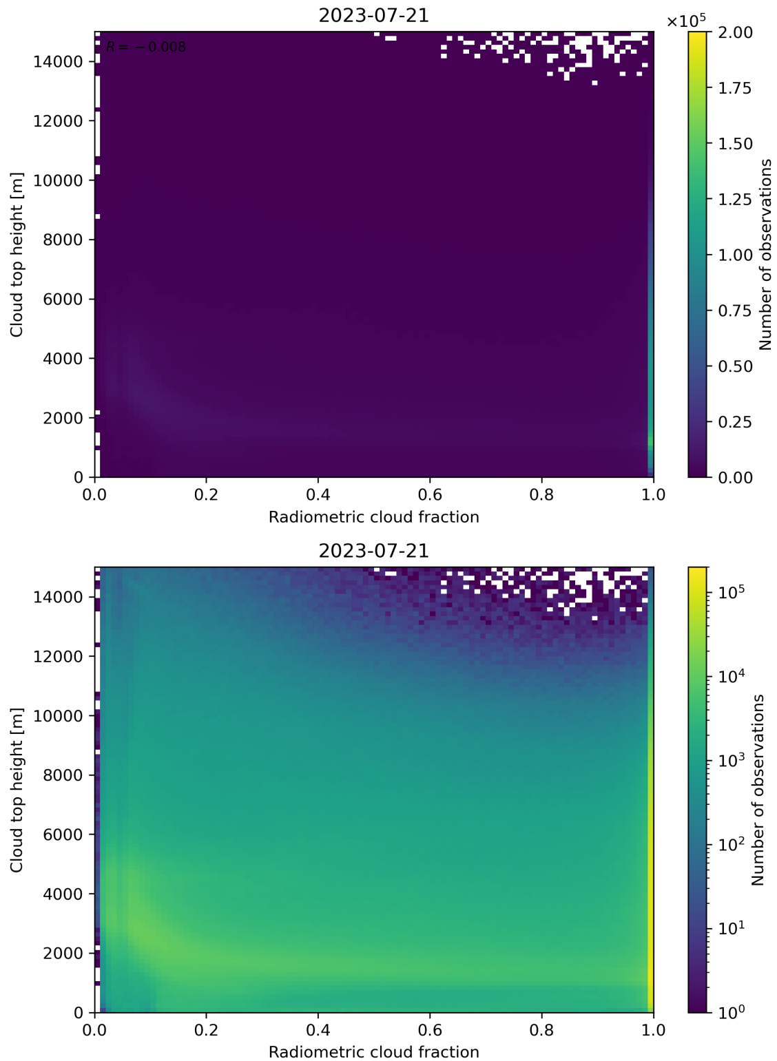
Figure 76: Scatter density plot of “Radiometric cloud fraction” against “Cloud top height” for 2023-07-20 to 2023-07-22.
