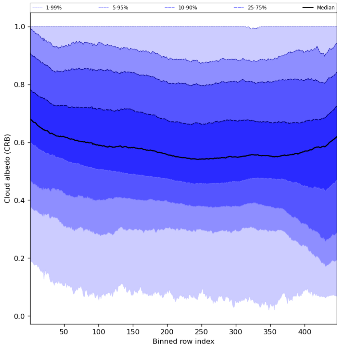
Figure 60: Along track statistics of “Cloud albedo (CRB)” for 2023-07-20 to 2023-07-22
