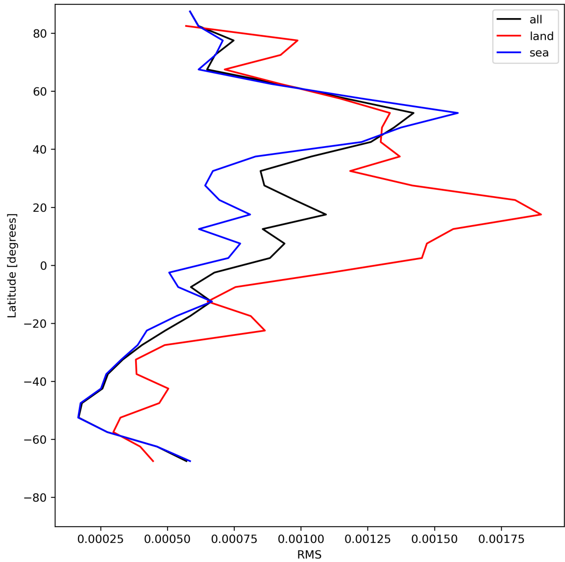
Figure 31: Zonal average of “RMS” for 2023-07-20 to 2023-07-22.
