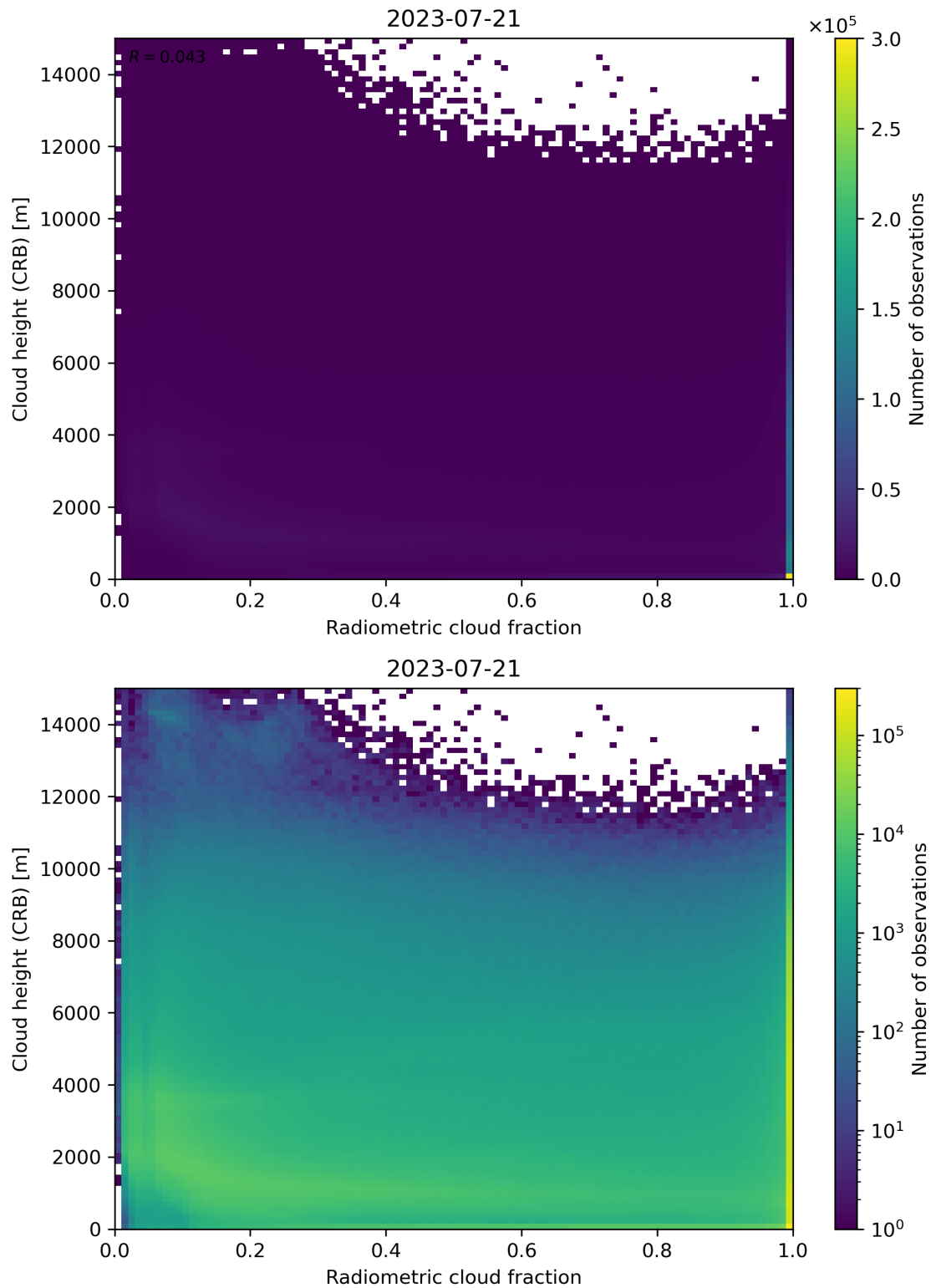
Figure 74: Scatter density plot of “Radiometric cloud fraction” against “Cloud height (CRB)” for 2023-07-20 to 2023-07-22.
