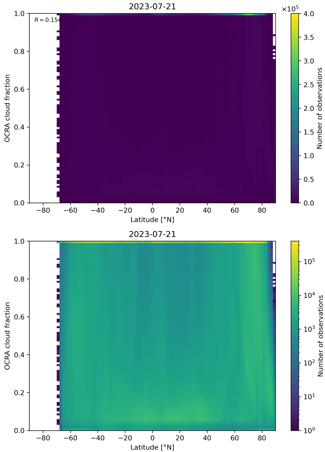
Figure 93: Scatter density plot of “Latitude” against “OCRA cloud fraction” for 2023-07-20 to 2023-07-22.
