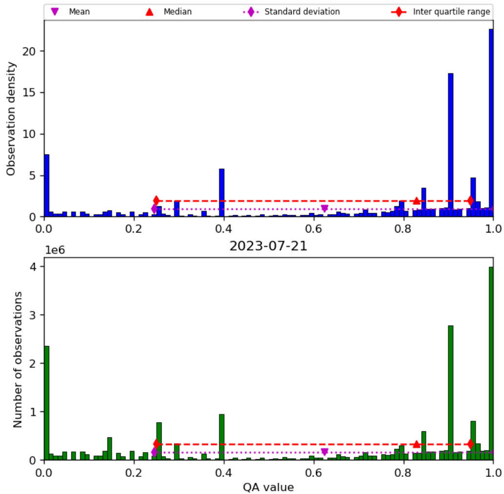
Figure 38: Histogram of “QA value” for 2023-07-20 to 2023-07-22
