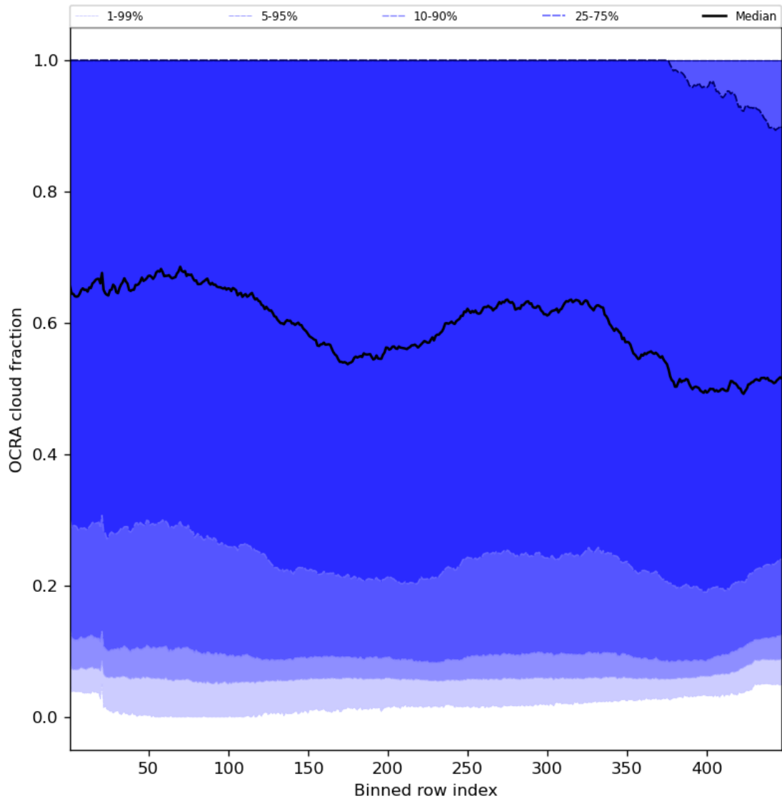
Figure 66: Along track statistics of “OCRA cloud fraction” for 2023-07-20 to 2023-07-22
