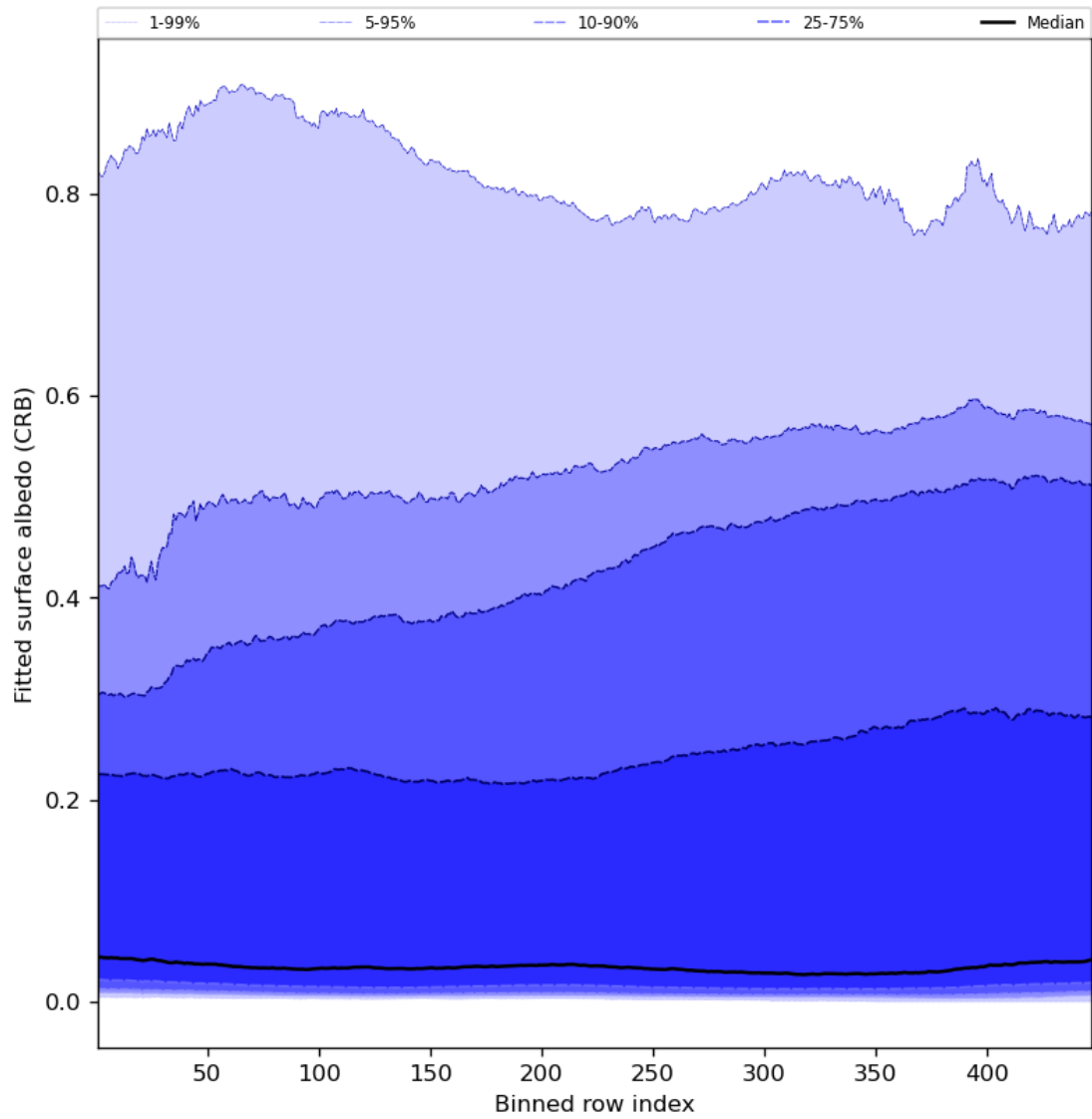
Figure 62: Along track statistics of “Fitted surface albedo (CRB)” for 2023-07-20 to 2023-07-22
