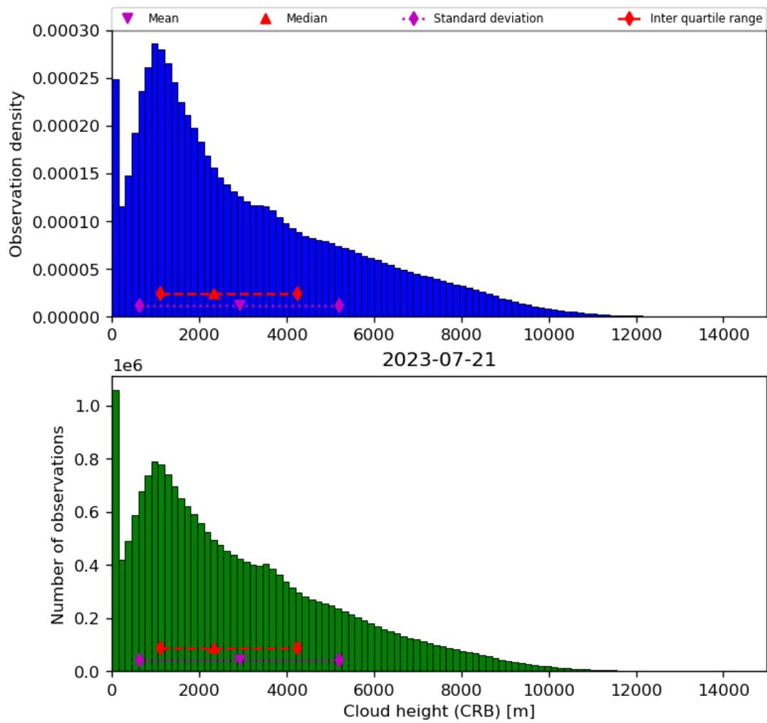
Figure 43: Histogram of “Cloud height (CRB)” for 2023-07-20 to 2023-07-22
