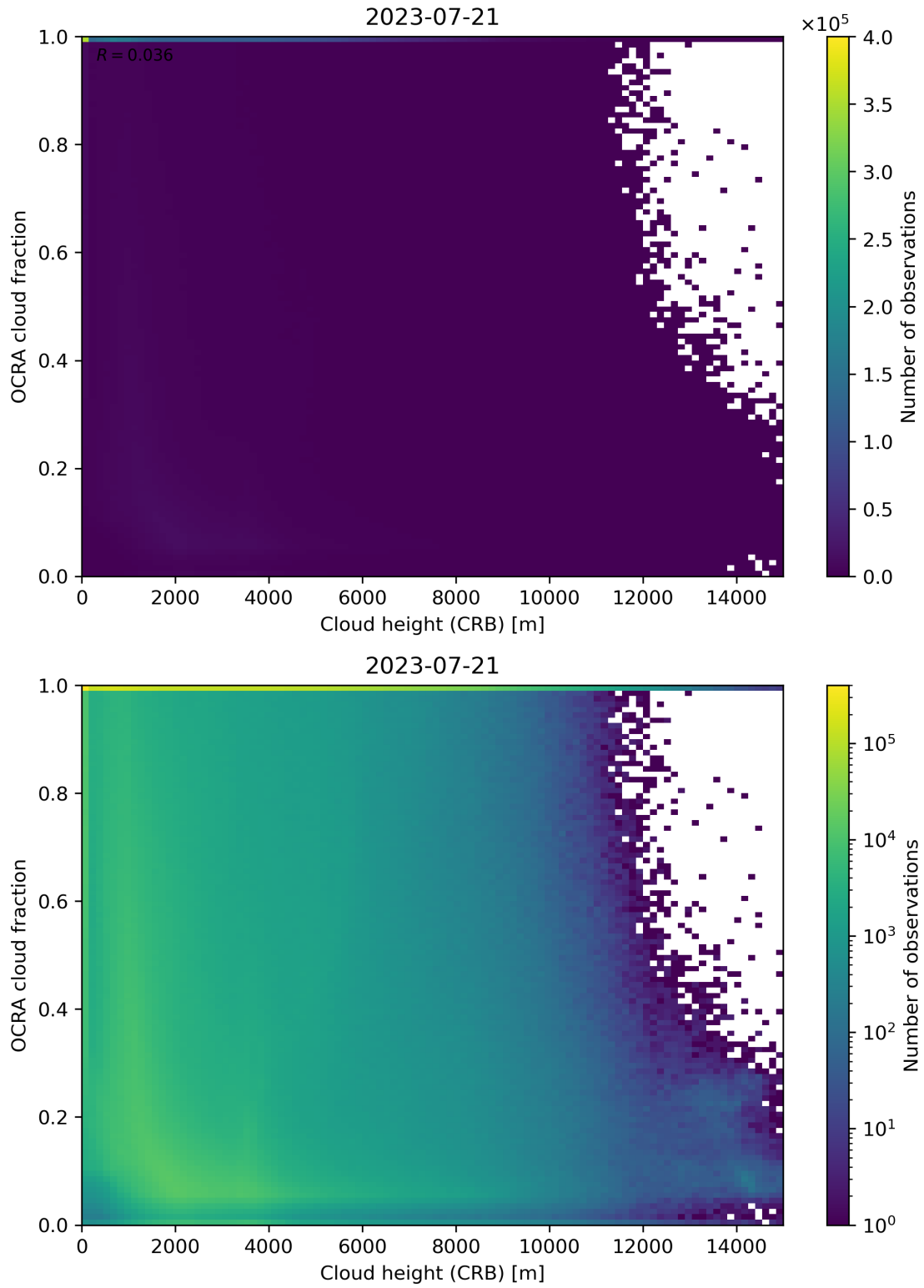
Figure 81: Scatter density plot of “Cloud height (CRB)” against “OCRA cloud fraction” for 2023-07-20 to 2023-07-22.
