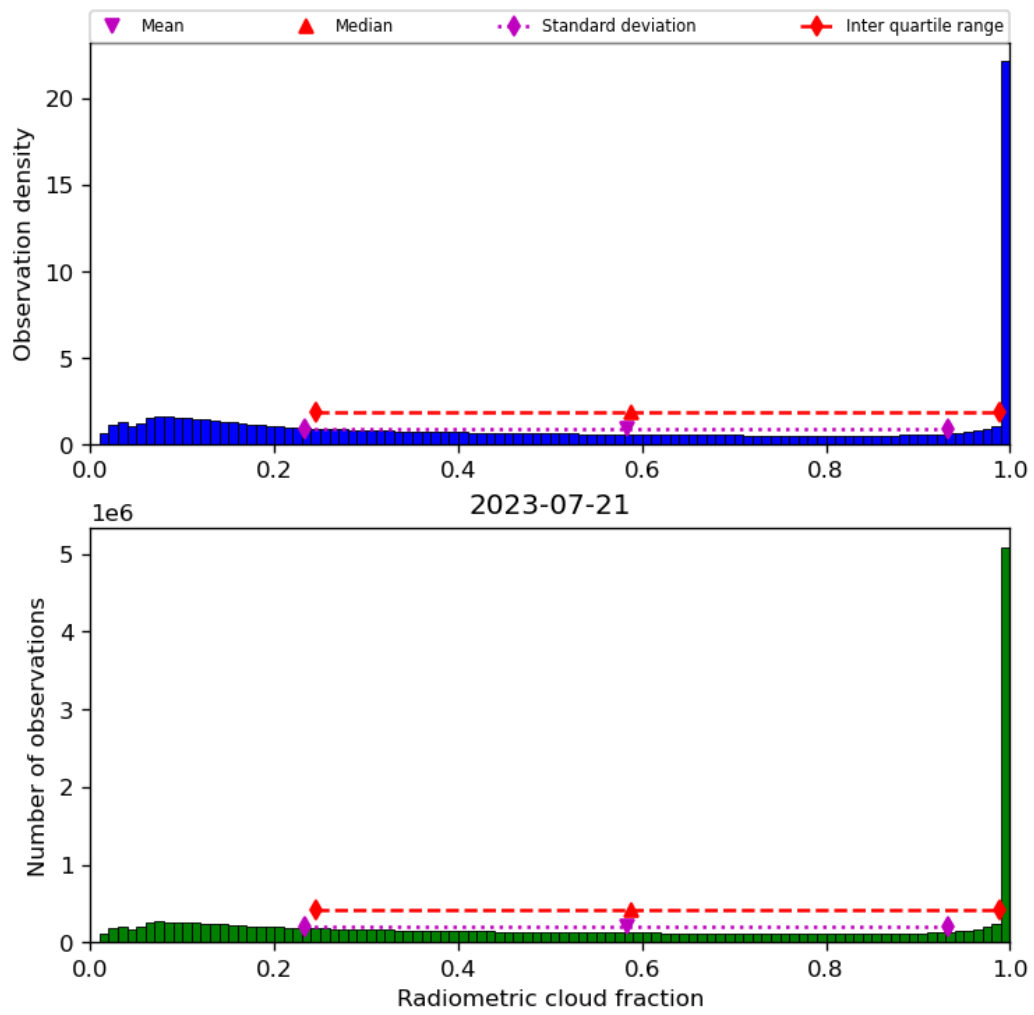
Figure 39: Histogram of “Radiometric cloud fraction” for 2023-07-20 to 2023-07-22
