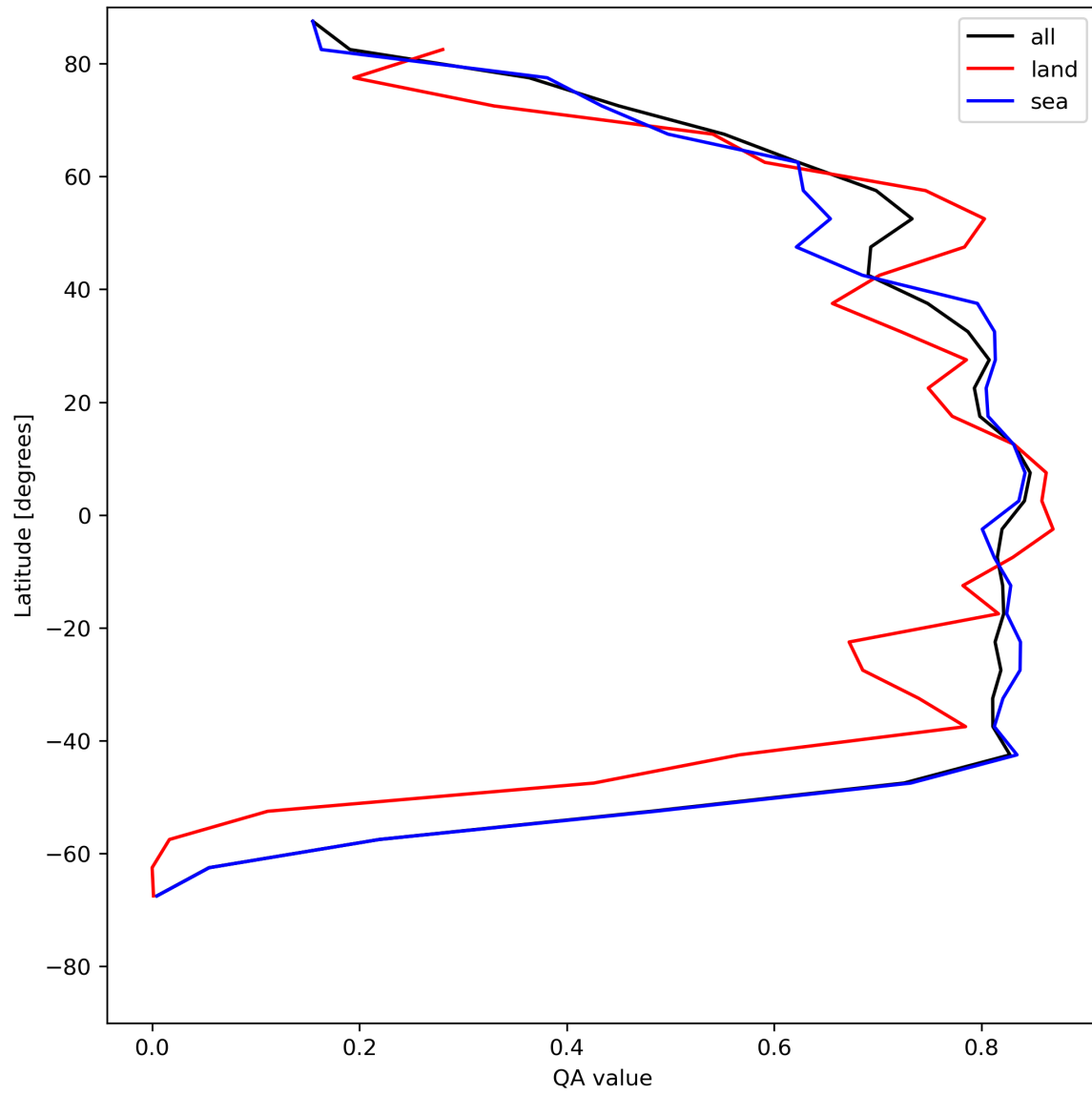
Figure 22: Zonal average of “QA value” for 2023-07-20 to 2023-07-22.
