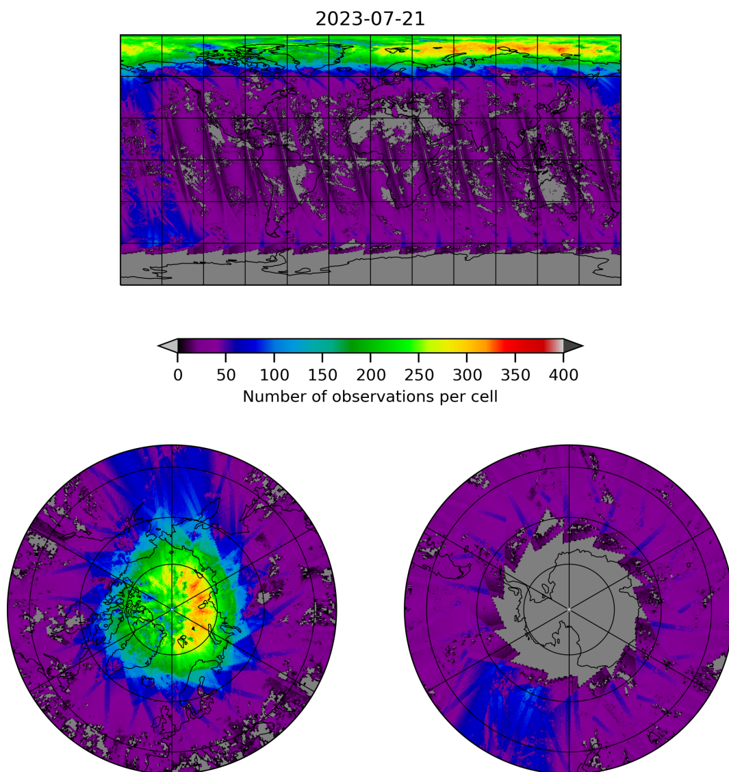
Figure 21: Map of the number of observations for 2023-07-20 to 2023-07-22
