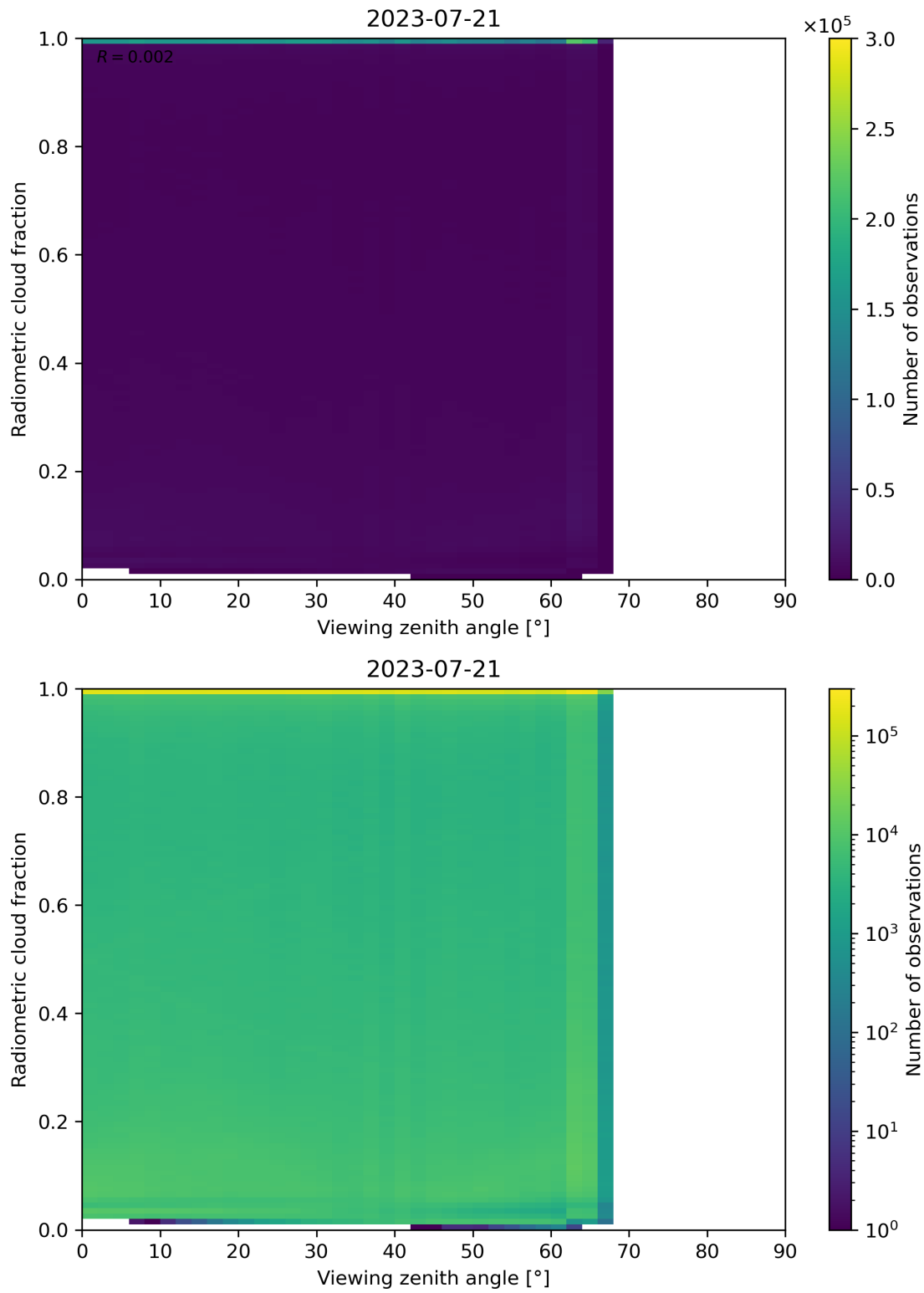
Figure 107: Scatter density plot of “Viewing zenith angle” against “Radiometric cloud fraction” for 2023-07-20 to 2023-07-22.
