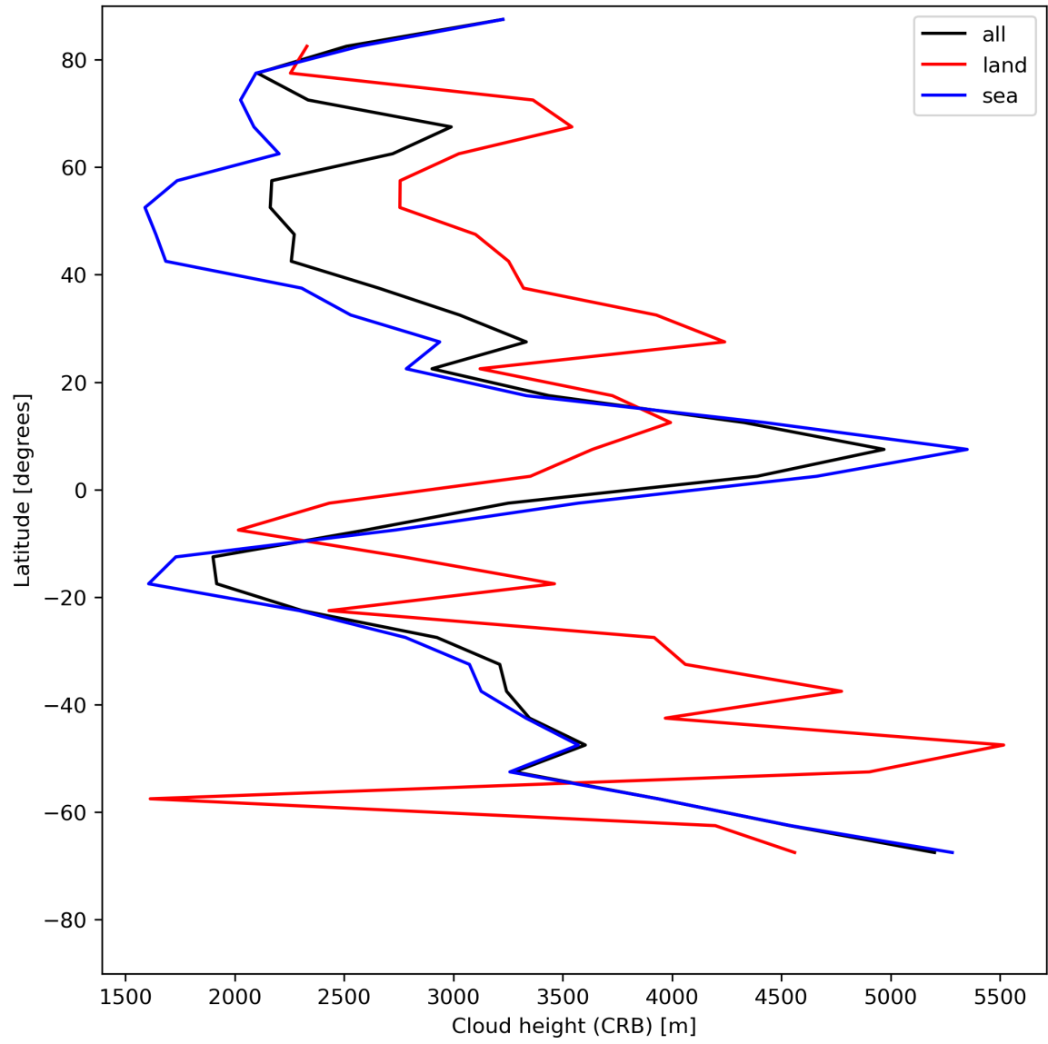
Figure 27: Zonal average of “Cloud height (CRB)” for 2023-07-20 to 2023-07-22.
