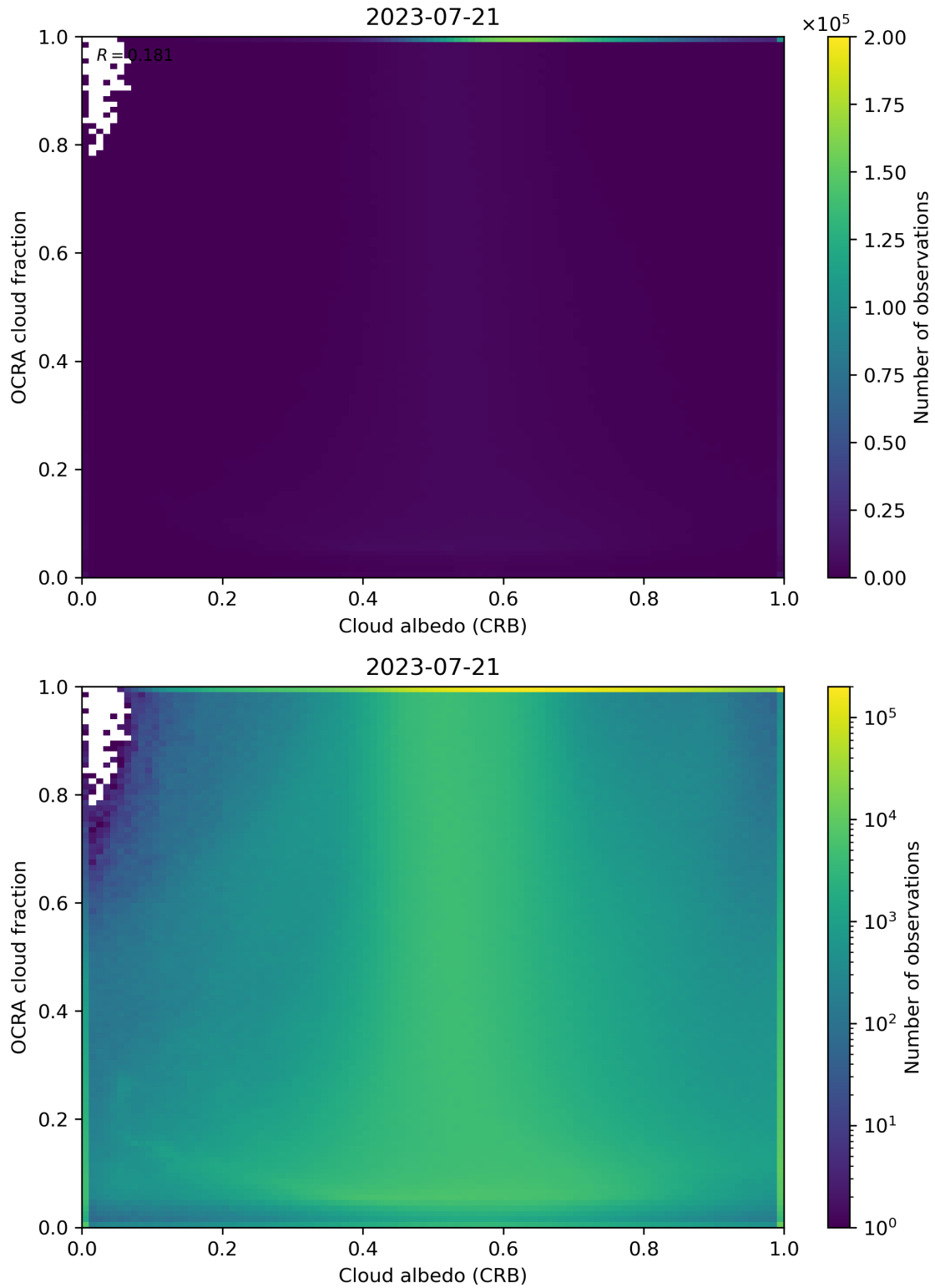
Figure 70: Scatter density plot of “Cloud albedo (CRB)” against “OCRA cloud fraction” for 2023-07-20 to 2023-07-22.
