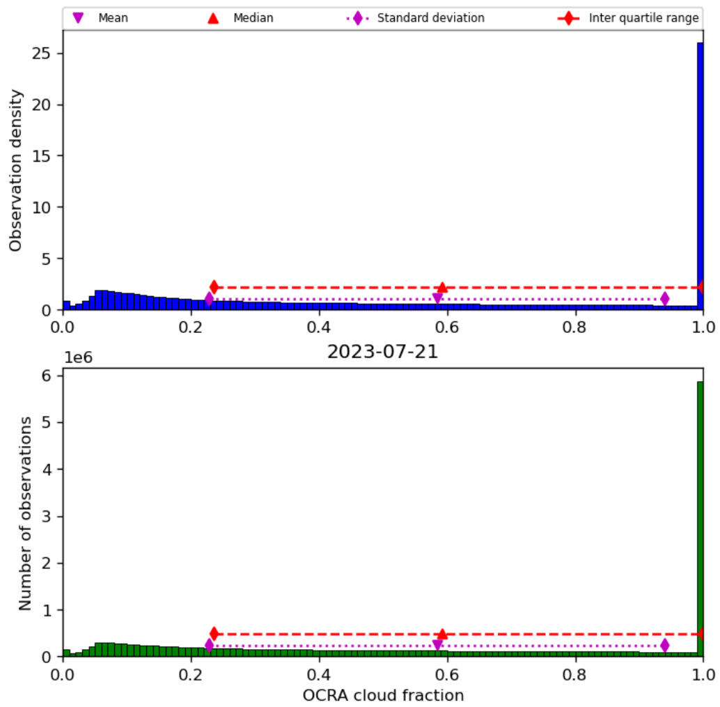
Figure 50: Histogram of “OCRA cloud fraction” for 2023-07-20 to 2023-07-22
