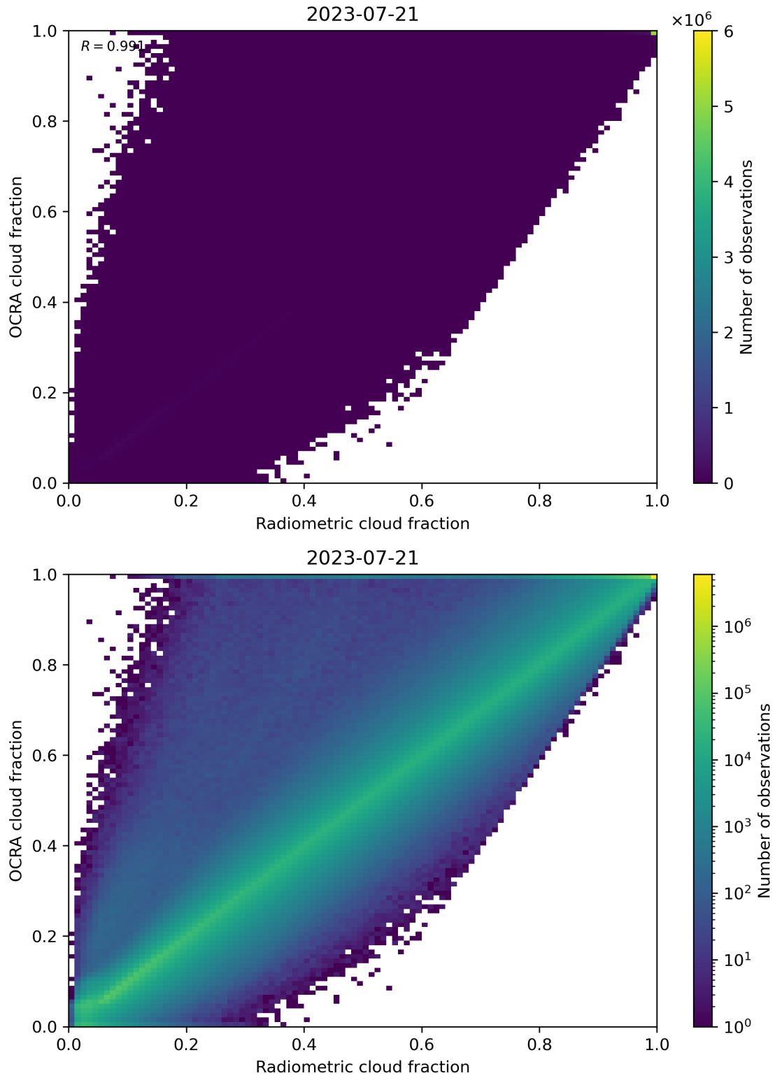
Figure 72: Scatter density plot of “Radiometric cloud fraction” against “OCRA cloud fraction” for 2023-07-20 to 2023-07-22.
