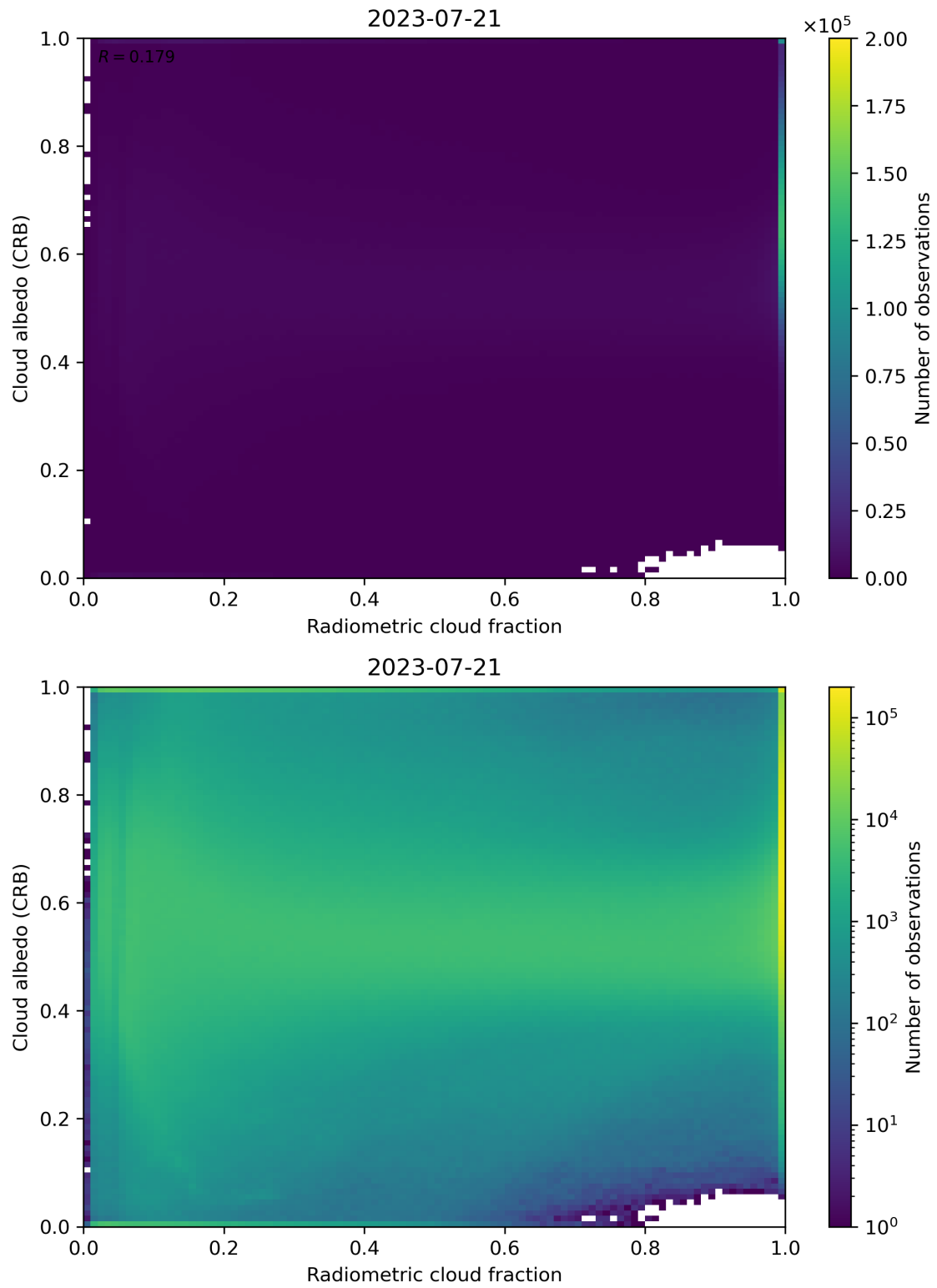
Figure 71: Scatter density plot of “Radiometric cloud fraction” against “Cloud albedo (CRB)” for 2023-07-20 to 2023-07-22.
