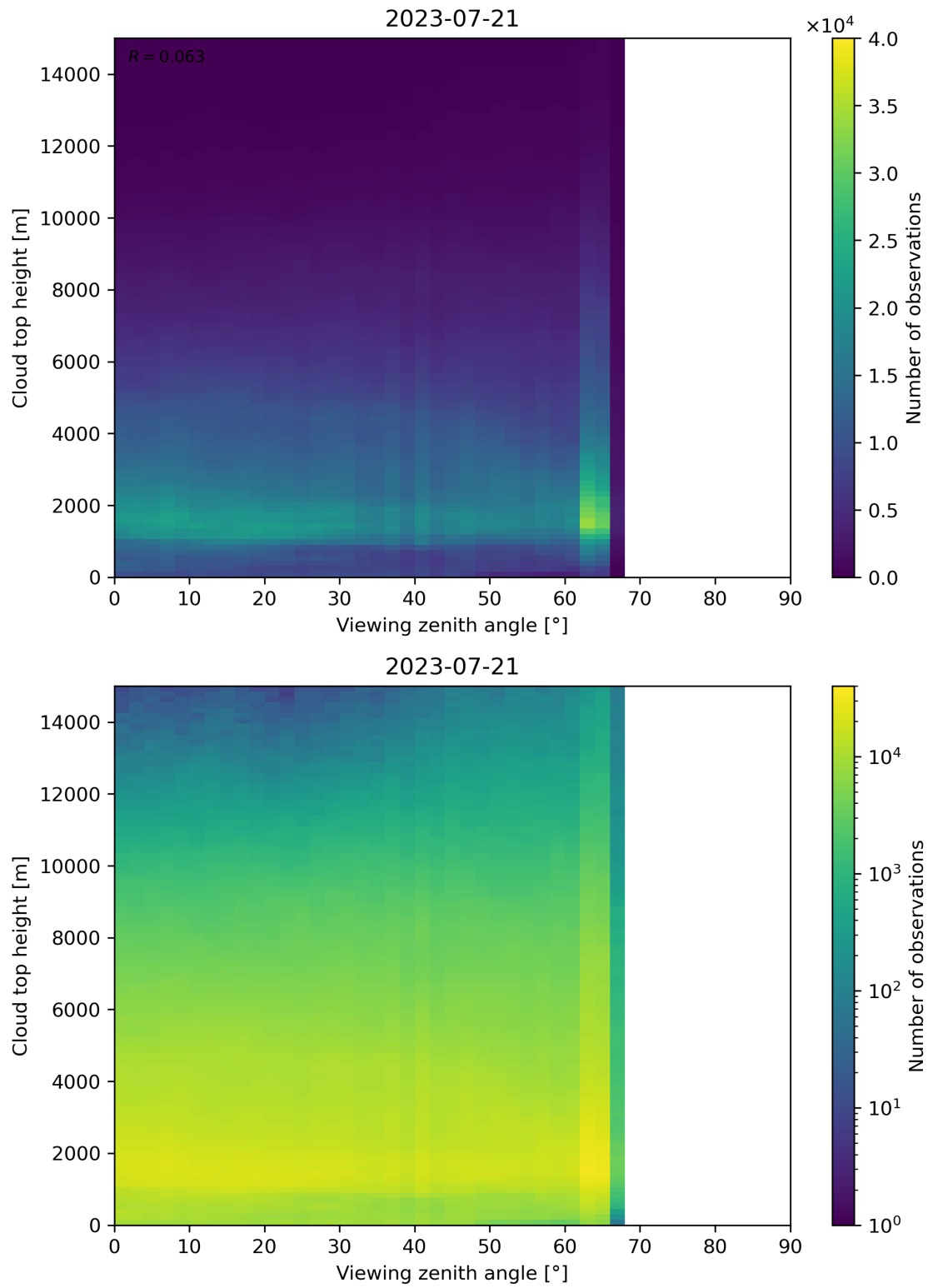
Figure 112: Scatter density plot of “Viewing zenith angle” against “Cloud top height” for 2023-07-20 to 2023-07-22.
