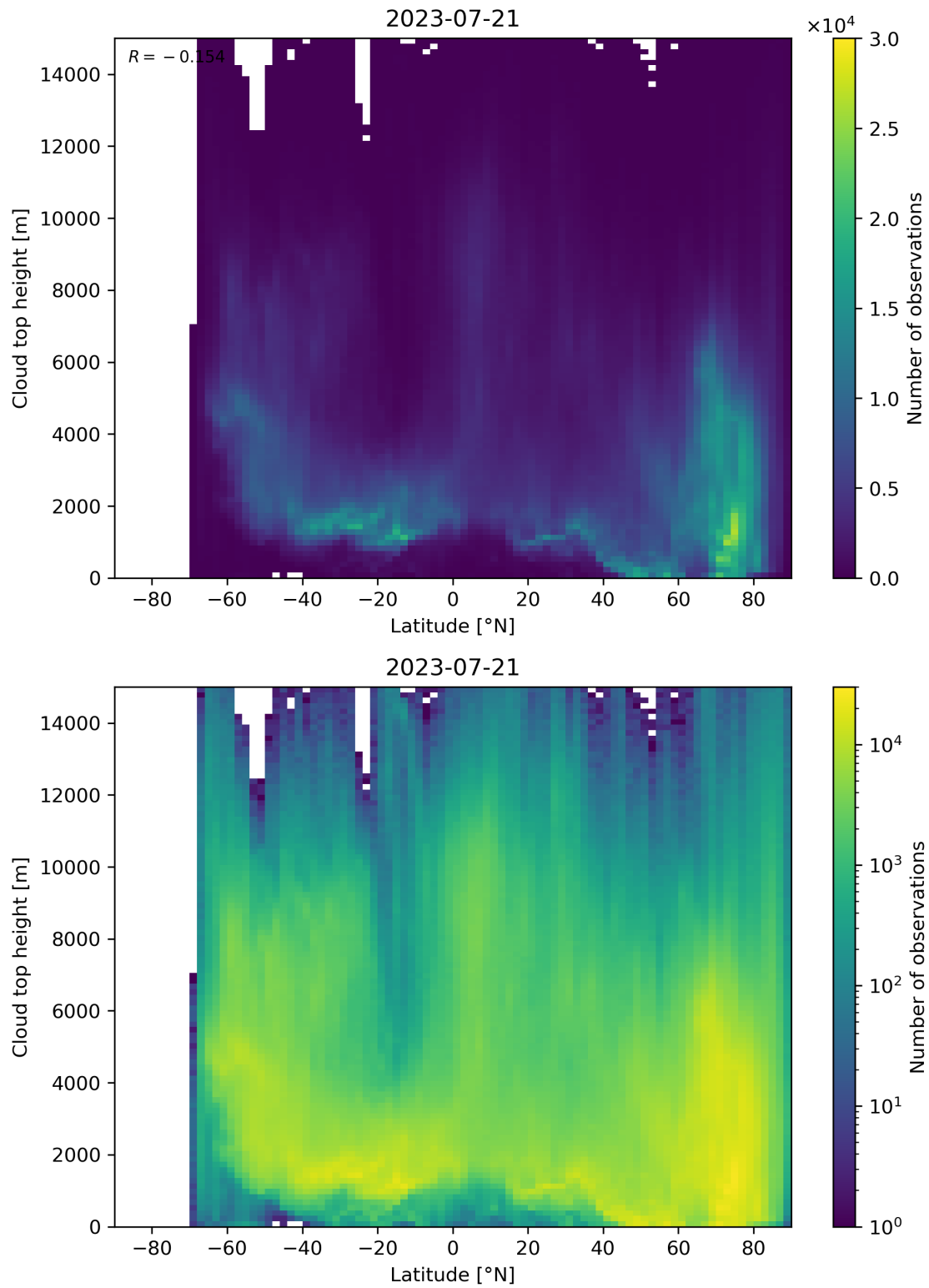
Figure 97: Scatter density plot of “Latitude” against “Cloud top height” for 2023-07-20 to 2023-07-22.
