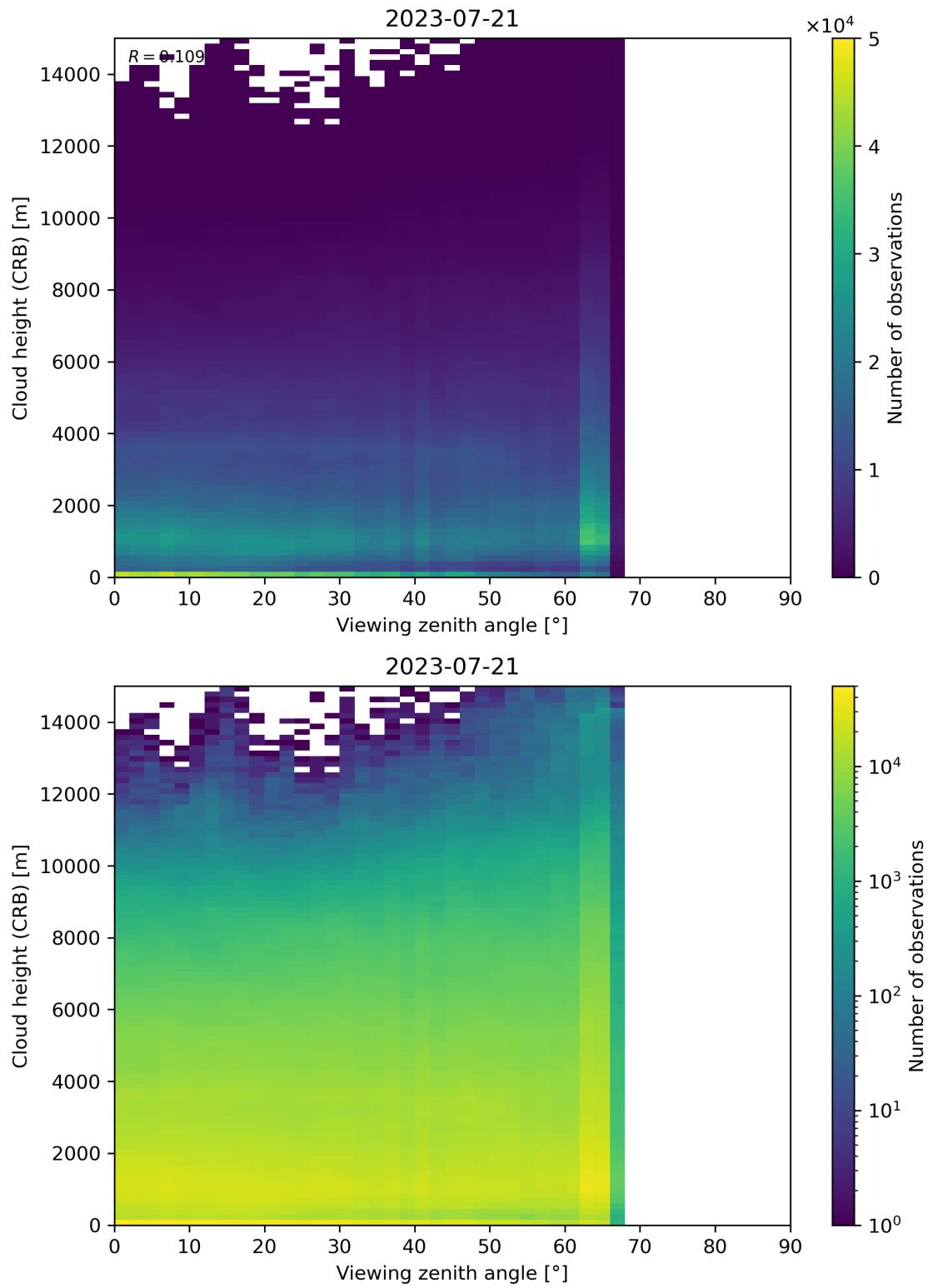
Figure 110: Scatter density plot of “Viewing zenith angle” against “Cloud height (CRB)” for 2023-07-20 to 2023-07-22.
