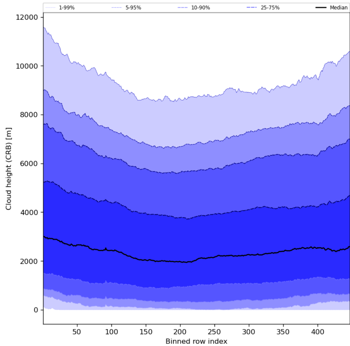
Figure 59: Along track statistics of “Cloud height (CRB)” for 2023-07-20 to 2023-07-22
