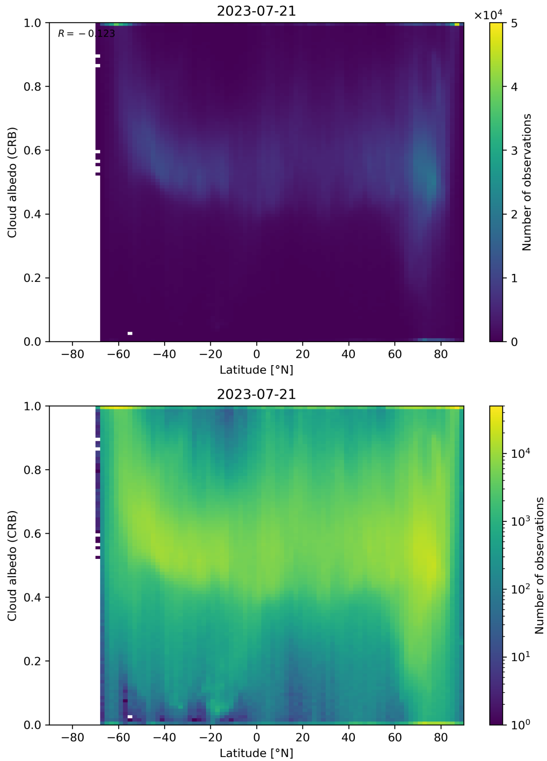
Figure 91: Scatter density plot of “Latitude” against “Cloud albedo (CRB)” for 2023-07-20 to 2023-07-22.
