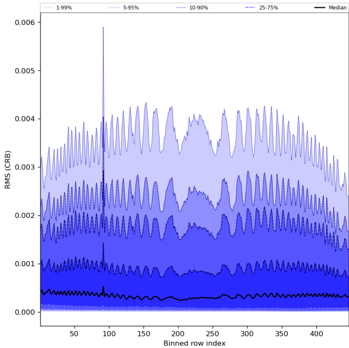
Figure 64: Along track statistics of “RMS (CRB)” for 2023-07-20 to 2023-07-22
