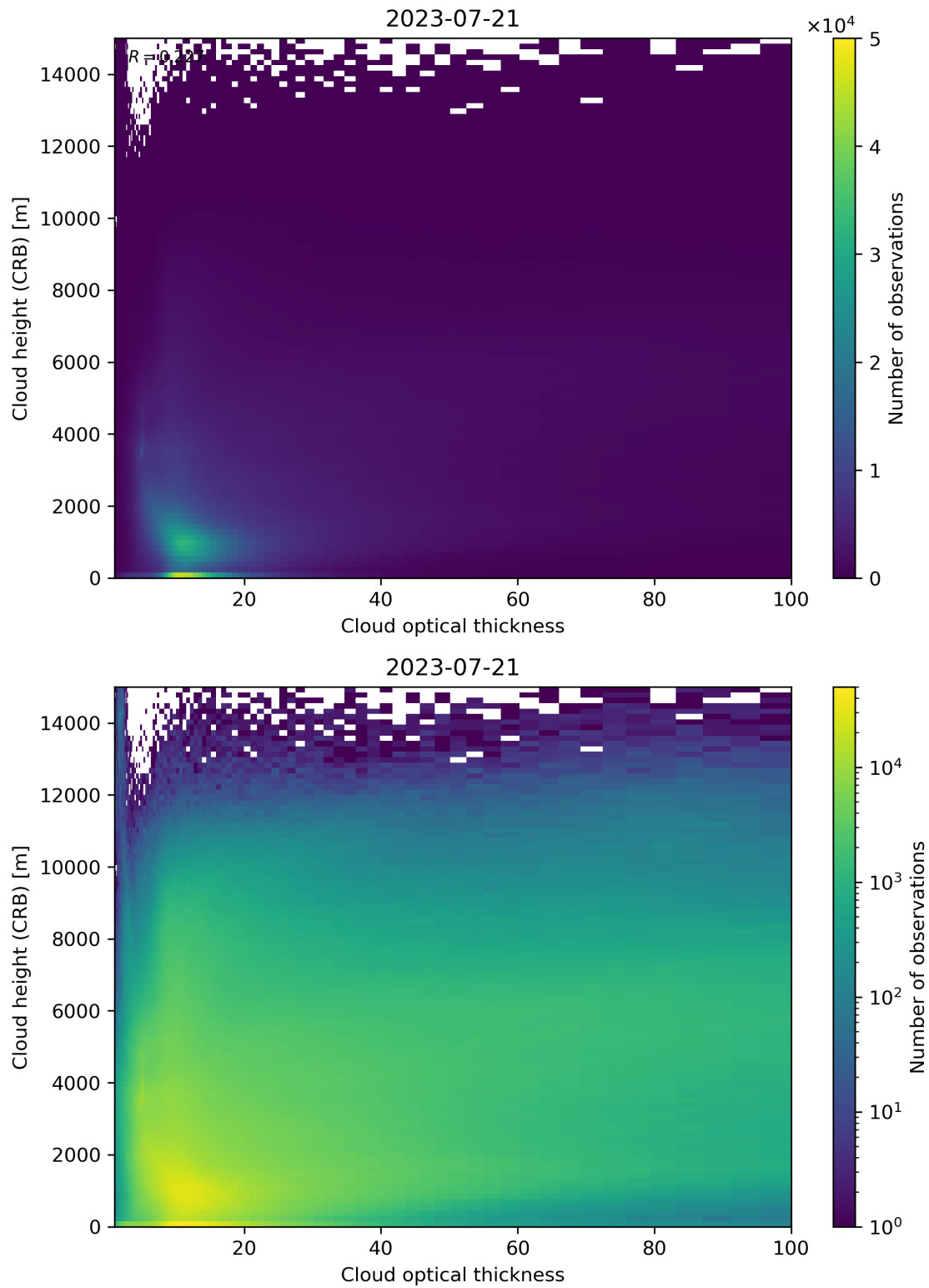
Figure 85: Scatter density plot of “Cloud optical thickness” against “Cloud height (CRB)” for 2023-07-20 to 2023-07-22.
