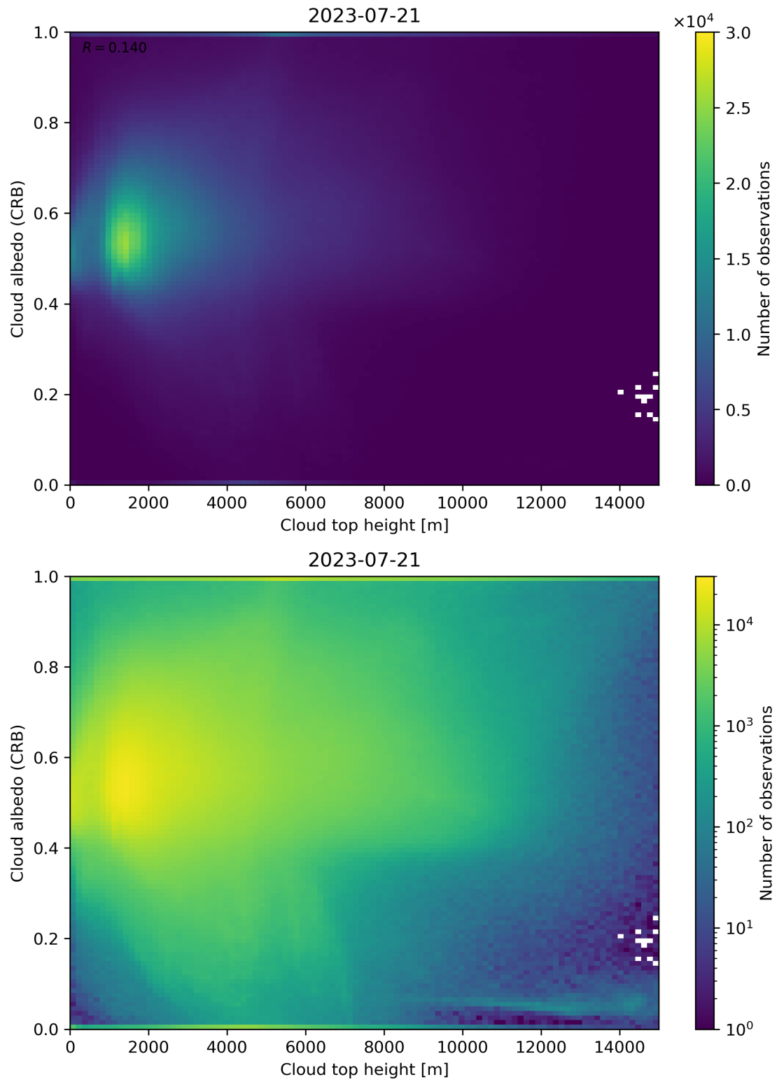
Figure 86: Scatter density plot of “Cloud top height” against “Cloud albedo (CRB)” for 2023-07-20 to 2023-07-22.
