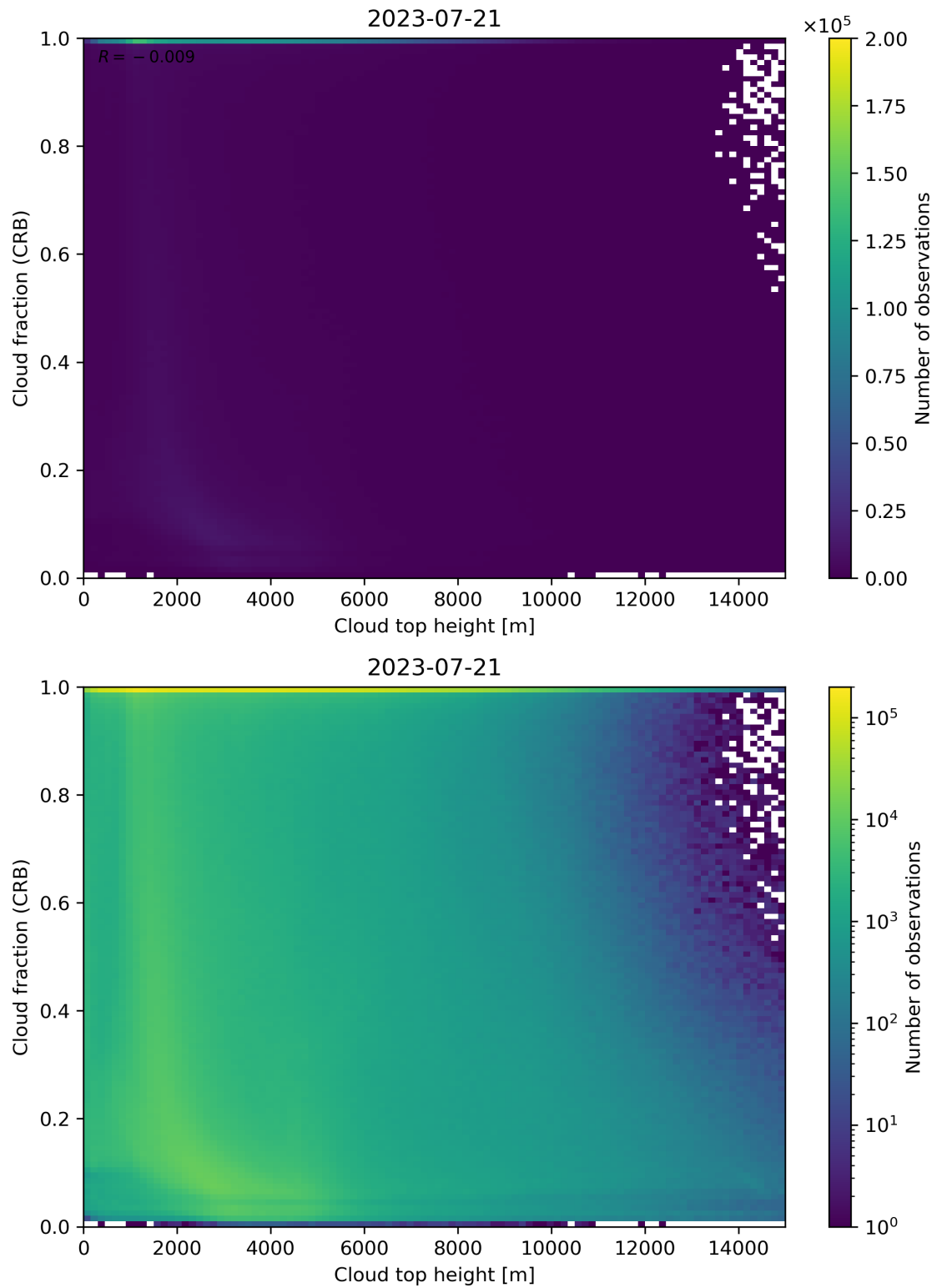
Figure 88: Scatter density plot of “Cloud top height” against “Cloud fraction (CRB)” for 2023-07-20 to 2023-07-22.
