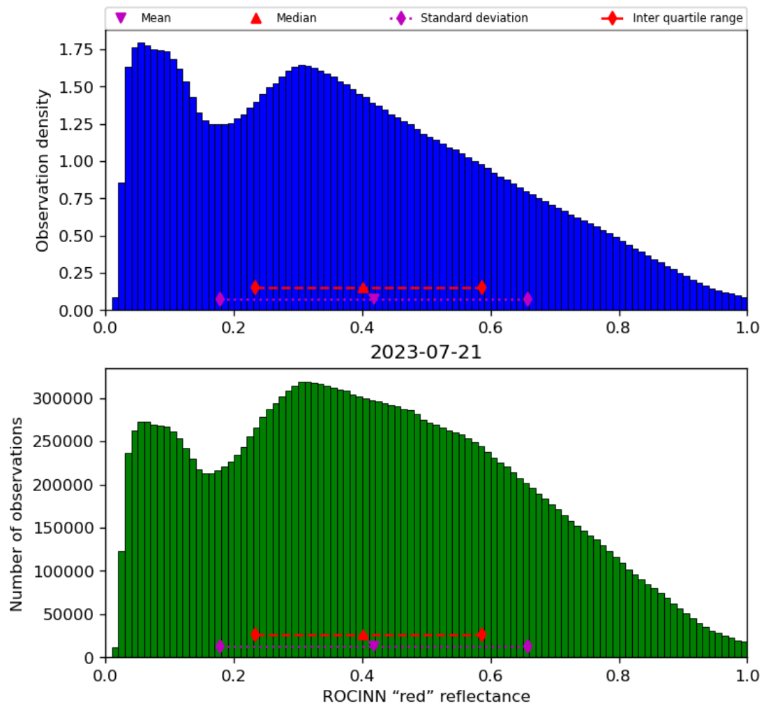
Figure 53: Histogram of “ROCINN “red” reflectance” for 2023-07-20 to 2023-07-22
