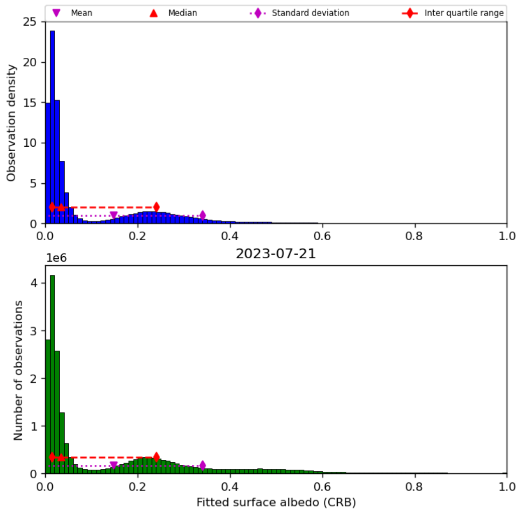
Figure 46: Histogram of “Fitted surface albedo (CRB)” for 2023-07-20 to 2023-07-22
