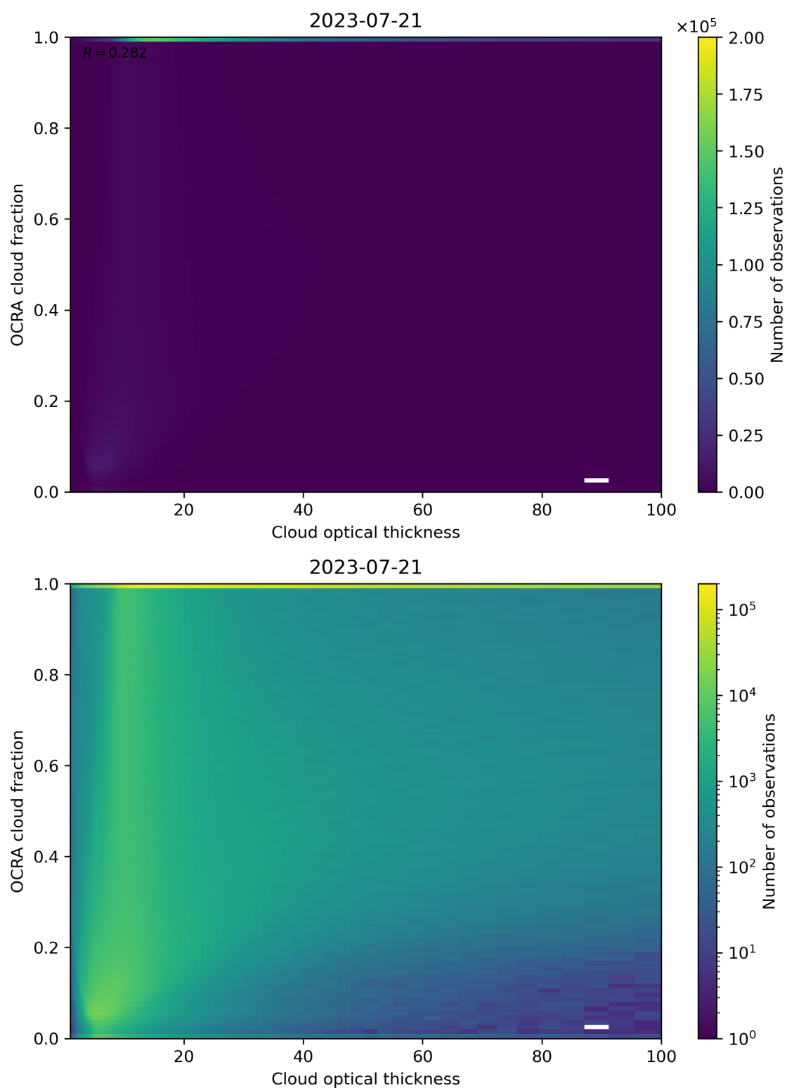
Figure 83: Scatter density plot of “Cloud optical thickness” against “OCRA cloud fraction” for 2023-07-20 to 2023-07-22.
