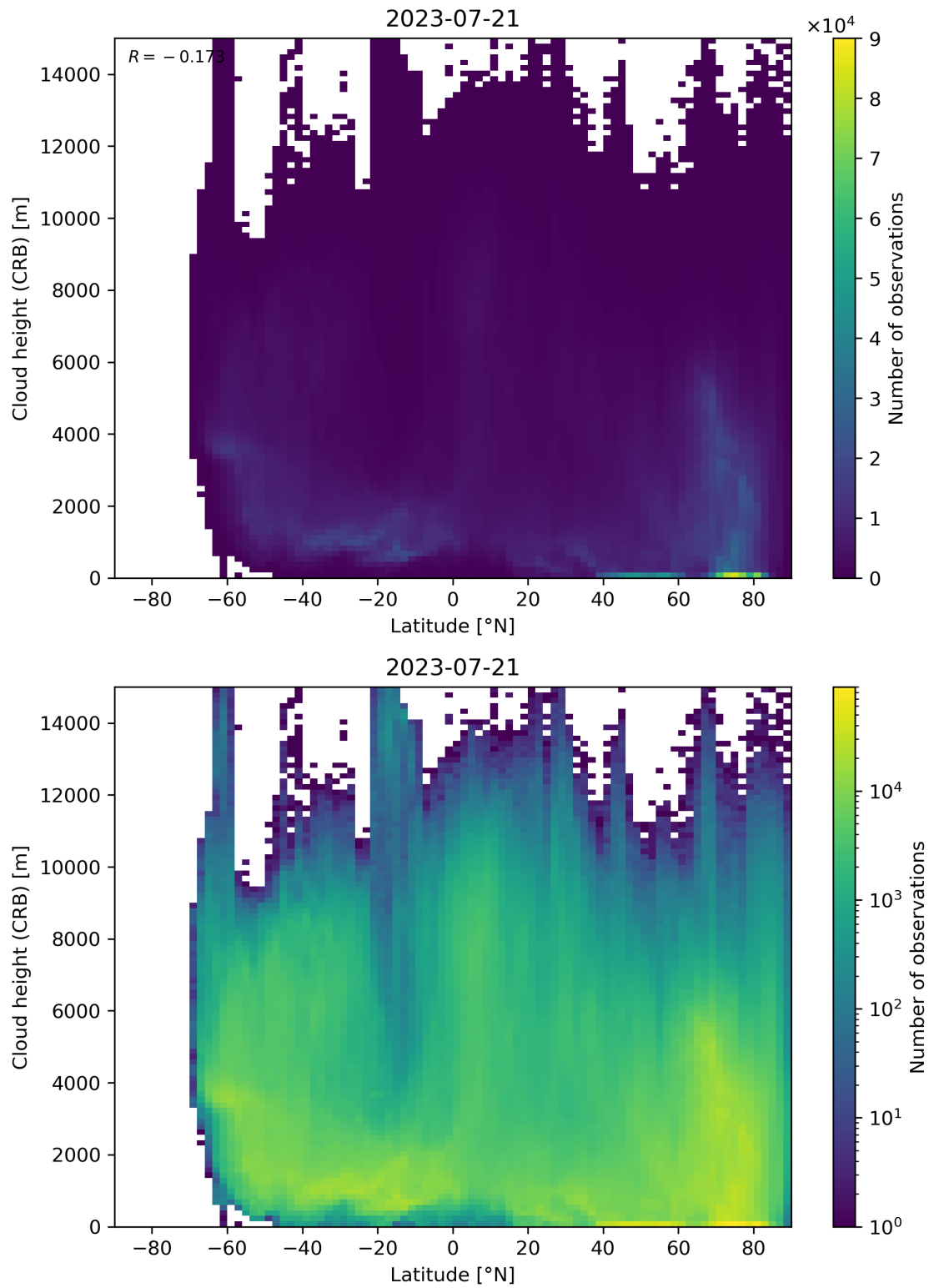
Figure 95: Scatter density plot of “Latitude” against “Cloud height (CRB)” for 2023-07-20 to 2023-07-22.
