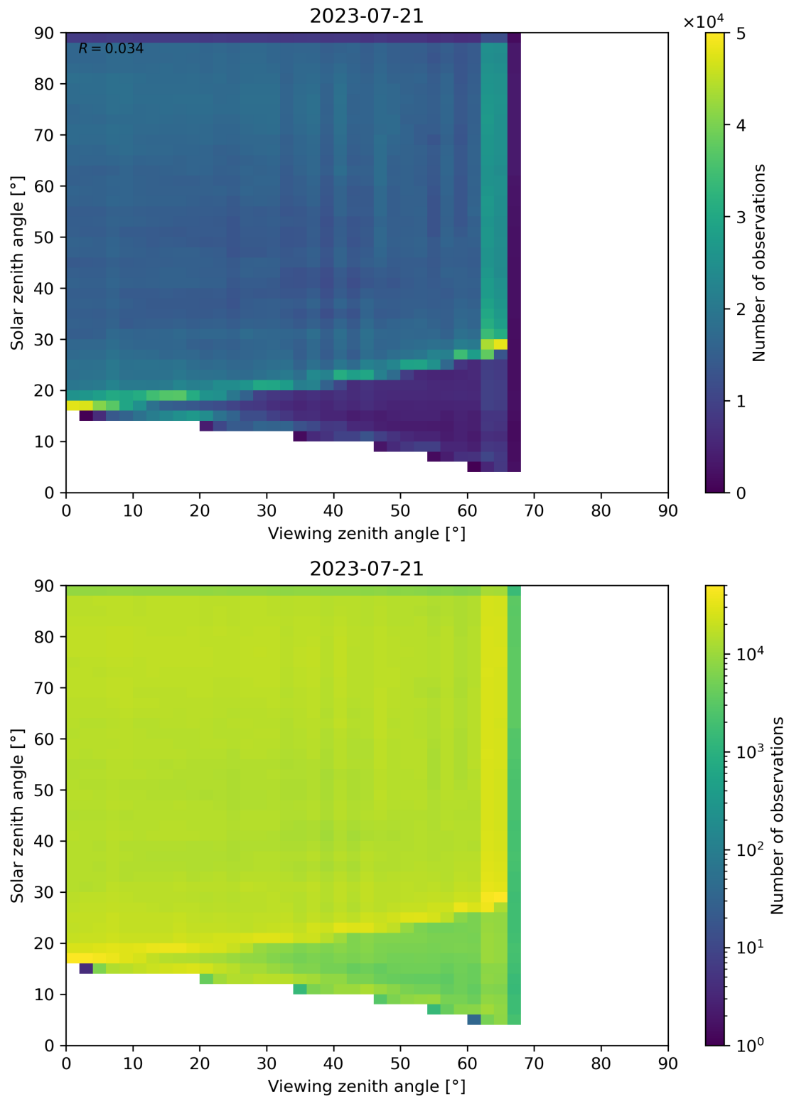
Figure 114: Scatter density plot of “Viewing zenith angle” against “Solar zenith angle” for 2023-07-20 to 2023-07-22.
