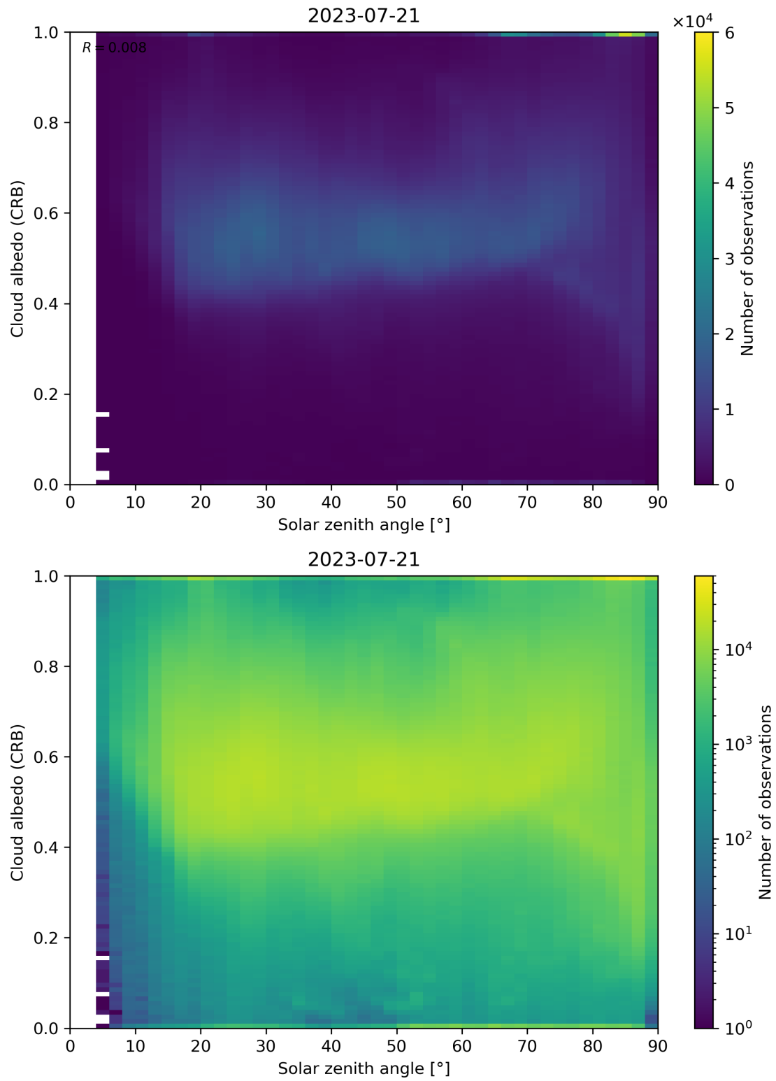
Figure 98: Scatter density plot of “Solar zenith angle” against “Cloud albedo (CRB)” for 2023-07-20 to 2023-07-22.
