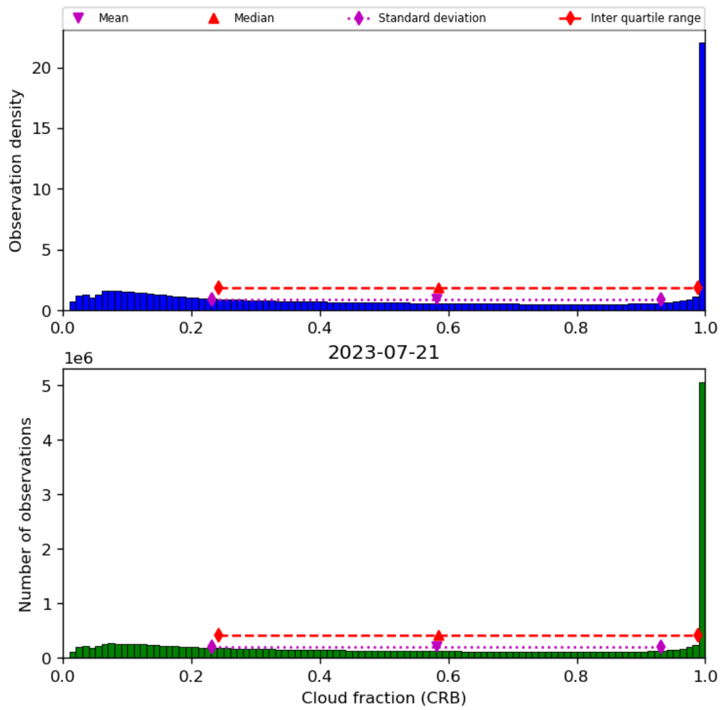
Figure 42: Histogram of “Cloud fraction (CRB)” for 2023-07-20 to 2023-07-22
