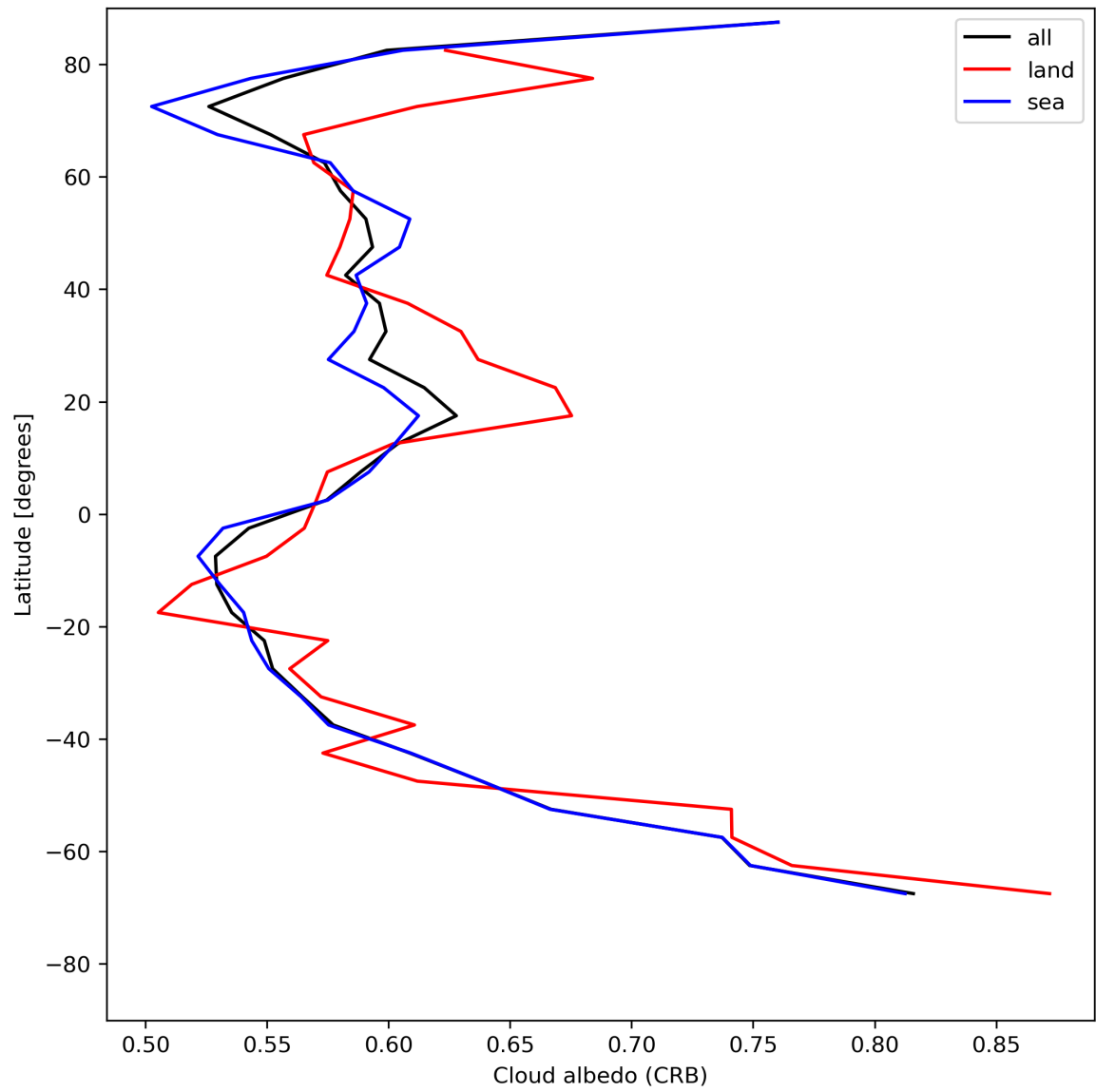
Figure 28: Zonal average of “Cloud albedo (CRB)” for 2023-07-20 to 2023-07-22.
