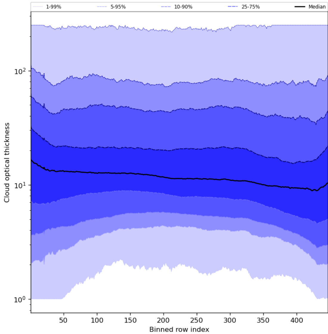
Figure 57: Along track statistics of “Cloud optical thickness” for 2023-07-20 to 2023-07-22
