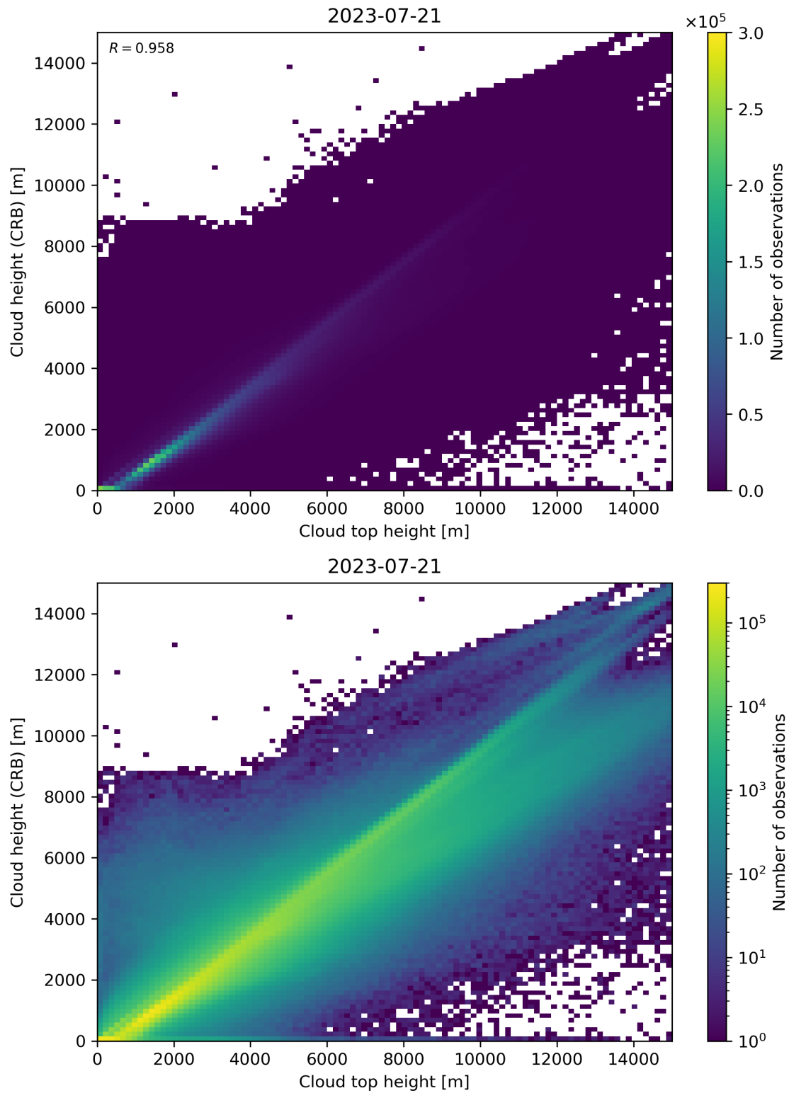
Figure 89: Scatter density plot of “Cloud top height” against “Cloud height (CRB)” for 2023-07-20 to 2023-07-22.
