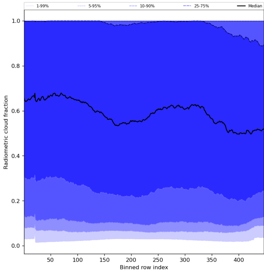
Figure 55: Along track statistics of “Radiometric cloud fraction” for 2023-07-20 to 2023-07-22
