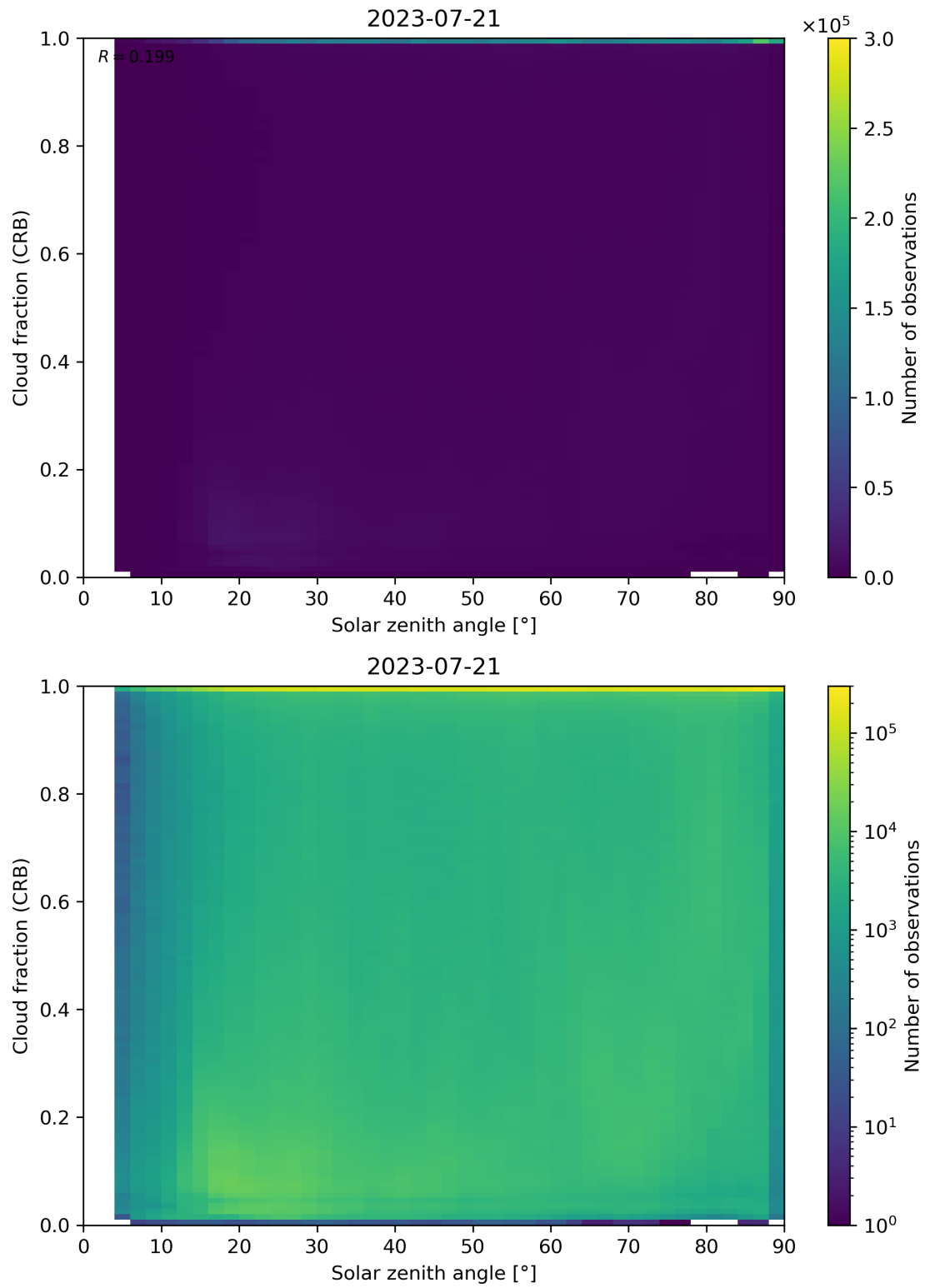
Figure 101: Scatter density plot of “Solar zenith angle” against “Cloud fraction (CRB)” for 2023-07-20 to 2023-07-22.
