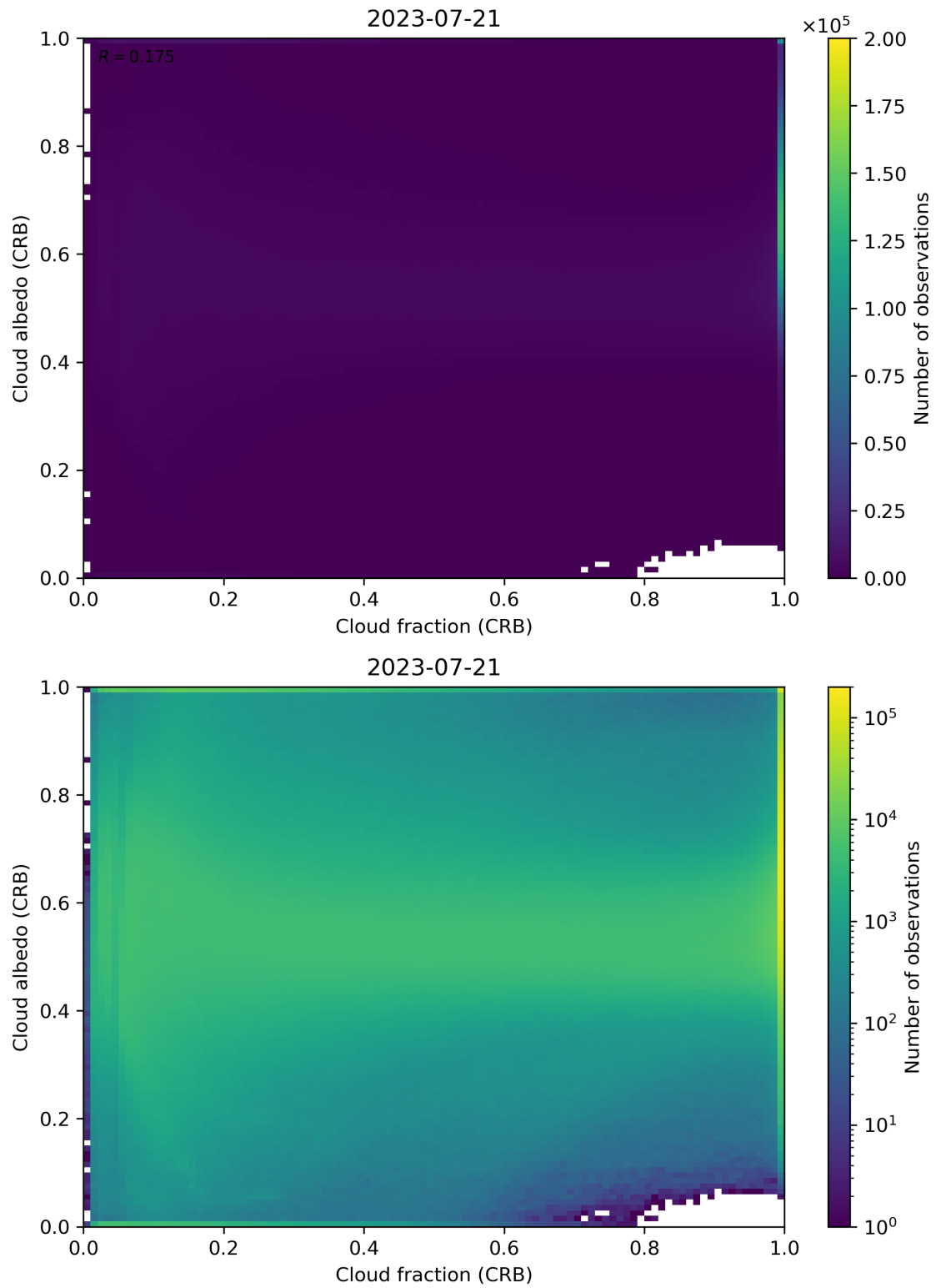
Figure 77: Scatter density plot of “Cloud fraction (CRB)” against “Cloud albedo (CRB)” for 2023-07-20 to 2023-07-22.
