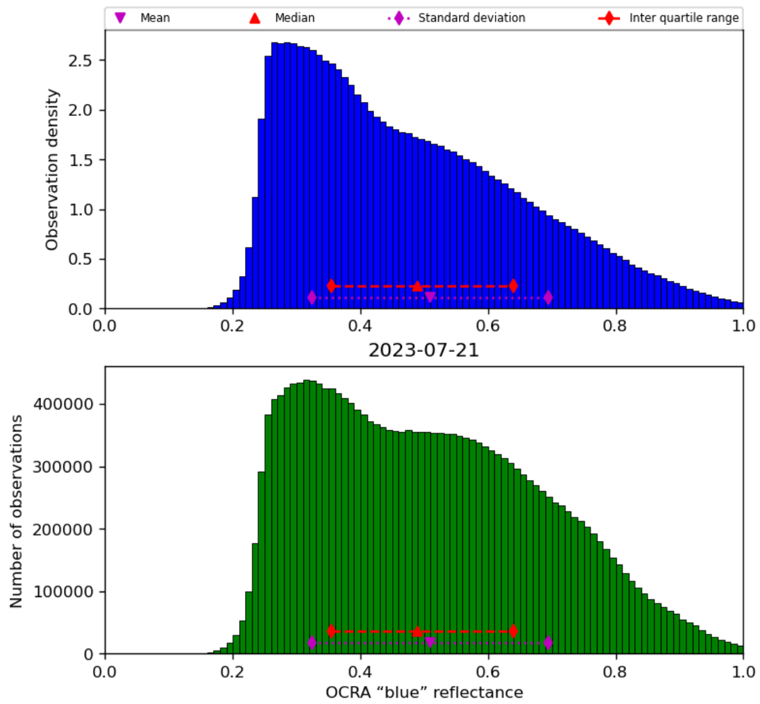
Figure 51: Histogram of “OCRA “blue” reflectance” for 2023-07-20 to 2023-07-22
