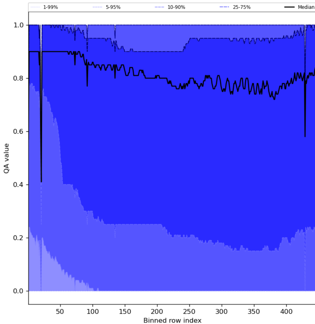
Figure 54: Along track statistics of “QA value” for 2023-07-20 to 2023-07-22
