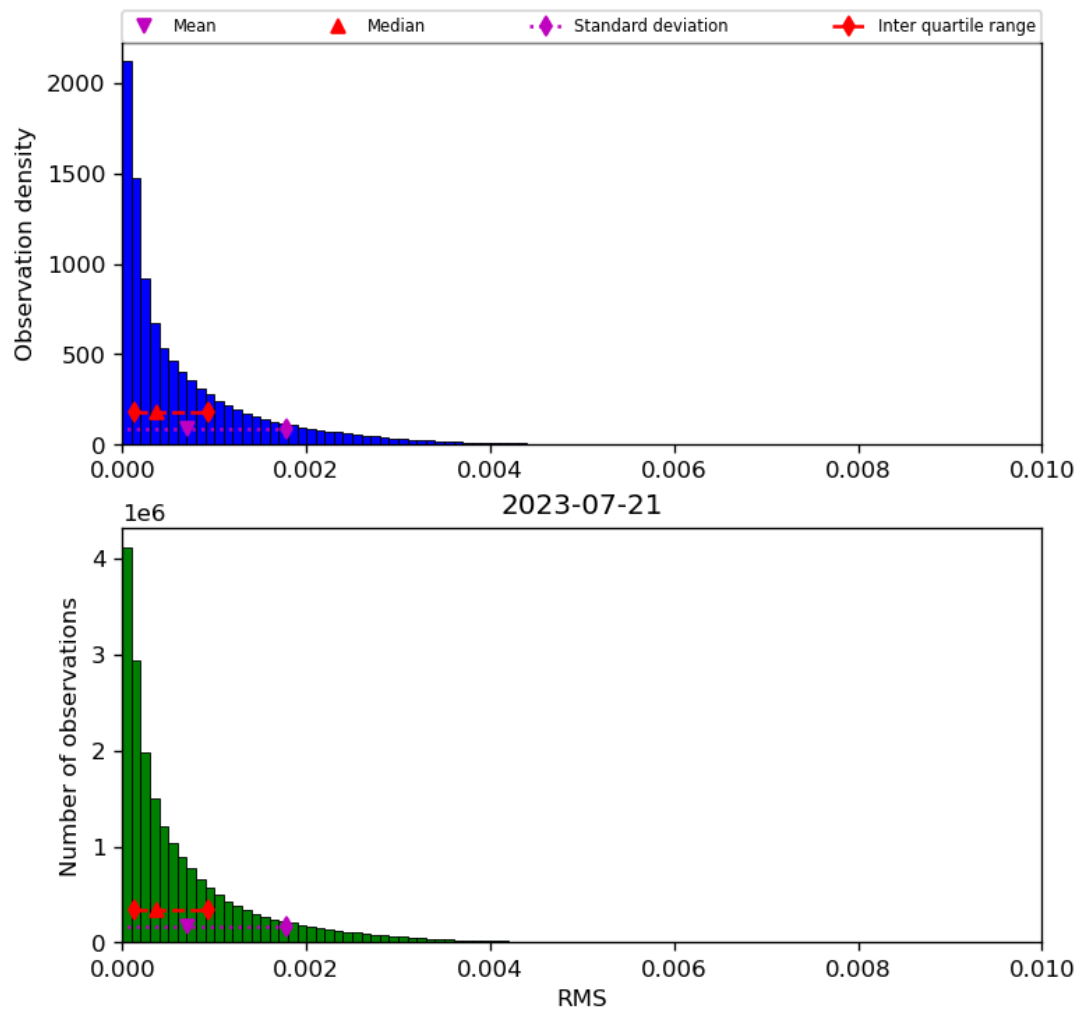
Figure 47: Histogram of “RMS” for 2023-07-20 to 2023-07-22
