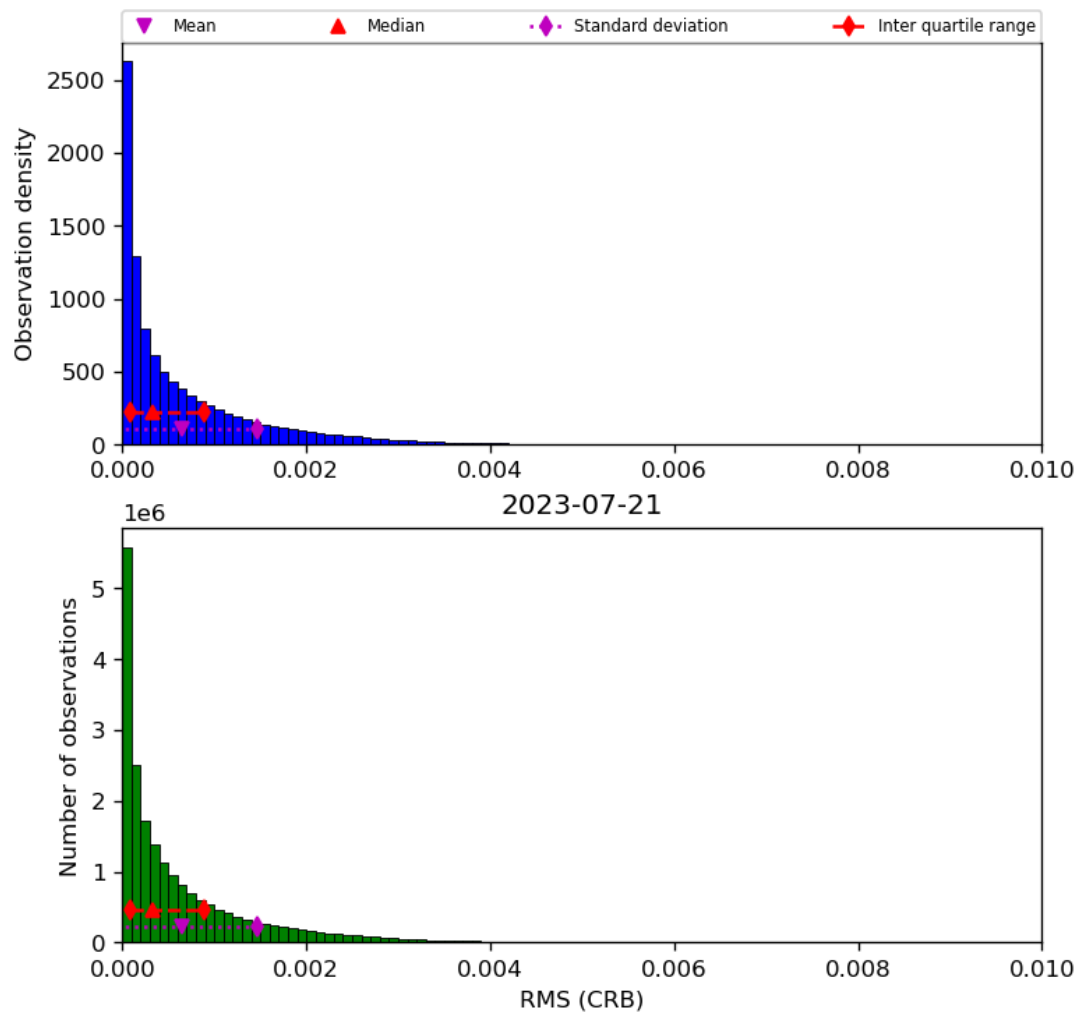
Figure 48: Histogram of “RMS (CRB)” for 2023-07-20 to 2023-07-22
