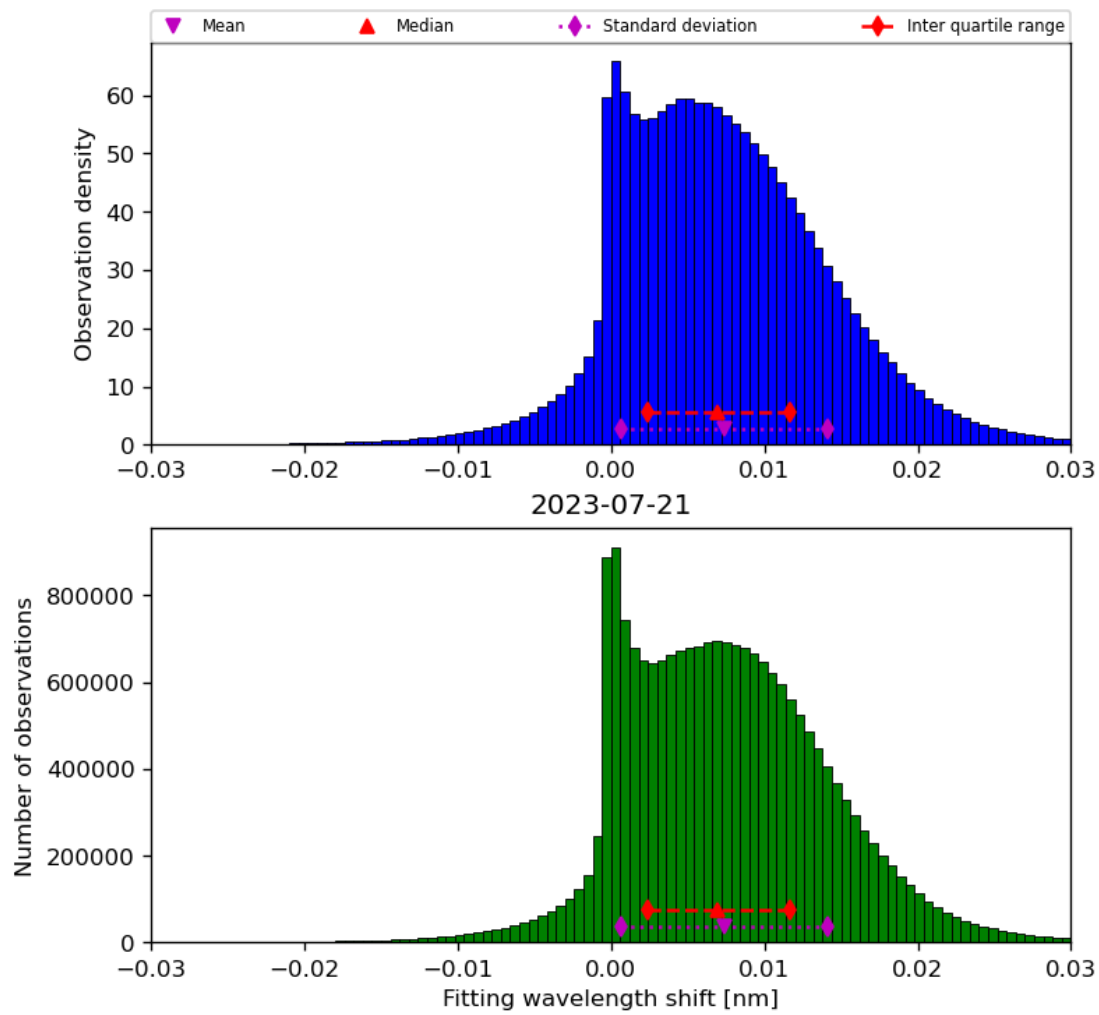
Figure 49: Histogram of “Fitting wavelength shift” for 2023-07-20 to 2023-07-22
