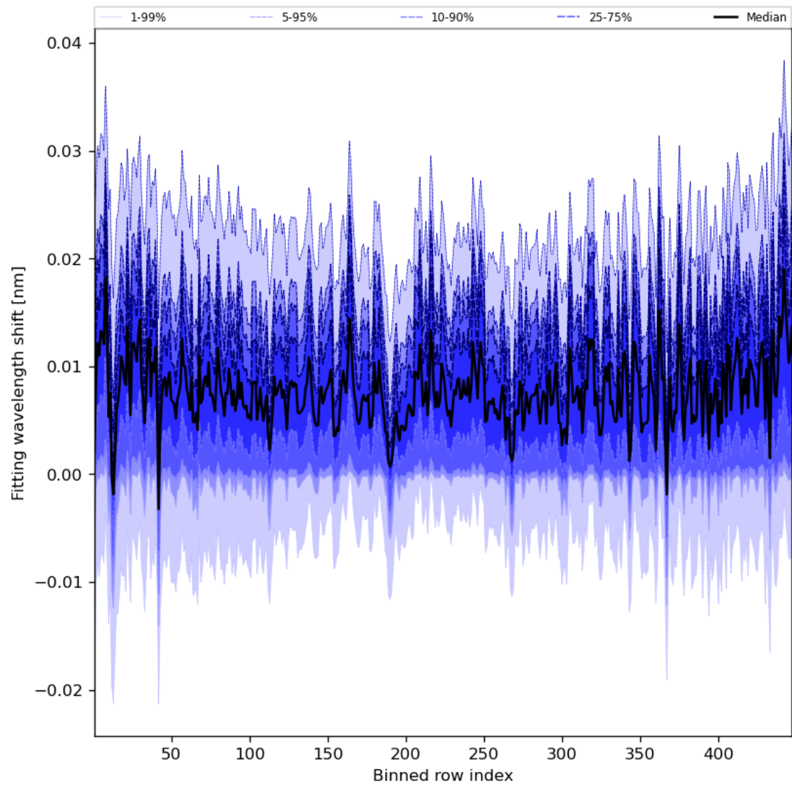
Figure 65: Along track statistics of “Fitting wavelength shift” for 2023-07-20 to 2023-07-22
