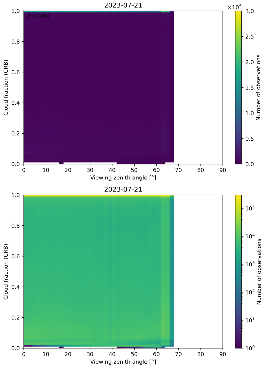
Figure 109: Scatter density plot of “Viewing zenith angle” against “Cloud fraction (CRB)” for 2023-07-20 to 2023-07-22.
