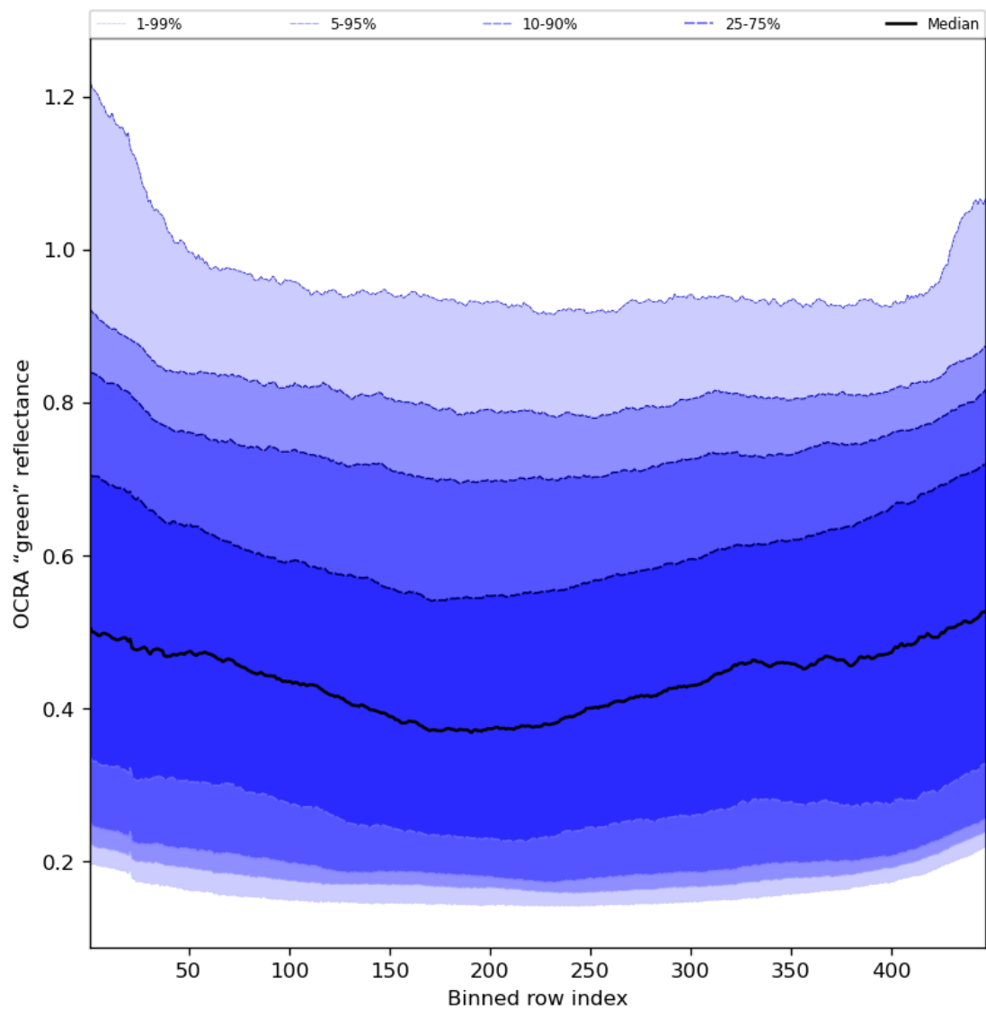
Figure 68: Along track statistics of “OCRA “green” reflectance” for 2023-07-20 to 2023-07-22
