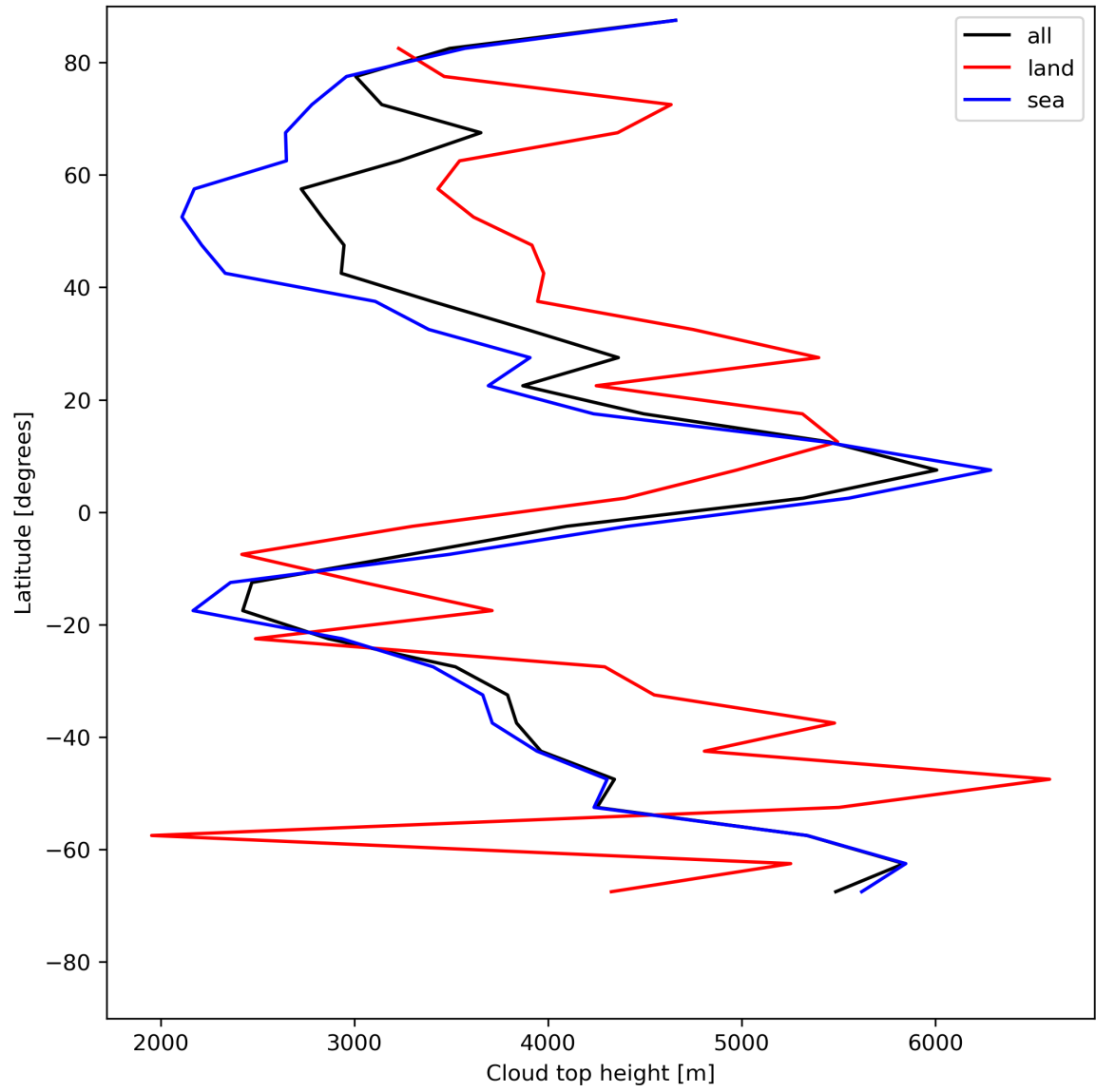
Figure 24: Zonal average of “Cloud top height” for 2023-07-20 to 2023-07-22.
