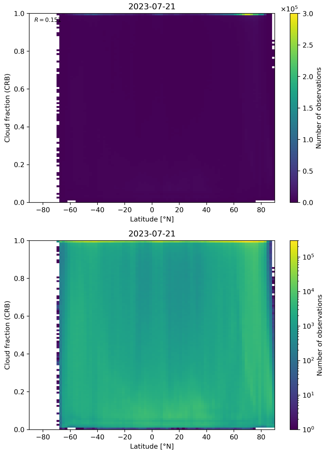
Figure 94: Scatter density plot of “Latitude” against “Cloud fraction (CRB)” for 2023-07-20 to 2023-07-22.
