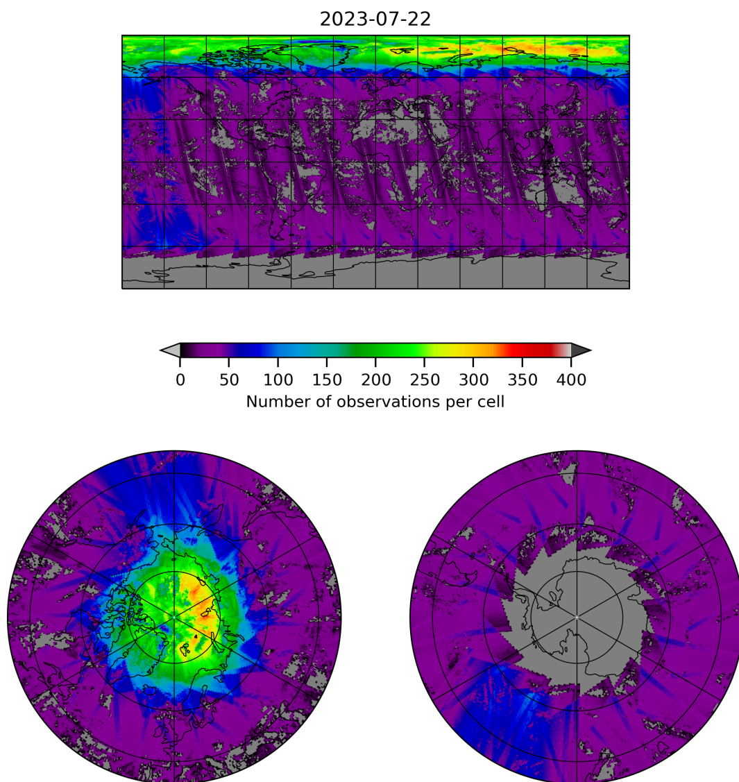
Figure 21: Map of the number of observations for 2023-07-21 to 2023-07-23
