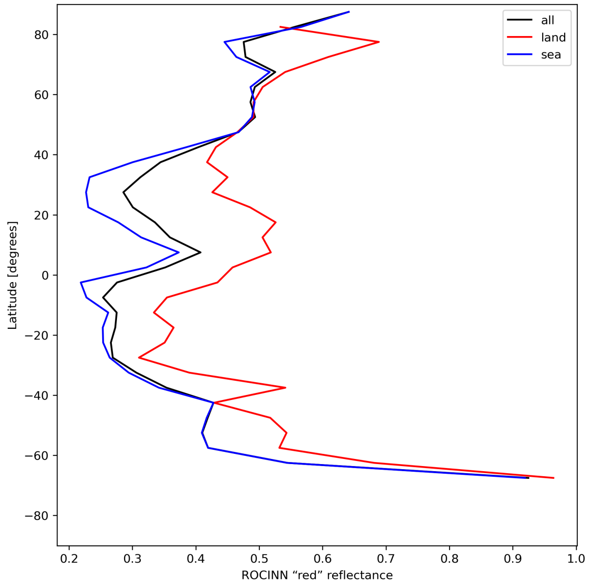
Figure 37: Zonal average of “ROCINN “red” reflectance” for 2023-07-21 to 2023-07-23.
