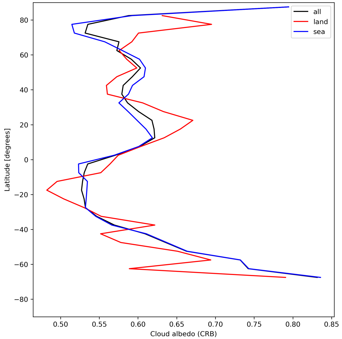
Figure 28: Zonal average of “Cloud albedo (CRB)” for 2023-07-21 to 2023-07-23.
