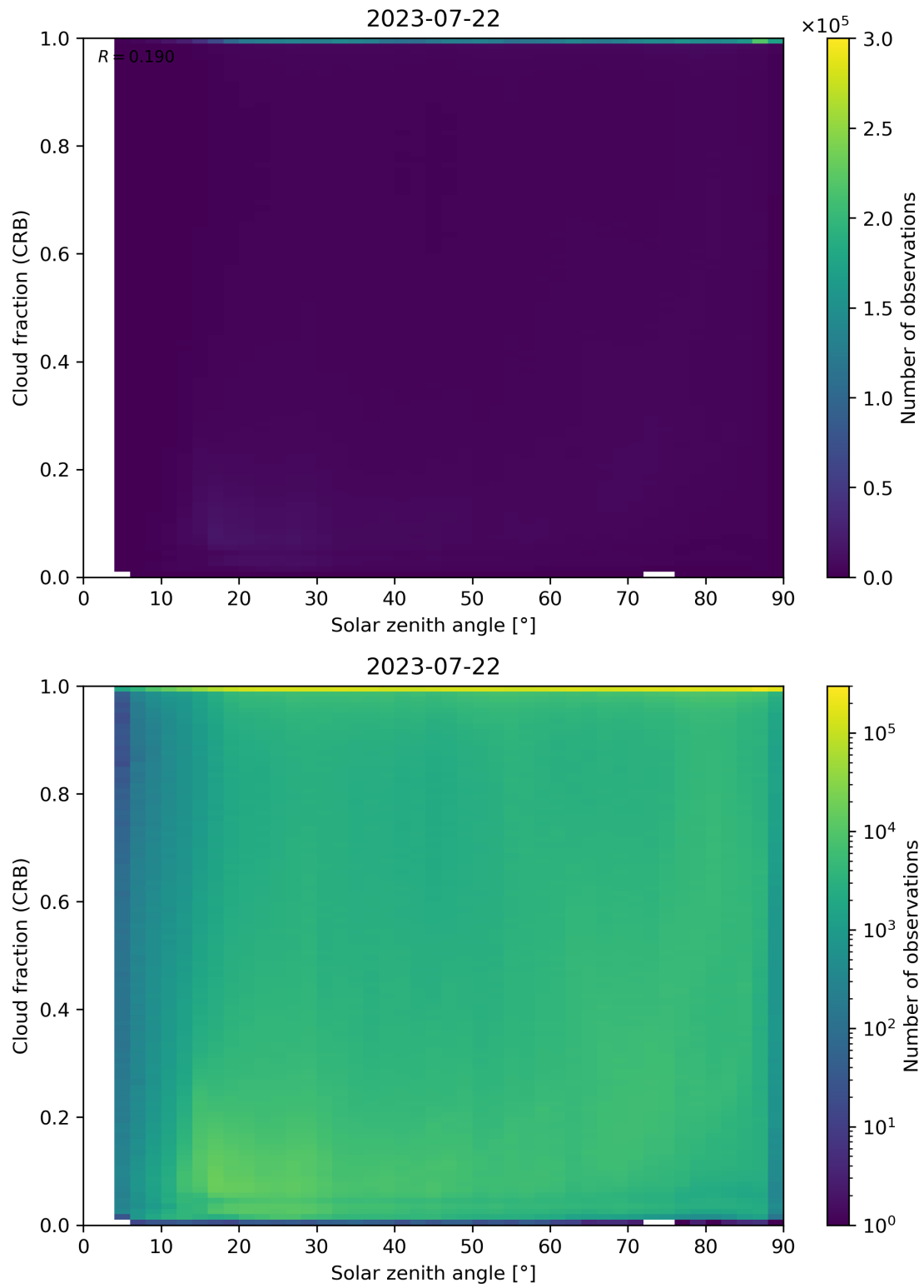
Figure 101: Scatter density plot of “Solar zenith angle” against “Cloud fraction (CRB)” for 2023-07-21 to 2023-07-23.
