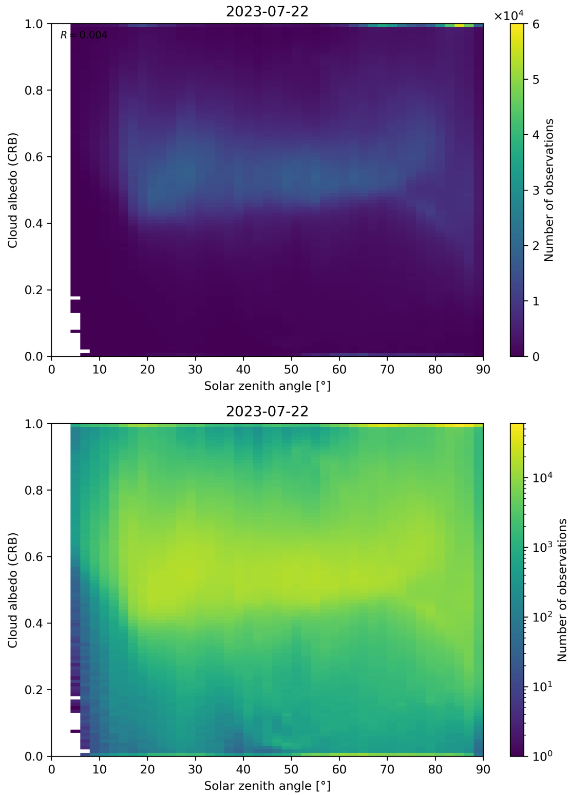
Figure 98: Scatter density plot of “Solar zenith angle” against “Cloud albedo (CRB)” for 2023-07-21 to 2023-07-23.
