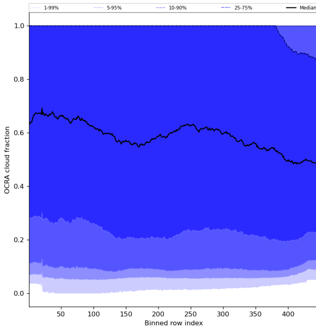
Figure 66: Along track statistics of “OCRA cloud fraction” for 2023-07-21 to 2023-07-23
