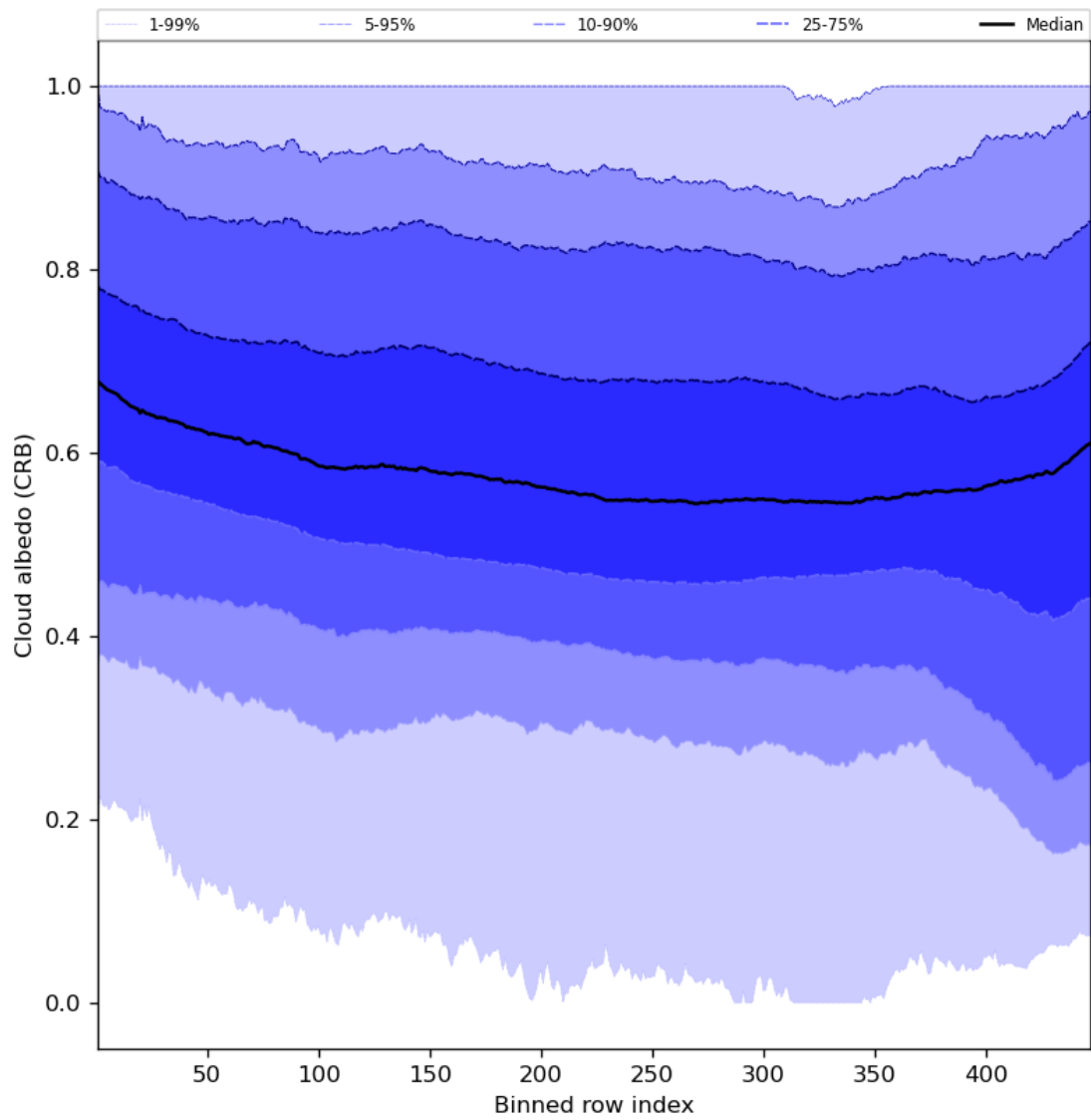
Figure 60: Along track statistics of “Cloud albedo (CRB)” for 2023-07-21 to 2023-07-23
