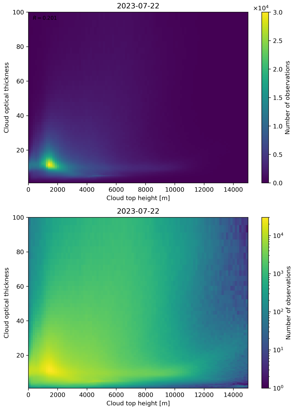
Figure 90: Scatter density plot of “Cloud top height” against “Cloud optical thickness” for 2023-07-21 to 2023-07-23.
