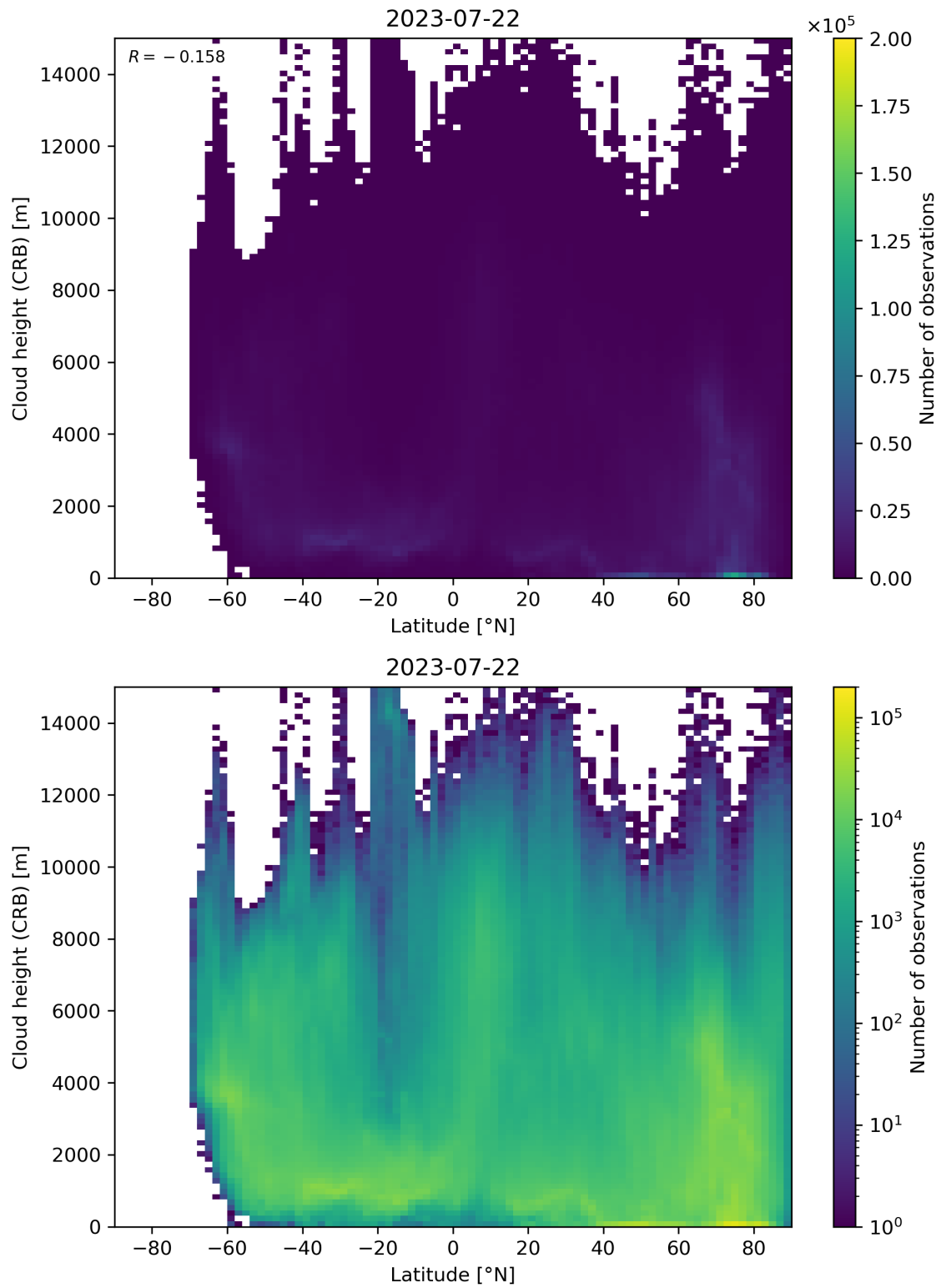
Figure 95: Scatter density plot of “Latitude” against “Cloud height (CRB)” for 2023-07-21 to 2023-07-23.
