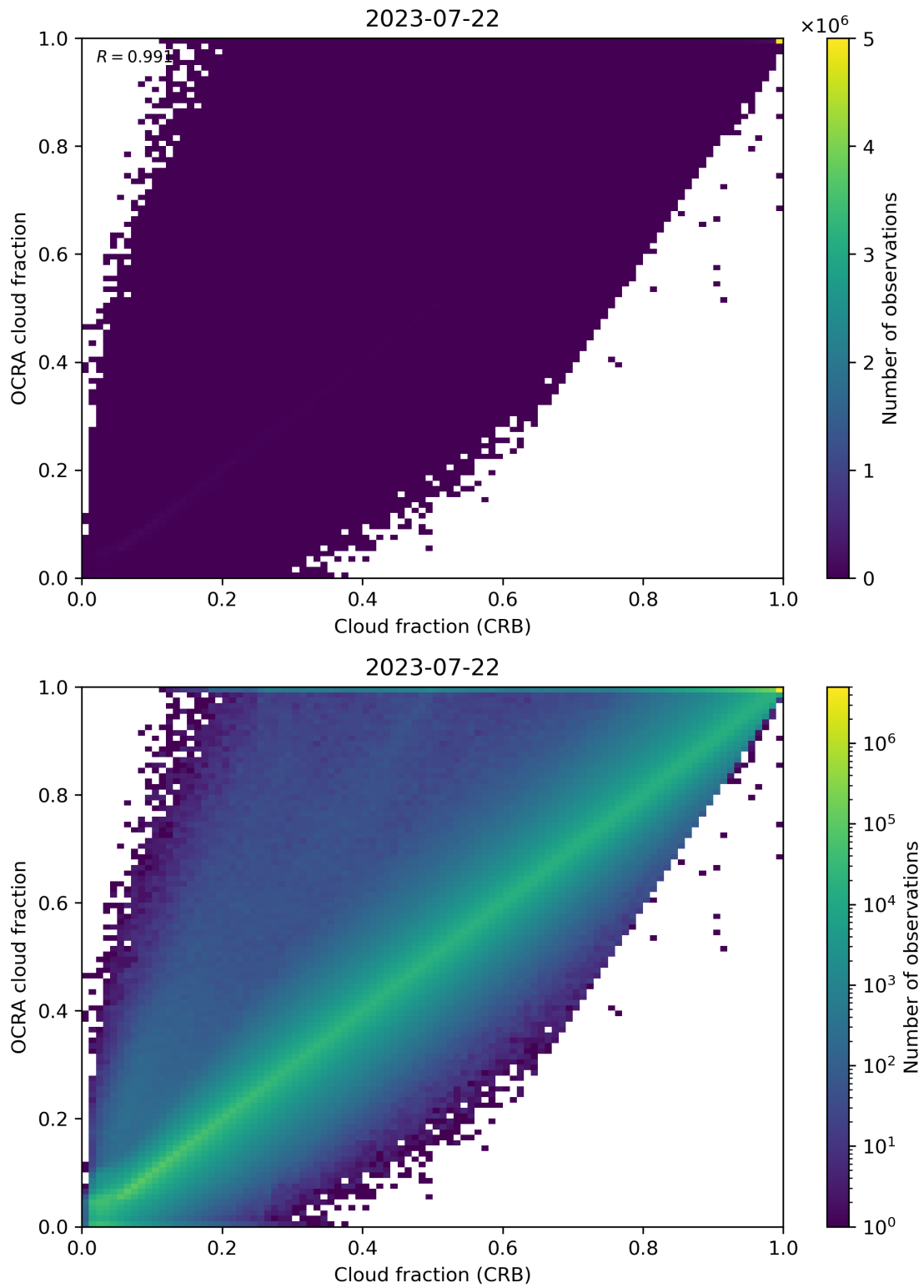
Figure 78: Scatter density plot of “Cloud fraction (CRB)” against “OCRA cloud fraction” for 2023-07-21 to 2023-07-23.
