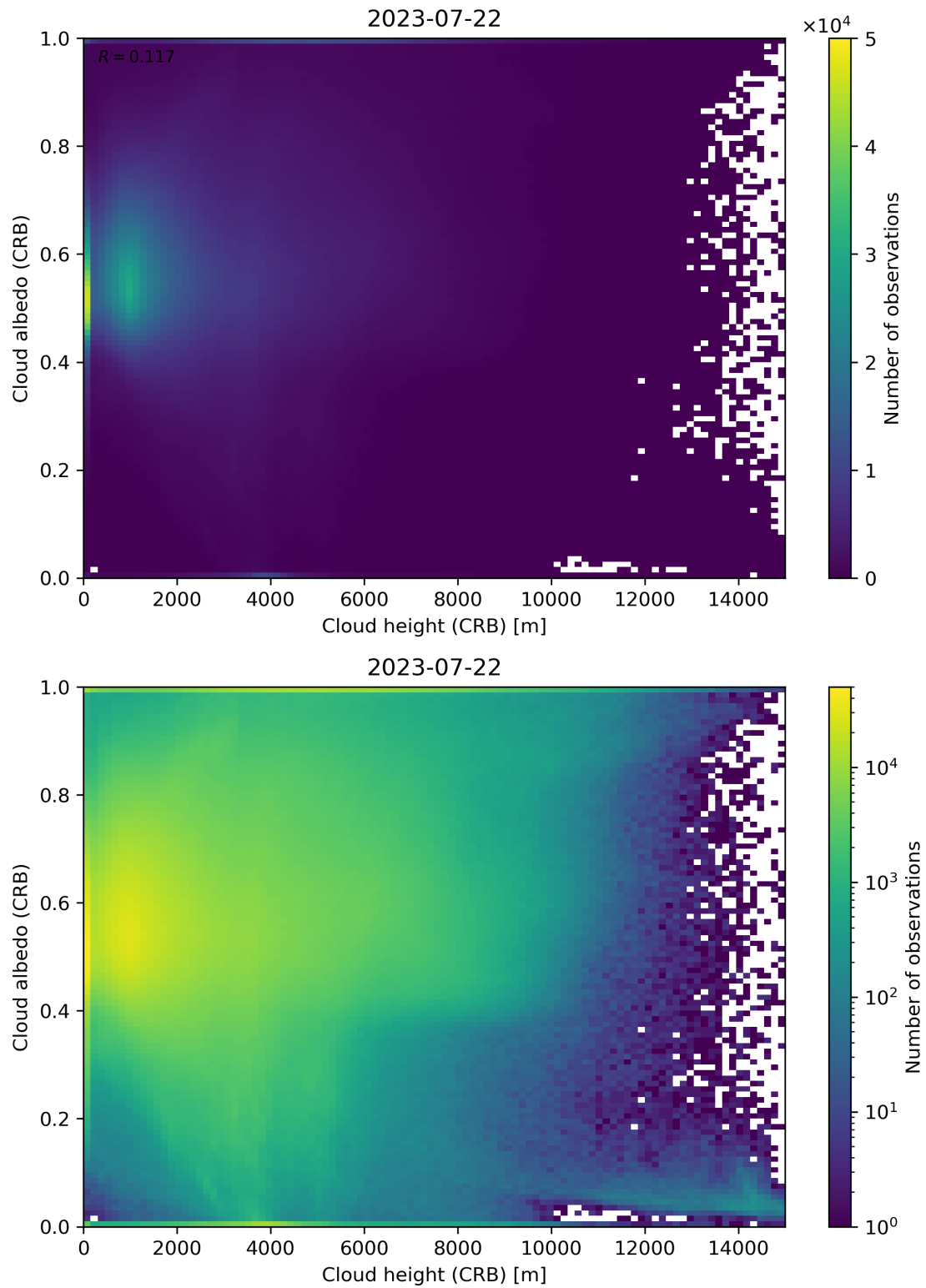
Figure 80: Scatter density plot of “Cloud height (CRB)” against “Cloud albedo (CRB)” for 2023-07-21 to 2023-07-23.
