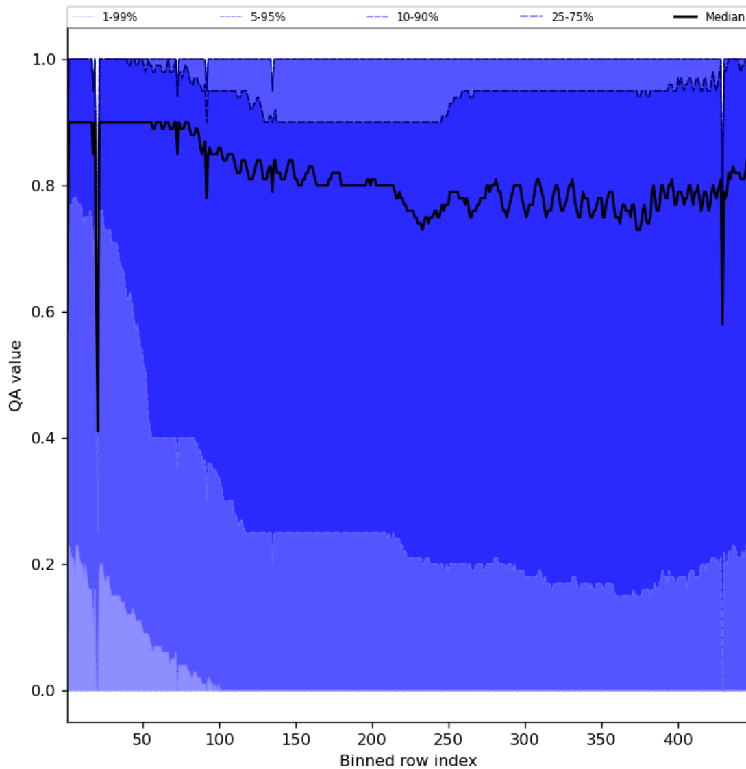
Figure 54: Along track statistics of “QA value” for 2023-07-21 to 2023-07-23
