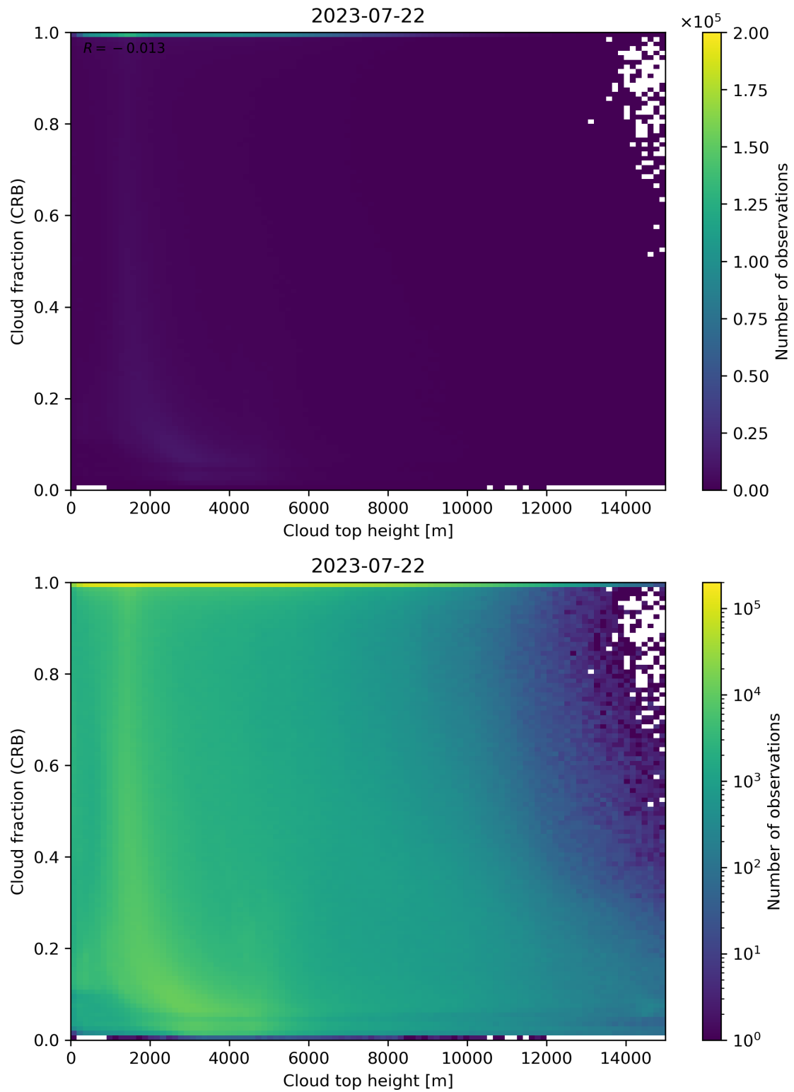
Figure 88: Scatter density plot of “Cloud top height” against “Cloud fraction (CRB)” for 2023-07-21 to 2023-07-23.
