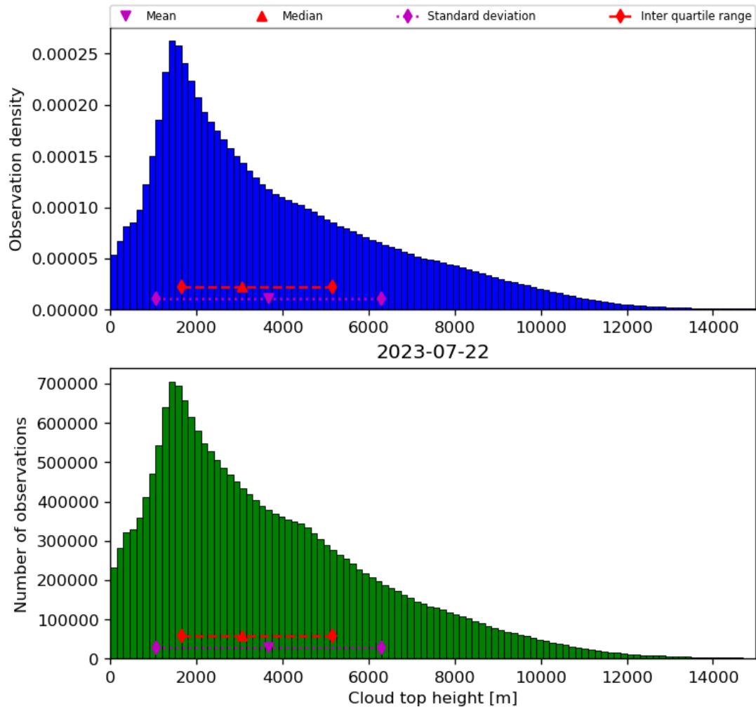
Figure 40: Histogram of “Cloud top height” for 2023-07-21 to 2023-07-23
