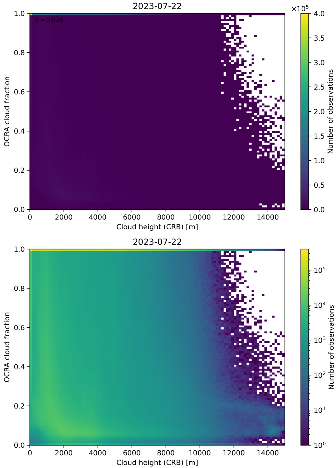
Figure 81: Scatter density plot of “Cloud height (CRB)” against “OCRA cloud fraction” for 2023-07-21 to 2023-07-23.
