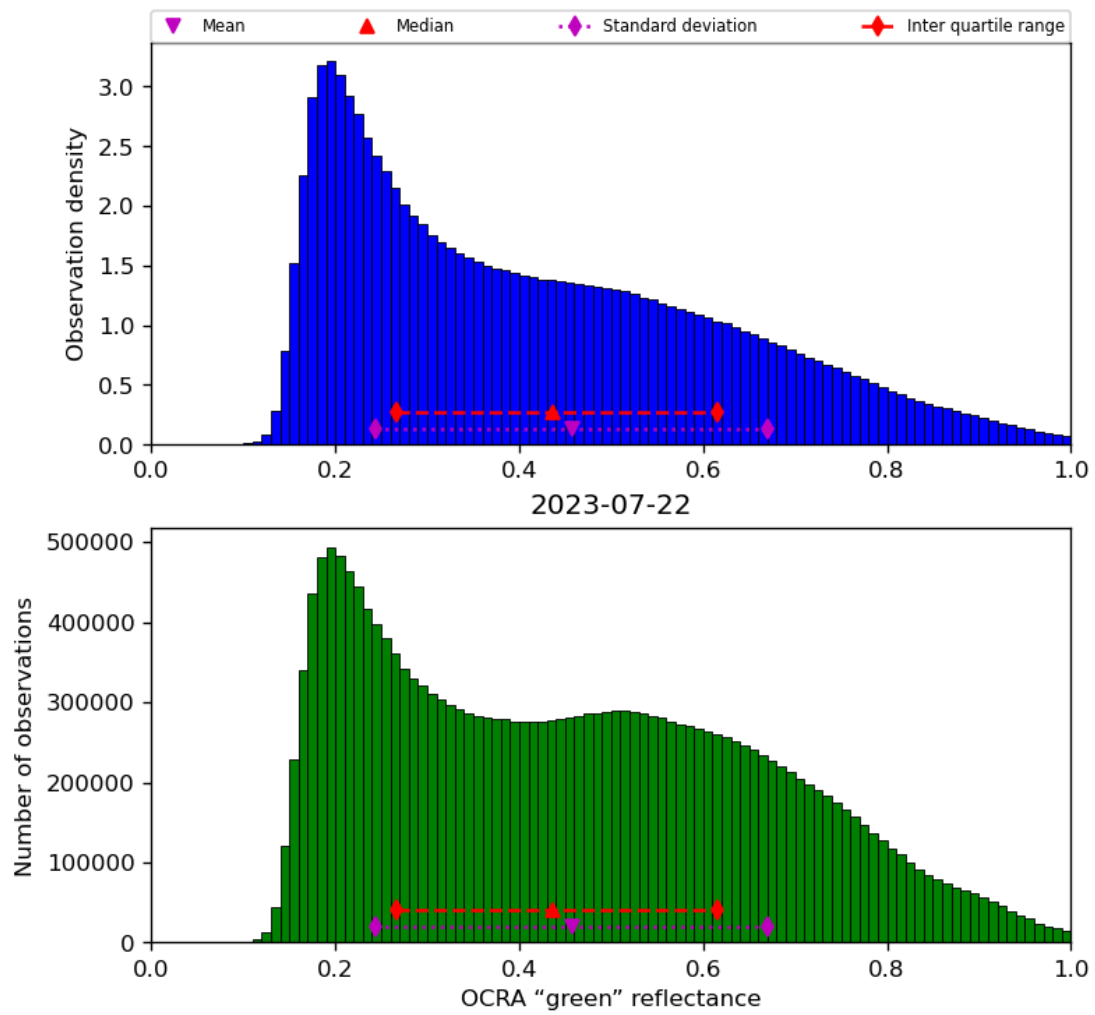
Figure 52: Histogram of “OCRA “green” reflectance” for 2023-07-21 to 2023-07-23
