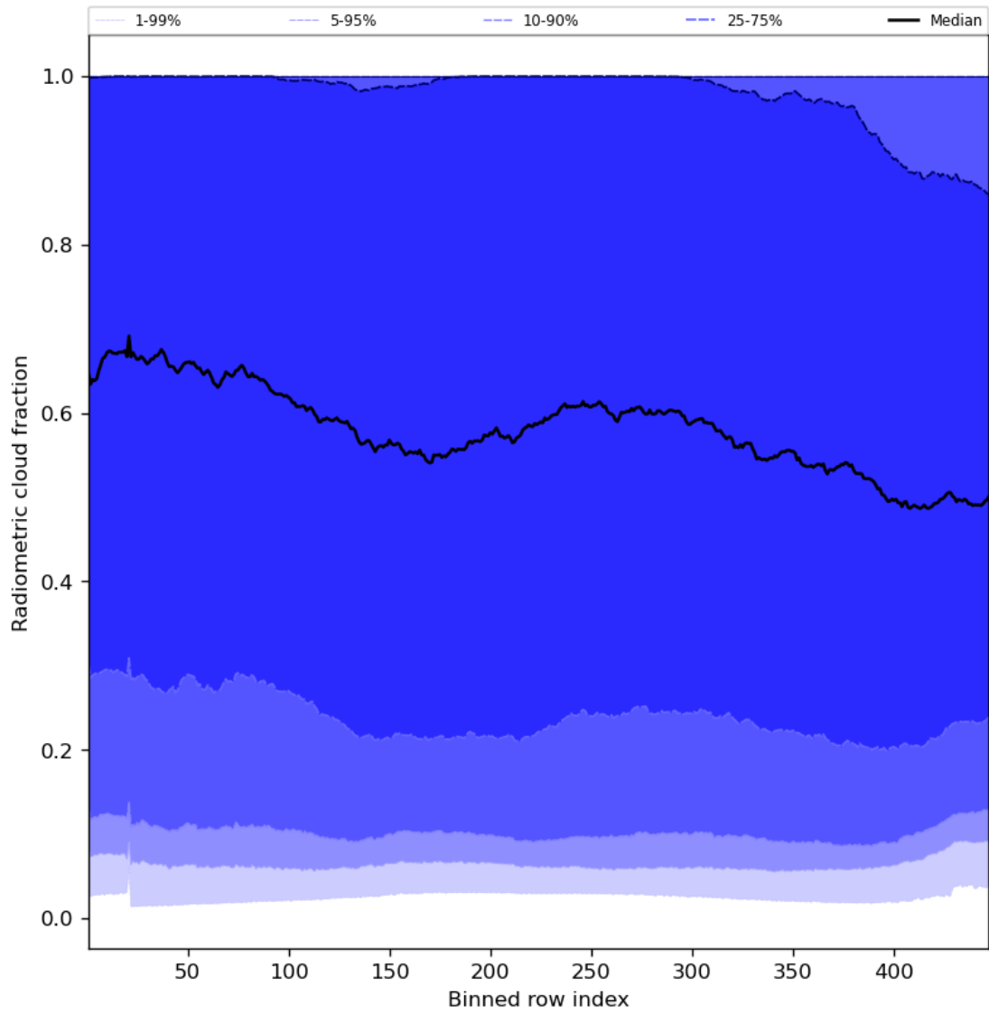
Figure 55: Along track statistics of “Radiometric cloud fraction” for 2023-07-21 to 2023-07-23
