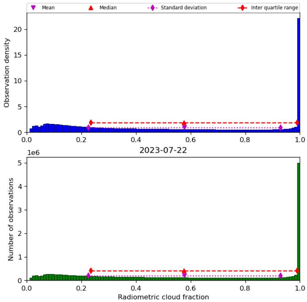
Figure 39: Histogram of “Radiometric cloud fraction” for 2023-07-21 to 2023-07-23
