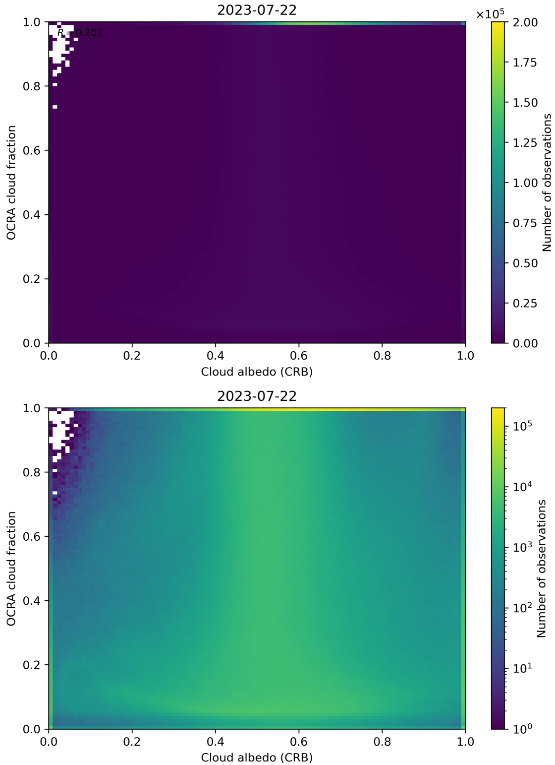
Figure 70: Scatter density plot of “Cloud albedo (CRB)” against “OCRA cloud fraction” for 2023-07-21 to 2023-07-23.
