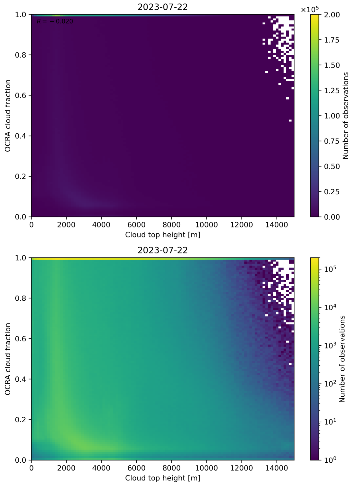
Figure 87: Scatter density plot of “Cloud top height” against “OCRA cloud fraction” for 2023-07-21 to 2023-07-23.
