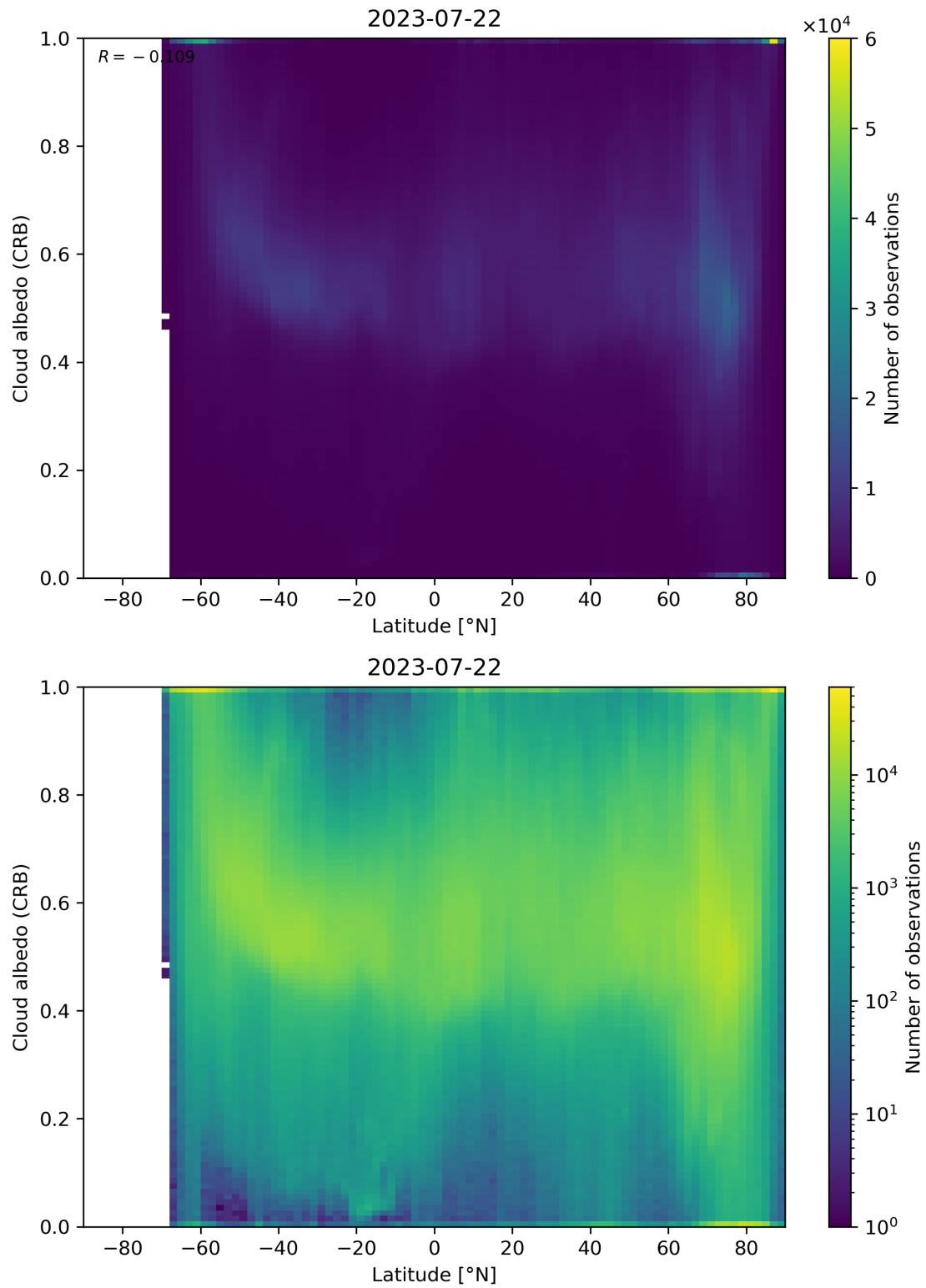
Figure 91: Scatter density plot of “Latitude” against “Cloud albedo (CRB)” for 2023-07-21 to 2023-07-23.
