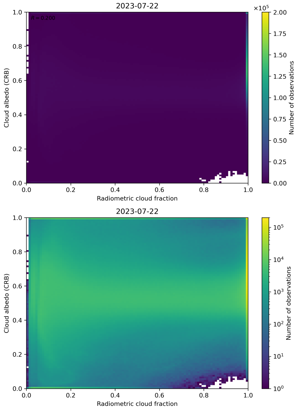
Figure 71: Scatter density plot of “Radiometric cloud fraction” against “Cloud albedo (CRB)” for 2023-07-21 to 2023-07-23.
