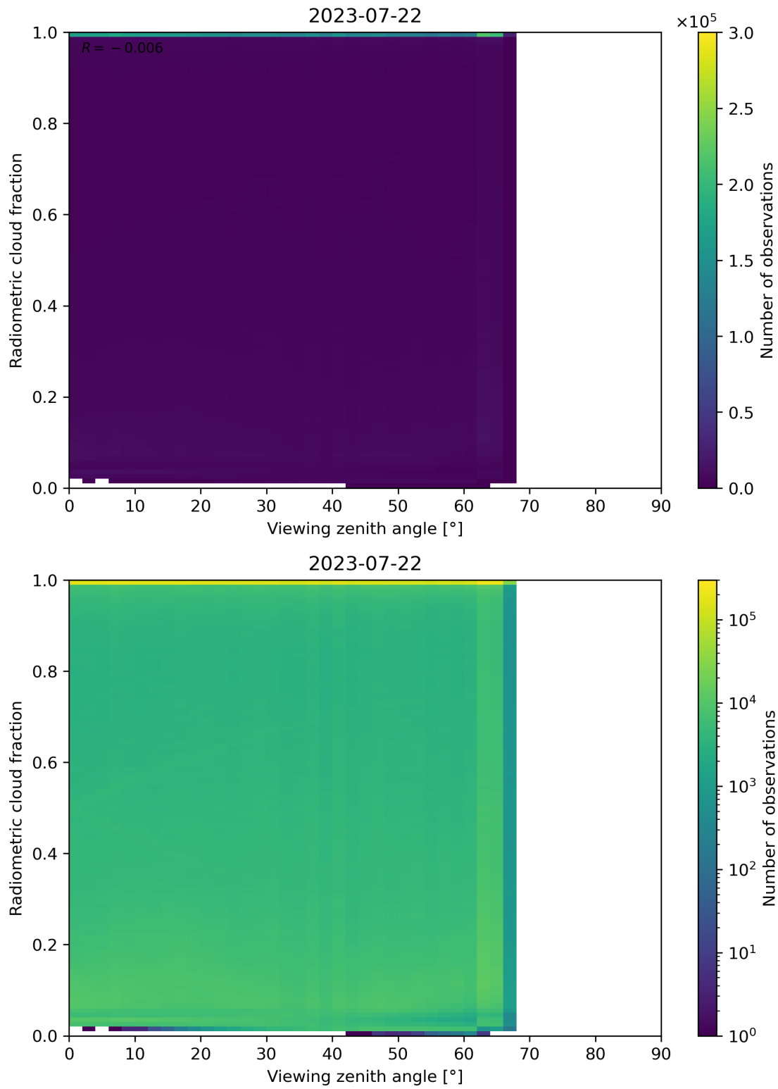
Figure 107: Scatter density plot of “Viewing zenith angle” against “Radiometric cloud fraction” for 2023-07-21 to 2023-07-23.
