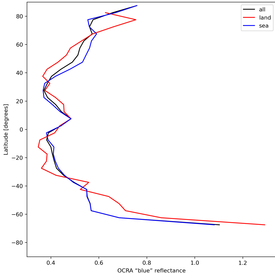
Figure 35: Zonal average of “OCRA “blue” reflectance” for 2023-07-21 to 2023-07-23.
