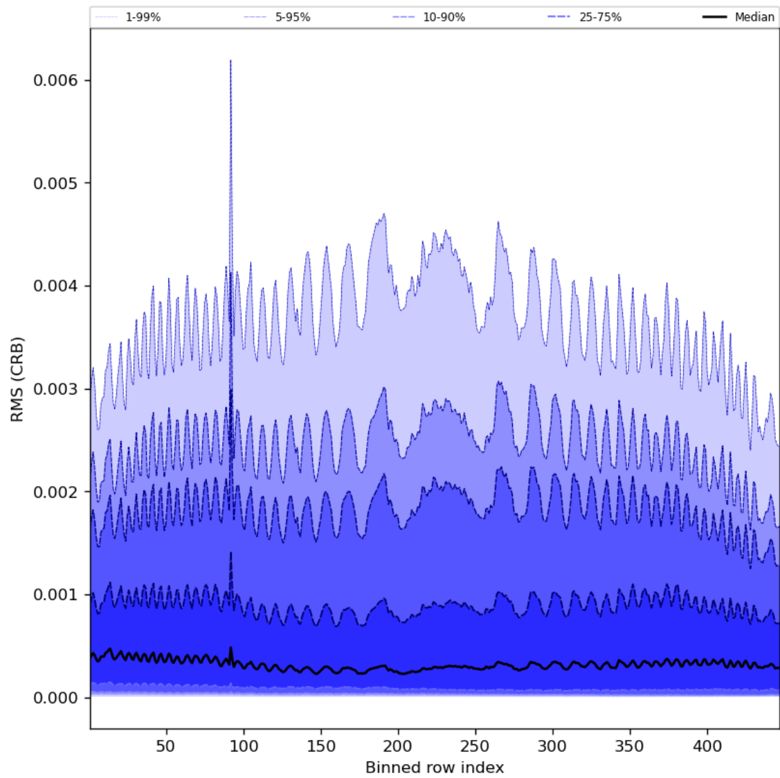
Figure 64: Along track statistics of “RMS (CRB)” for 2023-07-21 to 2023-07-23
