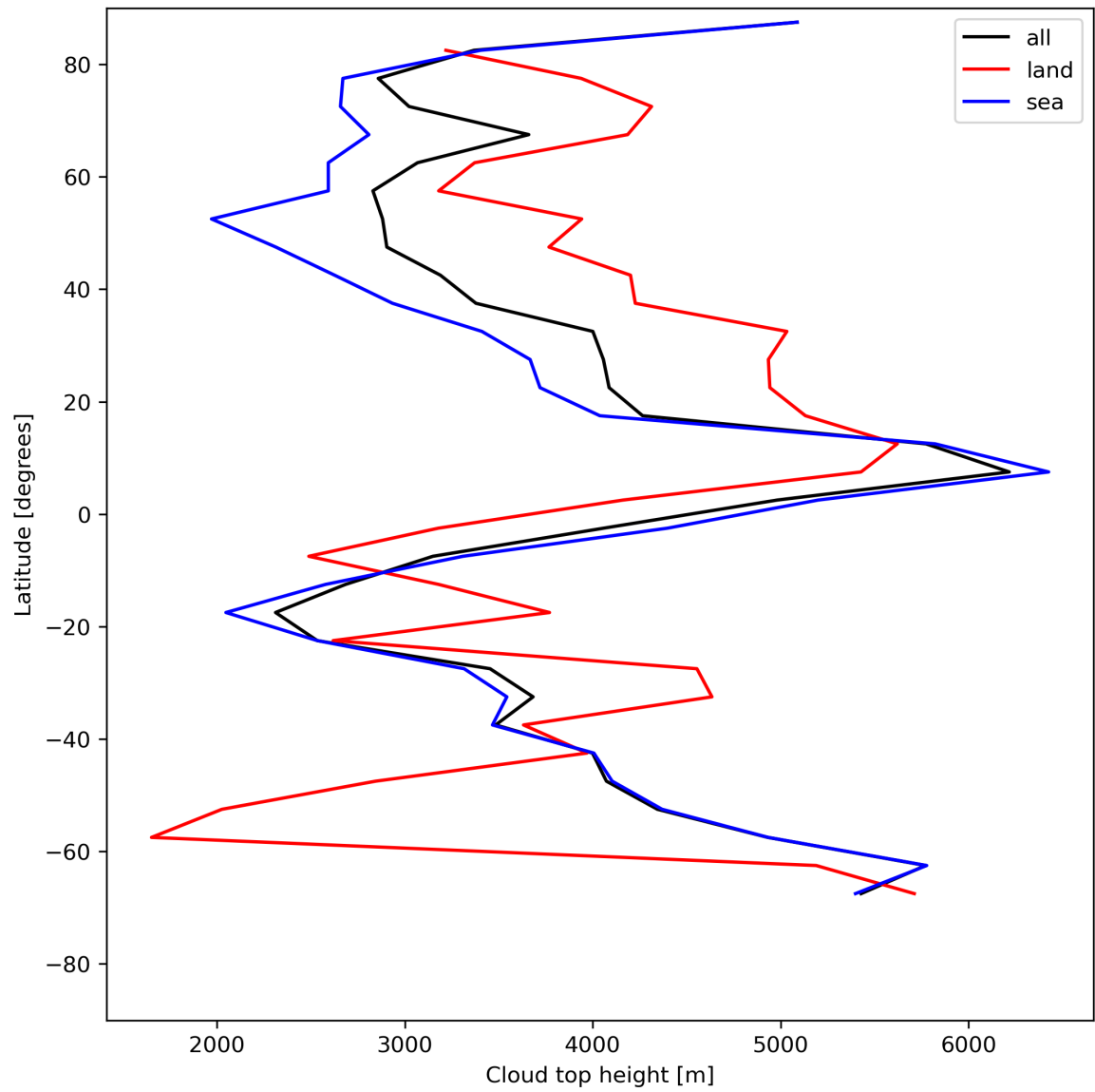
Figure 24: Zonal average of “Cloud top height” for 2023-07-21 to 2023-07-23.
