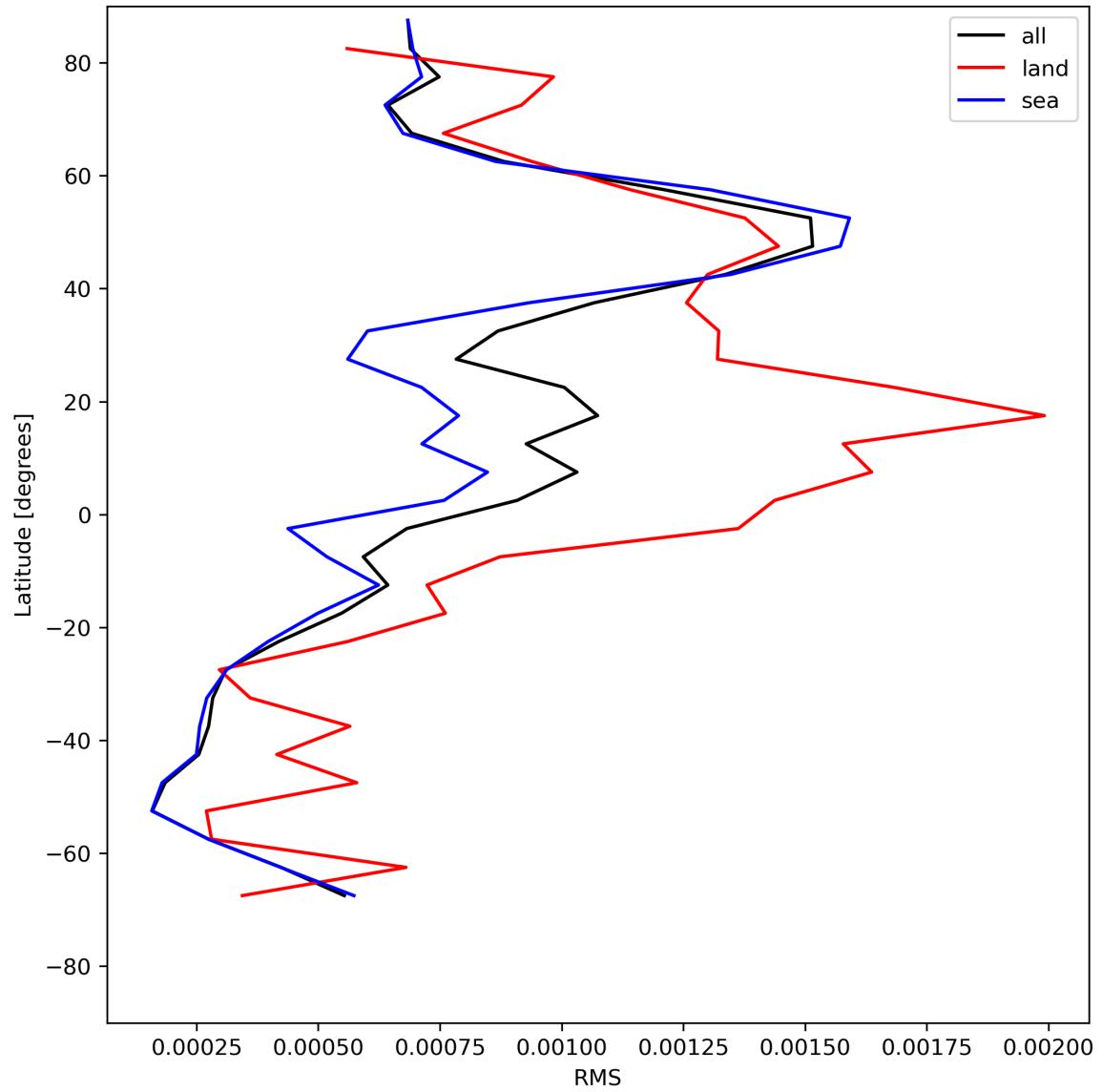
Figure 31: Zonal average of “RMS” for 2023-07-21 to 2023-07-23.
