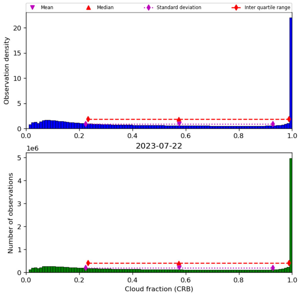
Figure 42: Histogram of “Cloud fraction (CRB)” for 2023-07-21 to 2023-07-23
