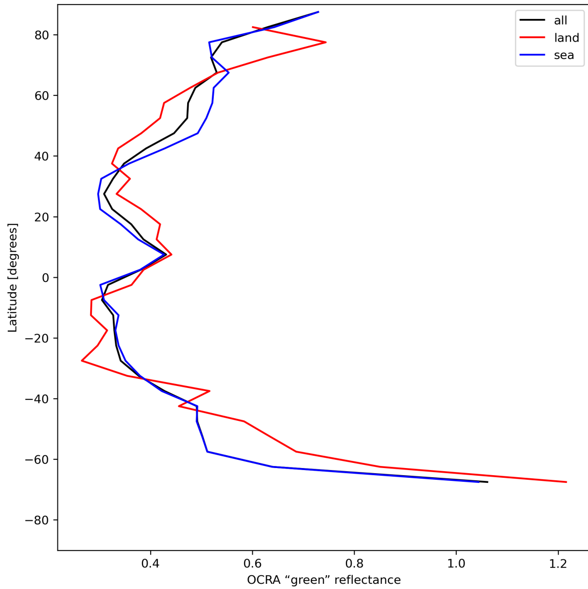
Figure 36: Zonal average of “OCRA “green” reflectance” for 2023-07-21 to 2023-07-23.
