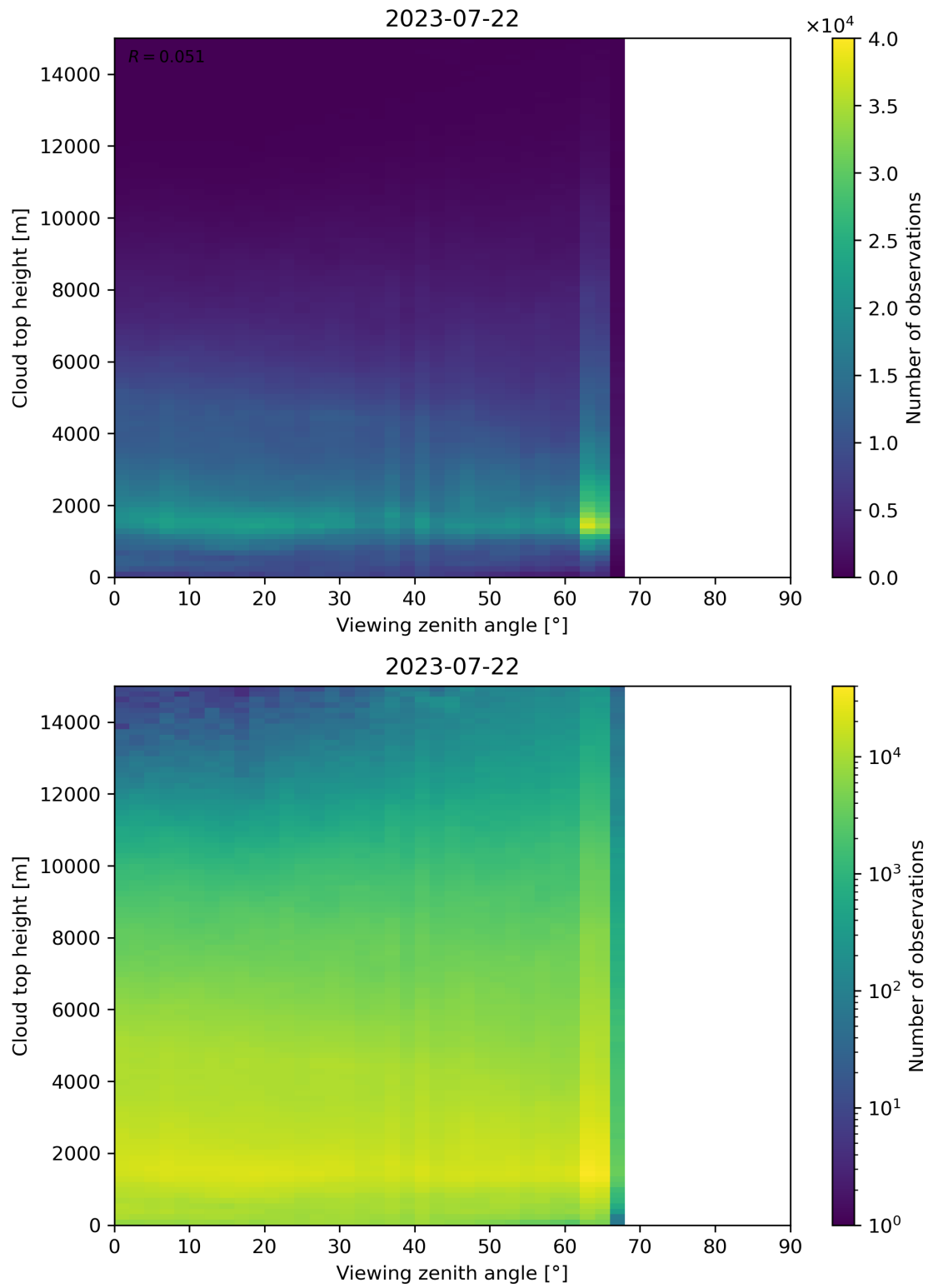
Figure 112: Scatter density plot of “Viewing zenith angle” against “Cloud top height” for 2023-07-21 to 2023-07-23.
