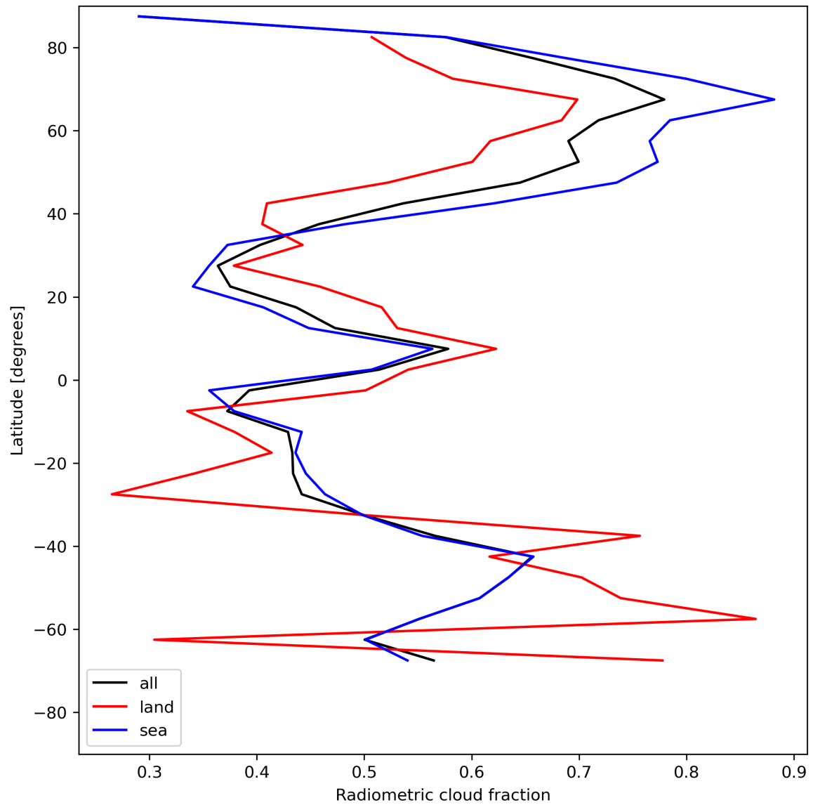
Figure 23: Zonal average of “Radiometric cloud fraction” for 2023-07-21 to 2023-07-23.
