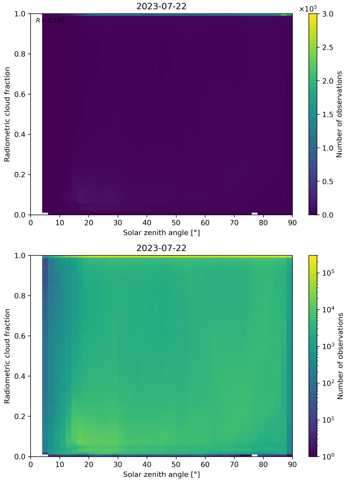
Figure 99: Scatter density plot of “Solar zenith angle” against “Radiometric cloud fraction” for 2023-07-21 to 2023-07-23.
