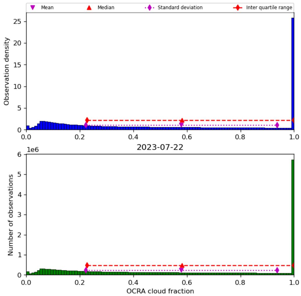
Figure 50: Histogram of “OCRA cloud fraction” for 2023-07-21 to 2023-07-23
