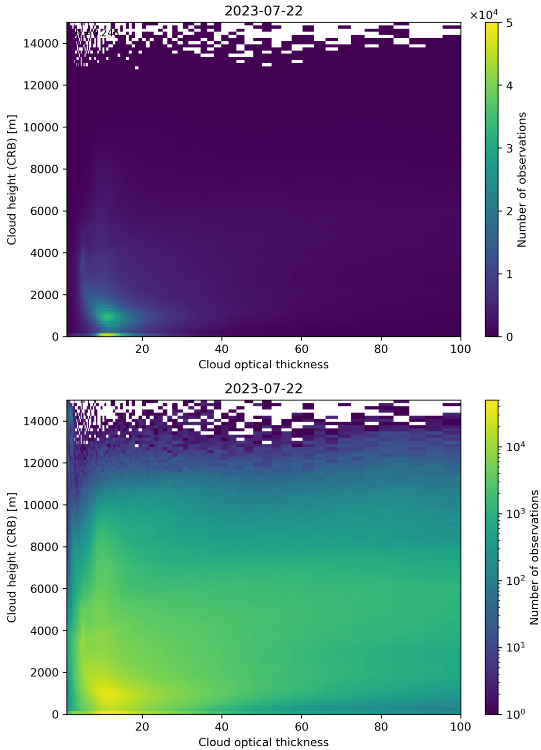
Figure 85: Scatter density plot of “Cloud optical thickness” against “Cloud height (CRB)” for 2023-07-21 to 2023-07-23.
