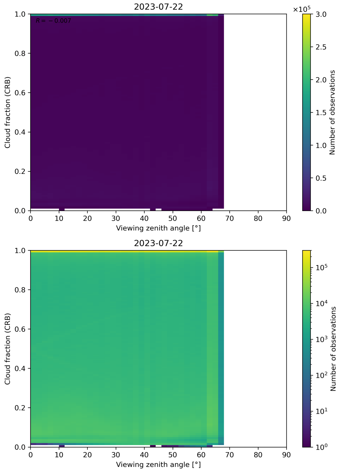
Figure 109: Scatter density plot of “Viewing zenith angle” against “Cloud fraction (CRB)” for 2023-07-21 to 2023-07-23.
