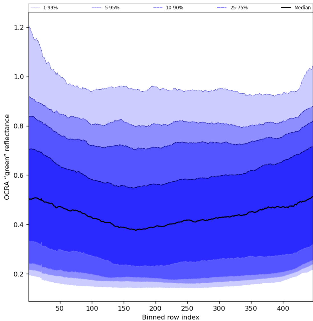
Figure 68: Along track statistics of “OCRA “green” reflectance” for 2023-07-21 to 2023-07-23
