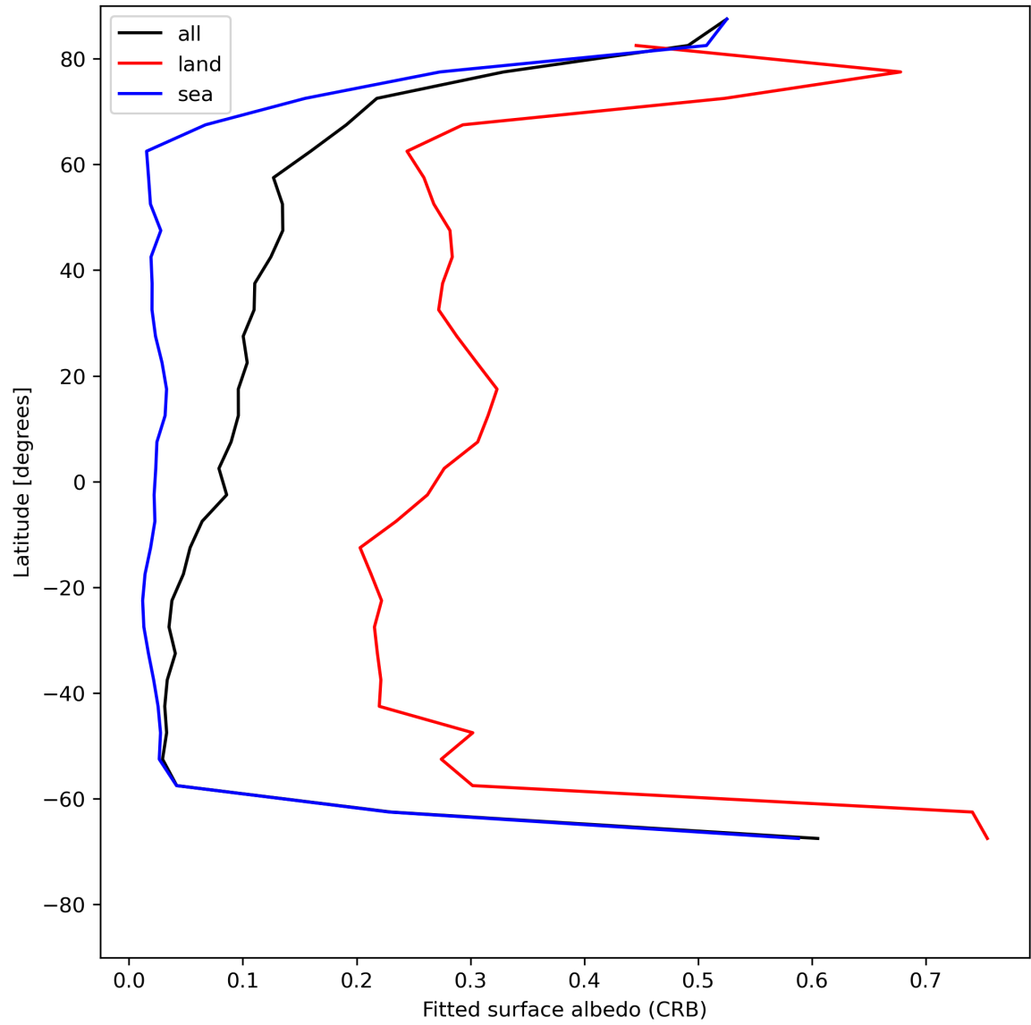
Figure 30: Zonal average of “Fitted surface albedo (CRB)” for 2023-07-21 to 2023-07-23.
