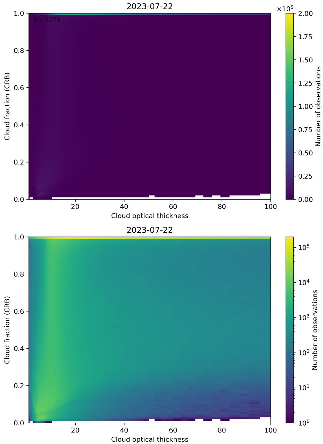
Figure 84: Scatter density plot of “Cloud optical thickness” against “Cloud fraction (CRB)” for 2023-07-21 to 2023-07-23.
