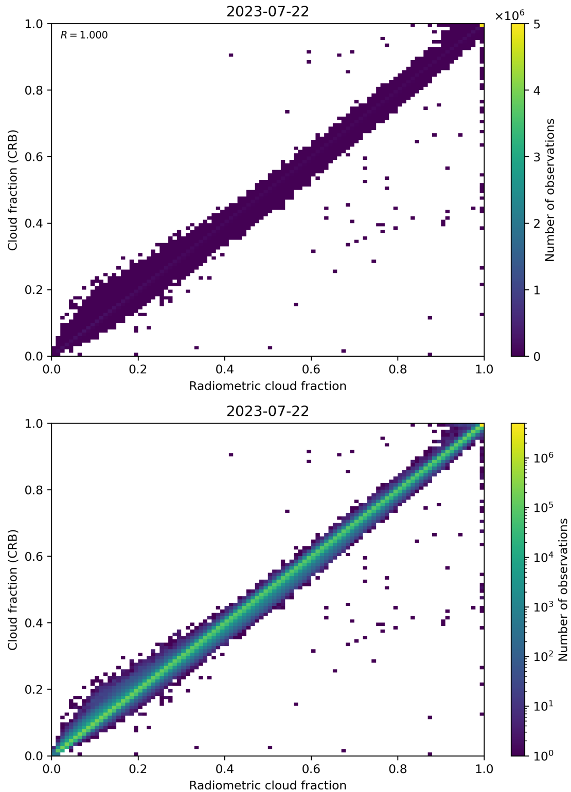
Figure 73: Scatter density plot of “Radiometric cloud fraction” against “Cloud fraction (CRB)” for 2023-07-21 to 2023-07-23.
