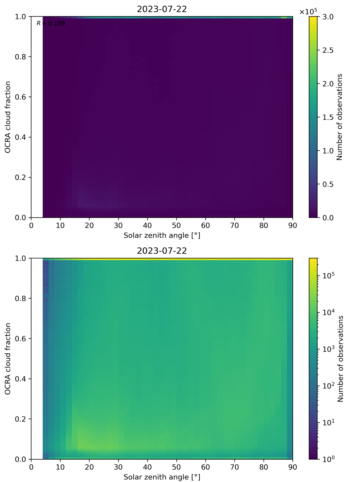
Figure 100: Scatter density plot of “Solar zenith angle” against “OCRA cloud fraction” for 2023-07-21 to 2023-07-23.
