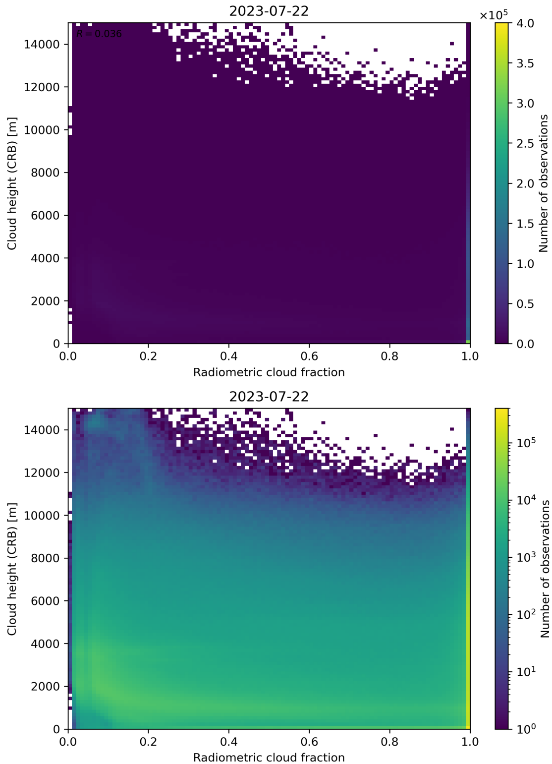
Figure 74: Scatter density plot of “Radiometric cloud fraction” against “Cloud height (CRB)” for 2023-07-21 to 2023-07-23.
