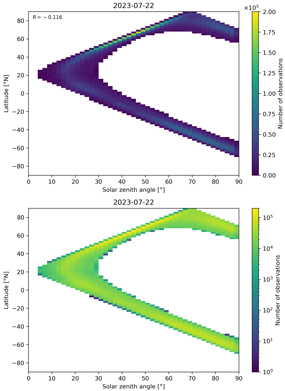
Figure 105: Scatter density plot of “Solar zenith angle” against “Latitude” for 2023-07-21 to 2023-07-23.
