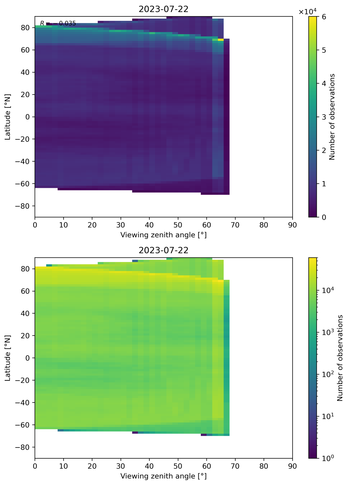
Figure 113: Scatter density plot of “Viewing zenith angle” against “Latitude” for 2023-07-21 to 2023-07-23.
