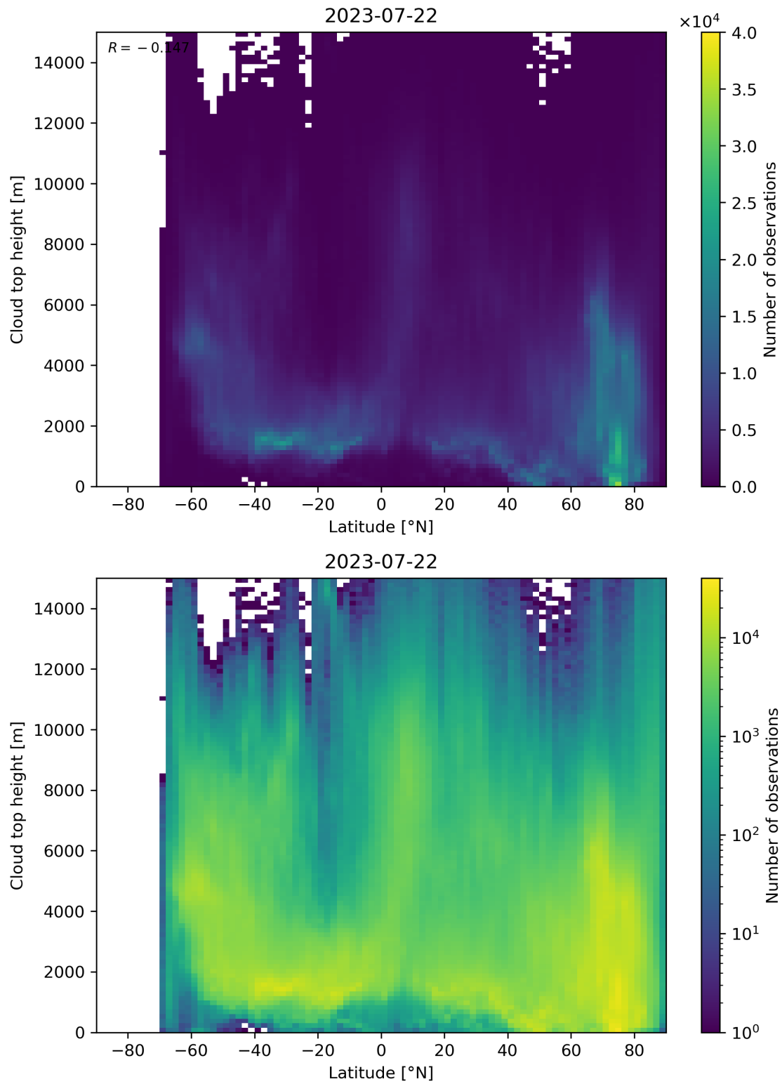
Figure 97: Scatter density plot of “Latitude” against “Cloud top height” for 2023-07-21 to 2023-07-23.
