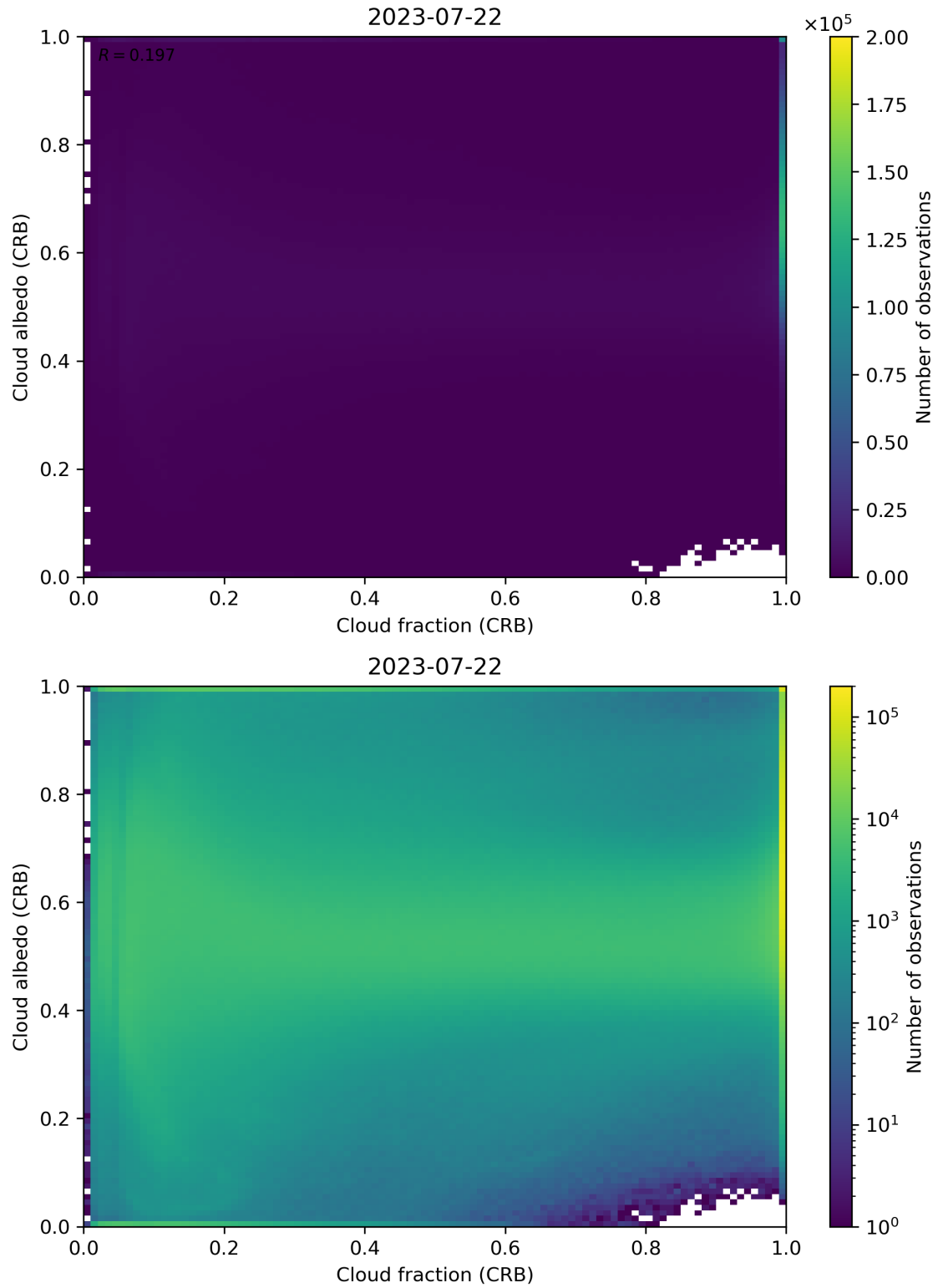
Figure 77: Scatter density plot of “Cloud fraction (CRB)” against “Cloud albedo (CRB)” for 2023-07-21 to 2023-07-23.
