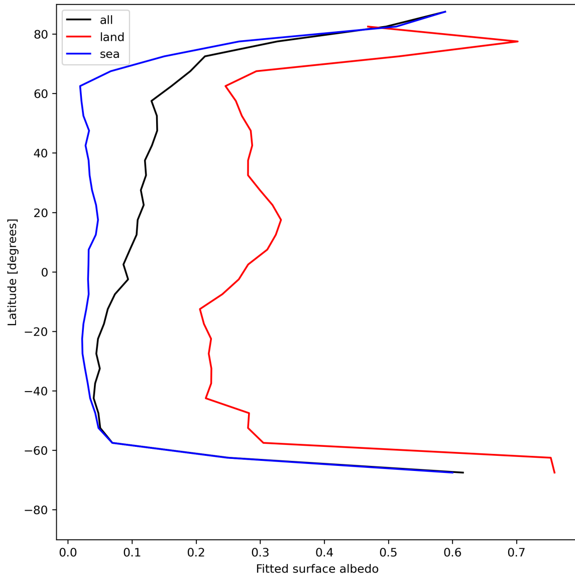
Figure 29: Zonal average of “Fitted surface albedo” for 2023-07-21 to 2023-07-23.
