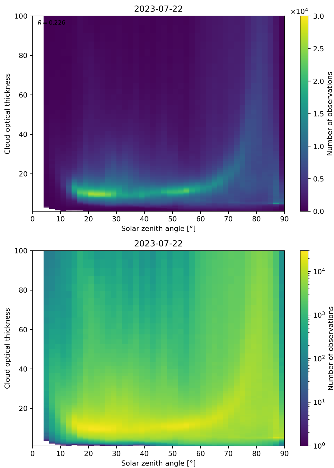
Figure 103: Scatter density plot of “Solar zenith angle” against “Cloud optical thickness” for 2023-07-21 to 2023-07-23.
