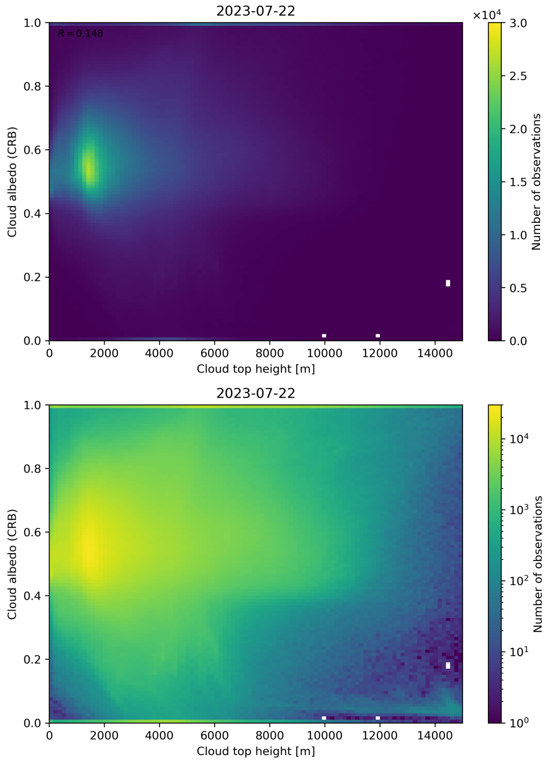
Figure 86: Scatter density plot of “Cloud top height” against “Cloud albedo (CRB)” for 2023-07-21 to 2023-07-23.
