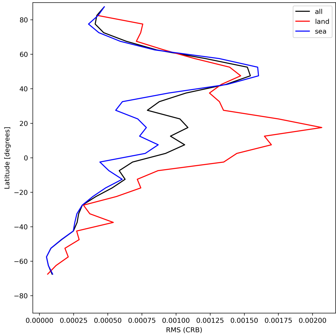
Figure 32: Zonal average of “RMS (CRB)” for 2023-07-21 to 2023-07-23.
