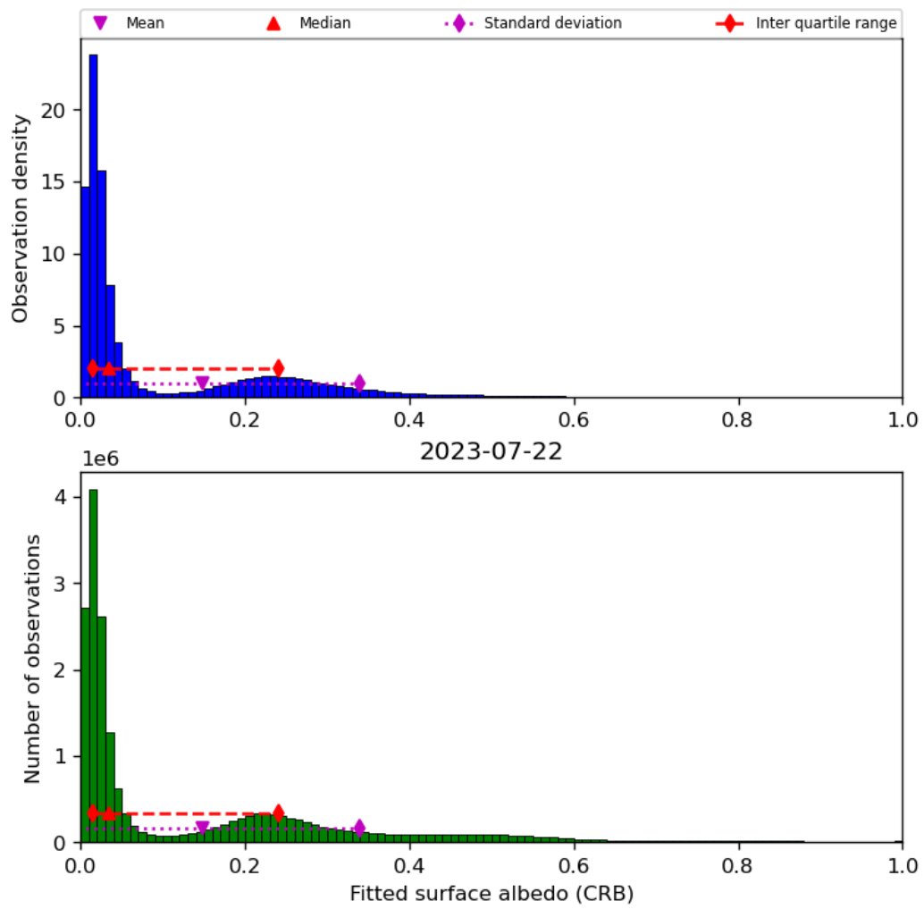
Figure 46: Histogram of “Fitted surface albedo (CRB)” for 2023-07-21 to 2023-07-23
