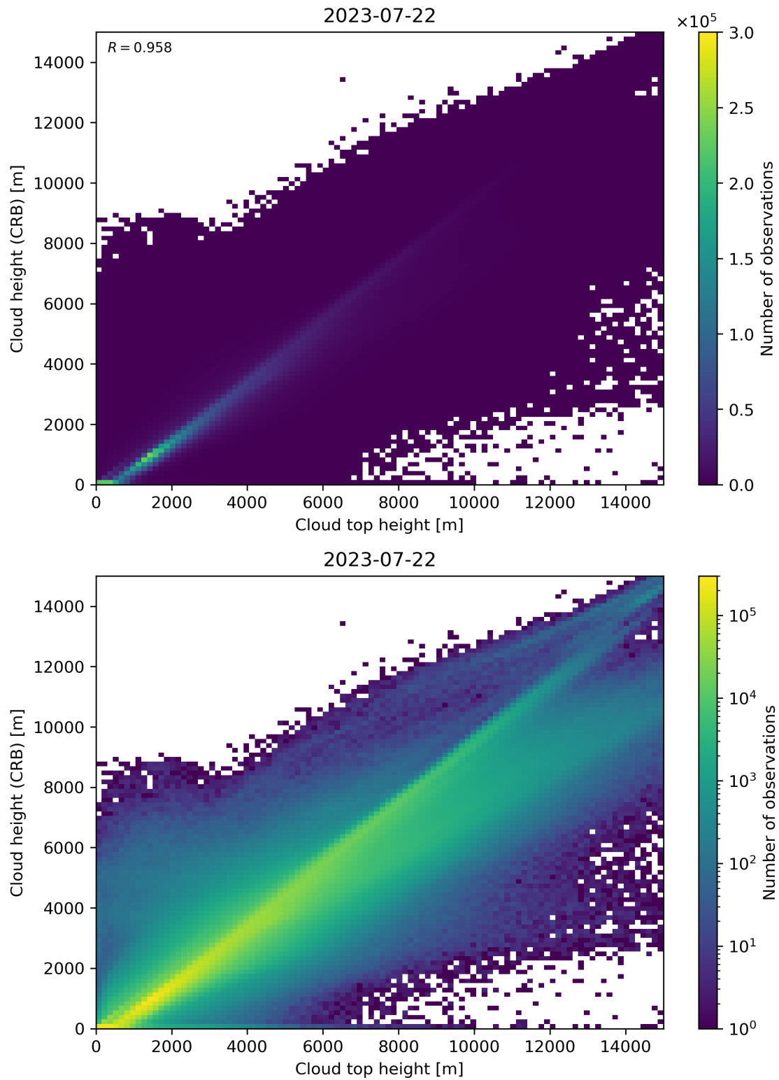
Figure 89: Scatter density plot of “Cloud top height” against “Cloud height (CRB)” for 2023-07-21 to 2023-07-23.
