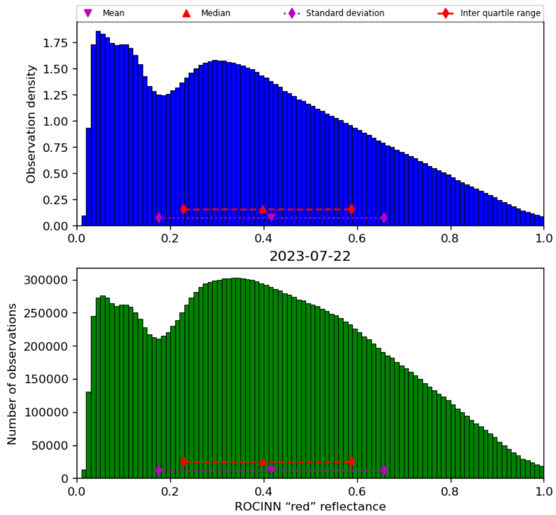
Figure 53: Histogram of “ROCINN “red” reflectance” for 2023-07-21 to 2023-07-23
