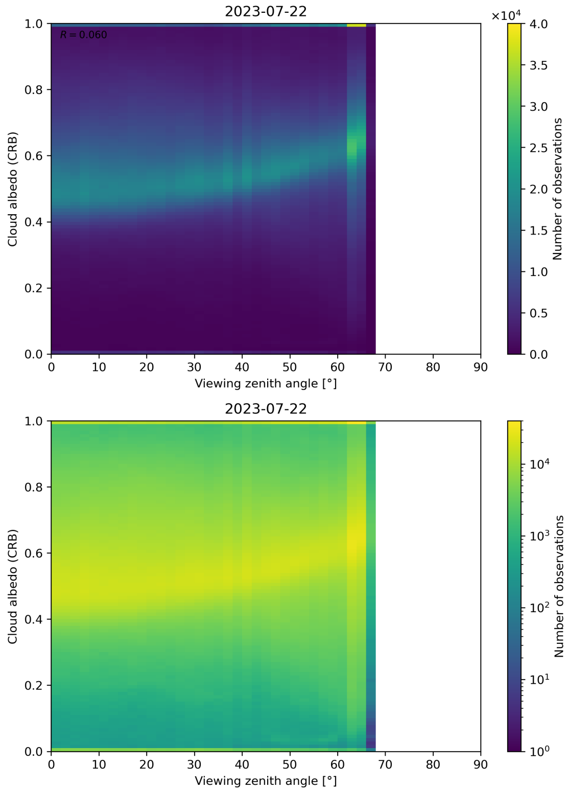
Figure 106: Scatter density plot of “Viewing zenith angle” against “Cloud albedo (CRB)” for 2023-07-21 to 2023-07-23.
