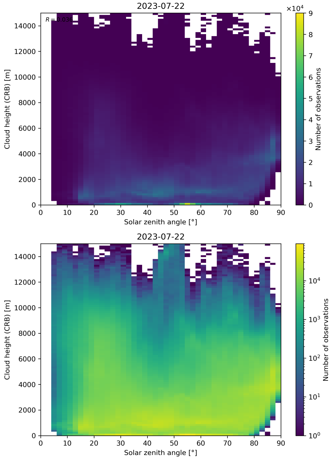
Figure 102: Scatter density plot of “Solar zenith angle” against “Cloud height (CRB)” for 2023-07-21 to 2023-07-23.
