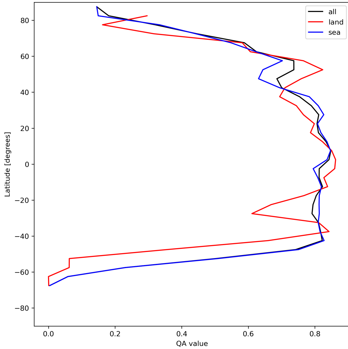
Figure 22: Zonal average of “QA value” for 2023-07-21 to 2023-07-23.
