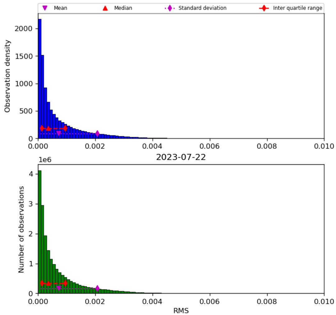
Figure 47: Histogram of “RMS” for 2023-07-21 to 2023-07-23
