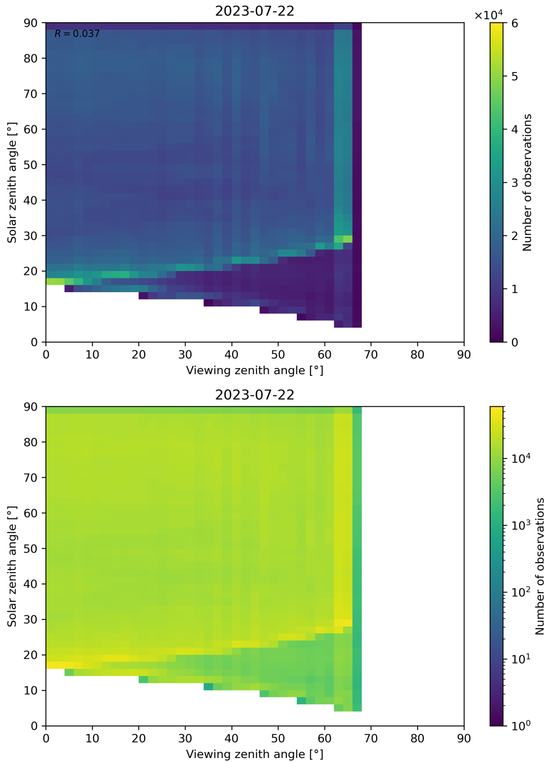
Figure 114: Scatter density plot of “Viewing zenith angle” against “Solar zenith angle” for 2023-07-21 to 2023-07-23.
