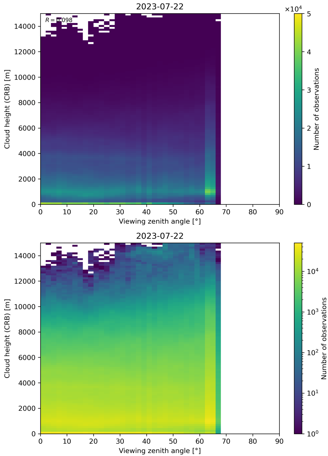
Figure 110: Scatter density plot of “Viewing zenith angle” against “Cloud height (CRB)” for 2023-07-21 to 2023-07-23.
