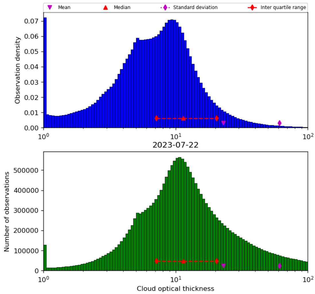
Figure 41: Histogram of “Cloud optical thickness” for 2023-07-21 to 2023-07-23
