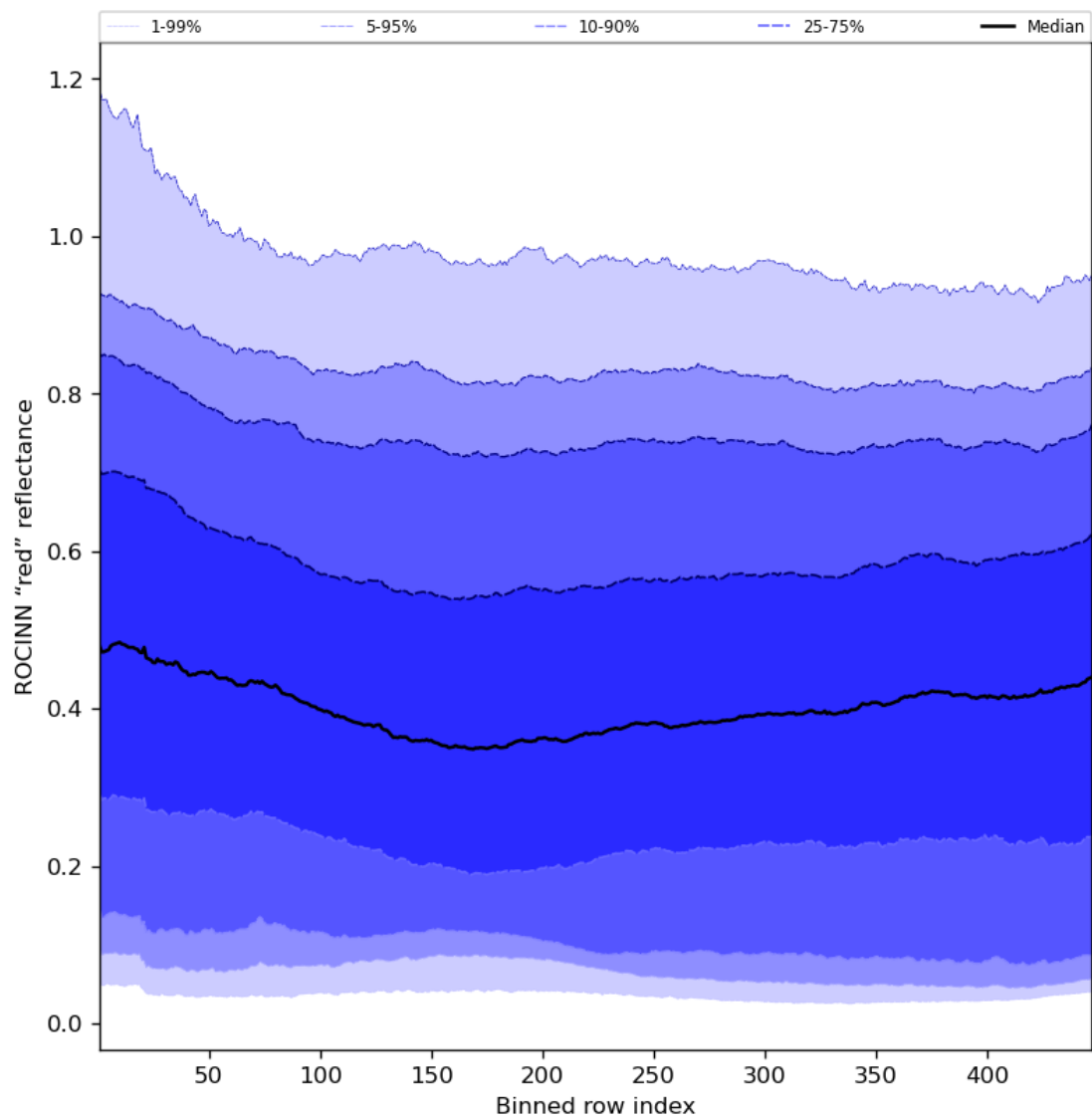
Figure 69: Along track statistics of “ROCINN “red” reflectance” for 2023-07-21 to 2023-07-23
