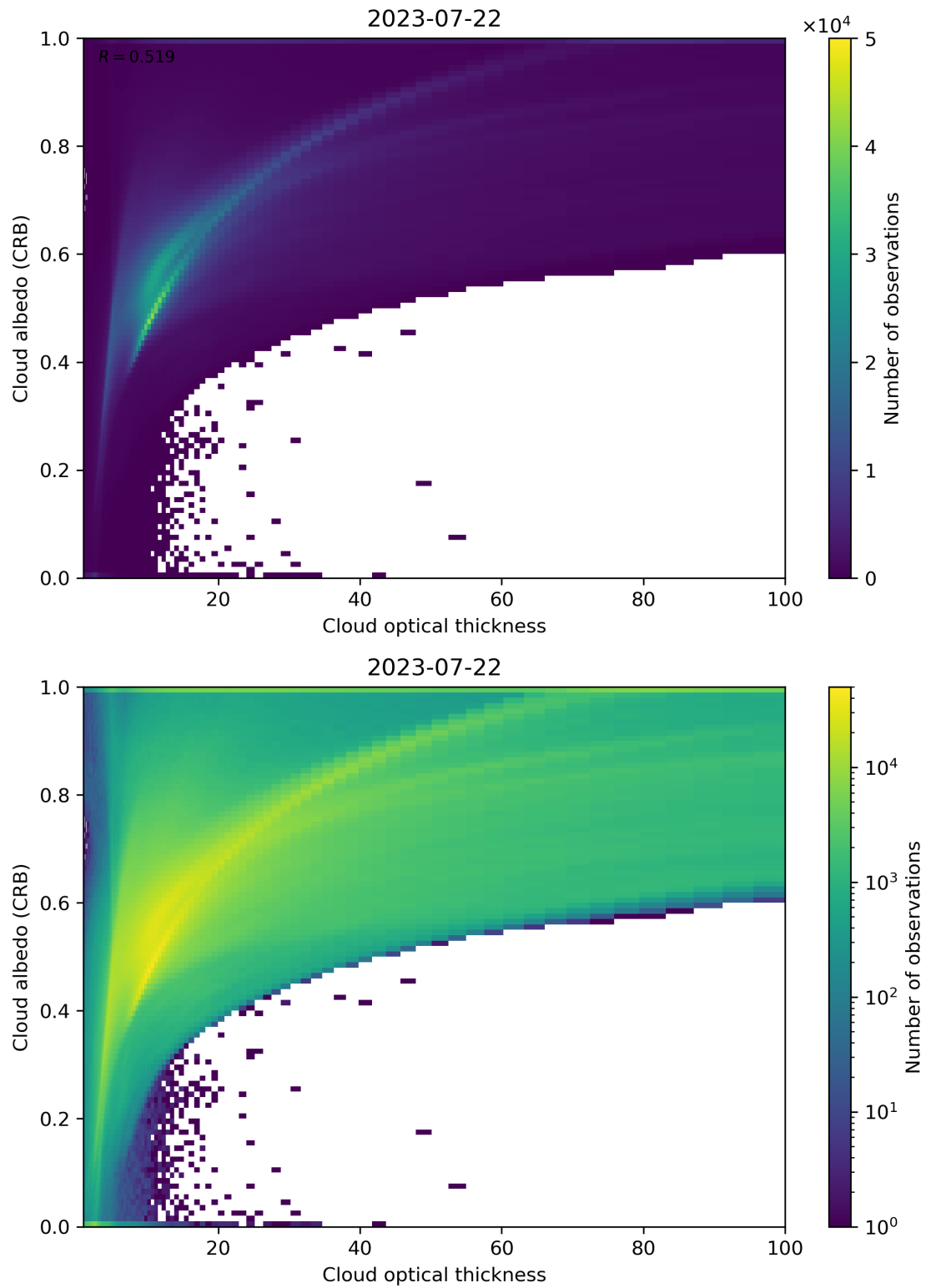
Figure 82: Scatter density plot of “Cloud optical thickness” against “Cloud albedo (CRB)” for 2023-07-21 to 2023-07-23.
