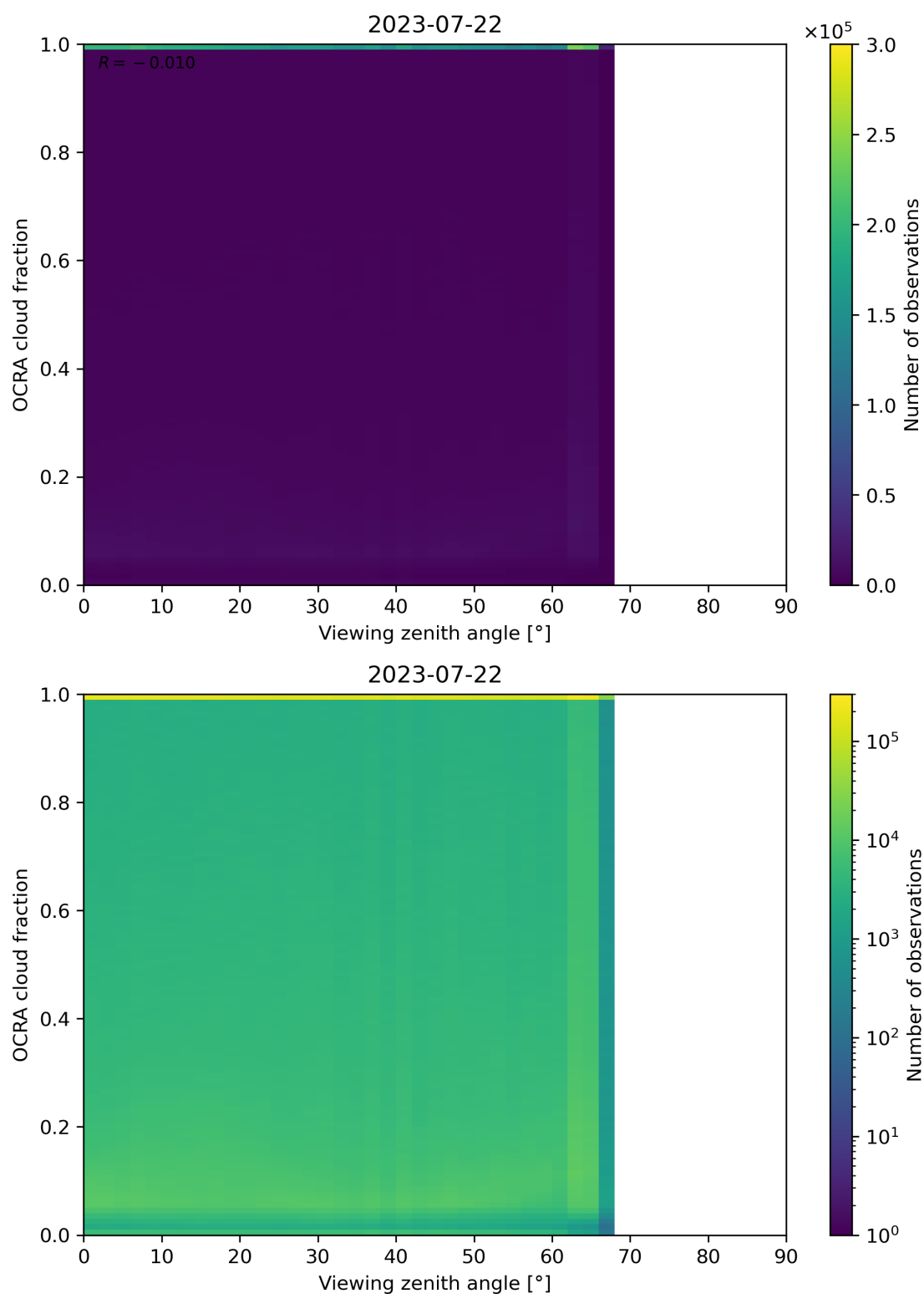
Figure 108: Scatter density plot of “Viewing zenith angle” against “OCRA cloud fraction” for 2023-07-21 to 2023-07-23.
