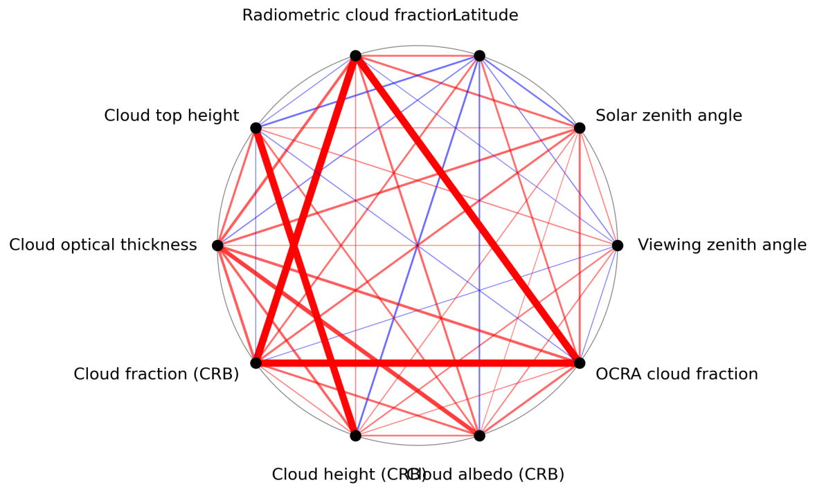
Figure 1: Map of correlation graph for 2023-07-21 to 2023-07-23.
