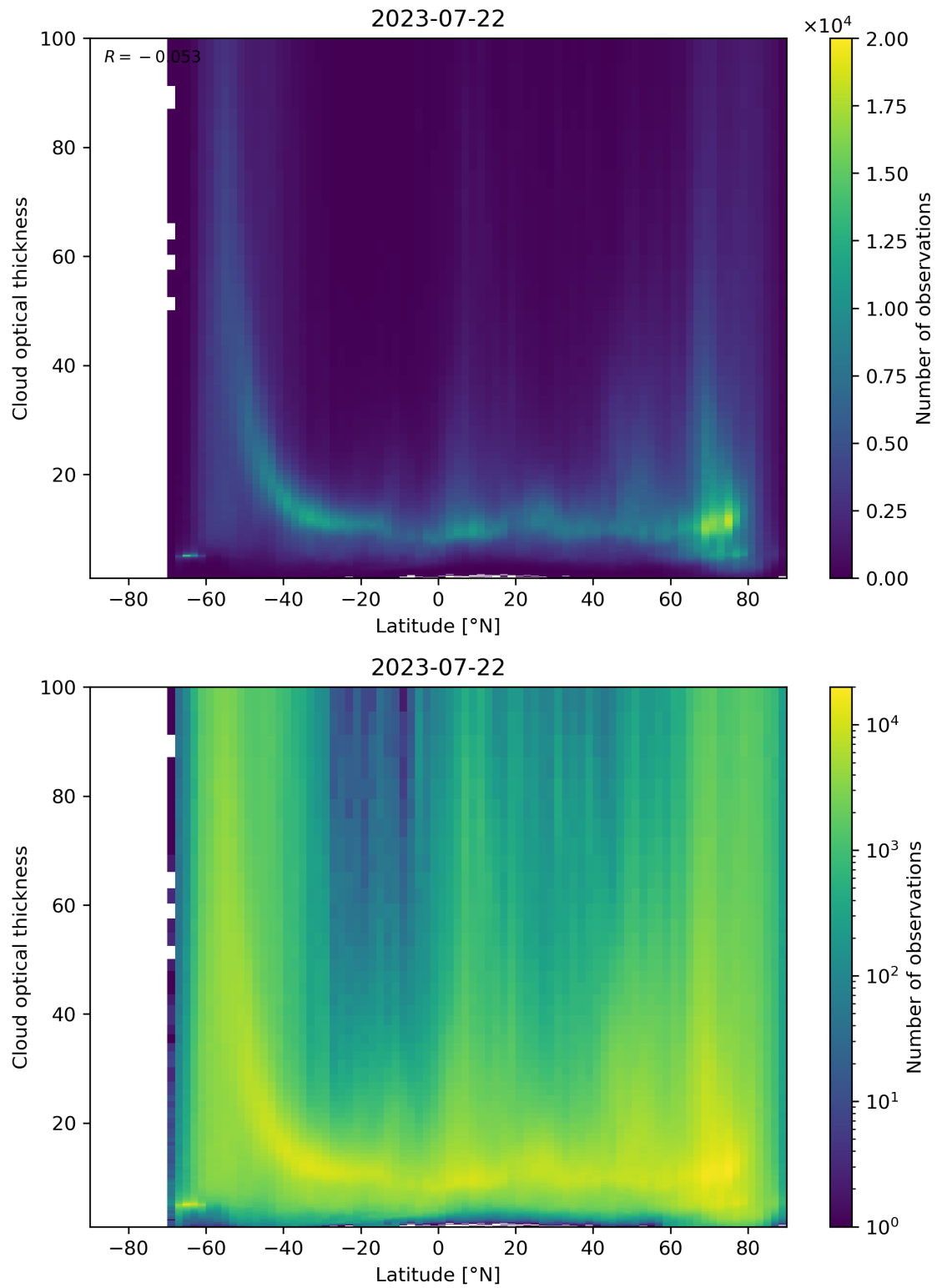
Figure 96: Scatter density plot of “Latitude” against “Cloud optical thickness” for 2023-07-21 to 2023-07-23.
