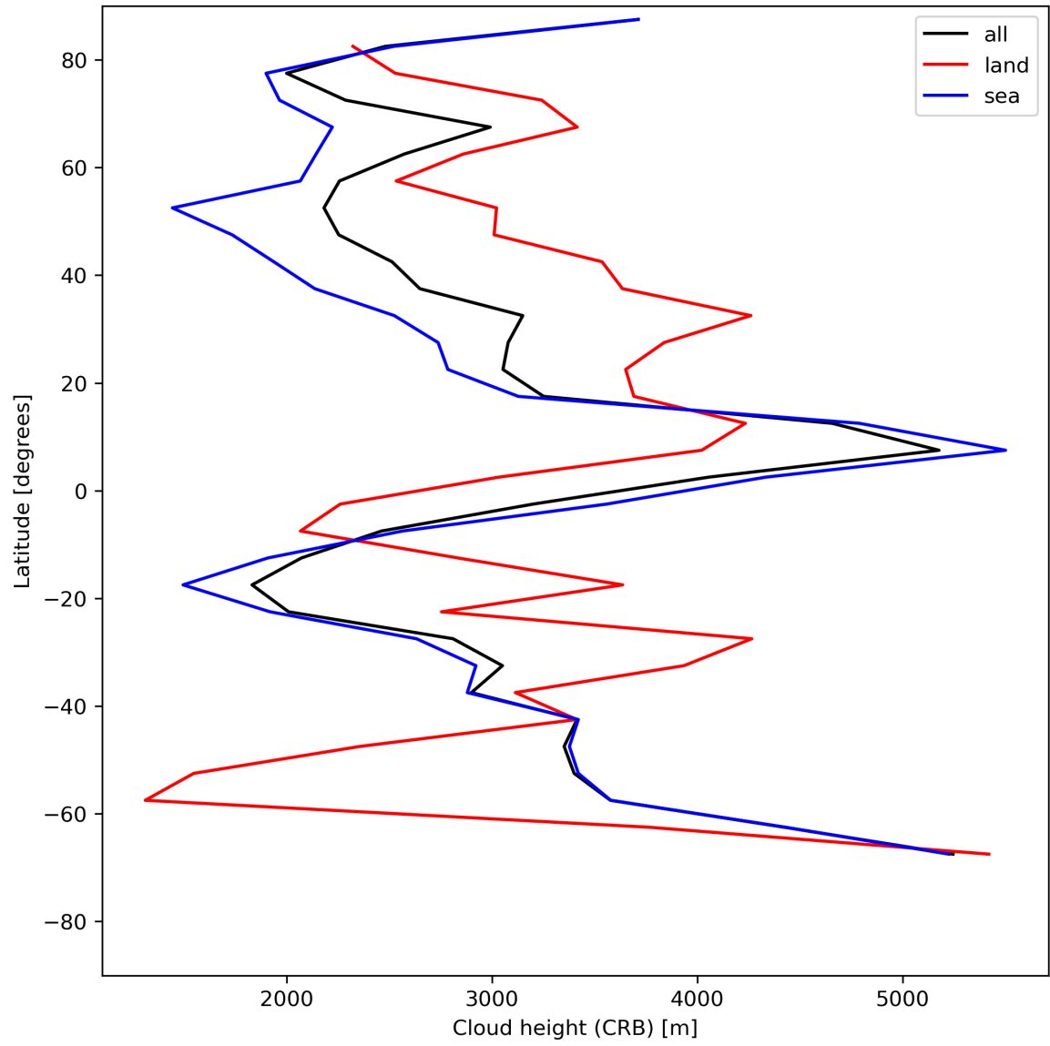
Figure 27: Zonal average of “Cloud height (CRB)” for 2023-07-21 to 2023-07-23.
