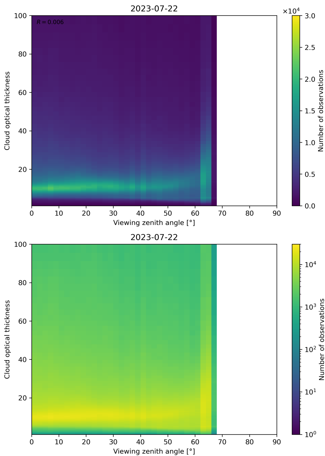
Figure 111: Scatter density plot of “Viewing zenith angle” against “Cloud optical thickness” for 2023-07-21 to 2023-07-23.
