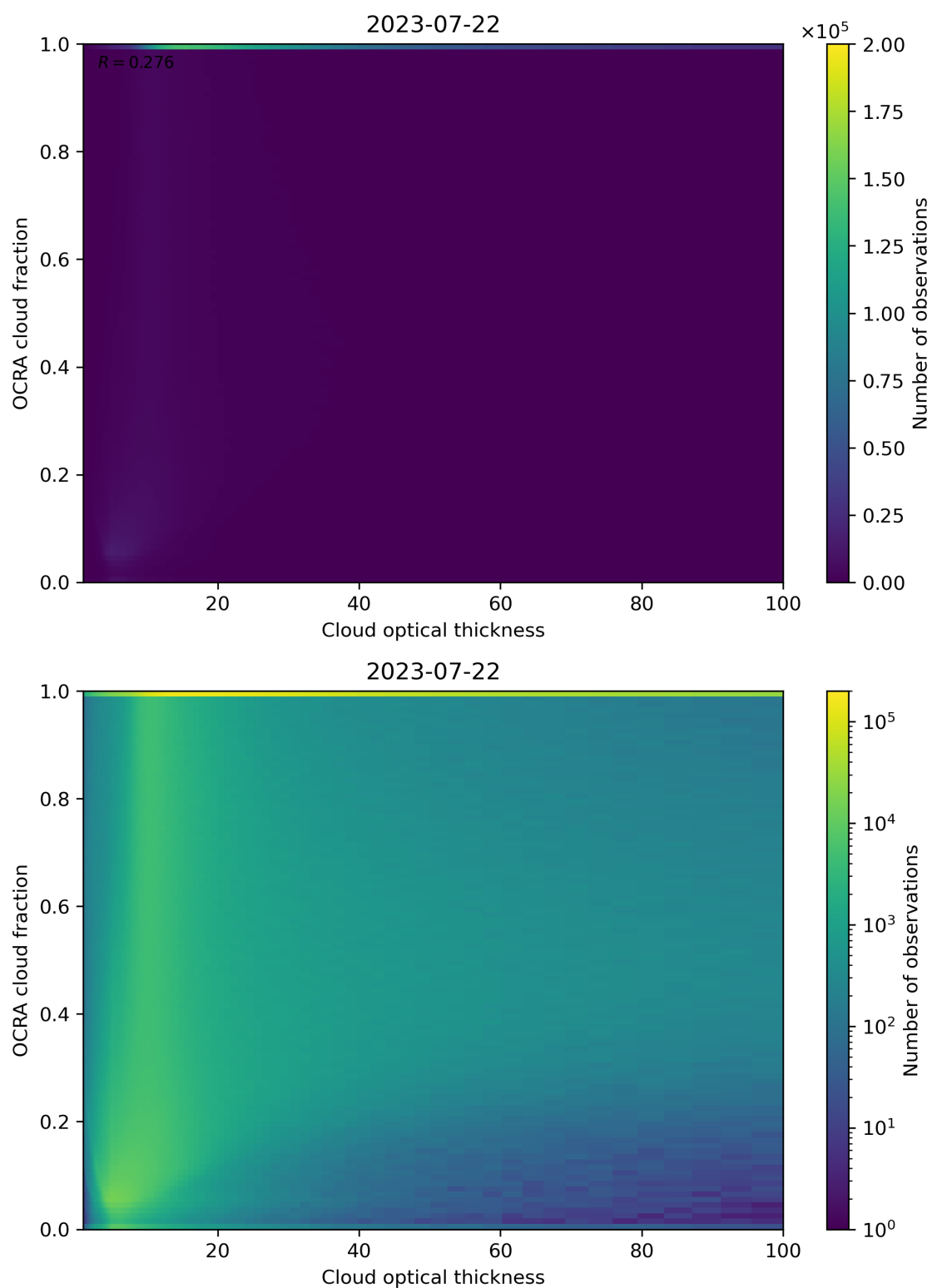
Figure 83: Scatter density plot of “Cloud optical thickness” against “OCRA cloud fraction” for 2023-07-21 to 2023-07-23.
