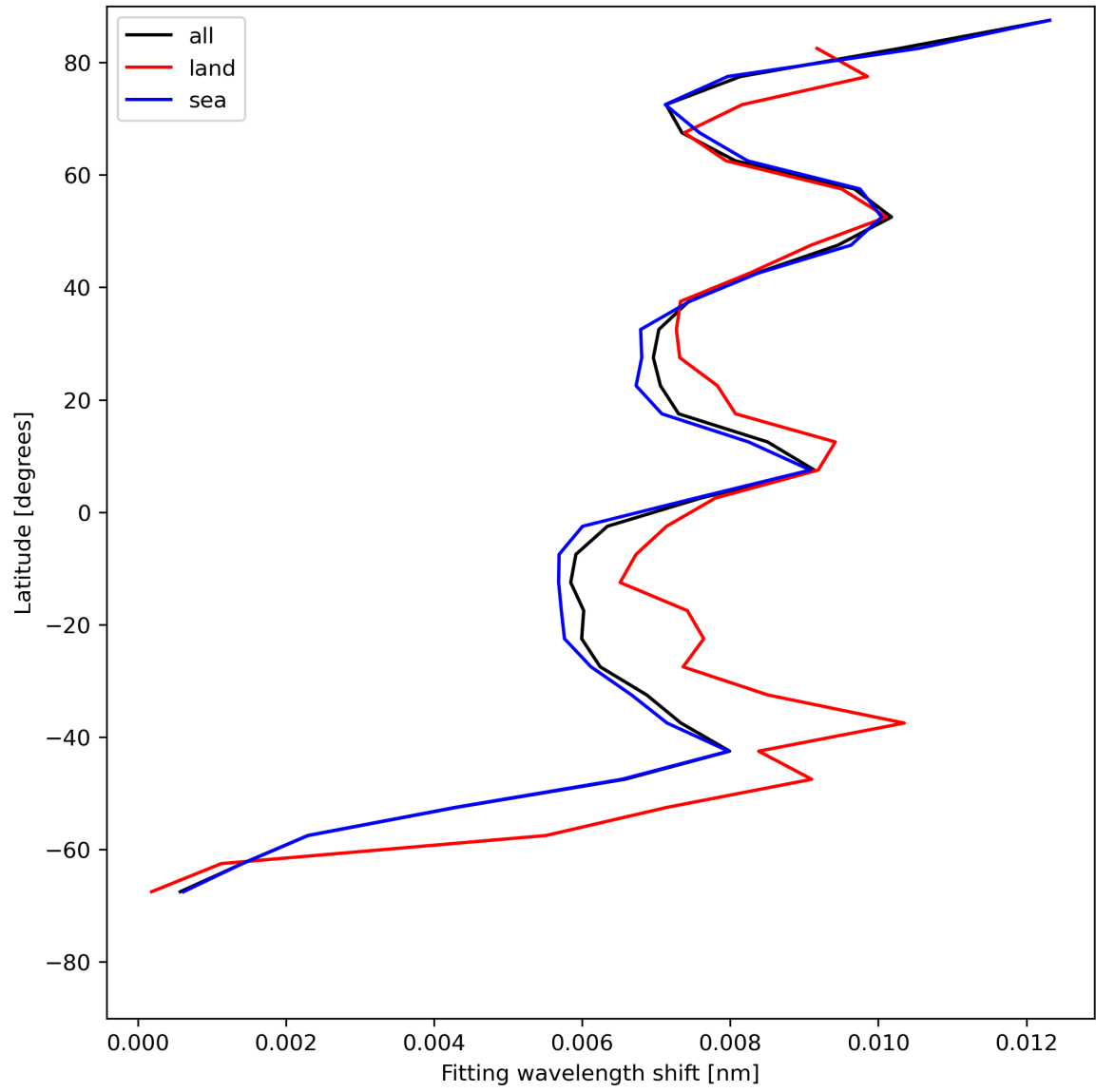
Figure 33: Zonal average of “Fitting wavelength shift” for 2023-07-21 to 2023-07-23.
