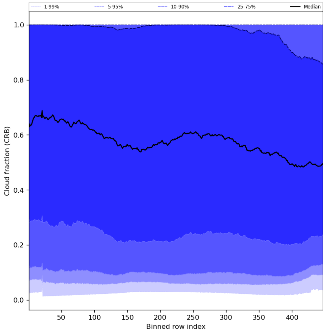
Figure 58: Along track statistics of “Cloud fraction (CRB)” for 2023-07-21 to 2023-07-23
