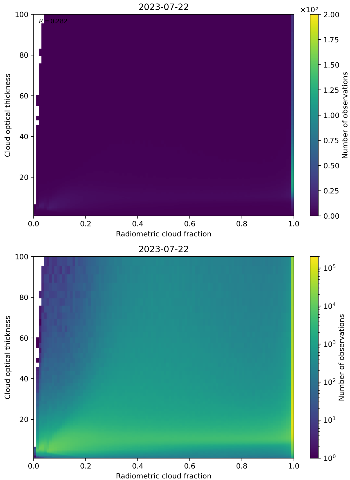
Figure 75: Scatter density plot of “Radiometric cloud fraction” against “Cloud optical thickness” for 2023-07-21 to 2023-07-23.
