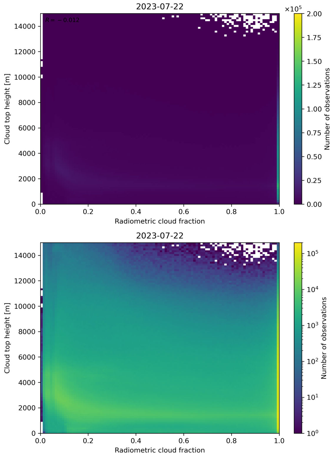
Figure 76: Scatter density plot of “Radiometric cloud fraction” against “Cloud top height” for 2023-07-21 to 2023-07-23.
