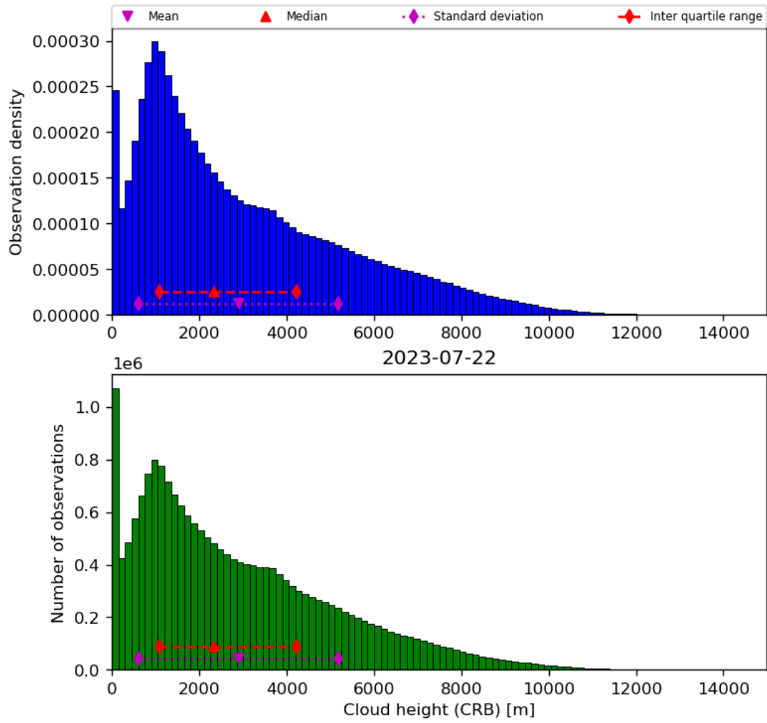
Figure 43: Histogram of “Cloud height (CRB)” for 2023-07-21 to 2023-07-23
