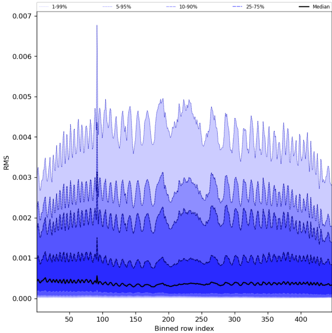
Figure 63: Along track statistics of “RMS” for 2023-07-21 to 2023-07-23
