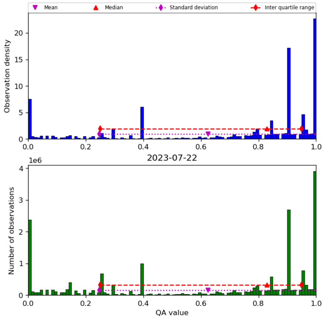
Figure 38: Histogram of “QA value” for 2023-07-21 to 2023-07-23
