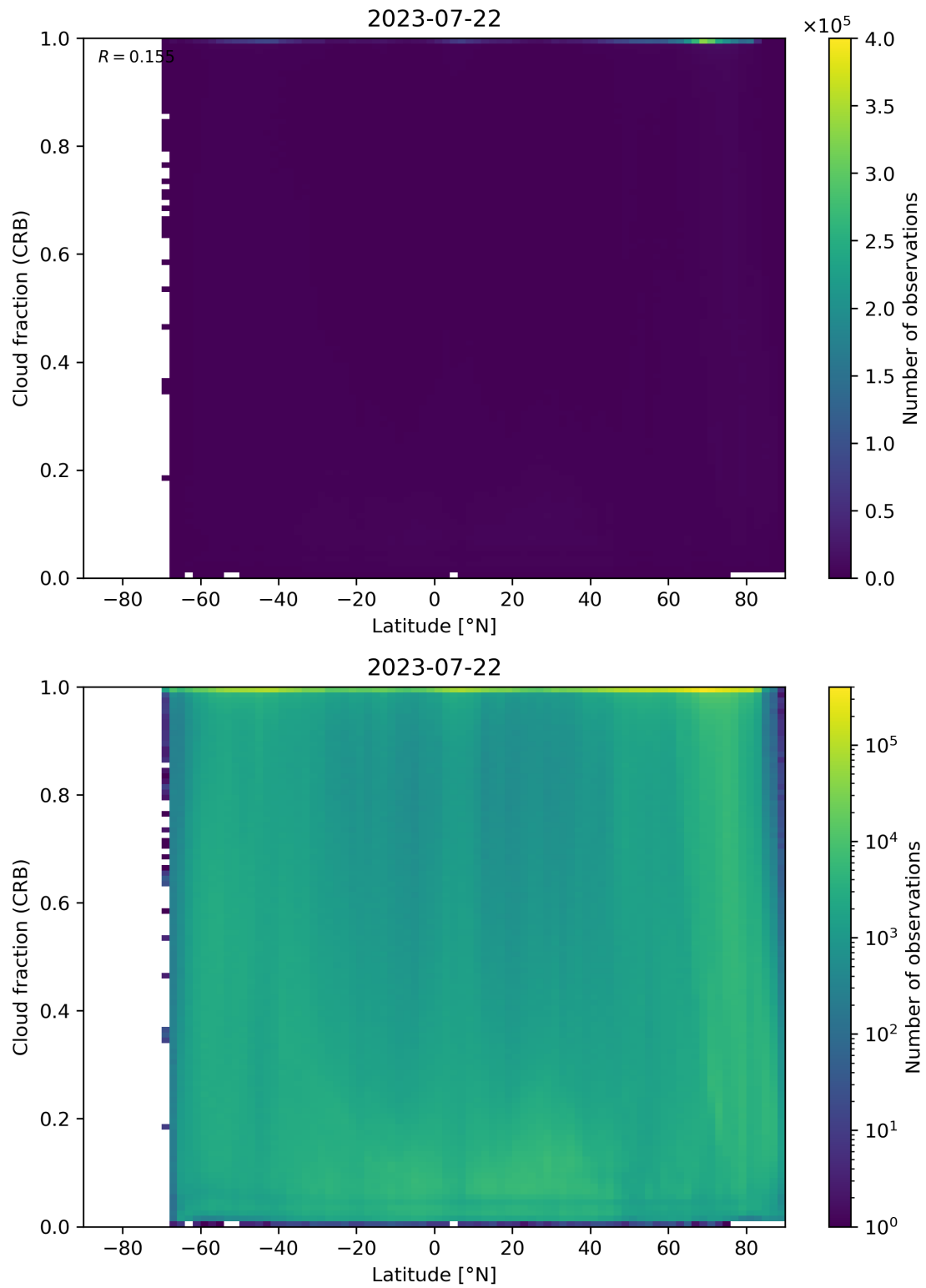
Figure 94: Scatter density plot of “Latitude” against “Cloud fraction (CRB)” for 2023-07-21 to 2023-07-23.
