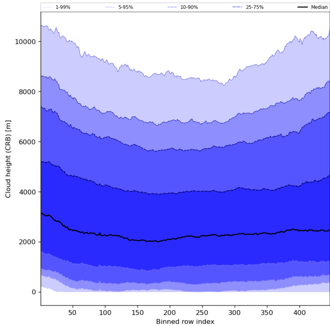
Figure 59: Along track statistics of “Cloud height (CRB)” for 2023-07-21 to 2023-07-23
