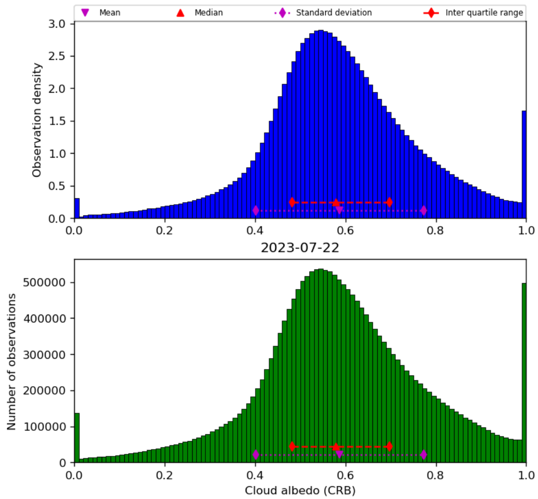
Figure 44: Histogram of “Cloud albedo (CRB)” for 2023-07-21 to 2023-07-23
