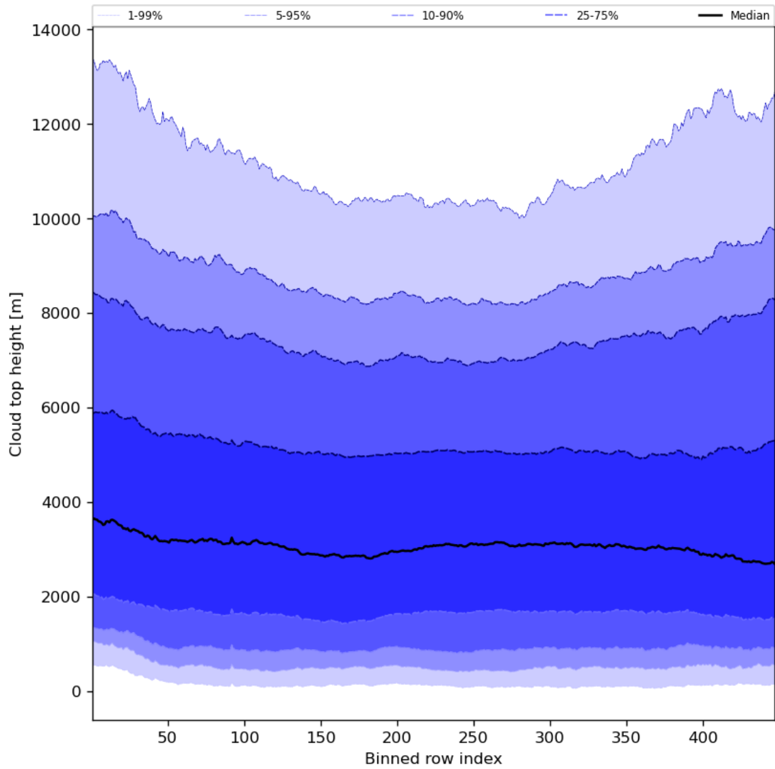
Figure 56: Along track statistics of “Cloud top height” for 2023-07-21 to 2023-07-23
