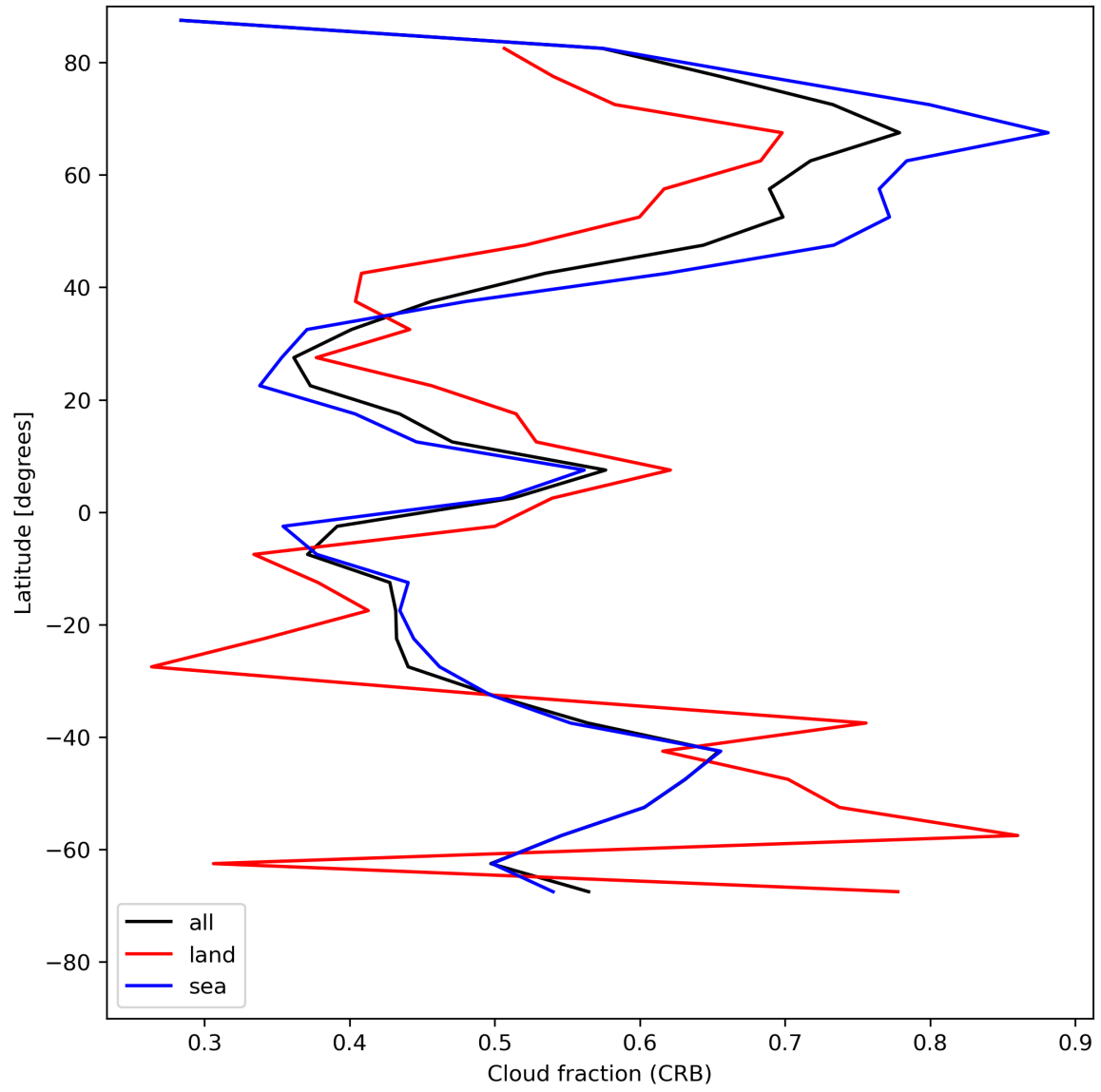
Figure 26: Zonal average of “Cloud fraction (CRB)” for 2023-07-21 to 2023-07-23.
