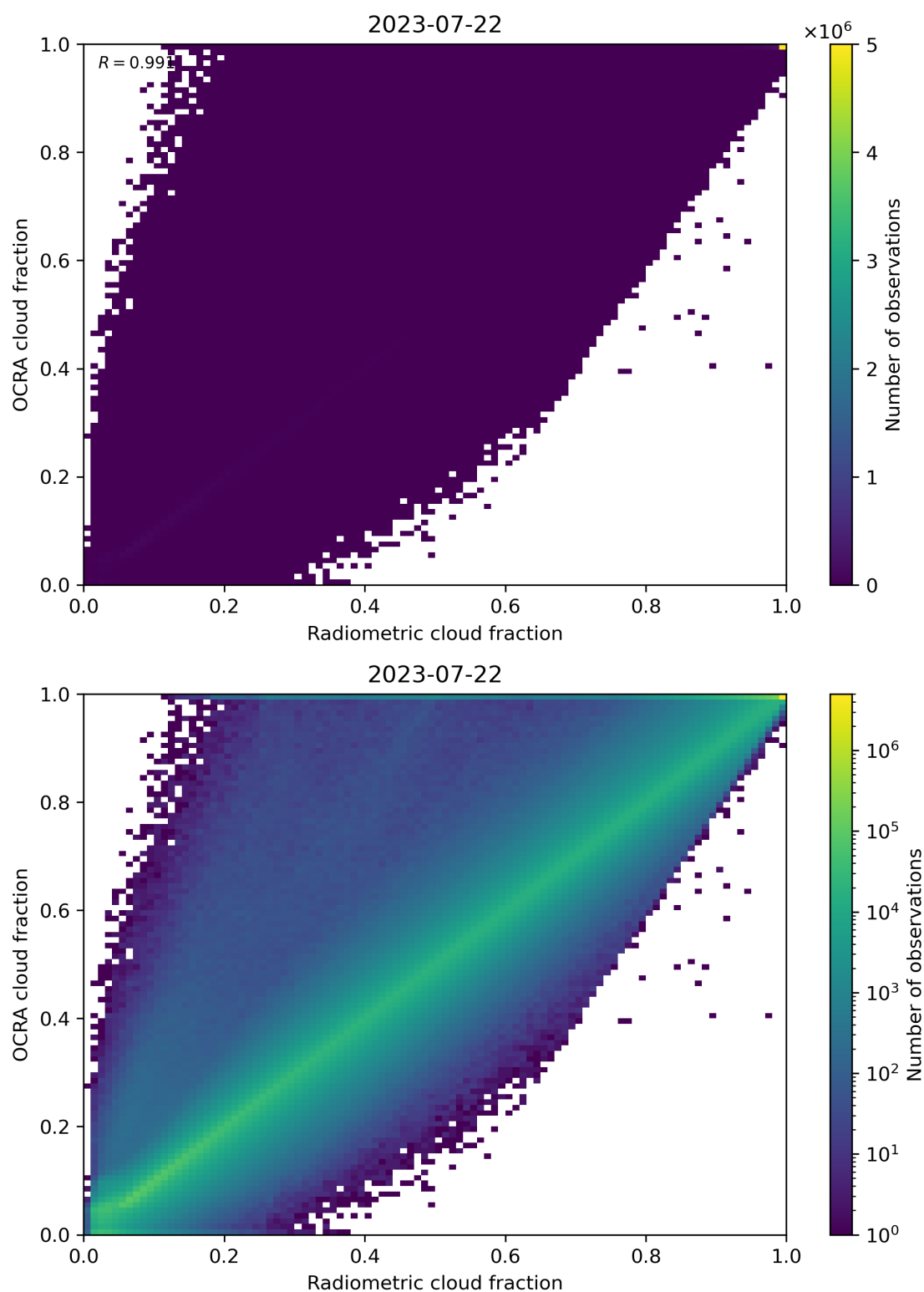
Figure 72: Scatter density plot of “Radiometric cloud fraction” against “OCRA cloud fraction” for 2023-07-21 to 2023-07-23.
