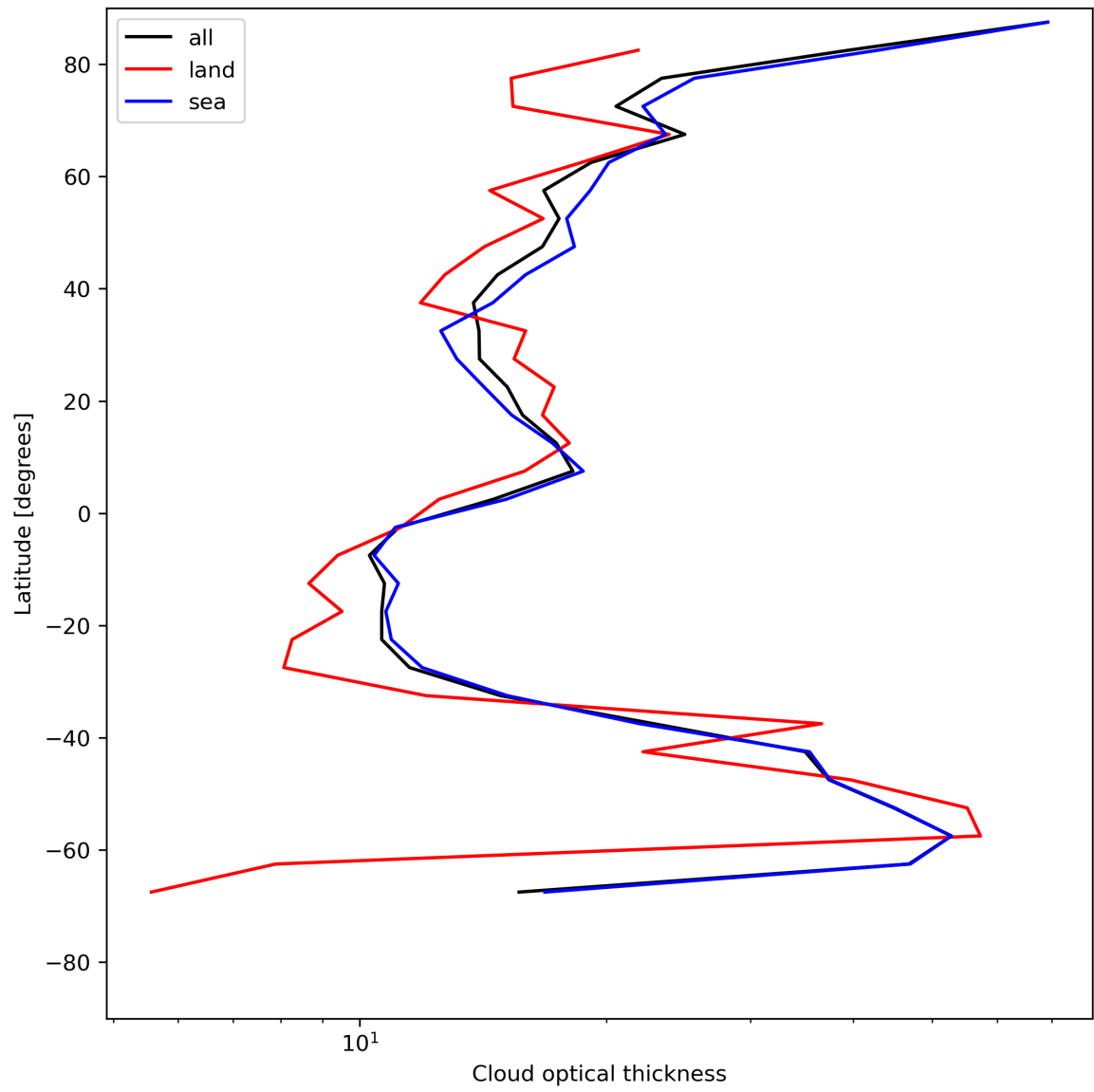
Figure 25: Zonal average of “Cloud optical thickness” for 2023-07-21 to 2023-07-23.
