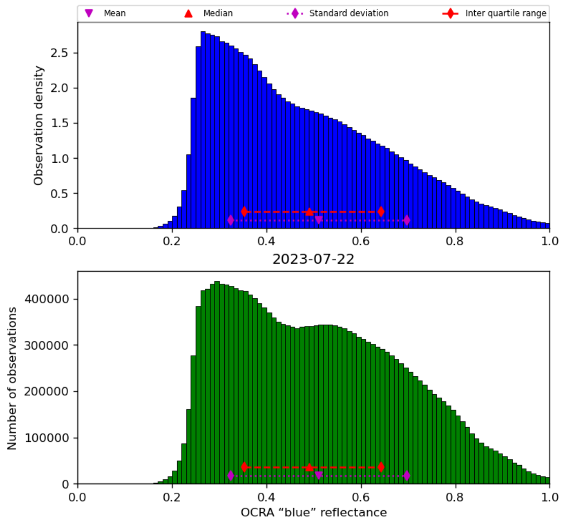
Figure 51: Histogram of “OCRA “blue” reflectance” for 2023-07-21 to 2023-07-23
