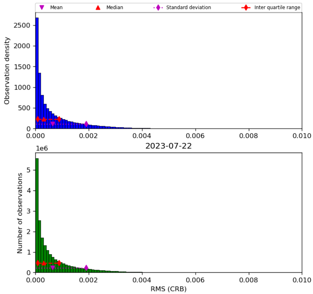
Figure 48: Histogram of “RMS (CRB)” for 2023-07-21 to 2023-07-23
