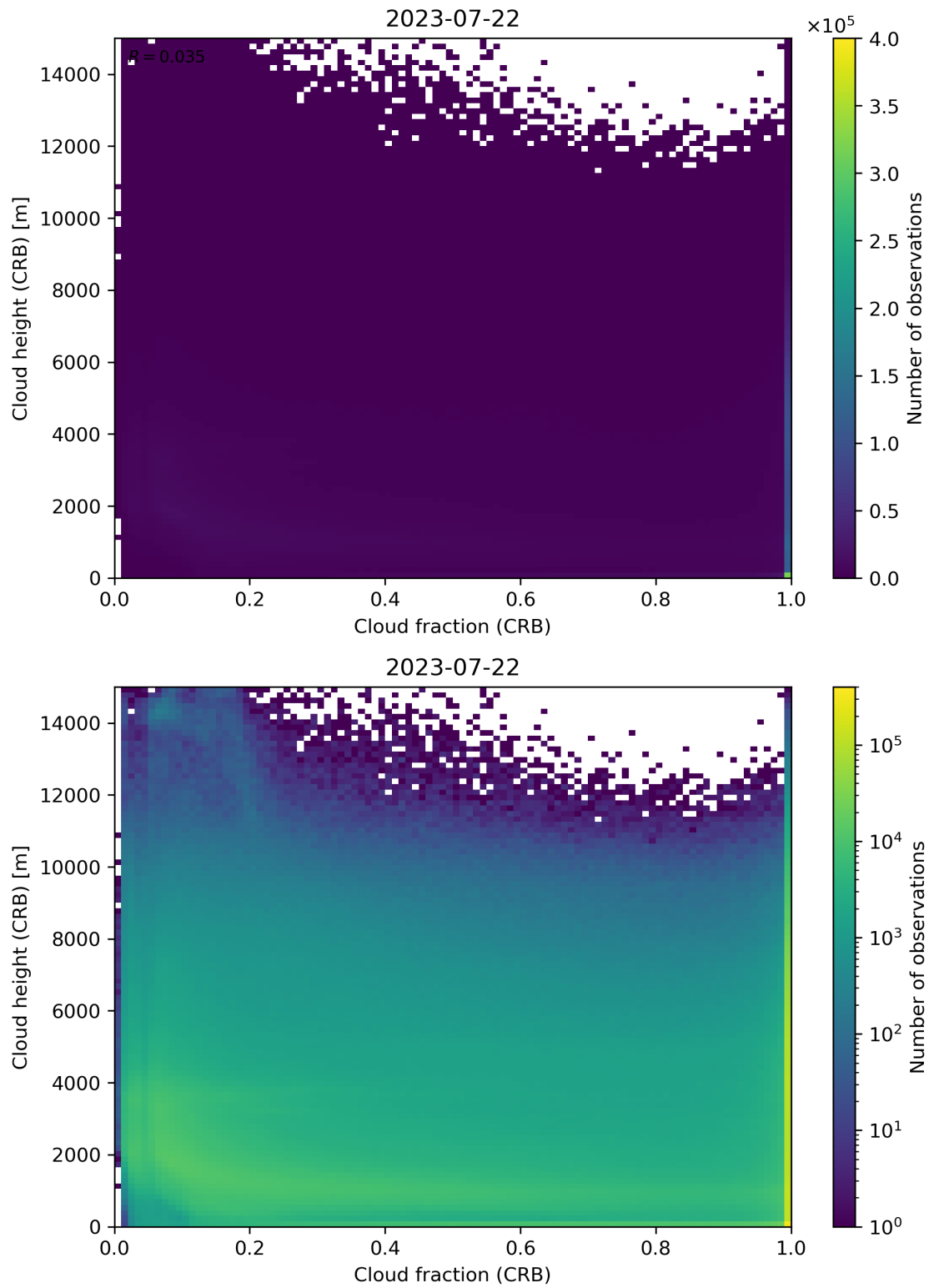
Figure 79: Scatter density plot of “Cloud fraction (CRB)” against “Cloud height (CRB)” for 2023-07-21 to 2023-07-23.
