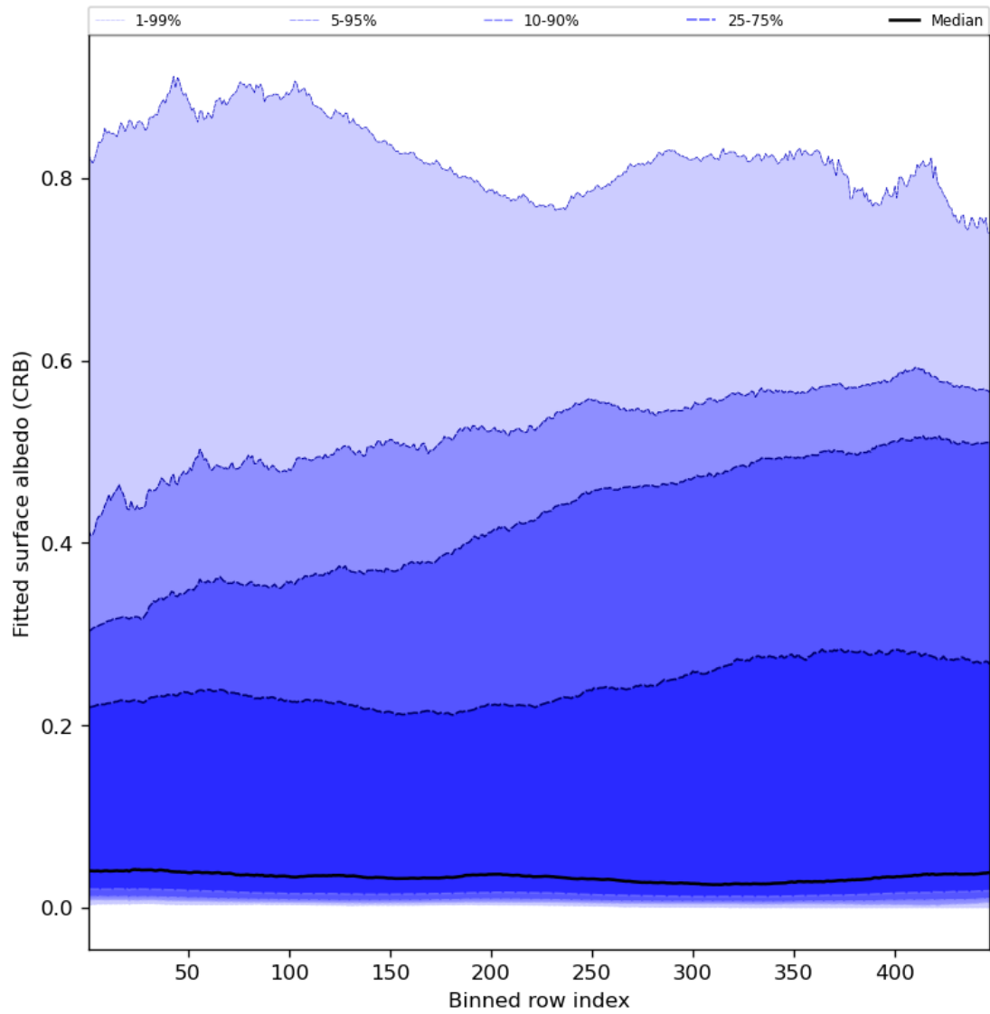
Figure 62: Along track statistics of “Fitted surface albedo (CRB)” for 2023-07-21 to 2023-07-23
