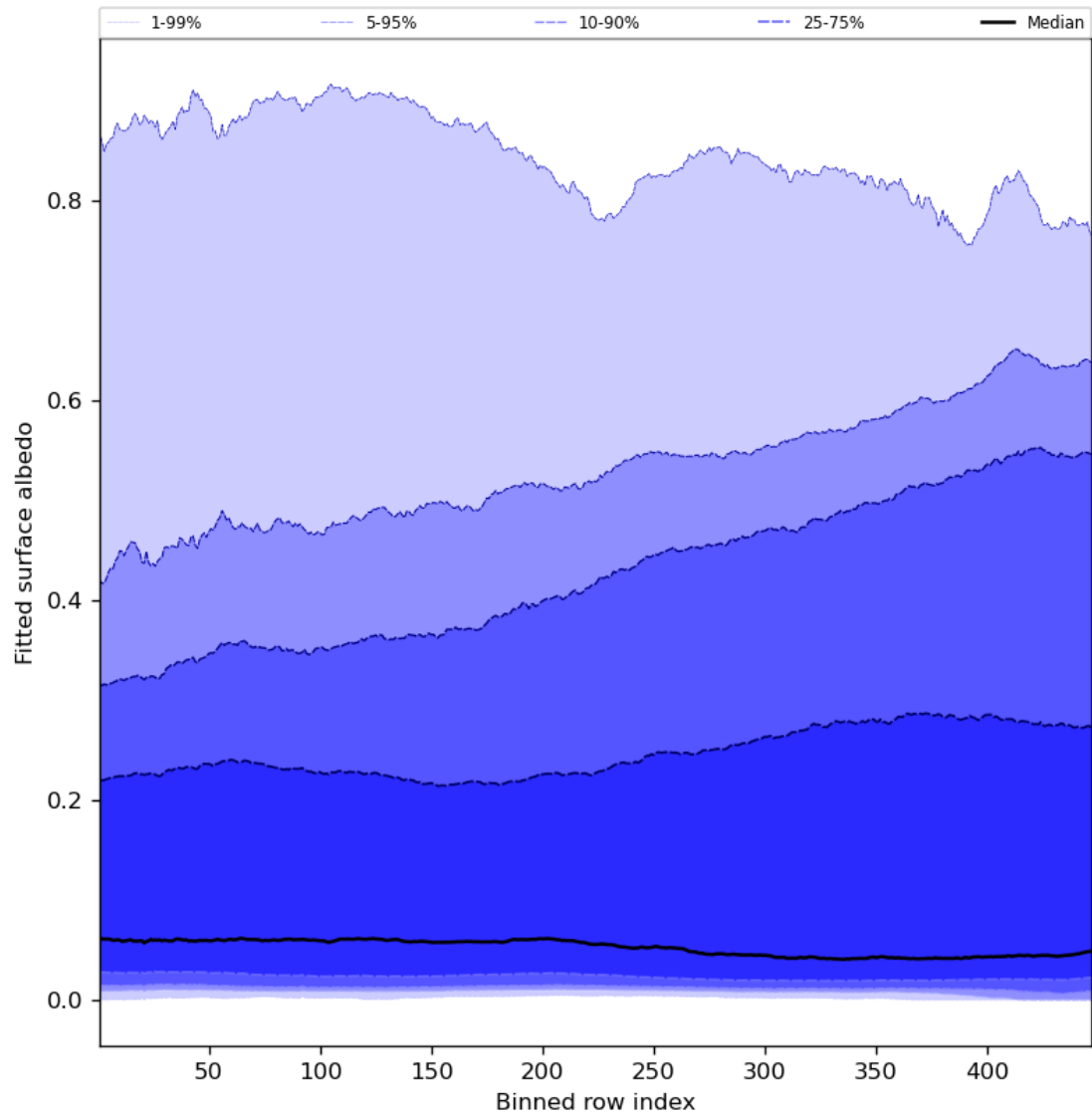
Figure 61: Along track statistics of “Fitted surface albedo” for 2023-07-21 to 2023-07-23
