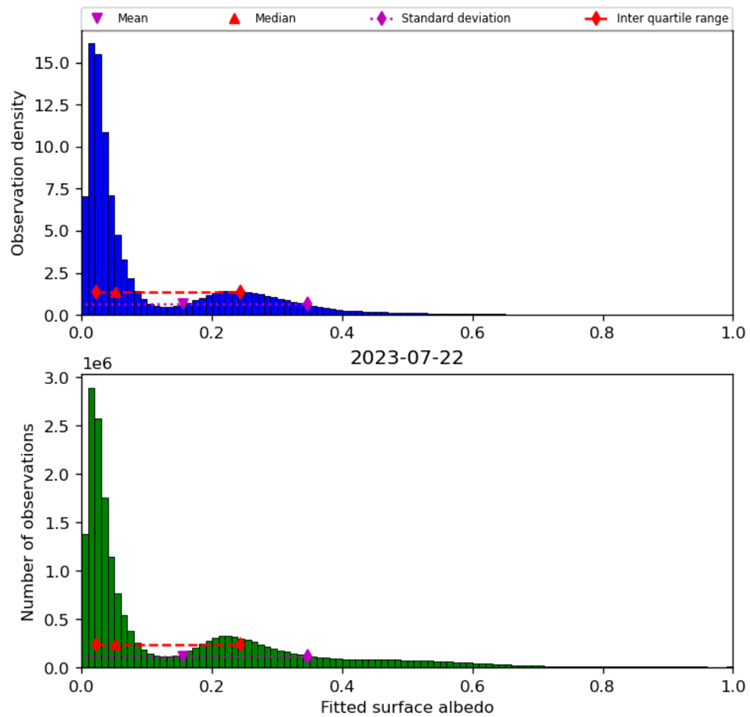
Figure 45: Histogram of “Fitted surface albedo” for 2023-07-21 to 2023-07-23
