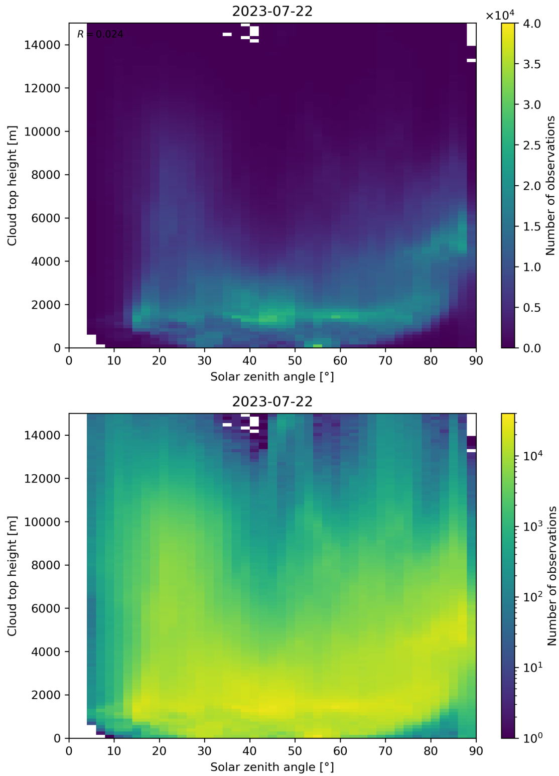
Figure 104: Scatter density plot of “Solar zenith angle” against “Cloud top height” for 2023-07-21 to 2023-07-23.
