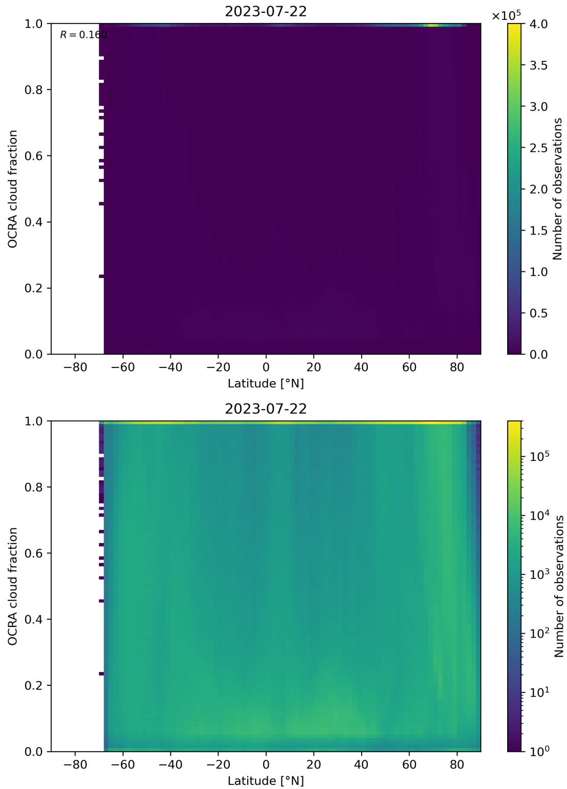
Figure 93: Scatter density plot of “Latitude” against “OCRA cloud fraction” for 2023-07-21 to 2023-07-23.
