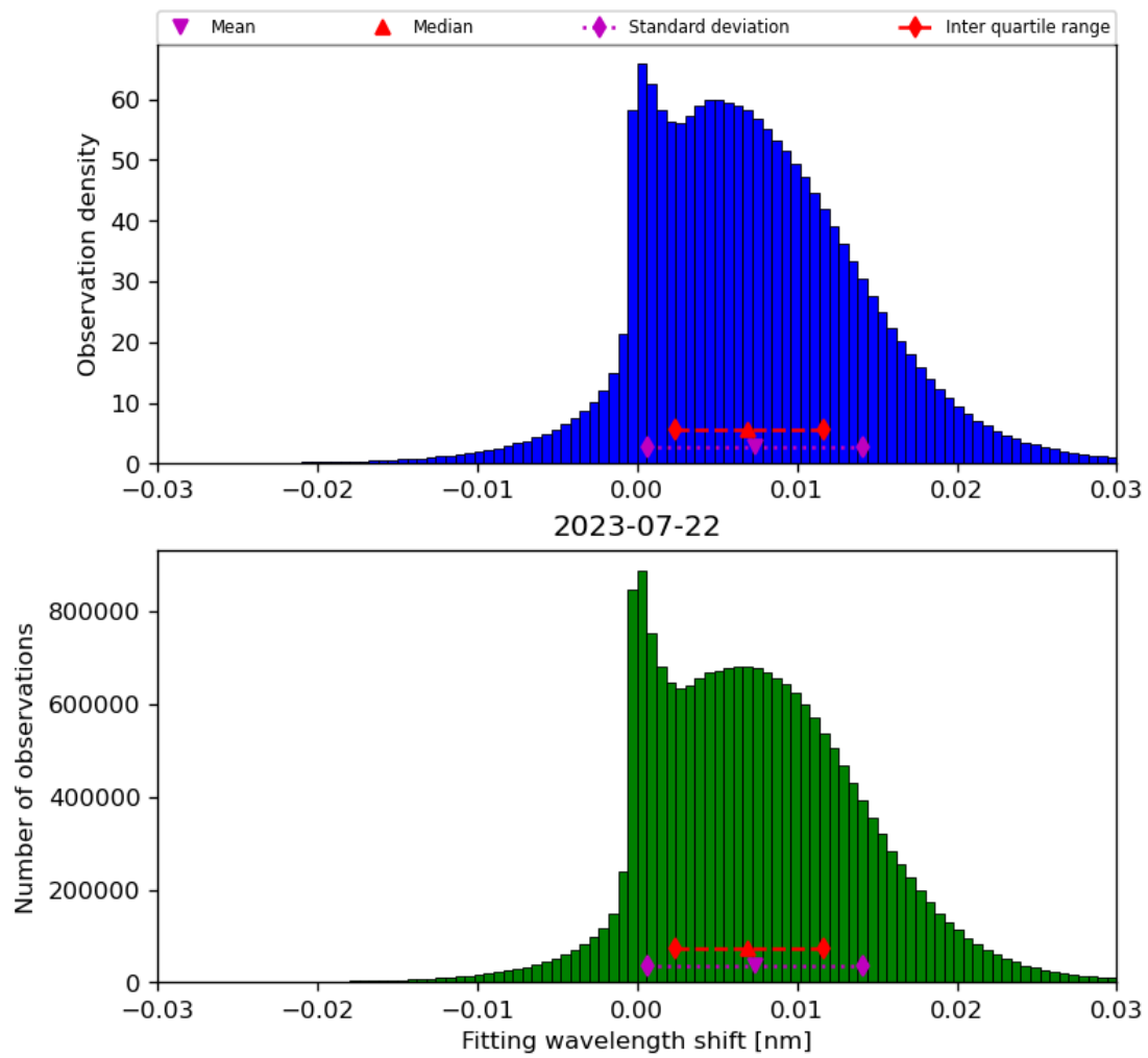
Figure 49: Histogram of “Fitting wavelength shift” for 2023-07-21 to 2023-07-23
