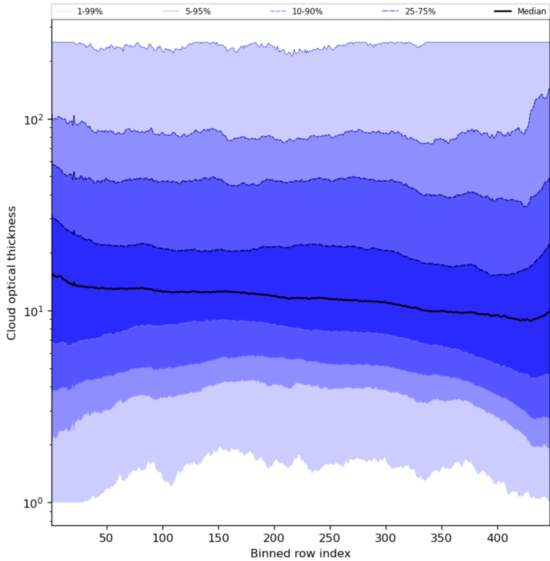
Figure 57: Along track statistics of “Cloud optical thickness” for 2023-07-21 to 2023-07-23
