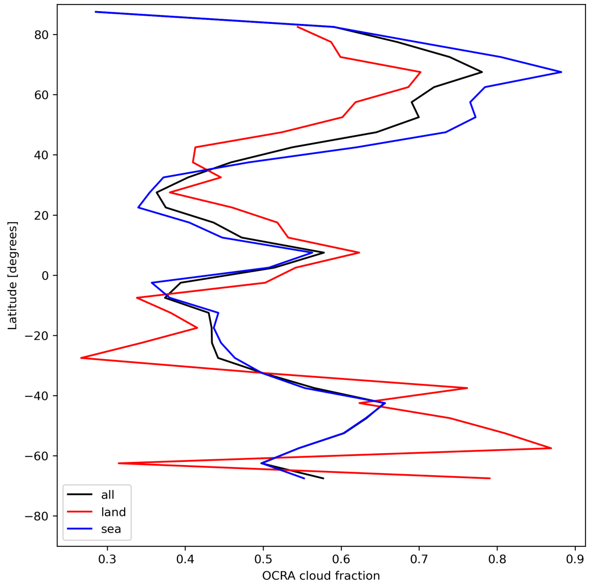
Figure 34: Zonal average of “OCRA cloud fraction” for 2023-07-21 to 2023-07-23.
