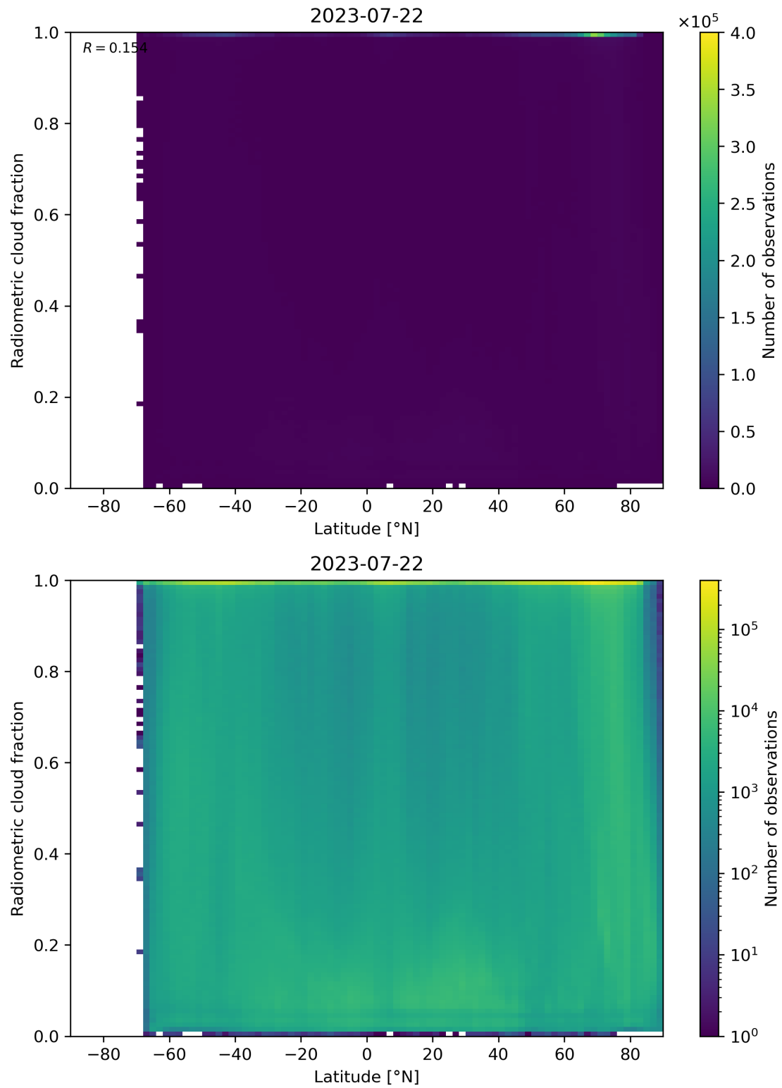
Figure 92: Scatter density plot of “Latitude” against “Radiometric cloud fraction” for 2023-07-21 to 2023-07-23.
