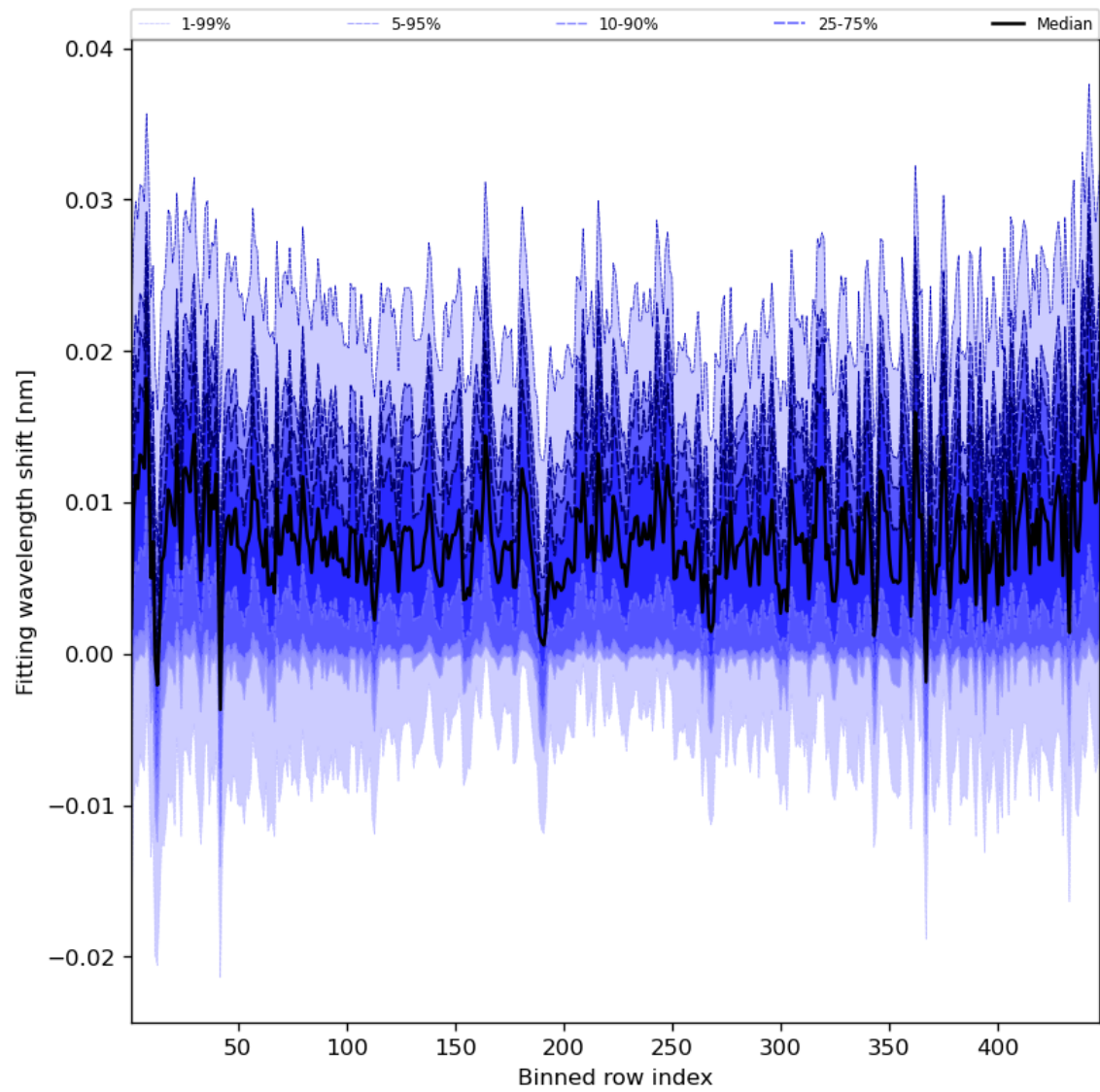
Figure 65: Along track statistics of “Fitting wavelength shift” for 2023-07-21 to 2023-07-23
