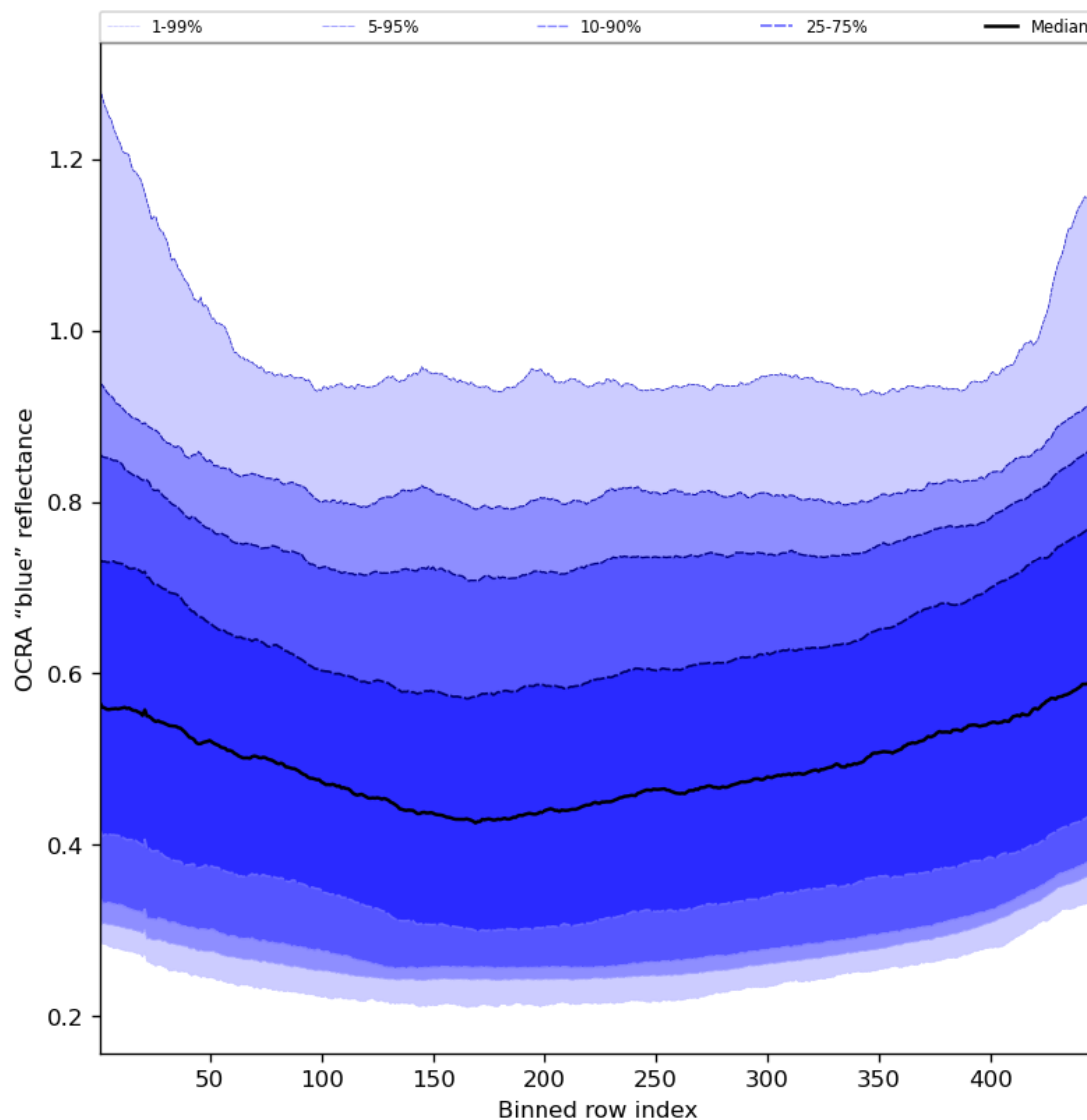
Figure 67: Along track statistics of “OCRA “blue” reflectance” for 2023-07-21 to 2023-07-23
