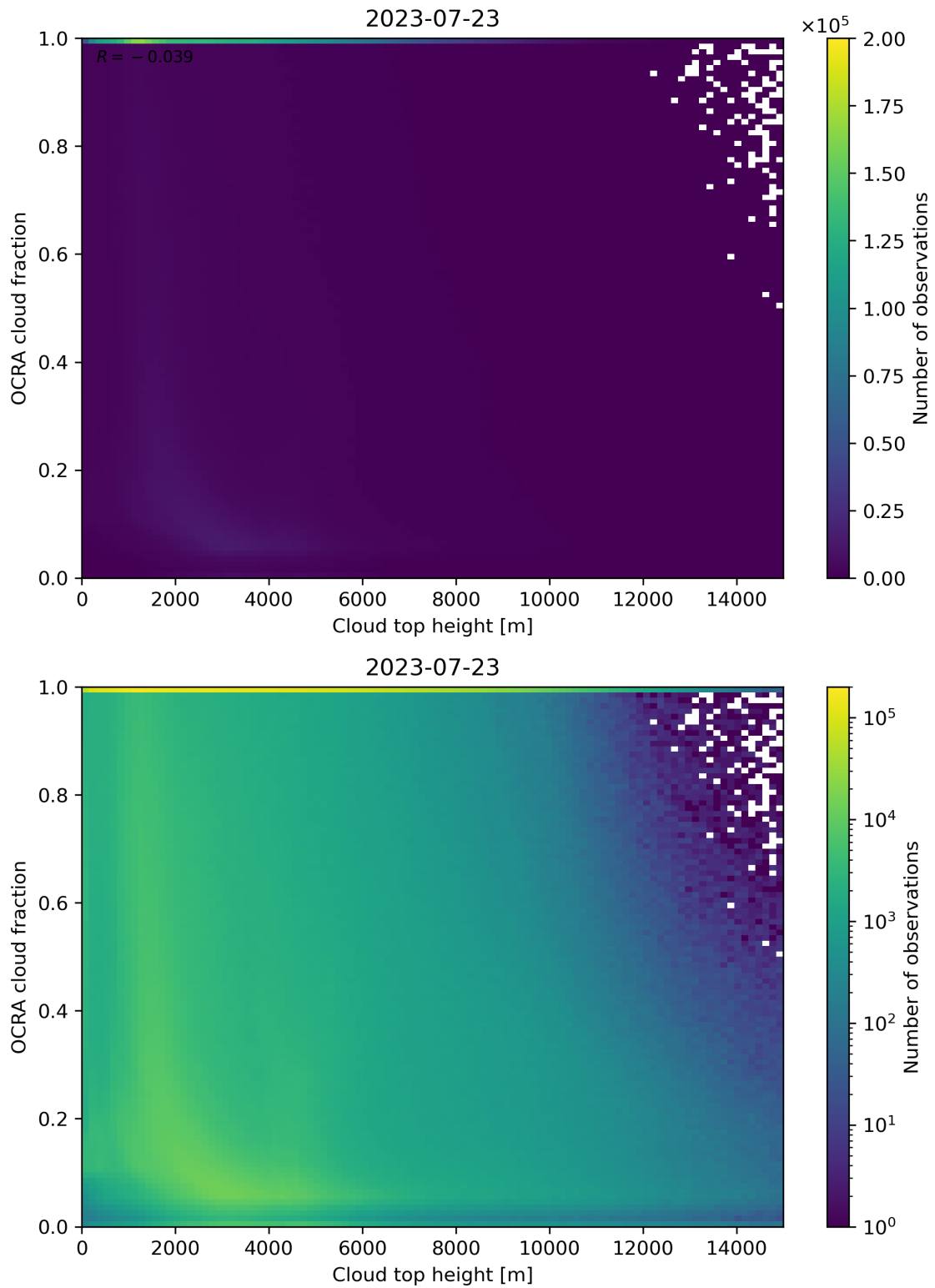
Figure 87: Scatter density plot of “Cloud top height” against “OCRA cloud fraction” for 2023-07-22 to 2023-07-24.
