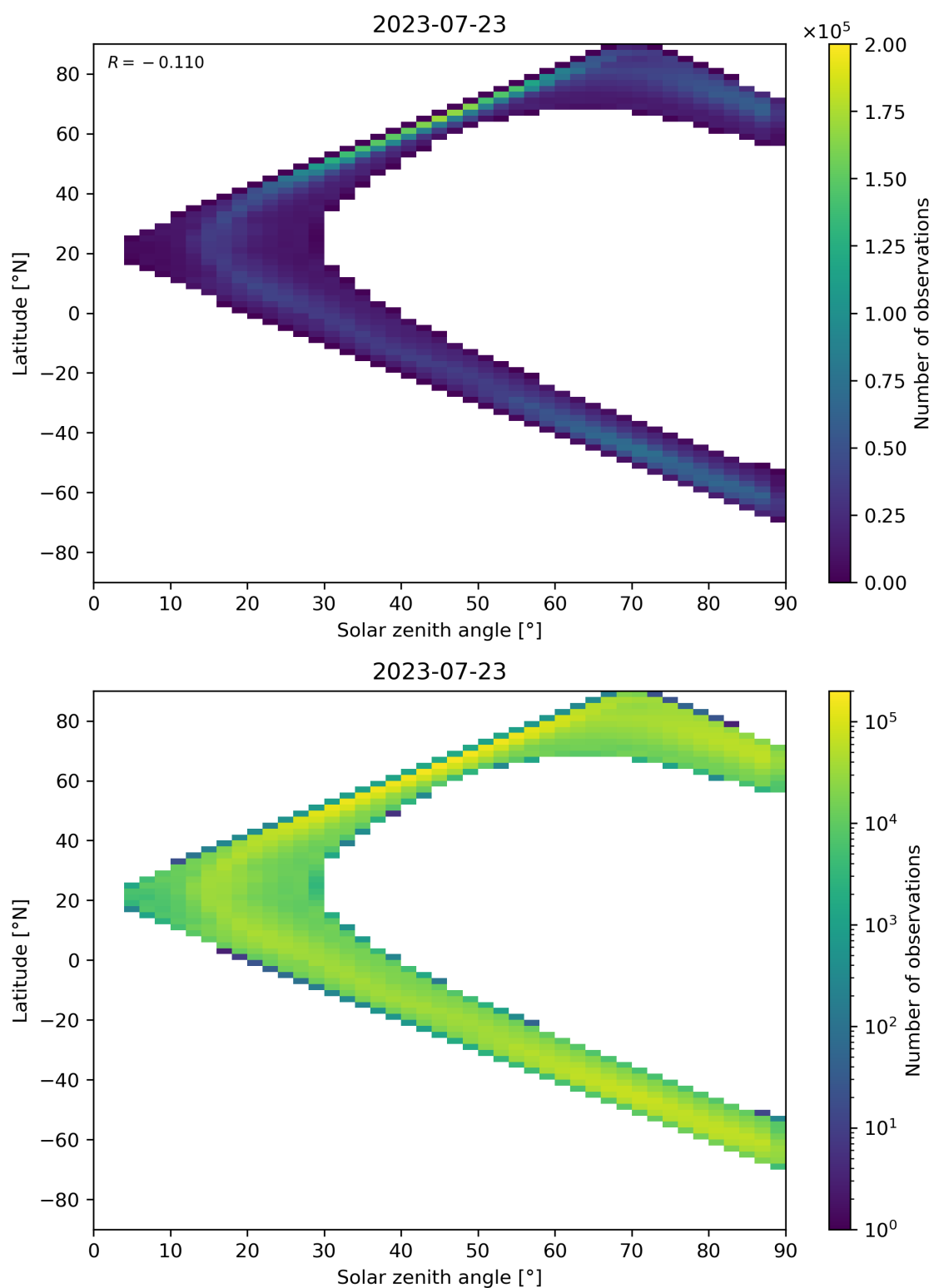
Figure 105: Scatter density plot of “Solar zenith angle” against “Latitude” for 2023-07-22 to 2023-07-24.
