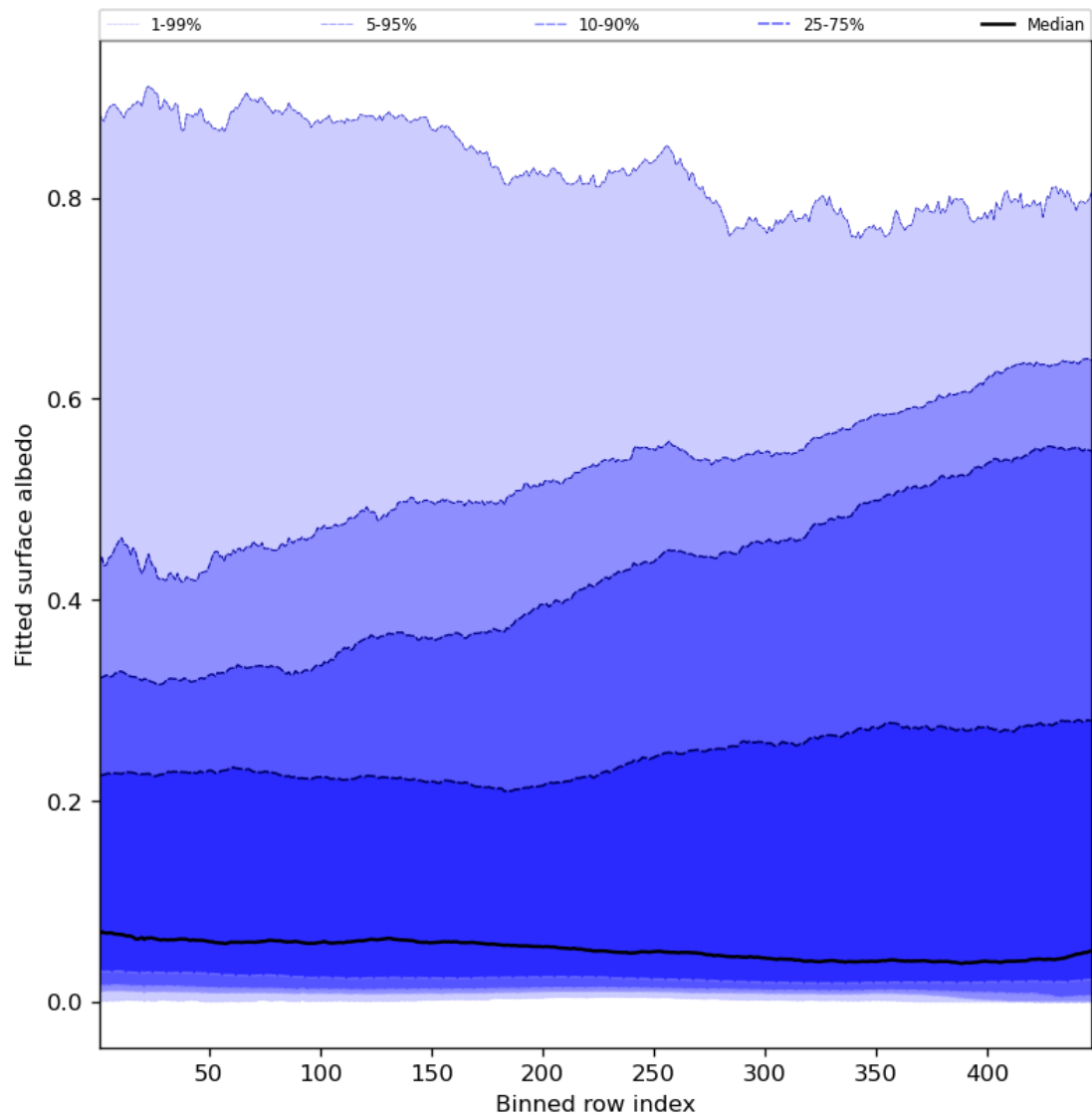
Figure 61: Along track statistics of “Fitted surface albedo” for 2023-07-22 to 2023-07-24
