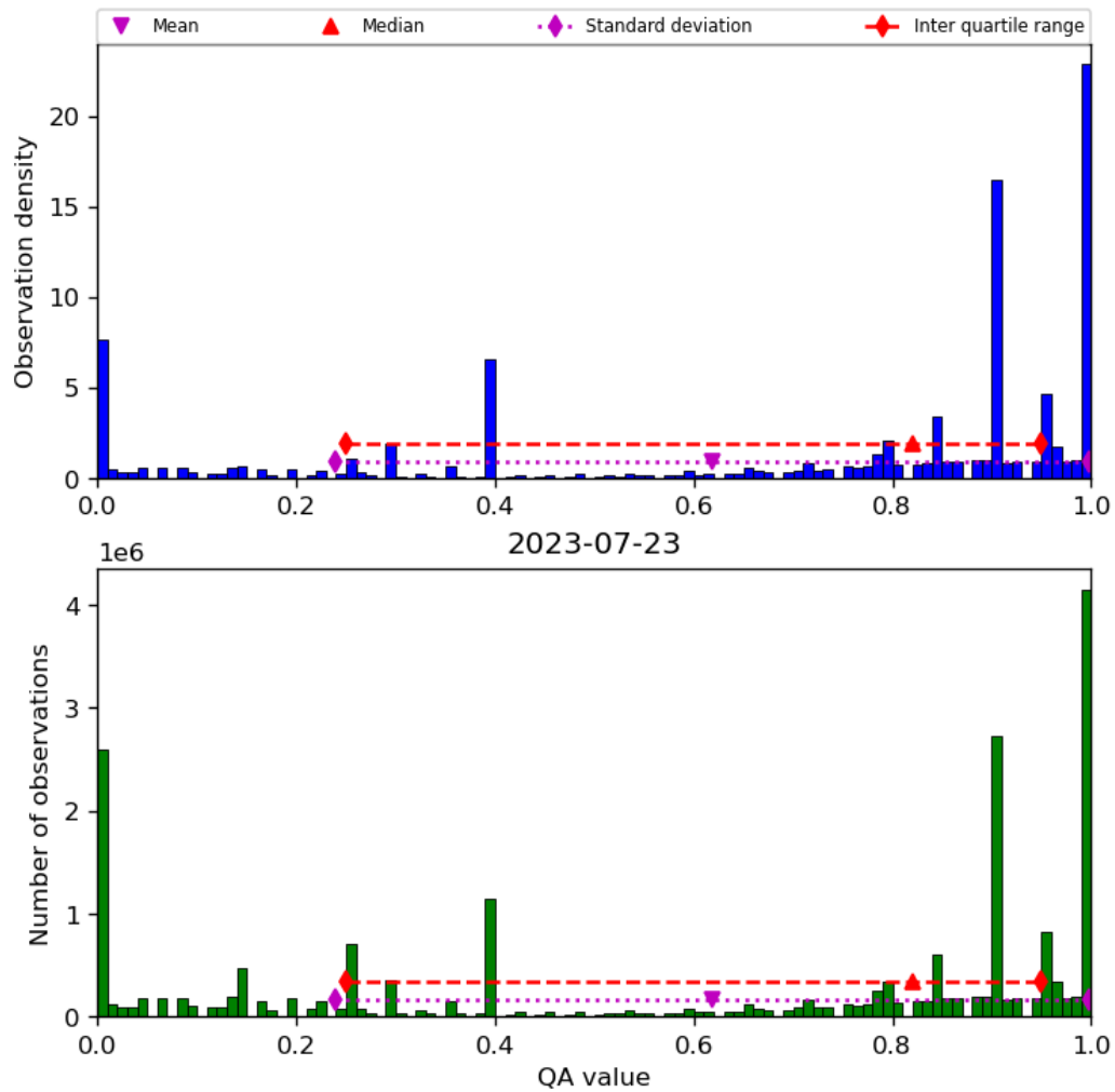
Figure 38: Histogram of “QA value” for 2023-07-22 to 2023-07-24
