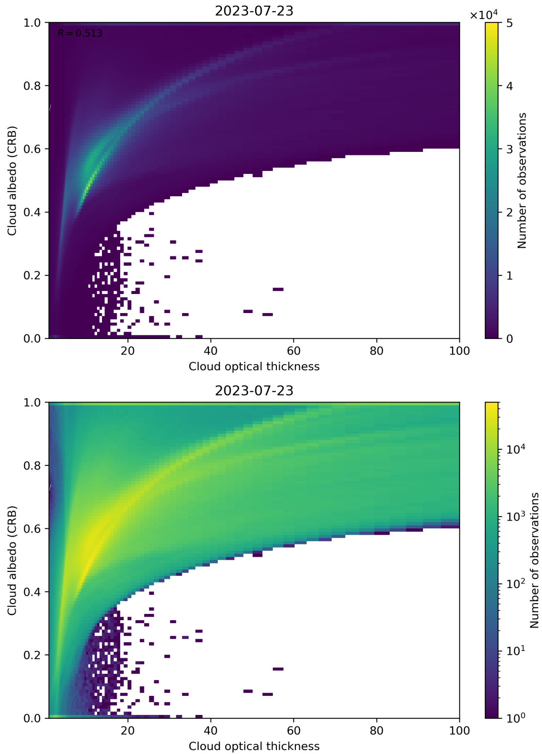
Figure 82: Scatter density plot of “Cloud optical thickness” against “Cloud albedo (CRB)” for 2023-07-22 to 2023-07-24.
