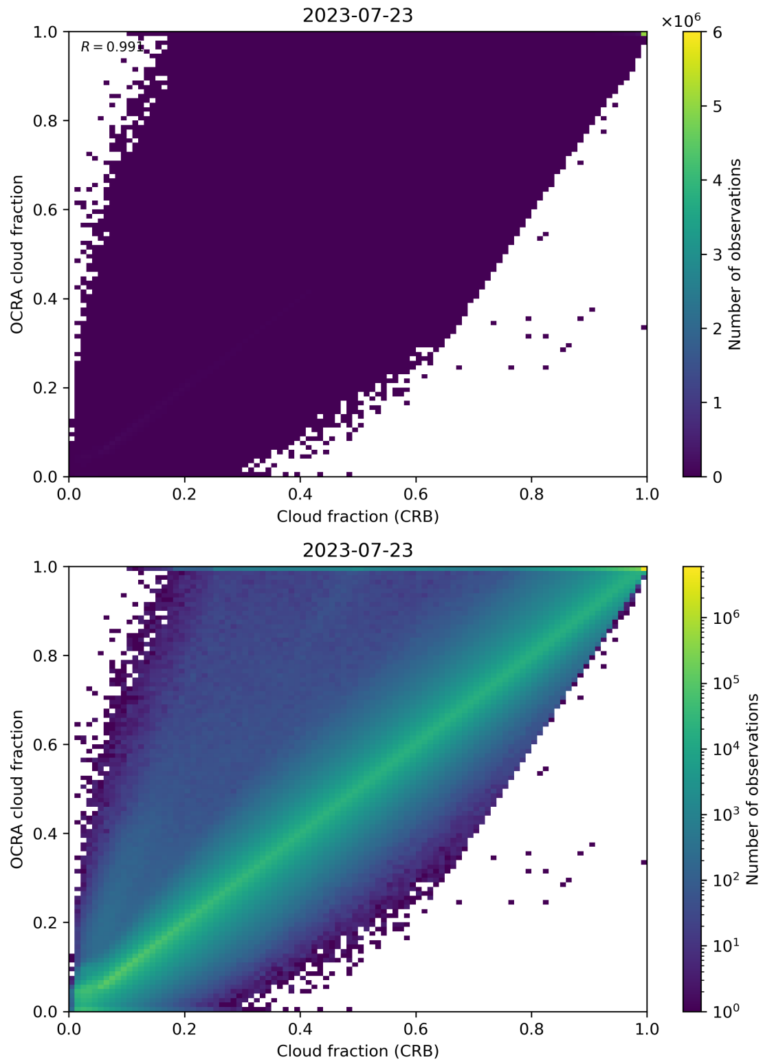
Figure 78: Scatter density plot of “Cloud fraction (CRB)” against “OCRA cloud fraction” for 2023-07-22 to 2023-07-24.
