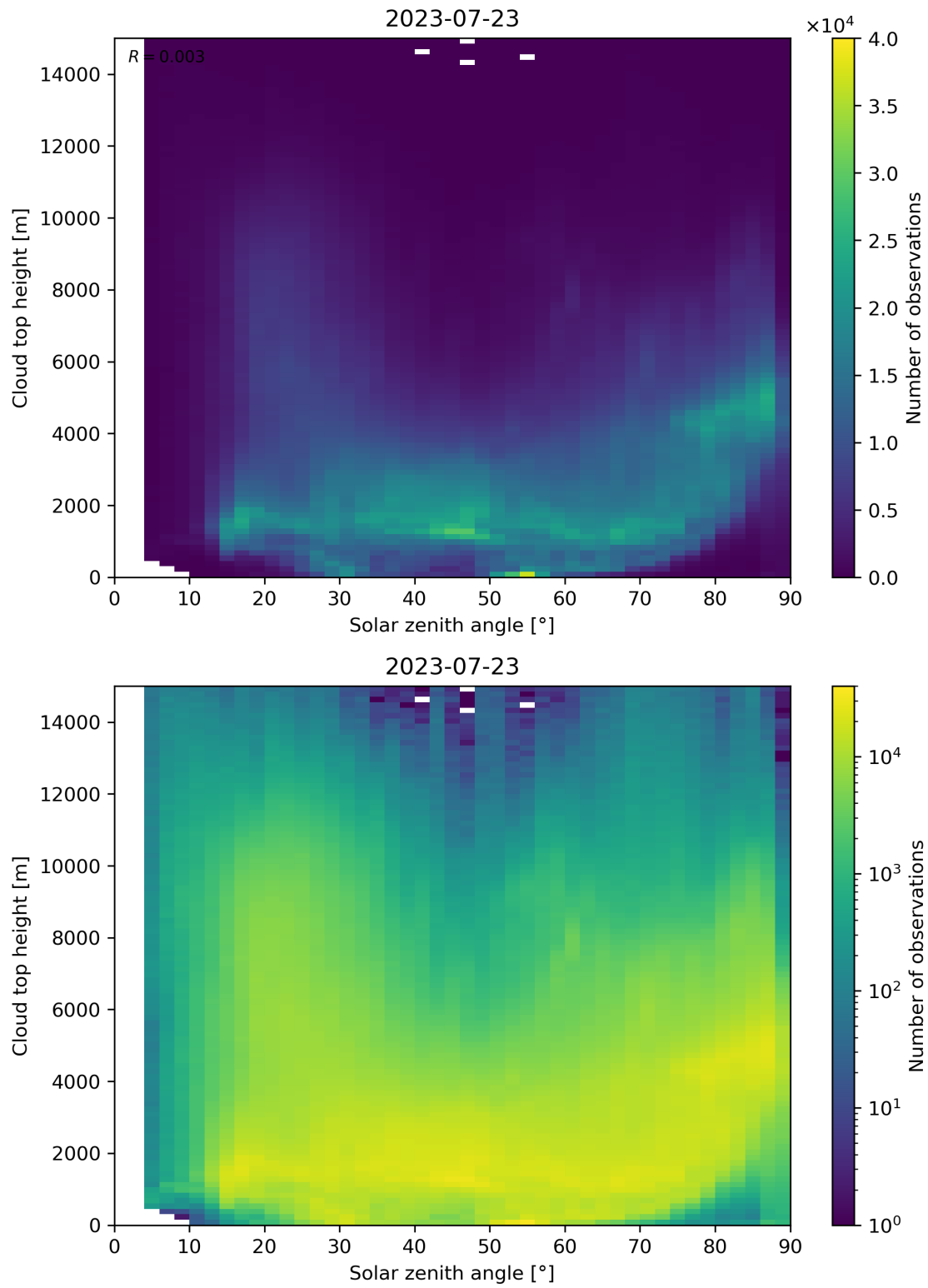
Figure 104: Scatter density plot of “Solar zenith angle” against “Cloud top height” for 2023-07-22 to 2023-07-24.
