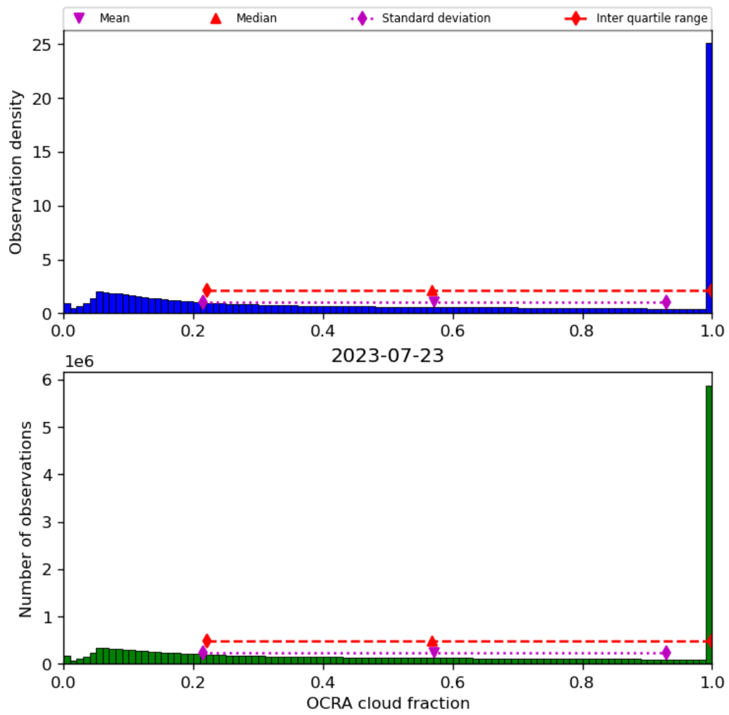
Figure 50: Histogram of “OCRA cloud fraction” for 2023-07-22 to 2023-07-24
