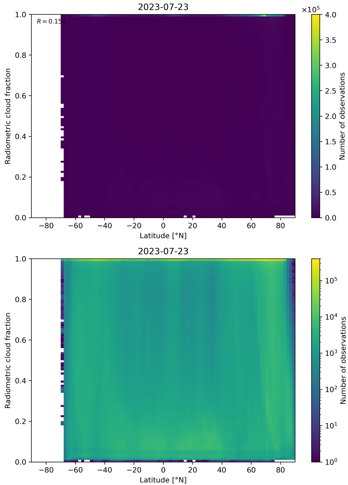
Figure 92: Scatter density plot of “Latitude” against “Radiometric cloud fraction” for 2023-07-22 to 2023-07-24.
