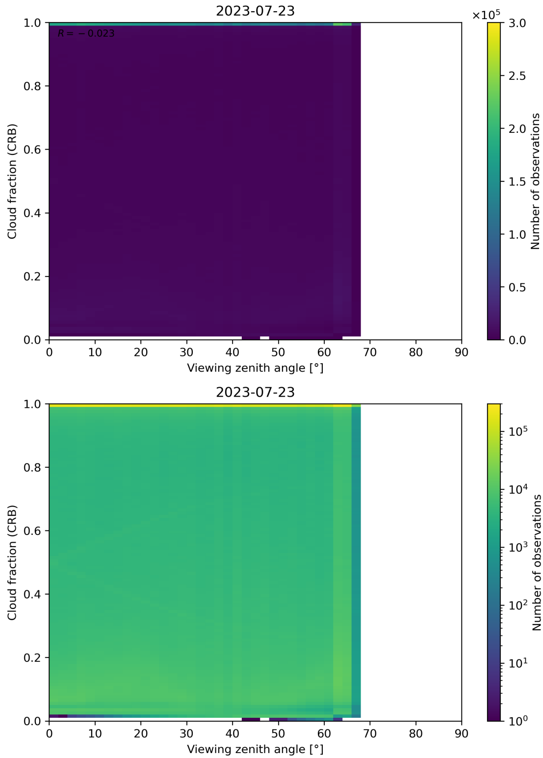
Figure 109: Scatter density plot of “Viewing zenith angle” against “Cloud fraction (CRB)” for 2023-07-22 to 2023-07-24.
