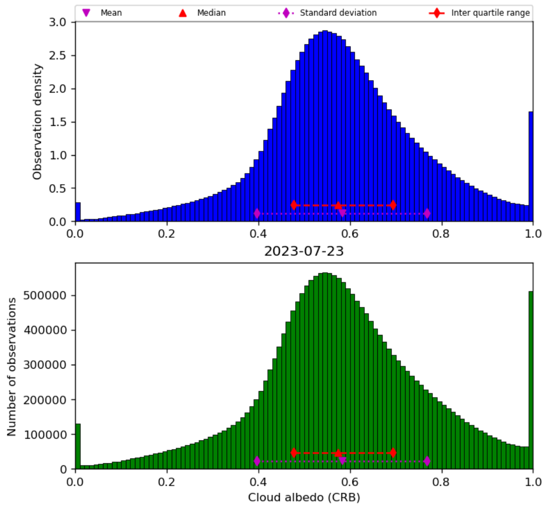
Figure 44: Histogram of “Cloud albedo (CRB)” for 2023-07-22 to 2023-07-24
