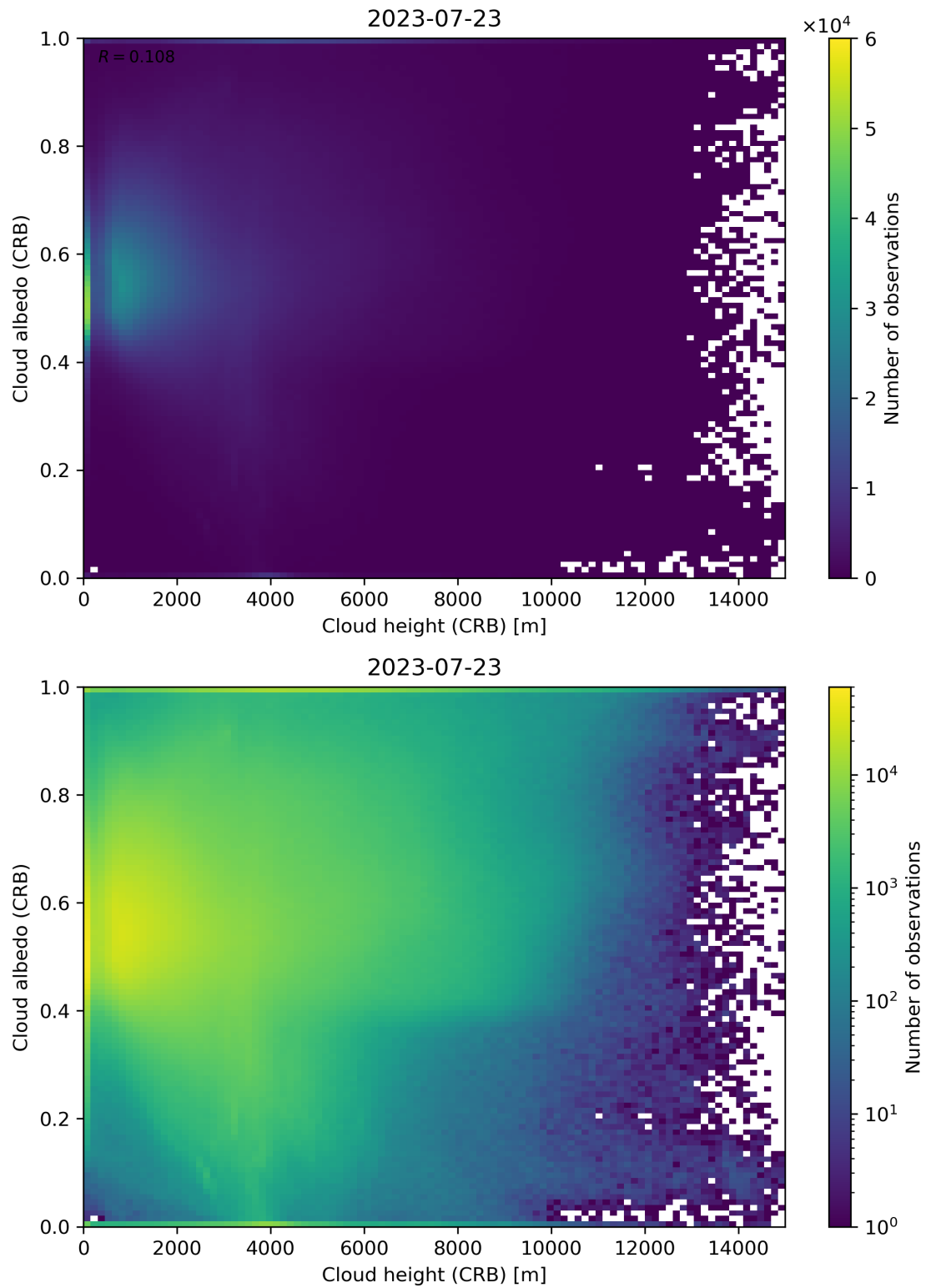
Figure 80: Scatter density plot of “Cloud height (CRB)” against “Cloud albedo (CRB)” for 2023-07-22 to 2023-07-24.
