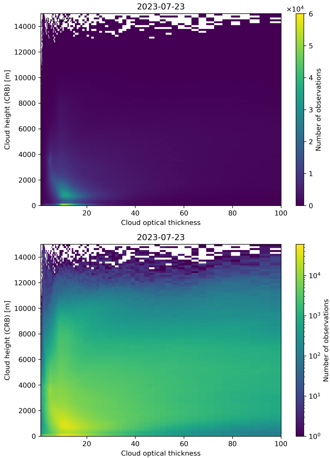
Figure 85: Scatter density plot of “Cloud optical thickness” against “Cloud height (CRB)” for 2023-07-22 to 2023-07-24.
