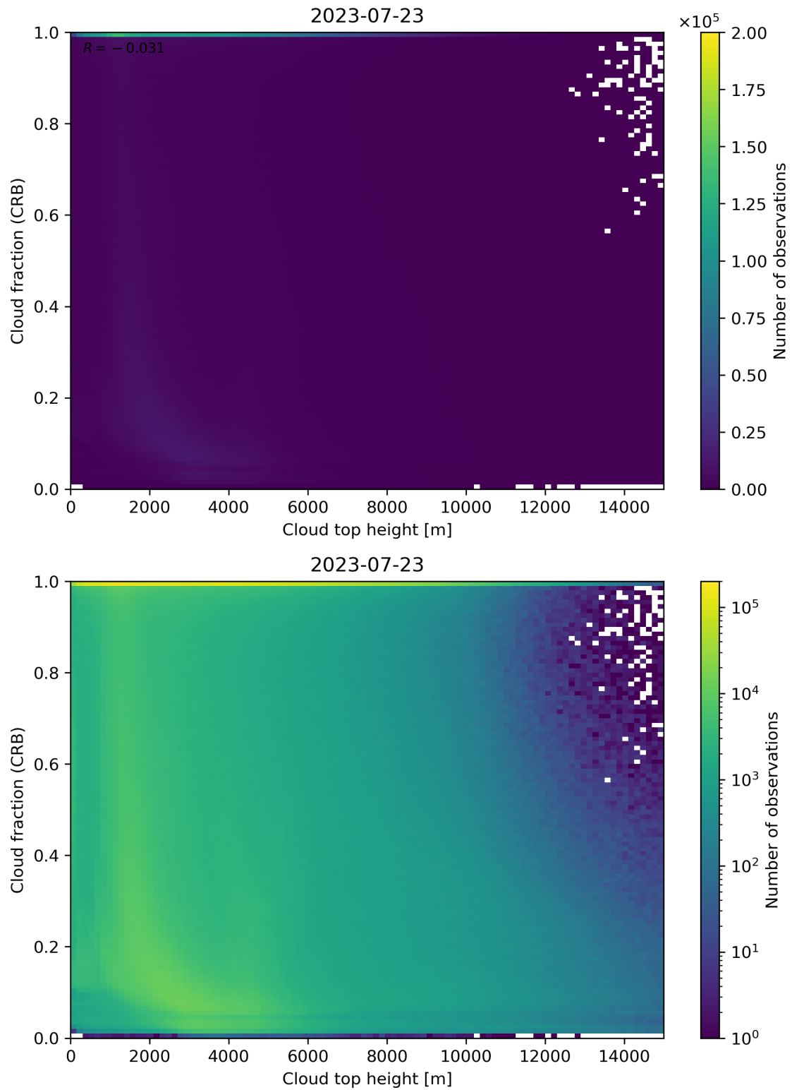
Figure 88: Scatter density plot of “Cloud top height” against “Cloud fraction (CRB)” for 2023-07-22 to 2023-07-24.
