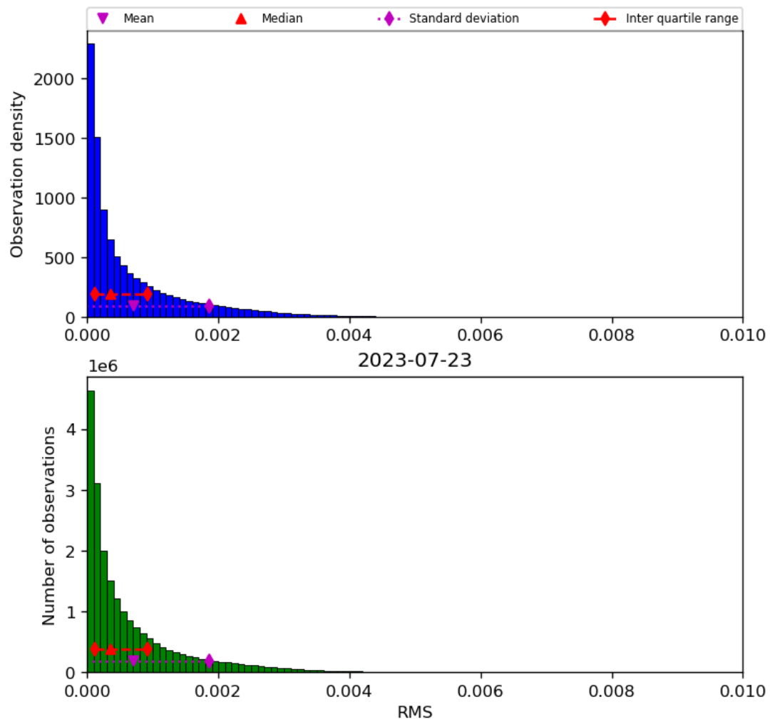
Figure 47: Histogram of “RMS” for 2023-07-22 to 2023-07-24
