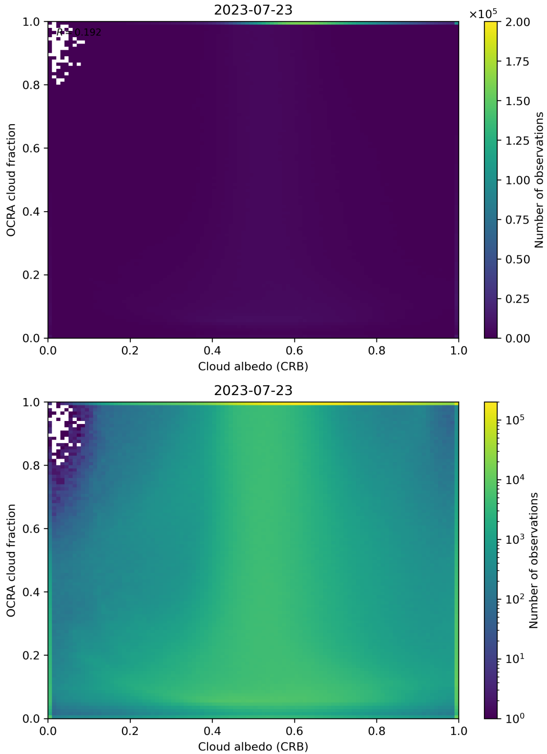
Figure 70: Scatter density plot of “Cloud albedo (CRB)” against “OCRA cloud fraction” for 2023-07-22 to 2023-07-24.
