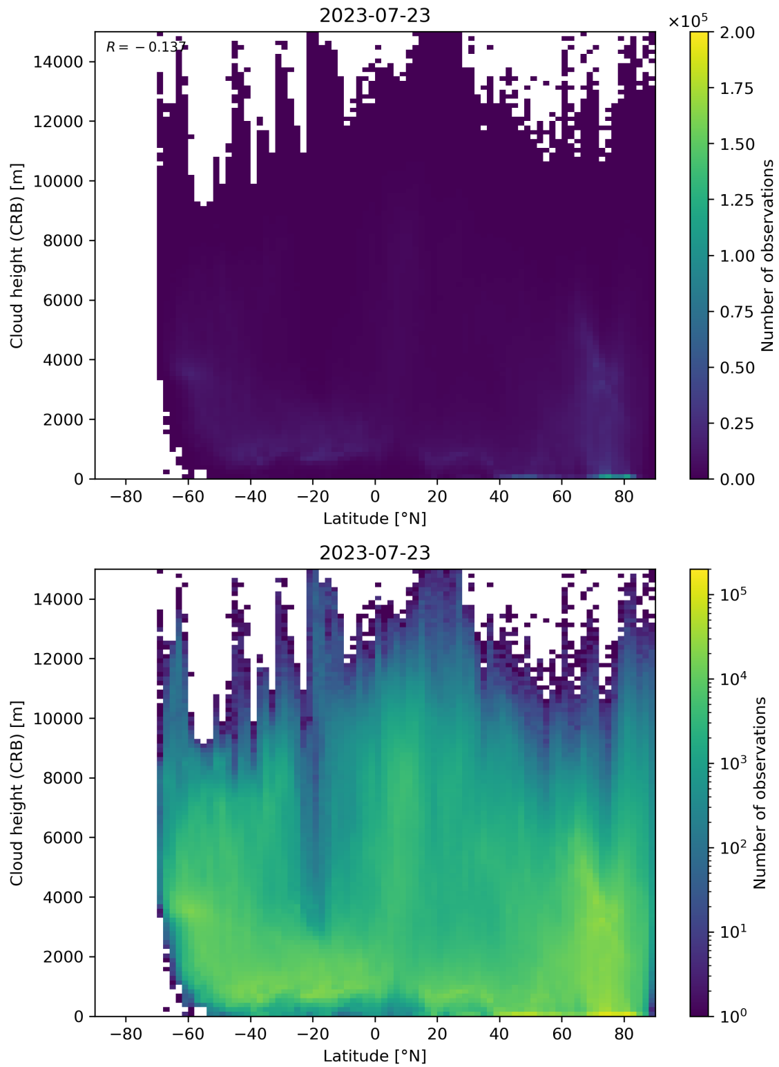
Figure 95: Scatter density plot of “Latitude” against “Cloud height (CRB)” for 2023-07-22 to 2023-07-24.
