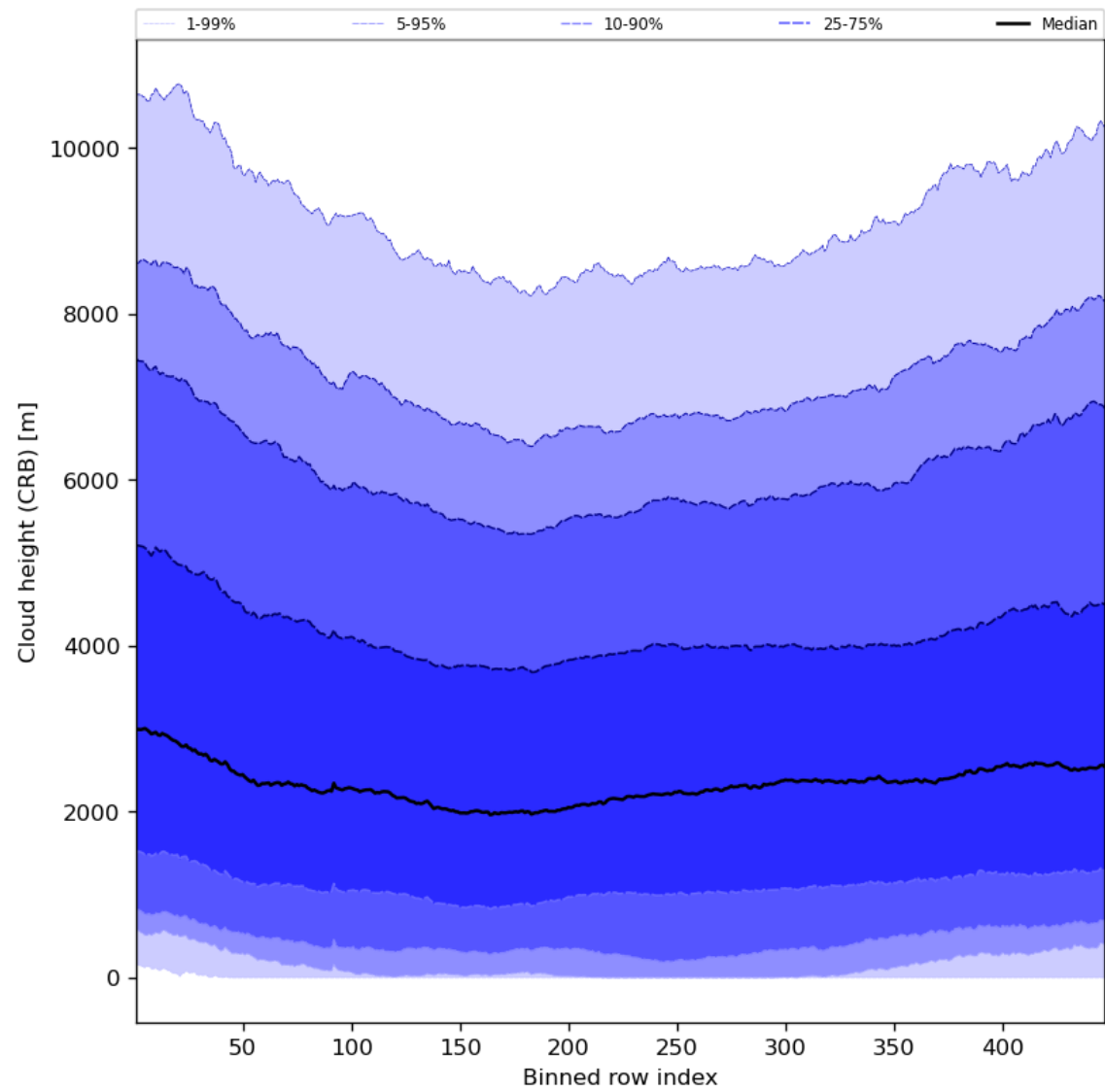
Figure 59: Along track statistics of “Cloud height (CRB)” for 2023-07-22 to 2023-07-24
