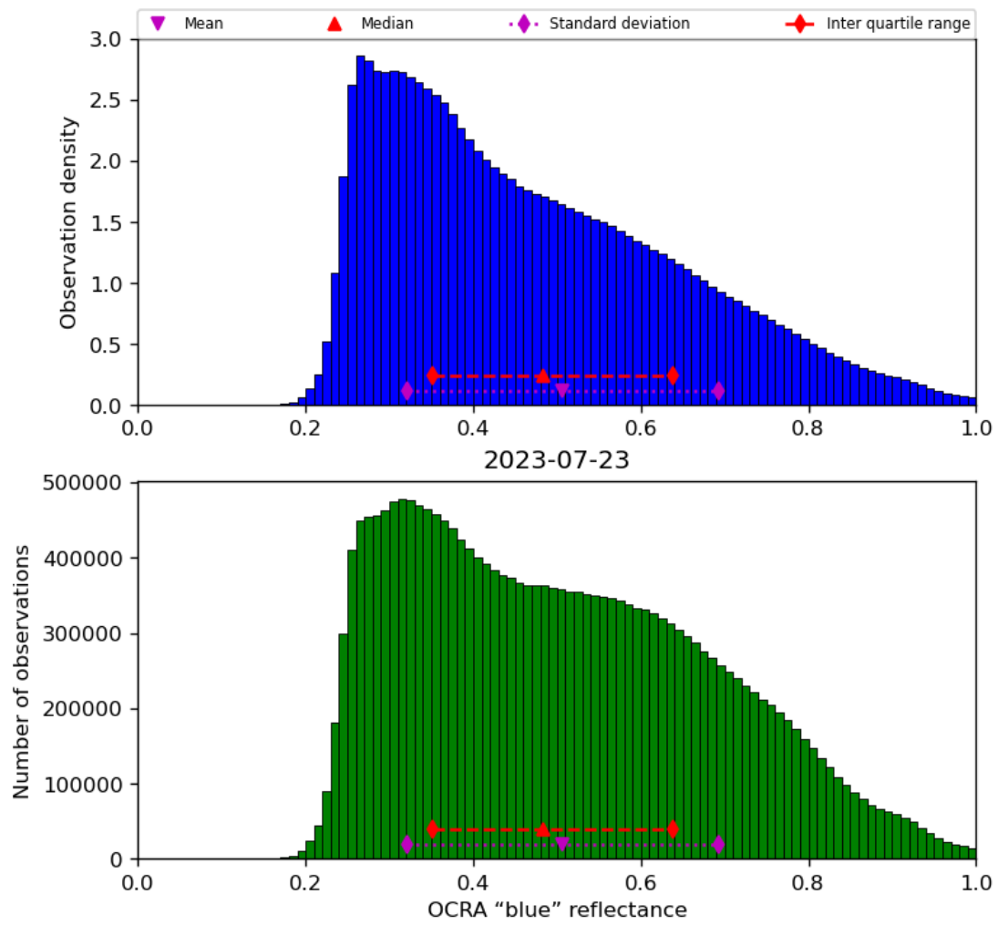
Figure 51: Histogram of “OCRA “blue” reflectance” for 2023-07-22 to 2023-07-24
