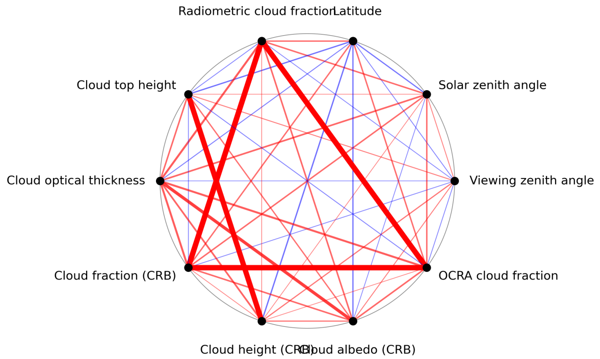
Figure 1: Map of correlation graph for 2023-07-22 to 2023-07-24.
