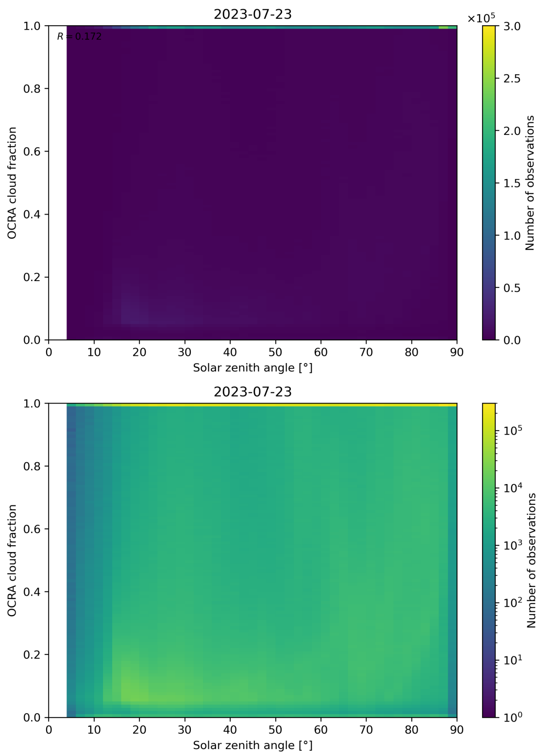
Figure 100: Scatter density plot of “Solar zenith angle” against “OCRA cloud fraction” for 2023-07-22 to 2023-07-24.
