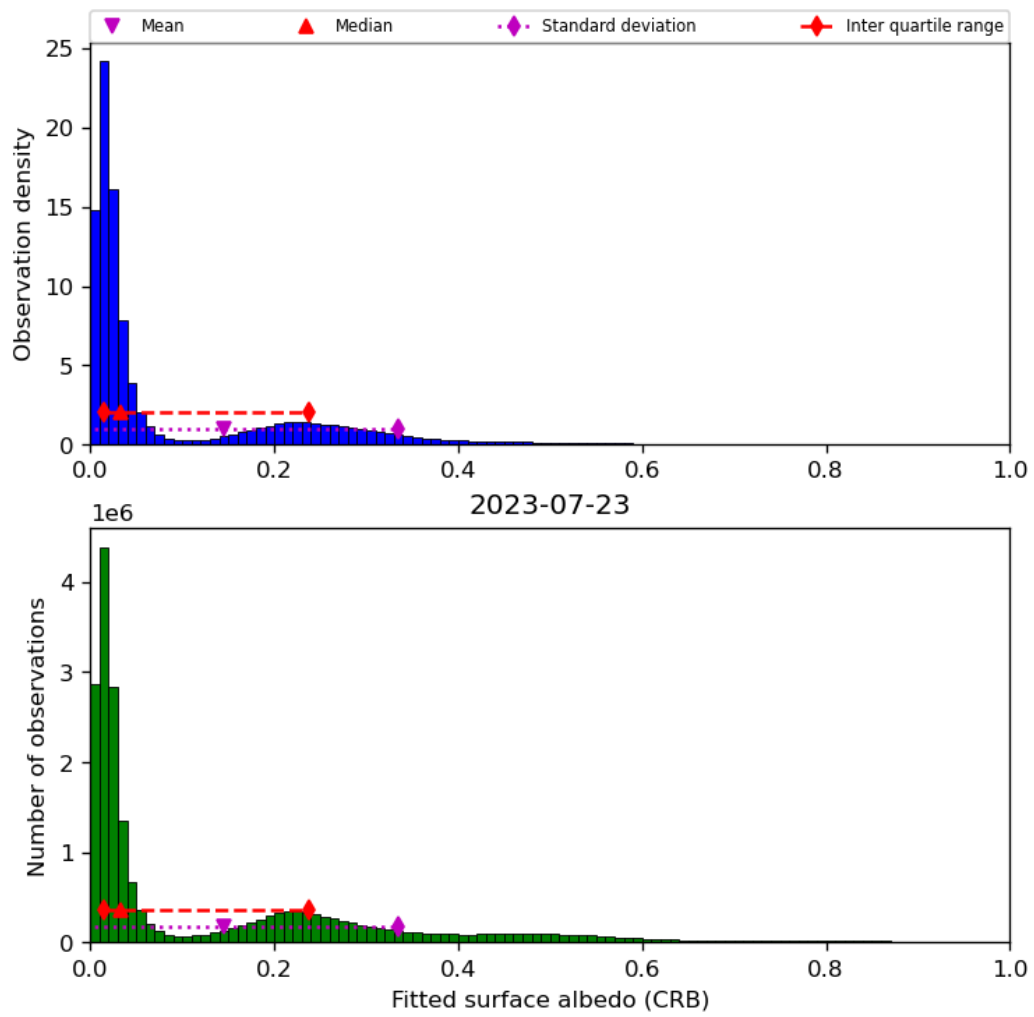
Figure 46: Histogram of “Fitted surface albedo (CRB)” for 2023-07-22 to 2023-07-24
