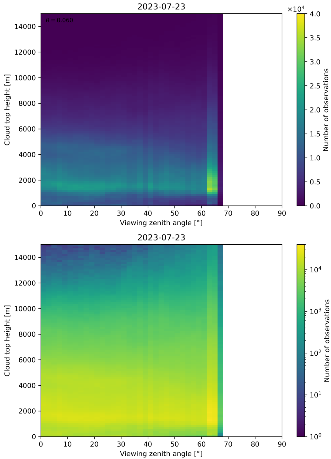
Figure 112: Scatter density plot of “Viewing zenith angle” against “Cloud top height” for 2023-07-22 to 2023-07-24.
