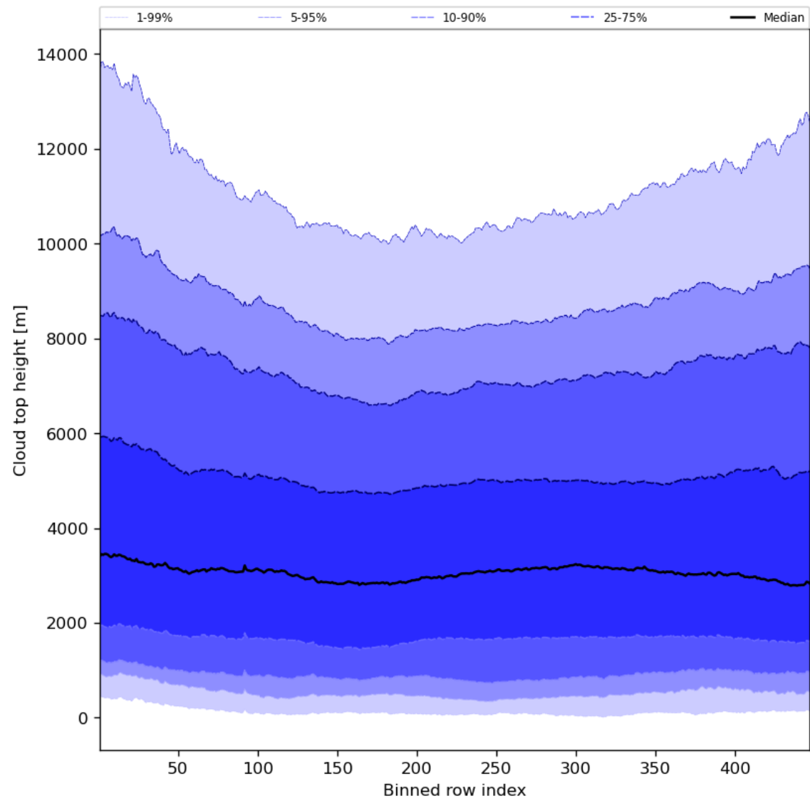
Figure 56: Along track statistics of “Cloud top height” for 2023-07-22 to 2023-07-24
