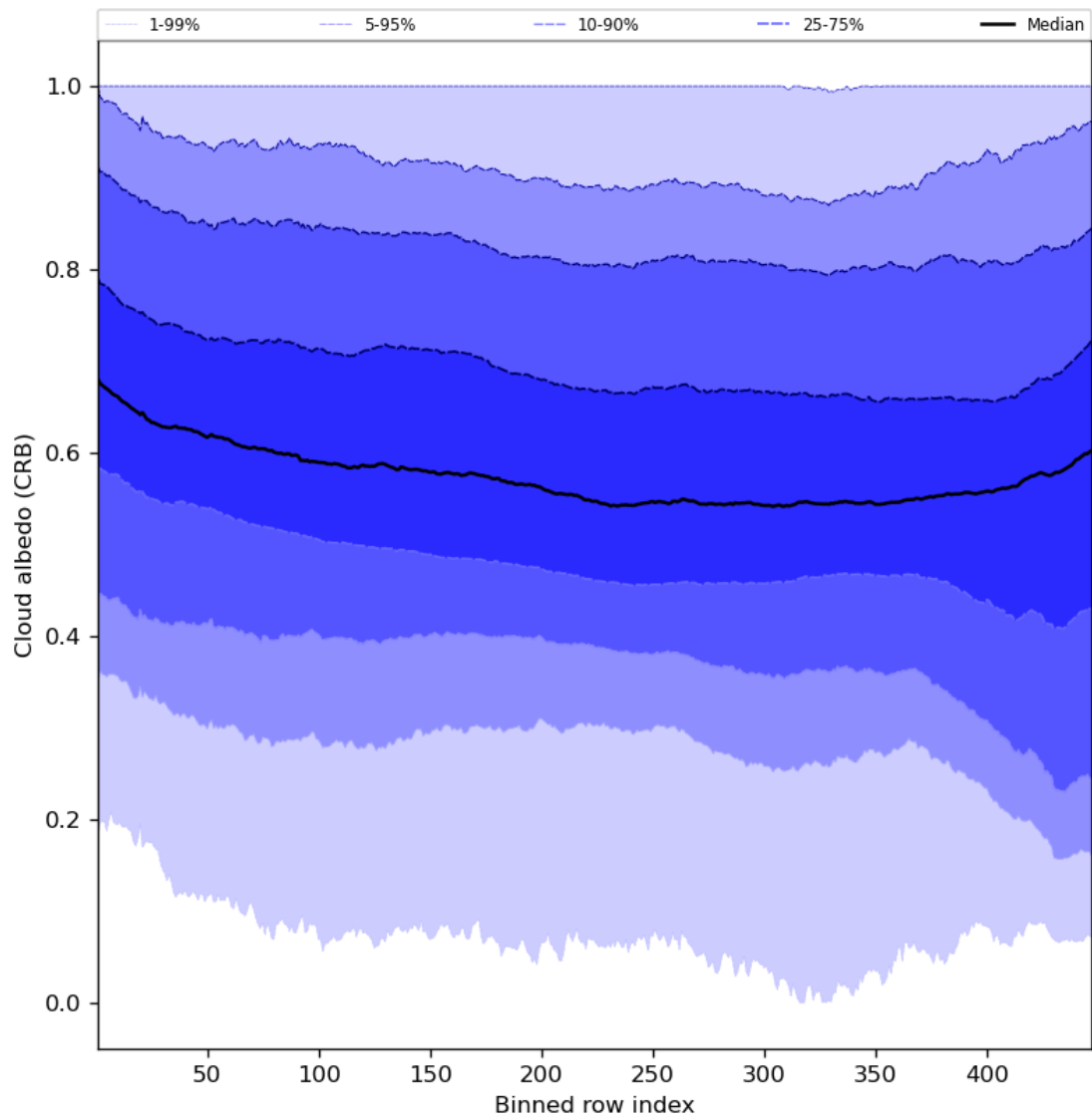
Figure 60: Along track statistics of “Cloud albedo (CRB)” for 2023-07-22 to 2023-07-24
