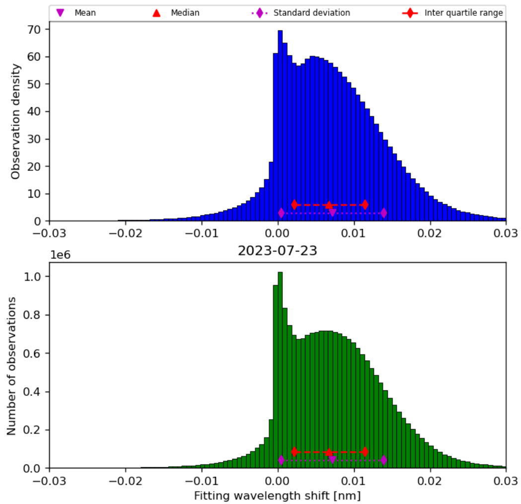
Figure 49: Histogram of “Fitting wavelength shift” for 2023-07-22 to 2023-07-24
