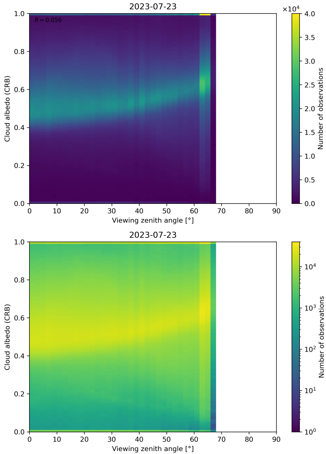
Figure 106: Scatter density plot of “Viewing zenith angle” against “Cloud albedo (CRB)” for 2023-07-22 to 2023-07-24.
