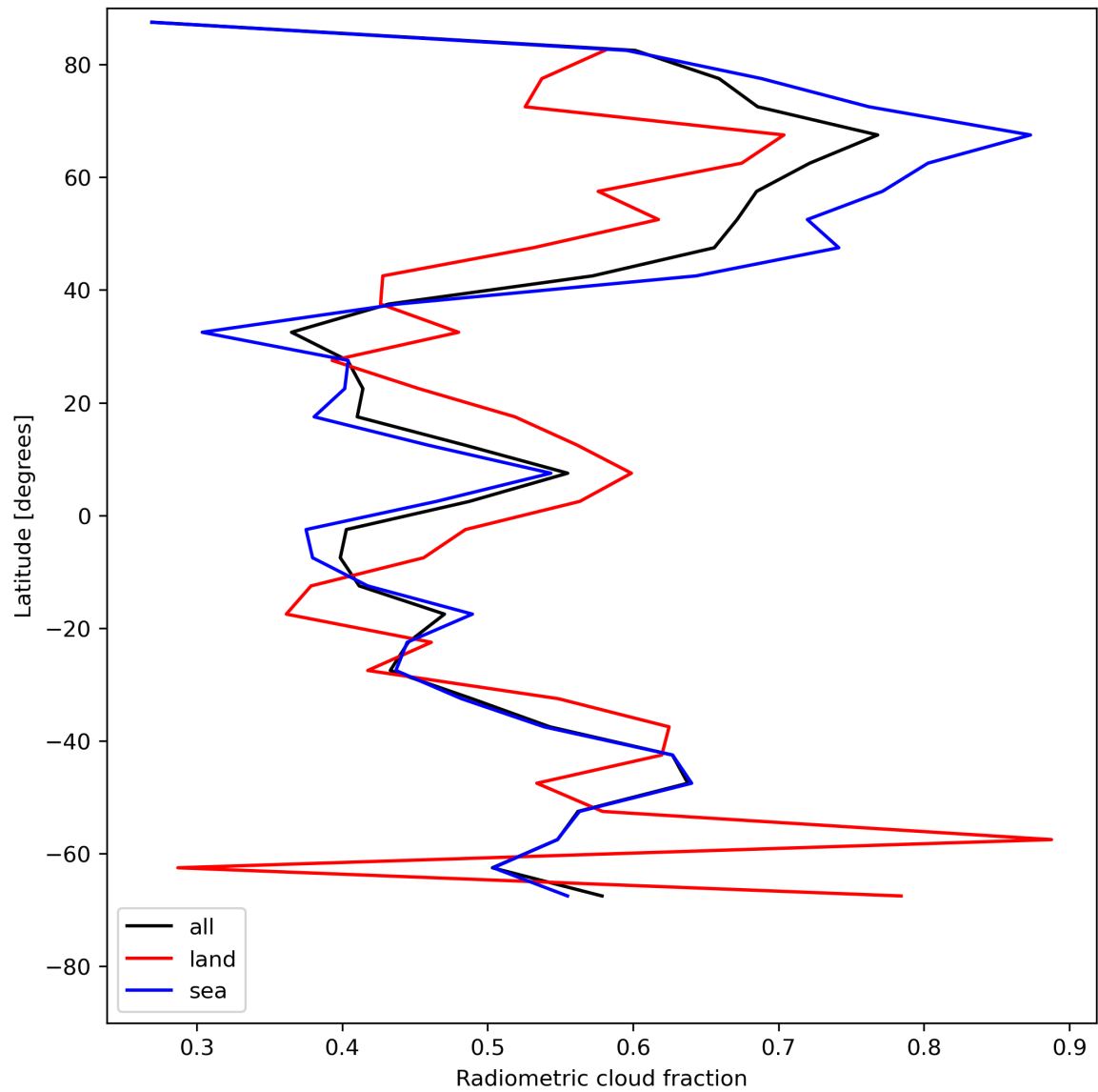
Figure 23: Zonal average of “Radiometric cloud fraction” for 2023-07-22 to 2023-07-24.
