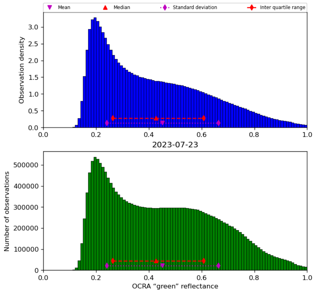
Figure 52: Histogram of “OCRA “green” reflectance” for 2023-07-22 to 2023-07-24
