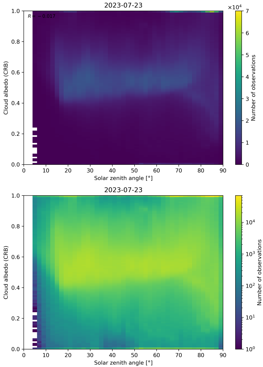
Figure 98: Scatter density plot of “Solar zenith angle” against “Cloud albedo (CRB)” for 2023-07-22 to 2023-07-24.
