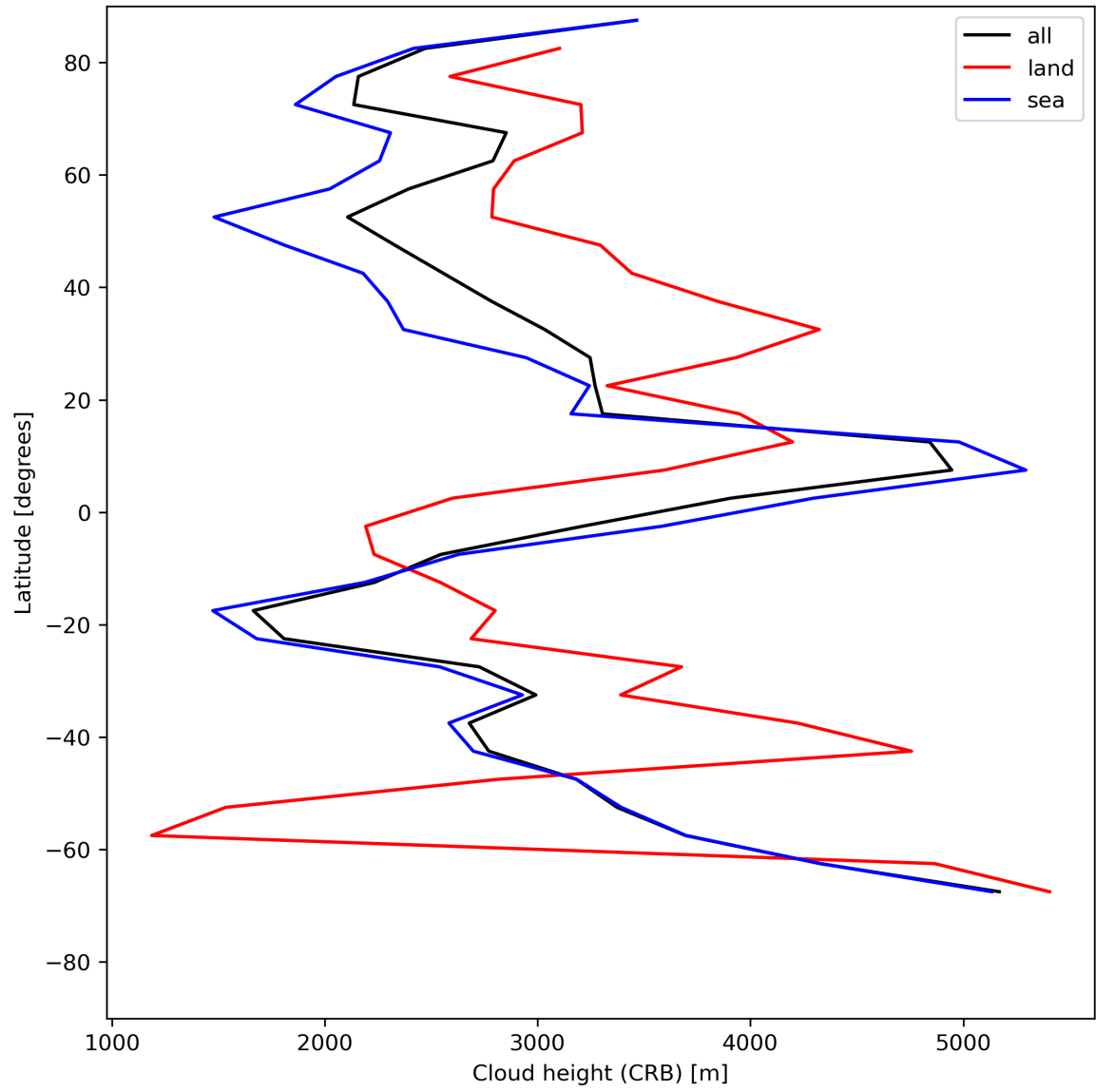
Figure 27: Zonal average of “Cloud height (CRB)” for 2023-07-22 to 2023-07-24.
