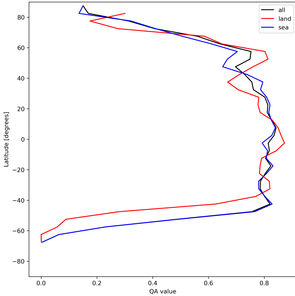
Figure 22: Zonal average of “QA value” for 2023-07-22 to 2023-07-24.
