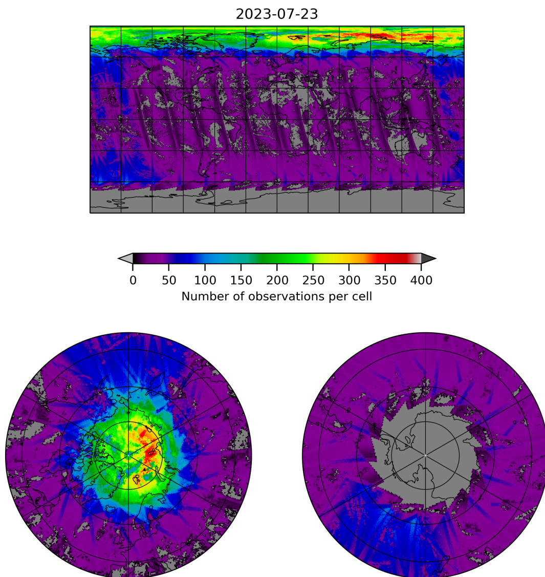
Figure 21: Map of the number of observations for 2023-07-22 to 2023-07-24
