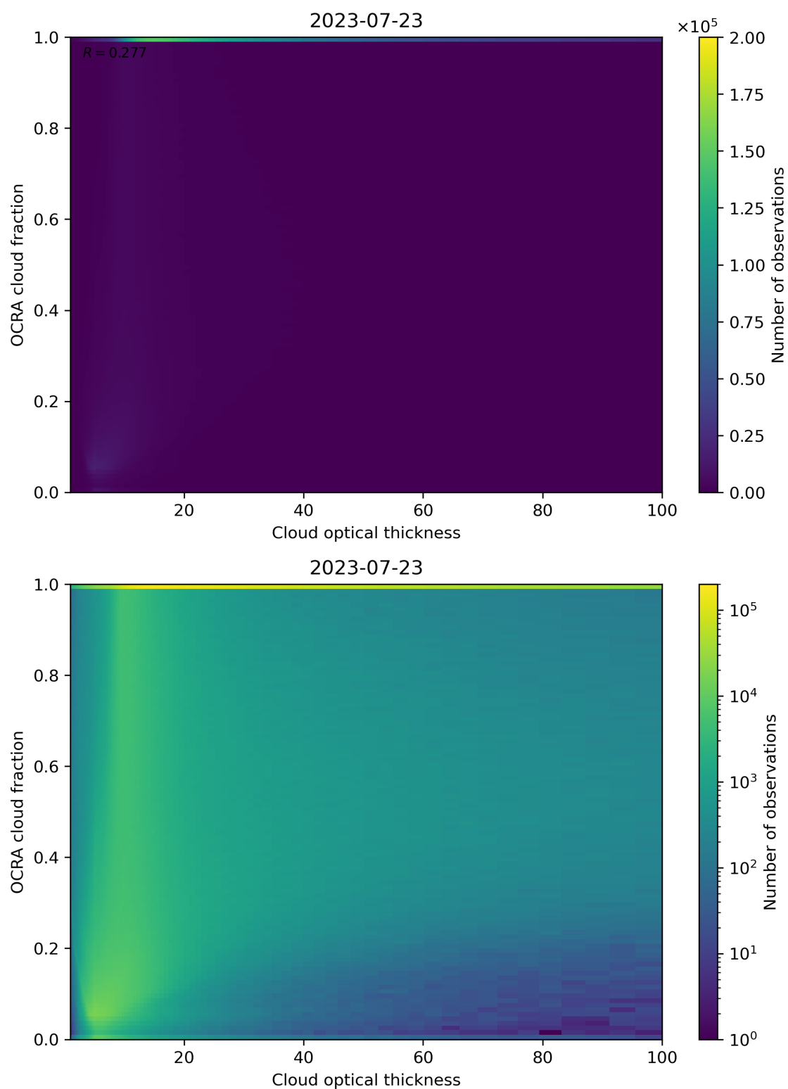
Figure 83: Scatter density plot of “Cloud optical thickness” against “OCRA cloud fraction” for 2023-07-22 to 2023-07-24.
