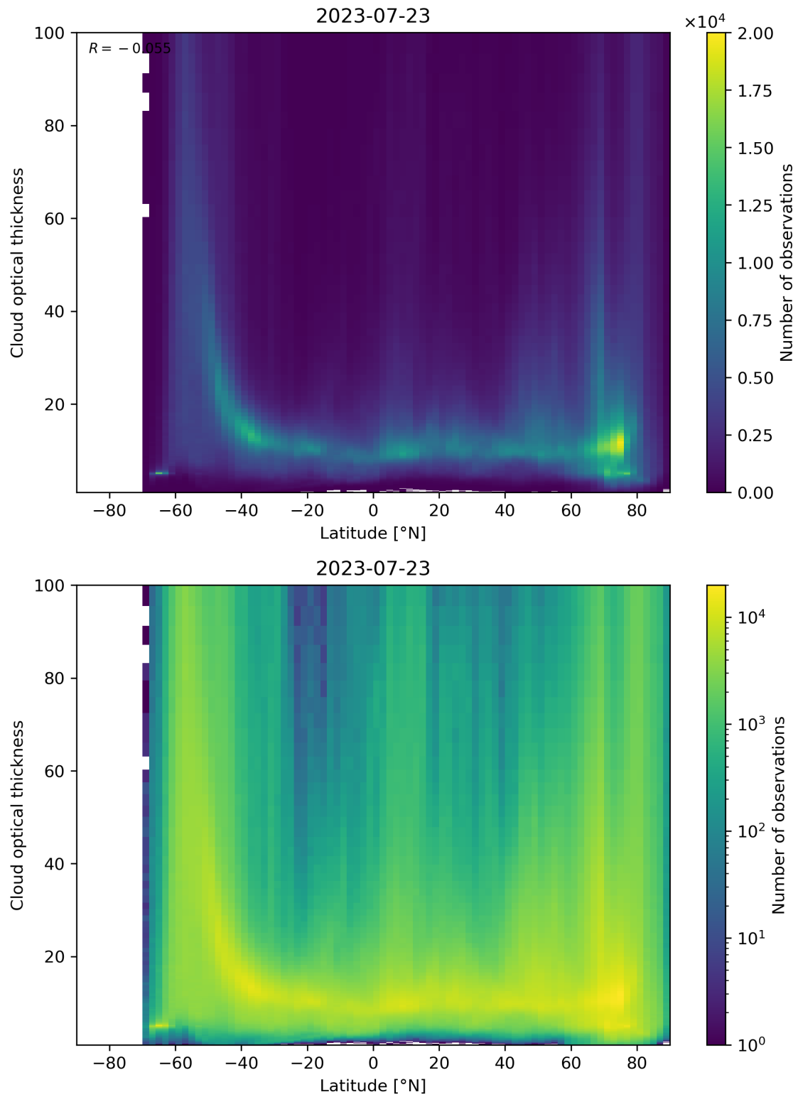
Figure 96: Scatter density plot of “Latitude” against “Cloud optical thickness” for 2023-07-22 to 2023-07-24.
