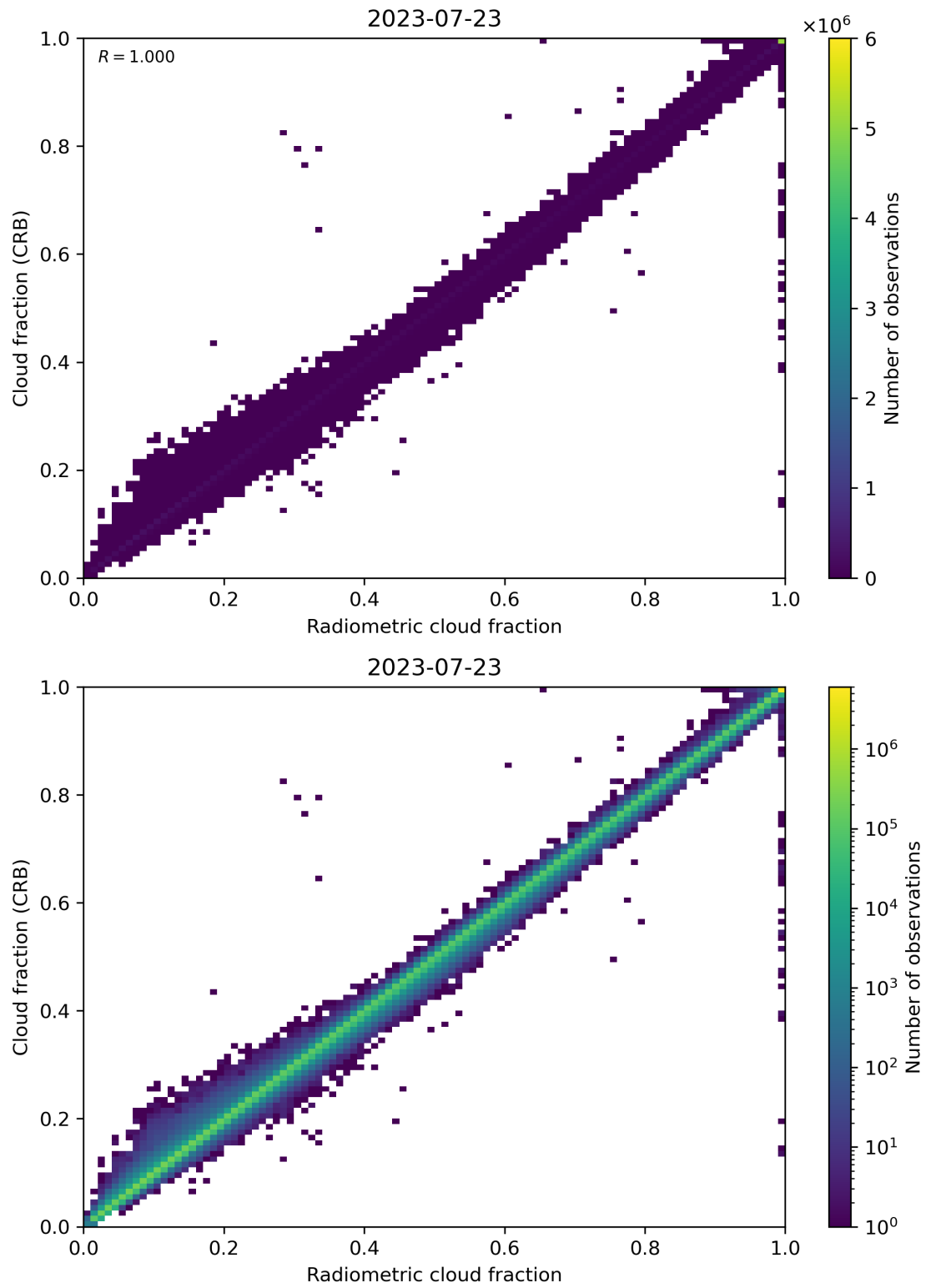
Figure 73: Scatter density plot of “Radiometric cloud fraction” against “Cloud fraction (CRB)” for 2023-07-22 to 2023-07-24.
