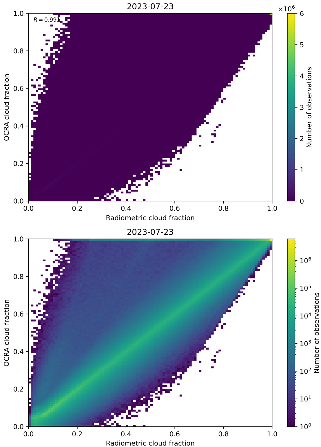
Figure 72: Scatter density plot of “Radiometric cloud fraction” against “OCRA cloud fraction” for 2023-07-22 to 2023-07-24.
