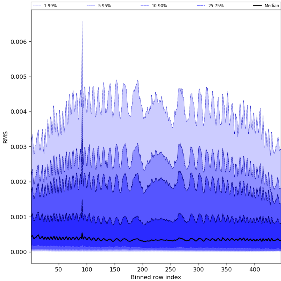
Figure 63: Along track statistics of “RMS” for 2023-07-22 to 2023-07-24
