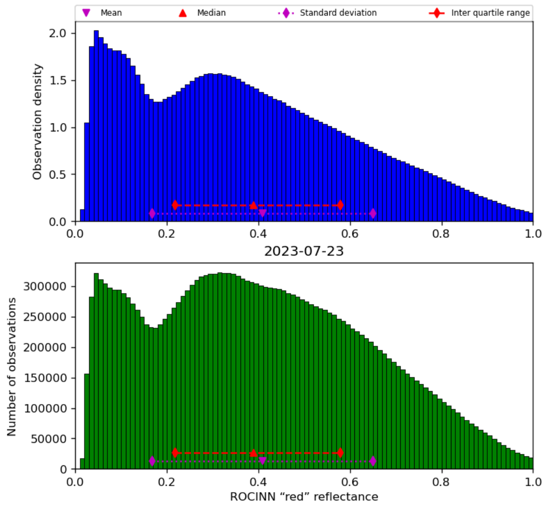
Figure 53: Histogram of “ROCINN “red” reflectance” for 2023-07-22 to 2023-07-24
