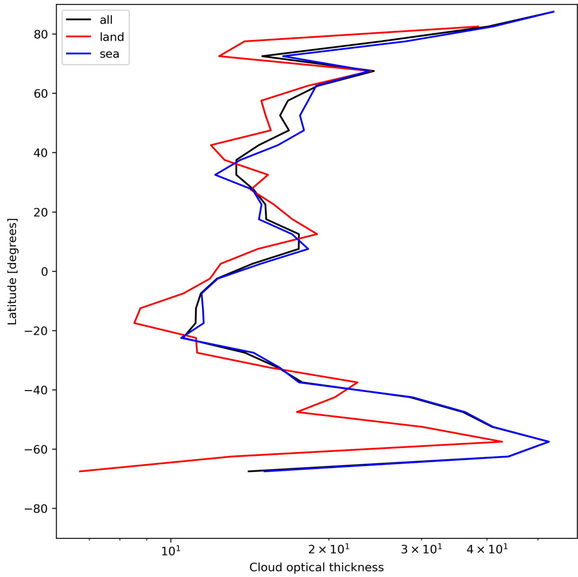
Figure 25: Zonal average of “Cloud optical thickness” for 2023-07-22 to 2023-07-24.
