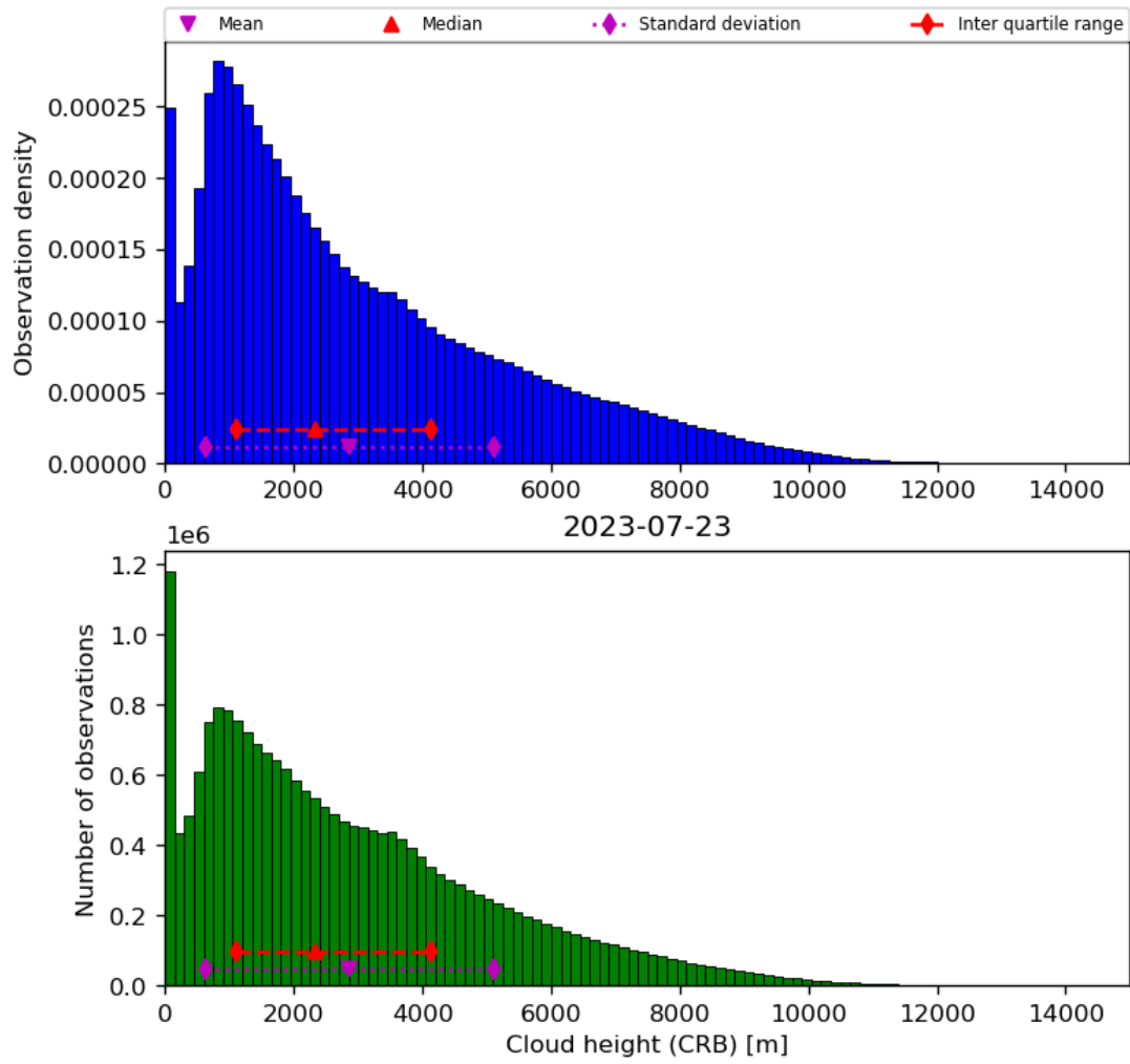
Figure 43: Histogram of “Cloud height (CRB)” for 2023-07-22 to 2023-07-24
