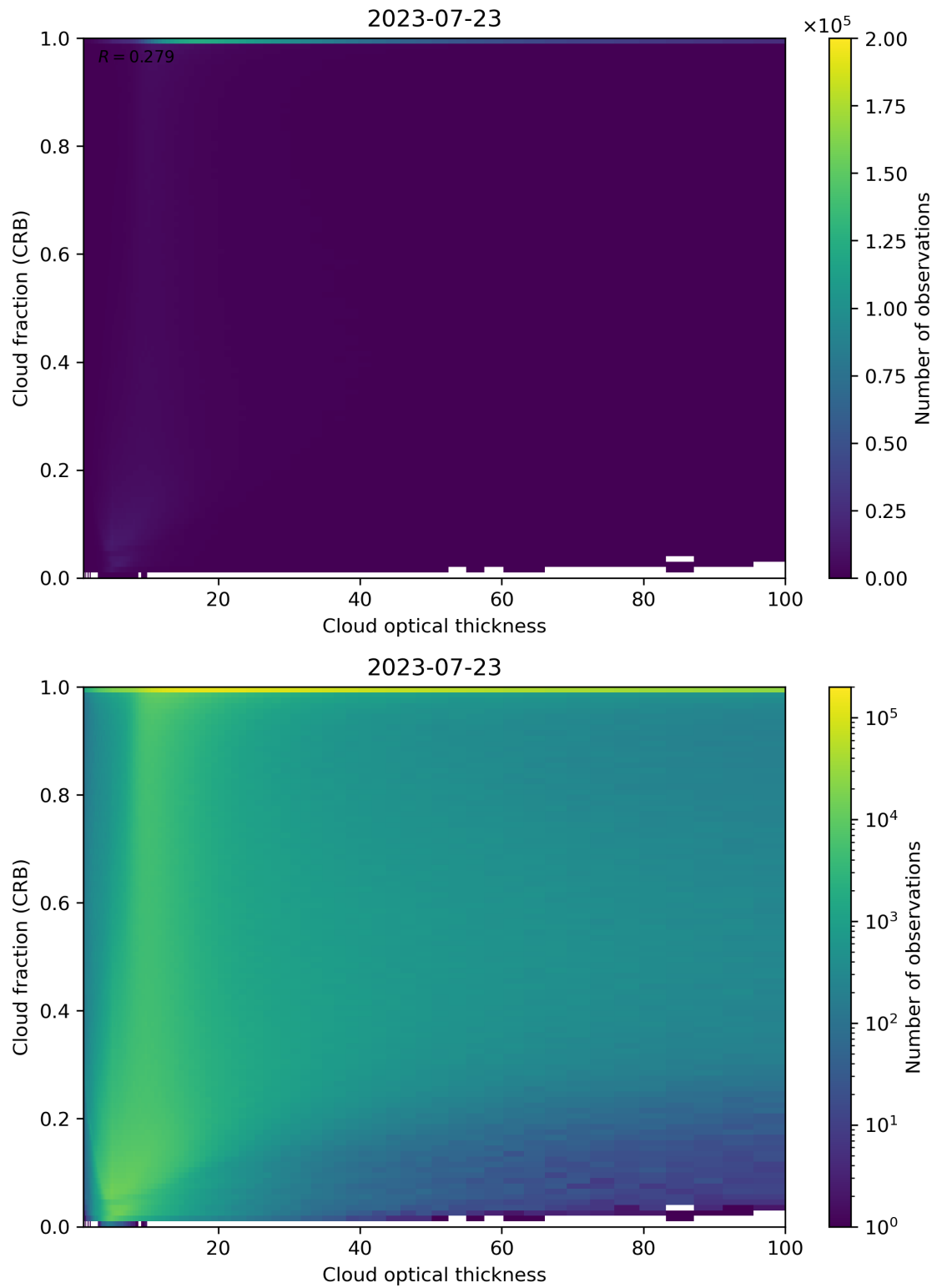
Figure 84: Scatter density plot of “Cloud optical thickness” against “Cloud fraction (CRB)” for 2023-07-22 to 2023-07-24.
