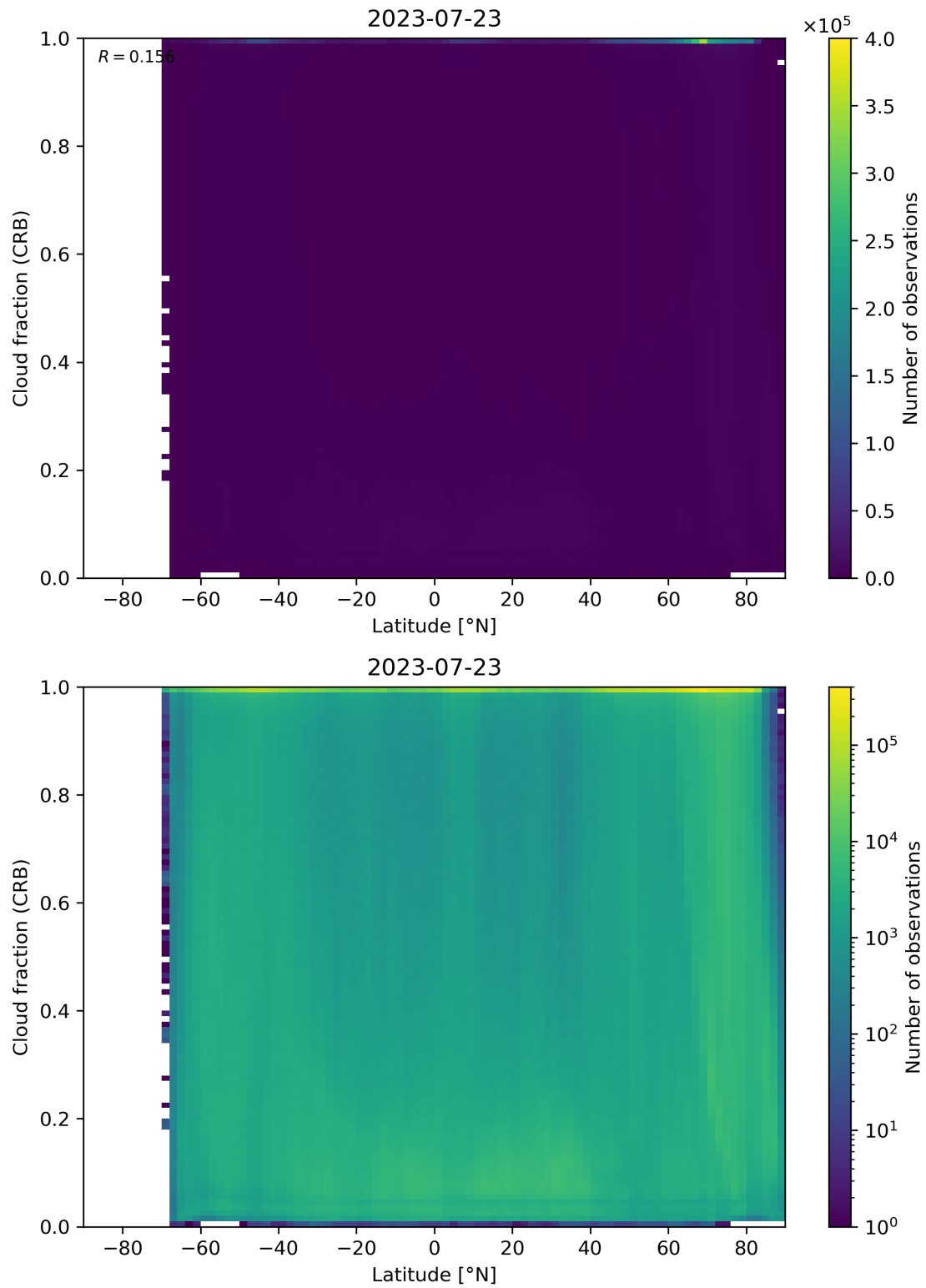
Figure 94: Scatter density plot of “Latitude” against “Cloud fraction (CRB)” for 2023-07-22 to 2023-07-24.
