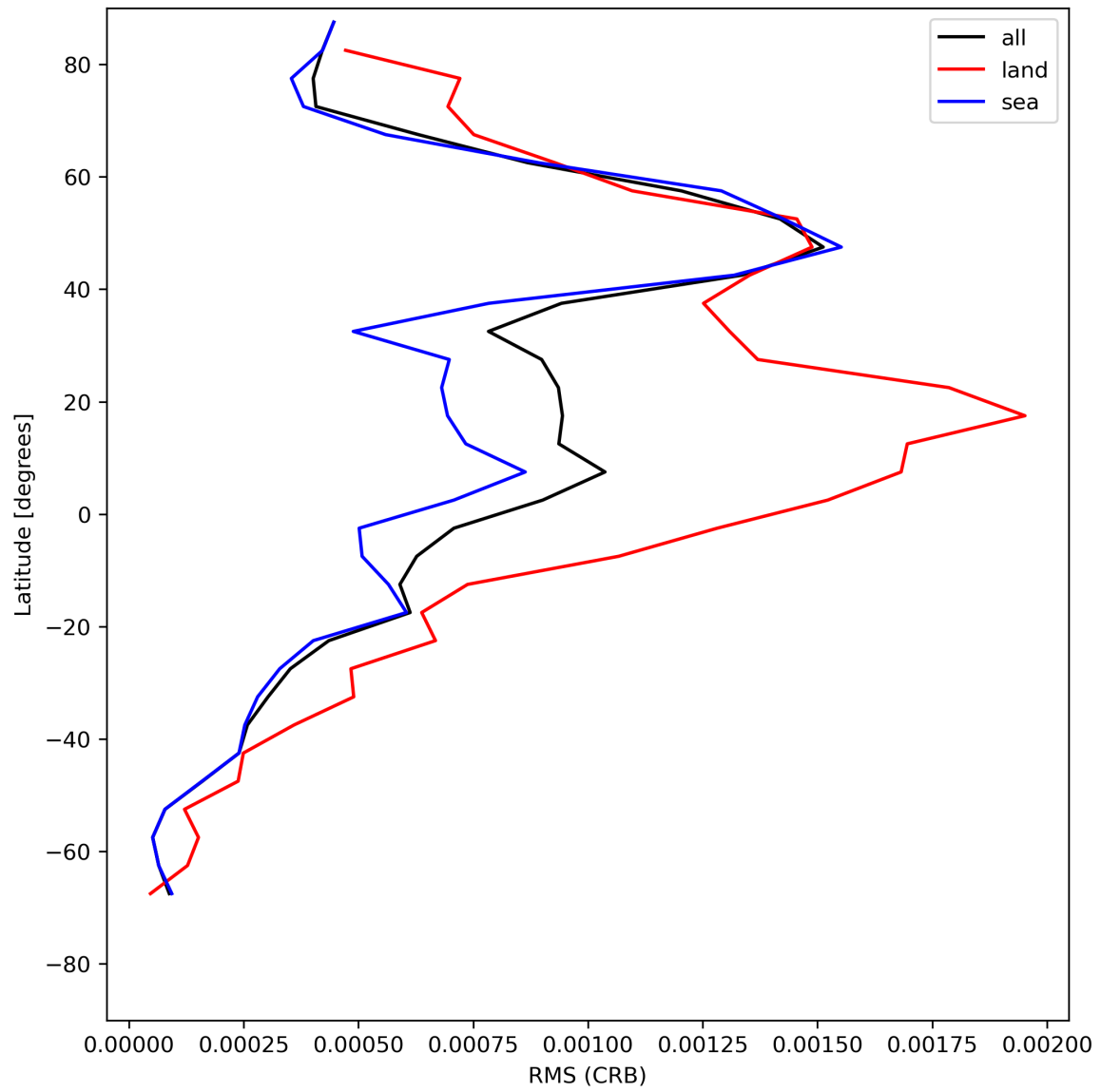
Figure 32: Zonal average of “RMS (CRB)” for 2023-07-22 to 2023-07-24.
