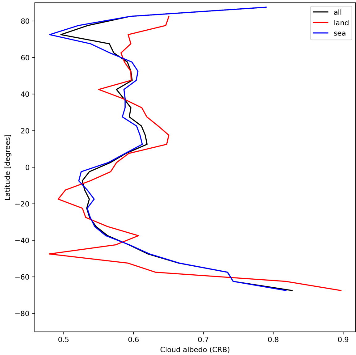
Figure 28: Zonal average of “Cloud albedo (CRB)” for 2023-07-22 to 2023-07-24.
