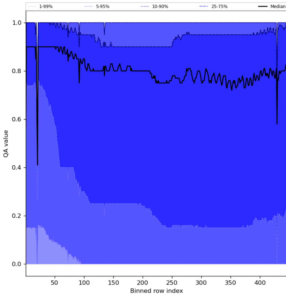
Figure 54: Along track statistics of “QA value” for 2023-07-22 to 2023-07-24
