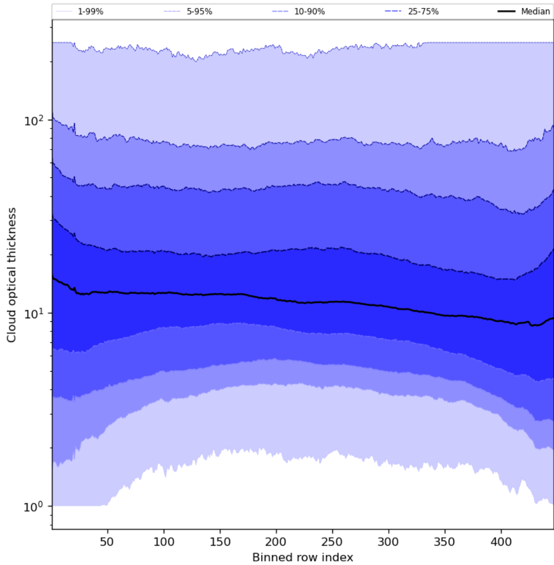
Figure 57: Along track statistics of “Cloud optical thickness” for 2023-07-22 to 2023-07-24
