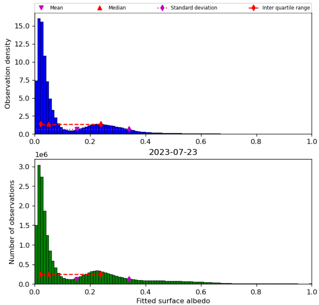
Figure 45: Histogram of “Fitted surface albedo” for 2023-07-22 to 2023-07-24
