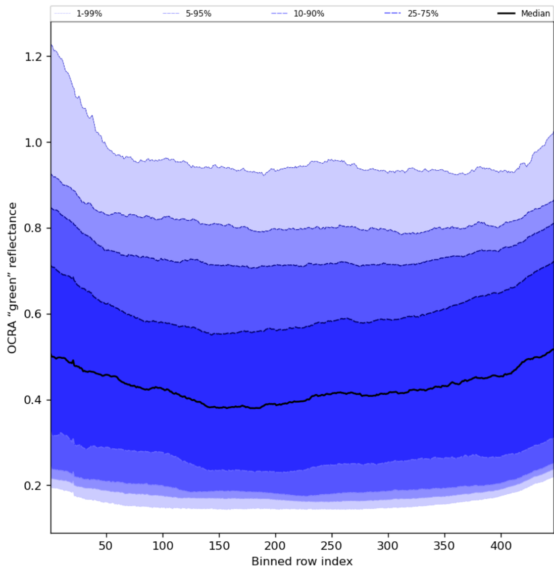
Figure 68: Along track statistics of “OCRA “green” reflectance” for 2023-07-22 to 2023-07-24
