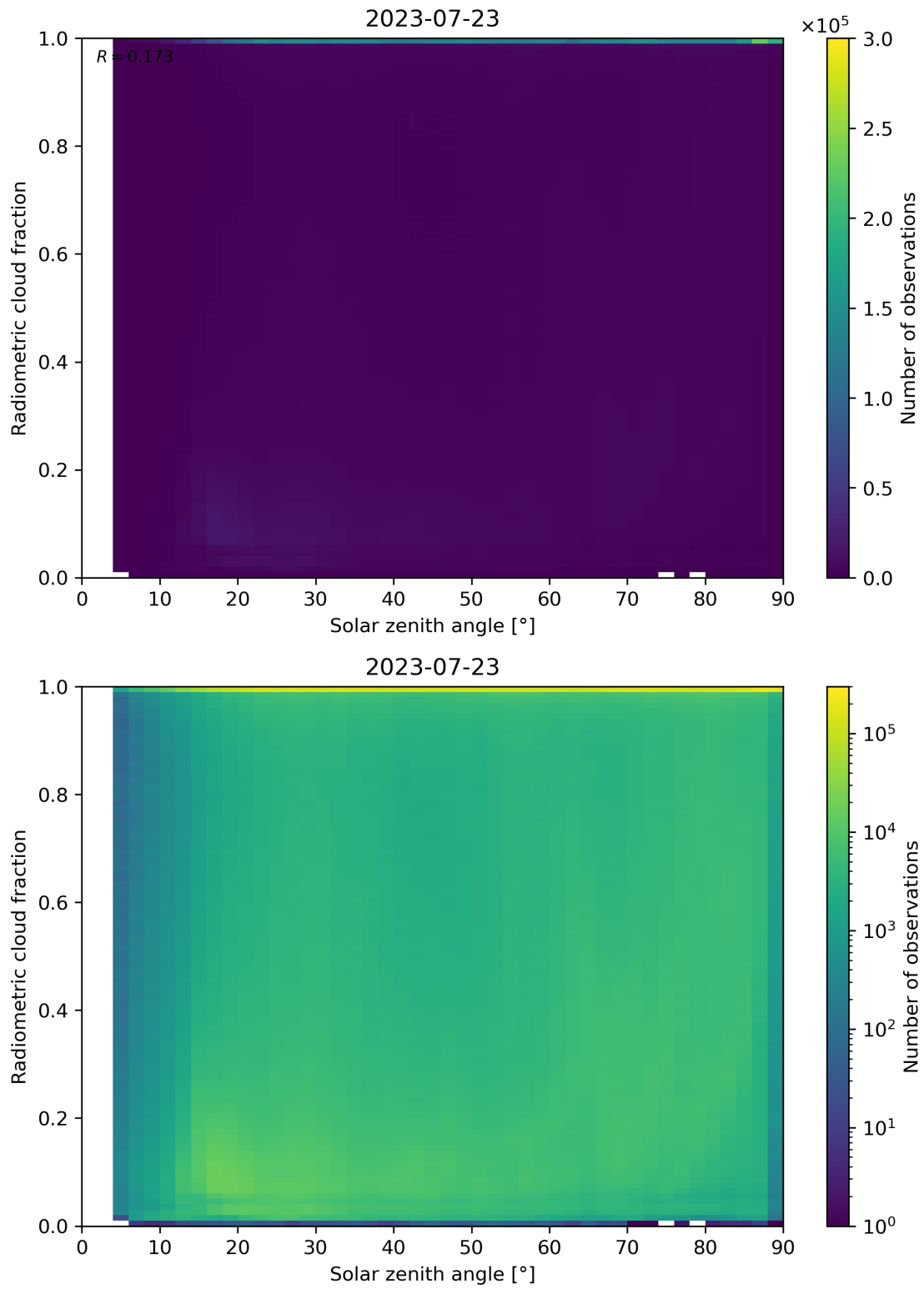
Figure 99: Scatter density plot of “Solar zenith angle” against “Radiometric cloud fraction” for 2023-07-22 to 2023-07-24.
