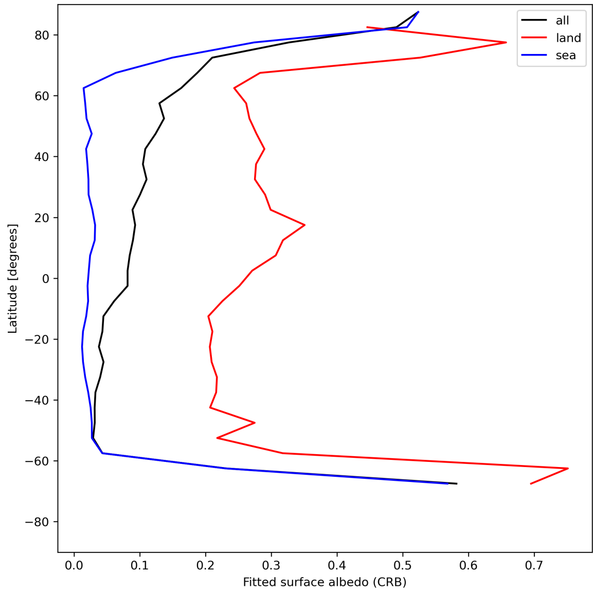
Figure 30: Zonal average of “Fitted surface albedo (CRB)” for 2023-07-22 to 2023-07-24.
