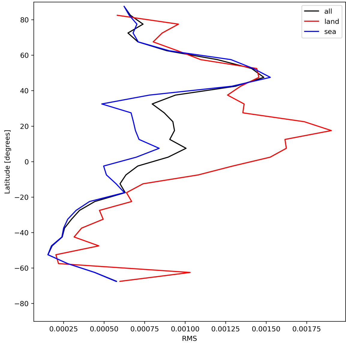
Figure 31: Zonal average of “RMS” for 2023-07-22 to 2023-07-24.
