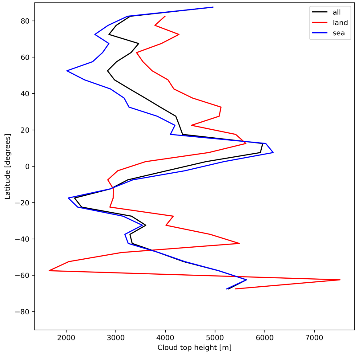
Figure 24: Zonal average of “Cloud top height” for 2023-07-22 to 2023-07-24.
