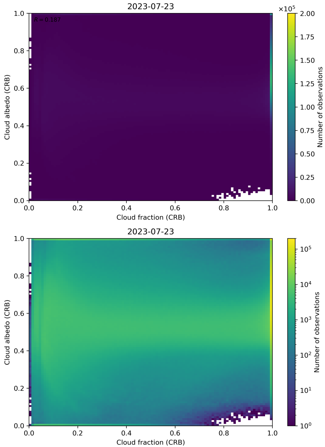
Figure 77: Scatter density plot of “Cloud fraction (CRB)” against “Cloud albedo (CRB)” for 2023-07-22 to 2023-07-24.
