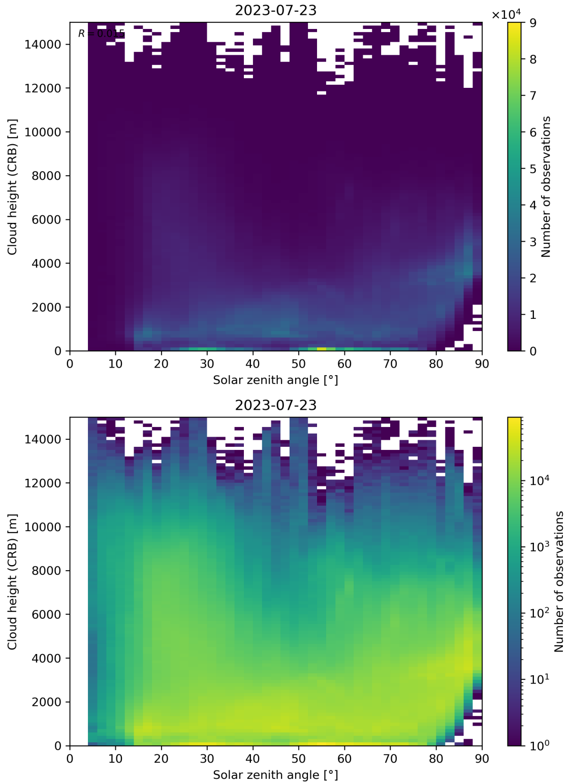
Figure 102: Scatter density plot of “Solar zenith angle” against “Cloud height (CRB)” for 2023-07-22 to 2023-07-24.
