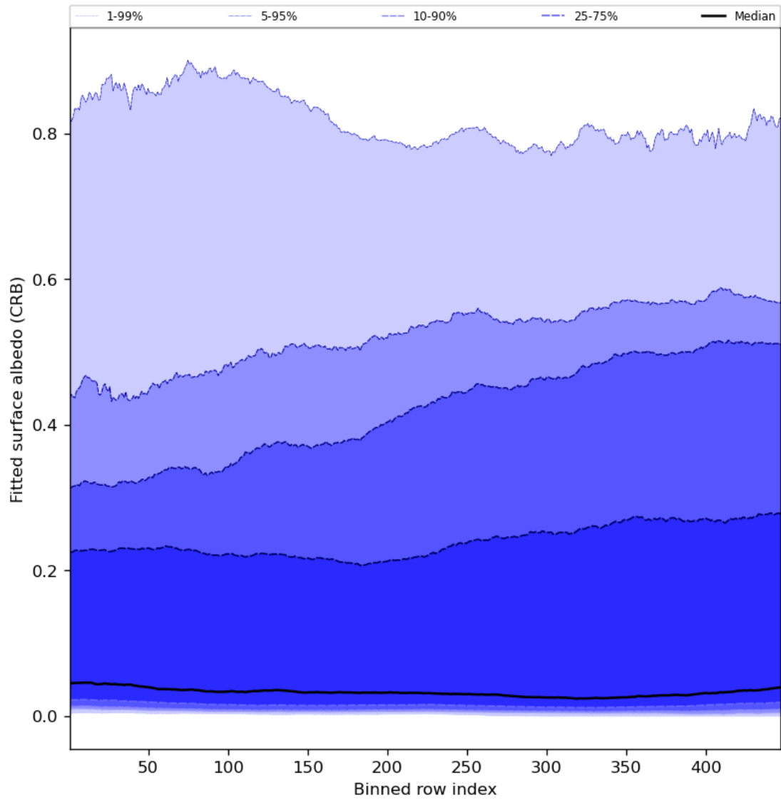
Figure 62: Along track statistics of “Fitted surface albedo (CRB)” for 2023-07-22 to 2023-07-24
