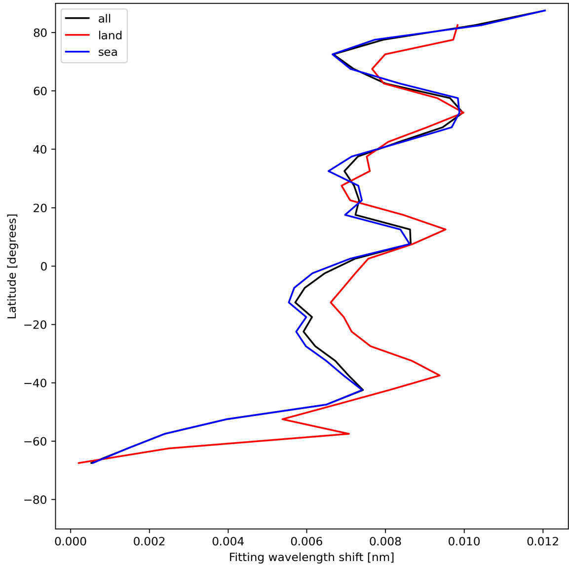
Figure 33: Zonal average of “Fitting wavelength shift” for 2023-07-22 to 2023-07-24.
