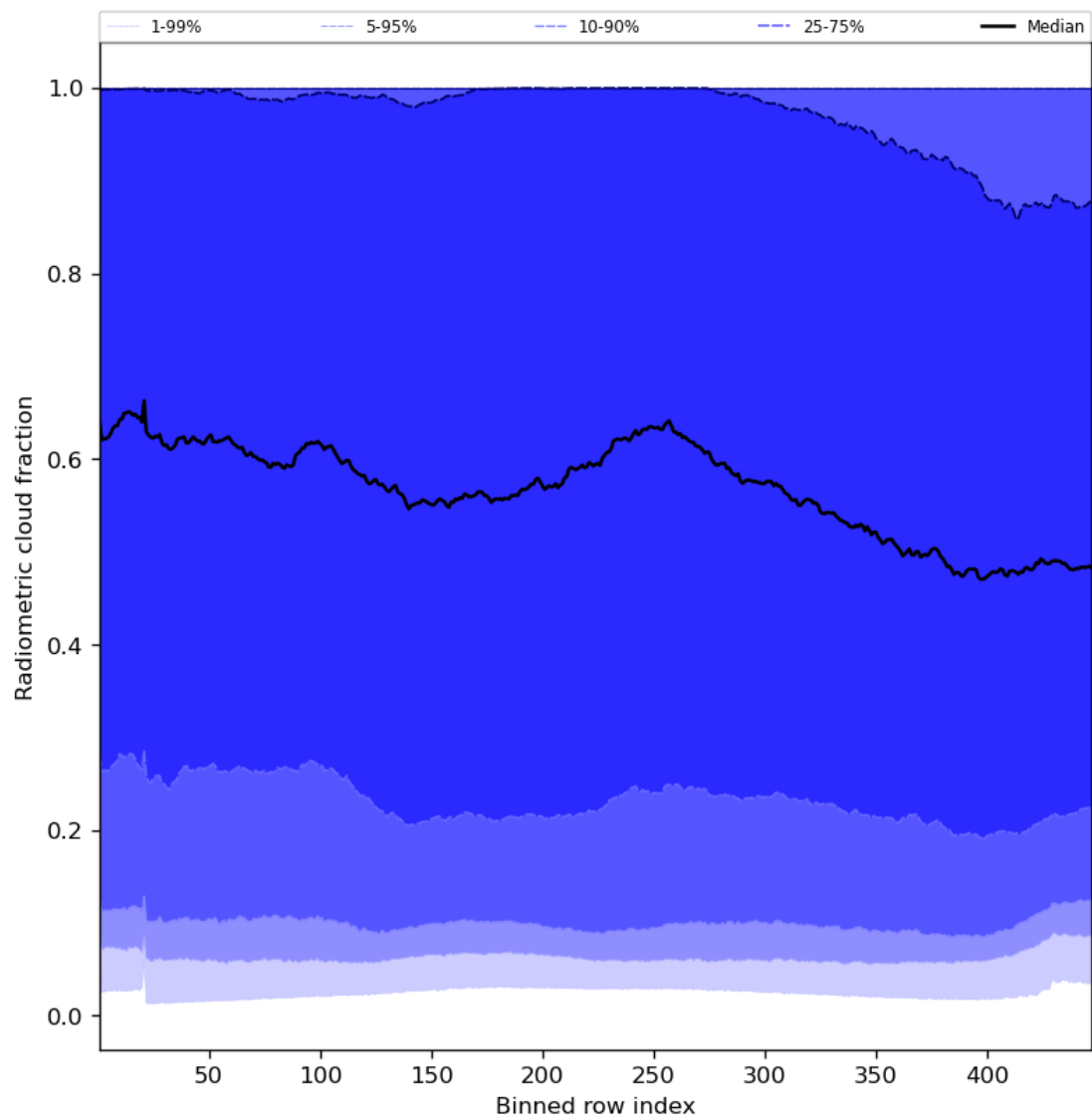
Figure 55: Along track statistics of “Radiometric cloud fraction” for 2023-07-22 to 2023-07-24
