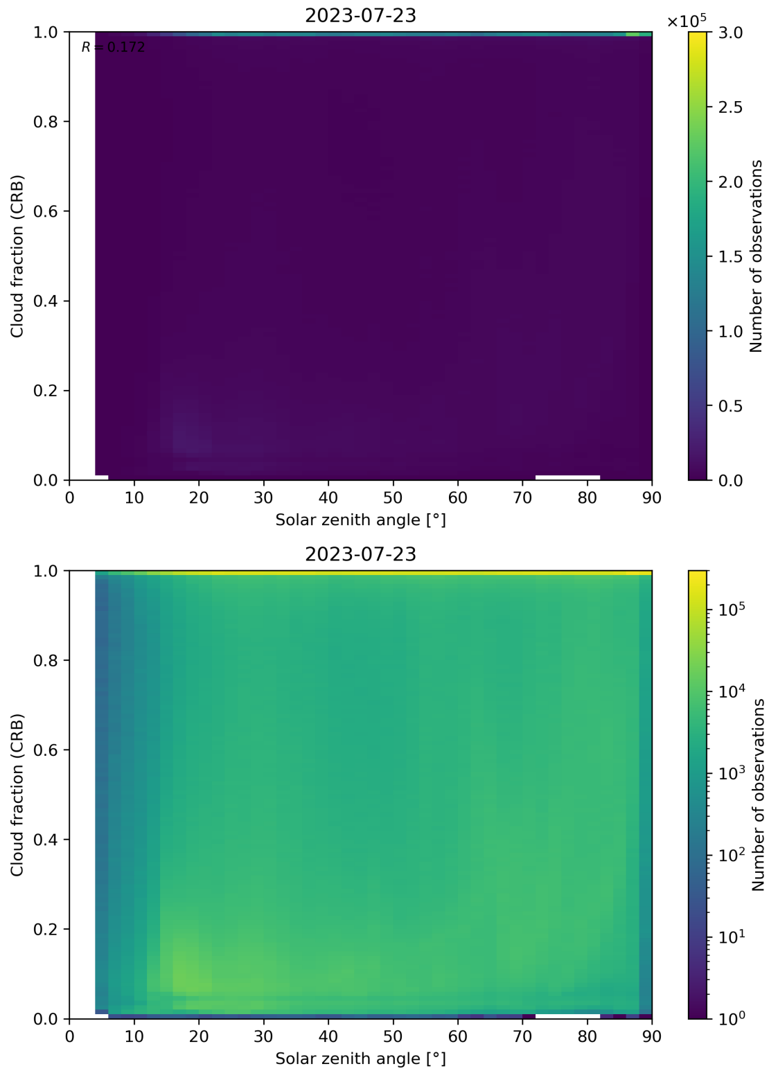
Figure 101: Scatter density plot of “Solar zenith angle” against “Cloud fraction (CRB)” for 2023-07-22 to 2023-07-24.
