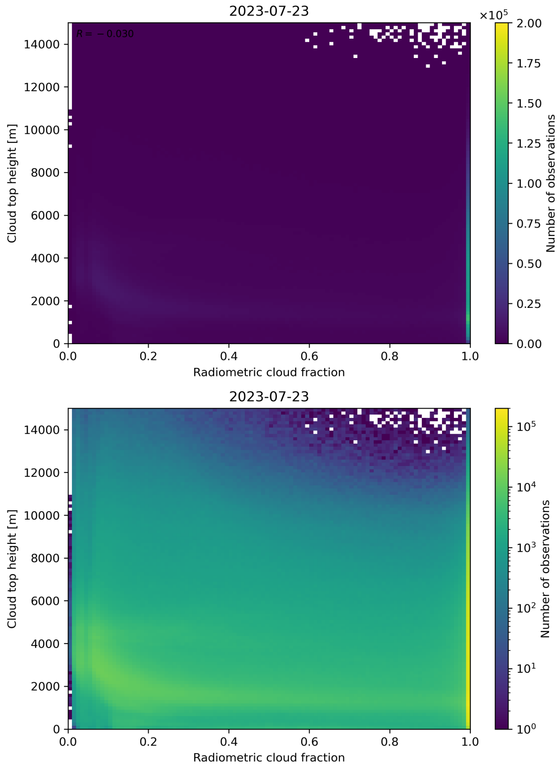
Figure 76: Scatter density plot of “Radiometric cloud fraction” against “Cloud top height” for 2023-07-22 to 2023-07-24.
