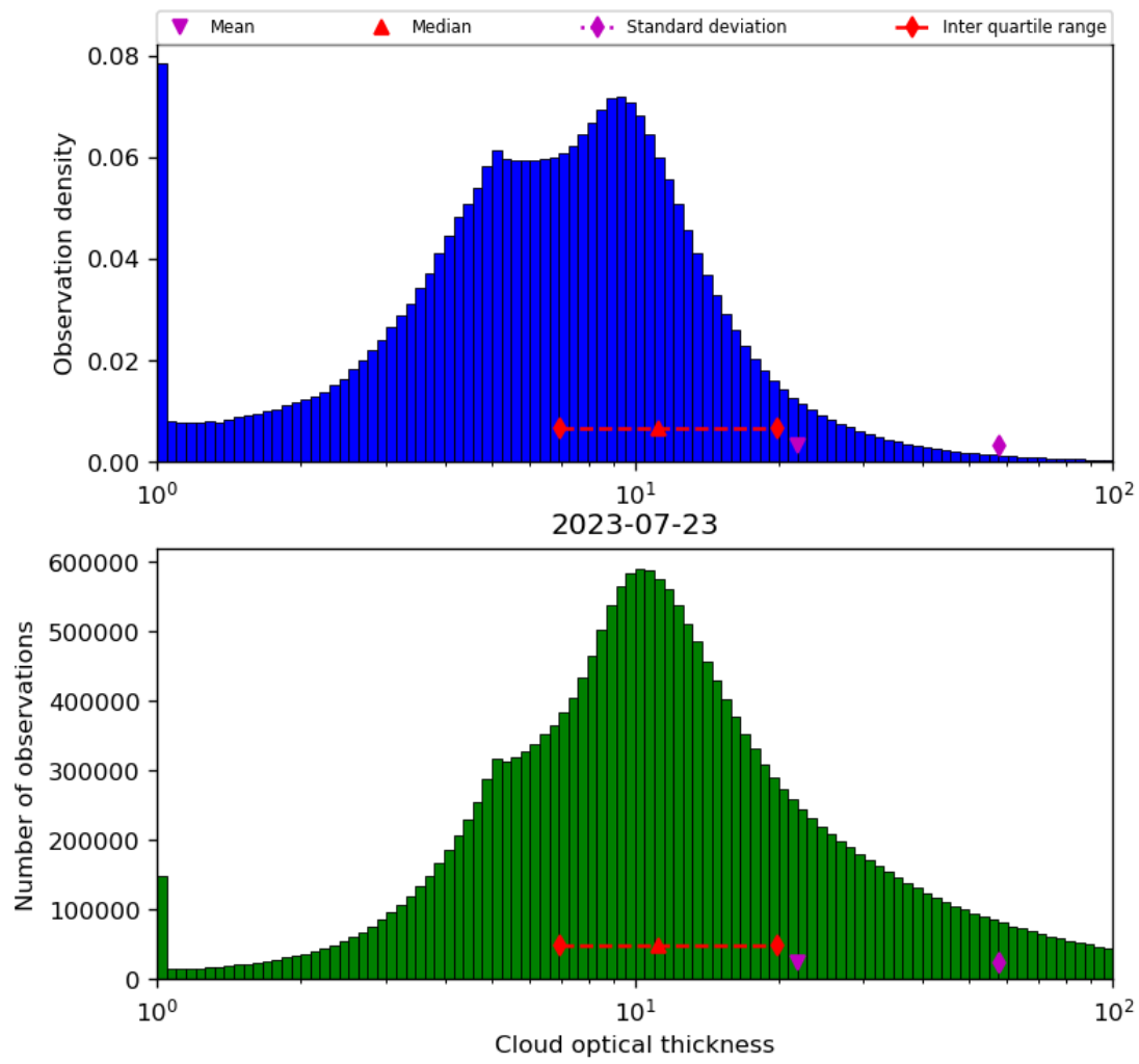
Figure 41: Histogram of “Cloud optical thickness” for 2023-07-22 to 2023-07-24
