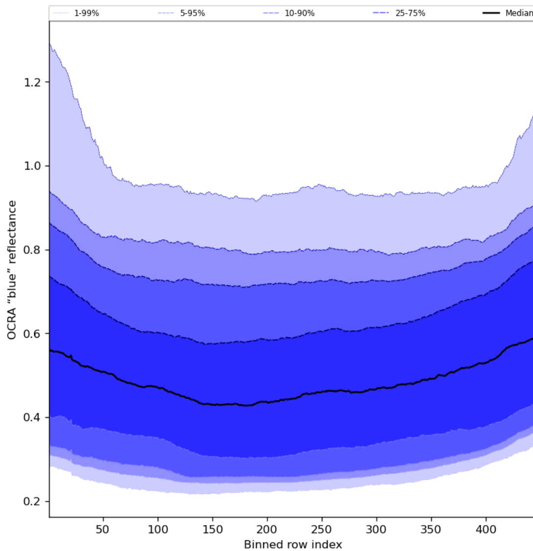
Figure 67: Along track statistics of “OCRA “blue” reflectance” for 2023-07-22 to 2023-07-24
