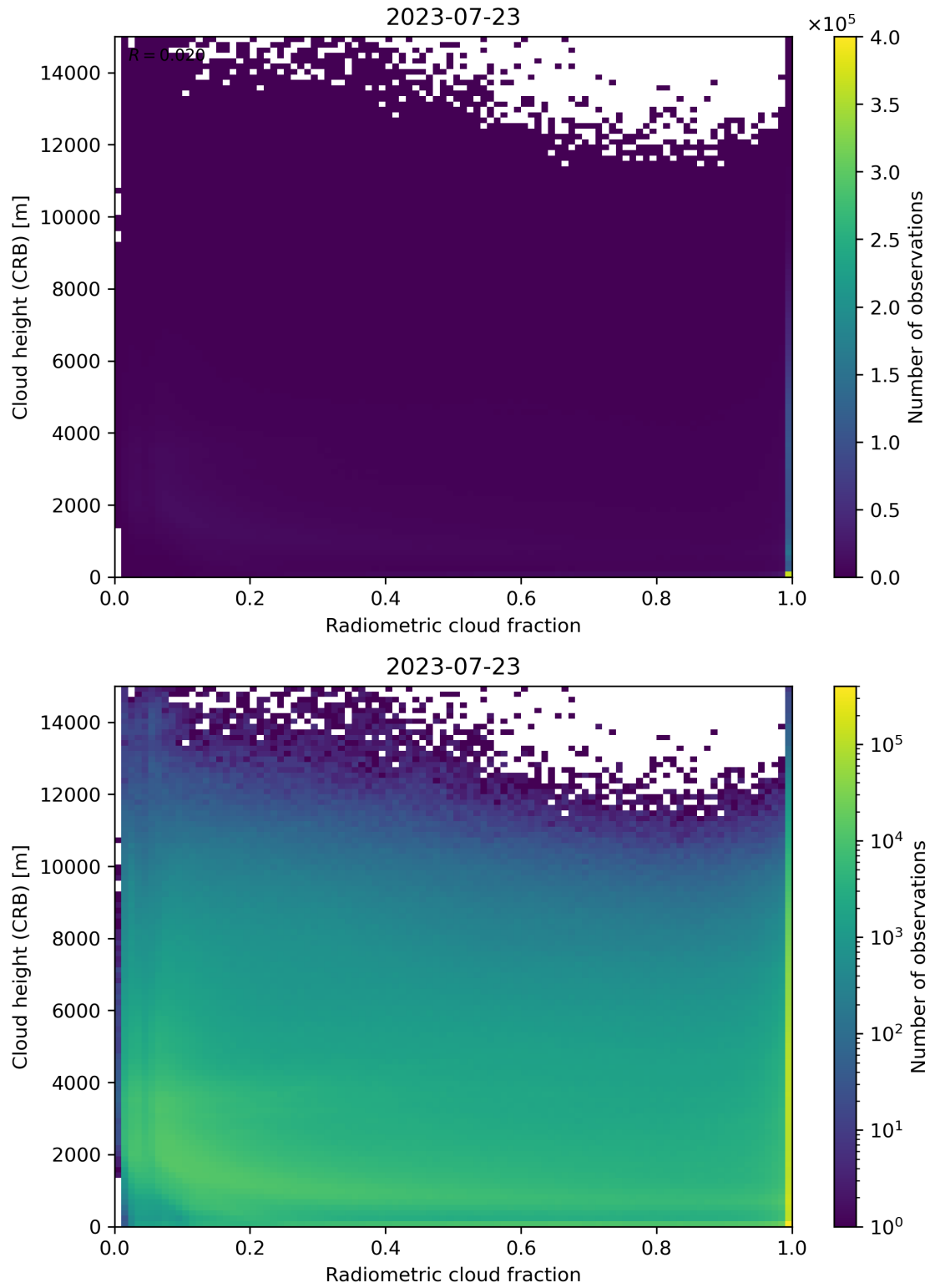
Figure 74: Scatter density plot of “Radiometric cloud fraction” against “Cloud height (CRB)” for 2023-07-22 to 2023-07-24.
