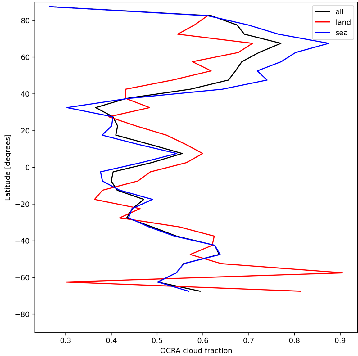
Figure 34: Zonal average of “OCRA cloud fraction” for 2023-07-22 to 2023-07-24.
