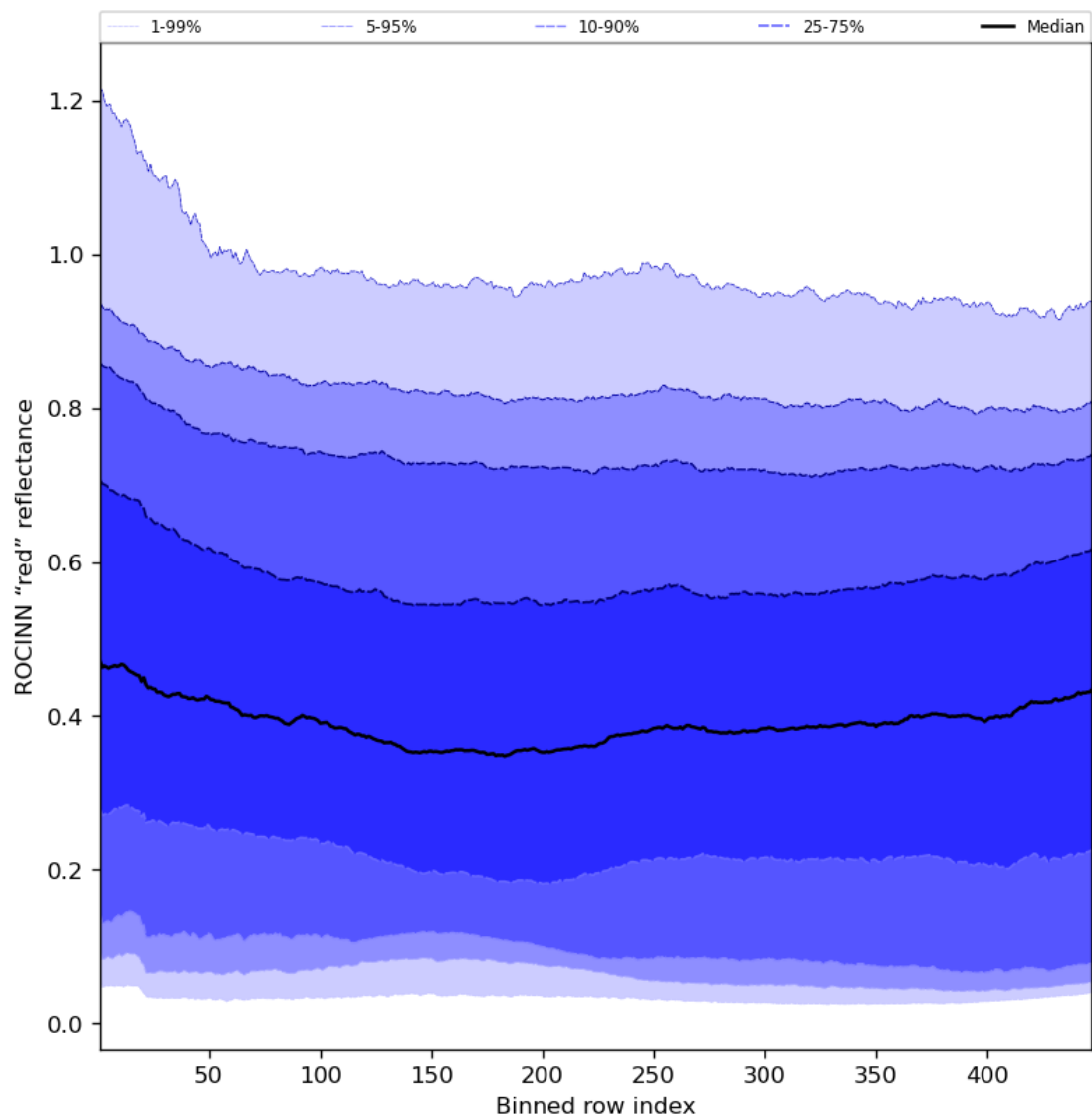
Figure 69: Along track statistics of “ROCINN “red” reflectance” for 2023-07-22 to 2023-07-24
