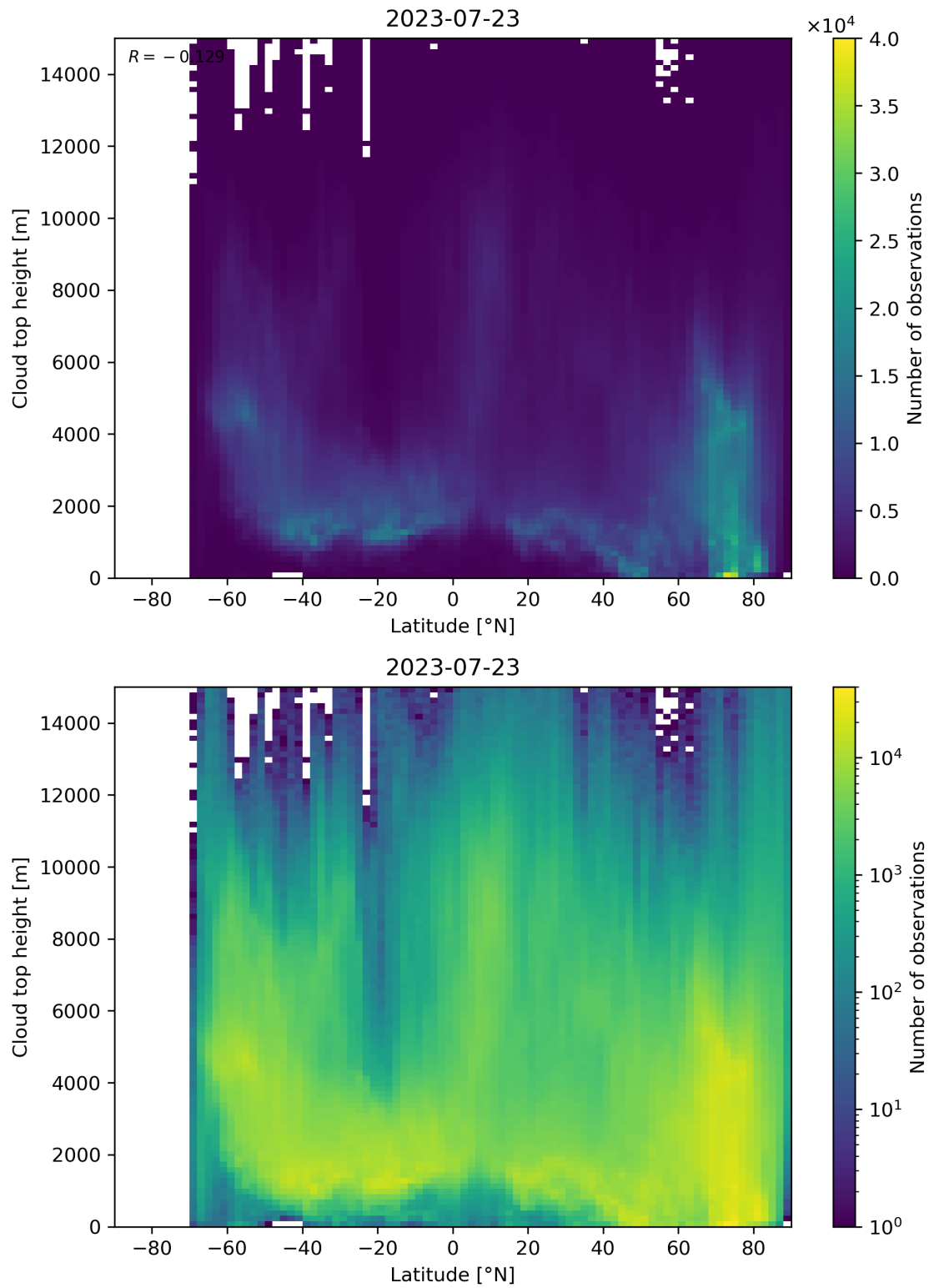
Figure 97: Scatter density plot of “Latitude” against “Cloud top height” for 2023-07-22 to 2023-07-24.
