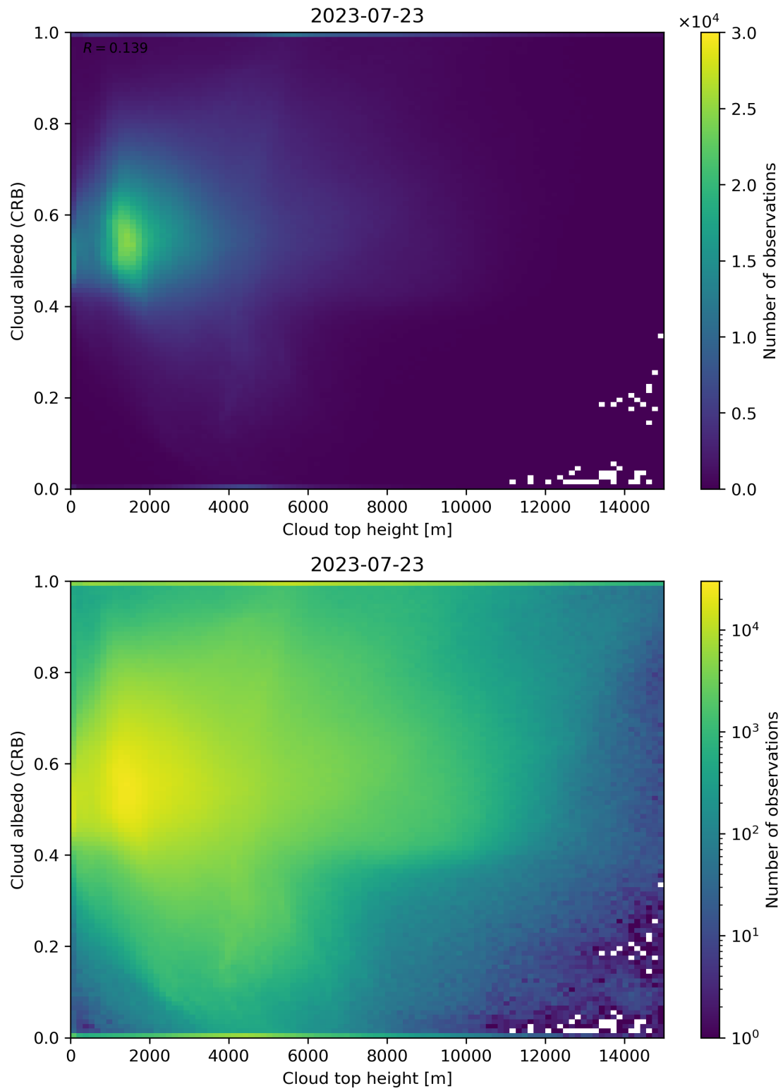
Figure 86: Scatter density plot of “Cloud top height” against “Cloud albedo (CRB)” for 2023-07-22 to 2023-07-24.
