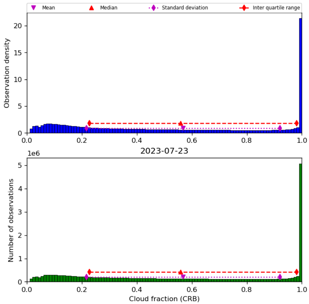
Figure 42: Histogram of “Cloud fraction (CRB)” for 2023-07-22 to 2023-07-24
