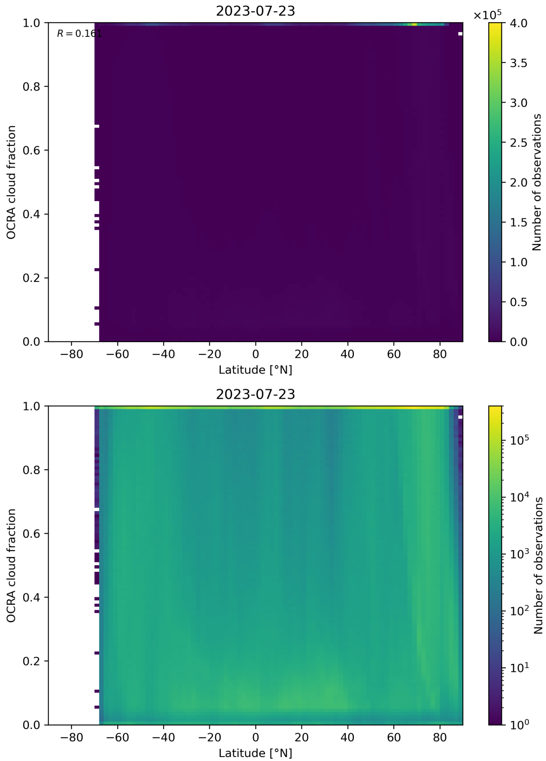
Figure 93: Scatter density plot of “Latitude” against “OCRA cloud fraction” for 2023-07-22 to 2023-07-24.
