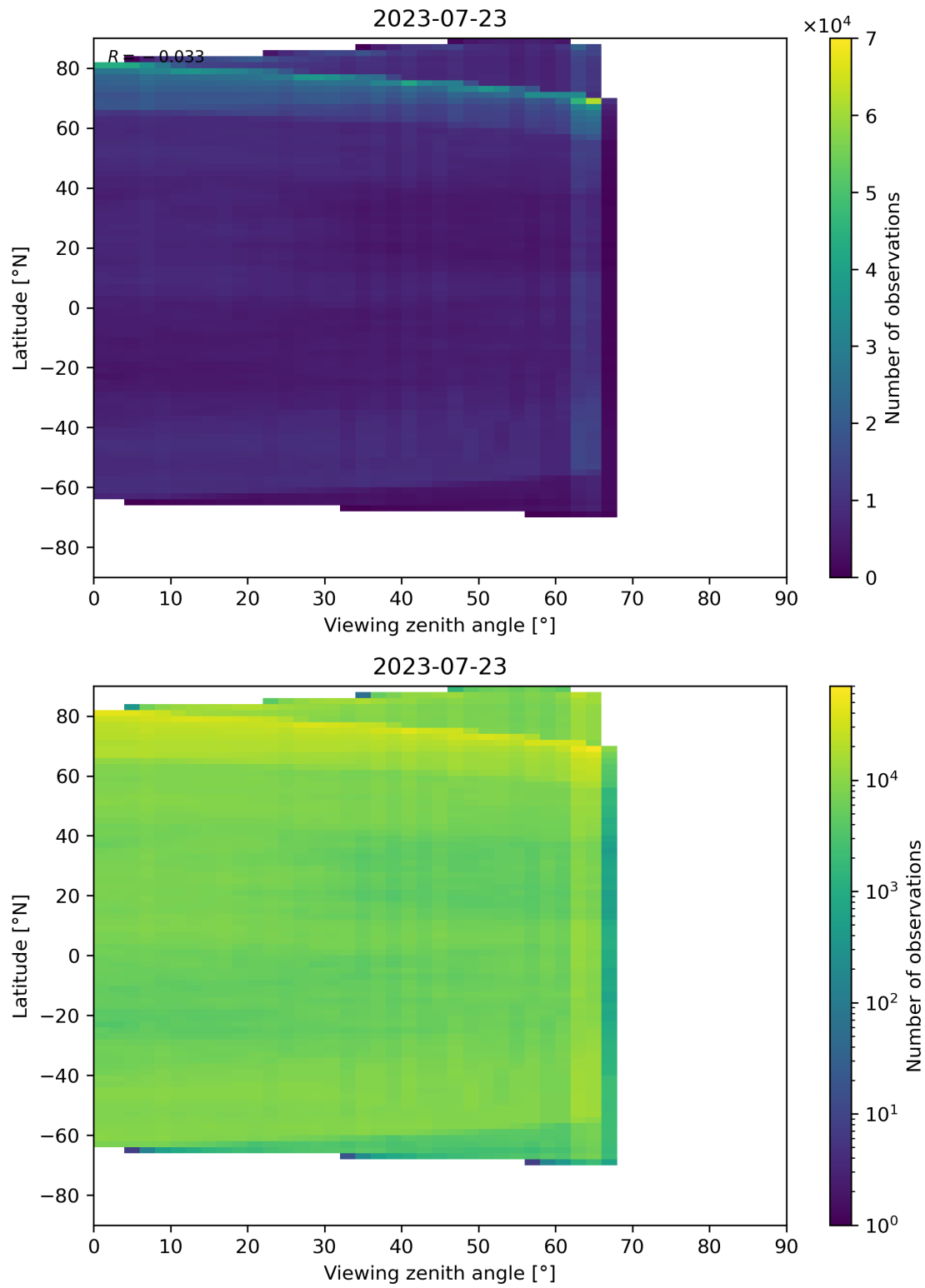
Figure 113: Scatter density plot of “Viewing zenith angle” against “Latitude” for 2023-07-22 to 2023-07-24.
