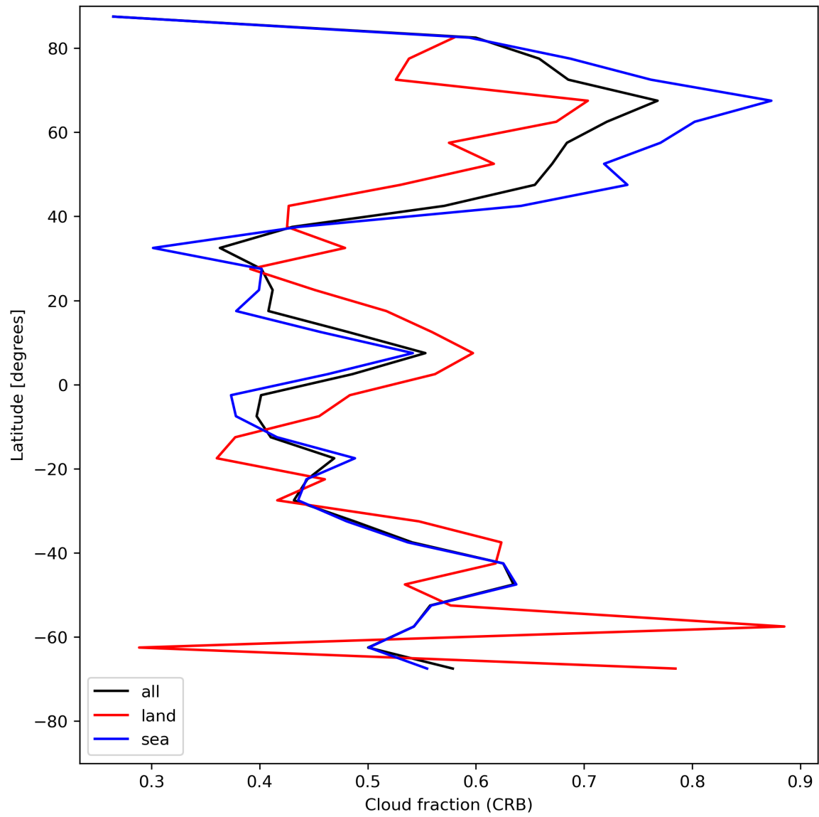
Figure 26: Zonal average of “Cloud fraction (CRB)” for 2023-07-22 to 2023-07-24.
