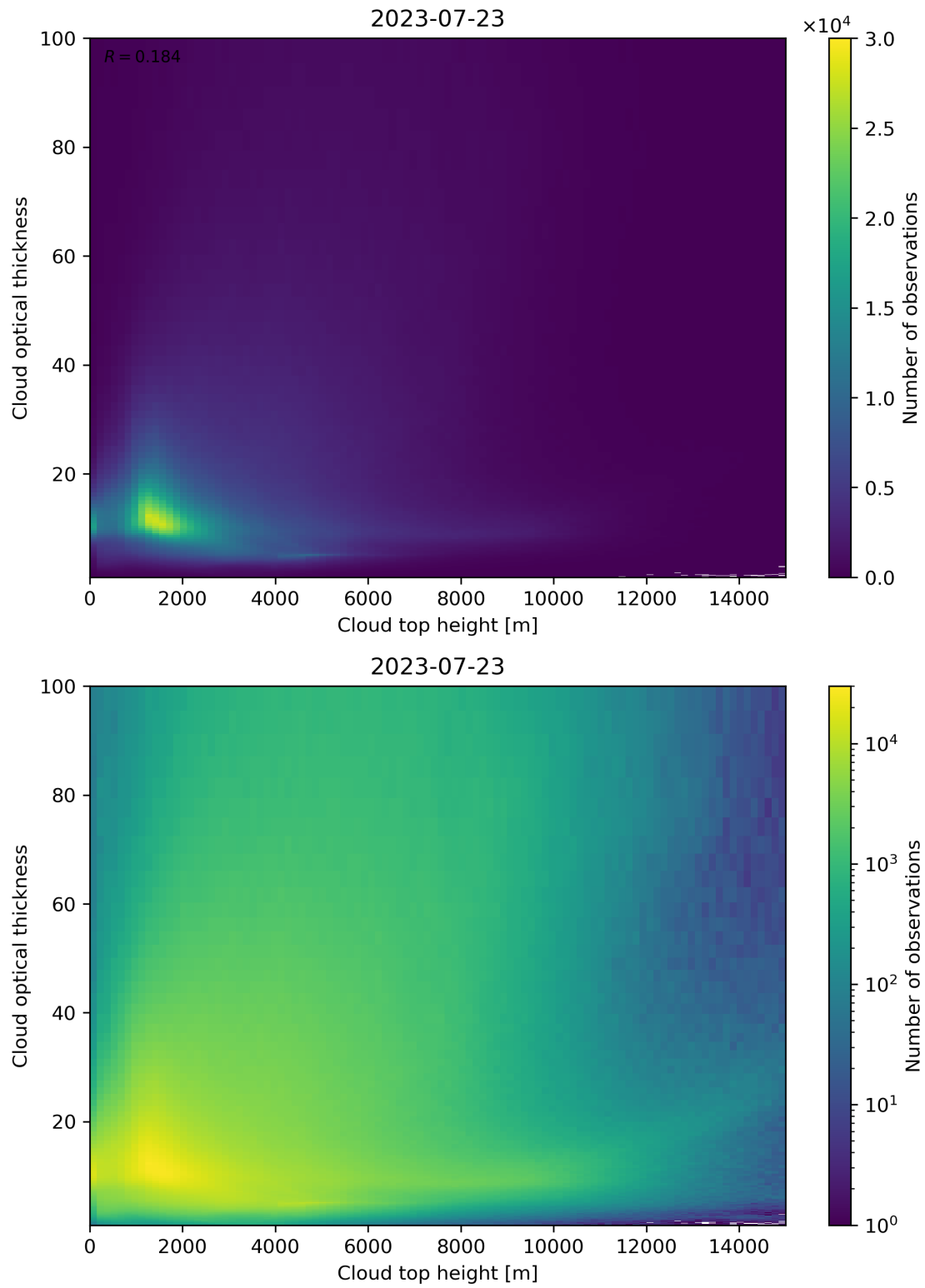
Figure 90: Scatter density plot of “Cloud top height” against “Cloud optical thickness” for 2023-07-22 to 2023-07-24.
