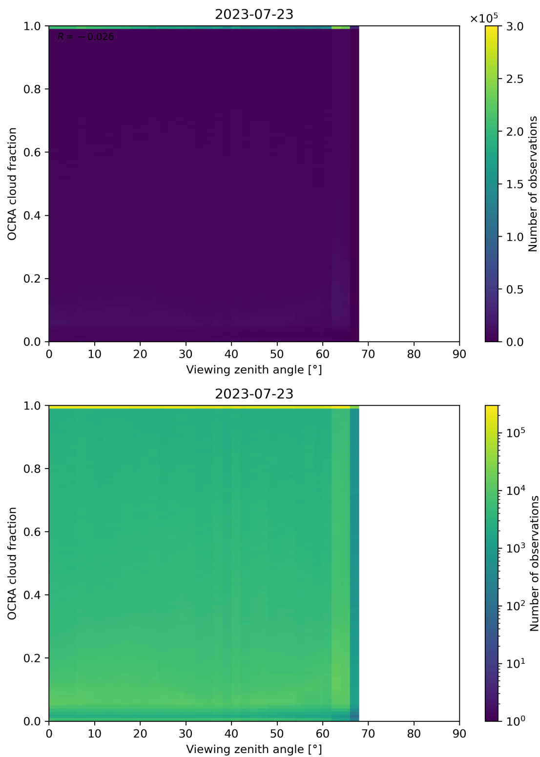
Figure 108: Scatter density plot of “Viewing zenith angle” against “OCRA cloud fraction” for 2023-07-22 to 2023-07-24.
