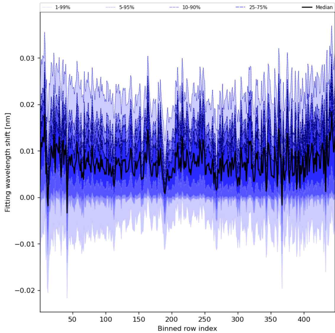
Figure 65: Along track statistics of “Fitting wavelength shift” for 2023-07-22 to 2023-07-24
