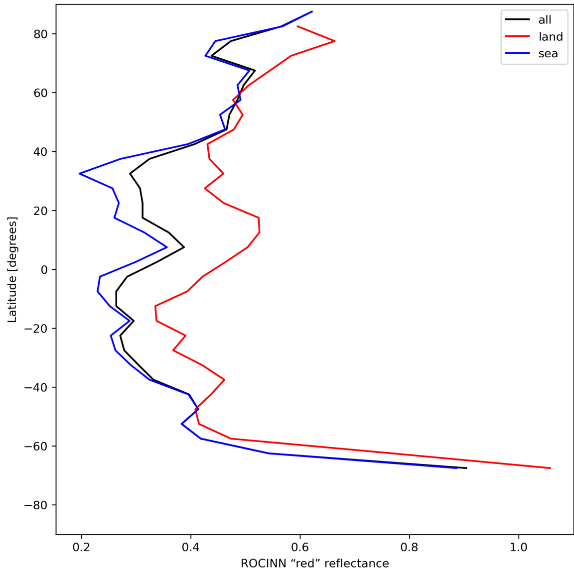
Figure 37: Zonal average of “ROCINN “red” reflectance” for 2023-07-22 to 2023-07-24.
