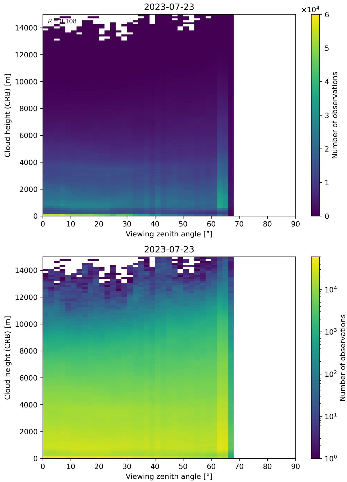
Figure 110: Scatter density plot of “Viewing zenith angle” against “Cloud height (CRB)” for 2023-07-22 to 2023-07-24.
