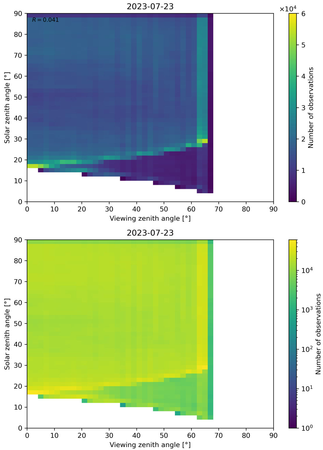
Figure 114: Scatter density plot of “Viewing zenith angle” against “Solar zenith angle” for 2023-07-22 to 2023-07-24.
