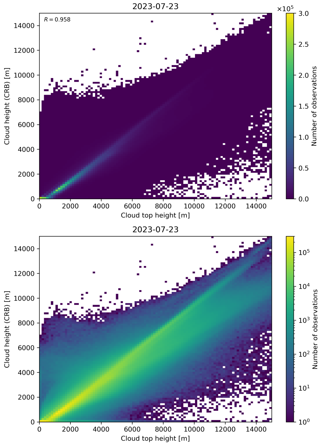
Figure 89: Scatter density plot of “Cloud top height” against “Cloud height (CRB)” for 2023-07-22 to 2023-07-24.
