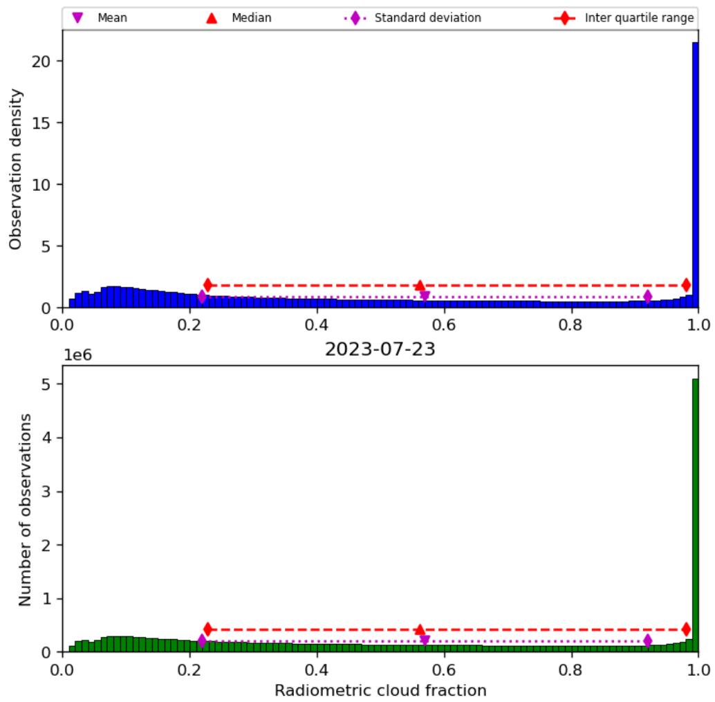
Figure 39: Histogram of “Radiometric cloud fraction” for 2023-07-22 to 2023-07-24
