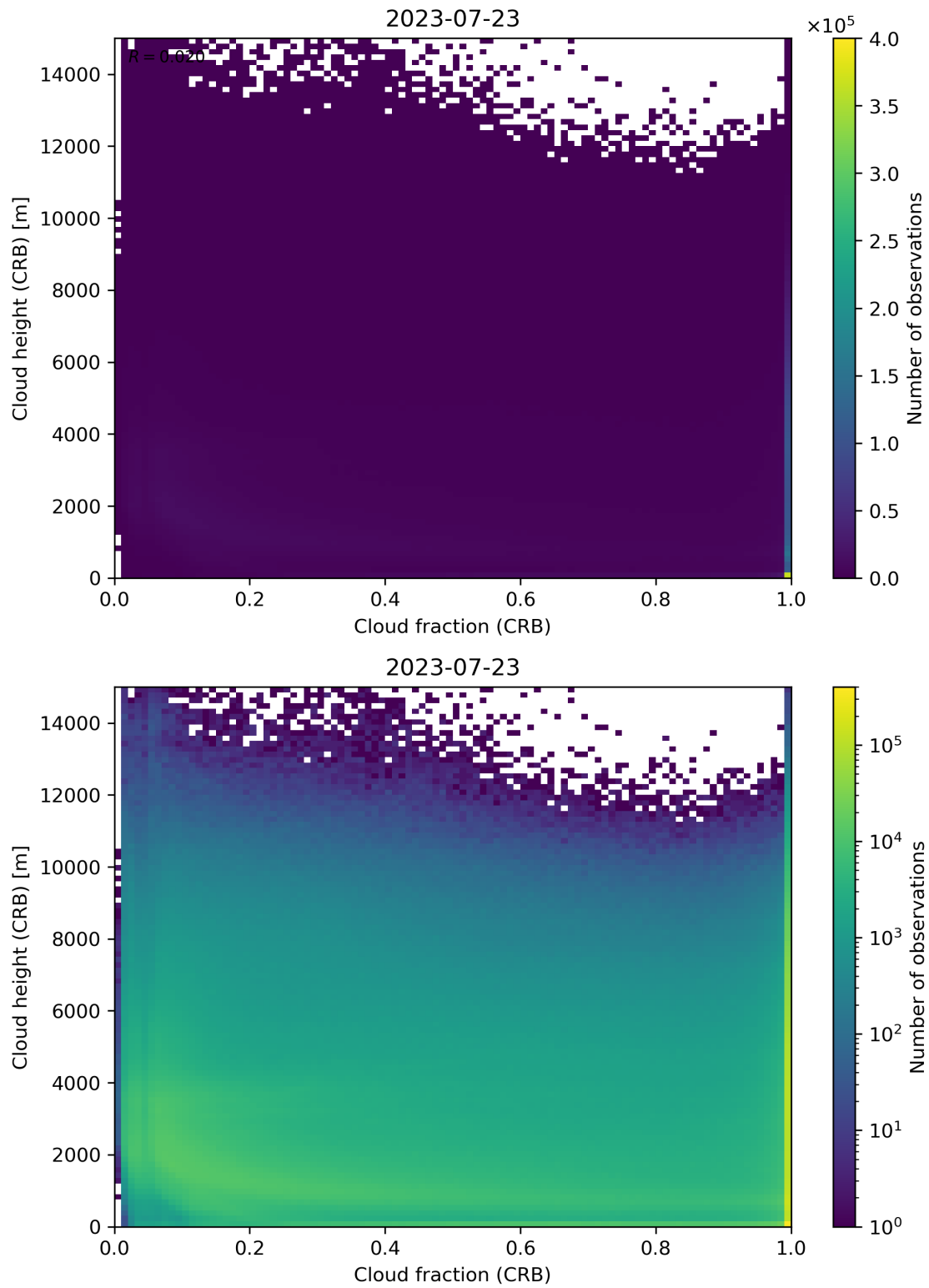
Figure 79: Scatter density plot of “Cloud fraction (CRB)” against “Cloud height (CRB)” for 2023-07-22 to 2023-07-24.
