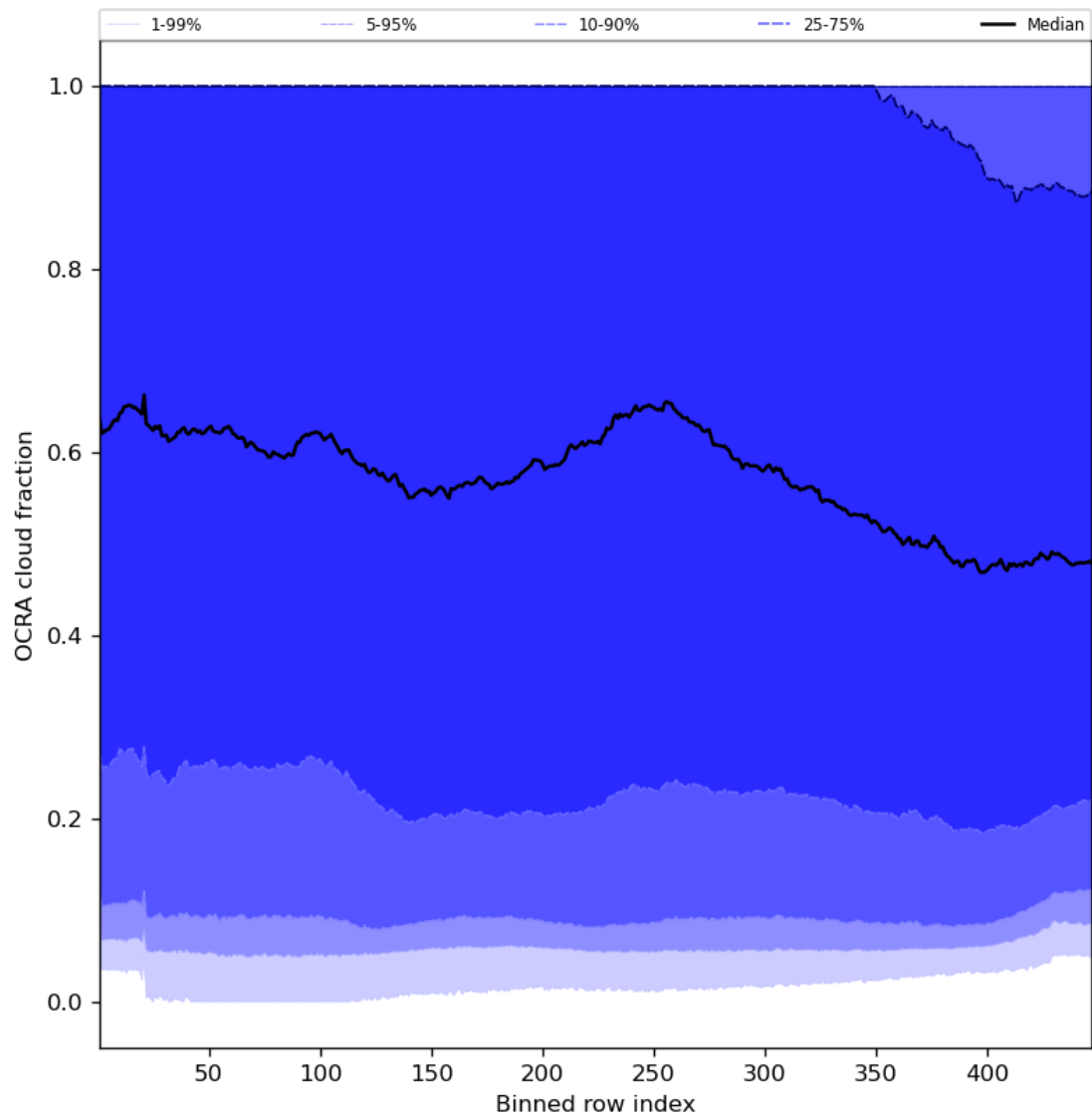
Figure 66: Along track statistics of “OCRA cloud fraction” for 2023-07-22 to 2023-07-24
