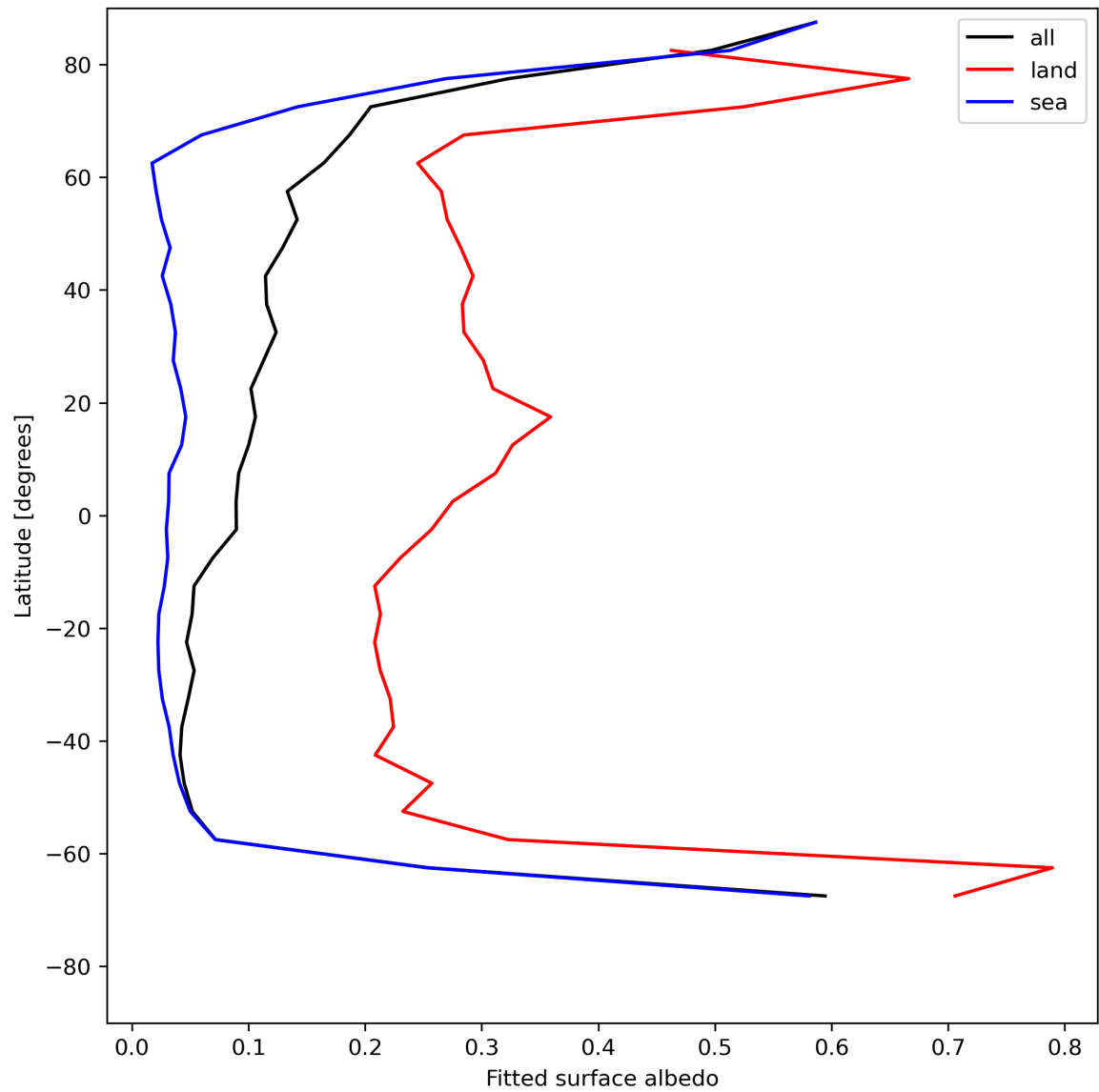
Figure 29: Zonal average of “Fitted surface albedo” for 2023-07-22 to 2023-07-24.
