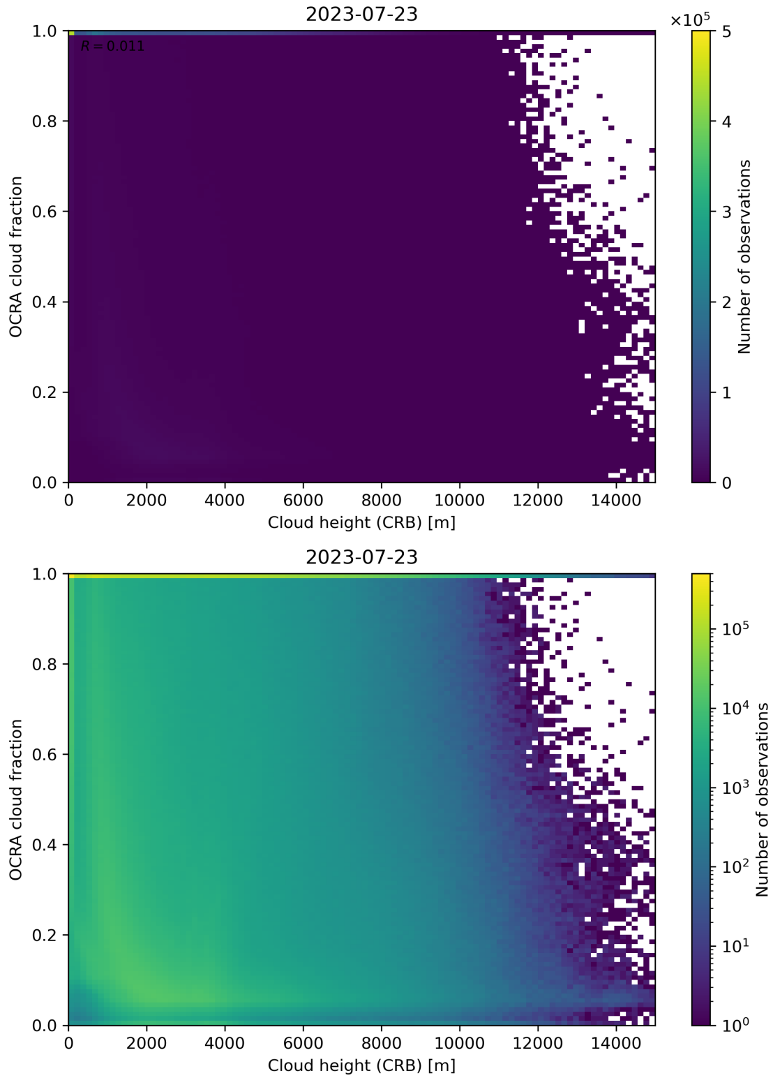
Figure 81: Scatter density plot of “Cloud height (CRB)” against “OCRA cloud fraction” for 2023-07-22 to 2023-07-24.
