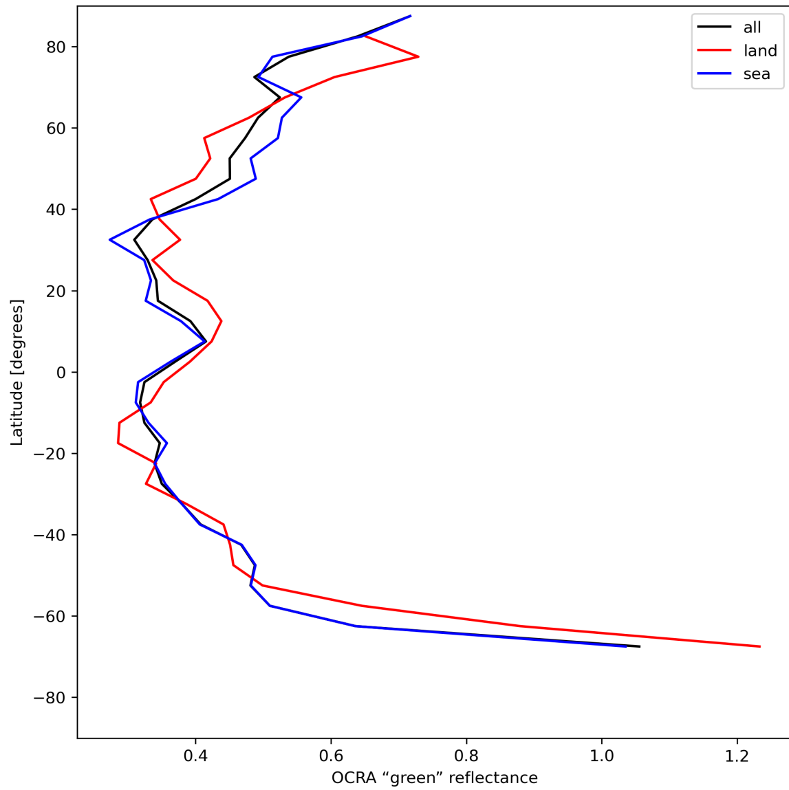
Figure 36: Zonal average of “OCRA “green” reflectance” for 2023-07-22 to 2023-07-24.
