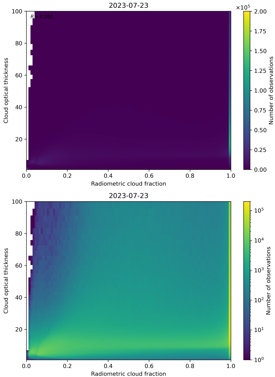
Figure 75: Scatter density plot of “Radiometric cloud fraction” against “Cloud optical thickness” for 2023-07-22 to 2023-07-24.
