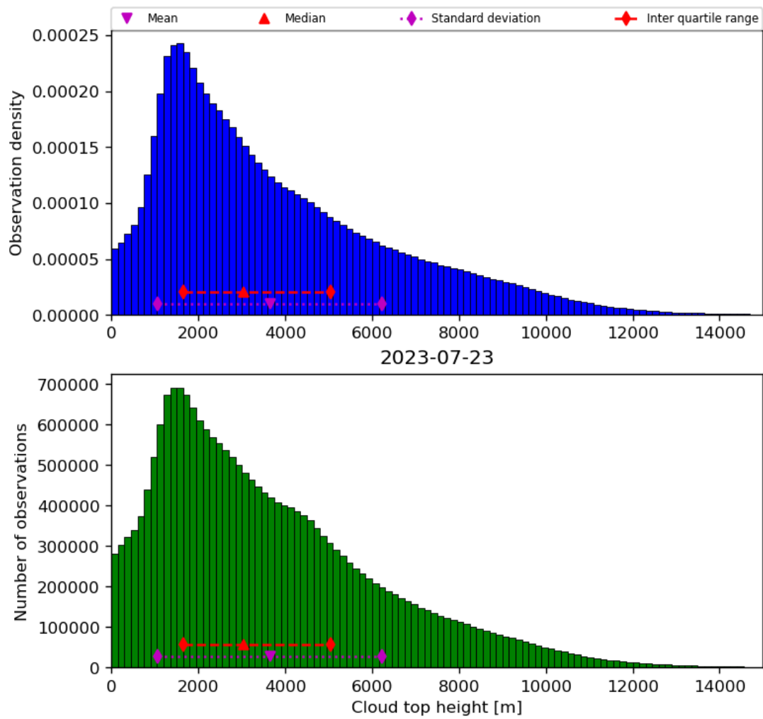
Figure 40: Histogram of “Cloud top height” for 2023-07-22 to 2023-07-24
