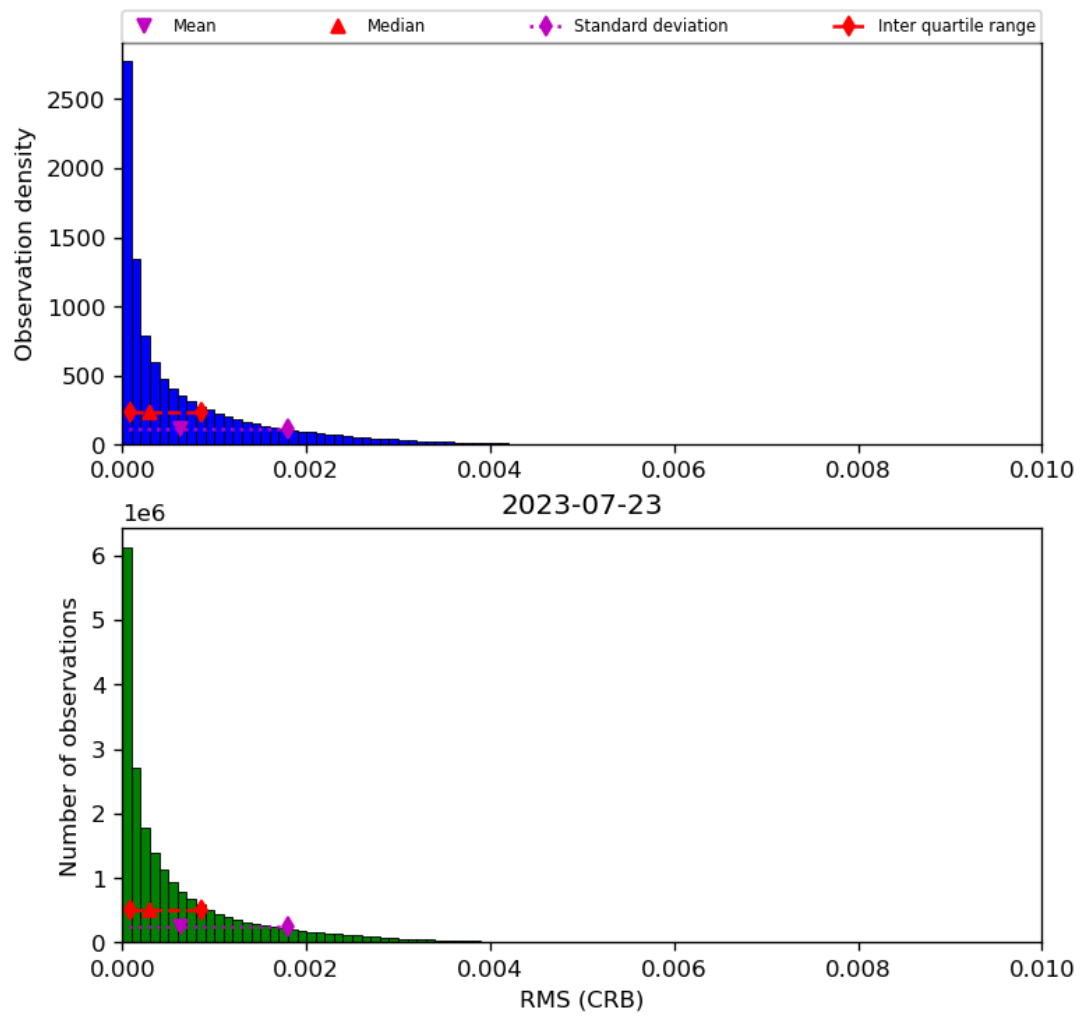
Figure 48: Histogram of “RMS (CRB)” for 2023-07-22 to 2023-07-24
