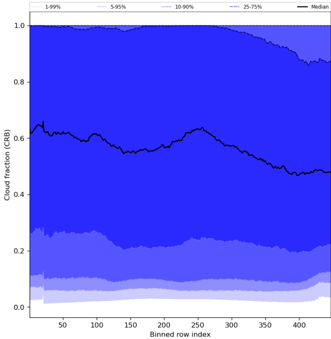
Figure 58: Along track statistics of “Cloud fraction (CRB)” for 2023-07-22 to 2023-07-24
