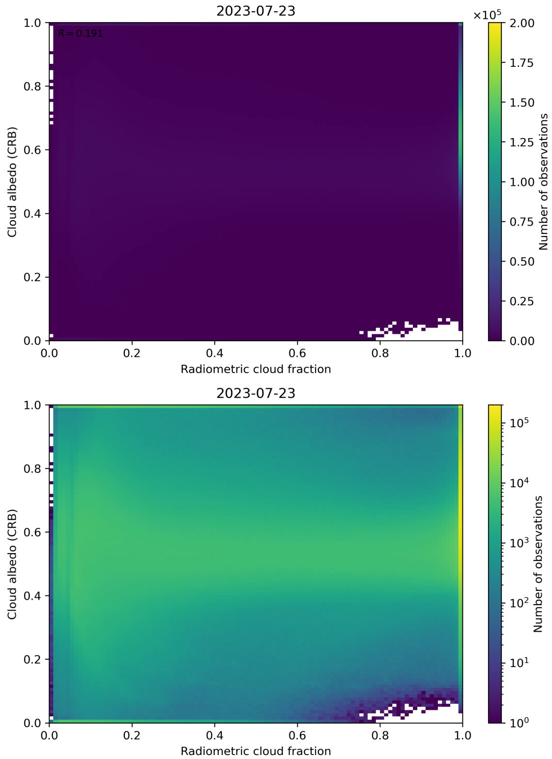
Figure 71: Scatter density plot of “Radiometric cloud fraction” against “Cloud albedo (CRB)” for 2023-07-22 to 2023-07-24.
