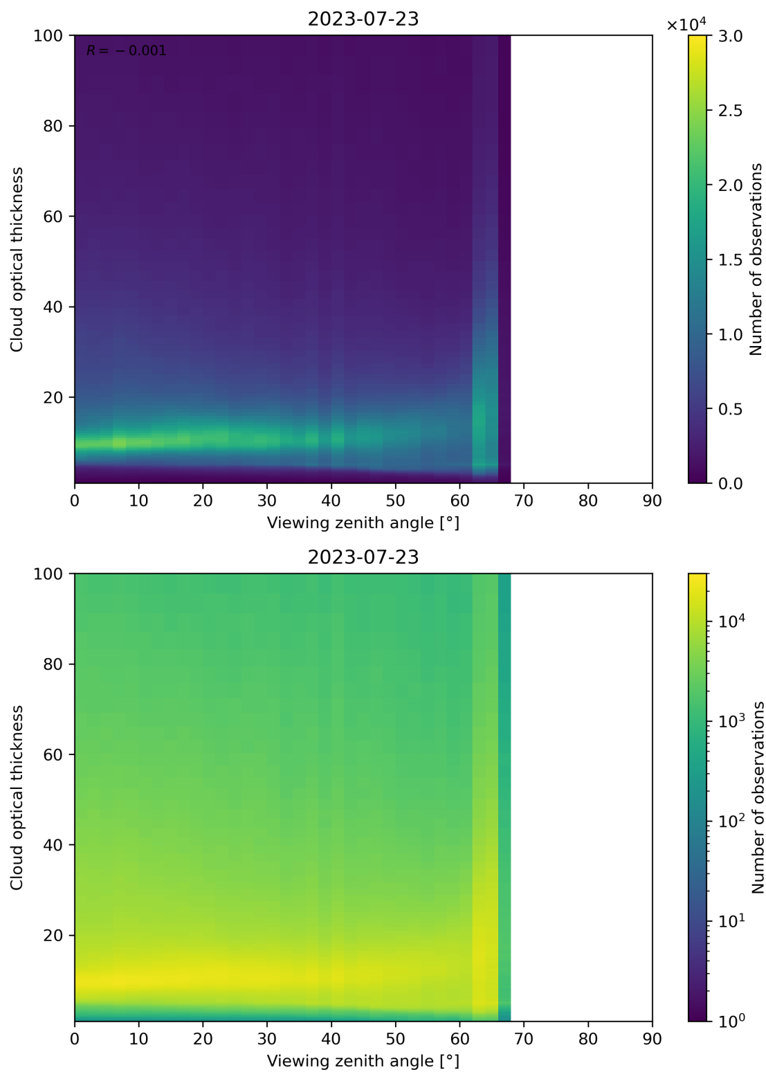
Figure 111: Scatter density plot of “Viewing zenith angle” against “Cloud optical thickness” for 2023-07-22 to 2023-07-24.
