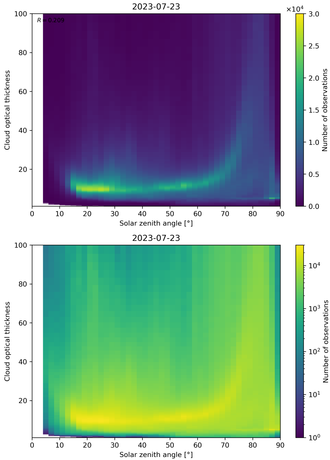
Figure 103: Scatter density plot of “Solar zenith angle” against “Cloud optical thickness” for 2023-07-22 to 2023-07-24.
