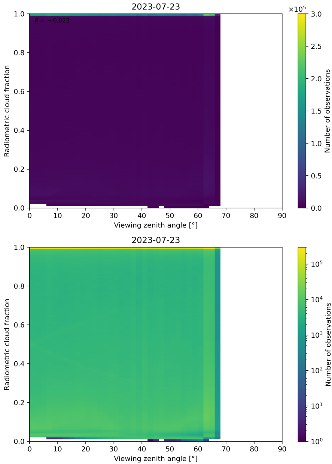
Figure 107: Scatter density plot of “Viewing zenith angle” against “Radiometric cloud fraction” for 2023-07-22 to 2023-07-24.
