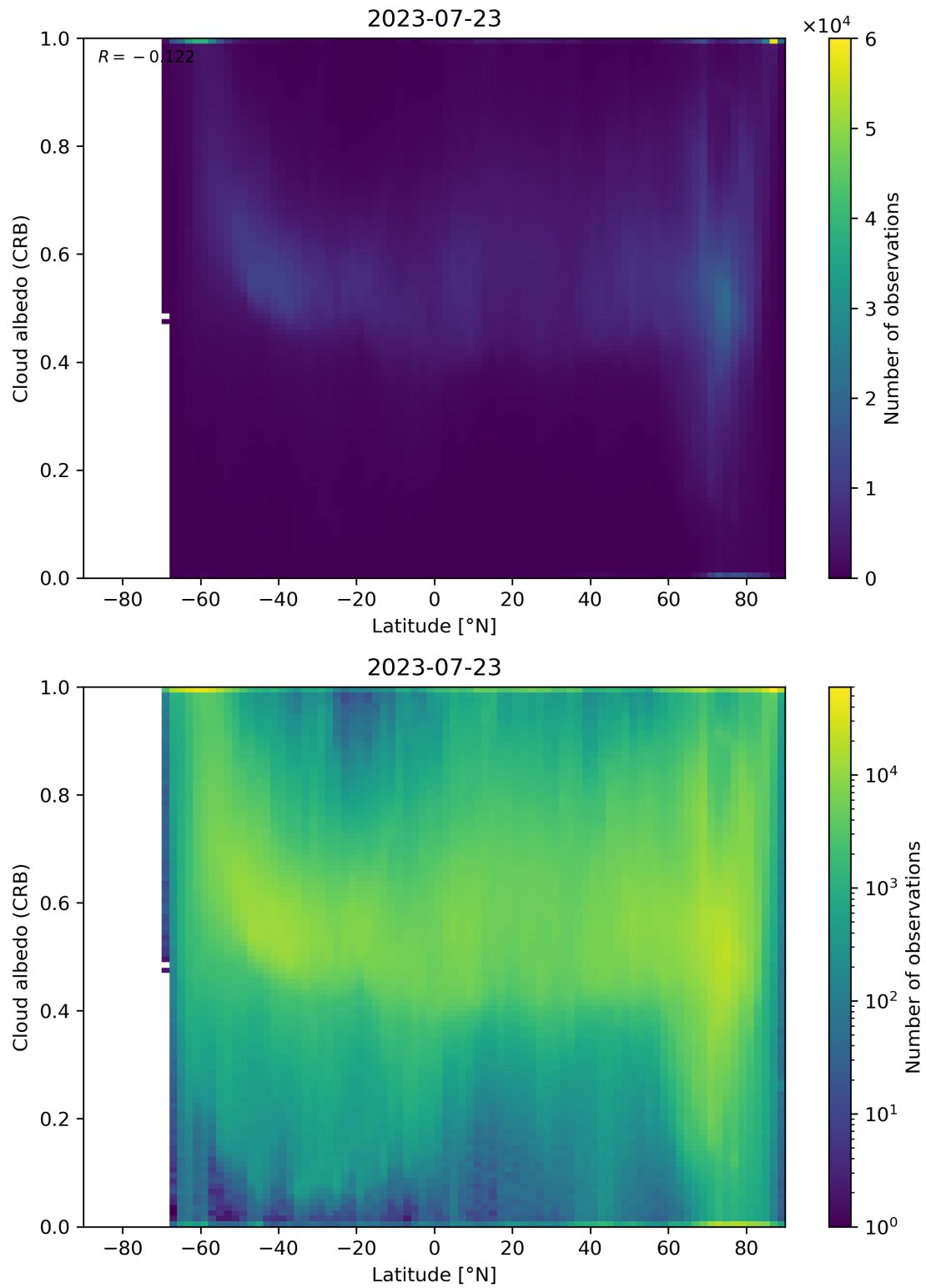
Figure 91: Scatter density plot of “Latitude” against “Cloud albedo (CRB)” for 2023-07-22 to 2023-07-24.
