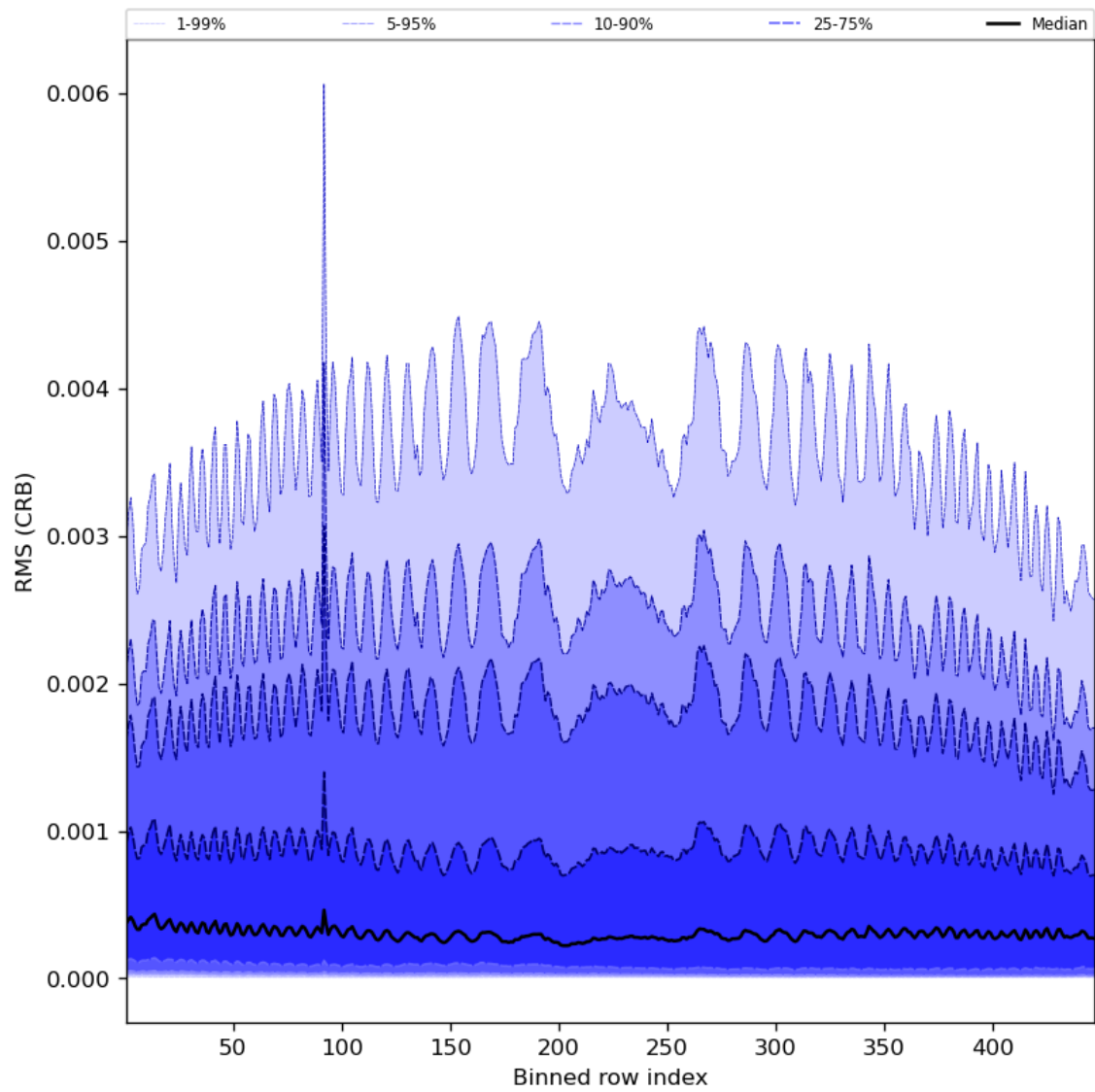
Figure 64: Along track statistics of “RMS (CRB)” for 2023-07-22 to 2023-07-24
