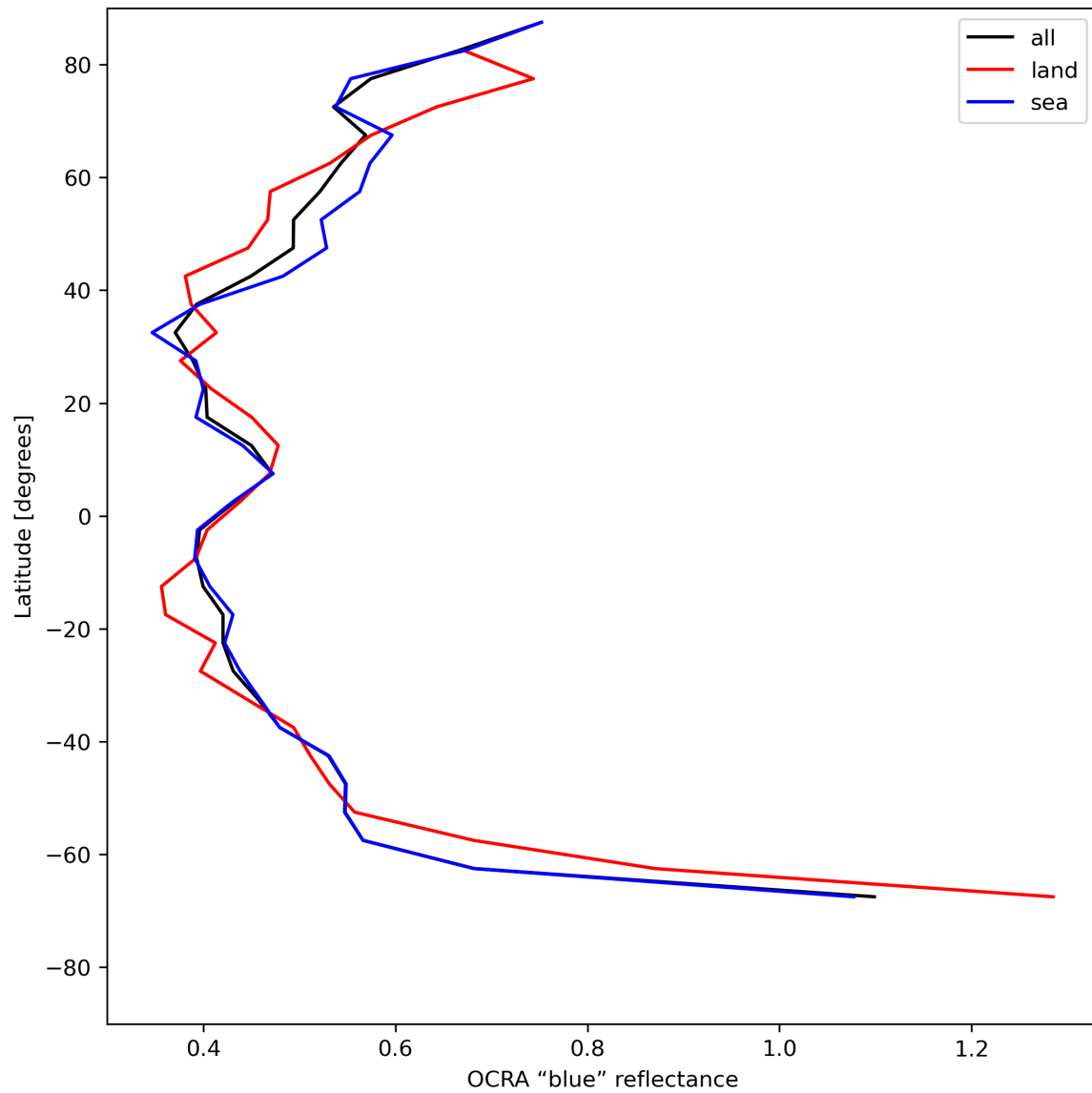
Figure 35: Zonal average of “OCRA “blue” reflectance” for 2023-07-22 to 2023-07-24.
