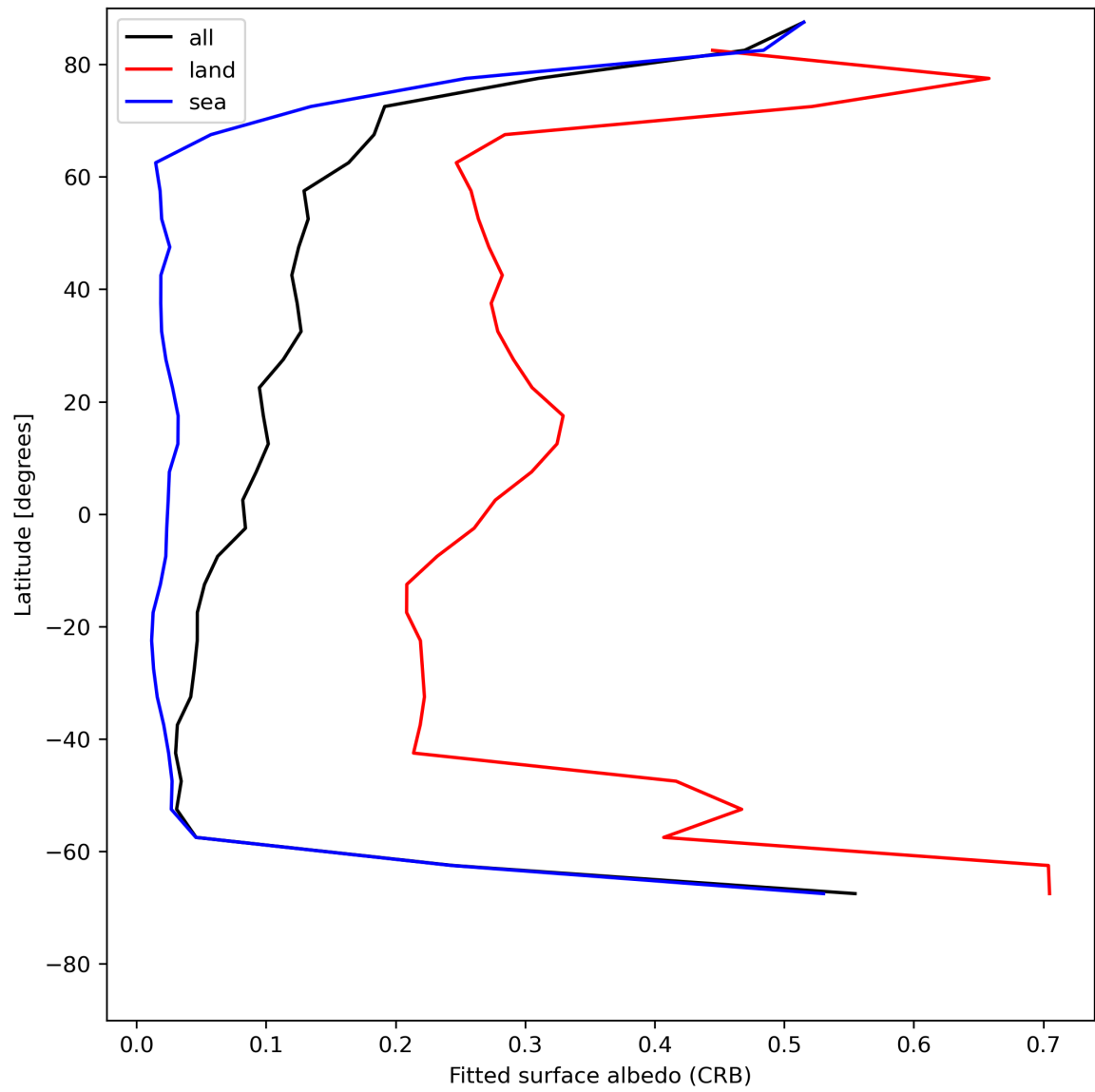
Figure 30: Zonal average of “Fitted surface albedo (CRB)” for 2023-07-26 to 2023-07-28.
