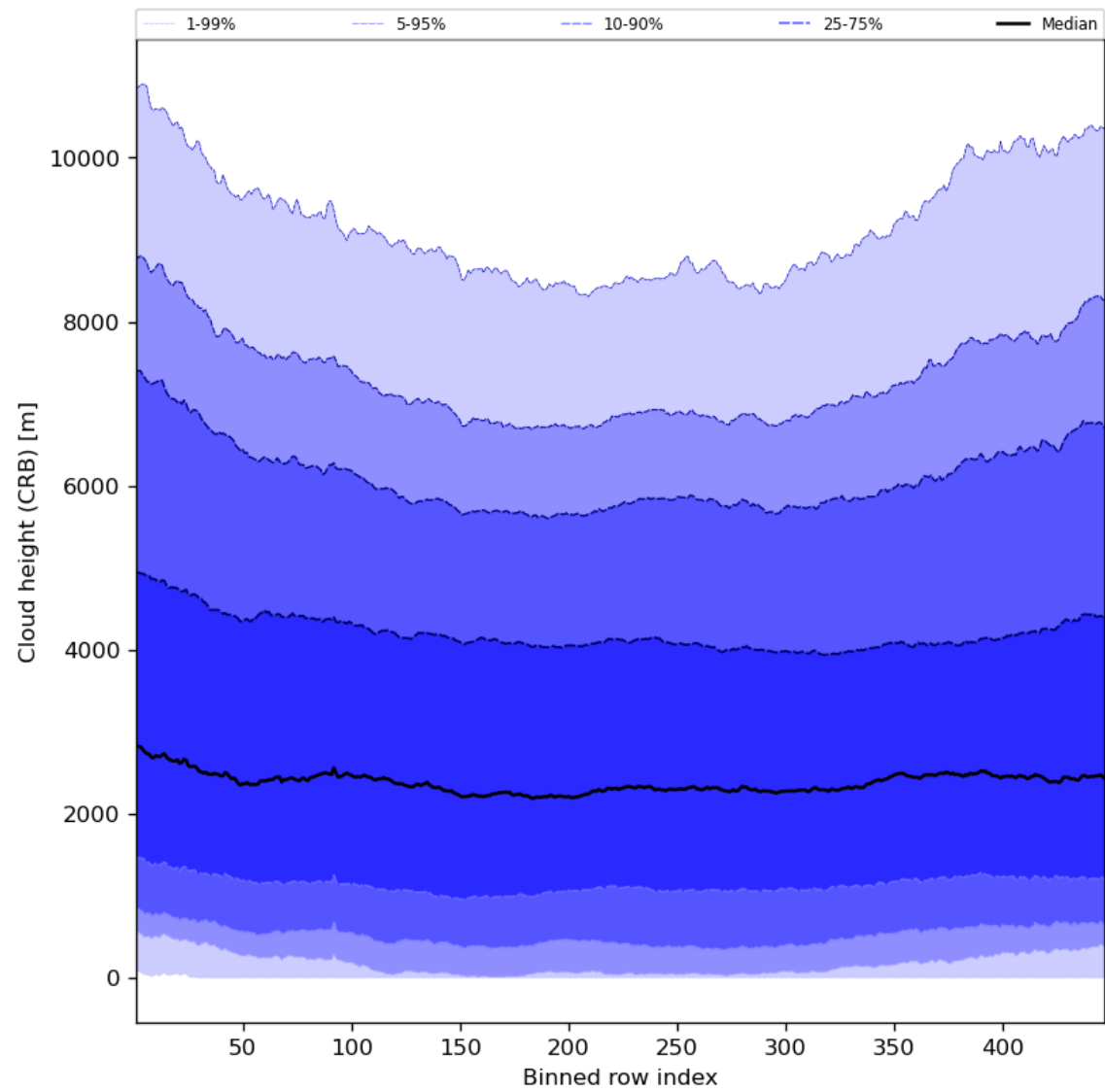
Figure 59: Along track statistics of “Cloud height (CRB)” for 2023-07-26 to 2023-07-28
