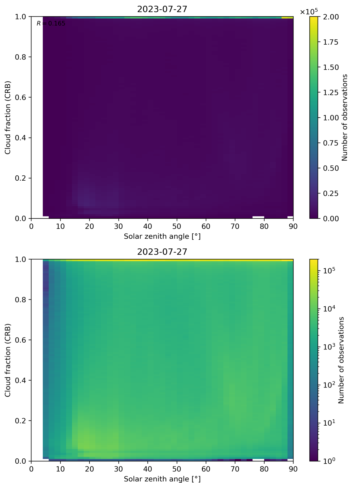
Figure 101: Scatter density plot of “Solar zenith angle” against “Cloud fraction (CRB)” for 2023-07-26 to 2023-07-28.
