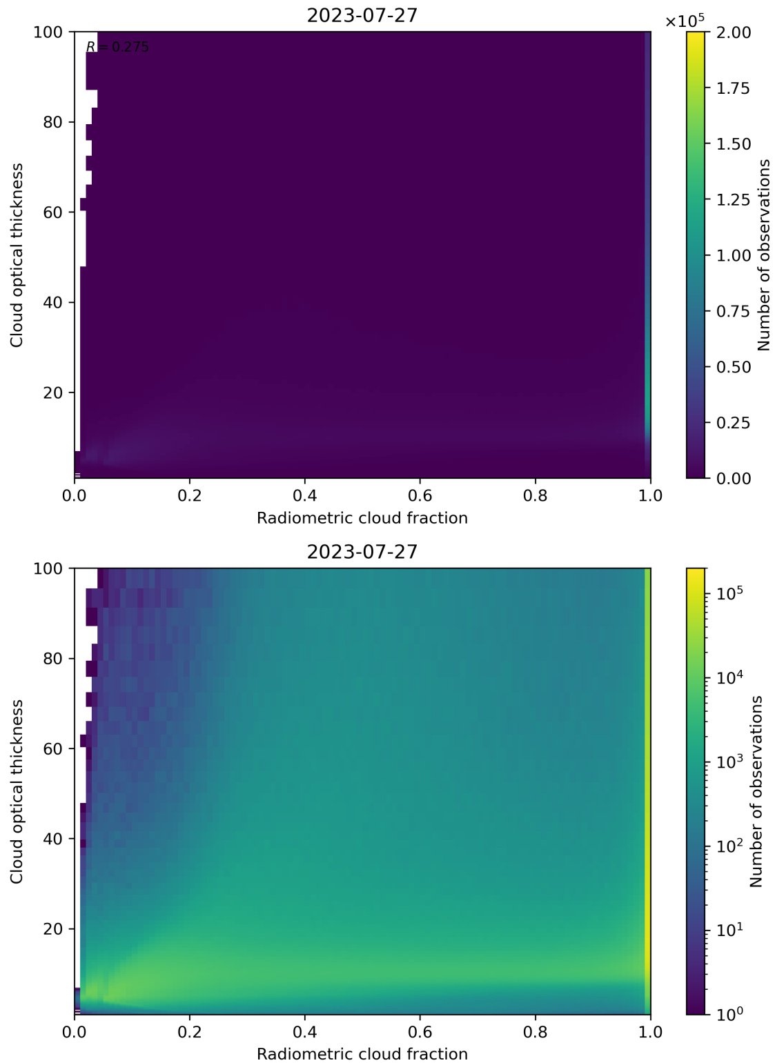
Figure 75: Scatter density plot of “Radiometric cloud fraction” against “Cloud optical thickness” for 2023-07-26 to 2023-07-28.
