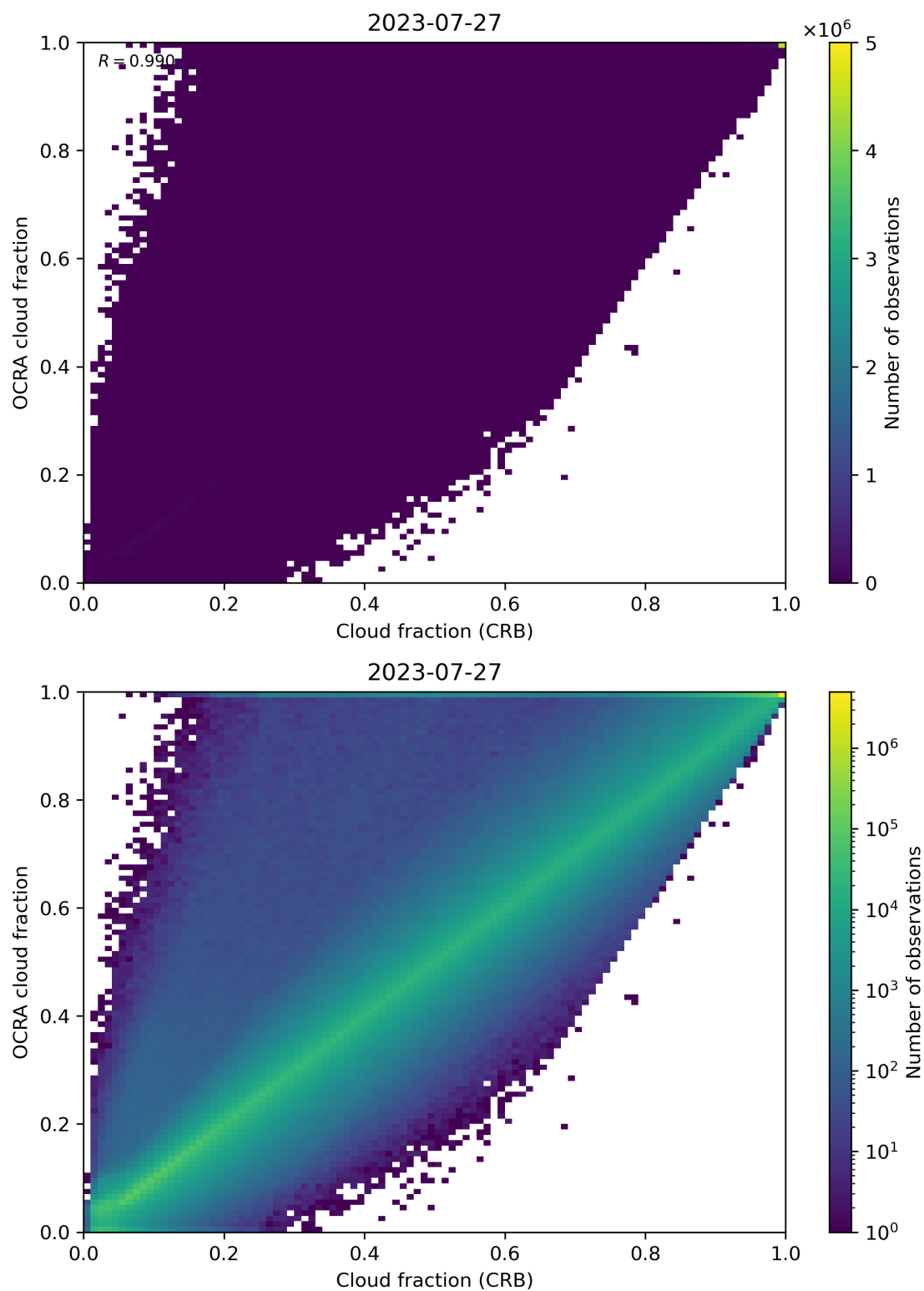
Figure 78: Scatter density plot of “Cloud fraction (CRB)” against “OCRA cloud fraction” for 2023-07-26 to 2023-07-28.
