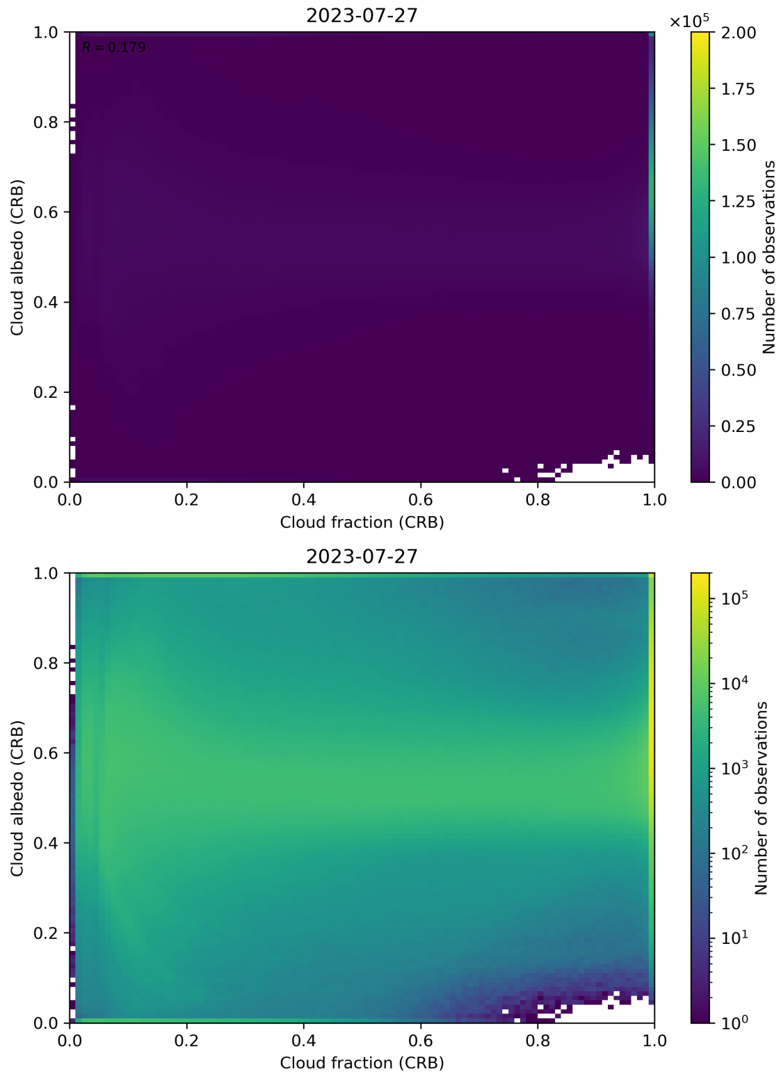
Figure 77: Scatter density plot of “Cloud fraction (CRB)” against “Cloud albedo (CRB)” for 2023-07-26 to 2023-07-28.
