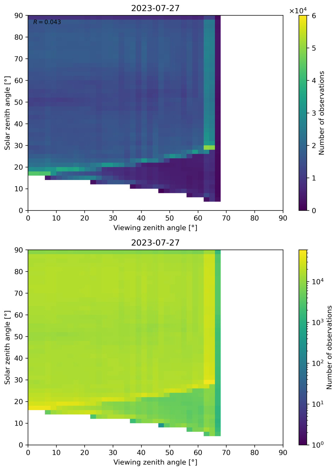
Figure 114: Scatter density plot of “Viewing zenith angle” against “Solar zenith angle” for 2023-07-26 to 2023-07-28.
