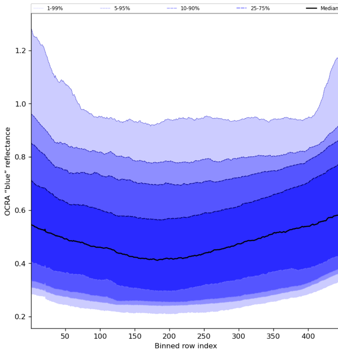
Figure 67: Along track statistics of “OCRA “blue” reflectance” for 2023-07-26 to 2023-07-28
