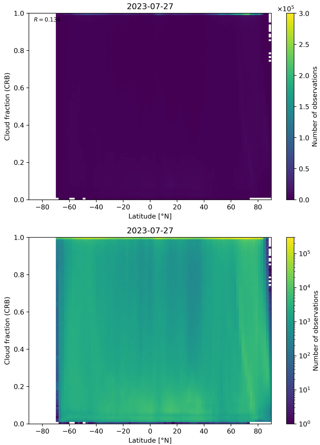
Figure 94: Scatter density plot of “Latitude” against “Cloud fraction (CRB)” for 2023-07-26 to 2023-07-28.
