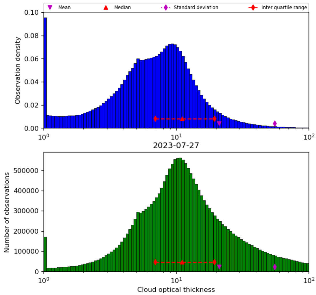
Figure 41: Histogram of “Cloud optical thickness” for 2023-07-26 to 2023-07-28
