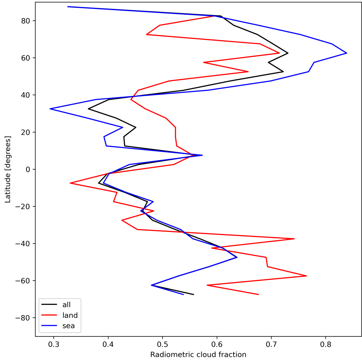
Figure 23: Zonal average of “Radiometric cloud fraction” for 2023-07-26 to 2023-07-28.
