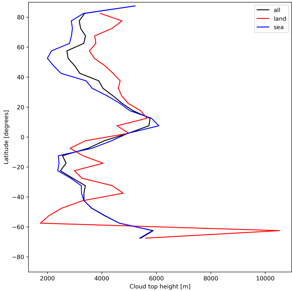
Figure 24: Zonal average of “Cloud top height” for 2023-07-26 to 2023-07-28.
