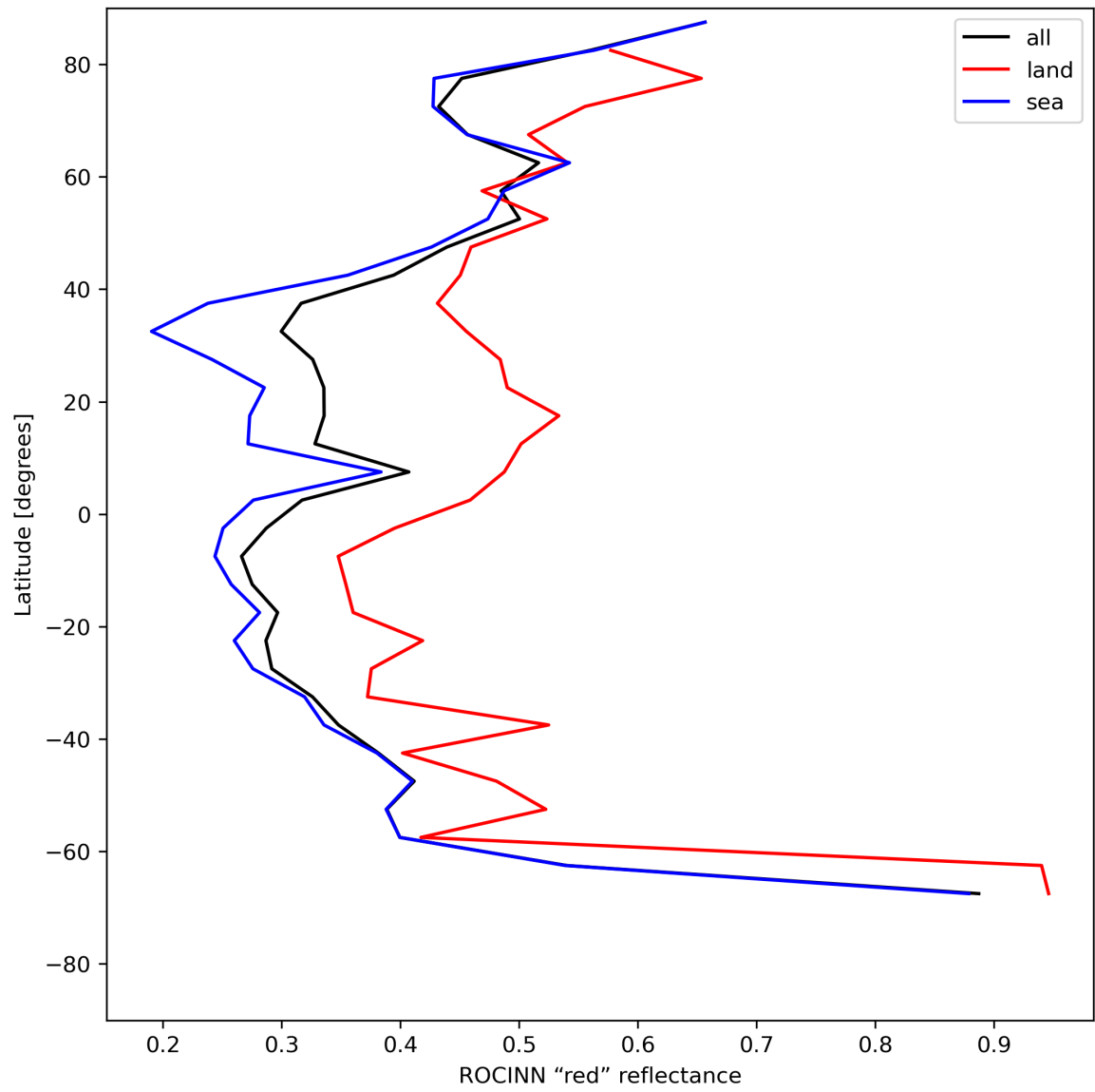
Figure 37: Zonal average of “ROCINN “red” reflectance” for 2023-07-26 to 2023-07-28.
