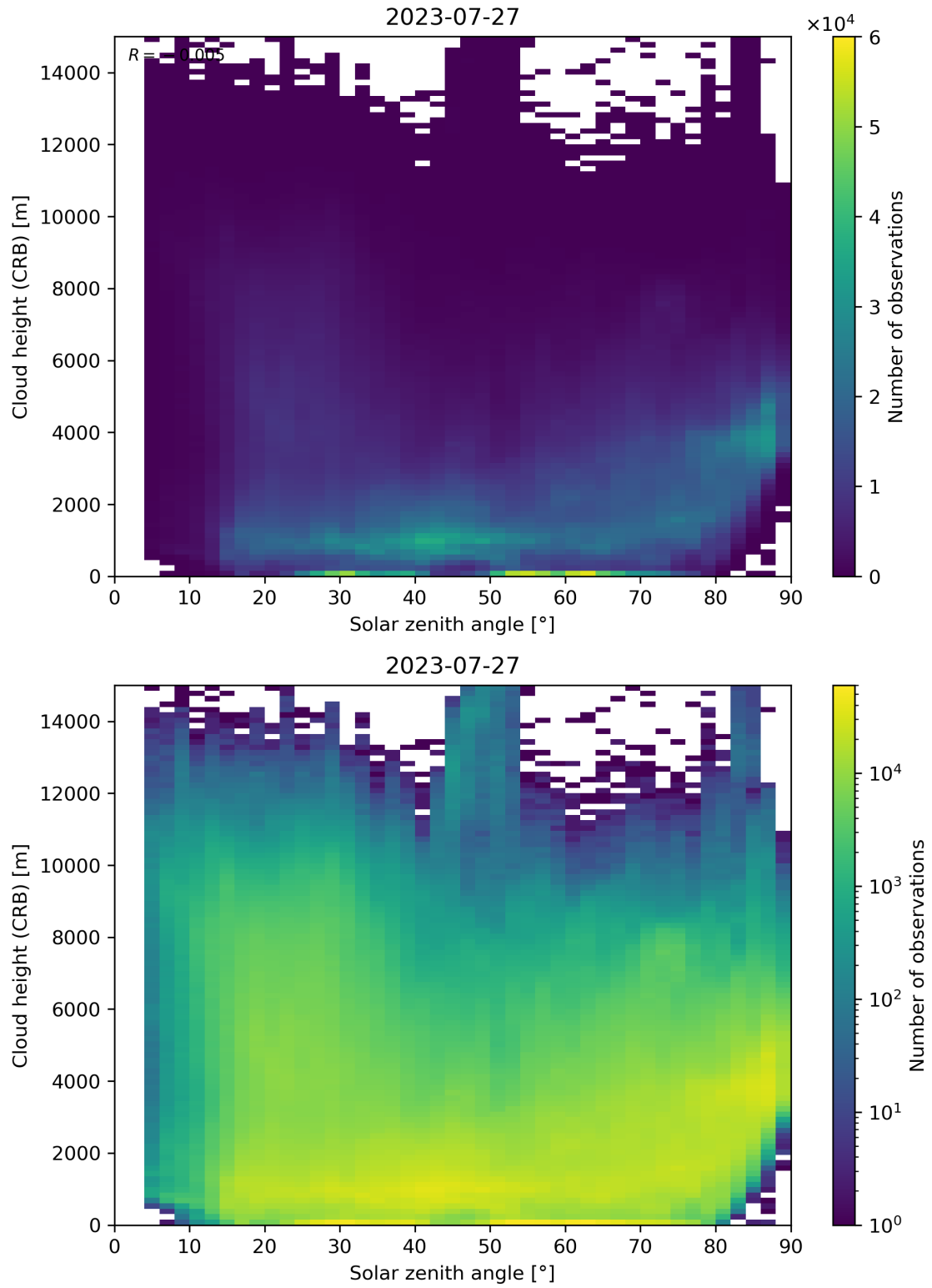
Figure 102: Scatter density plot of “Solar zenith angle” against “Cloud height (CRB)” for 2023-07-26 to 2023-07-28.
