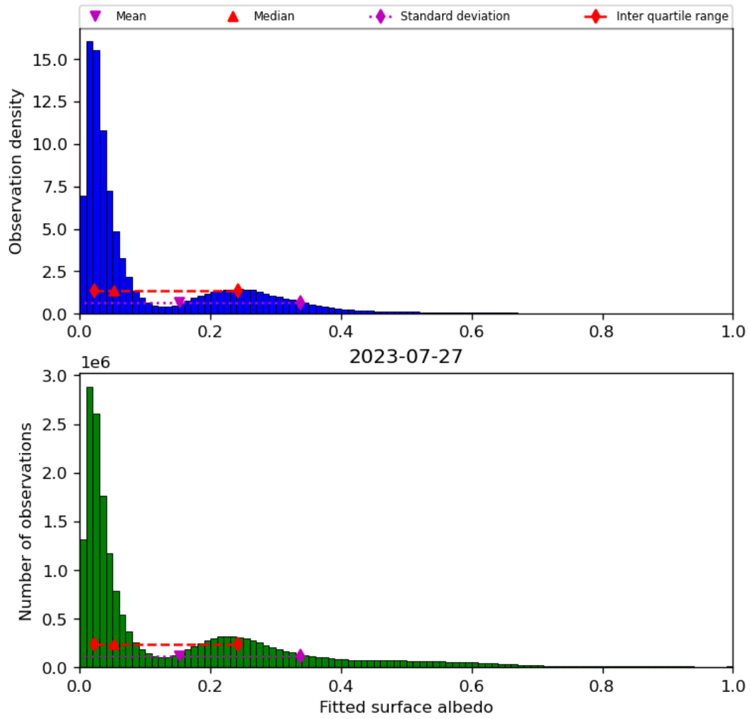
Figure 45: Histogram of “Fitted surface albedo” for 2023-07-26 to 2023-07-28
