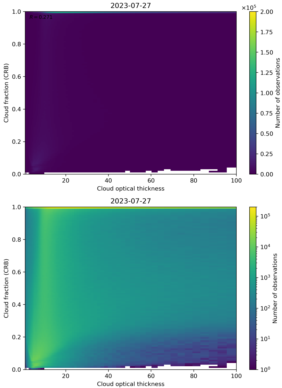
Figure 84: Scatter density plot of “Cloud optical thickness” against “Cloud fraction (CRB)” for 2023-07-26 to 2023-07-28.
