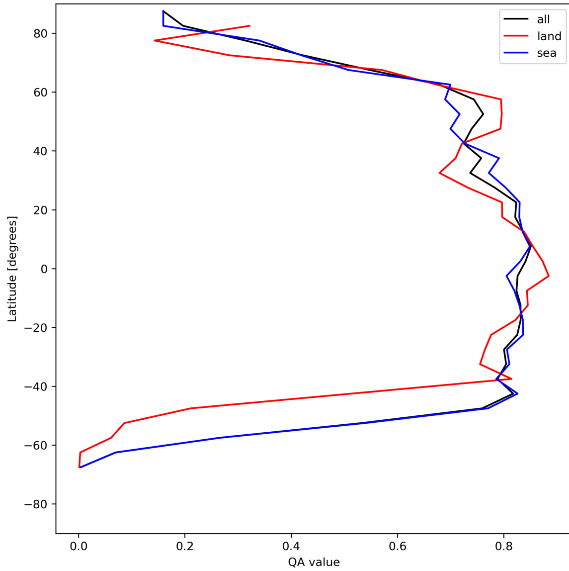
Figure 22: Zonal average of “QA value” for 2023-07-26 to 2023-07-28.
