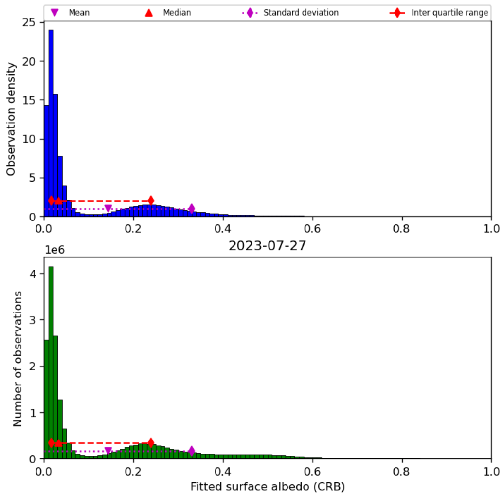
Figure 46: Histogram of “Fitted surface albedo (CRB)” for 2023-07-26 to 2023-07-28
