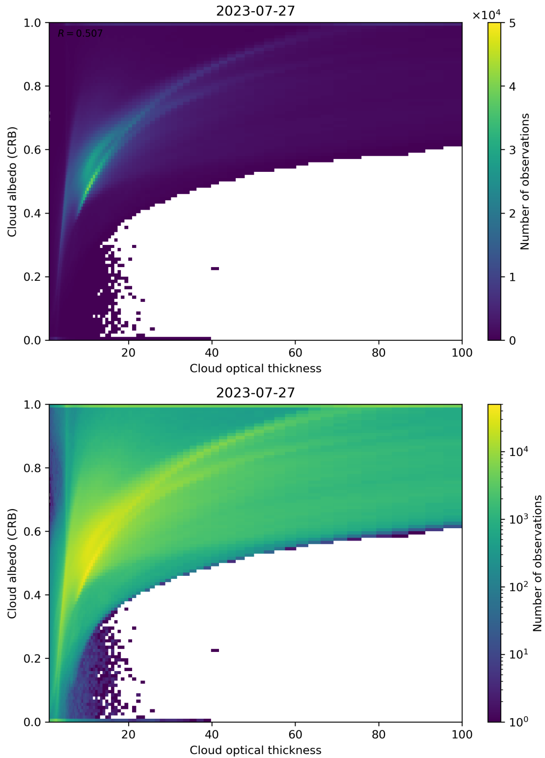
Figure 82: Scatter density plot of “Cloud optical thickness” against “Cloud albedo (CRB)” for 2023-07-26 to 2023-07-28.
