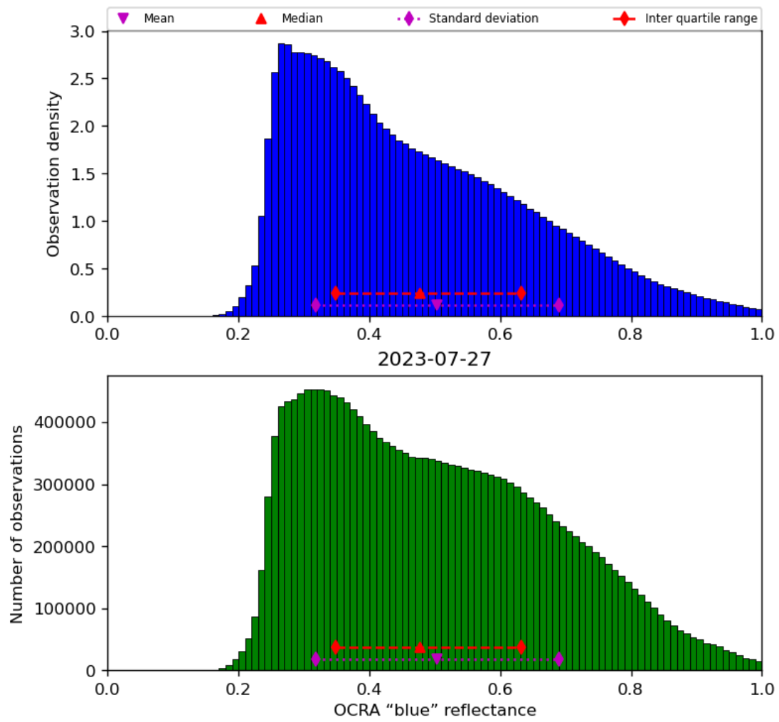
Figure 51: Histogram of “OCRA “blue” reflectance” for 2023-07-26 to 2023-07-28
