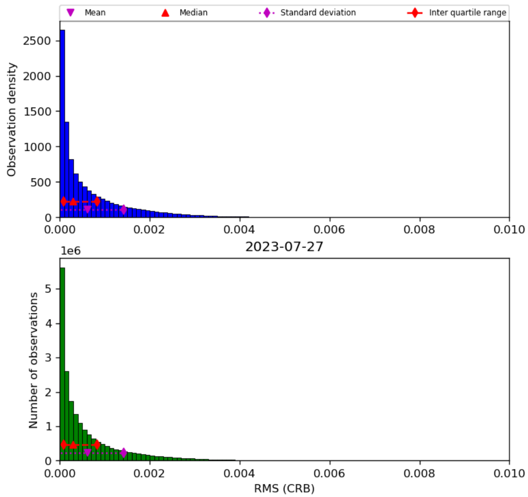
Figure 48: Histogram of “RMS (CRB)” for 2023-07-26 to 2023-07-28
