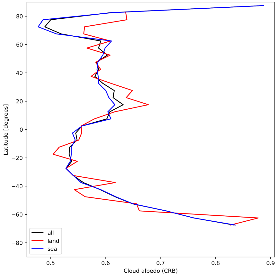
Figure 28: Zonal average of “Cloud albedo (CRB)” for 2023-07-26 to 2023-07-28.
