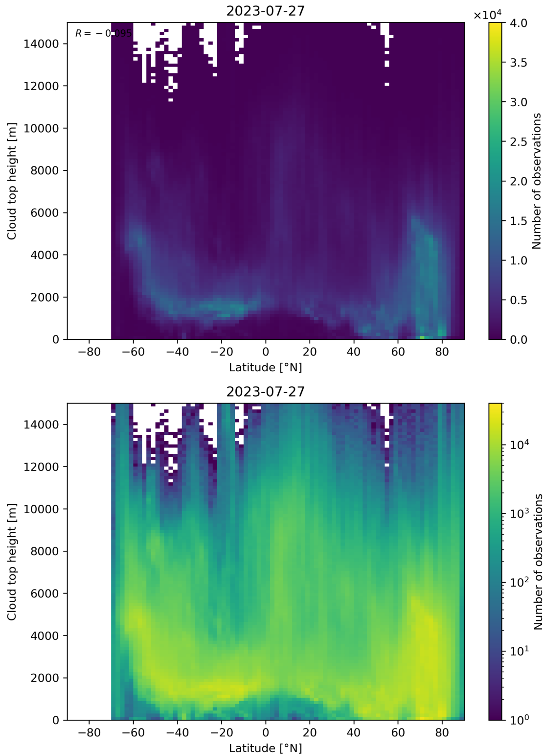
Figure 97: Scatter density plot of “Latitude” against “Cloud top height” for 2023-07-26 to 2023-07-28.
