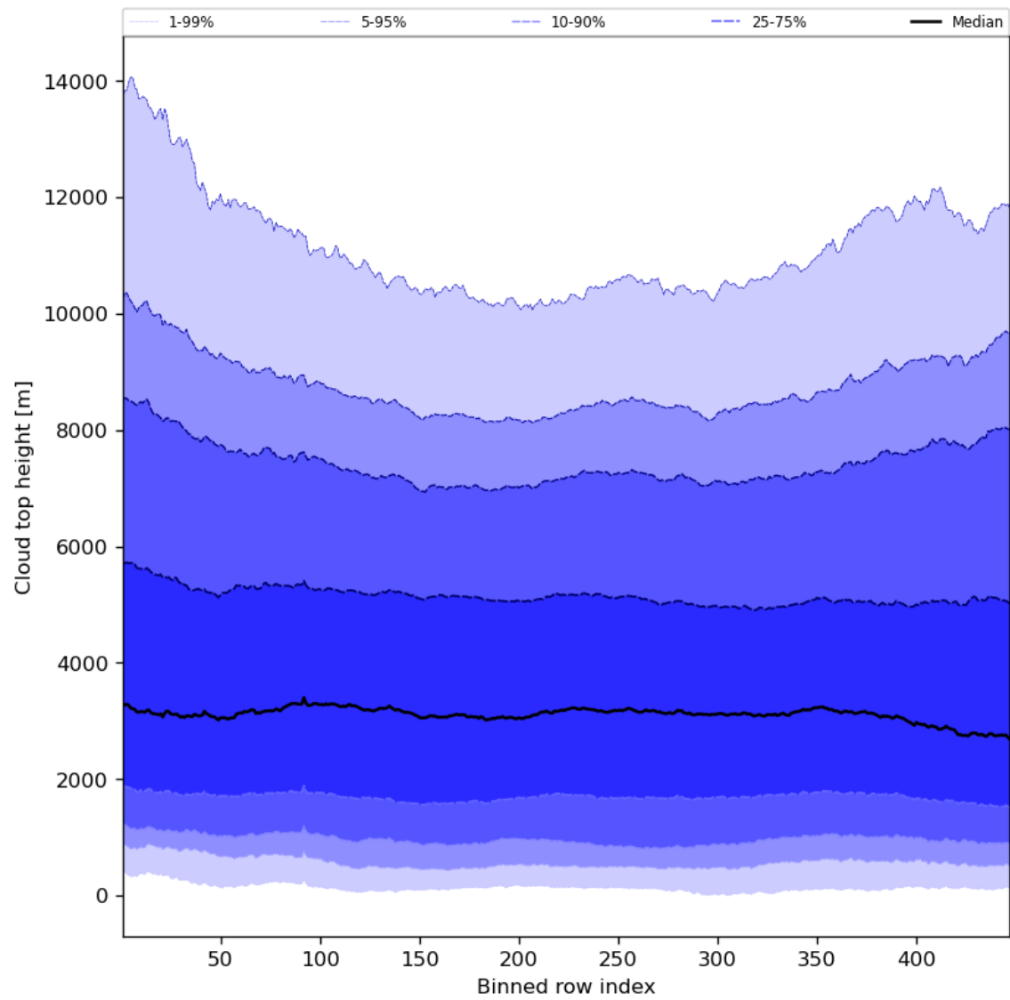
Figure 56: Along track statistics of “Cloud top height” for 2023-07-26 to 2023-07-28
