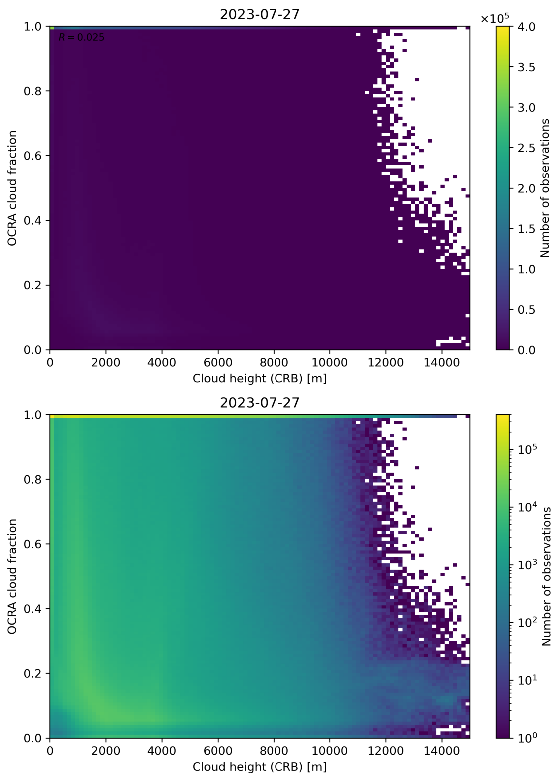
Figure 81: Scatter density plot of “Cloud height (CRB)” against “OCRA cloud fraction” for 2023-07-26 to 2023-07-28.
