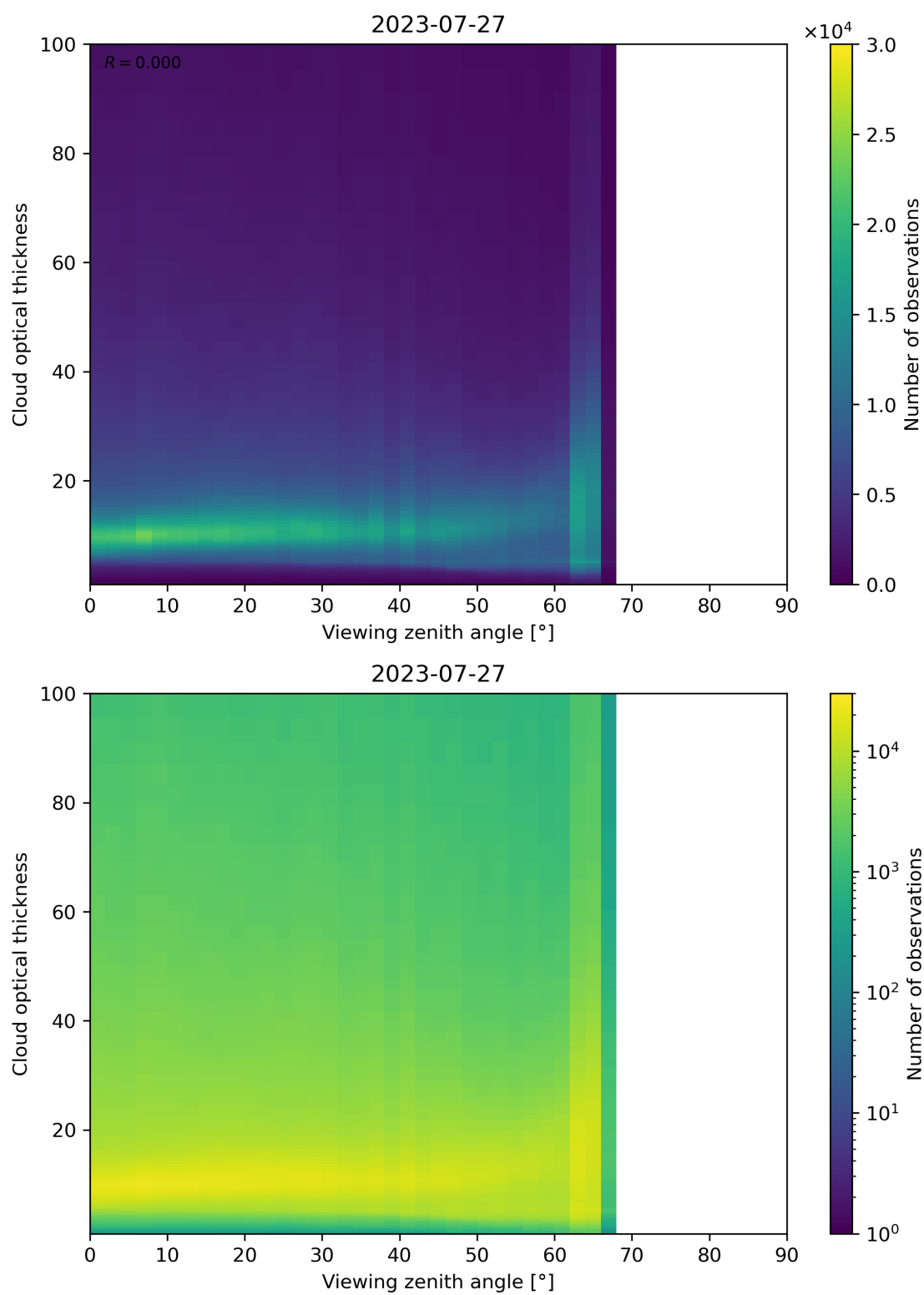
Figure 111: Scatter density plot of “Viewing zenith angle” against “Cloud optical thickness” for 2023-07-26 to 2023-07-28.
