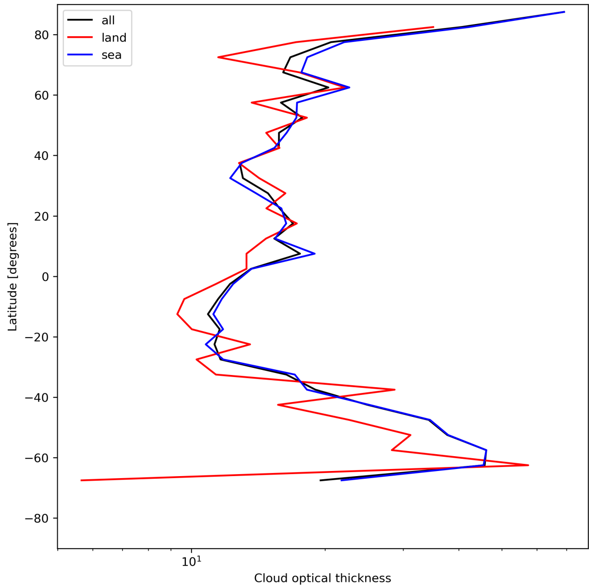
Figure 25: Zonal average of “Cloud optical thickness” for 2023-07-26 to 2023-07-28.
