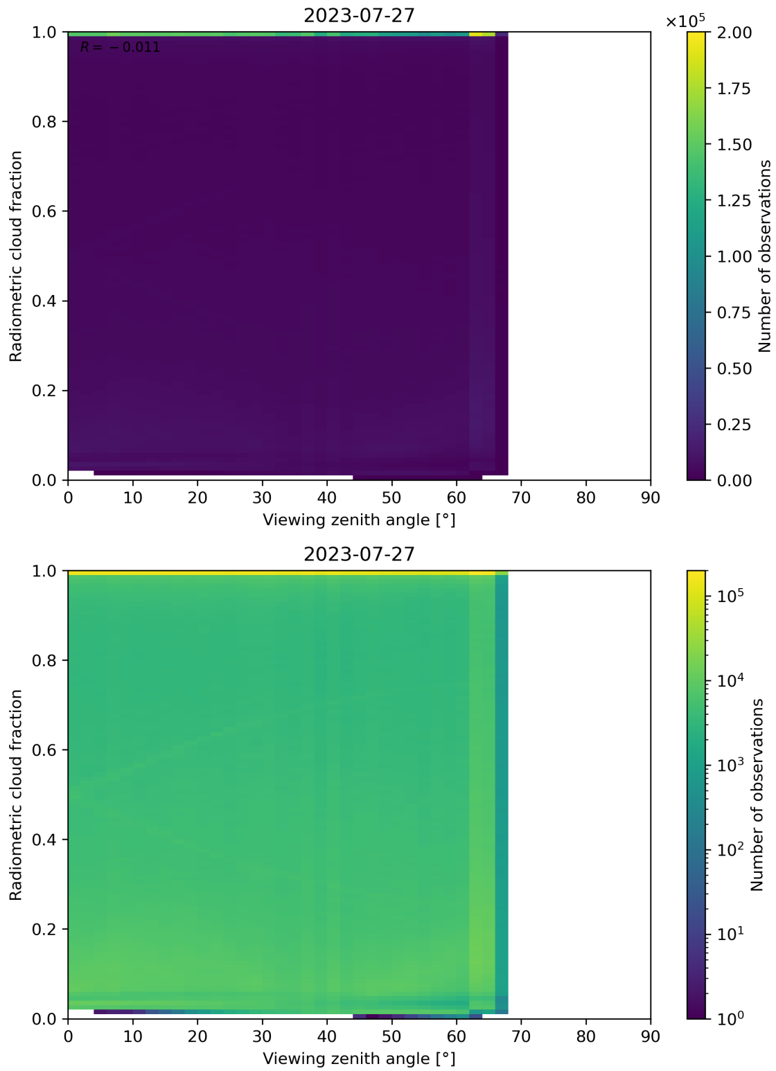
Figure 107: Scatter density plot of “Viewing zenith angle” against “Radiometric cloud fraction” for 2023-07-26 to 2023-07-28.
