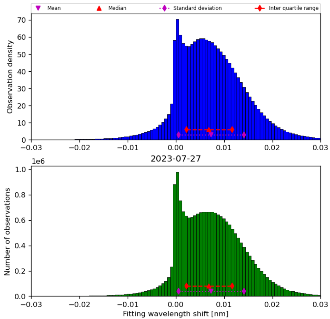
Figure 49: Histogram of “Fitting wavelength shift” for 2023-07-26 to 2023-07-28
