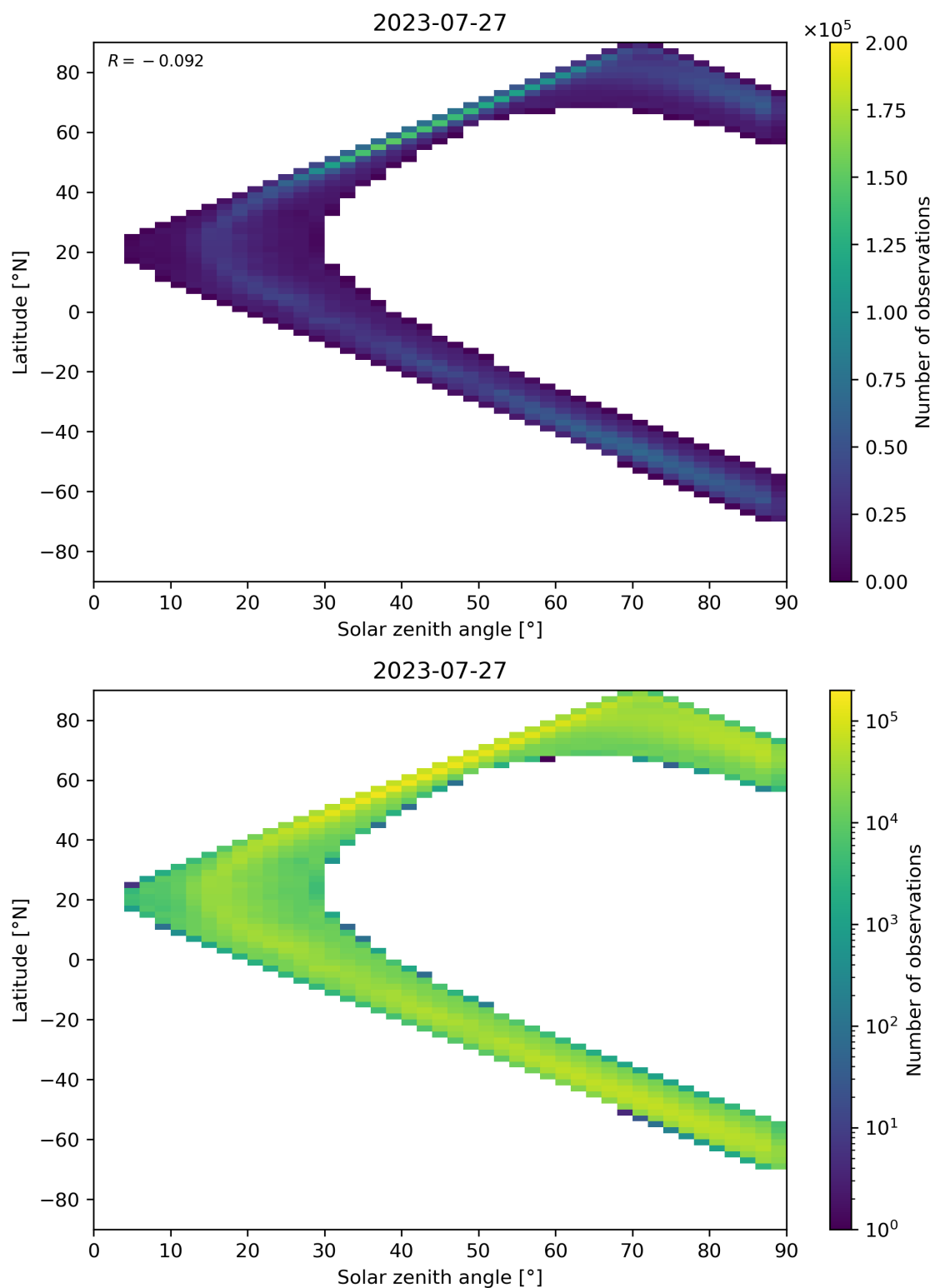
Figure 105: Scatter density plot of “Solar zenith angle” against “Latitude” for 2023-07-26 to 2023-07-28.
