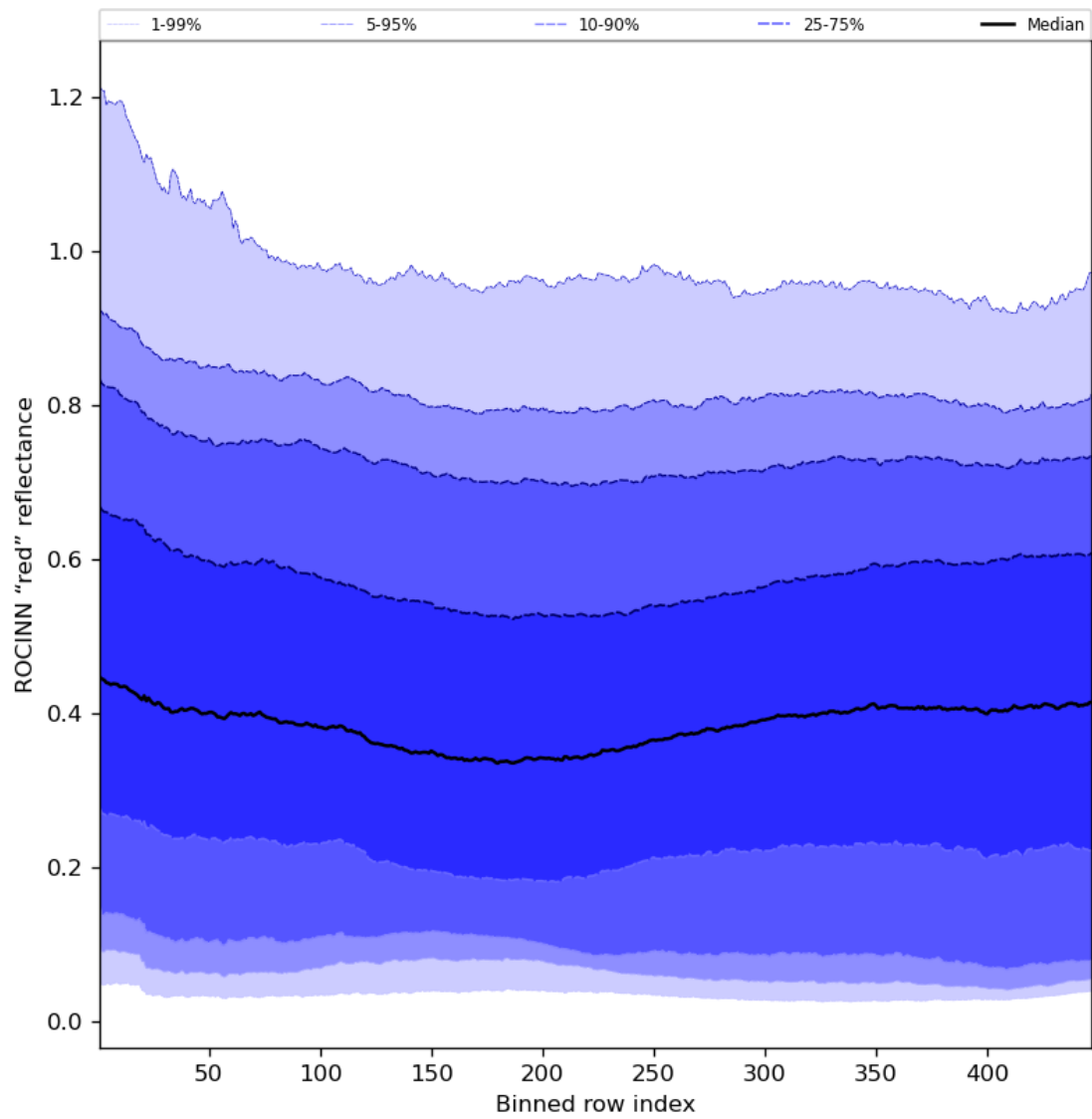
Figure 69: Along track statistics of “ROCINN “red” reflectance” for 2023-07-26 to 2023-07-28
