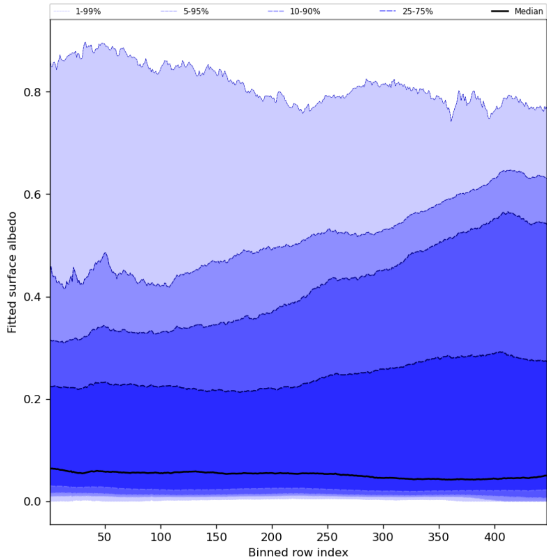
Figure 61: Along track statistics of “Fitted surface albedo” for 2023-07-26 to 2023-07-28
