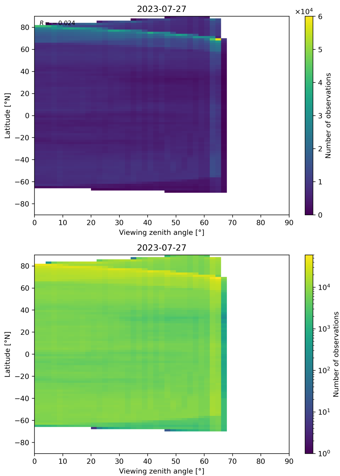
Figure 113: Scatter density plot of “Viewing zenith angle” against “Latitude” for 2023-07-26 to 2023-07-28.
