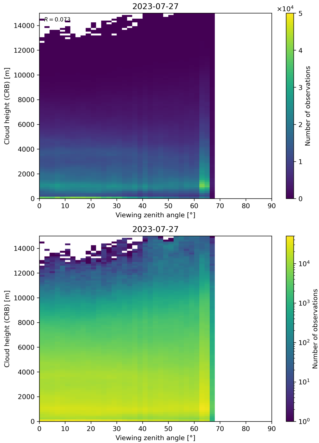
Figure 110: Scatter density plot of “Viewing zenith angle” against “Cloud height (CRB)” for 2023-07-26 to 2023-07-28.
