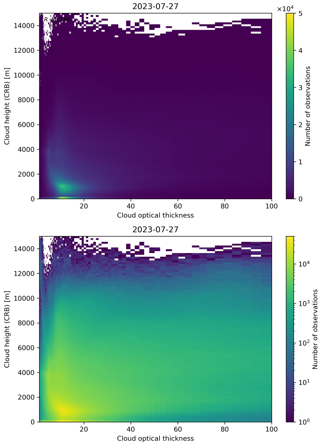
Figure 85: Scatter density plot of “Cloud optical thickness” against “Cloud height (CRB)” for 2023-07-26 to 2023-07-28.
