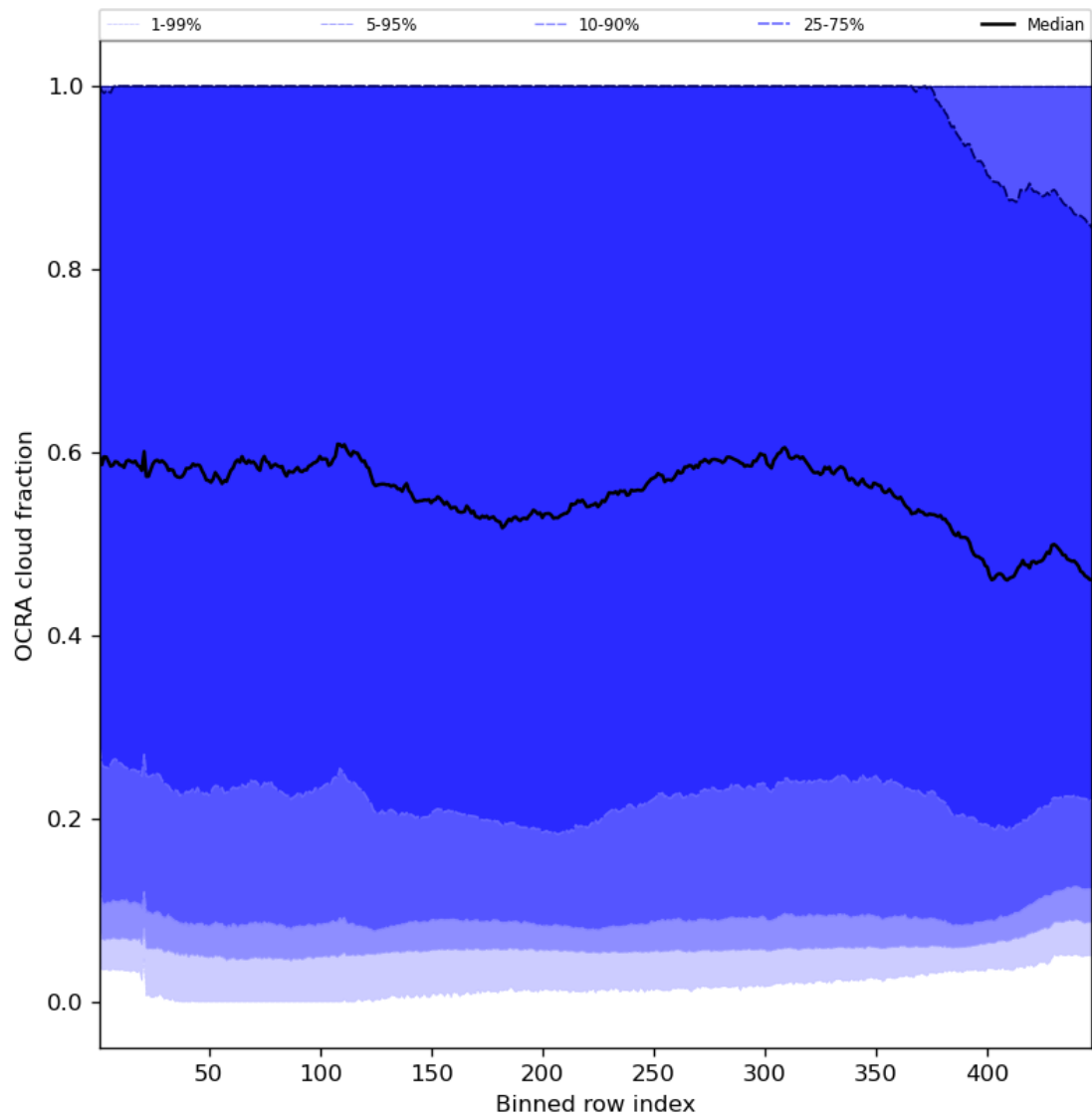
Figure 66: Along track statistics of “OCRA cloud fraction” for 2023-07-26 to 2023-07-28
