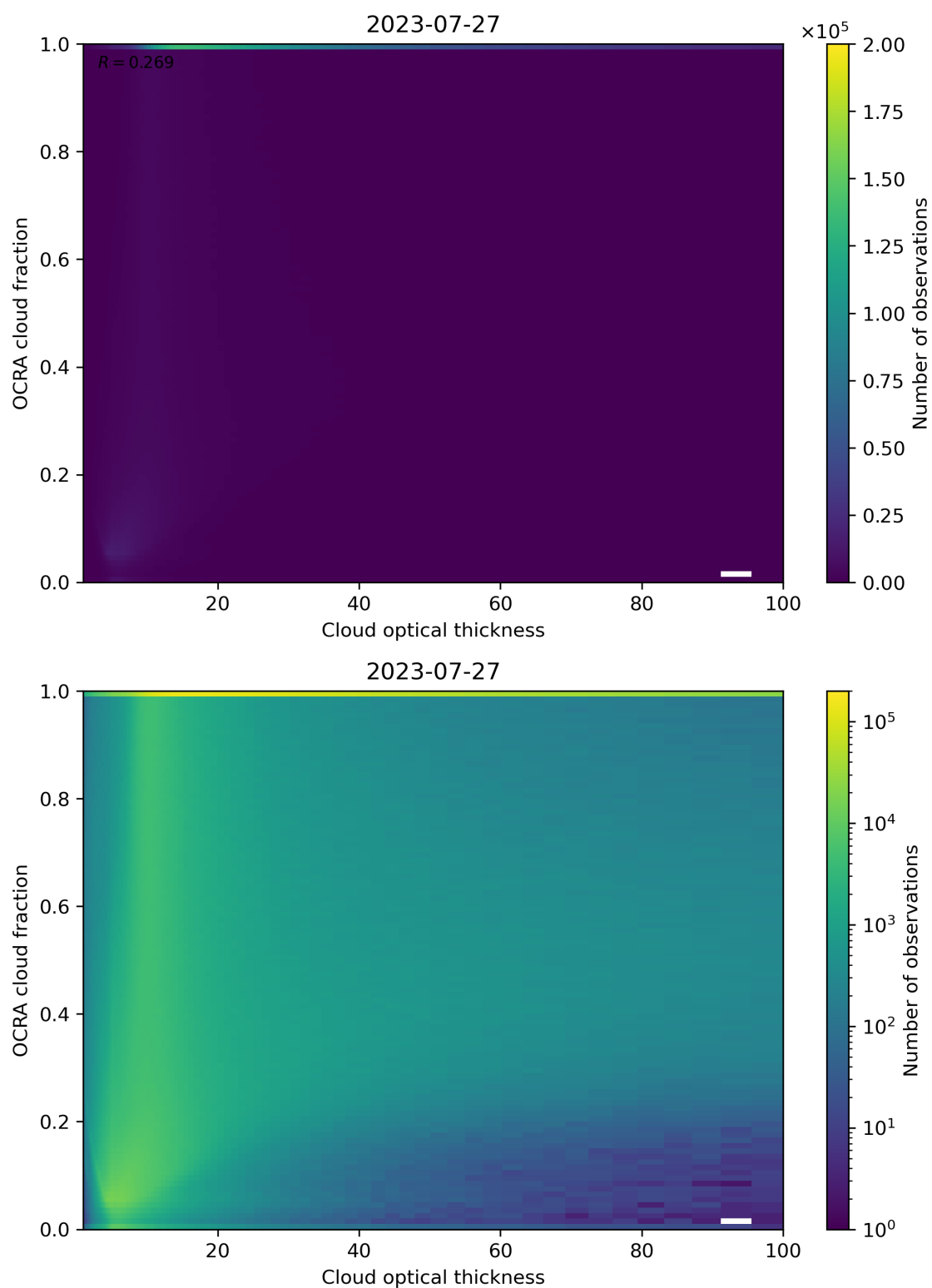
Figure 83: Scatter density plot of “Cloud optical thickness” against “OCRA cloud fraction” for 2023-07-26 to 2023-07-28.
