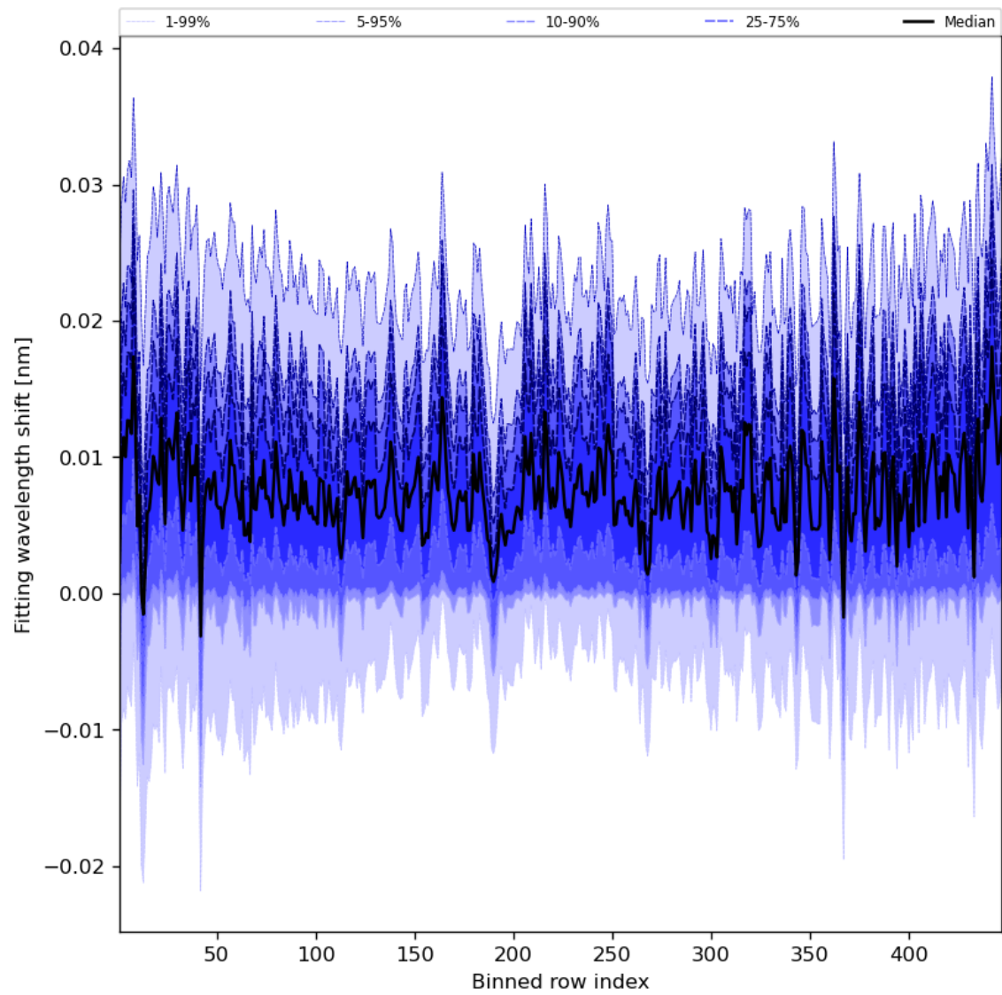
Figure 65: Along track statistics of “Fitting wavelength shift” for 2023-07-26 to 2023-07-28
