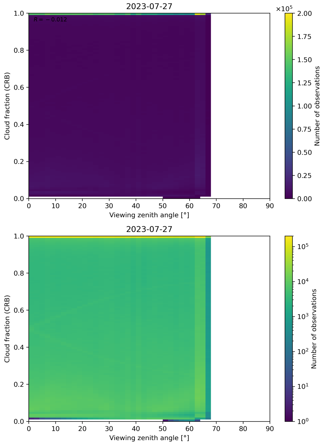
Figure 109: Scatter density plot of “Viewing zenith angle” against “Cloud fraction (CRB)” for 2023-07-26 to 2023-07-28.
