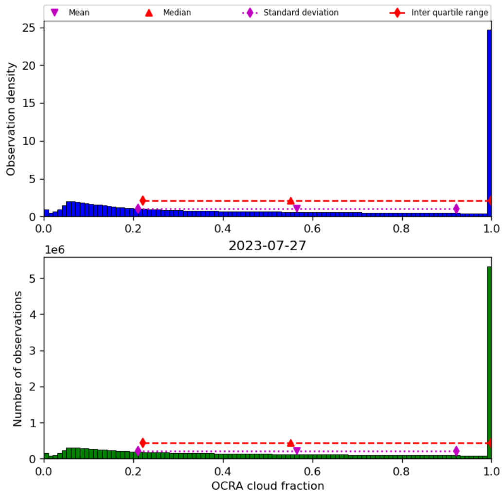
Figure 50: Histogram of “OCRA cloud fraction” for 2023-07-26 to 2023-07-28
