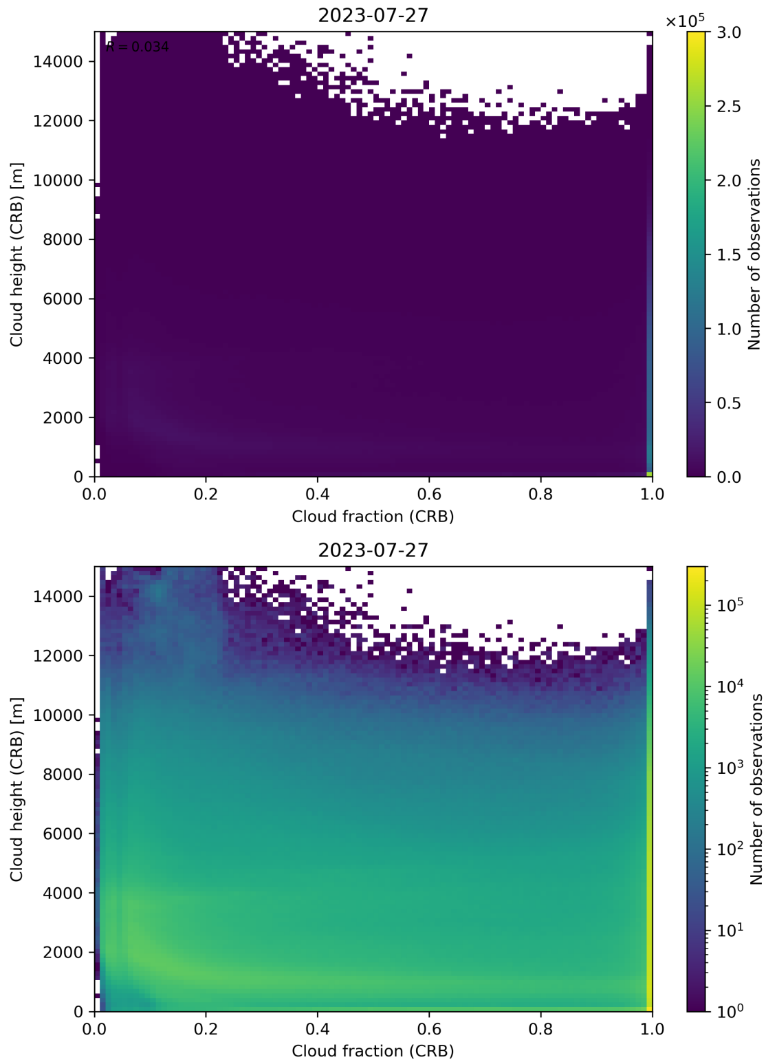
Figure 79: Scatter density plot of “Cloud fraction (CRB)” against “Cloud height (CRB)” for 2023-07-26 to 2023-07-28.
