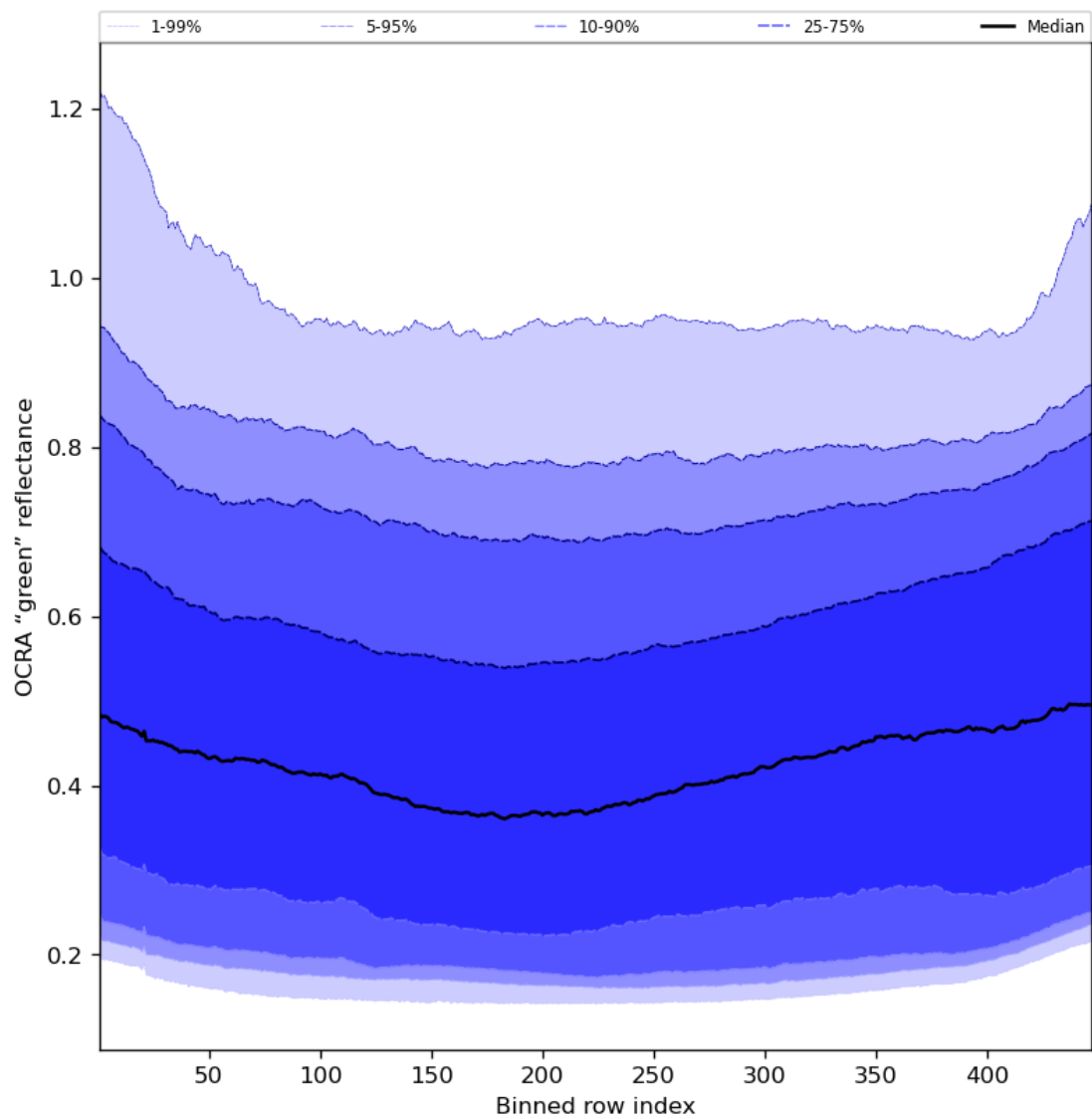
Figure 68: Along track statistics of “OCRA “green” reflectance” for 2023-07-26 to 2023-07-28
