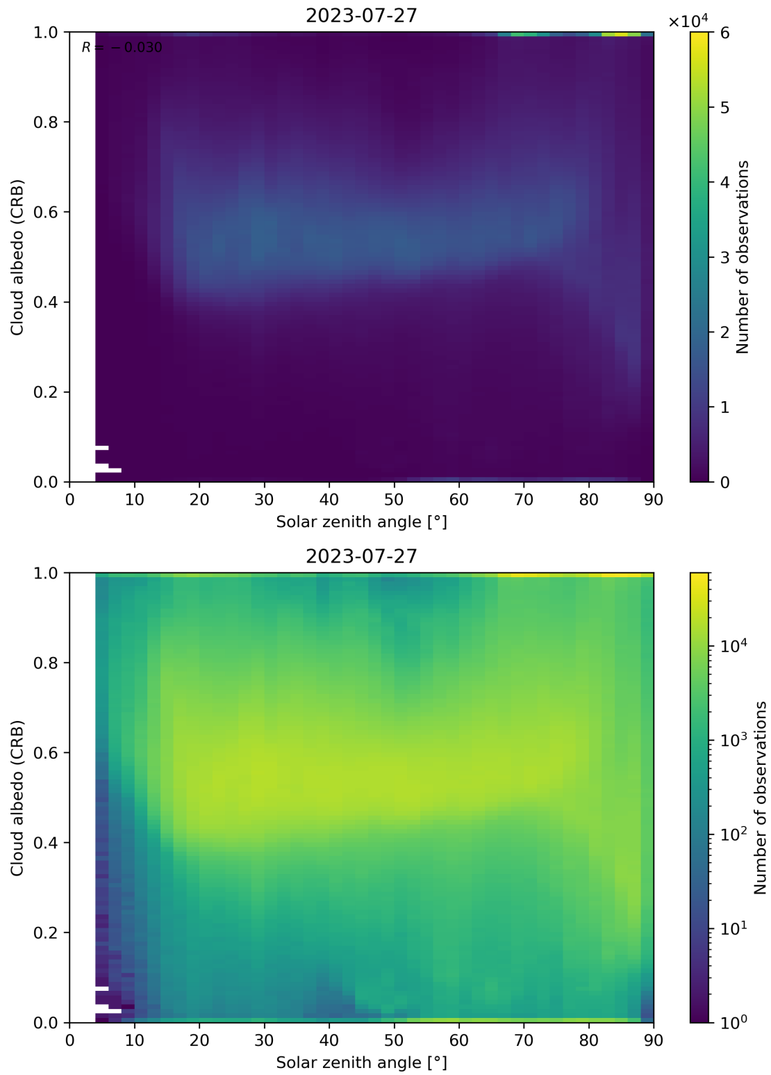
Figure 98: Scatter density plot of “Solar zenith angle” against “Cloud albedo (CRB)” for 2023-07-26 to 2023-07-28.
