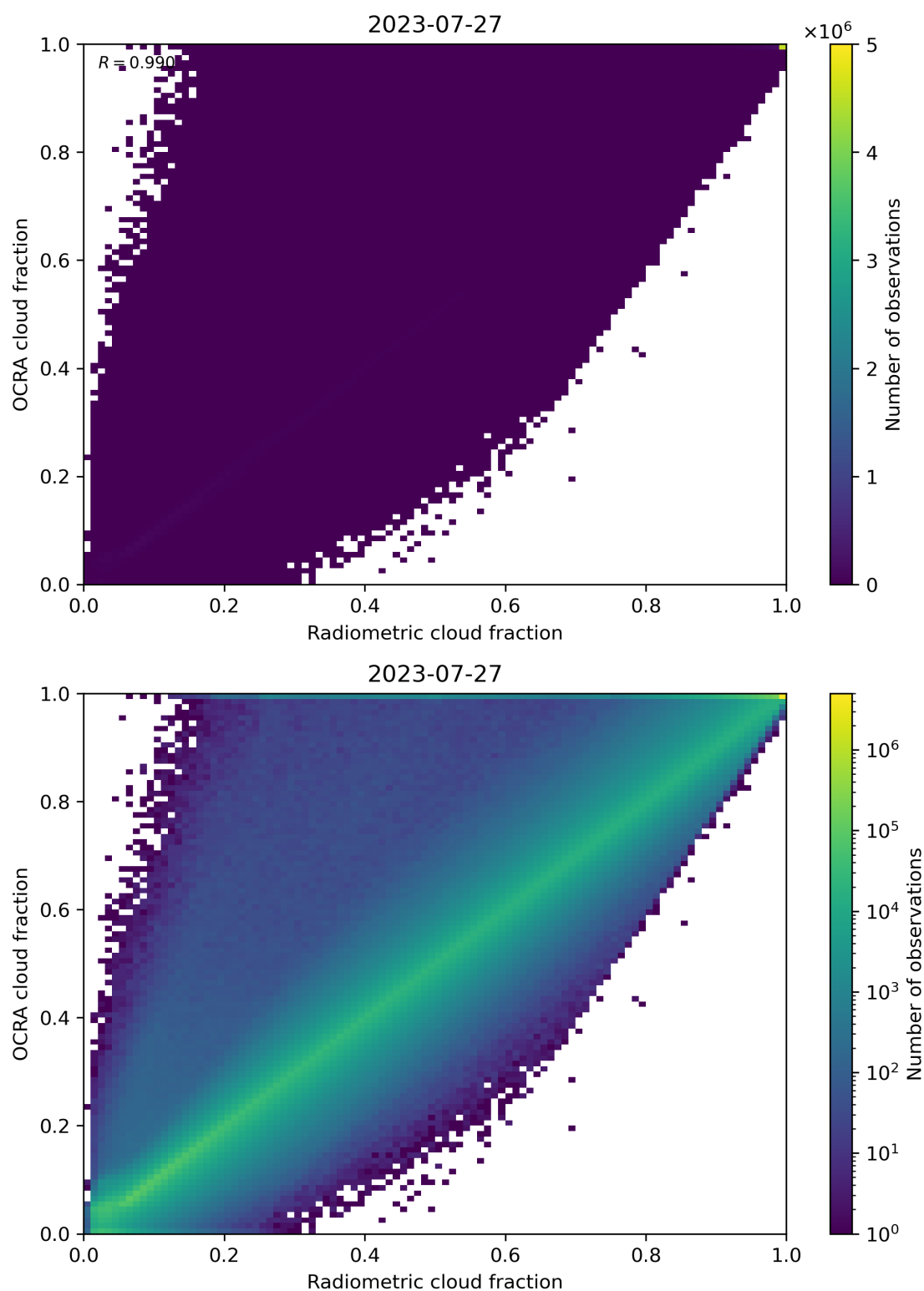
Figure 72: Scatter density plot of “Radiometric cloud fraction” against “OCRA cloud fraction” for 2023-07-26 to 2023-07-28.
