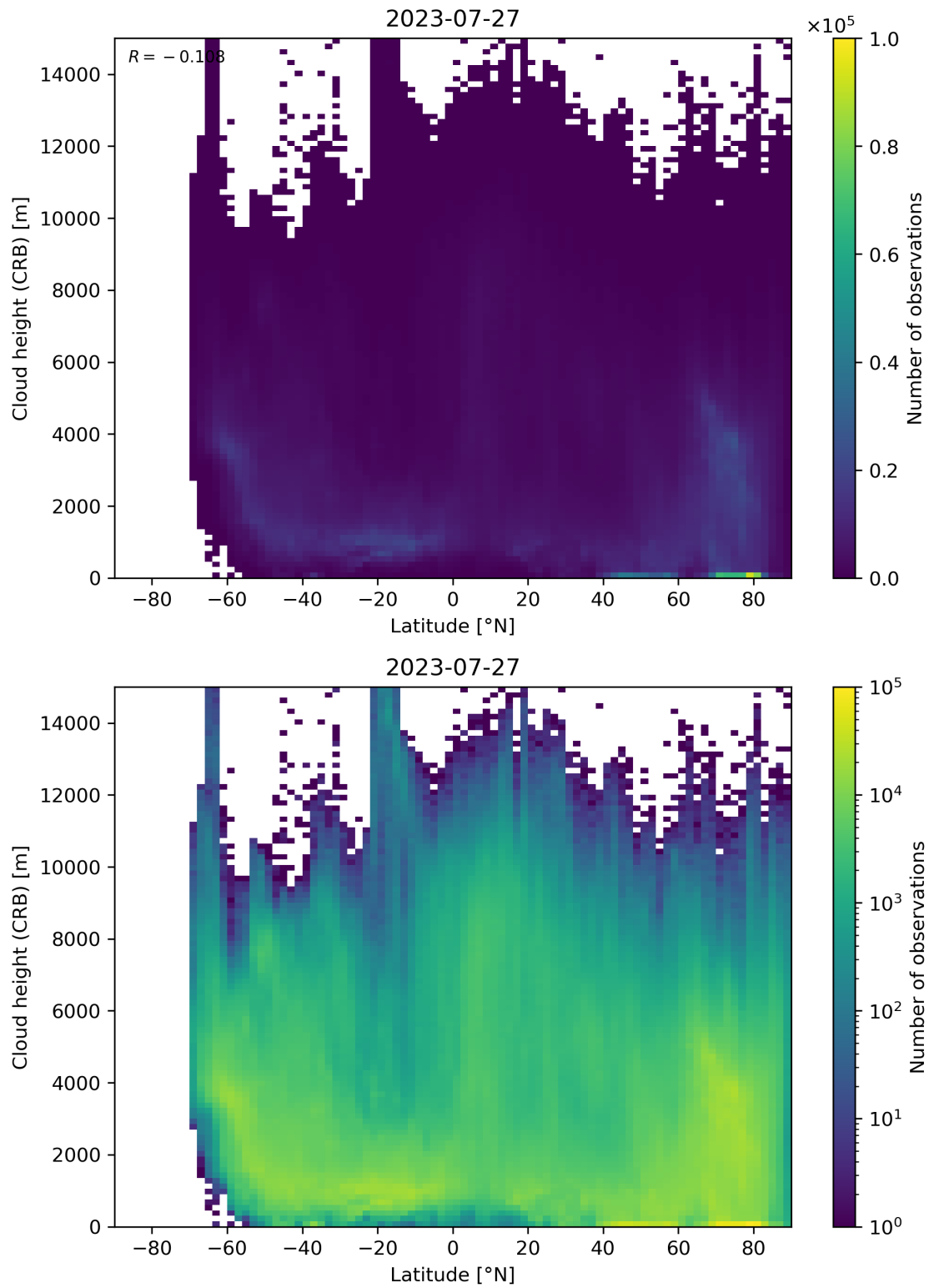
Figure 95: Scatter density plot of “Latitude” against “Cloud height (CRB)” for 2023-07-26 to 2023-07-28.
