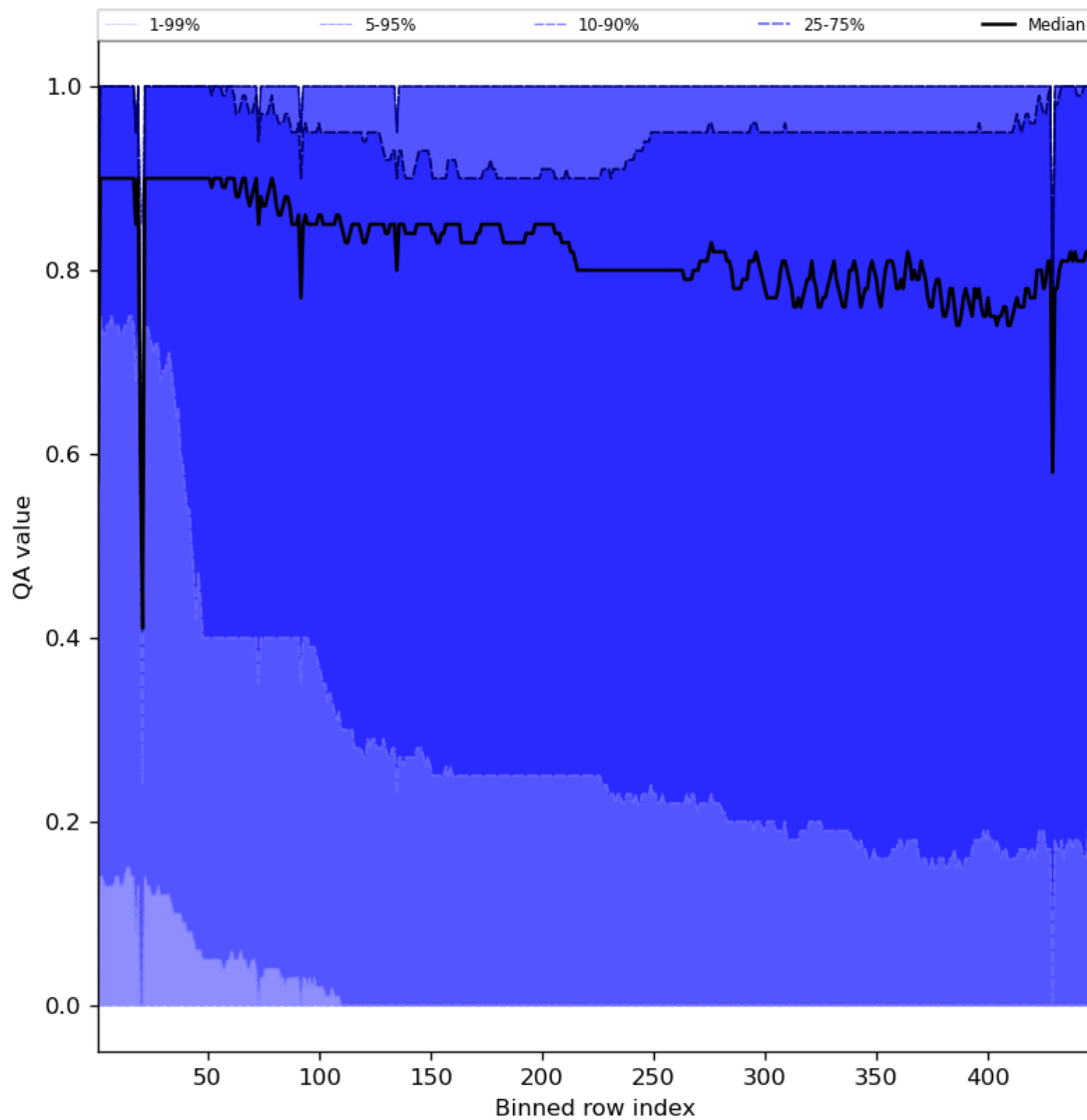
Figure 54: Along track statistics of “QA value” for 2023-07-26 to 2023-07-28
