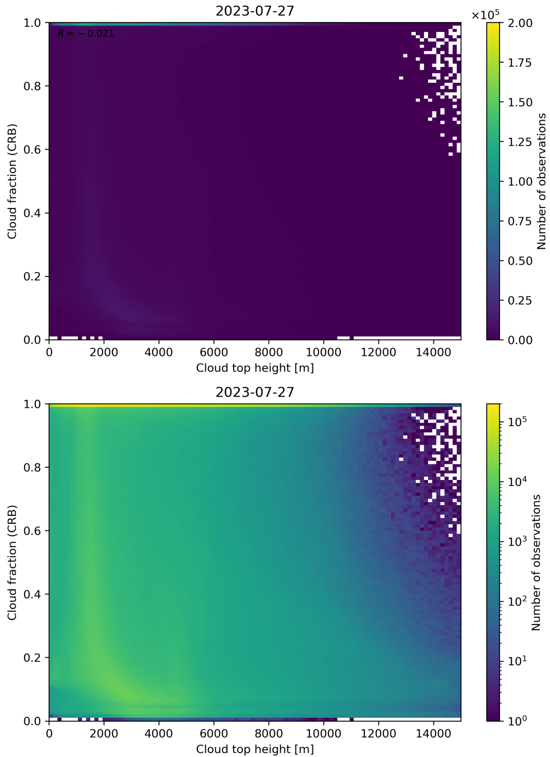
Figure 88: Scatter density plot of “Cloud top height” against “Cloud fraction (CRB)” for 2023-07-26 to 2023-07-28.
