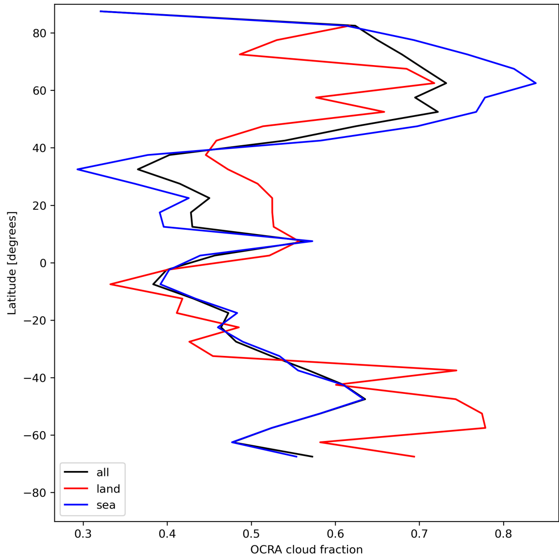
Figure 34: Zonal average of “OCRA cloud fraction” for 2023-07-26 to 2023-07-28.
