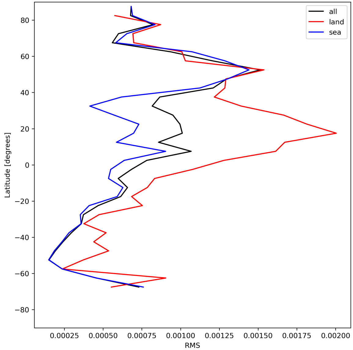
Figure 31: Zonal average of “RMS” for 2023-07-26 to 2023-07-28.
