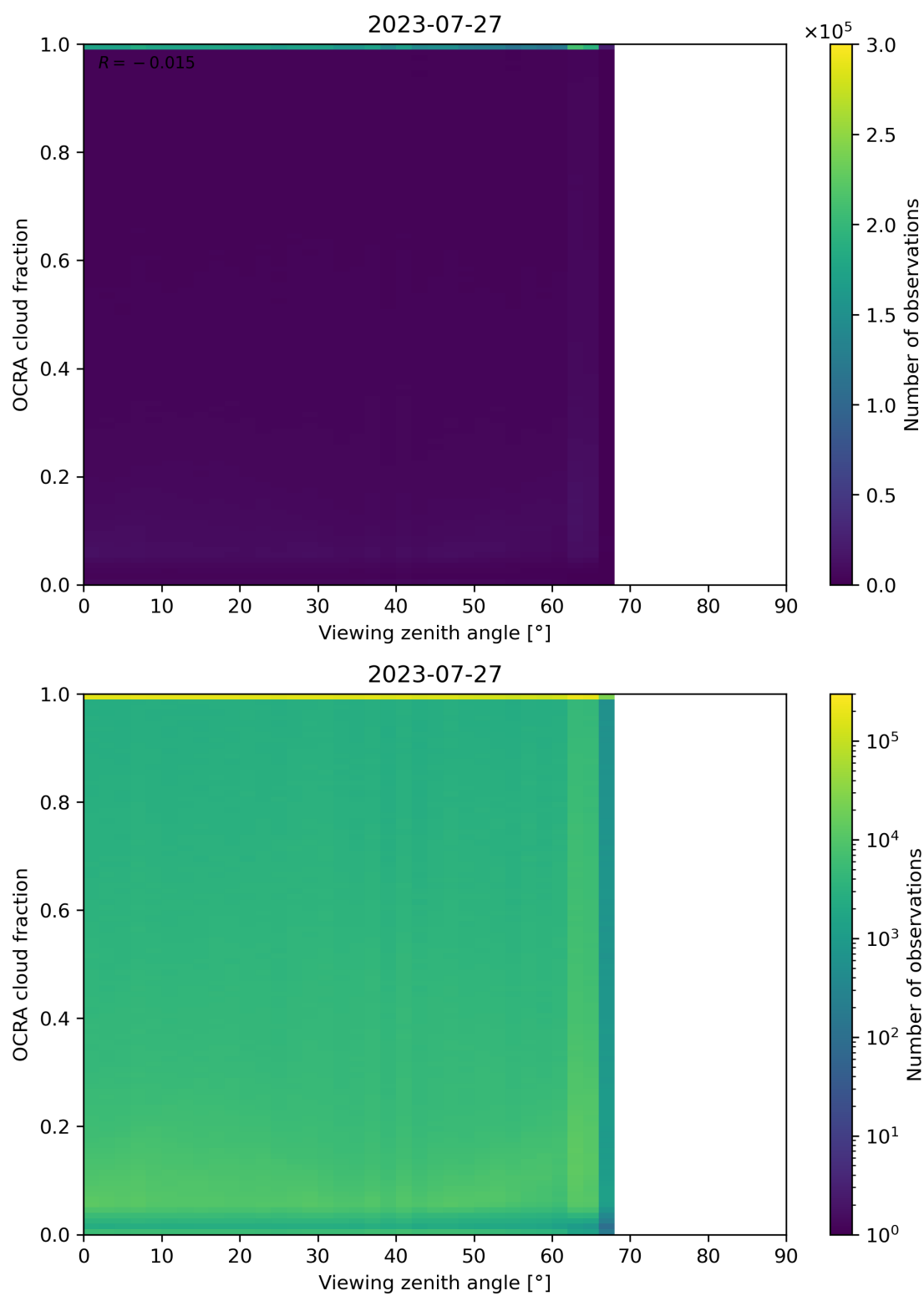
Figure 108: Scatter density plot of “Viewing zenith angle” against “OCRA cloud fraction” for 2023-07-26 to 2023-07-28.
