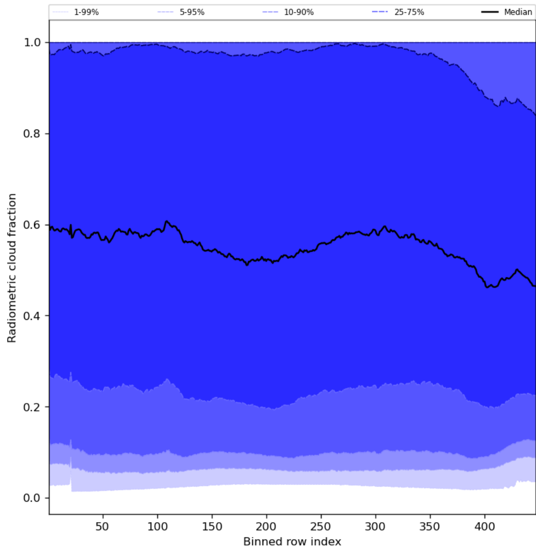
Figure 55: Along track statistics of “Radiometric cloud fraction” for 2023-07-26 to 2023-07-28
