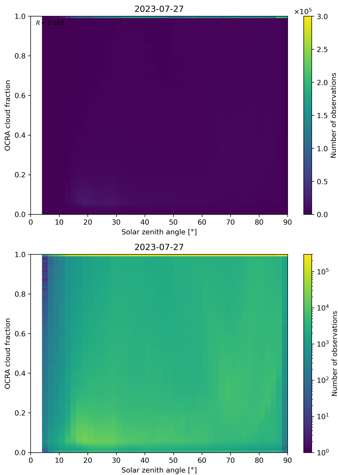
Figure 100: Scatter density plot of “Solar zenith angle” against “OCRA cloud fraction” for 2023-07-26 to 2023-07-28.
