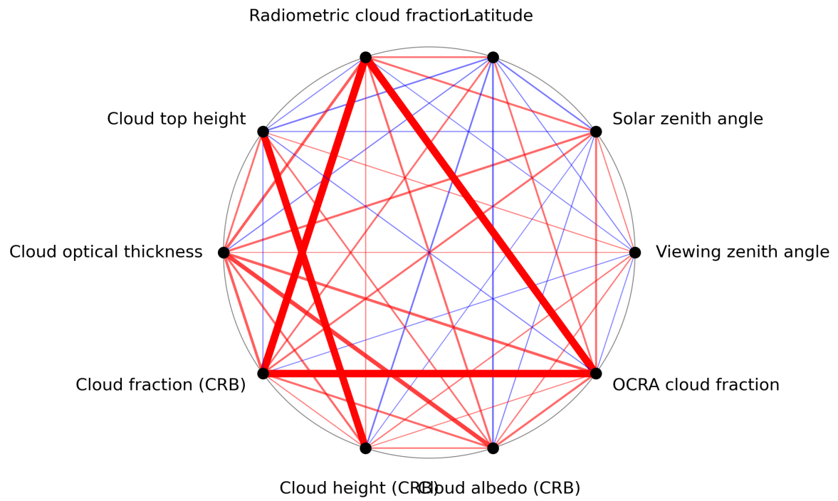
Figure 1: Map of correlation graph for 2023-07-26 to 2023-07-28.
