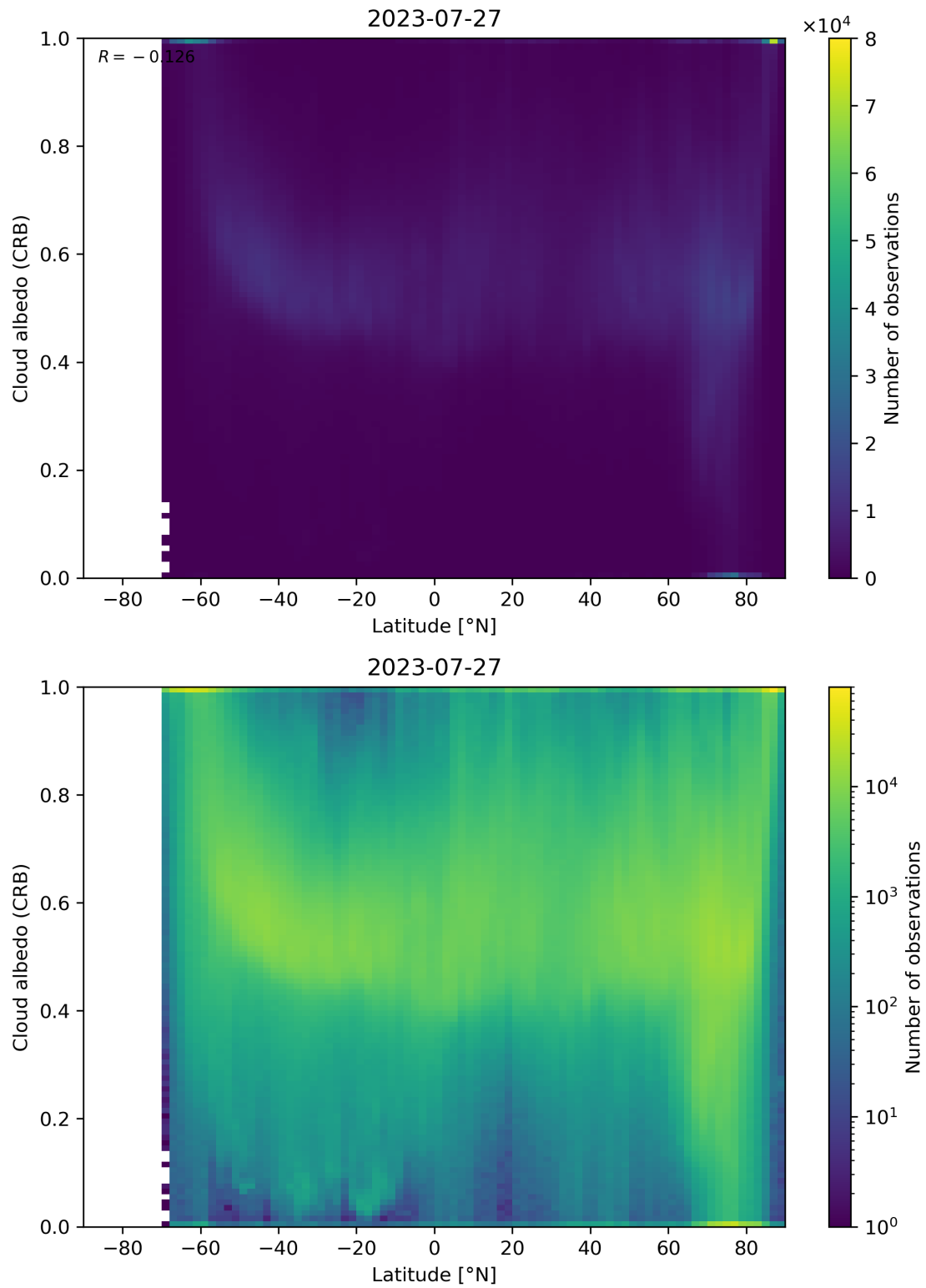
Figure 91: Scatter density plot of “Latitude” against “Cloud albedo (CRB)” for 2023-07-26 to 2023-07-28.
