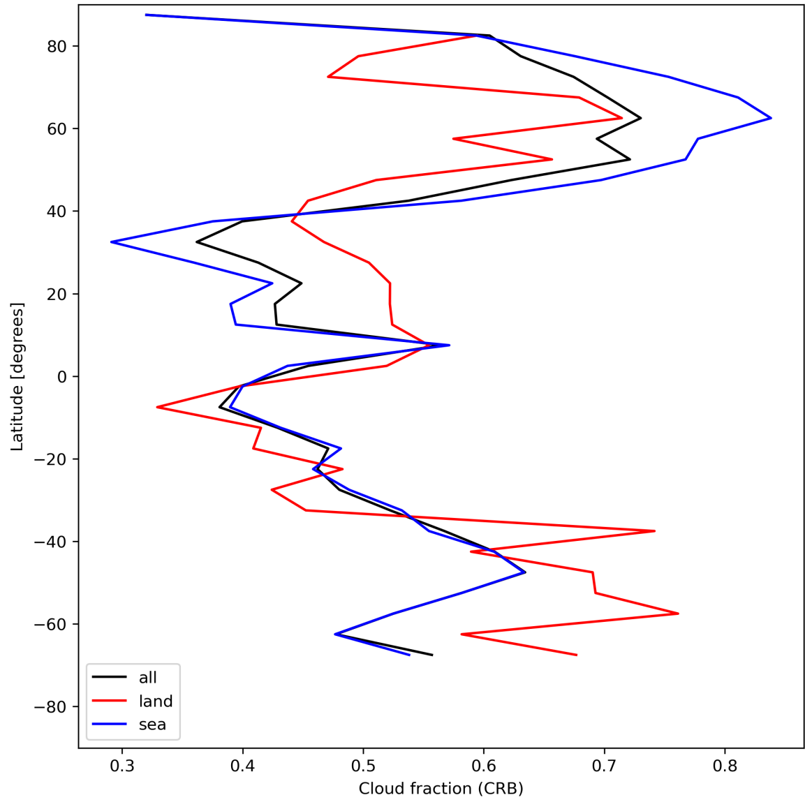
Figure 26: Zonal average of “Cloud fraction (CRB)” for 2023-07-26 to 2023-07-28.
