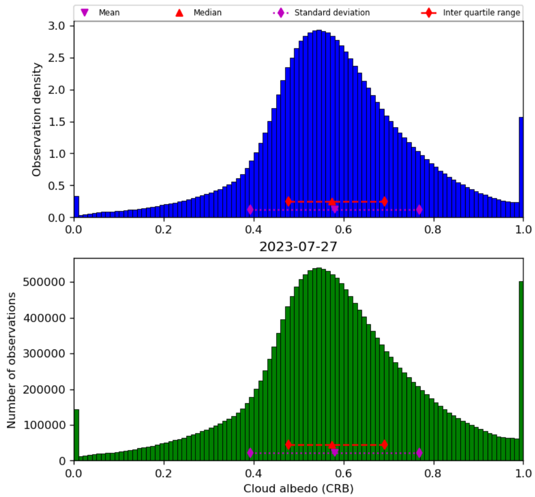
Figure 44: Histogram of “Cloud albedo (CRB)” for 2023-07-26 to 2023-07-28
