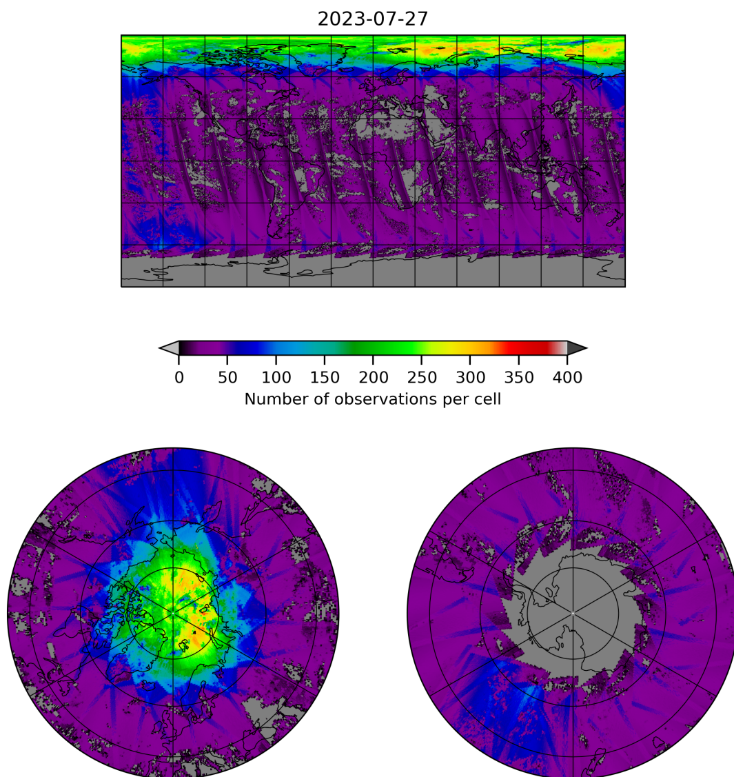
Figure 21: Map of the number of observations for 2023-07-26 to 2023-07-28
