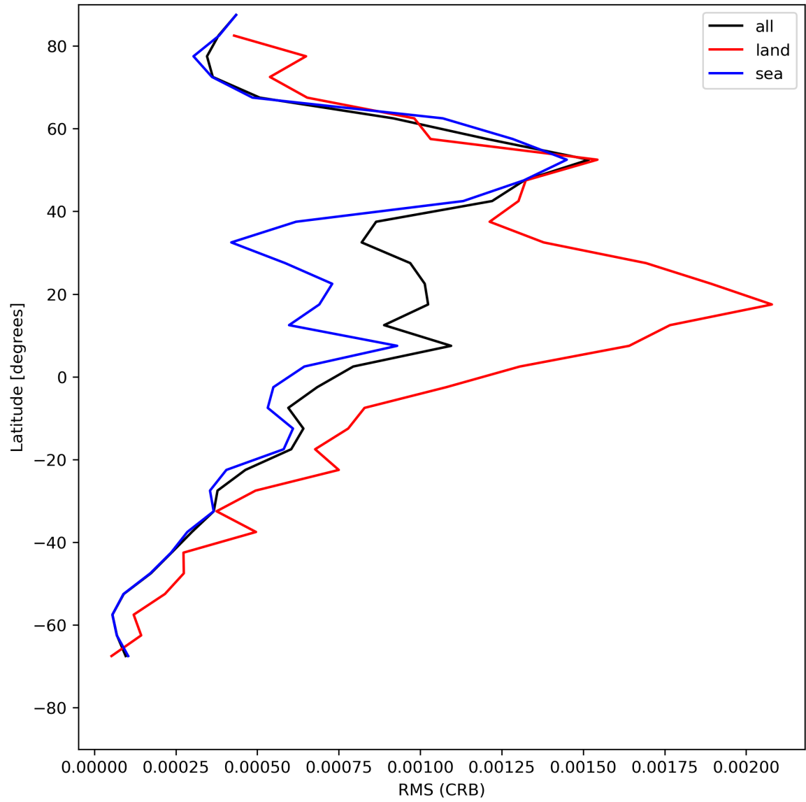
Figure 32: Zonal average of “RMS (CRB)” for 2023-07-26 to 2023-07-28.
