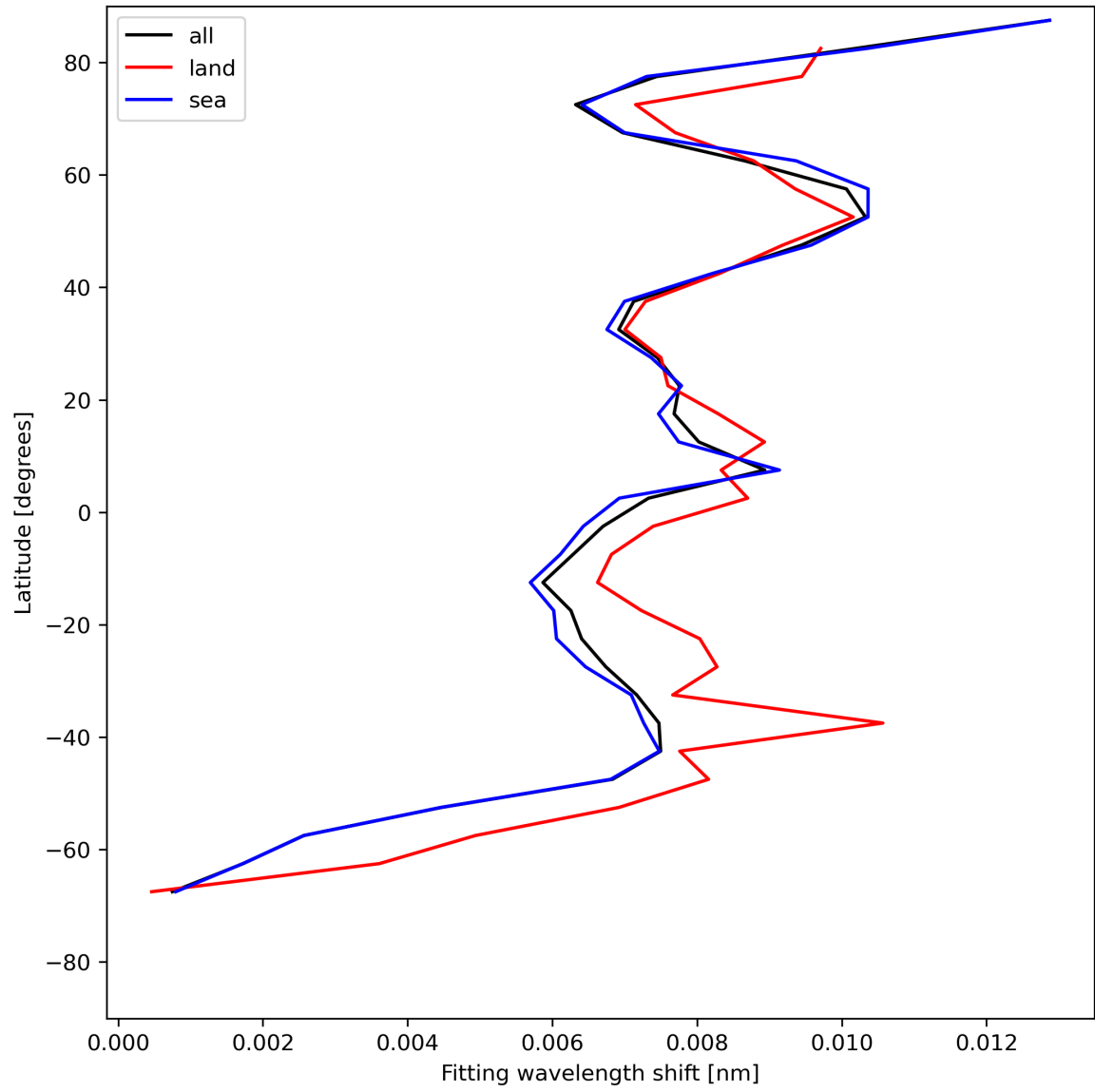
Figure 33: Zonal average of “Fitting wavelength shift” for 2023-07-26 to 2023-07-28.
