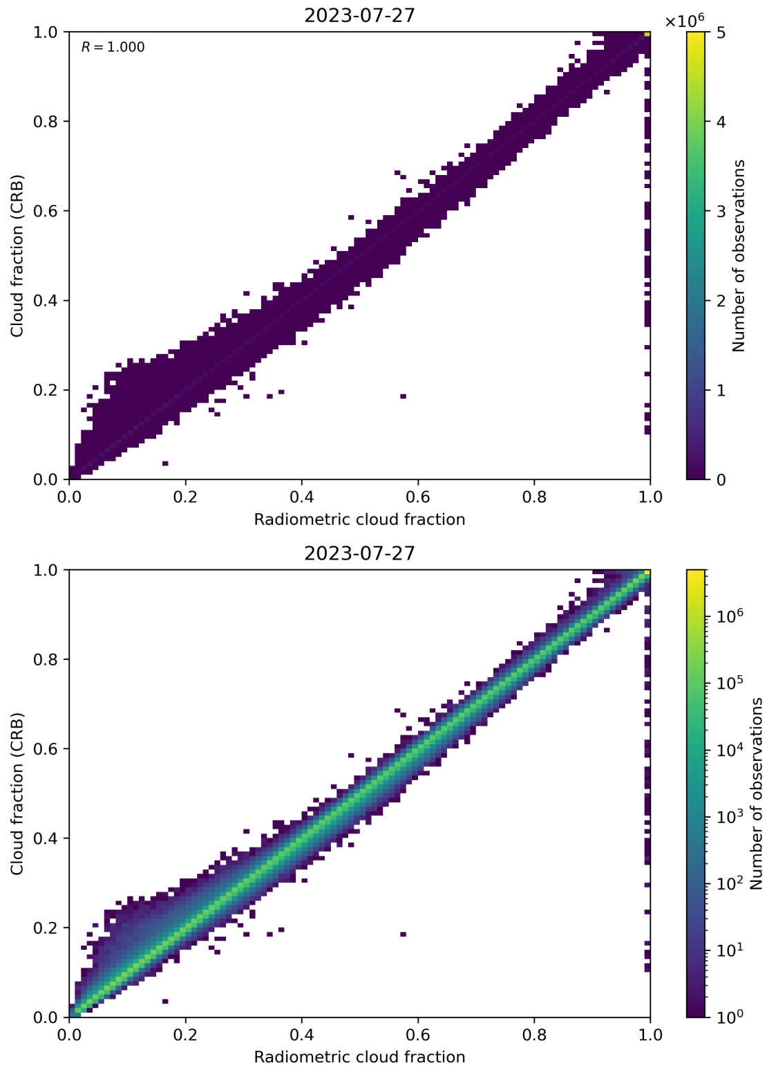
Figure 73: Scatter density plot of “Radiometric cloud fraction” against “Cloud fraction (CRB)” for 2023-07-26 to 2023-07-28.
