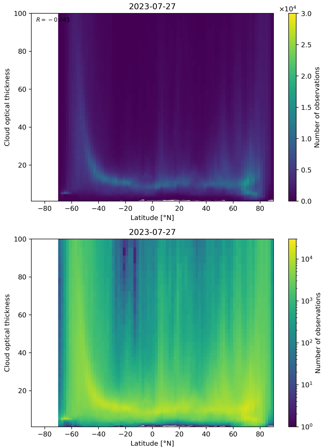
Figure 96: Scatter density plot of “Latitude” against “Cloud optical thickness” for 2023-07-26 to 2023-07-28.
