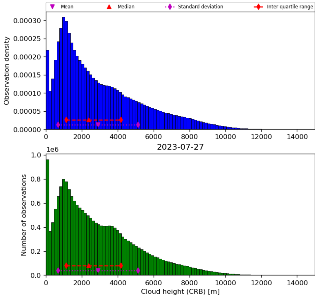
Figure 43: Histogram of “Cloud height (CRB)” for 2023-07-26 to 2023-07-28
