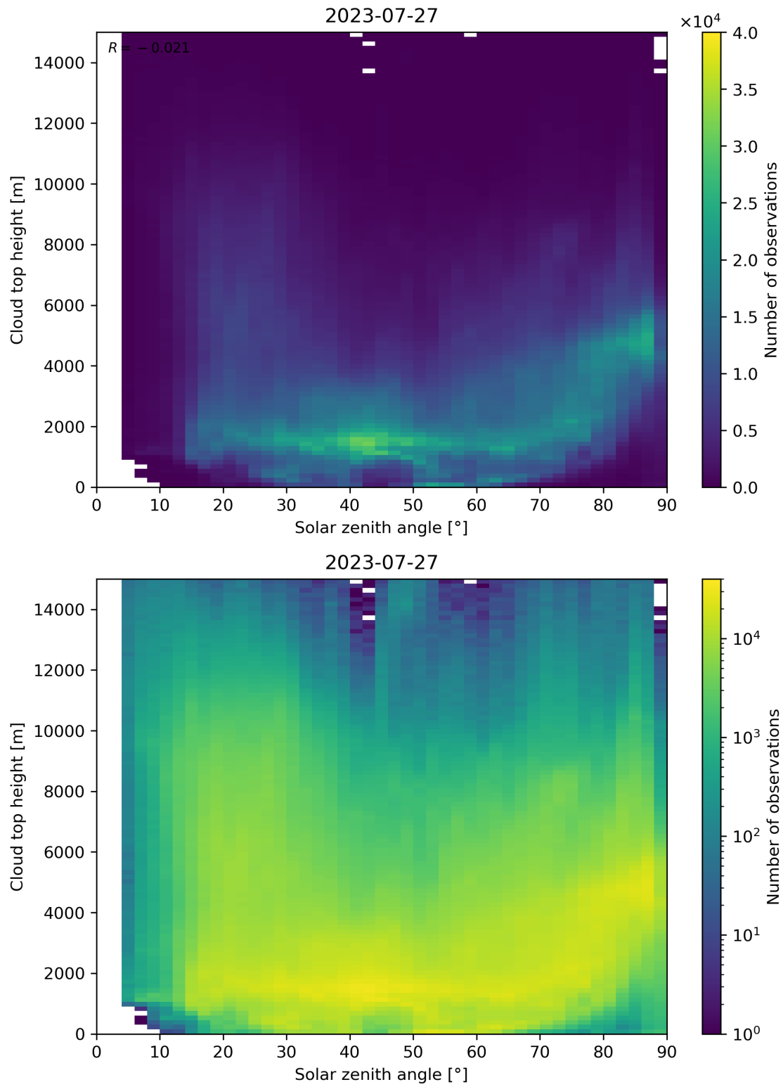
Figure 104: Scatter density plot of “Solar zenith angle” against “Cloud top height” for 2023-07-26 to 2023-07-28.
