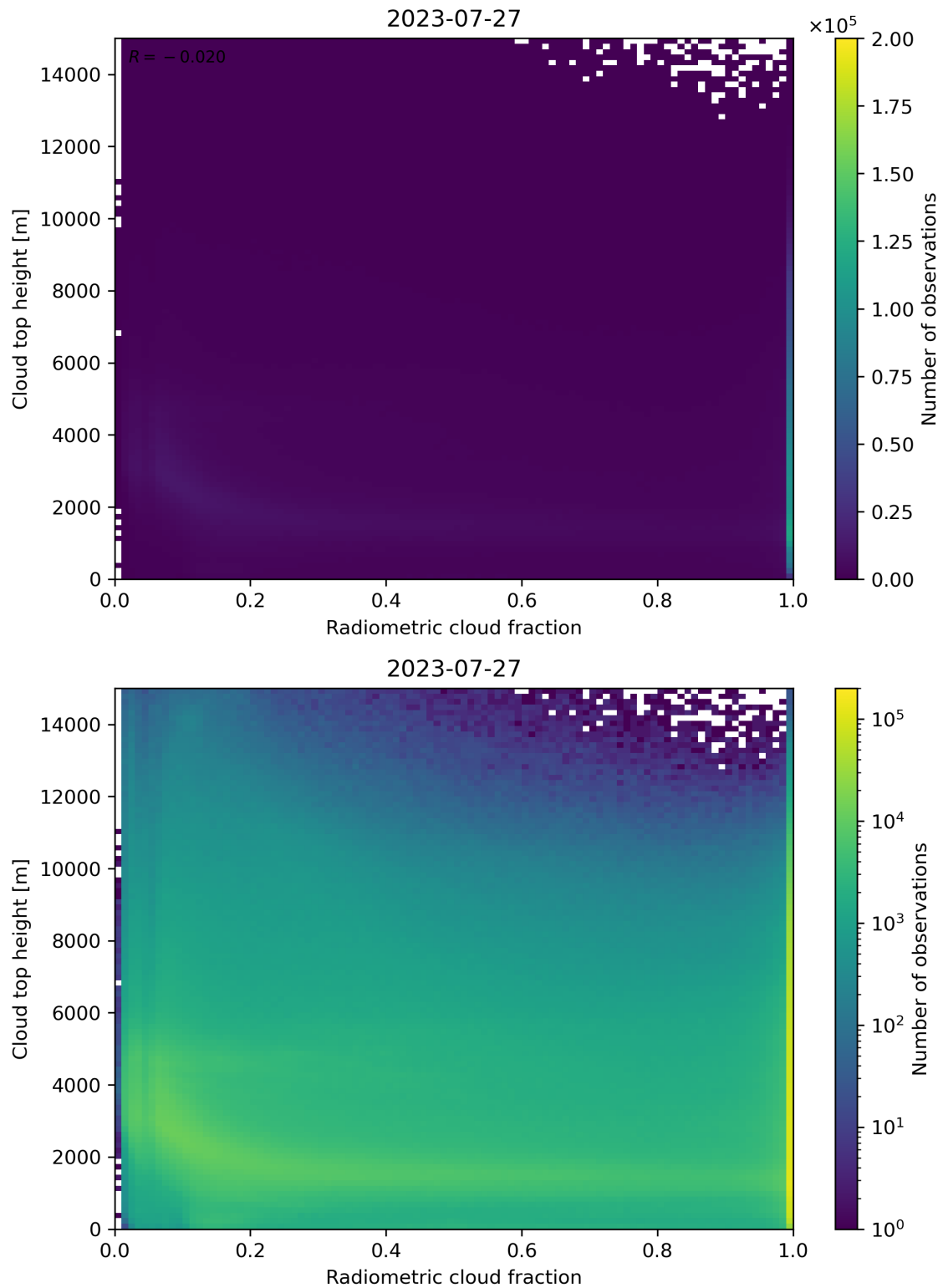
Figure 76: Scatter density plot of “Radiometric cloud fraction” against “Cloud top height” for 2023-07-26 to 2023-07-28.
