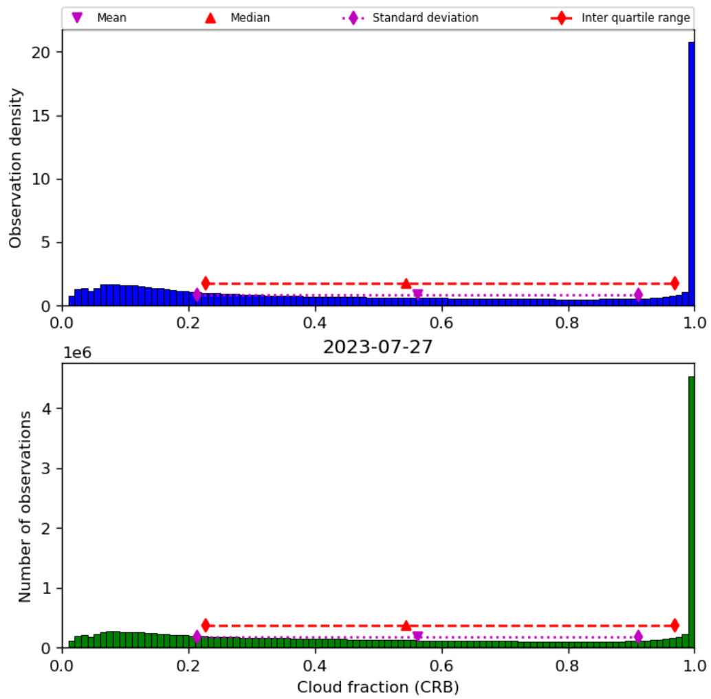
Figure 42: Histogram of “Cloud fraction (CRB)” for 2023-07-26 to 2023-07-28
