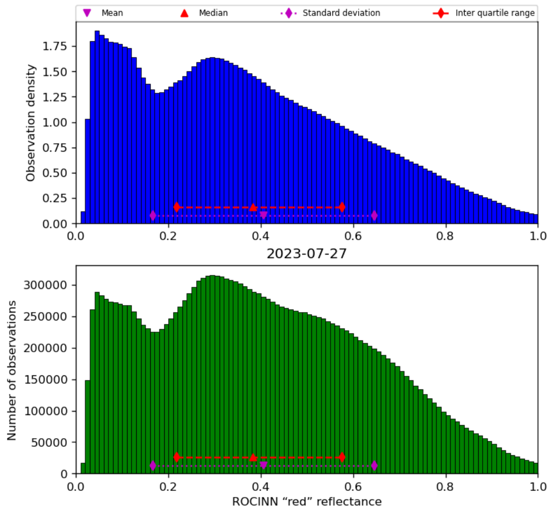
Figure 53: Histogram of “ROCINN “red” reflectance” for 2023-07-26 to 2023-07-28
