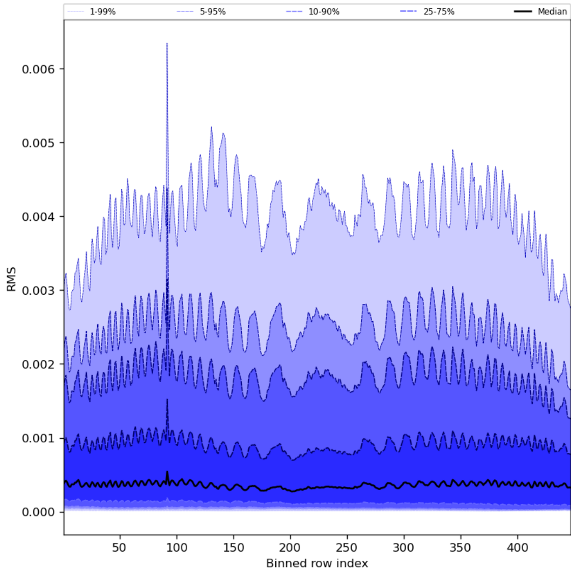
Figure 63: Along track statistics of “RMS” for 2023-07-26 to 2023-07-28
