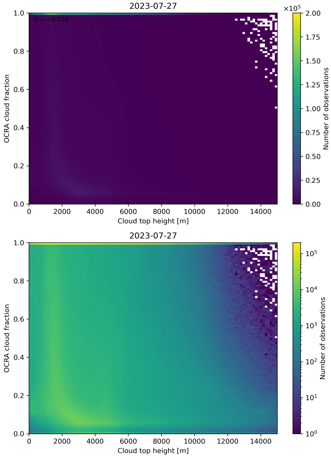
Figure 87: Scatter density plot of “Cloud top height” against “OCRA cloud fraction” for 2023-07-26 to 2023-07-28.
