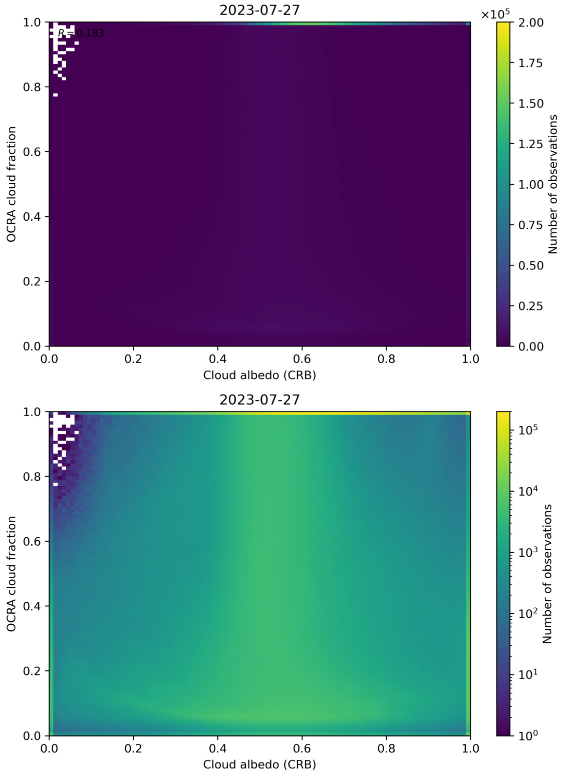
Figure 70: Scatter density plot of “Cloud albedo (CRB)” against “OCRA cloud fraction” for 2023-07-26 to 2023-07-28.
