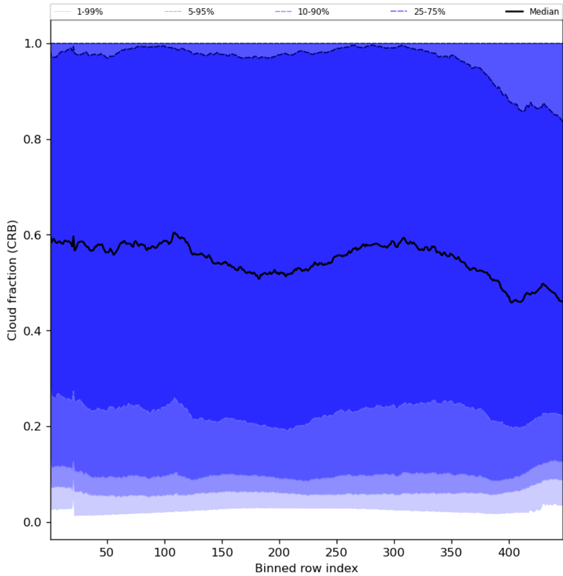
Figure 58: Along track statistics of “Cloud fraction (CRB)” for 2023-07-26 to 2023-07-28
