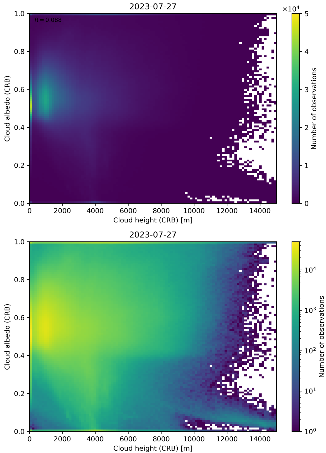
Figure 80: Scatter density plot of “Cloud height (CRB)” against “Cloud albedo (CRB)” for 2023-07-26 to 2023-07-28.
