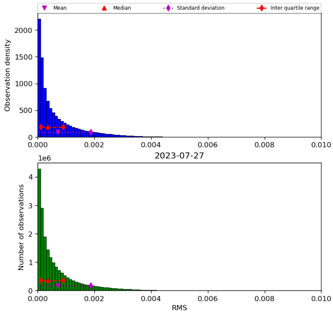
Figure 47: Histogram of “RMS” for 2023-07-26 to 2023-07-28
