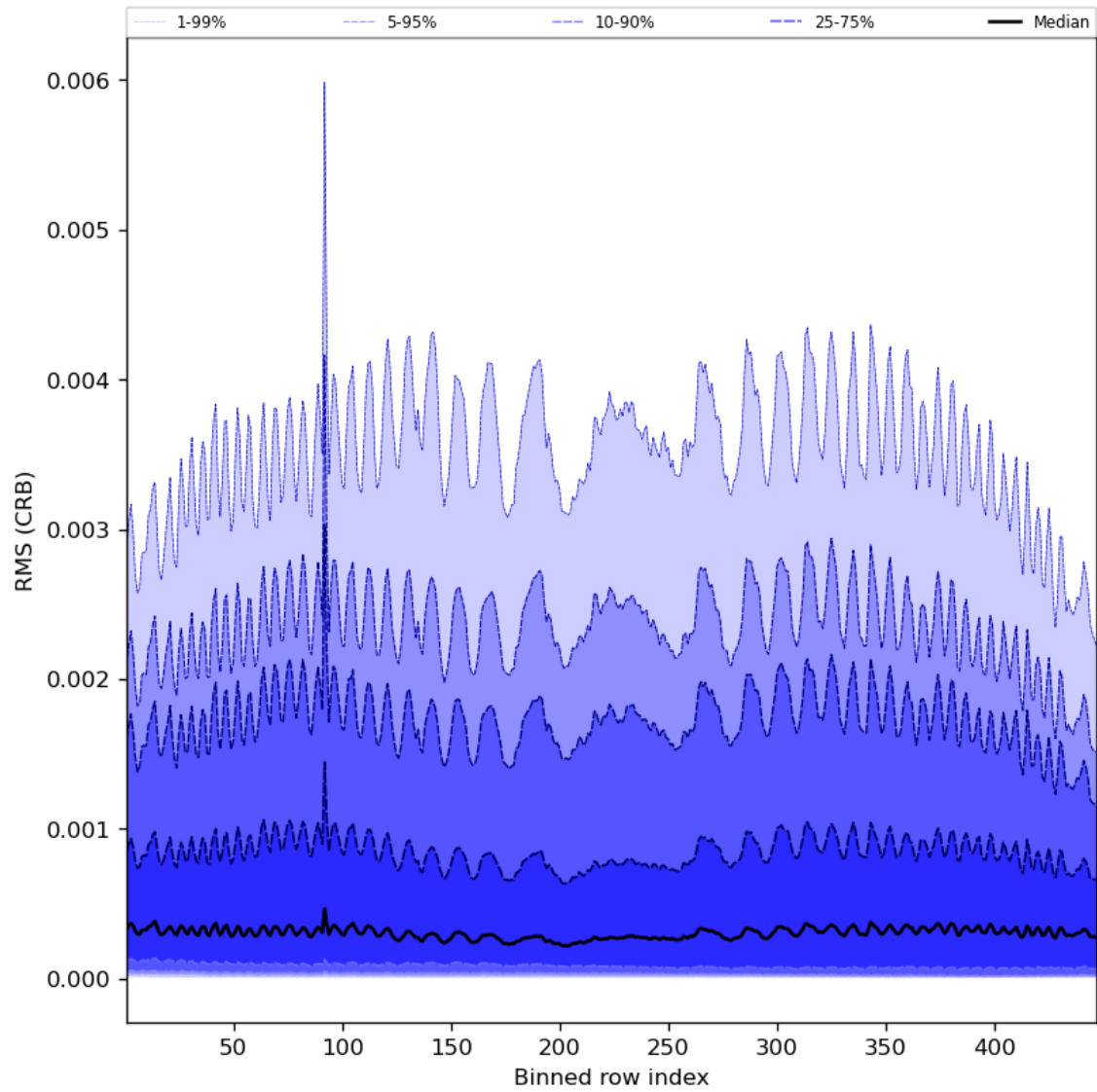
Figure 64: Along track statistics of “RMS (CRB)” for 2023-07-26 to 2023-07-28
