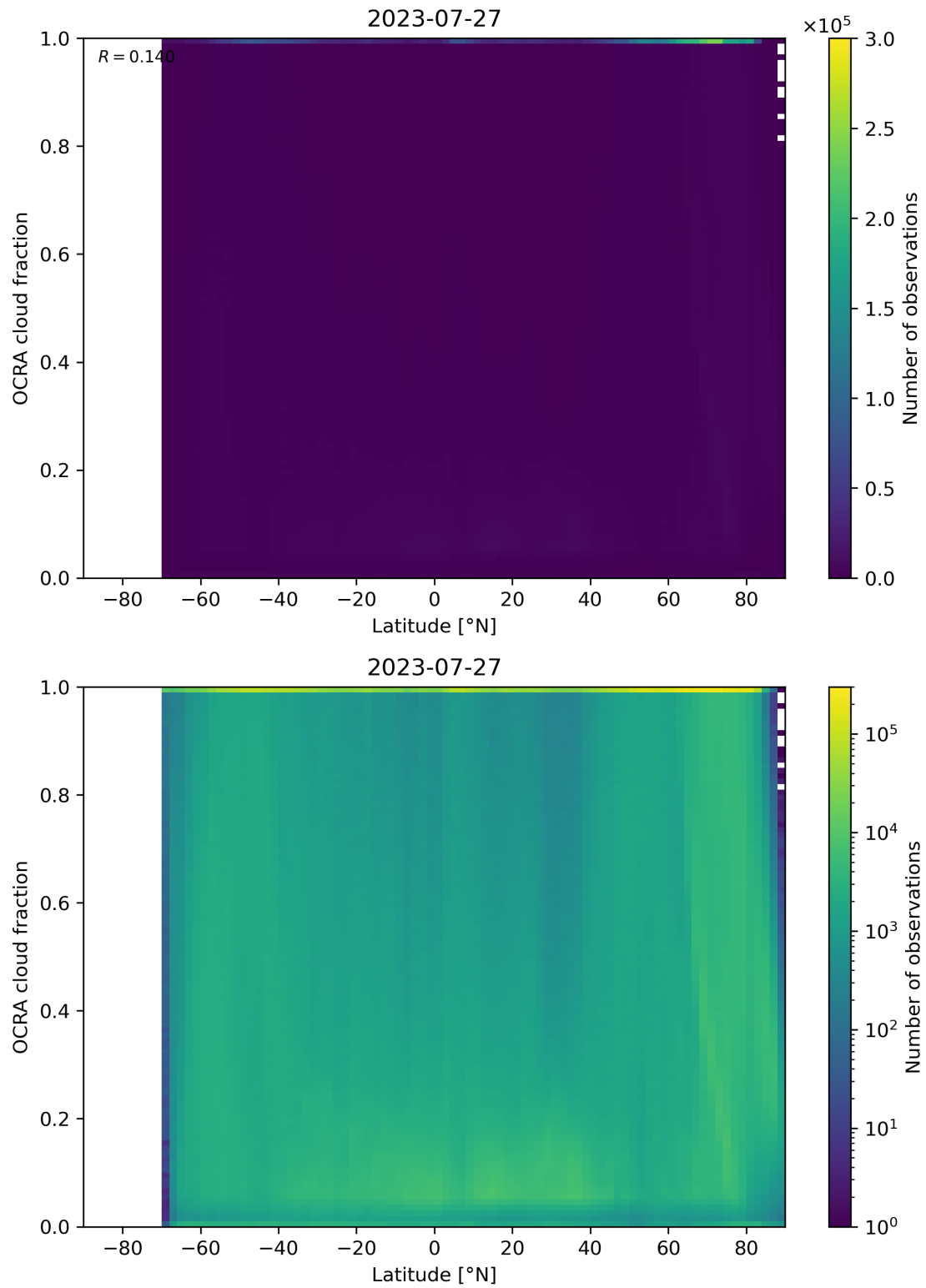
Figure 93: Scatter density plot of “Latitude” against “OCRA cloud fraction” for 2023-07-26 to 2023-07-28.
