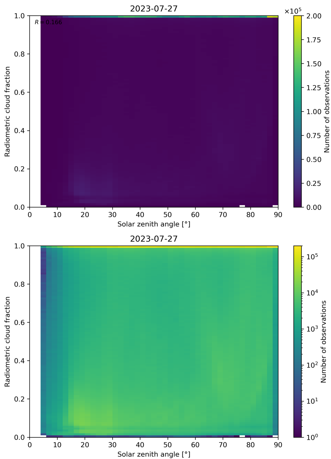
Figure 99: Scatter density plot of “Solar zenith angle” against “Radiometric cloud fraction” for 2023-07-26 to 2023-07-28.
