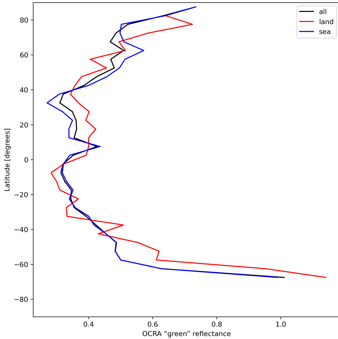
Figure 36: Zonal average of “OCRA “green” reflectance” for 2023-07-26 to 2023-07-28.
