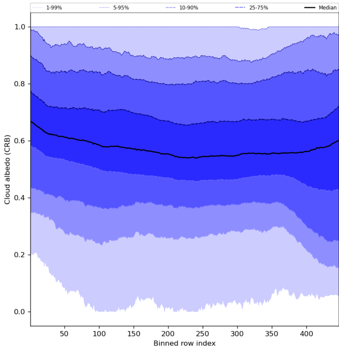
Figure 60: Along track statistics of “Cloud albedo (CRB)” for 2023-07-26 to 2023-07-28
