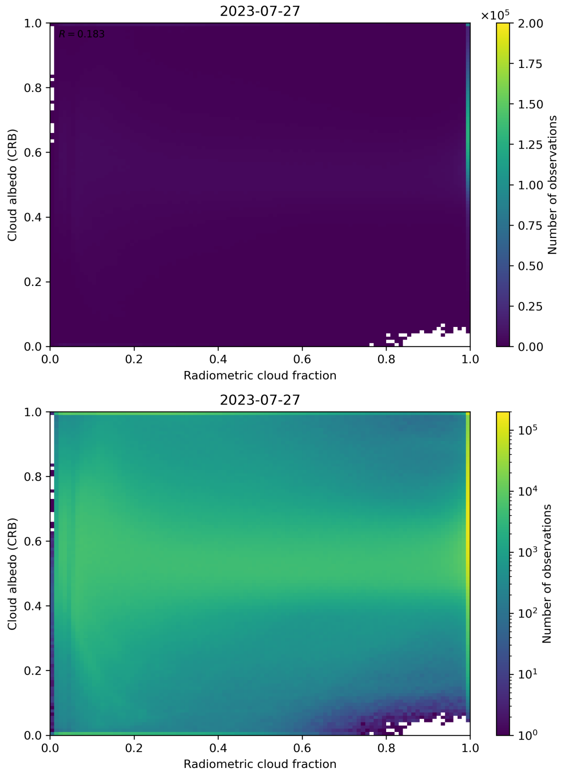
Figure 71: Scatter density plot of “Radiometric cloud fraction” against “Cloud albedo (CRB)” for 2023-07-26 to 2023-07-28.
