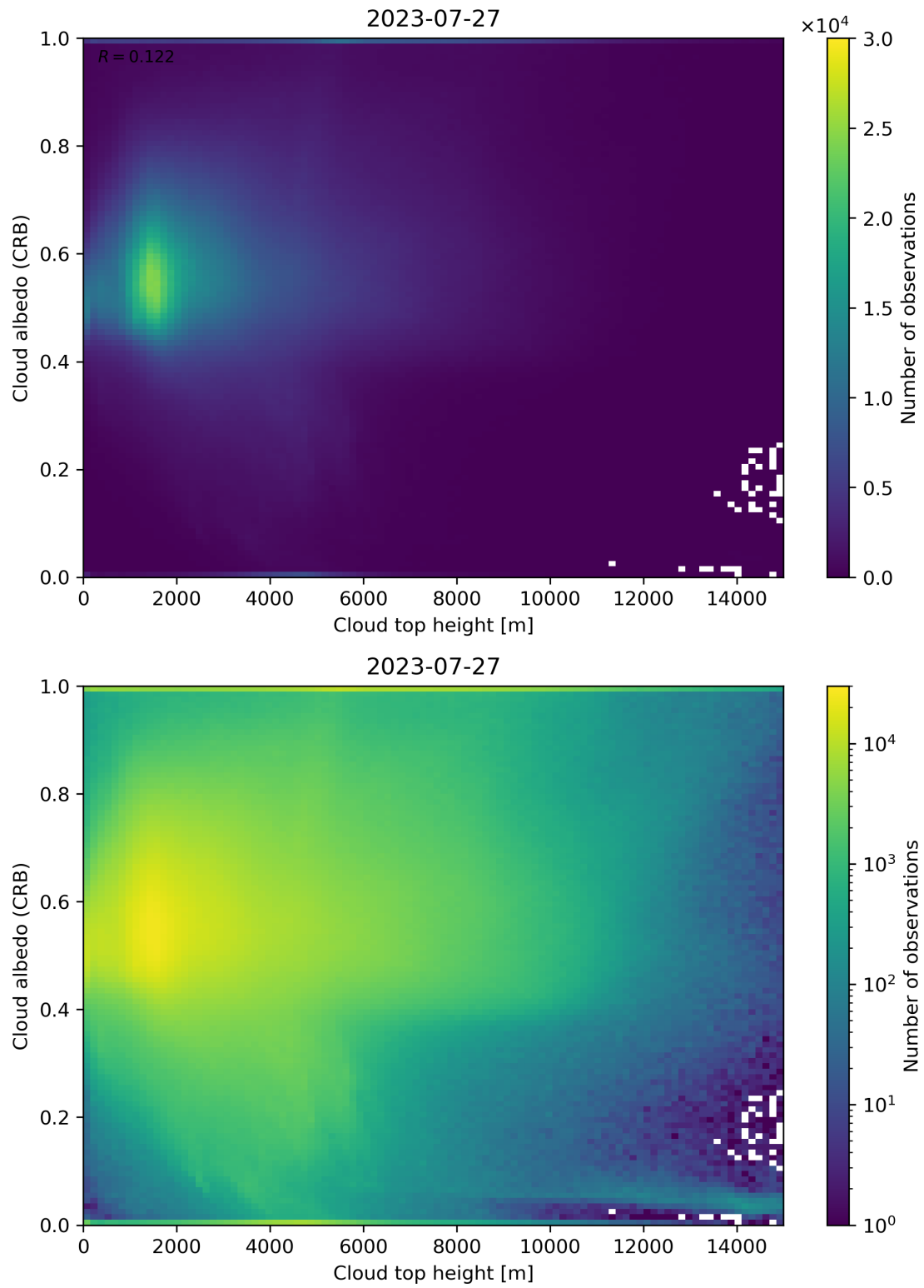
Figure 86: Scatter density plot of “Cloud top height” against “Cloud albedo (CRB)” for 2023-07-26 to 2023-07-28.
