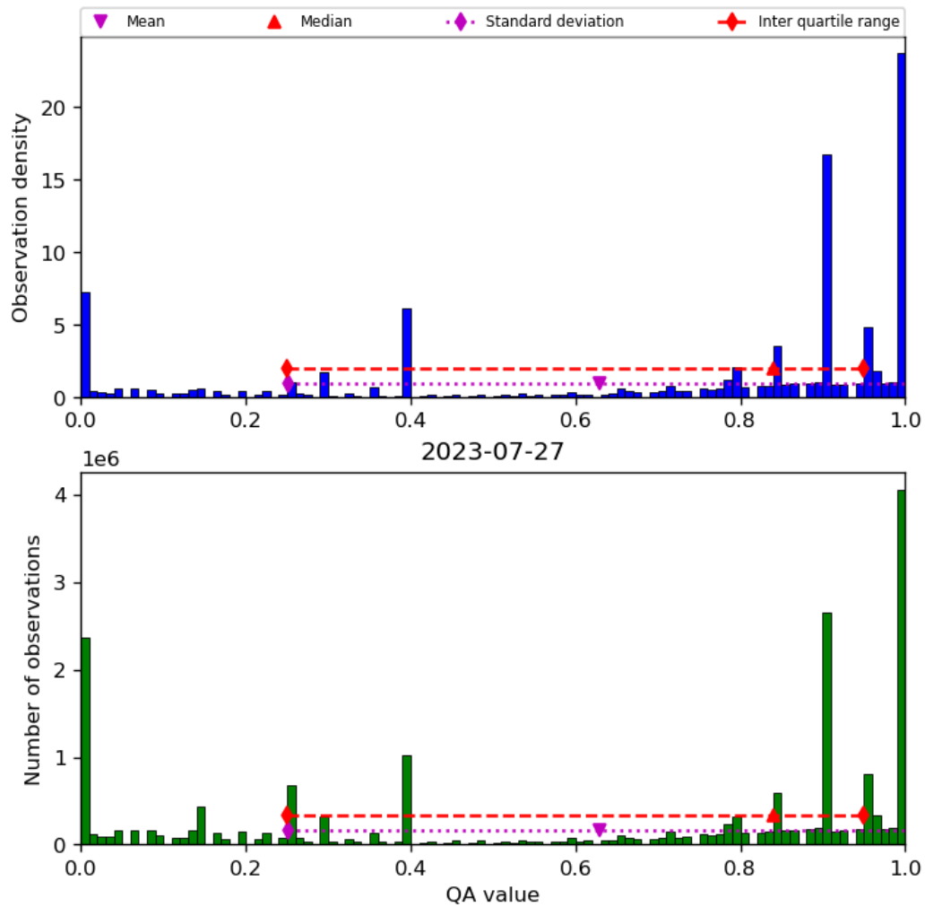
Figure 38: Histogram of “QA value” for 2023-07-26 to 2023-07-28
