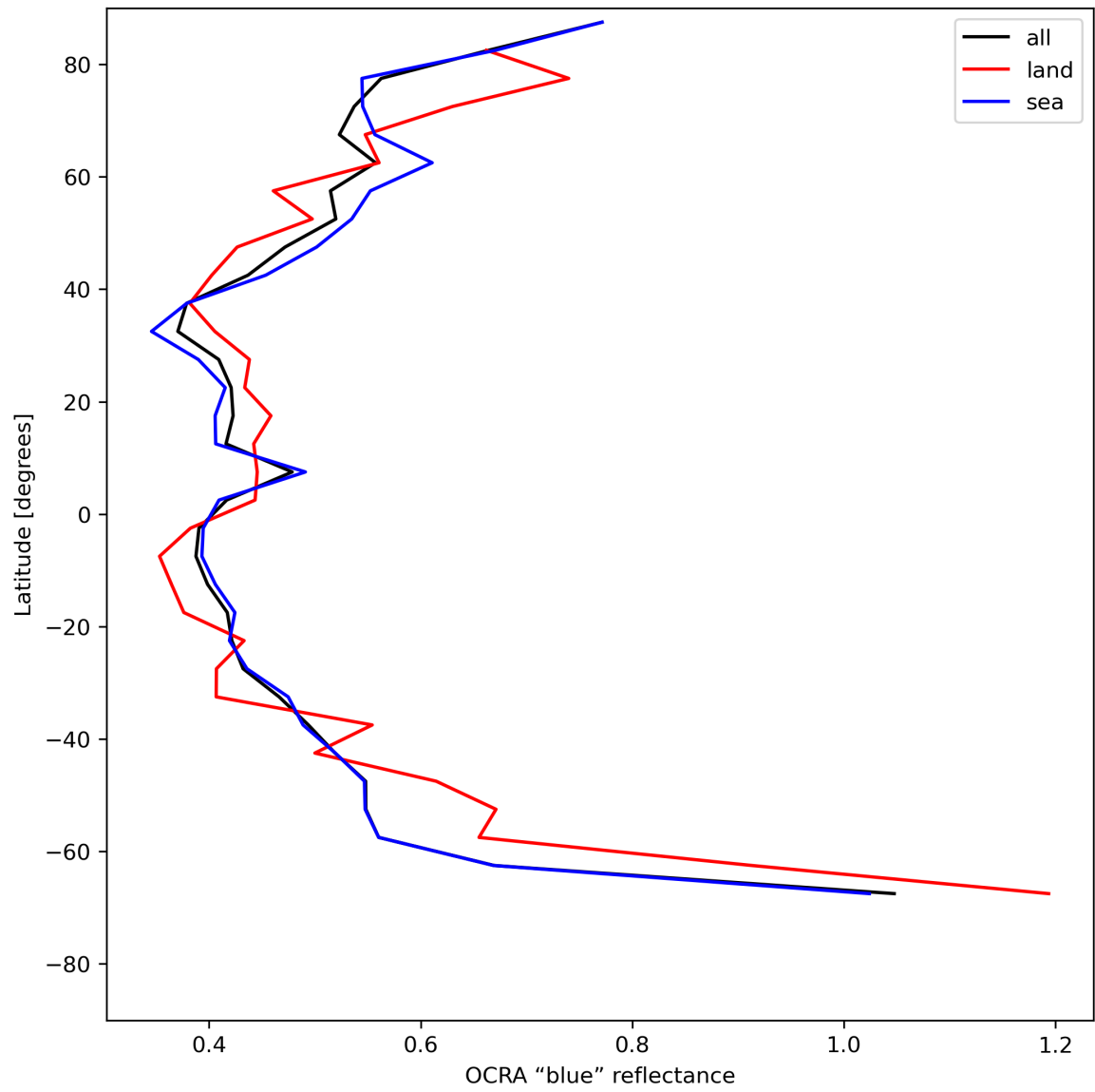
Figure 35: Zonal average of "OCRA "blue" reflectance" for 2023-07-26 to 2023-07-28.
