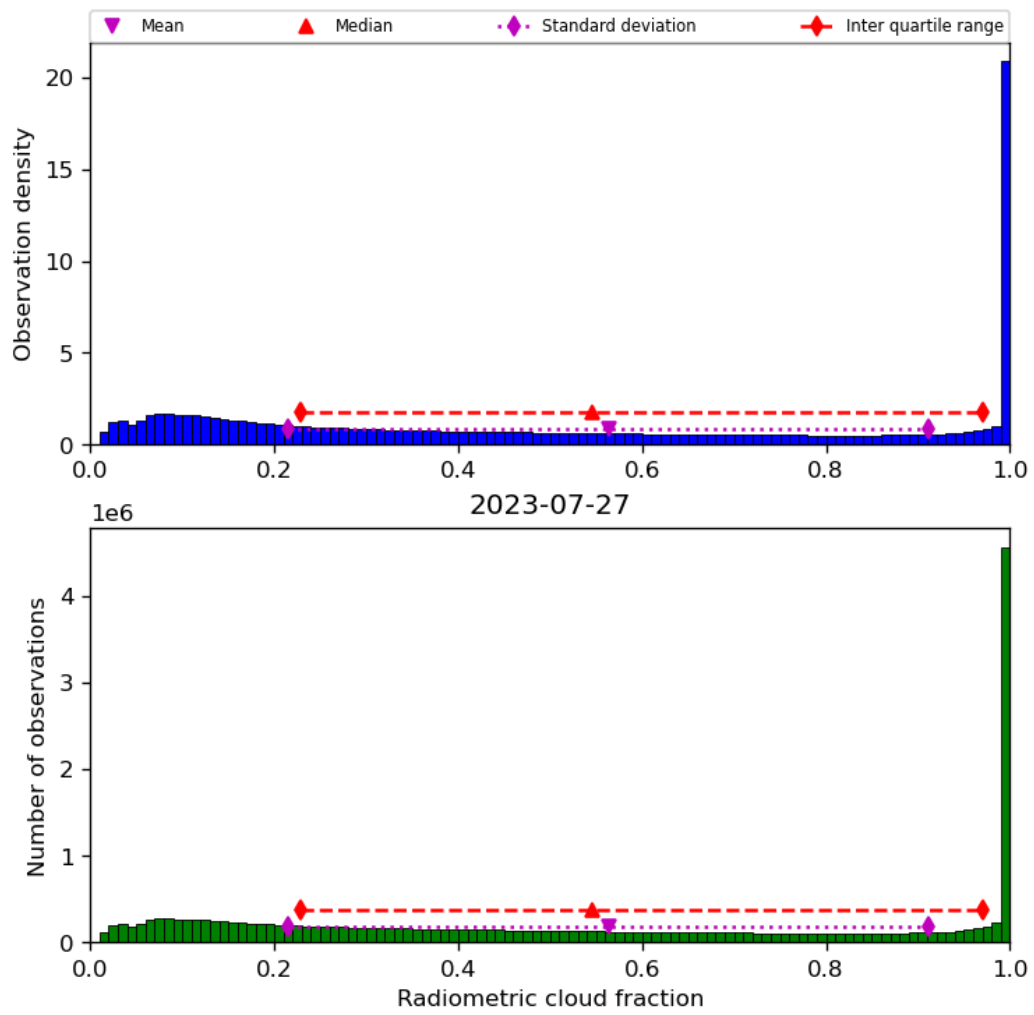
Figure 39: Histogram of “Radiometric cloud fraction” for 2023-07-26 to 2023-07-28
