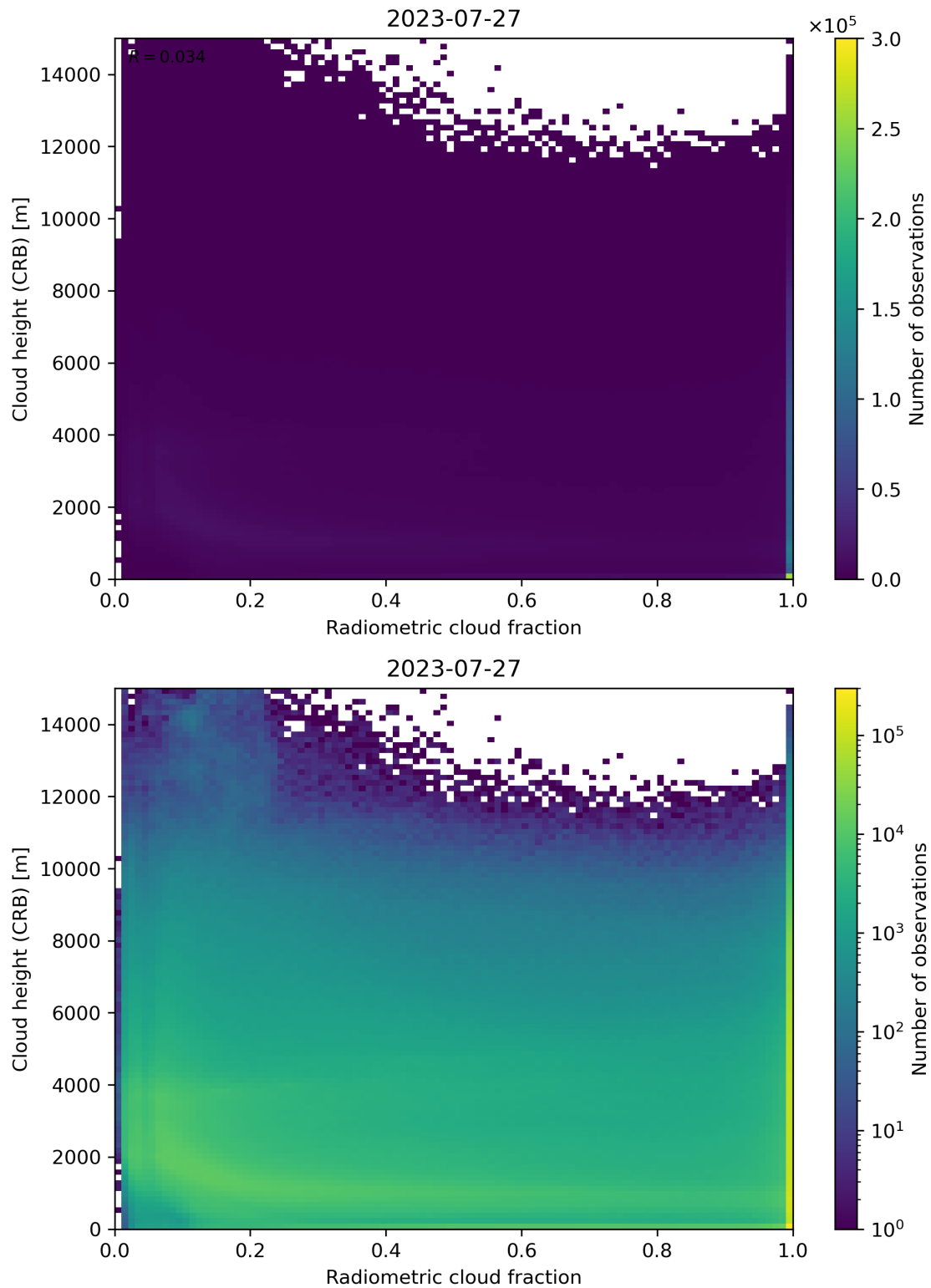
Figure 74: Scatter density plot of “Radiometric cloud fraction” against “Cloud height (CRB)” for 2023-07-26 to 2023-07-28.
