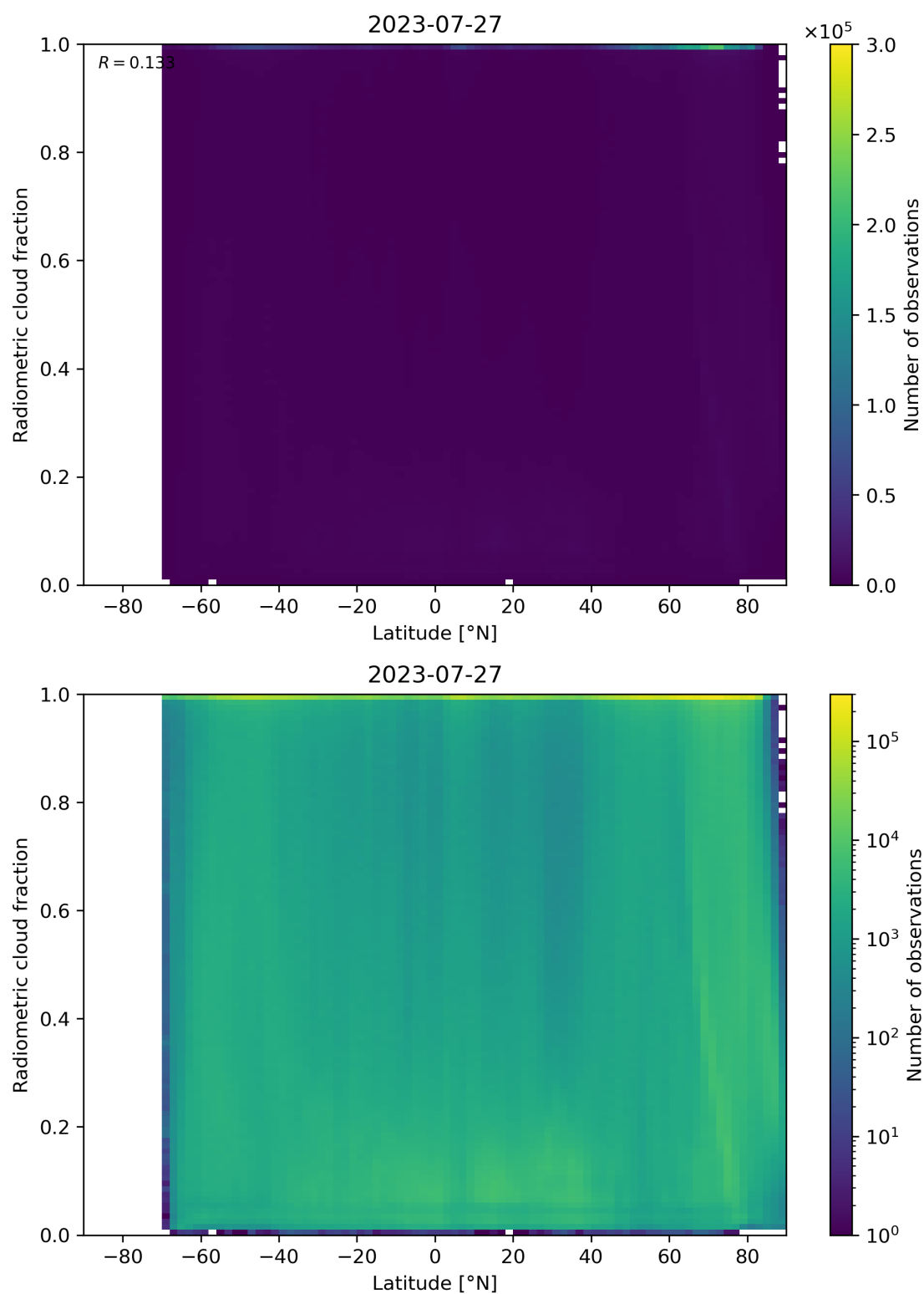
Figure 92: Scatter density plot of “Latitude” against “Radiometric cloud fraction” for 2023-07-26 to 2023-07-28.
