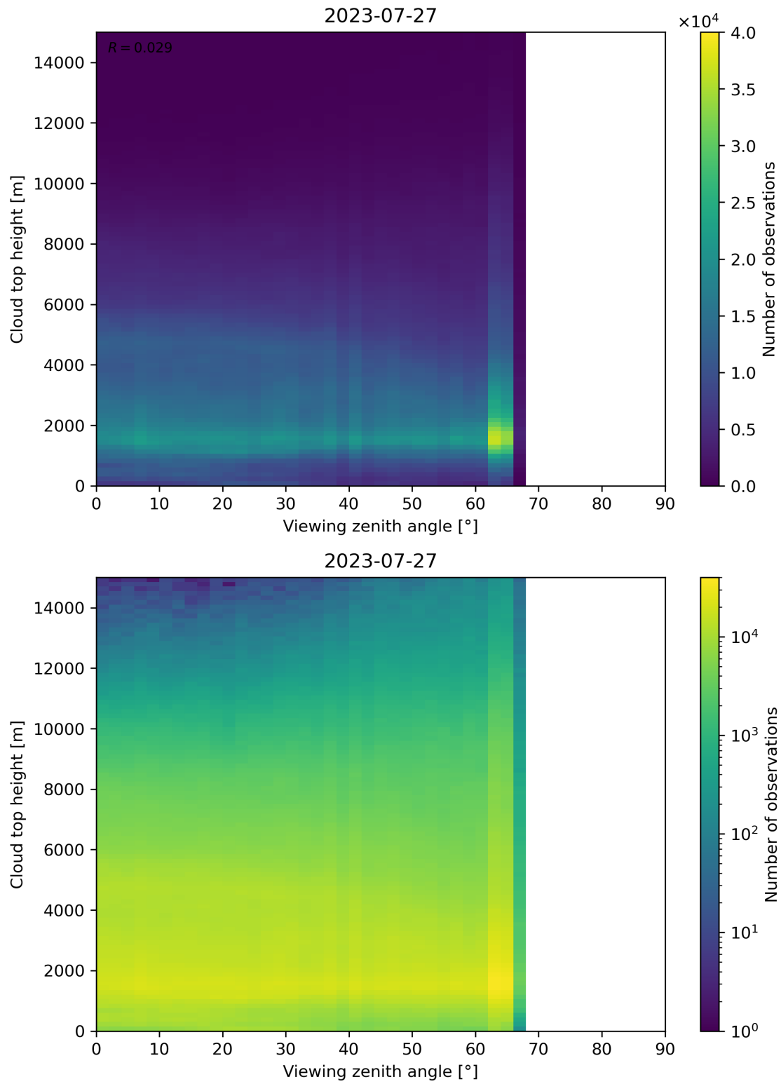
Figure 112: Scatter density plot of “Viewing zenith angle” against “Cloud top height” for 2023-07-26 to 2023-07-28.
