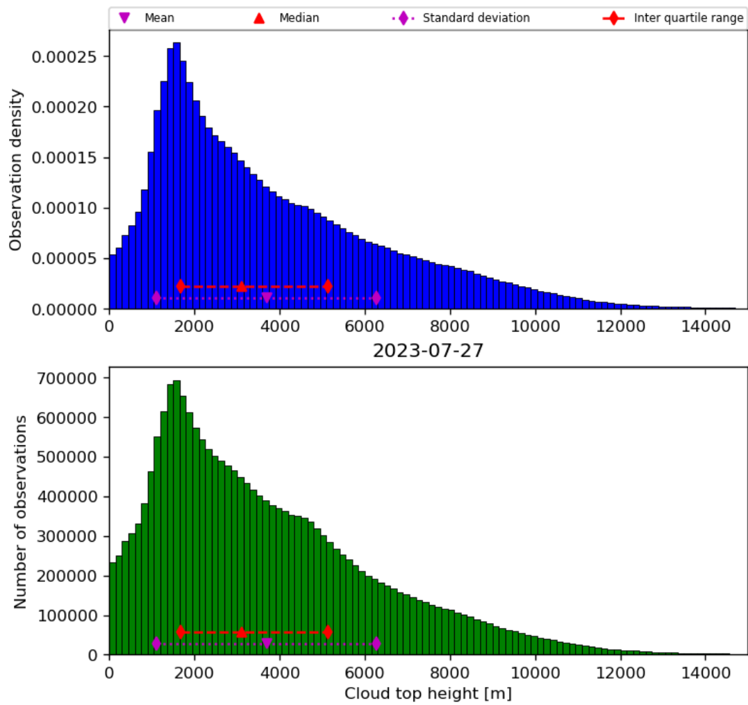
Figure 40: Histogram of “Cloud top height” for 2023-07-26 to 2023-07-28
