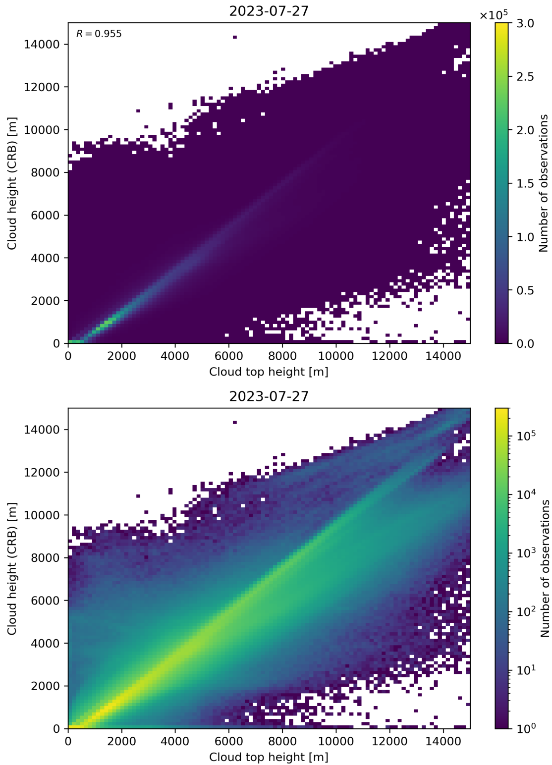
Figure 89: Scatter density plot of “Cloud top height” against “Cloud height (CRB)” for 2023-07-26 to 2023-07-28.
