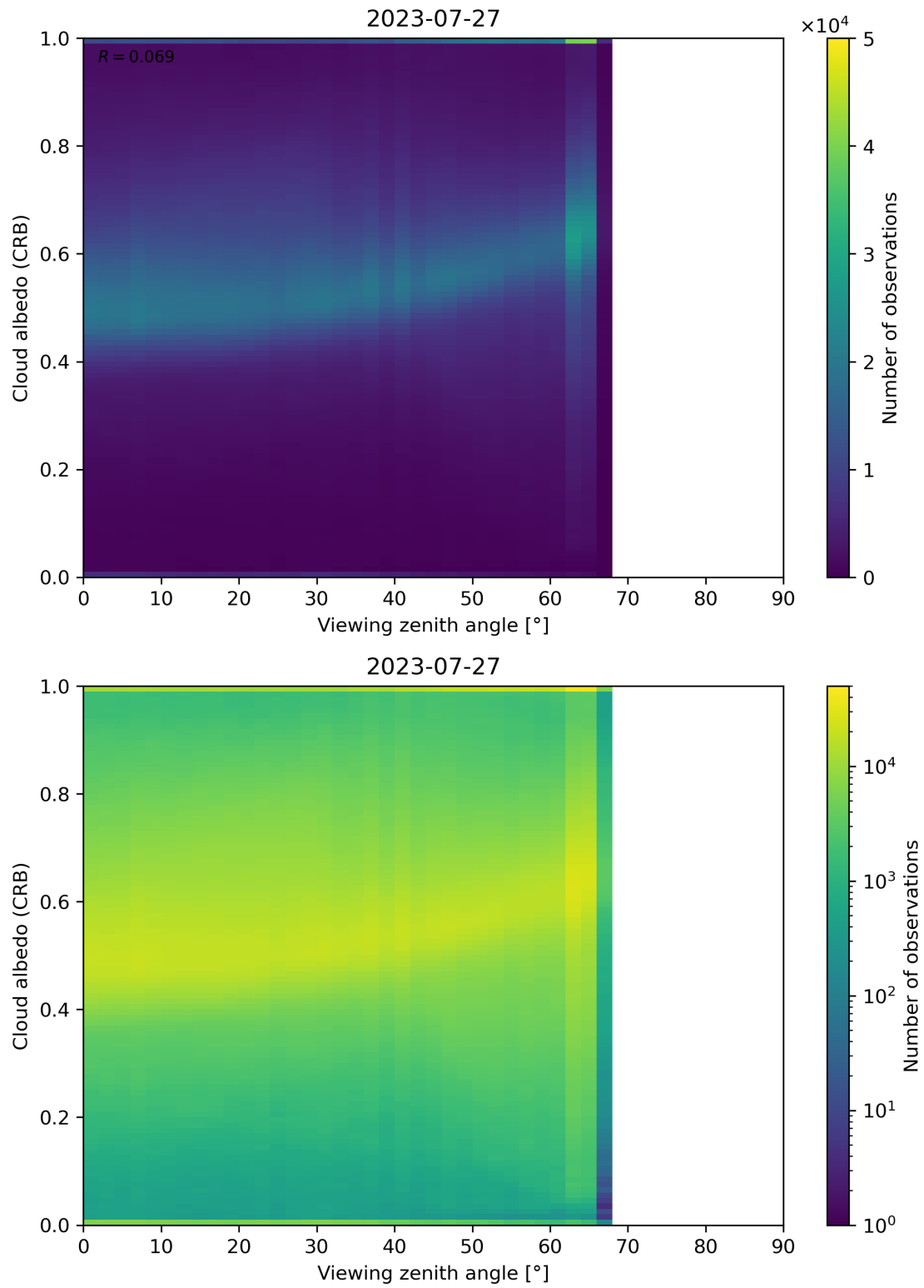
Figure 106: Scatter density plot of “Viewing zenith angle” against “Cloud albedo (CRB)” for 2023-07-26 to 2023-07-28.
