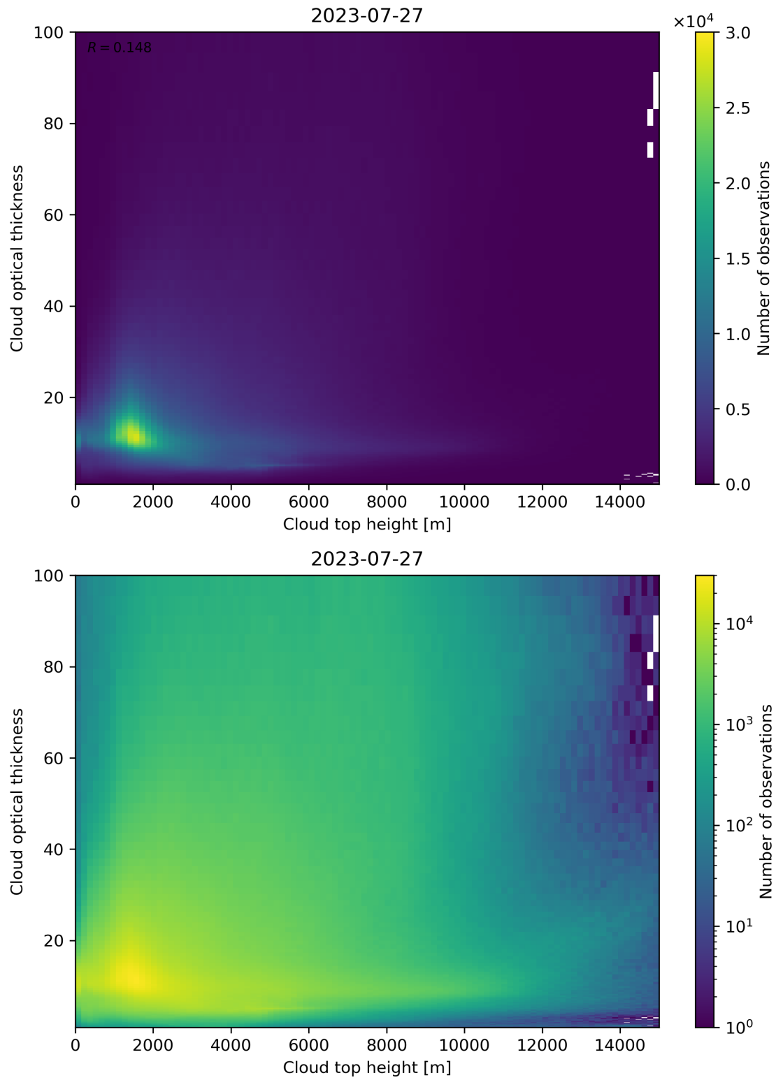
Figure 90: Scatter density plot of “Cloud top height” against “Cloud optical thickness” for 2023-07-26 to 2023-07-28.
