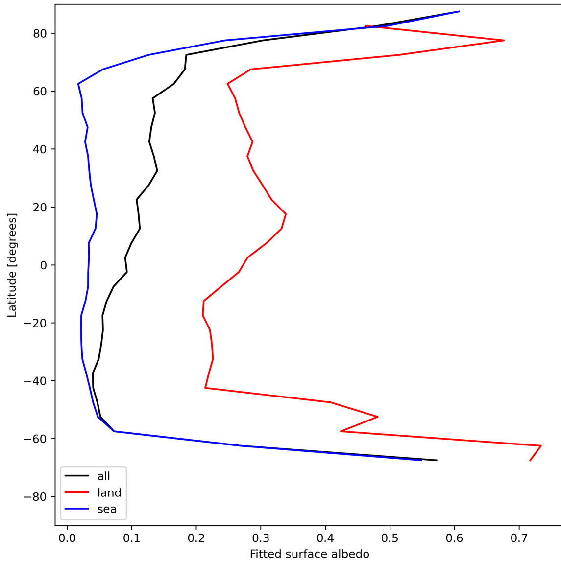
Figure 29: Zonal average of “Fitted surface albedo” for 2023-07-26 to 2023-07-28.
