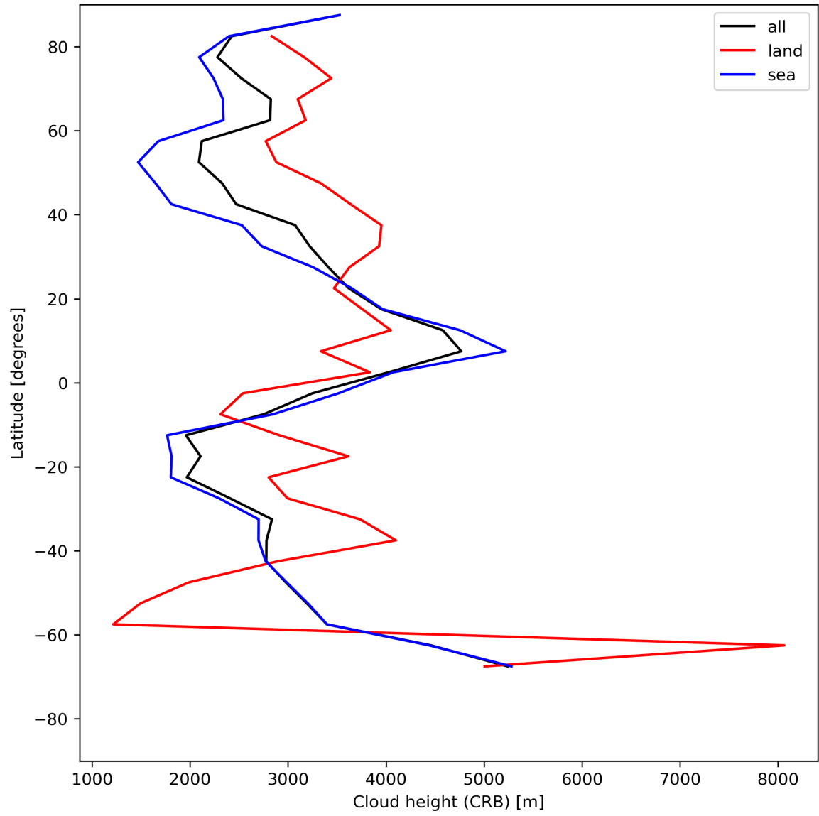
Figure 27: Zonal average of “Cloud height (CRB)” for 2023-07-26 to 2023-07-28.
