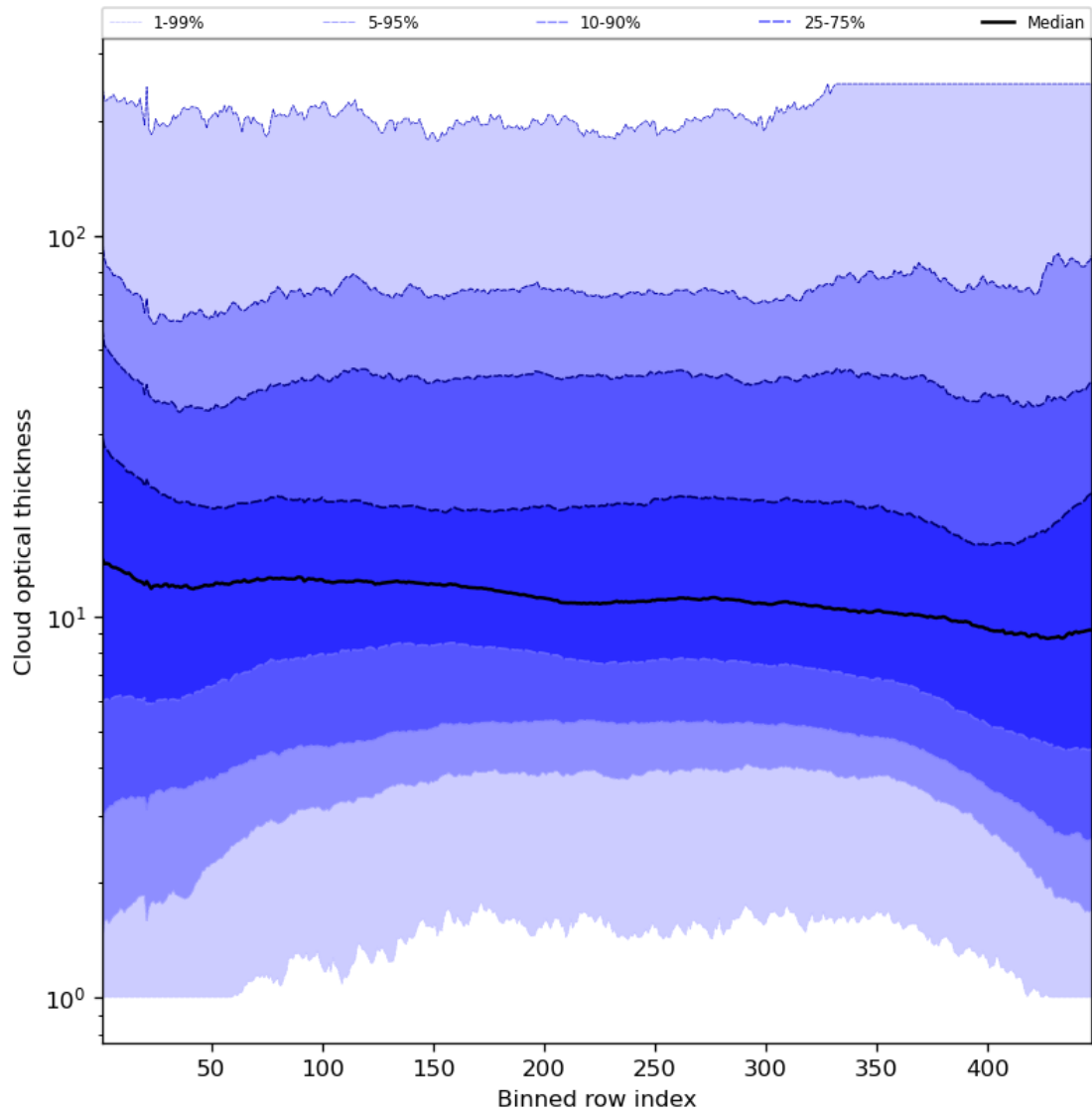
Figure 57: Along track statistics of “Cloud optical thickness” for 2023-07-26 to 2023-07-28
