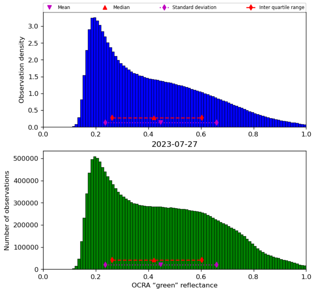
Figure 52: Histogram of “OCRA “green” reflectance” for 2023-07-26 to 2023-07-28
