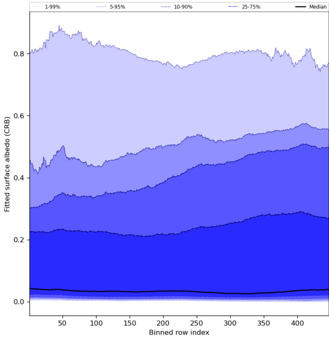
Figure 62: Along track statistics of “Fitted surface albedo (CRB)” for 2023-07-26 to 2023-07-28
