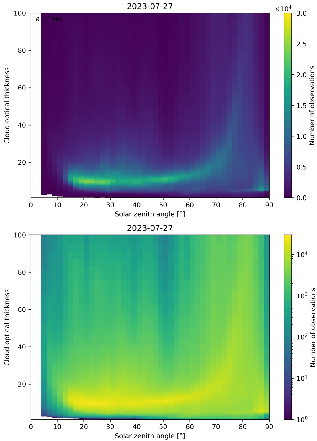
Figure 103: Scatter density plot of “Solar zenith angle” against “Cloud optical thickness” for 2023-07-26 to 2023-07-28.
