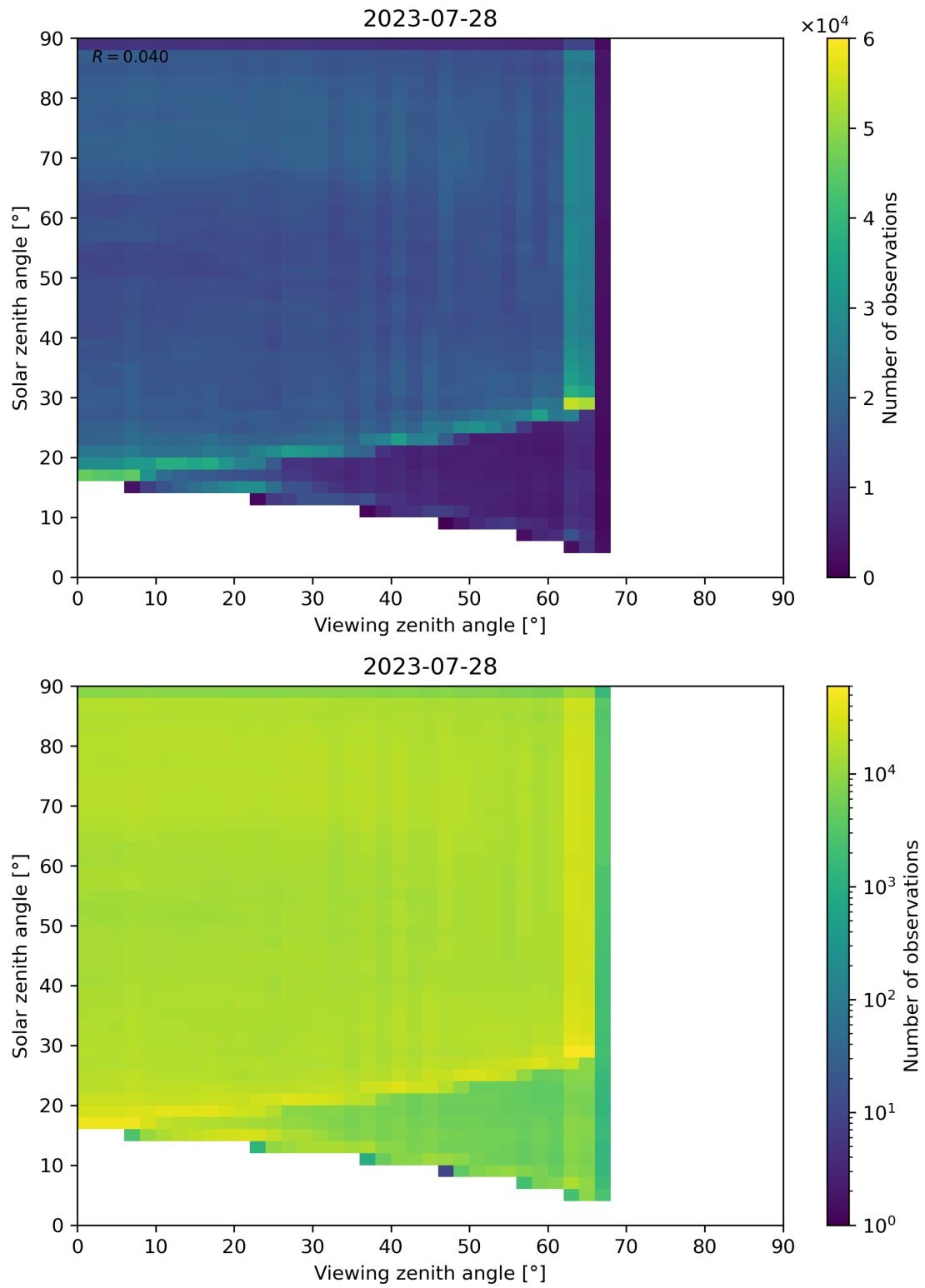
Figure 114: Scatter density plot of “Viewing zenith angle” against “Solar zenith angle” for 2023-07-27 to 2023-07-29.
