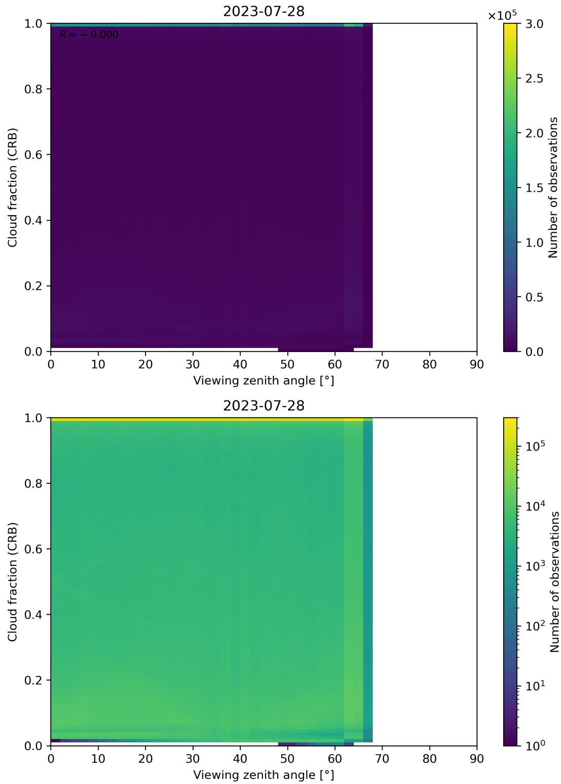
Figure 109: Scatter density plot of “Viewing zenith angle” against “Cloud fraction (CRB)” for 2023-07-27 to 2023-07-29.
