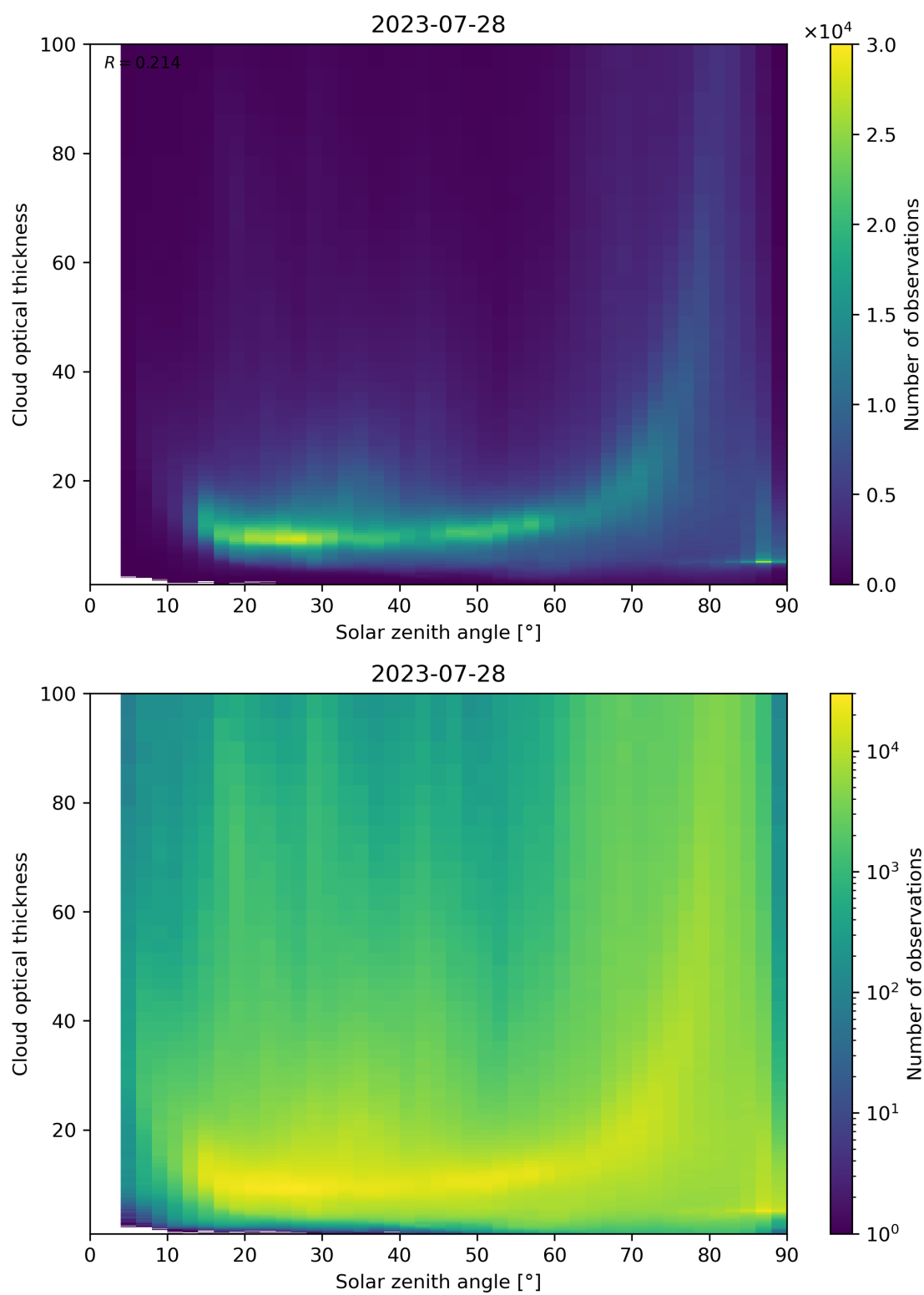
Figure 103: Scatter density plot of “Solar zenith angle” against “Cloud optical thickness” for 2023-07-27 to 2023-07-29.
