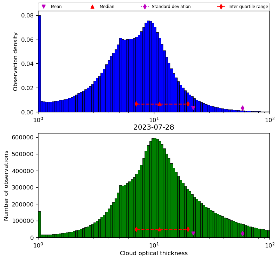
Figure 41: Histogram of “Cloud optical thickness” for 2023-07-27 to 2023-07-29
