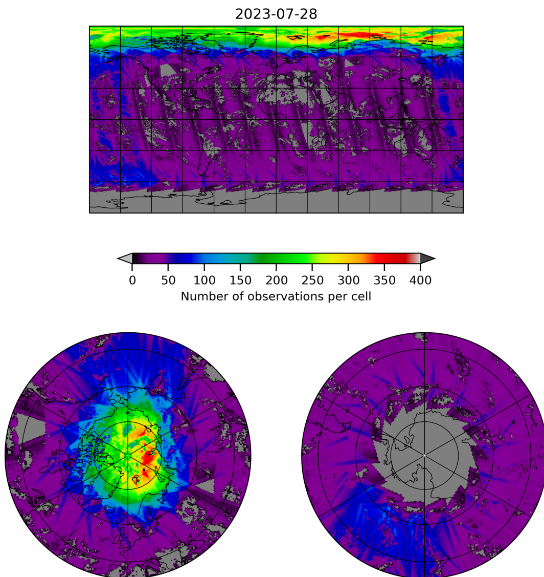
Figure 21: Map of the number of observations for 2023-07-27 to 2023-07-29
