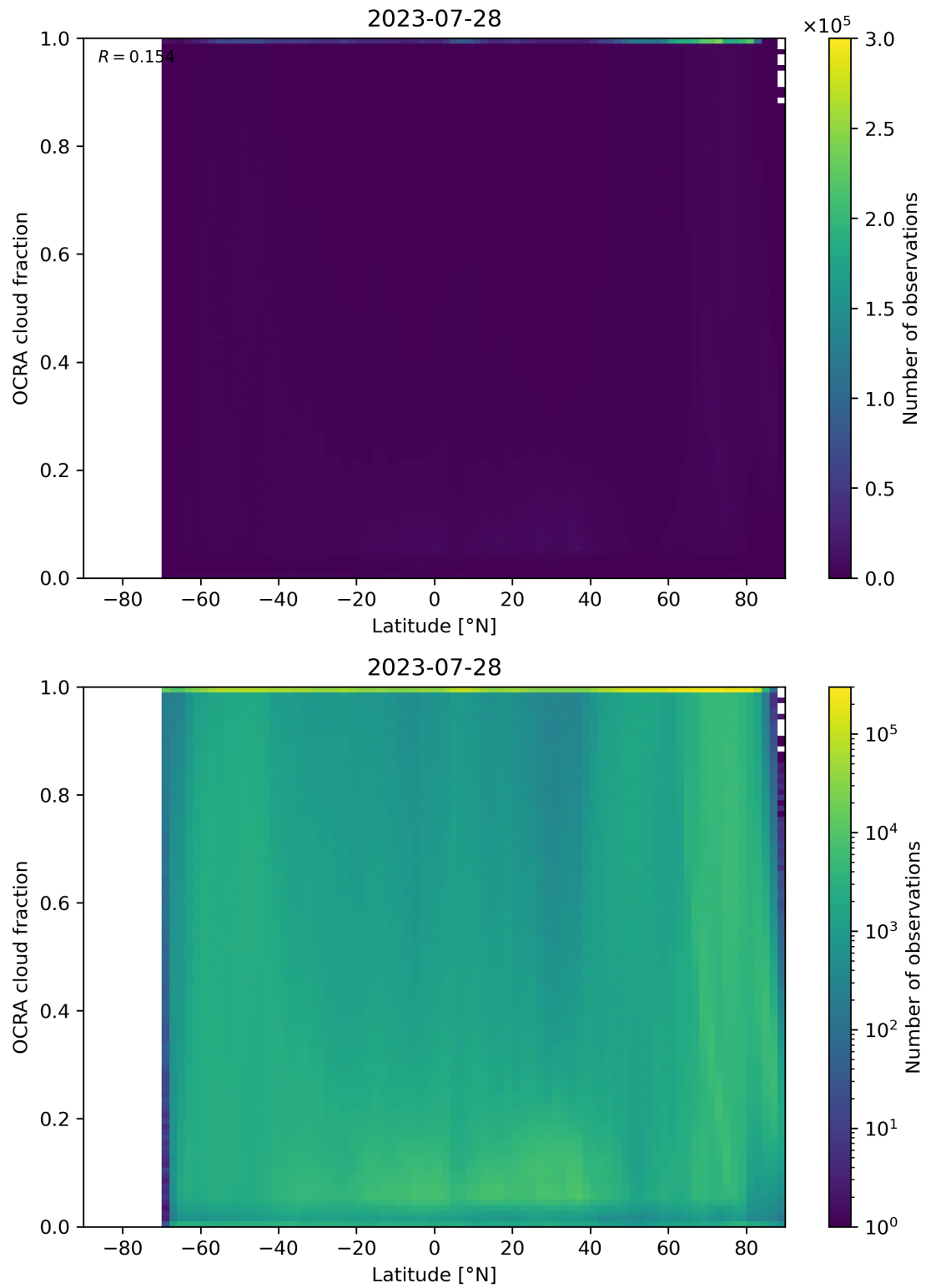
Figure 93: Scatter density plot of “Latitude” against “OCRA cloud fraction” for 2023-07-27 to 2023-07-29.
