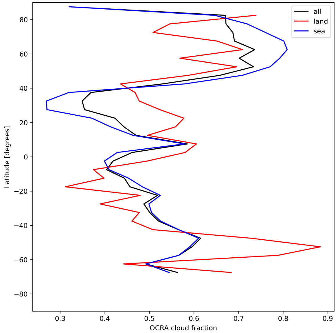
Figure 34: Zonal average of “OCRA cloud fraction” for 2023-07-27 to 2023-07-29.
