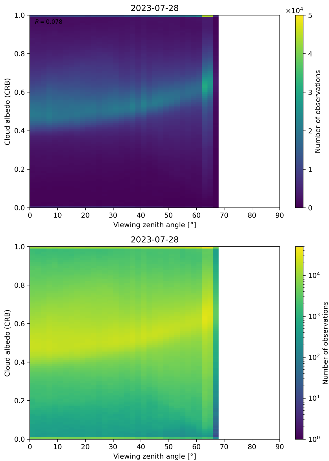
Figure 106: Scatter density plot of “Viewing zenith angle” against “Cloud albedo (CRB)” for 2023-07-27 to 2023-07-29.
