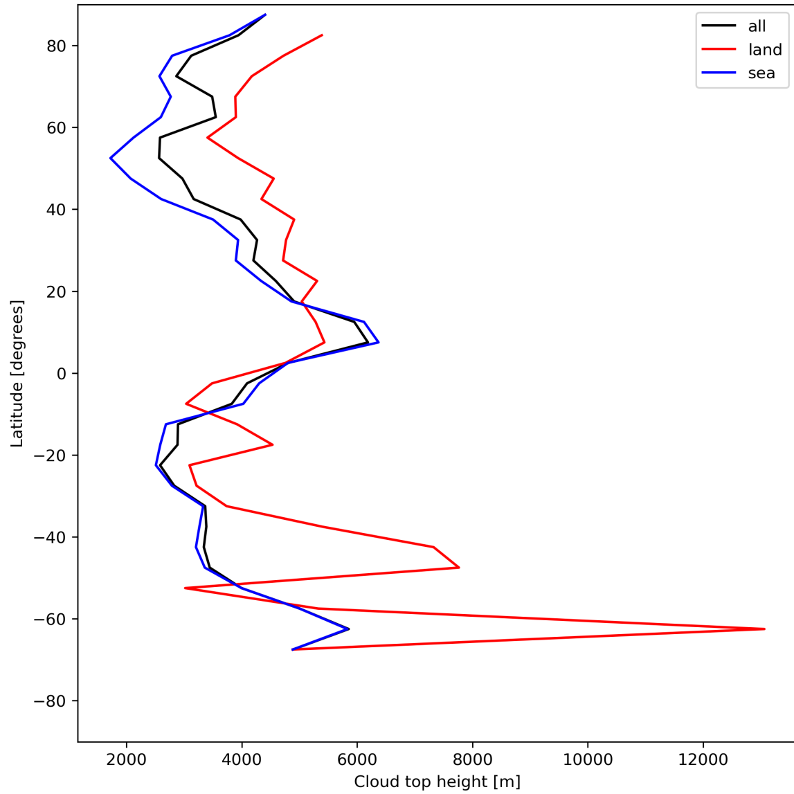
Figure 24: Zonal average of “Cloud top height” for 2023-07-27 to 2023-07-29.
