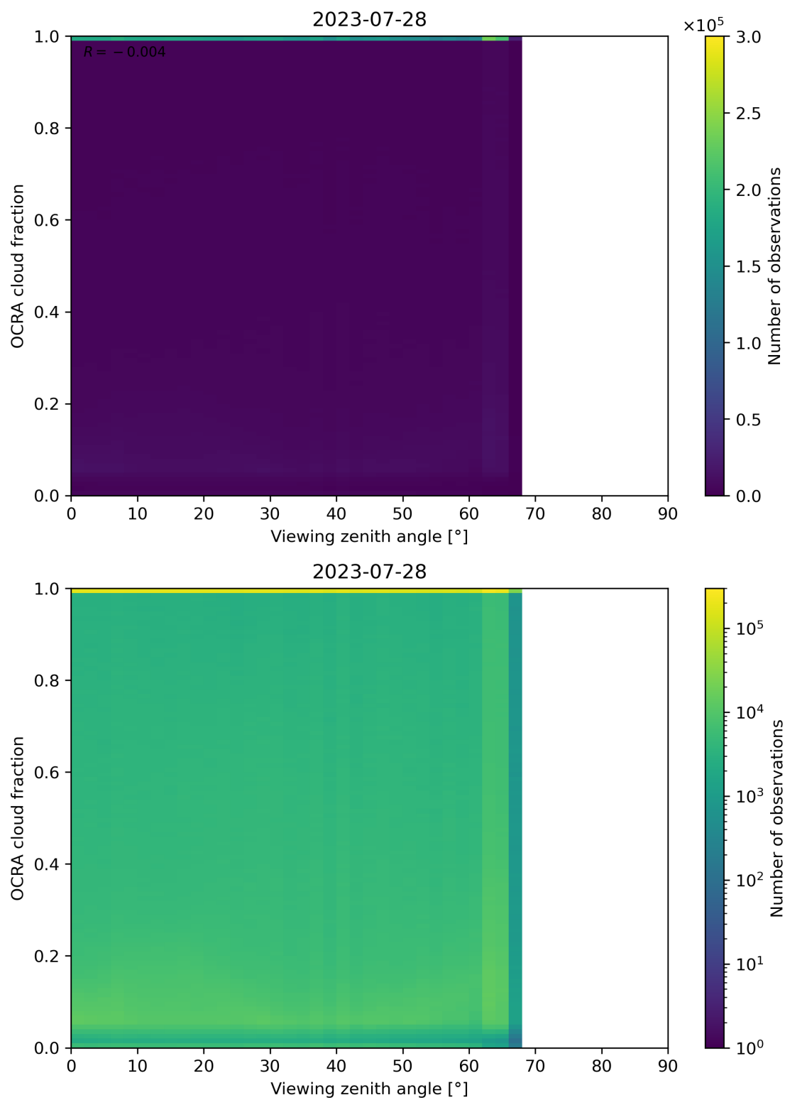
Figure 108: Scatter density plot of “Viewing zenith angle” against “OCRA cloud fraction” for 2023-07-27 to 2023-07-29.
