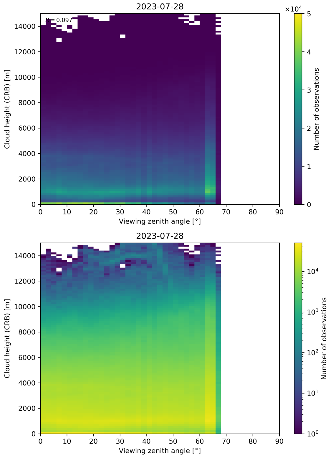
Figure 110: Scatter density plot of “Viewing zenith angle” against “Cloud height (CRB)” for 2023-07-27 to 2023-07-29.
