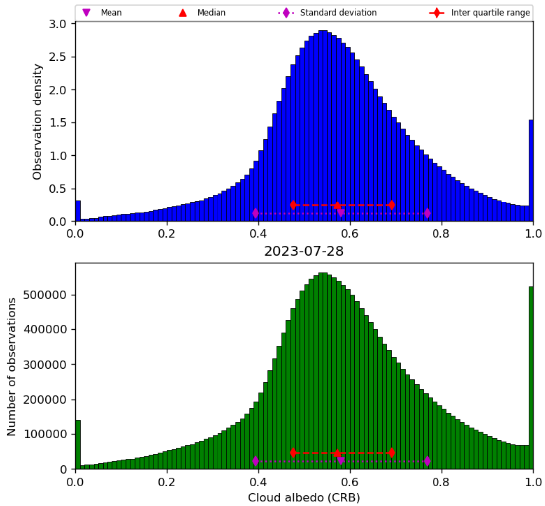
Figure 44: Histogram of “Cloud albedo (CRB)” for 2023-07-27 to 2023-07-29
