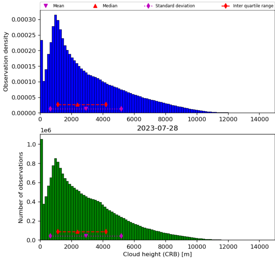
Figure 43: Histogram of “Cloud height (CRB)” for 2023-07-27 to 2023-07-29
