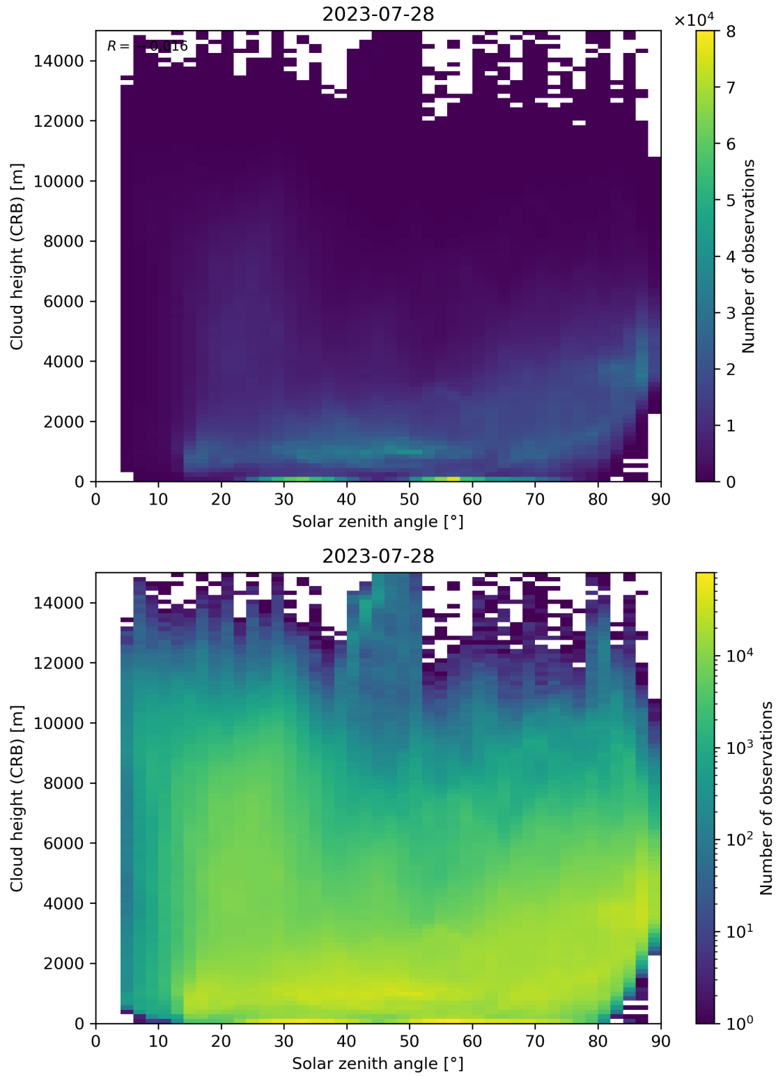
Figure 102: Scatter density plot of “Solar zenith angle” against “Cloud height (CRB)” for 2023-07-27 to 2023-07-29.
