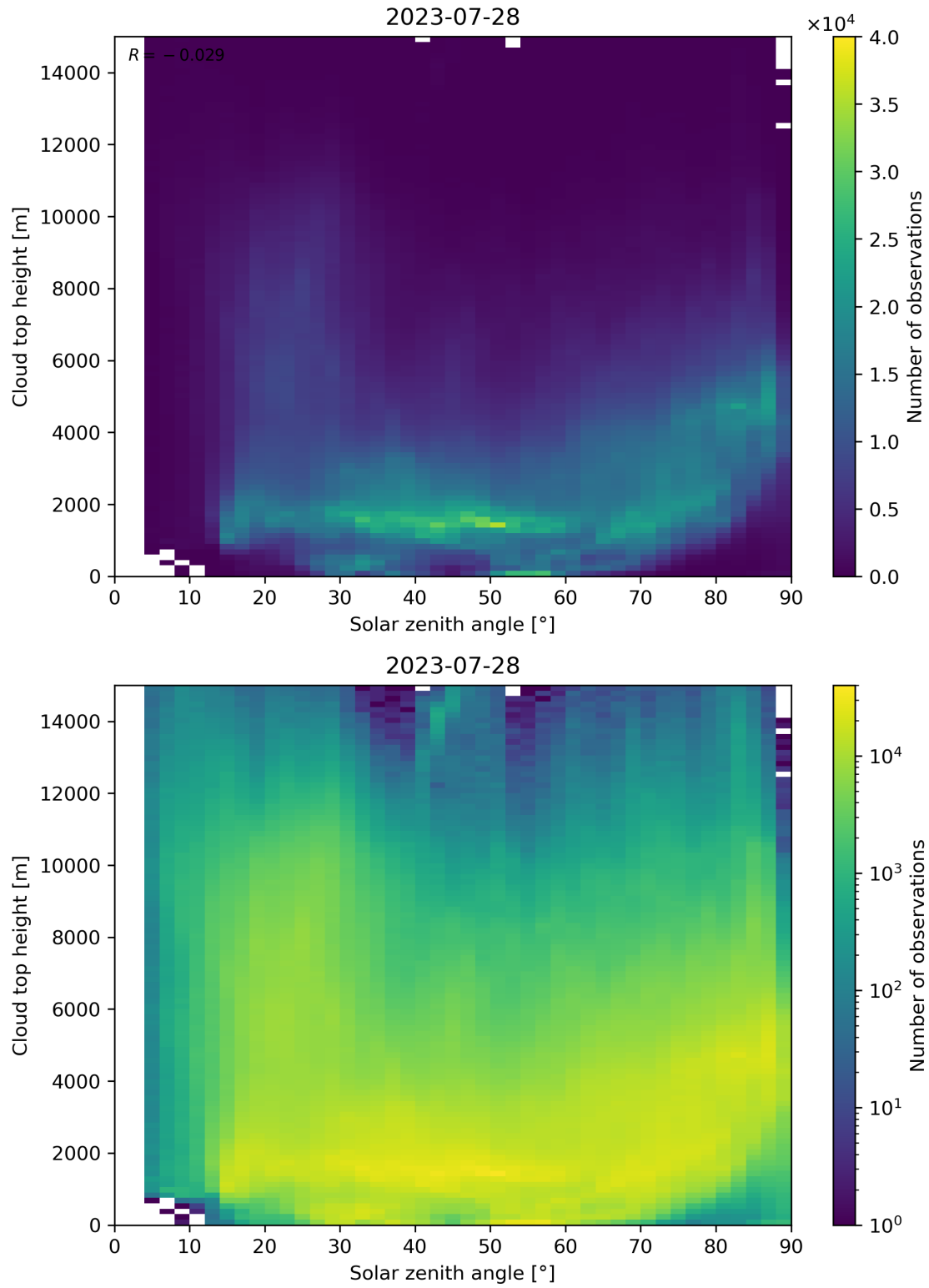
Figure 104: Scatter density plot of “Solar zenith angle” against “Cloud top height” for 2023-07-27 to 2023-07-29.
