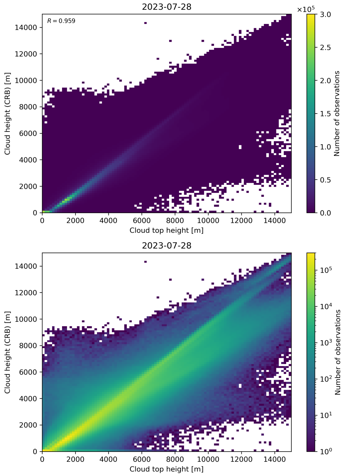
Figure 89: Scatter density plot of “Cloud top height” against “Cloud height (CRB)” for 2023-07-27 to 2023-07-29.
