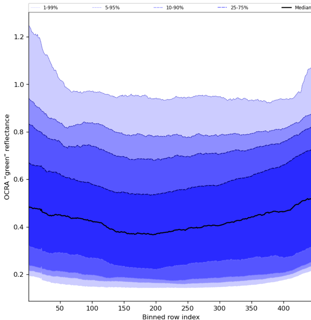
Figure 68: Along track statistics of “OCRA “green” reflectance” for 2023-07-27 to 2023-07-29
