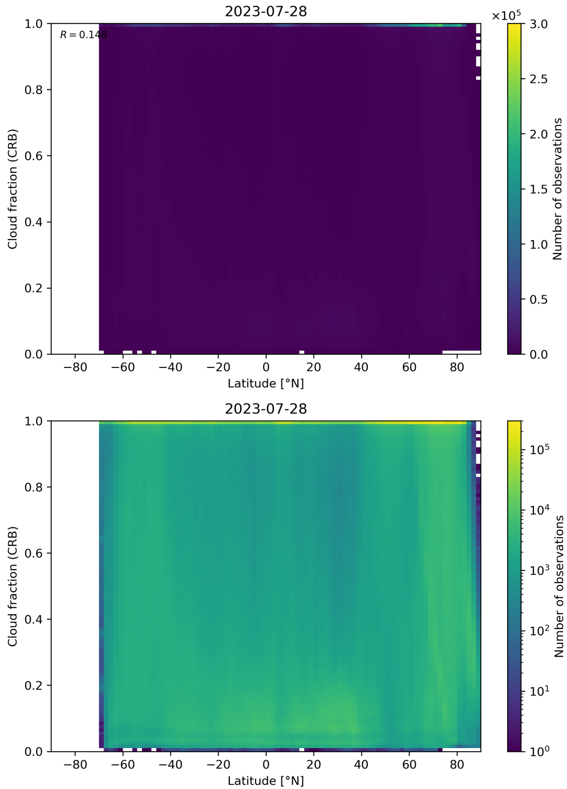
Figure 94: Scatter density plot of “Latitude” against “Cloud fraction (CRB)” for 2023-07-27 to 2023-07-29.
