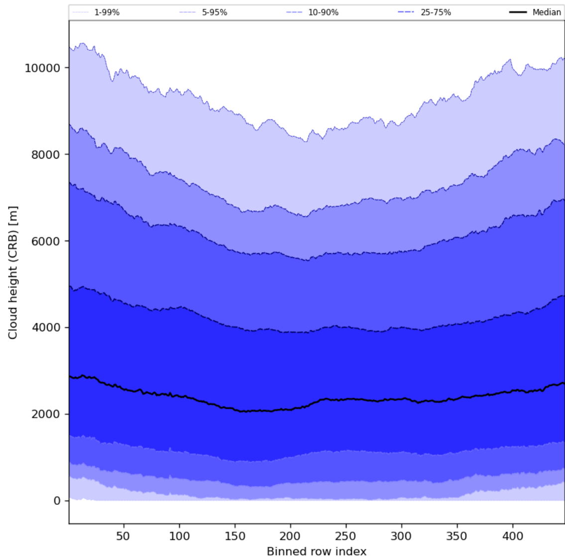
Figure 59: Along track statistics of “Cloud height (CRB)” for 2023-07-27 to 2023-07-29
