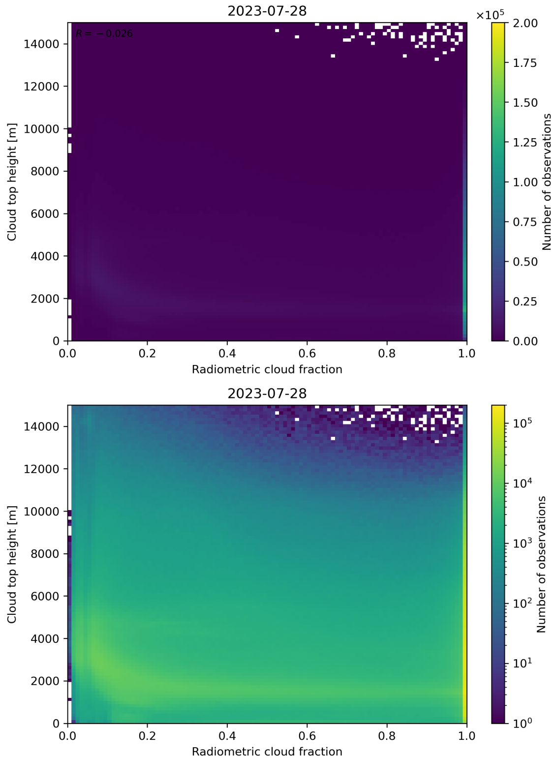
Figure 76: Scatter density plot of “Radiometric cloud fraction” against “Cloud top height” for 2023-07-27 to 2023-07-29.
