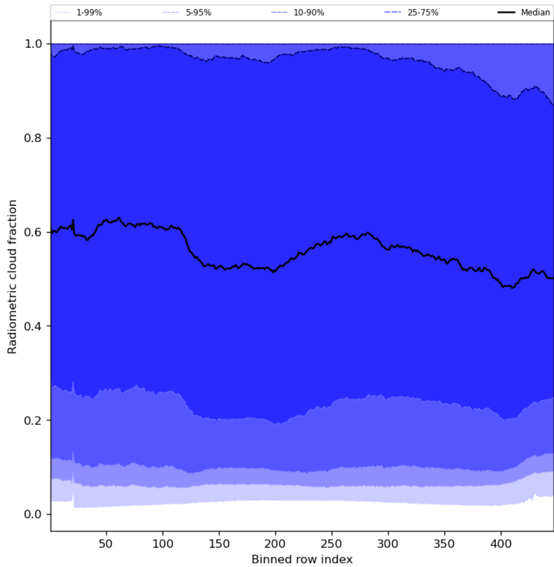
Figure 55: Along track statistics of “Radiometric cloud fraction” for 2023-07-27 to 2023-07-29
