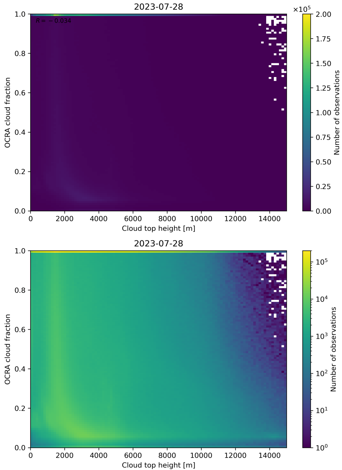
Figure 87: Scatter density plot of “Cloud top height” against “OCRA cloud fraction” for 2023-07-27 to 2023-07-29.
