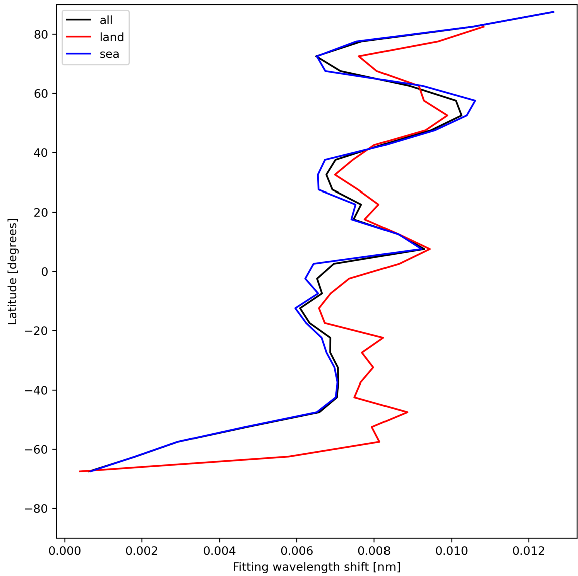
Figure 33: Zonal average of “Fitting wavelength shift” for 2023-07-27 to 2023-07-29.
