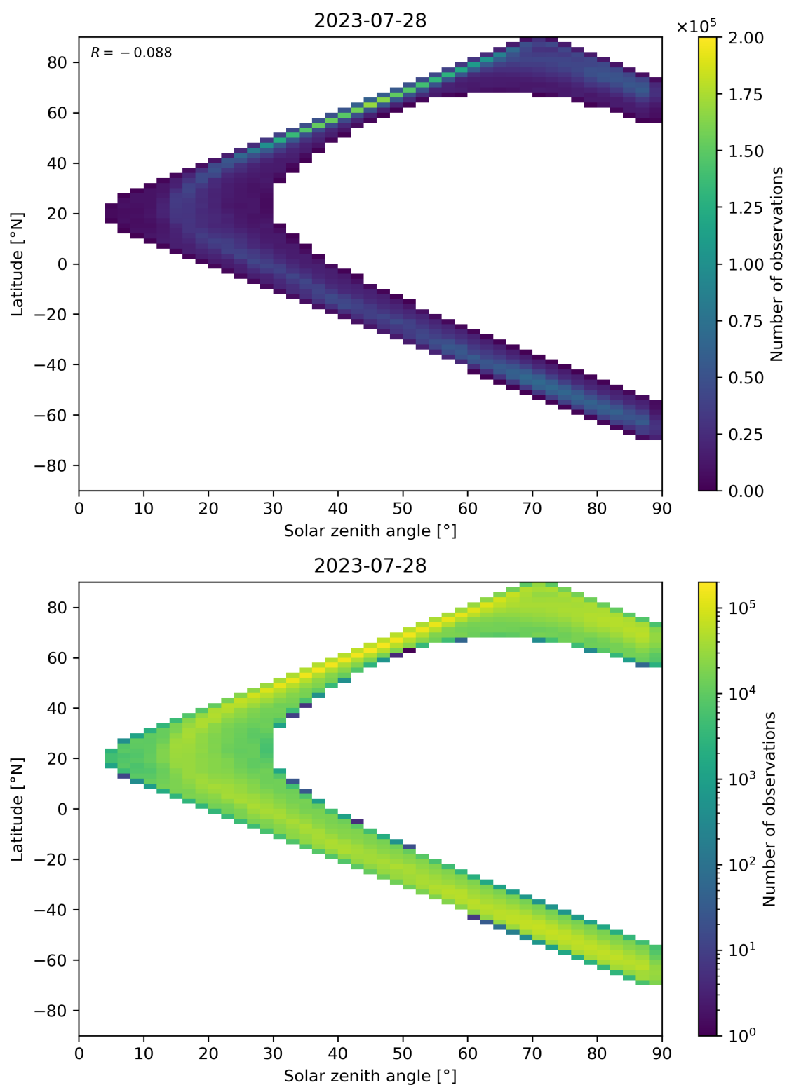
Figure 105: Scatter density plot of “Solar zenith angle” against “Latitude” for 2023-07-27 to 2023-07-29.
