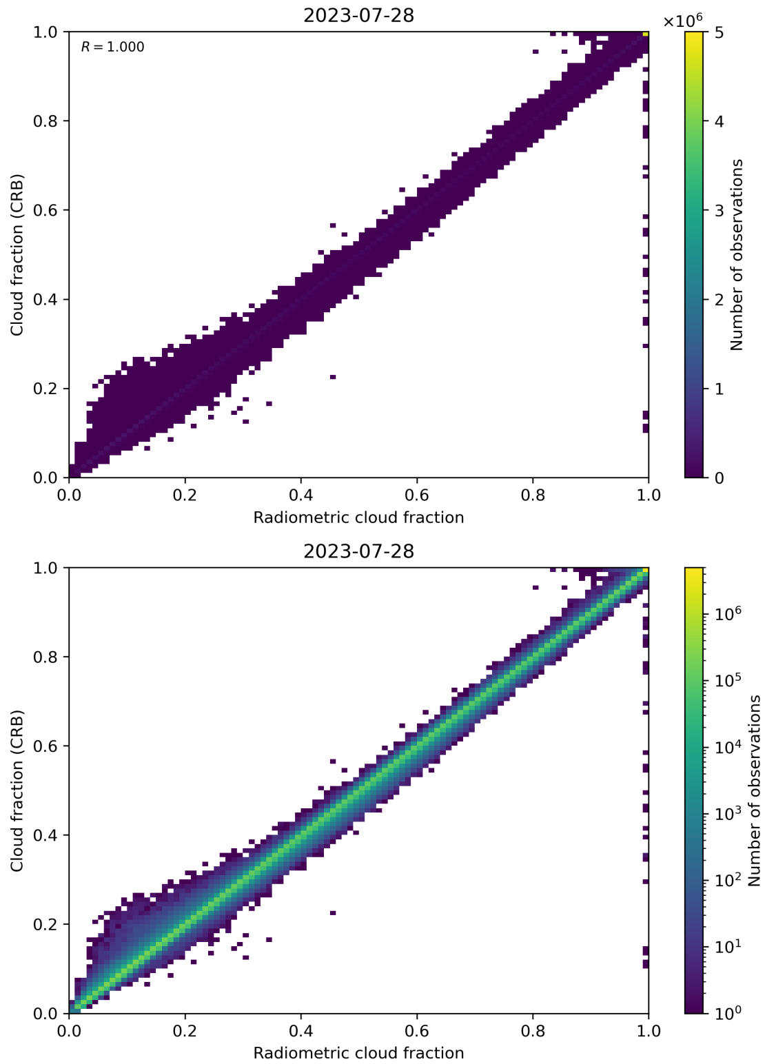
Figure 73: Scatter density plot of “Radiometric cloud fraction” against “Cloud fraction (CRB)” for 2023-07-27 to 2023-07-29.
