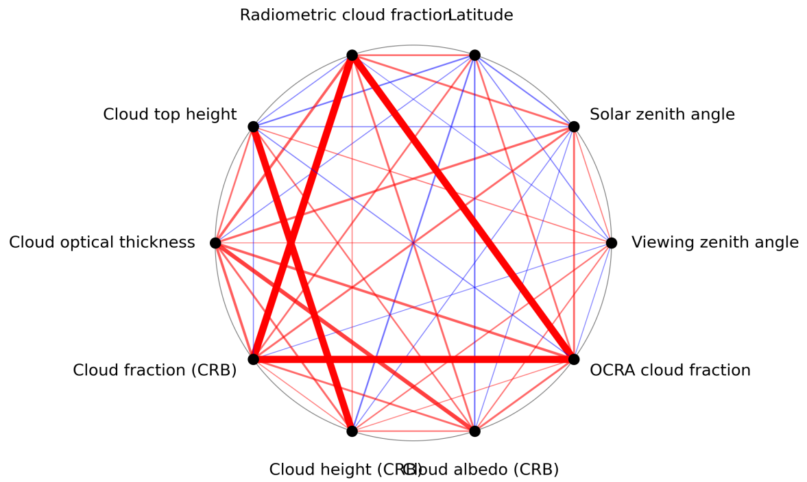
Figure 1: Map of correlation graph for 2023-07-27 to 2023-07-29.
