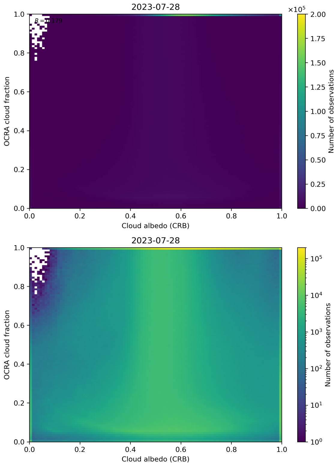
Figure 70: Scatter density plot of “Cloud albedo (CRB)” against “OCRA cloud fraction” for 2023-07-27 to 2023-07-29.
