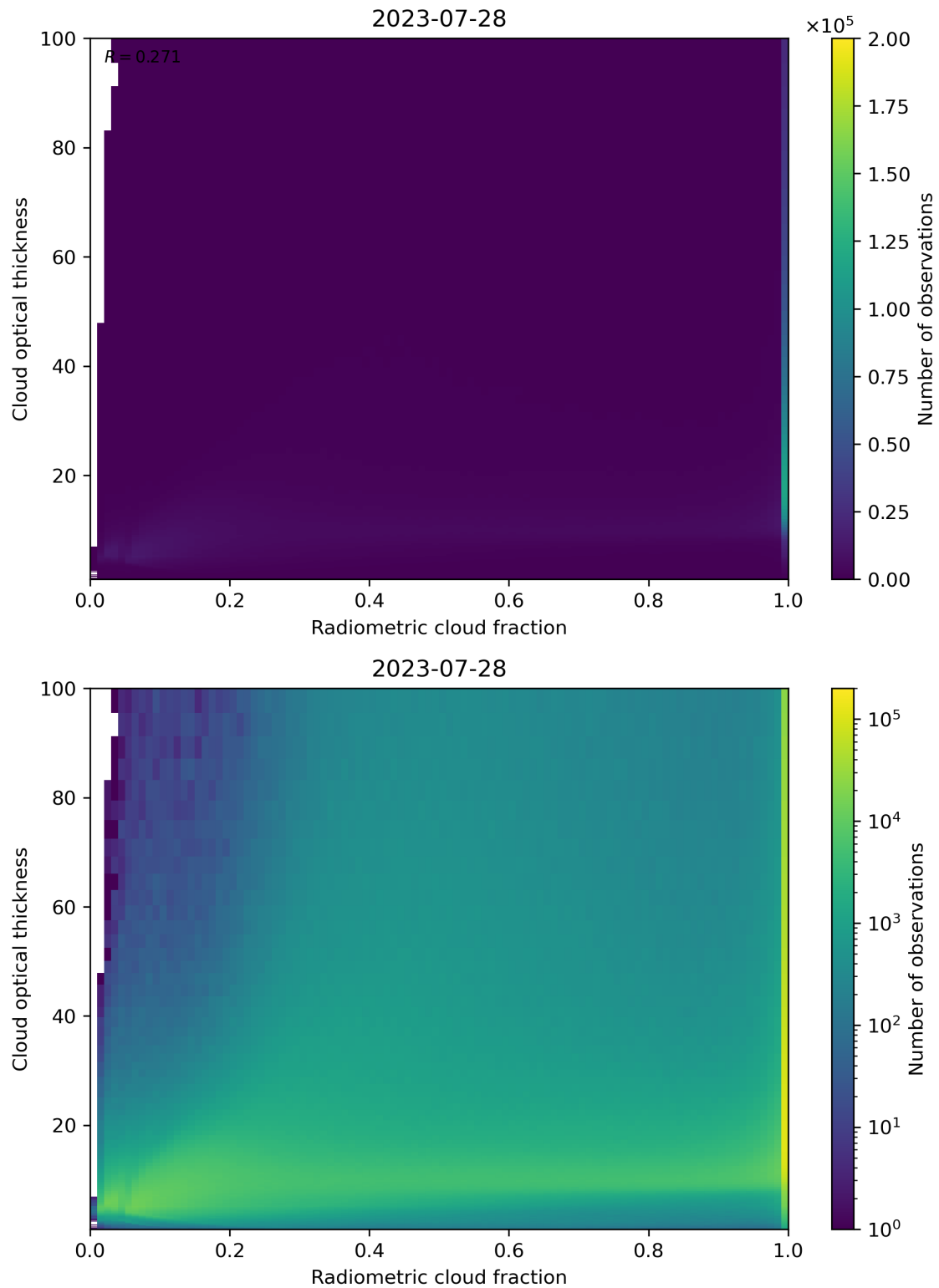
Figure 75: Scatter density plot of “Radiometric cloud fraction” against “Cloud optical thickness” for 2023-07-27 to 2023-07-29.
