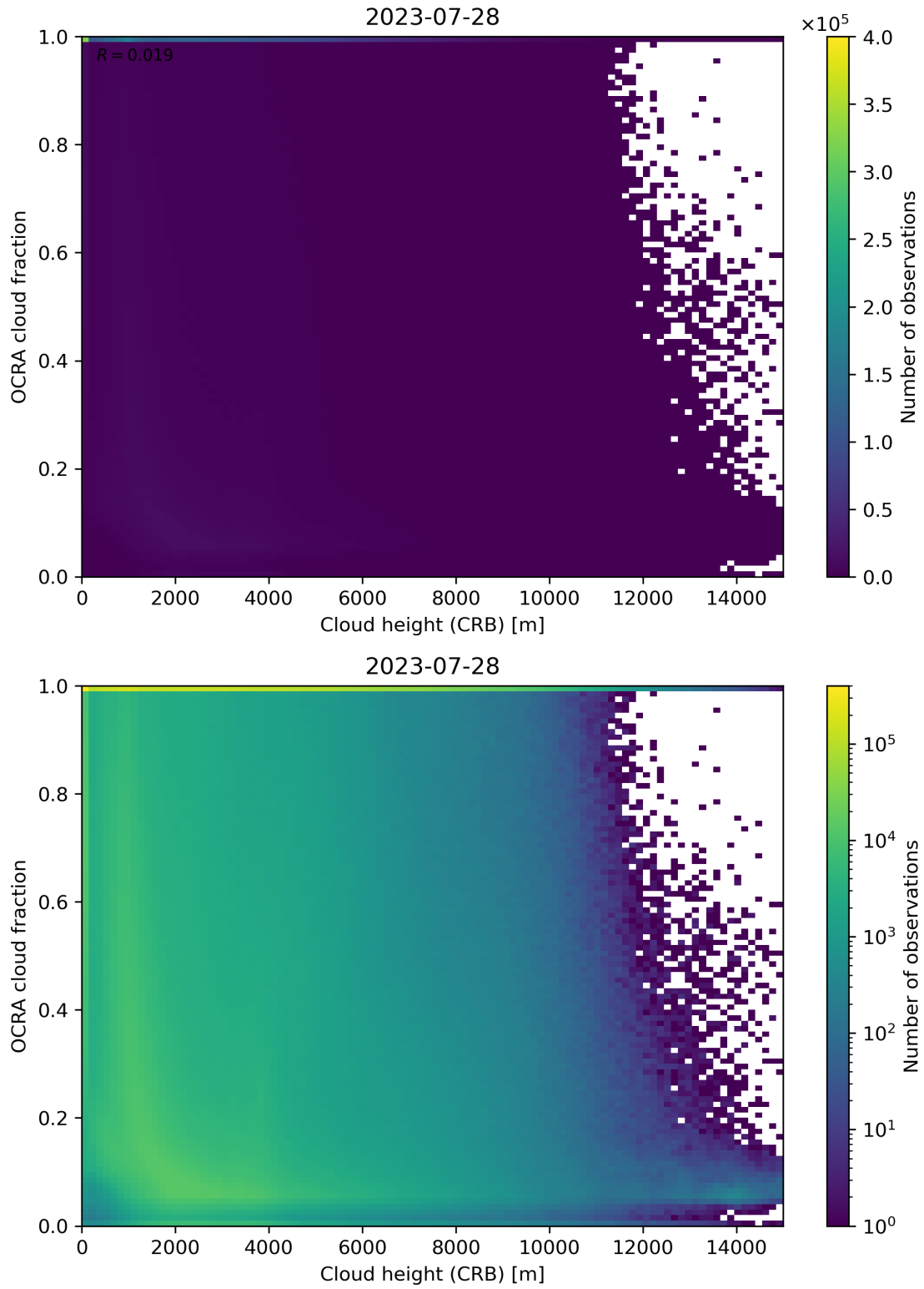
Figure 81: Scatter density plot of “Cloud height (CRB)” against “OCRA cloud fraction” for 2023-07-27 to 2023-07-29.
