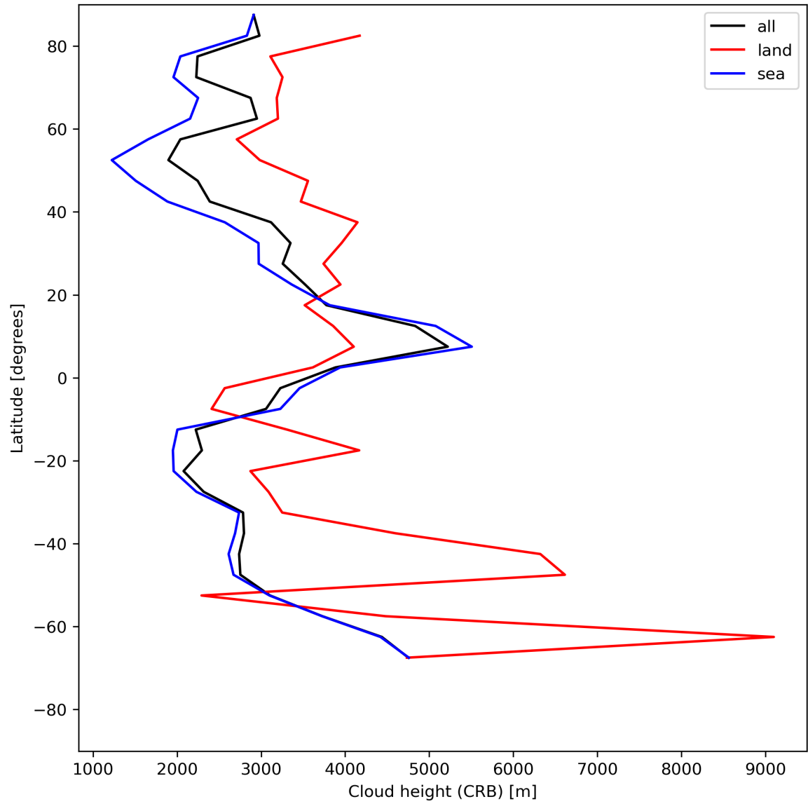
Figure 27: Zonal average of “Cloud height (CRB)” for 2023-07-27 to 2023-07-29.
