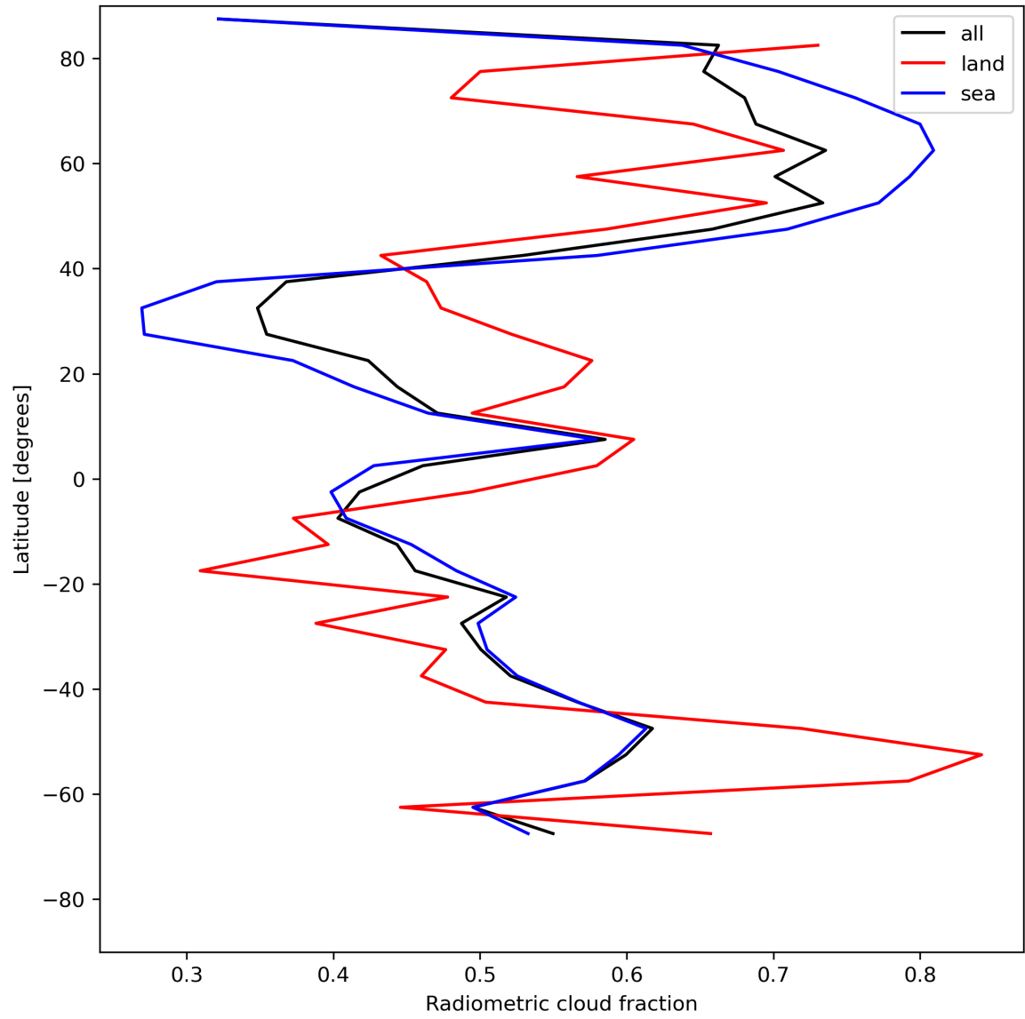
Figure 23: Zonal average of “Radiometric cloud fraction” for 2023-07-27 to 2023-07-29.
