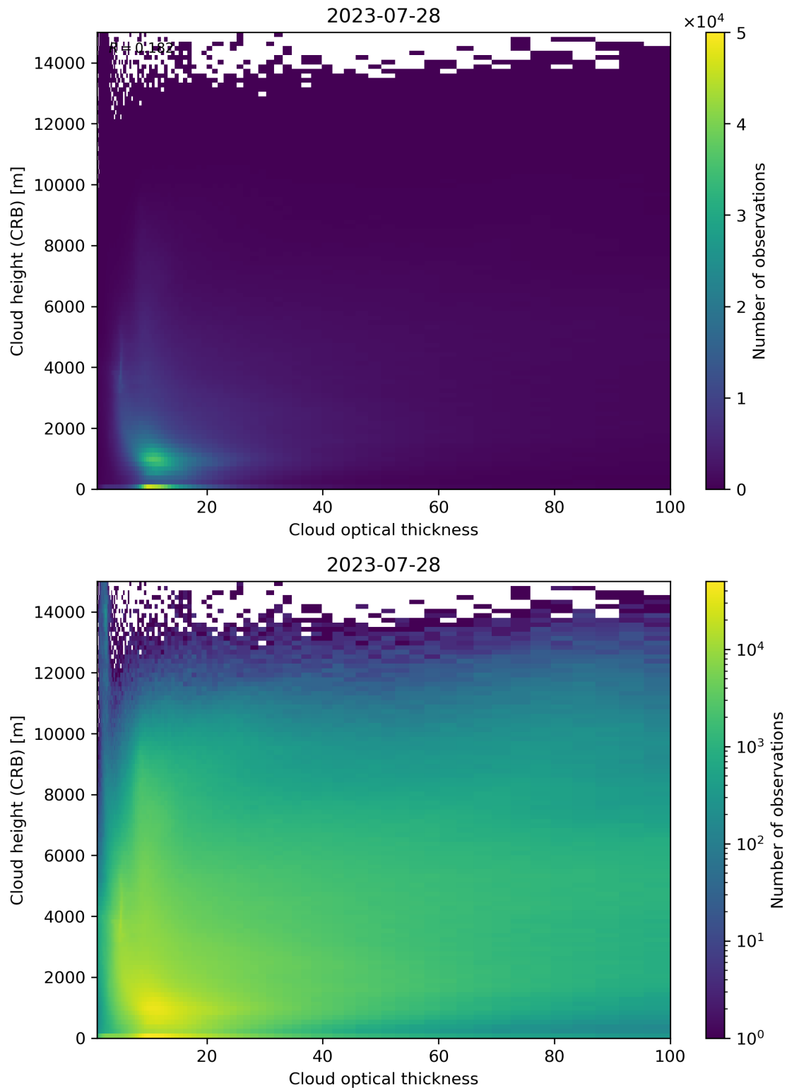
Figure 85: Scatter density plot of “Cloud optical thickness” against “Cloud height (CRB)” for 2023-07-27 to 2023-07-29.
