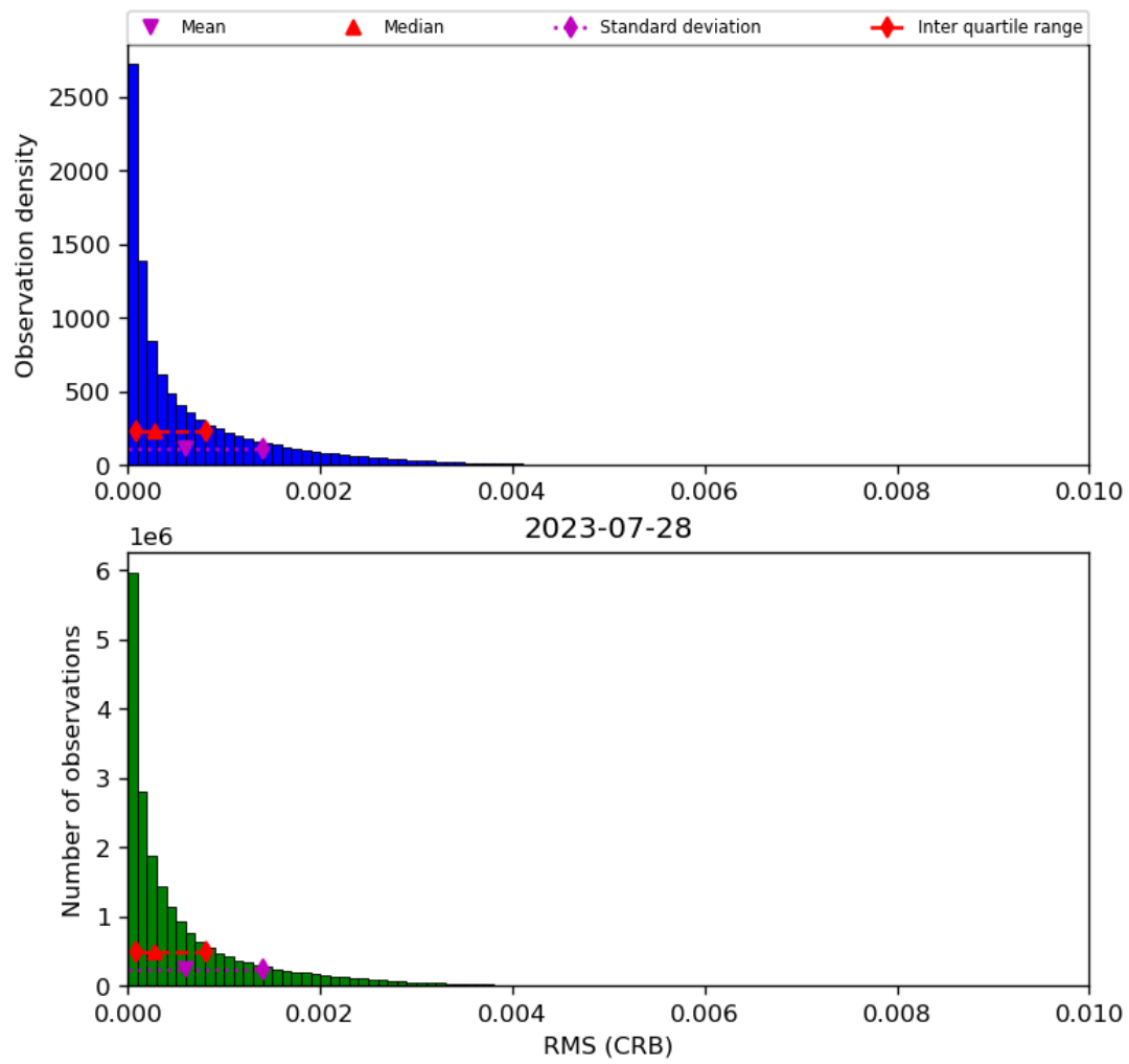
Figure 48: Histogram of “RMS (CRB)” for 2023-07-27 to 2023-07-29
