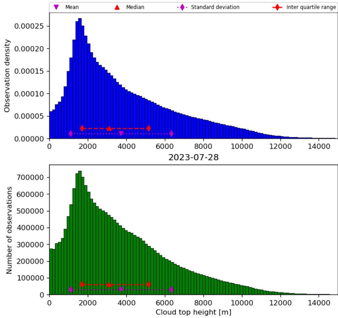
Figure 40: Histogram of “Cloud top height” for 2023-07-27 to 2023-07-29
