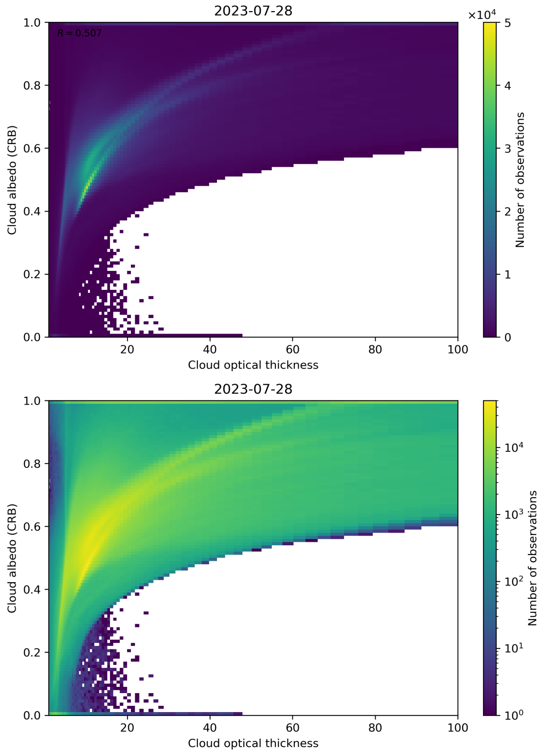
Figure 82: Scatter density plot of “Cloud optical thickness” against “Cloud albedo (CRB)” for 2023-07-27 to 2023-07-29.
