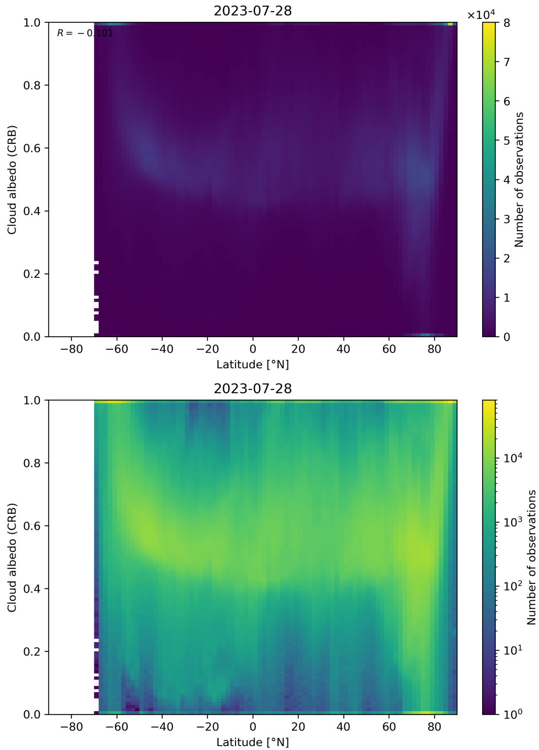
Figure 91: Scatter density plot of “Latitude” against “Cloud albedo (CRB)” for 2023-07-27 to 2023-07-29.
