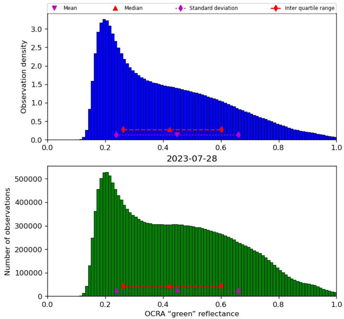
Figure 52: Histogram of “OCRA “green” reflectance” for 2023-07-27 to 2023-07-29
