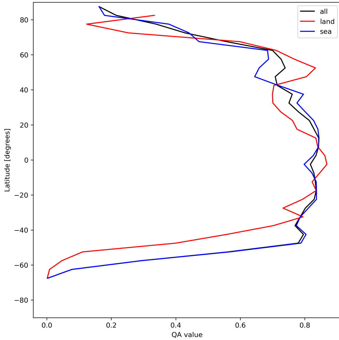
Figure 22: Zonal average of “QA value” for 2023-07-27 to 2023-07-29.
