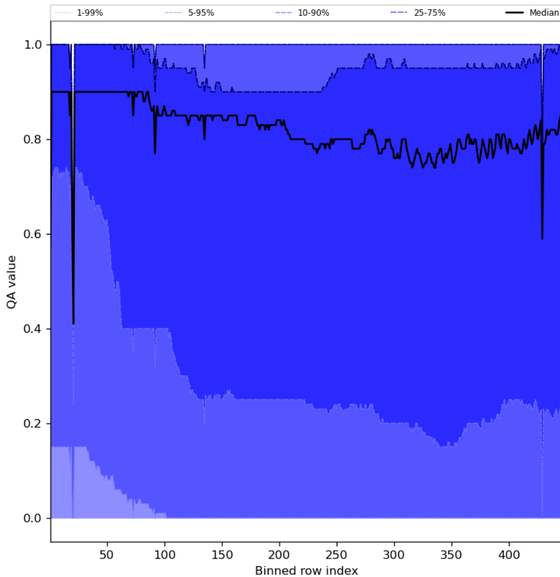
Figure 54: Along track statistics of “QA value” for 2023-07-27 to 2023-07-29
