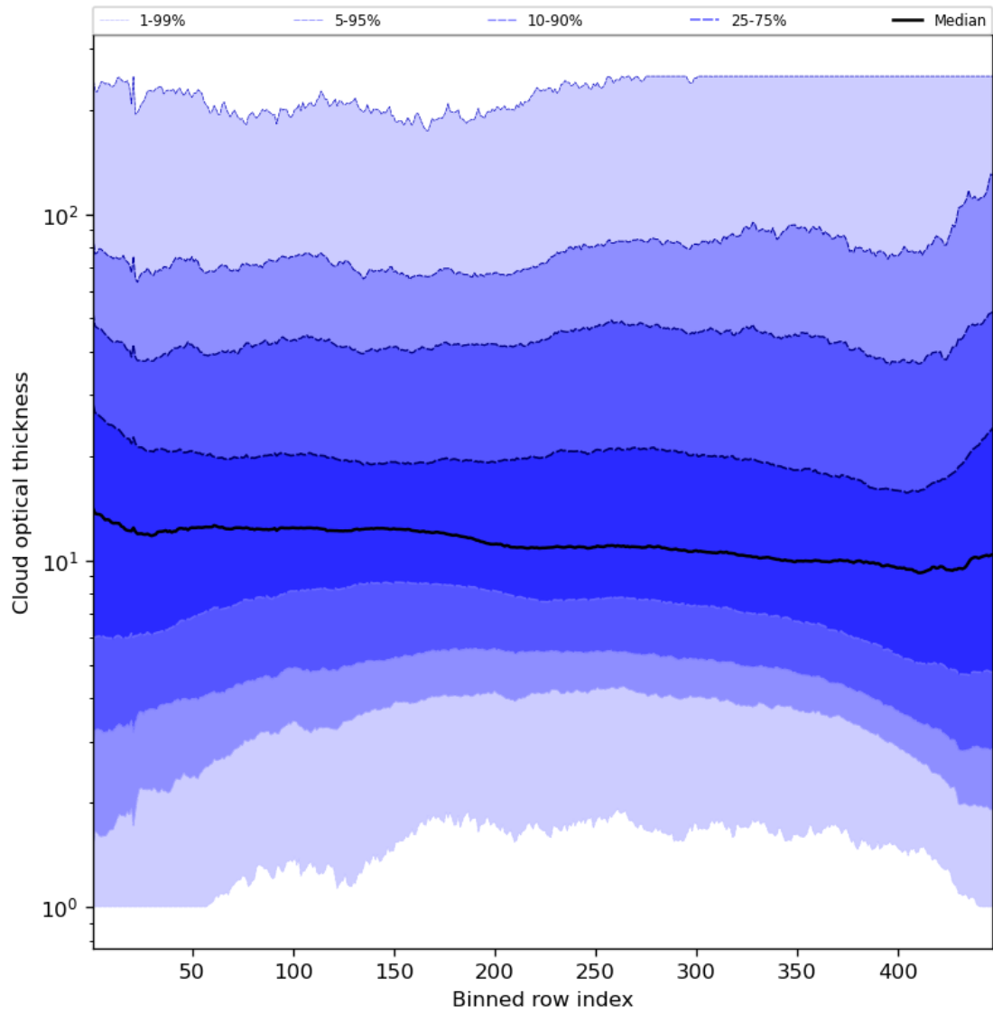
Figure 57: Along track statistics of “Cloud optical thickness” for 2023-07-27 to 2023-07-29
