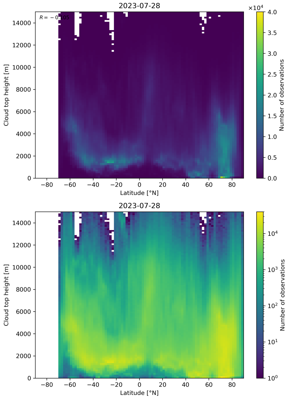
Figure 97: Scatter density plot of “Latitude” against “Cloud top height” for 2023-07-27 to 2023-07-29.
