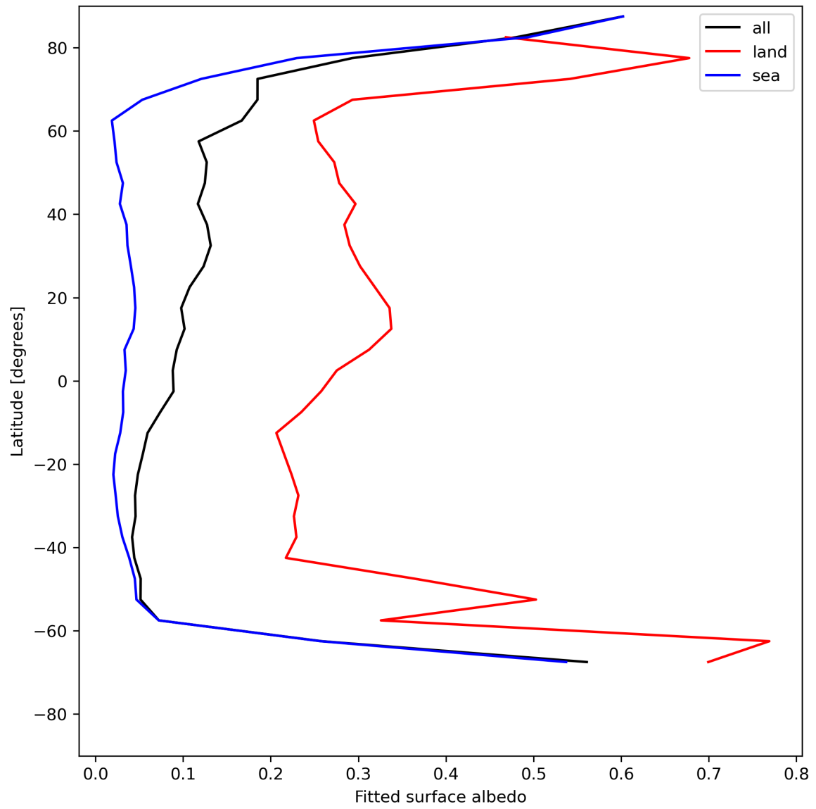
Figure 29: Zonal average of “Fitted surface albedo” for 2023-07-27 to 2023-07-29.
