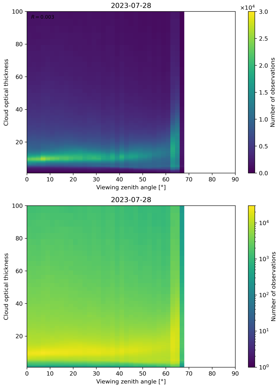
Figure 111: Scatter density plot of “Viewing zenith angle” against “Cloud optical thickness” for 2023-07-27 to 2023-07-29.
