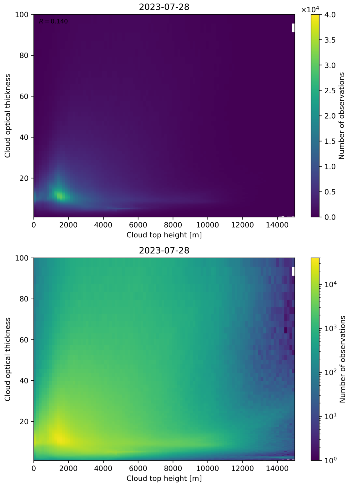
Figure 90: Scatter density plot of “Cloud top height” against “Cloud optical thickness” for 2023-07-27 to 2023-07-29.
