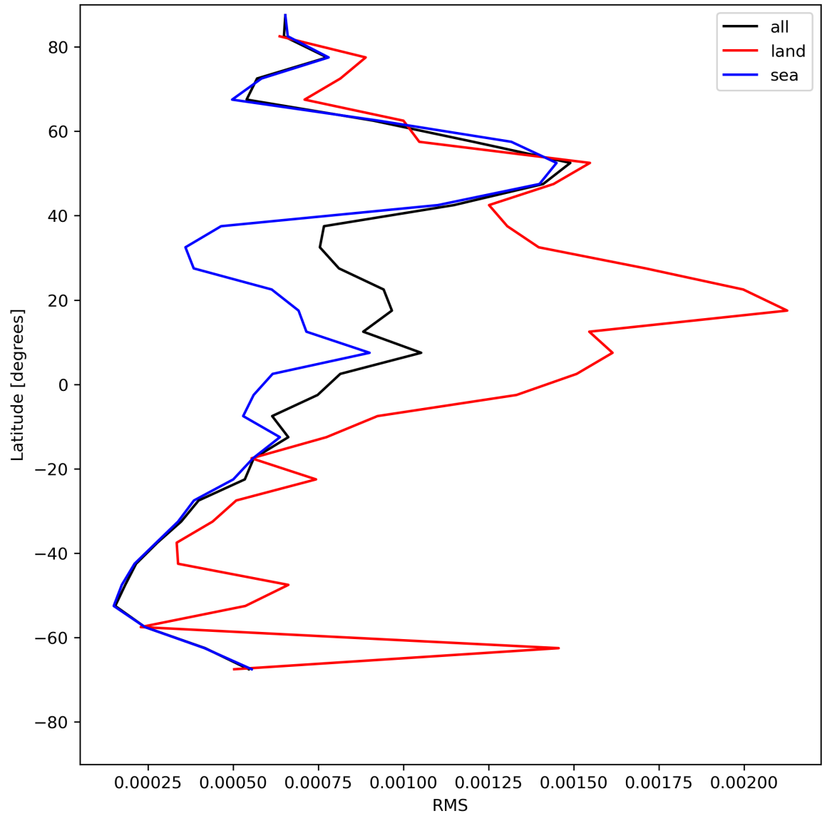
Figure 31: Zonal average of “RMS” for 2023-07-27 to 2023-07-29.
