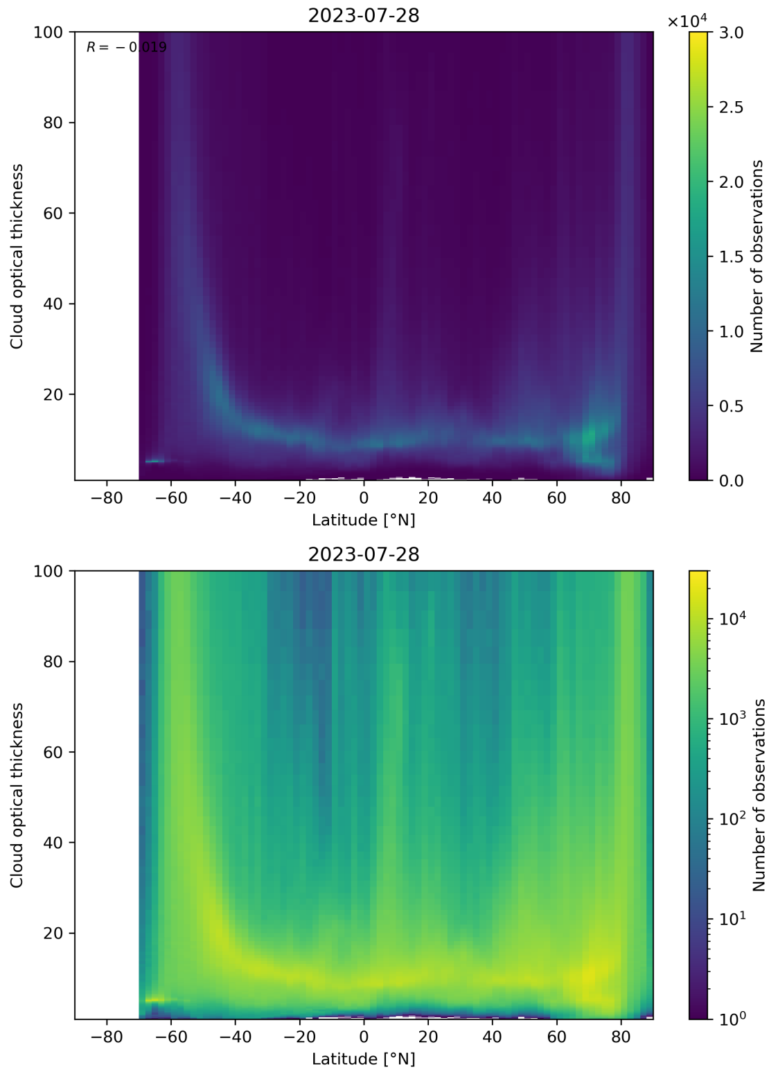
Figure 96: Scatter density plot of “Latitude” against “Cloud optical thickness” for 2023-07-27 to 2023-07-29.
