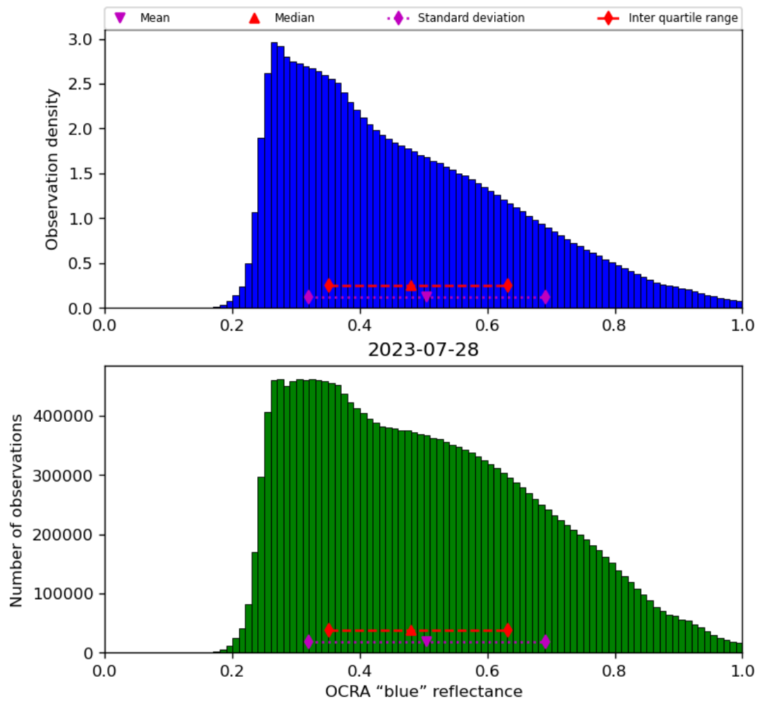
Figure 51: Histogram of “OCRA “blue” reflectance” for 2023-07-27 to 2023-07-29
