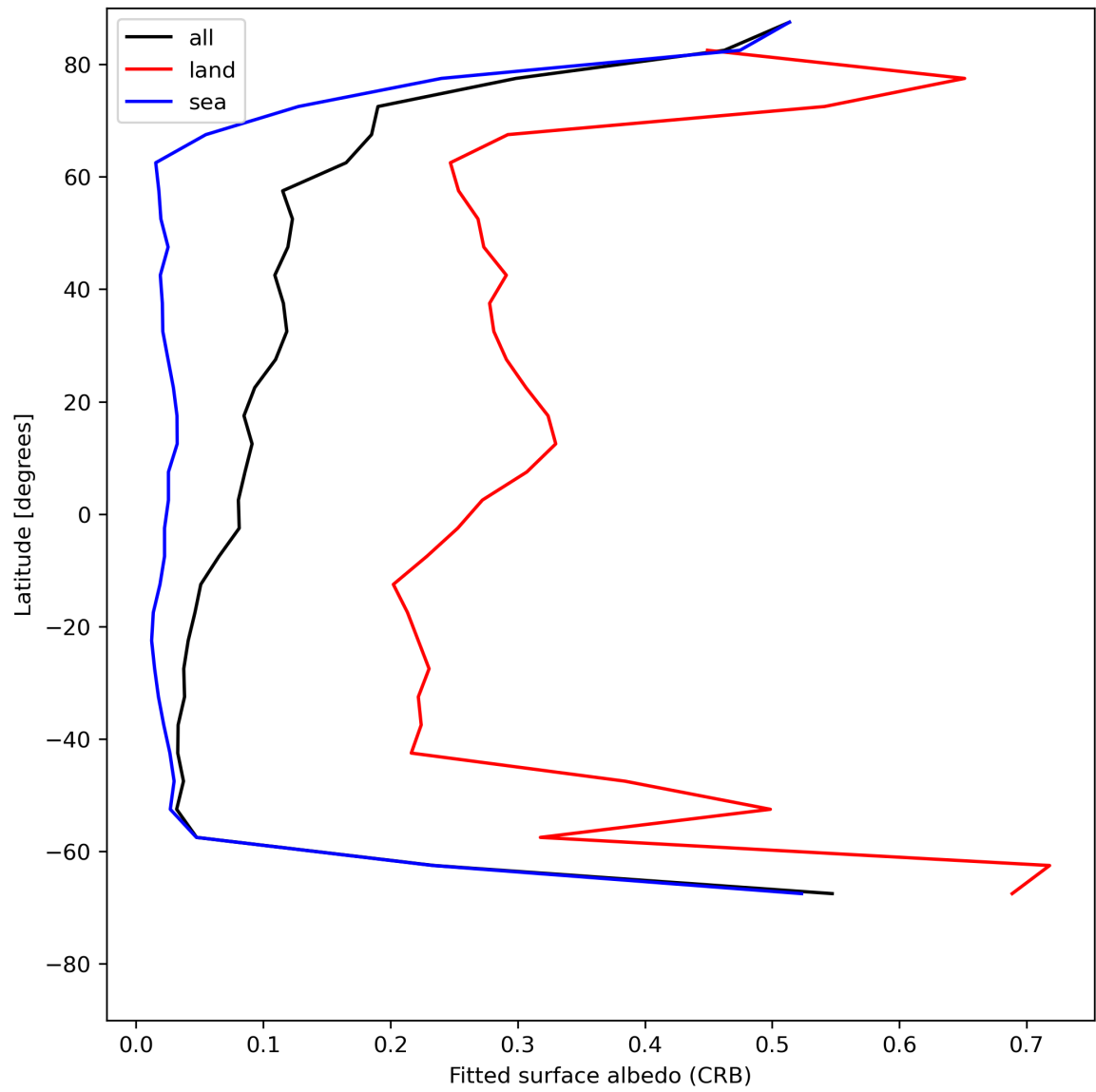
Figure 30: Zonal average of “Fitted surface albedo (CRB)” for 2023-07-27 to 2023-07-29.
