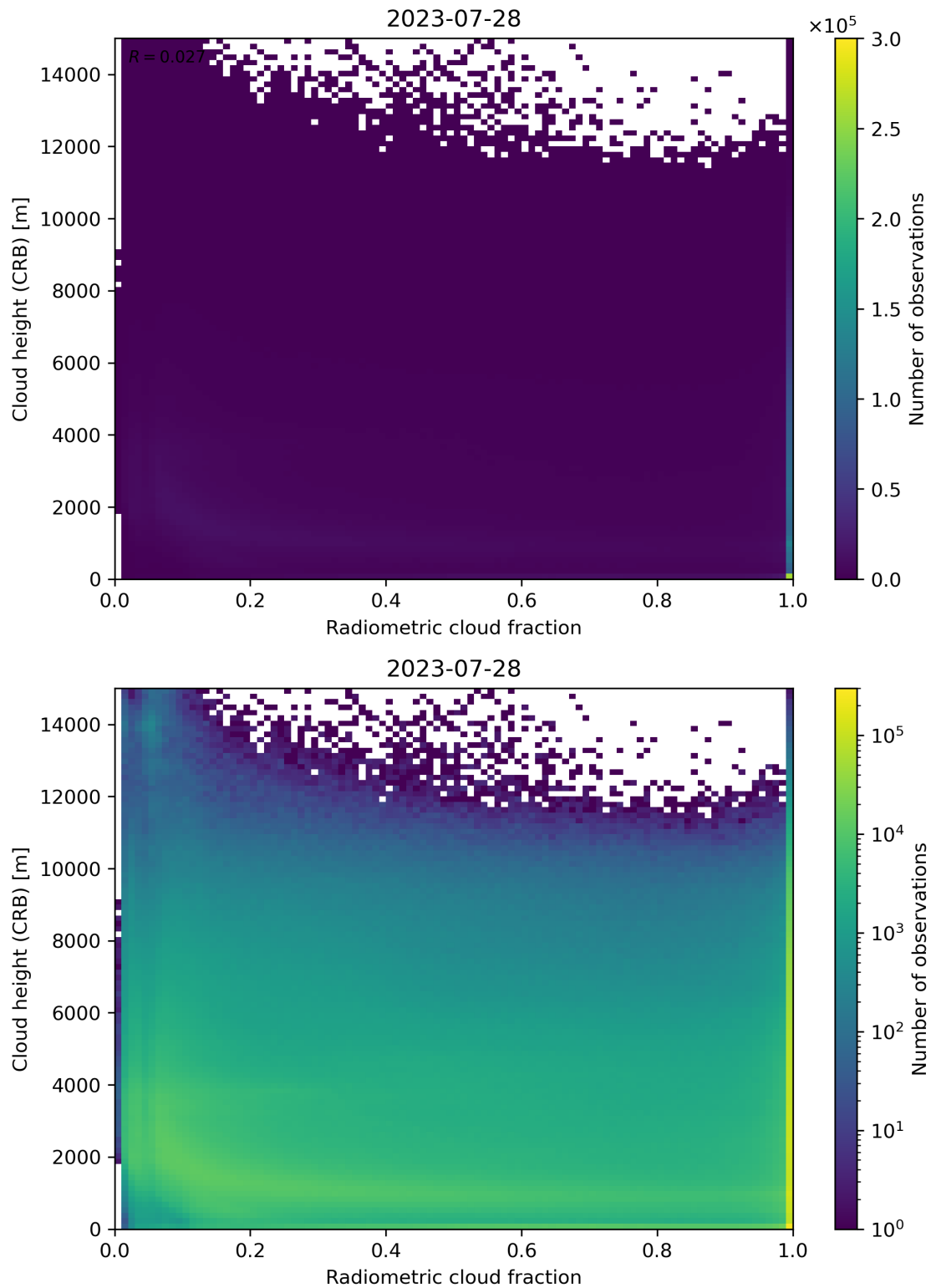
Figure 74: Scatter density plot of “Radiometric cloud fraction” against “Cloud height (CRB)” for 2023-07-27 to 2023-07-29.
