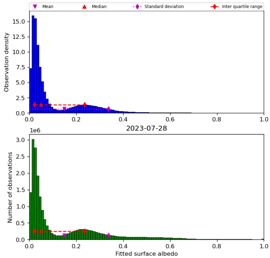
Figure 45: Histogram of “Fitted surface albedo” for 2023-07-27 to 2023-07-29
