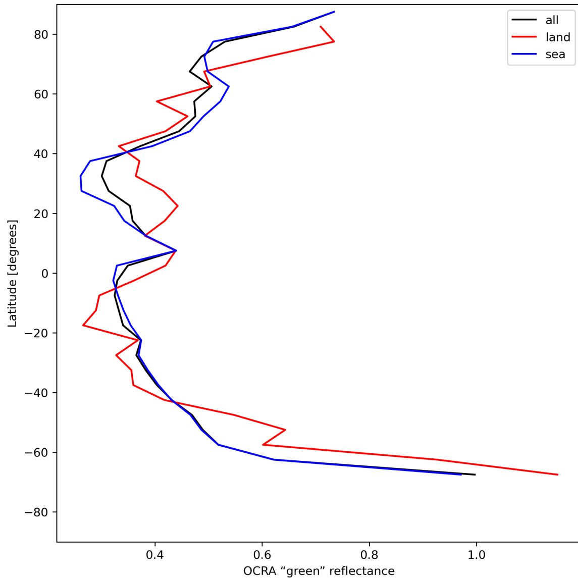
Figure 36: Zonal average of “OCRA “green” reflectance” for 2023-07-27 to 2023-07-29.
