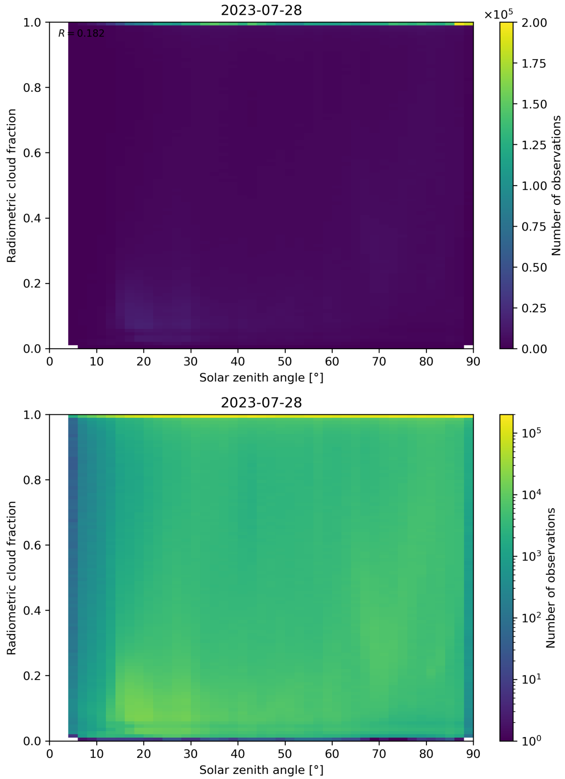
Figure 99: Scatter density plot of “Solar zenith angle” against “Radiometric cloud fraction” for 2023-07-27 to 2023-07-29.
