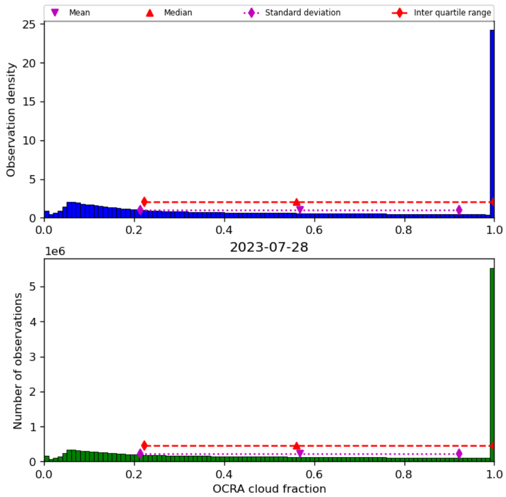
Figure 50: Histogram of “OCRA cloud fraction” for 2023-07-27 to 2023-07-29
