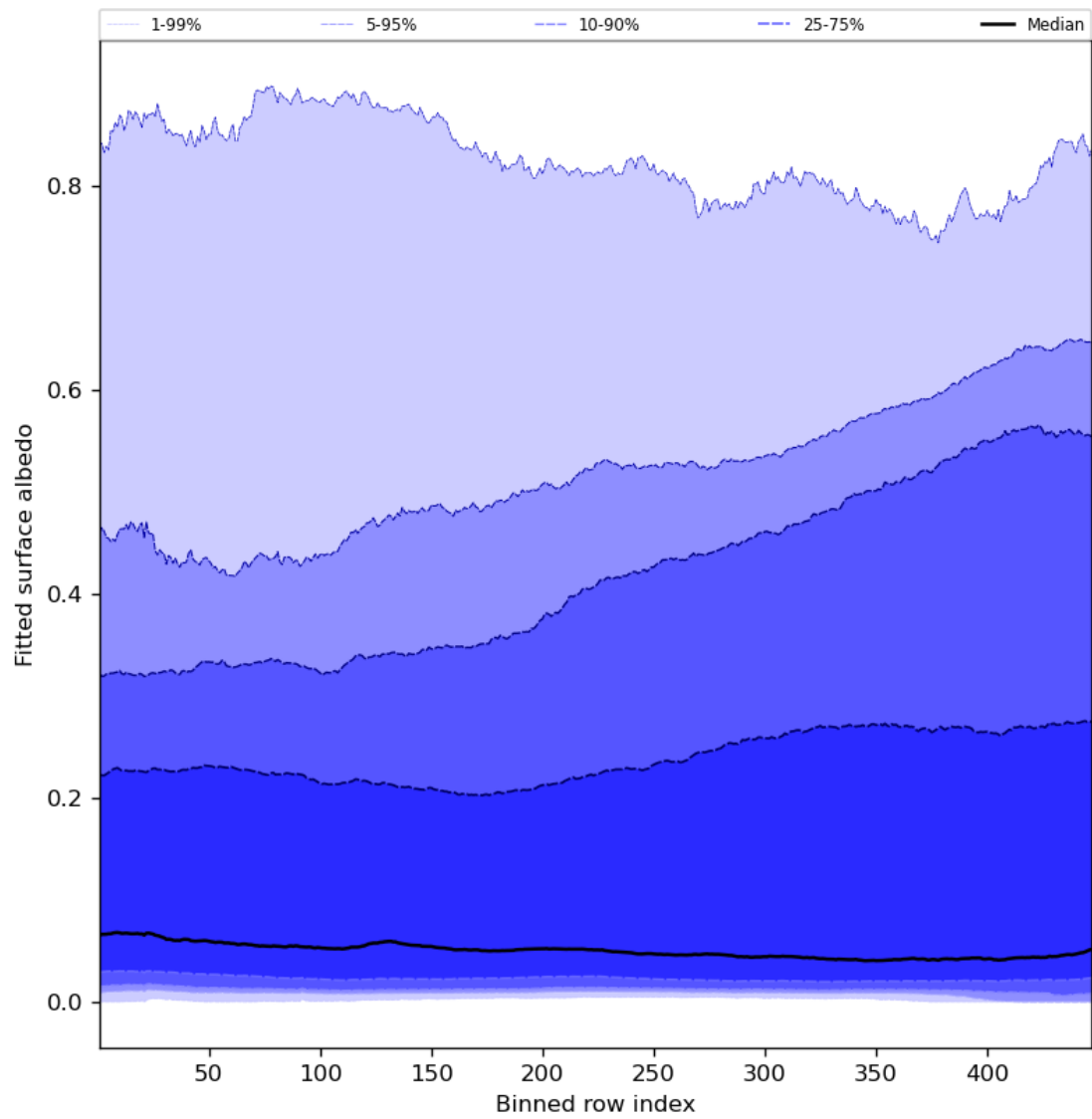
Figure 61: Along track statistics of “Fitted surface albedo” for 2023-07-27 to 2023-07-29
