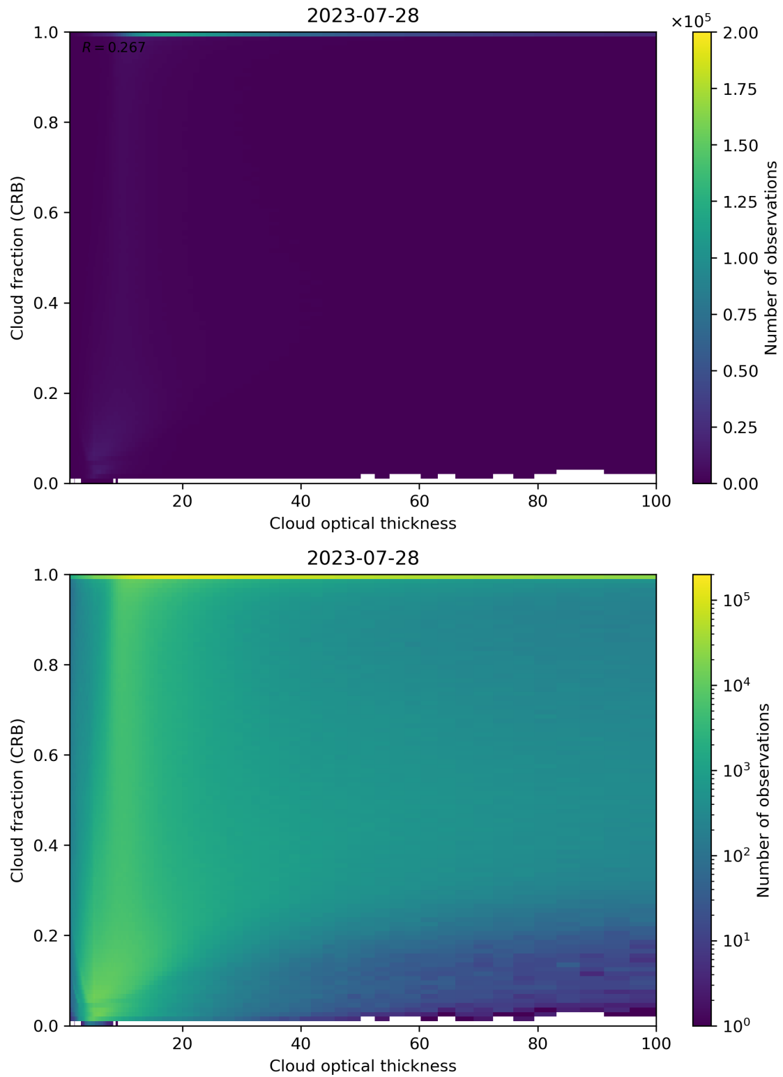
Figure 84: Scatter density plot of “Cloud optical thickness” against “Cloud fraction (CRB)” for 2023-07-27 to 2023-07-29.
