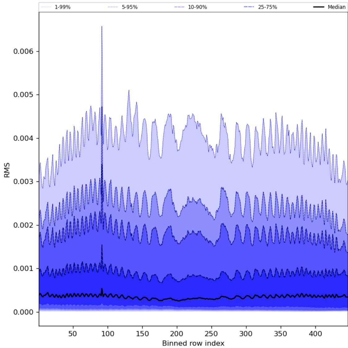
Figure 63: Along track statistics of “RMS” for 2023-07-27 to 2023-07-29
