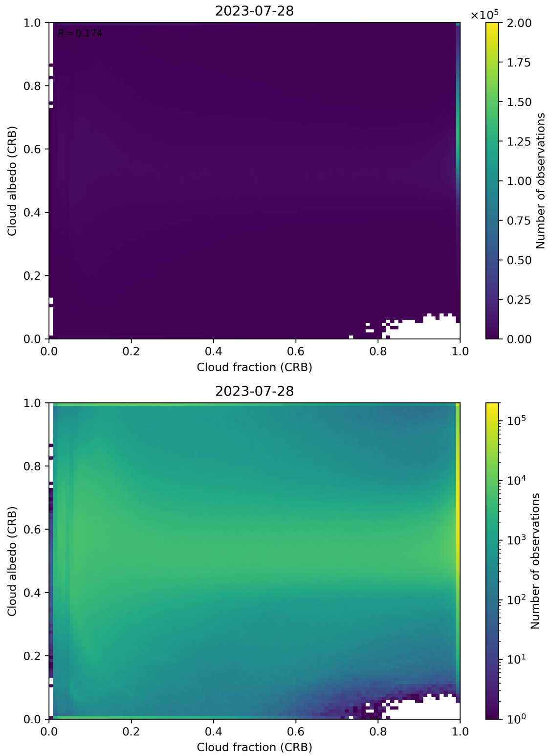
Figure 77: Scatter density plot of “Cloud fraction (CRB)” against “Cloud albedo (CRB)” for 2023-07-27 to 2023-07-29.
