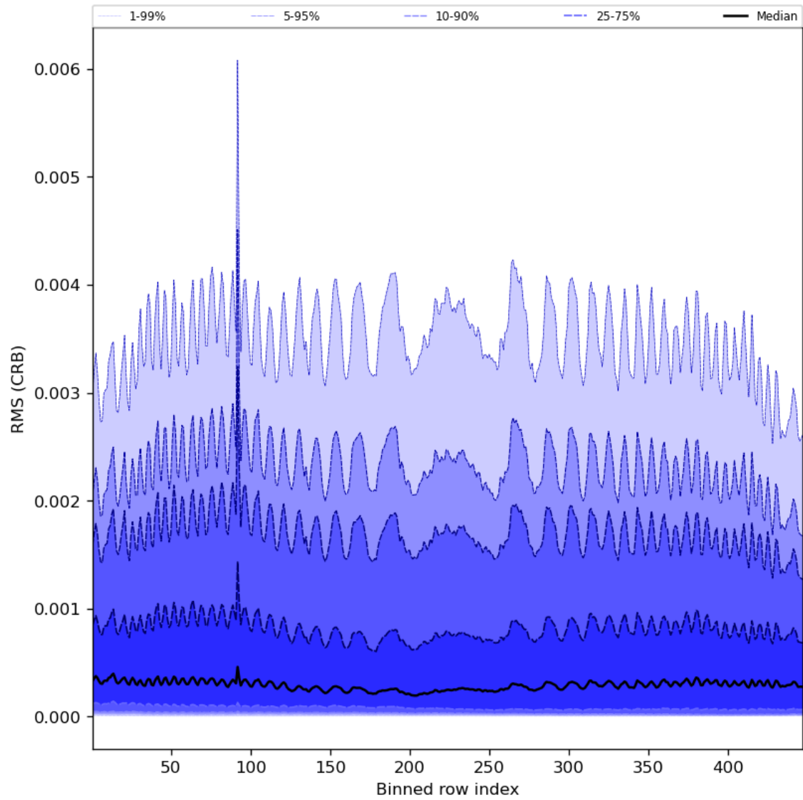
Figure 64: Along track statistics of "RMS (CRB)" for 2023-07-27 to 2023-07-29
