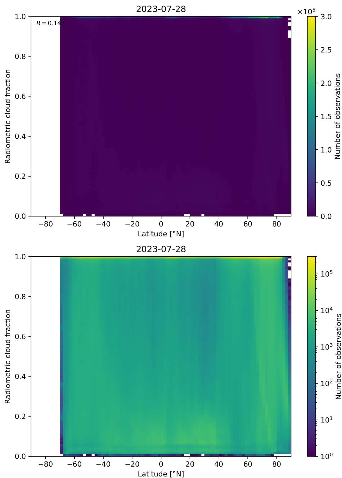
Figure 92: Scatter density plot of “Latitude” against “Radiometric cloud fraction” for 2023-07-27 to 2023-07-29.
