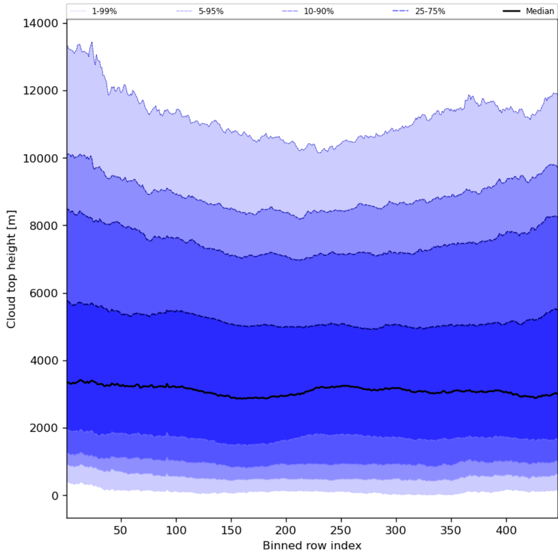
Figure 56: Along track statistics of “Cloud top height” for 2023-07-27 to 2023-07-29
