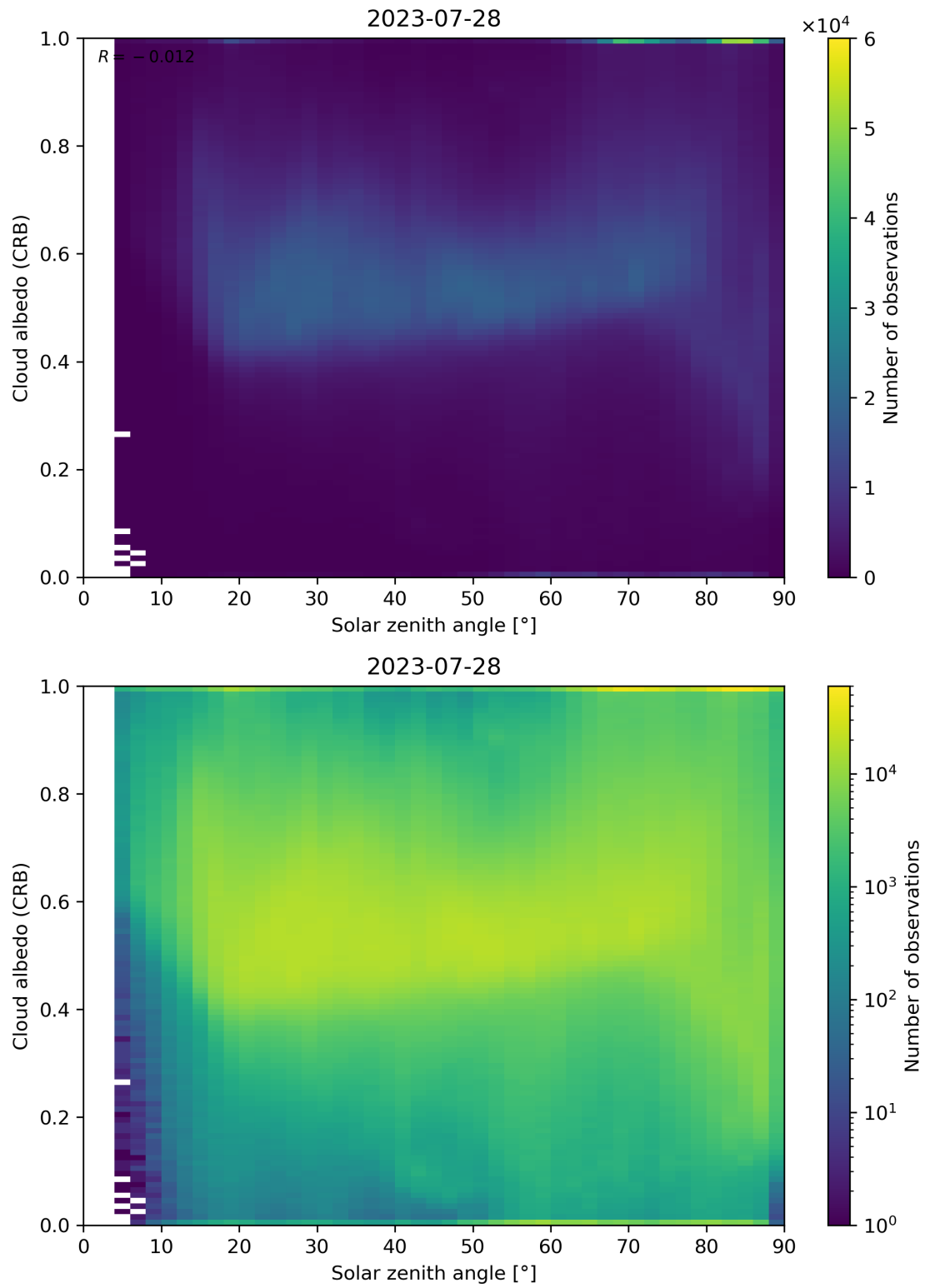
Figure 98: Scatter density plot of “Solar zenith angle” against “Cloud albedo (CRB)” for 2023-07-27 to 2023-07-29.
