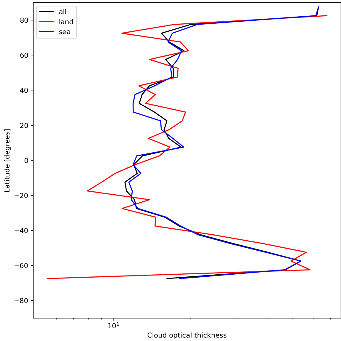
Figure 25: Zonal average of “Cloud optical thickness” for 2023-07-27 to 2023-07-29.
