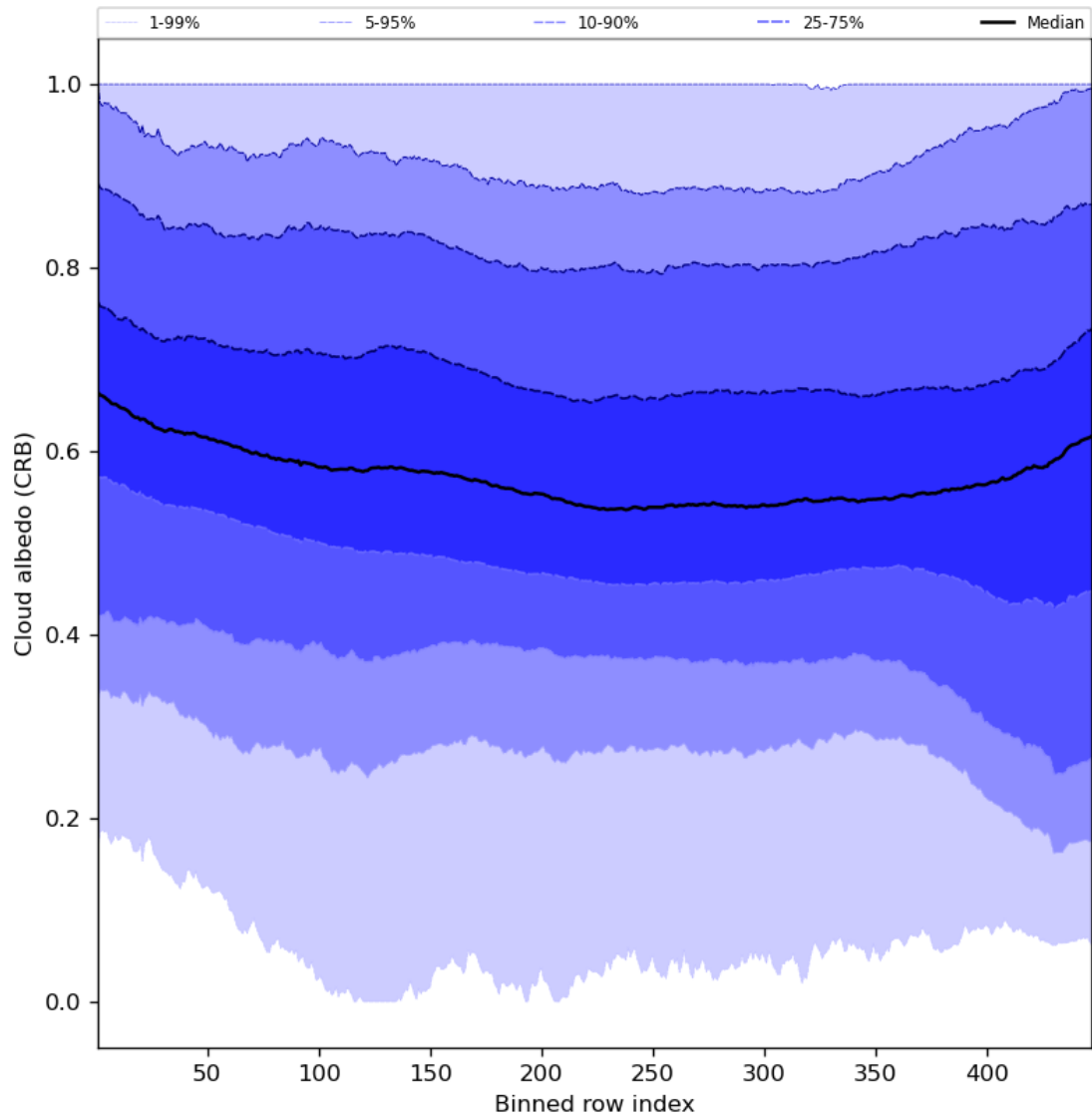
Figure 60: Along track statistics of “Cloud albedo (CRB)” for 2023-07-27 to 2023-07-29
