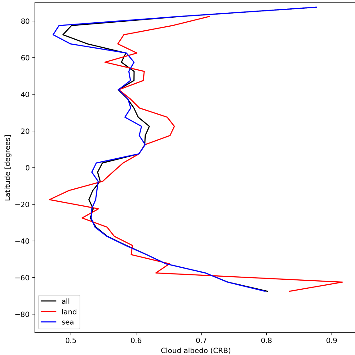
Figure 28: Zonal average of “Cloud albedo (CRB)” for 2023-07-27 to 2023-07-29.
