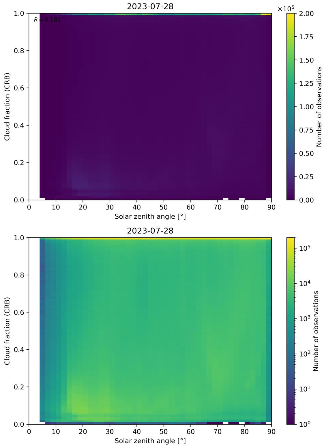
Figure 101: Scatter density plot of “Solar zenith angle” against “Cloud fraction (CRB)” for 2023-07-27 to 2023-07-29.
