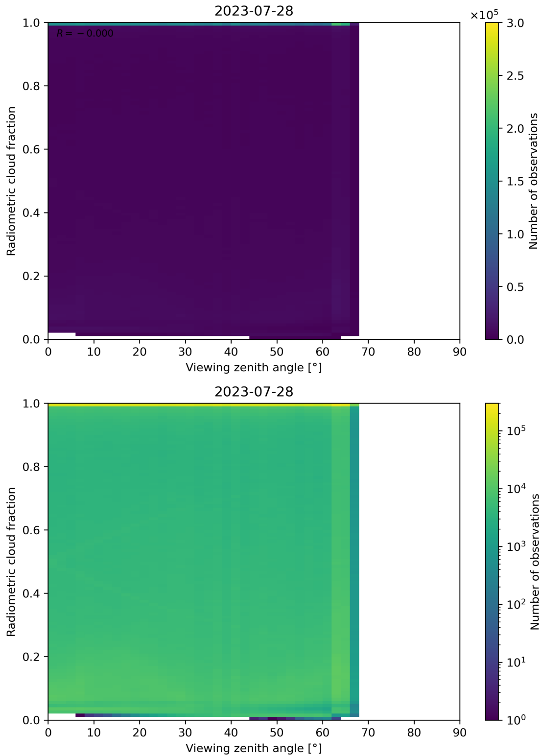
Figure 107: Scatter density plot of “Viewing zenith angle” against “Radiometric cloud fraction” for 2023-07-27 to 2023-07-29.
