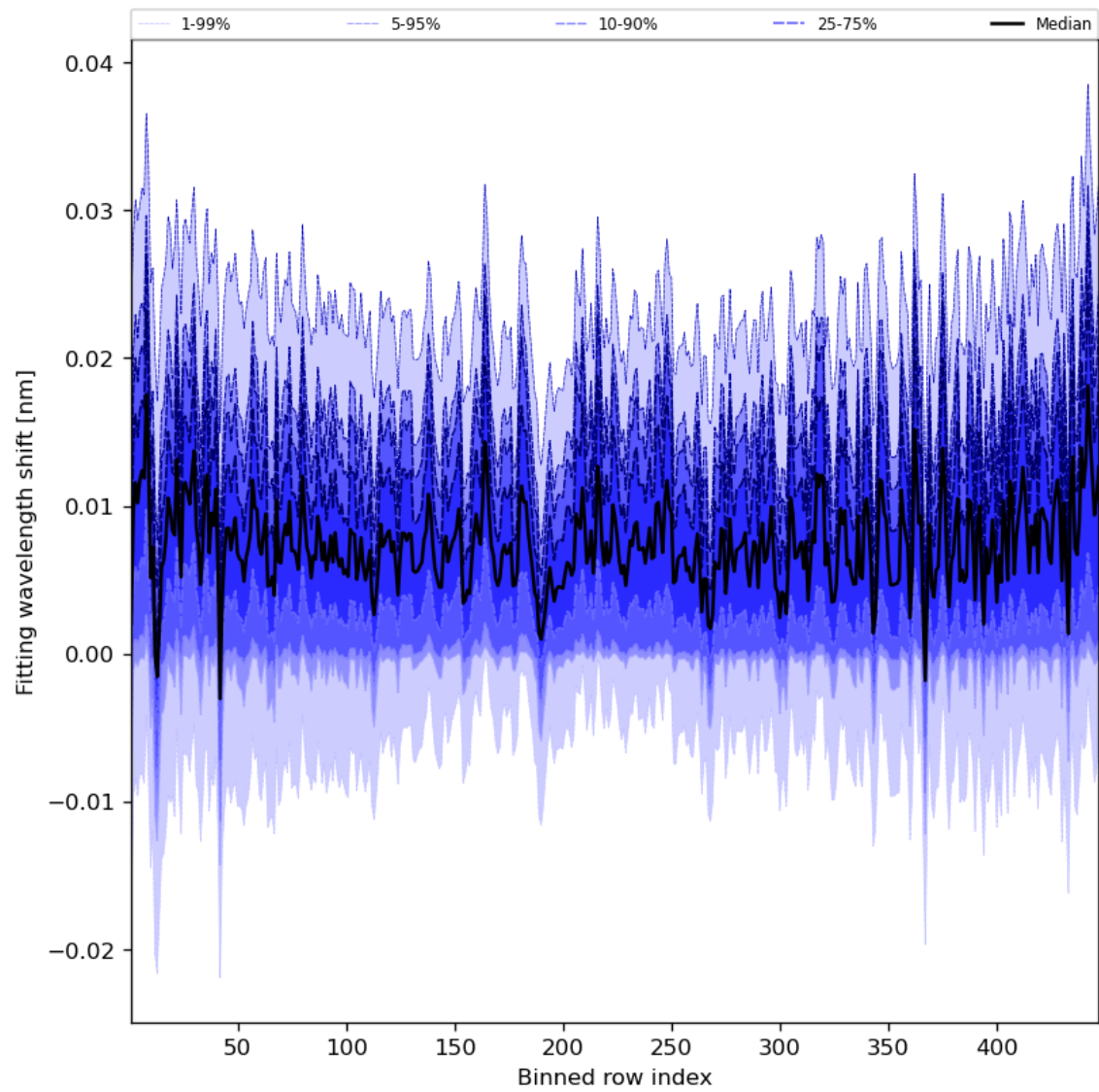
Figure 65: Along track statistics of “Fitting wavelength shift” for 2023-07-27 to 2023-07-29
