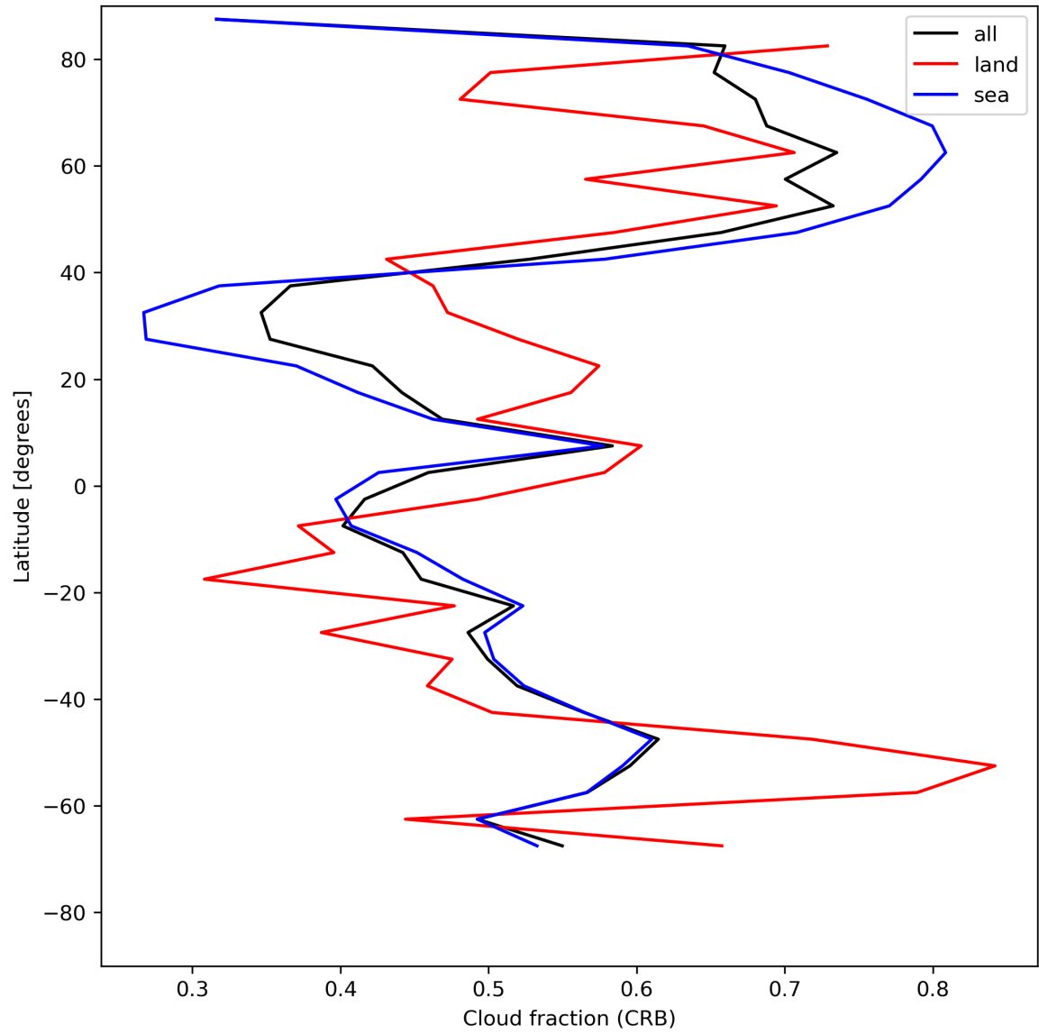
Figure 26: Zonal average of “Cloud fraction (CRB)” for 2023-07-27 to 2023-07-29.
