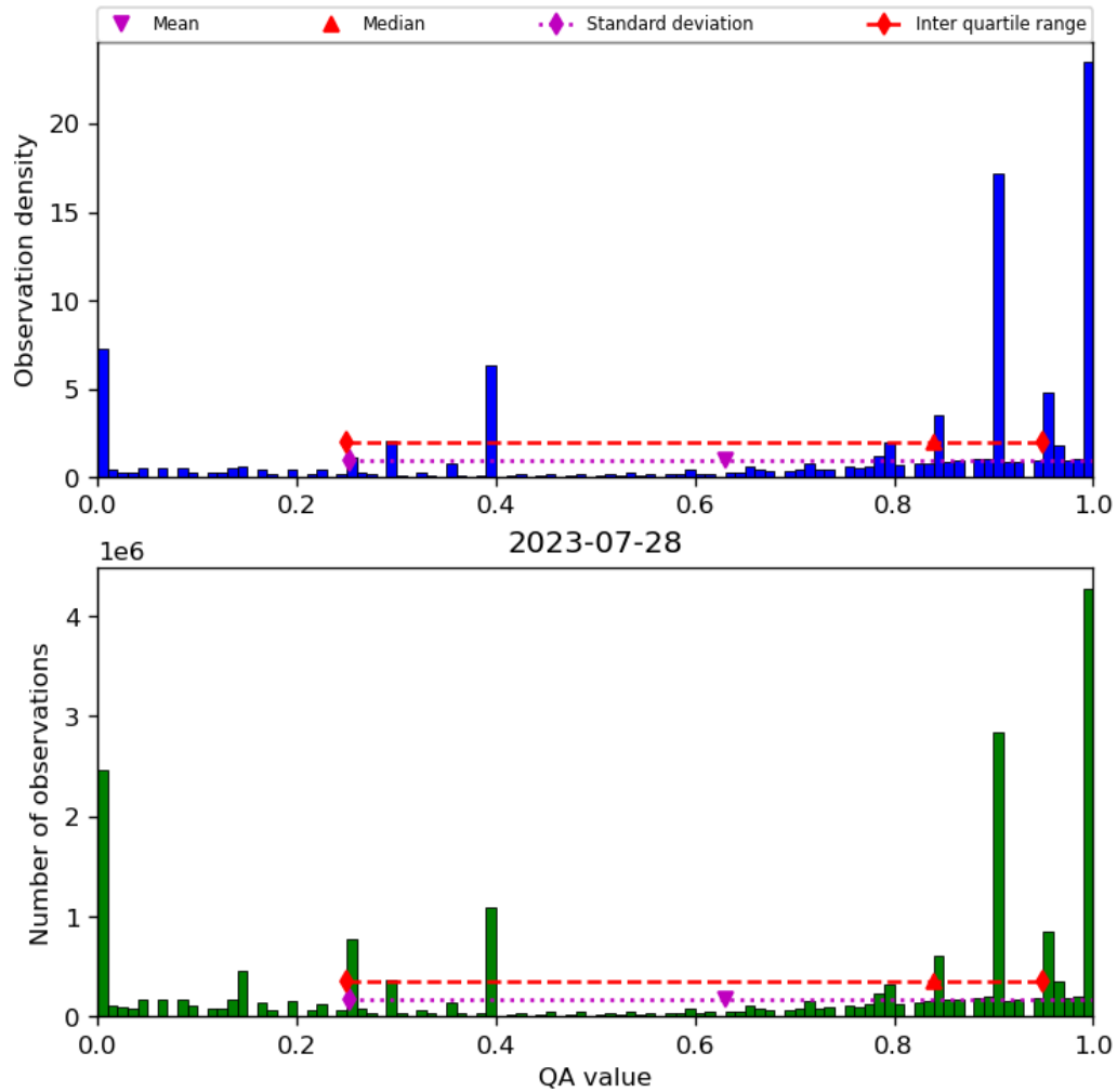
Figure 38: Histogram of “QA value” for 2023-07-27 to 2023-07-29
