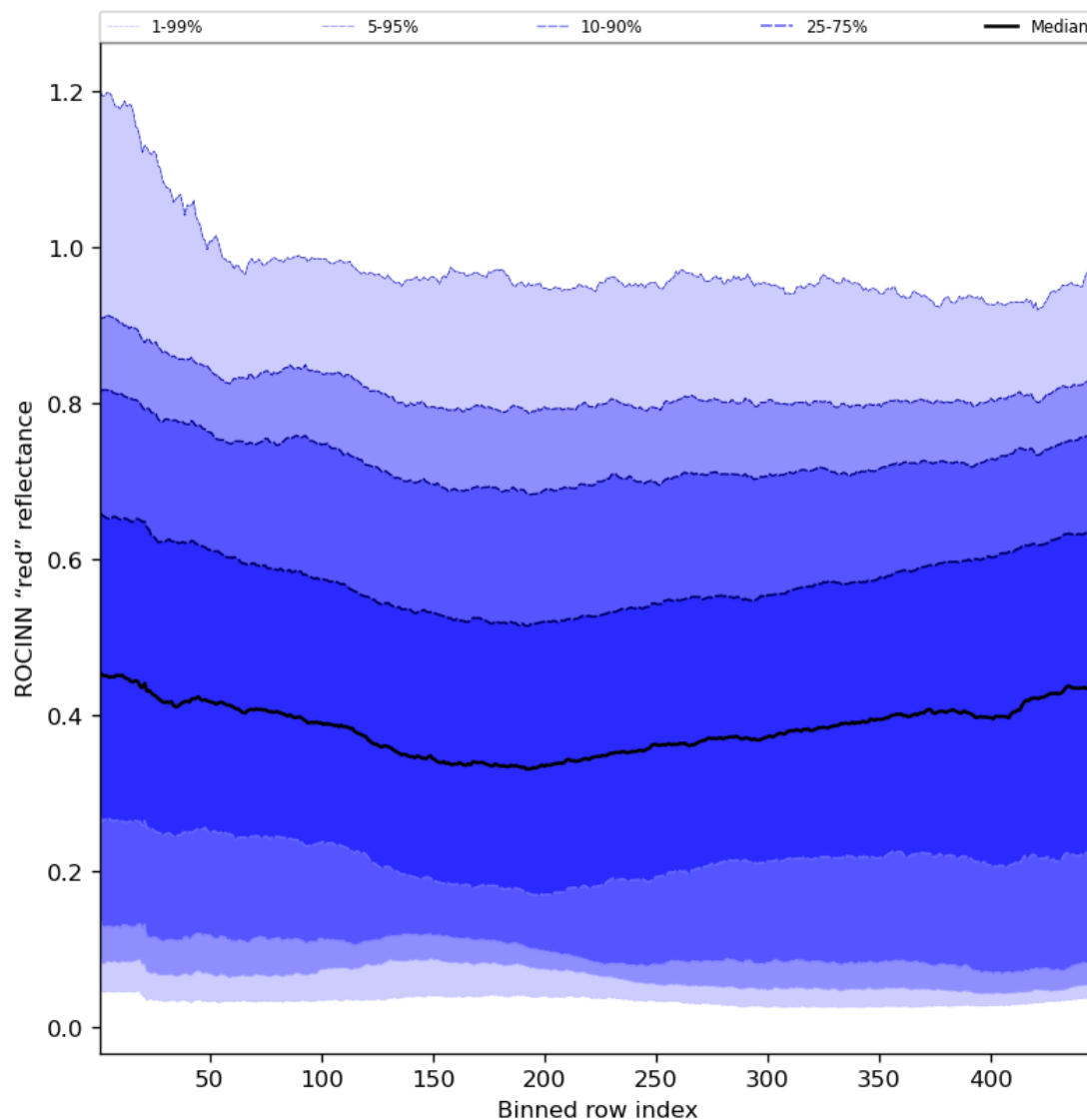
Figure 69: Along track statistics of “ROCINN “red” reflectance” for 2023-07-27 to 2023-07-29
