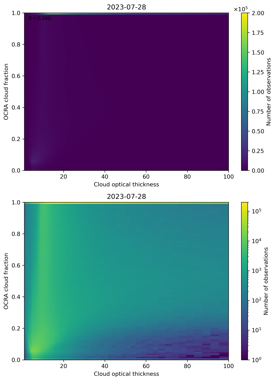
Figure 83: Scatter density plot of “Cloud optical thickness” against “OCRA cloud fraction” for 2023-07-27 to 2023-07-29.
