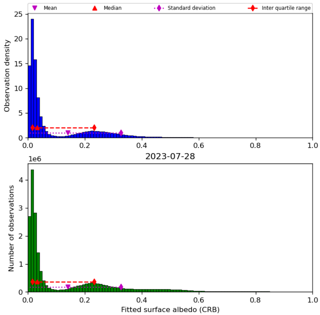
Figure 46: Histogram of “Fitted surface albedo (CRB)” for 2023-07-27 to 2023-07-29
