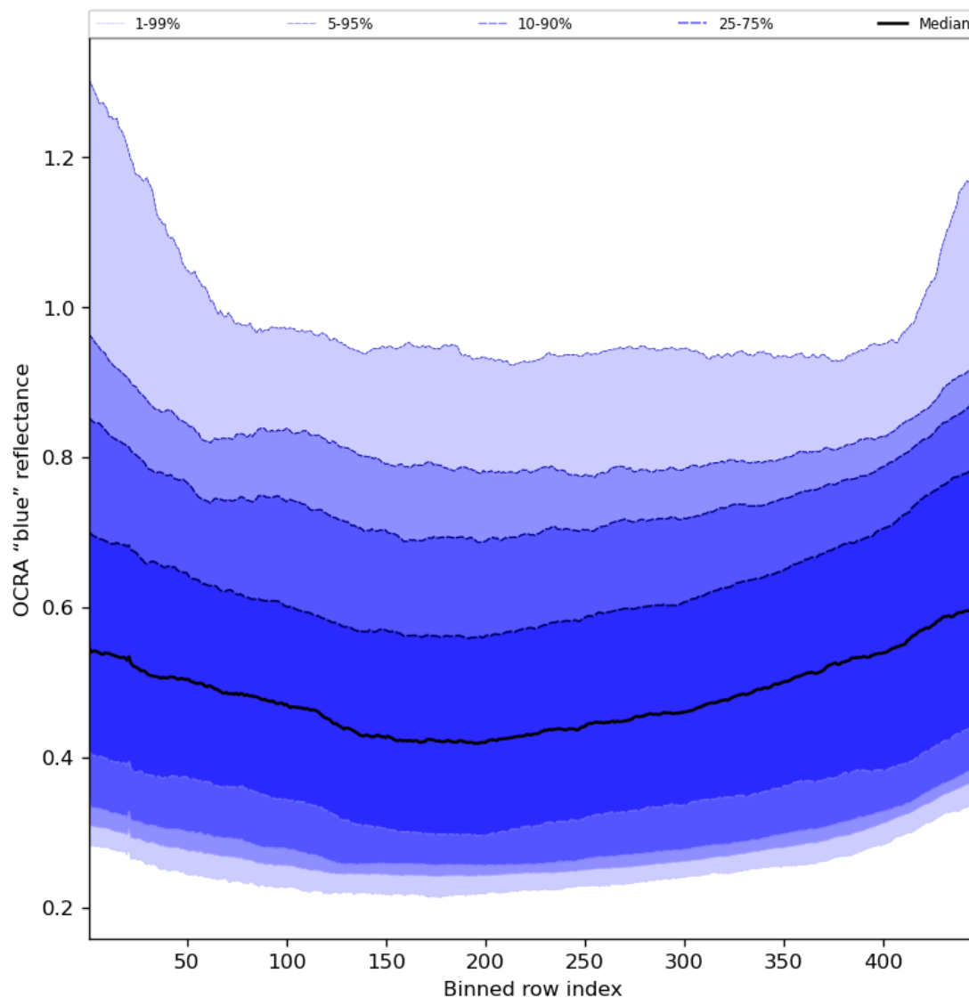
Figure 67: Along track statistics of “OCRA “blue” reflectance” for 2023-07-27 to 2023-07-29
