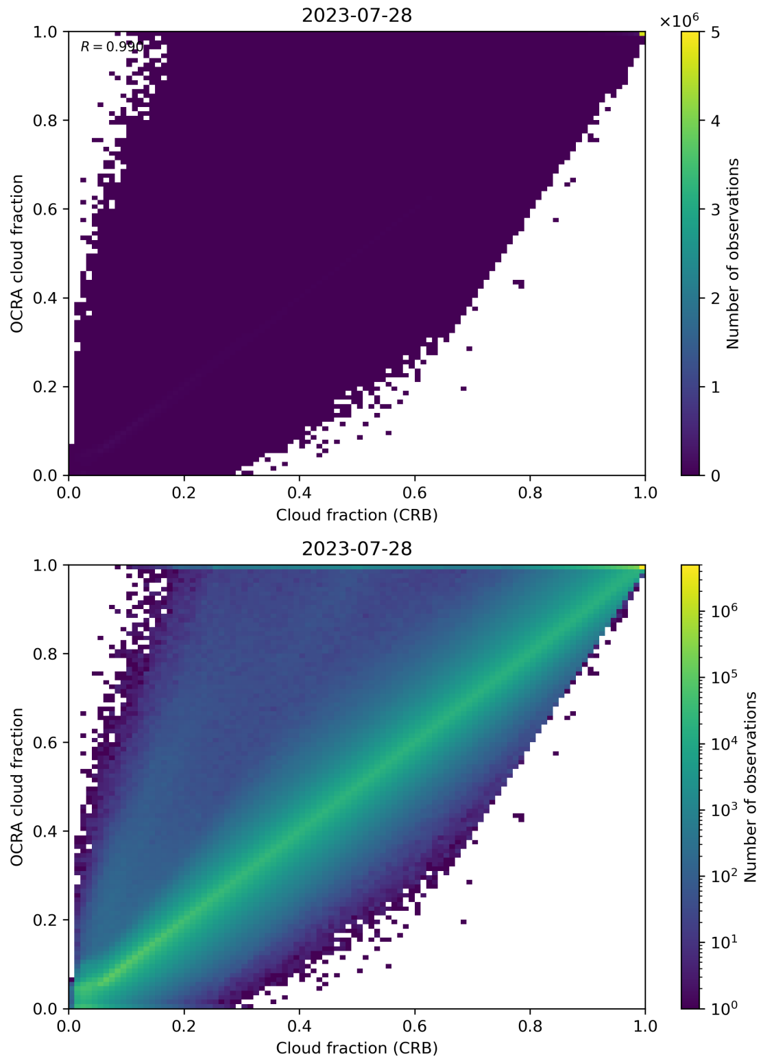
Figure 78: Scatter density plot of “Cloud fraction (CRB)” against “OCRA cloud fraction” for 2023-07-27 to 2023-07-29.
