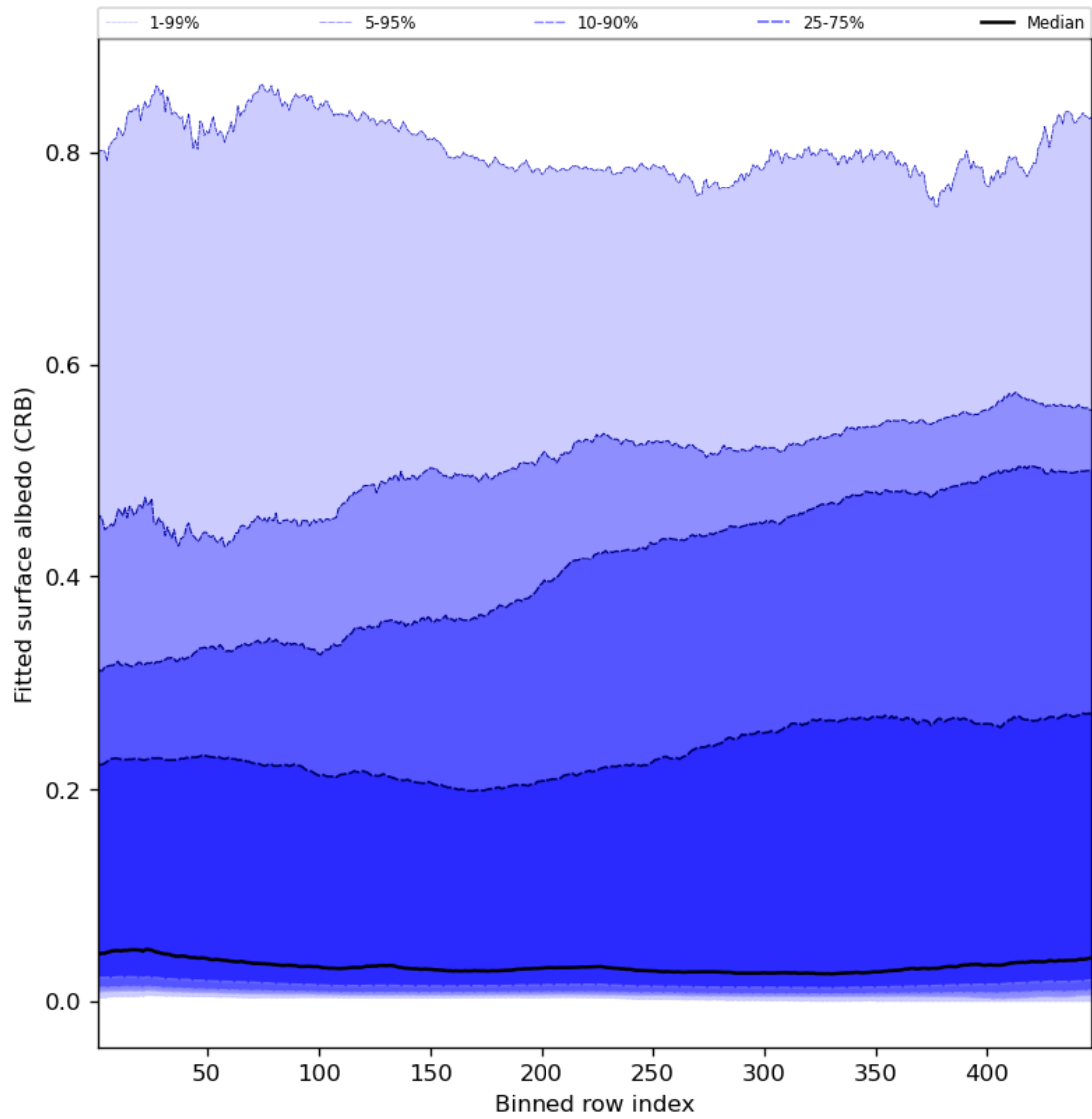
Figure 62: Along track statistics of “Fitted surface albedo (CRB)” for 2023-07-27 to 2023-07-29
