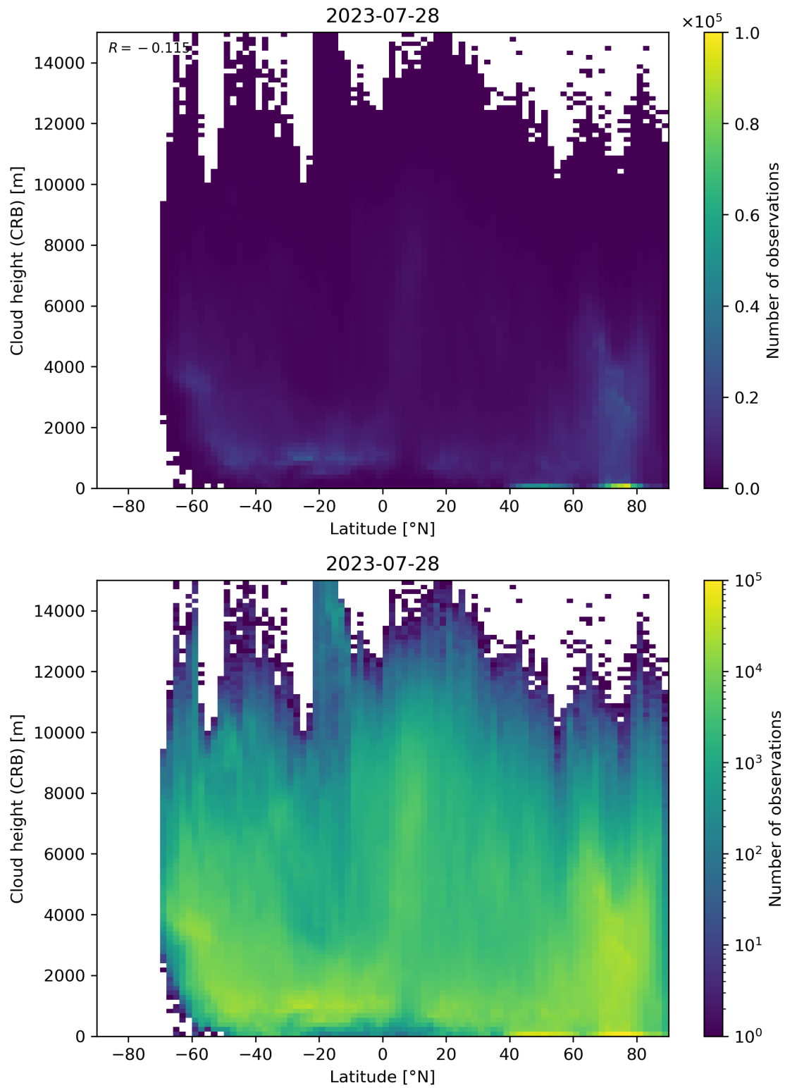
Figure 95: Scatter density plot of “Latitude” against “Cloud height (CRB)” for 2023-07-27 to 2023-07-29.
