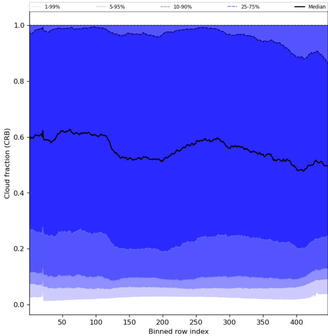
Figure 58: Along track statistics of “Cloud fraction (CRB)” for 2023-07-27 to 2023-07-29
