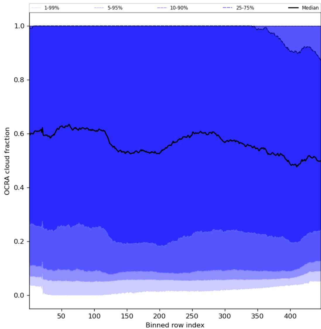
Figure 66: Along track statistics of “OCRA cloud fraction” for 2023-07-27 to 2023-07-29
