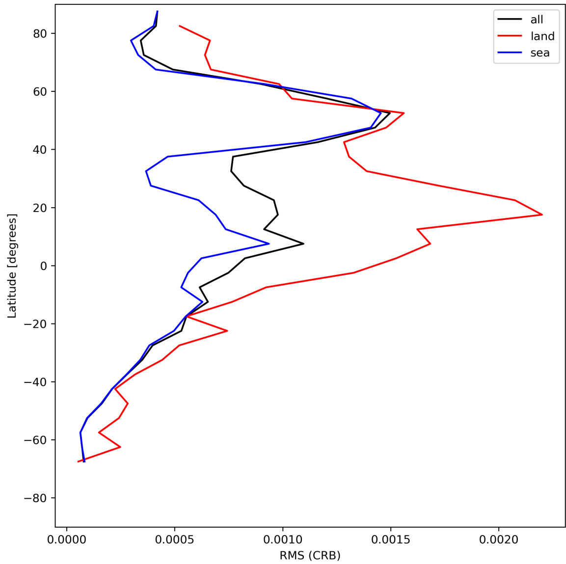
Figure 32: Zonal average of “RMS (CRB)” for 2023-07-27 to 2023-07-29.
