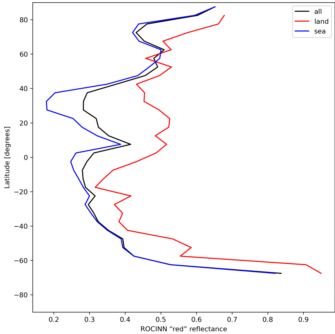
Figure 37: Zonal average of “ROCINN “red” reflectance” for 2023-07-27 to 2023-07-29.
