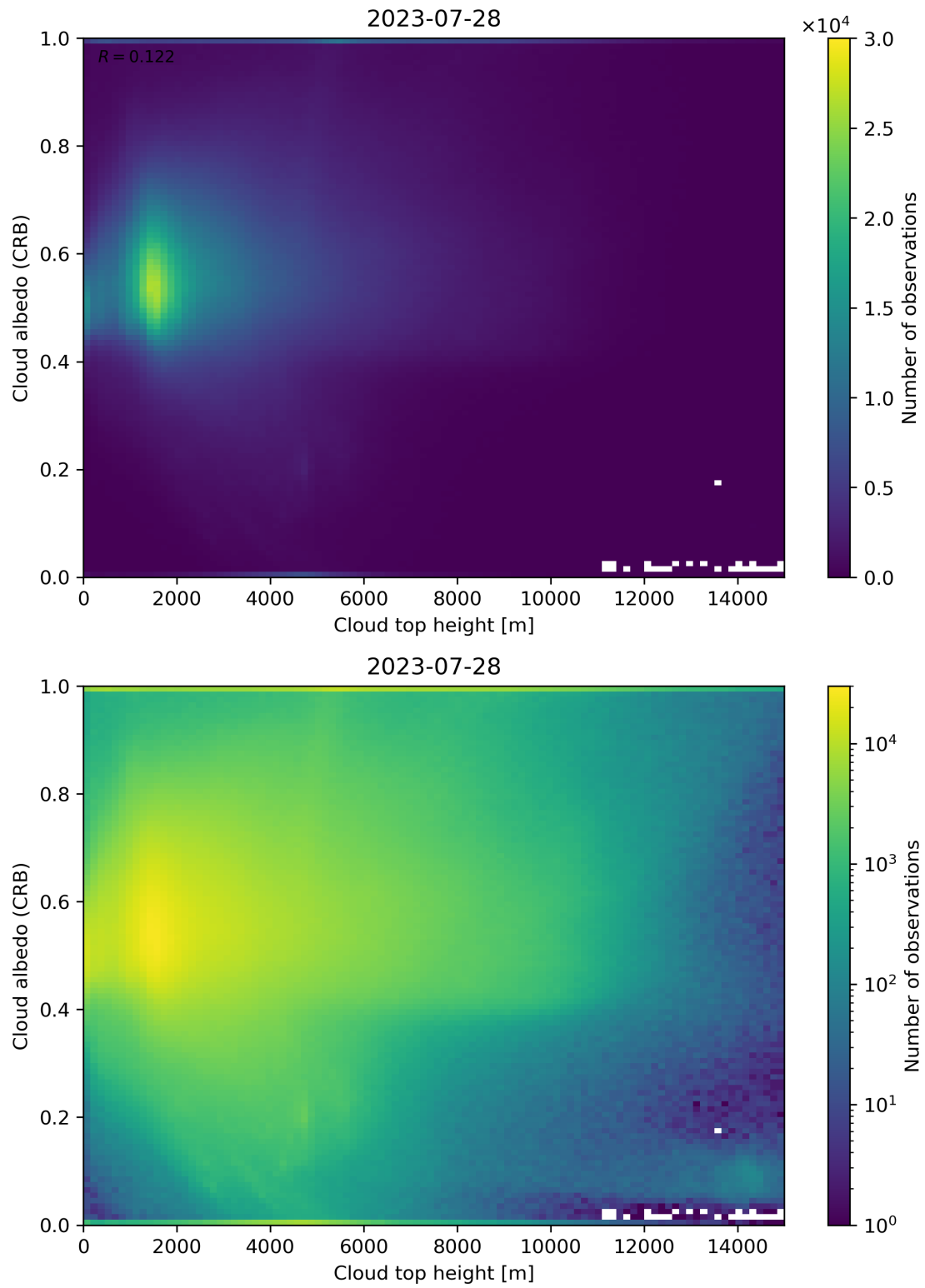
Figure 86: Scatter density plot of “Cloud top height” against “Cloud albedo (CRB)” for 2023-07-27 to 2023-07-29.
