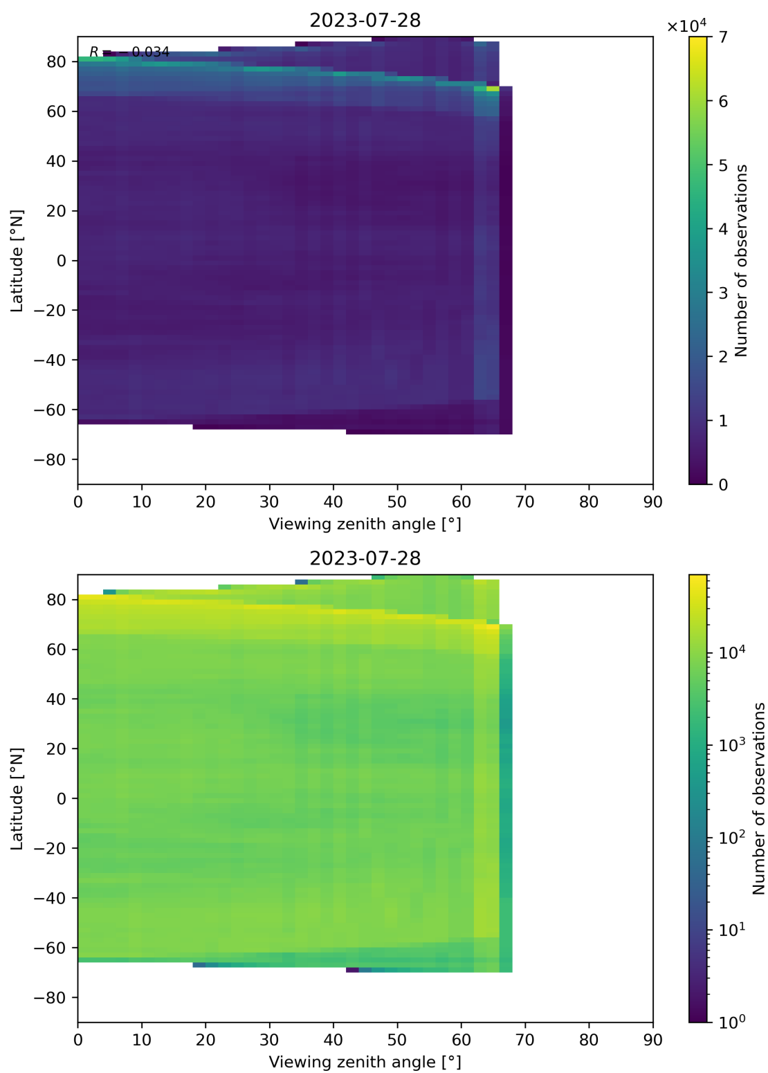
Figure 113: Scatter density plot of “Viewing zenith angle” against “Latitude” for 2023-07-27 to 2023-07-29.
