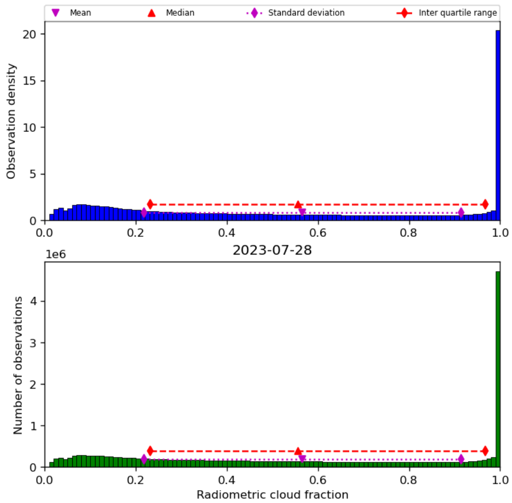
Figure 39: Histogram of “Radiometric cloud fraction” for 2023-07-27 to 2023-07-29
