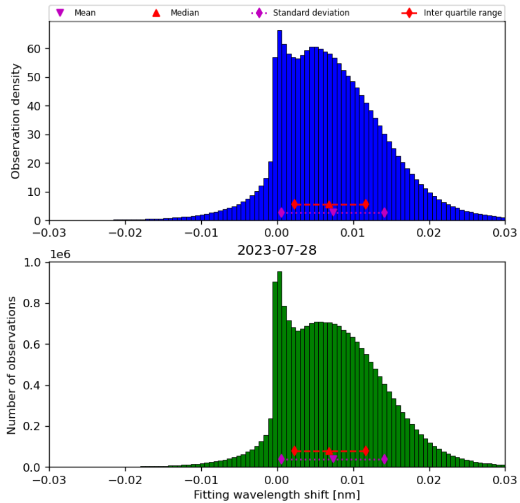
Figure 49: Histogram of “Fitting wavelength shift” for 2023-07-27 to 2023-07-29
