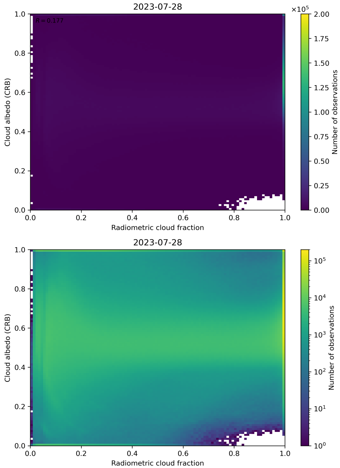
Figure 71: Scatter density plot of “Radiometric cloud fraction” against “Cloud albedo (CRB)” for 2023-07-27 to 2023-07-29.
