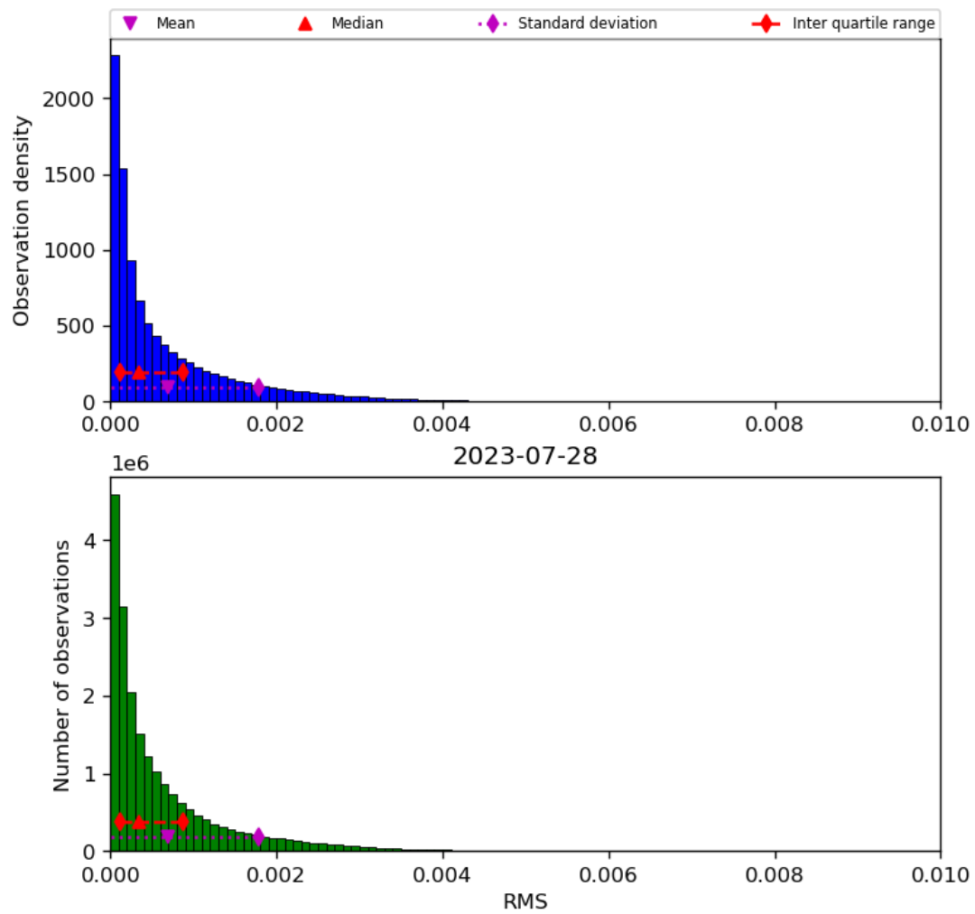
Figure 47: Histogram of “RMS” for 2023-07-27 to 2023-07-29
