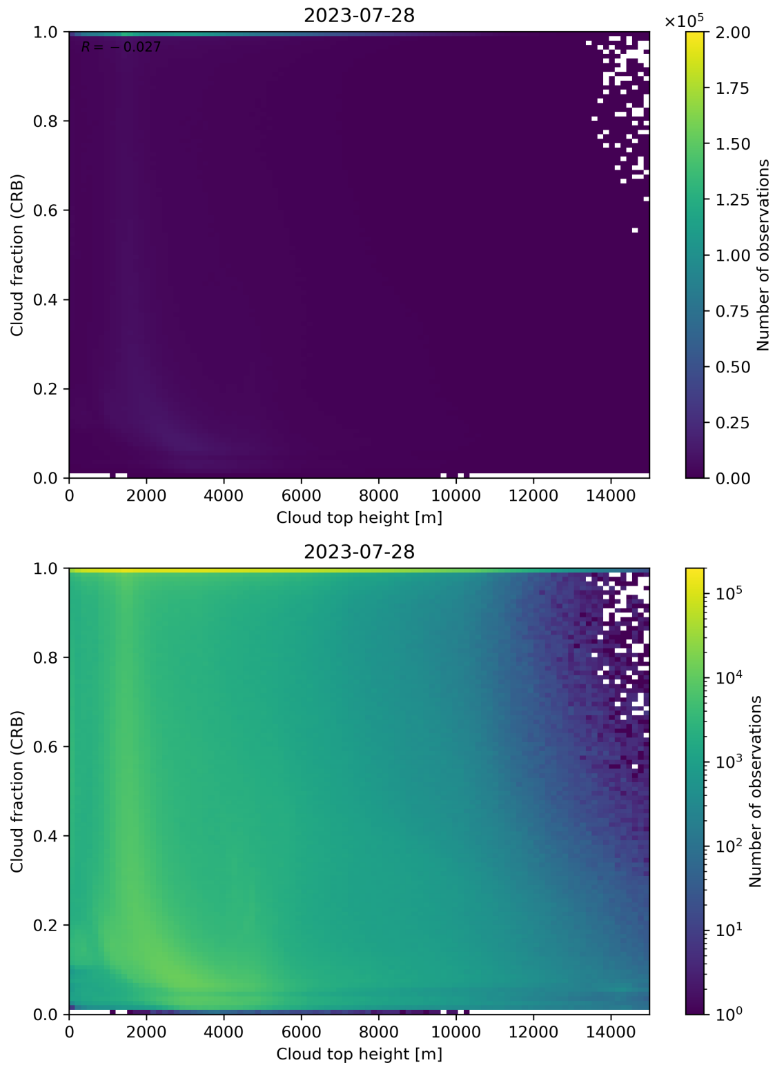
Figure 88: Scatter density plot of “Cloud top height” against “Cloud fraction (CRB)” for 2023-07-27 to 2023-07-29.
