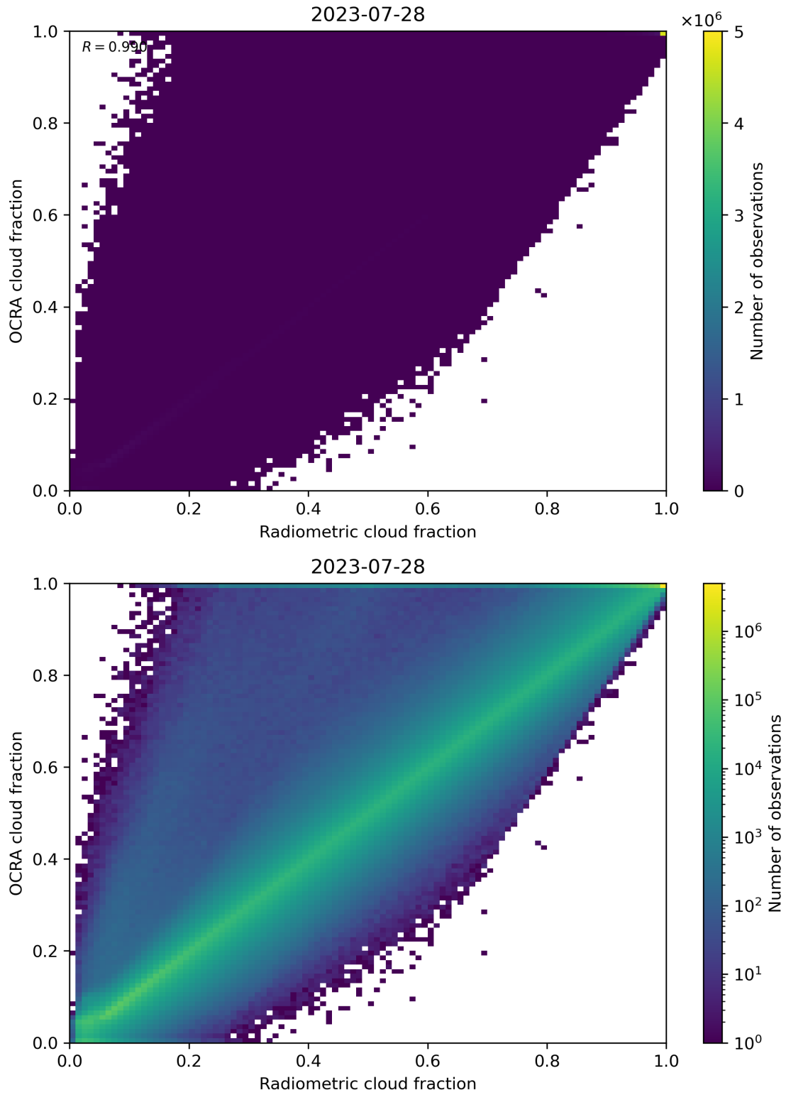
Figure 72: Scatter density plot of “Radiometric cloud fraction” against “OCRA cloud fraction” for 2023-07-27 to 2023-07-29.
