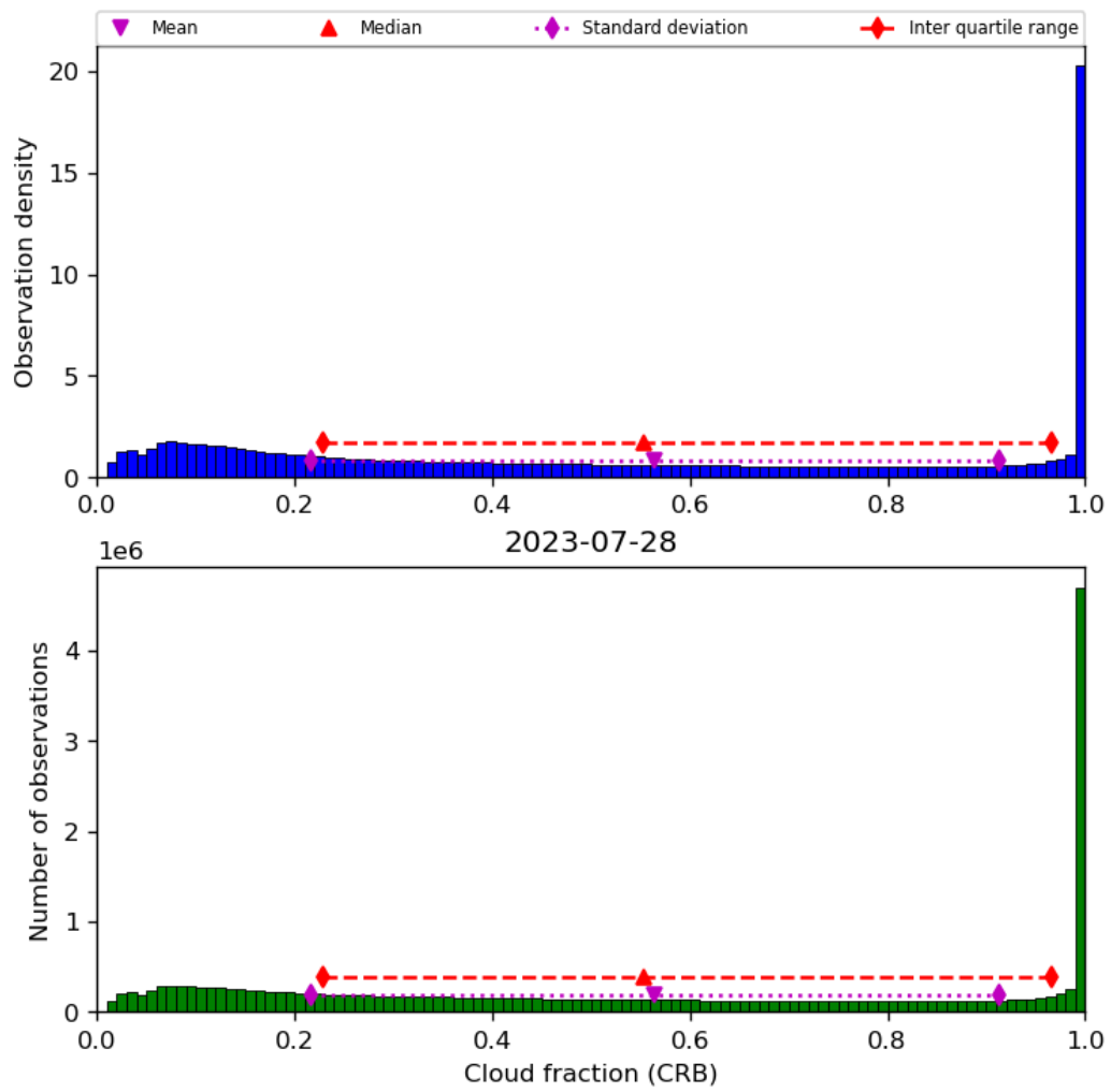
Figure 42: Histogram of “Cloud fraction (CRB)” for 2023-07-27 to 2023-07-29
