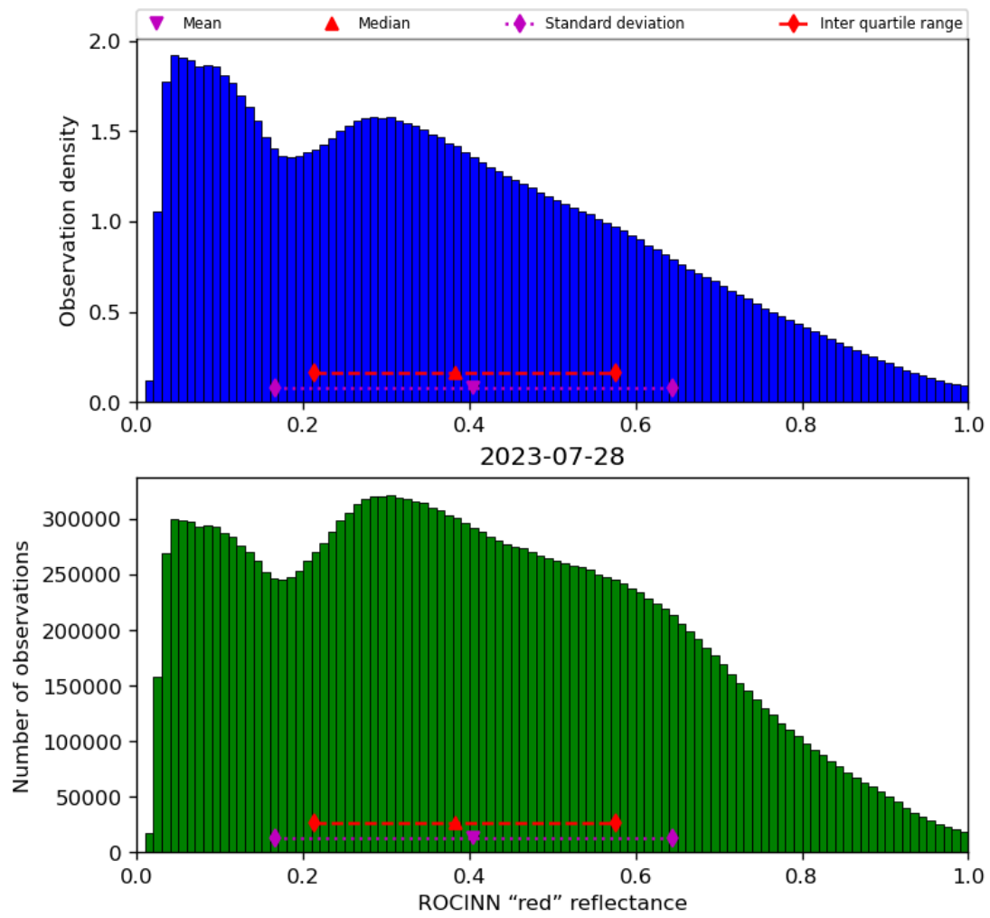
Figure 53: Histogram of “ROCINN “red” reflectance” for 2023-07-27 to 2023-07-29
