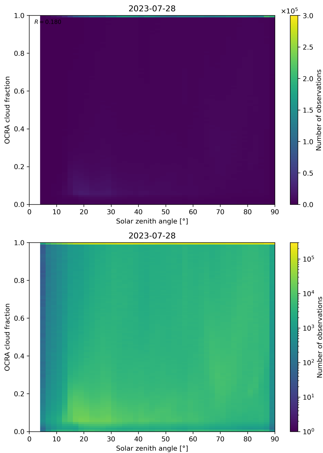
Figure 100: Scatter density plot of “Solar zenith angle” against “OCRA cloud fraction” for 2023-07-27 to 2023-07-29.
