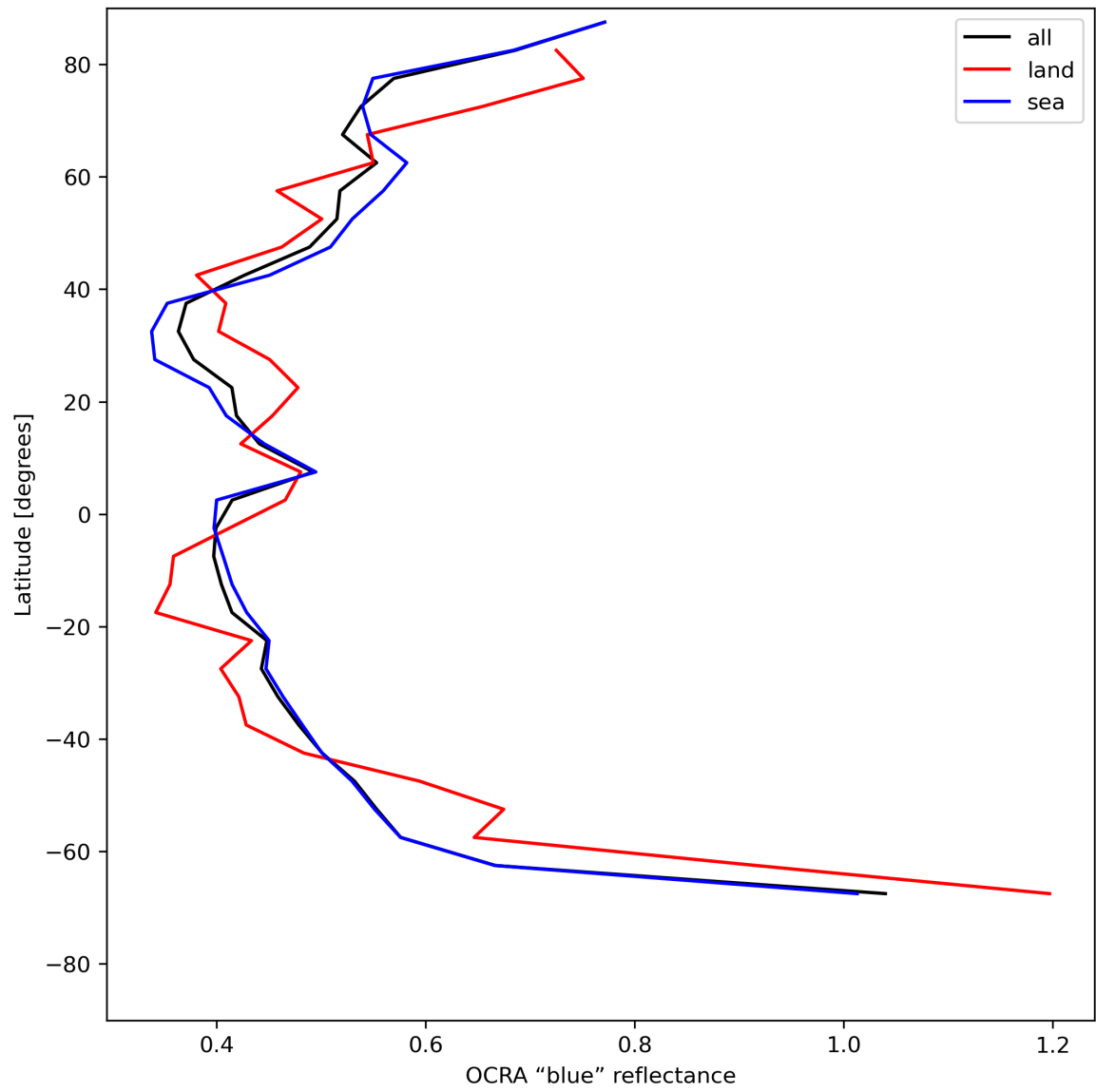
Figure 35: Zonal average of "OCRA "blue" reflectance" for 2023-07-27 to 2023-07-29.
