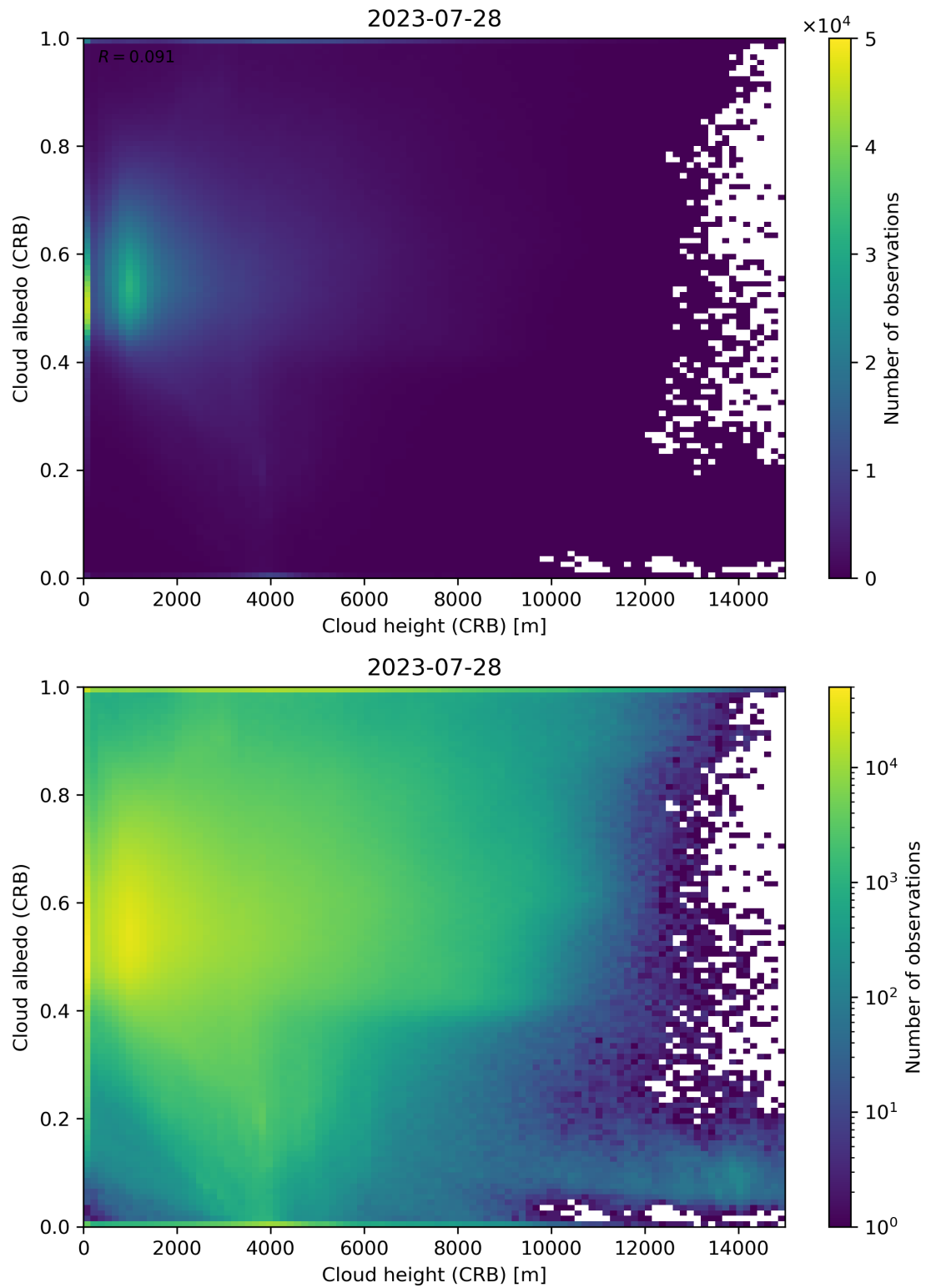
Figure 80: Scatter density plot of “Cloud height (CRB)” against “Cloud albedo (CRB)” for 2023-07-27 to 2023-07-29.
