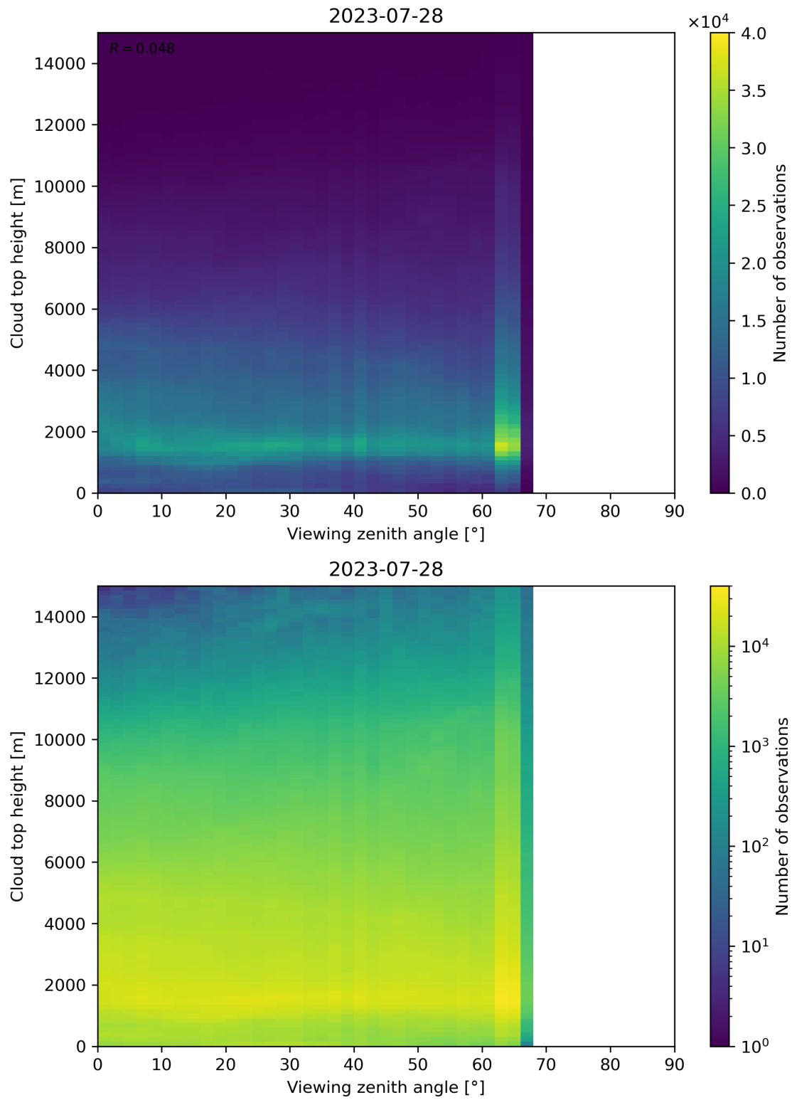
Figure 112: Scatter density plot of “Viewing zenith angle” against “Cloud top height” for 2023-07-27 to 2023-07-29.
