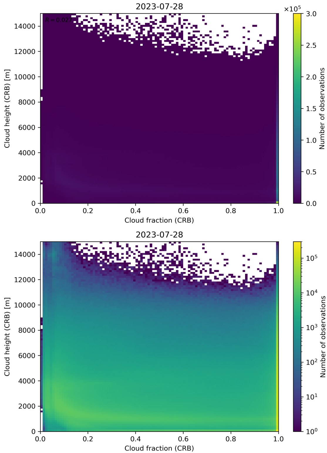
Figure 79: Scatter density plot of “Cloud fraction (CRB)” against “Cloud height (CRB)” for 2023-07-27 to 2023-07-29.
