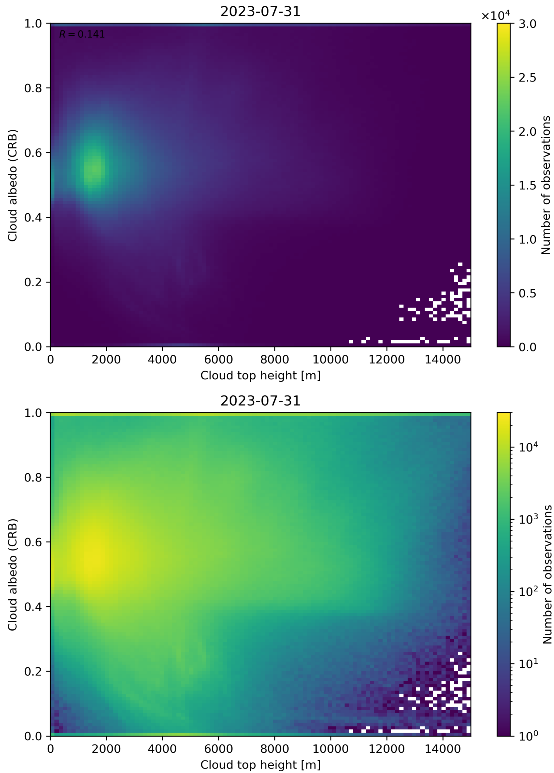
Figure 86: Scatter density plot of “Cloud top height” against “Cloud albedo (CRB)” for 2023-07-30 to 2023-08-01.
