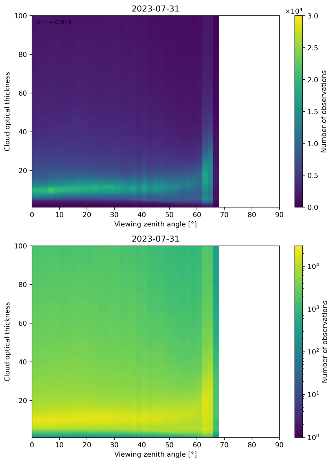
Figure 111: Scatter density plot of “Viewing zenith angle” against “Cloud optical thickness” for 2023-07-30 to 2023-08-01.
