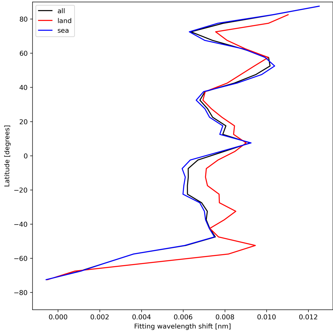
Figure 33: Zonal average of “Fitting wavelength shift” for 2023-07-30 to 2023-08-01.
