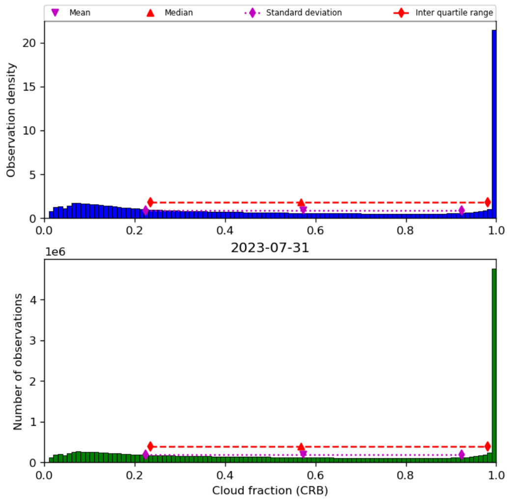
Figure 42: Histogram of “Cloud fraction (CRB)” for 2023-07-30 to 2023-08-01
