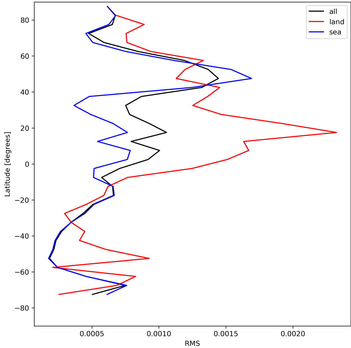
Figure 31: Zonal average of “RMS” for 2023-07-30 to 2023-08-01.
