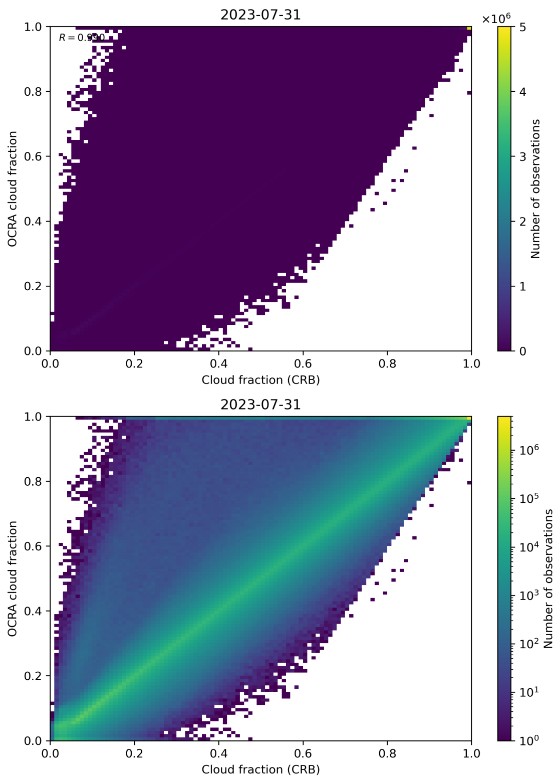
Figure 78: Scatter density plot of “Cloud fraction (CRB)” against “OCRA cloud fraction” for 2023-07-30 to 2023-08-01.
