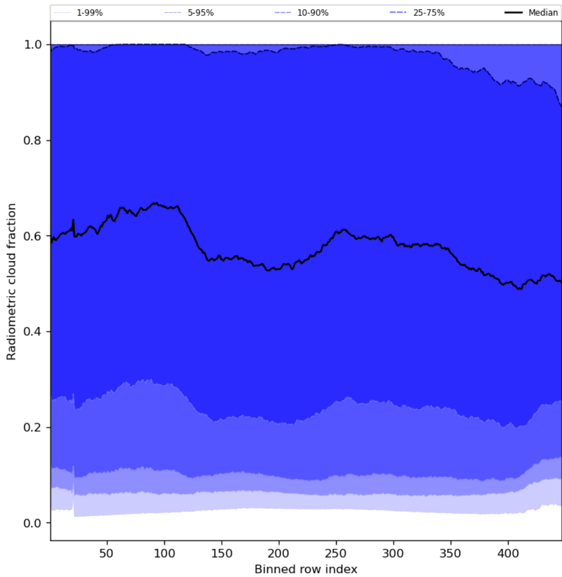
Figure 55: Along track statistics of “Radiometric cloud fraction” for 2023-07-30 to 2023-08-01
