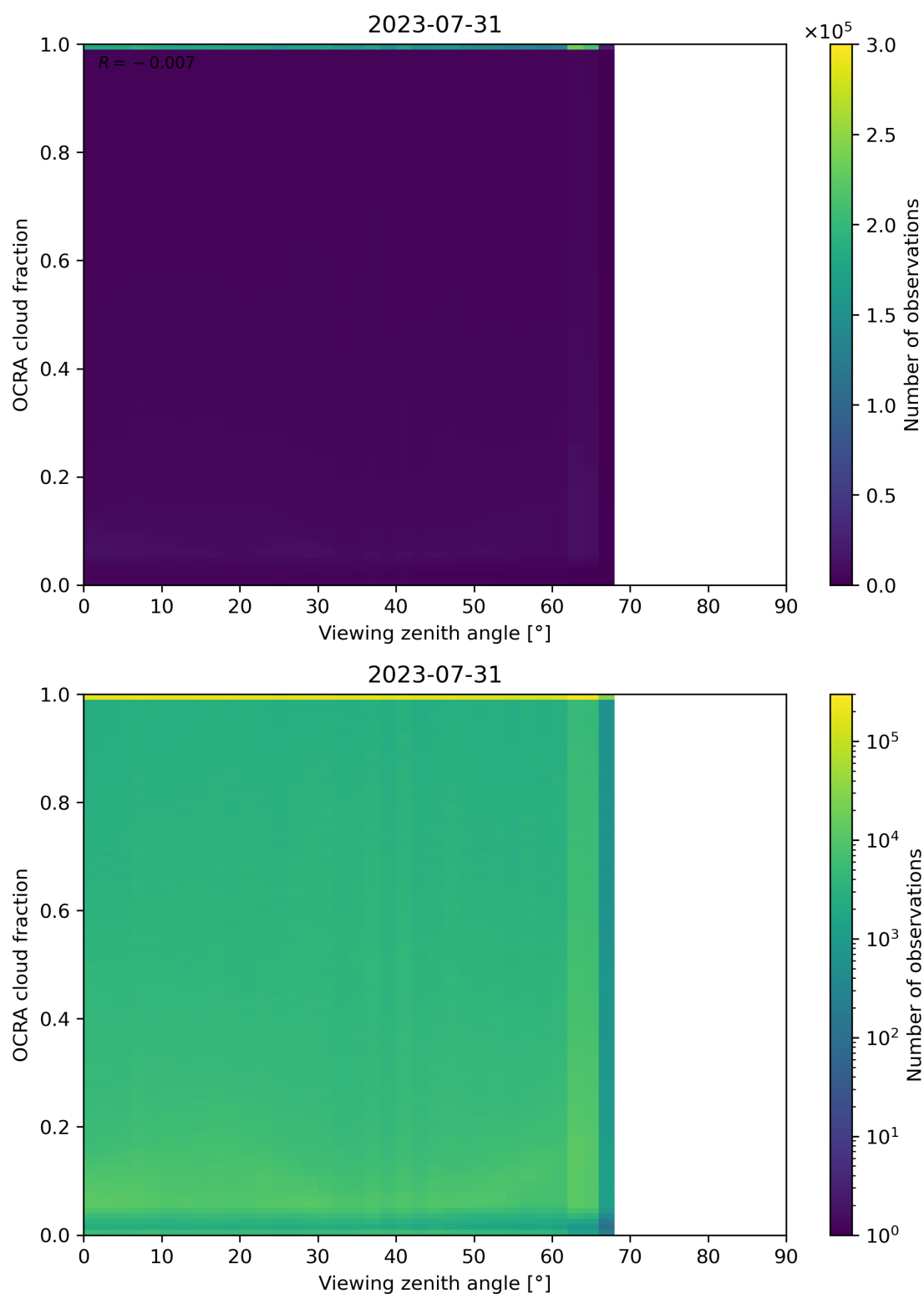
Figure 108: Scatter density plot of “Viewing zenith angle” against “OCRA cloud fraction” for 2023-07-30 to 2023-08-01.
