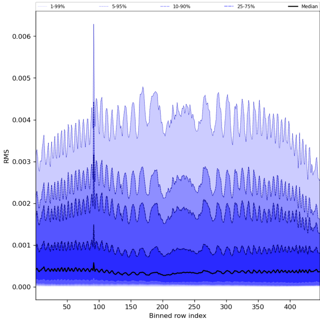
Figure 63: Along track statistics of “RMS” for 2023-07-30 to 2023-08-01
