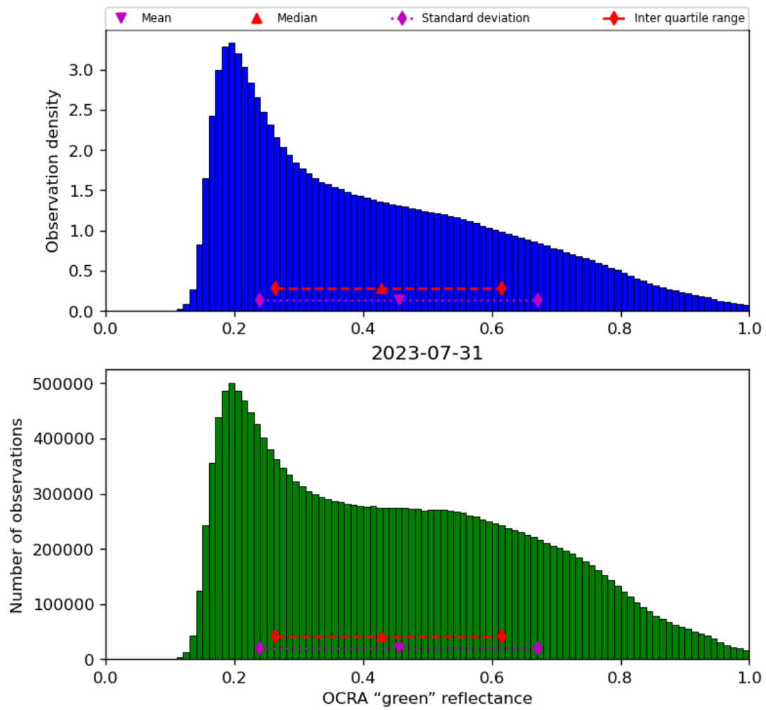
Figure 52: Histogram of “OCRA “green” reflectance” for 2023-07-30 to 2023-08-01
