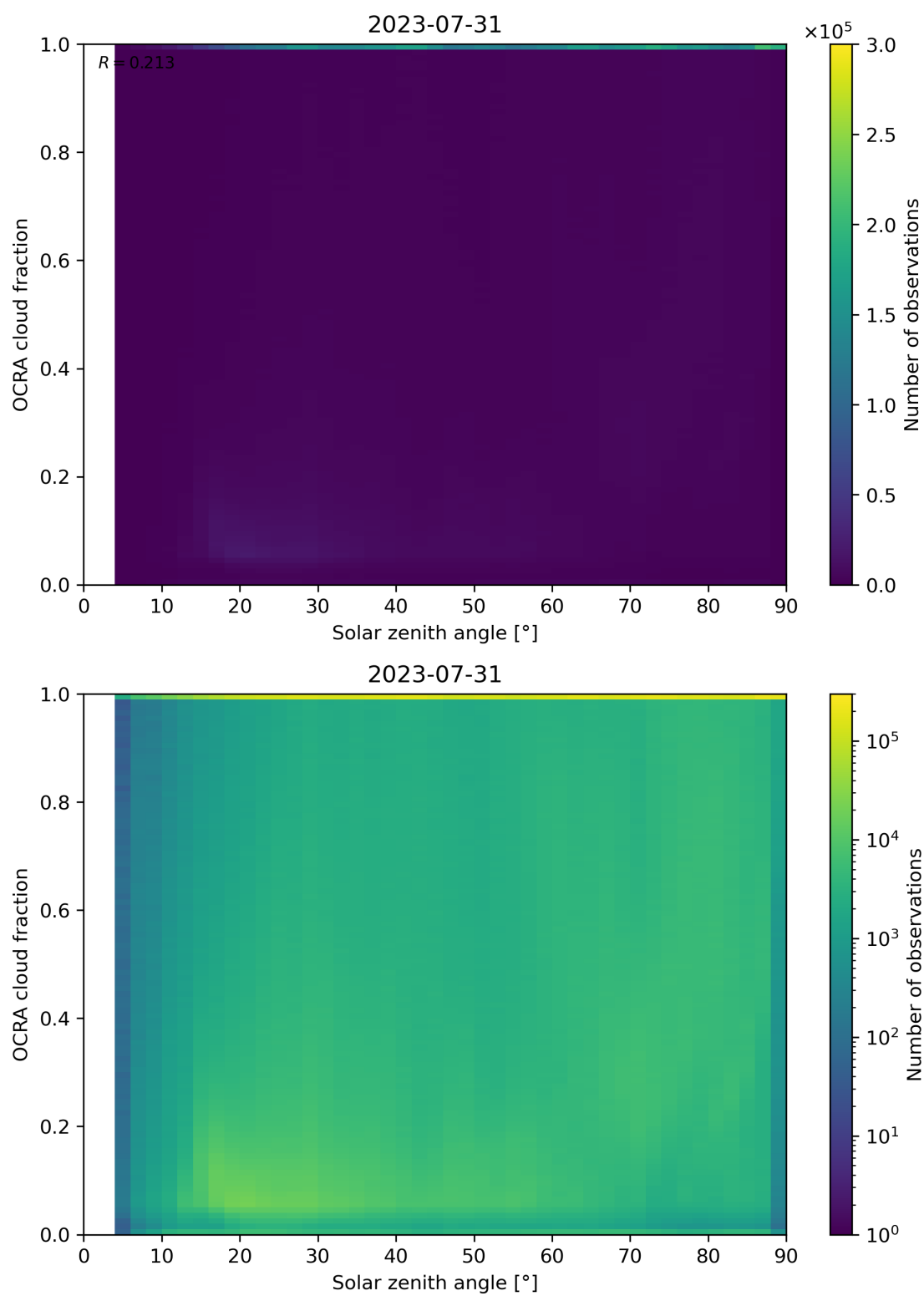
Figure 100: Scatter density plot of “Solar zenith angle” against “OCRA cloud fraction” for 2023-07-30 to 2023-08-01.
