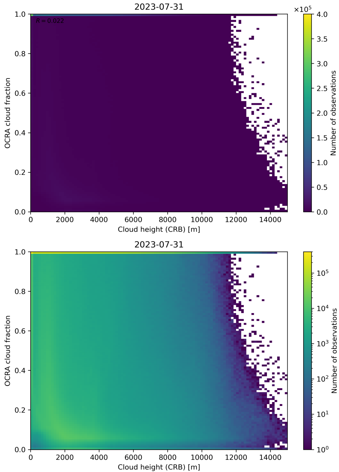
Figure 81: Scatter density plot of “Cloud height (CRB)” against “OCRA cloud fraction” for 2023-07-30 to 2023-08-01.
