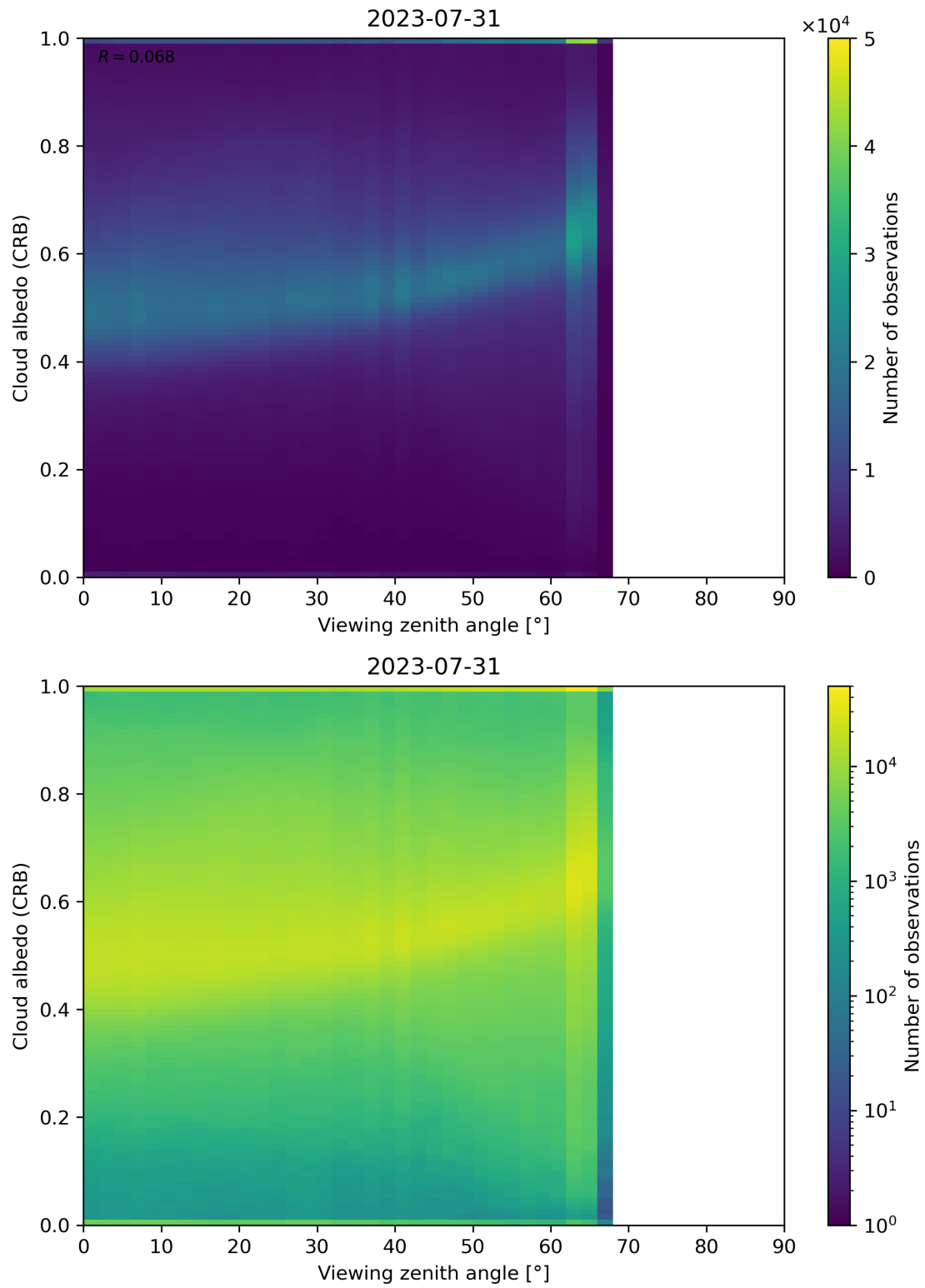
Figure 106: Scatter density plot of “Viewing zenith angle” against “Cloud albedo (CRB)” for 2023-07-30 to 2023-08-01.
