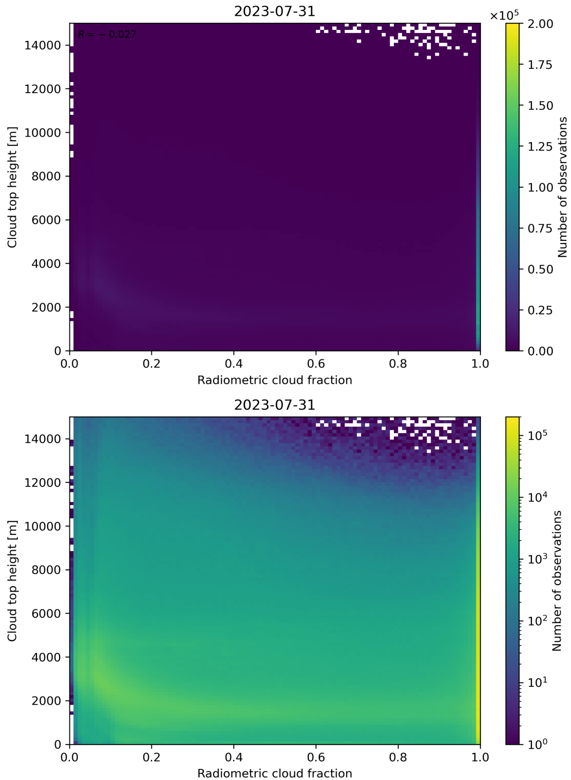
Figure 76: Scatter density plot of “Radiometric cloud fraction” against “Cloud top height” for 2023-07-30 to 2023-08-01.
