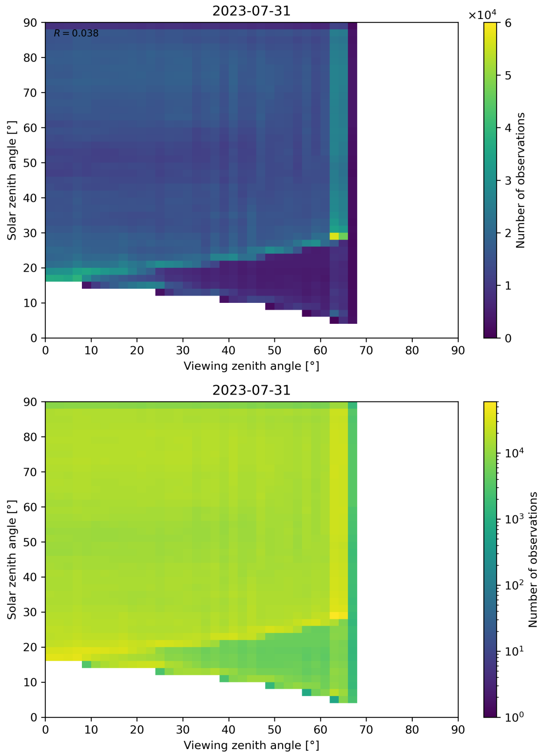
Figure 114: Scatter density plot of “Viewing zenith angle” against “Solar zenith angle” for 2023-07-30 to 2023-08-01.
