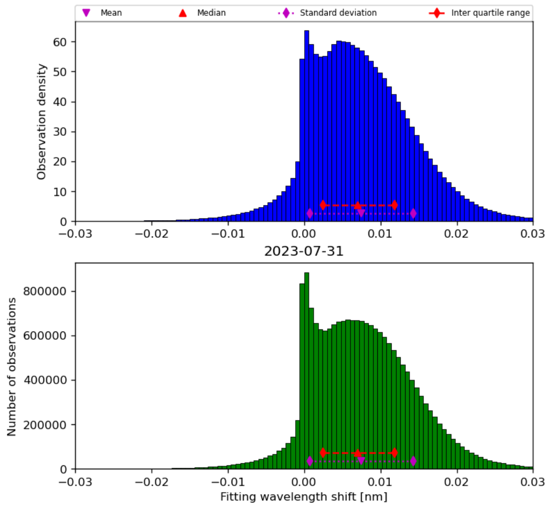
Figure 49: Histogram of “Fitting wavelength shift” for 2023-07-30 to 2023-08-01
