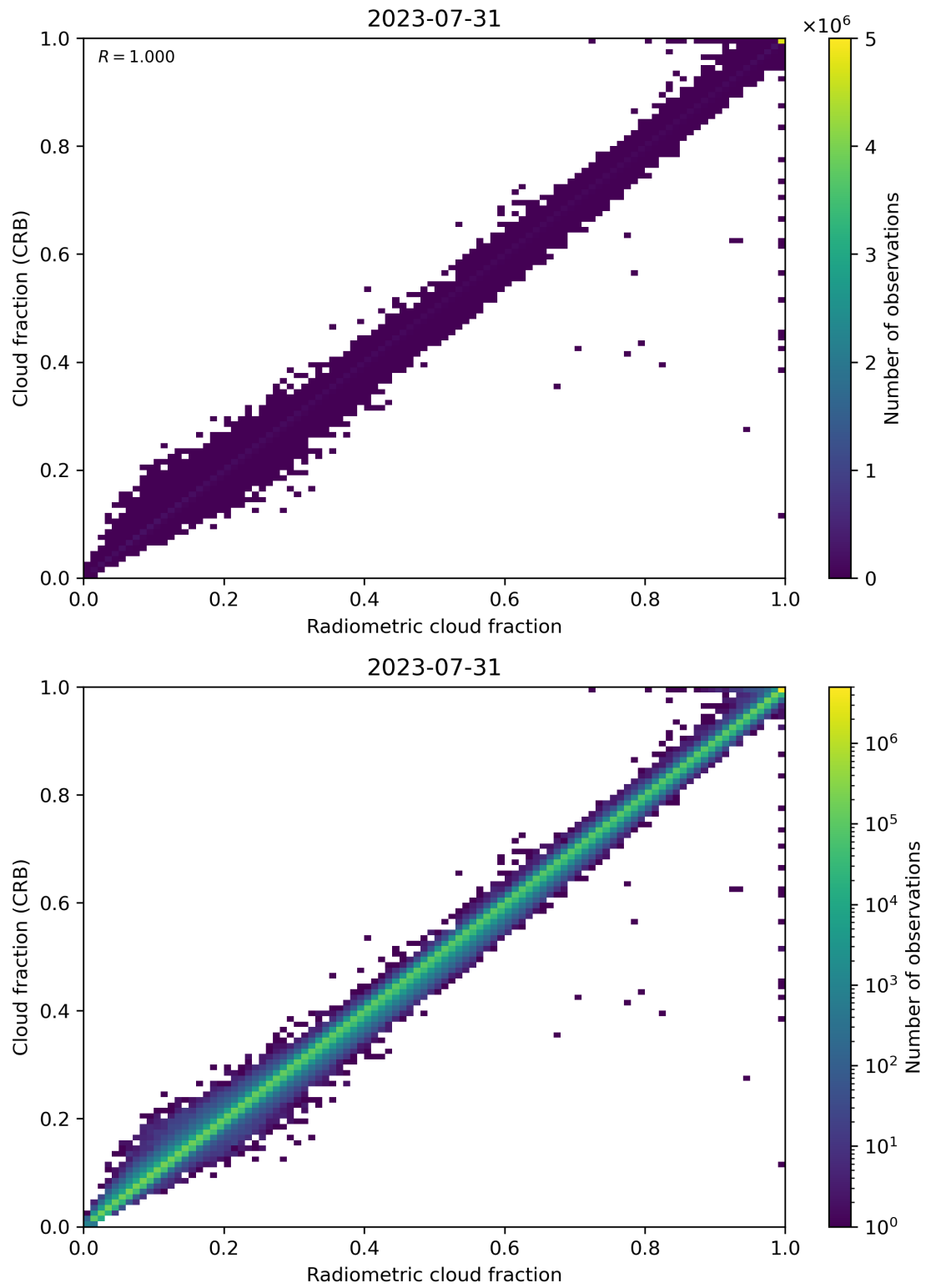
Figure 73: Scatter density plot of “Radiometric cloud fraction” against “Cloud fraction (CRB)” for 2023-07-30 to 2023-08-01.
