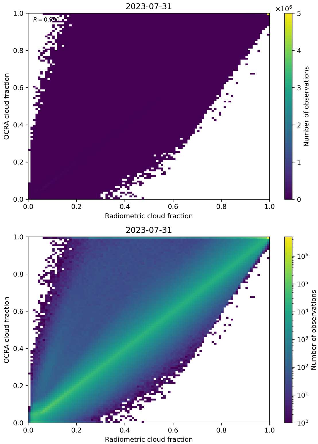
Figure 72: Scatter density plot of “Radiometric cloud fraction” against “OCRA cloud fraction” for 2023-07-30 to 2023-08-01.
