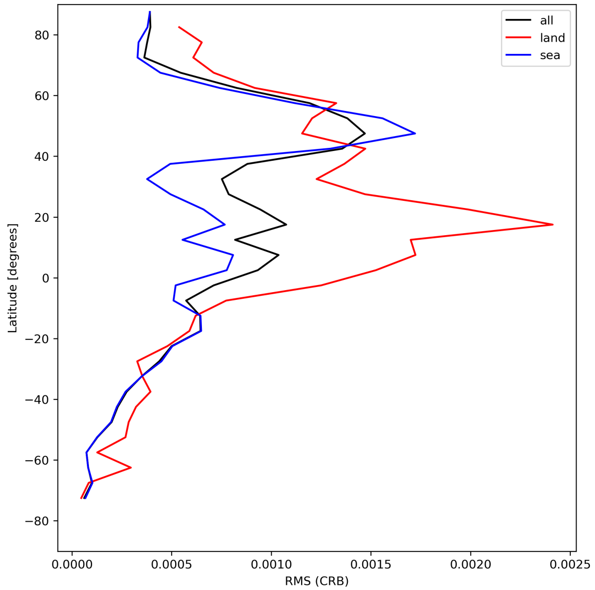
Figure 32: Zonal average of “RMS (CRB)” for 2023-07-30 to 2023-08-01.
