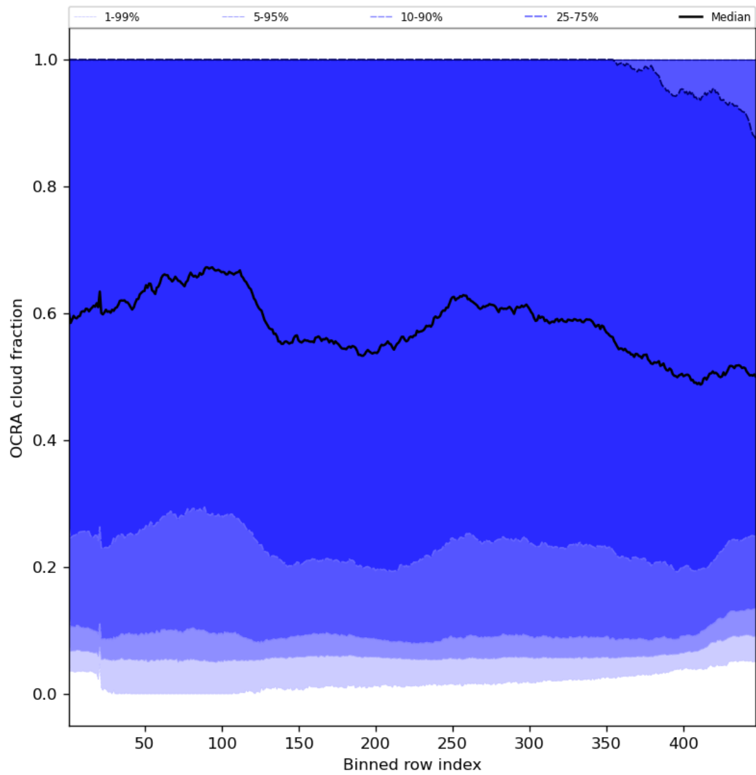
Figure 66: Along track statistics of “OCRA cloud fraction” for 2023-07-30 to 2023-08-01
