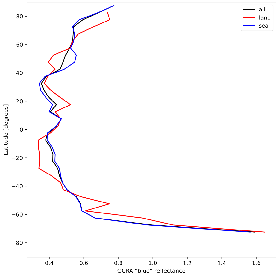
Figure 35: Zonal average of “OCRA “blue” reflectance” for 2023-07-30 to 2023-08-01.
