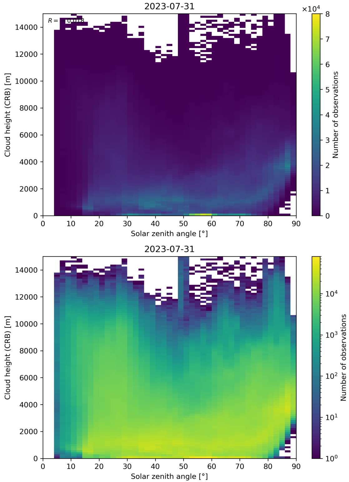
Figure 102: Scatter density plot of “Solar zenith angle” against “Cloud height (CRB)” for 2023-07-30 to 2023-08-01.
