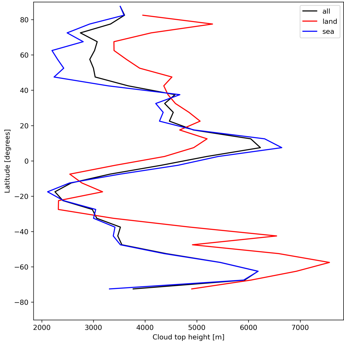
Figure 24: Zonal average of “Cloud top height” for 2023-07-30 to 2023-08-01.
