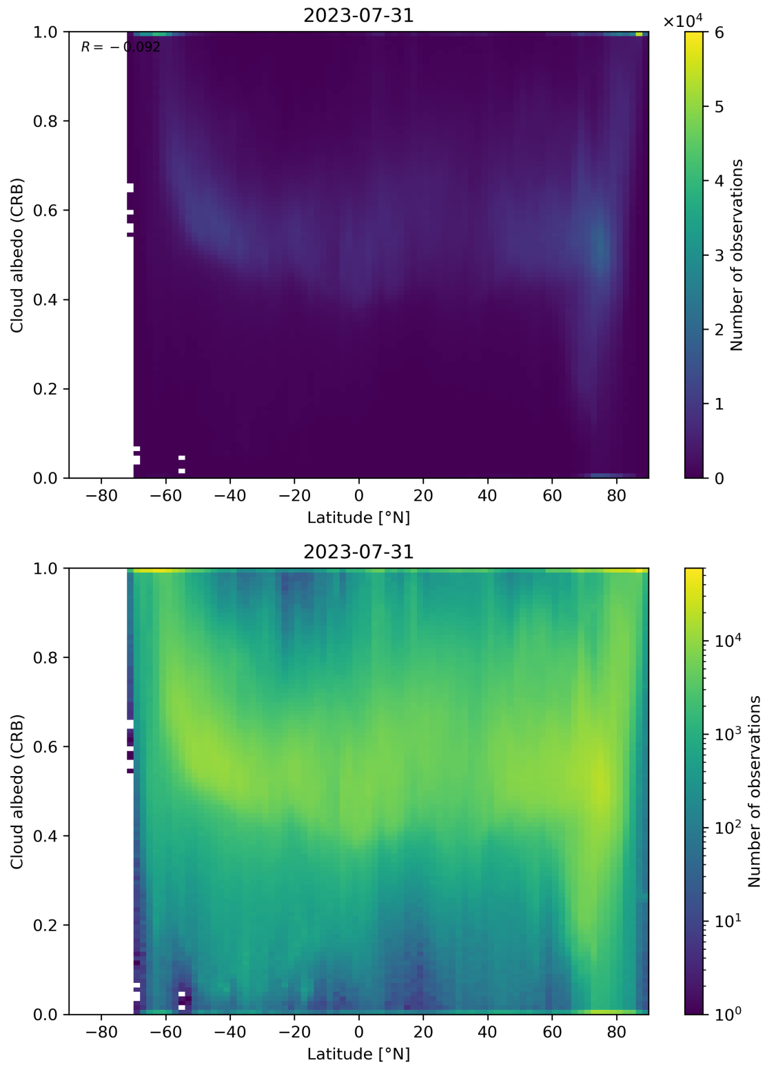
Figure 91: Scatter density plot of “Latitude” against “Cloud albedo (CRB)” for 2023-07-30 to 2023-08-01.
