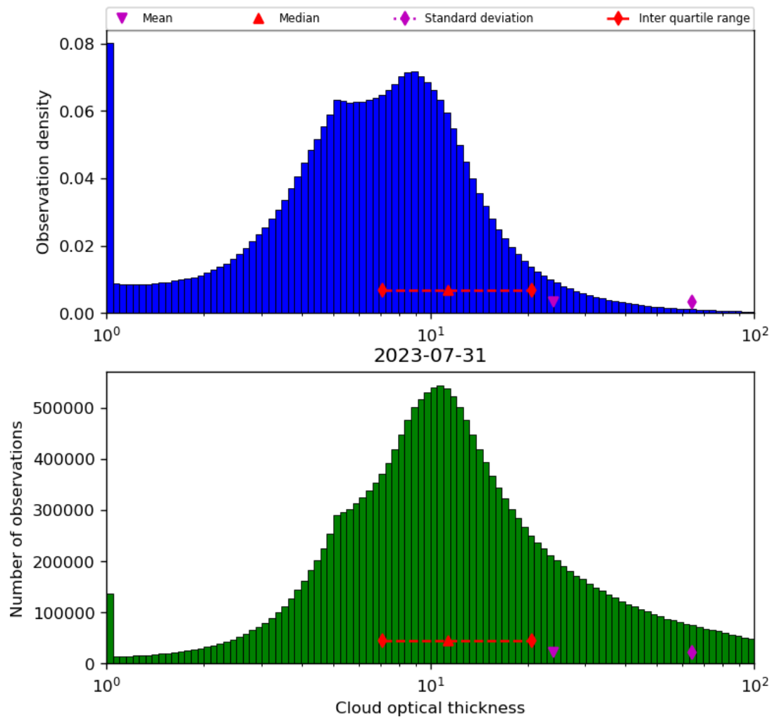
Figure 41: Histogram of “Cloud optical thickness” for 2023-07-30 to 2023-08-01
