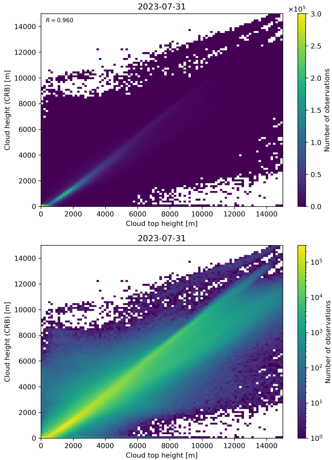
Figure 89: Scatter density plot of “Cloud top height” against “Cloud height (CRB)” for 2023-07-30 to 2023-08-01.
