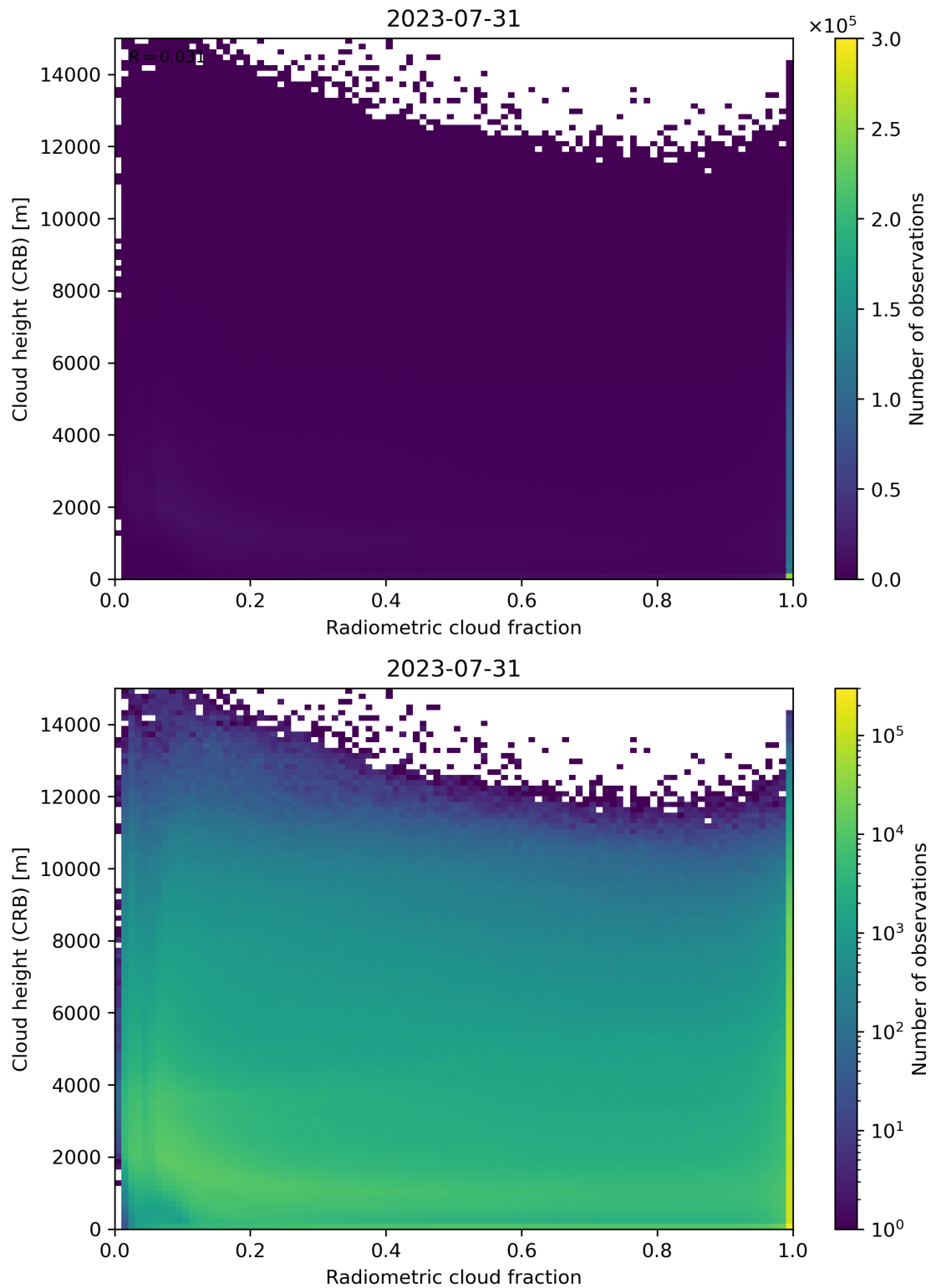
Figure 74: Scatter density plot of “Radiometric cloud fraction” against “Cloud height (CRB)” for 2023-07-30 to 2023-08-01.
