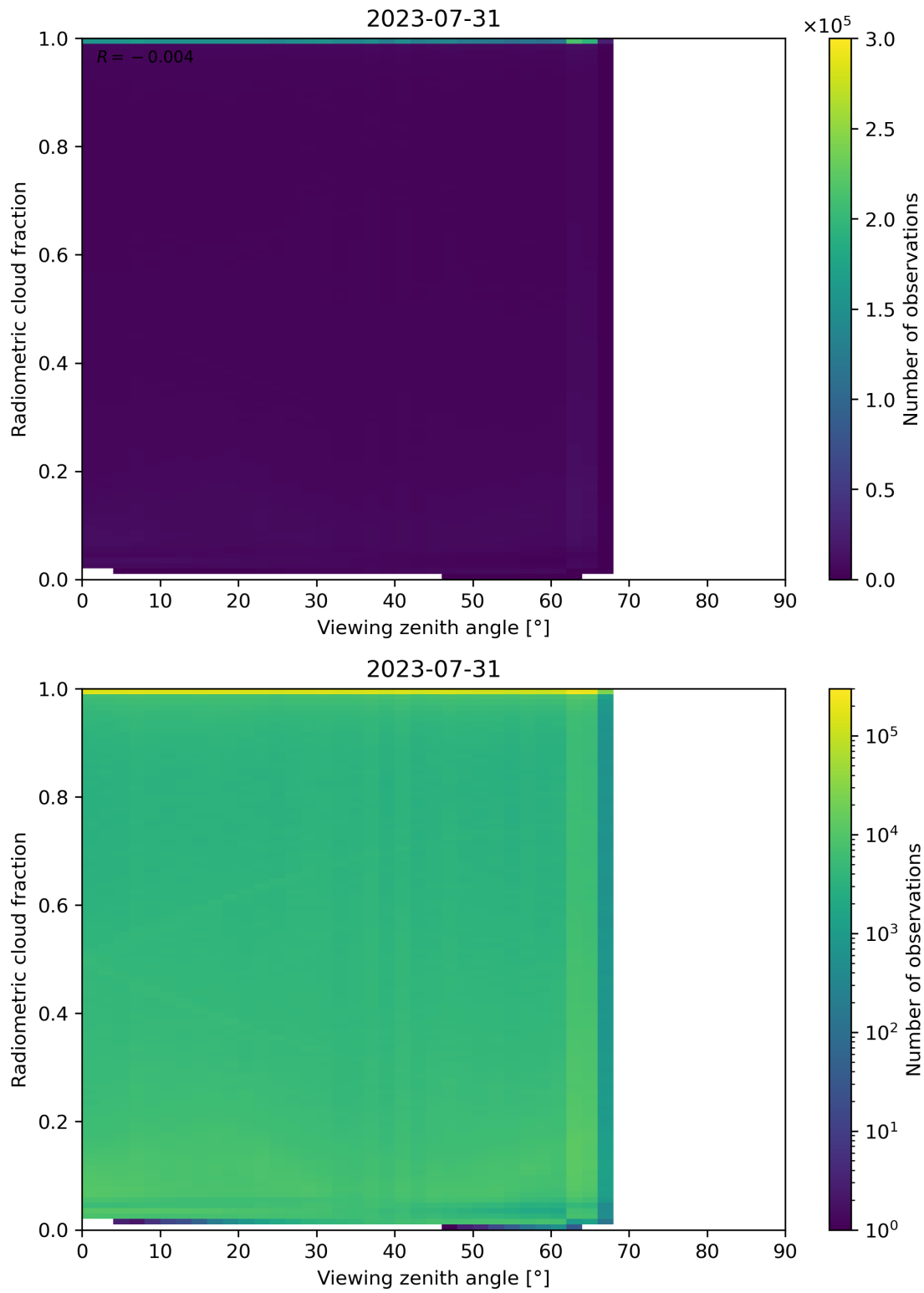
Figure 107: Scatter density plot of “Viewing zenith angle” against “Radiometric cloud fraction” for 2023-07-30 to 2023-08-01.
