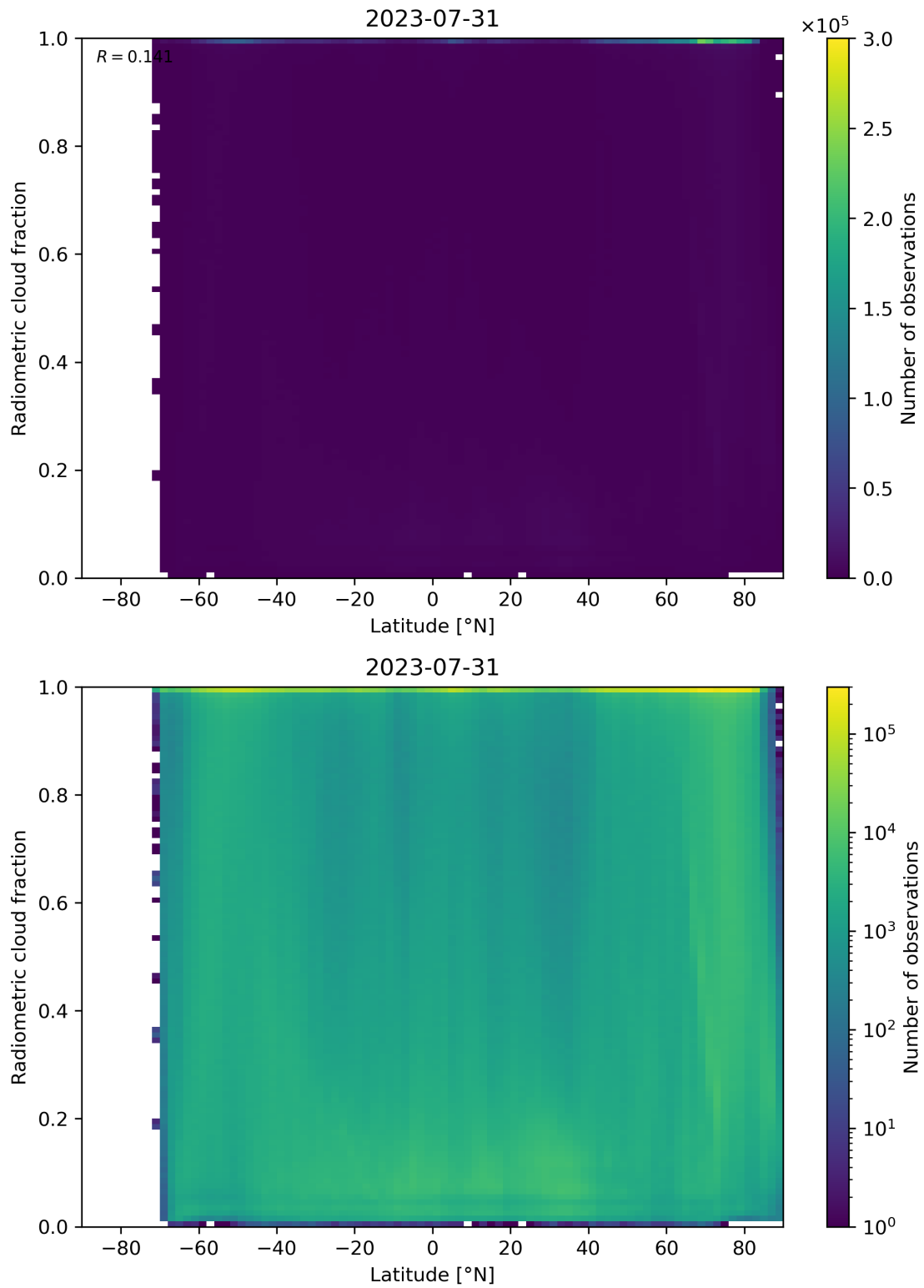
Figure 92: Scatter density plot of “Latitude” against “Radiometric cloud fraction” for 2023-07-30 to 2023-08-01.
