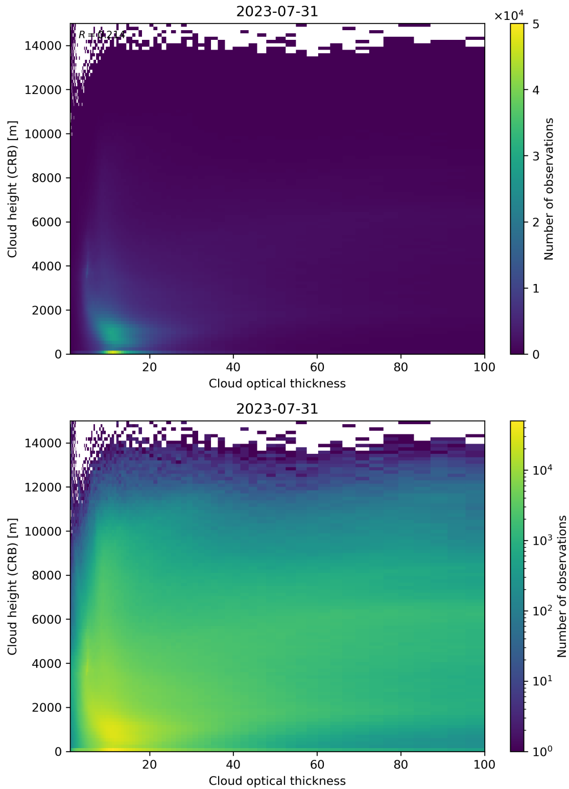
Figure 85: Scatter density plot of “Cloud optical thickness” against “Cloud height (CRB)” for 2023-07-30 to 2023-08-01.
