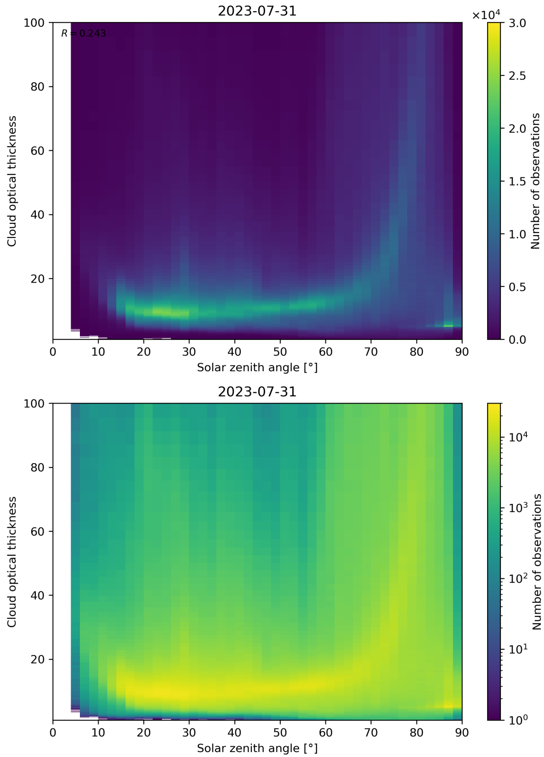
Figure 103: Scatter density plot of “Solar zenith angle” against “Cloud optical thickness” for 2023-07-30 to 2023-08-01.
