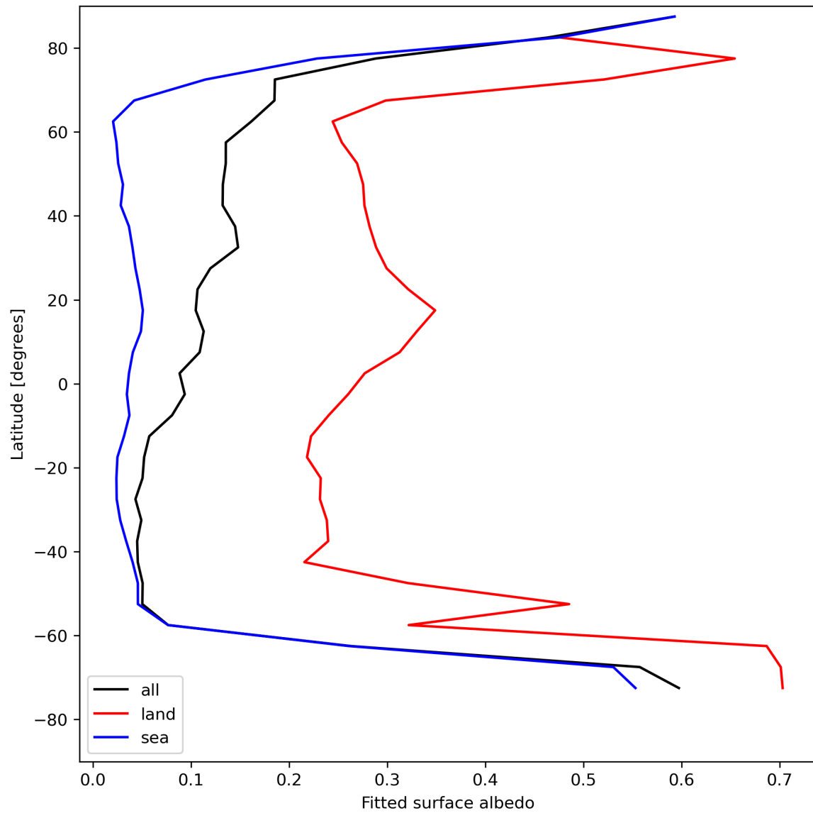
Figure 29: Zonal average of “Fitted surface albedo” for 2023-07-30 to 2023-08-01.
