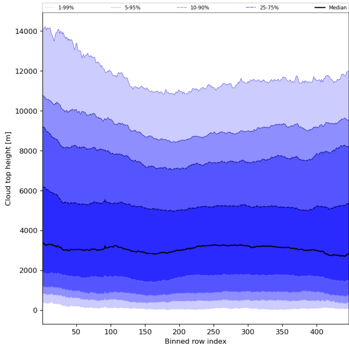
Figure 56: Along track statistics of “Cloud top height” for 2023-07-30 to 2023-08-01
