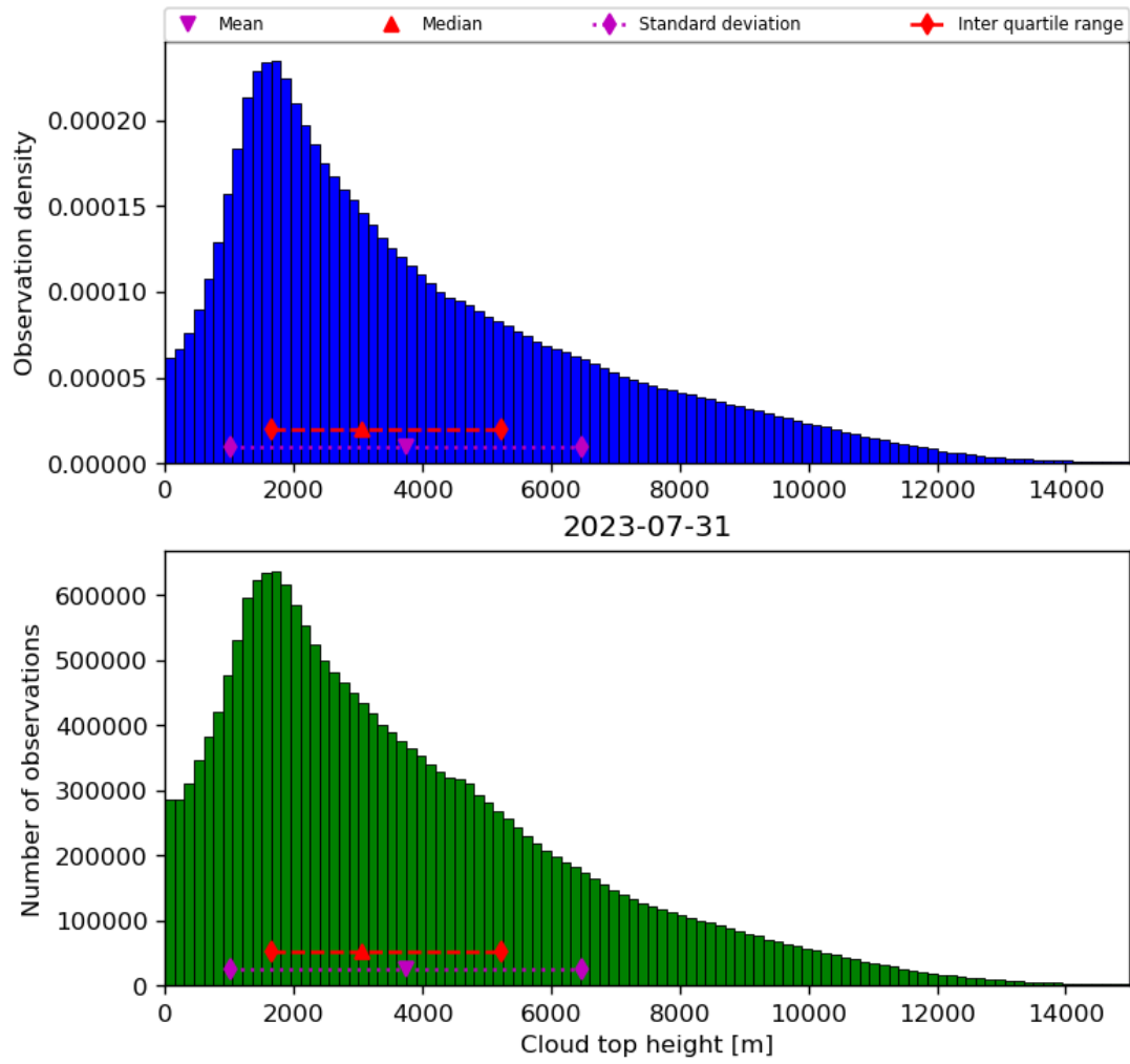
Figure 40: Histogram of “Cloud top height” for 2023-07-30 to 2023-08-01
