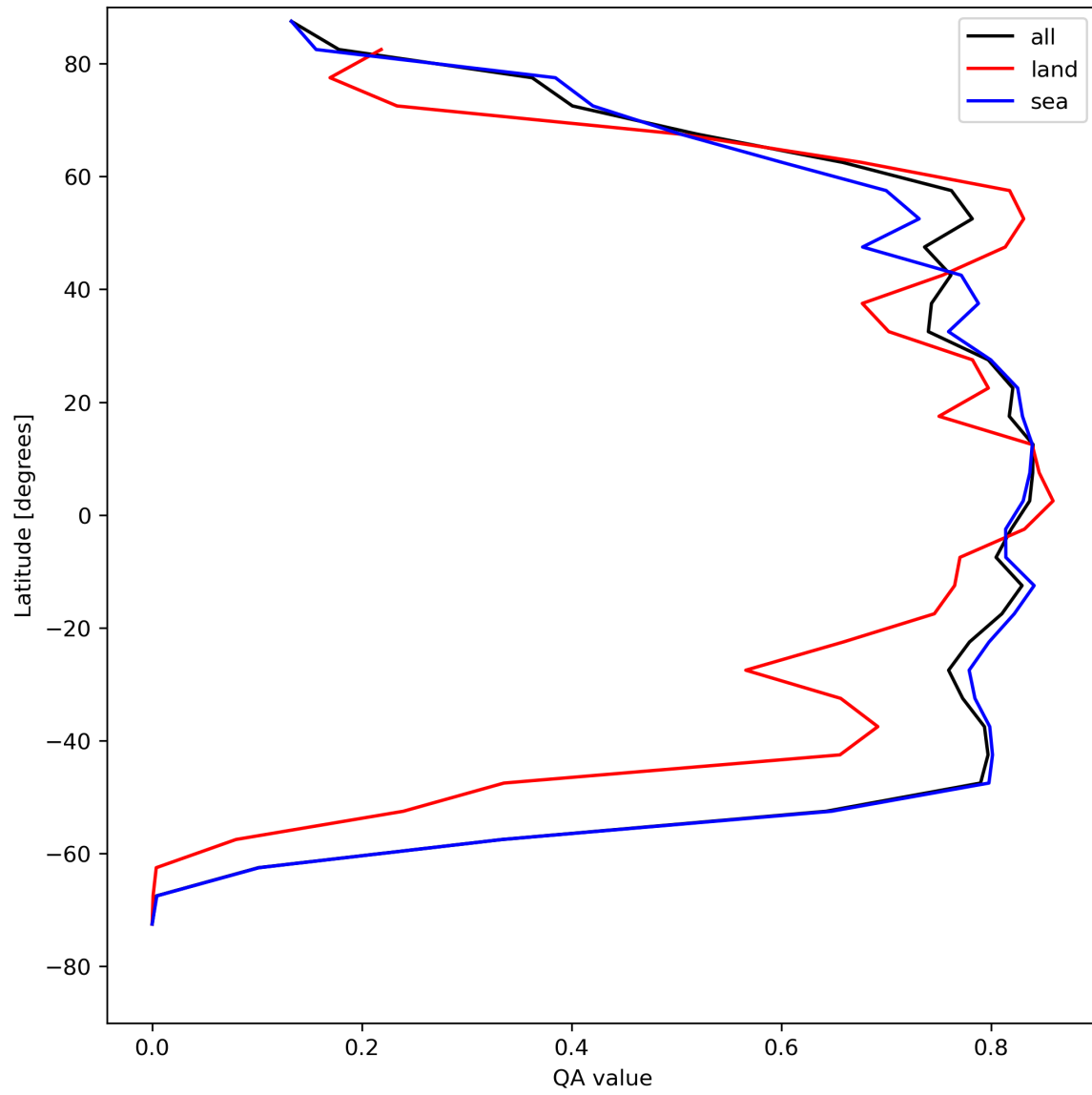
Figure 22: Zonal average of “QA value” for 2023-07-30 to 2023-08-01.
