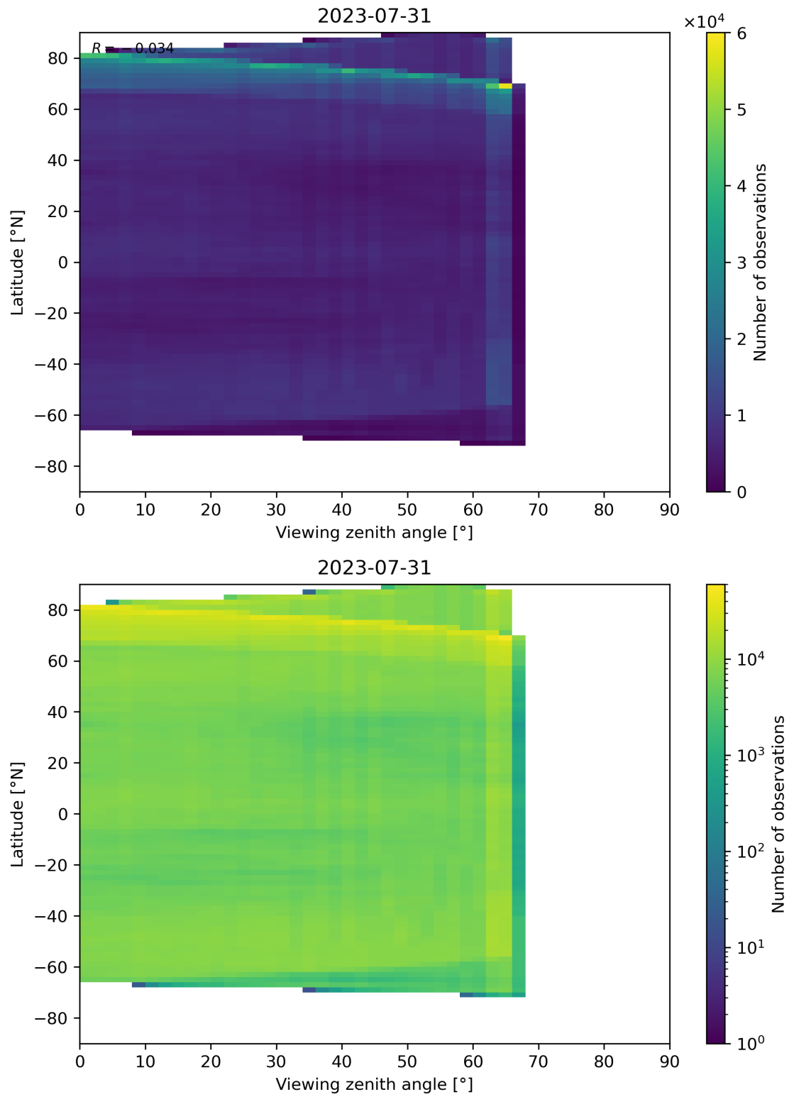
Figure 113: Scatter density plot of “Viewing zenith angle” against “Latitude” for 2023-07-30 to 2023-08-01.
