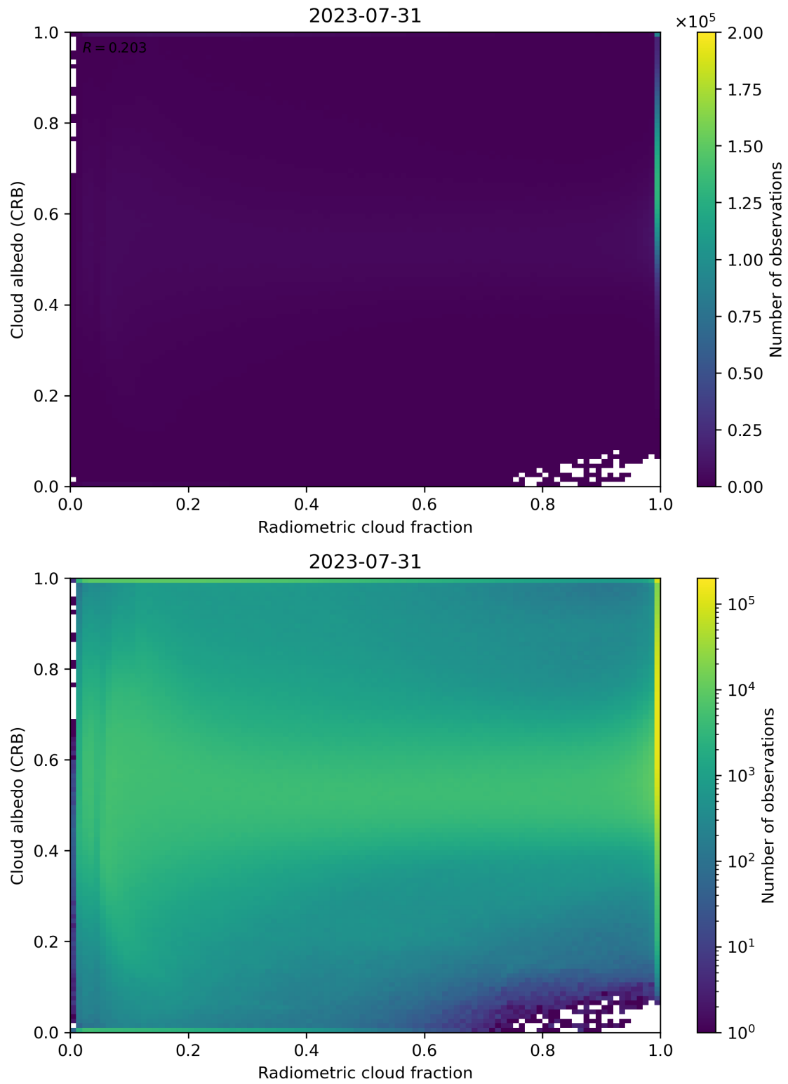
Figure 71: Scatter density plot of “Radiometric cloud fraction” against “Cloud albedo (CRB)” for 2023-07-30 to 2023-08-01.
