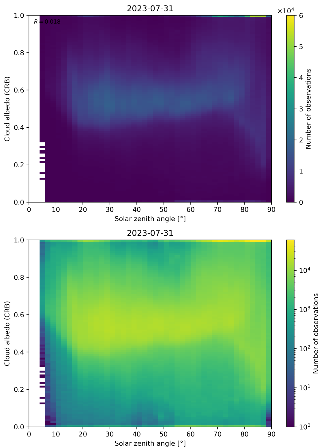
Figure 98: Scatter density plot of “Solar zenith angle” against “Cloud albedo (CRB)” for 2023-07-30 to 2023-08-01.
