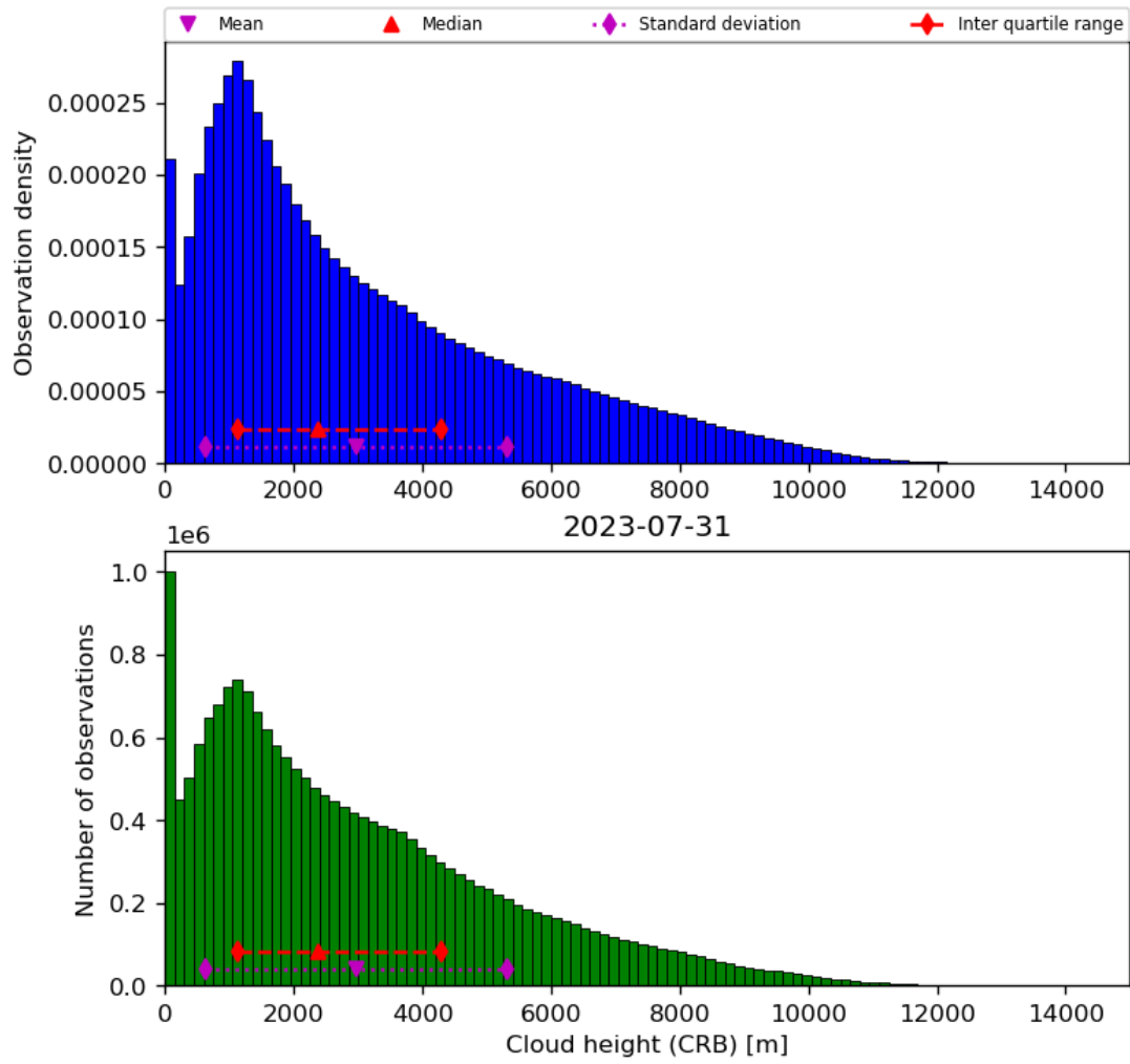
Figure 43: Histogram of “Cloud height (CRB)” for 2023-07-30 to 2023-08-01
