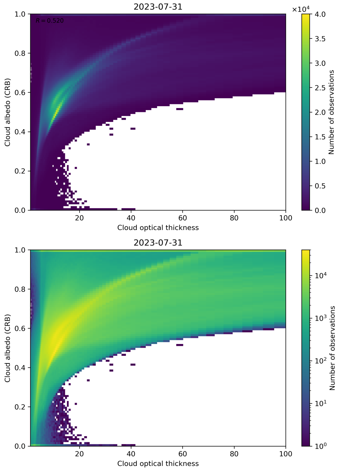
Figure 82: Scatter density plot of “Cloud optical thickness” against “Cloud albedo (CRB)” for 2023-07-30 to 2023-08-01.
