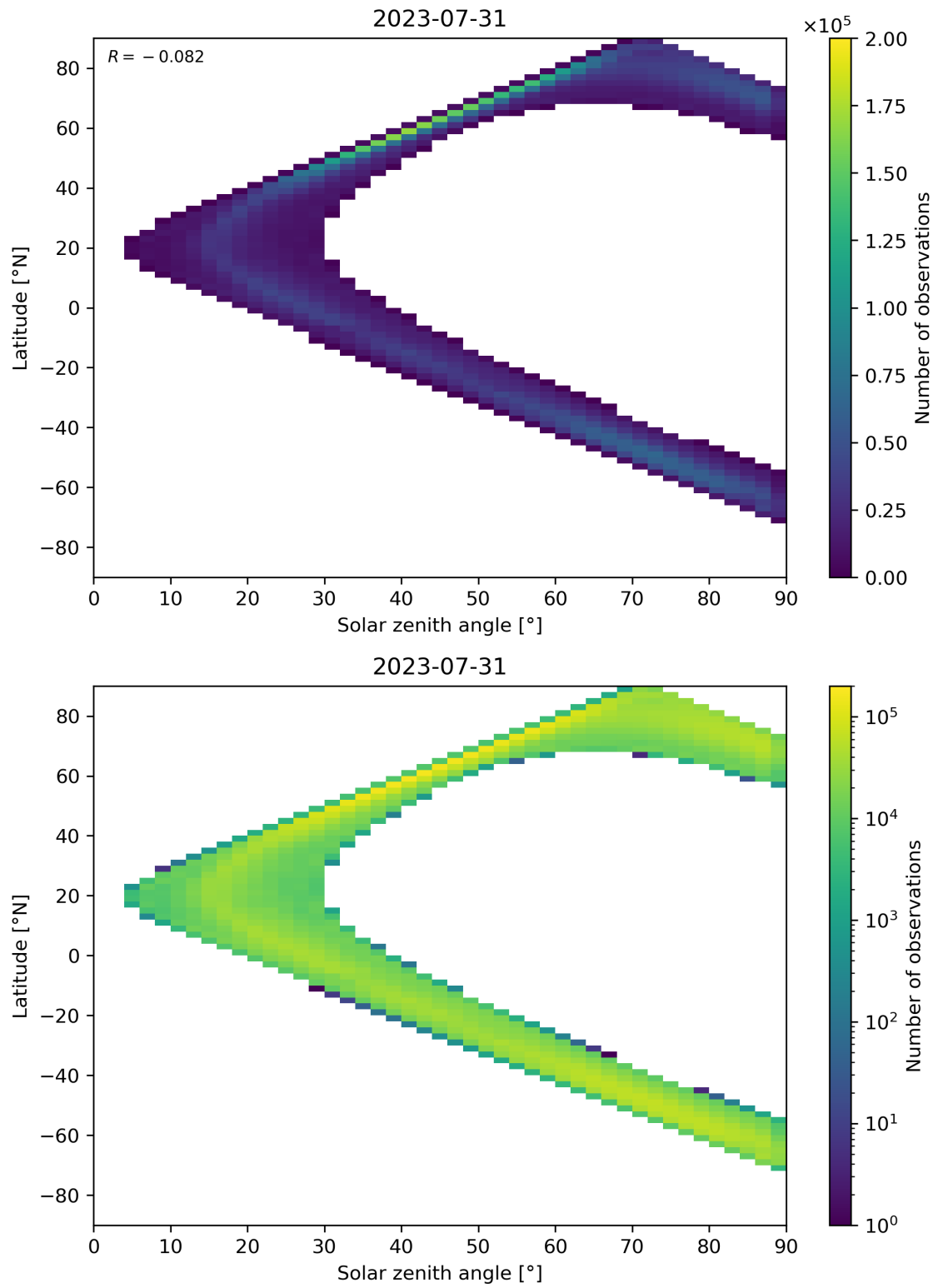
Figure 105: Scatter density plot of “Solar zenith angle” against “Latitude” for 2023-07-30 to 2023-08-01.
