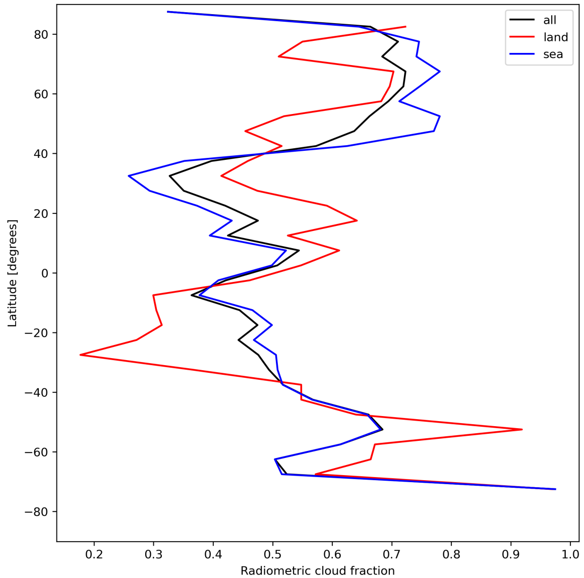
Figure 23: Zonal average of “Radiometric cloud fraction” for 2023-07-30 to 2023-08-01.
