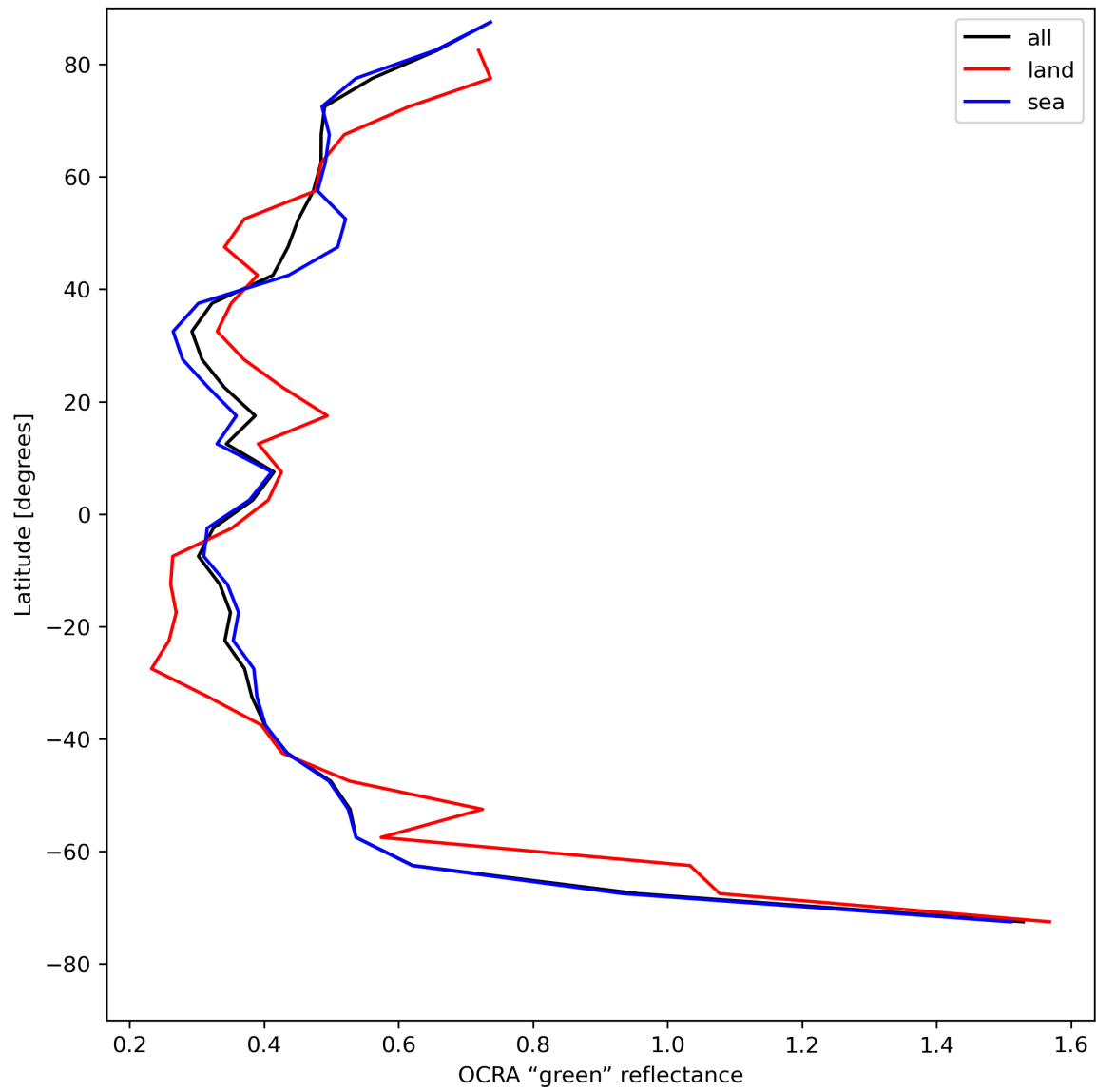
Figure 36: Zonal average of “OCRA “green” reflectance” for 2023-07-30 to 2023-08-01.
