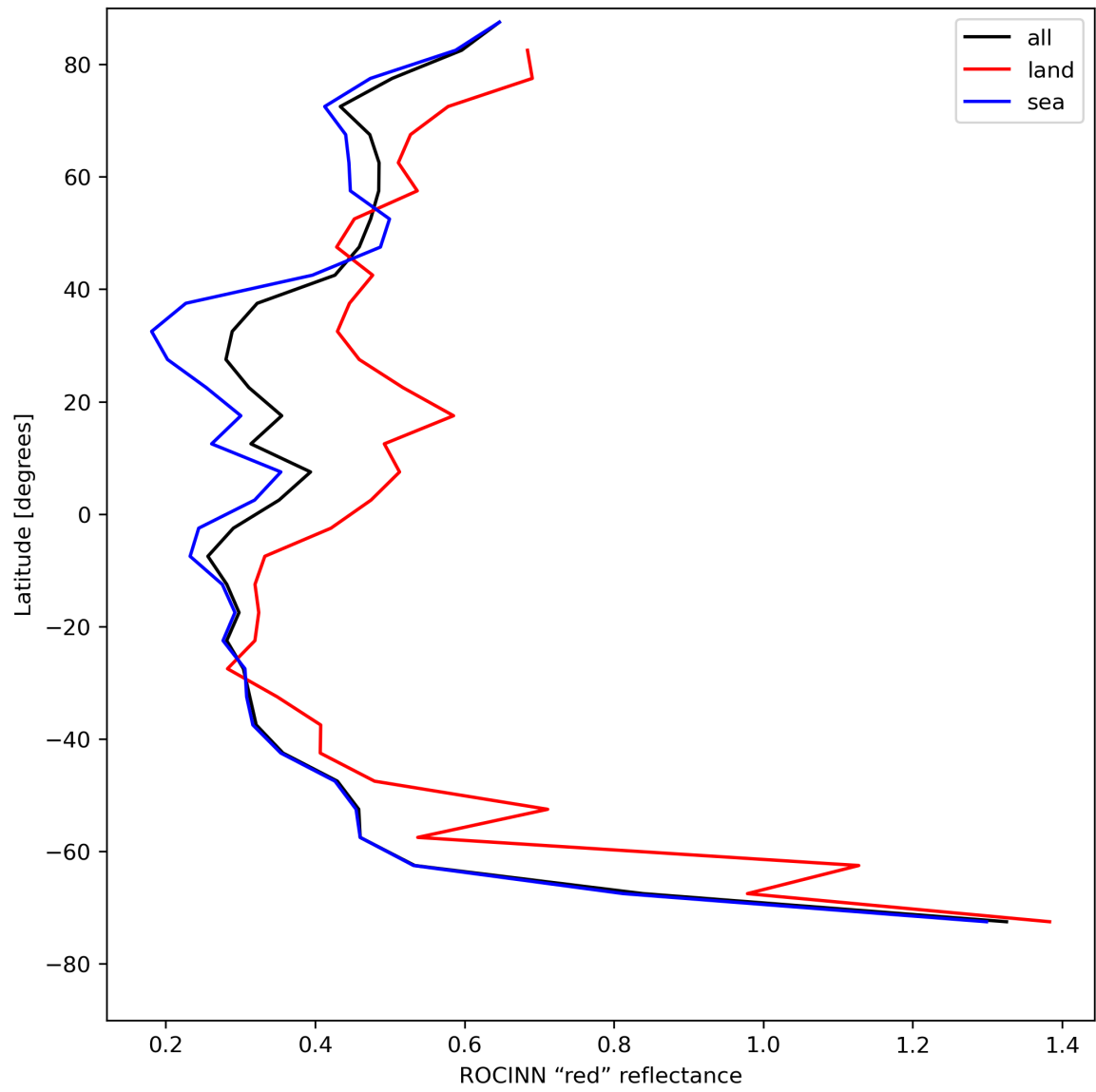
Figure 37: Zonal average of “ROCINN “red” reflectance” for 2023-07-30 to 2023-08-01.
