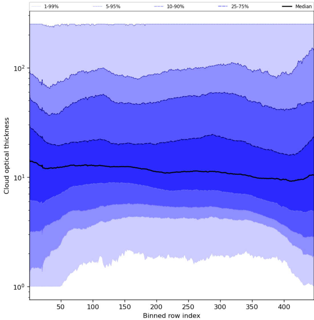
Figure 57: Along track statistics of “Cloud optical thickness” for 2023-07-30 to 2023-08-01
