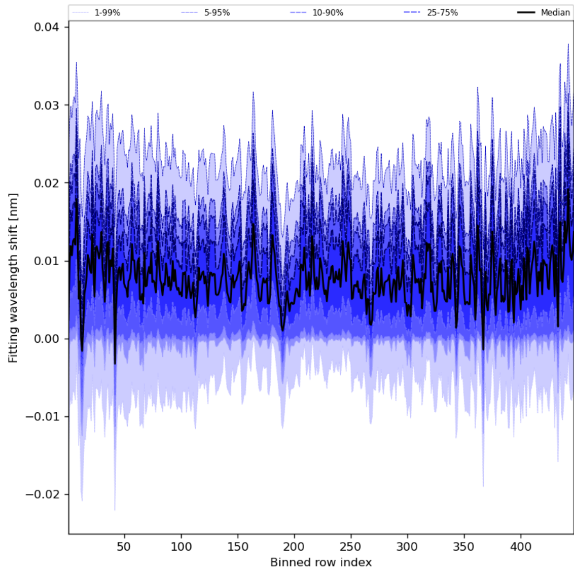
Figure 65: Along track statistics of “Fitting wavelength shift” for 2023-07-30 to 2023-08-01
