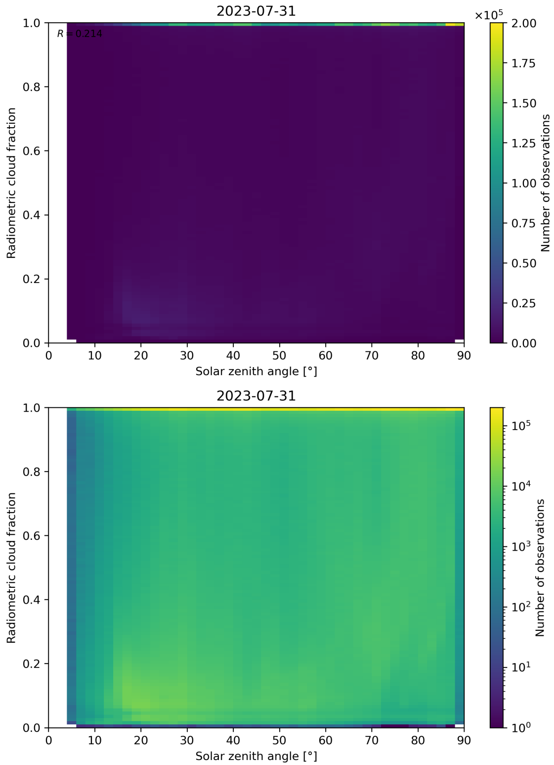
Figure 99: Scatter density plot of “Solar zenith angle” against “Radiometric cloud fraction” for 2023-07-30 to 2023-08-01.
