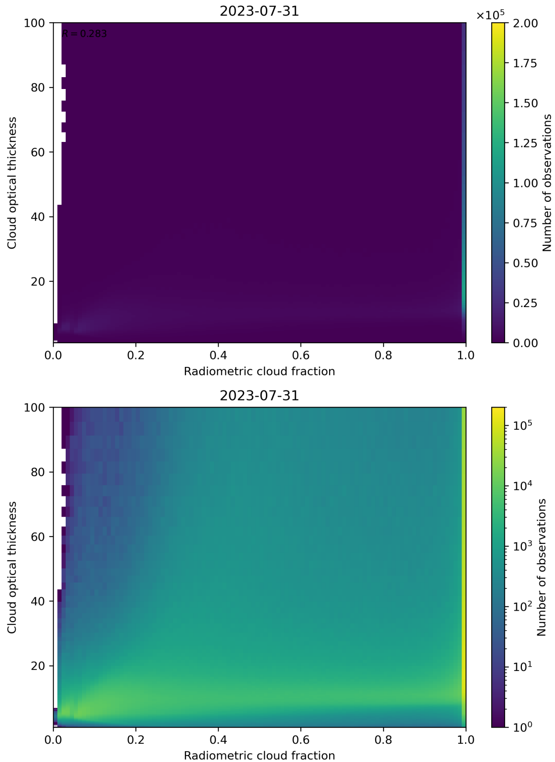
Figure 75: Scatter density plot of “Radiometric cloud fraction” against “Cloud optical thickness” for 2023-07-30 to 2023-08-01.
