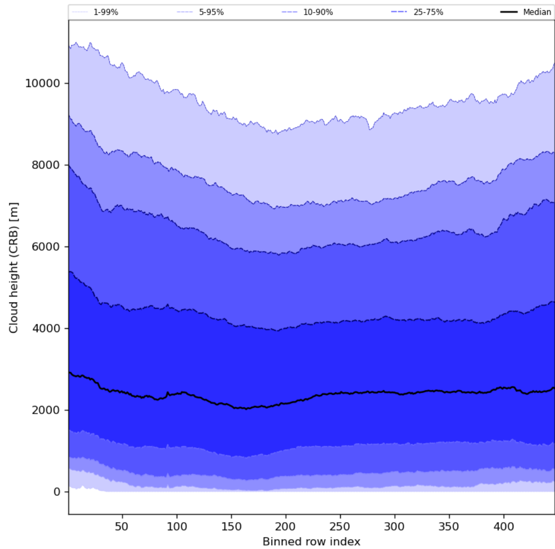
Figure 59: Along track statistics of “Cloud height (CRB)” for 2023-07-30 to 2023-08-01
