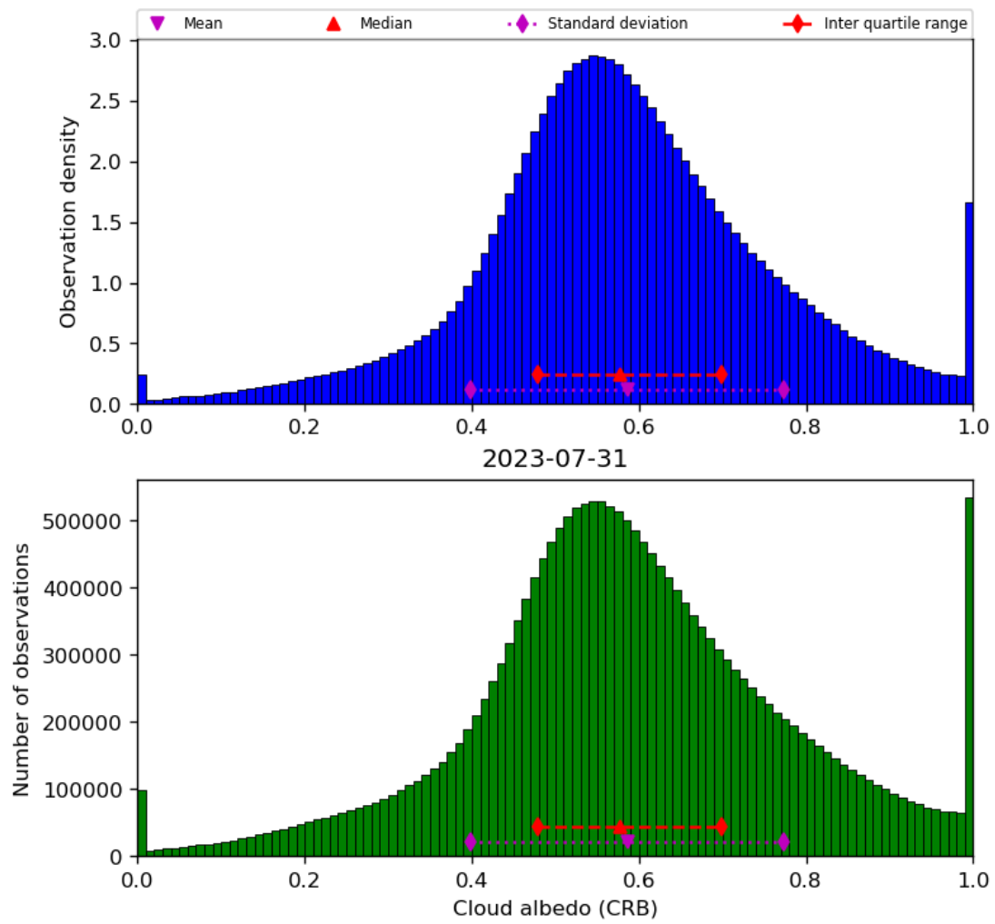
Figure 44: Histogram of “Cloud albedo (CRB)” for 2023-07-30 to 2023-08-01
