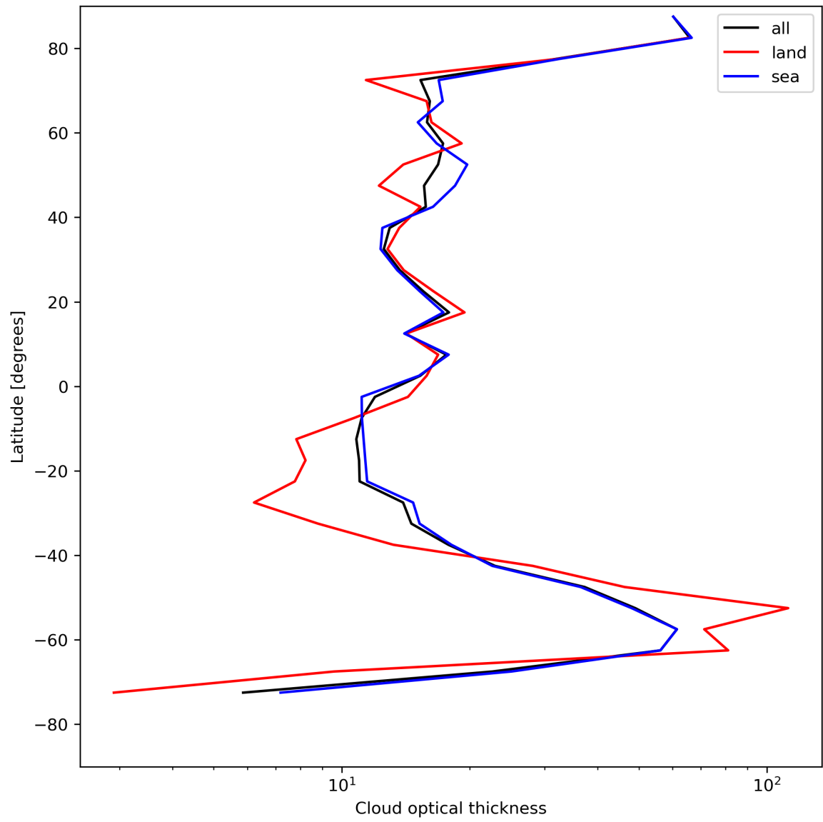
Figure 25: Zonal average of “Cloud optical thickness” for 2023-07-30 to 2023-08-01.
