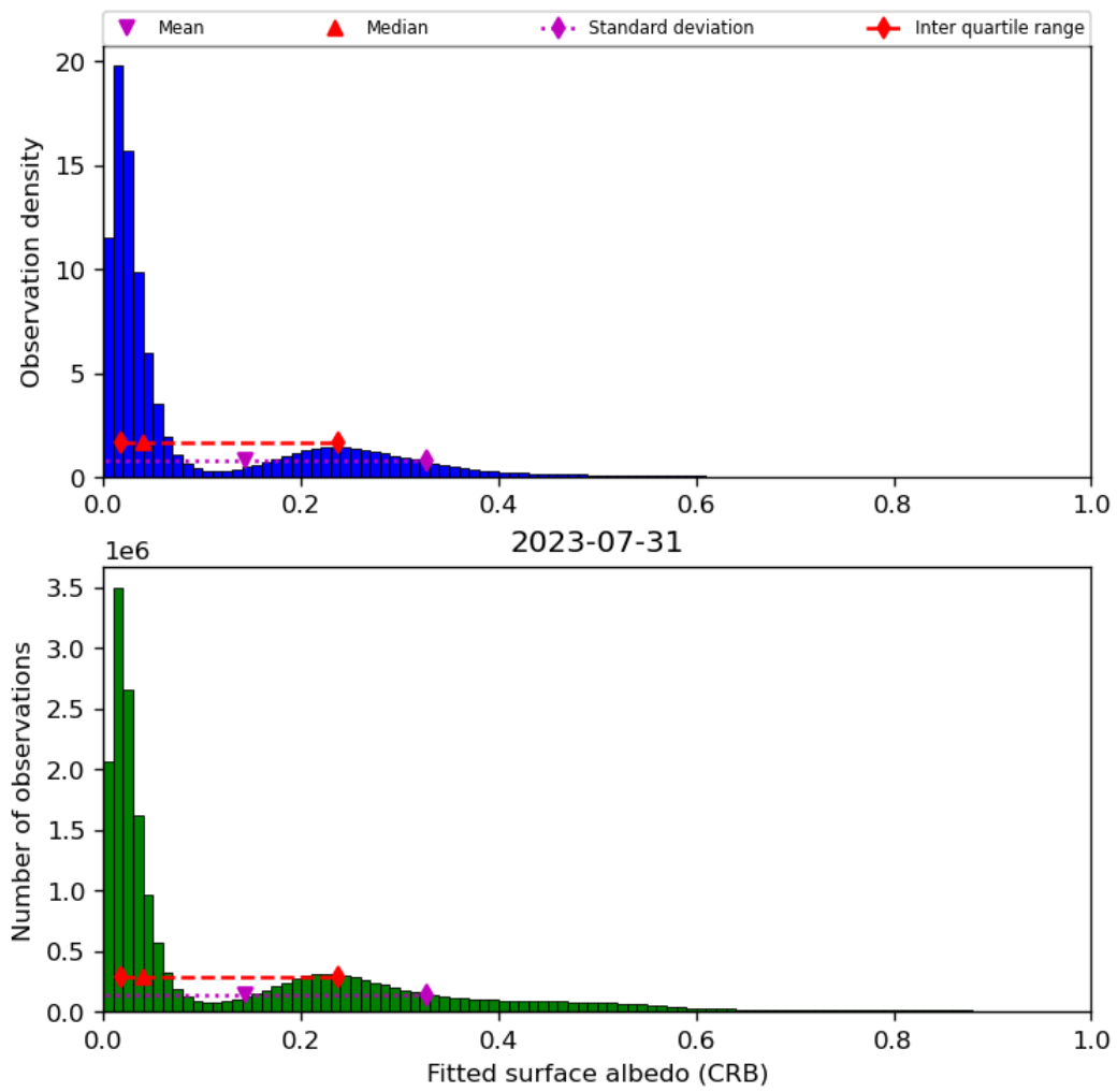
Figure 46: Histogram of “Fitted surface albedo (CRB)” for 2023-07-30 to 2023-08-01
