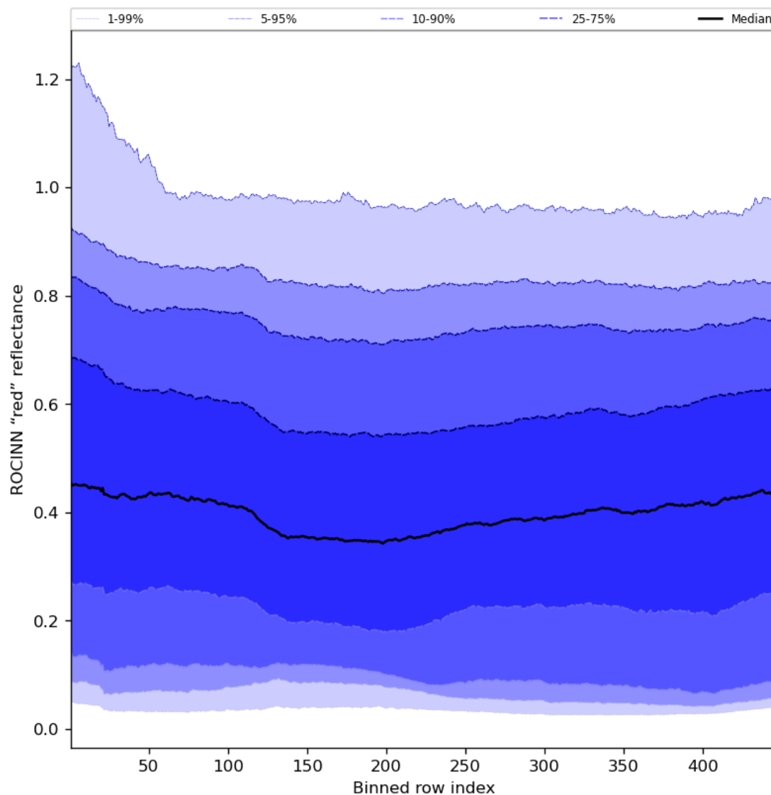
Figure 69: Along track statistics of "ROCINN "red" reflectance" for 2023-07-30 to 2023-08-01
