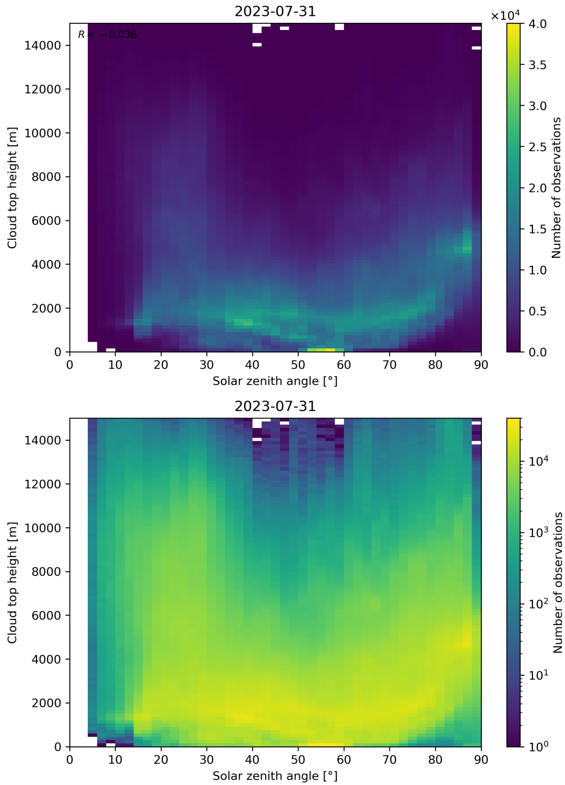
Figure 104: Scatter density plot of “Solar zenith angle” against “Cloud top height” for 2023-07-30 to 2023-08-01.
