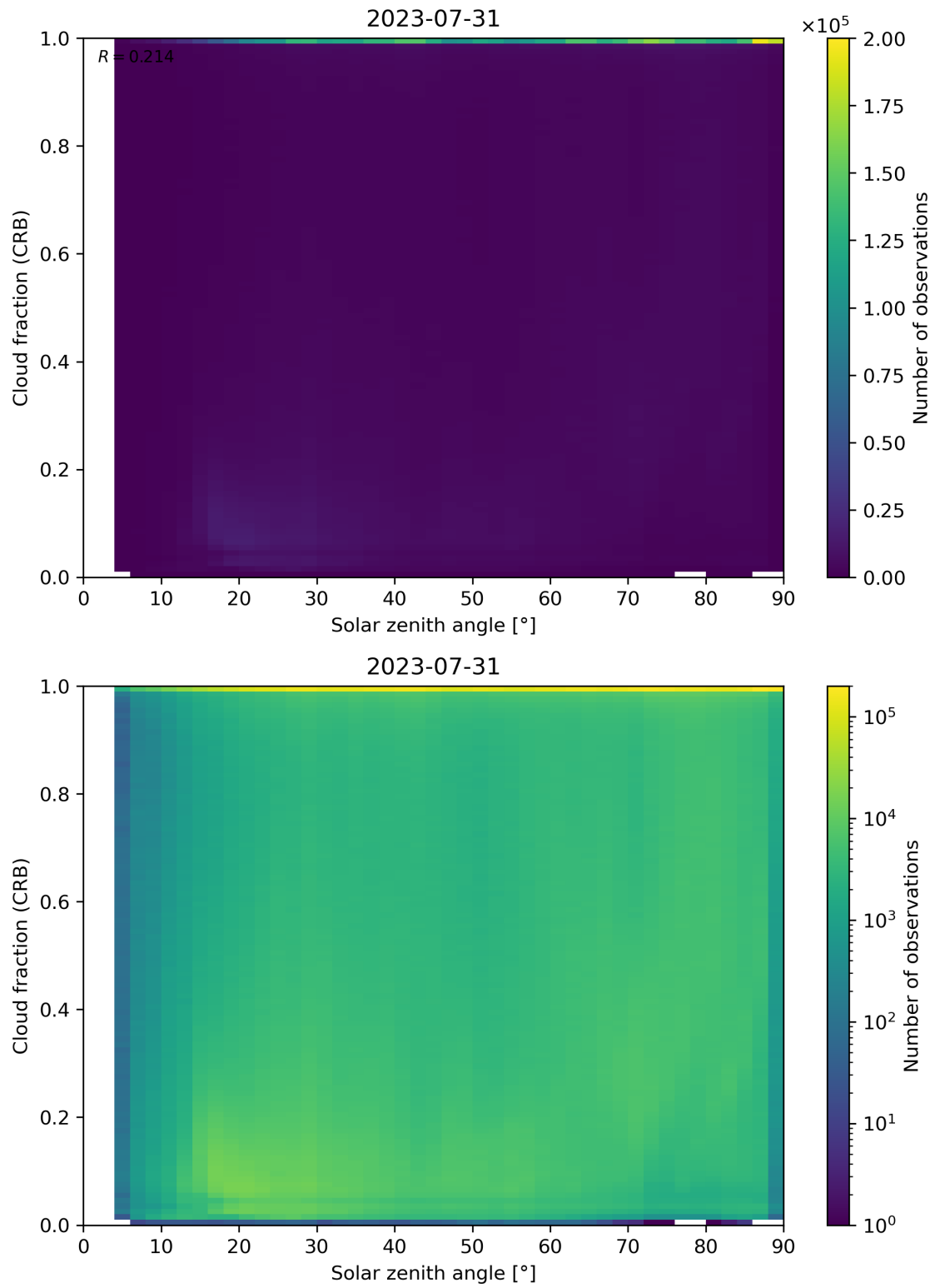
Figure 101: Scatter density plot of “Solar zenith angle” against “Cloud fraction (CRB)” for 2023-07-30 to 2023-08-01.
