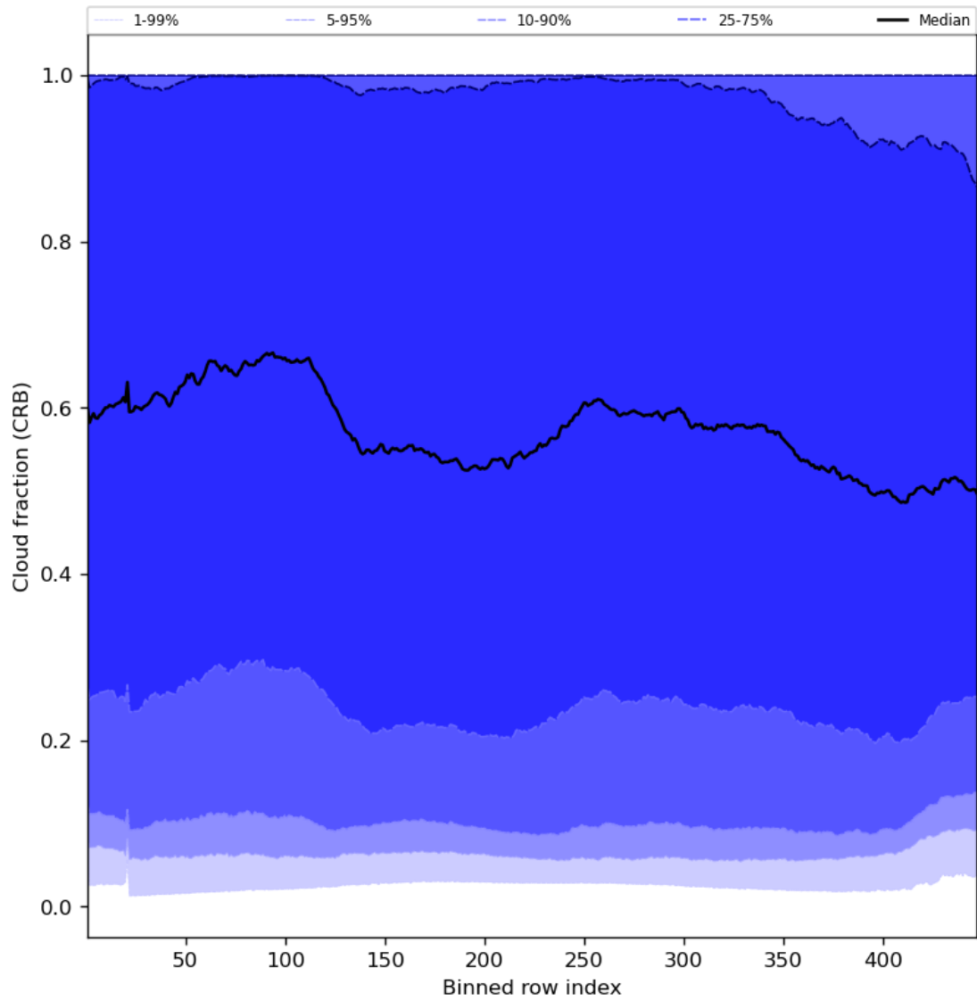
Figure 58: Along track statistics of “Cloud fraction (CRB)” for 2023-07-30 to 2023-08-01
