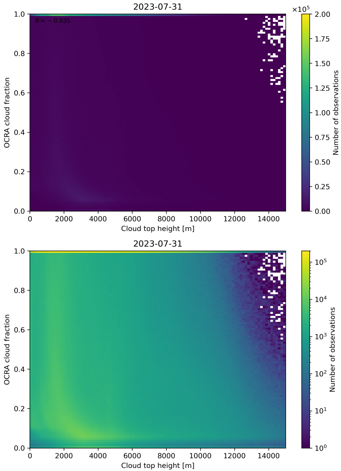
Figure 87: Scatter density plot of “Cloud top height” against “OCRA cloud fraction” for 2023-07-30 to 2023-08-01.
