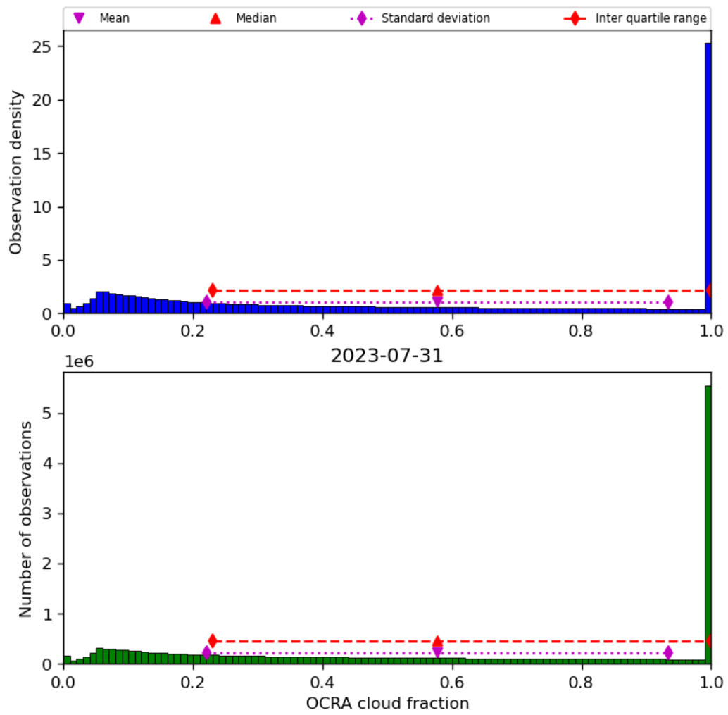
Figure 50: Histogram of “OCRA cloud fraction” for 2023-07-30 to 2023-08-01
