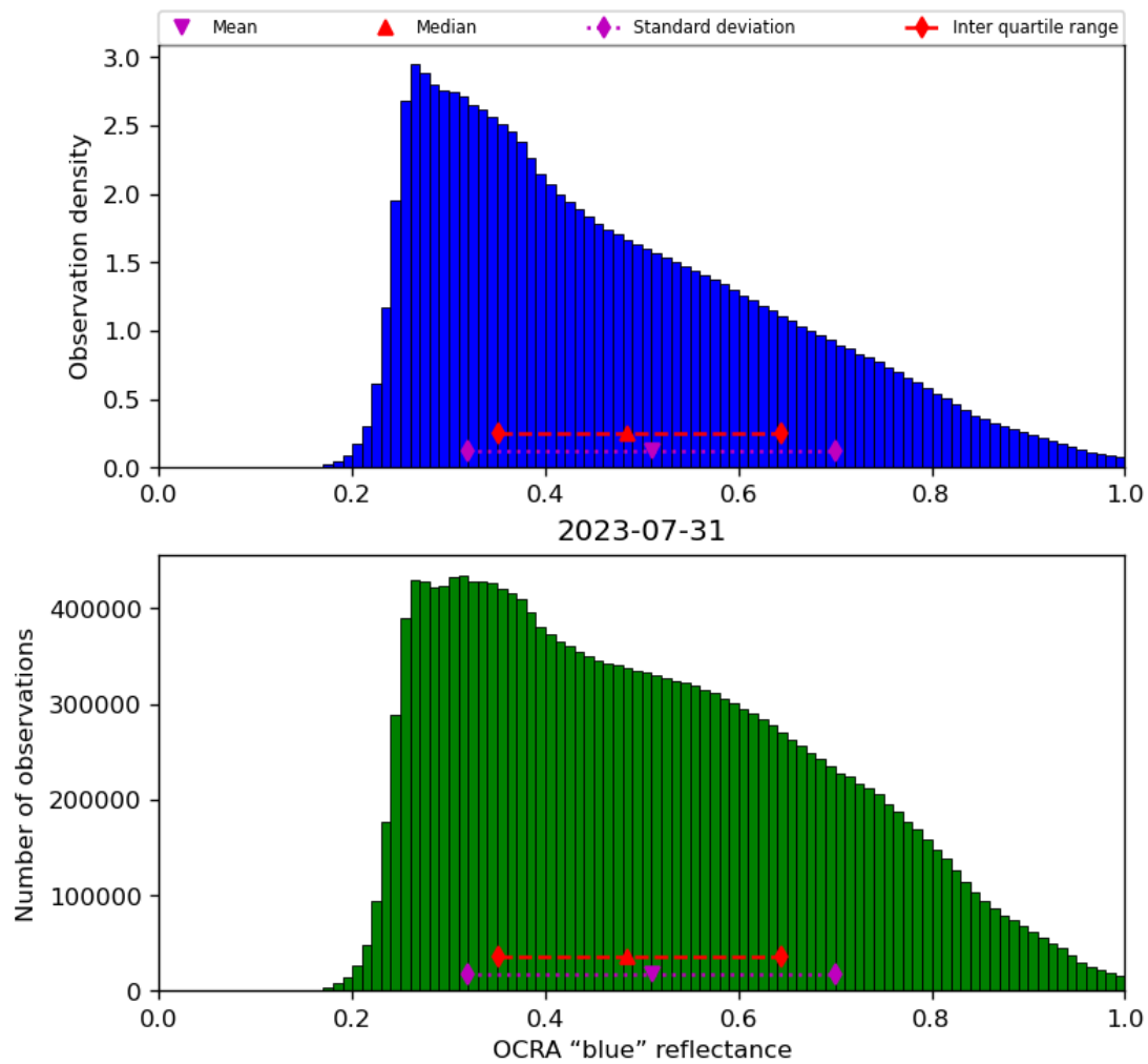
Figure 51: Histogram of “OCRA “blue” reflectance” for 2023-07-30 to 2023-08-01
