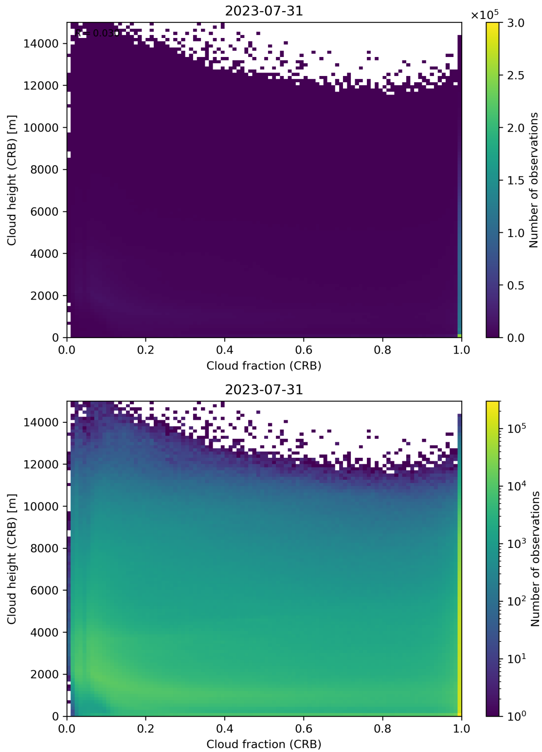
Figure 79: Scatter density plot of “Cloud fraction (CRB)” against “Cloud height (CRB)” for 2023-07-30 to 2023-08-01.
