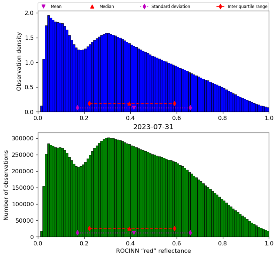
Figure 53: Histogram of “ROCINN “red” reflectance” for 2023-07-30 to 2023-08-01
