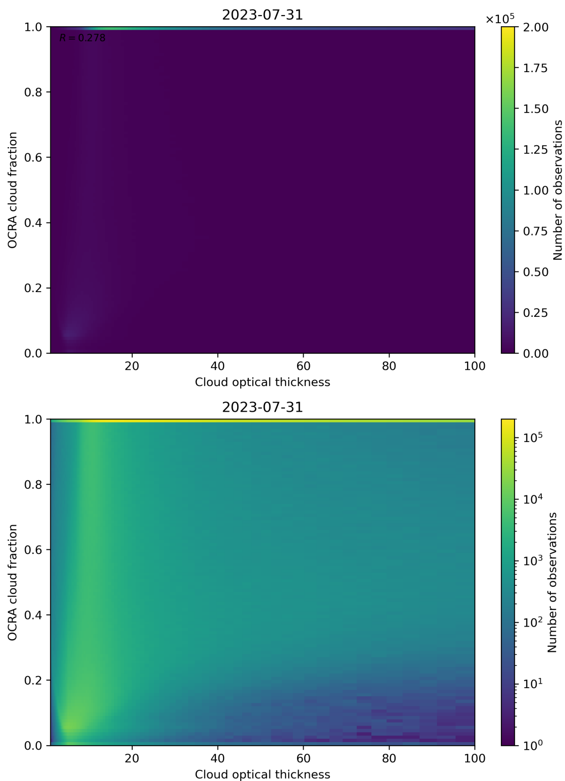
Figure 83: Scatter density plot of “Cloud optical thickness” against “OCRA cloud fraction” for 2023-07-30 to 2023-08-01.
