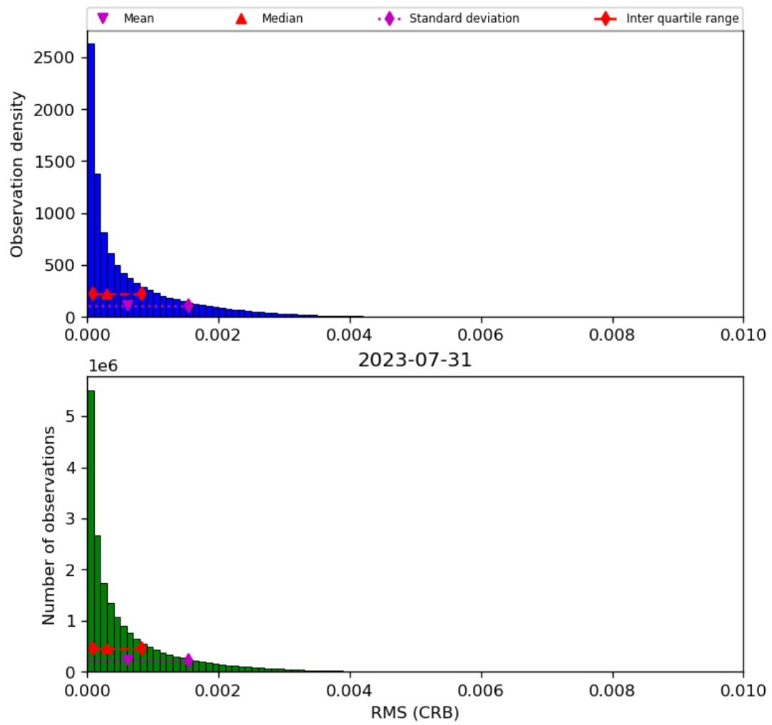
Figure 48: Histogram of “RMS (CRB)” for 2023-07-30 to 2023-08-01
