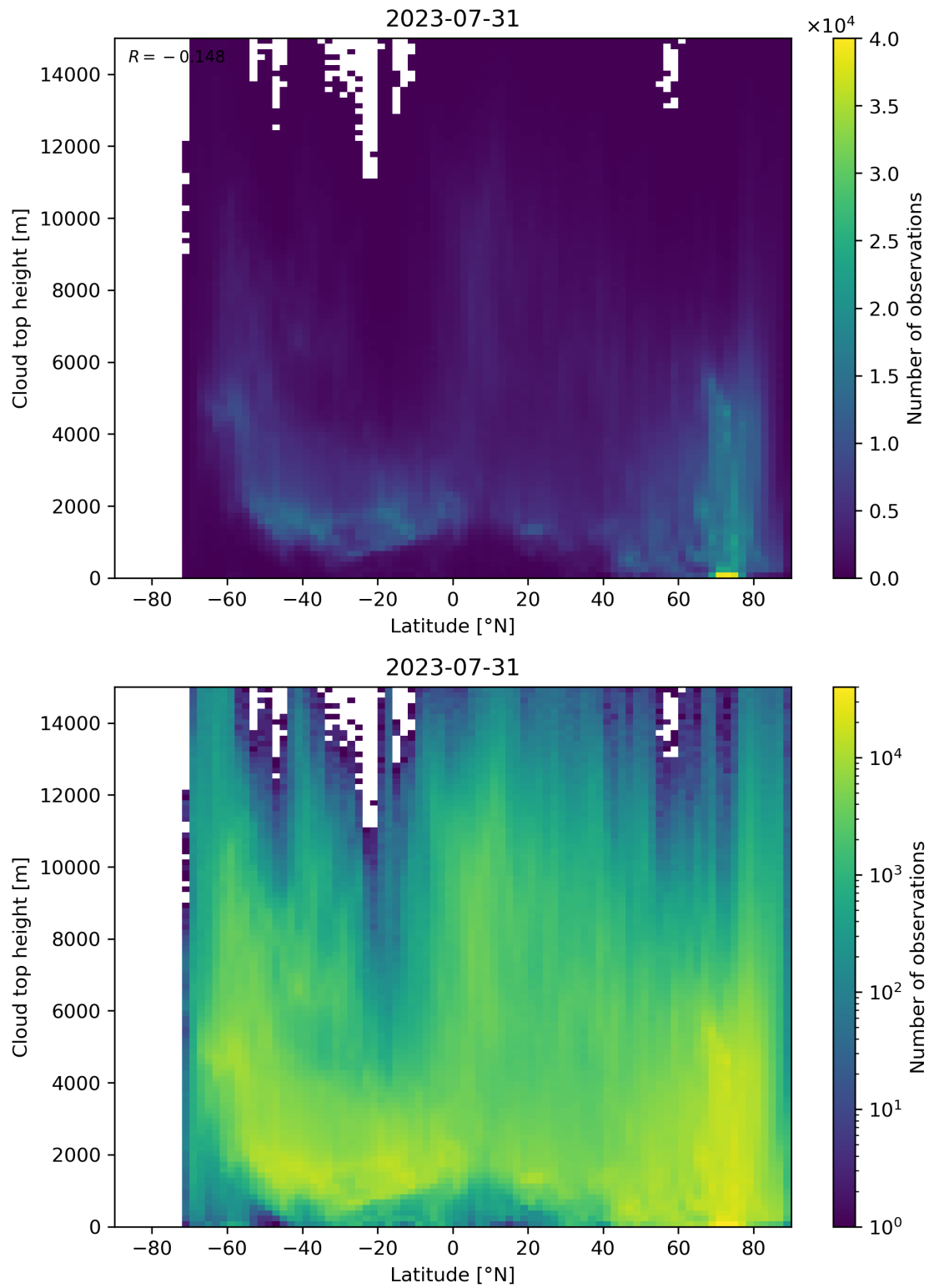
Figure 97: Scatter density plot of “Latitude” against “Cloud top height” for 2023-07-30 to 2023-08-01.
