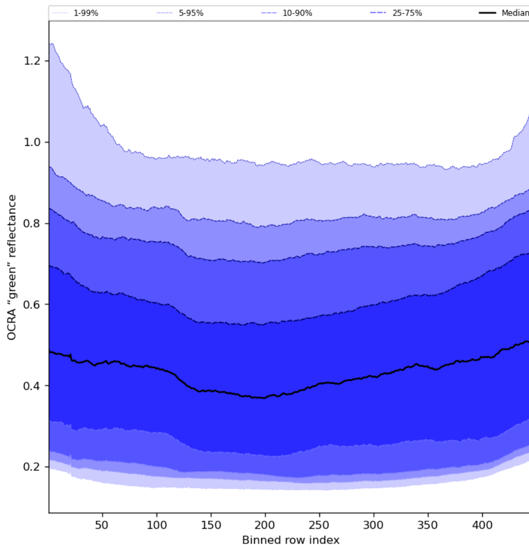
Figure 68: Along track statistics of “OCRA “green” reflectance” for 2023-07-30 to 2023-08-01
