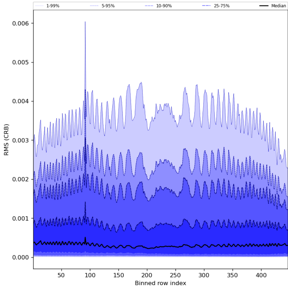
Figure 64: Along track statistics of “RMS (CRB)” for 2023-07-30 to 2023-08-01
