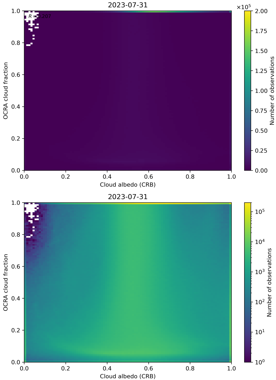
Figure 70: Scatter density plot of “Cloud albedo (CRB)” against “OCRA cloud fraction” for 2023-07-30 to 2023-08-01.
