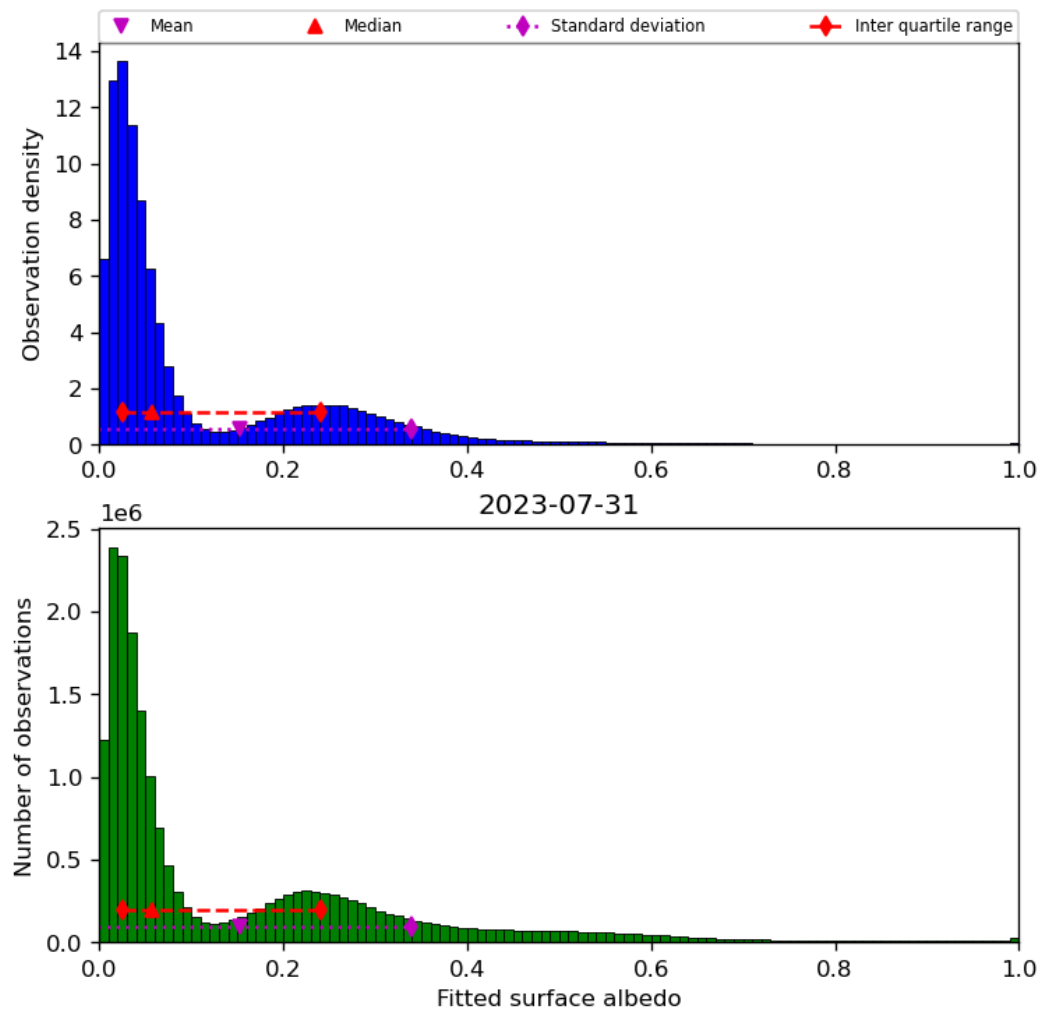
Figure 45: Histogram of “Fitted surface albedo” for 2023-07-30 to 2023-08-01
