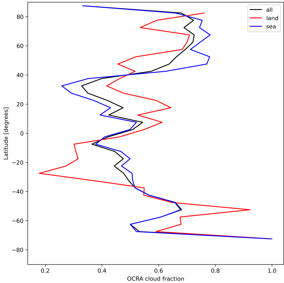
Figure 34: Zonal average of “OCRA cloud fraction” for 2023-07-30 to 2023-08-01.
