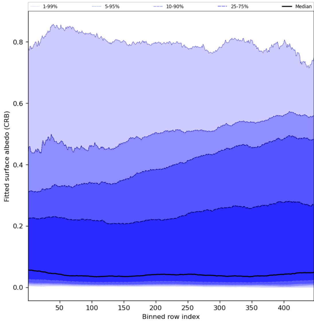
Figure 62: Along track statistics of “Fitted surface albedo (CRB)” for 2023-07-30 to 2023-08-01
