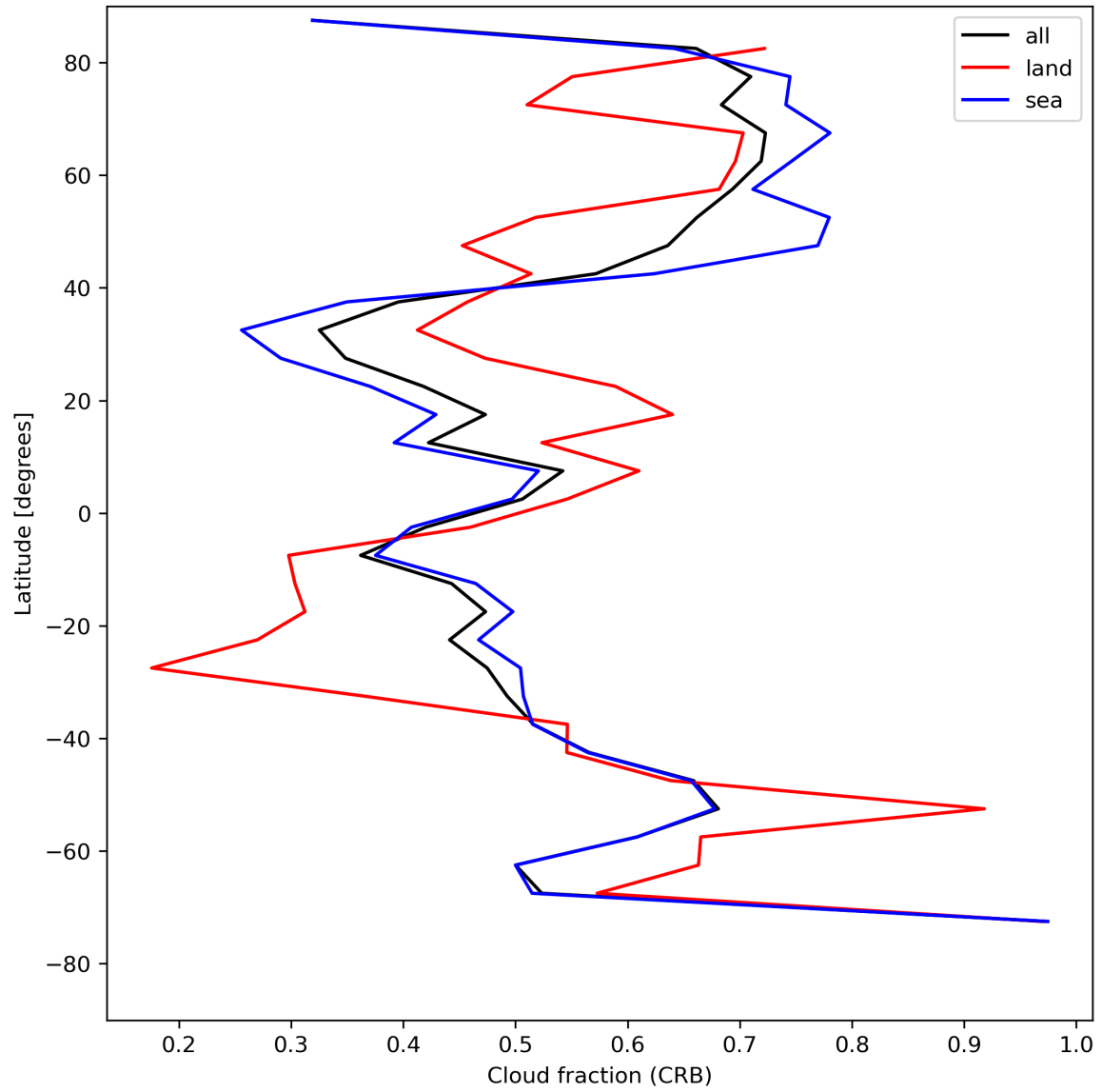
Figure 26: Zonal average of “Cloud fraction (CRB)” for 2023-07-30 to 2023-08-01.
