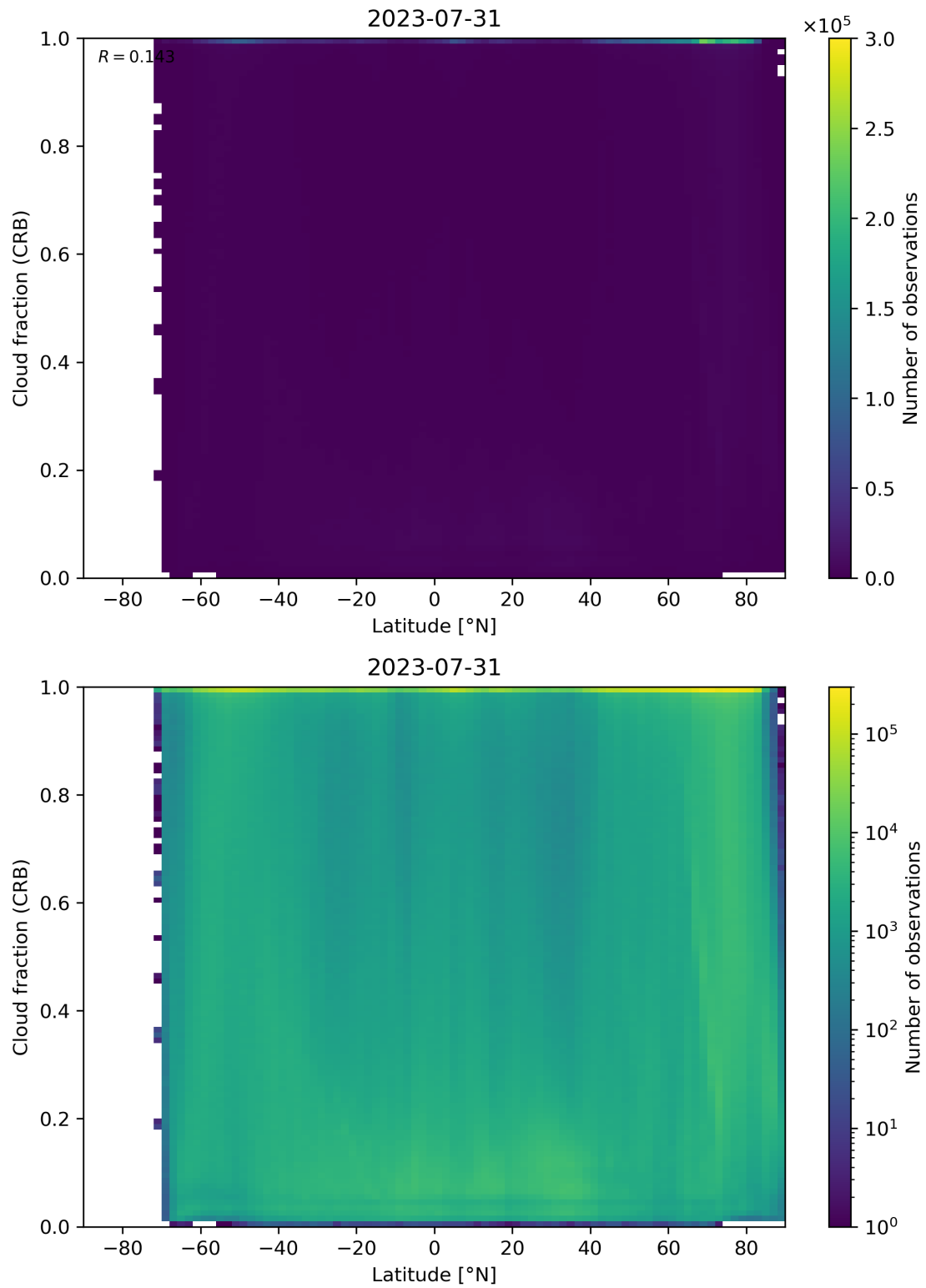
Figure 94: Scatter density plot of “Latitude” against “Cloud fraction (CRB)” for 2023-07-30 to 2023-08-01.
