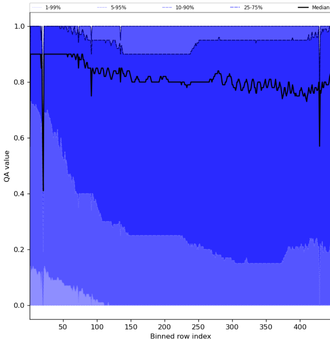
Figure 54: Along track statistics of “QA value” for 2023-07-30 to 2023-08-01
