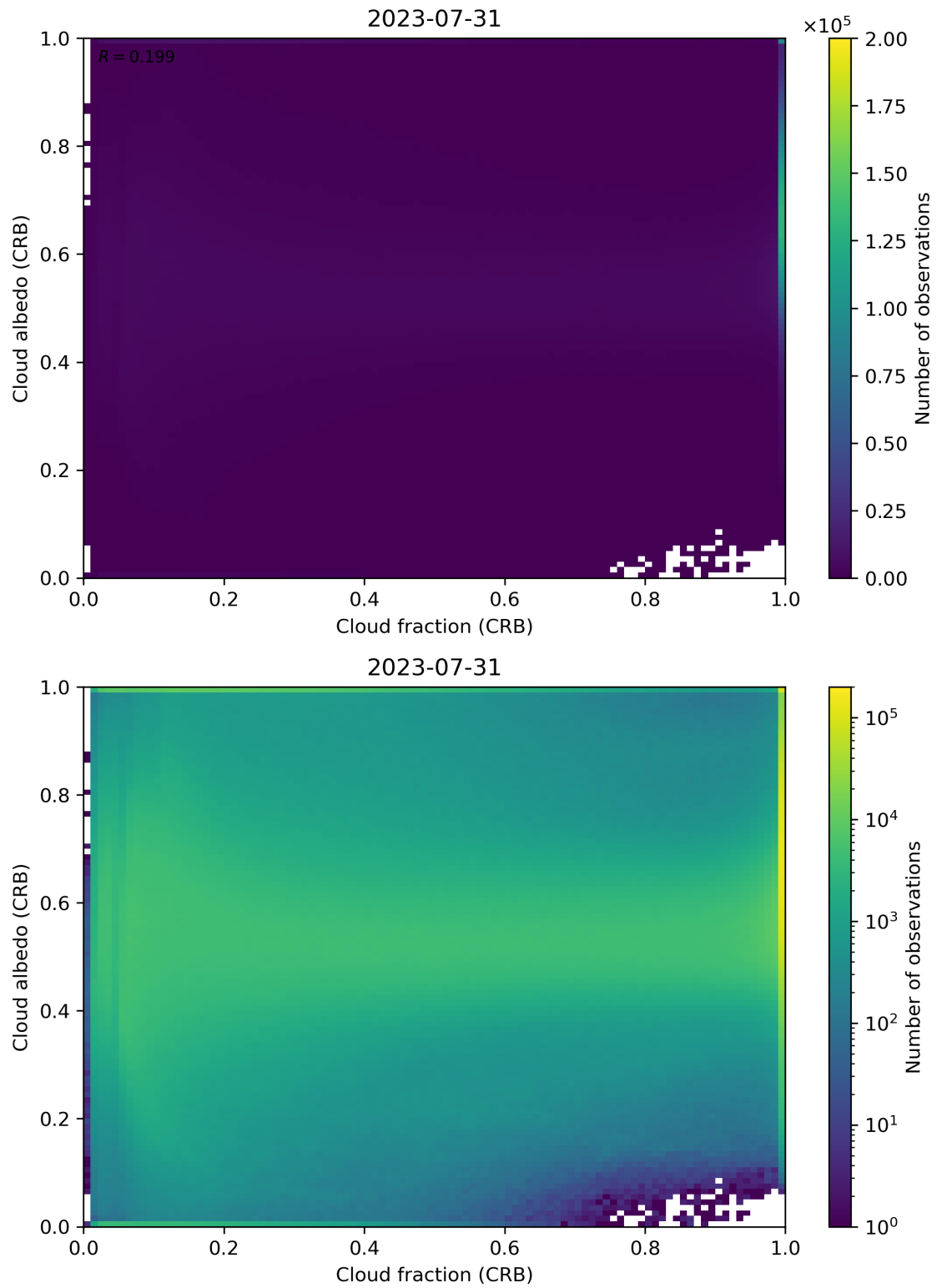
Figure 77: Scatter density plot of “Cloud fraction (CRB)” against “Cloud albedo (CRB)” for 2023-07-30 to 2023-08-01.
