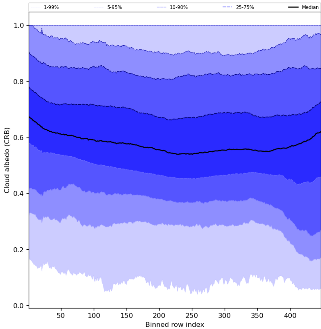
Figure 60: Along track statistics of “Cloud albedo (CRB)” for 2023-07-30 to 2023-08-01
