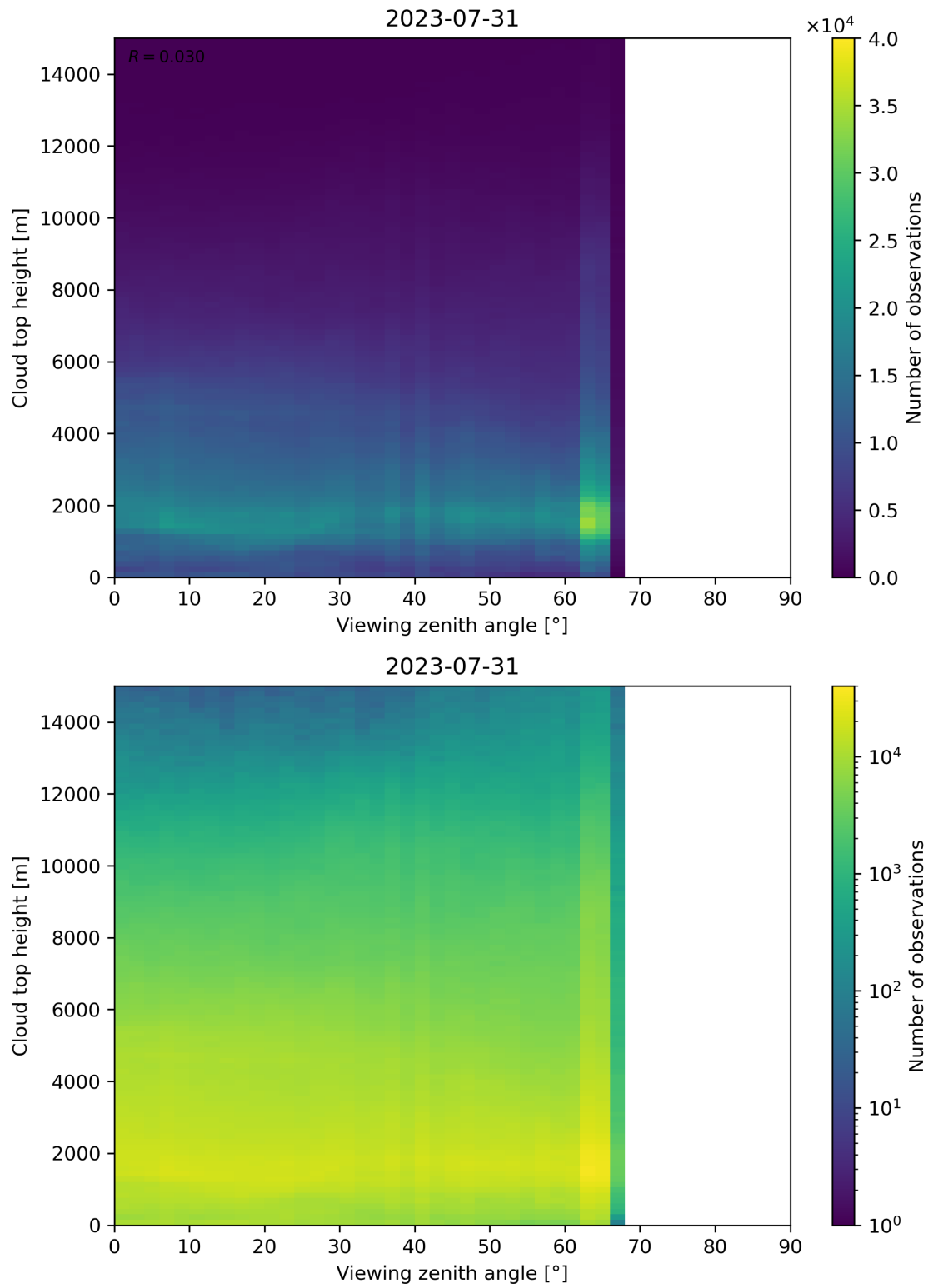
Figure 112: Scatter density plot of “Viewing zenith angle” against “Cloud top height” for 2023-07-30 to 2023-08-01.
