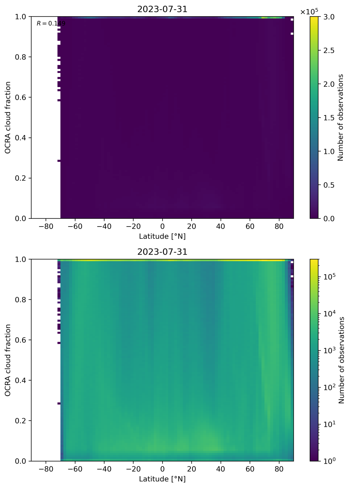
Figure 93: Scatter density plot of “Latitude” against “OCRA cloud fraction” for 2023-07-30 to 2023-08-01.
