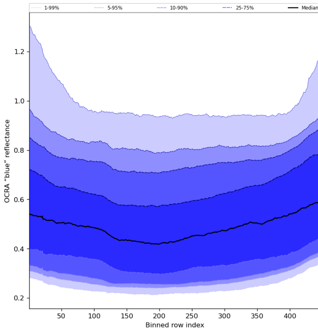
Figure 67: Along track statistics of “OCRA “blue” reflectance” for 2023-07-30 to 2023-08-01
