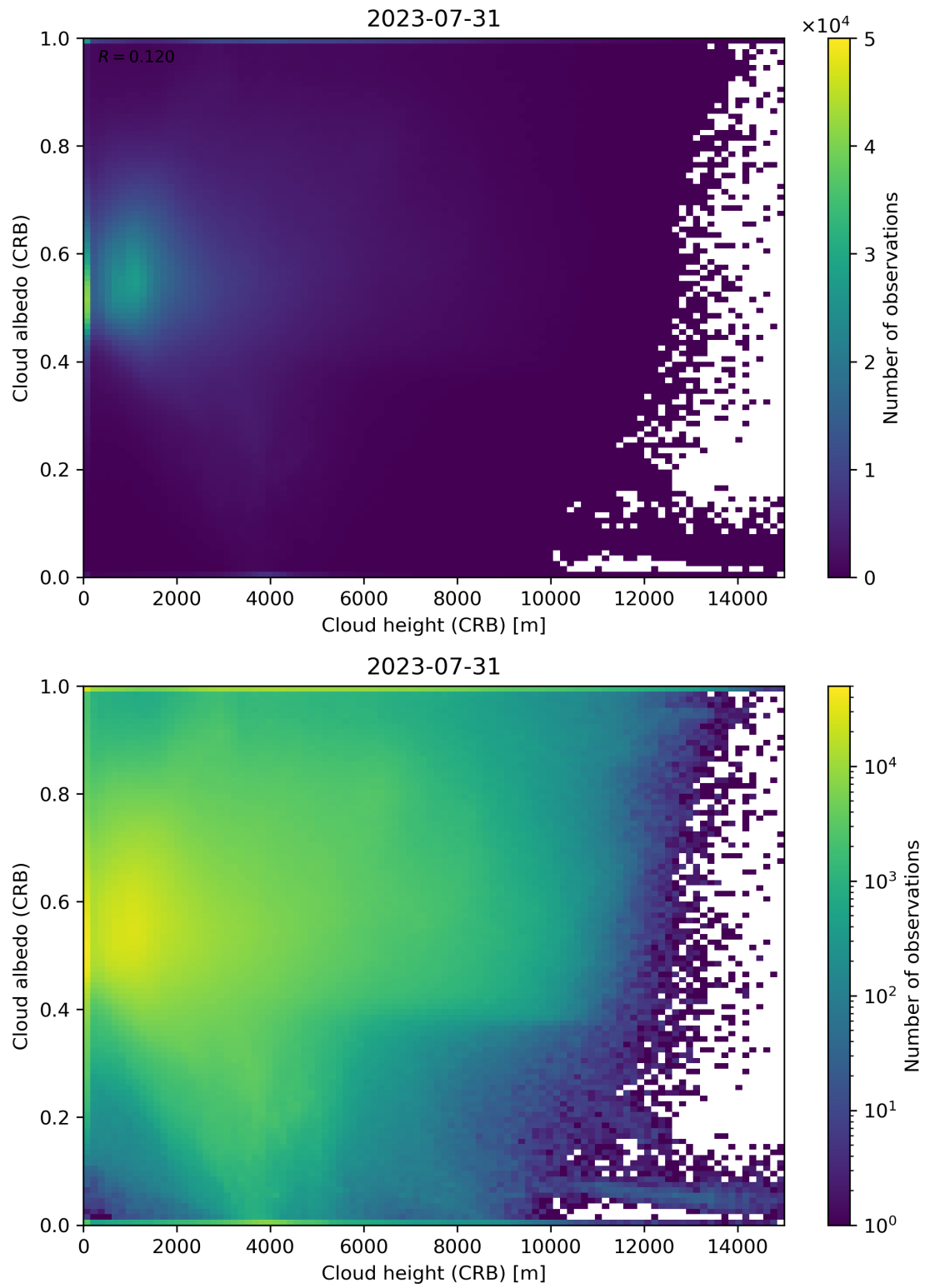
Figure 80: Scatter density plot of “Cloud height (CRB)” against “Cloud albedo (CRB)” for 2023-07-30 to 2023-08-01.
