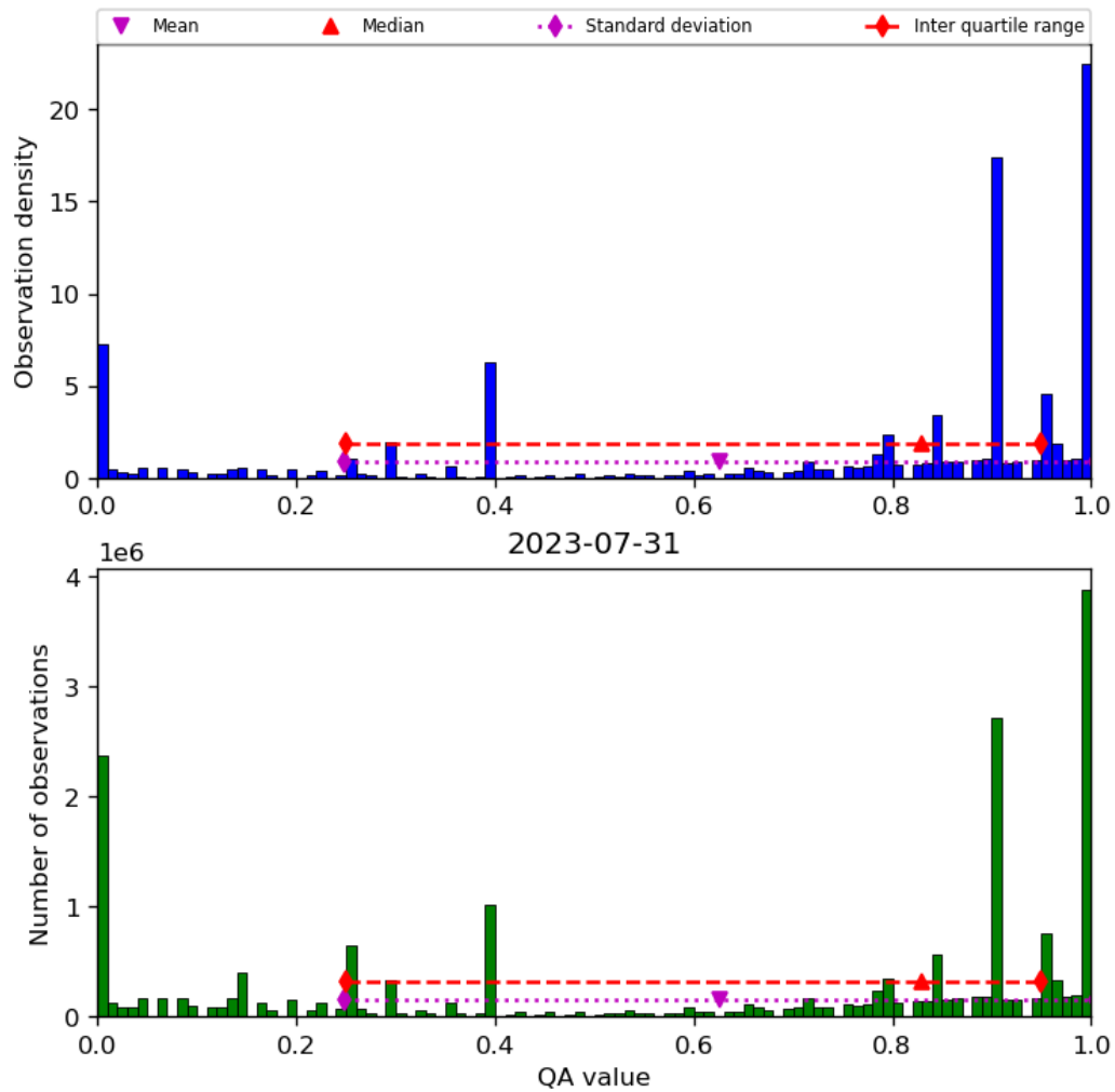
Figure 38: Histogram of “QA value” for 2023-07-30 to 2023-08-01
