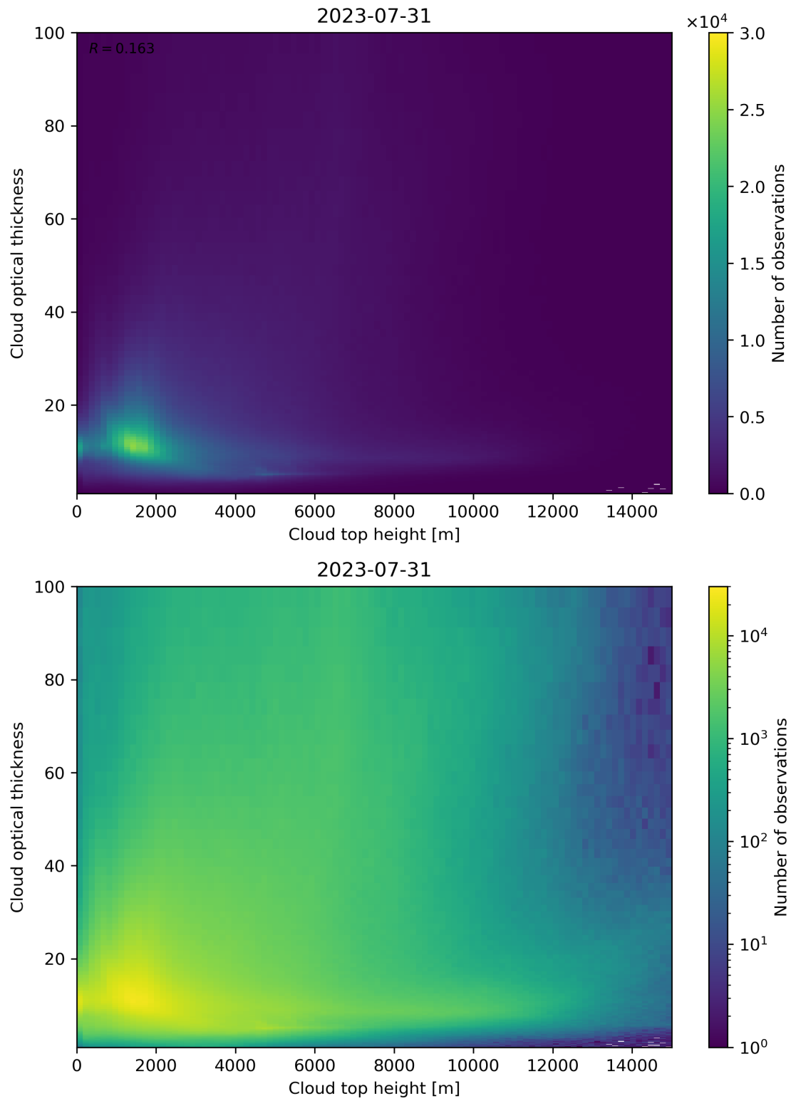
Figure 90: Scatter density plot of “Cloud top height” against “Cloud optical thickness” for 2023-07-30 to 2023-08-01.
