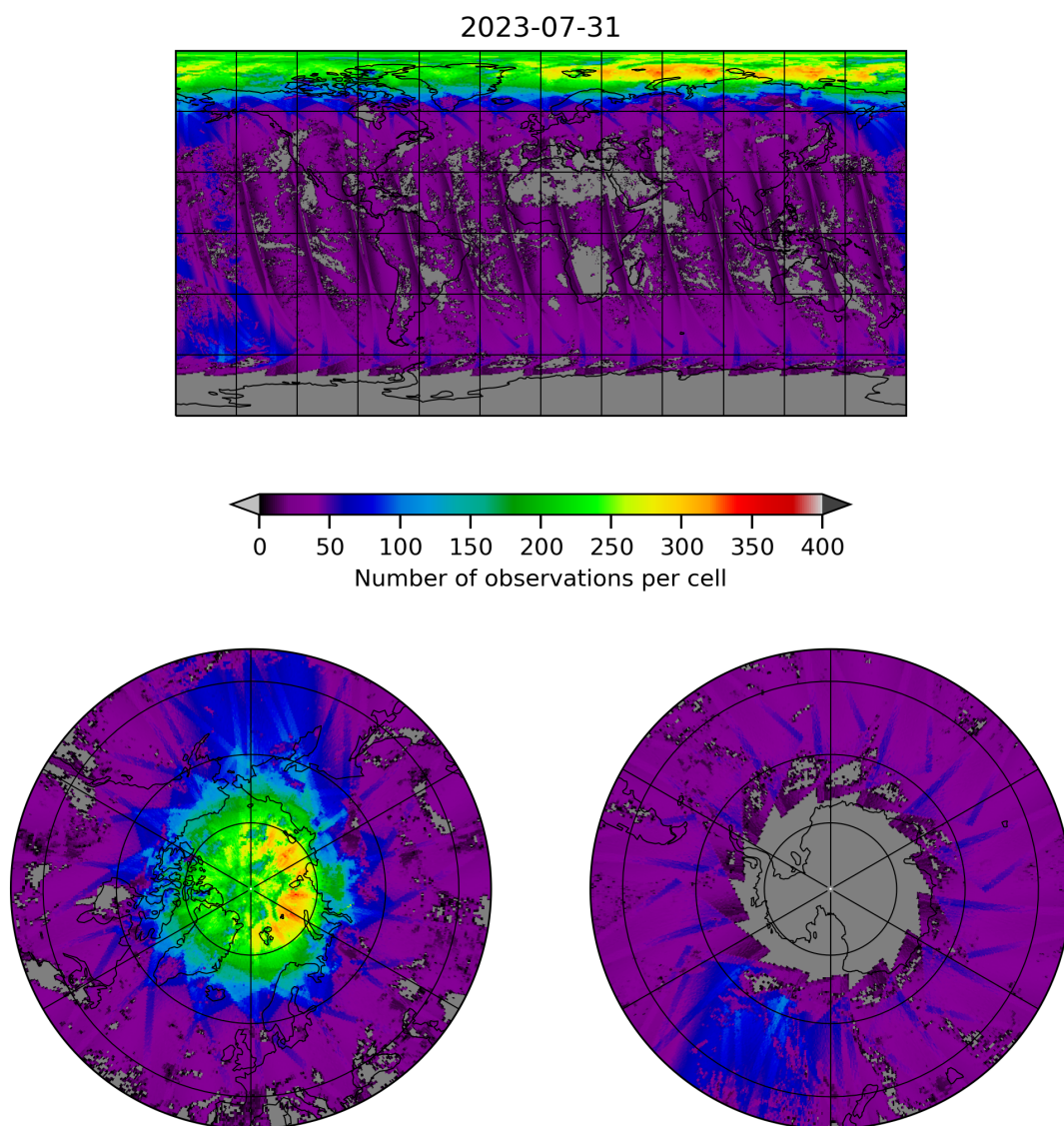
Figure 21: Map of the number of observations for 2023-07-30 to 2023-08-01
