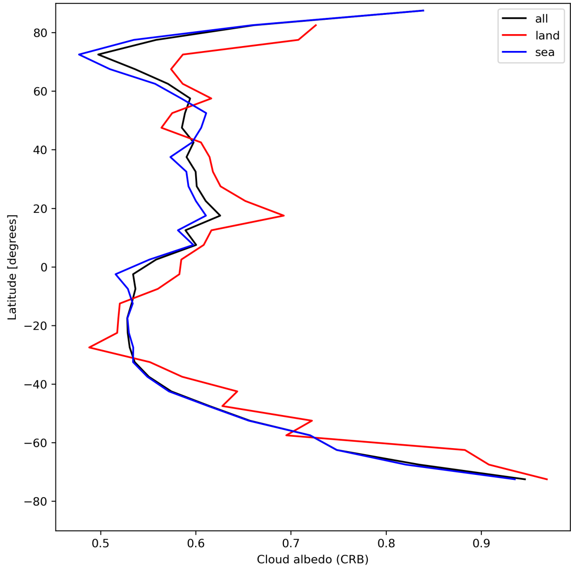
Figure 28: Zonal average of “Cloud albedo (CRB)” for 2023-07-30 to 2023-08-01.
