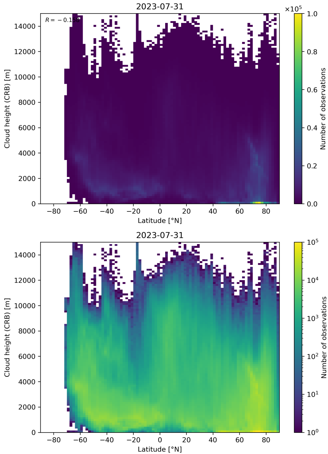
Figure 95: Scatter density plot of “Latitude” against “Cloud height (CRB)” for 2023-07-30 to 2023-08-01.
