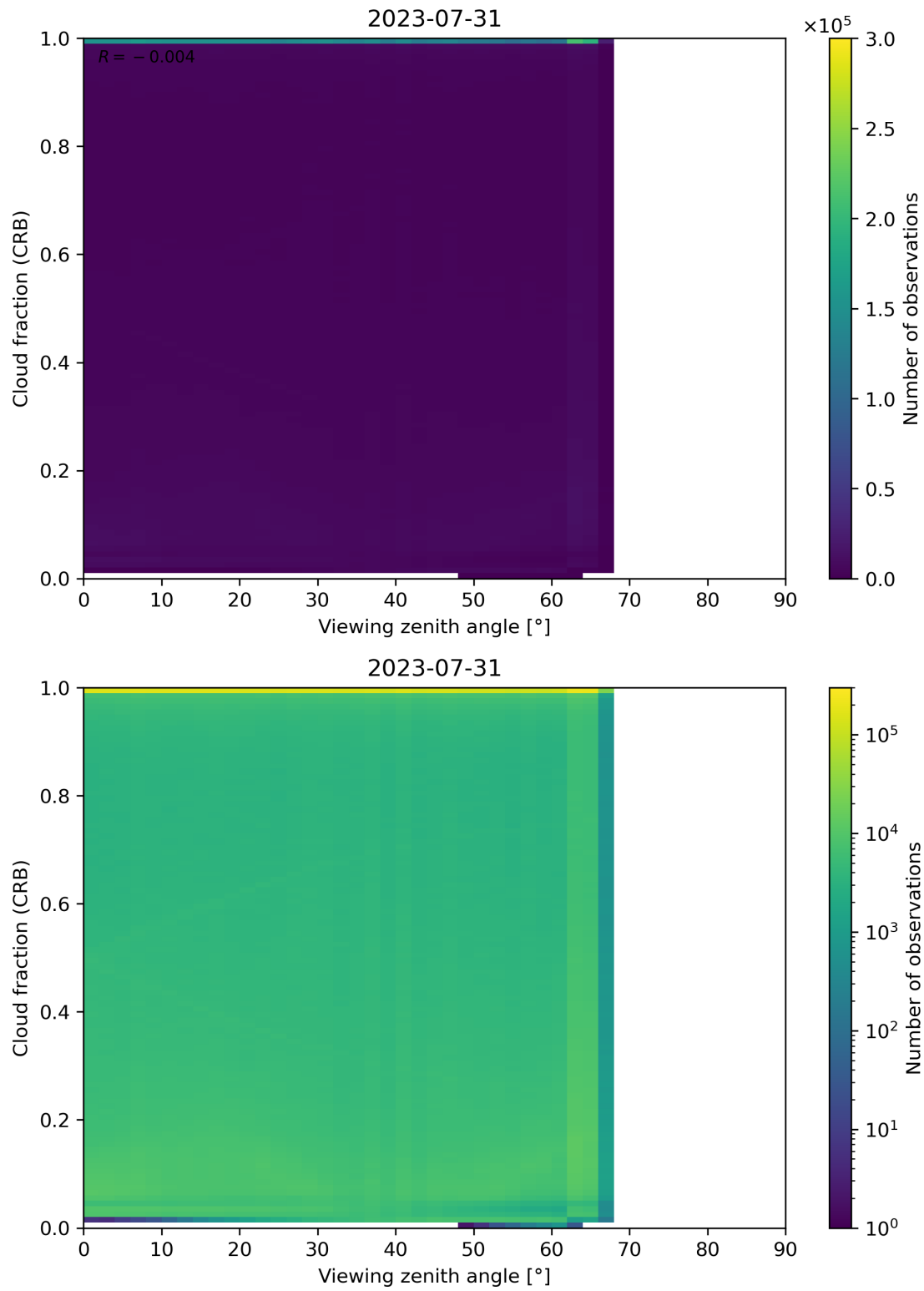
Figure 109: Scatter density plot of “Viewing zenith angle” against “Cloud fraction (CRB)” for 2023-07-30 to 2023-08-01.
