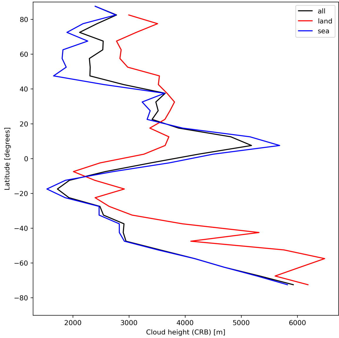
Figure 27: Zonal average of “Cloud height (CRB)” for 2023-07-30 to 2023-08-01.
