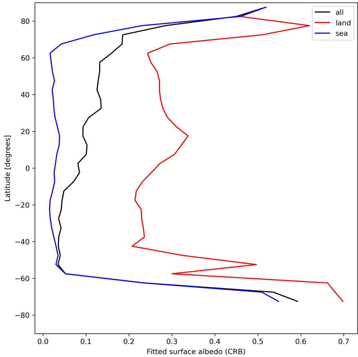
Figure 30: Zonal average of “Fitted surface albedo (CRB)” for 2023-07-30 to 2023-08-01.
