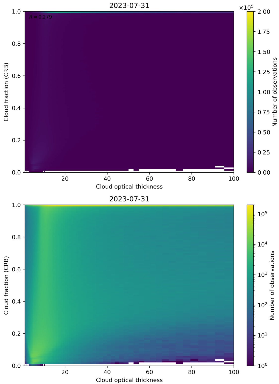
Figure 84: Scatter density plot of “Cloud optical thickness” against “Cloud fraction (CRB)” for 2023-07-30 to 2023-08-01.
