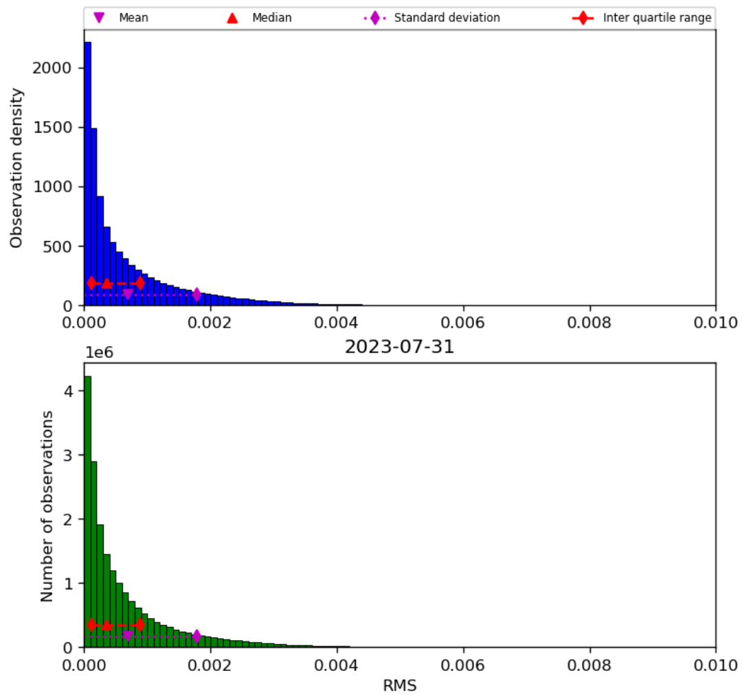
Figure 47: Histogram of “RMS” for 2023-07-30 to 2023-08-01
