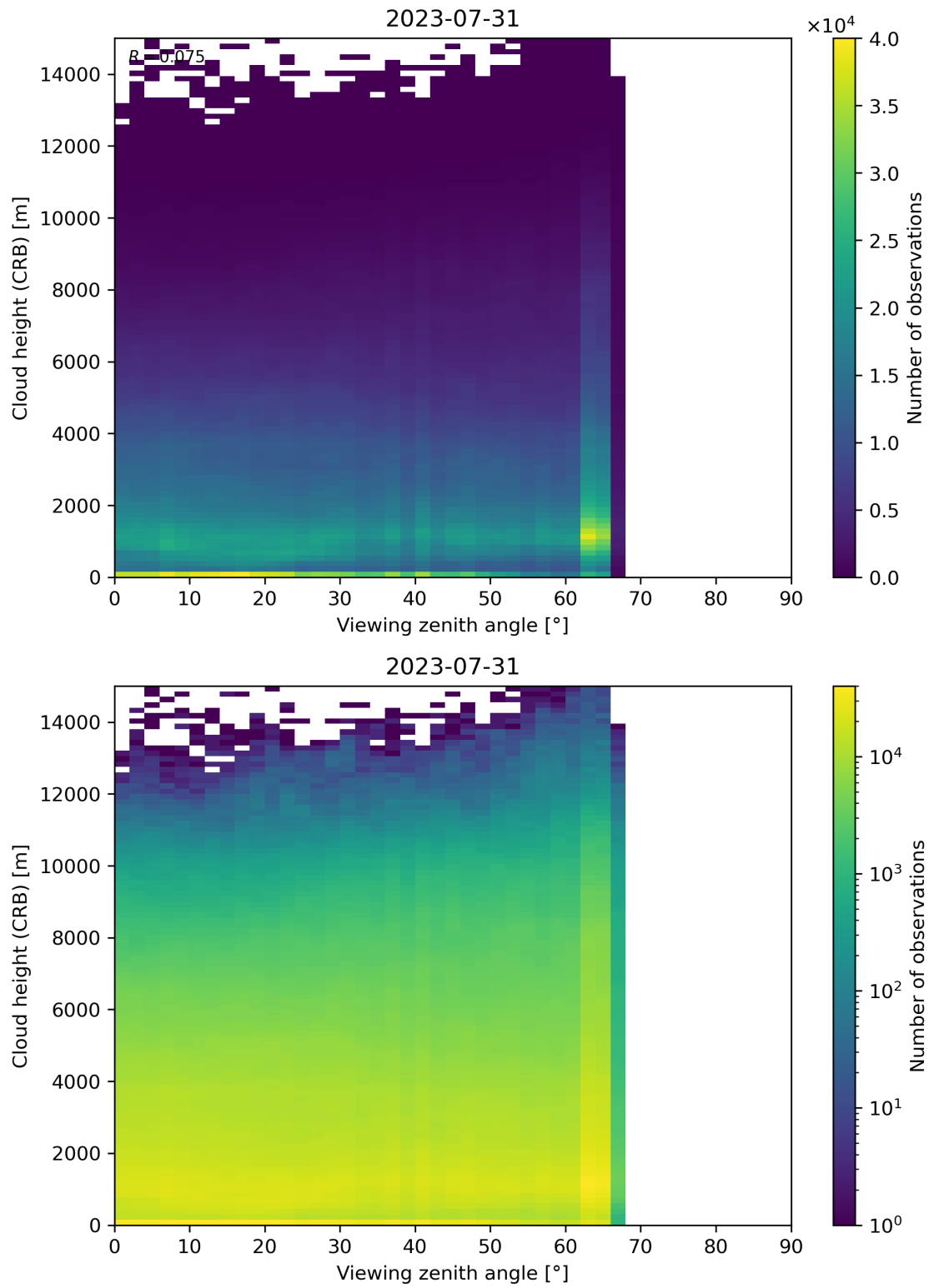
Figure 110: Scatter density plot of “Viewing zenith angle” against “Cloud height (CRB)” for 2023-07-30 to 2023-08-01.
