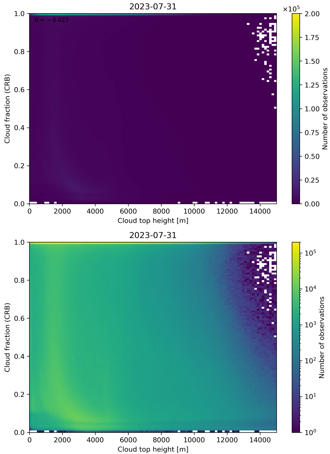
Figure 88: Scatter density plot of “Cloud top height” against “Cloud fraction (CRB)” for 2023-07-30 to 2023-08-01.
