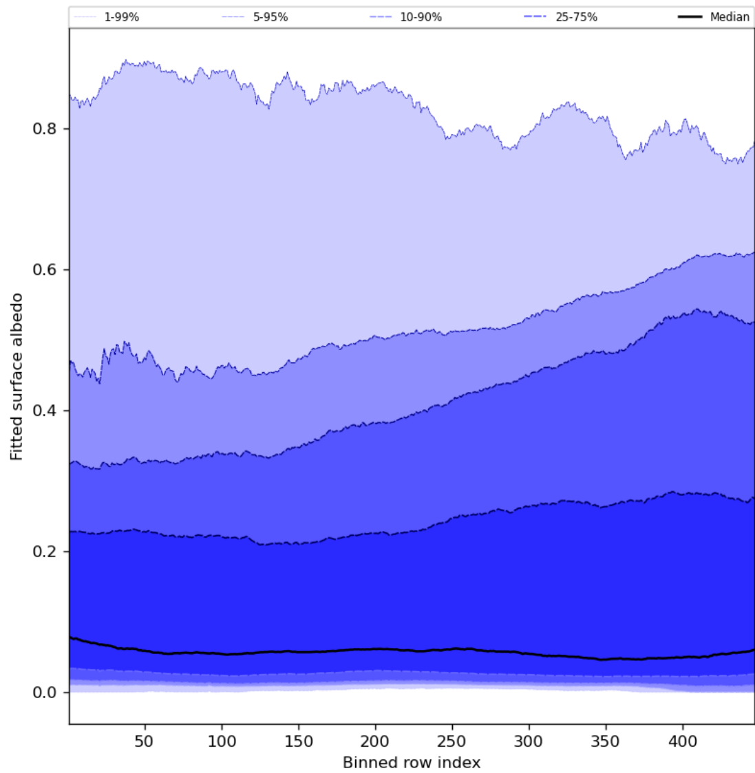
Figure 61: Along track statistics of “Fitted surface albedo” for 2023-07-30 to 2023-08-01
