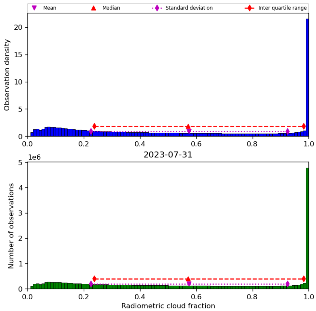
Figure 39: Histogram of “Radiometric cloud fraction” for 2023-07-30 to 2023-08-01
