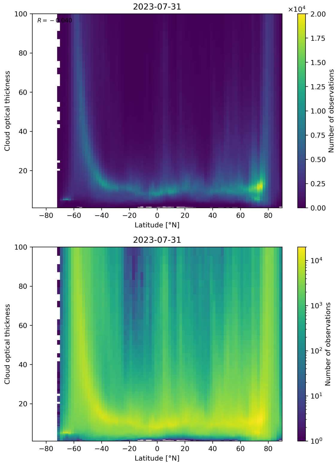
Figure 96: Scatter density plot of “Latitude” against “Cloud optical thickness” for 2023-07-30 to 2023-08-01.
