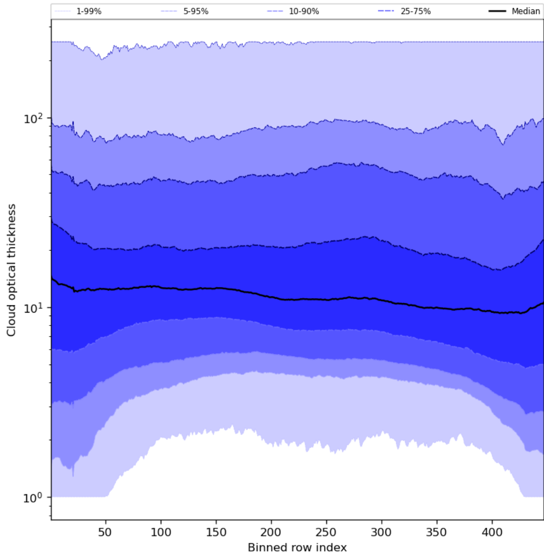
Figure 57: Along track statistics of “Cloud optical thickness” for 2023-07-31 to 2023-08-02
