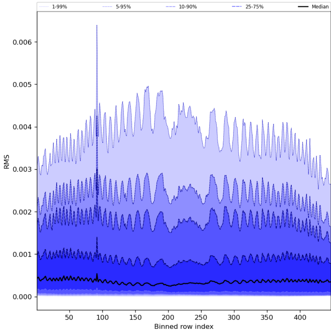
Figure 63: Along track statistics of “RMS” for 2023-07-31 to 2023-08-02
