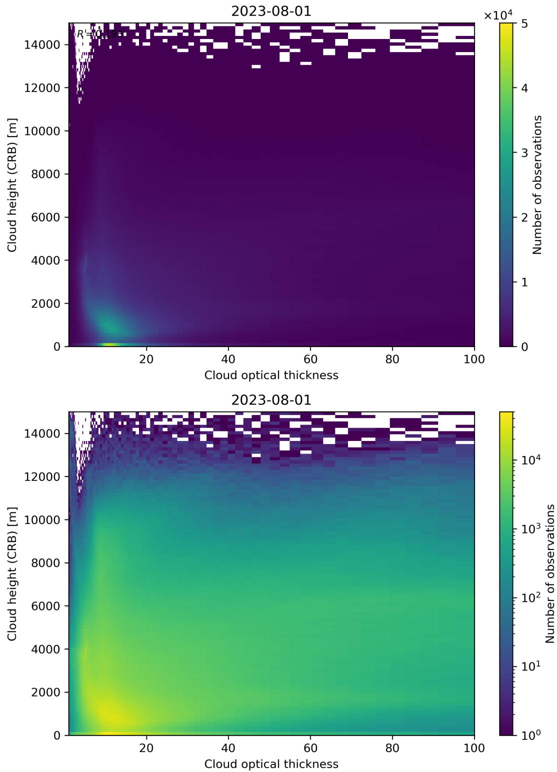
Figure 85: Scatter density plot of “Cloud optical thickness” against “Cloud height (CRB)” for 2023-07-31 to 2023-08-02.
