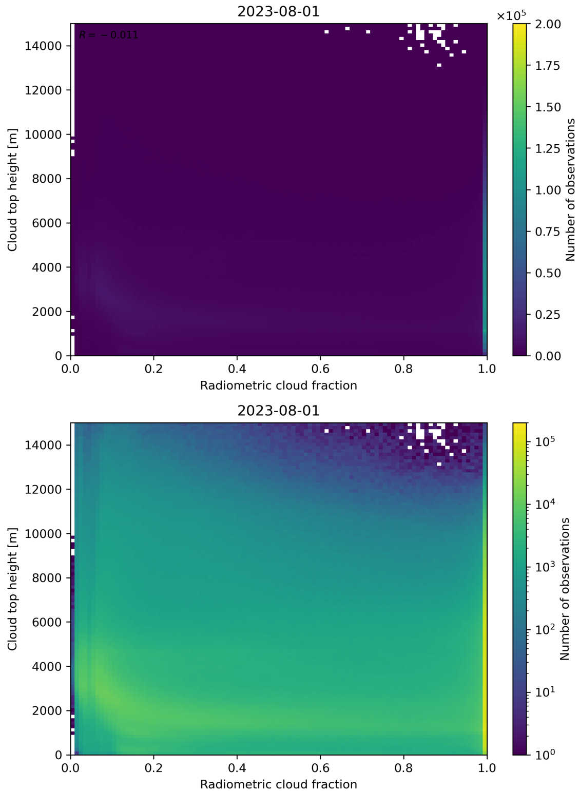
Figure 76: Scatter density plot of “Radiometric cloud fraction” against “Cloud top height” for 2023-07-31 to 2023-08-02.
