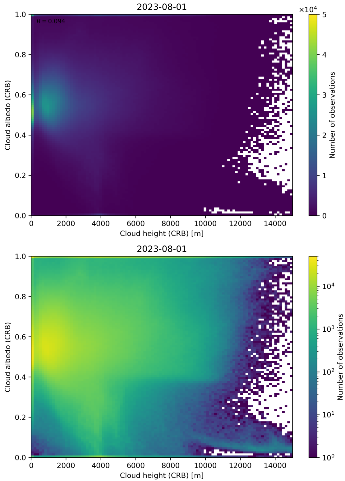
Figure 80: Scatter density plot of “Cloud height (CRB)” against “Cloud albedo (CRB)” for 2023-07-31 to 2023-08-02.
