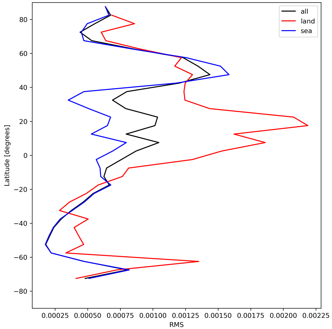
Figure 31: Zonal average of “RMS” for 2023-07-31 to 2023-08-02.
