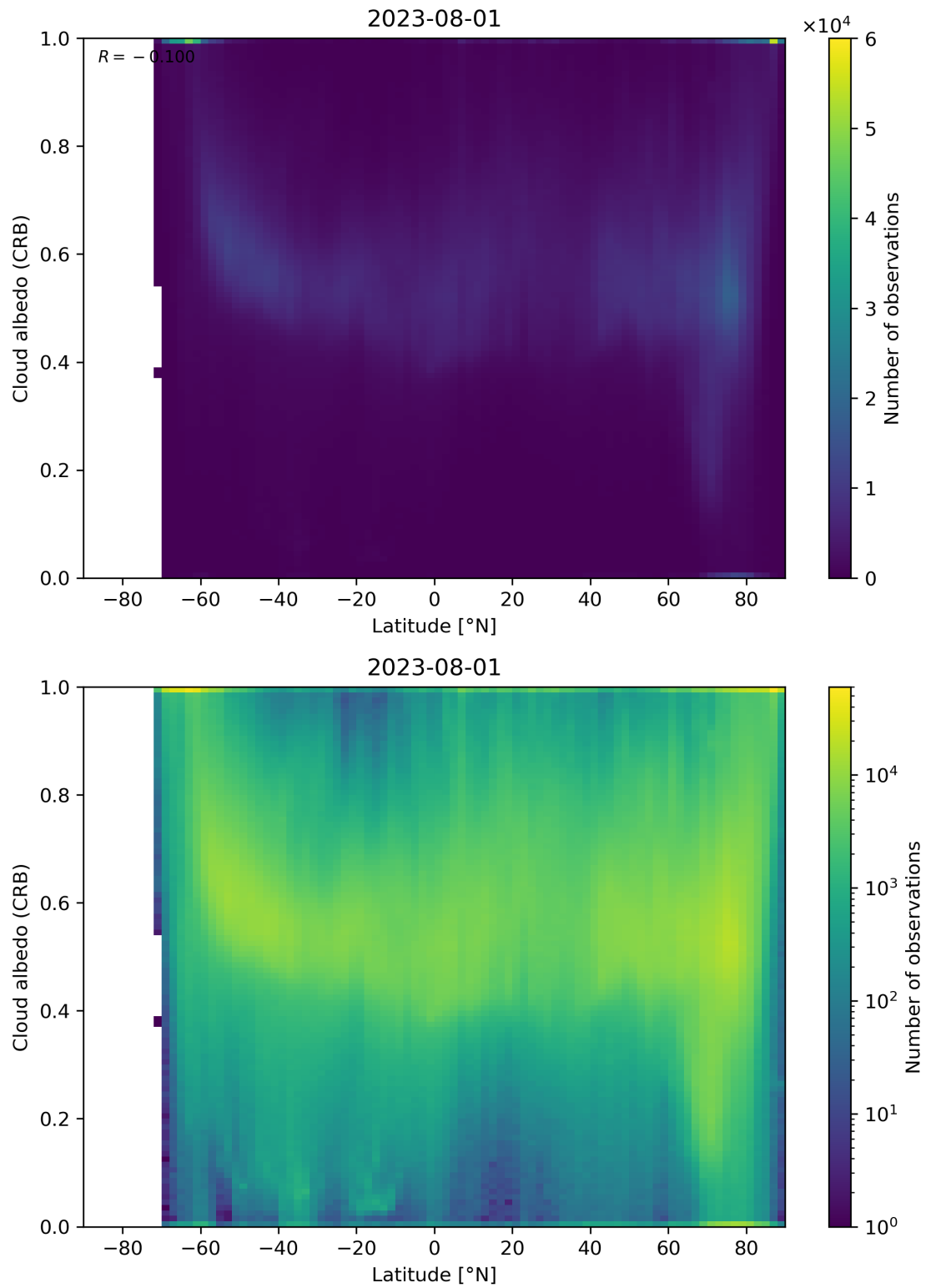
Figure 91: Scatter density plot of “Latitude” against “Cloud albedo (CRB)” for 2023-07-31 to 2023-08-02.
