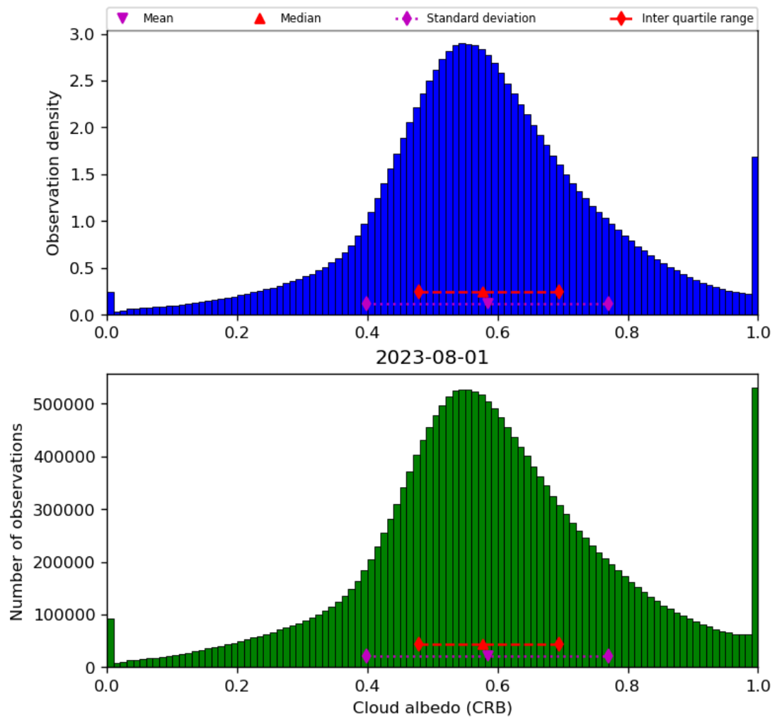
Figure 44: Histogram of “Cloud albedo (CRB)” for 2023-07-31 to 2023-08-02
