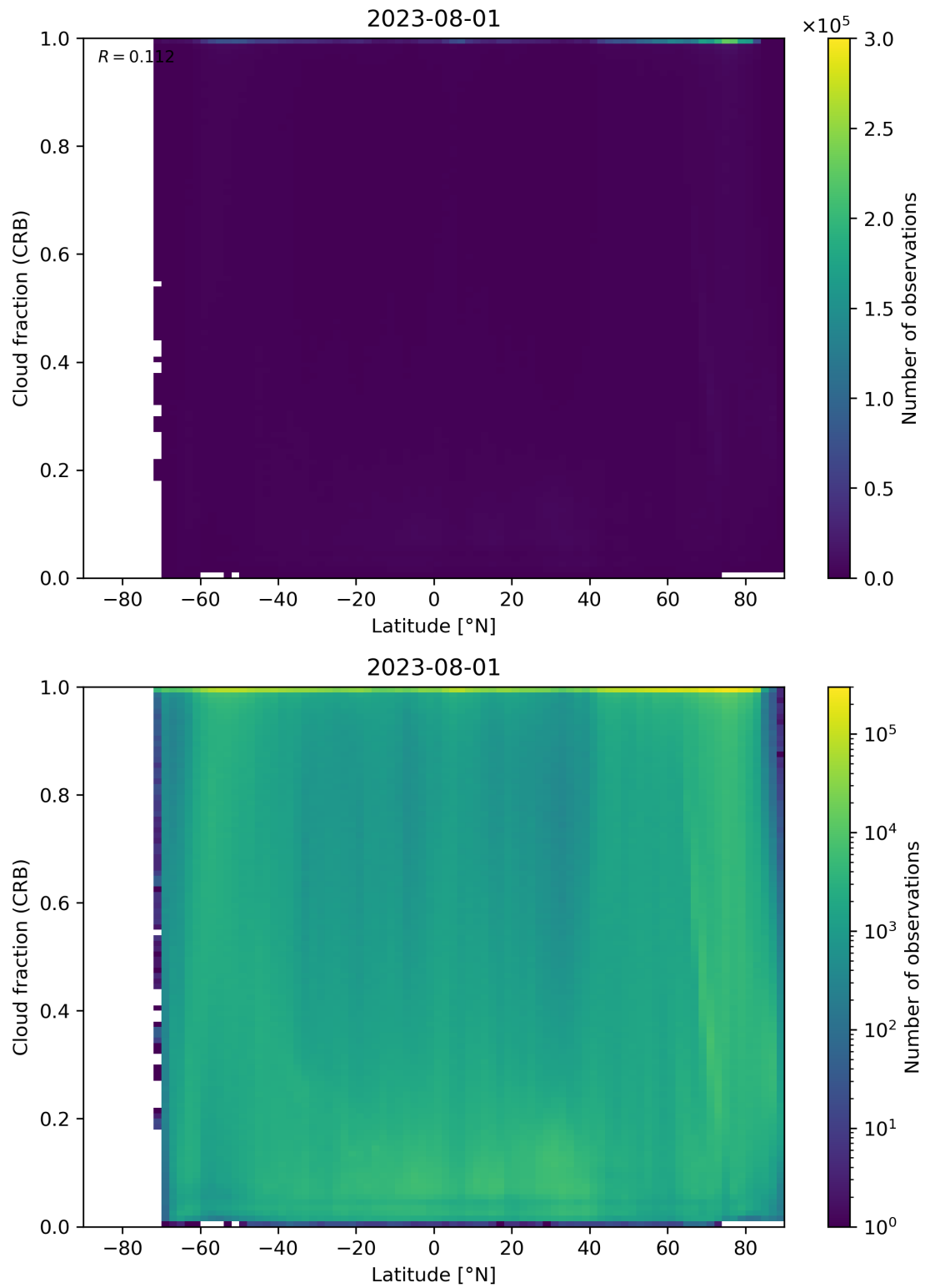
Figure 94: Scatter density plot of “Latitude” against “Cloud fraction (CRB)” for 2023-07-31 to 2023-08-02.
