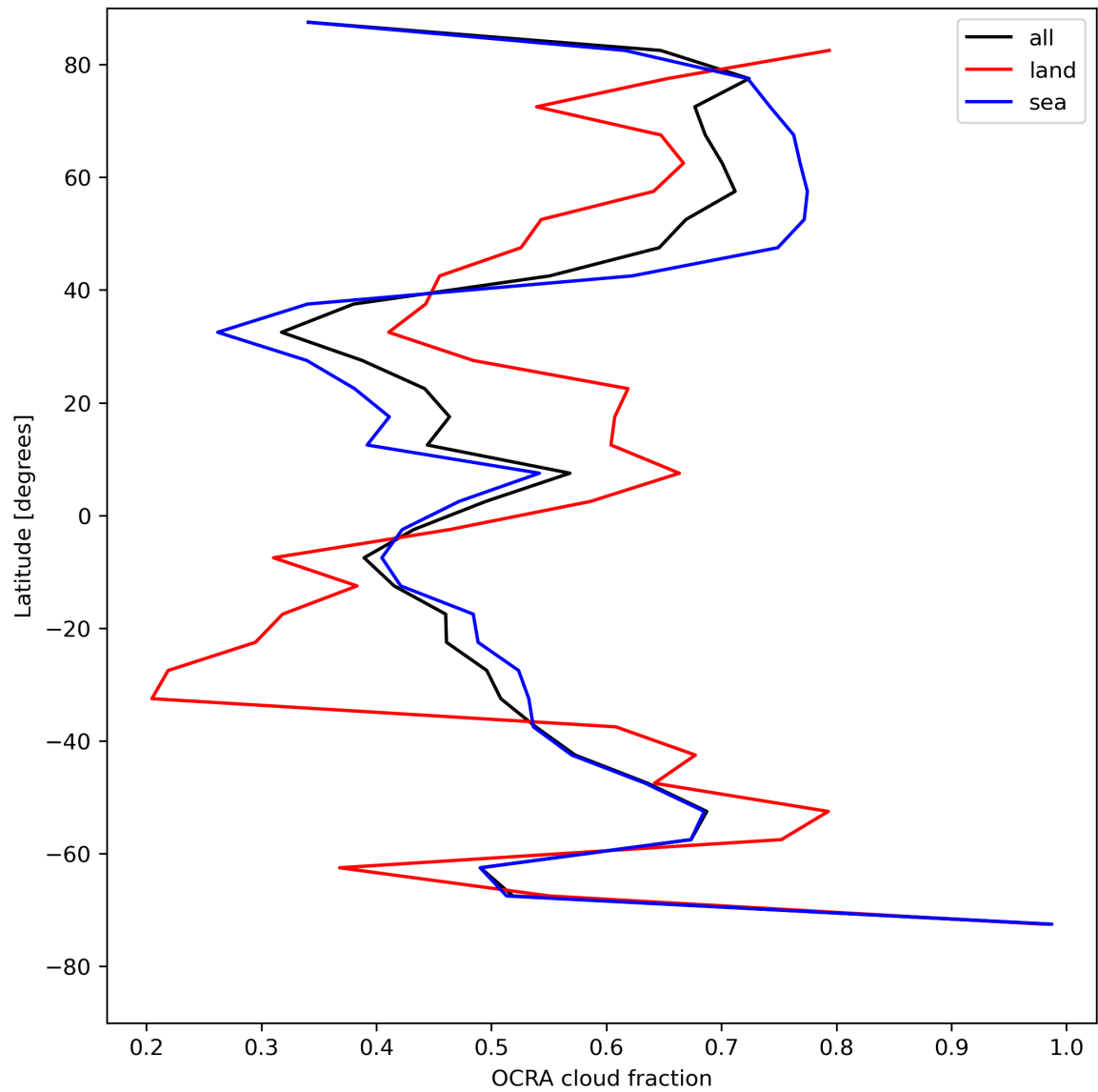
Figure 34: Zonal average of “OCRA cloud fraction” for 2023-07-31 to 2023-08-02.
