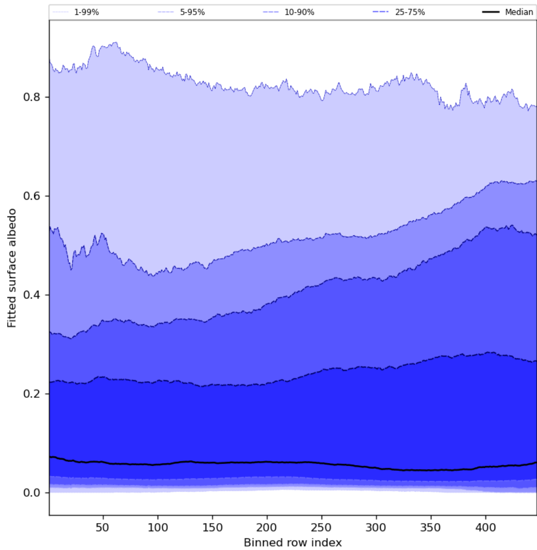
Figure 61: Along track statistics of “Fitted surface albedo” for 2023-07-31 to 2023-08-02
