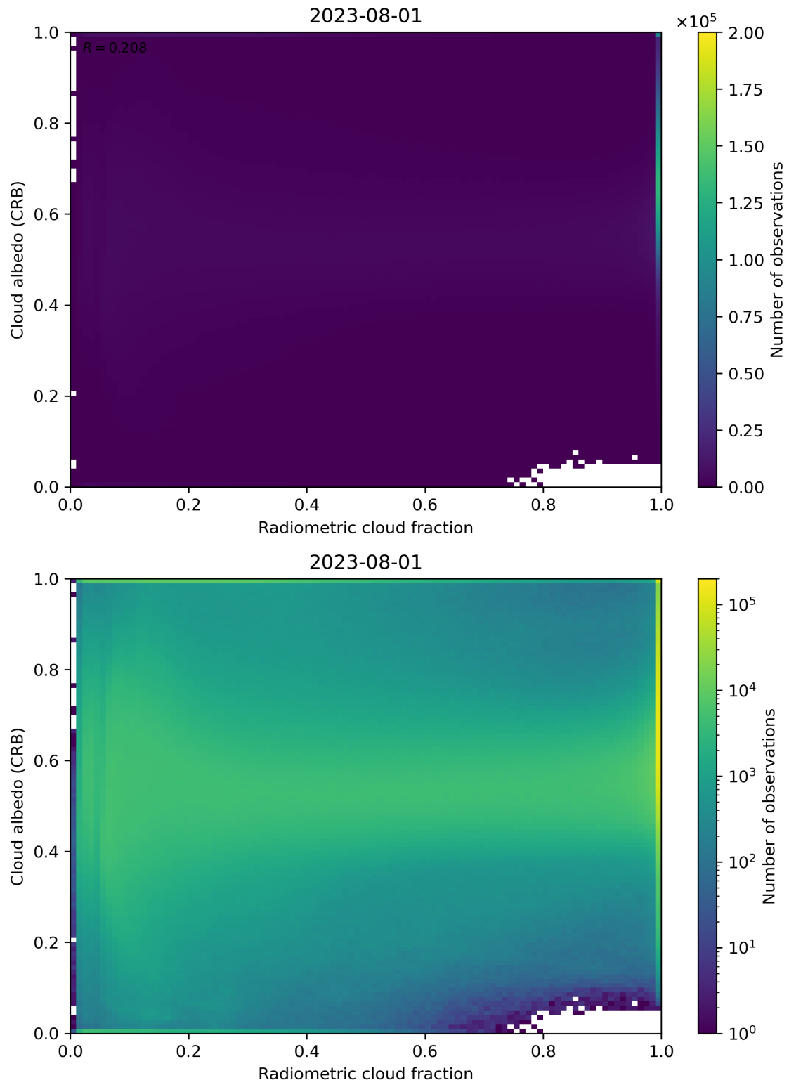
Figure 71: Scatter density plot of “Radiometric cloud fraction” against “Cloud albedo (CRB)” for 2023-07-31 to 2023-08-02.
