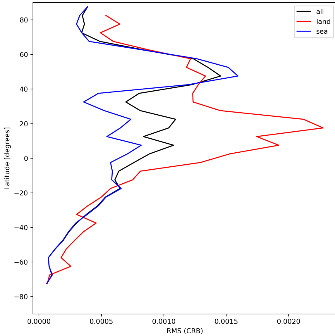
Figure 32: Zonal average of “RMS (CRB)” for 2023-07-31 to 2023-08-02.
