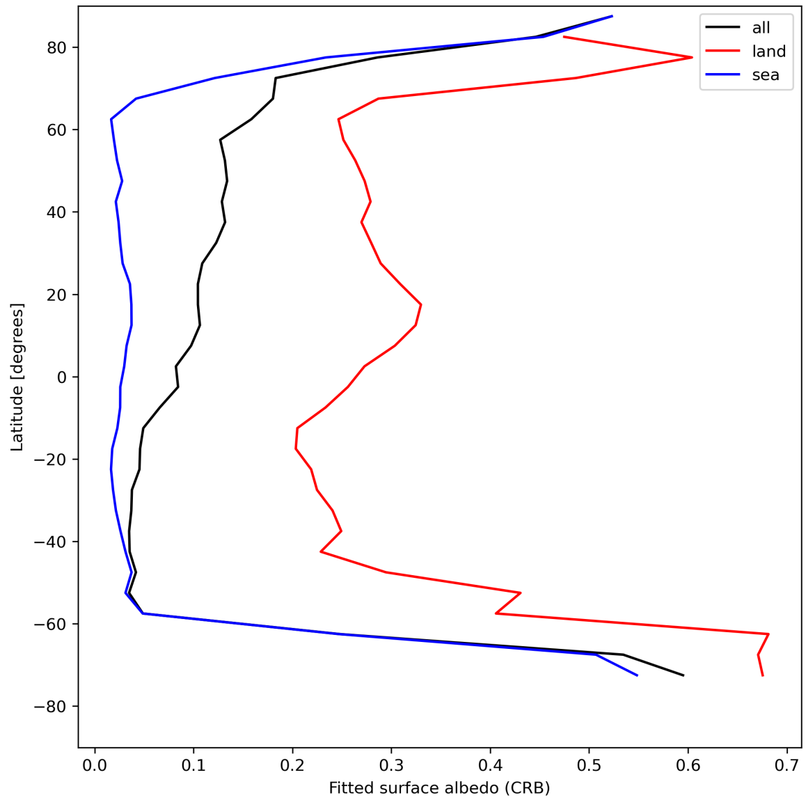
Figure 30: Zonal average of “Fitted surface albedo (CRB)” for 2023-07-31 to 2023-08-02.
