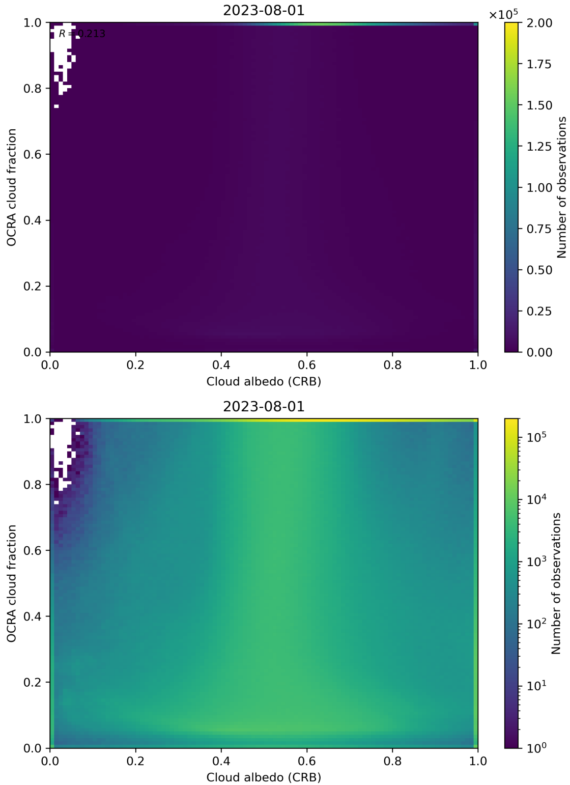
Figure 70: Scatter density plot of “Cloud albedo (CRB)” against “OCRA cloud fraction” for 2023-07-31 to 2023-08-02.
