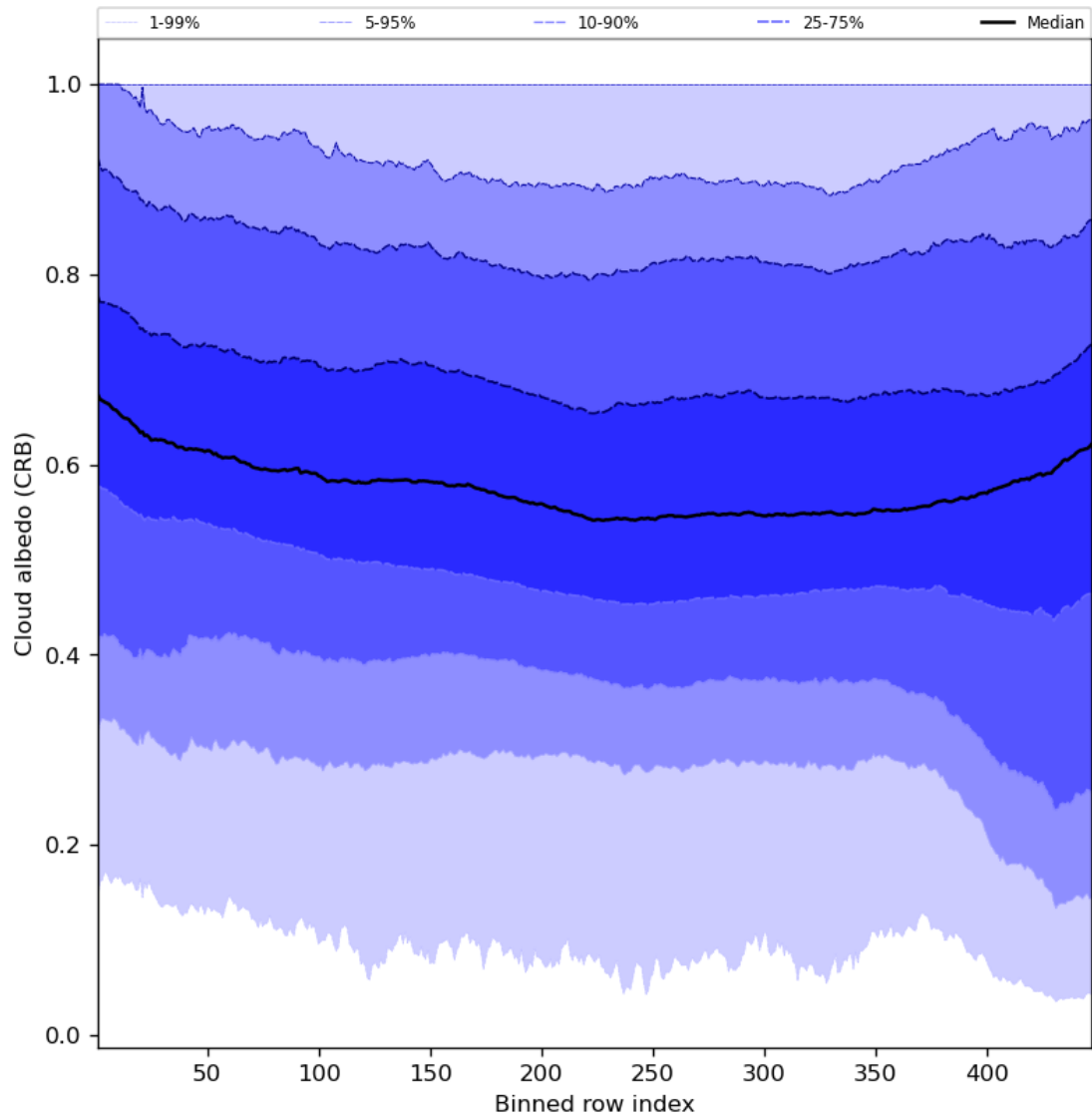
Figure 60: Along track statistics of “Cloud albedo (CRB)” for 2023-07-31 to 2023-08-02
