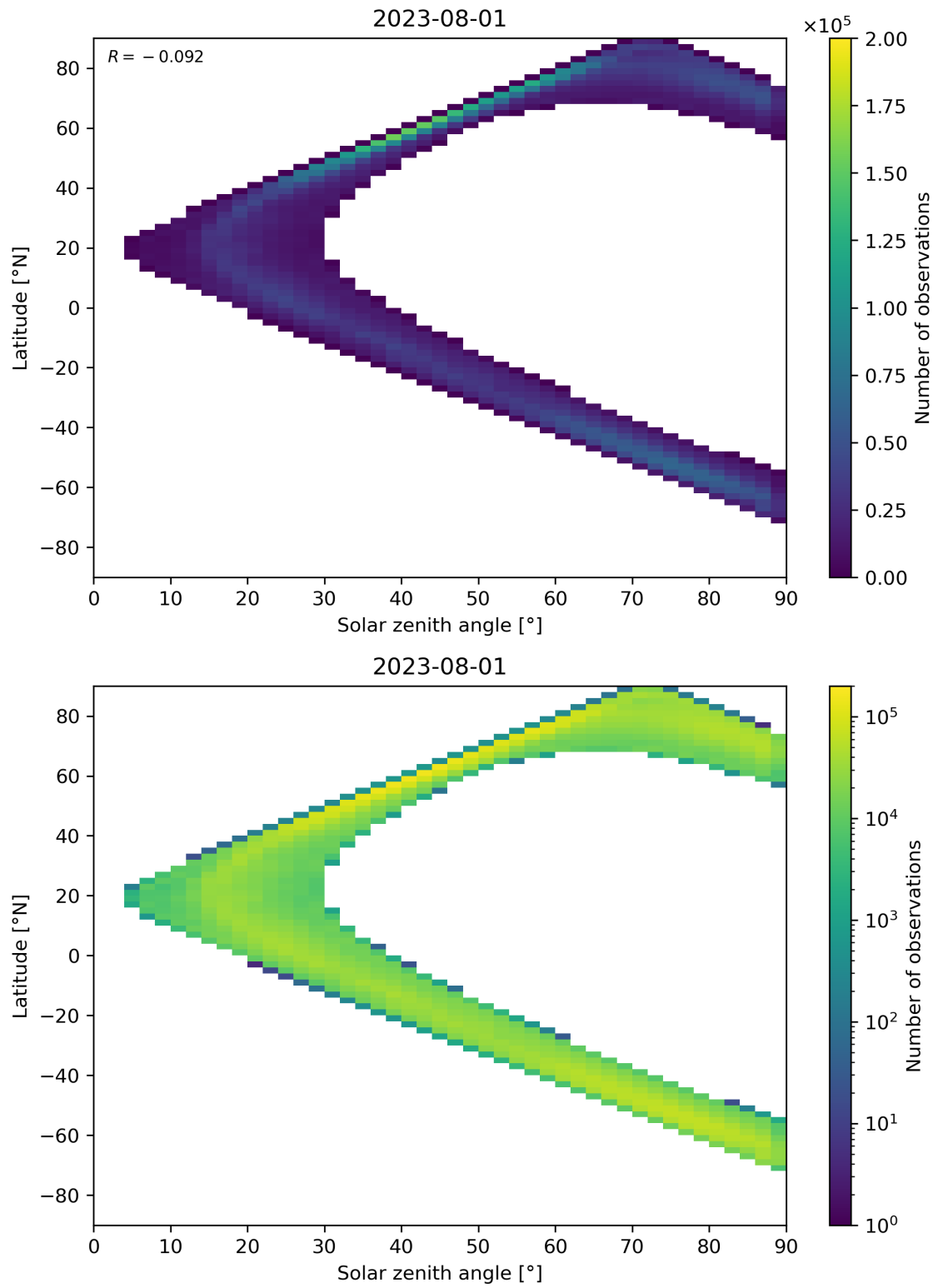
Figure 105: Scatter density plot of “Solar zenith angle” against “Latitude” for 2023-07-31 to 2023-08-02.
