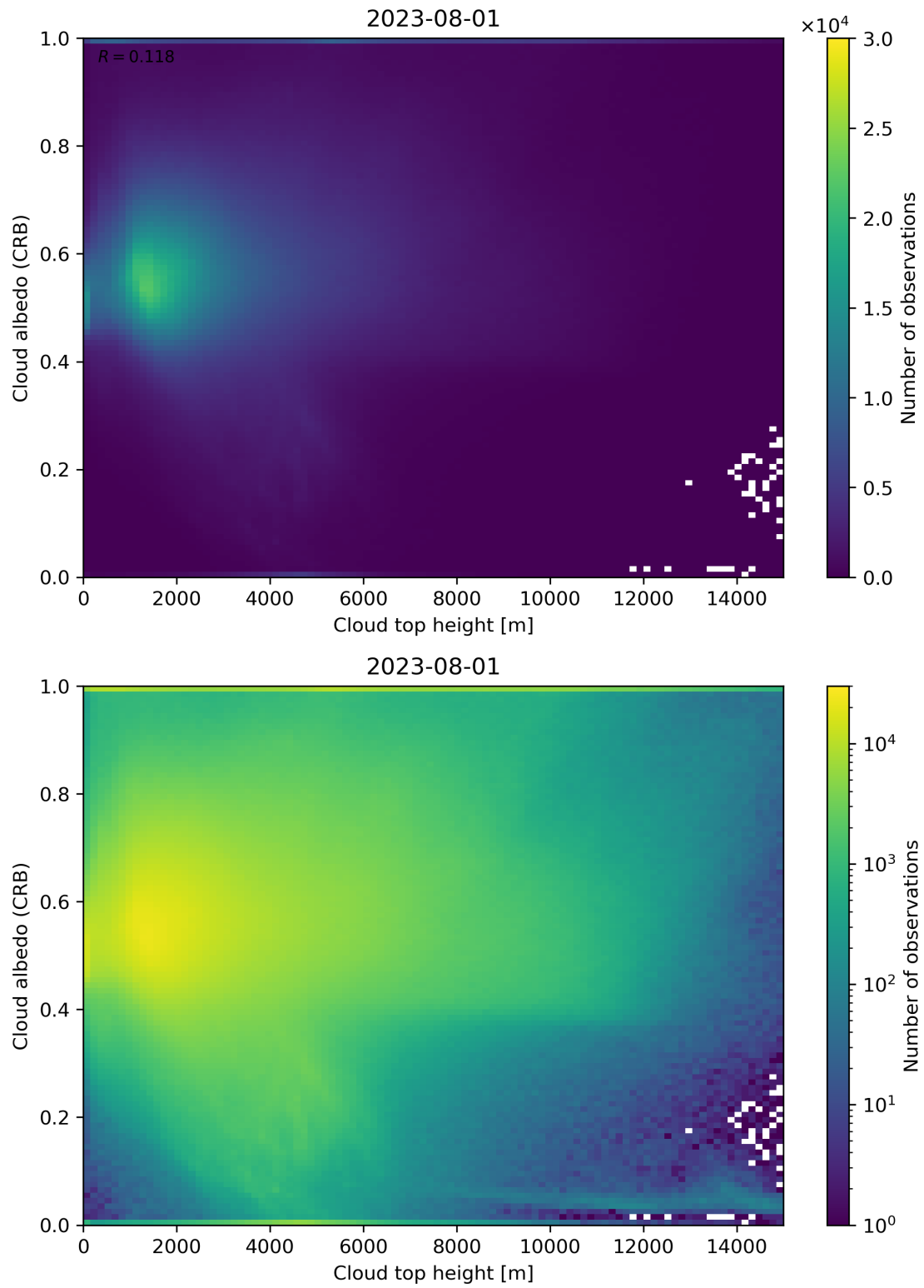
Figure 86: Scatter density plot of “Cloud top height” against “Cloud albedo (CRB)” for 2023-07-31 to 2023-08-02.
