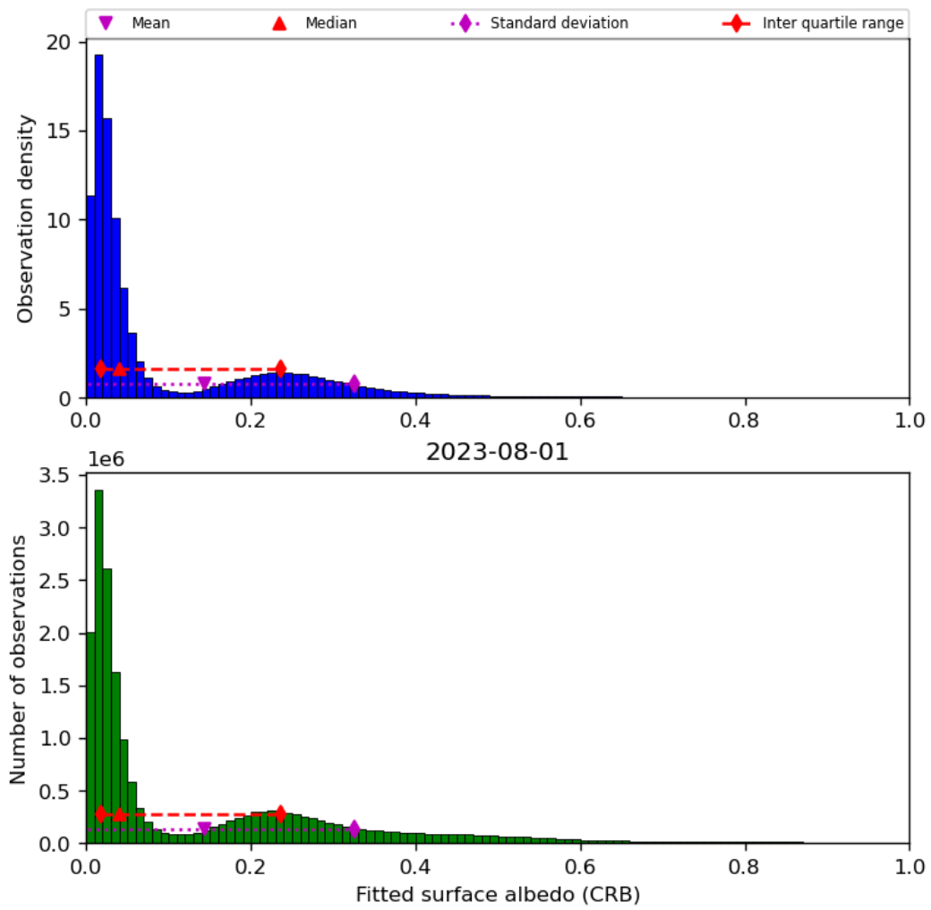
Figure 46: Histogram of “Fitted surface albedo (CRB)” for 2023-07-31 to 2023-08-02
