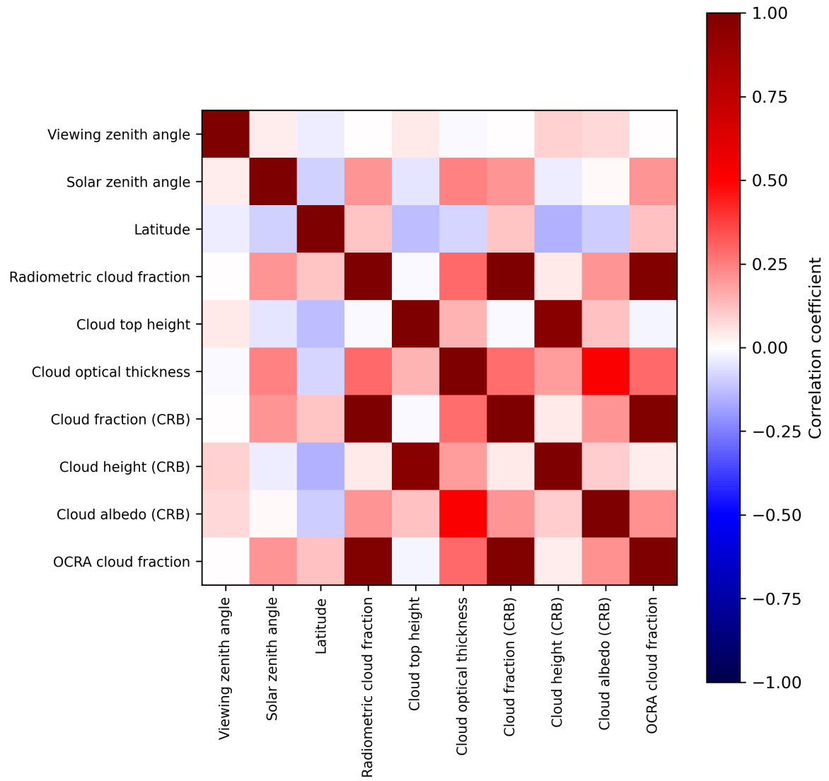
Figure 2: Map of correlation matrix for 2023-07-31 to 2023-08-02.
