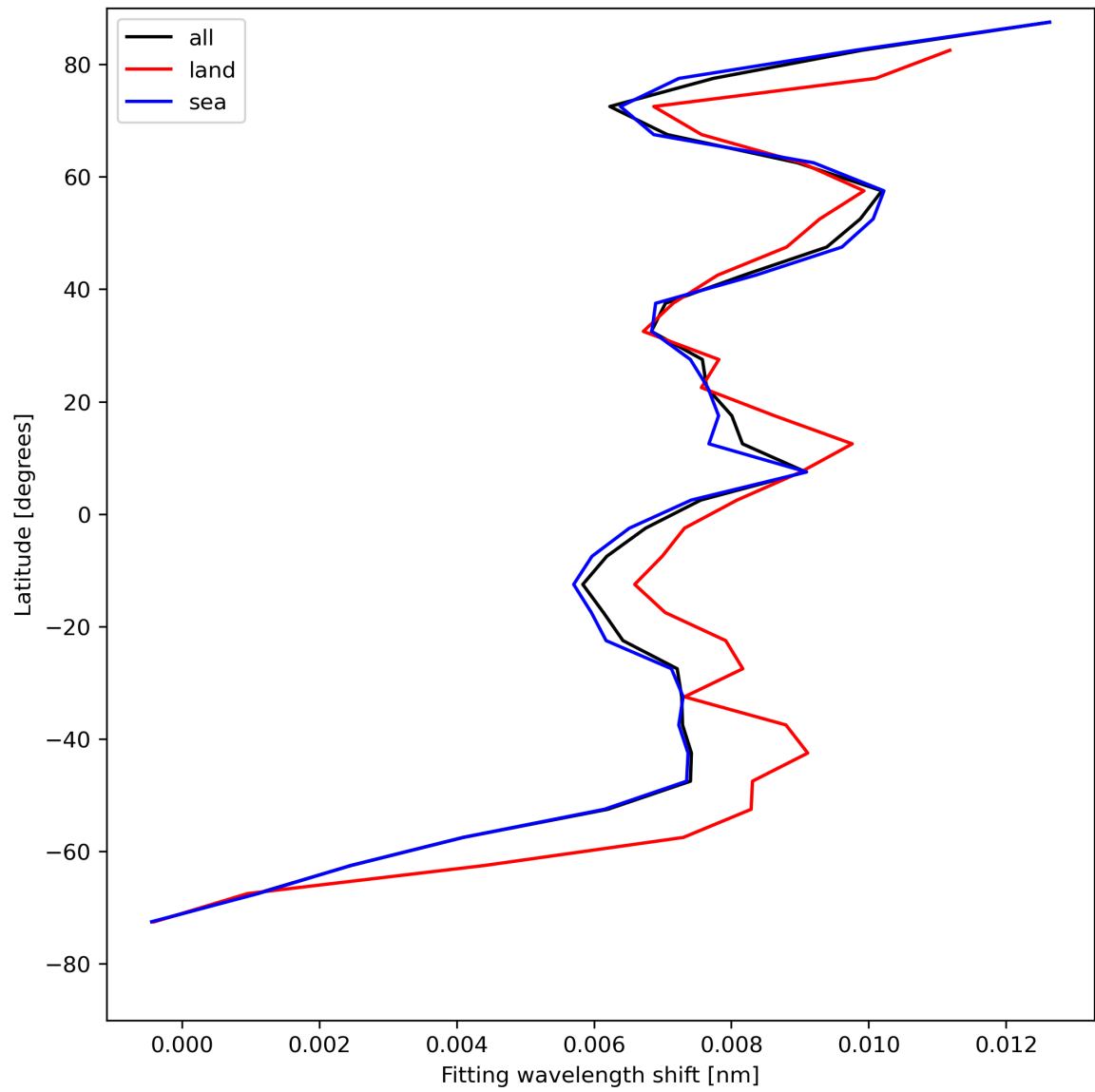
Figure 33: Zonal average of “Fitting wavelength shift” for 2023-07-31 to 2023-08-02.
