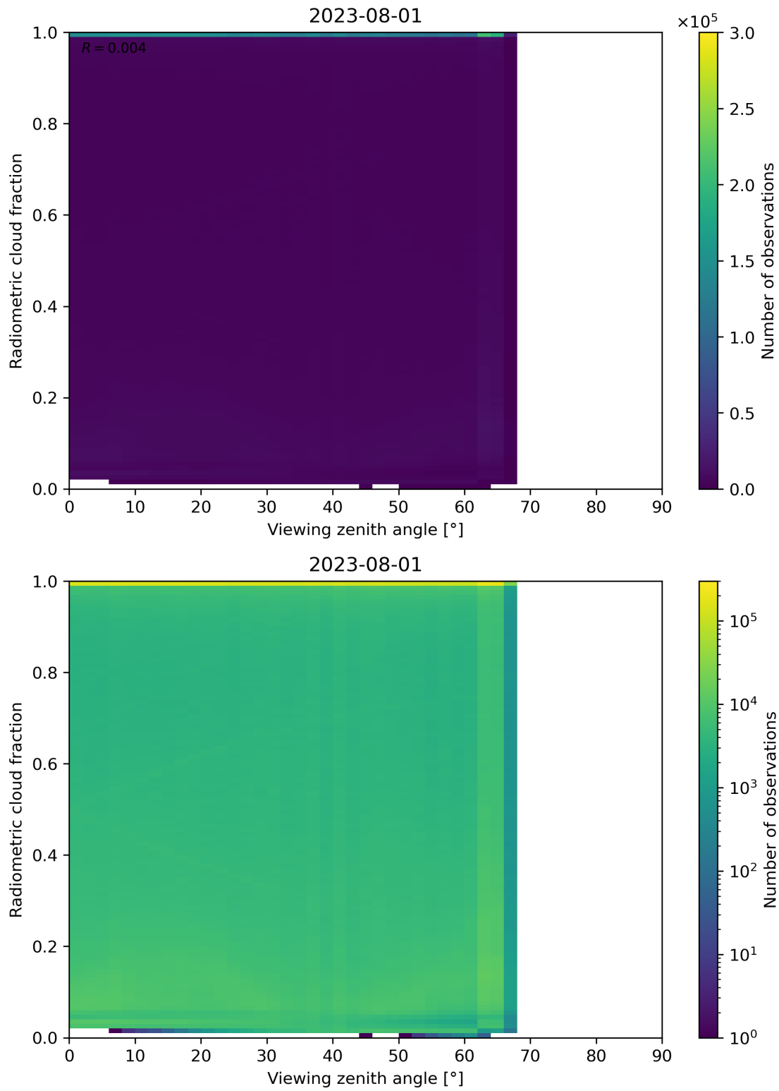
Figure 107: Scatter density plot of “Viewing zenith angle” against “Radiometric cloud fraction” for 2023-07-31 to 2023-08-02.
