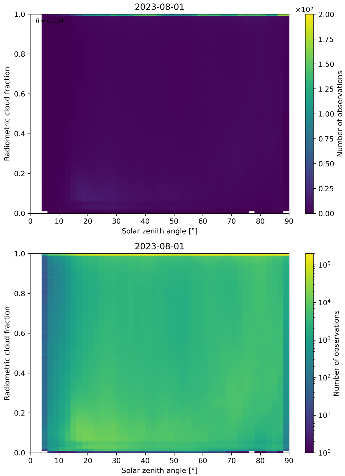
Figure 99: Scatter density plot of “Solar zenith angle” against “Radiometric cloud fraction” for 2023-07-31 to 2023-08-02.
