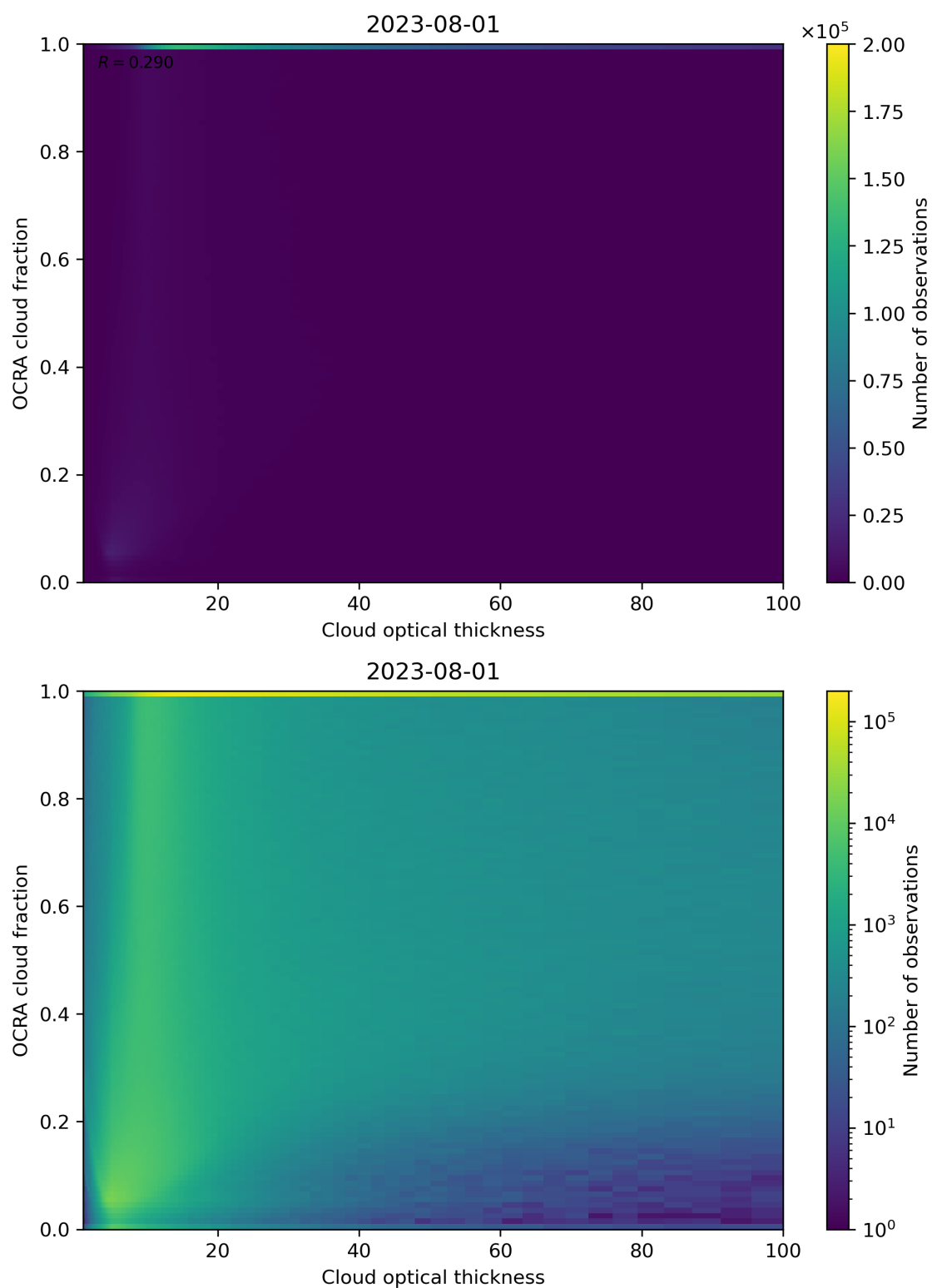
Figure 83: Scatter density plot of “Cloud optical thickness” against “OCRA cloud fraction” for 2023-07-31 to 2023-08-02.
