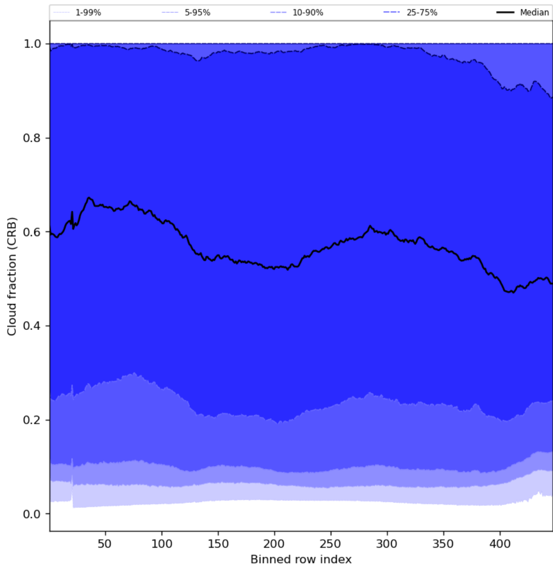
Figure 58: Along track statistics of “Cloud fraction (CRB)” for 2023-07-31 to 2023-08-02
