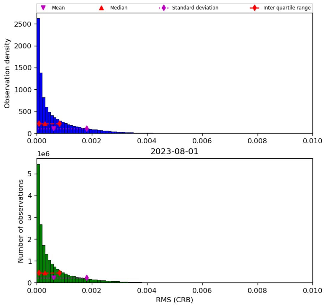
Figure 48: Histogram of “RMS (CRB)” for 2023-07-31 to 2023-08-02
