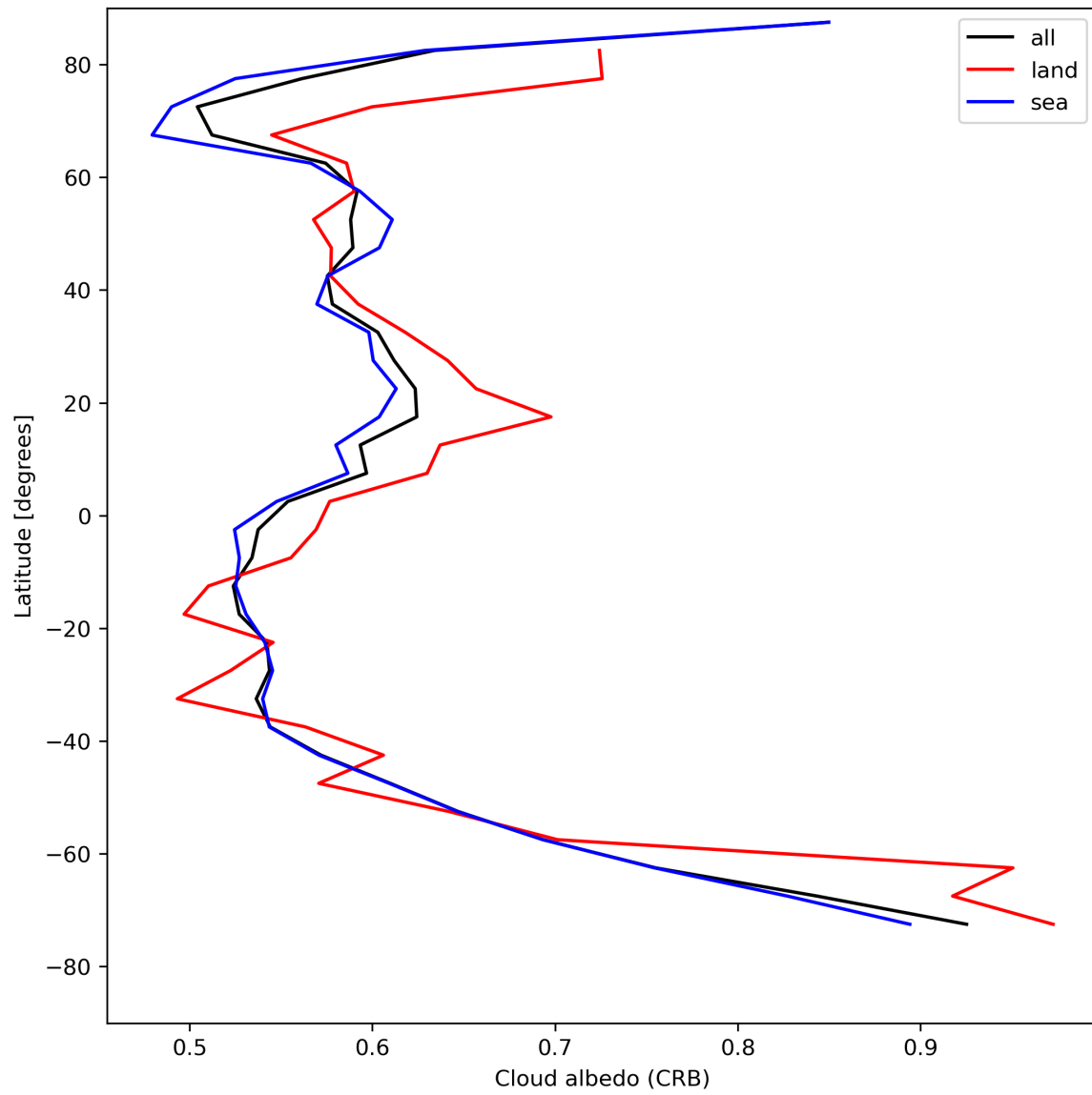
Figure 28: Zonal average of “Cloud albedo (CRB)” for 2023-07-31 to 2023-08-02.
