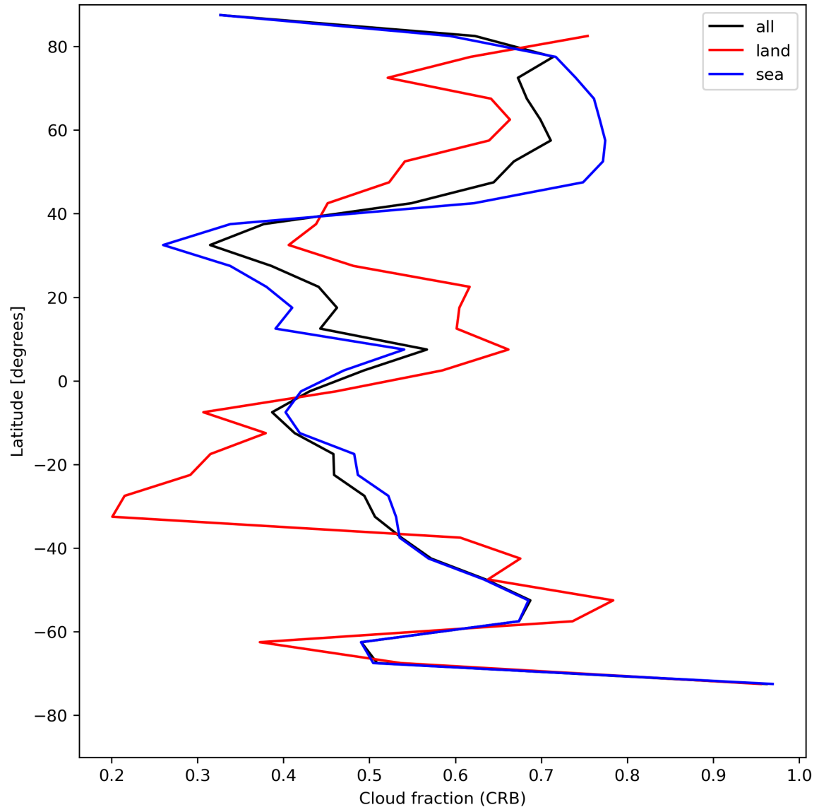
Figure 26: Zonal average of “Cloud fraction (CRB)” for 2023-07-31 to 2023-08-02.
