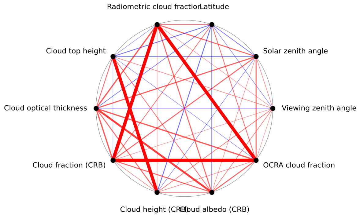
Figure 1: Map of correlation graph for 2023-07-31 to 2023-08-02.
