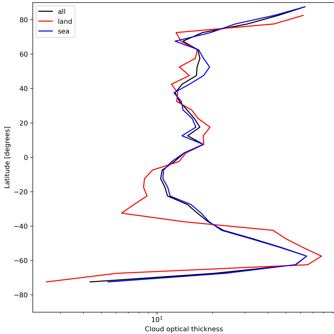
Figure 25: Zonal average of “Cloud optical thickness” for 2023-07-31 to 2023-08-02.
