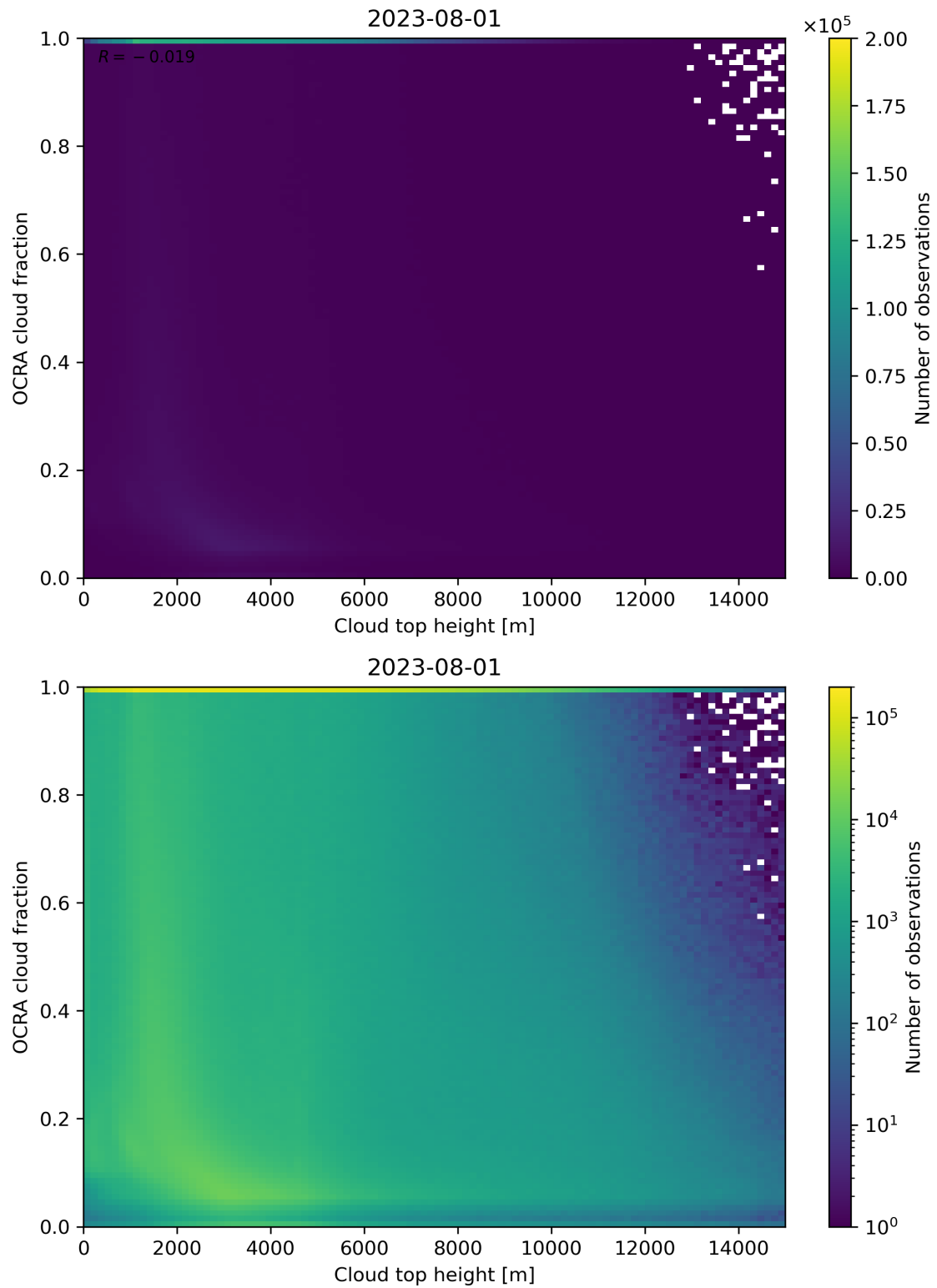
Figure 87: Scatter density plot of “Cloud top height” against “OCRA cloud fraction” for 2023-07-31 to 2023-08-02.
