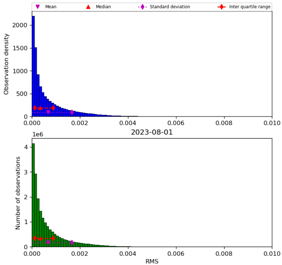
Figure 47: Histogram of “RMS” for 2023-07-31 to 2023-08-02
