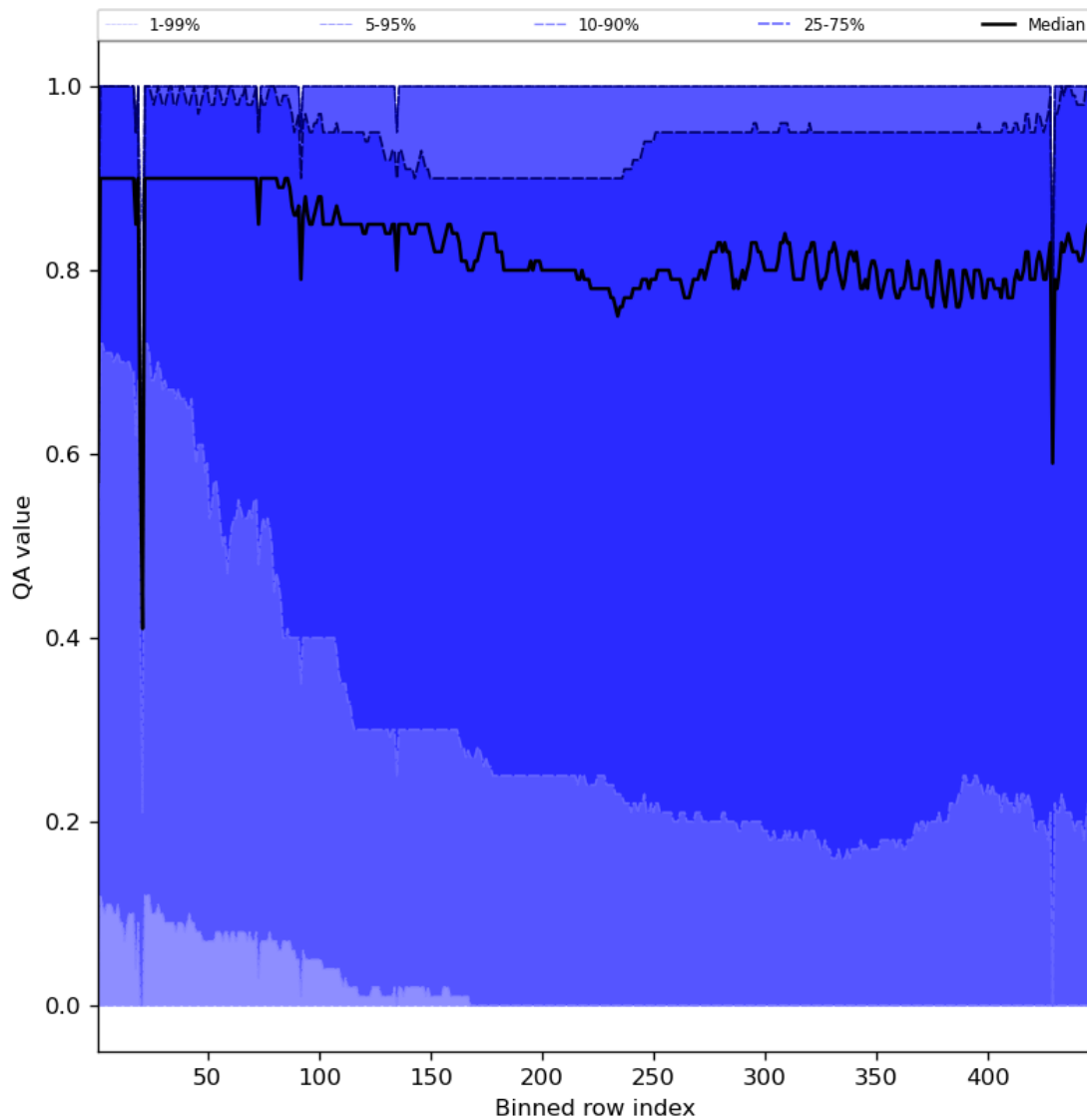
Figure 54: Along track statistics of “QA value” for 2023-07-31 to 2023-08-02
