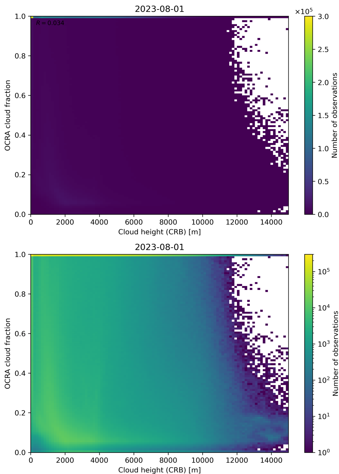
Figure 81: Scatter density plot of “Cloud height (CRB)” against “OCRA cloud fraction” for 2023-07-31 to 2023-08-02.
