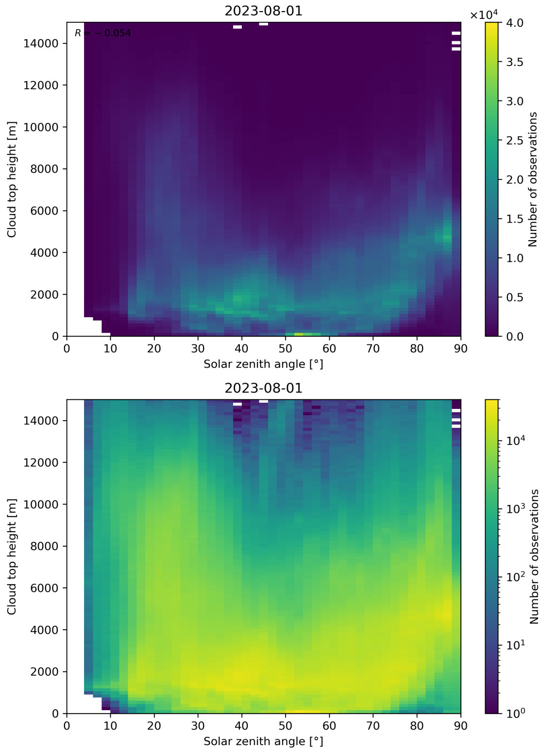
Figure 104: Scatter density plot of “Solar zenith angle” against “Cloud top height” for 2023-07-31 to 2023-08-02.
