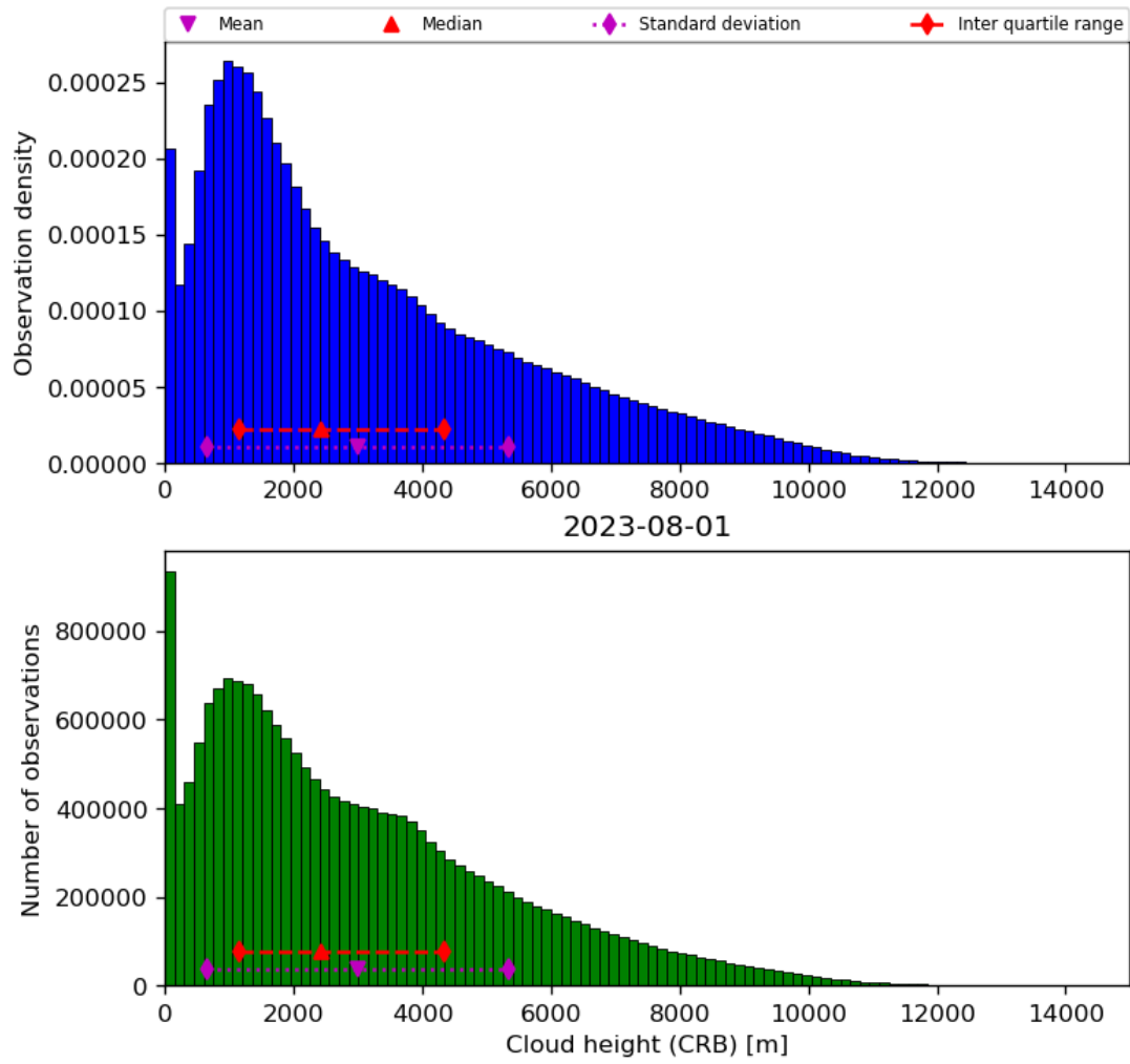
Figure 43: Histogram of “Cloud height (CRB)” for 2023-07-31 to 2023-08-02
