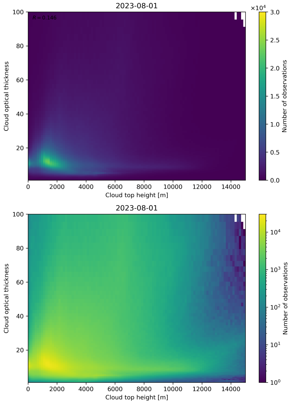
Figure 90: Scatter density plot of “Cloud top height” against “Cloud optical thickness” for 2023-07-31 to 2023-08-02.
