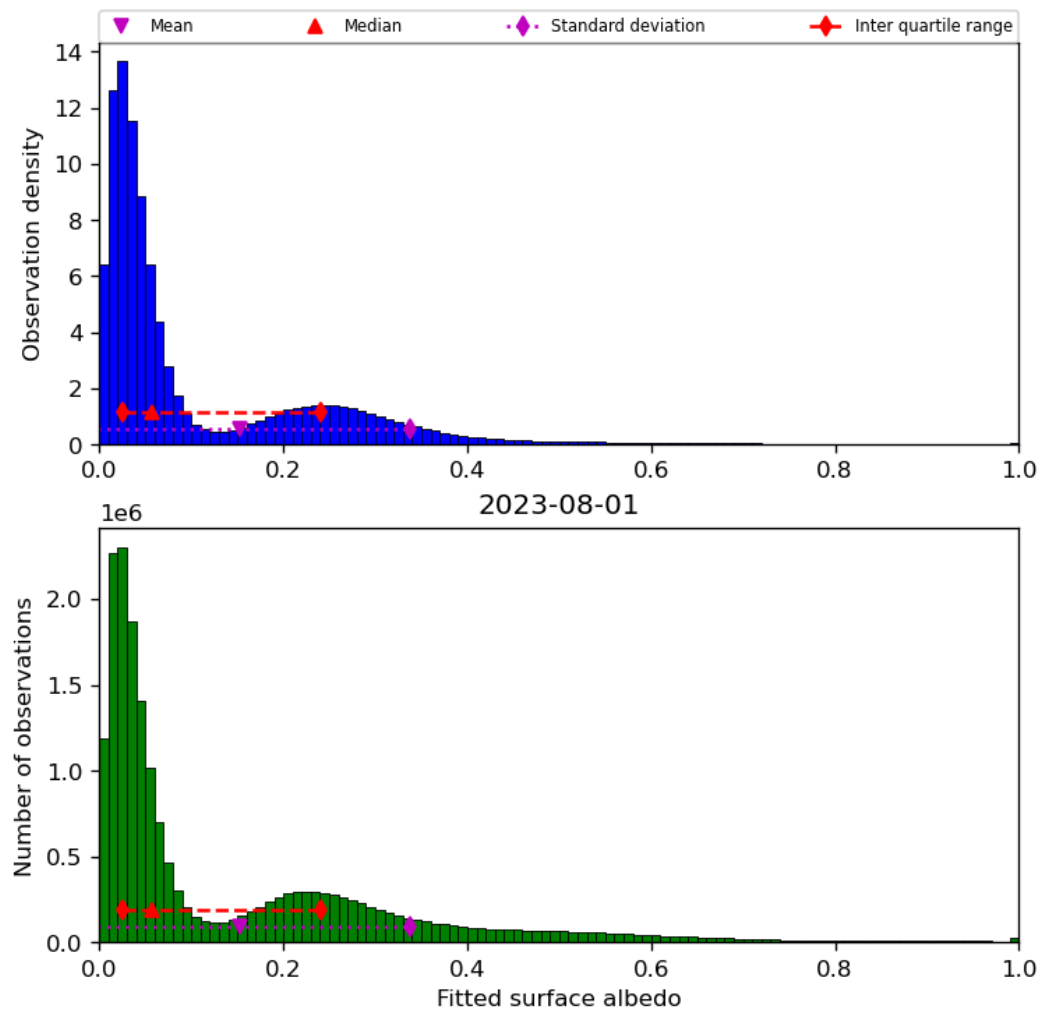
Figure 45: Histogram of “Fitted surface albedo” for 2023-07-31 to 2023-08-02
