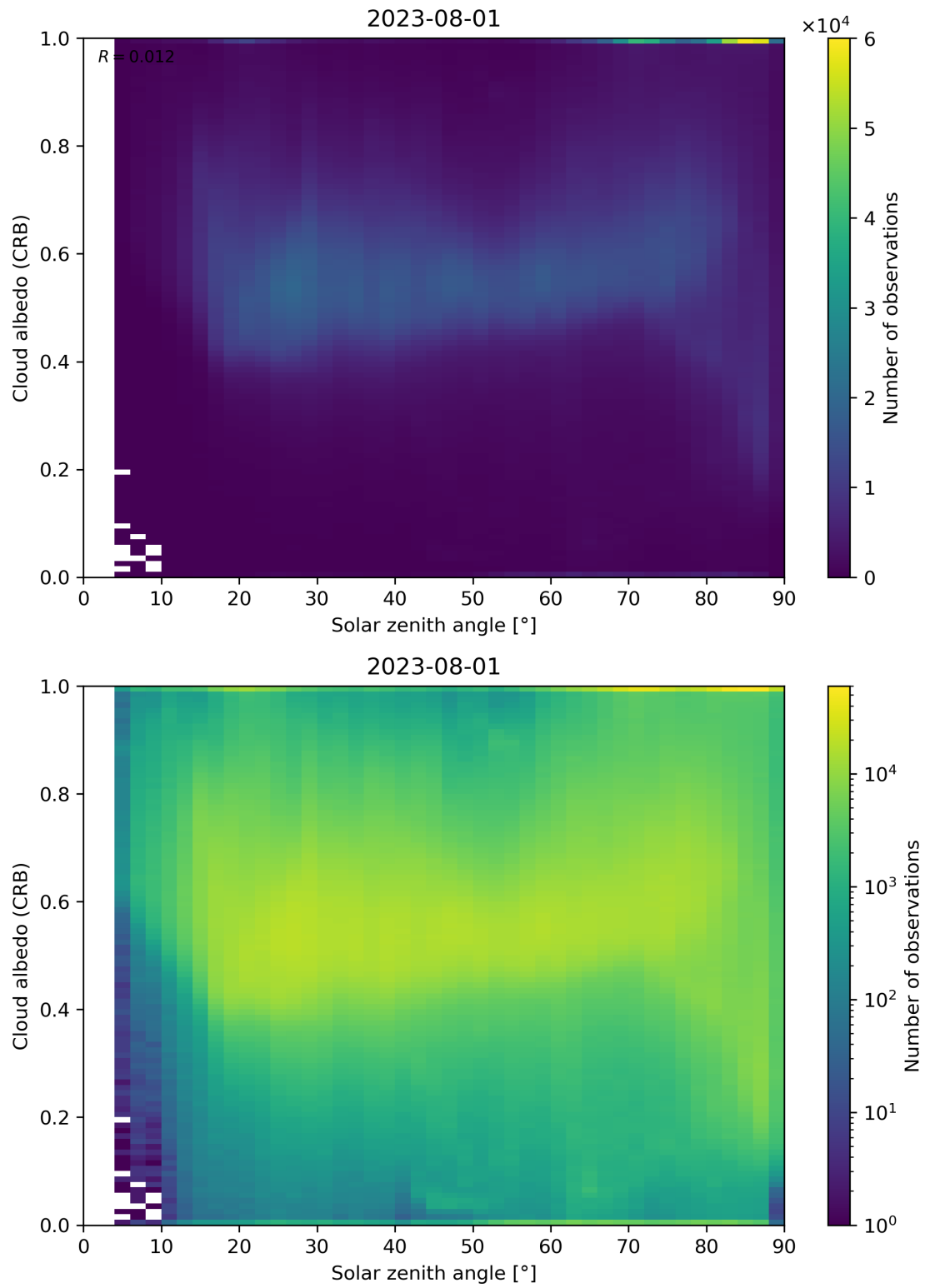
Figure 98: Scatter density plot of “Solar zenith angle” against “Cloud albedo (CRB)” for 2023-07-31 to 2023-08-02.
