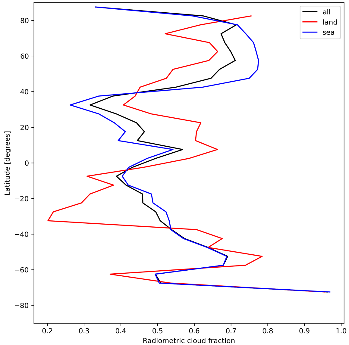
Figure 23: Zonal average of “Radiometric cloud fraction” for 2023-07-31 to 2023-08-02.
