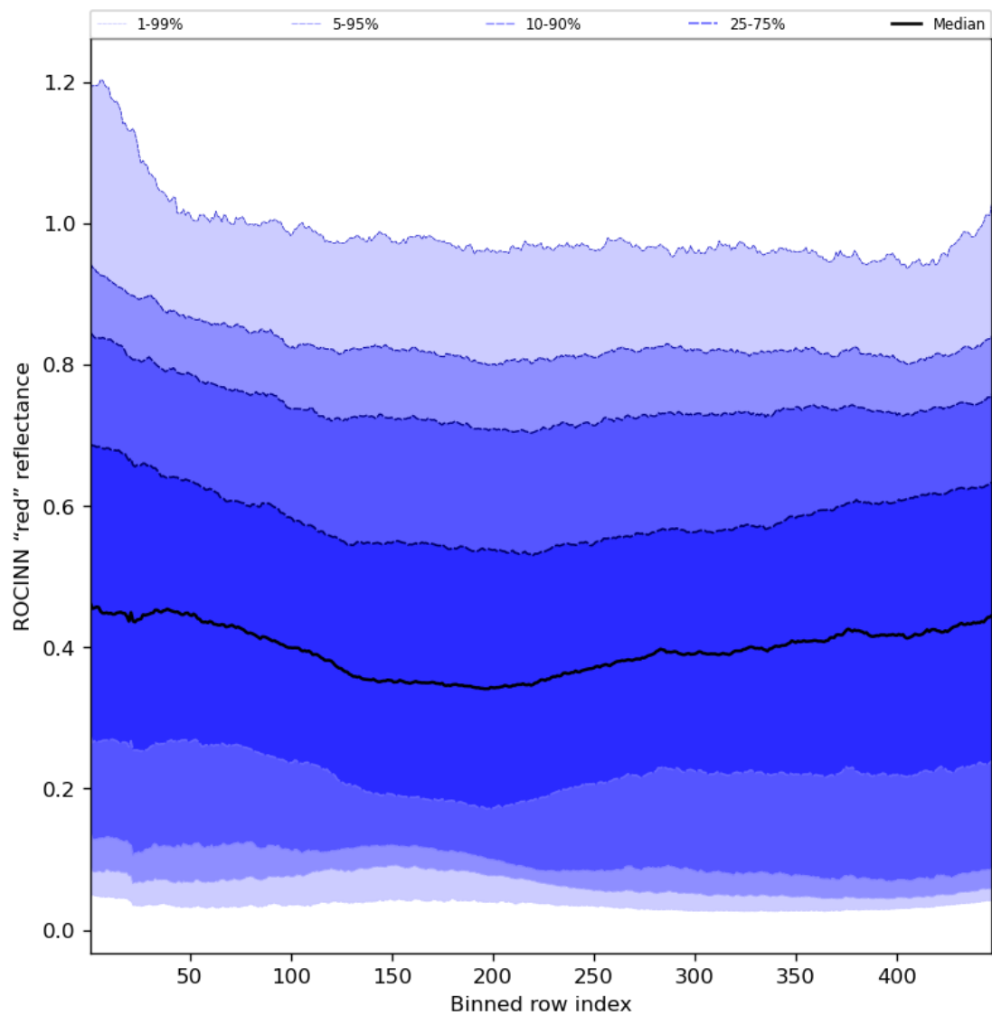
Figure 69: Along track statistics of "ROCINN "red" reflectance" for 2023-07-31 to 2023-08-02
