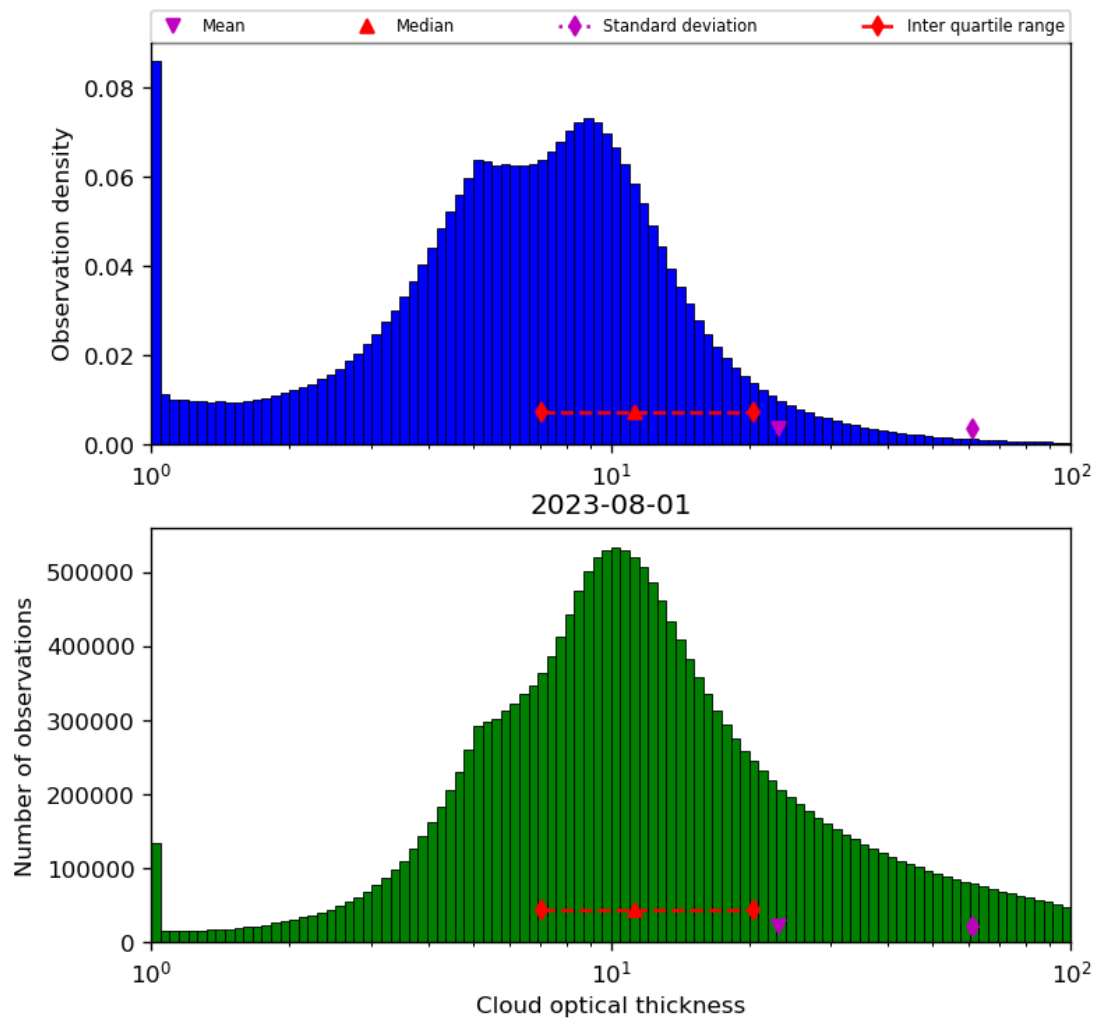
Figure 41: Histogram of “Cloud optical thickness” for 2023-07-31 to 2023-08-02
