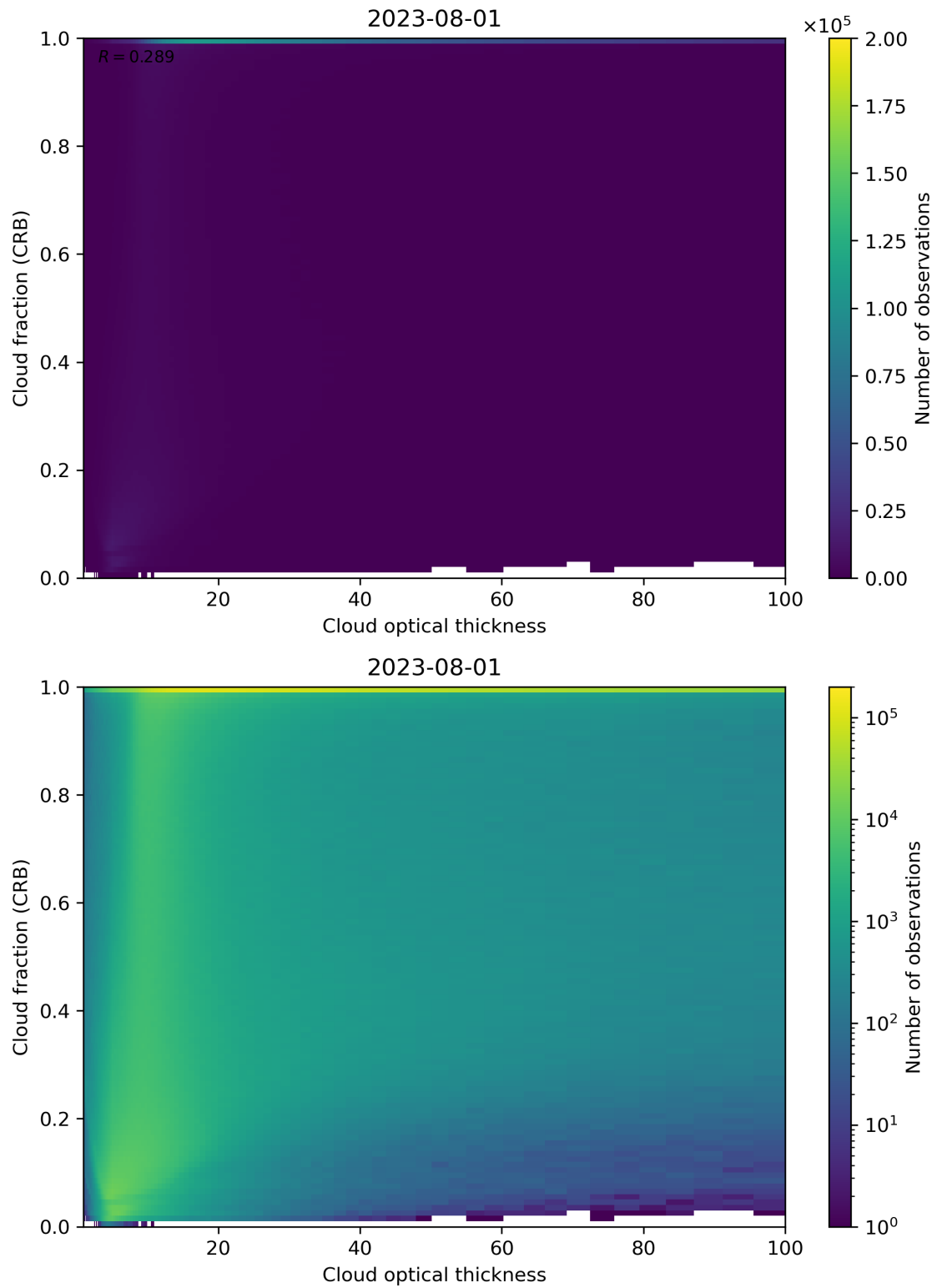
Figure 84: Scatter density plot of “Cloud optical thickness” against “Cloud fraction (CRB)” for 2023-07-31 to 2023-08-02.
