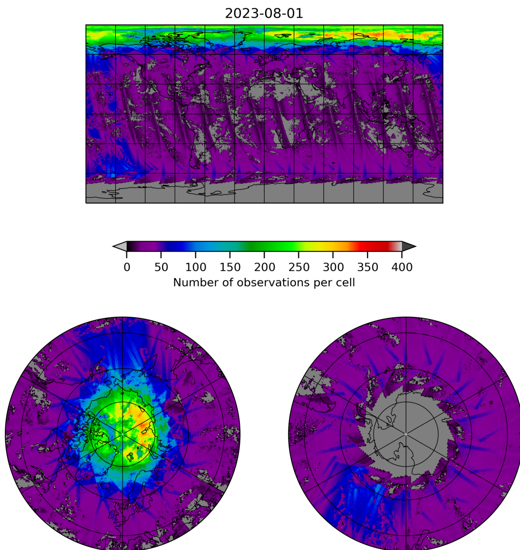
Figure 21: Map of the number of observations for 2023-07-31 to 2023-08-02
