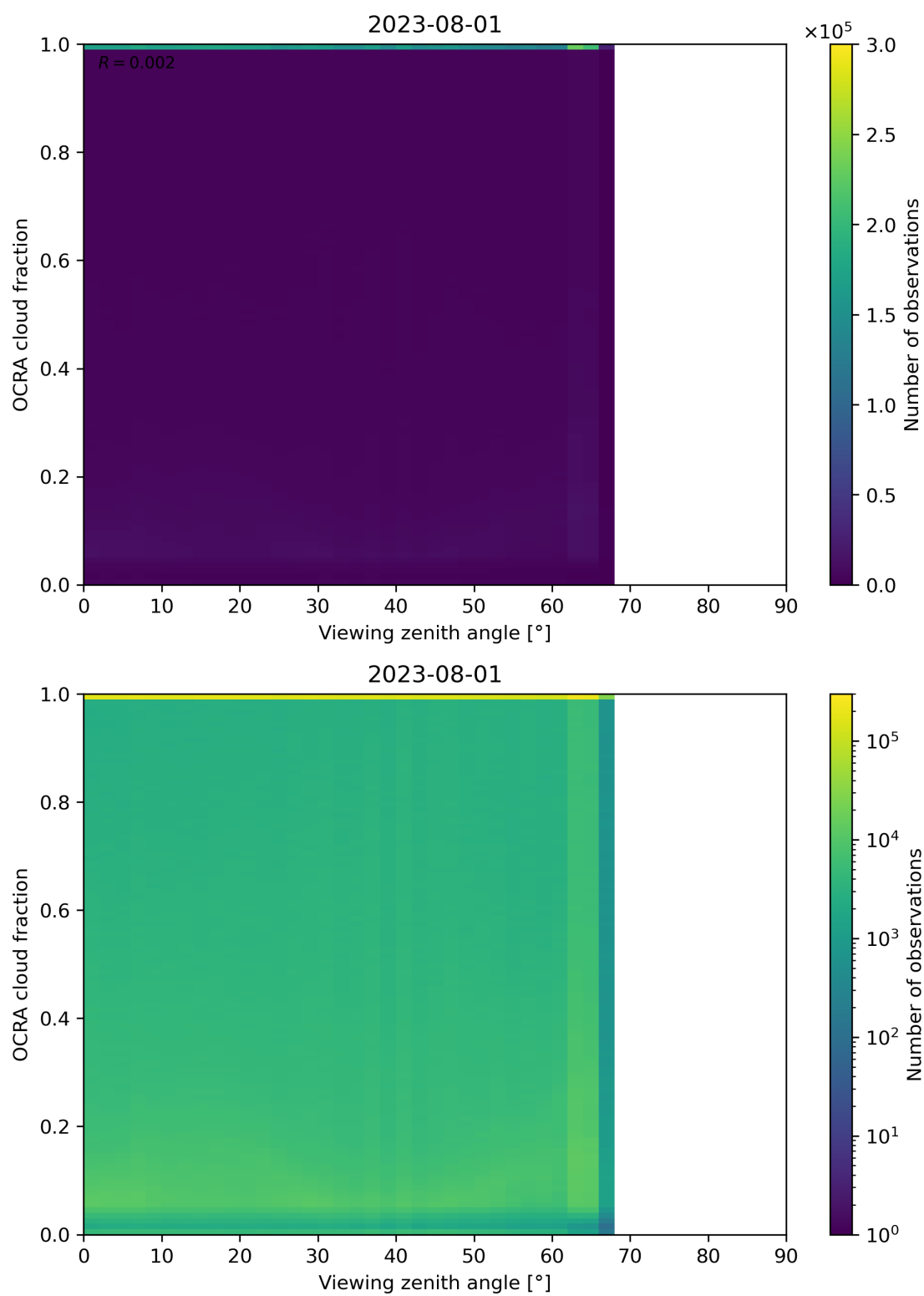
Figure 108: Scatter density plot of “Viewing zenith angle” against “OCRA cloud fraction” for 2023-07-31 to 2023-08-02.
