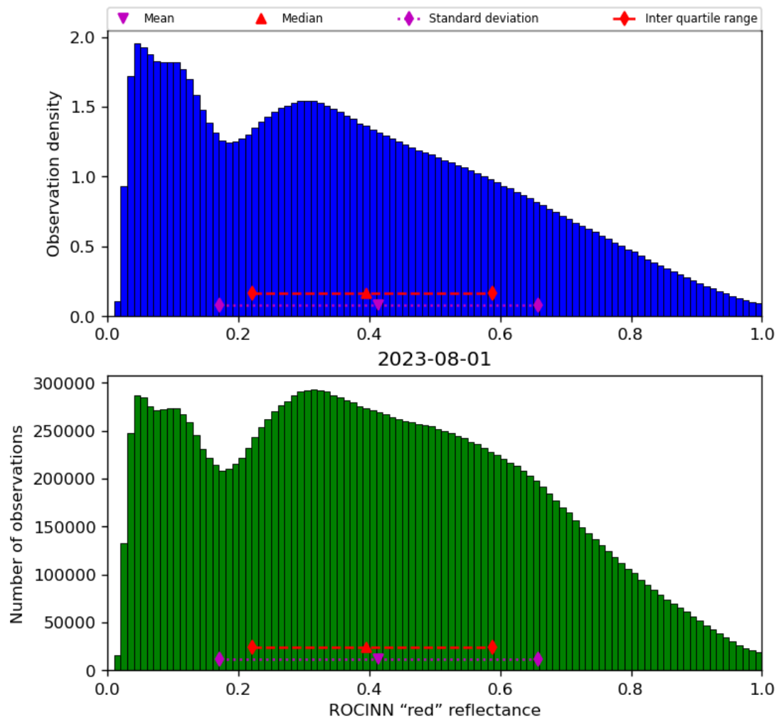
Figure 53: Histogram of “ROCINN “red” reflectance” for 2023-07-31 to 2023-08-02
