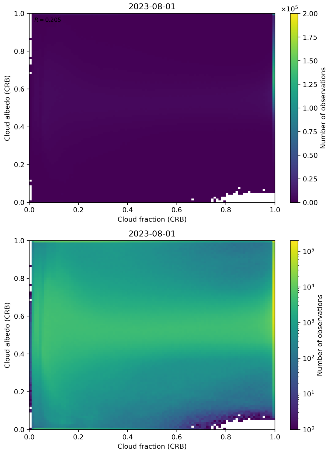
Figure 77: Scatter density plot of “Cloud fraction (CRB)” against “Cloud albedo (CRB)” for 2023-07-31 to 2023-08-02.
