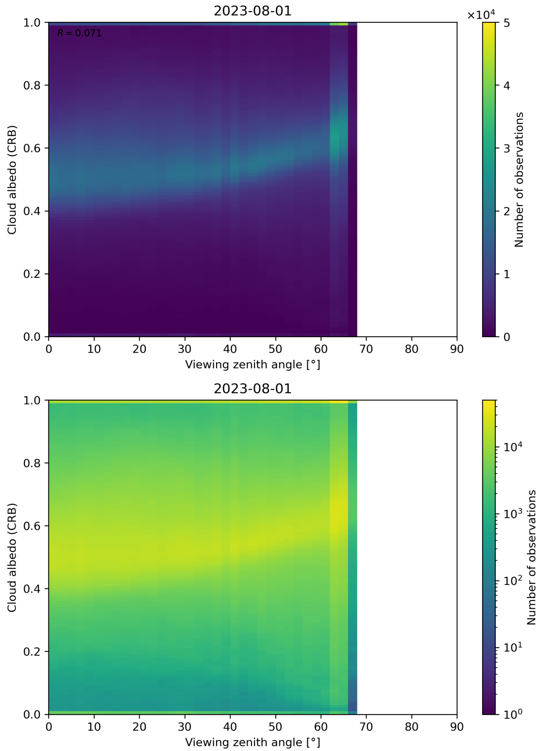
Figure 106: Scatter density plot of “Viewing zenith angle” against “Cloud albedo (CRB)” for 2023-07-31 to 2023-08-02.
