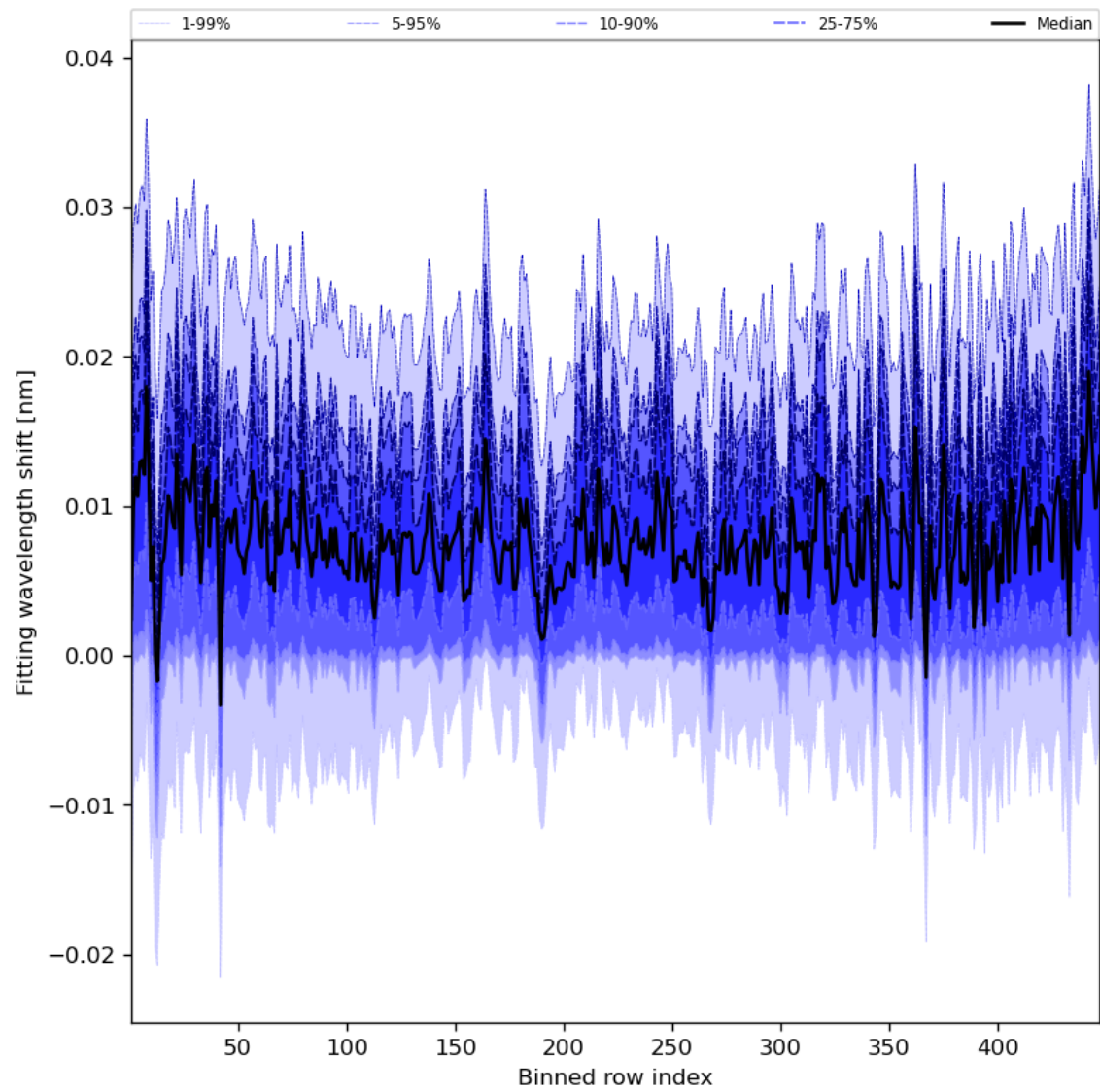
Figure 65: Along track statistics of “Fitting wavelength shift” for 2023-07-31 to 2023-08-02
