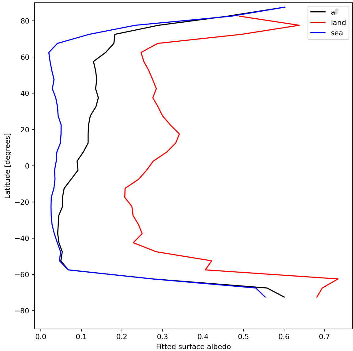
Figure 29: Zonal average of “Fitted surface albedo” for 2023-07-31 to 2023-08-02.
