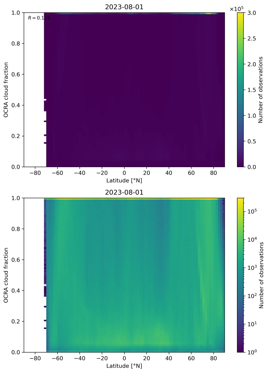
Figure 93: Scatter density plot of “Latitude” against “OCRA cloud fraction” for 2023-07-31 to 2023-08-02.
