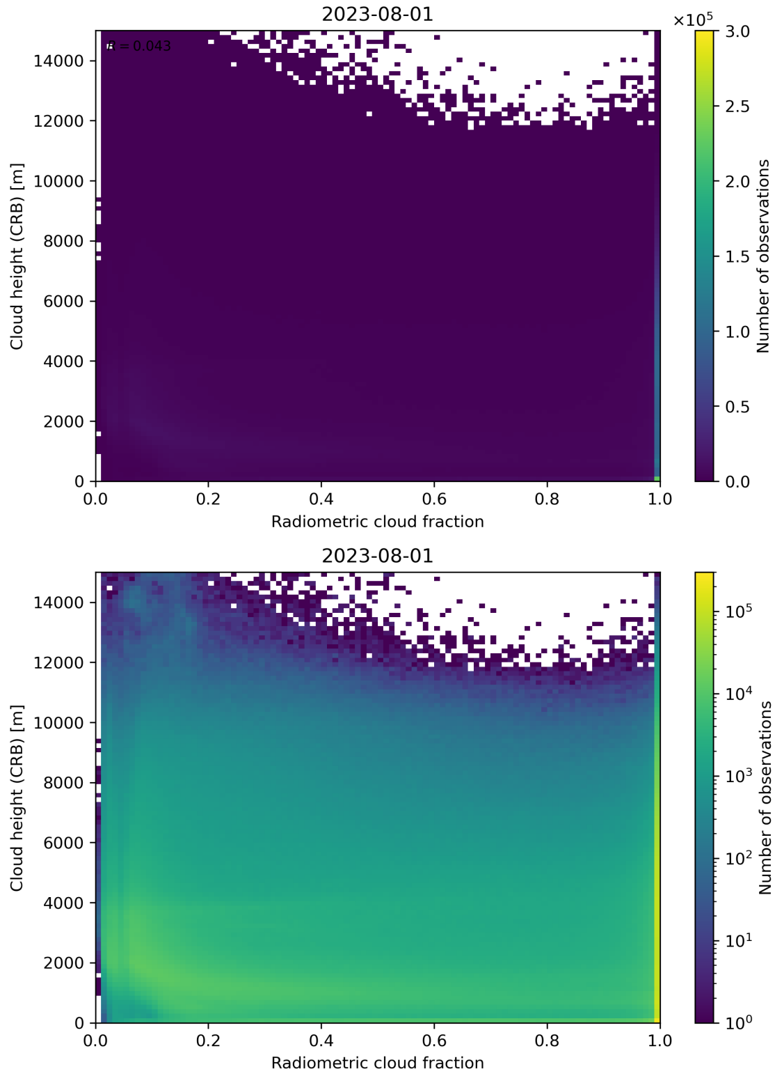
Figure 74: Scatter density plot of “Radiometric cloud fraction” against “Cloud height (CRB)” for 2023-07-31 to 2023-08-02.
