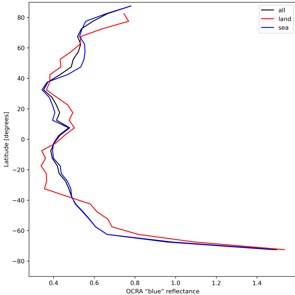
Figure 35: Zonal average of “OCRA “blue” reflectance” for 2023-07-31 to 2023-08-02.
