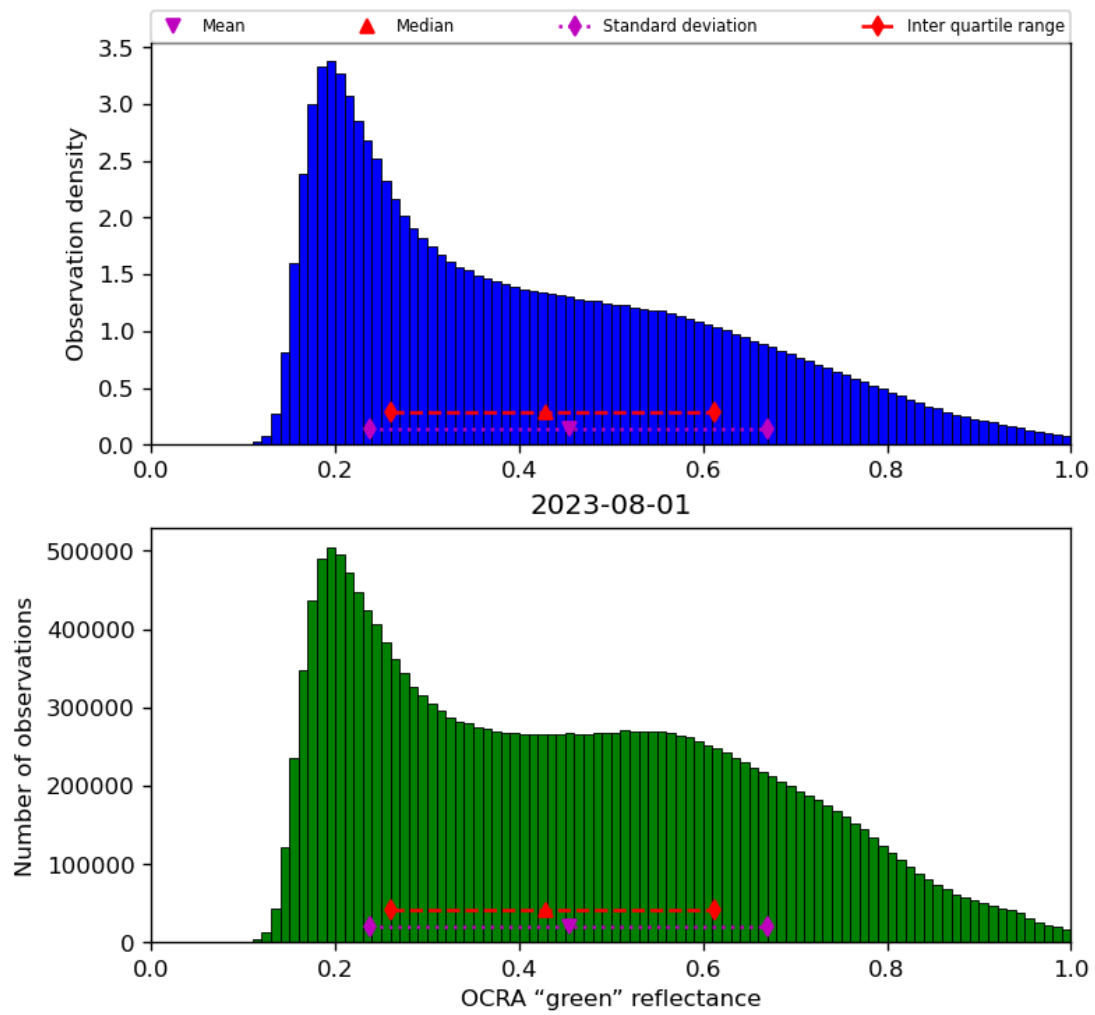
Figure 52: Histogram of “OCRA “green” reflectance” for 2023-07-31 to 2023-08-02
