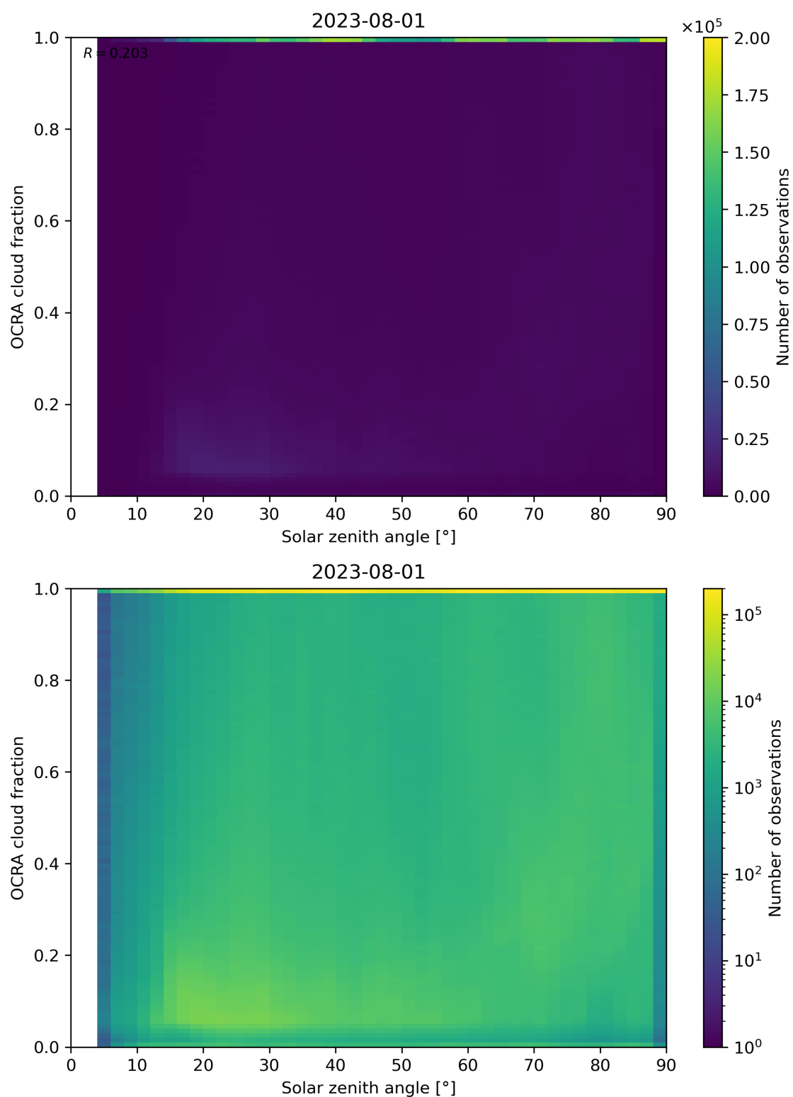
Figure 100: Scatter density plot of “Solar zenith angle” against “OCRA cloud fraction” for 2023-07-31 to 2023-08-02.
