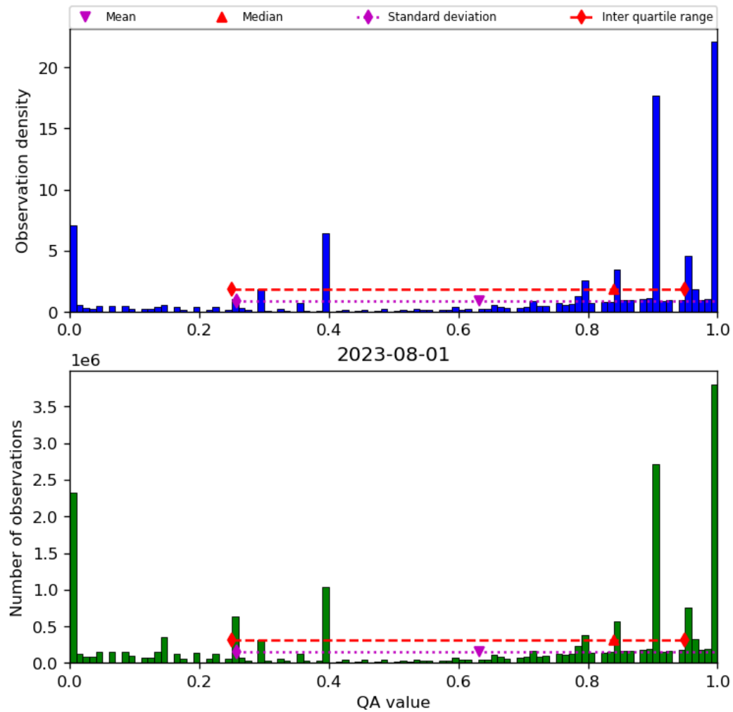
Figure 38: Histogram of “QA value” for 2023-07-31 to 2023-08-02
