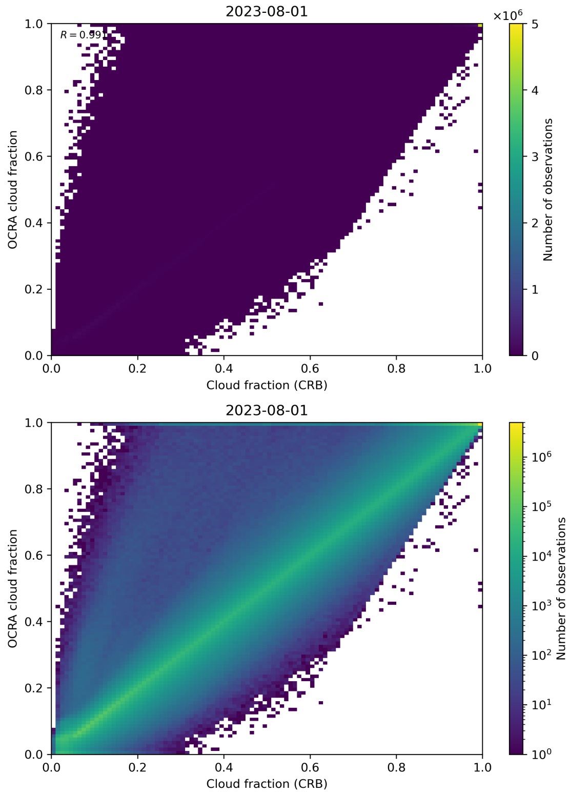
Figure 78: Scatter density plot of “Cloud fraction (CRB)” against “OCRA cloud fraction” for 2023-07-31 to 2023-08-02.
