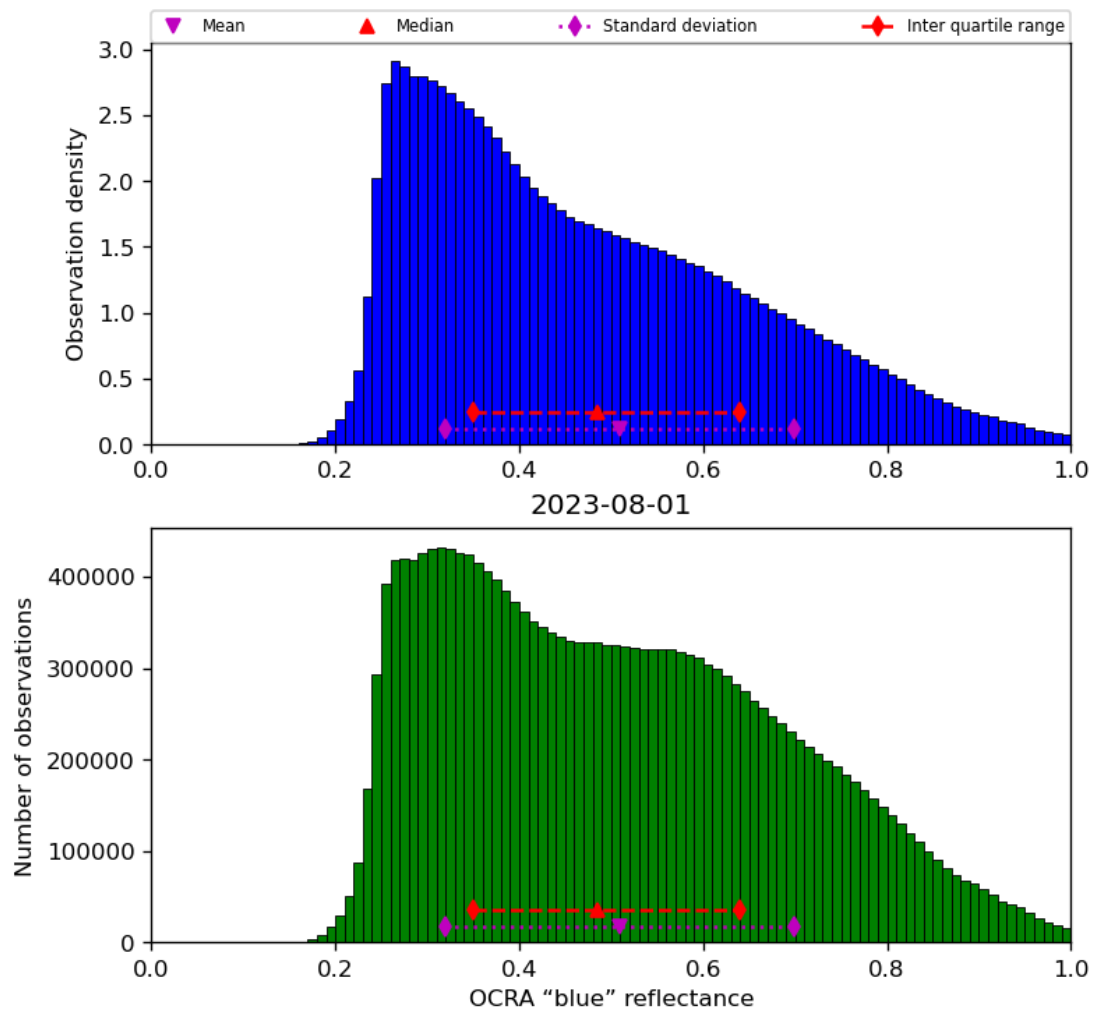
Figure 51: Histogram of “OCRA “blue” reflectance” for 2023-07-31 to 2023-08-02
