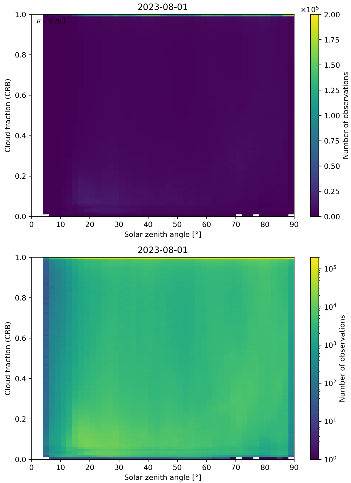
Figure 101: Scatter density plot of “Solar zenith angle” against “Cloud fraction (CRB)” for 2023-07-31 to 2023-08-02.
