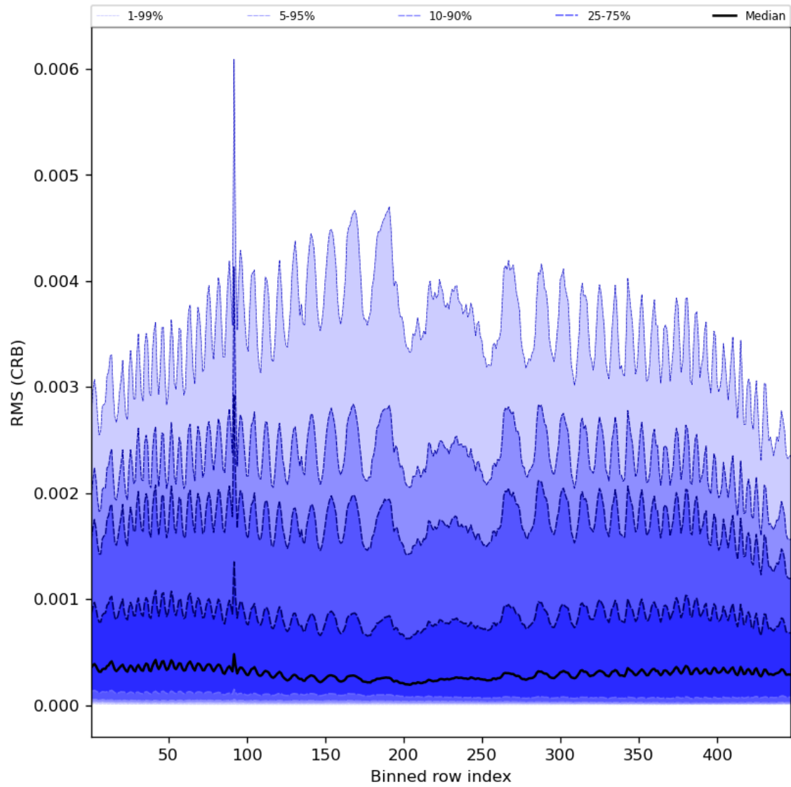
Figure 64: Along track statistics of “RMS (CRB)” for 2023-07-31 to 2023-08-02
