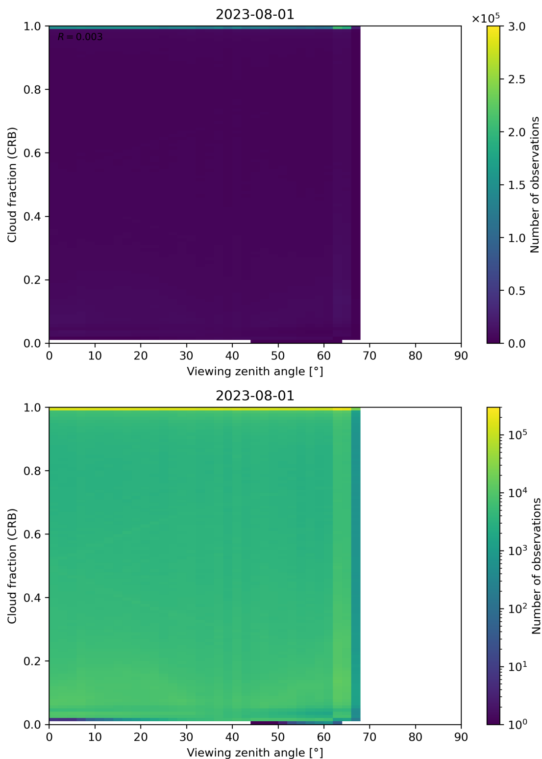
Figure 109: Scatter density plot of “Viewing zenith angle” against “Cloud fraction (CRB)” for 2023-07-31 to 2023-08-02.
