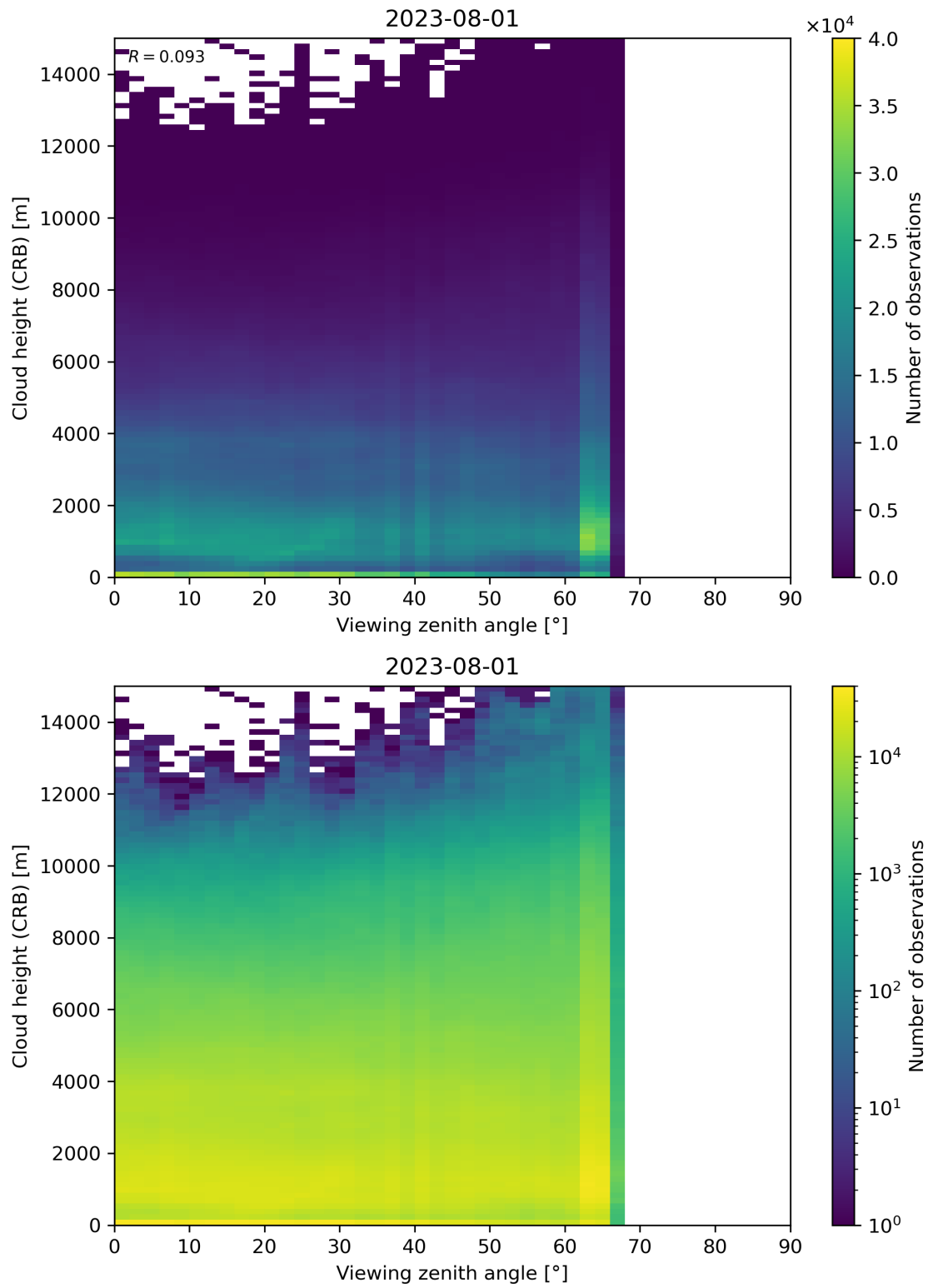
Figure 110: Scatter density plot of “Viewing zenith angle” against “Cloud height (CRB)” for 2023-07-31 to 2023-08-02.
