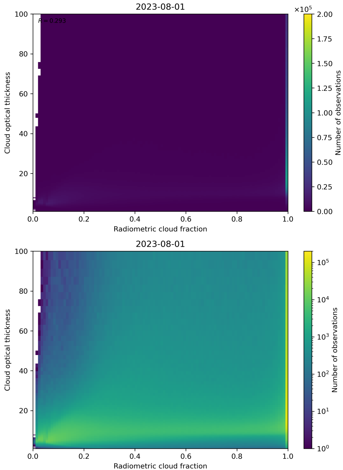
Figure 75: Scatter density plot of “Radiometric cloud fraction” against “Cloud optical thickness” for 2023-07-31 to 2023-08-02.
