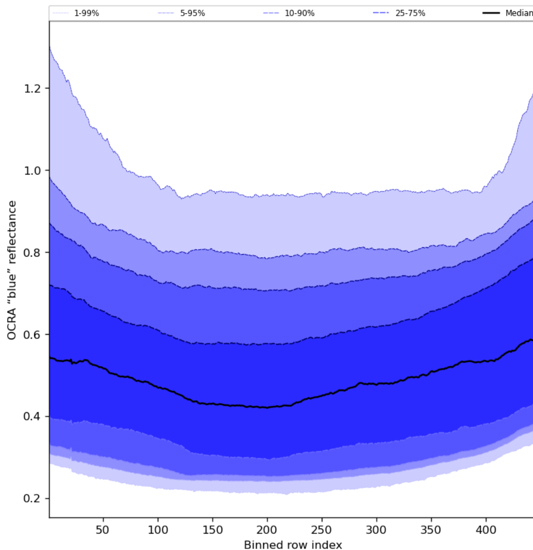
Figure 67: Along track statistics of “OCRA “blue” reflectance” for 2023-07-31 to 2023-08-02
