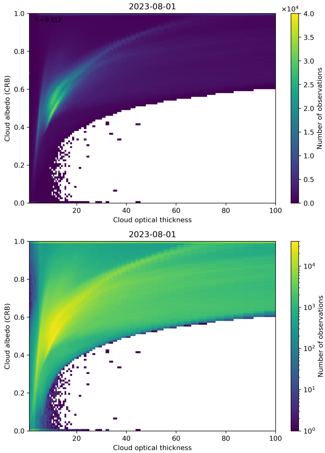
Figure 82: Scatter density plot of “Cloud optical thickness” against “Cloud albedo (CRB)” for 2023-07-31 to 2023-08-02.
