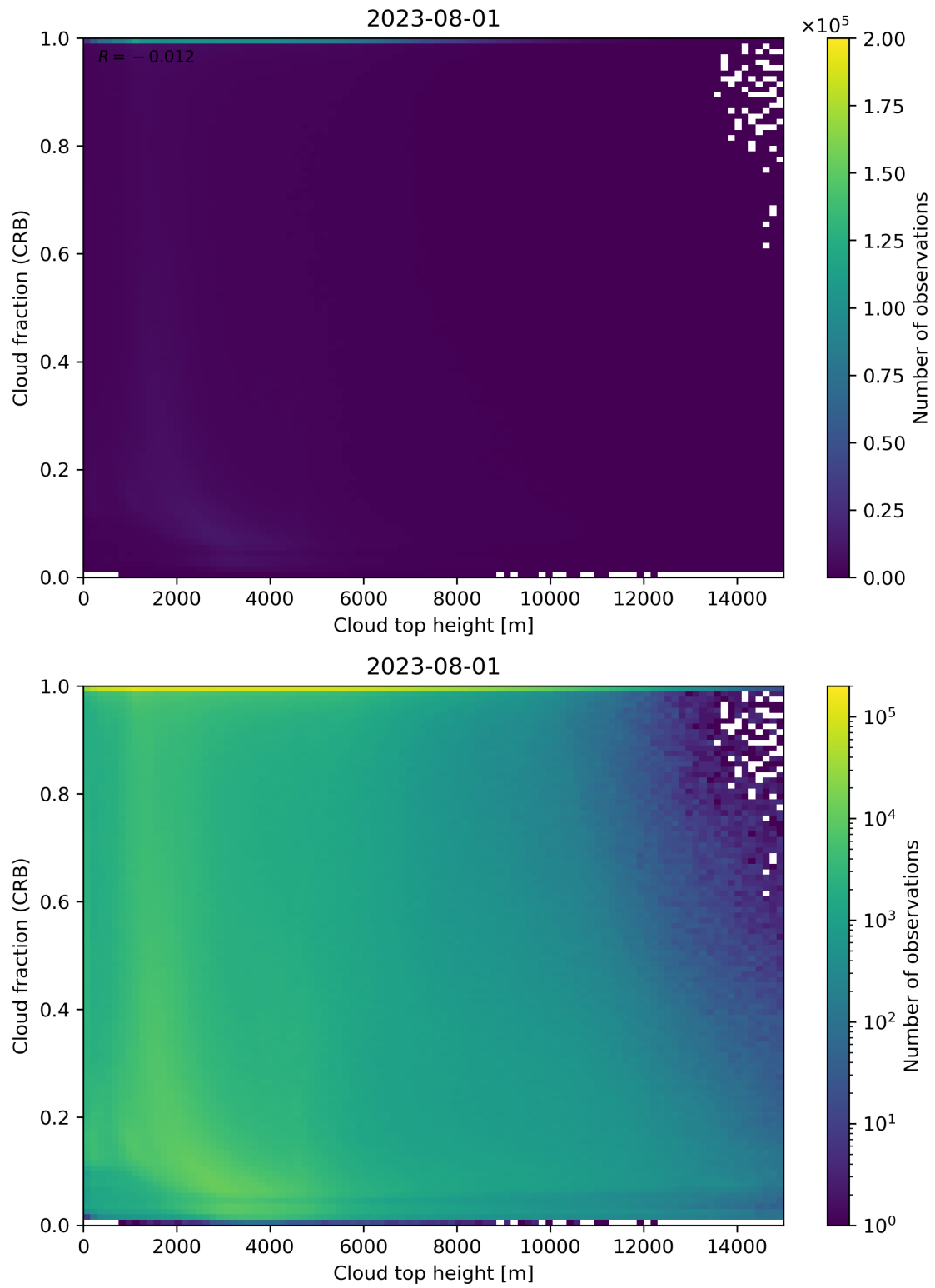
Figure 88: Scatter density plot of “Cloud top height” against “Cloud fraction (CRB)” for 2023-07-31 to 2023-08-02.
