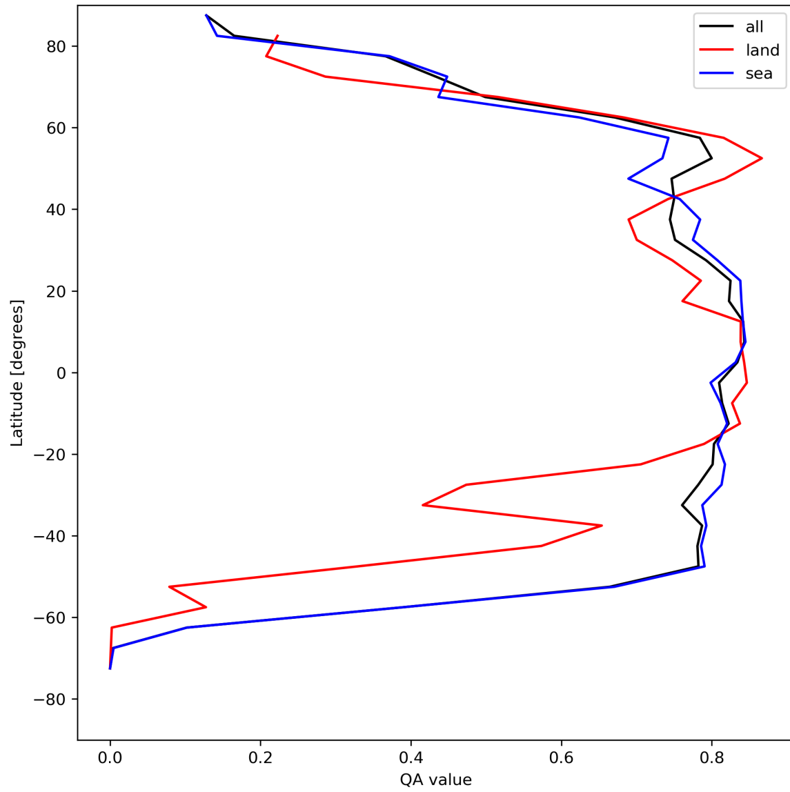
Figure 22: Zonal average of “QA value” for 2023-07-31 to 2023-08-02.
