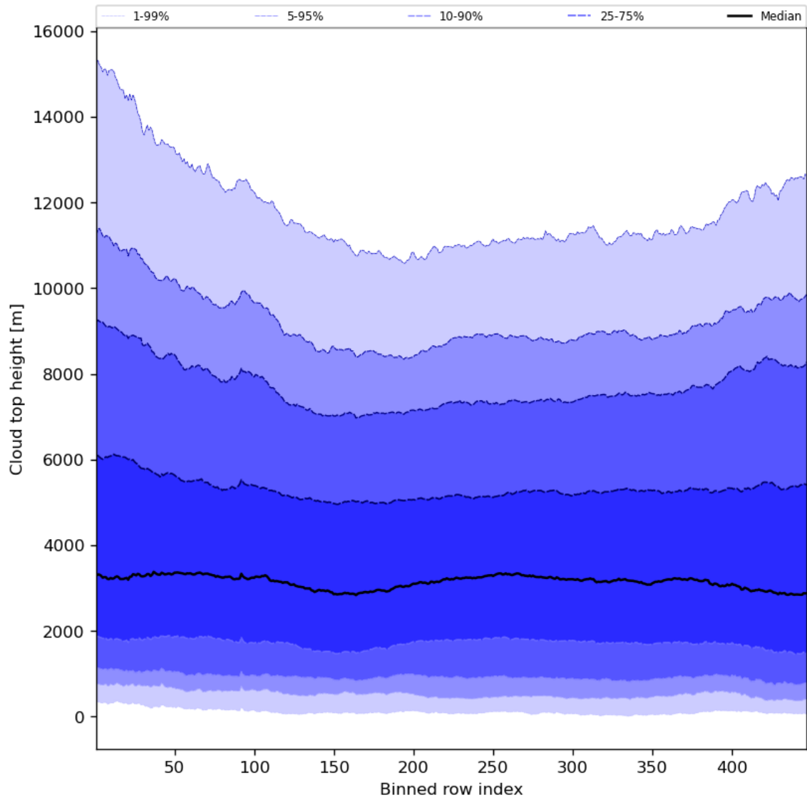
Figure 56: Along track statistics of “Cloud top height” for 2023-07-31 to 2023-08-02
