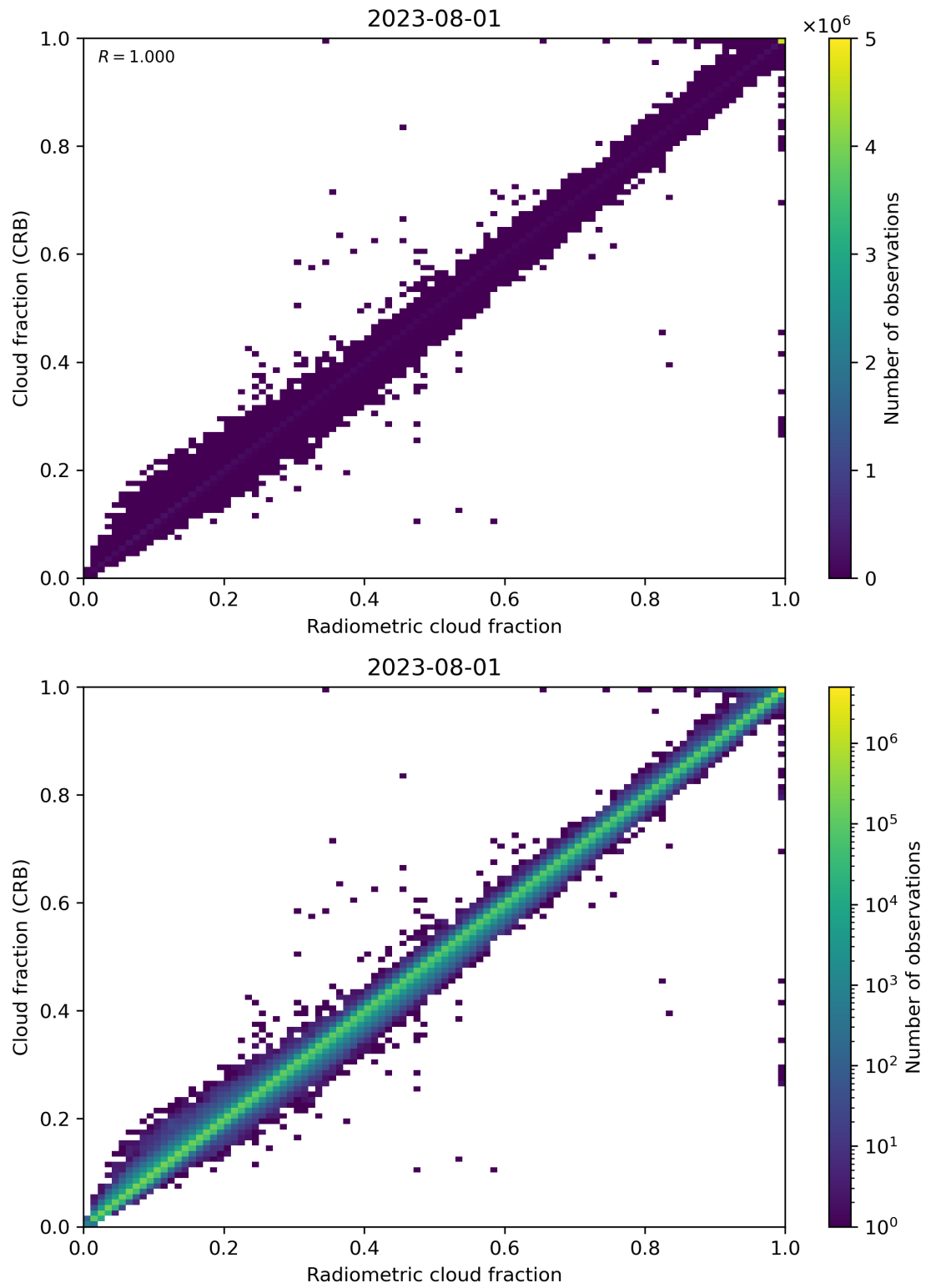
Figure 73: Scatter density plot of “Radiometric cloud fraction” against “Cloud fraction (CRB)” for 2023-07-31 to 2023-08-02.
