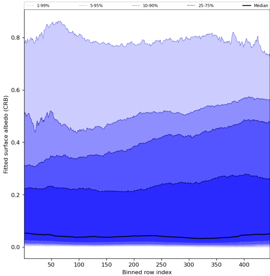
Figure 62: Along track statistics of “Fitted surface albedo (CRB)” for 2023-07-31 to 2023-08-02
