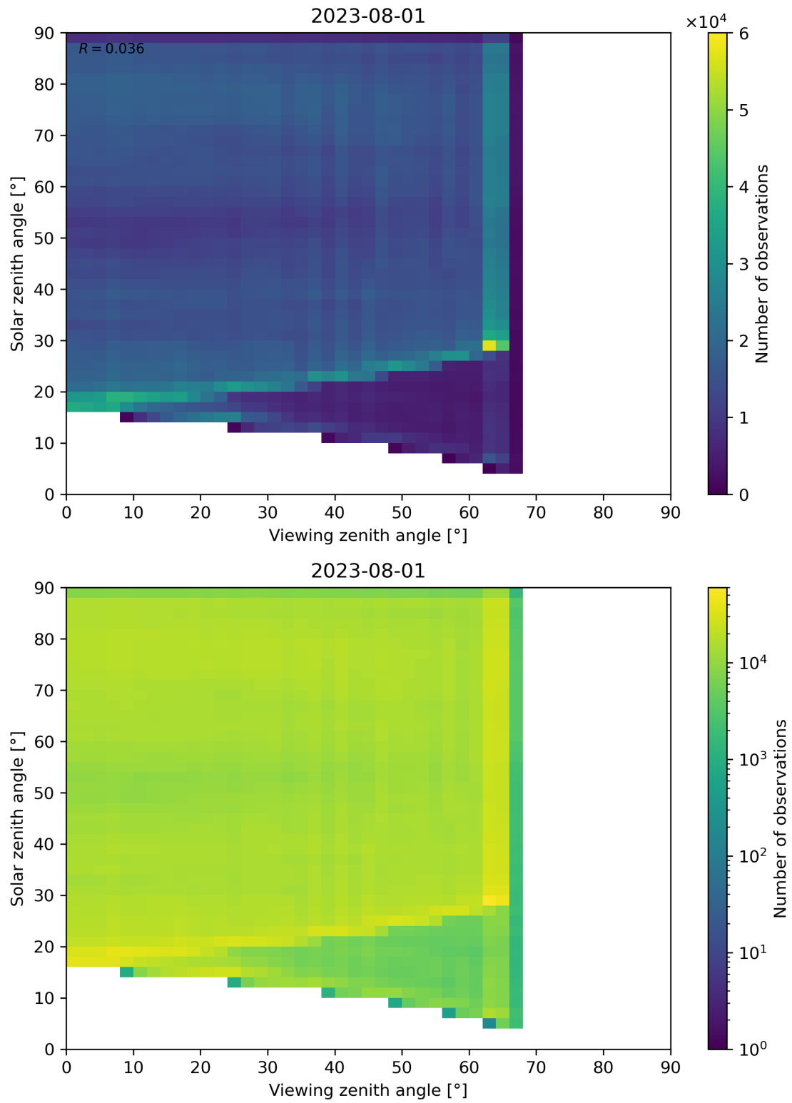
Figure 114: Scatter density plot of “Viewing zenith angle” against “Solar zenith angle” for 2023-07-31 to 2023-08-02.
