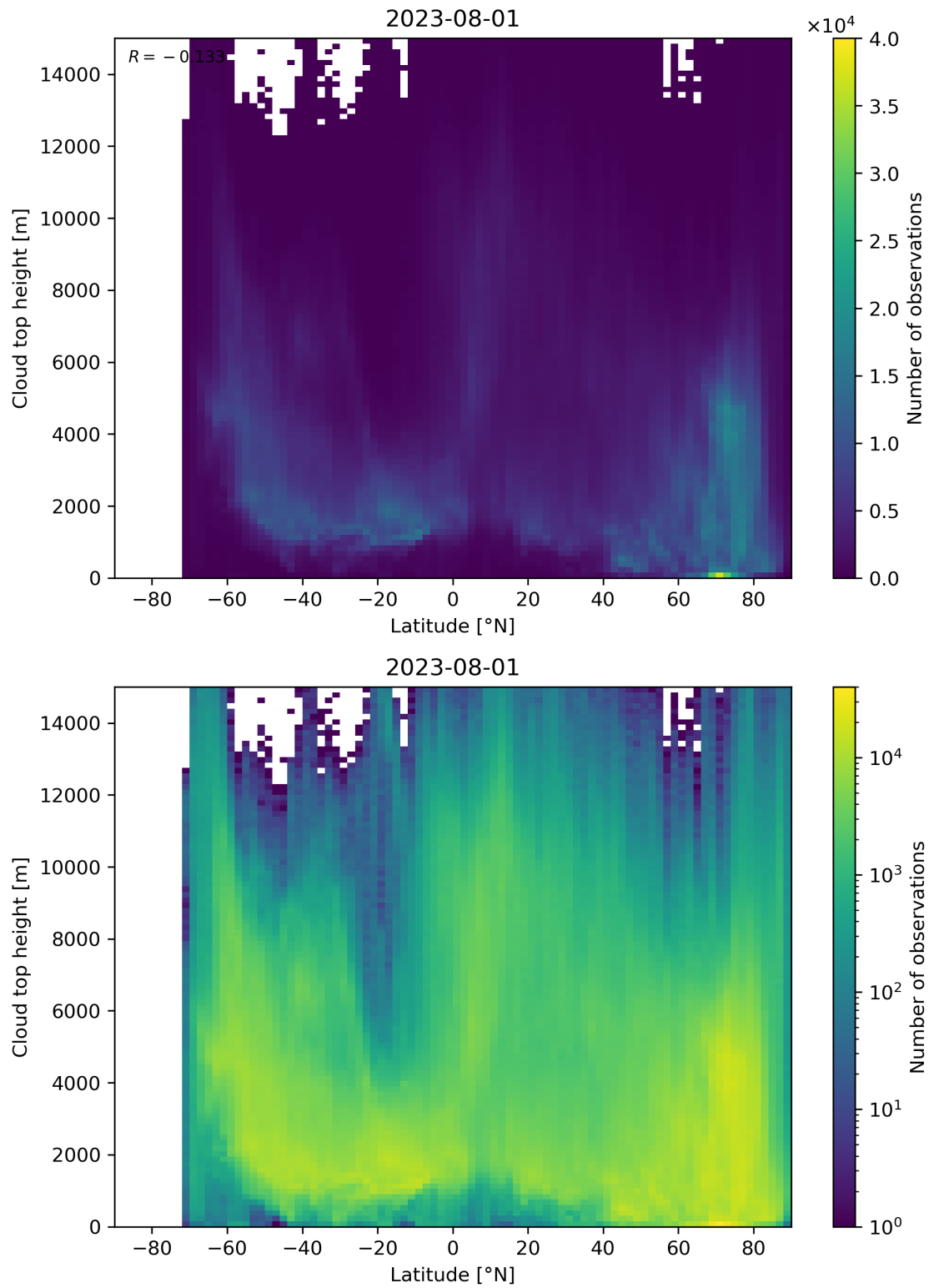
Figure 97: Scatter density plot of “Latitude” against “Cloud top height” for 2023-07-31 to 2023-08-02.
