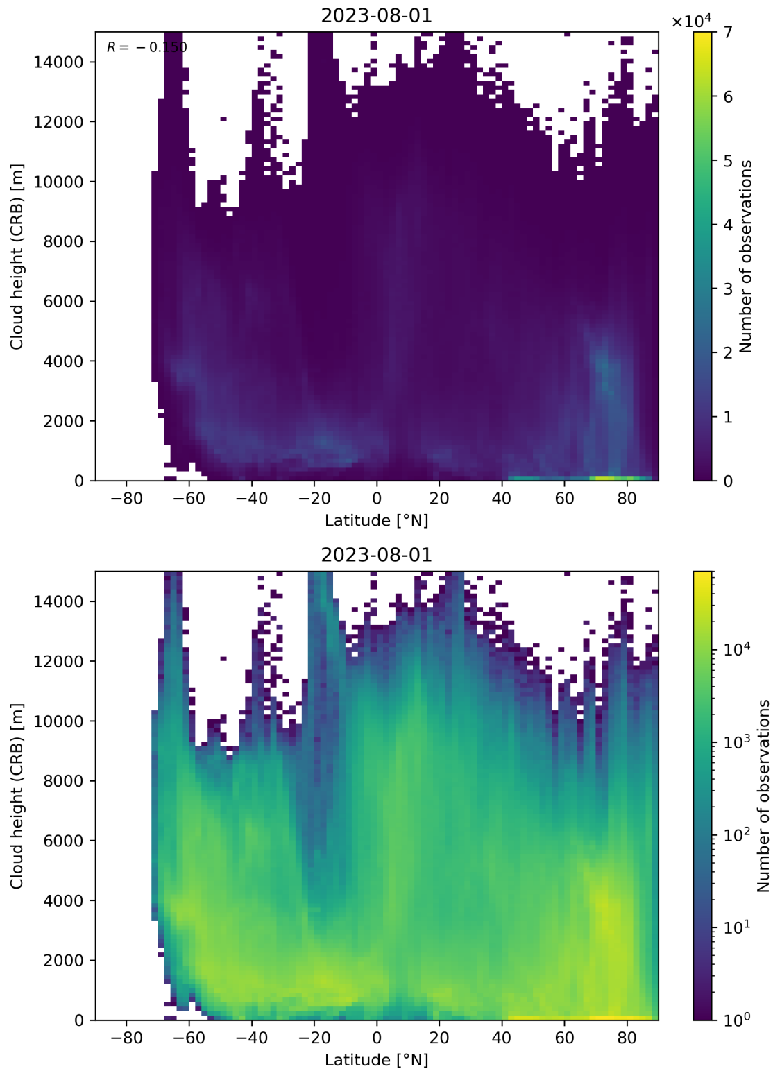
Figure 95: Scatter density plot of “Latitude” against “Cloud height (CRB)” for 2023-07-31 to 2023-08-02.
