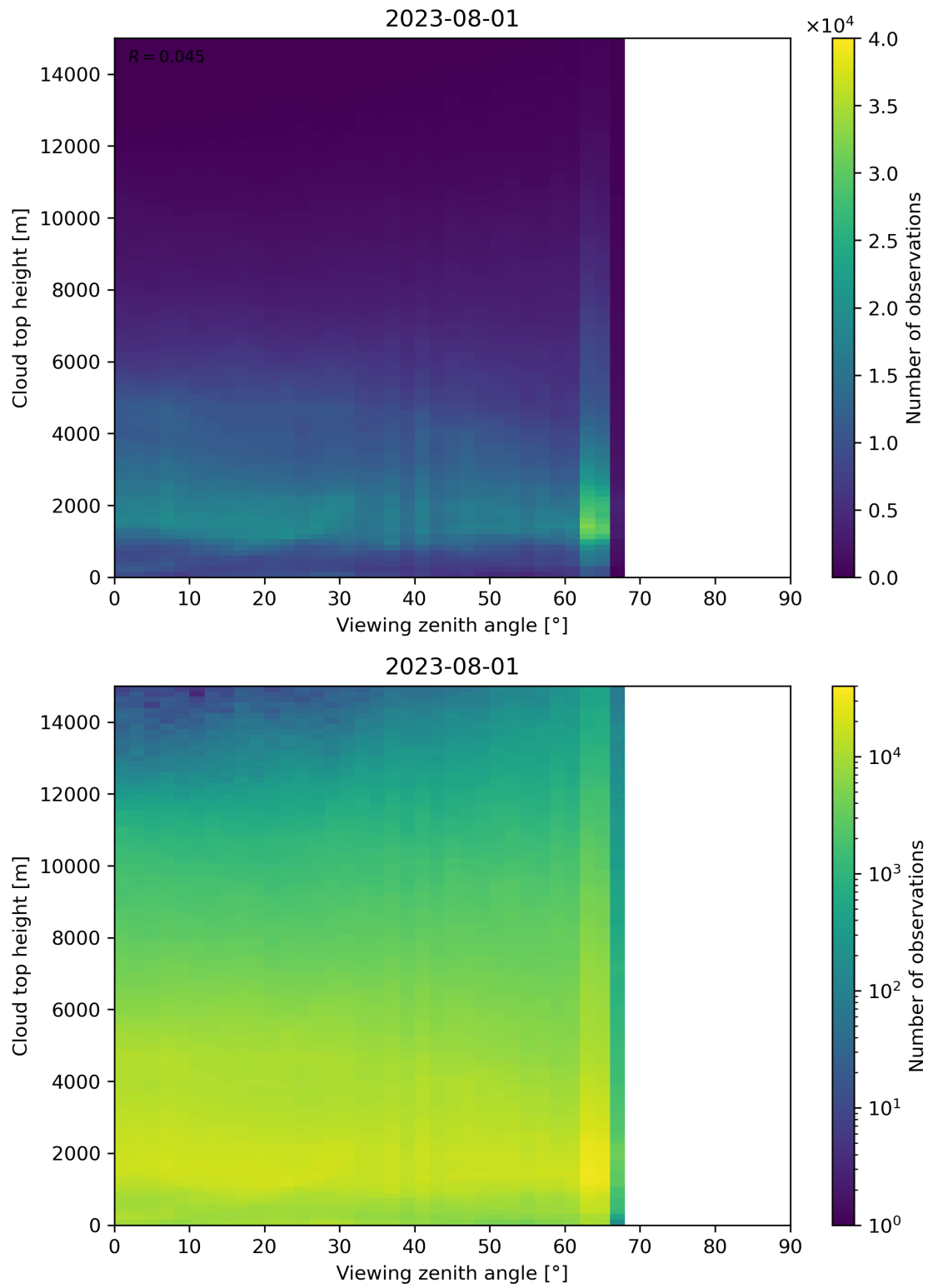
Figure 112: Scatter density plot of “Viewing zenith angle” against “Cloud top height” for 2023-07-31 to 2023-08-02.
