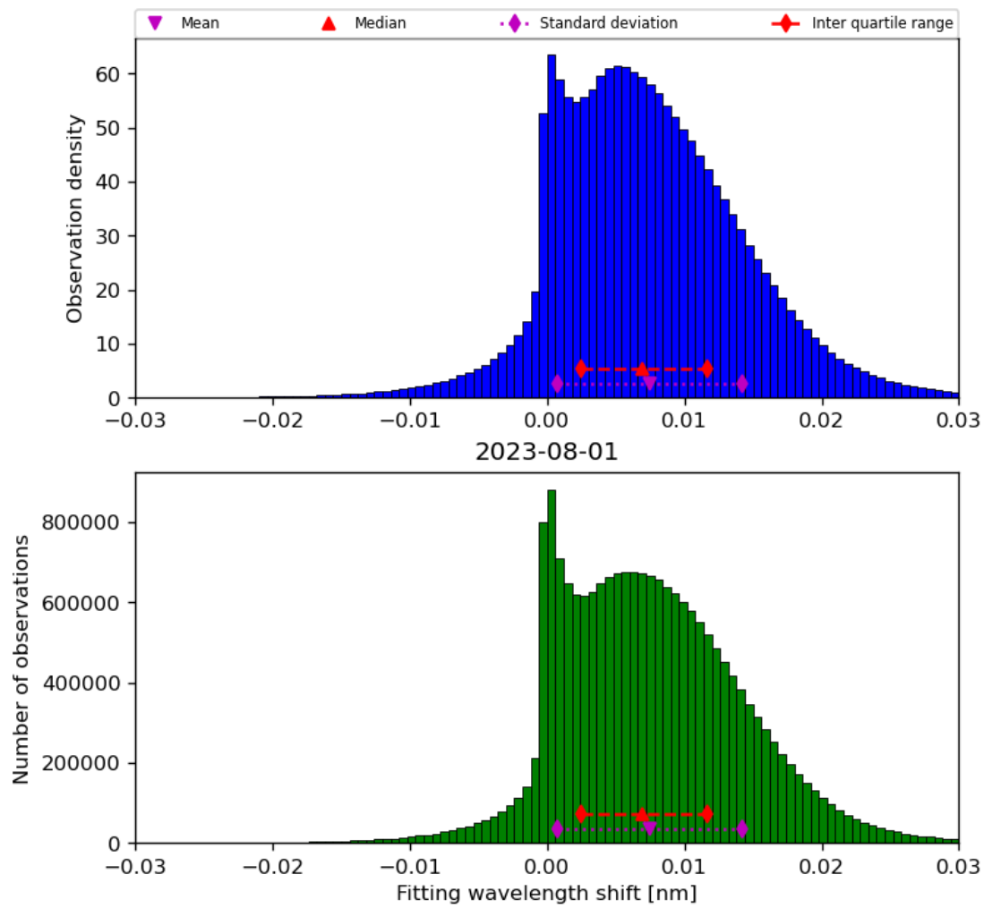
Figure 49: Histogram of “Fitting wavelength shift” for 2023-07-31 to 2023-08-02
