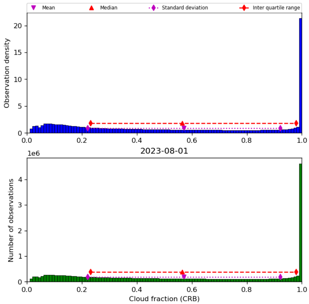
Figure 42: Histogram of “Cloud fraction (CRB)” for 2023-07-31 to 2023-08-02
