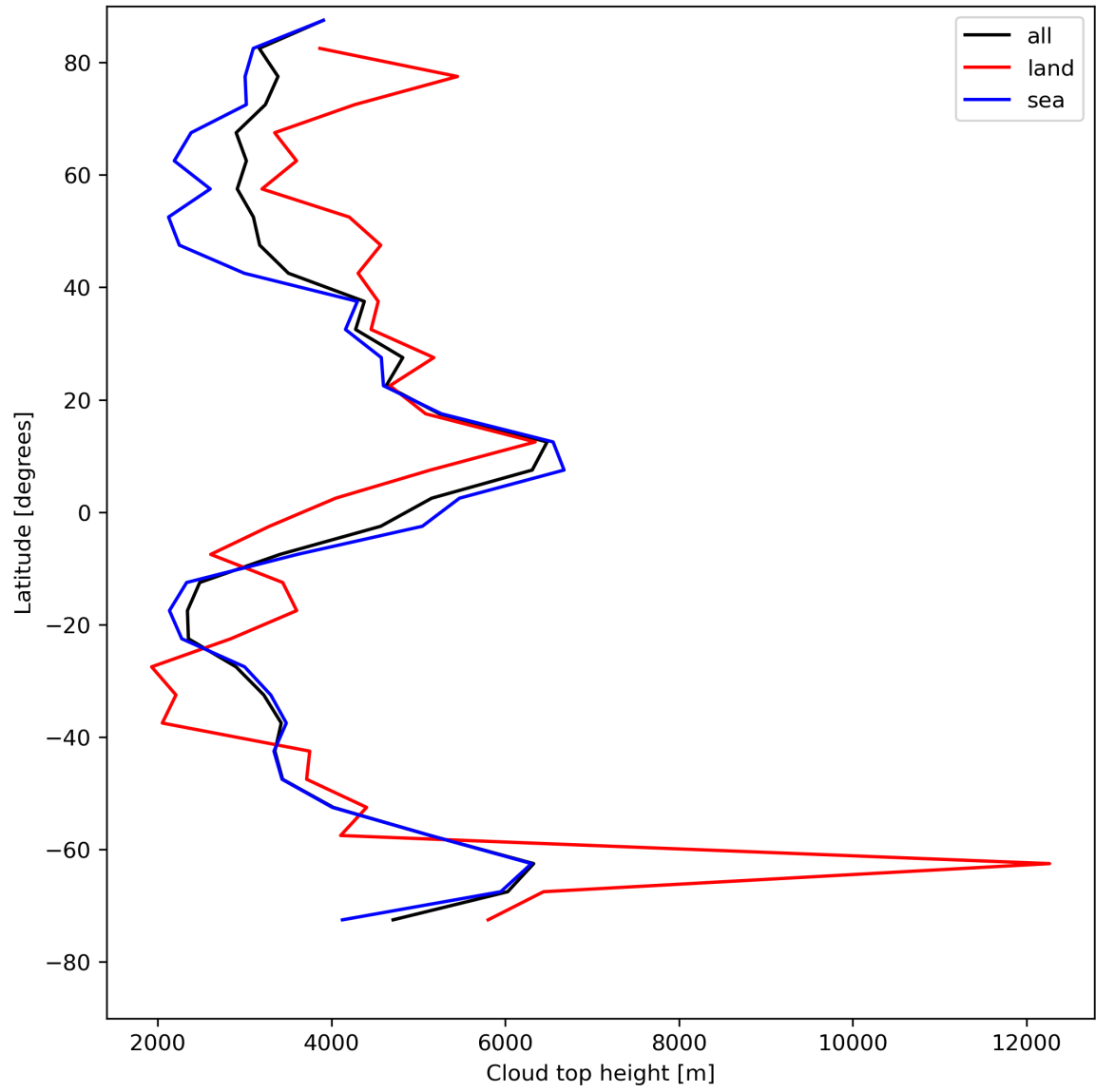
Figure 24: Zonal average of “Cloud top height” for 2023-07-31 to 2023-08-02.
