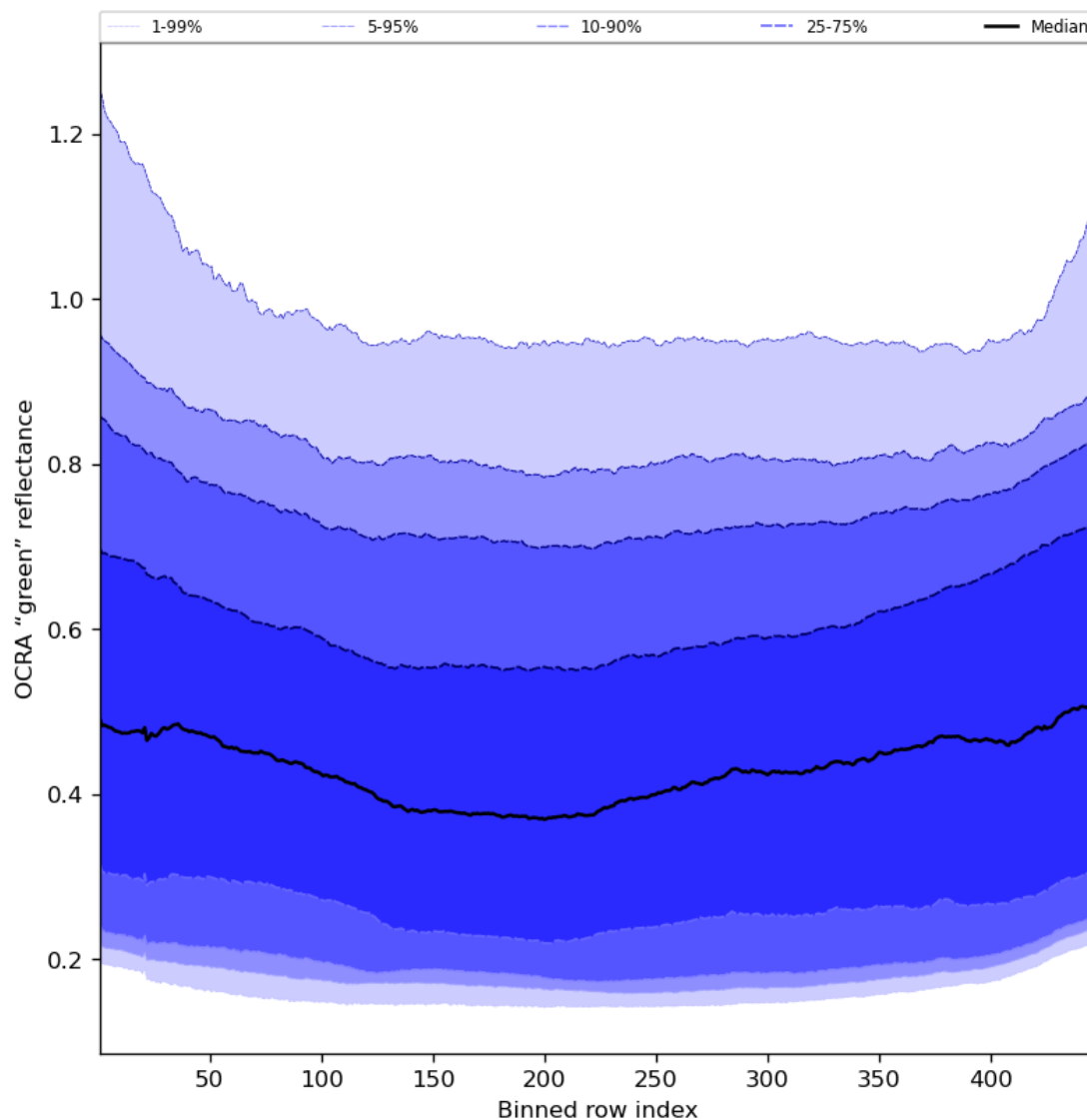
Figure 68: Along track statistics of “OCRA “green” reflectance” for 2023-07-31 to 2023-08-02
