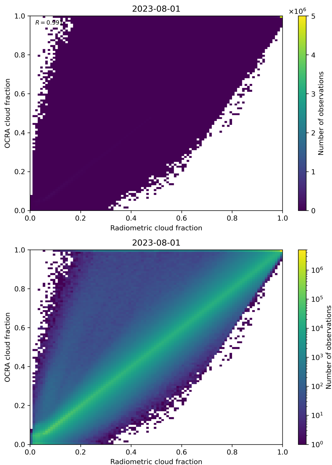
Figure 72: Scatter density plot of “Radiometric cloud fraction” against “OCRA cloud fraction” for 2023-07-31 to 2023-08-02.
