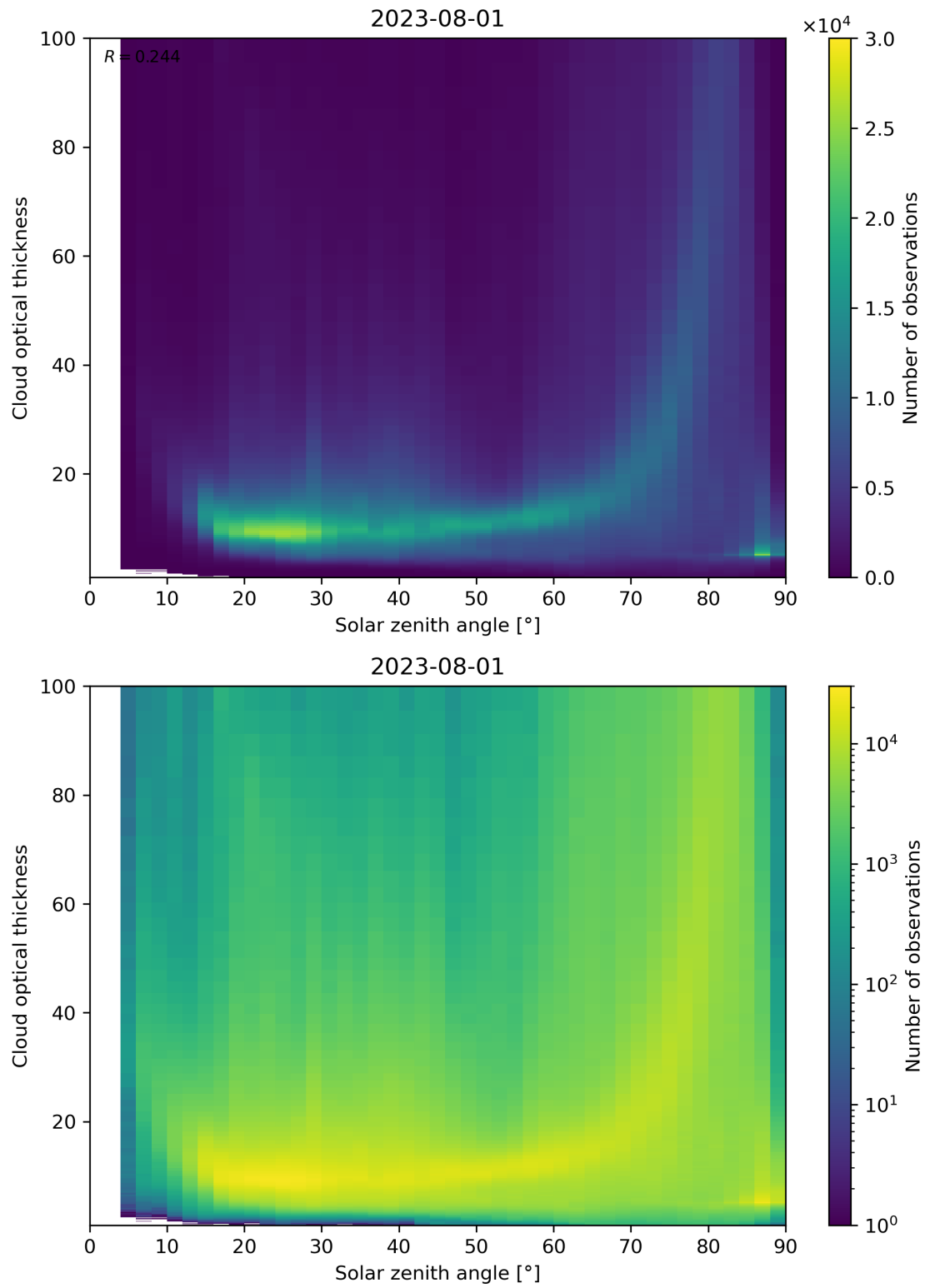
Figure 103: Scatter density plot of “Solar zenith angle” against “Cloud optical thickness” for 2023-07-31 to 2023-08-02.
