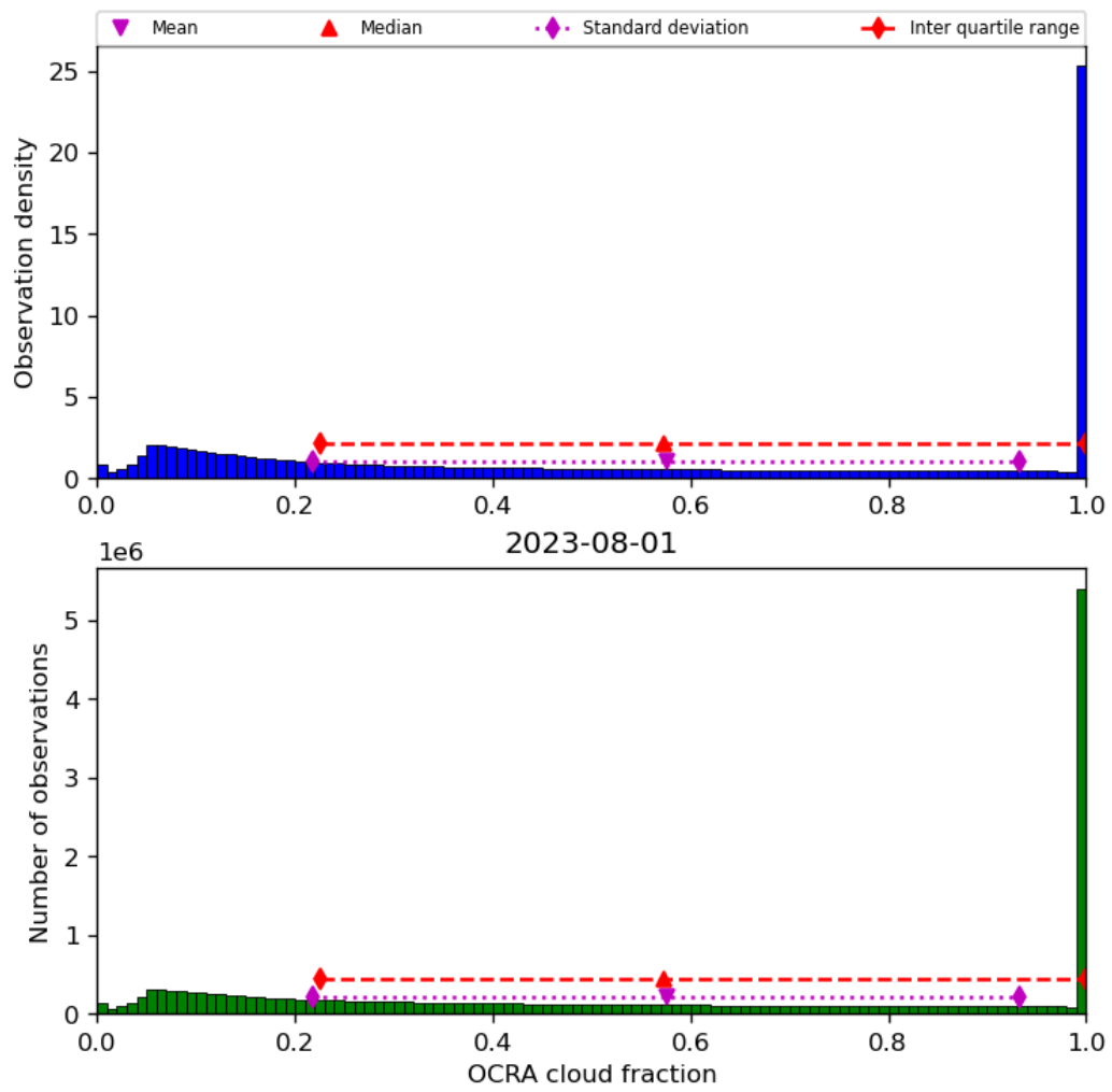
Figure 50: Histogram of “OCRA cloud fraction” for 2023-07-31 to 2023-08-02
