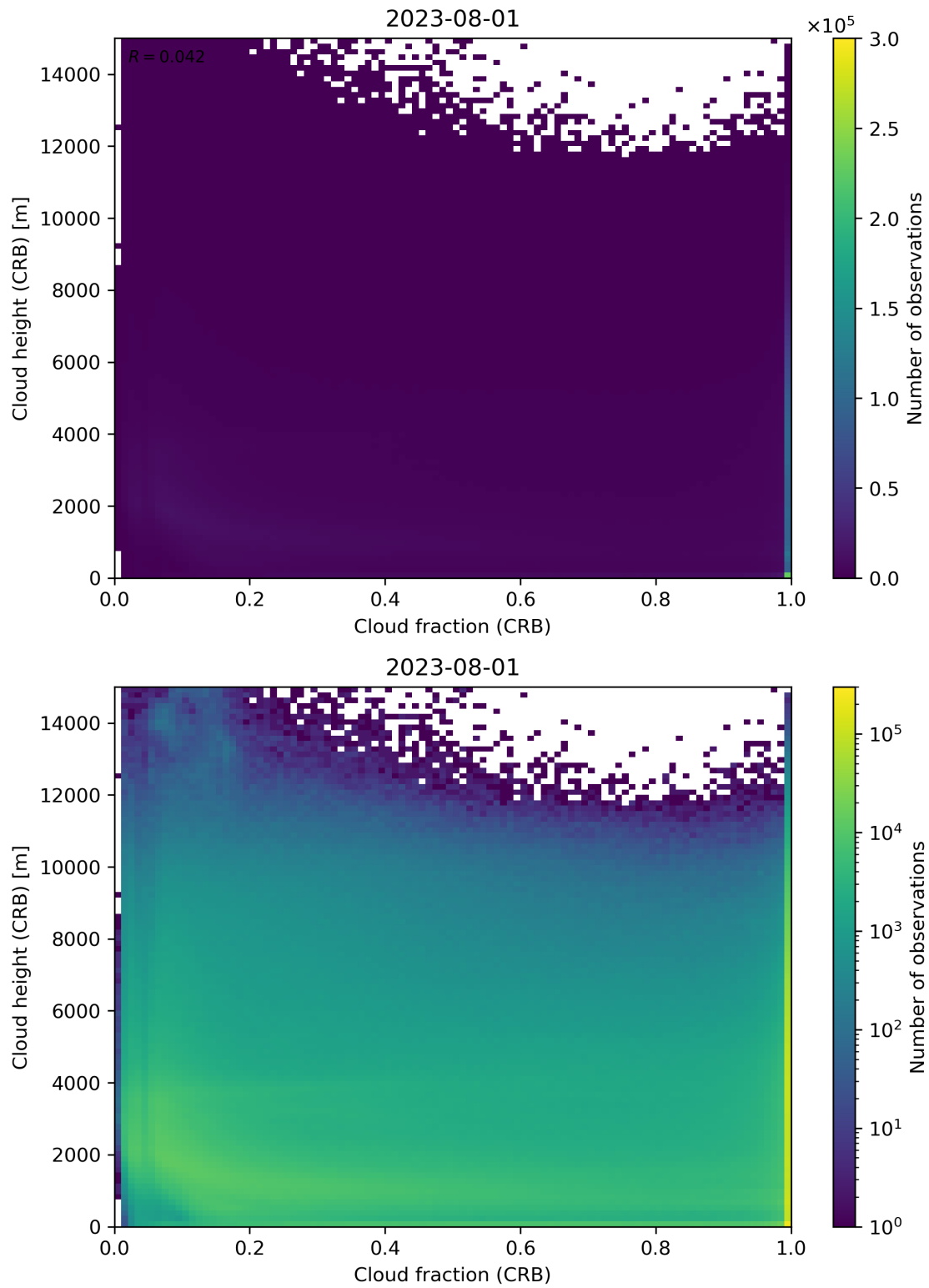
Figure 79: Scatter density plot of “Cloud fraction (CRB)” against “Cloud height (CRB)” for 2023-07-31 to 2023-08-02.
