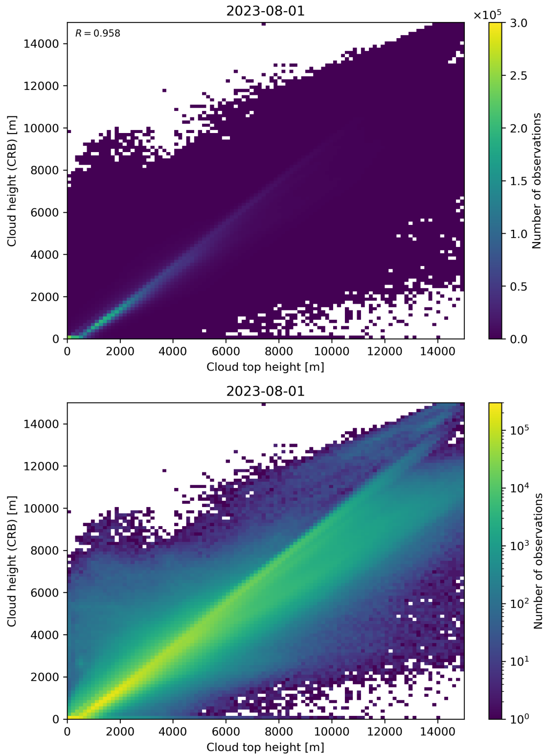
Figure 89: Scatter density plot of “Cloud top height” against “Cloud height (CRB)” for 2023-07-31 to 2023-08-02.
