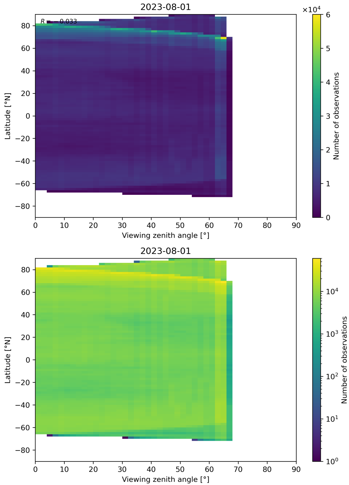
Figure 113: Scatter density plot of “Viewing zenith angle” against “Latitude” for 2023-07-31 to 2023-08-02.
