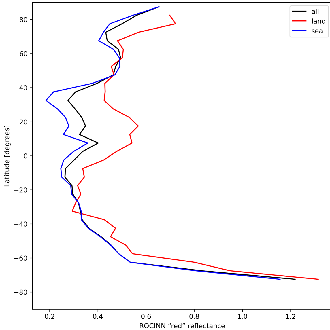
Figure 37: Zonal average of “ROCINN “red” reflectance” for 2023-07-31 to 2023-08-02.
