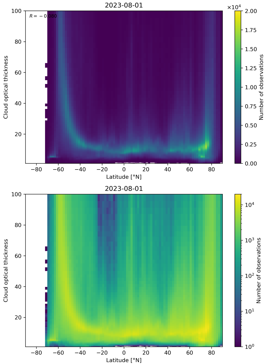
Figure 96: Scatter density plot of “Latitude” against “Cloud optical thickness” for 2023-07-31 to 2023-08-02.
