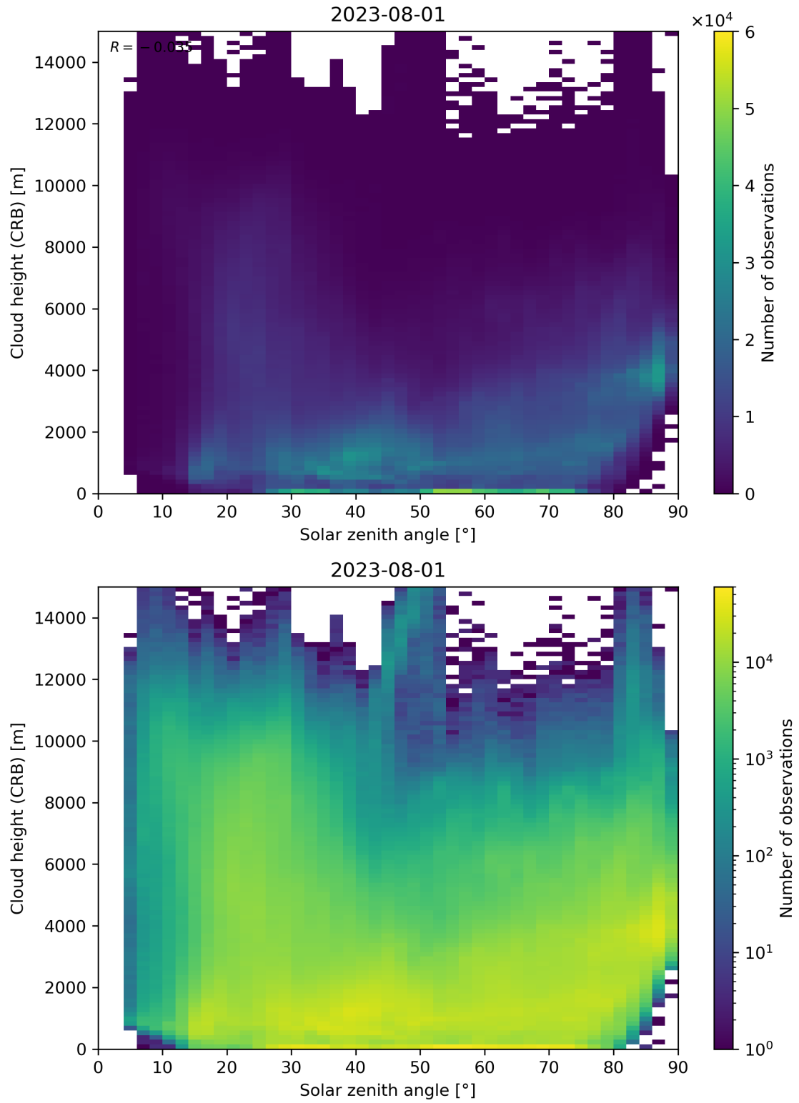
Figure 102: Scatter density plot of “Solar zenith angle” against “Cloud height (CRB)” for 2023-07-31 to 2023-08-02.
