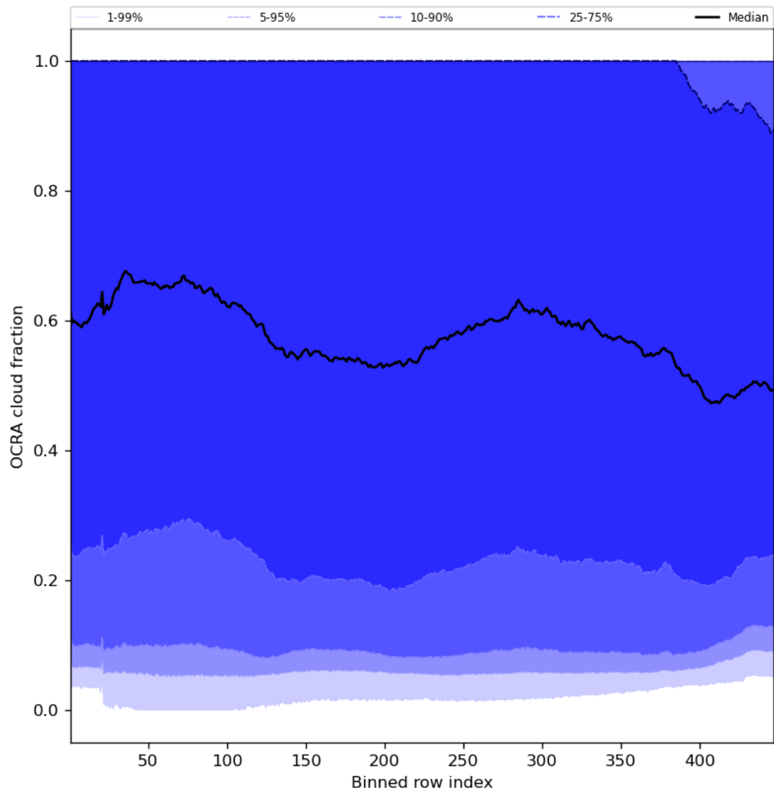
Figure 66: Along track statistics of “OCRA cloud fraction” for 2023-07-31 to 2023-08-02
