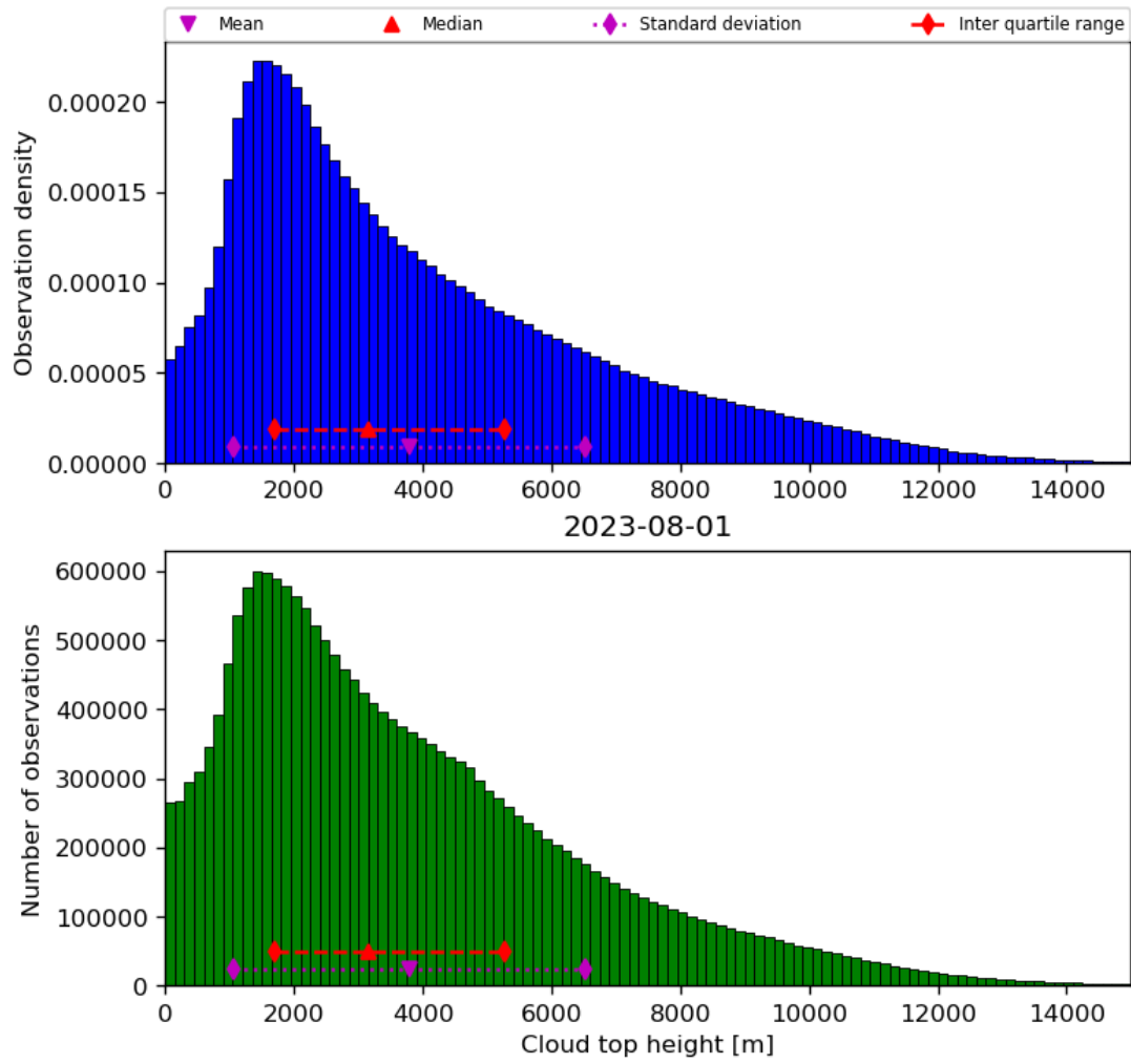
Figure 40: Histogram of “Cloud top height” for 2023-07-31 to 2023-08-02
