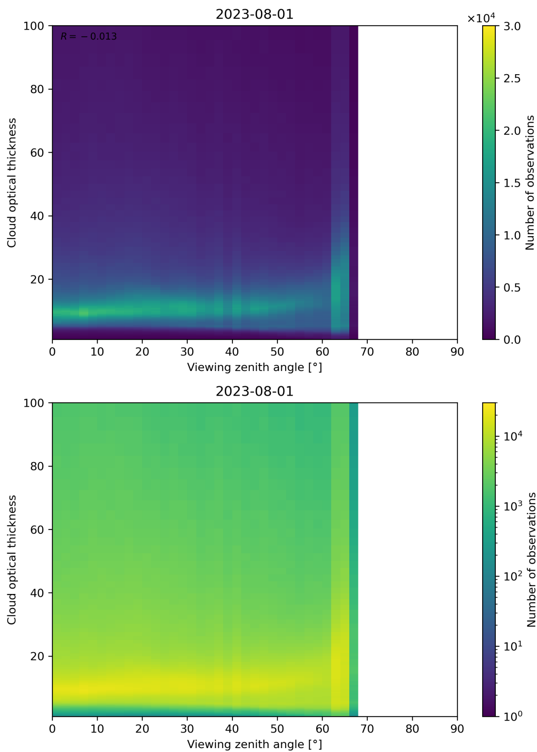
Figure 111: Scatter density plot of “Viewing zenith angle” against “Cloud optical thickness” for 2023-07-31 to 2023-08-02.
