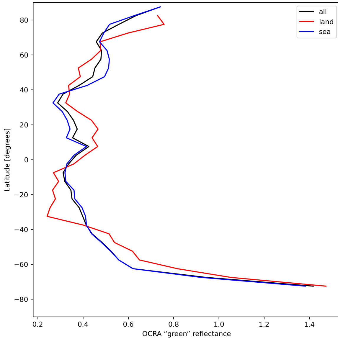
Figure 36: Zonal average of “OCRA “green” reflectance” for 2023-07-31 to 2023-08-02.
