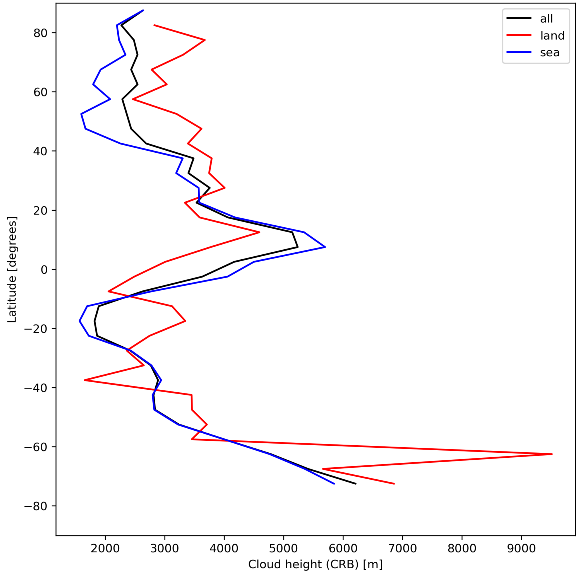
Figure 27: Zonal average of “Cloud height (CRB)” for 2023-07-31 to 2023-08-02.
