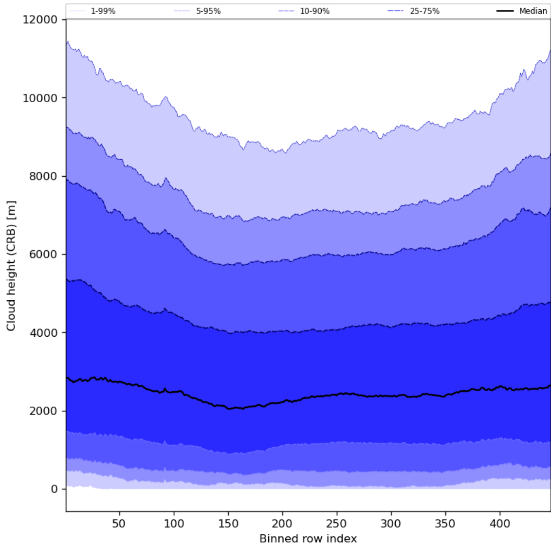
Figure 59: Along track statistics of “Cloud height (CRB)” for 2023-07-31 to 2023-08-02
