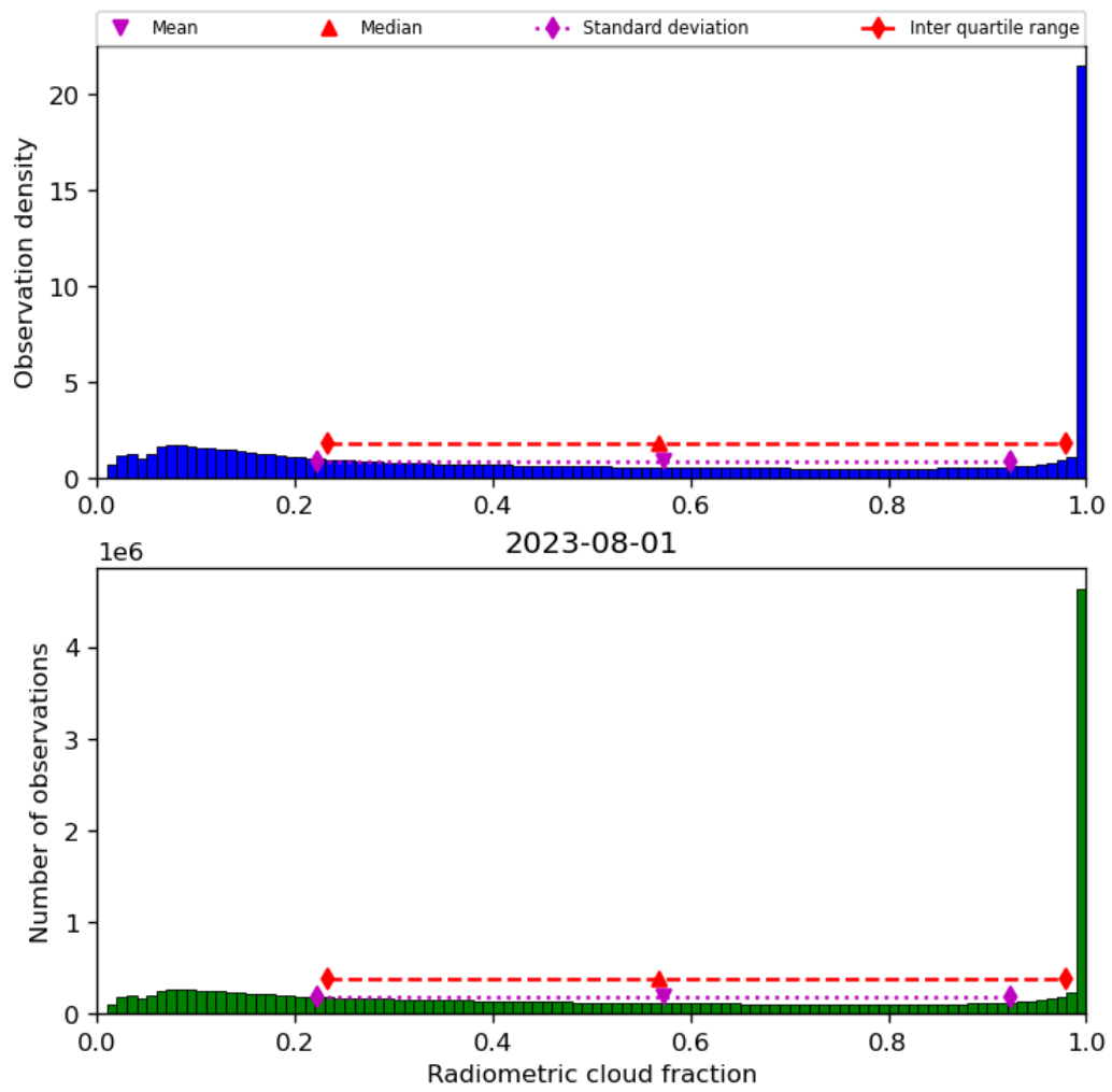
Figure 39: Histogram of “Radiometric cloud fraction” for 2023-07-31 to 2023-08-02
