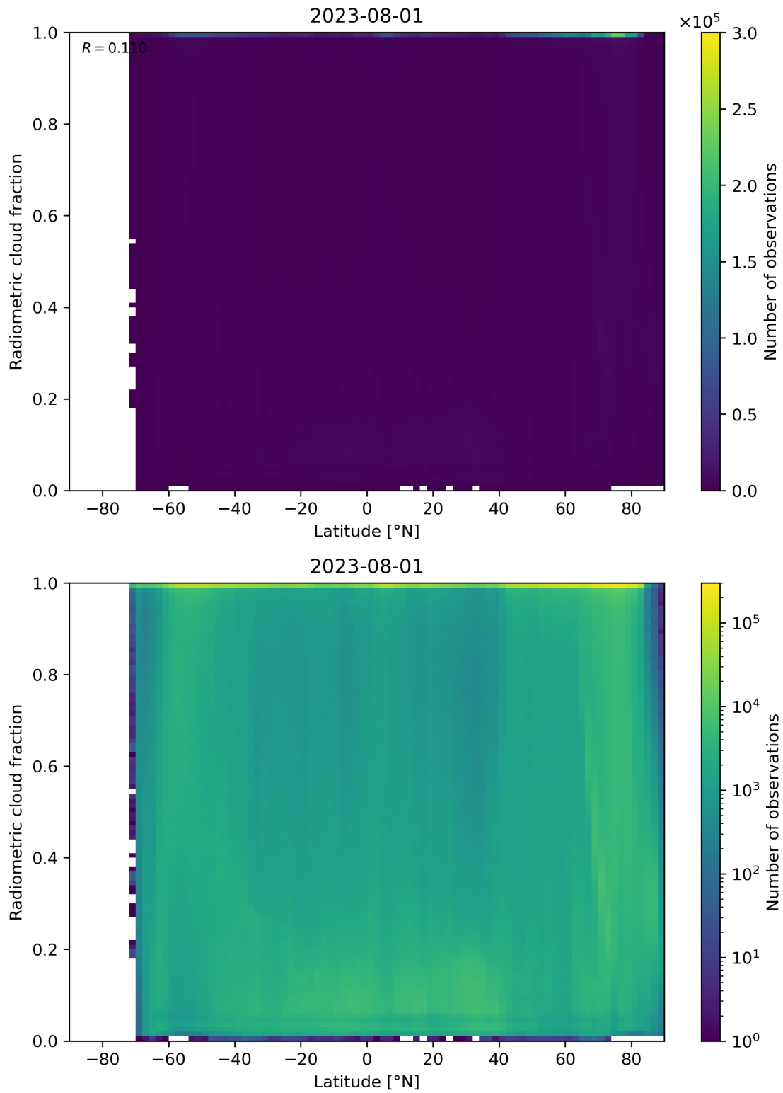
Figure 92: Scatter density plot of “Latitude” against “Radiometric cloud fraction” for 2023-07-31 to 2023-08-02.
