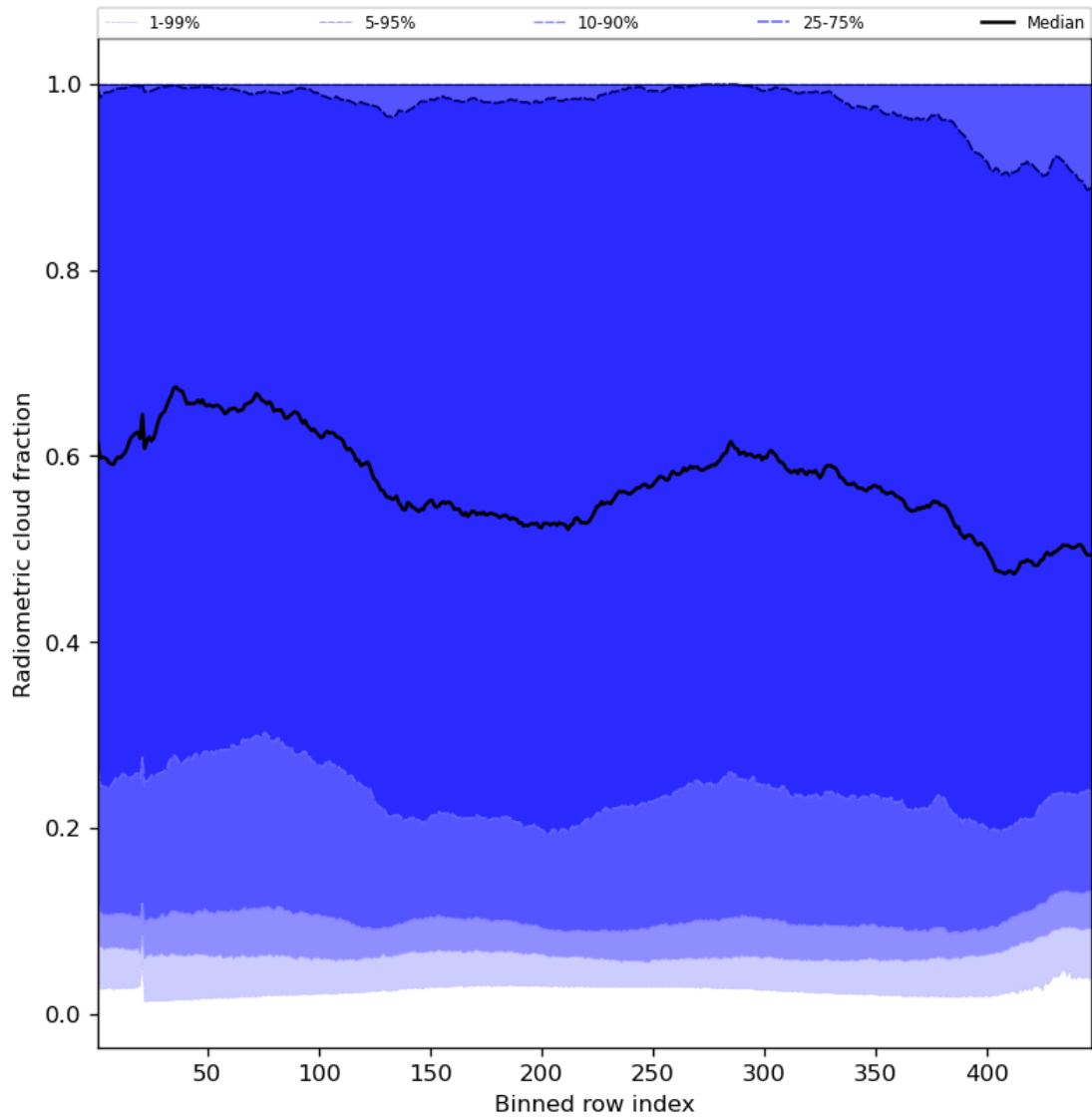
Figure 55: Along track statistics of “Radiometric cloud fraction” for 2023-07-31 to 2023-08-02
