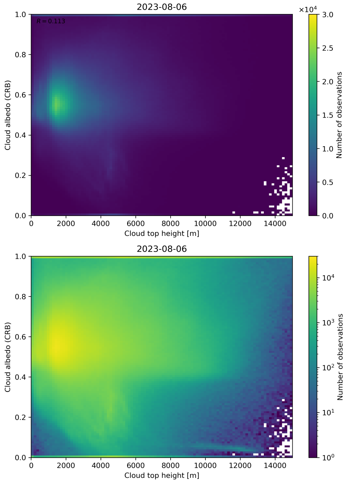
Figure 86: Scatter density plot of “Cloud top height” against “Cloud albedo (CRB)” for 2023-08-05 to 2023-08-07.
