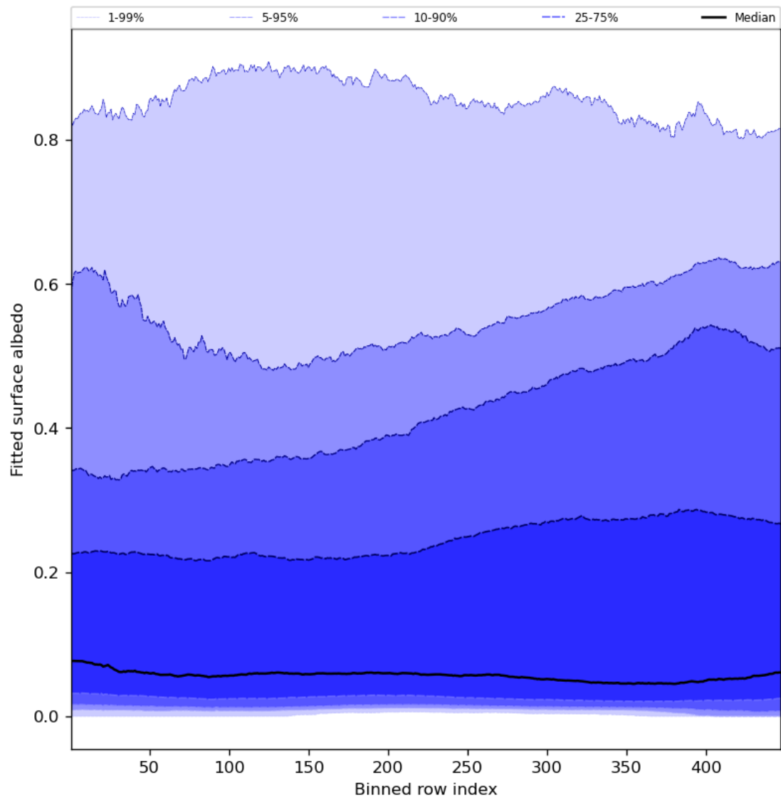
Figure 61: Along track statistics of “Fitted surface albedo” for 2023-08-05 to 2023-08-07
