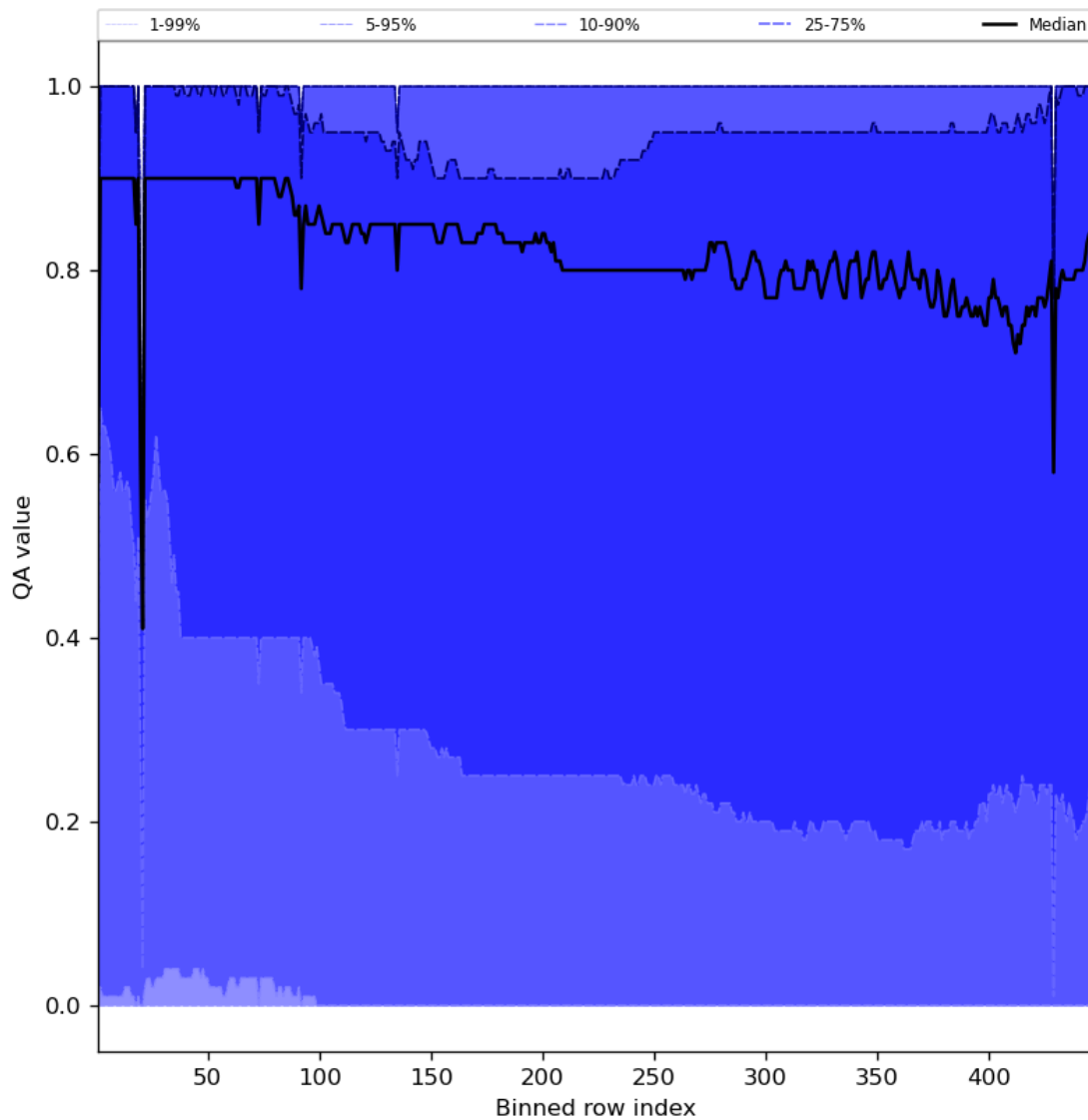
Figure 54: Along track statistics of “QA value” for 2023-08-05 to 2023-08-07
