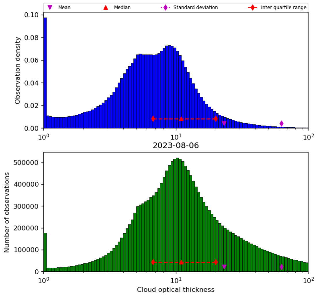
Figure 41: Histogram of “Cloud optical thickness” for 2023-08-05 to 2023-08-07
