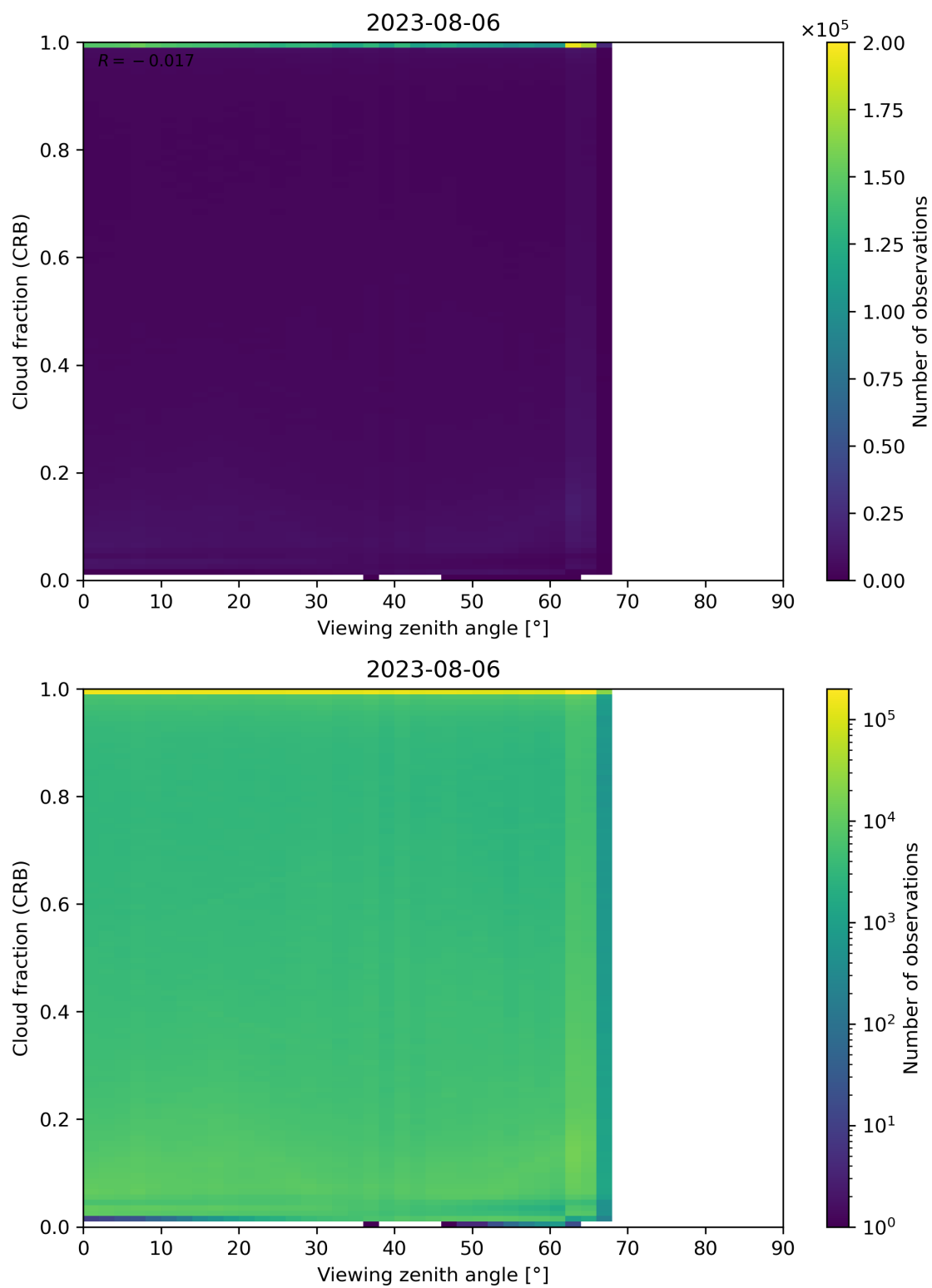
Figure 109: Scatter density plot of “Viewing zenith angle” against “Cloud fraction (CRB)” for 2023-08-05 to 2023-08-07.
