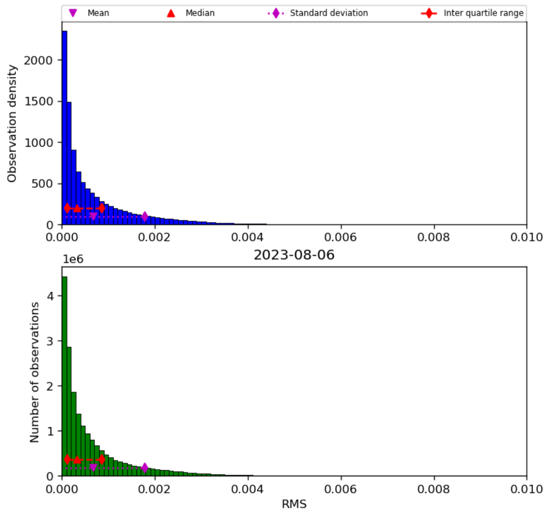
Figure 47: Histogram of “RMS” for 2023-08-05 to 2023-08-07
