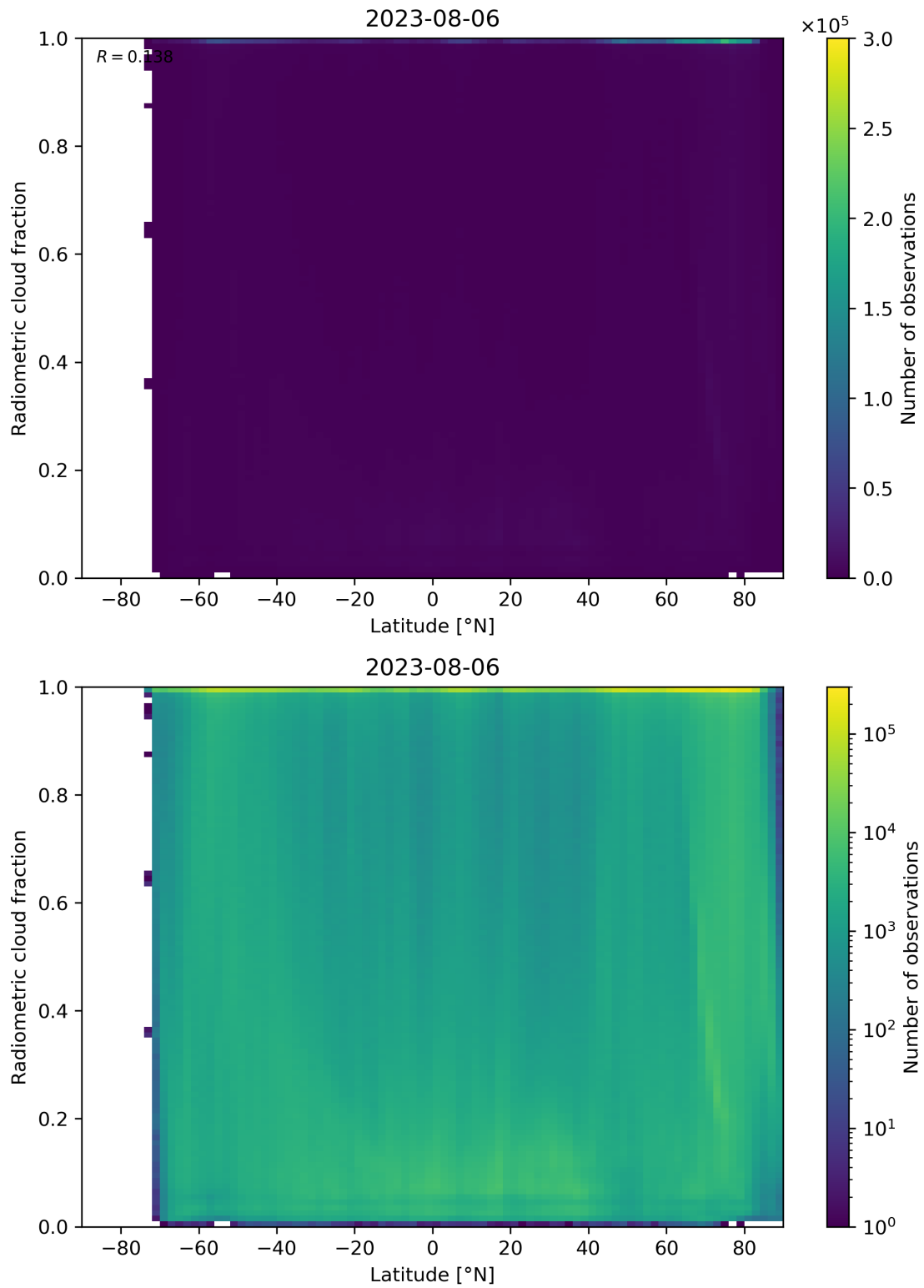
Figure 92: Scatter density plot of “Latitude” against “Radiometric cloud fraction” for 2023-08-05 to 2023-08-07.
