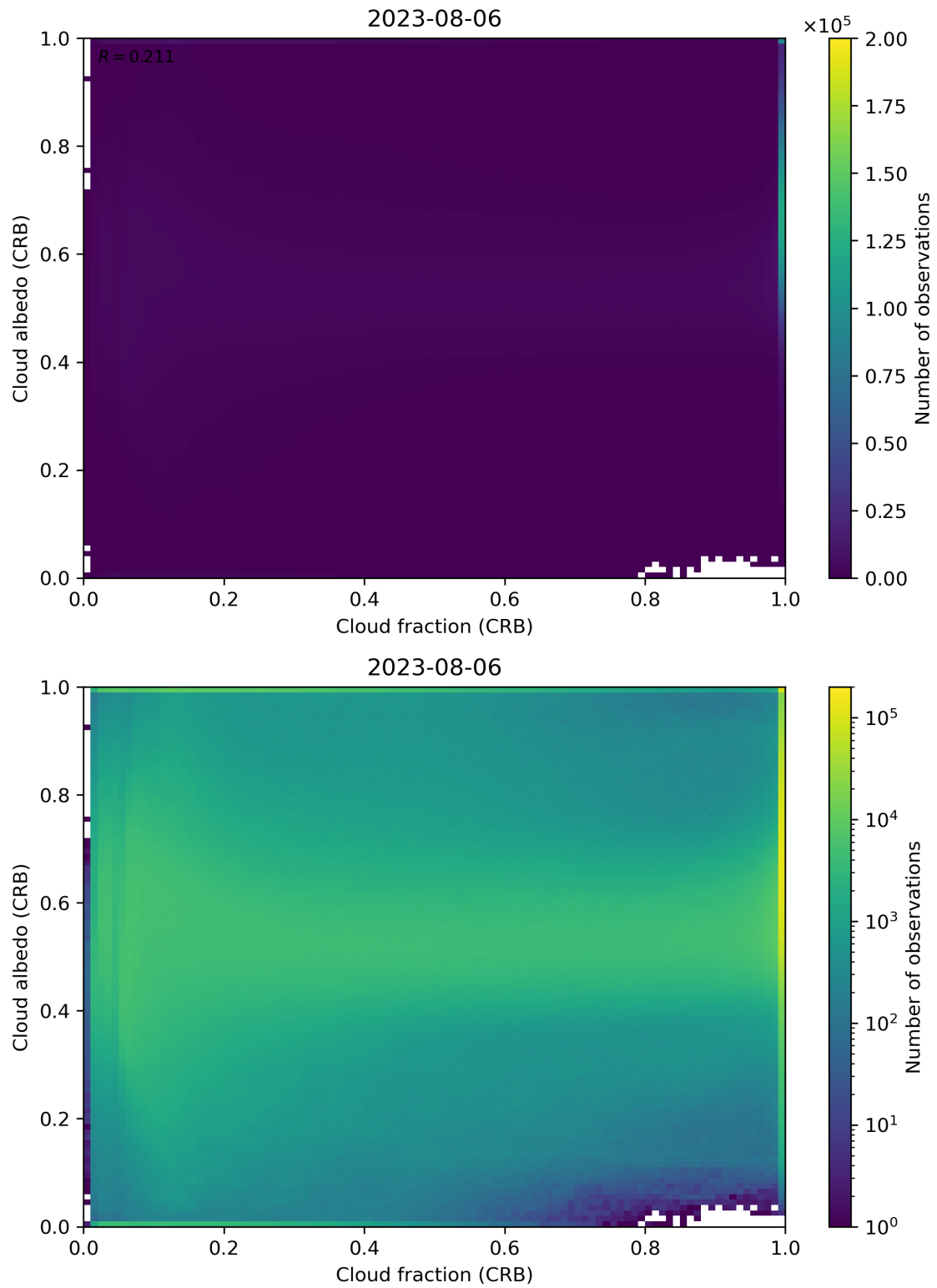
Figure 77: Scatter density plot of “Cloud fraction (CRB)” against “Cloud albedo (CRB)” for 2023-08-05 to 2023-08-07.
