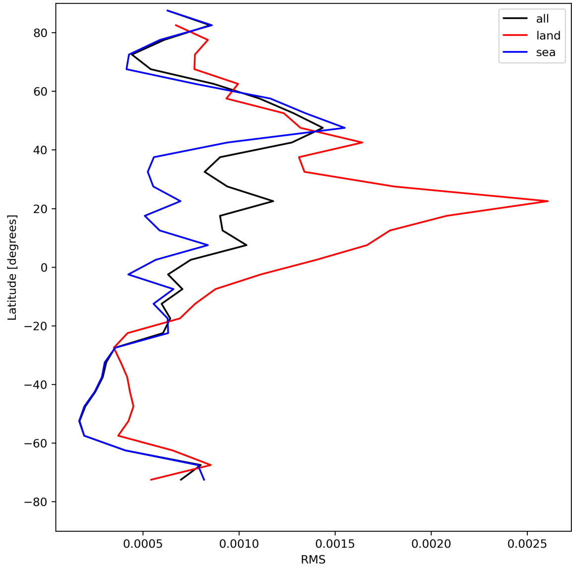
Figure 31: Zonal average of “RMS” for 2023-08-05 to 2023-08-07.
