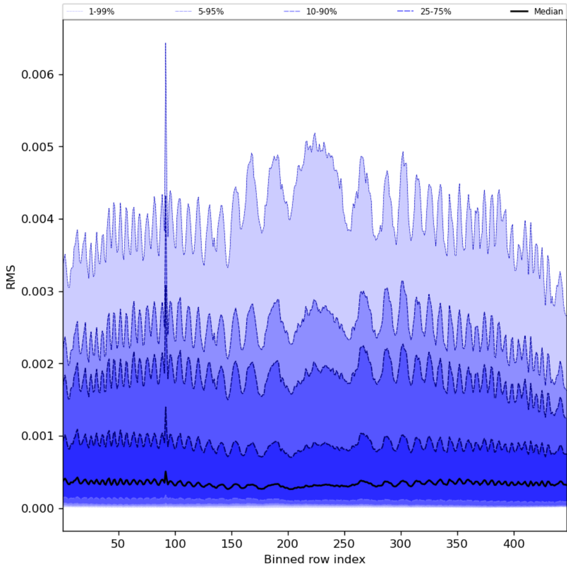
Figure 63: Along track statistics of “RMS” for 2023-08-05 to 2023-08-07
