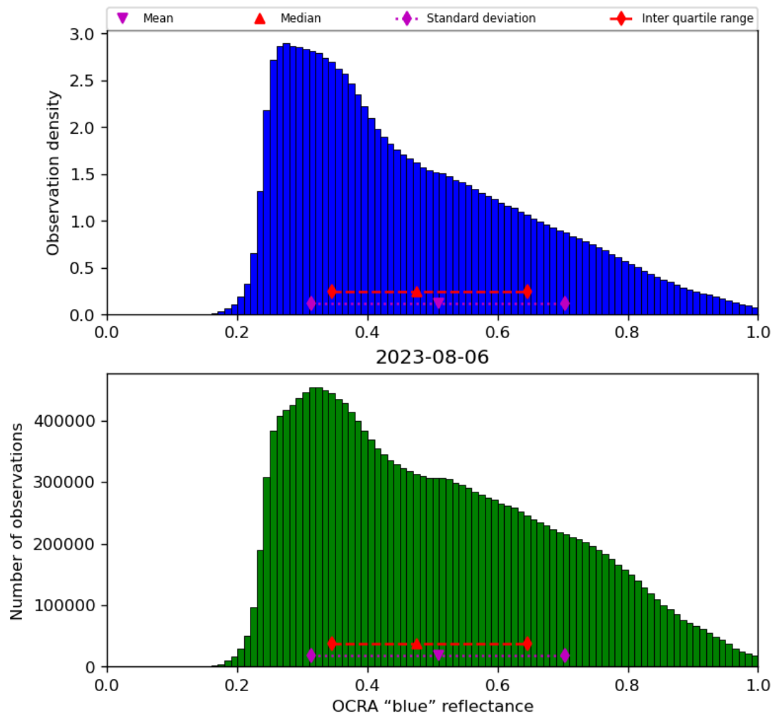
Figure 51: Histogram of “OCRA “blue” reflectance” for 2023-08-05 to 2023-08-07
