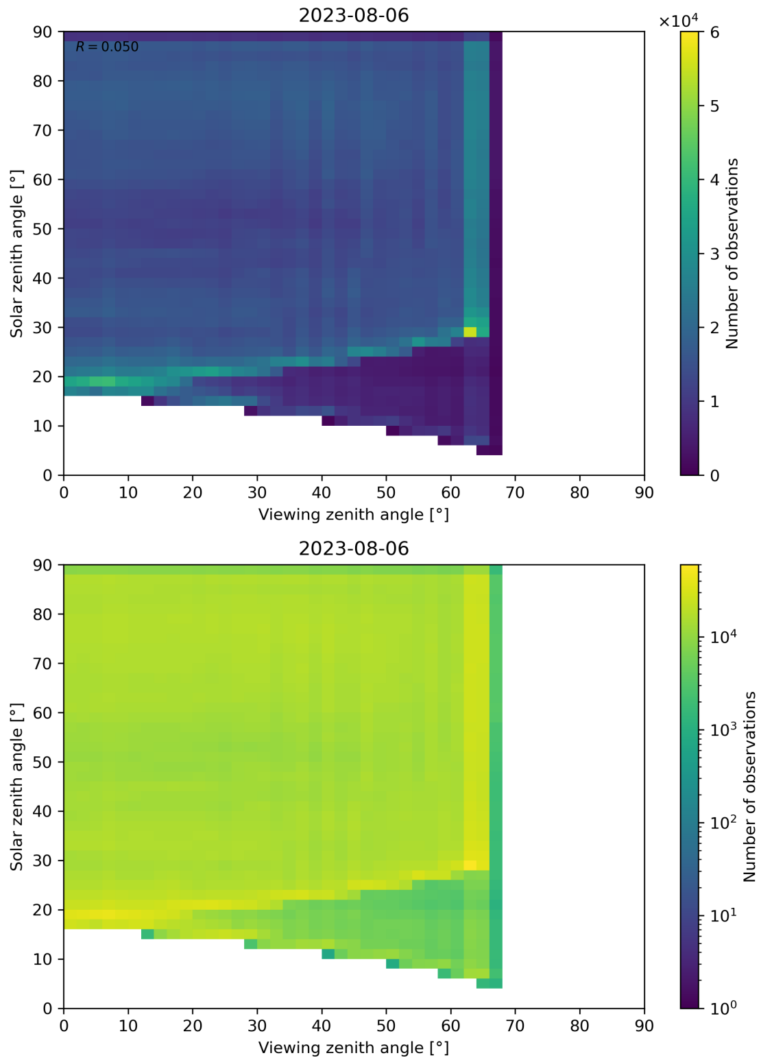
Figure 114: Scatter density plot of “Viewing zenith angle” against “Solar zenith angle” for 2023-08-05 to 2023-08-07.
