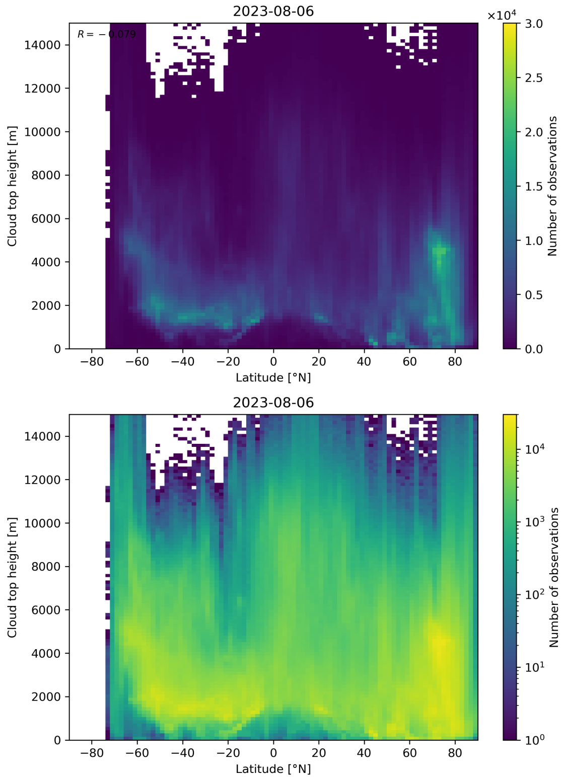
Figure 97: Scatter density plot of “Latitude” against “Cloud top height” for 2023-08-05 to 2023-08-07.
