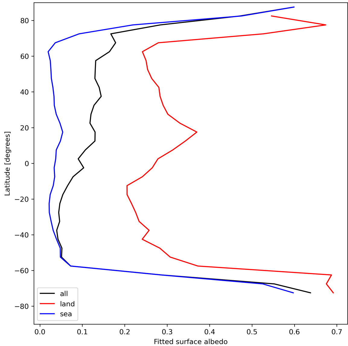
Figure 29: Zonal average of “Fitted surface albedo” for 2023-08-05 to 2023-08-07.
