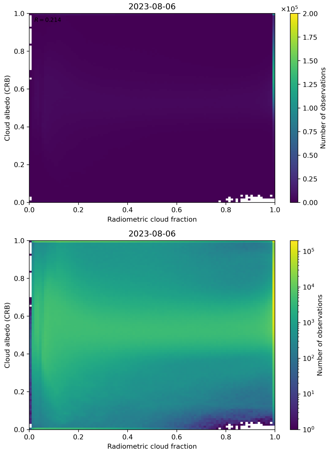
Figure 71: Scatter density plot of “Radiometric cloud fraction” against “Cloud albedo (CRB)” for 2023-08-05 to 2023-08-07.
