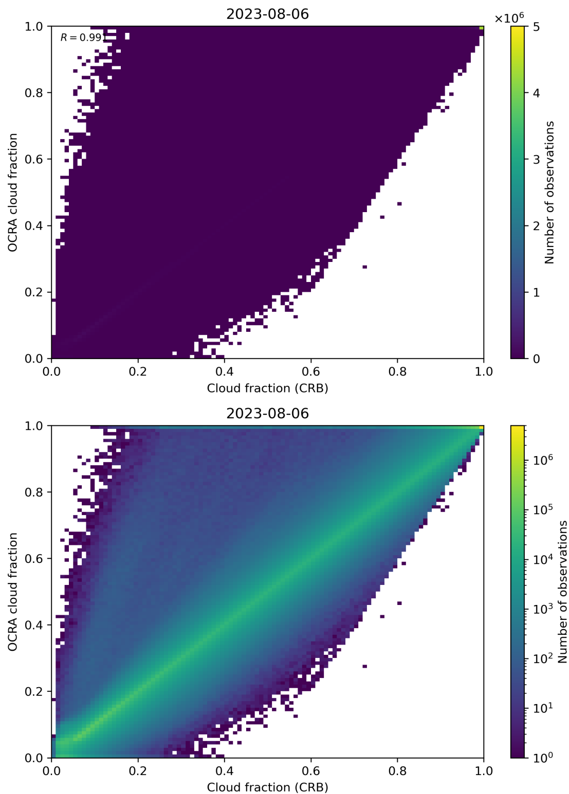
Figure 78: Scatter density plot of “Cloud fraction (CRB)” against “OCRA cloud fraction” for 2023-08-05 to 2023-08-07.
