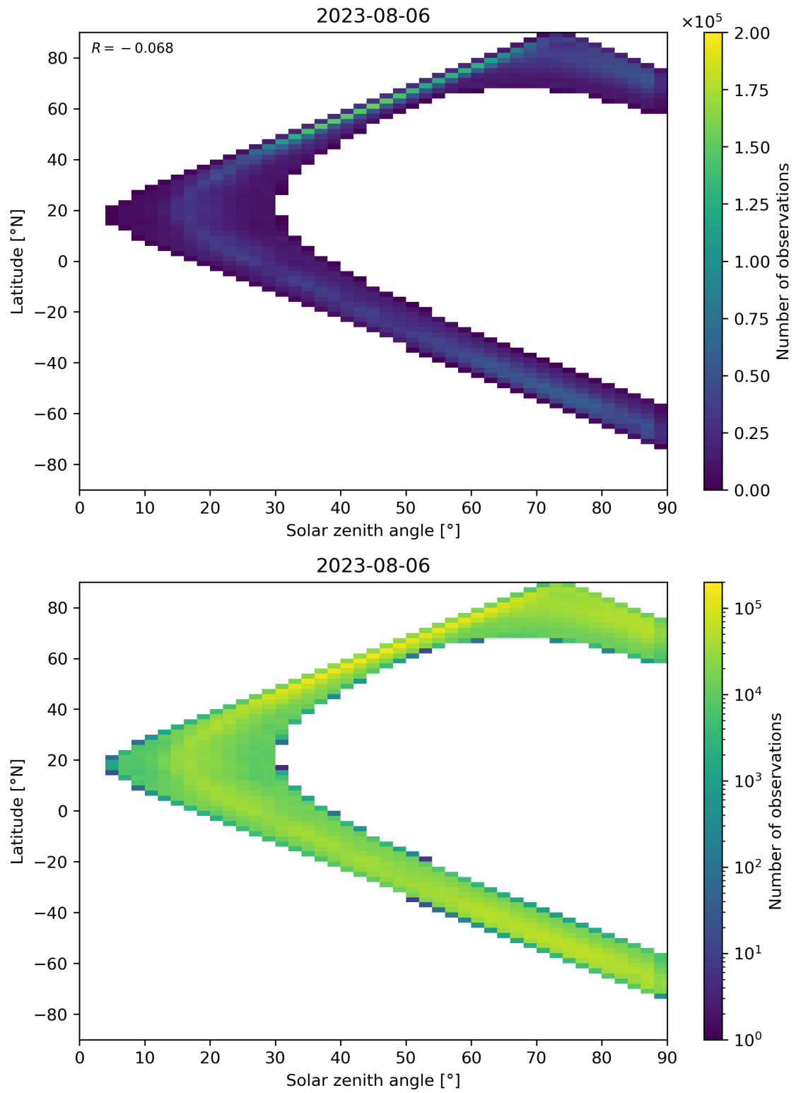
Figure 105: Scatter density plot of “Solar zenith angle” against “Latitude” for 2023-08-05 to 2023-08-07.
