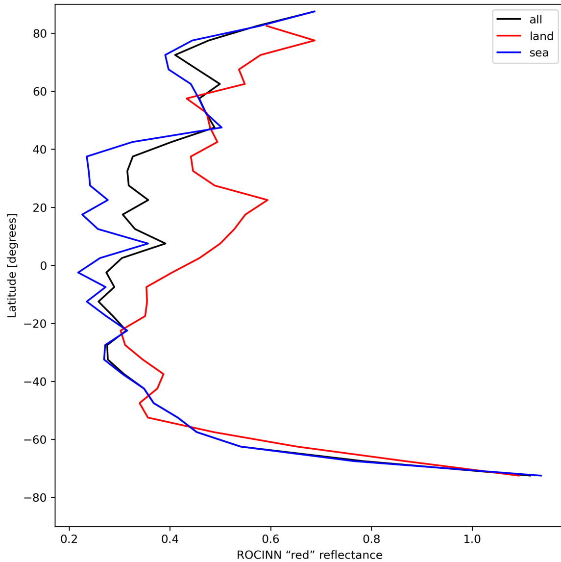
Figure 37: Zonal average of “ROCINN “red” reflectance” for 2023-08-05 to 2023-08-07.
