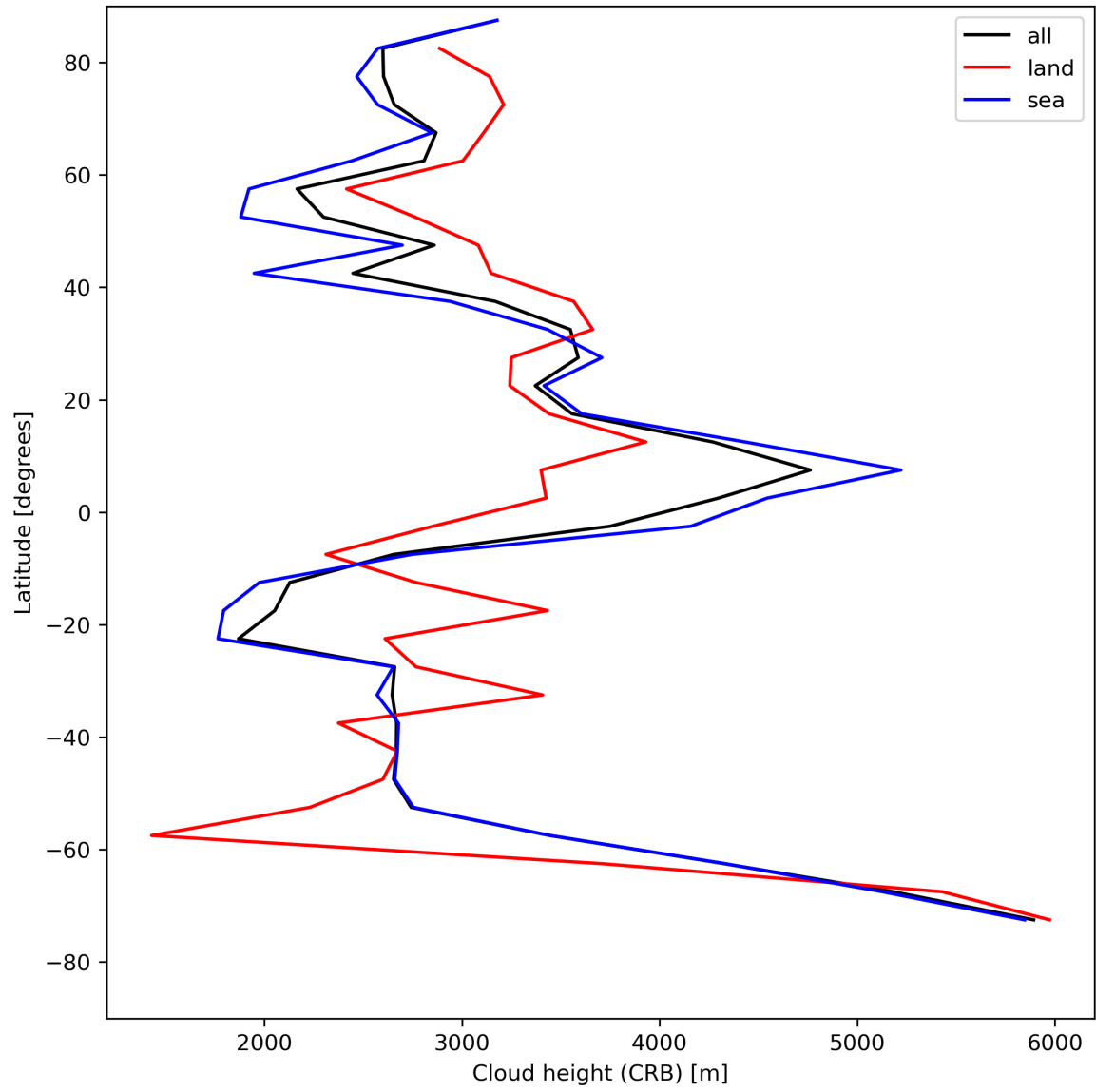
Figure 27: Zonal average of “Cloud height (CRB)” for 2023-08-05 to 2023-08-07.
