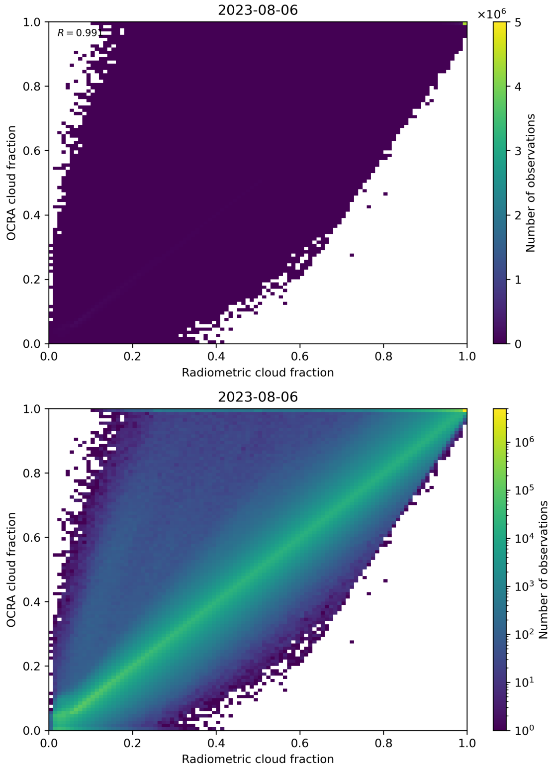
Figure 72: Scatter density plot of “Radiometric cloud fraction” against “OCRA cloud fraction” for 2023-08-05 to 2023-08-07.
