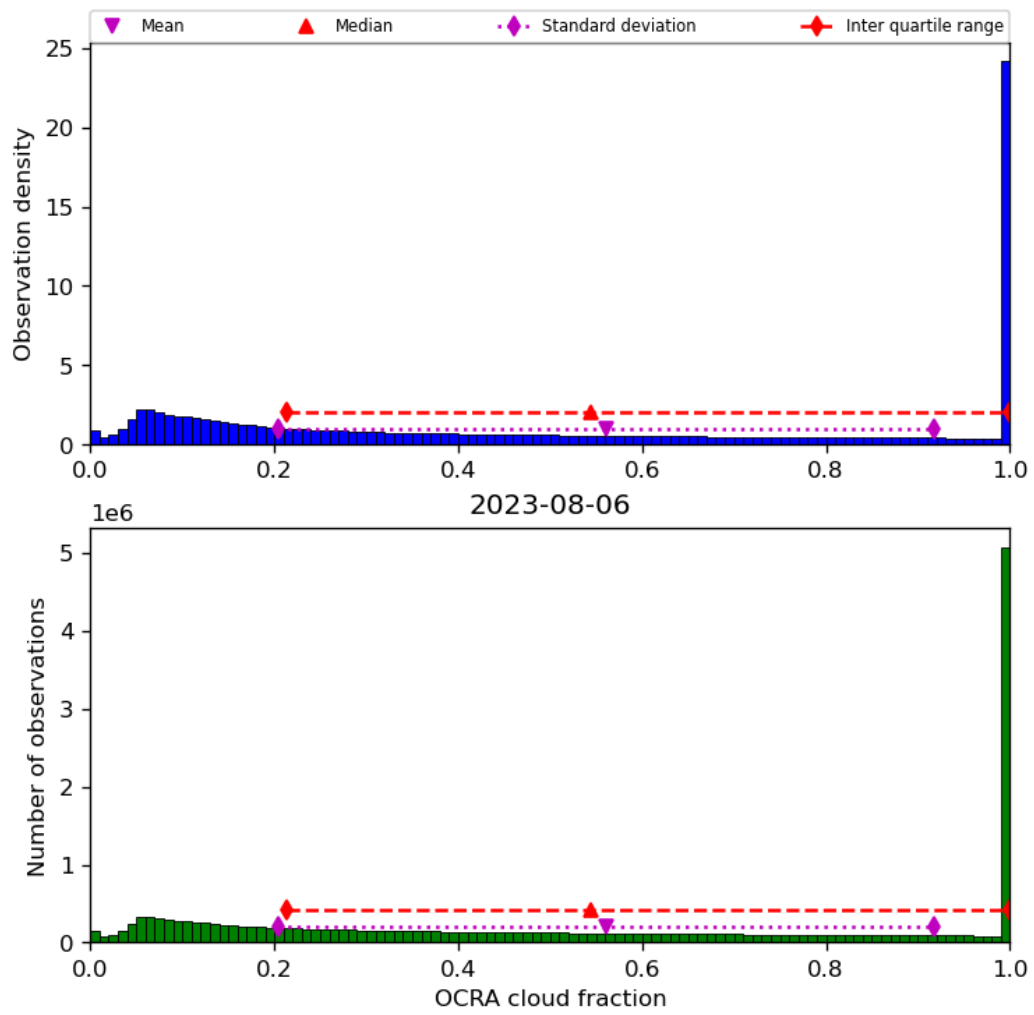
Figure 50: Histogram of “OCRA cloud fraction” for 2023-08-05 to 2023-08-07
