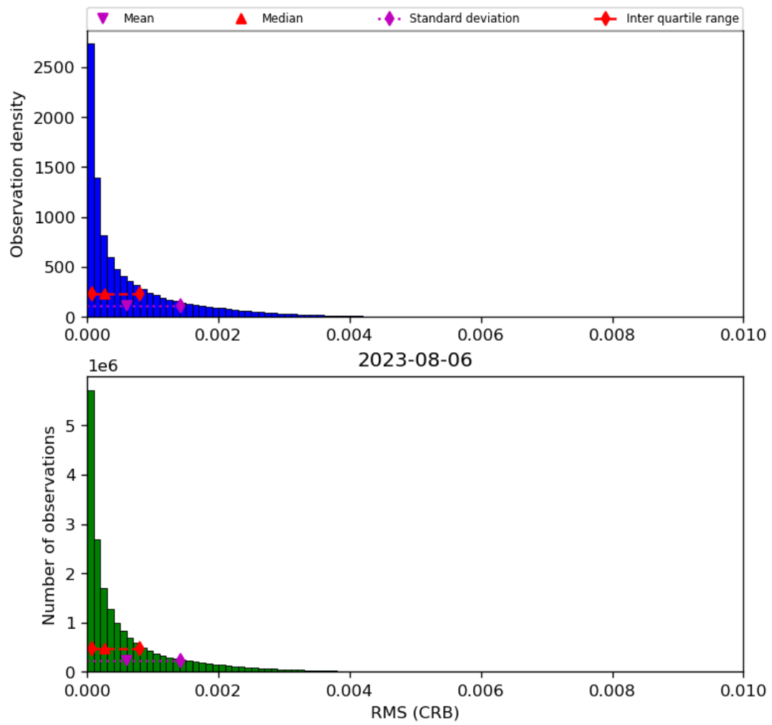
Figure 48: Histogram of “RMS (CRB)” for 2023-08-05 to 2023-08-07
