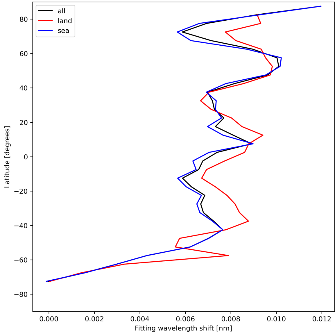
Figure 33: Zonal average of “Fitting wavelength shift” for 2023-08-05 to 2023-08-07.
