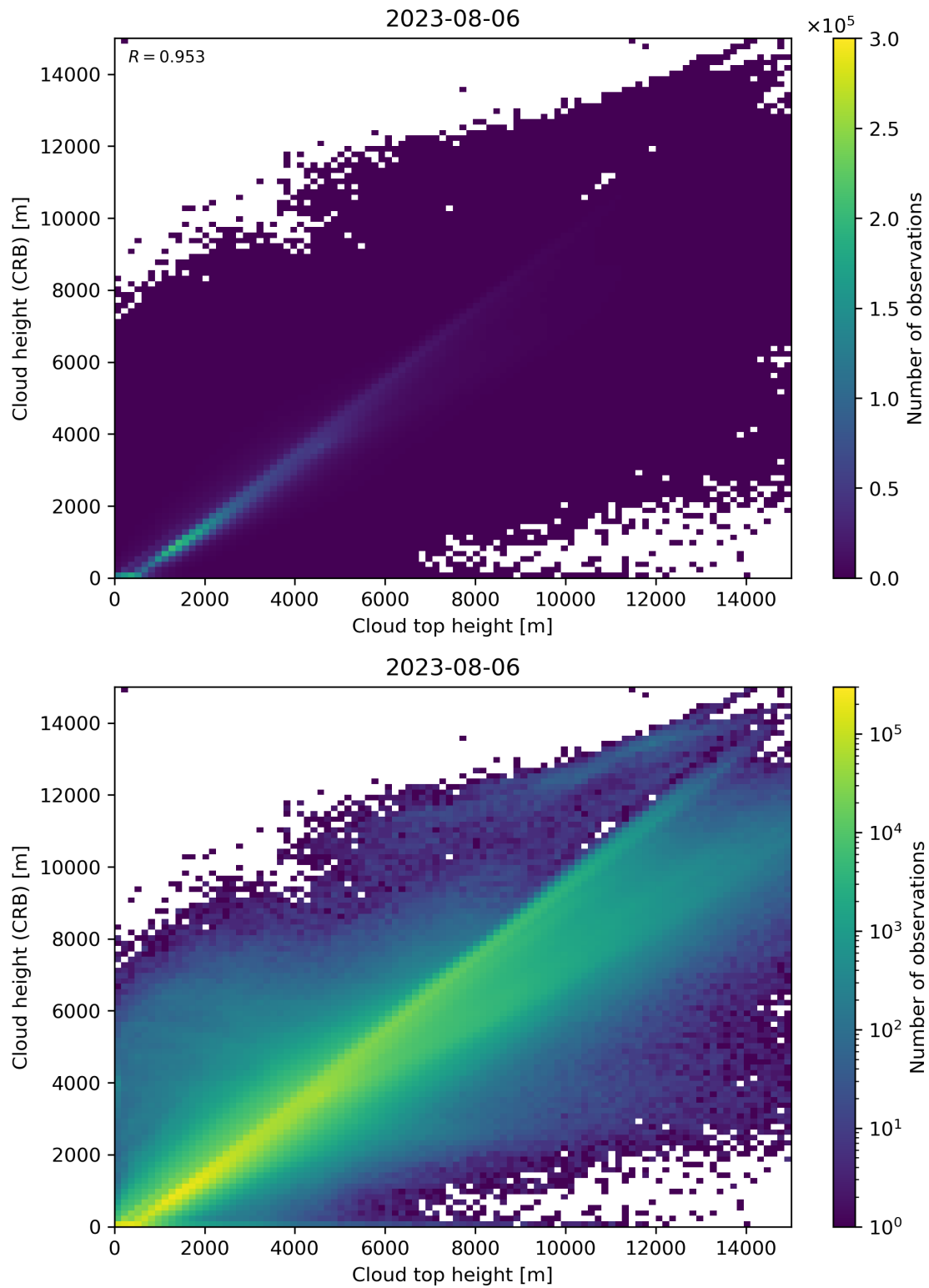
Figure 89: Scatter density plot of “Cloud top height” against “Cloud height (CRB)” for 2023-08-05 to 2023-08-07.
