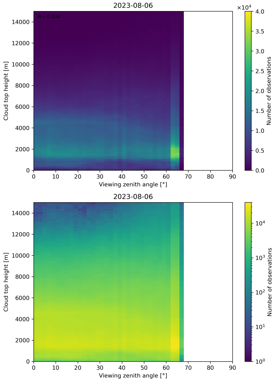
Figure 112: Scatter density plot of “Viewing zenith angle” against “Cloud top height” for 2023-08-05 to 2023-08-07.
