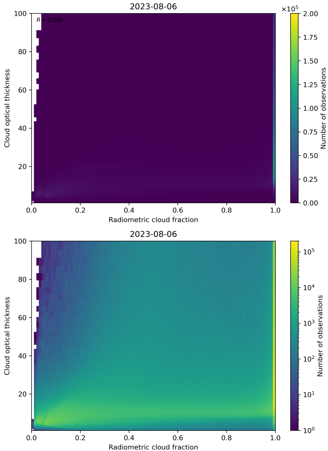
Figure 75: Scatter density plot of “Radiometric cloud fraction” against “Cloud optical thickness” for 2023-08-05 to 2023-08-07.
