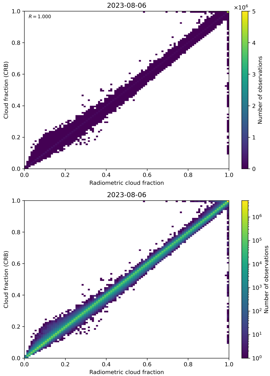
Figure 73: Scatter density plot of “Radiometric cloud fraction” against “Cloud fraction (CRB)” for 2023-08-05 to 2023-08-07.
