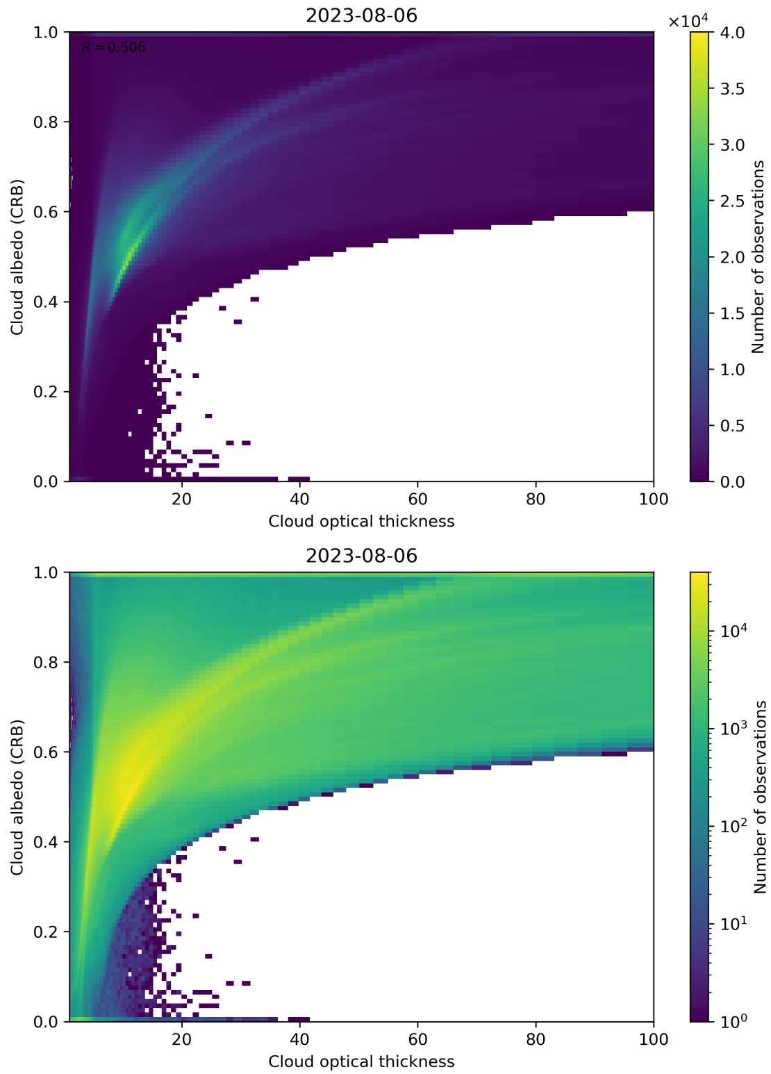
Figure 82: Scatter density plot of “Cloud optical thickness” against “Cloud albedo (CRB)” for 2023-08-05 to 2023-08-07.
