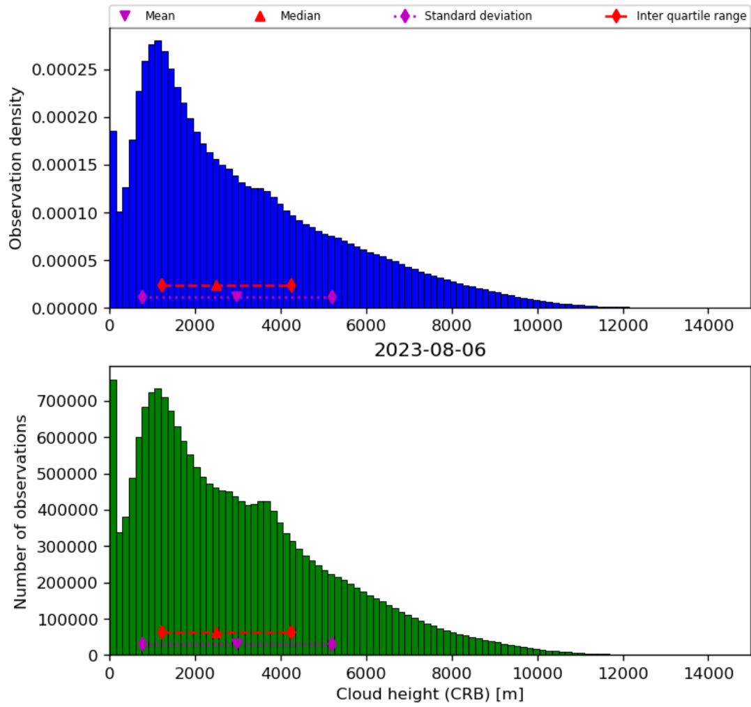
Figure 43: Histogram of “Cloud height (CRB)” for 2023-08-05 to 2023-08-07
