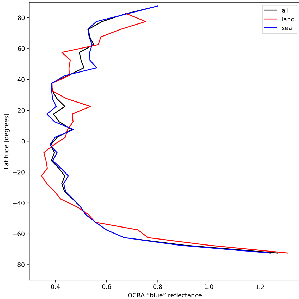
Figure 35: Zonal average of “OCRA “blue” reflectance” for 2023-08-05 to 2023-08-07.
