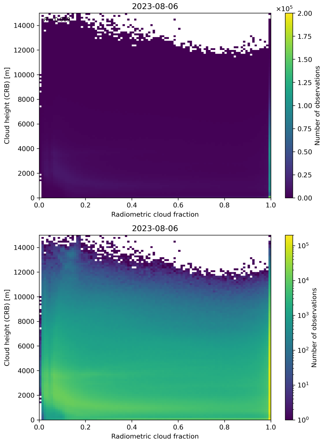
Figure 74: Scatter density plot of “Radiometric cloud fraction” against “Cloud height (CRB)” for 2023-08-05 to 2023-08-07.
