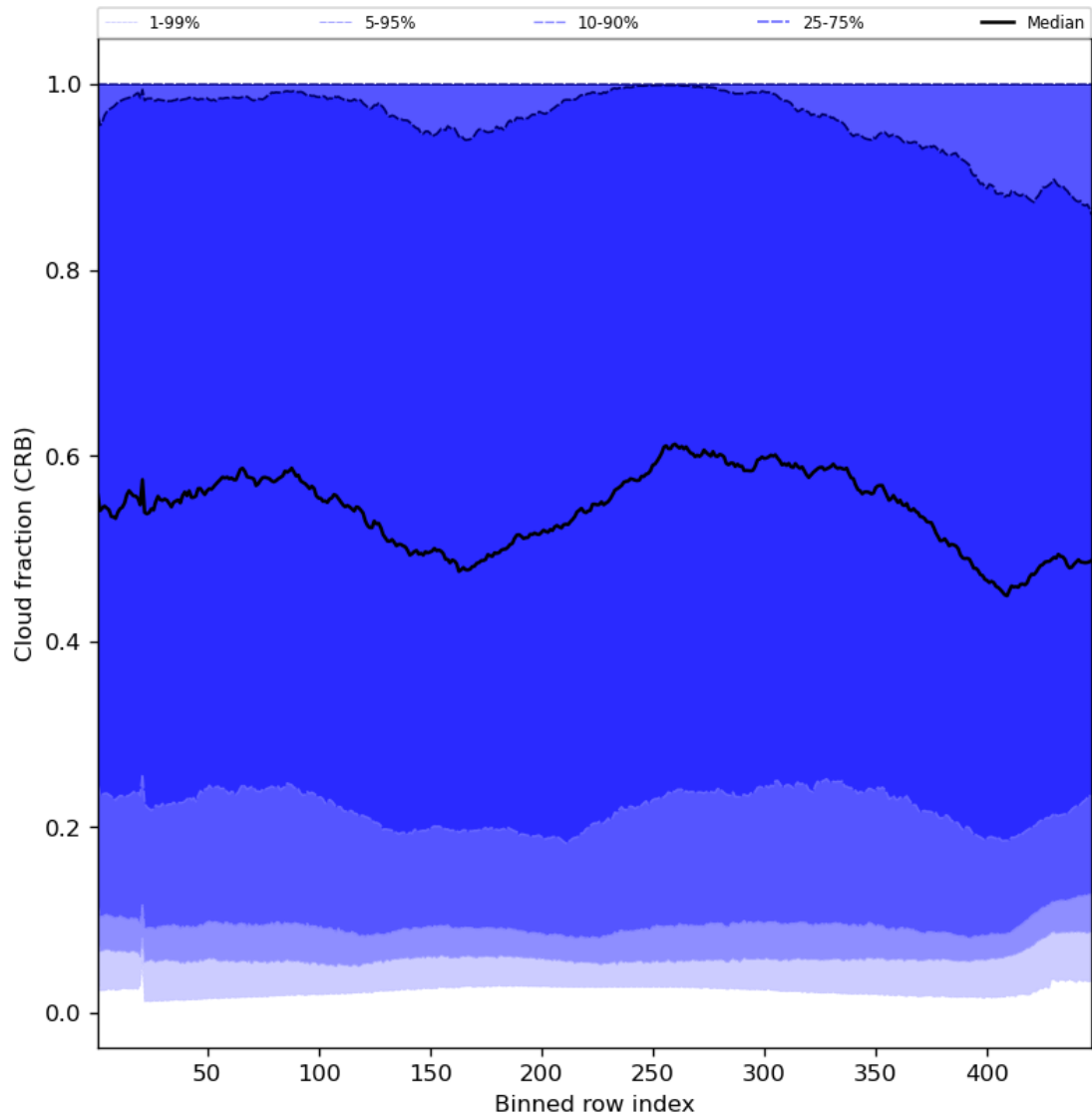
Figure 58: Along track statistics of “Cloud fraction (CRB)” for 2023-08-05 to 2023-08-07
