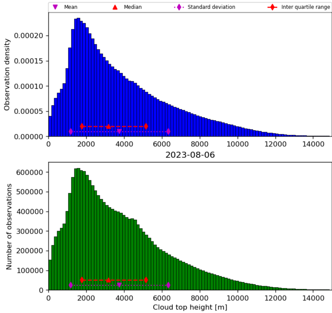
Figure 40: Histogram of “Cloud top height” for 2023-08-05 to 2023-08-07
