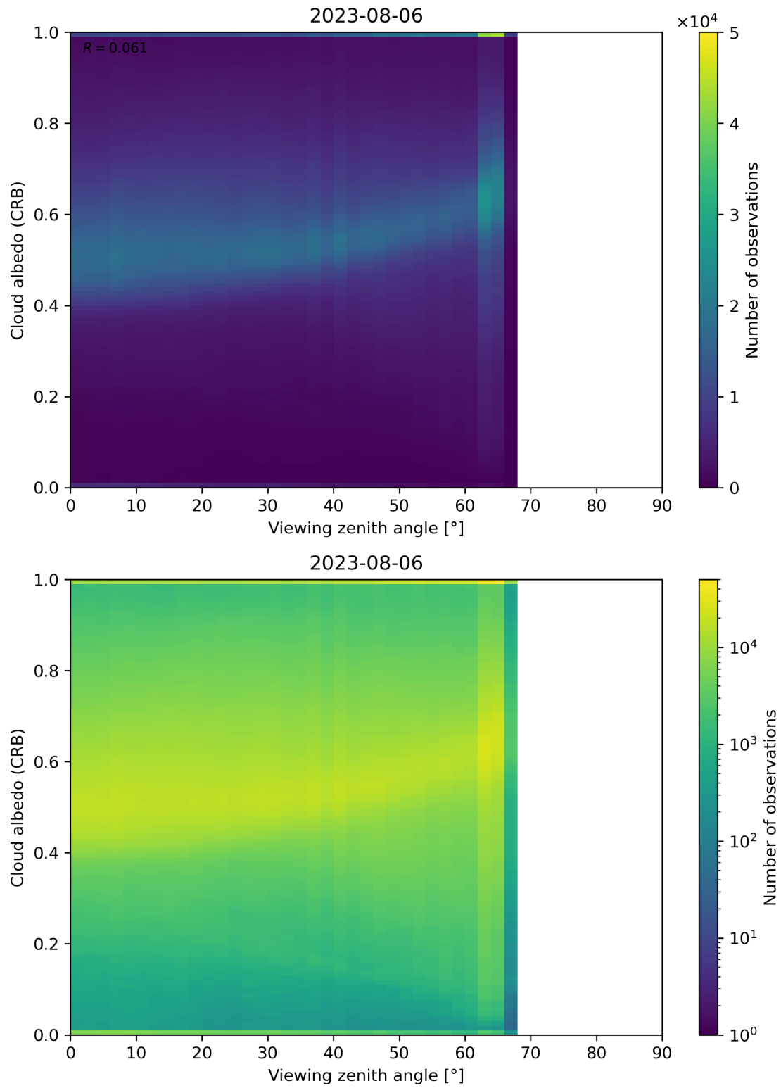
Figure 106: Scatter density plot of “Viewing zenith angle” against “Cloud albedo (CRB)” for 2023-08-05 to 2023-08-07.
