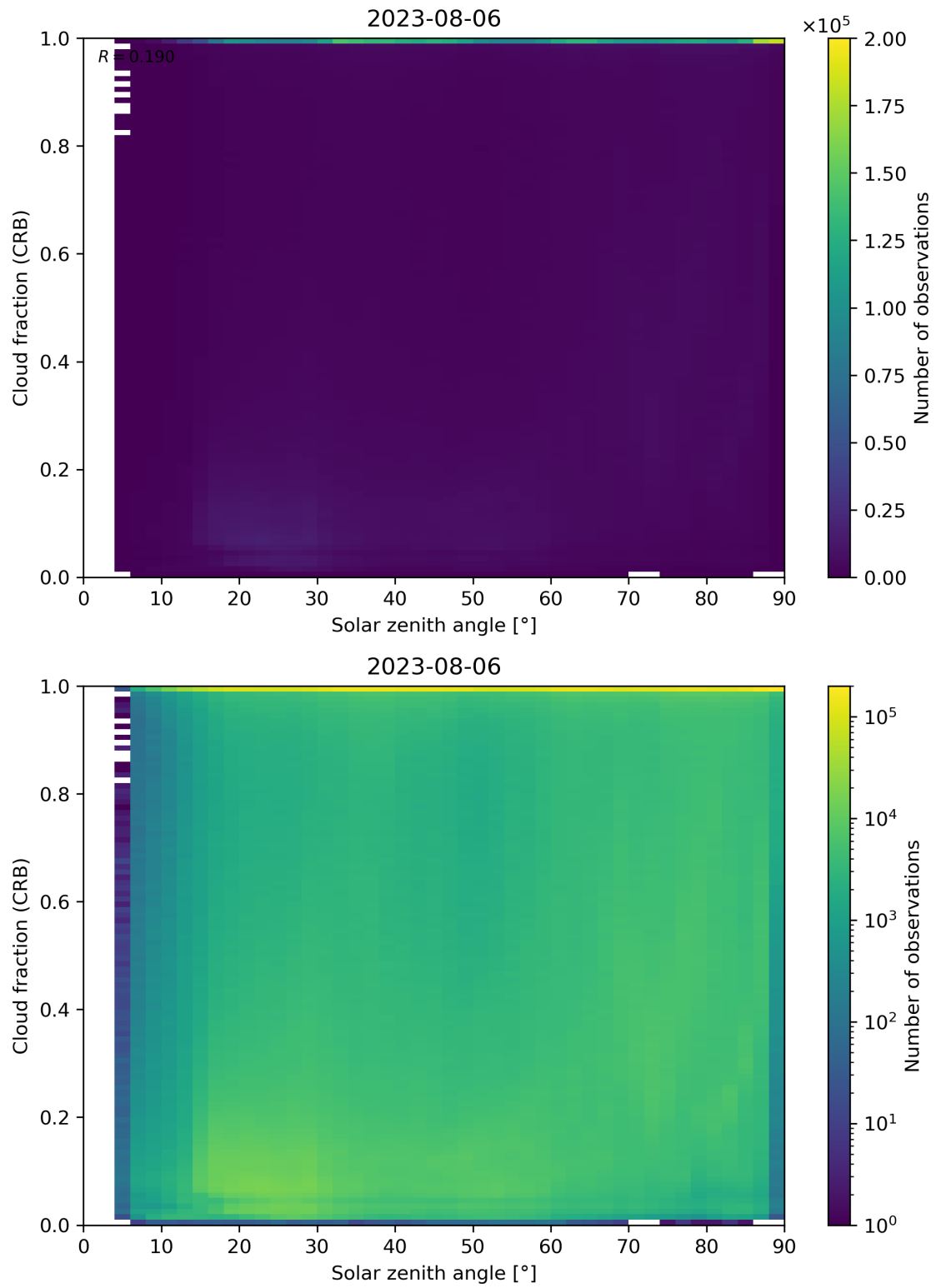
Figure 101: Scatter density plot of “Solar zenith angle” against “Cloud fraction (CRB)” for 2023-08-05 to 2023-08-07.
