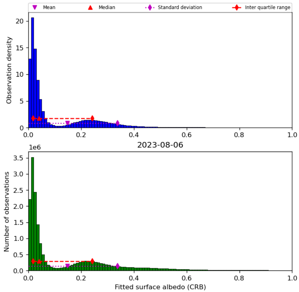
Figure 46: Histogram of “Fitted surface albedo (CRB)” for 2023-08-05 to 2023-08-07
