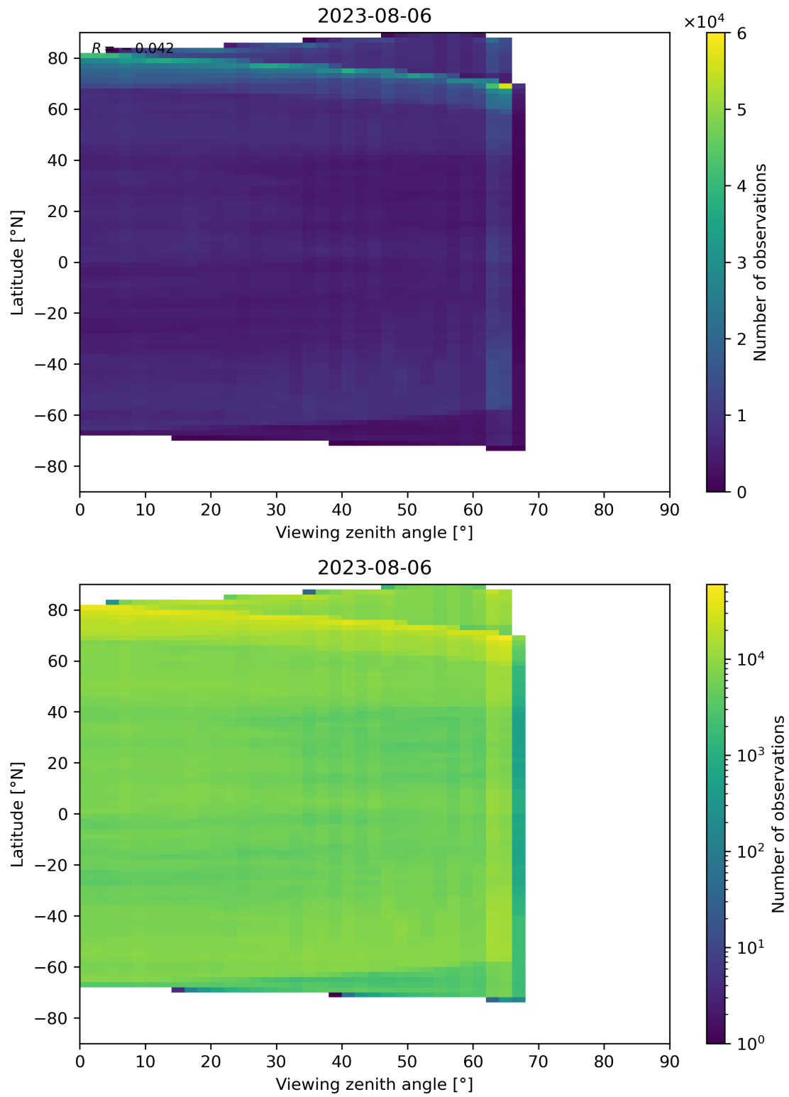
Figure 113: Scatter density plot of “Viewing zenith angle” against “Latitude” for 2023-08-05 to 2023-08-07.
