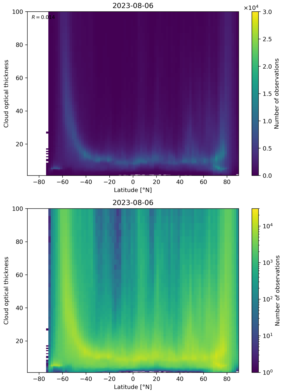
Figure 96: Scatter density plot of “Latitude” against “Cloud optical thickness” for 2023-08-05 to 2023-08-07.
