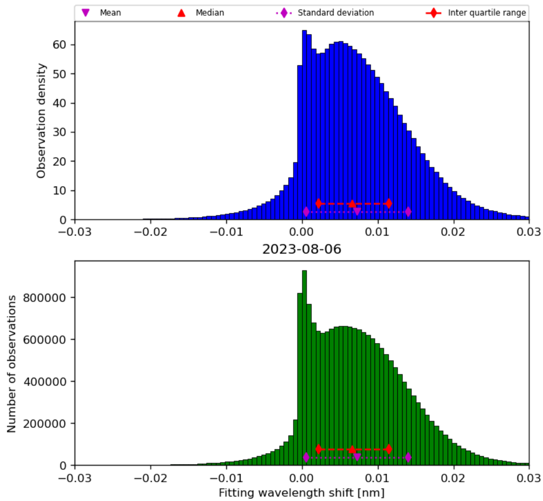
Figure 49: Histogram of “Fitting wavelength shift” for 2023-08-05 to 2023-08-07
