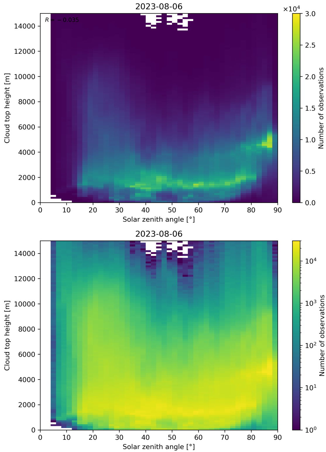
Figure 104: Scatter density plot of “Solar zenith angle” against “Cloud top height” for 2023-08-05 to 2023-08-07.
