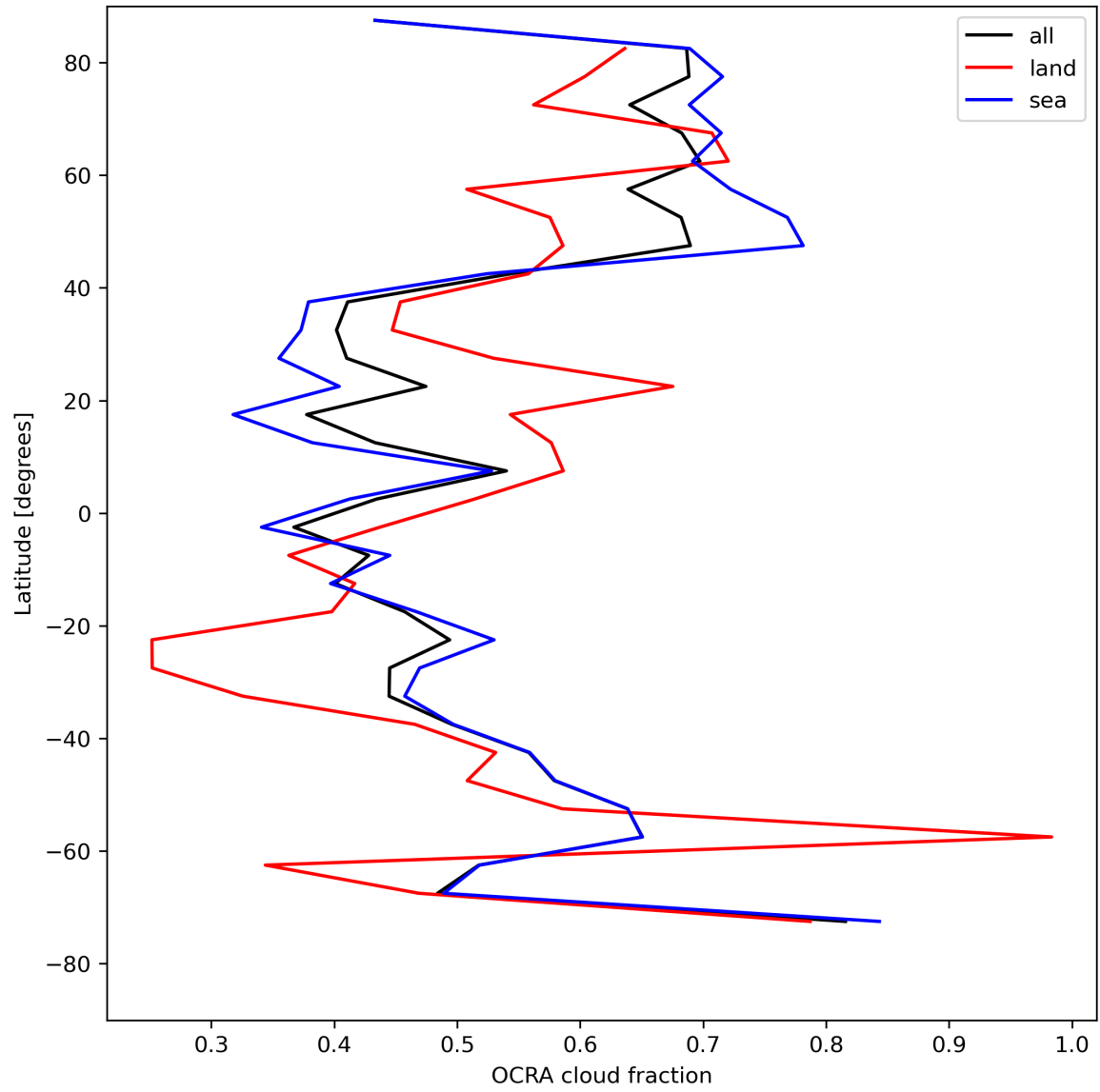
Figure 34: Zonal average of “OCRA cloud fraction” for 2023-08-05 to 2023-08-07.
