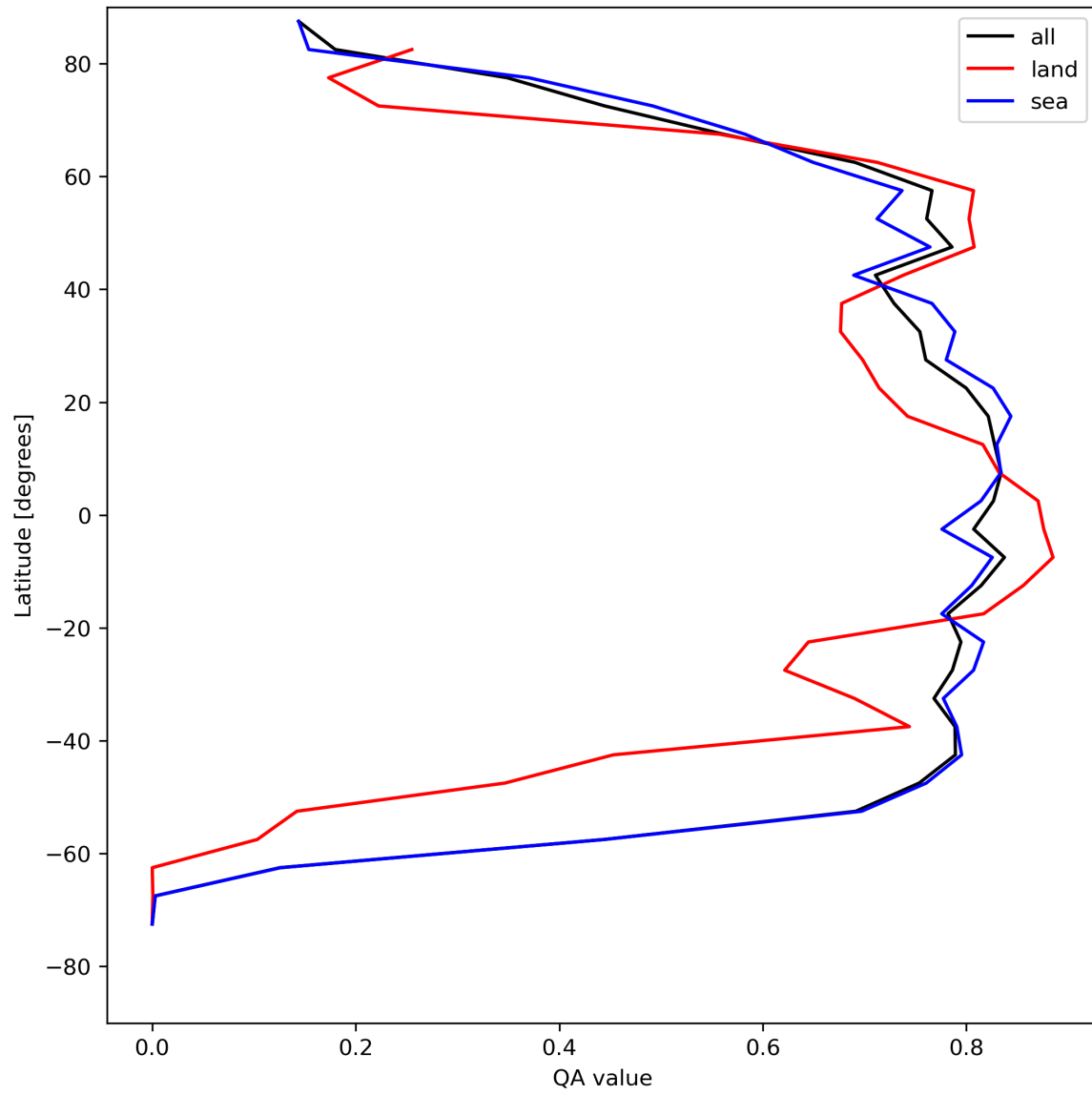
Figure 22: Zonal average of “QA value” for 2023-08-05 to 2023-08-07.
