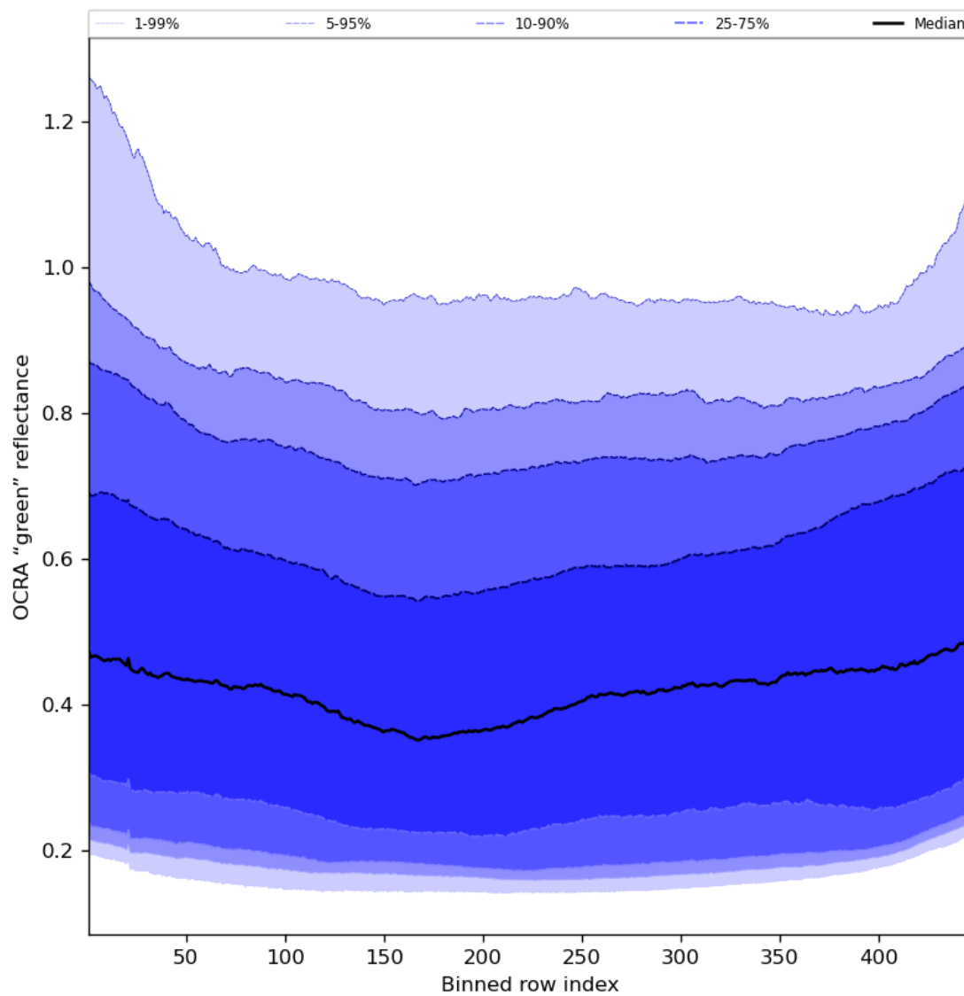
Figure 68: Along track statistics of “OCRA “green” reflectance” for 2023-08-05 to 2023-08-07
