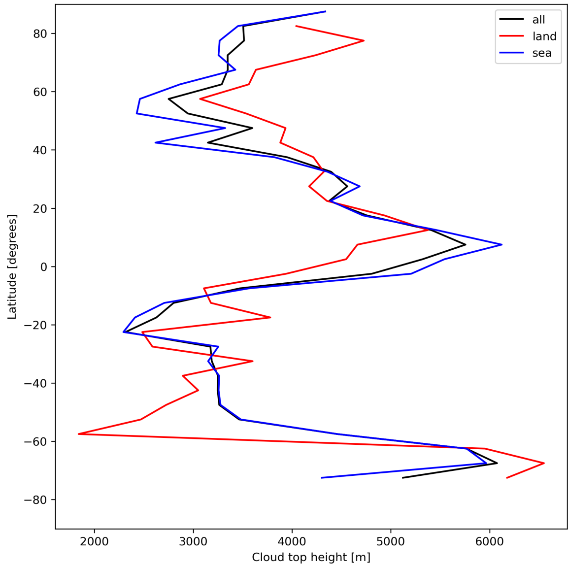
Figure 24: Zonal average of “Cloud top height” for 2023-08-05 to 2023-08-07.
