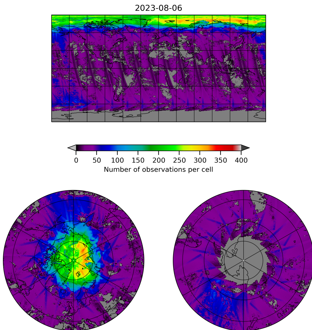
Figure 21: Map of the number of observations for 2023-08-05 to 2023-08-07
