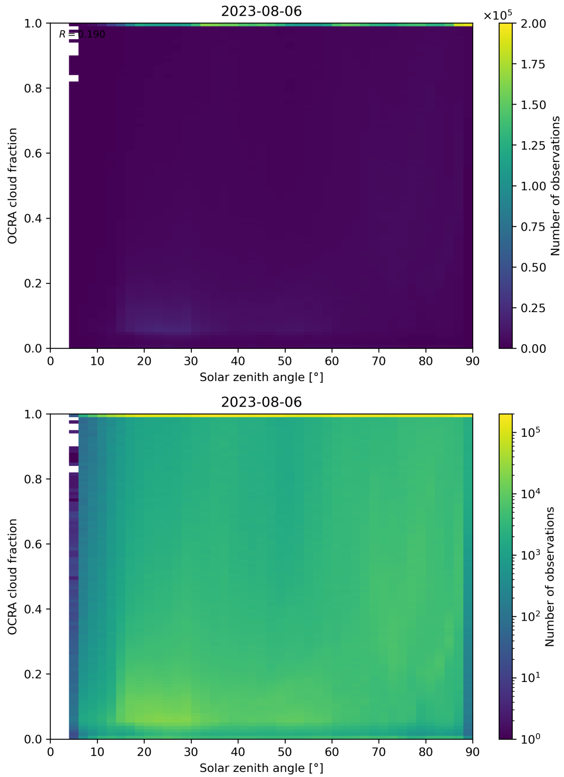
Figure 100: Scatter density plot of “Solar zenith angle” against “OCRA cloud fraction” for 2023-08-05 to 2023-08-07.
