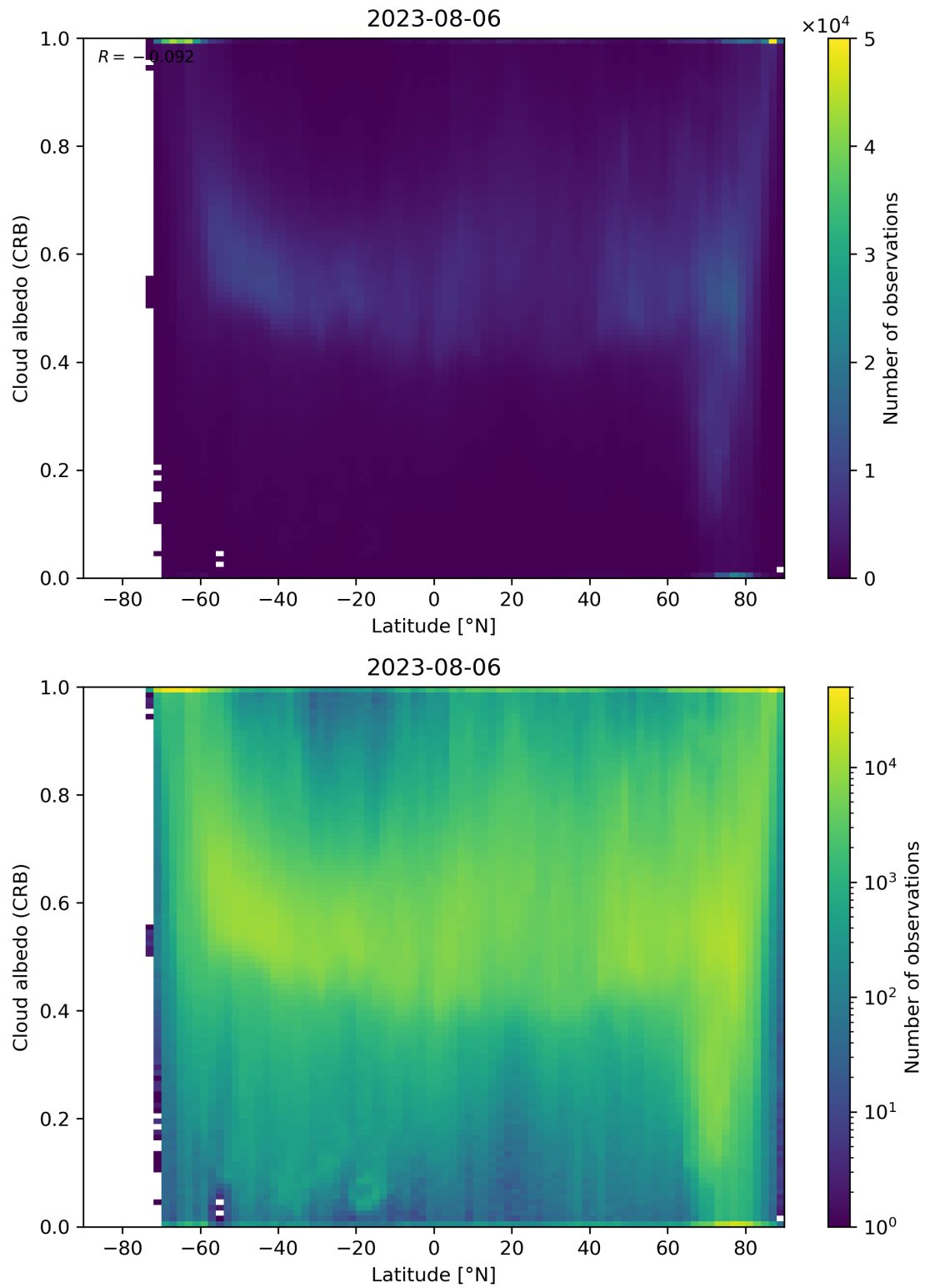
Figure 91: Scatter density plot of “Latitude” against “Cloud albedo (CRB)” for 2023-08-05 to 2023-08-07.
