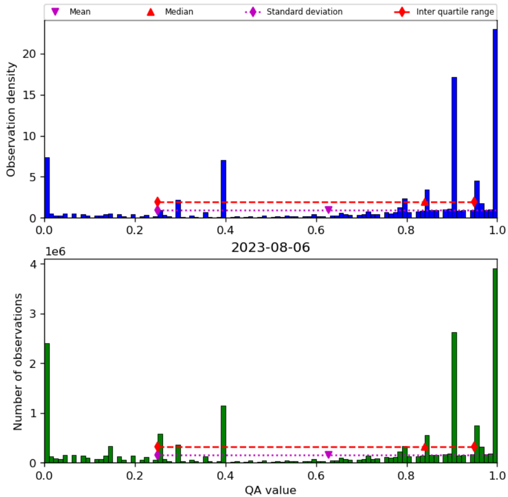
Figure 38: Histogram of “QA value” for 2023-08-05 to 2023-08-07
