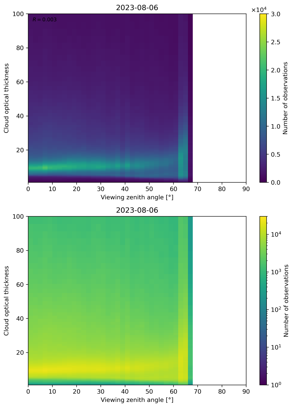
Figure 111: Scatter density plot of “Viewing zenith angle” against “Cloud optical thickness” for 2023-08-05 to 2023-08-07.
