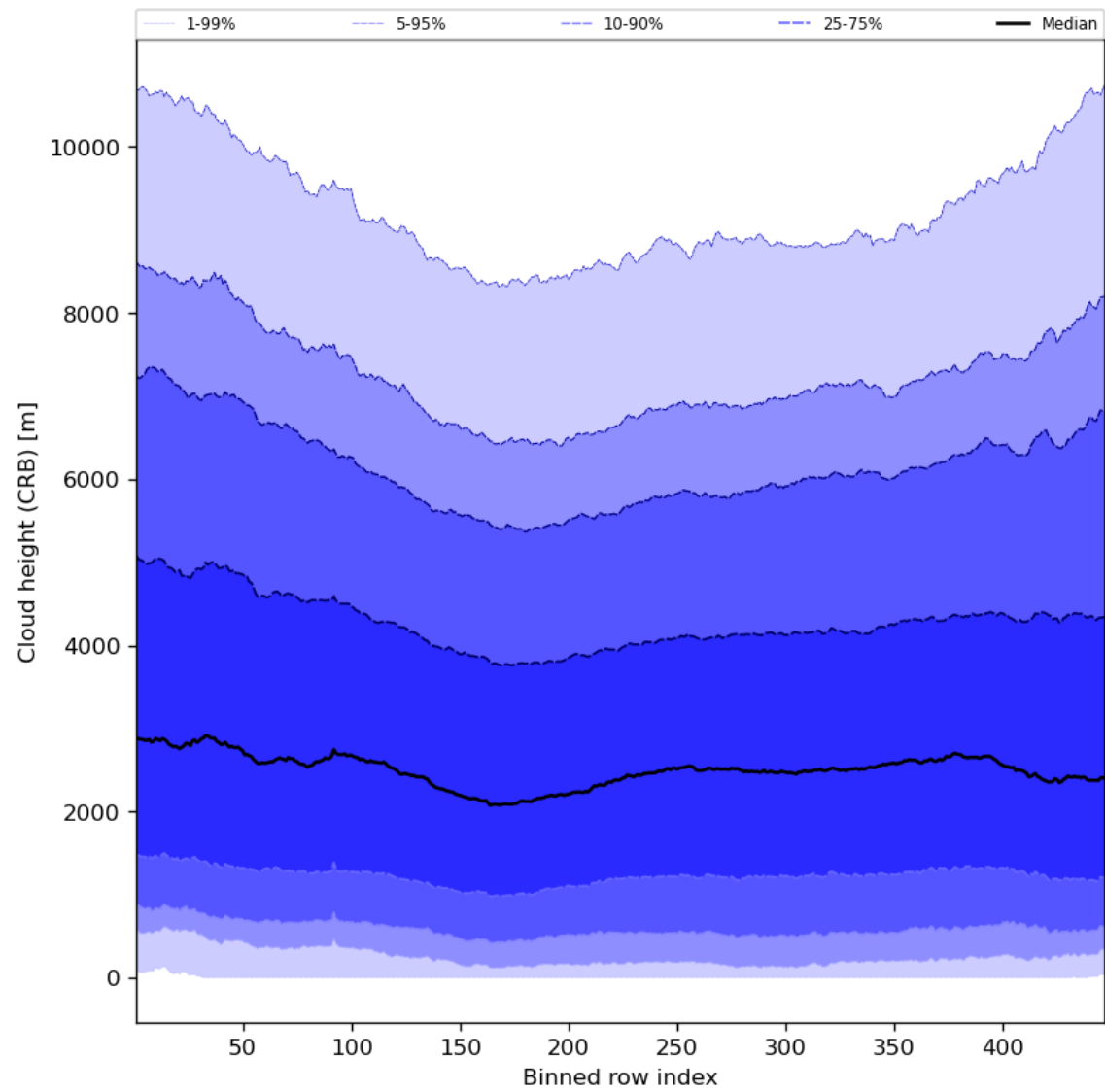
Figure 59: Along track statistics of “Cloud height (CRB)” for 2023-08-05 to 2023-08-07
