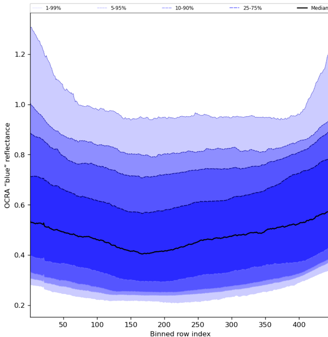
Figure 67: Along track statistics of "OCRA "blue" reflectance" for 2023-08-05 to 2023-08-07
