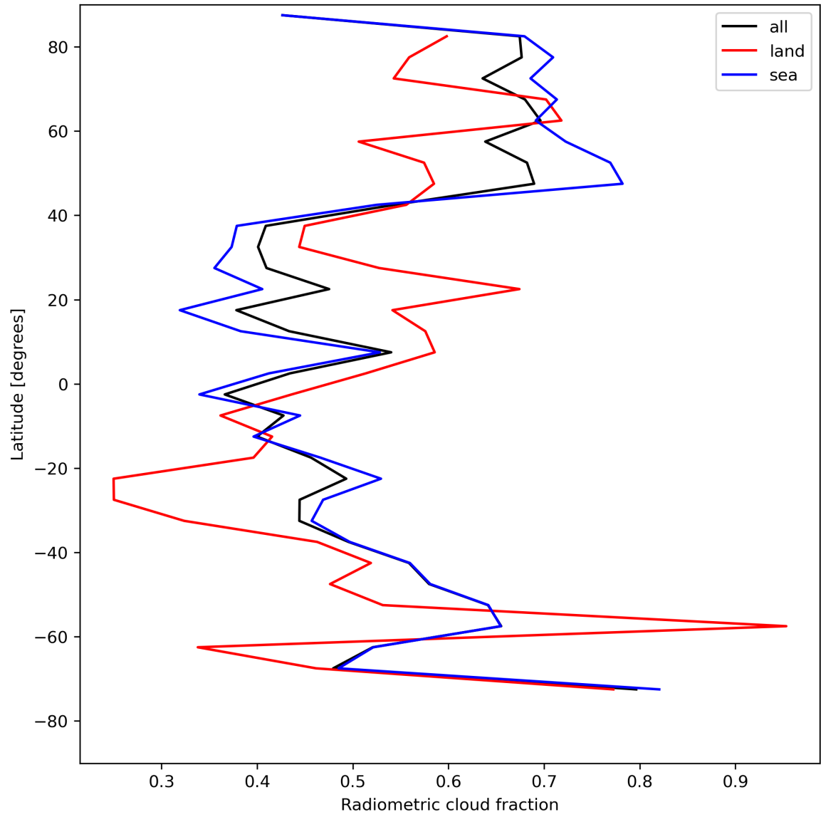
Figure 23: Zonal average of “Radiometric cloud fraction” for 2023-08-05 to 2023-08-07.
