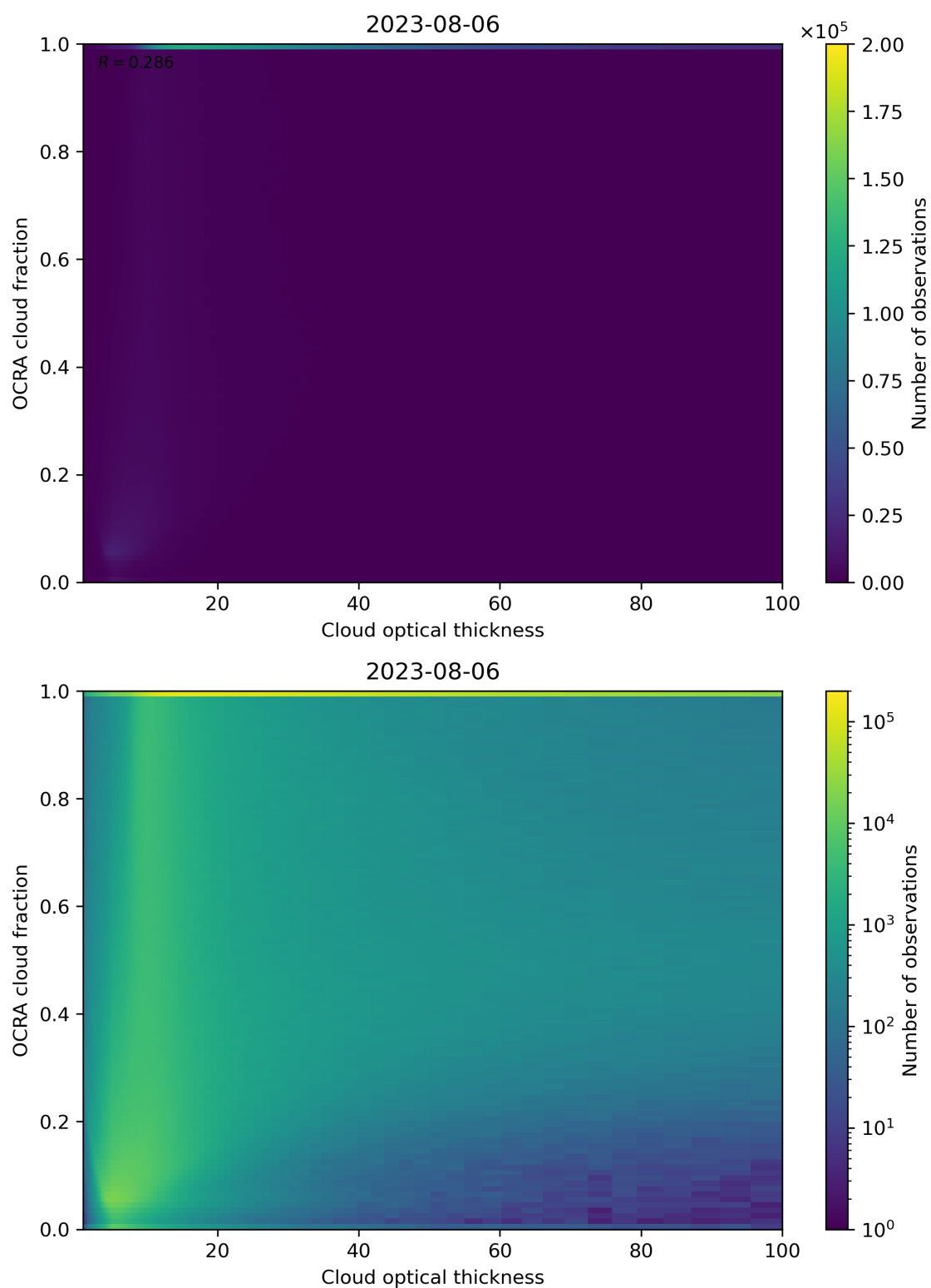
Figure 83: Scatter density plot of “Cloud optical thickness” against “OCRA cloud fraction” for 2023-08-05 to 2023-08-07.
