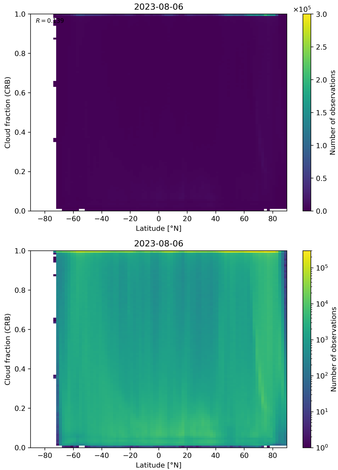
Figure 94: Scatter density plot of “Latitude” against “Cloud fraction (CRB)” for 2023-08-05 to 2023-08-07.
