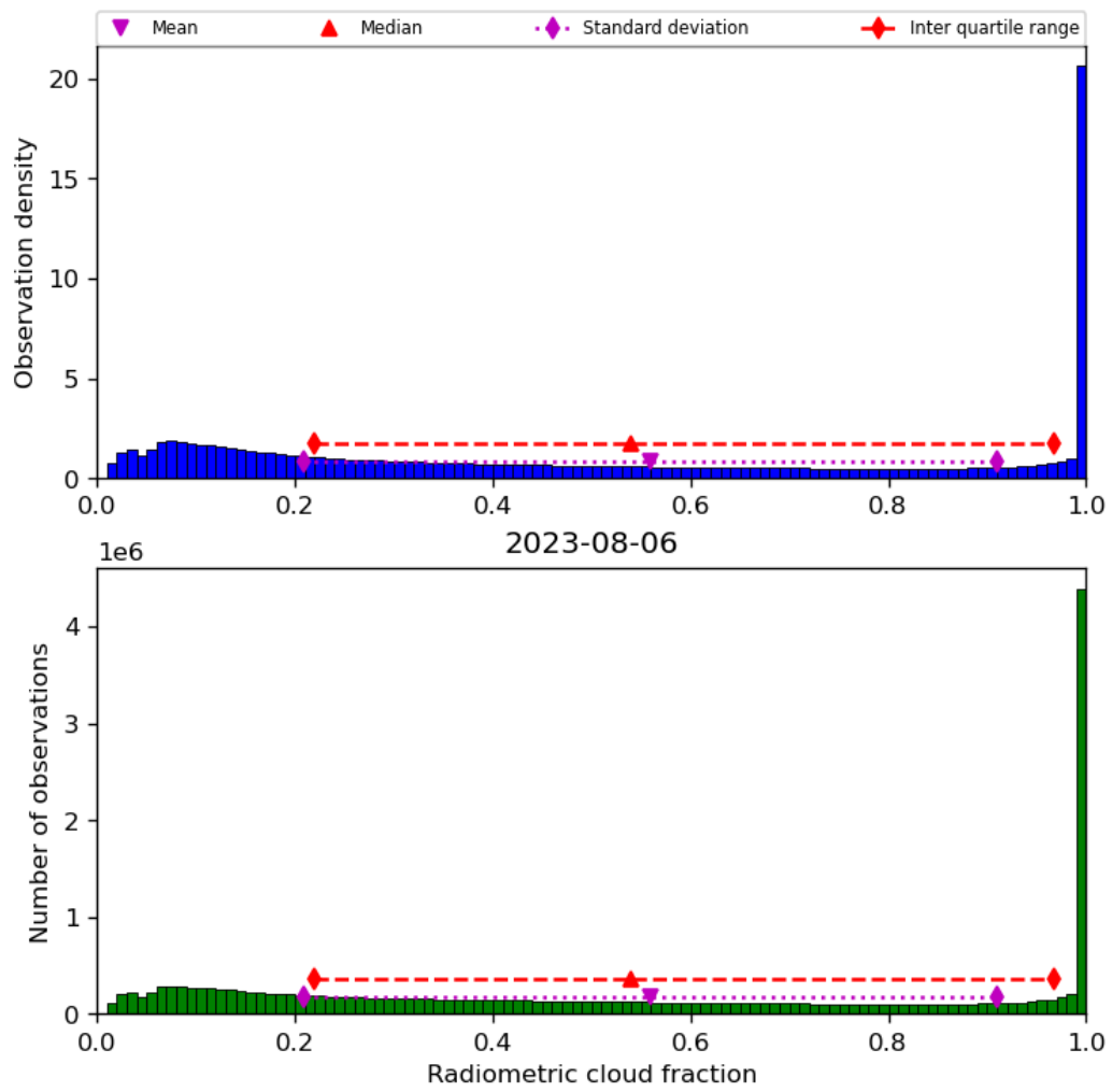
Figure 39: Histogram of “Radiometric cloud fraction” for 2023-08-05 to 2023-08-07
