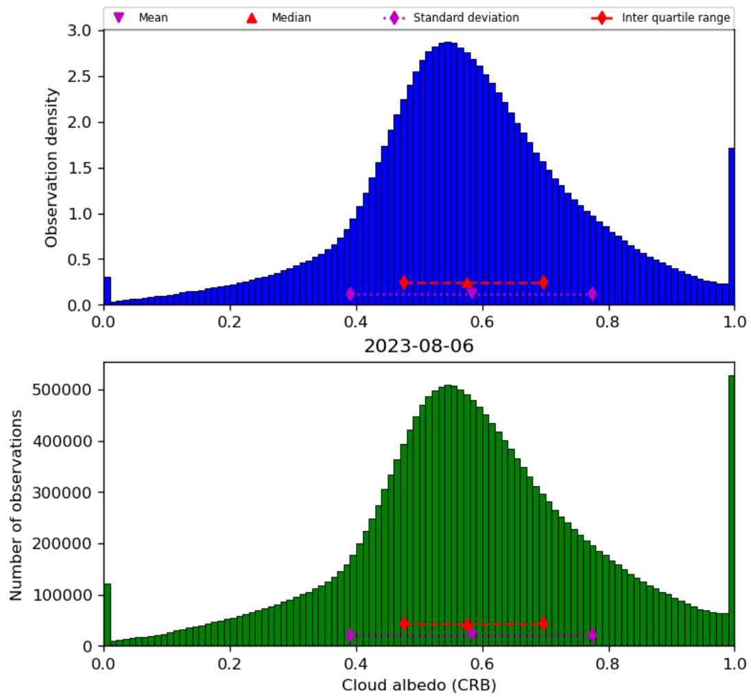
Figure 44: Histogram of “Cloud albedo (CRB)” for 2023-08-05 to 2023-08-07
