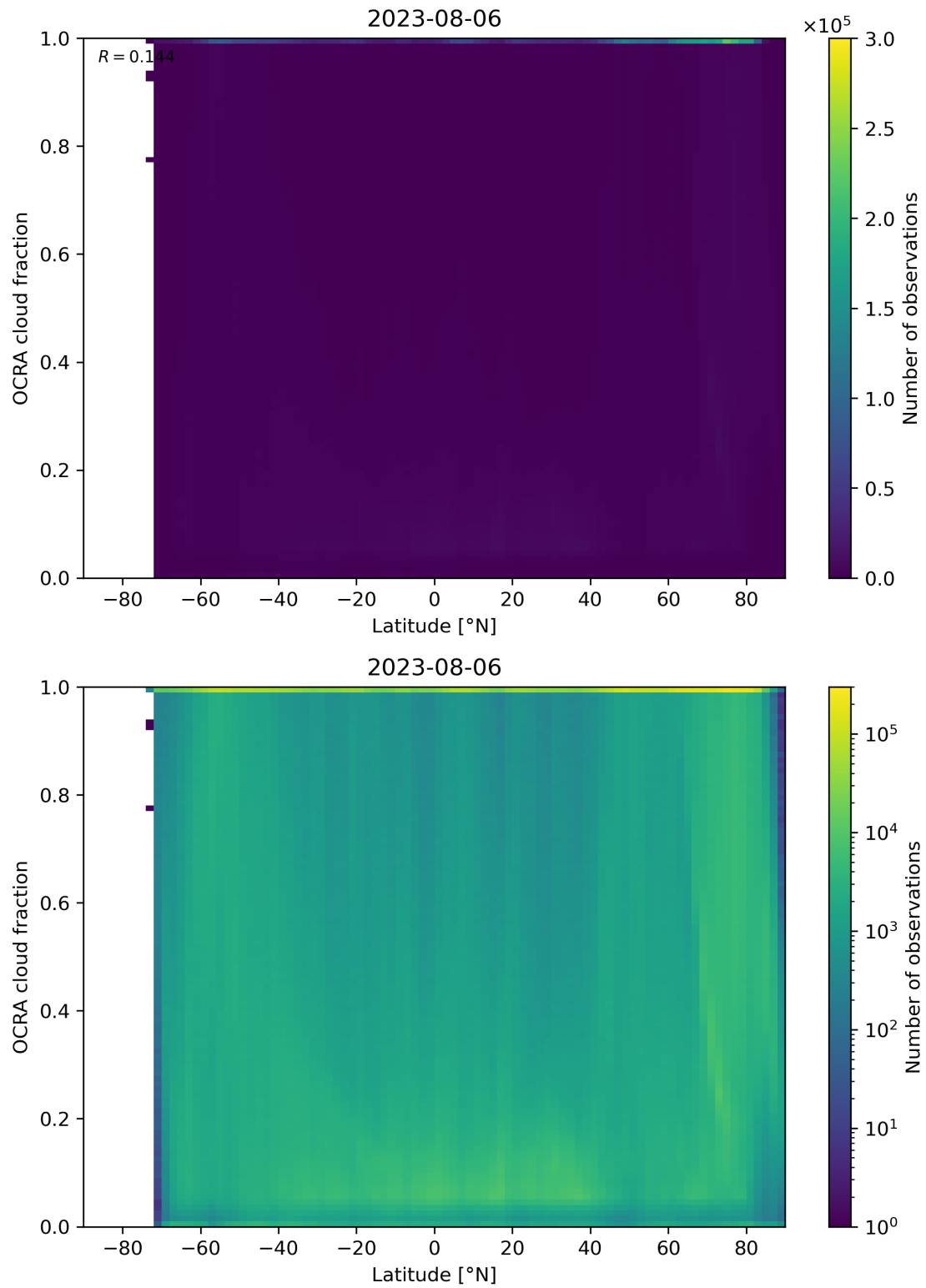
Figure 93: Scatter density plot of “Latitude” against “OCRA cloud fraction” for 2023-08-05 to 2023-08-07.
