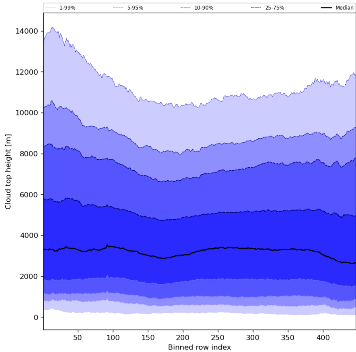
Figure 56: Along track statistics of “Cloud top height” for 2023-08-05 to 2023-08-07
