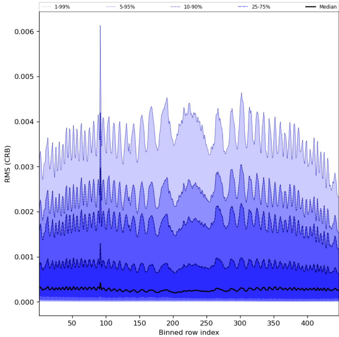
Figure 64: Along track statistics of “RMS (CRB)” for 2023-08-05 to 2023-08-07
