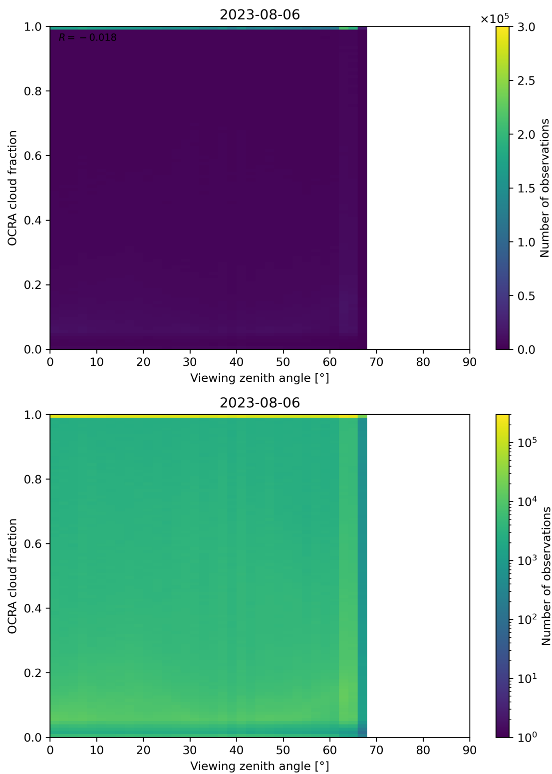
Figure 108: Scatter density plot of “Viewing zenith angle” against “OCRA cloud fraction” for 2023-08-05 to 2023-08-07.
