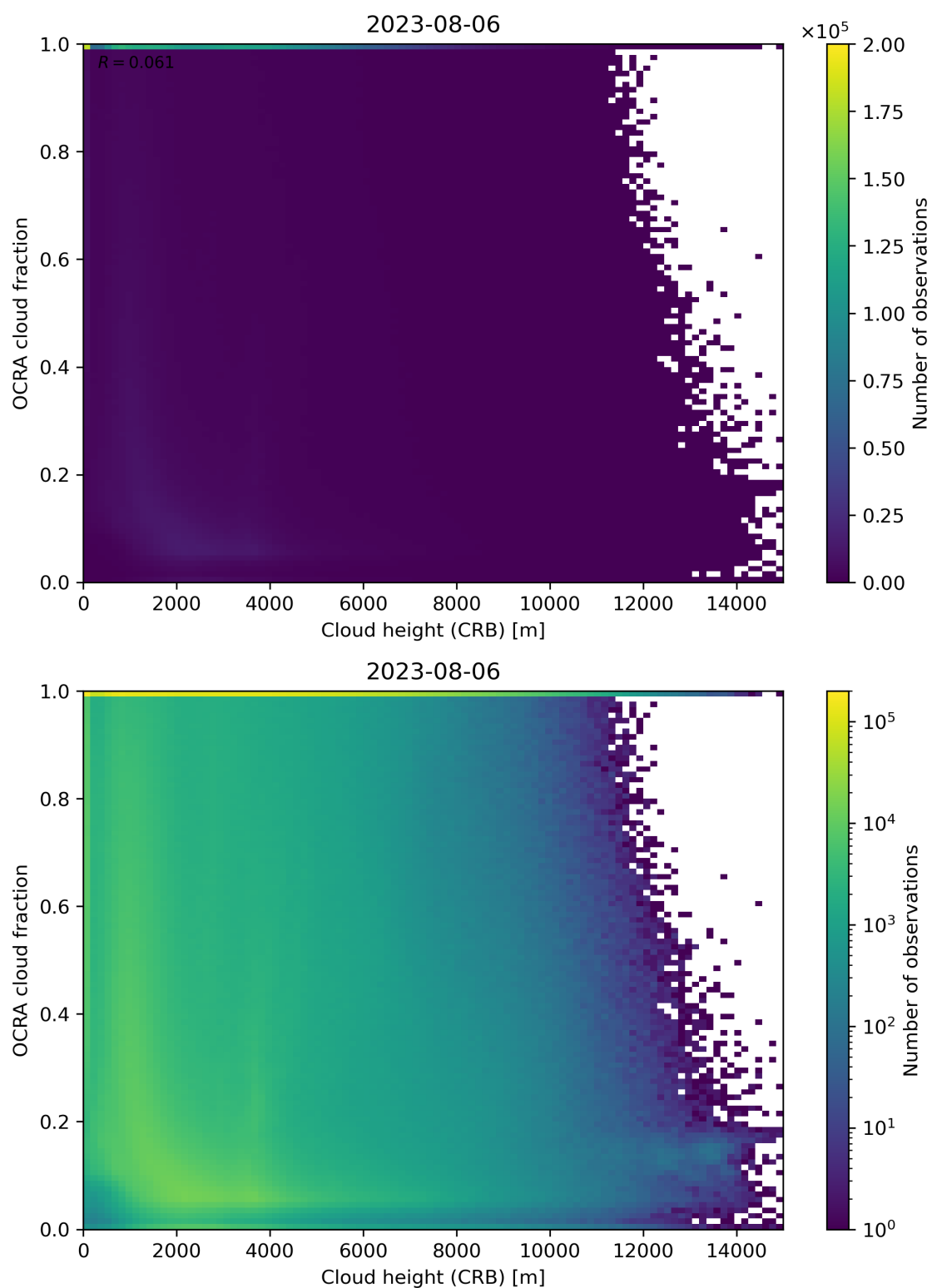
Figure 81: Scatter density plot of “Cloud height (CRB)” against “OCRA cloud fraction” for 2023-08-05 to 2023-08-07.
