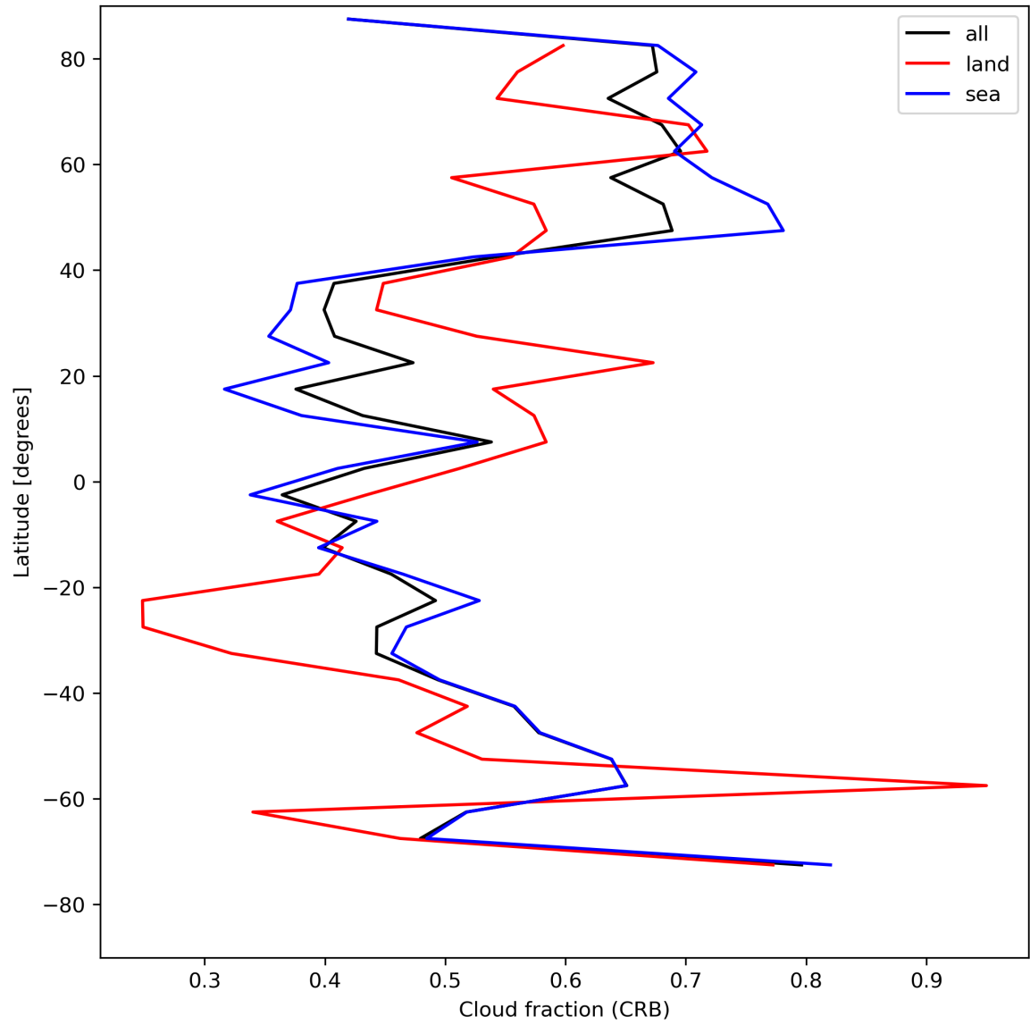
Figure 26: Zonal average of “Cloud fraction (CRB)” for 2023-08-05 to 2023-08-07.
