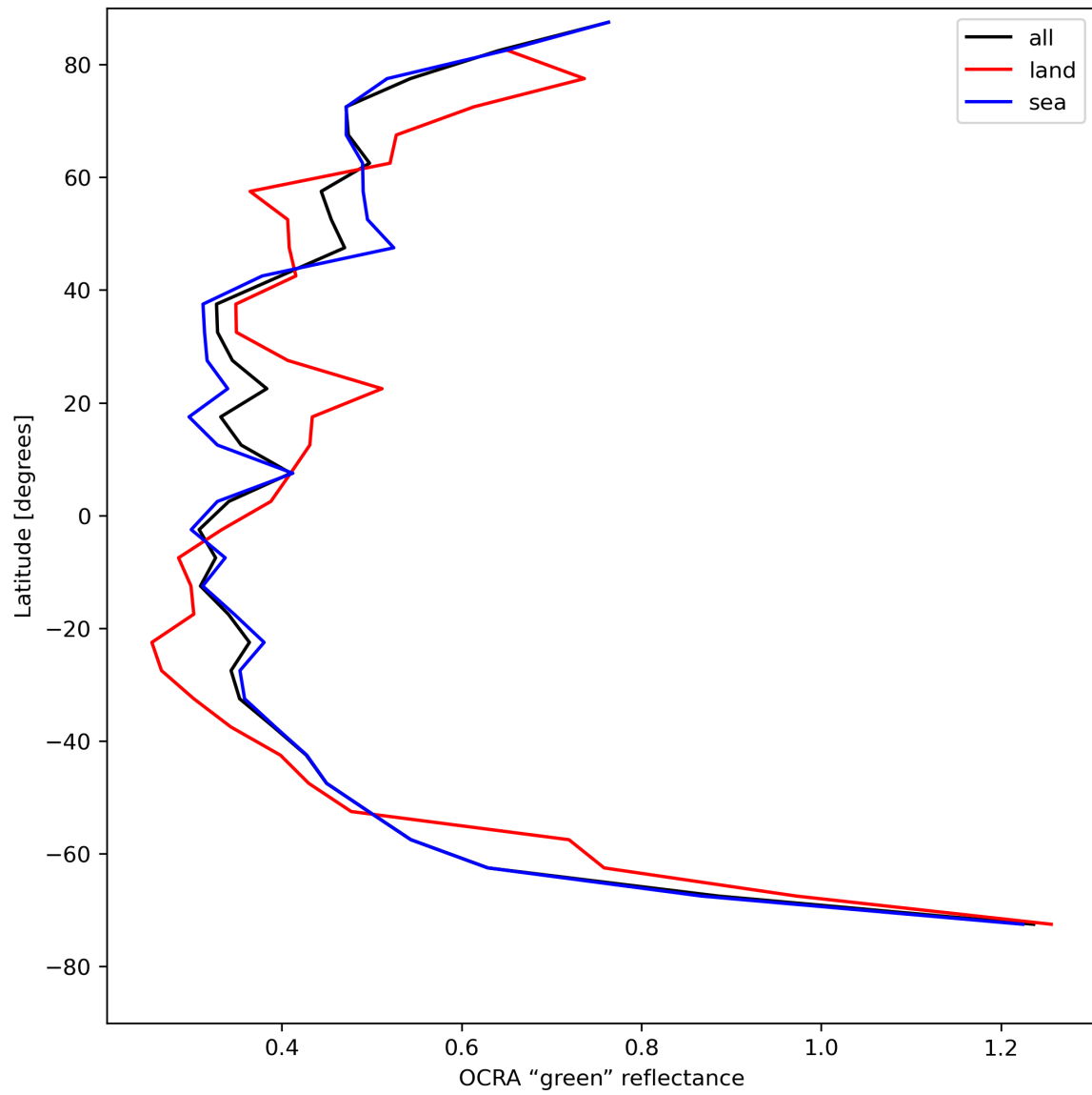
Figure 36: Zonal average of “OCRA “green” reflectance” for 2023-08-05 to 2023-08-07.
