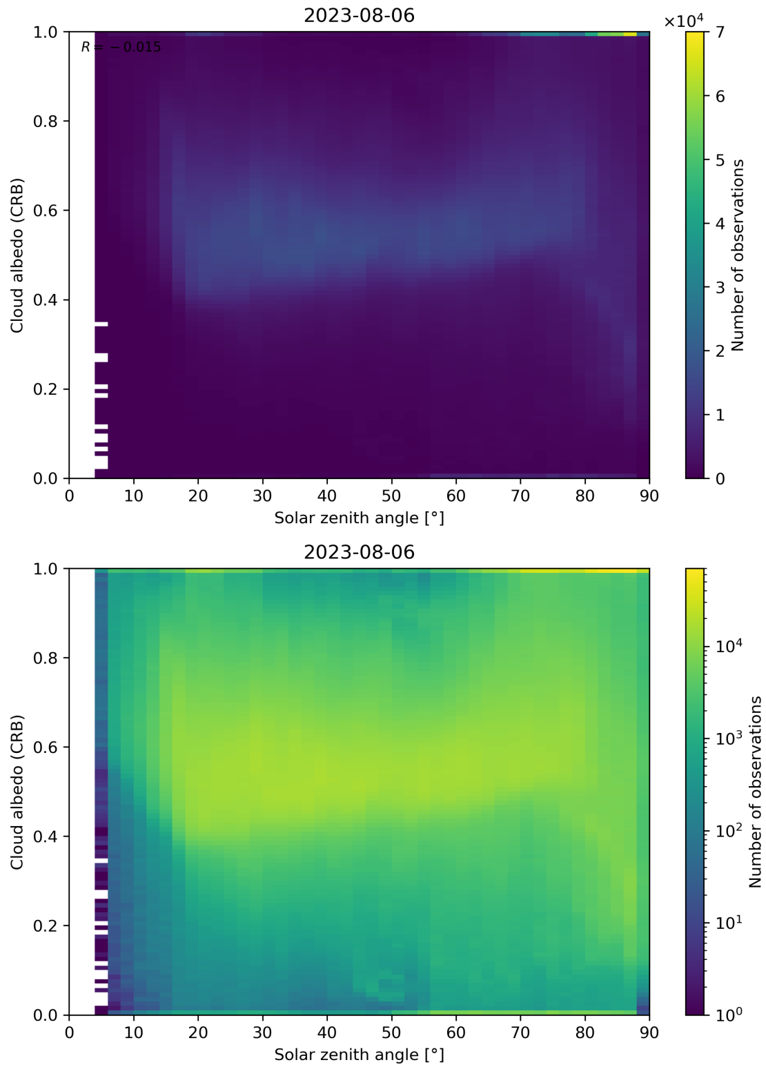
Figure 98: Scatter density plot of “Solar zenith angle” against “Cloud albedo (CRB)” for 2023-08-05 to 2023-08-07.
