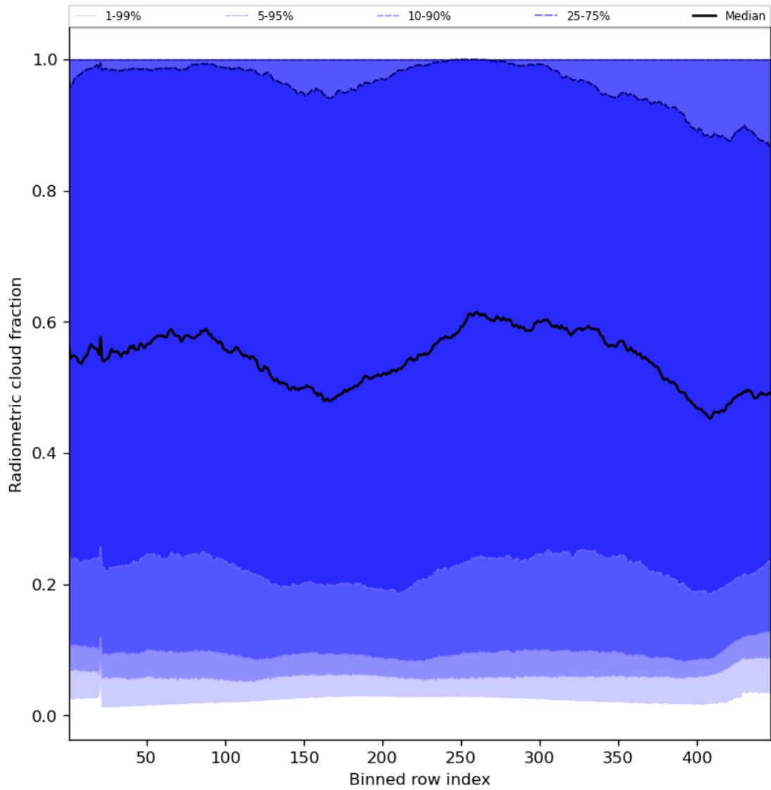
Figure 55: Along track statistics of “Radiometric cloud fraction” for 2023-08-05 to 2023-08-07
