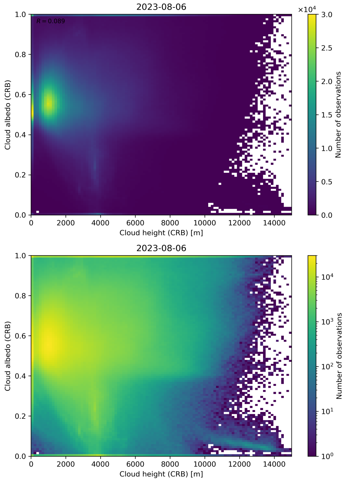
Figure 80: Scatter density plot of “Cloud height (CRB)” against “Cloud albedo (CRB)” for 2023-08-05 to 2023-08-07.
