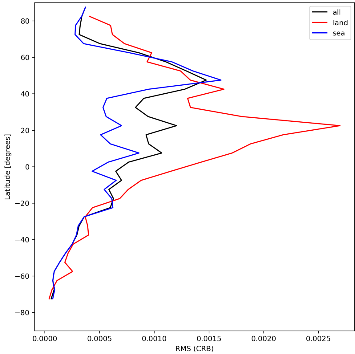
Figure 32: Zonal average of “RMS (CRB)” for 2023-08-05 to 2023-08-07.
