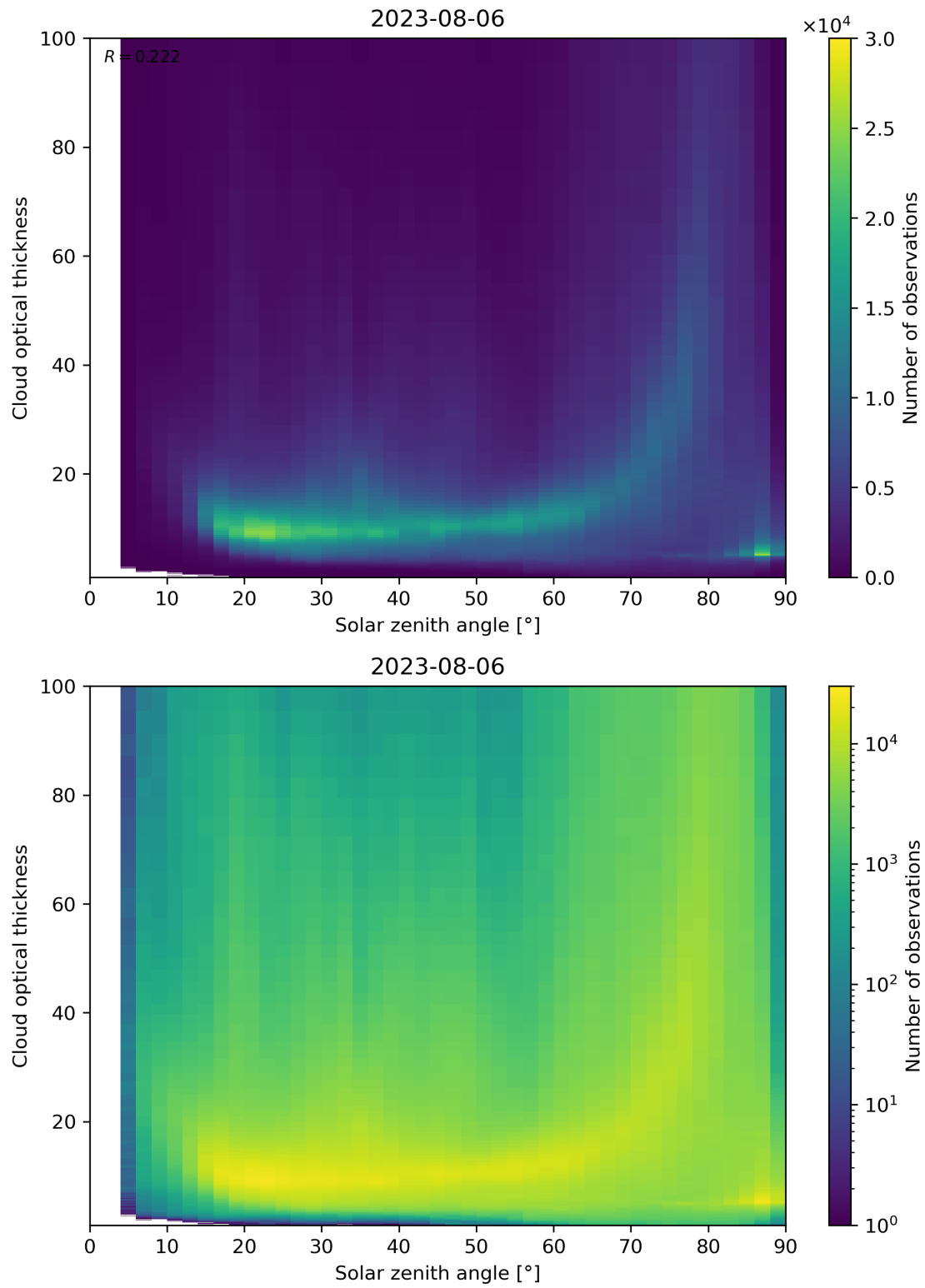
Figure 103: Scatter density plot of “Solar zenith angle” against “Cloud optical thickness” for 2023-08-05 to 2023-08-07.
