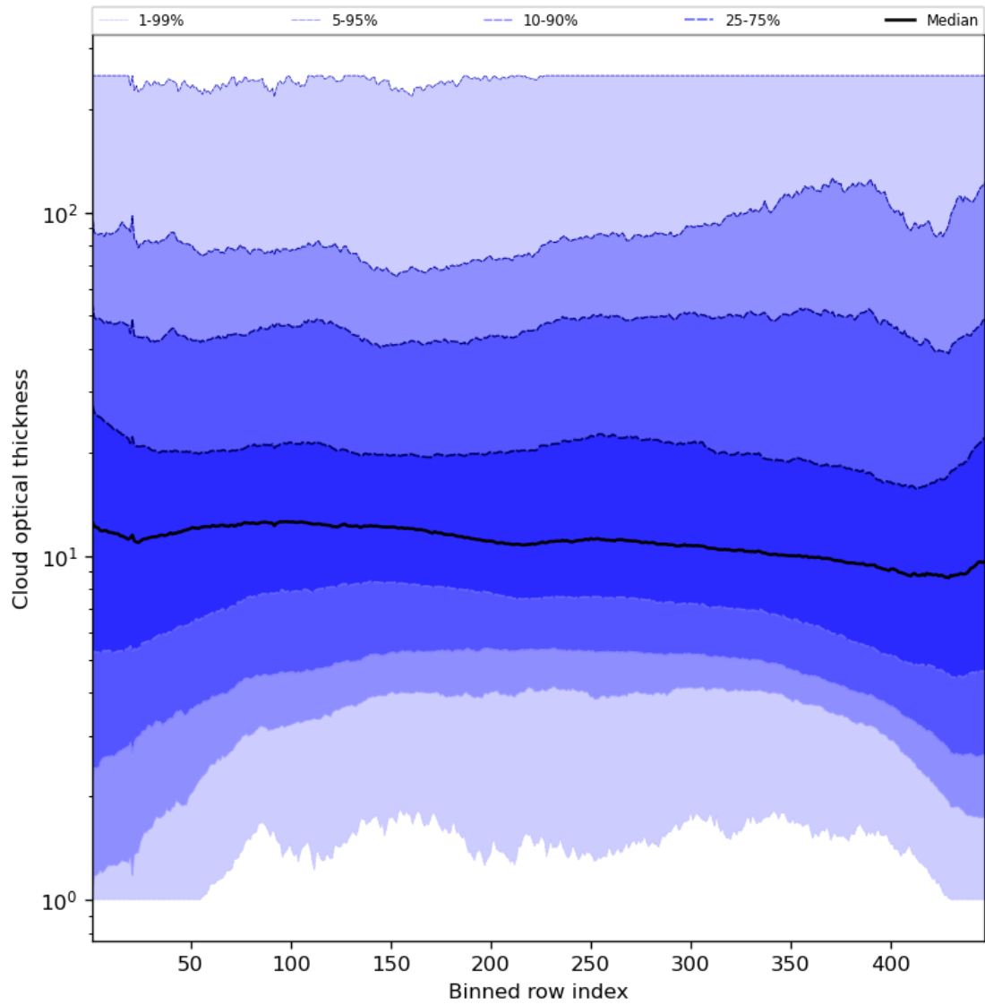
Figure 57: Along track statistics of “Cloud optical thickness” for 2023-08-05 to 2023-08-07
