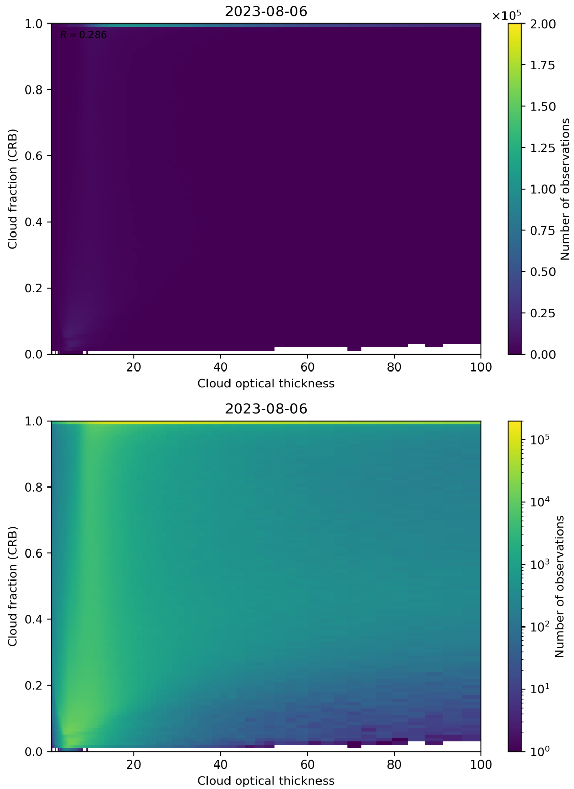
Figure 84: Scatter density plot of “Cloud optical thickness” against “Cloud fraction (CRB)” for 2023-08-05 to 2023-08-07.
