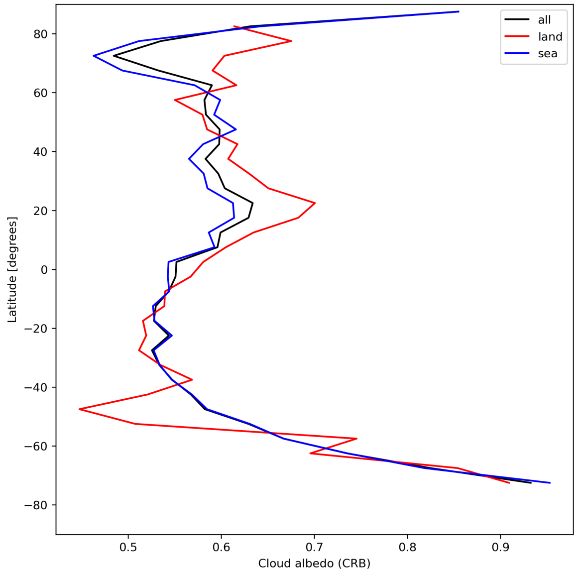
Figure 28: Zonal average of “Cloud albedo (CRB)” for 2023-08-05 to 2023-08-07.
