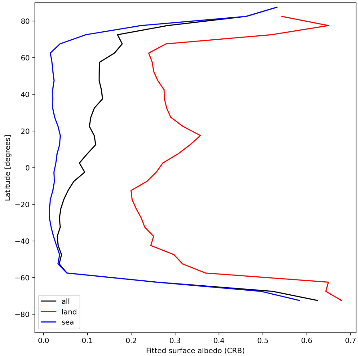
Figure 30: Zonal average of “Fitted surface albedo (CRB)” for 2023-08-05 to 2023-08-07.
