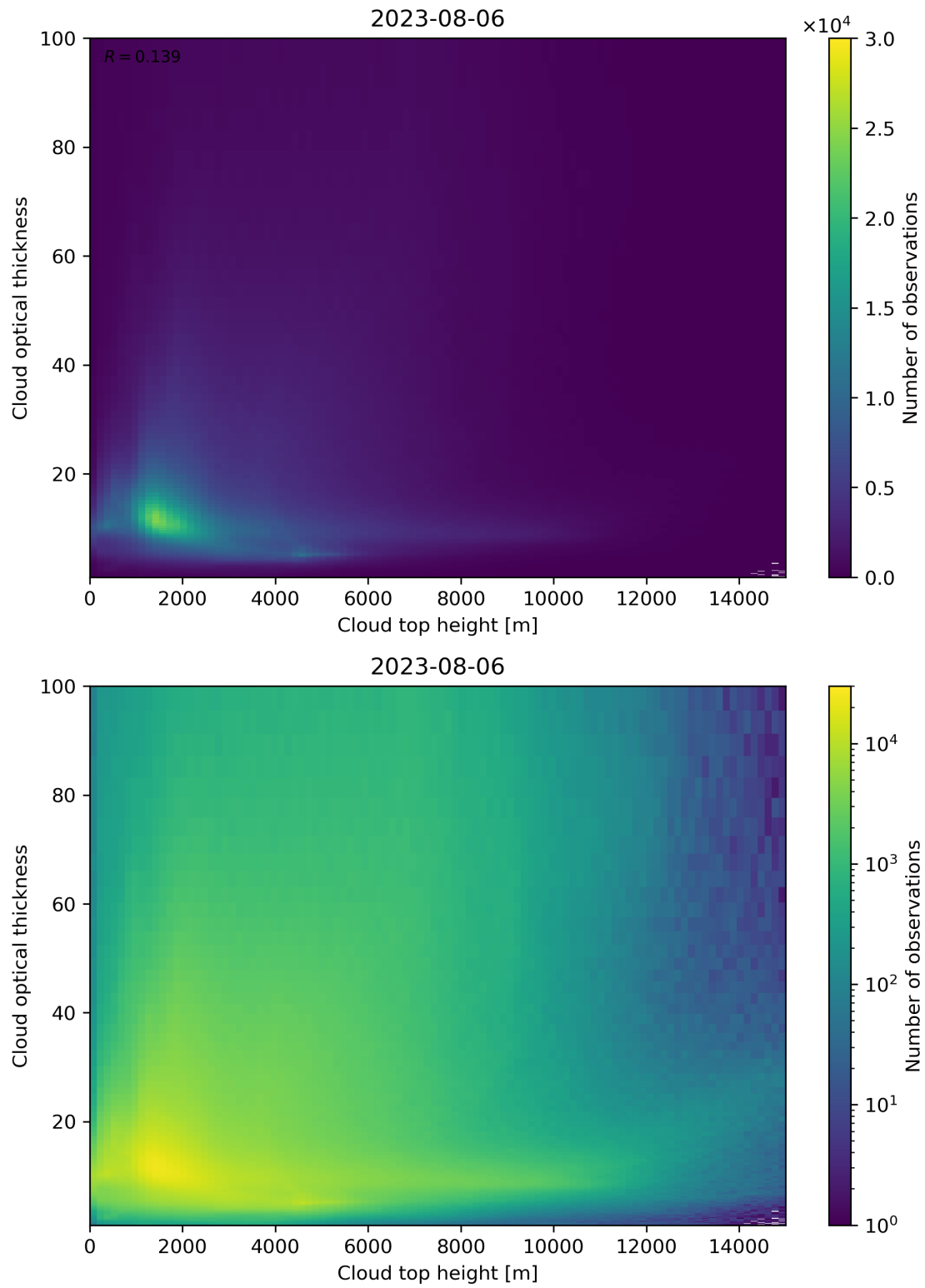
Figure 90: Scatter density plot of “Cloud top height” against “Cloud optical thickness” for 2023-08-05 to 2023-08-07.
