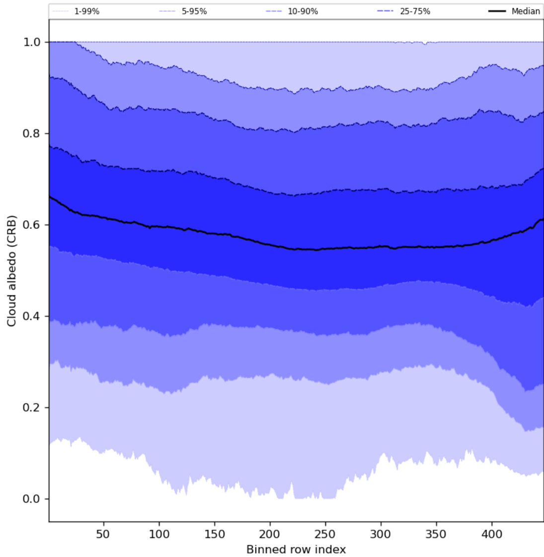
Figure 60: Along track statistics of “Cloud albedo (CRB)” for 2023-08-05 to 2023-08-07
