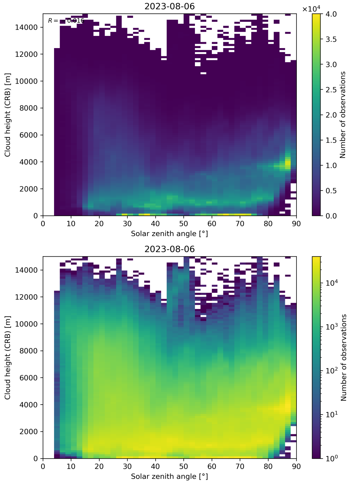
Figure 102: Scatter density plot of “Solar zenith angle” against “Cloud height (CRB)” for 2023-08-05 to 2023-08-07.
