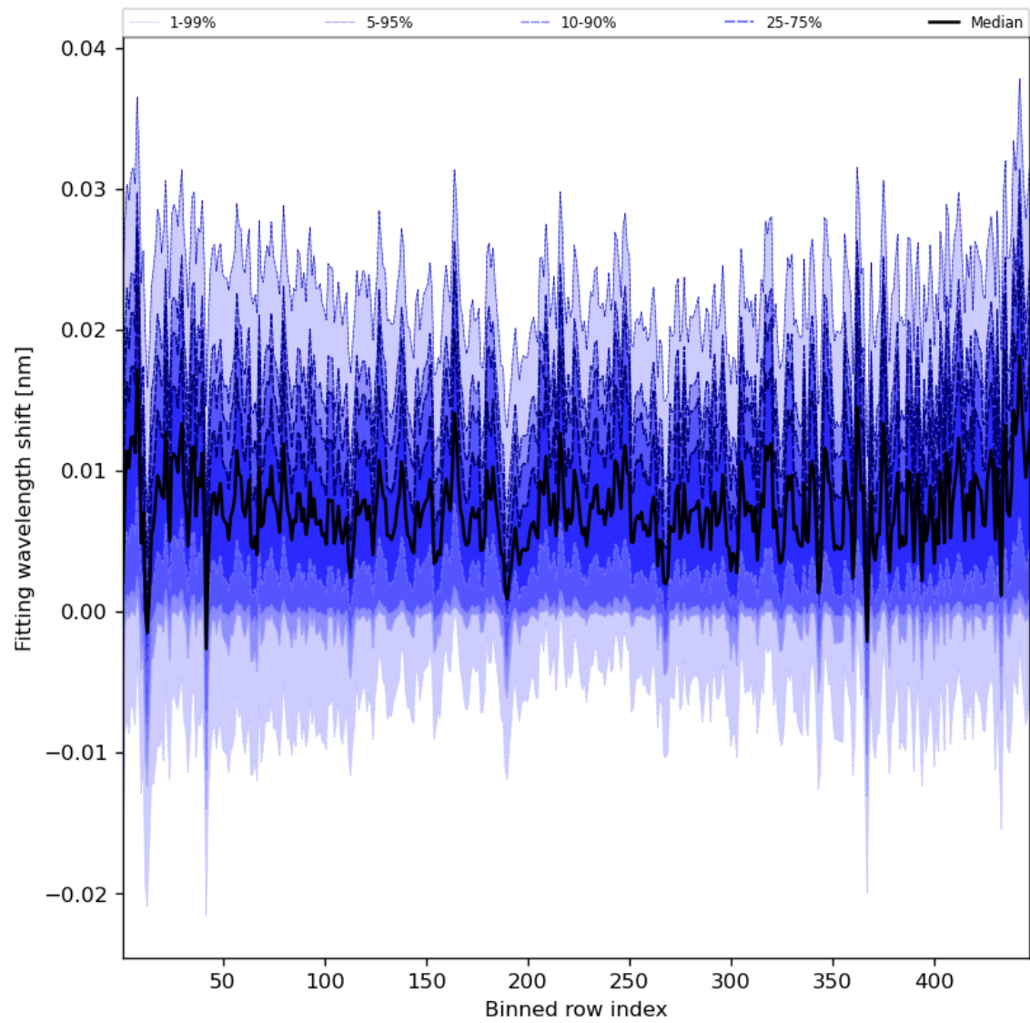
Figure 65: Along track statistics of “Fitting wavelength shift” for 2023-08-05 to 2023-08-07
