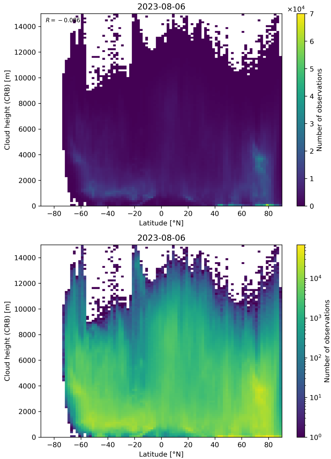
Figure 95: Scatter density plot of “Latitude” against “Cloud height (CRB)” for 2023-08-05 to 2023-08-07.
