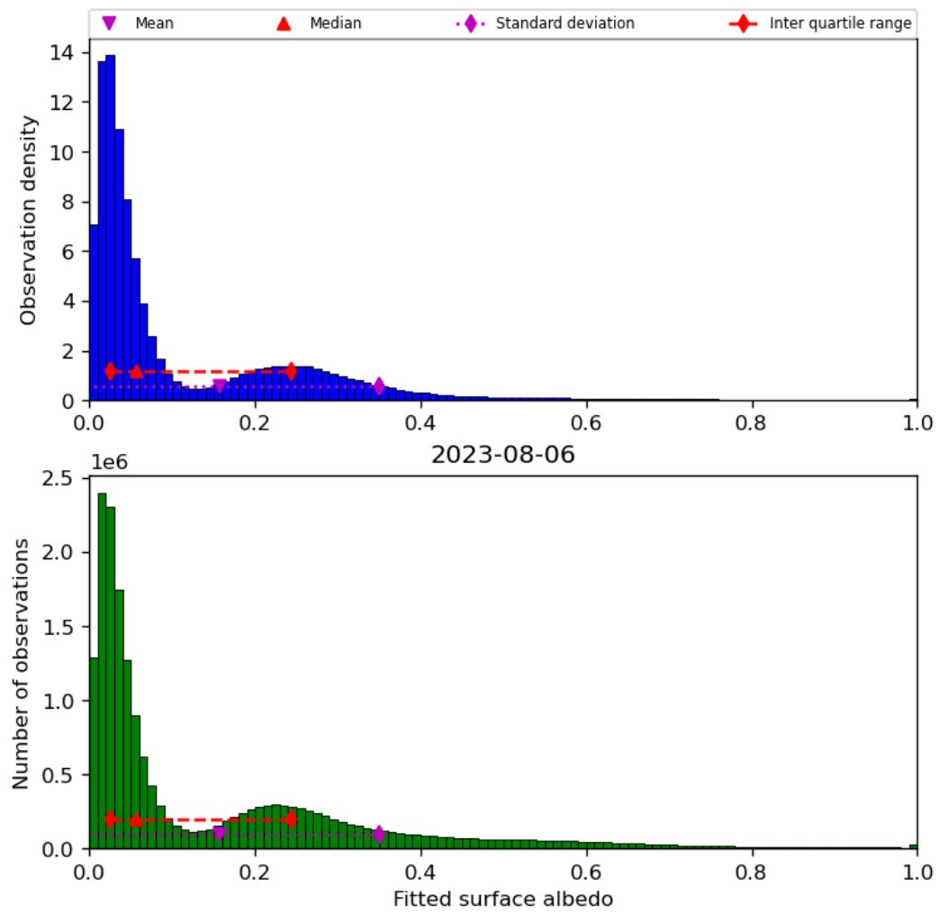
Figure 45: Histogram of “Fitted surface albedo” for 2023-08-05 to 2023-08-07
