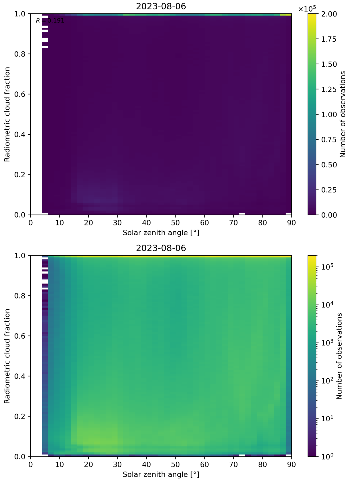
Figure 99: Scatter density plot of “Solar zenith angle” against “Radiometric cloud fraction” for 2023-08-05 to 2023-08-07.
