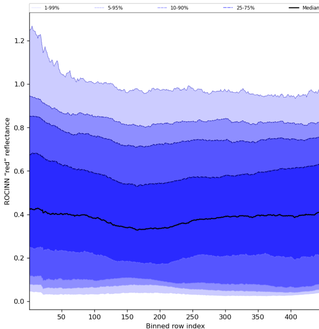
Figure 69: Along track statistics of “ROCINN “red” reflectance” for 2023-08-05 to 2023-08-07
