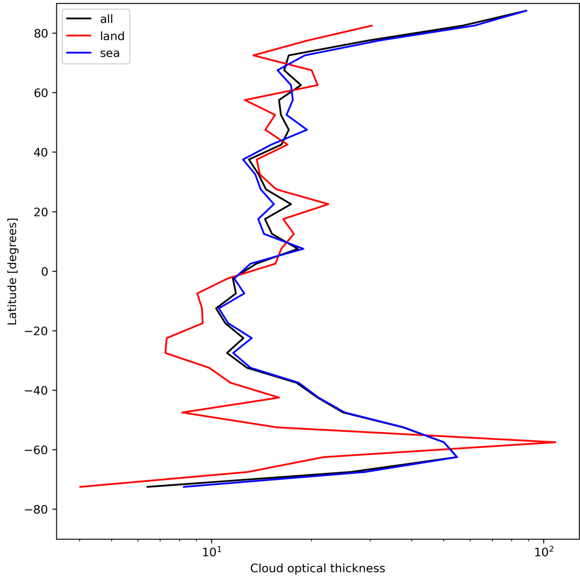
Figure 25: Zonal average of “Cloud optical thickness” for 2023-08-05 to 2023-08-07.
