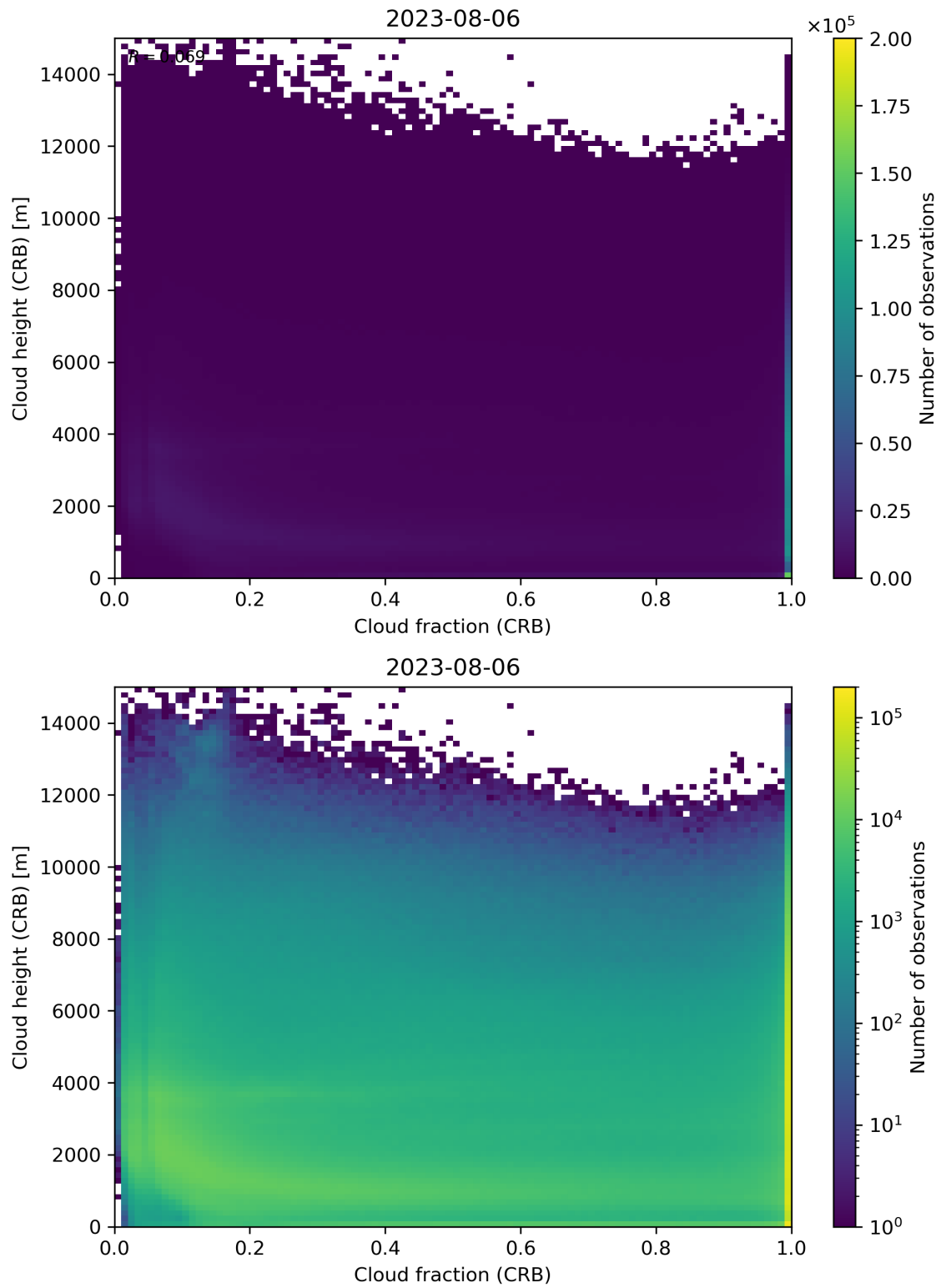
Figure 79: Scatter density plot of “Cloud fraction (CRB)” against “Cloud height (CRB)” for 2023-08-05 to 2023-08-07.
