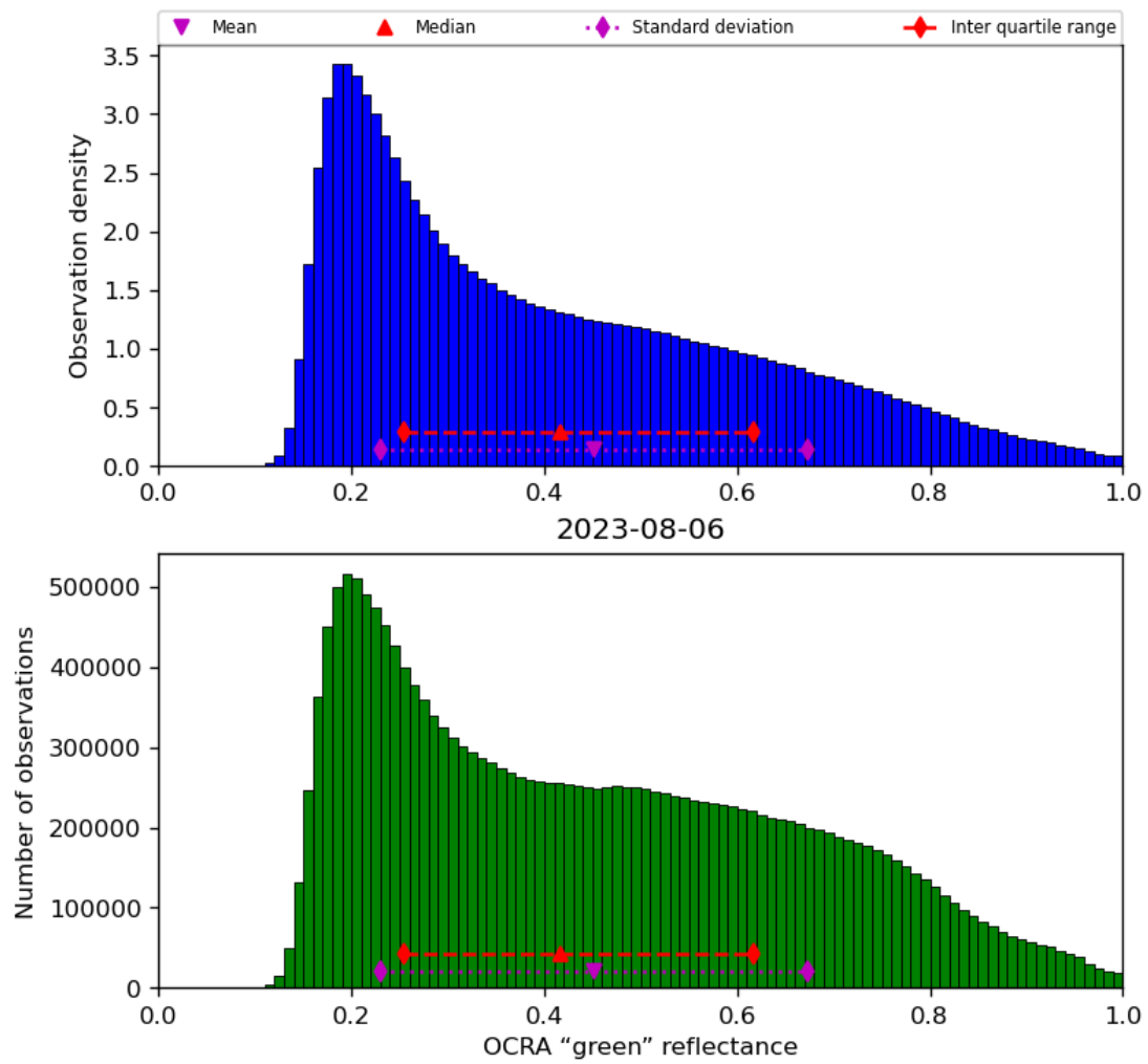
Figure 52: Histogram of “OCRA “green” reflectance” for 2023-08-05 to 2023-08-07
