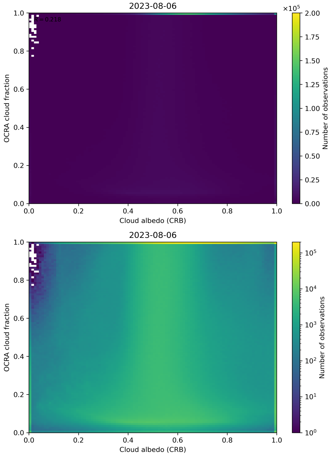
Figure 70: Scatter density plot of “Cloud albedo (CRB)” against “OCRA cloud fraction” for 2023-08-05 to 2023-08-07.
