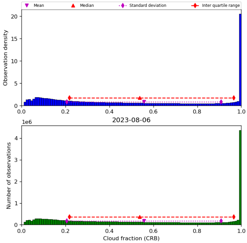
Figure 42: Histogram of “Cloud fraction (CRB)” for 2023-08-05 to 2023-08-07
