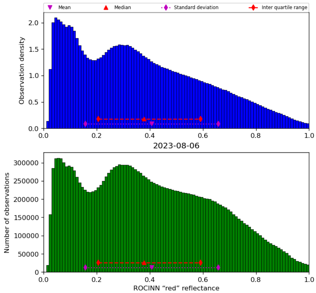
Figure 53: Histogram of “ROCINN “red” reflectance” for 2023-08-05 to 2023-08-07
