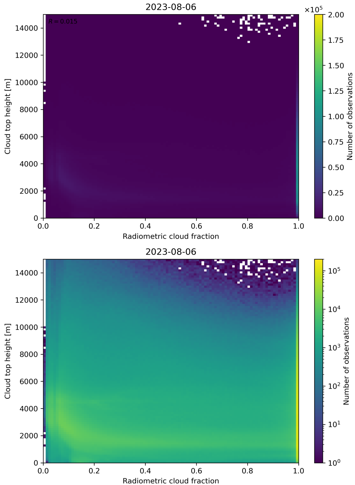
Figure 76: Scatter density plot of “Radiometric cloud fraction” against “Cloud top height” for 2023-08-05 to 2023-08-07.
