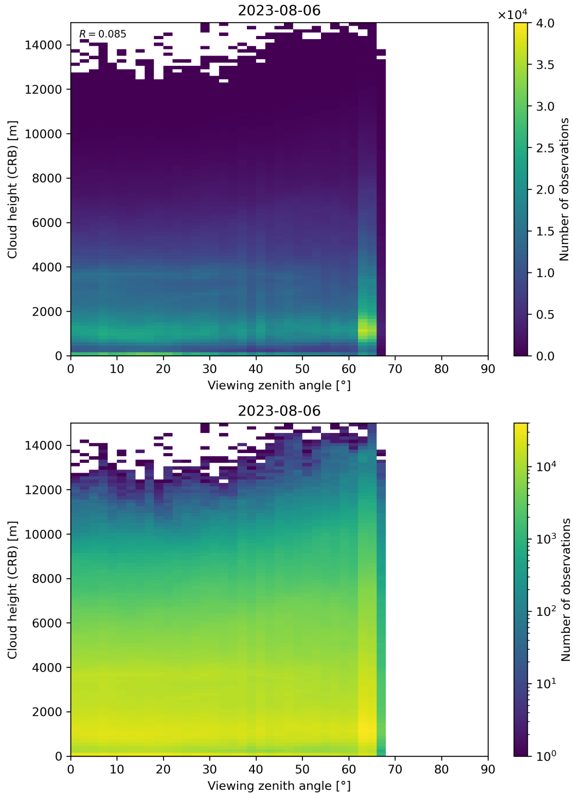
Figure 110: Scatter density plot of “Viewing zenith angle” against “Cloud height (CRB)” for 2023-08-05 to 2023-08-07.
