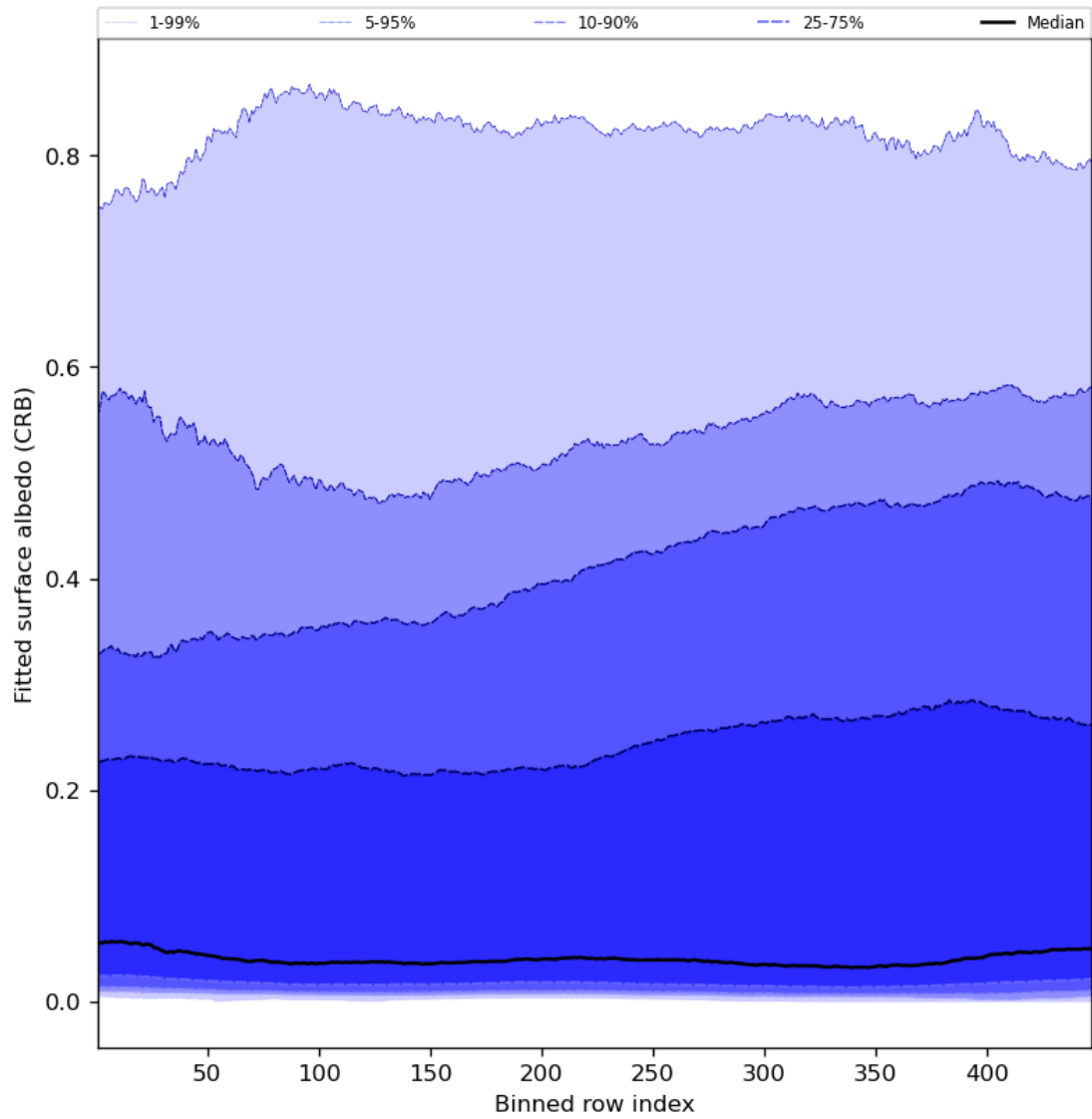
Figure 62: Along track statistics of “Fitted surface albedo (CRB)” for 2023-08-05 to 2023-08-07
