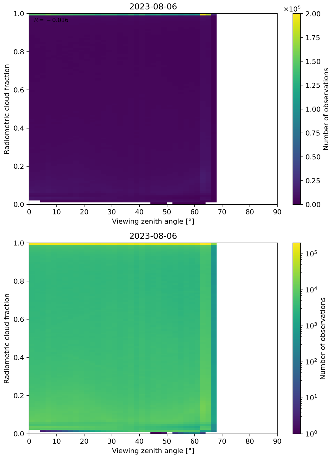
Figure 107: Scatter density plot of “Viewing zenith angle” against “Radiometric cloud fraction” for 2023-08-05 to 2023-08-07.
