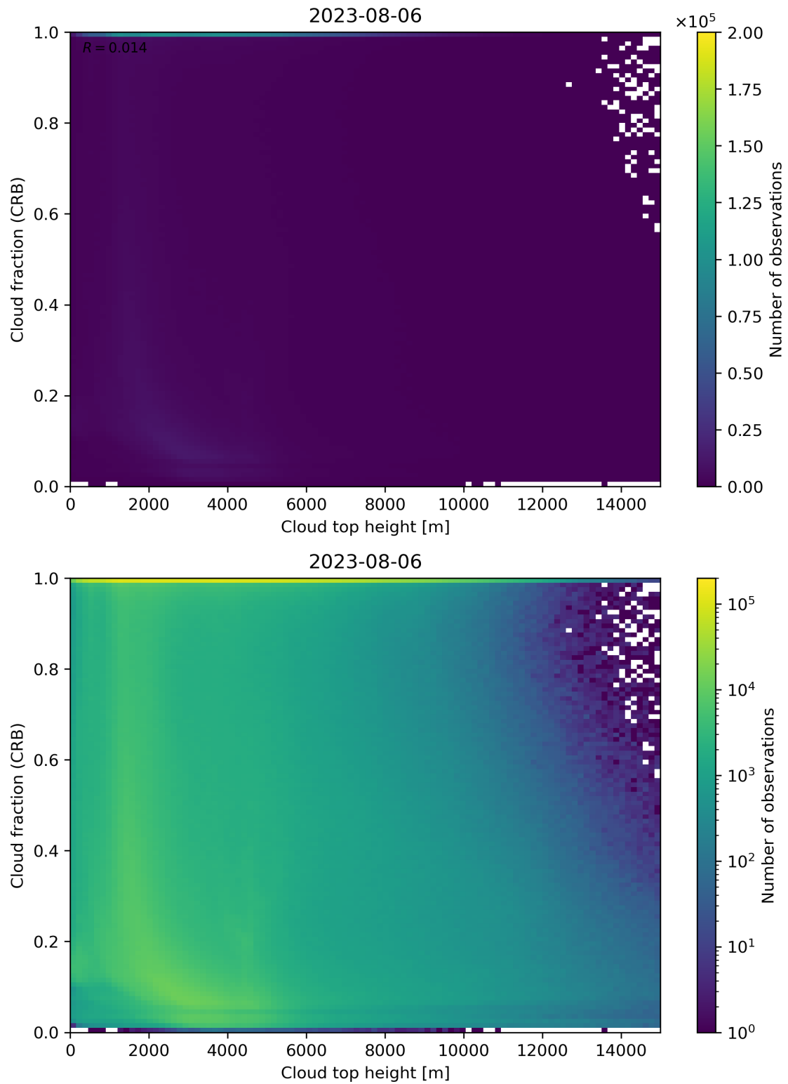
Figure 88: Scatter density plot of “Cloud top height” against “Cloud fraction (CRB)” for 2023-08-05 to 2023-08-07.
