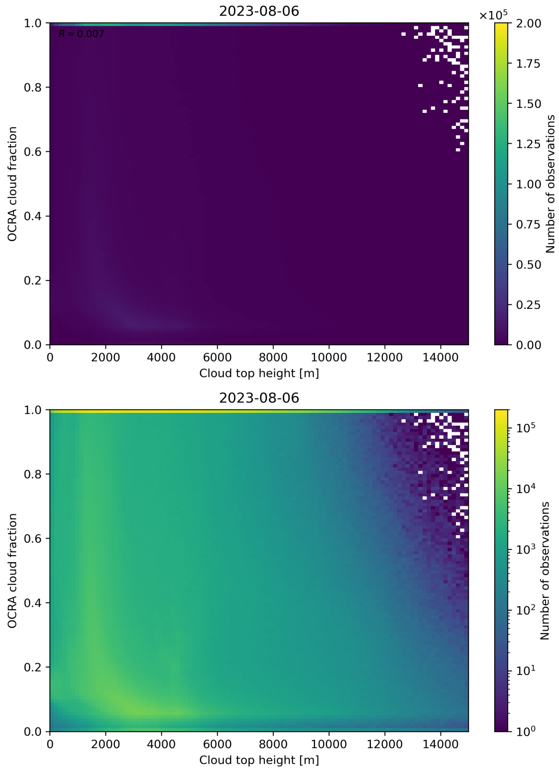
Figure 87: Scatter density plot of “Cloud top height” against “OCRA cloud fraction” for 2023-08-05 to 2023-08-07.
