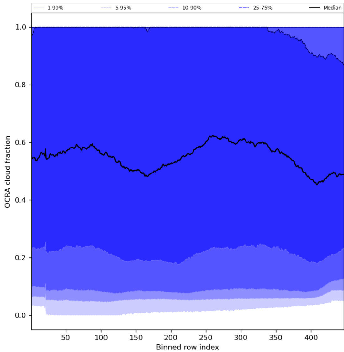
Figure 66: Along track statistics of “OCRA cloud fraction” for 2023-08-05 to 2023-08-07
