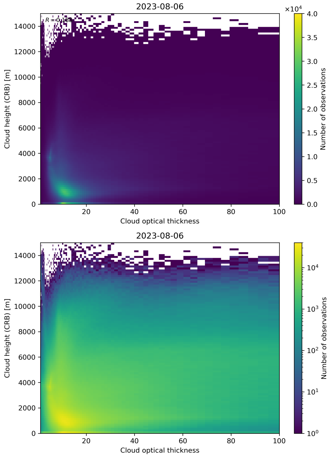
Figure 85: Scatter density plot of “Cloud optical thickness” against “Cloud height (CRB)” for 2023-08-05 to 2023-08-07.
