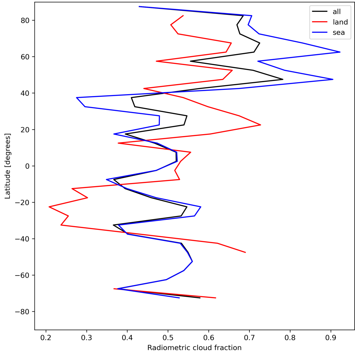
Figure 23: Zonal average of “Radiometric cloud fraction” for 2023-08-09 to 2023-08-10.
