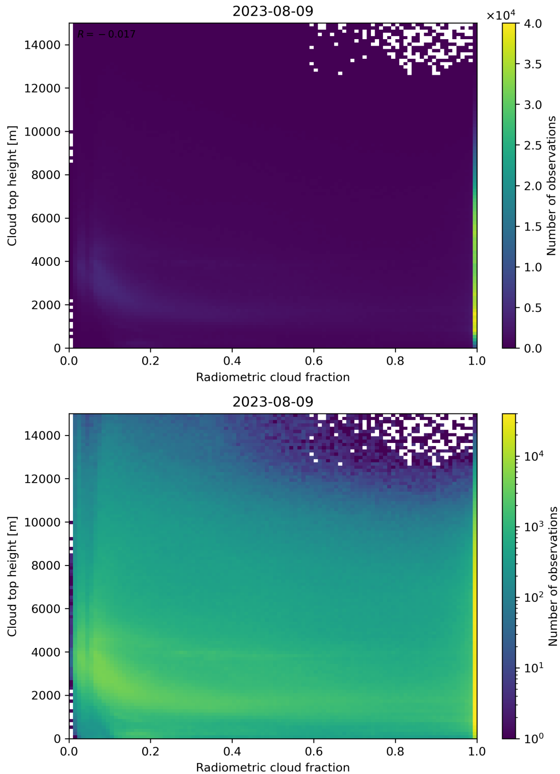
Figure 76: Scatter density plot of “Radiometric cloud fraction” against “Cloud top height” for 2023-08-09 to 2023-08-10.
