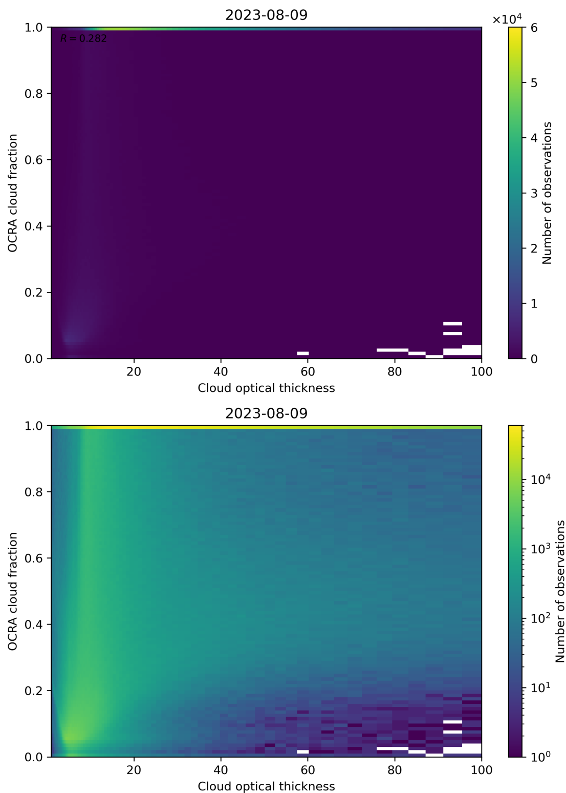
Figure 83: Scatter density plot of “Cloud optical thickness” against “OCRA cloud fraction” for 2023-08-09 to 2023-08-10.
