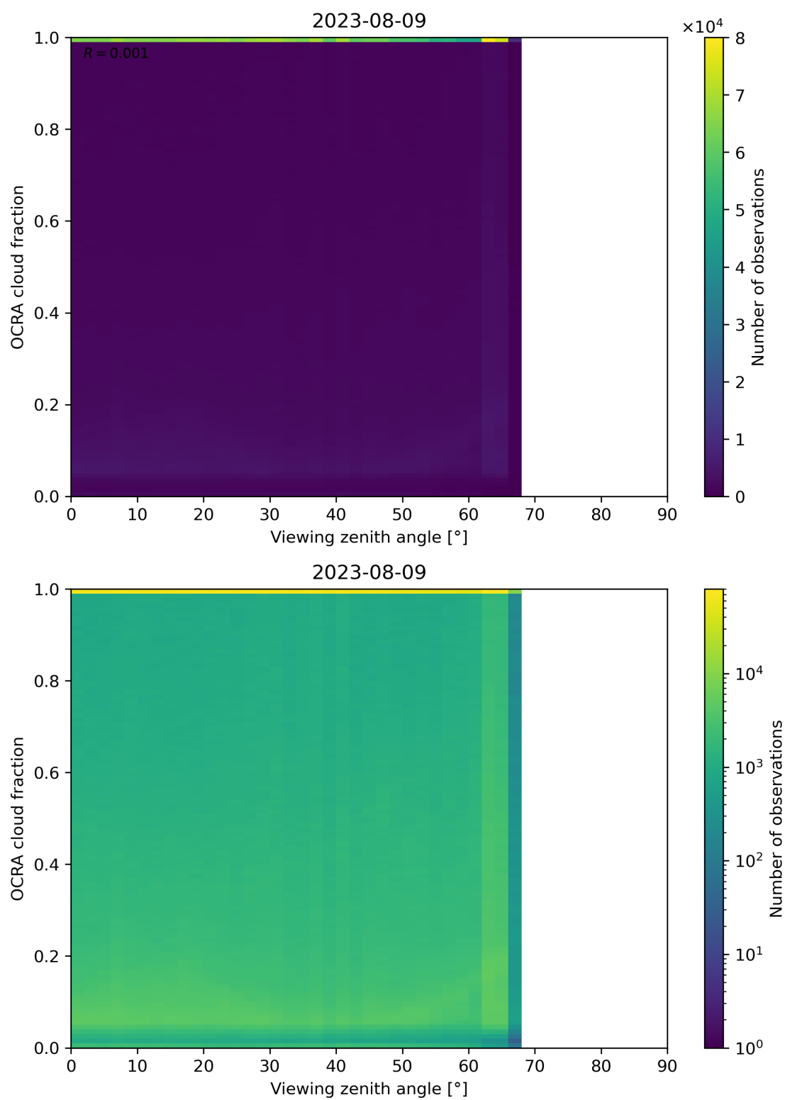
Figure 108: Scatter density plot of “Viewing zenith angle” against “OCRA cloud fraction” for 2023-08-09 to 2023-08-10.
