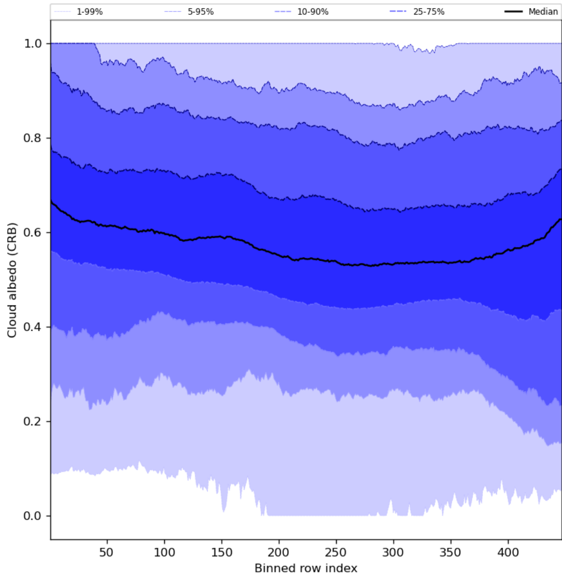
Figure 60: Along track statistics of “Cloud albedo (CRB)” for 2023-08-09 to 2023-08-10
