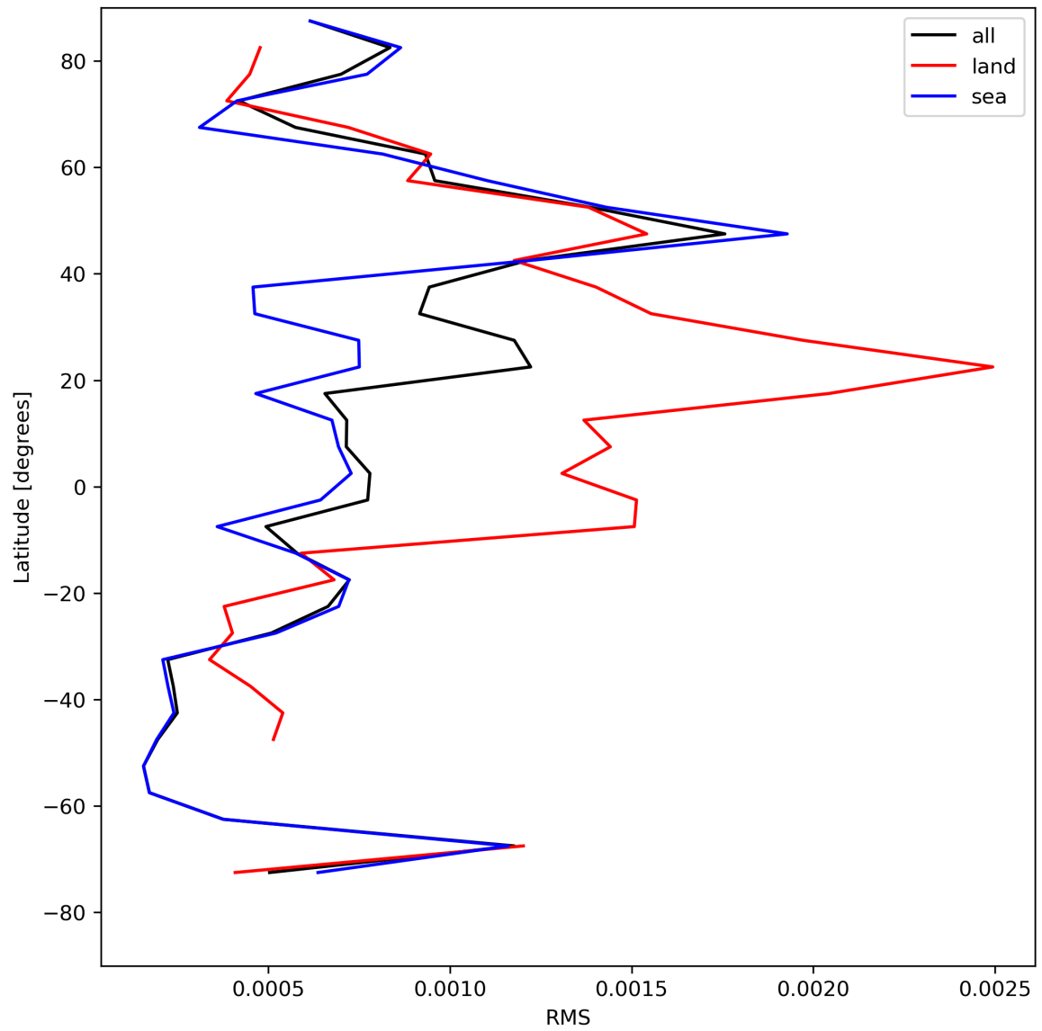
Figure 31: Zonal average of “RMS” for 2023-08-09 to 2023-08-10.
