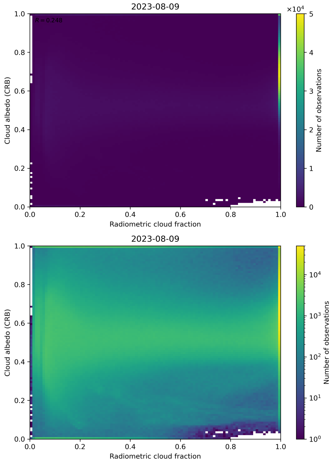
Figure 71: Scatter density plot of “Radiometric cloud fraction” against “Cloud albedo (CRB)” for 2023-08-09 to 2023-08-10.
