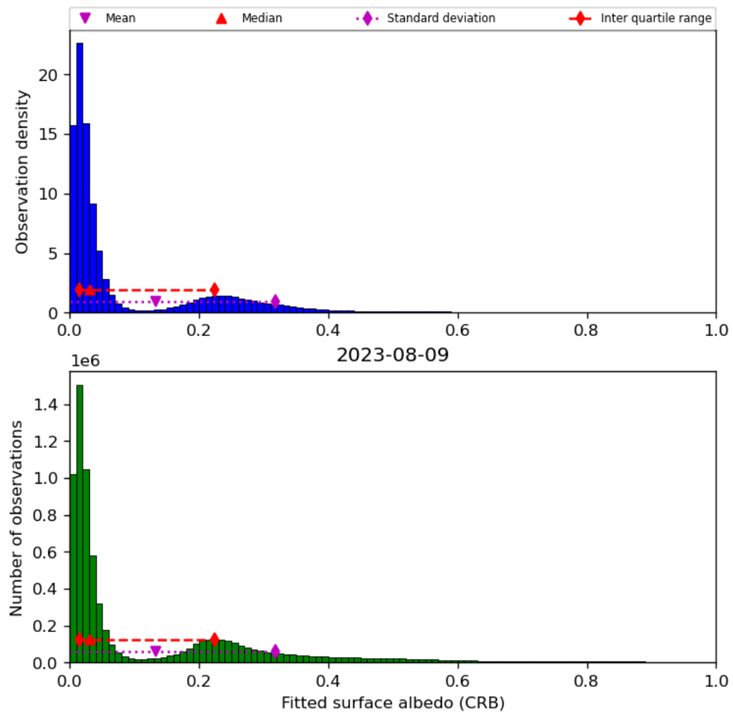
Figure 46: Histogram of “Fitted surface albedo (CRB)” for 2023-08-09 to 2023-08-10
