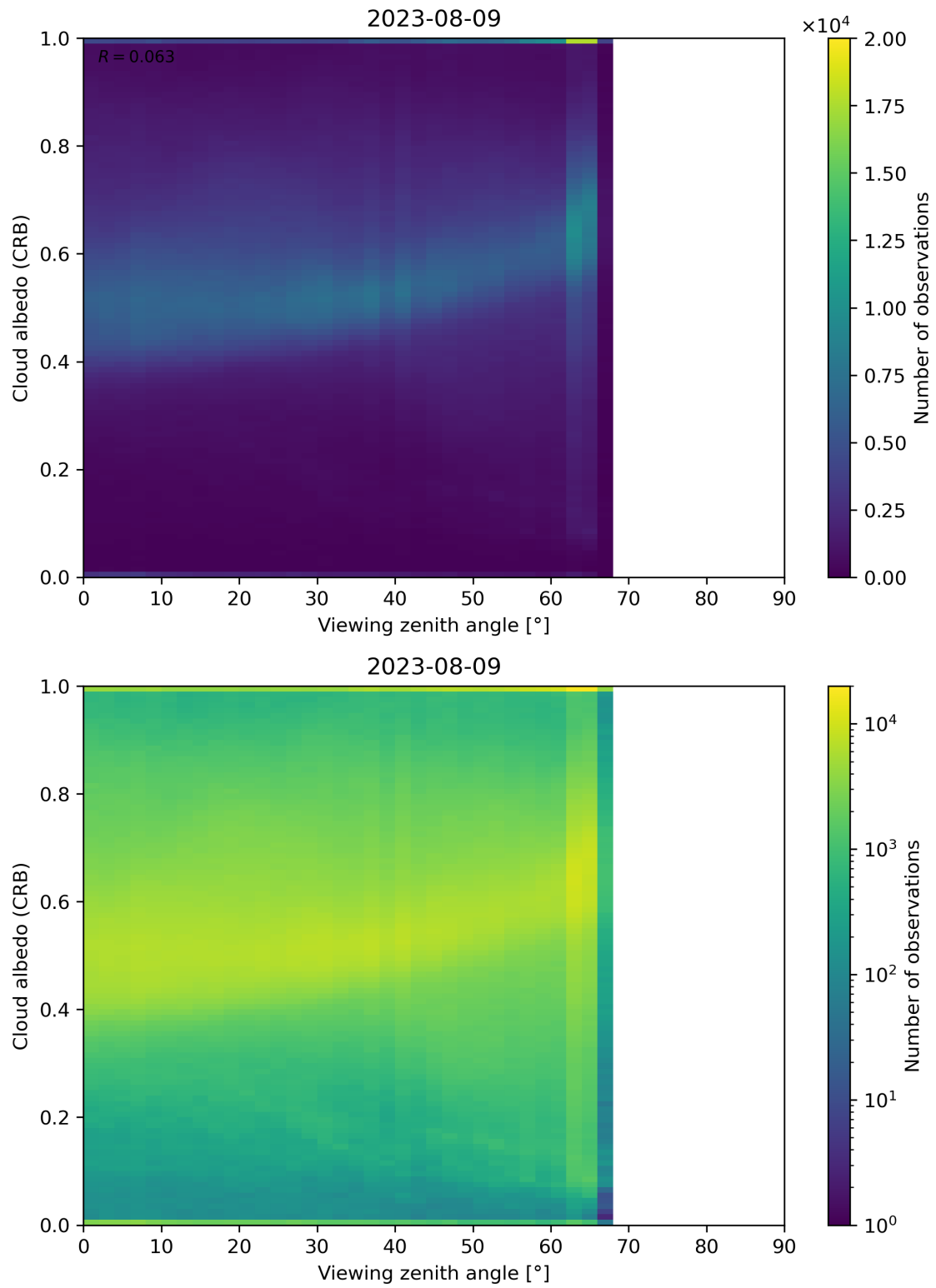
Figure 106: Scatter density plot of “Viewing zenith angle” against “Cloud albedo (CRB)” for 2023-08-09 to 2023-08-10.
