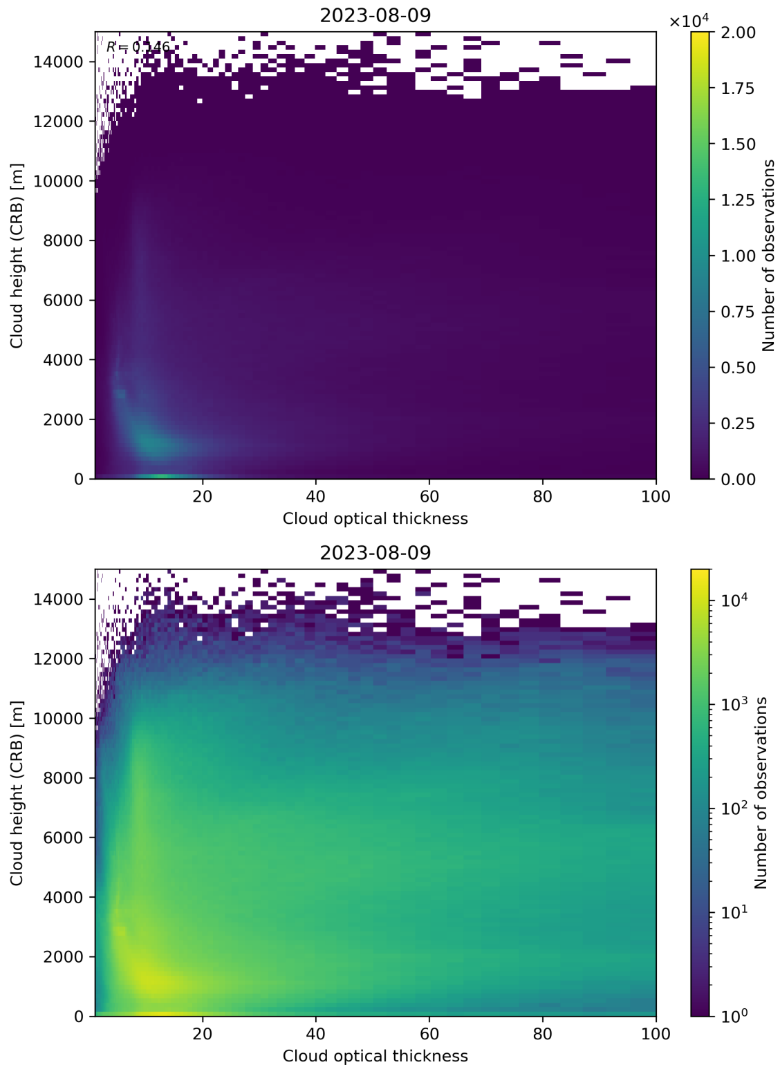
Figure 85: Scatter density plot of “Cloud optical thickness” against “Cloud height (CRB)” for 2023-08-09 to 2023-08-10.
