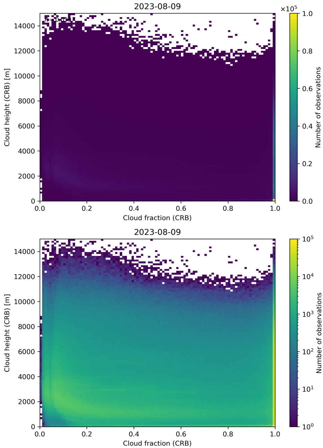
Figure 79: Scatter density plot of “Cloud fraction (CRB)” against “Cloud height (CRB)” for 2023-08-09 to 2023-08-10.
