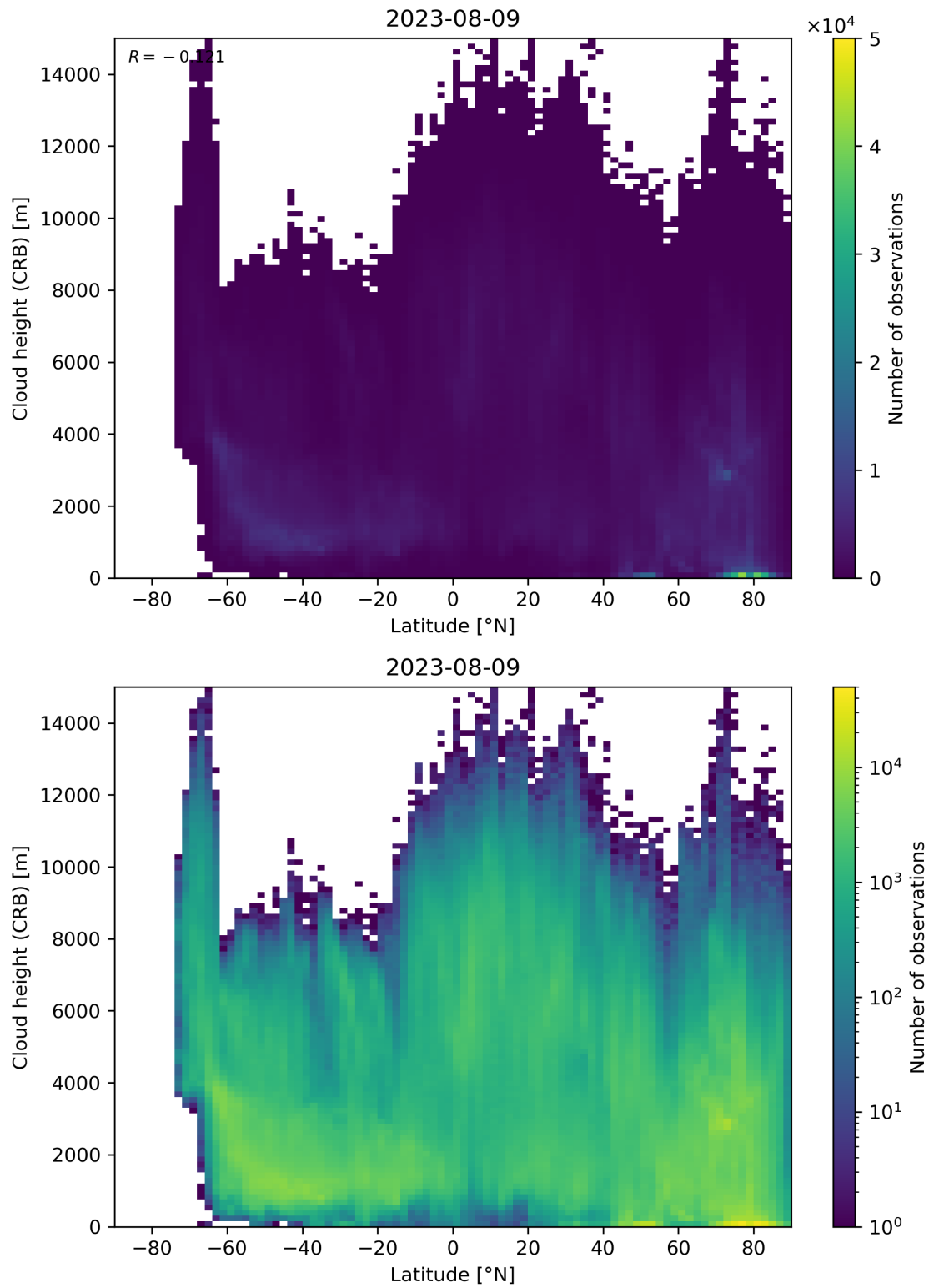
Figure 95: Scatter density plot of “Latitude” against “Cloud height (CRB)” for 2023-08-09 to 2023-08-10.
