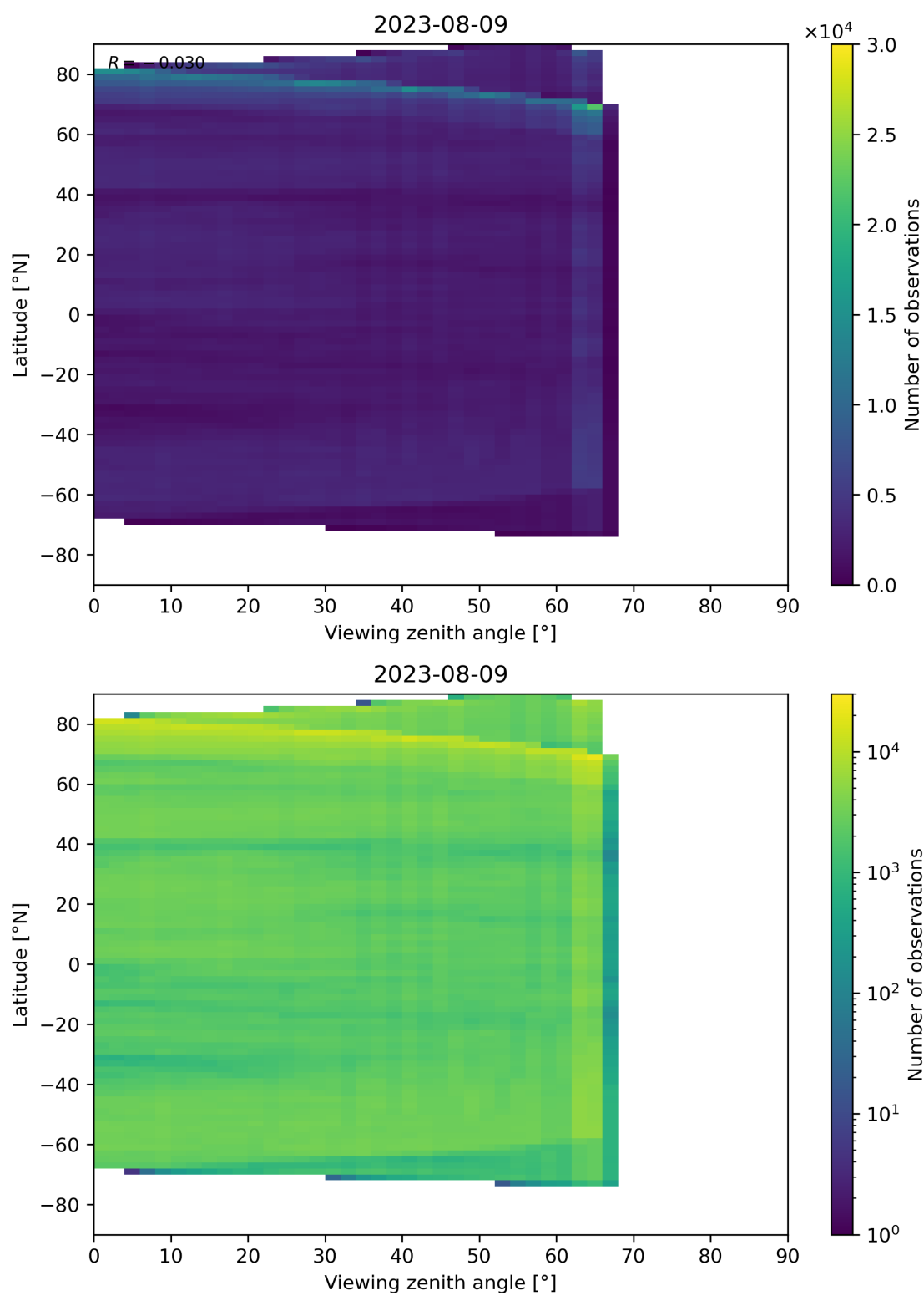
Figure 113: Scatter density plot of “Viewing zenith angle” against “Latitude” for 2023-08-09 to 2023-08-10.
