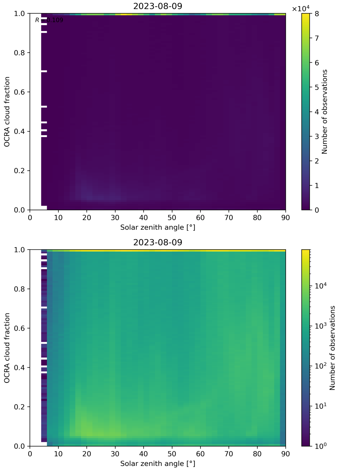
Figure 100: Scatter density plot of “Solar zenith angle” against “OCRA cloud fraction” for 2023-08-09 to 2023-08-10.
