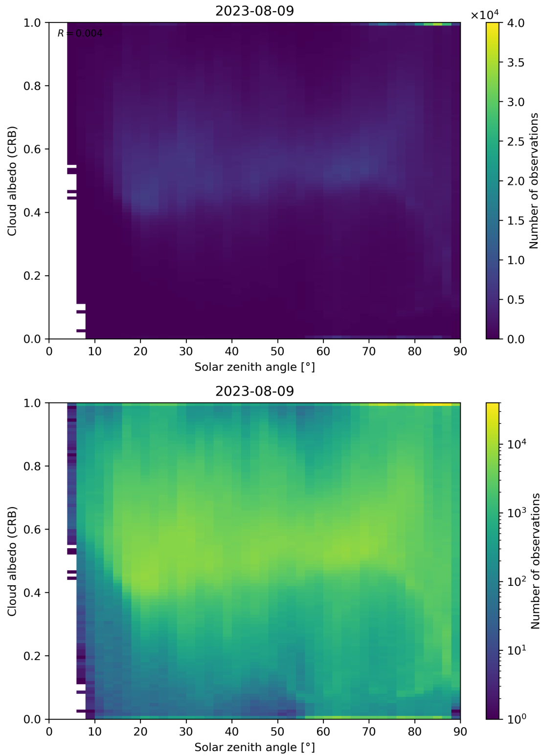
Figure 98: Scatter density plot of “Solar zenith angle” against “Cloud albedo (CRB)” for 2023-08-09 to 2023-08-10.
