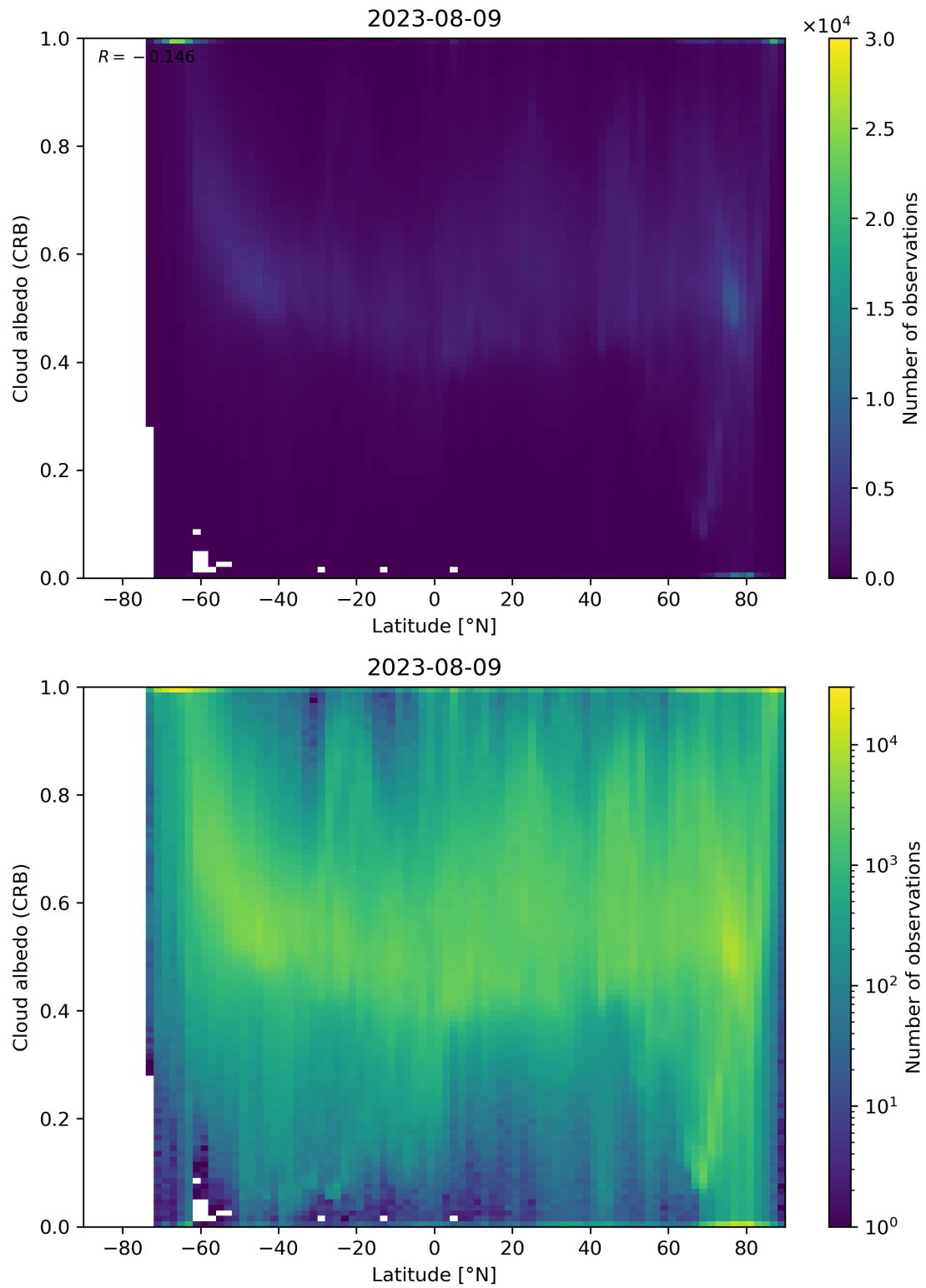
Figure 91: Scatter density plot of “Latitude” against “Cloud albedo (CRB)” for 2023-08-09 to 2023-08-10.
