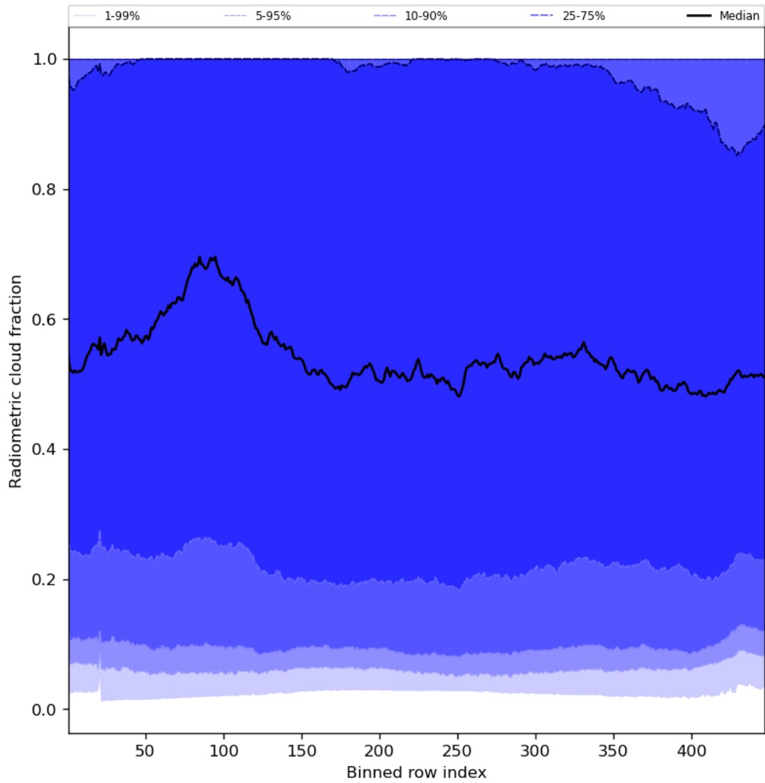
Figure 55: Along track statistics of “Radiometric cloud fraction” for 2023-08-09 to 2023-08-10
