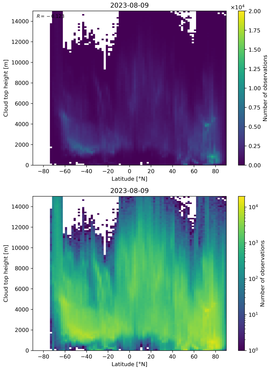
Figure 97: Scatter density plot of “Latitude” against “Cloud top height” for 2023-08-09 to 2023-08-10.
