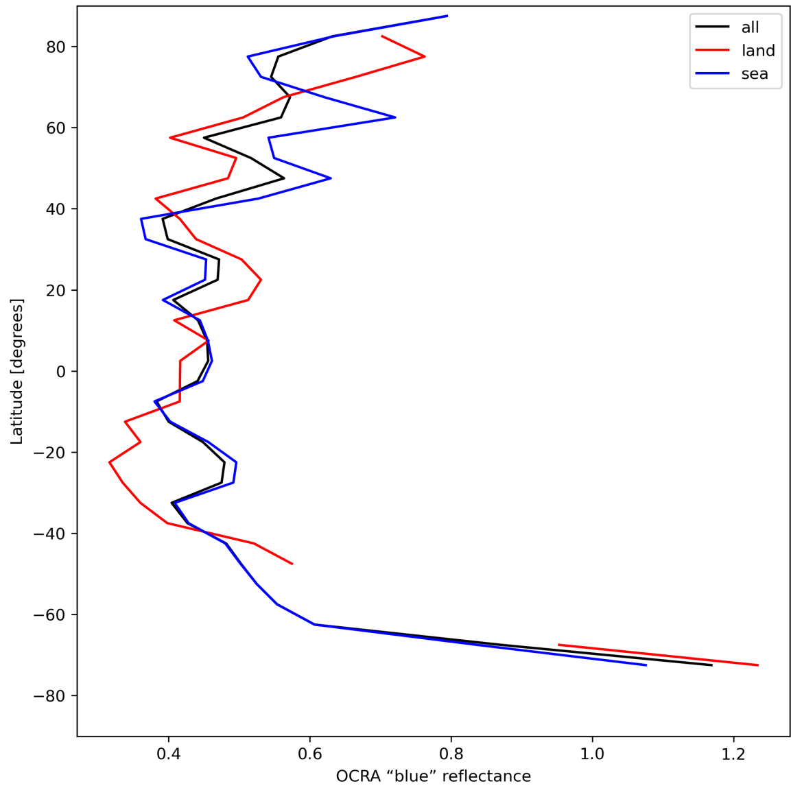
Figure 35: Zonal average of “OCRA “blue” reflectance” for 2023-08-09 to 2023-08-10.
