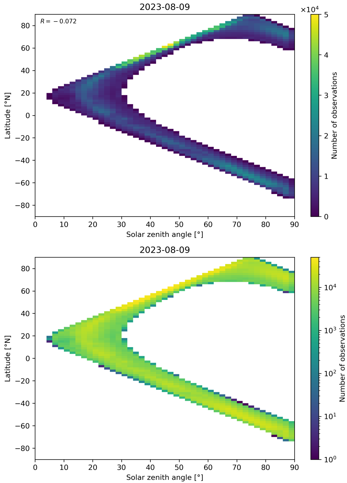
Figure 105: Scatter density plot of “Solar zenith angle” against “Latitude” for 2023-08-09 to 2023-08-10.
