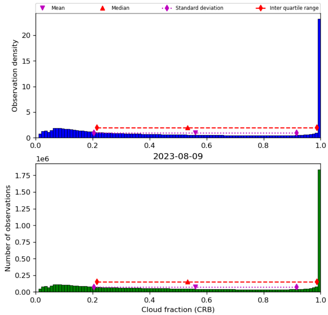
Figure 42: Histogram of “Cloud fraction (CRB)” for 2023-08-09 to 2023-08-10
