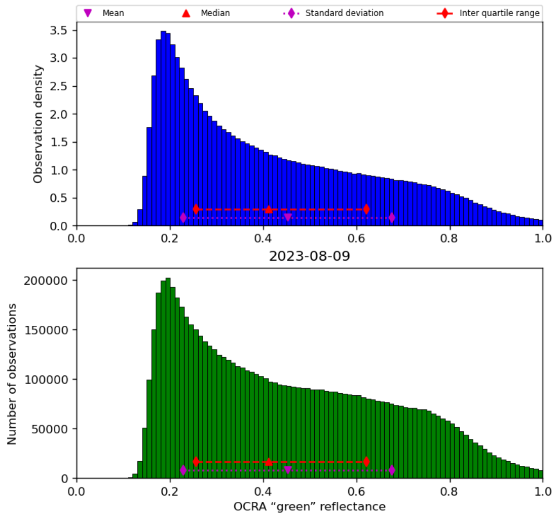
Figure 52: Histogram of “OCRA “green” reflectance” for 2023-08-09 to 2023-08-10
