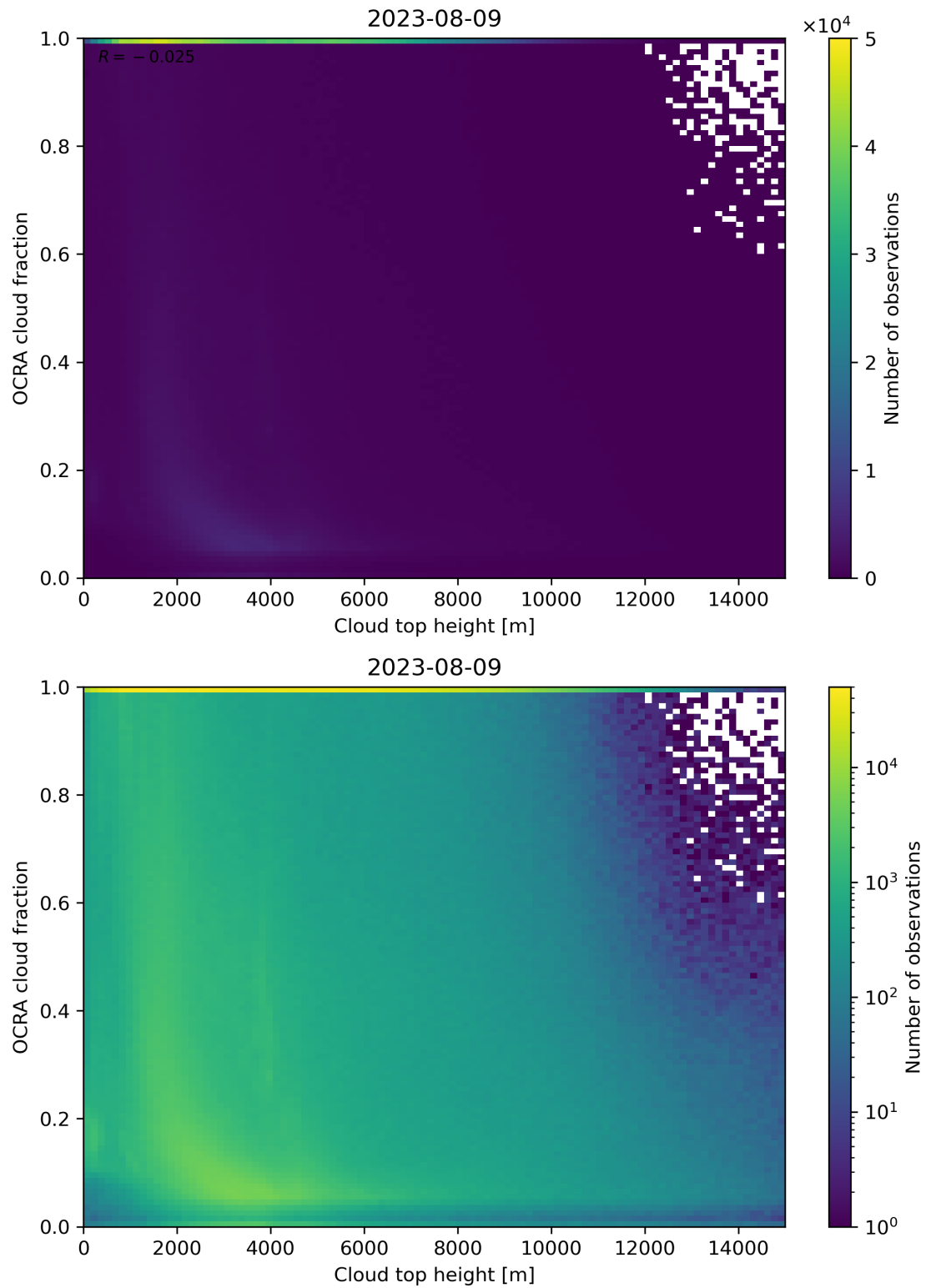
Figure 87: Scatter density plot of “Cloud top height” against “OCRA cloud fraction” for 2023-08-09 to 2023-08-10.
