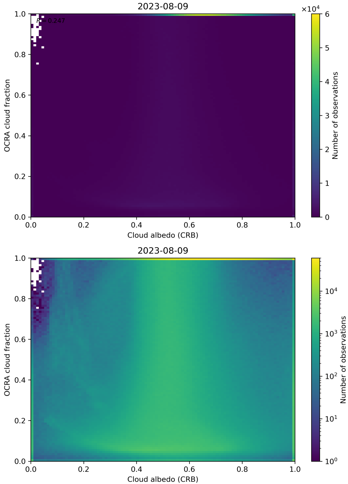
Figure 70: Scatter density plot of “Cloud albedo (CRB)” against “OCRA cloud fraction” for 2023-08-09 to 2023-08-10.
