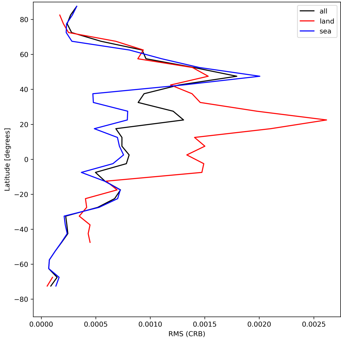
Figure 32: Zonal average of “RMS (CRB)” for 2023-08-09 to 2023-08-10.
