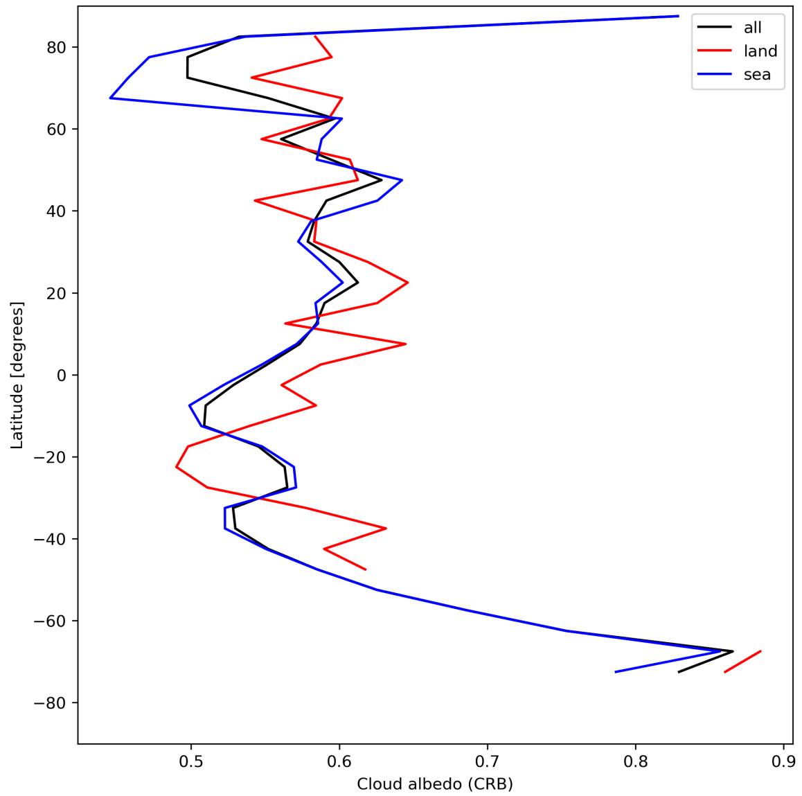
Figure 28: Zonal average of “Cloud albedo (CRB)” for 2023-08-09 to 2023-08-10.
