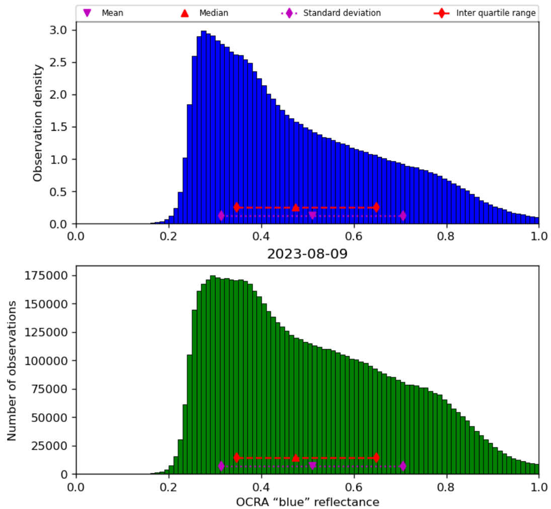
Figure 51: Histogram of “OCRA “blue” reflectance” for 2023-08-09 to 2023-08-10
