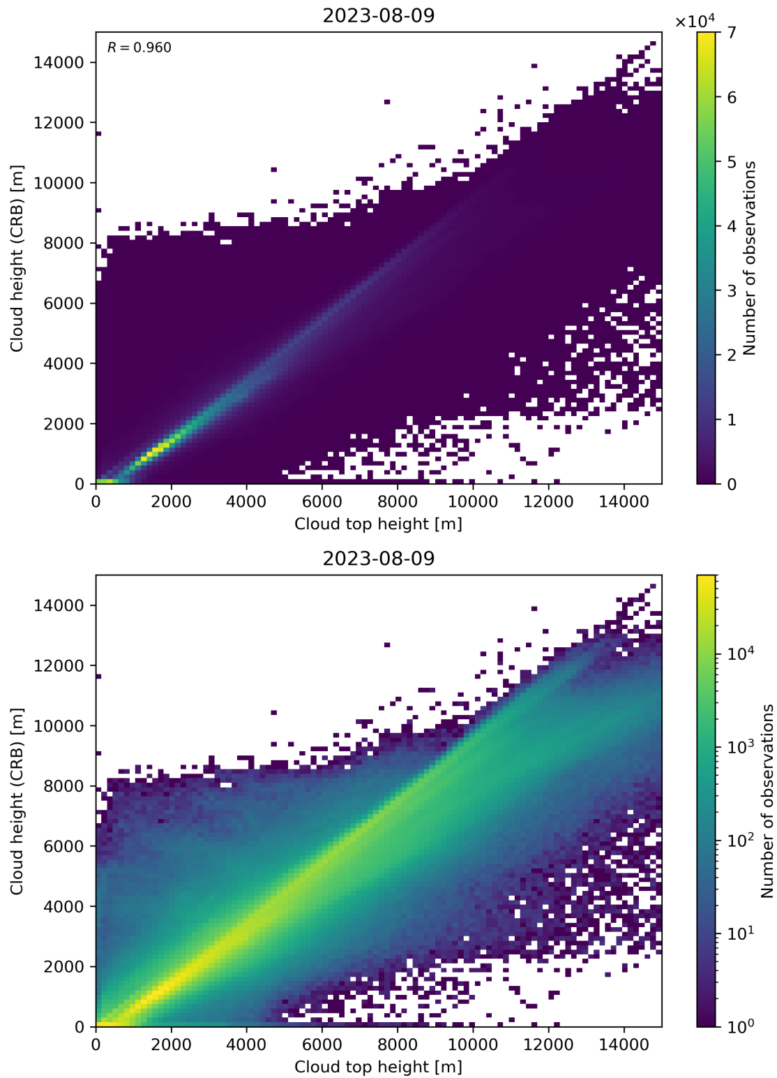
Figure 89: Scatter density plot of “Cloud top height” against “Cloud height (CRB)” for 2023-08-09 to 2023-08-10.
