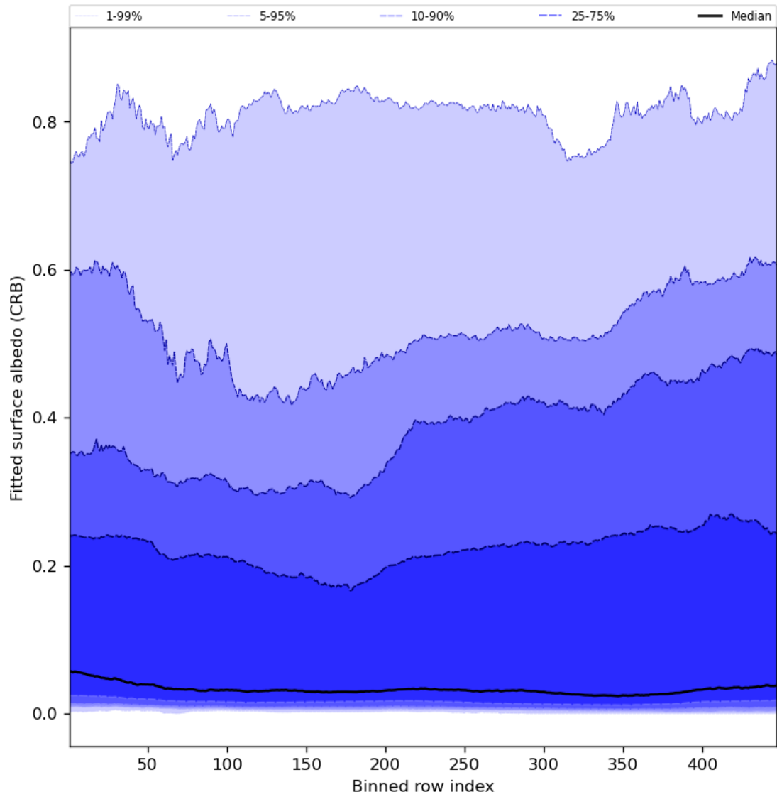
Figure 62: Along track statistics of “Fitted surface albedo (CRB)” for 2023-08-09 to 2023-08-10
