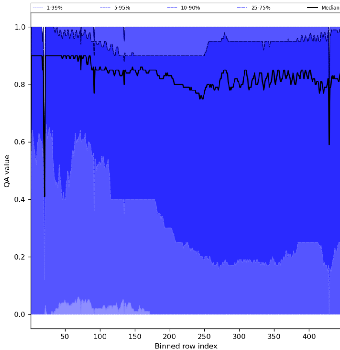
Figure 54: Along track statistics of “QA value” for 2023-08-09 to 2023-08-10
