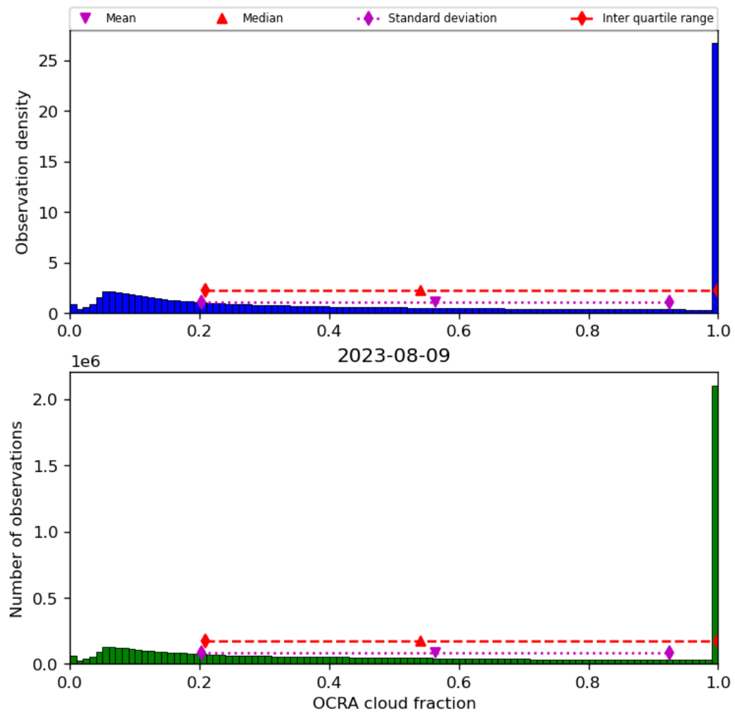
Figure 50: Histogram of “OCRA cloud fraction” for 2023-08-09 to 2023-08-10
