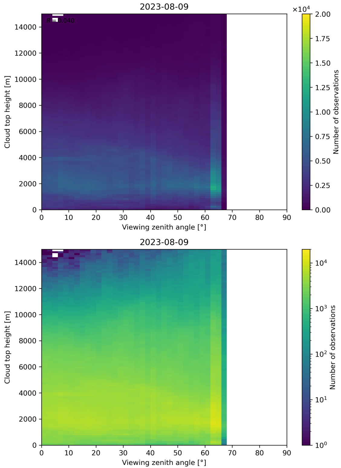
Figure 112: Scatter density plot of “Viewing zenith angle” against “Cloud top height” for 2023-08-09 to 2023-08-10.
