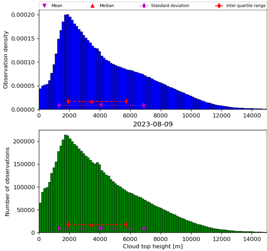
Figure 40: Histogram of “Cloud top height” for 2023-08-09 to 2023-08-10
