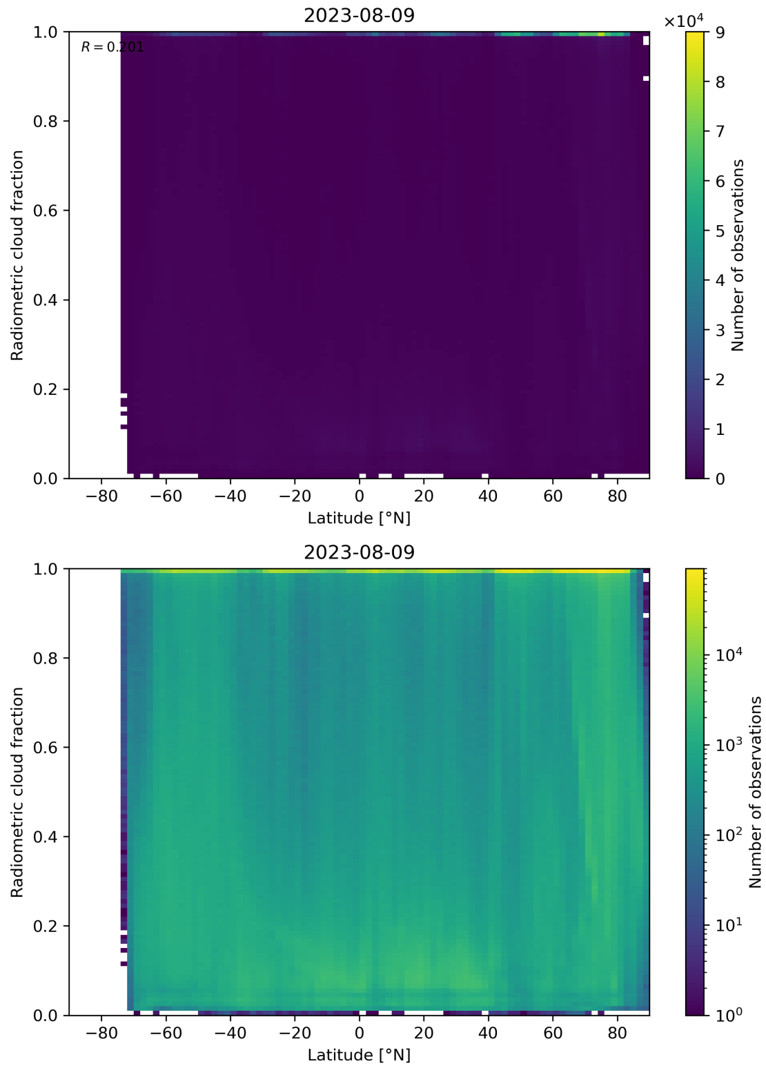
Figure 92: Scatter density plot of “Latitude” against “Radiometric cloud fraction” for 2023-08-09 to 2023-08-10.
