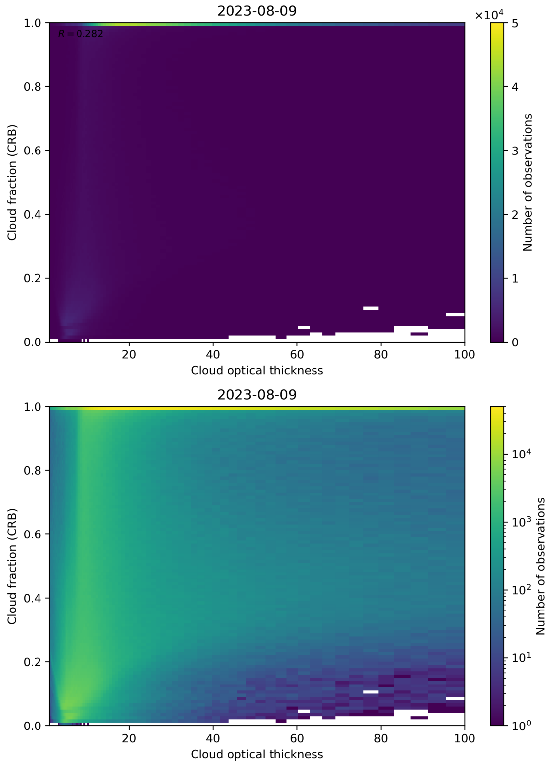
Figure 84: Scatter density plot of “Cloud optical thickness” against “Cloud fraction (CRB)” for 2023-08-09 to 2023-08-10.
