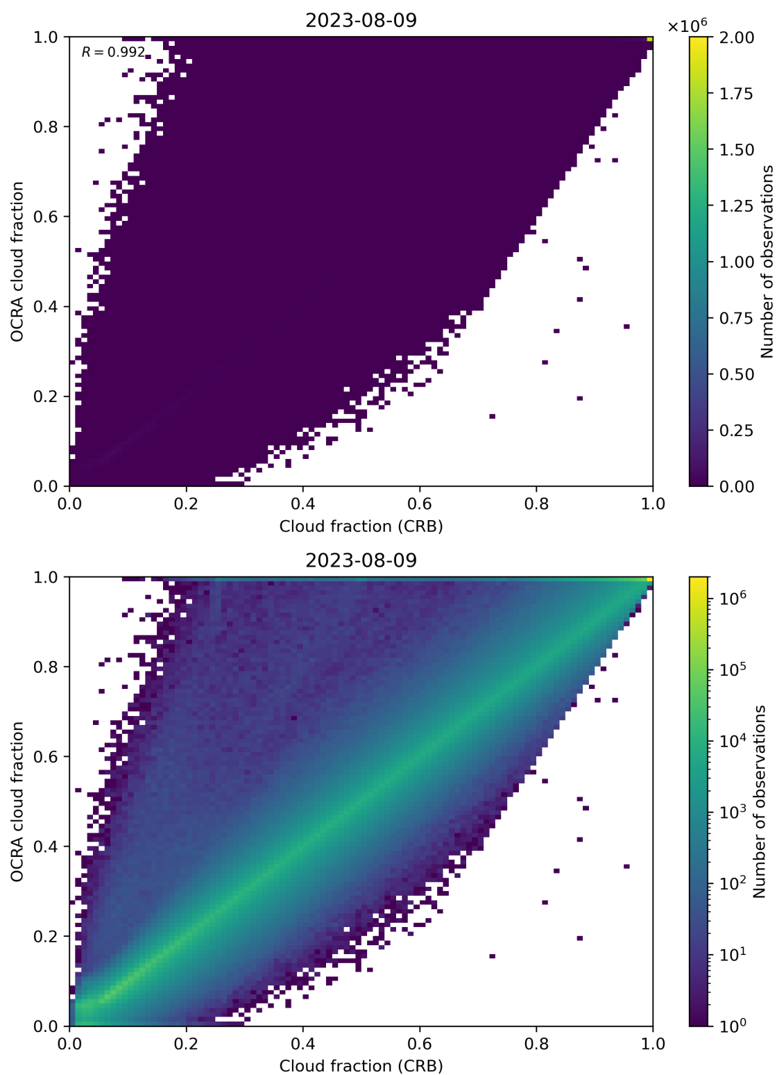
Figure 78: Scatter density plot of “Cloud fraction (CRB)” against “OCRA cloud fraction” for 2023-08-09 to 2023-08-10.
