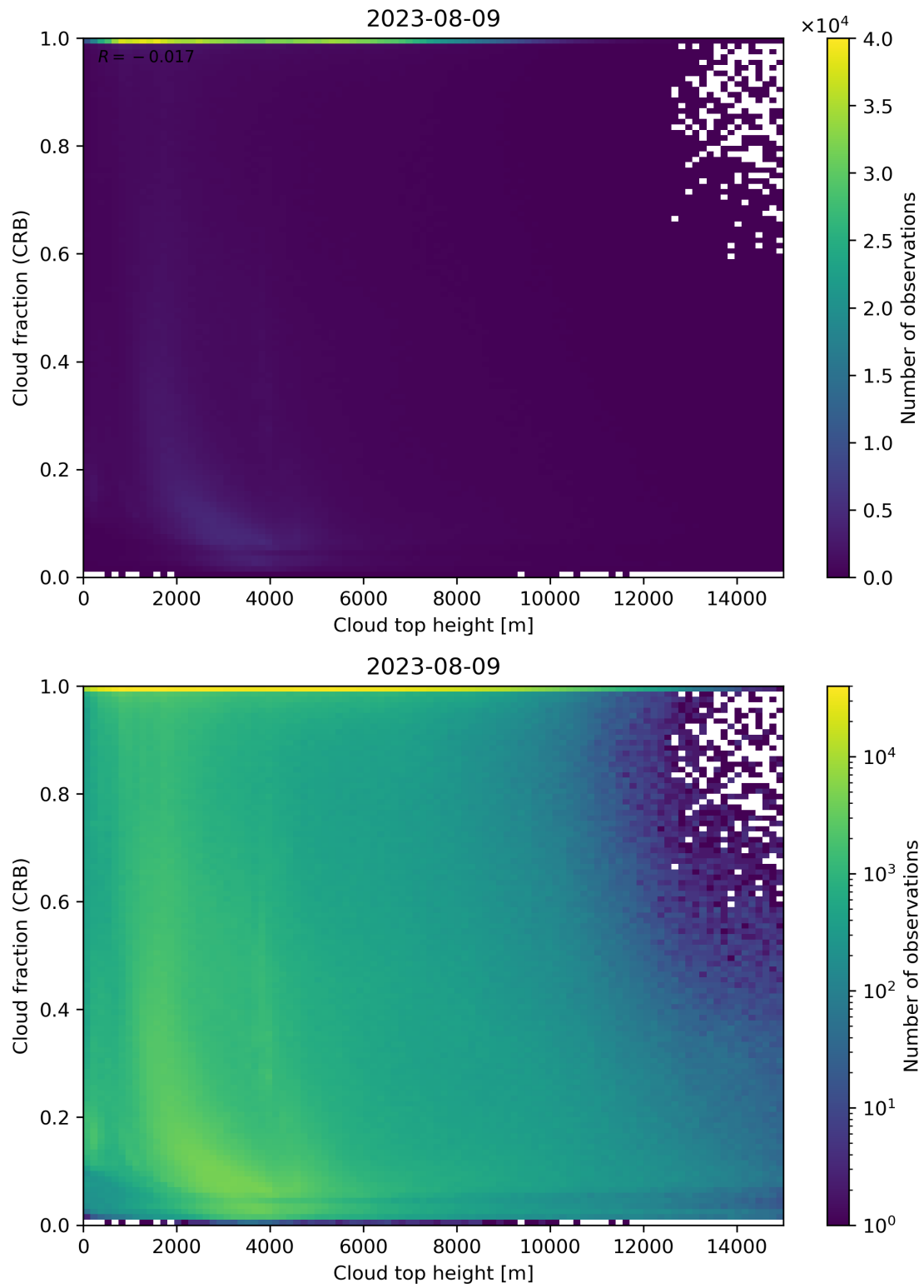
Figure 88: Scatter density plot of “Cloud top height” against “Cloud fraction (CRB)” for 2023-08-09 to 2023-08-10.
