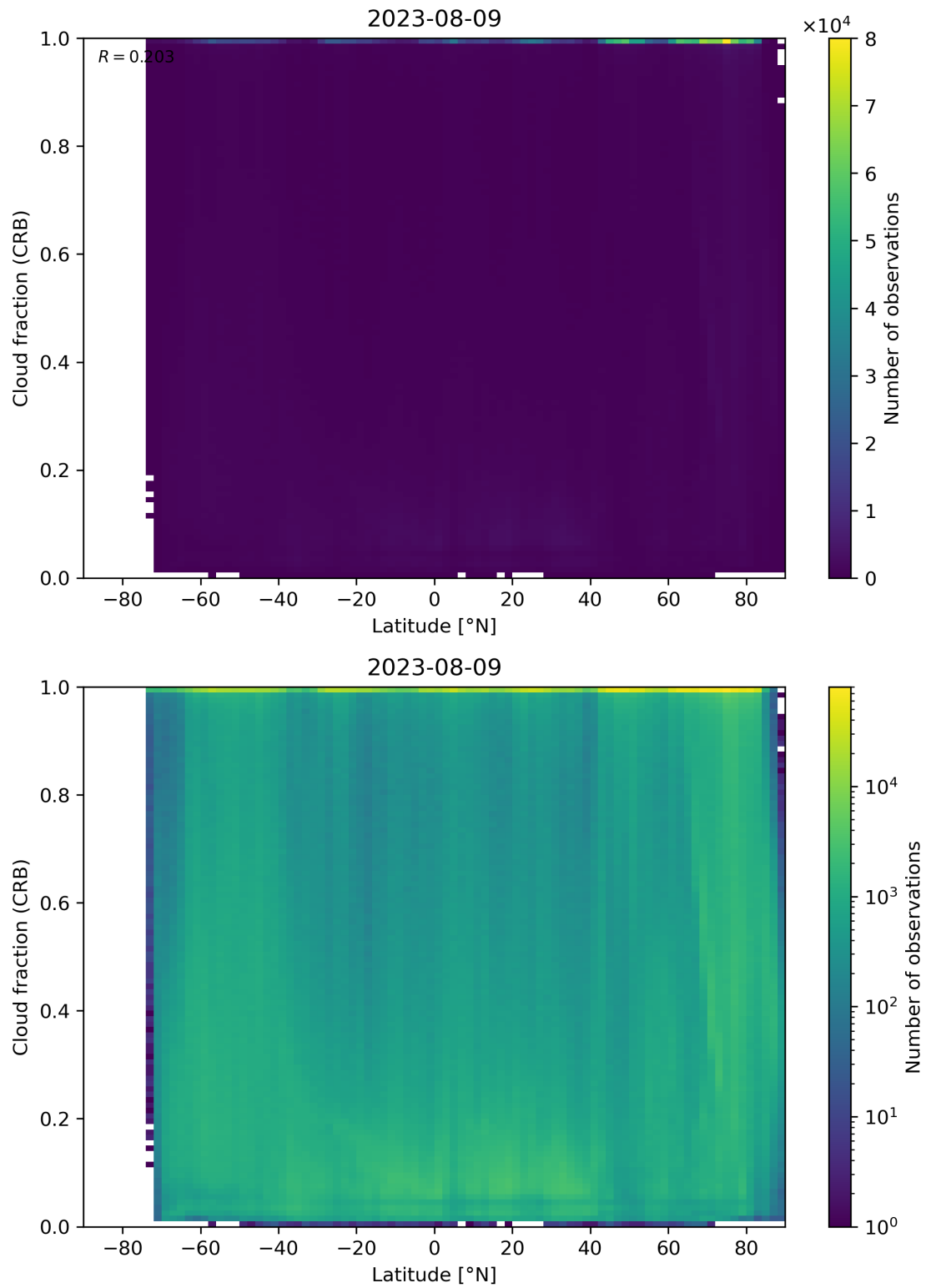
Figure 94: Scatter density plot of “Latitude” against “Cloud fraction (CRB)” for 2023-08-09 to 2023-08-10.
