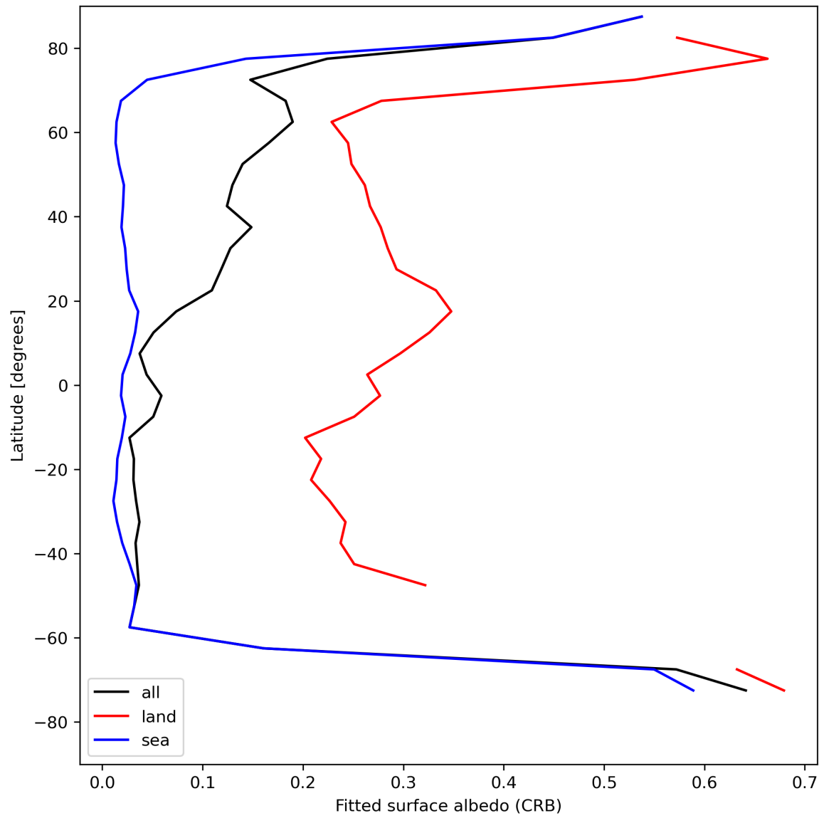
Figure 30: Zonal average of “Fitted surface albedo (CRB)” for 2023-08-09 to 2023-08-10.
