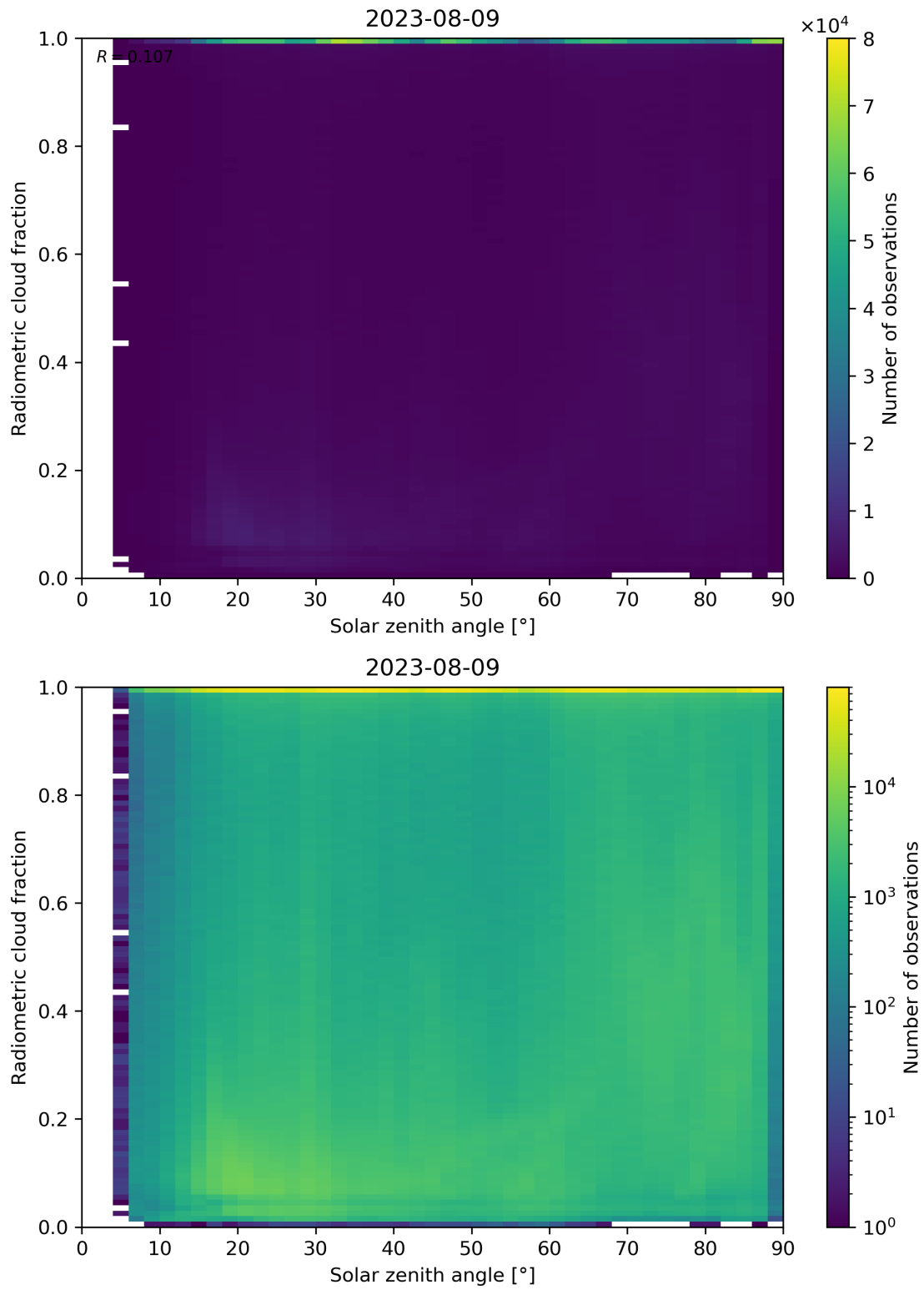
Figure 99: Scatter density plot of “Solar zenith angle” against “Radiometric cloud fraction” for 2023-08-09 to 2023-08-10.
