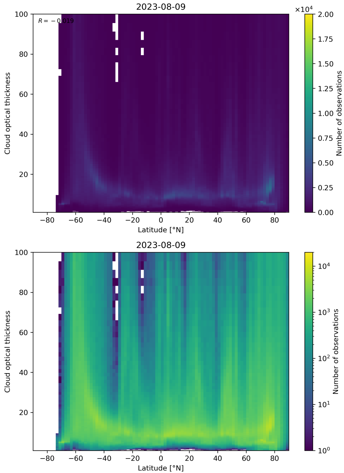
Figure 96: Scatter density plot of “Latitude” against “Cloud optical thickness” for 2023-08-09 to 2023-08-10.
