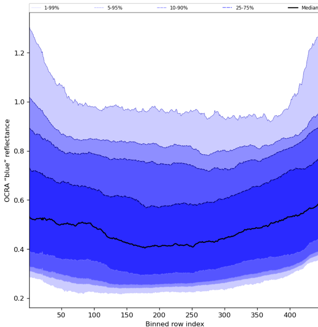
Figure 67: Along track statistics of “OCRA “blue” reflectance” for 2023-08-09 to 2023-08-10
