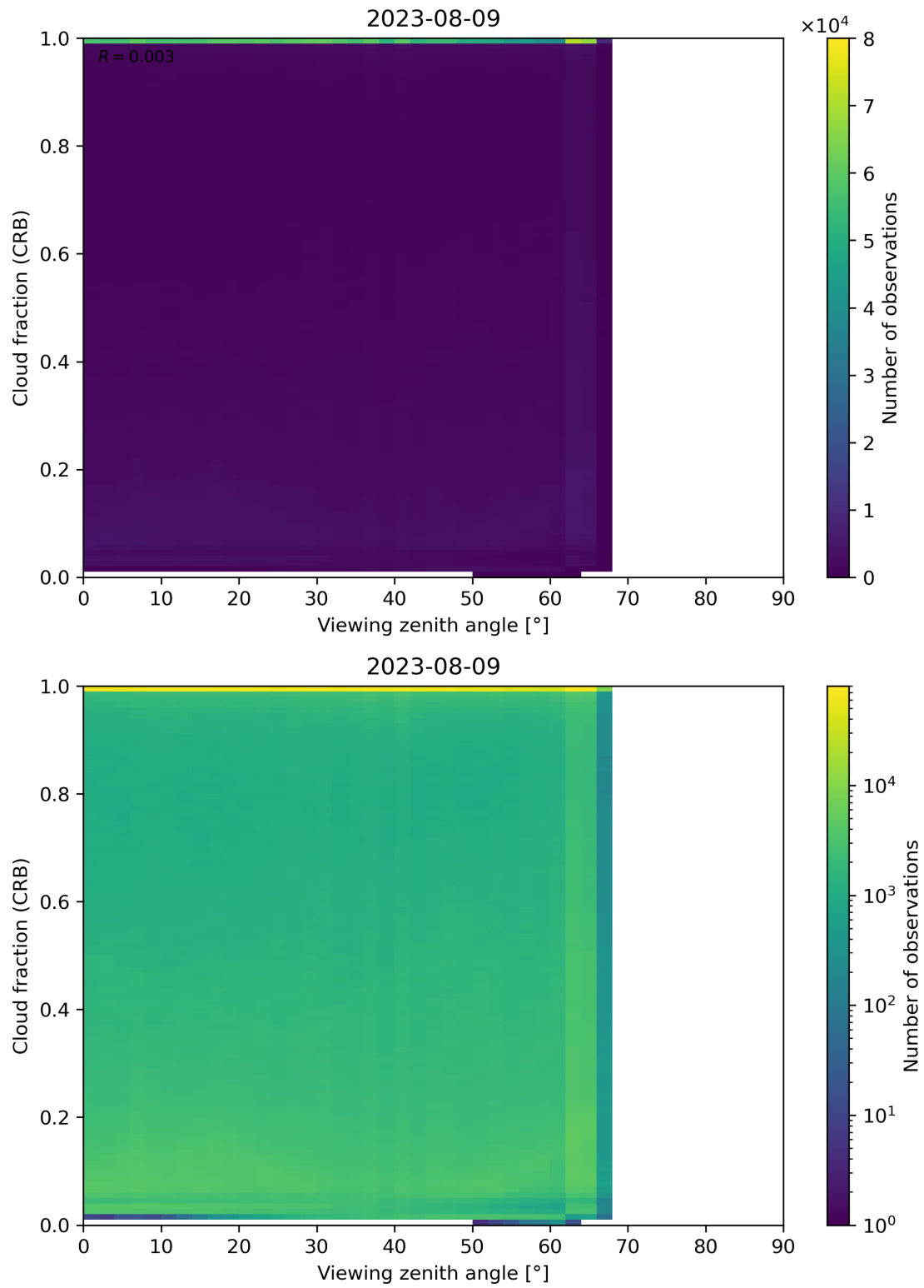
Figure 109: Scatter density plot of “Viewing zenith angle” against “Cloud fraction (CRB)” for 2023-08-09 to 2023-08-10.
