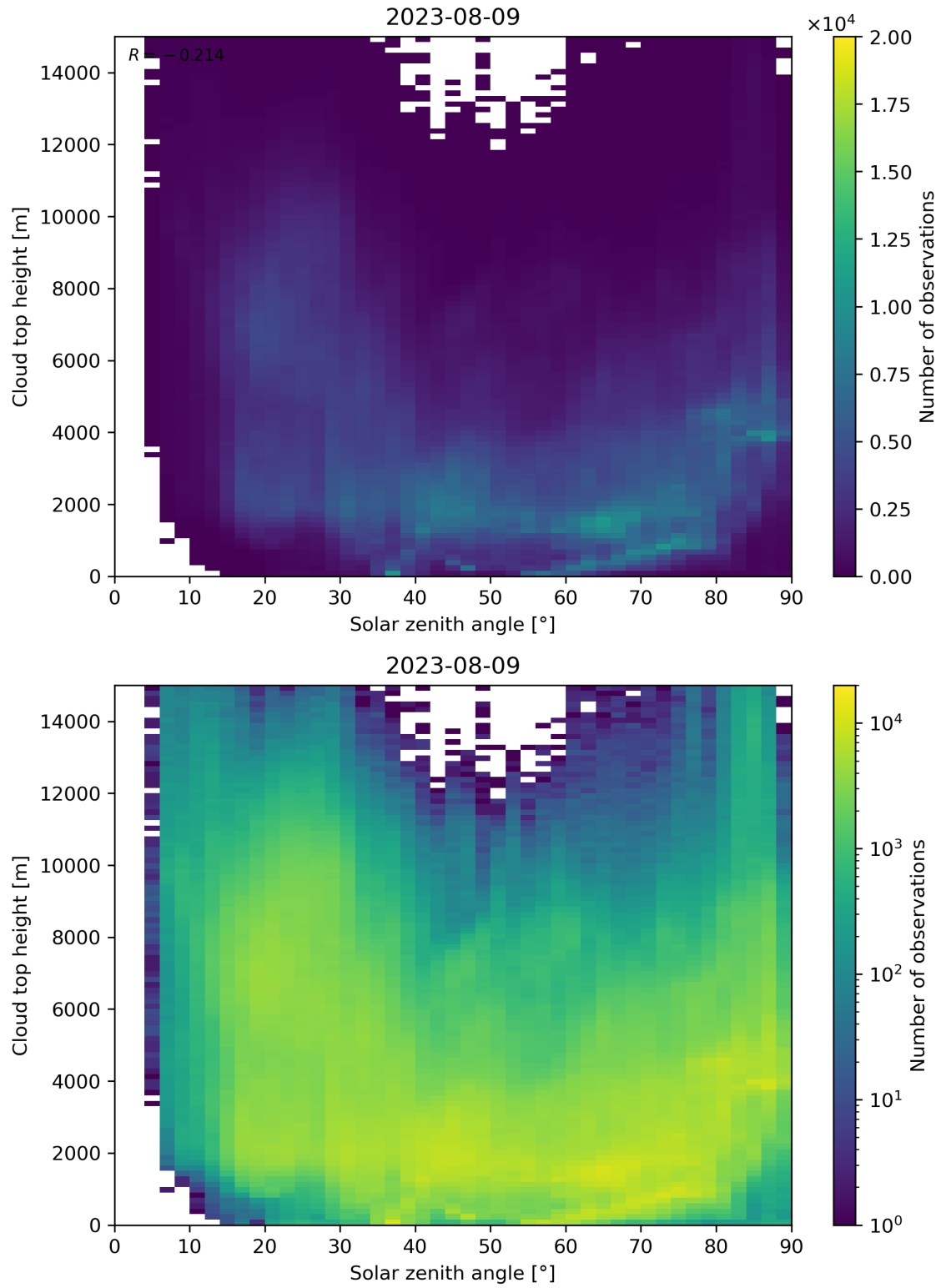
Figure 104: Scatter density plot of “Solar zenith angle” against “Cloud top height” for 2023-08-09 to 2023-08-10.
