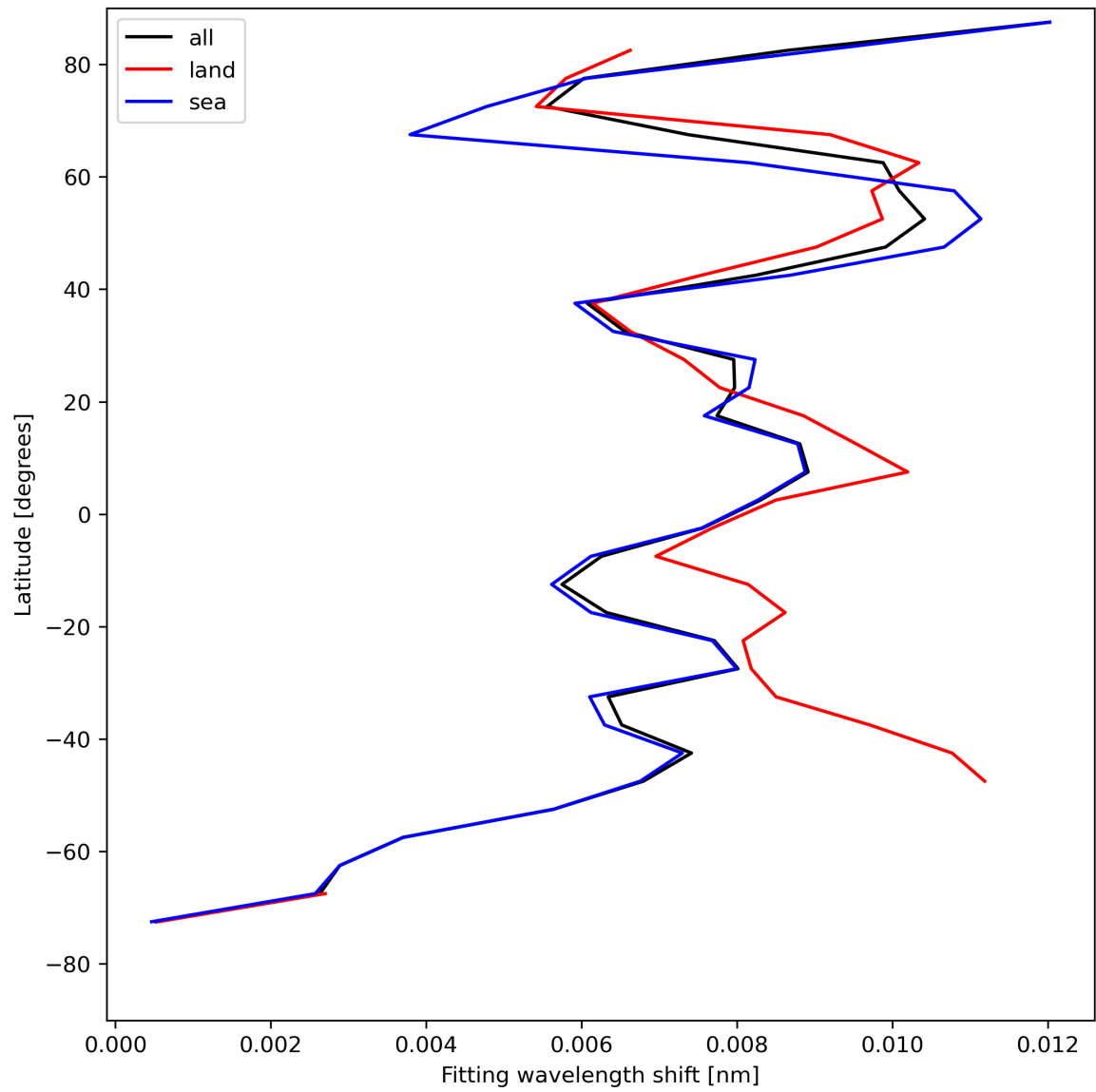
Figure 33: Zonal average of “Fitting wavelength shift” for 2023-08-09 to 2023-08-10.
