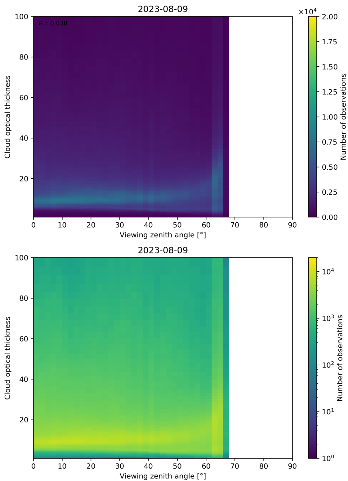
Figure 111: Scatter density plot of “Viewing zenith angle” against “Cloud optical thickness” for 2023-08-09 to 2023-08-10.
