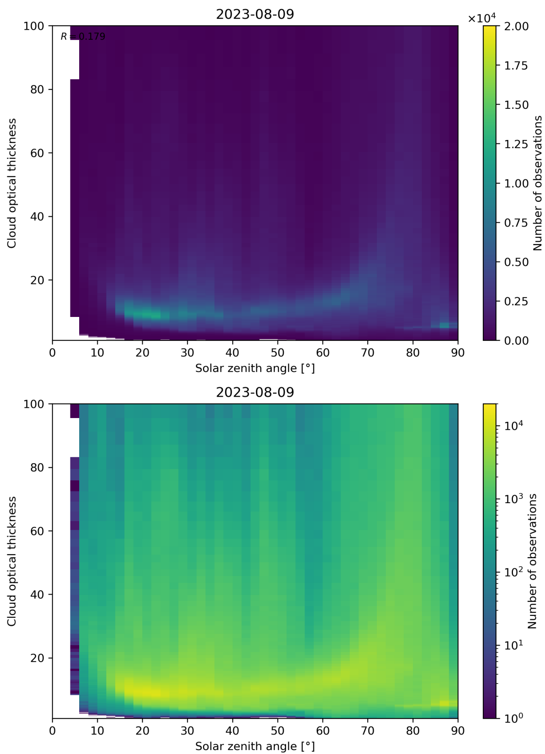
Figure 103: Scatter density plot of “Solar zenith angle” against “Cloud optical thickness” for 2023-08-09 to 2023-08-10.
