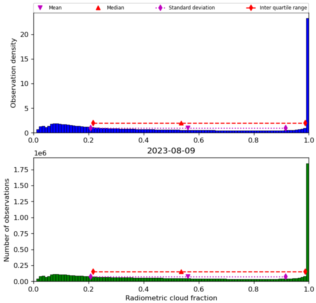
Figure 39: Histogram of “Radiometric cloud fraction” for 2023-08-09 to 2023-08-10
