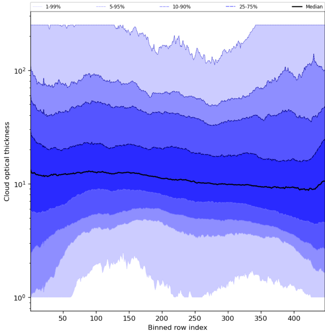
Figure 57: Along track statistics of “Cloud optical thickness” for 2023-08-09 to 2023-08-10
