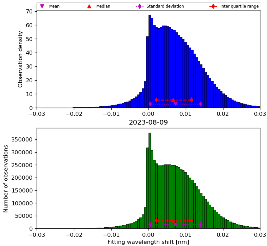
Figure 49: Histogram of “Fitting wavelength shift” for 2023-08-09 to 2023-08-10
