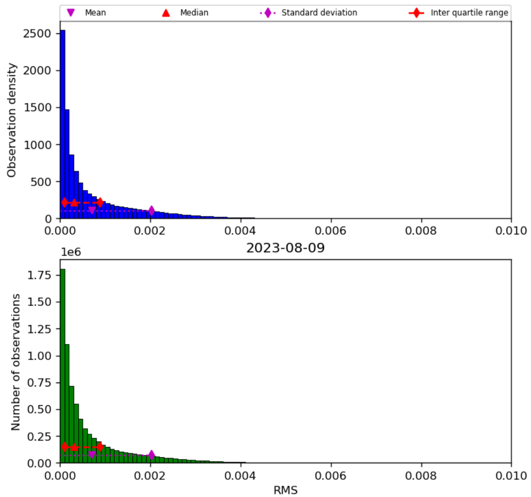
Figure 47: Histogram of “RMS” for 2023-08-09 to 2023-08-10
