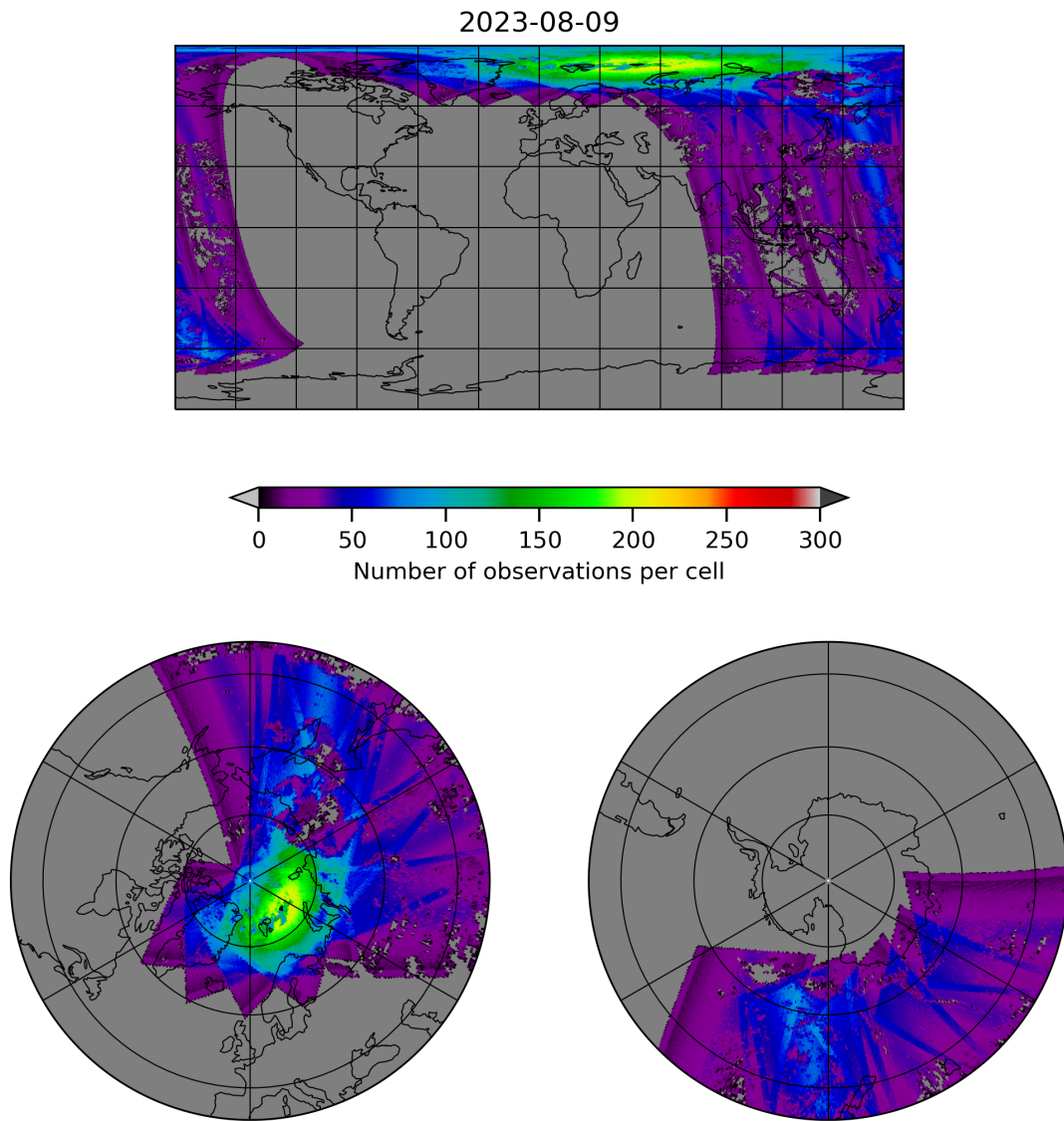
Figure 21: Map of the number of observations for 2023-08-09 to 2023-08-10
