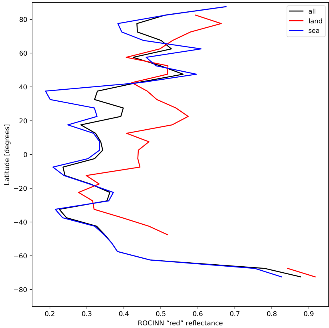
Figure 37: Zonal average of “ROCINN “red” reflectance” for 2023-08-09 to 2023-08-10.
