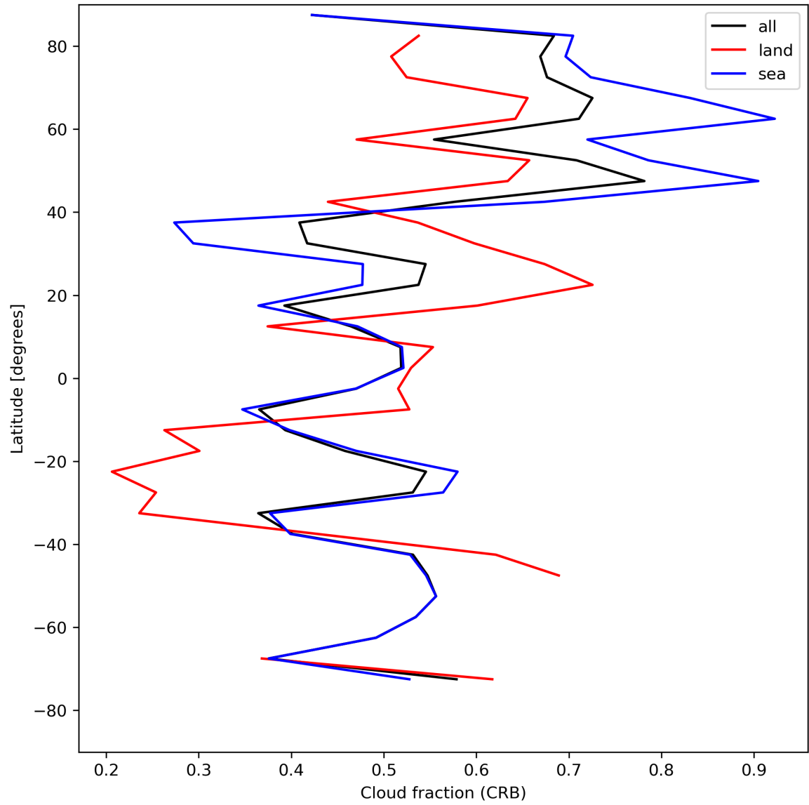
Figure 26: Zonal average of “Cloud fraction (CRB)” for 2023-08-09 to 2023-08-10.
