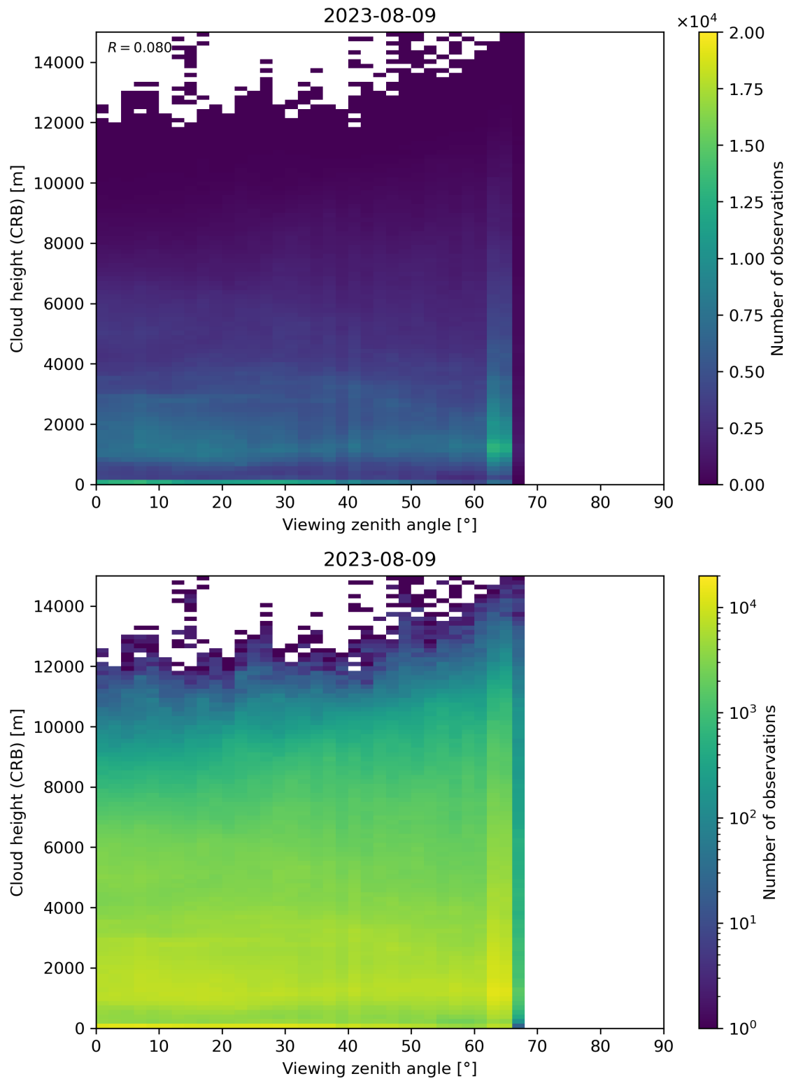
Figure 110: Scatter density plot of “Viewing zenith angle” against “Cloud height (CRB)” for 2023-08-09 to 2023-08-10.
