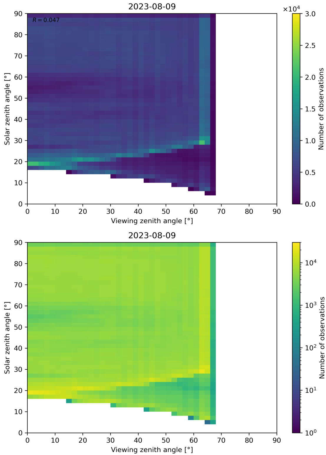
Figure 114: Scatter density plot of “Viewing zenith angle” against “Solar zenith angle” for 2023-08-09 to 2023-08-10.
