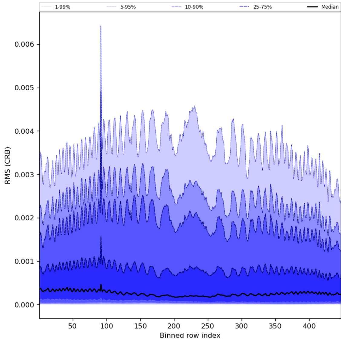
Figure 64: Along track statistics of “RMS (CRB)” for 2023-08-09 to 2023-08-10
