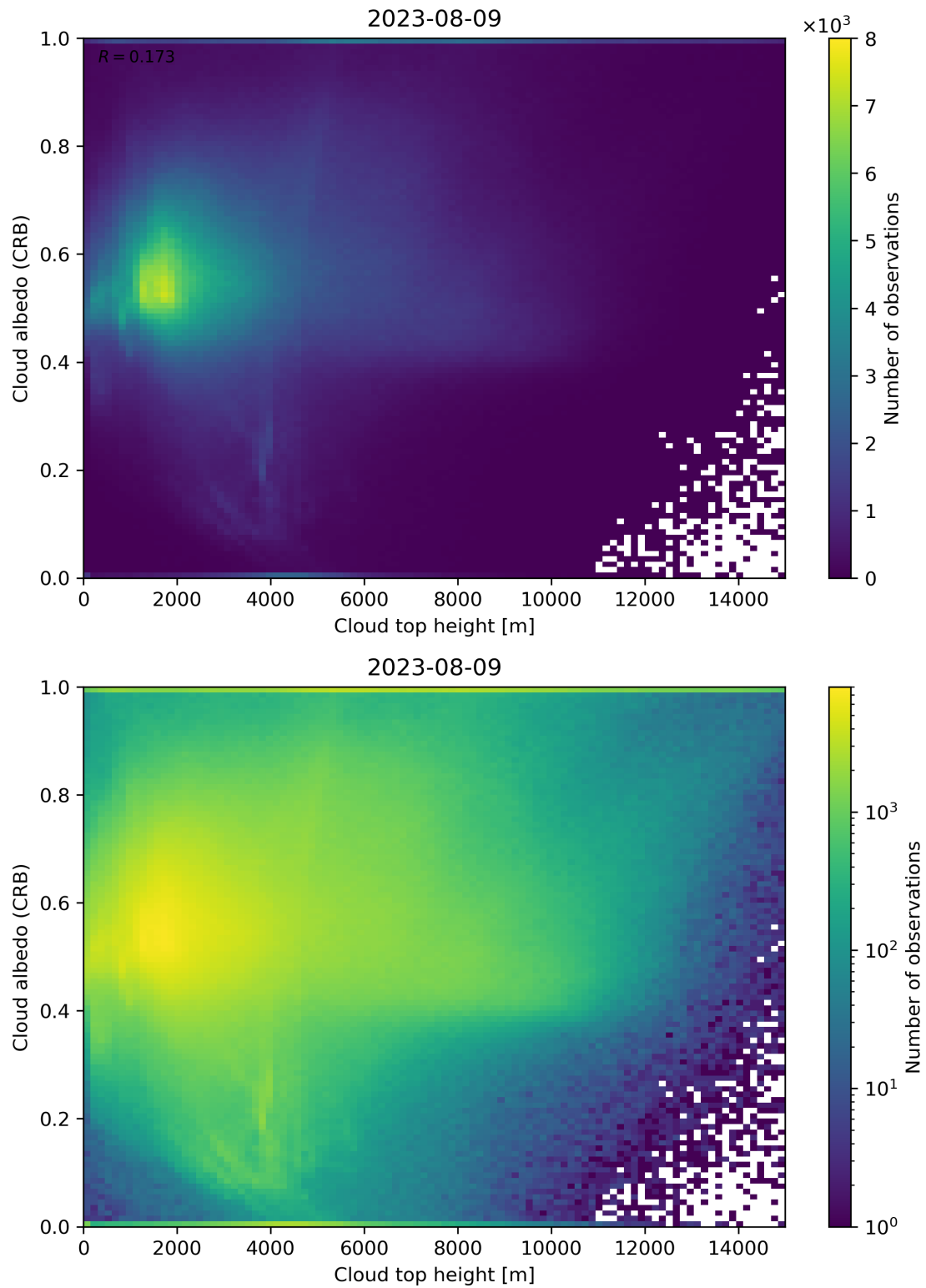
Figure 86: Scatter density plot of “Cloud top height” against “Cloud albedo (CRB)” for 2023-08-09 to 2023-08-10.
