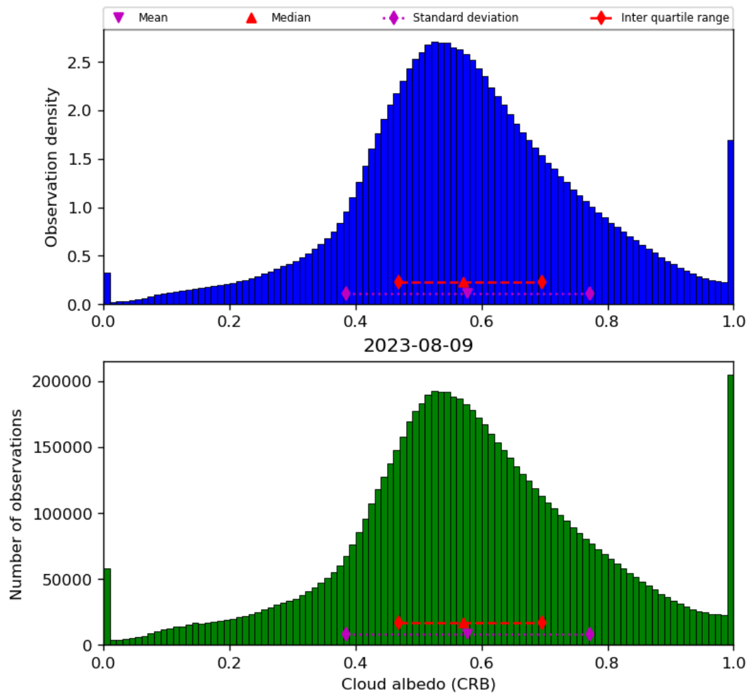
Figure 44: Histogram of “Cloud albedo (CRB)” for 2023-08-09 to 2023-08-10
