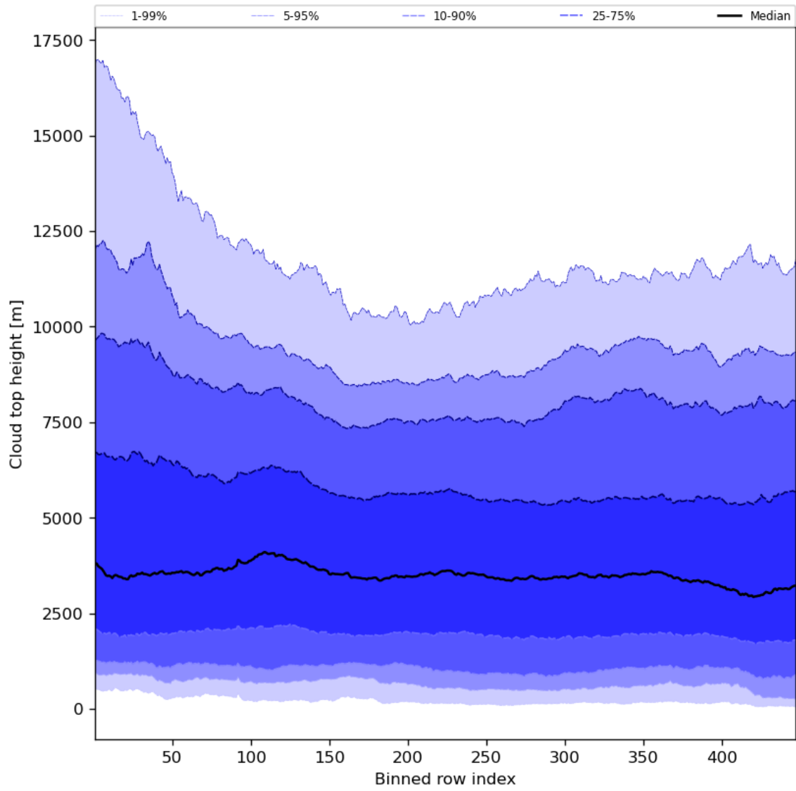
Figure 56: Along track statistics of “Cloud top height” for 2023-08-09 to 2023-08-10
