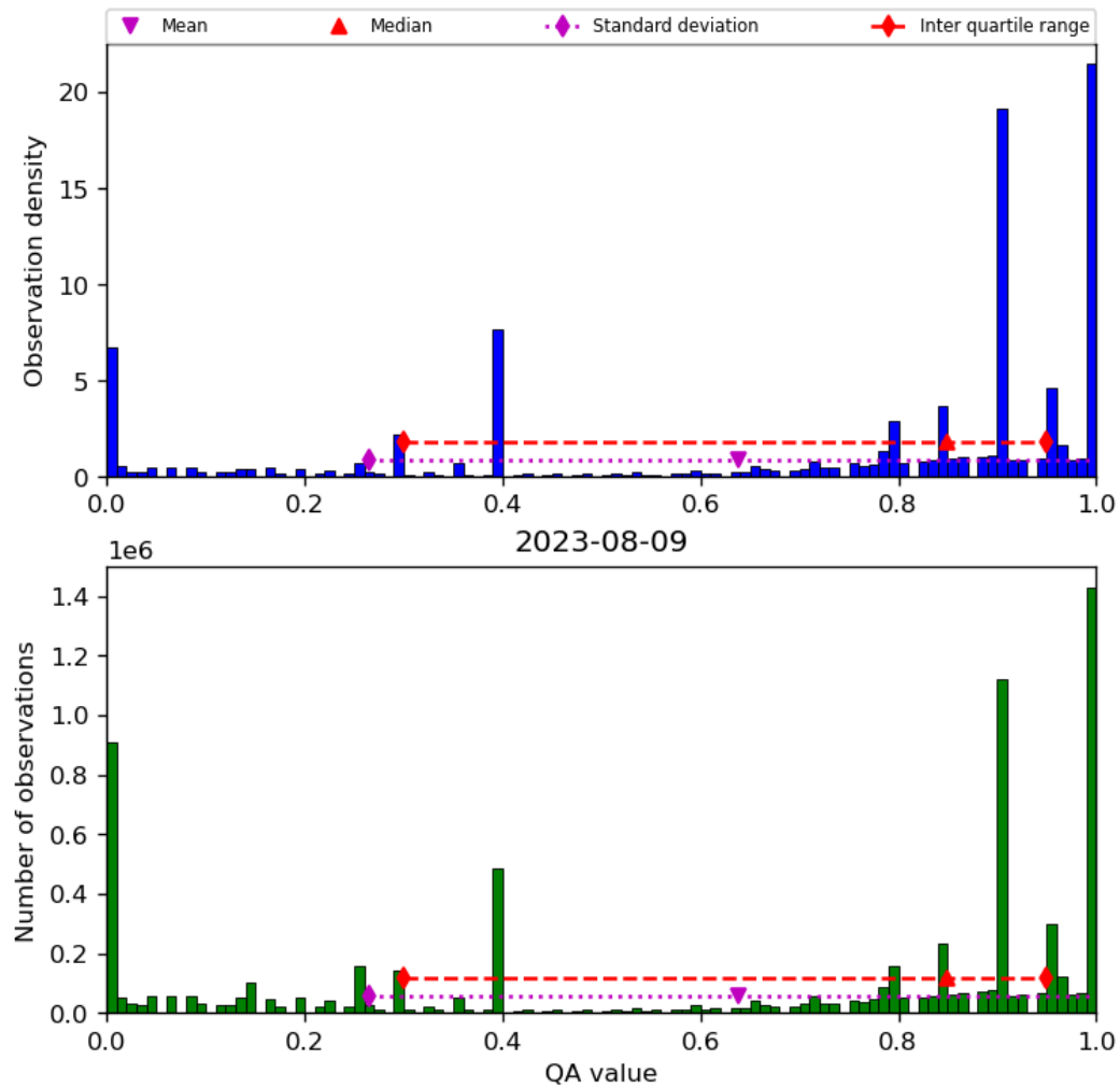
Figure 38: Histogram of “QA value” for 2023-08-09 to 2023-08-10
