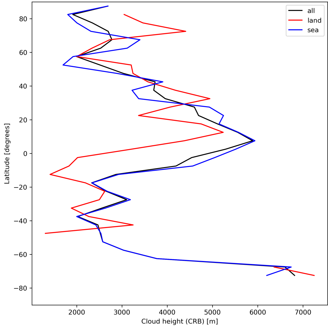
Figure 27: Zonal average of “Cloud height (CRB)” for 2023-08-09 to 2023-08-10.
