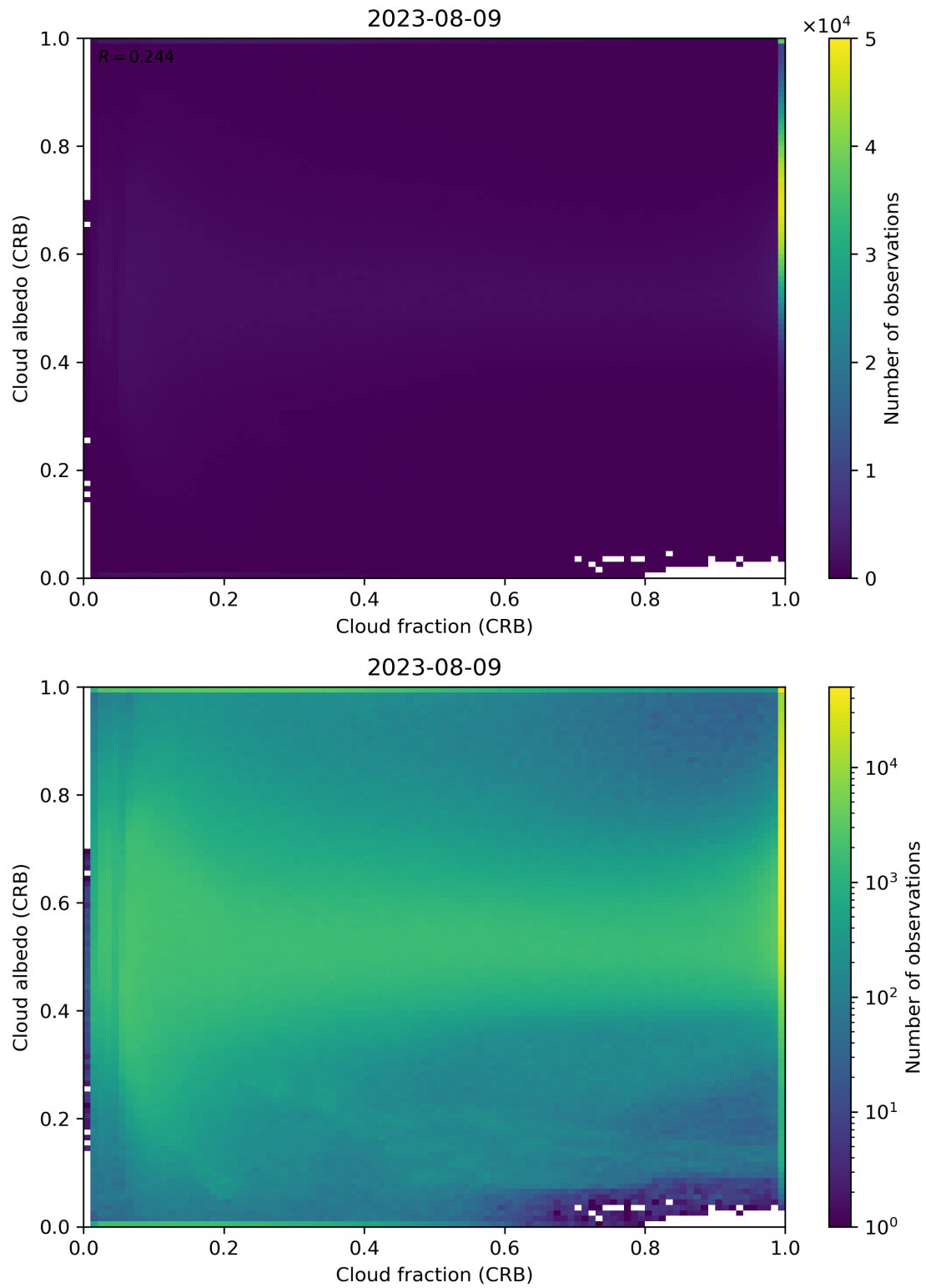
Figure 77: Scatter density plot of “Cloud fraction (CRB)” against “Cloud albedo (CRB)” for 2023-08-09 to 2023-08-10.
