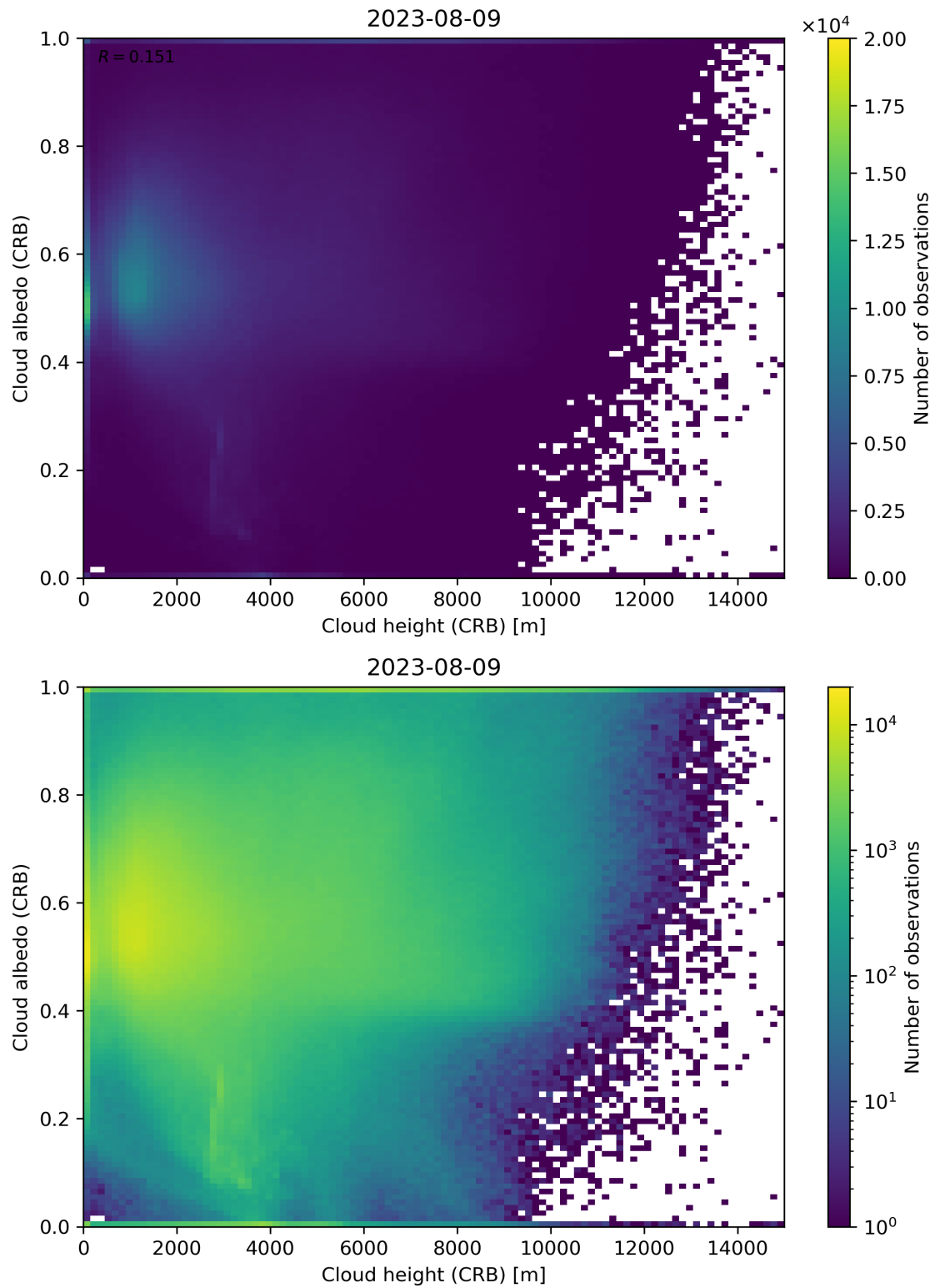
Figure 80: Scatter density plot of “Cloud height (CRB)” against “Cloud albedo (CRB)” for 2023-08-09 to 2023-08-10.
