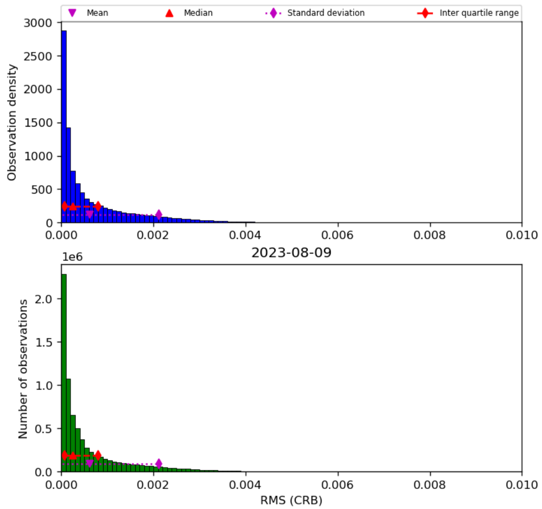
Figure 48: Histogram of “RMS (CRB)” for 2023-08-09 to 2023-08-10
