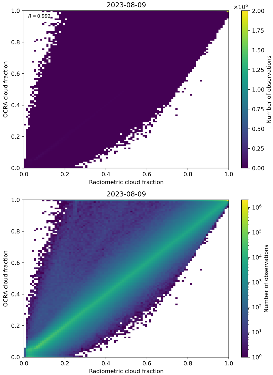
Figure 72: Scatter density plot of “Radiometric cloud fraction” against “OCRA cloud fraction” for 2023-08-09 to 2023-08-10.
