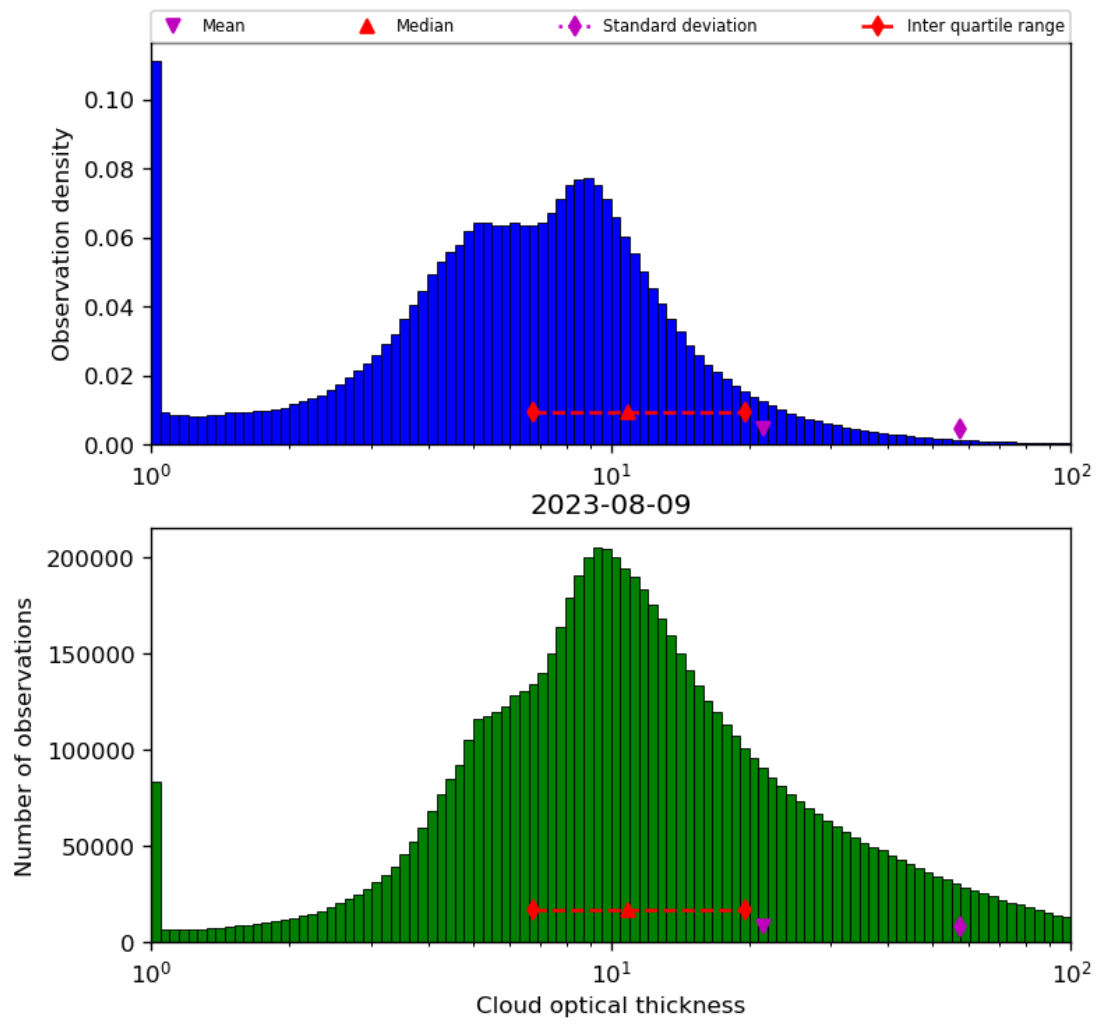
Figure 41: Histogram of “Cloud optical thickness” for 2023-08-09 to 2023-08-10
