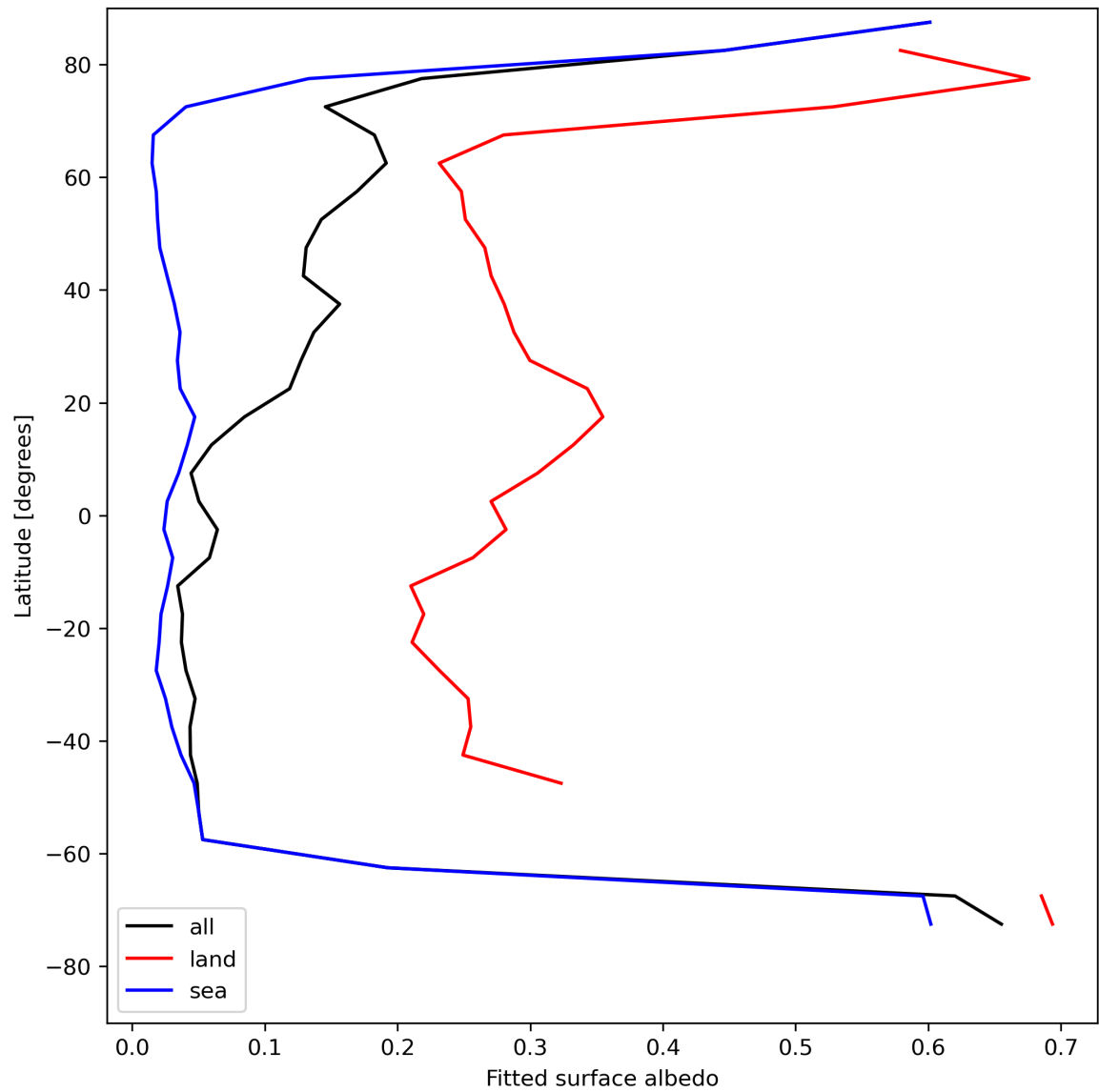
Figure 29: Zonal average of “Fitted surface albedo” for 2023-08-09 to 2023-08-10.
