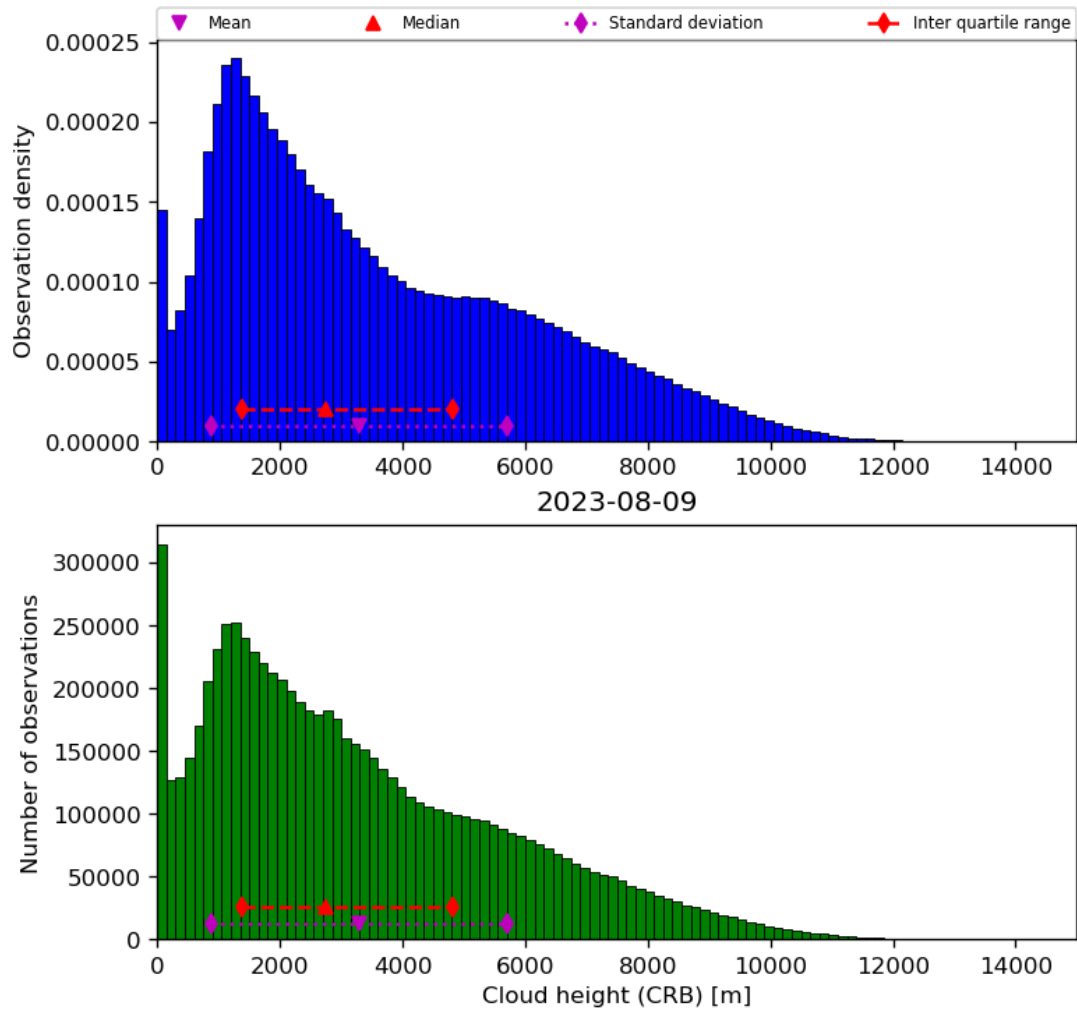
Figure 43: Histogram of “Cloud height (CRB)” for 2023-08-09 to 2023-08-10
