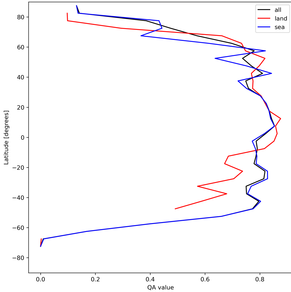
Figure 22: Zonal average of “QA value” for 2023-08-09 to 2023-08-10.
