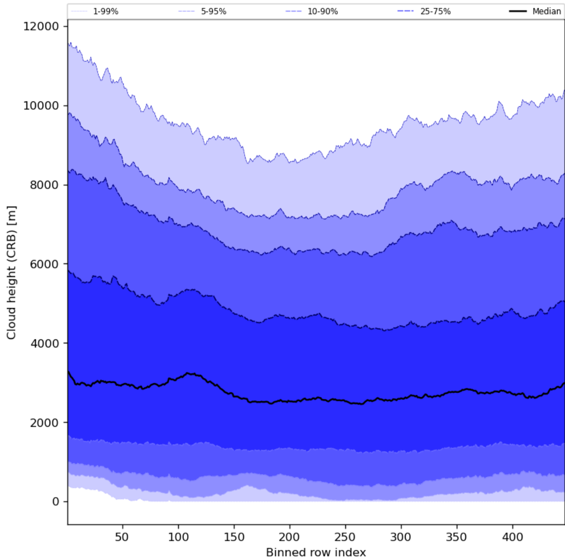
Figure 59: Along track statistics of “Cloud height (CRB)” for 2023-08-09 to 2023-08-10
