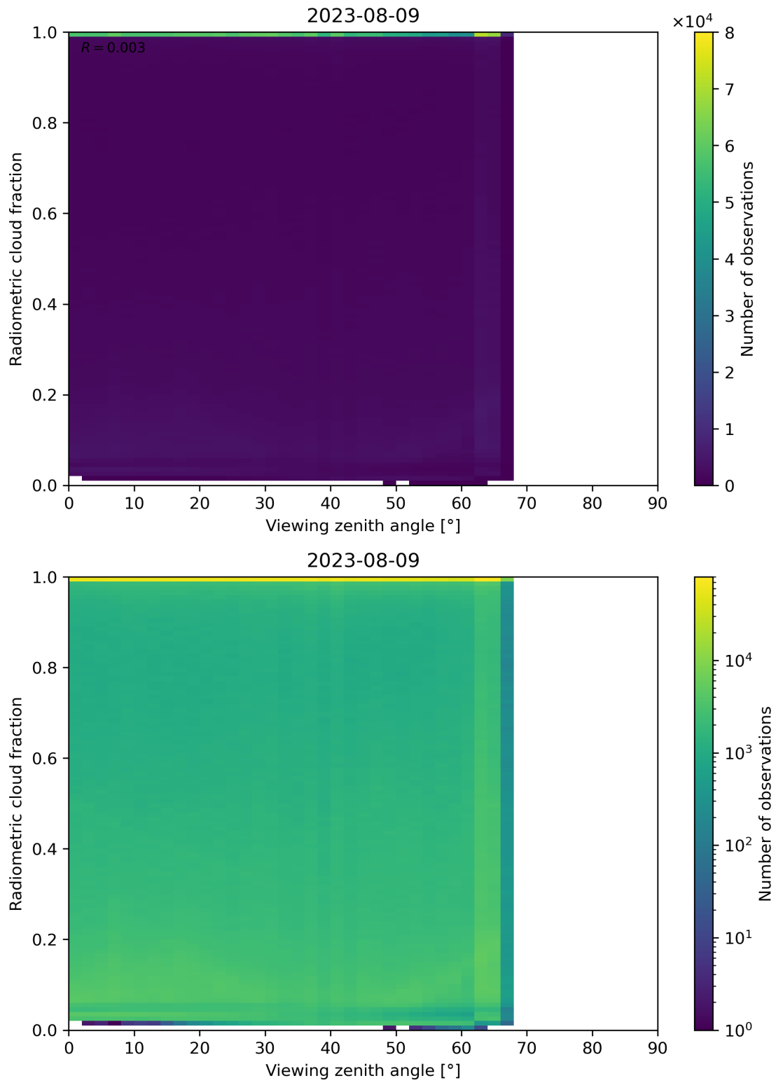
Figure 107: Scatter density plot of “Viewing zenith angle” against “Radiometric cloud fraction” for 2023-08-09 to 2023-08-10.
