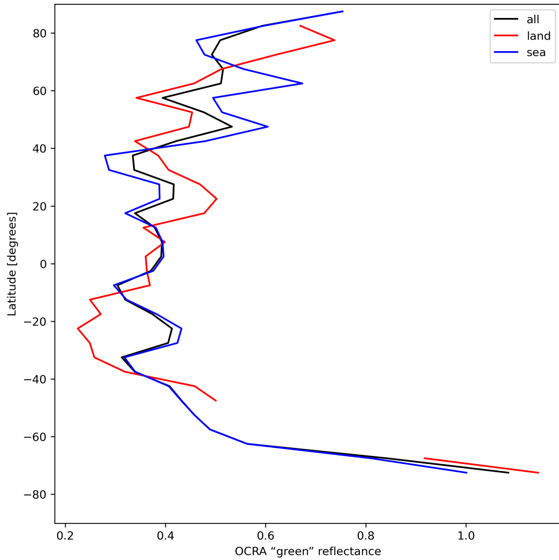
Figure 36: Zonal average of “OCRA “green” reflectance” for 2023-08-09 to 2023-08-10.
