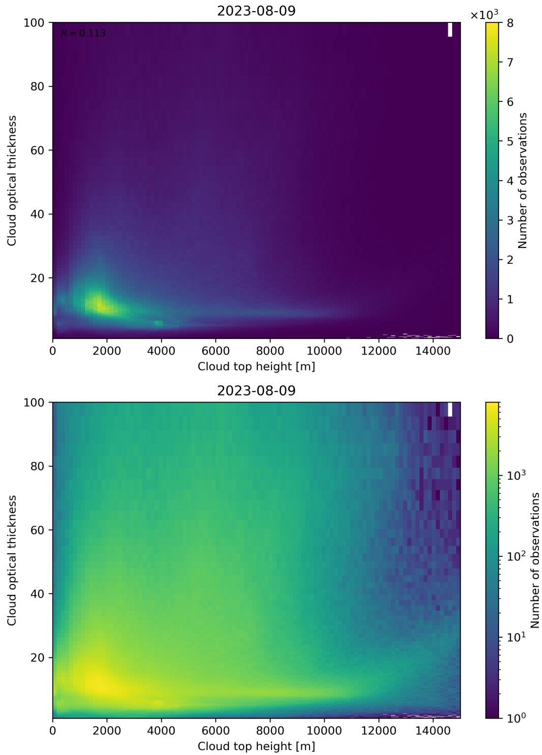
Figure 90: Scatter density plot of “Cloud top height” against “Cloud optical thickness” for 2023-08-09 to 2023-08-10.
