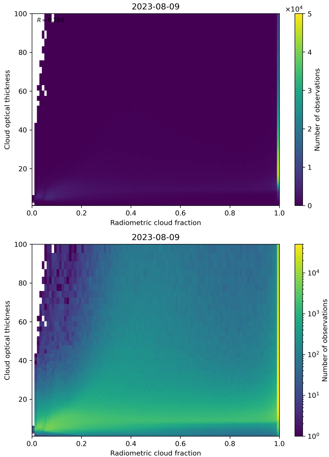
Figure 75: Scatter density plot of “Radiometric cloud fraction” against “Cloud optical thickness” for 2023-08-09 to 2023-08-10.
