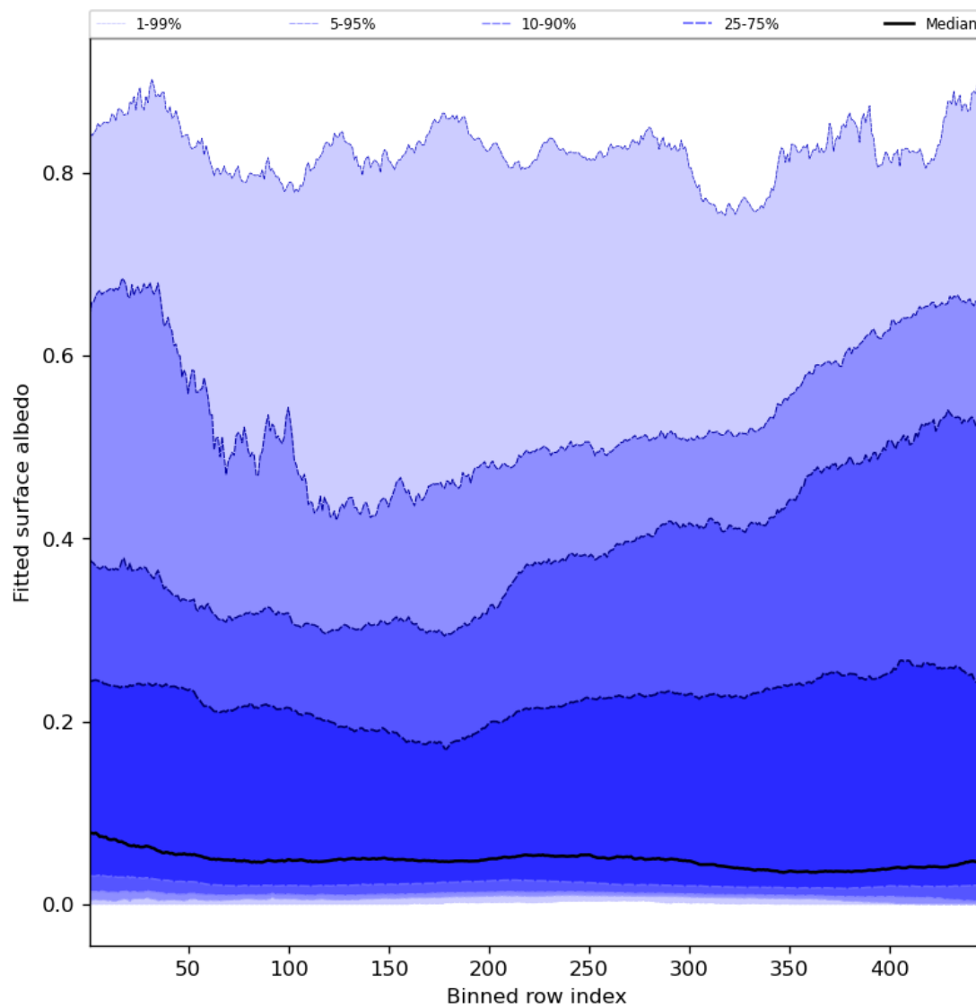
Figure 61: Along track statistics of “Fitted surface albedo” for 2023-08-09 to 2023-08-10
