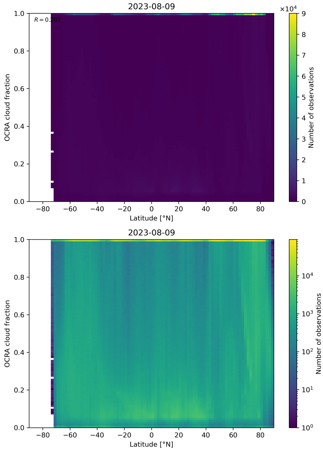
Figure 93: Scatter density plot of “Latitude” against “OCRA cloud fraction” for 2023-08-09 to 2023-08-10.
