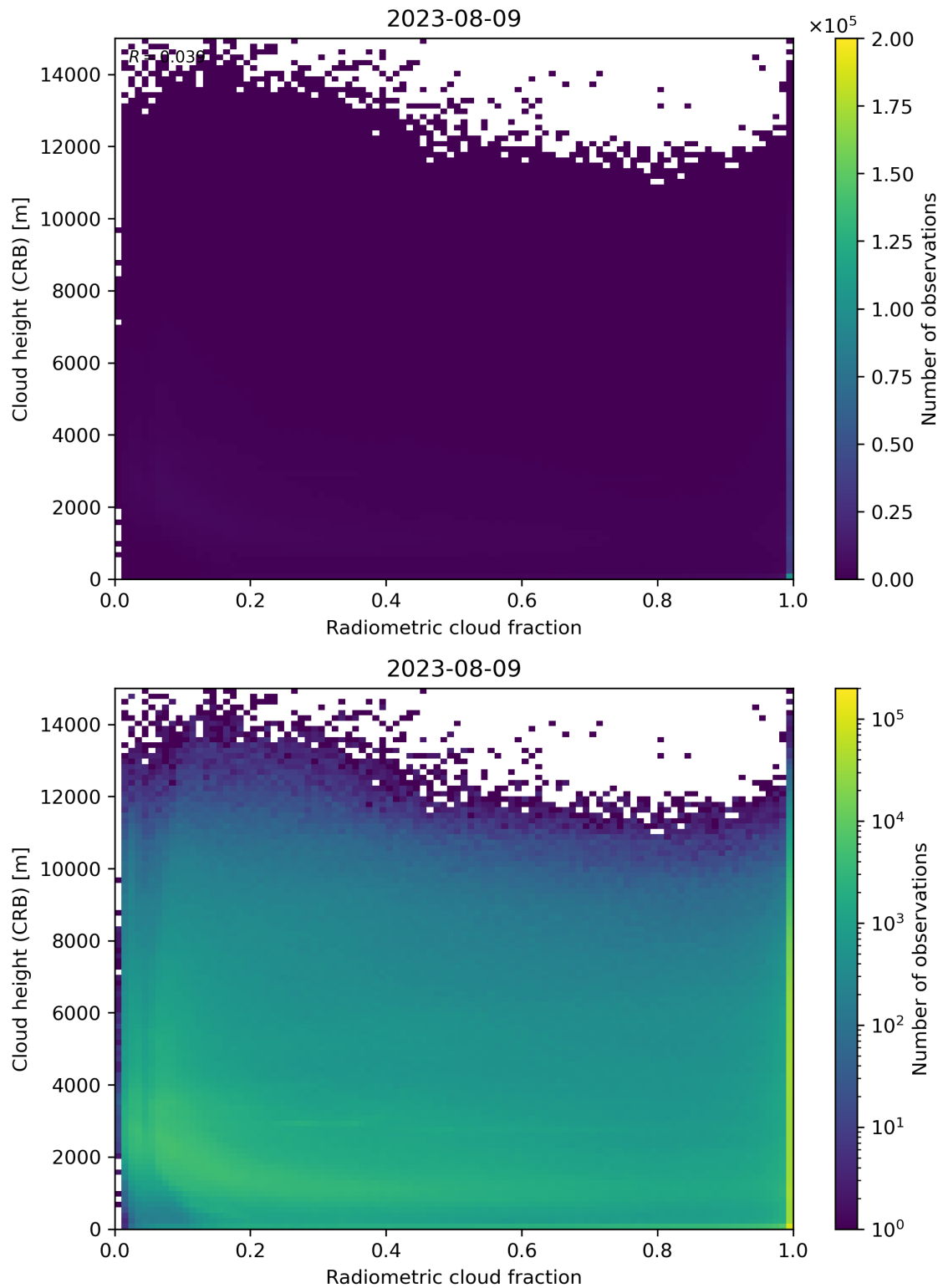
Figure 74: Scatter density plot of “Radiometric cloud fraction” against “Cloud height (CRB)” for 2023-08-09 to 2023-08-10.
