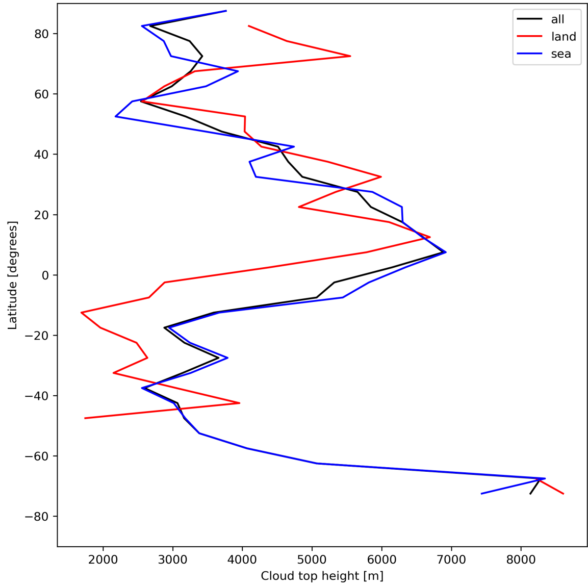
Figure 24: Zonal average of “Cloud top height” for 2023-08-09 to 2023-08-10.
