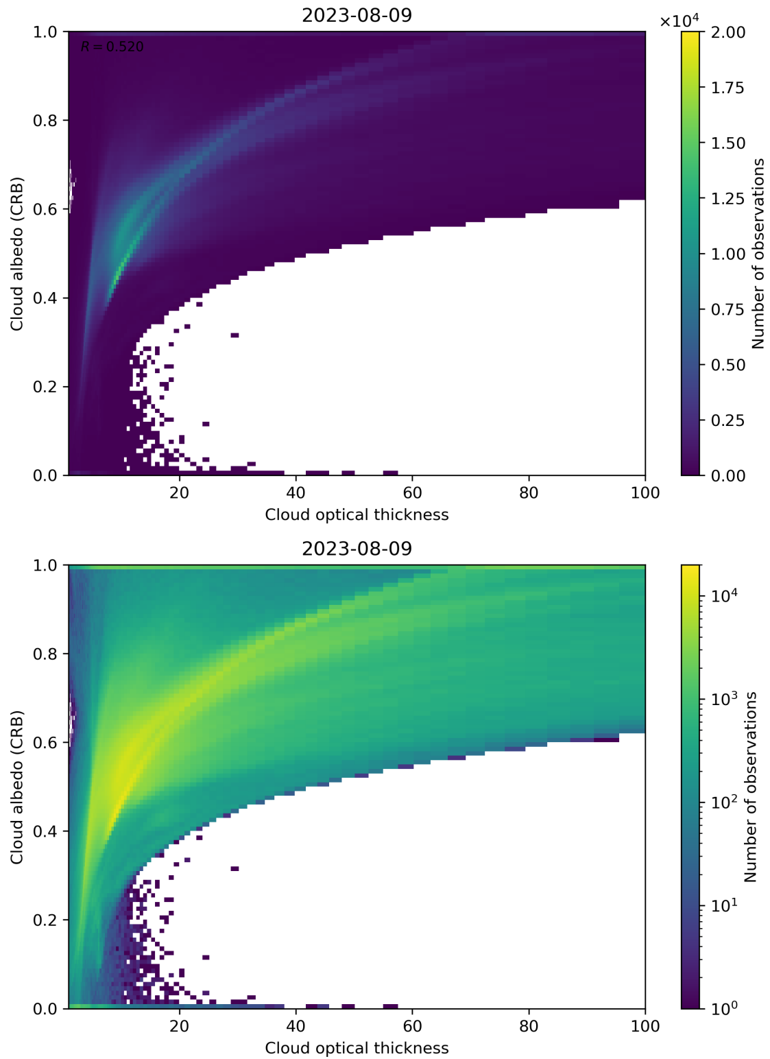
Figure 82: Scatter density plot of “Cloud optical thickness” against “Cloud albedo (CRB)” for 2023-08-09 to 2023-08-10.
