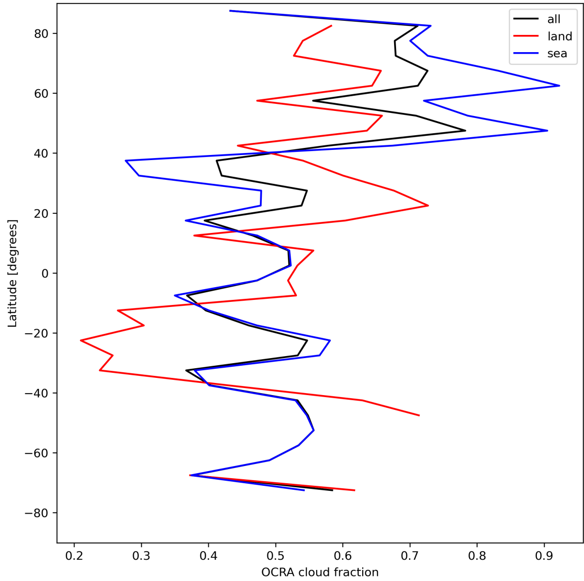
Figure 34: Zonal average of “OCRA cloud fraction” for 2023-08-09 to 2023-08-10.
