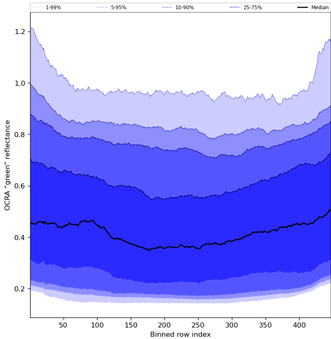
Figure 68: Along track statistics of “OCRA “green” reflectance” for 2023-08-09 to 2023-08-10
