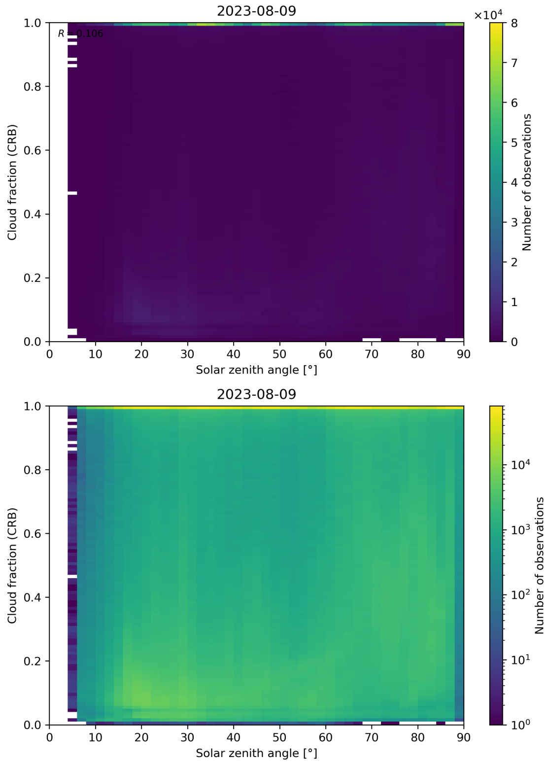
Figure 101: Scatter density plot of “Solar zenith angle” against “Cloud fraction (CRB)” for 2023-08-09 to 2023-08-10.
