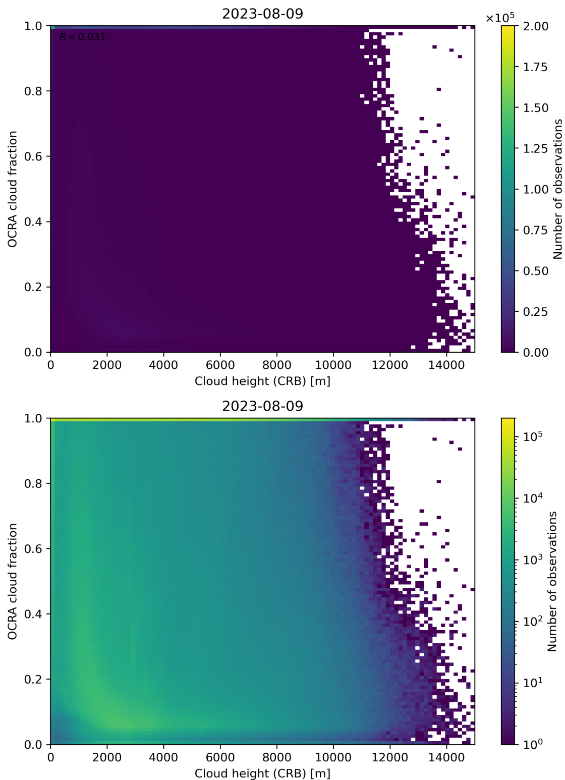
Figure 81: Scatter density plot of “Cloud height (CRB)” against “OCRA cloud fraction” for 2023-08-09 to 2023-08-10.
