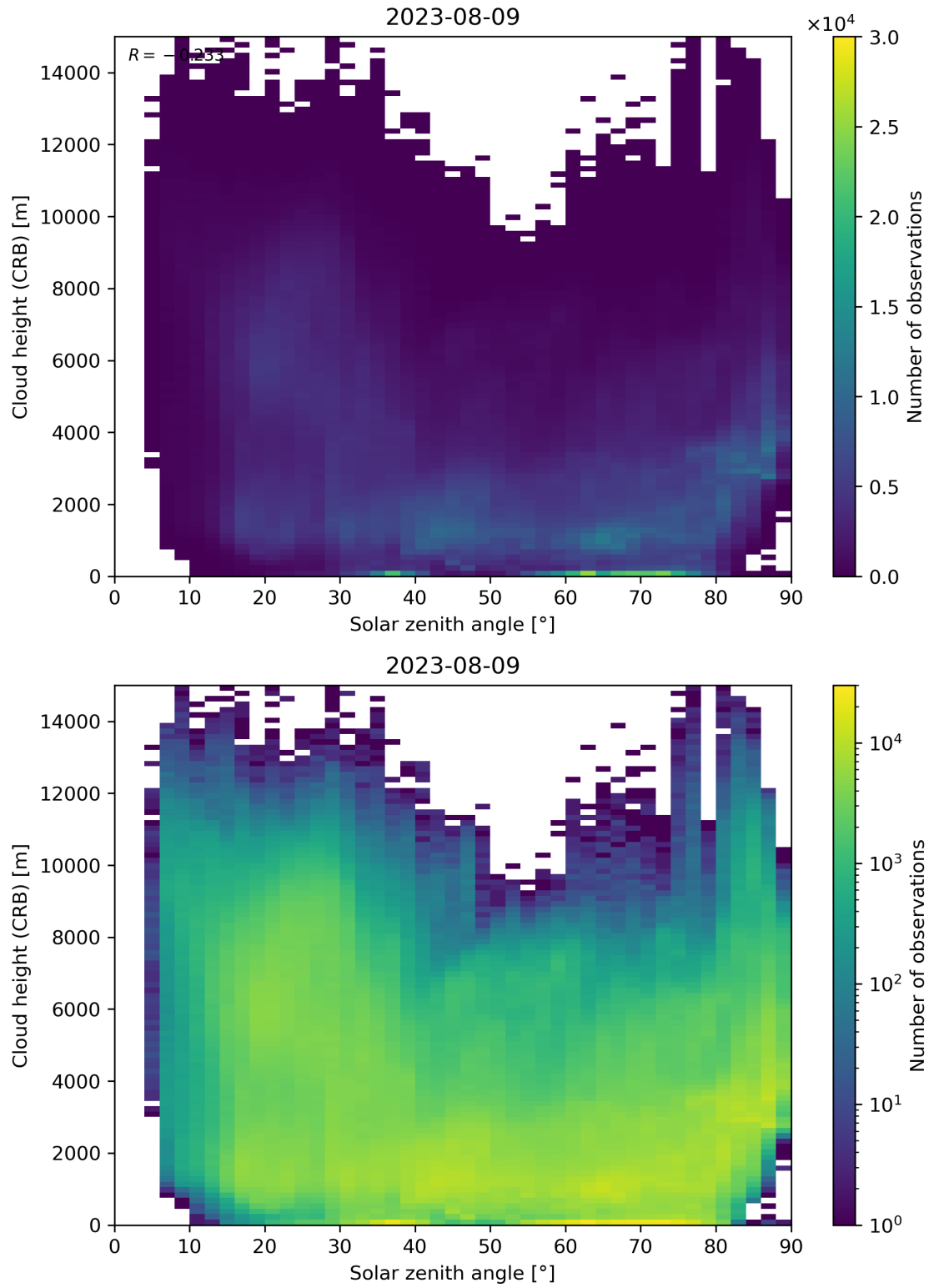
Figure 102: Scatter density plot of “Solar zenith angle” against “Cloud height (CRB)” for 2023-08-09 to 2023-08-10.
