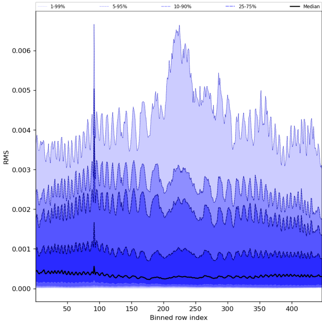
Figure 63: Along track statistics of “RMS” for 2023-08-09 to 2023-08-10
