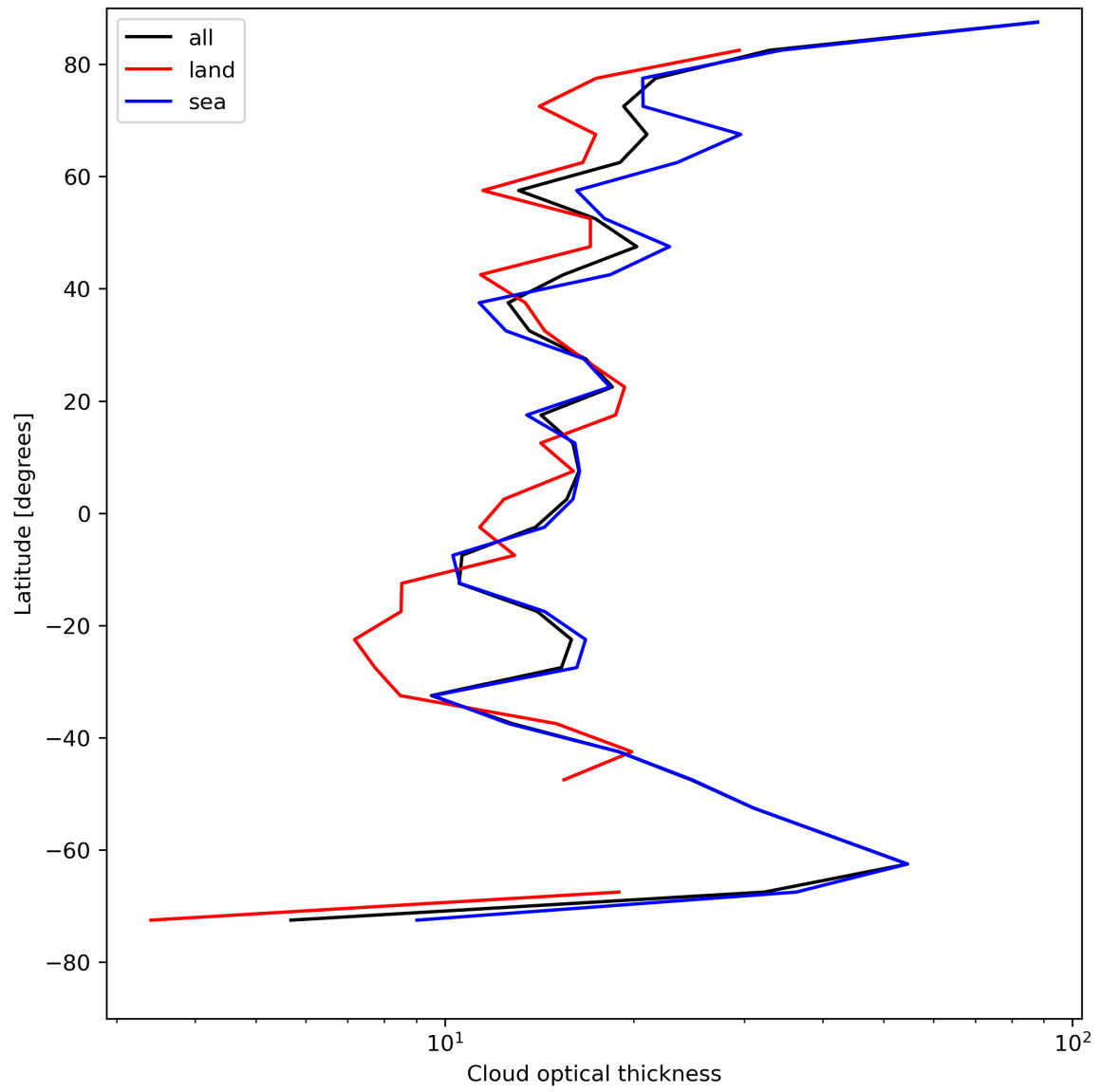
Figure 25: Zonal average of “Cloud optical thickness” for 2023-08-09 to 2023-08-10.
