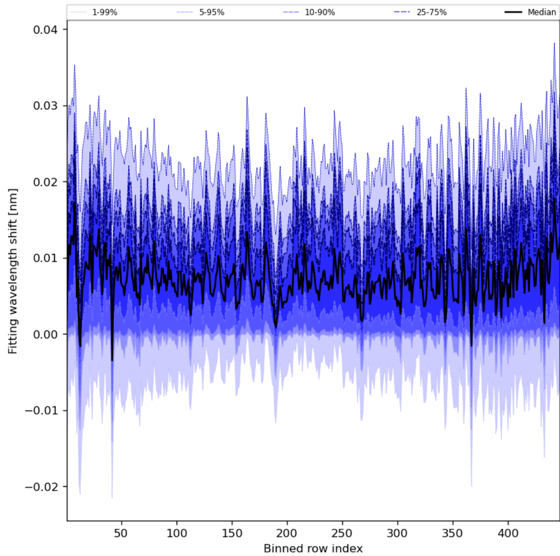
Figure 65: Along track statistics of “Fitting wavelength shift” for 2023-08-09 to 2023-08-10
