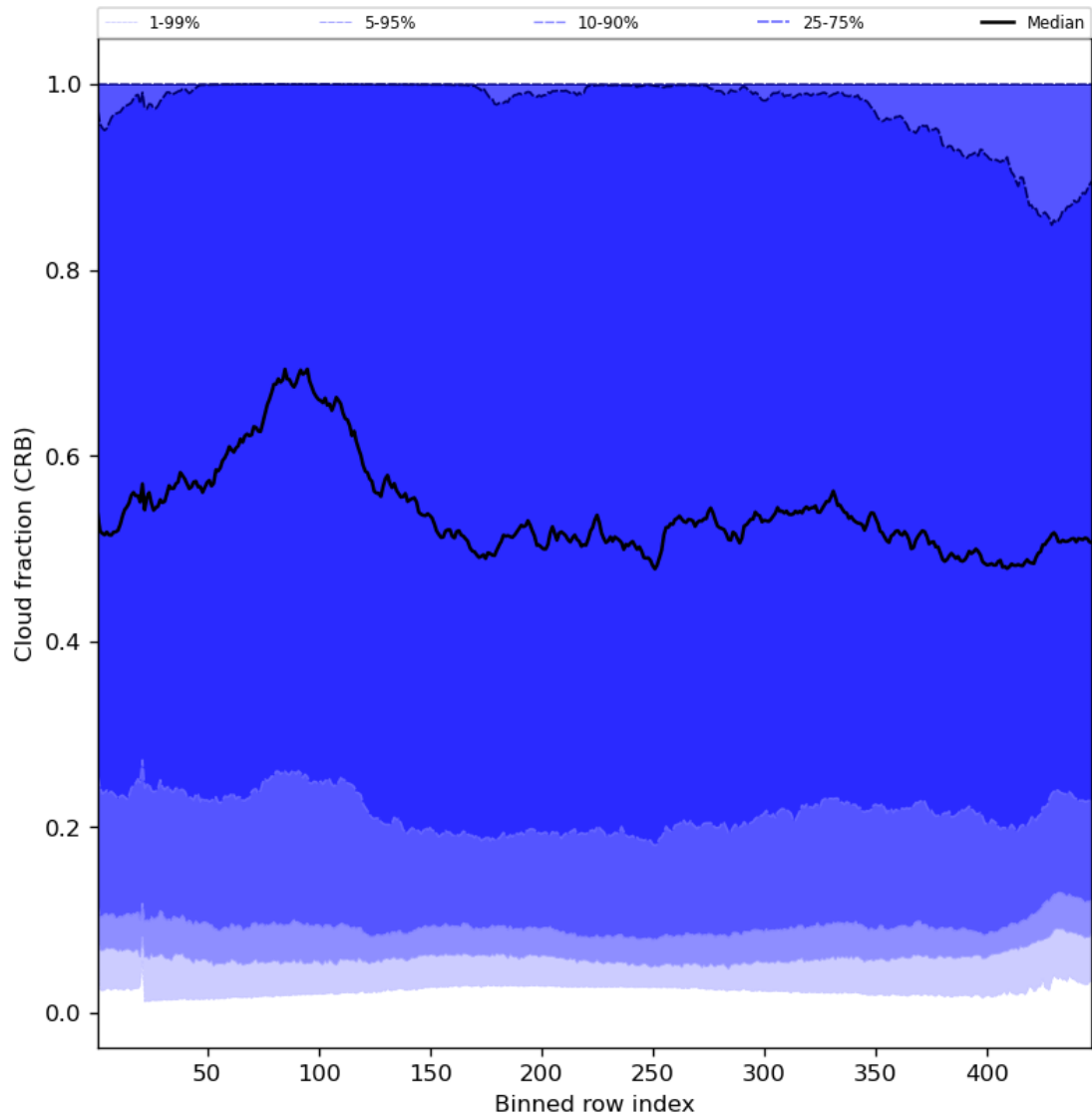
Figure 58: Along track statistics of “Cloud fraction (CRB)” for 2023-08-09 to 2023-08-10
