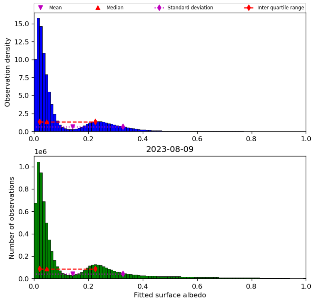
Figure 45: Histogram of “Fitted surface albedo” for 2023-08-09 to 2023-08-10
