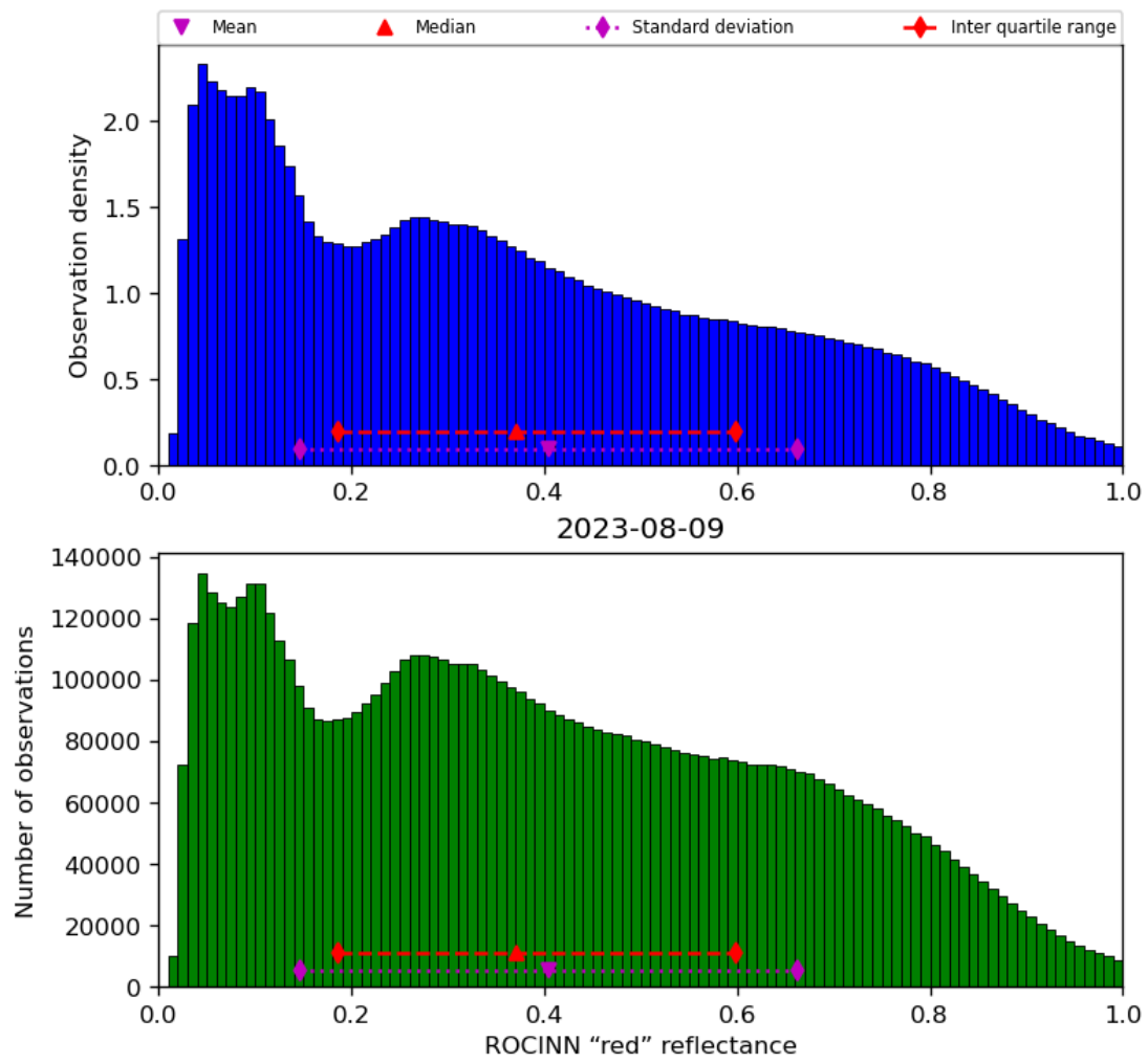
Figure 53: Histogram of “ROCINN “red” reflectance” for 2023-08-09 to 2023-08-10
