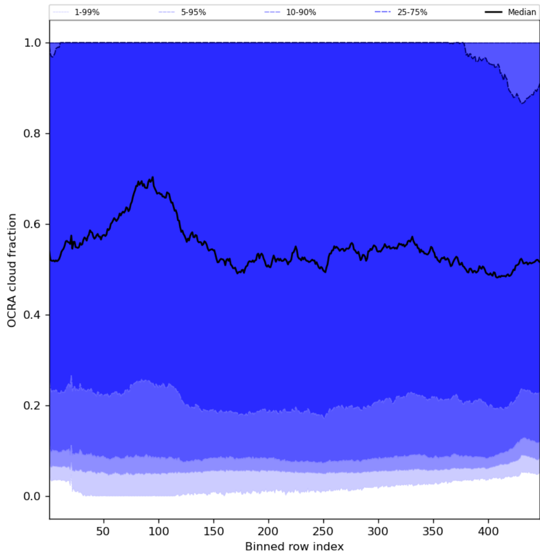
Figure 66: Along track statistics of “OCRA cloud fraction” for 2023-08-09 to 2023-08-10
