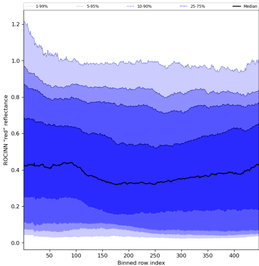
Figure 69: Along track statistics of “ROCINN “red” reflectance” for 2023-08-09 to 2023-08-10
