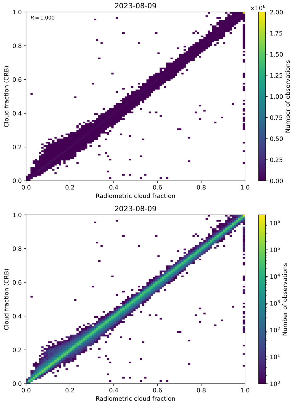
Figure 73: Scatter density plot of “Radiometric cloud fraction” against “Cloud fraction (CRB)” for 2023-08-09 to 2023-08-10.
