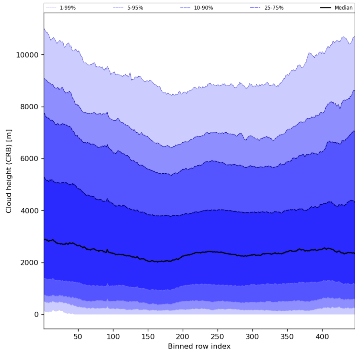
Figure 59: Along track statistics of “Cloud height (CRB)” for 2023-08-11 to 2023-08-13
