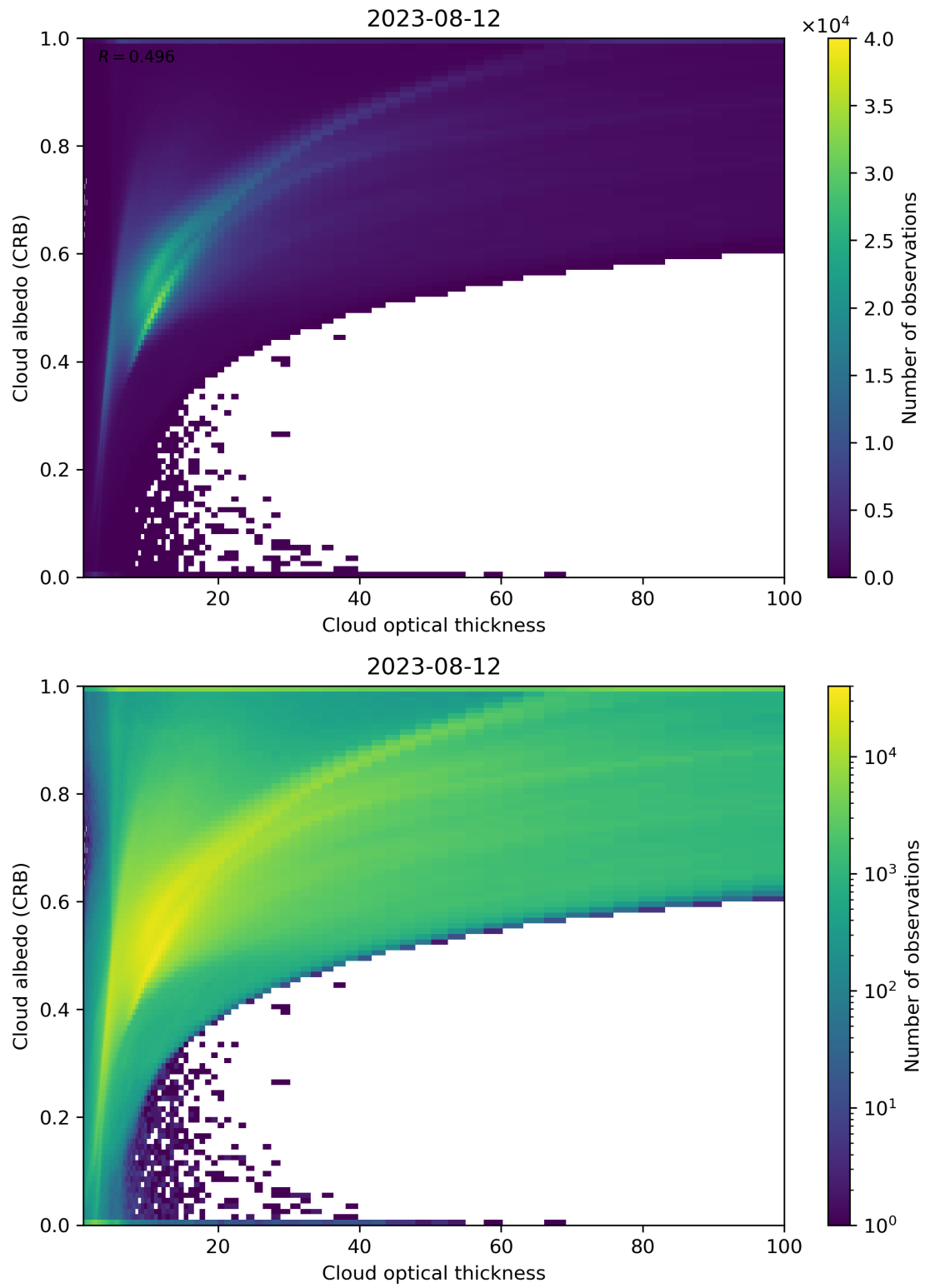
Figure 82: Scatter density plot of “Cloud optical thickness” against “Cloud albedo (CRB)” for 2023-08-11 to 2023-08-13.
