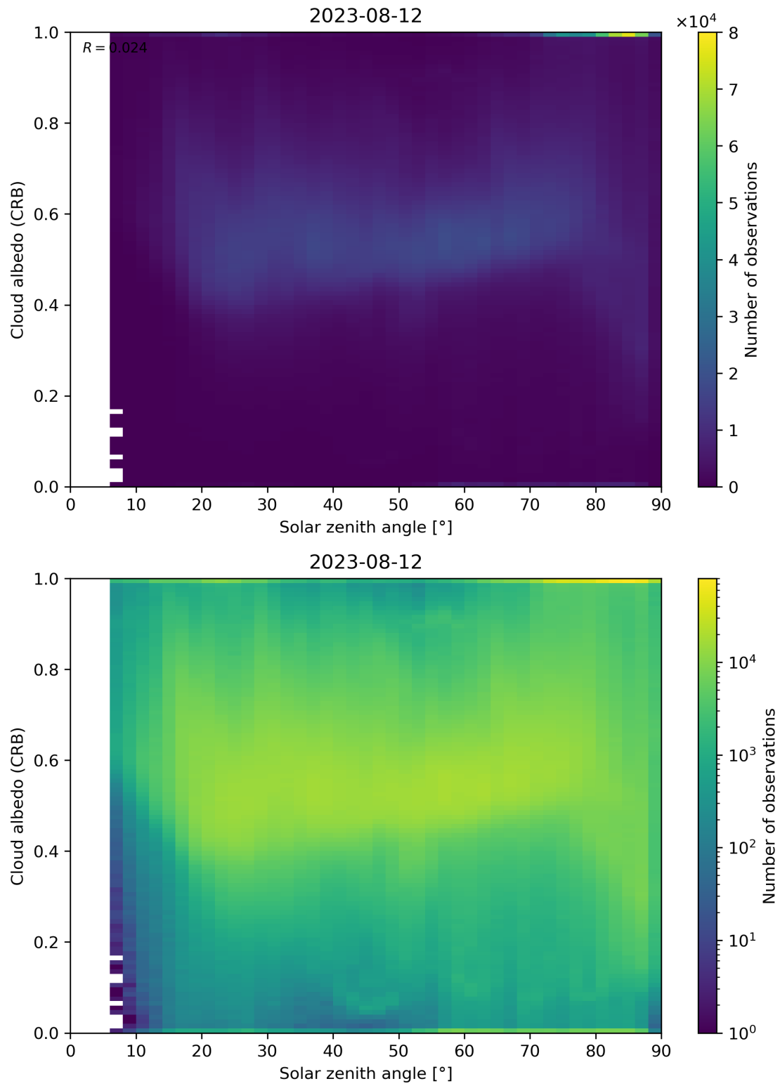
Figure 98: Scatter density plot of “Solar zenith angle” against “Cloud albedo (CRB)” for 2023-08-11 to 2023-08-13.
