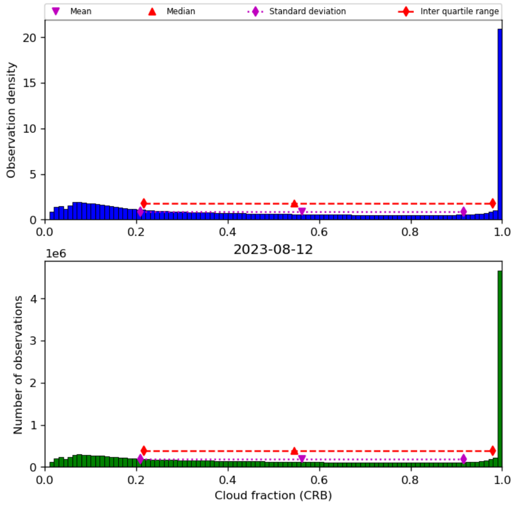
Figure 42: Histogram of “Cloud fraction (CRB)” for 2023-08-11 to 2023-08-13
