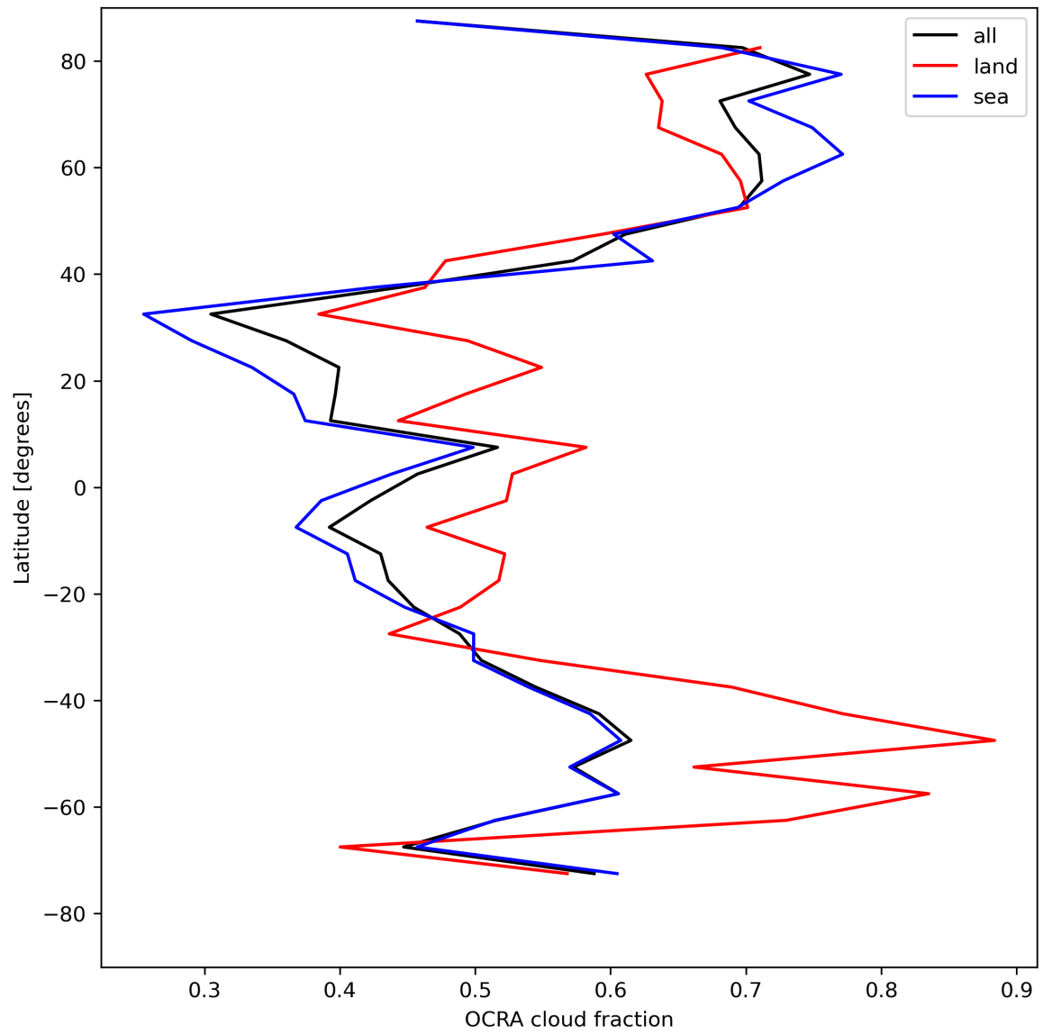
Figure 34: Zonal average of “OCRA cloud fraction” for 2023-08-11 to 2023-08-13.
