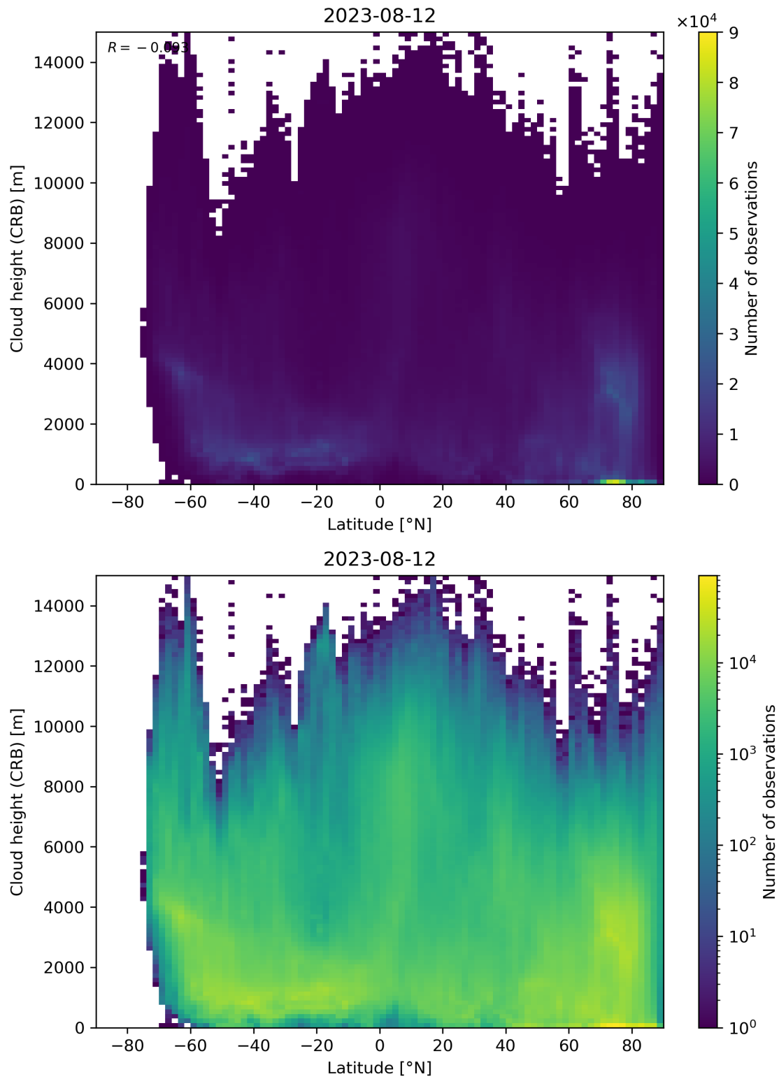
Figure 95: Scatter density plot of “Latitude” against “Cloud height (CRB)” for 2023-08-11 to 2023-08-13.
