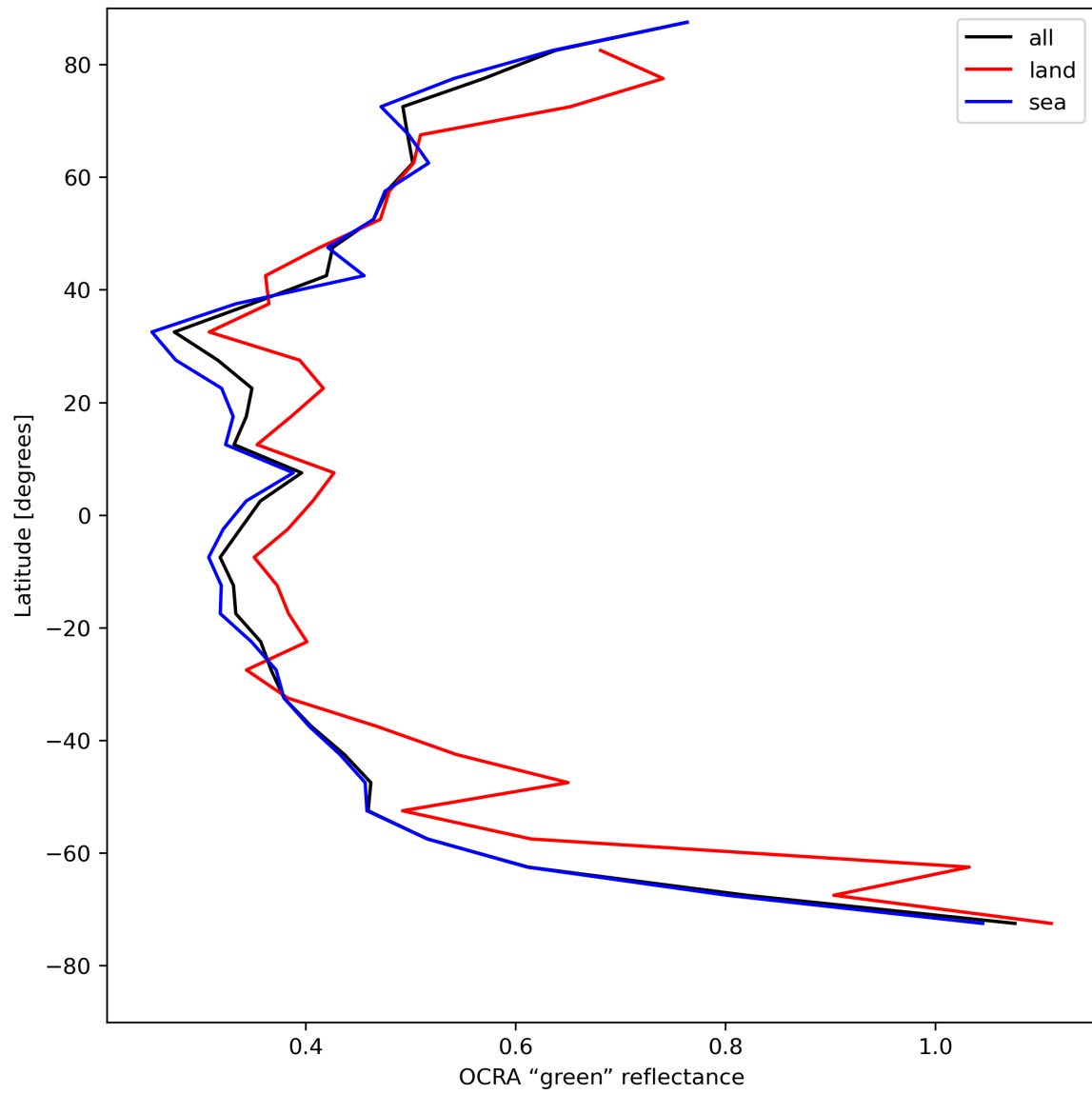
Figure 36: Zonal average of “OCRA “green” reflectance” for 2023-08-11 to 2023-08-13.
