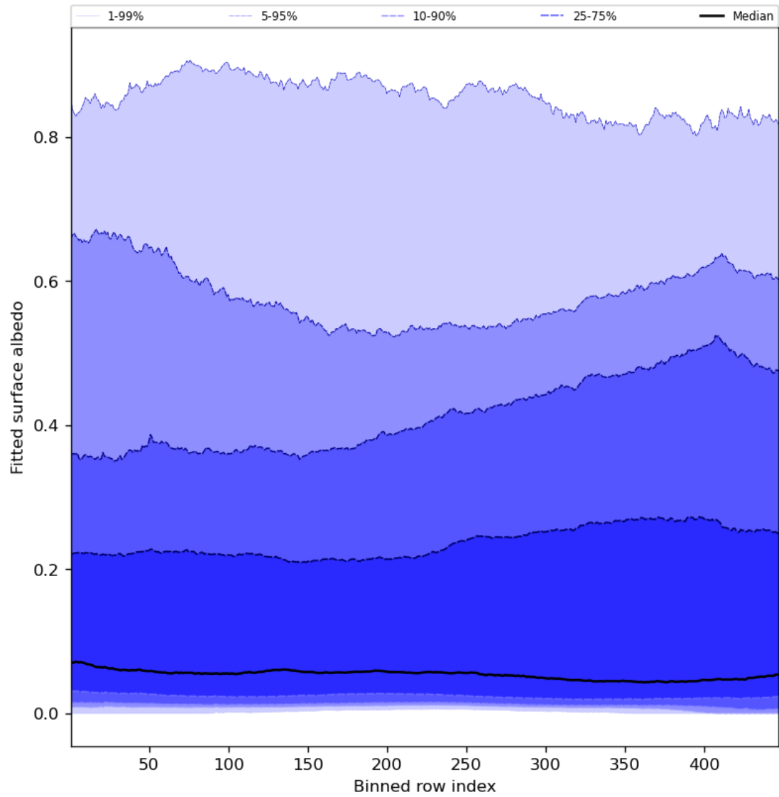
Figure 61: Along track statistics of “Fitted surface albedo” for 2023-08-11 to 2023-08-13
