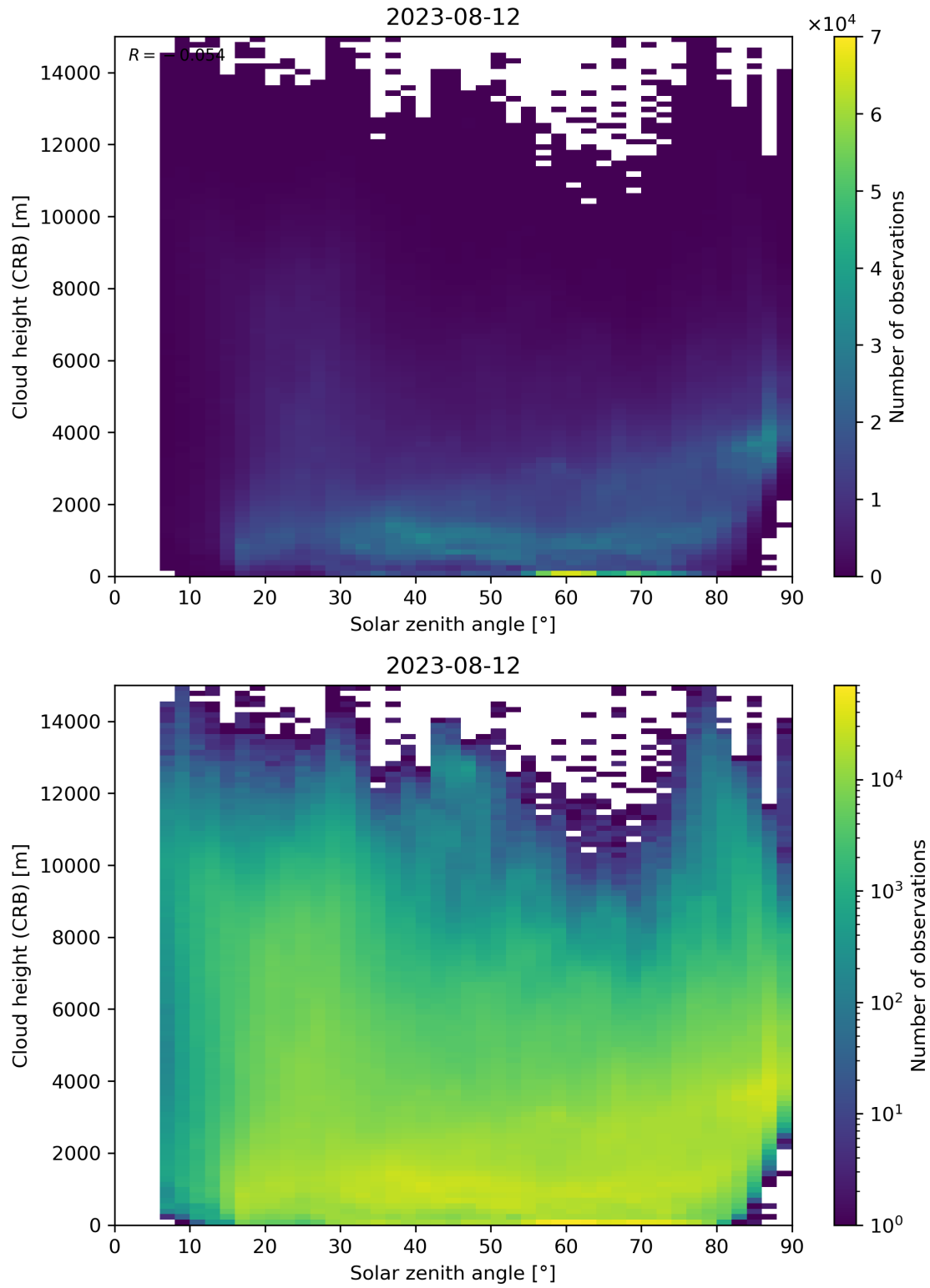
Figure 102: Scatter density plot of “Solar zenith angle” against “Cloud height (CRB)” for 2023-08-11 to 2023-08-13.
