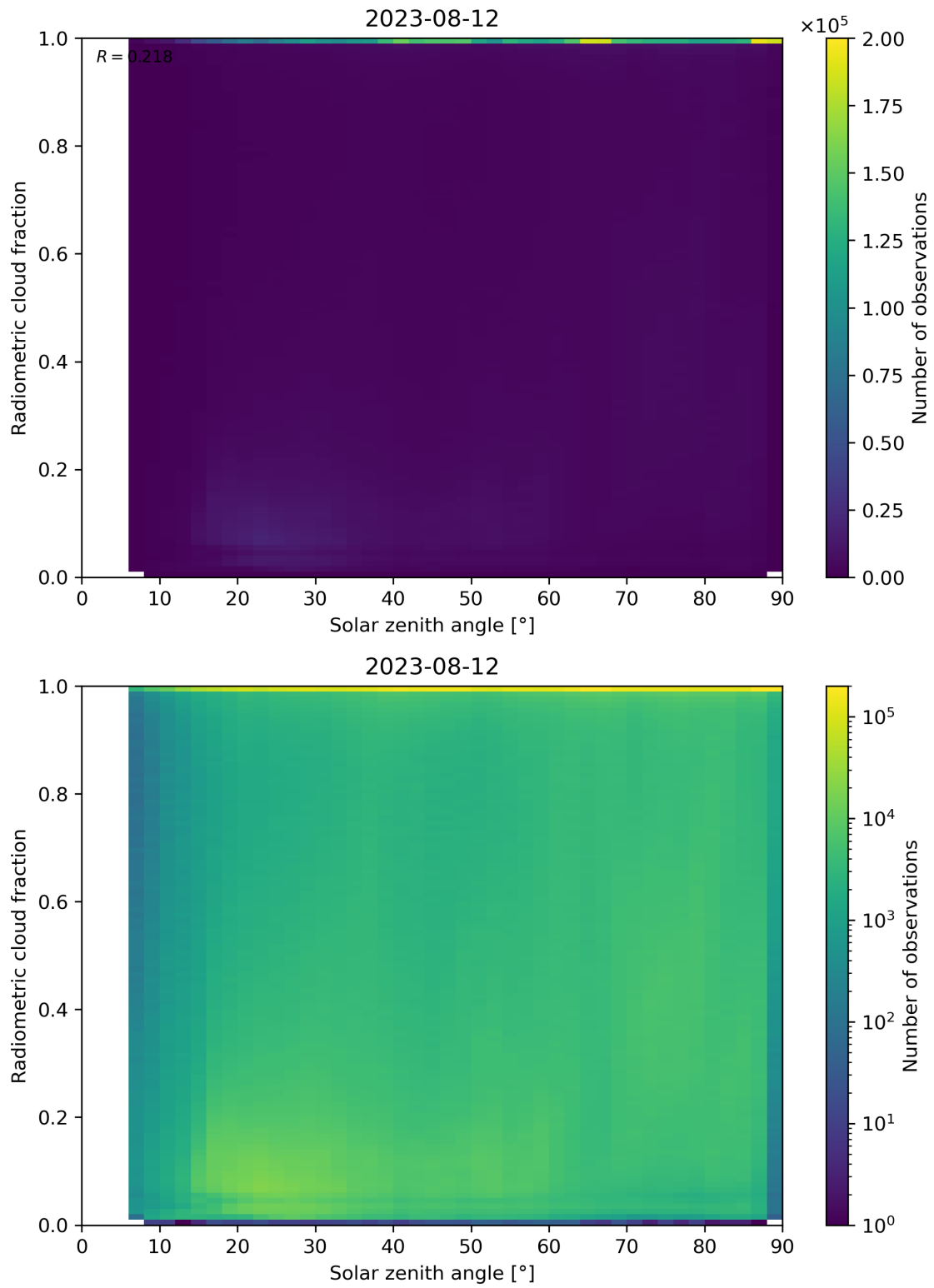
Figure 99: Scatter density plot of “Solar zenith angle” against “Radiometric cloud fraction” for 2023-08-11 to 2023-08-13.
