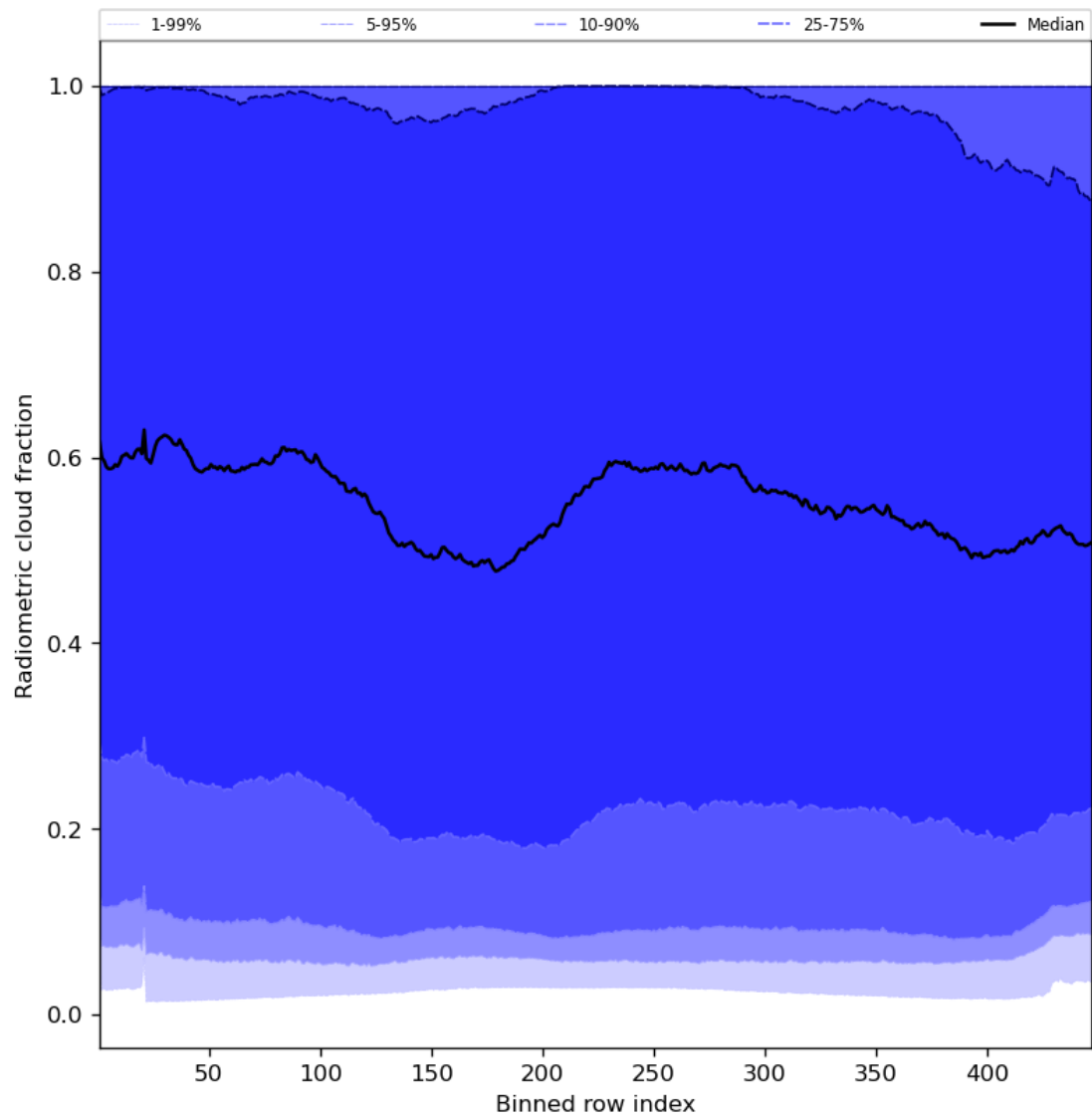
Figure 55: Along track statistics of “Radiometric cloud fraction” for 2023-08-11 to 2023-08-13
