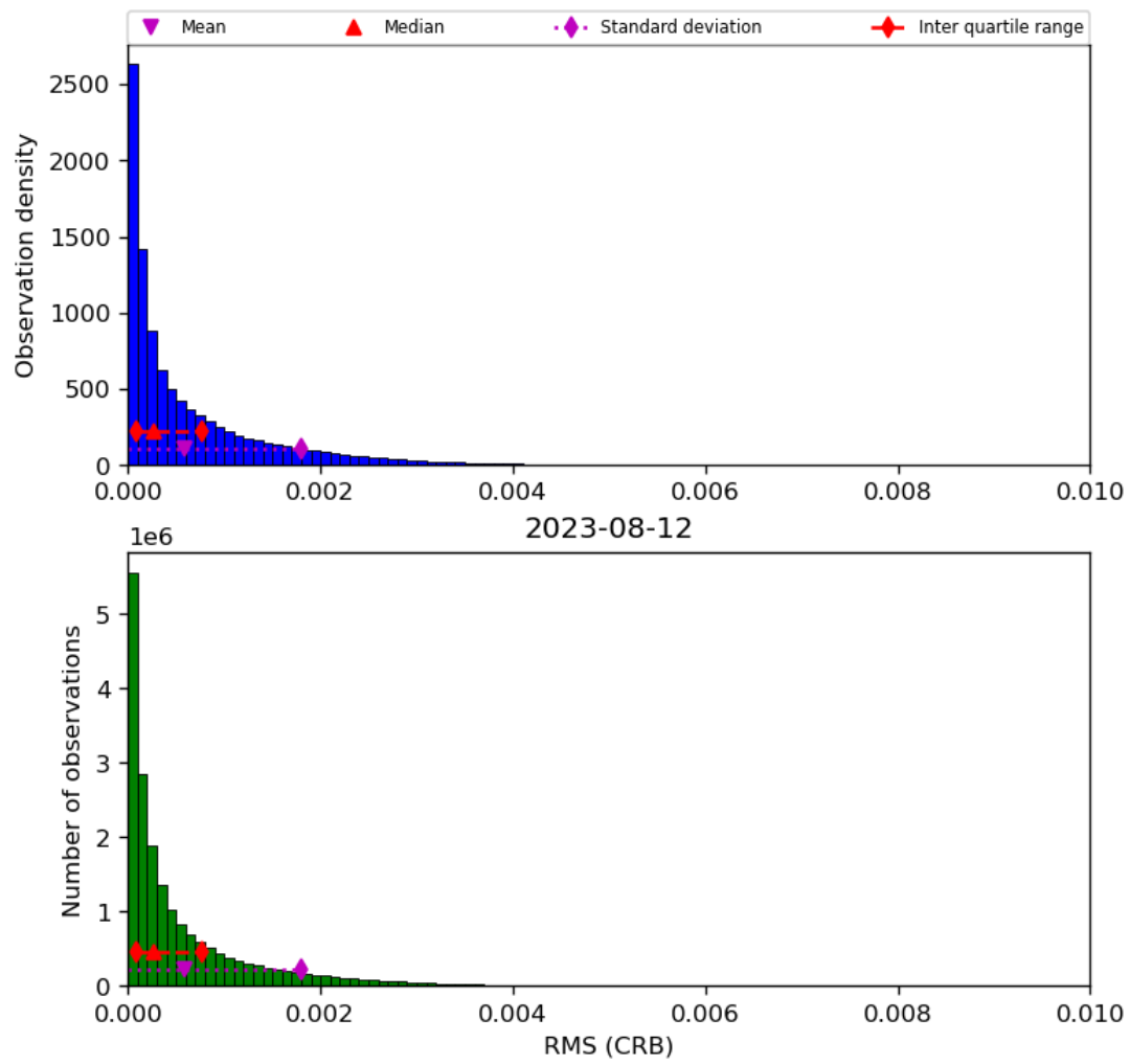
Figure 48: Histogram of “RMS (CRB)” for 2023-08-11 to 2023-08-13
