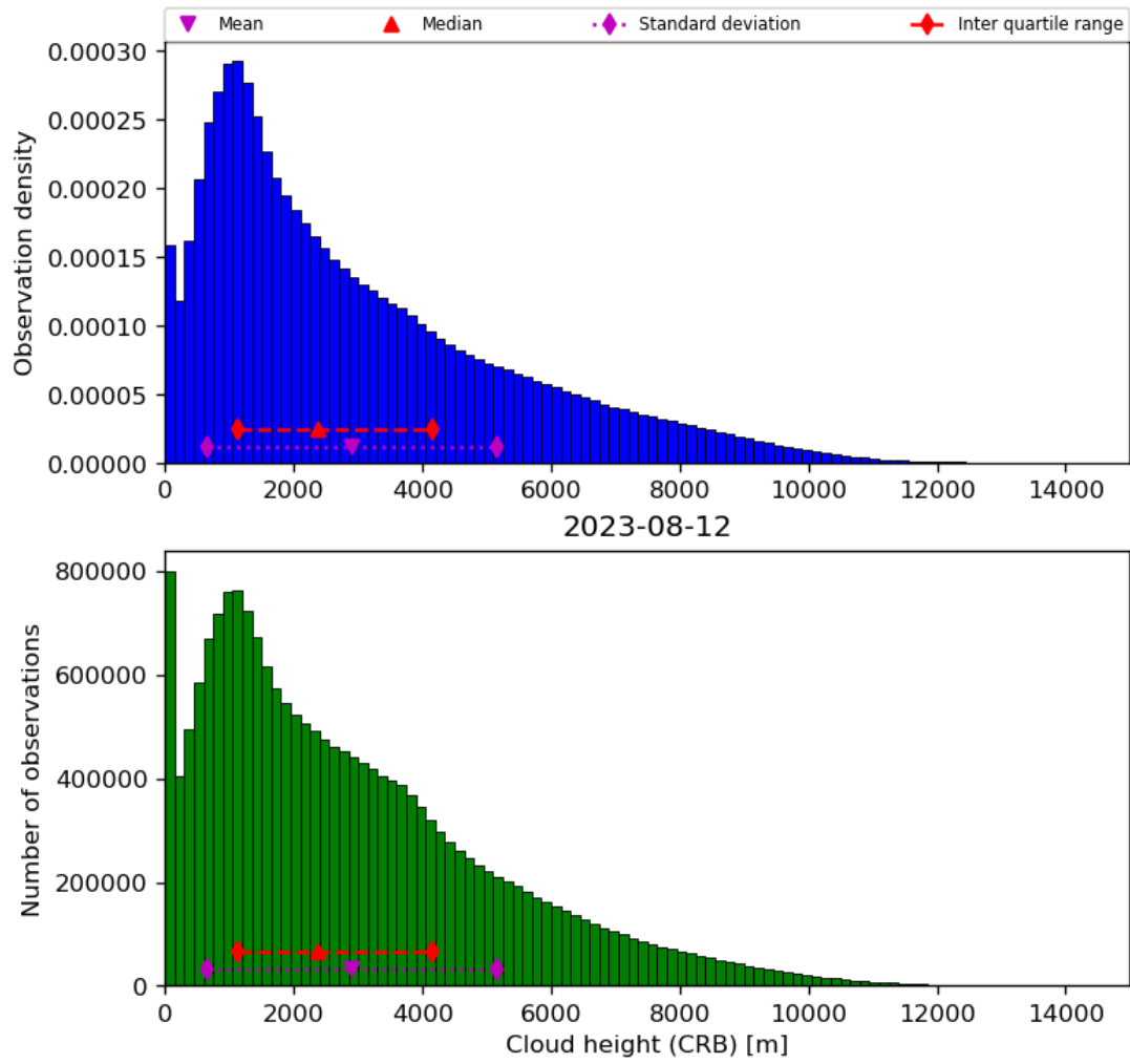
Figure 43: Histogram of “Cloud height (CRB)” for 2023-08-11 to 2023-08-13
