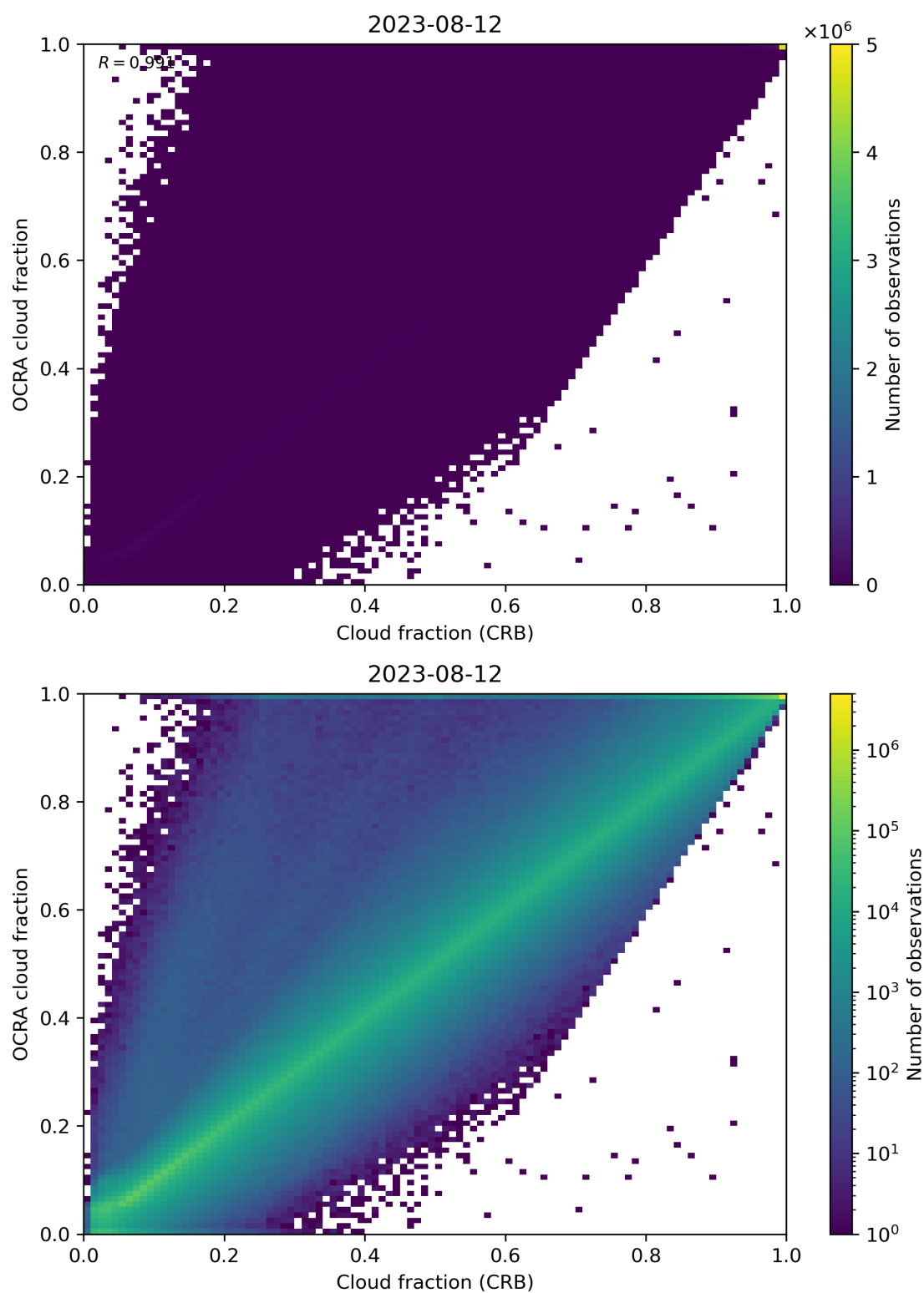
Figure 78: Scatter density plot of “Cloud fraction (CRB)” against “OCRA cloud fraction” for 2023-08-11 to 2023-08-13.
