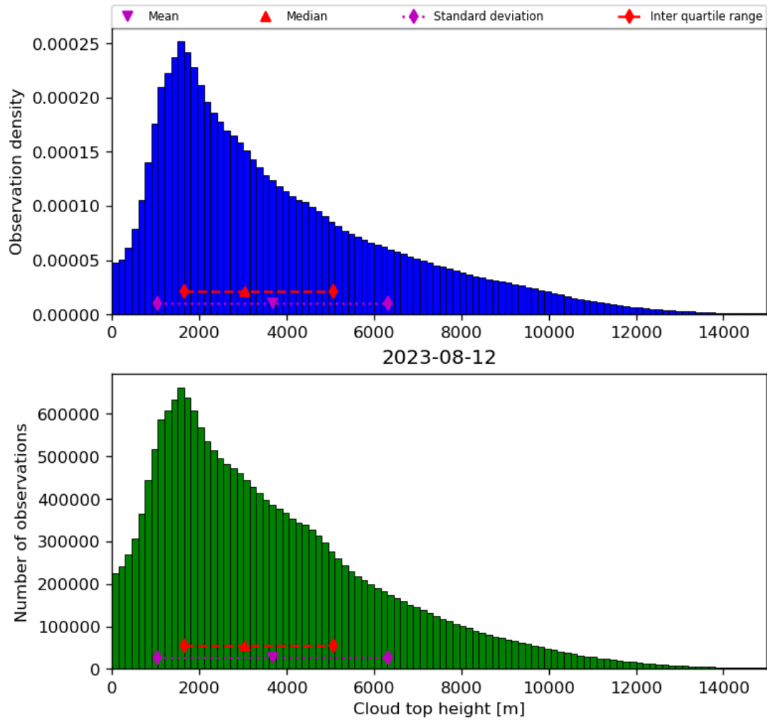
Figure 40: Histogram of “Cloud top height” for 2023-08-11 to 2023-08-13
