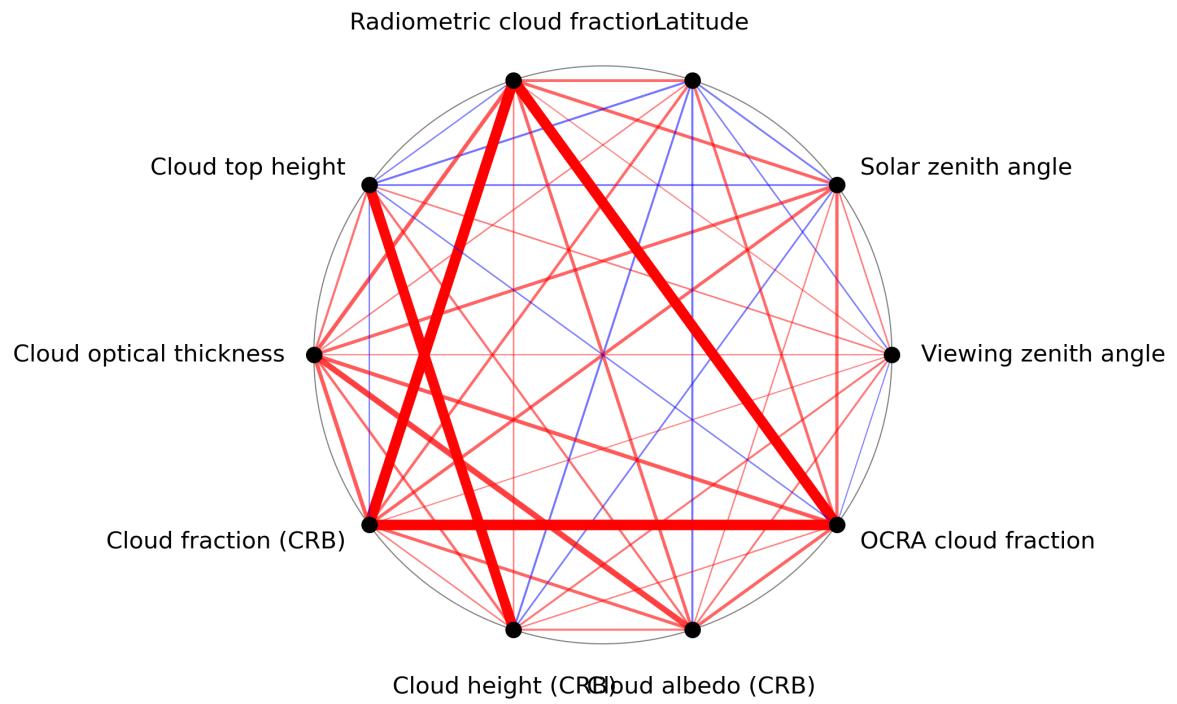
Figure 1: Map of correlation graph for 2023-08-11 to 2023-08-13.
