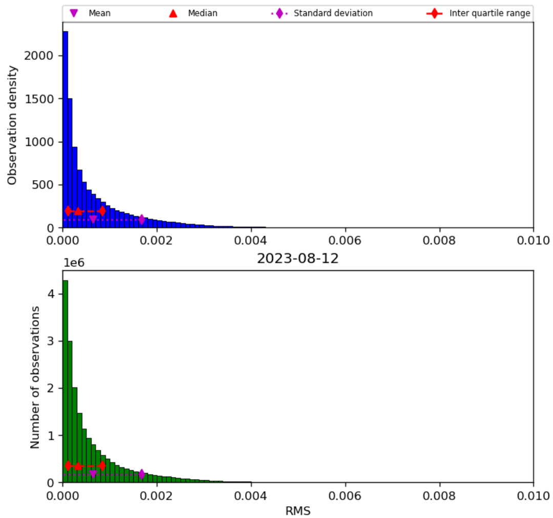
Figure 47: Histogram of “RMS” for 2023-08-11 to 2023-08-13
