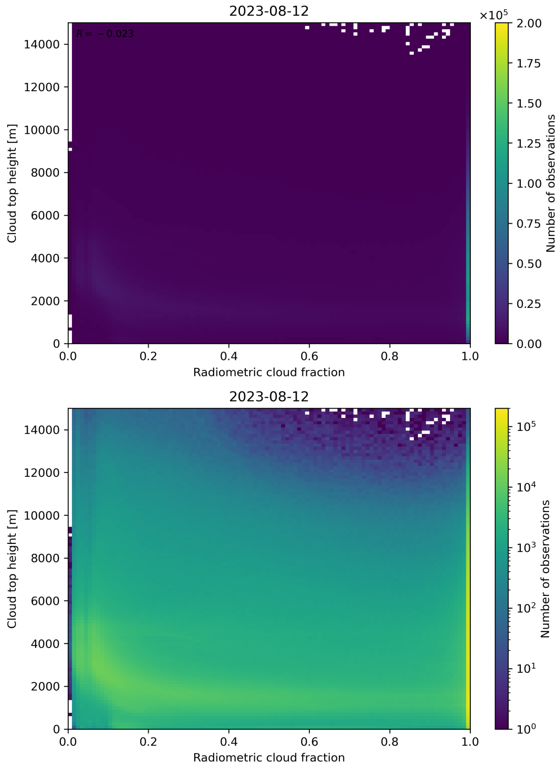
Figure 76: Scatter density plot of “Radiometric cloud fraction” against “Cloud top height” for 2023-08-11 to 2023-08-13.
