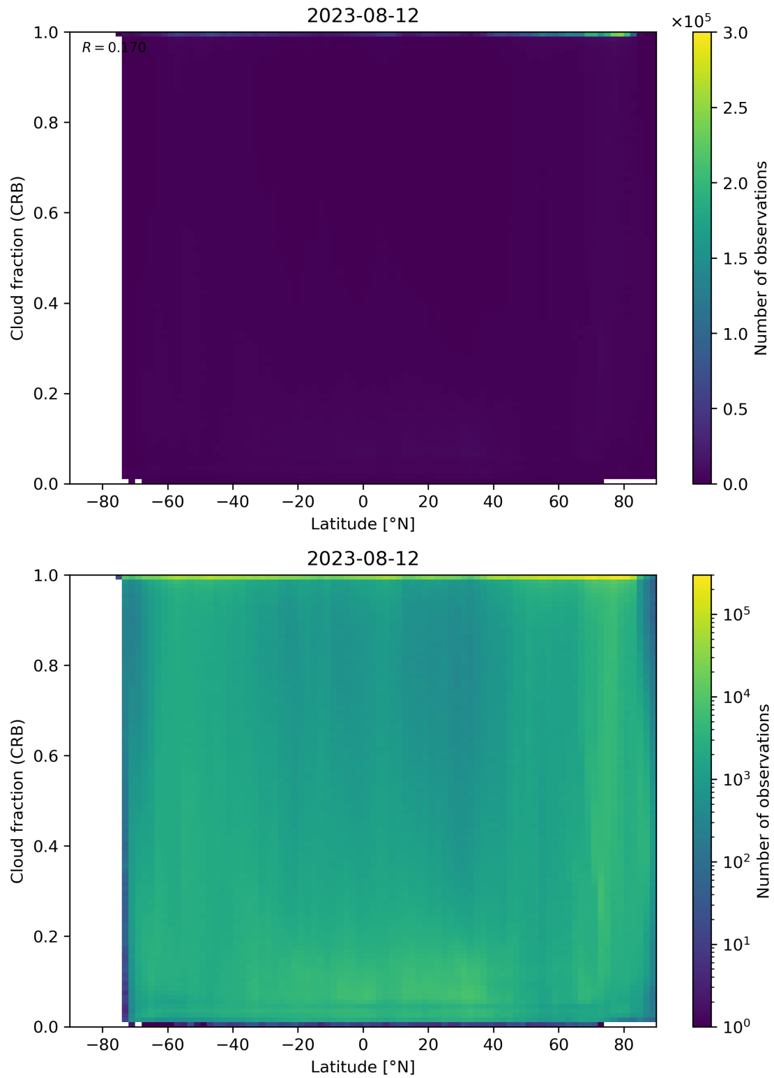
Figure 94: Scatter density plot of “Latitude” against “Cloud fraction (CRB)” for 2023-08-11 to 2023-08-13.
