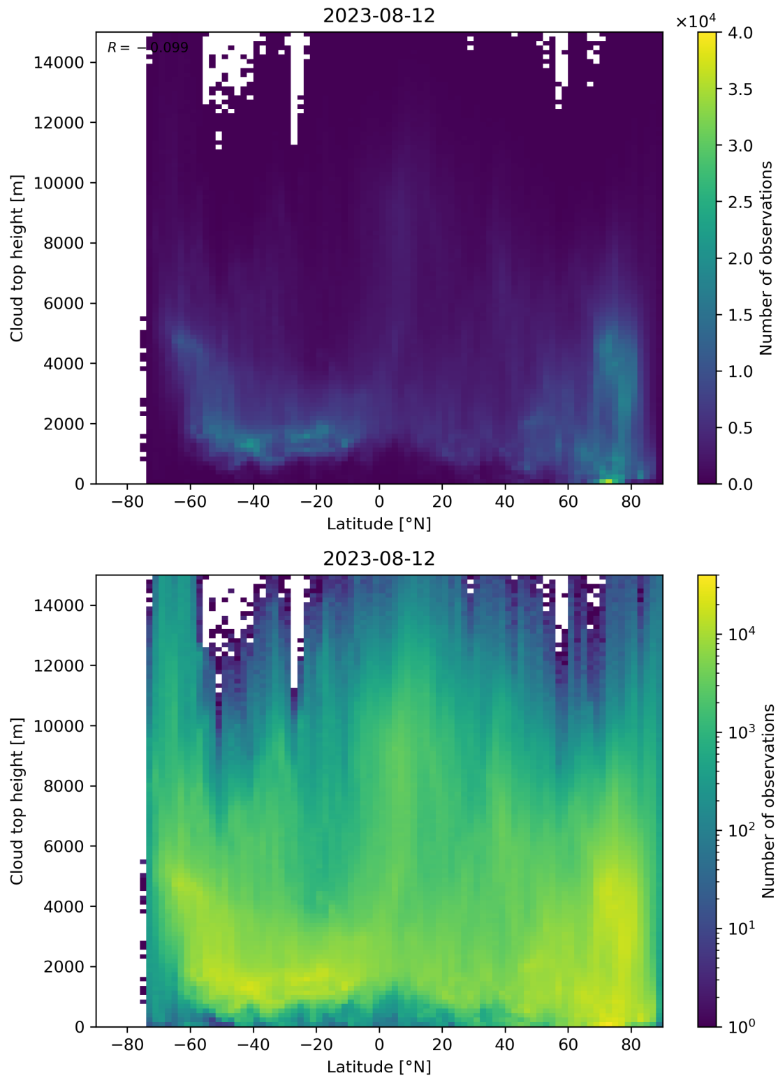
Figure 97: Scatter density plot of “Latitude” against “Cloud top height” for 2023-08-11 to 2023-08-13.
