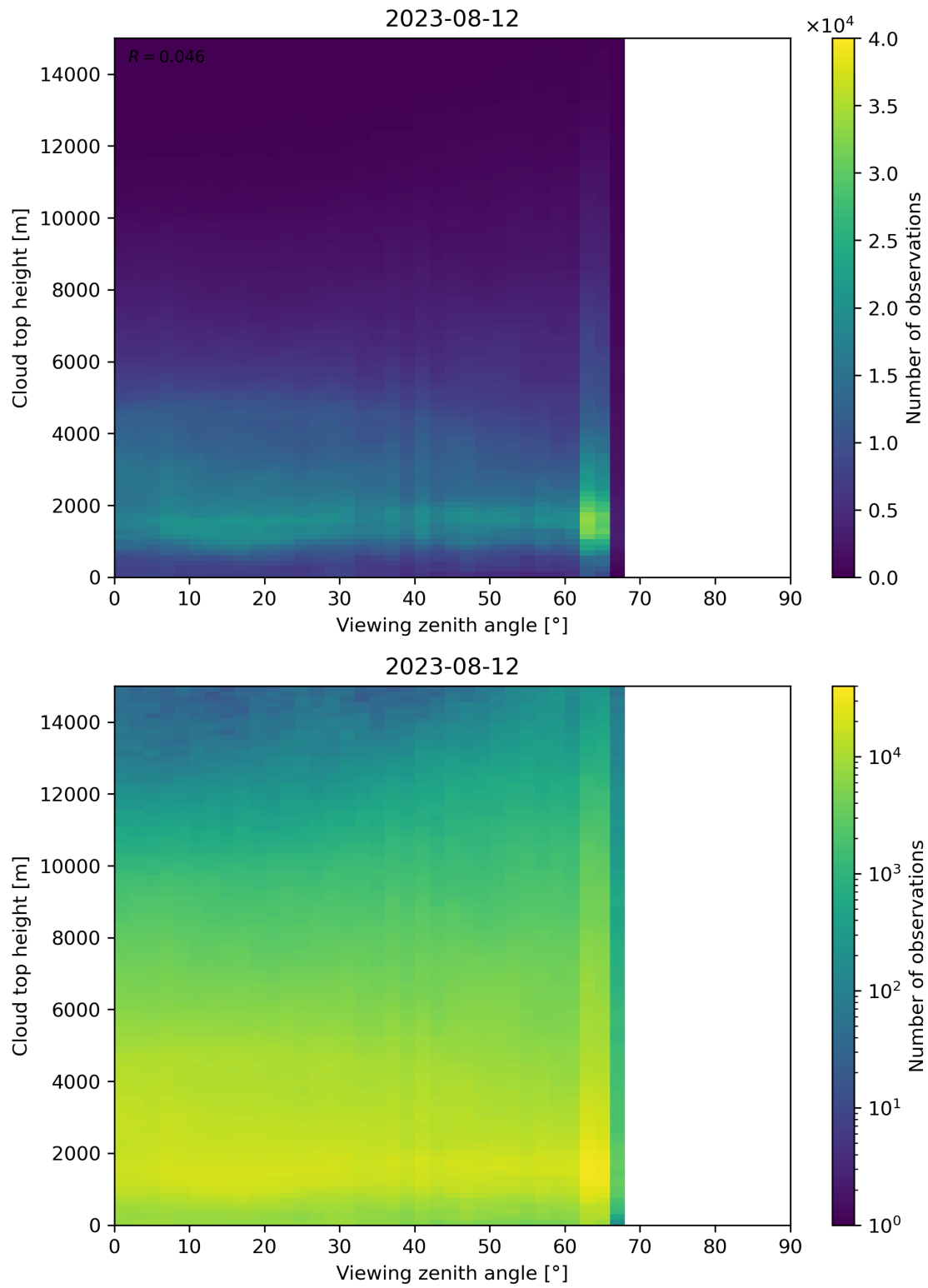
Figure 112: Scatter density plot of “Viewing zenith angle” against “Cloud top height” for 2023-08-11 to 2023-08-13.
