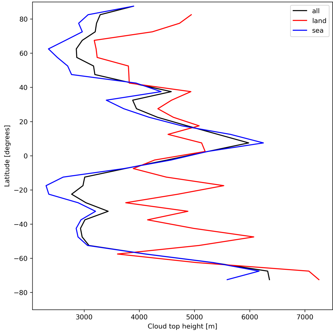
Figure 24: Zonal average of “Cloud top height” for 2023-08-11 to 2023-08-13.
