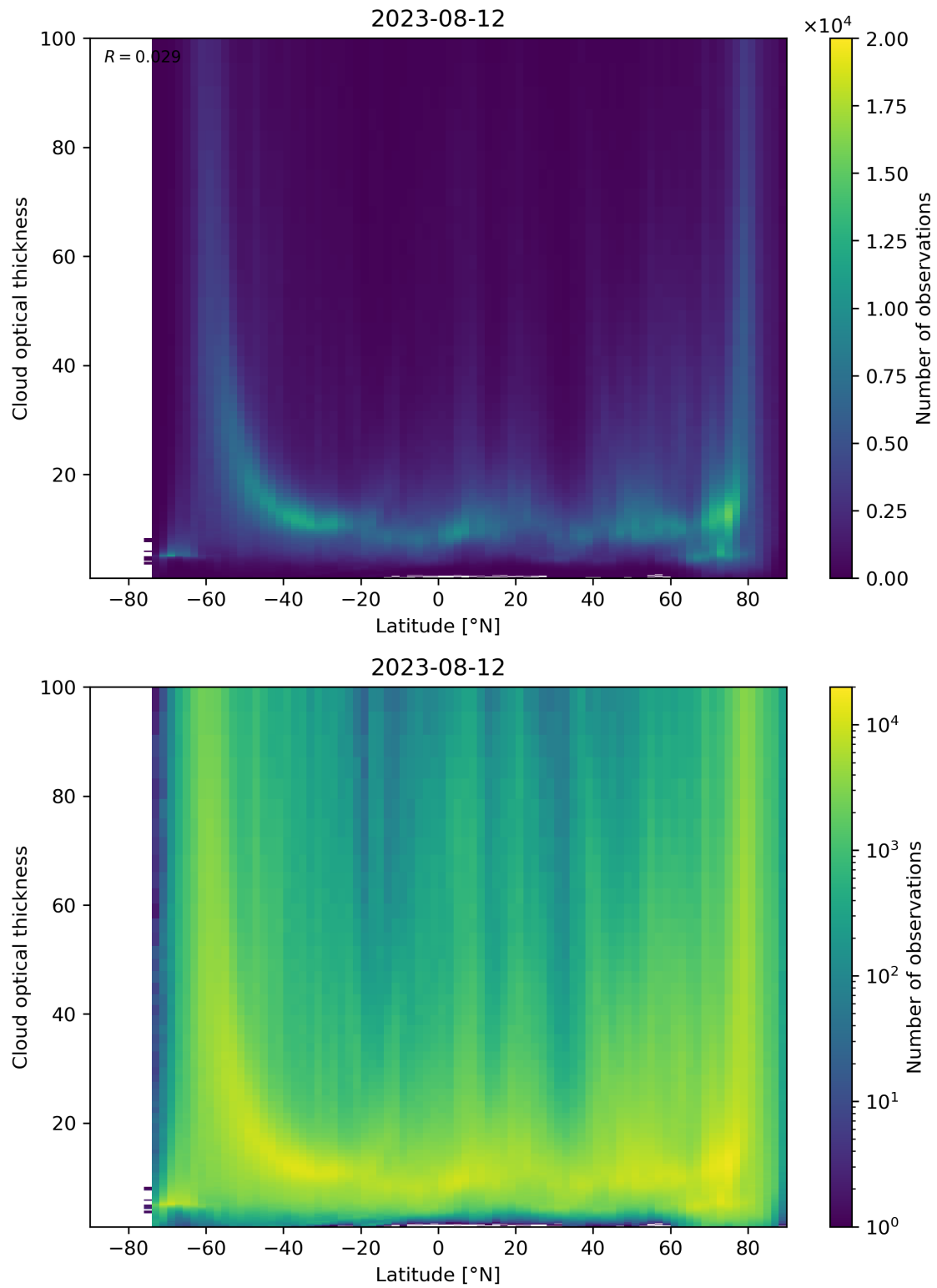
Figure 96: Scatter density plot of “Latitude” against “Cloud optical thickness” for 2023-08-11 to 2023-08-13.
