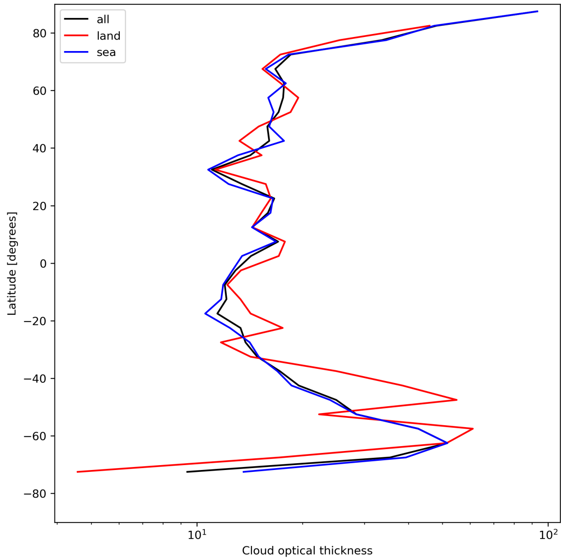
Figure 25: Zonal average of “Cloud optical thickness” for 2023-08-11 to 2023-08-13.
