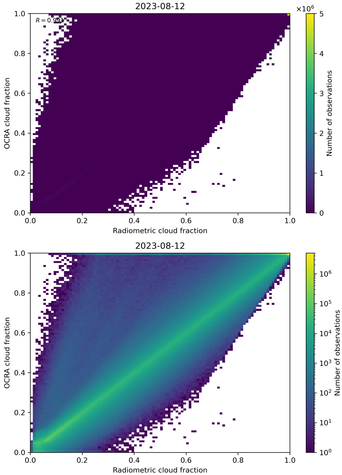
Figure 72: Scatter density plot of “Radiometric cloud fraction” against “OCRA cloud fraction” for 2023-08-11 to 2023-08-13.
