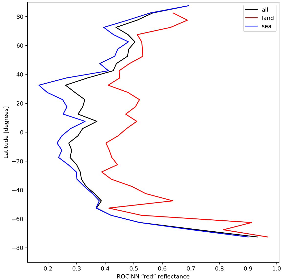
Figure 37: Zonal average of “ROCINN “red” reflectance” for 2023-08-11 to 2023-08-13.
