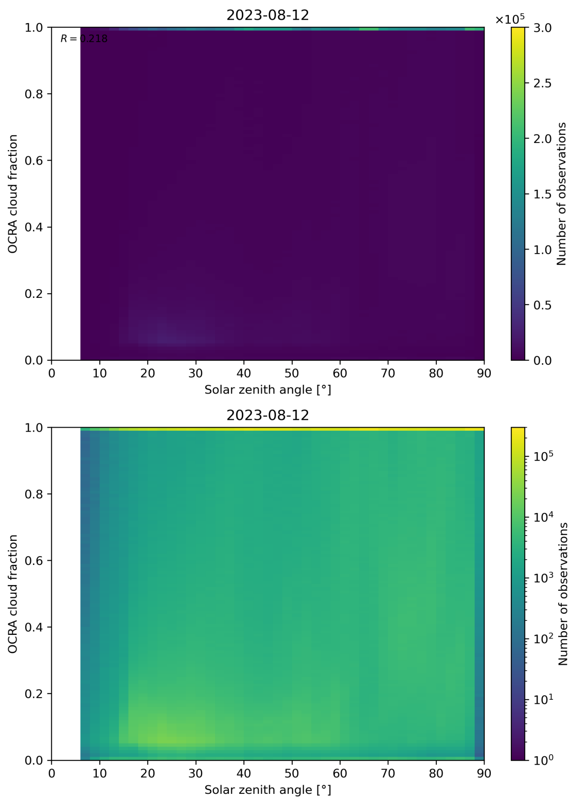
Figure 100: Scatter density plot of “Solar zenith angle” against “OCRA cloud fraction” for 2023-08-11 to 2023-08-13.
