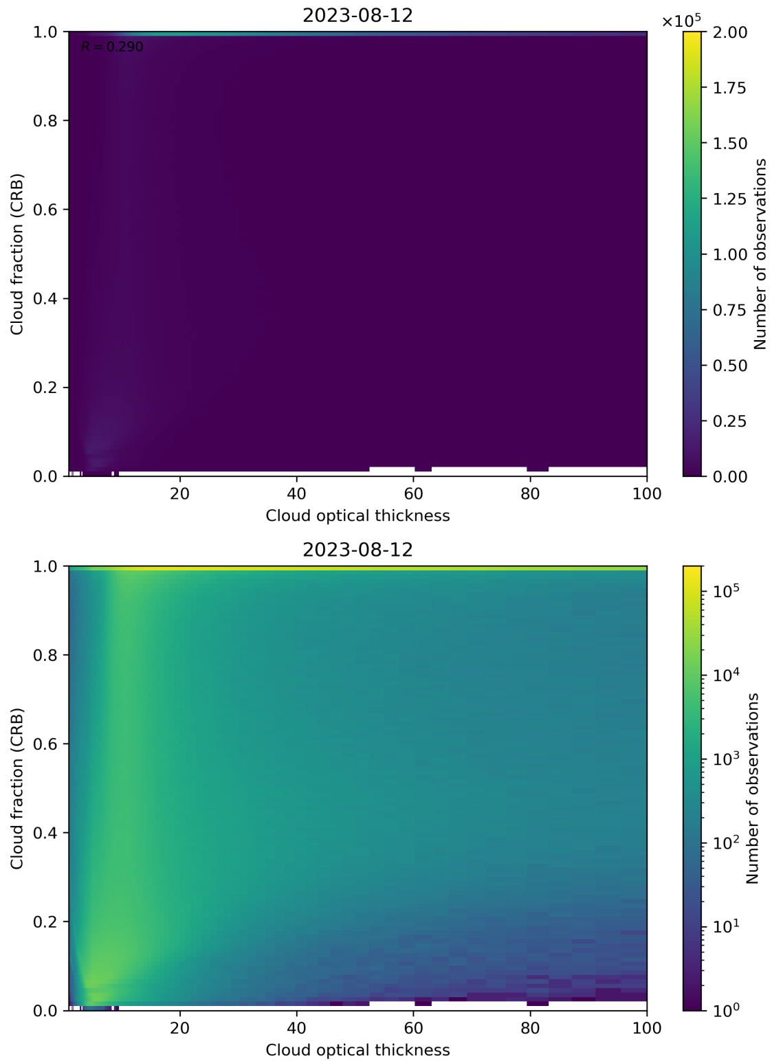
Figure 84: Scatter density plot of “Cloud optical thickness” against “Cloud fraction (CRB)” for 2023-08-11 to 2023-08-13.
