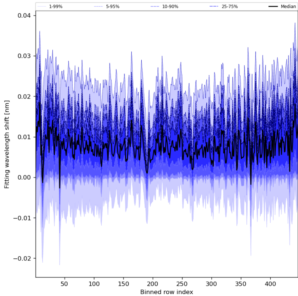
Figure 65: Along track statistics of “Fitting wavelength shift” for 2023-08-11 to 2023-08-13
