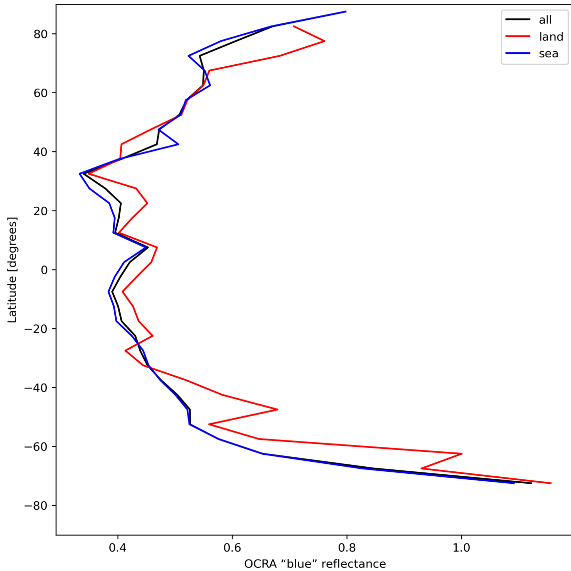
Figure 35: Zonal average of “OCRA “blue” reflectance” for 2023-08-11 to 2023-08-13.
