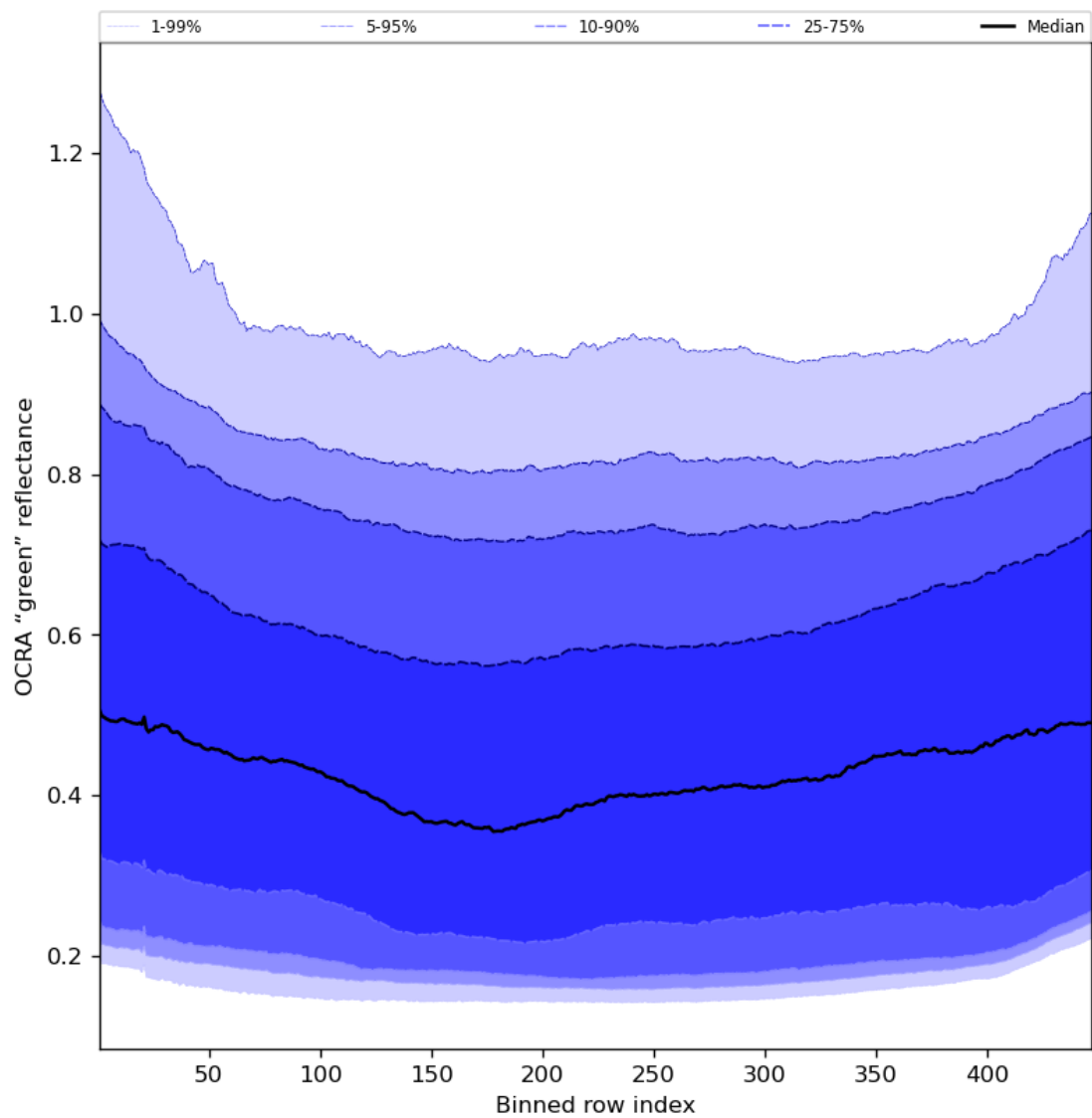
Figure 68: Along track statistics of “OCRA “green” reflectance” for 2023-08-11 to 2023-08-13
