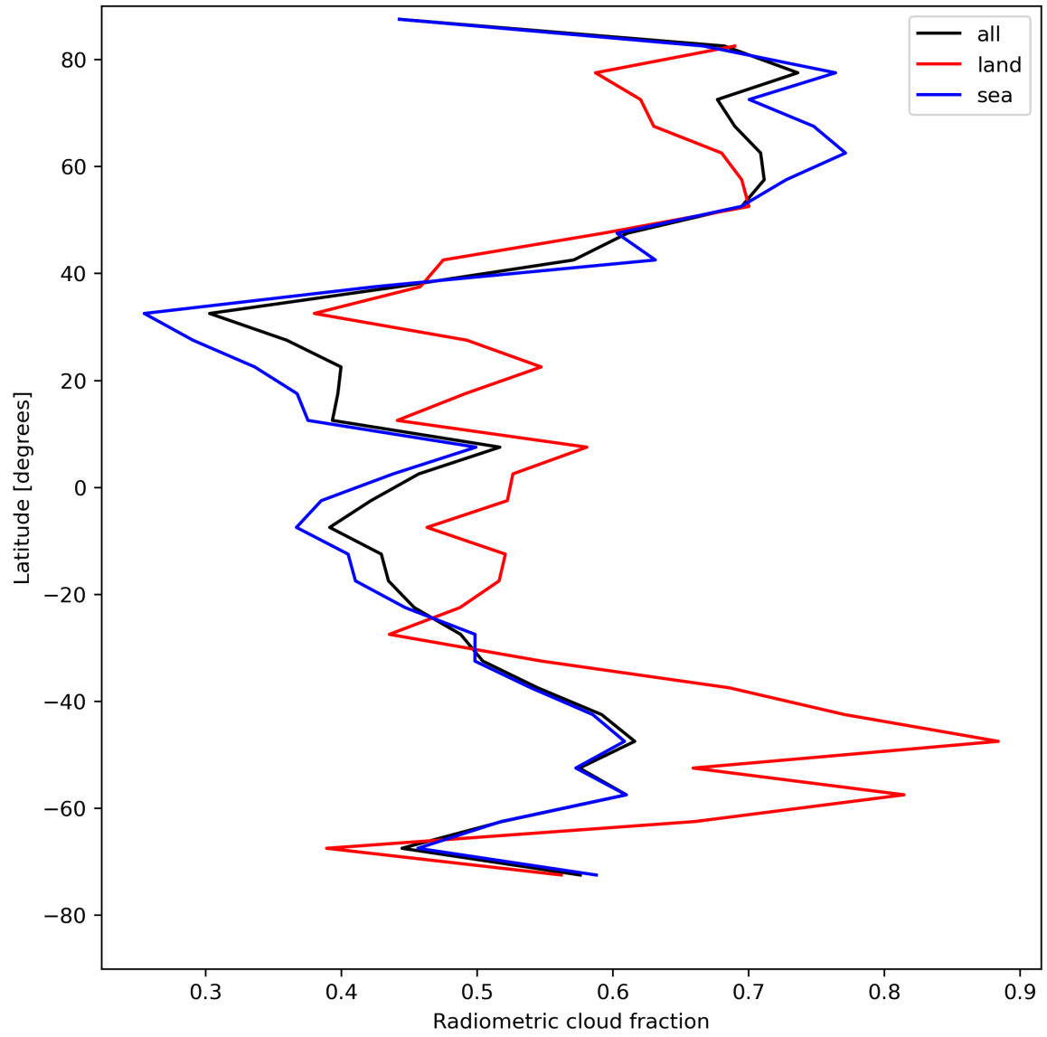
Figure 23: Zonal average of “Radiometric cloud fraction” for 2023-08-11 to 2023-08-13.
