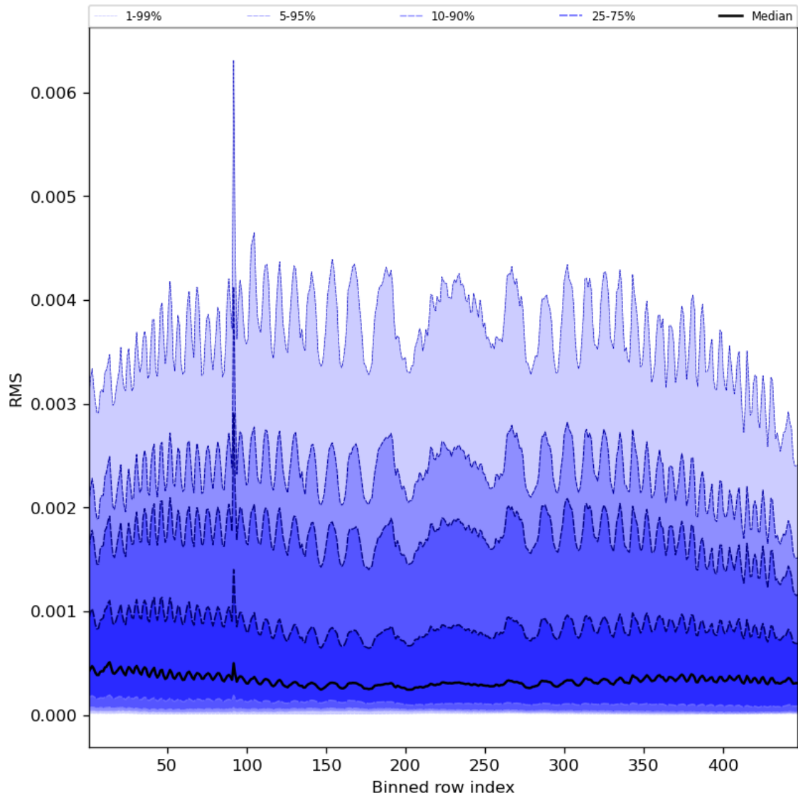
Figure 63: Along track statistics of “RMS” for 2023-08-11 to 2023-08-13
