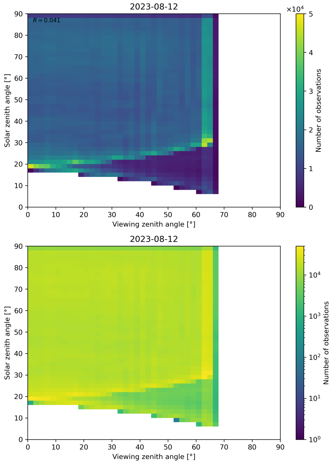
Figure 114: Scatter density plot of “Viewing zenith angle” against “Solar zenith angle” for 2023-08-11 to 2023-08-13.
