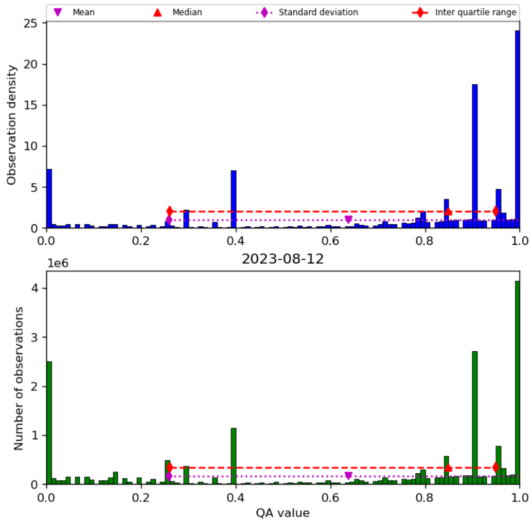
Figure 38: Histogram of “QA value” for 2023-08-11 to 2023-08-13
