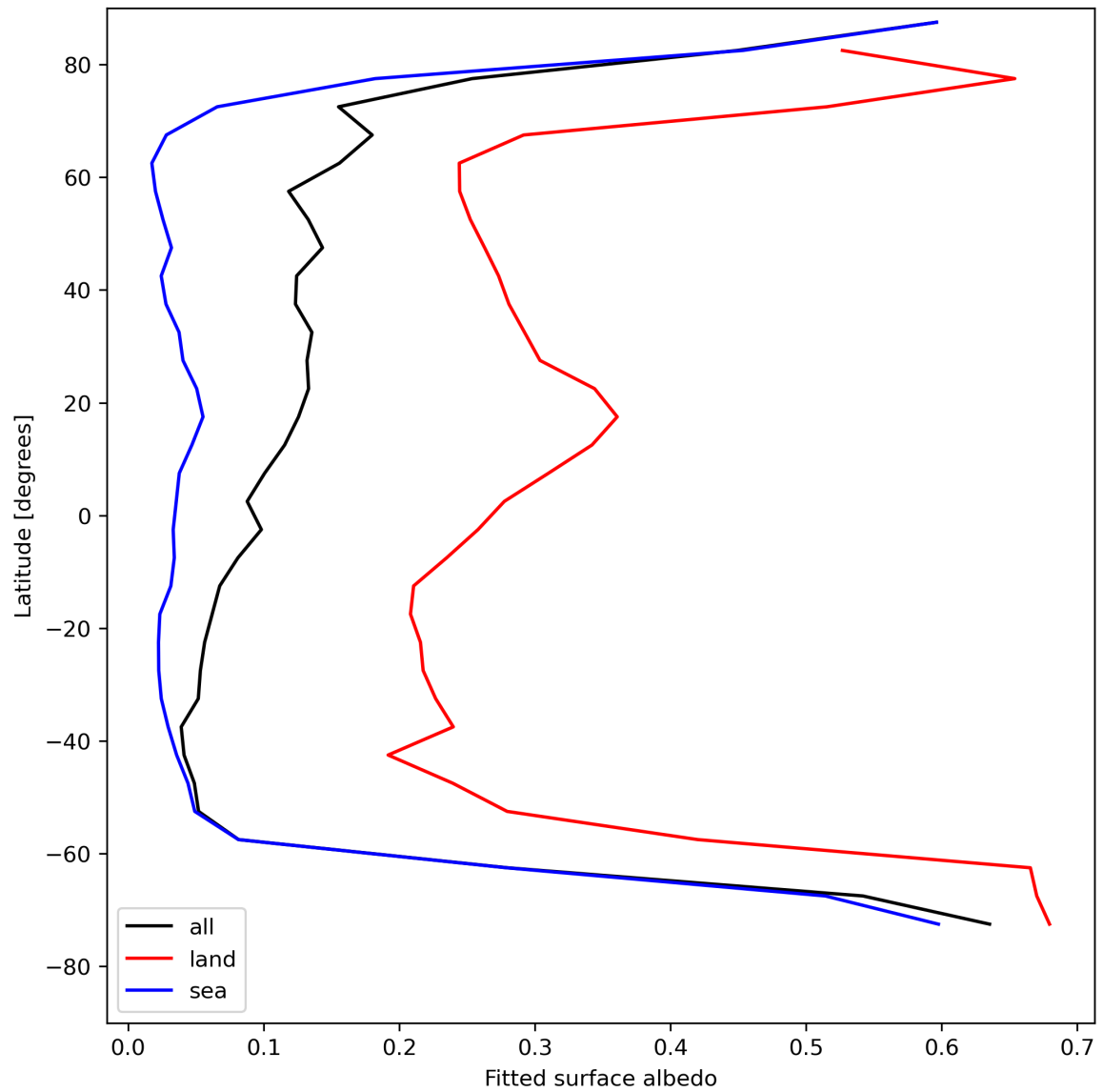
Figure 29: Zonal average of “Fitted surface albedo” for 2023-08-11 to 2023-08-13.
