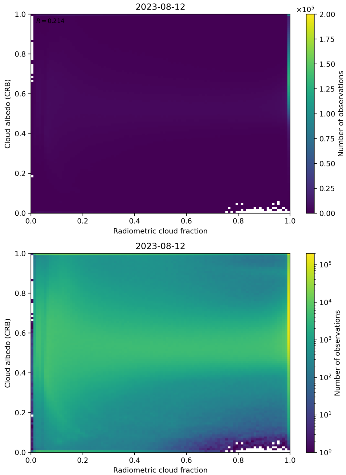
Figure 71: Scatter density plot of “Radiometric cloud fraction” against “Cloud albedo (CRB)” for 2023-08-11 to 2023-08-13.
