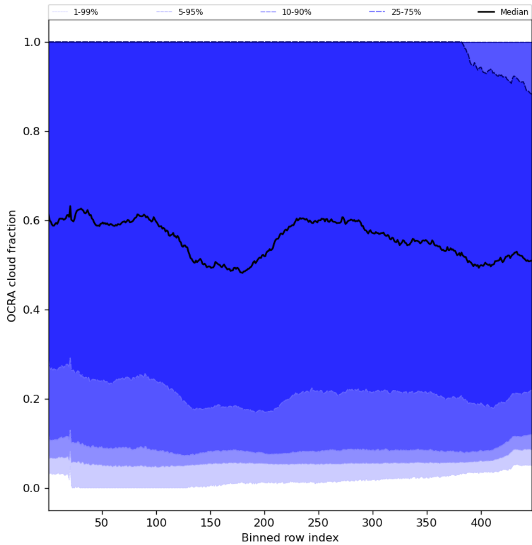
Figure 66: Along track statistics of “OCRA cloud fraction” for 2023-08-11 to 2023-08-13
