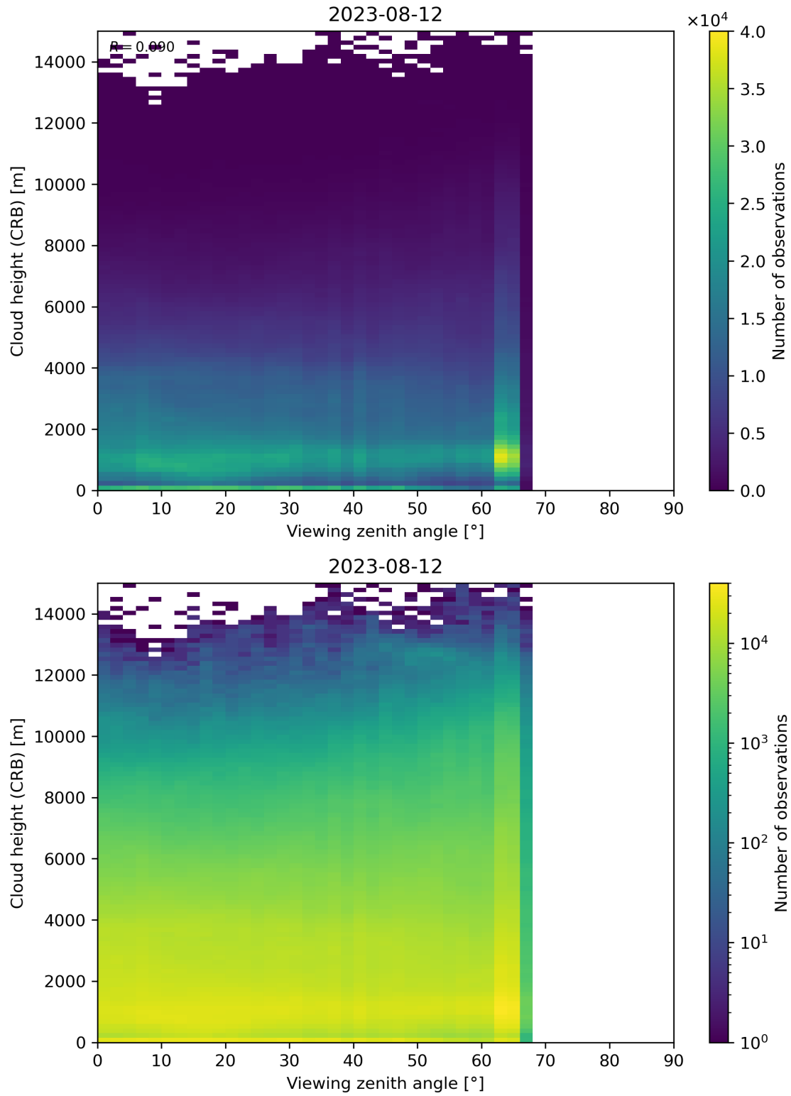
Figure 110: Scatter density plot of “Viewing zenith angle” against “Cloud height (CRB)” for 2023-08-11 to 2023-08-13.
