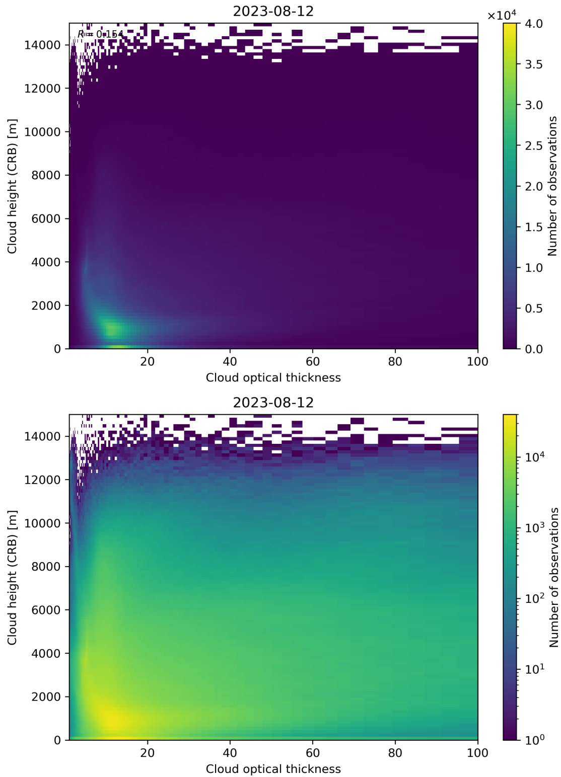
Figure 85: Scatter density plot of “Cloud optical thickness” against “Cloud height (CRB)” for 2023-08-11 to 2023-08-13.
