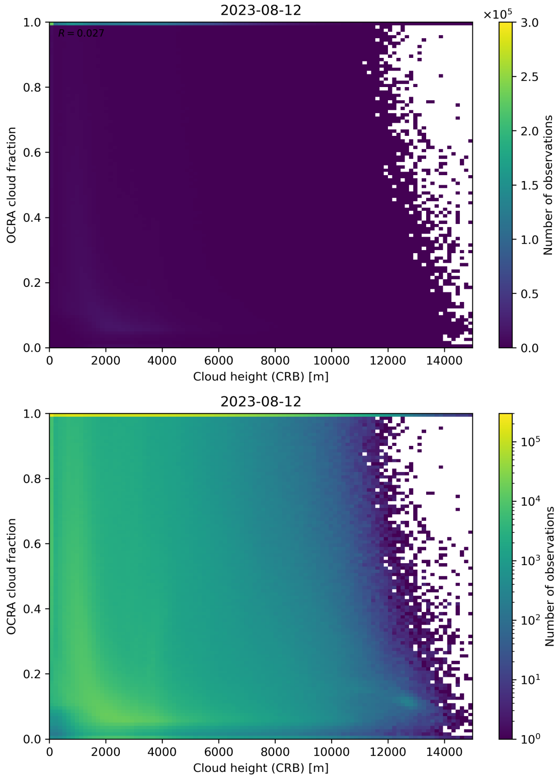
Figure 81: Scatter density plot of “Cloud height (CRB)” against “OCRA cloud fraction” for 2023-08-11 to 2023-08-13.
