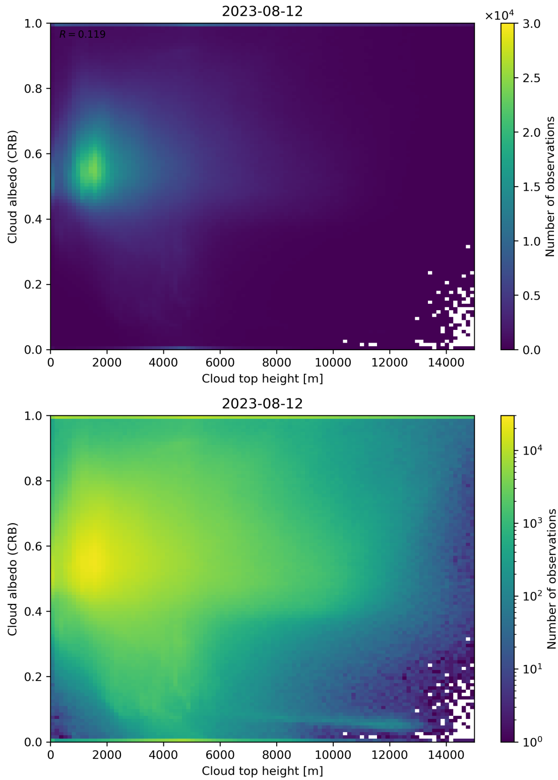
Figure 86: Scatter density plot of “Cloud top height” against “Cloud albedo (CRB)” for 2023-08-11 to 2023-08-13.
