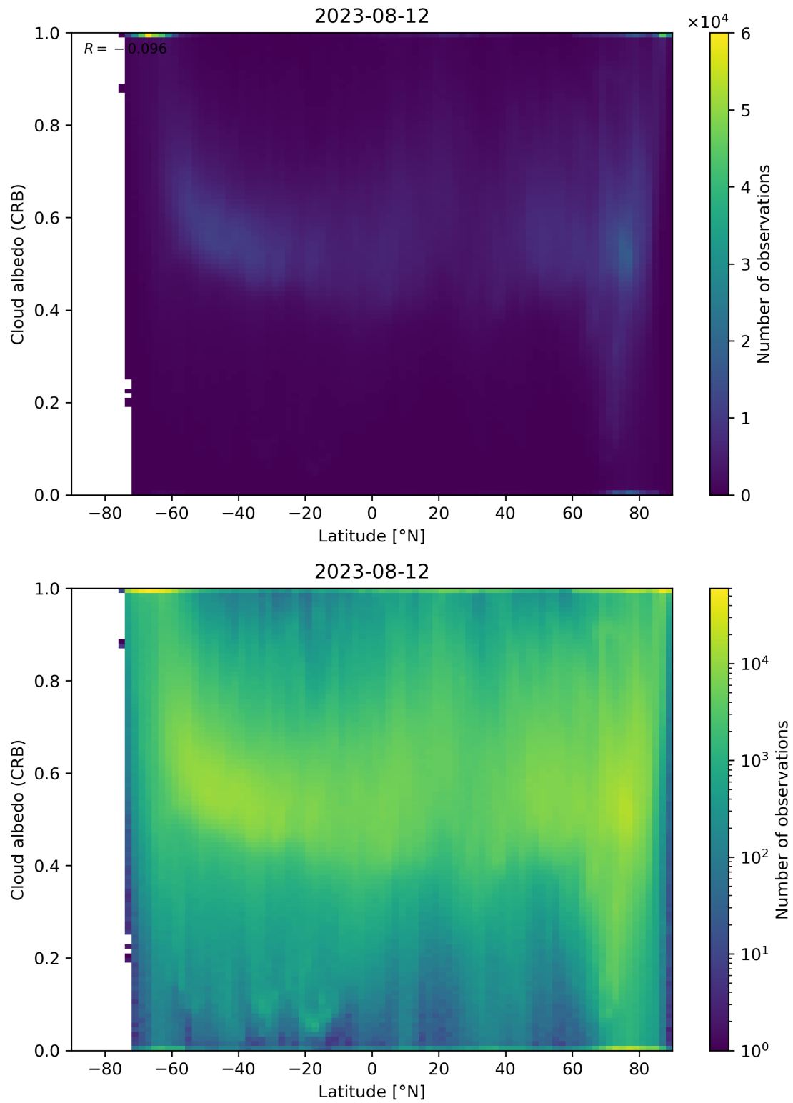
Figure 91: Scatter density plot of “Latitude” against “Cloud albedo (CRB)” for 2023-08-11 to 2023-08-13.
