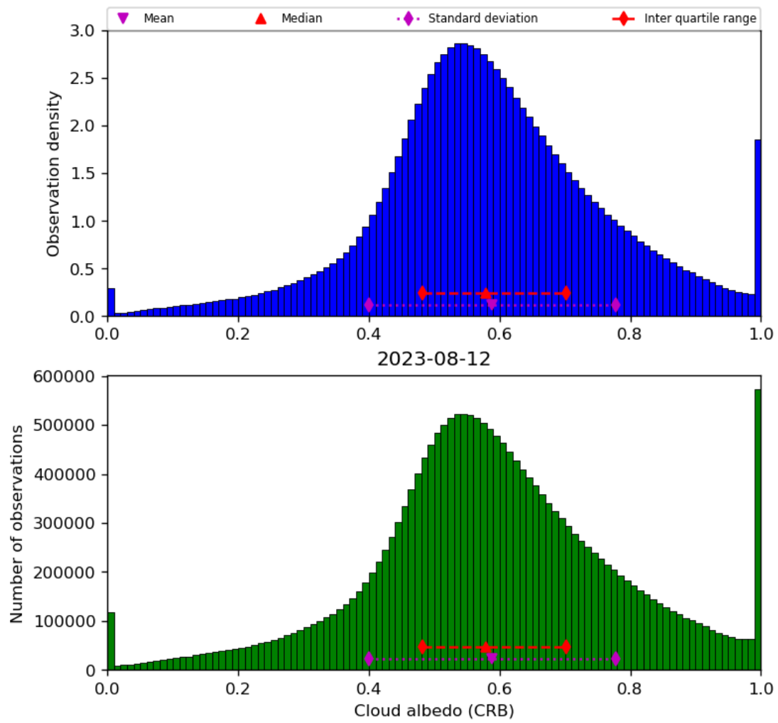
Figure 44: Histogram of “Cloud albedo (CRB)” for 2023-08-11 to 2023-08-13
