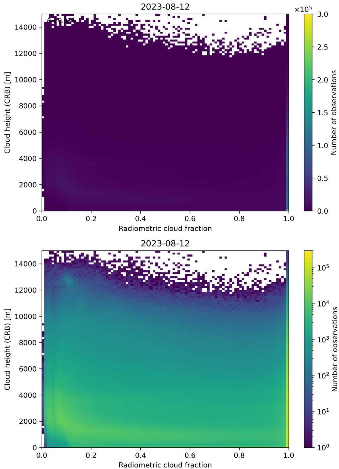
Figure 74: Scatter density plot of “Radiometric cloud fraction” against “Cloud height (CRB)” for 2023-08-11 to 2023-08-13.
