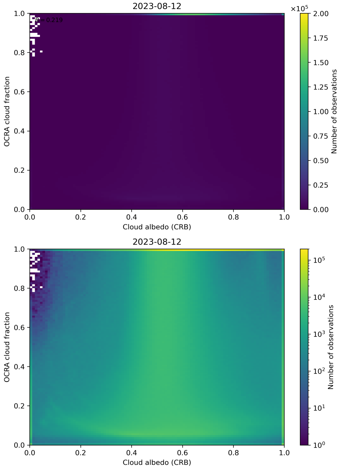
Figure 70: Scatter density plot of “Cloud albedo (CRB)” against “OCRA cloud fraction” for 2023-08-11 to 2023-08-13.
