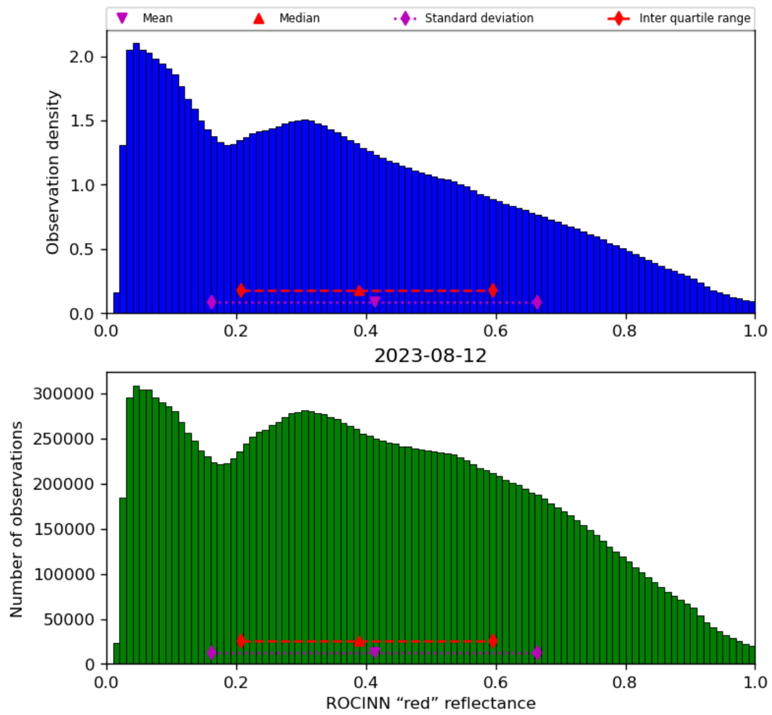
Figure 53: Histogram of “ROCINN “red” reflectance” for 2023-08-11 to 2023-08-13
