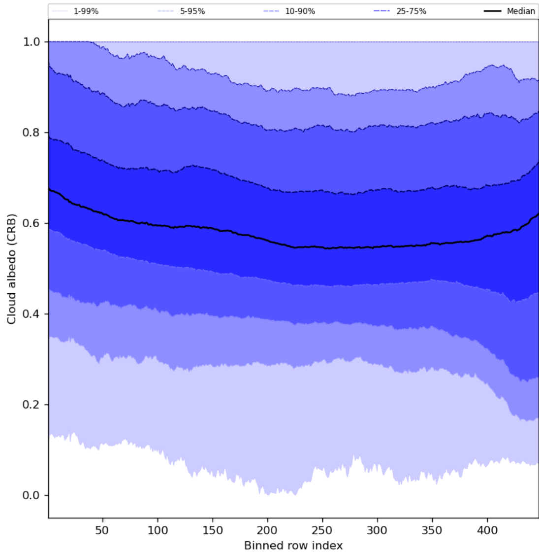
Figure 60: Along track statistics of “Cloud albedo (CRB)” for 2023-08-11 to 2023-08-13
