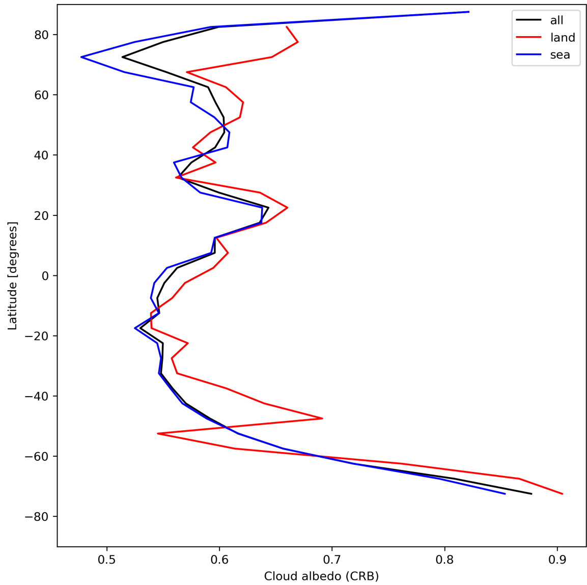
Figure 28: Zonal average of “Cloud albedo (CRB)” for 2023-08-11 to 2023-08-13.
