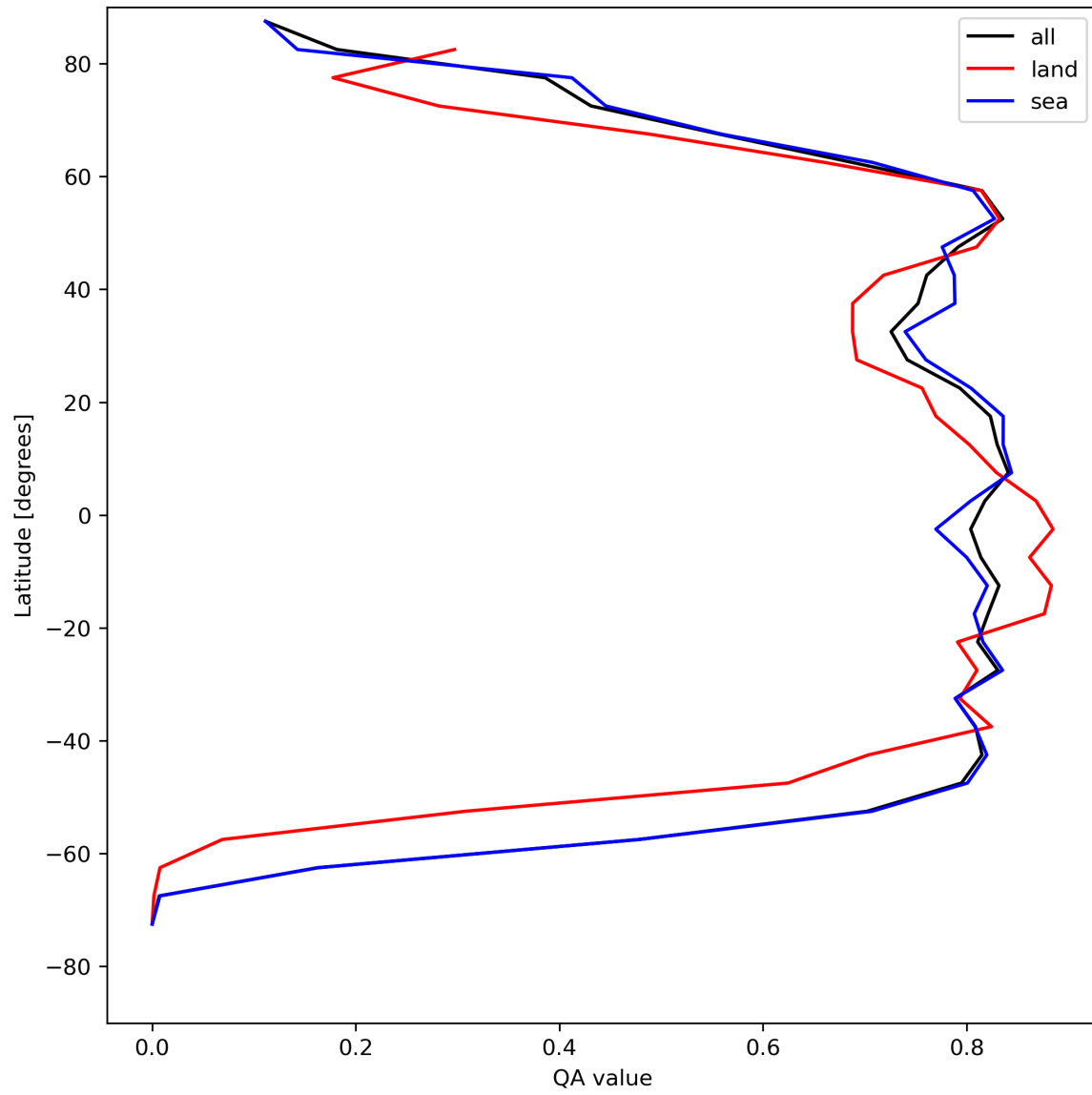
Figure 22: Zonal average of “QA value” for 2023-08-11 to 2023-08-13.
