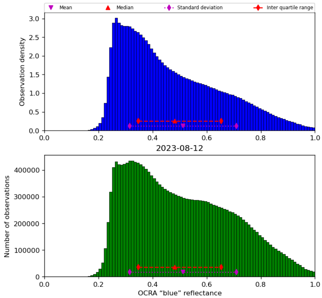
Figure 51: Histogram of “OCRA “blue” reflectance” for 2023-08-11 to 2023-08-13
