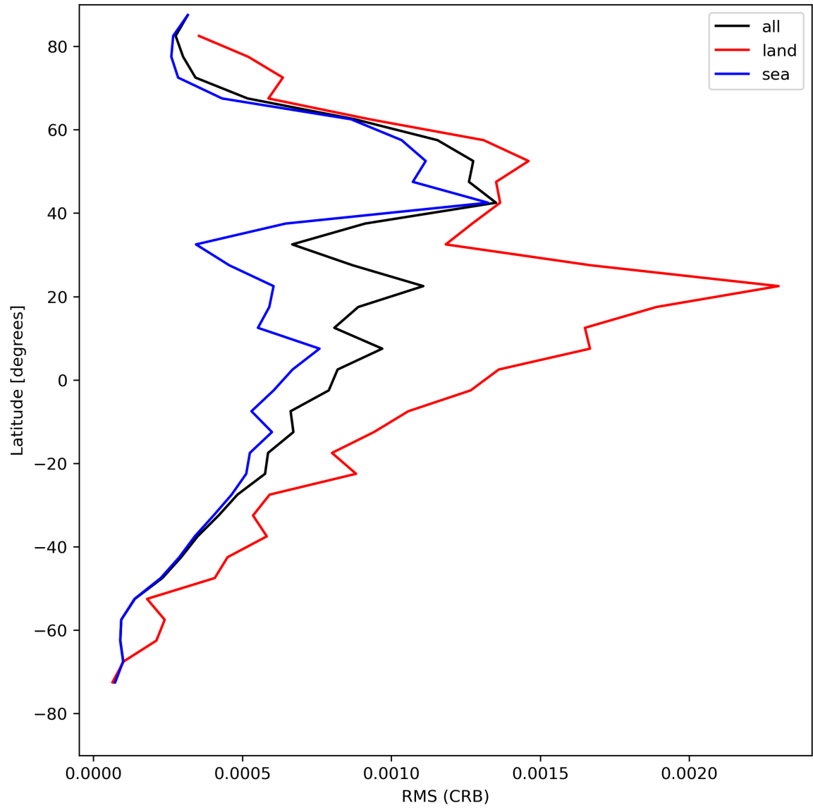
Figure 32: Zonal average of “RMS (CRB)” for 2023-08-11 to 2023-08-13.
