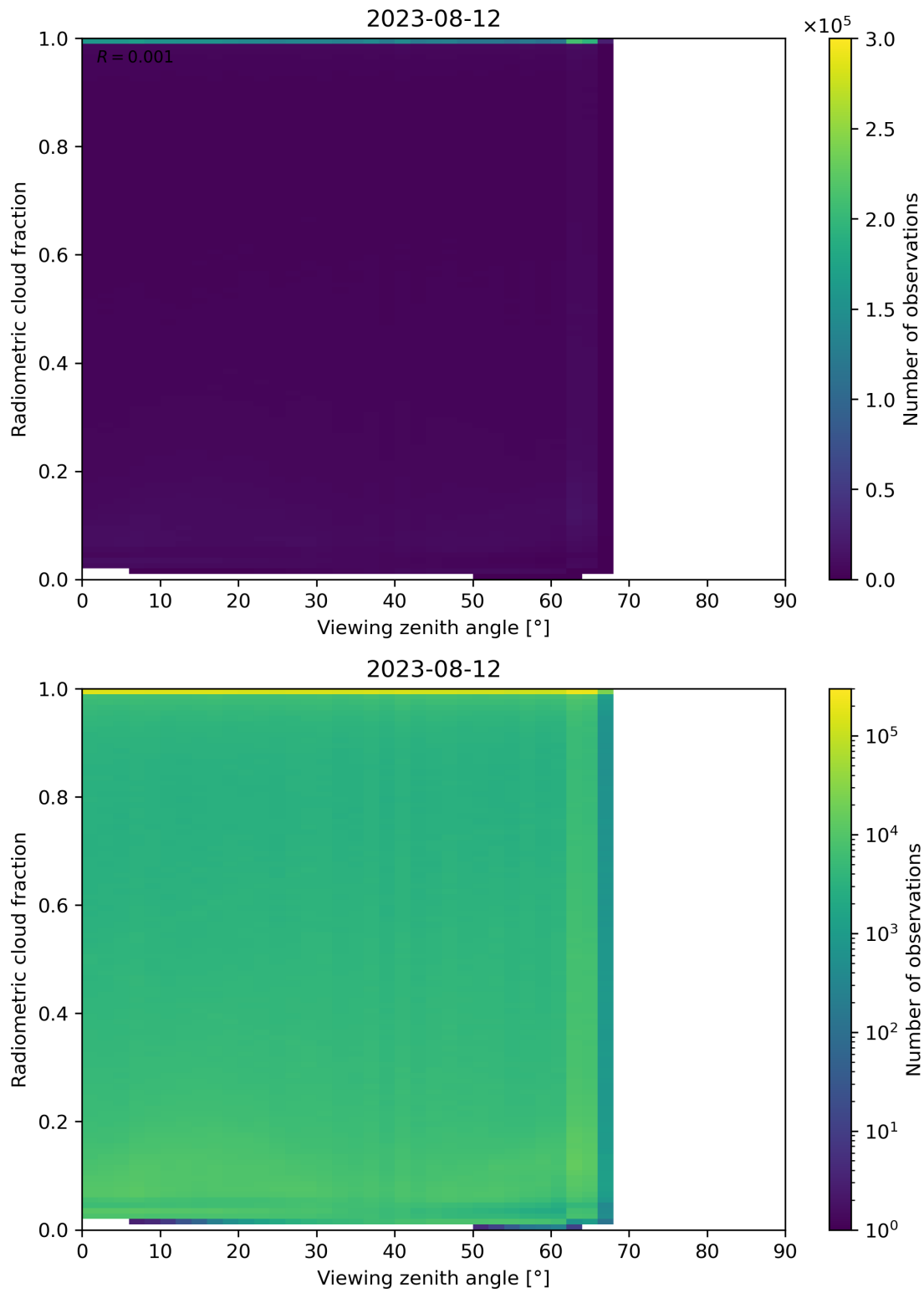
Figure 107: Scatter density plot of “Viewing zenith angle” against “Radiometric cloud fraction” for 2023-08-11 to 2023-08-13.
