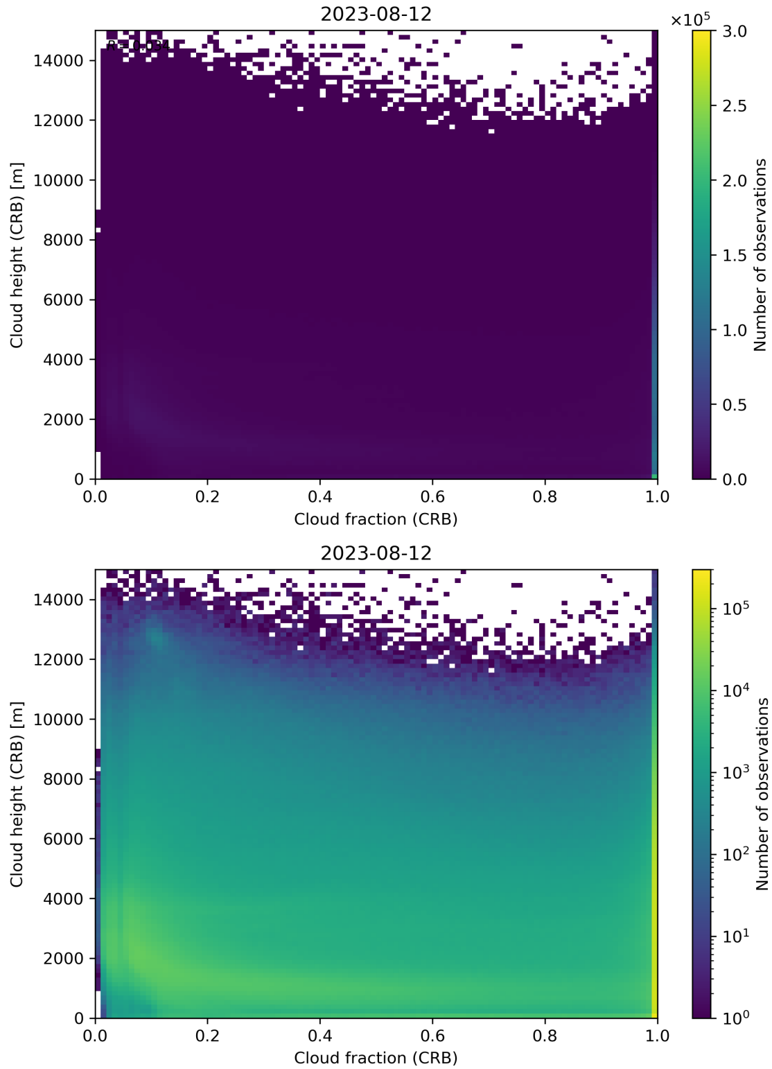
Figure 79: Scatter density plot of “Cloud fraction (CRB)” against “Cloud height (CRB)” for 2023-08-11 to 2023-08-13.
