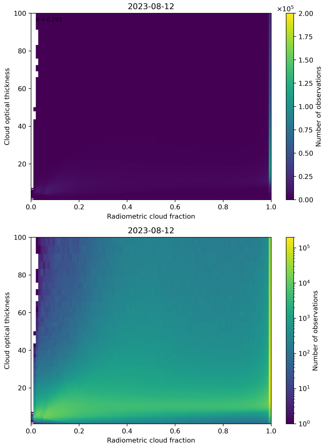
Figure 75: Scatter density plot of “Radiometric cloud fraction” against “Cloud optical thickness” for 2023-08-11 to 2023-08-13.
