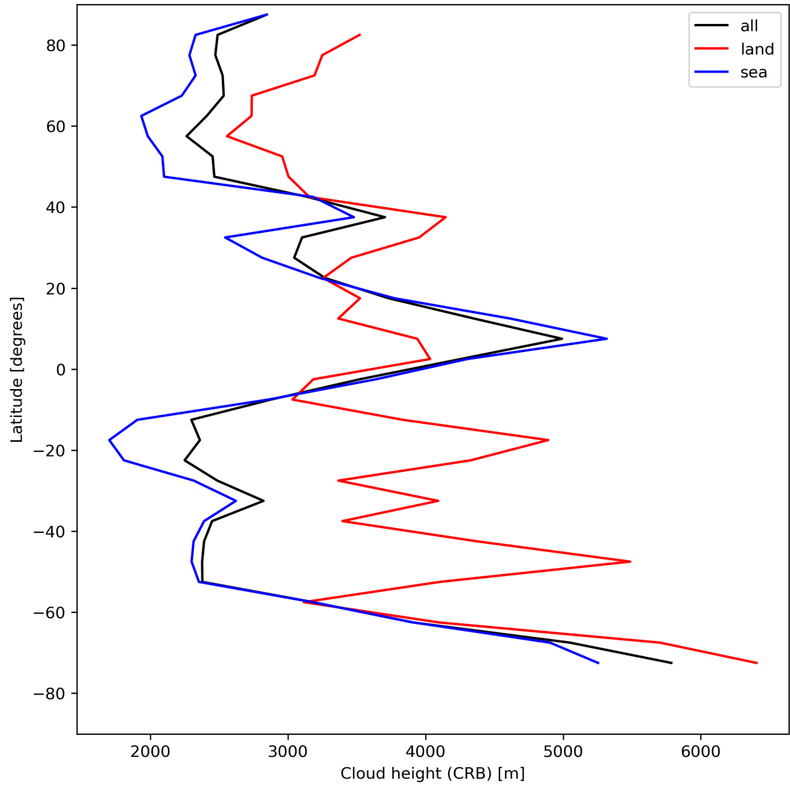
Figure 27: Zonal average of “Cloud height (CRB)” for 2023-08-11 to 2023-08-13.
