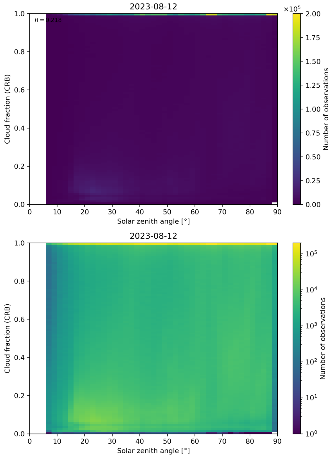
Figure 101: Scatter density plot of “Solar zenith angle” against “Cloud fraction (CRB)” for 2023-08-11 to 2023-08-13.
