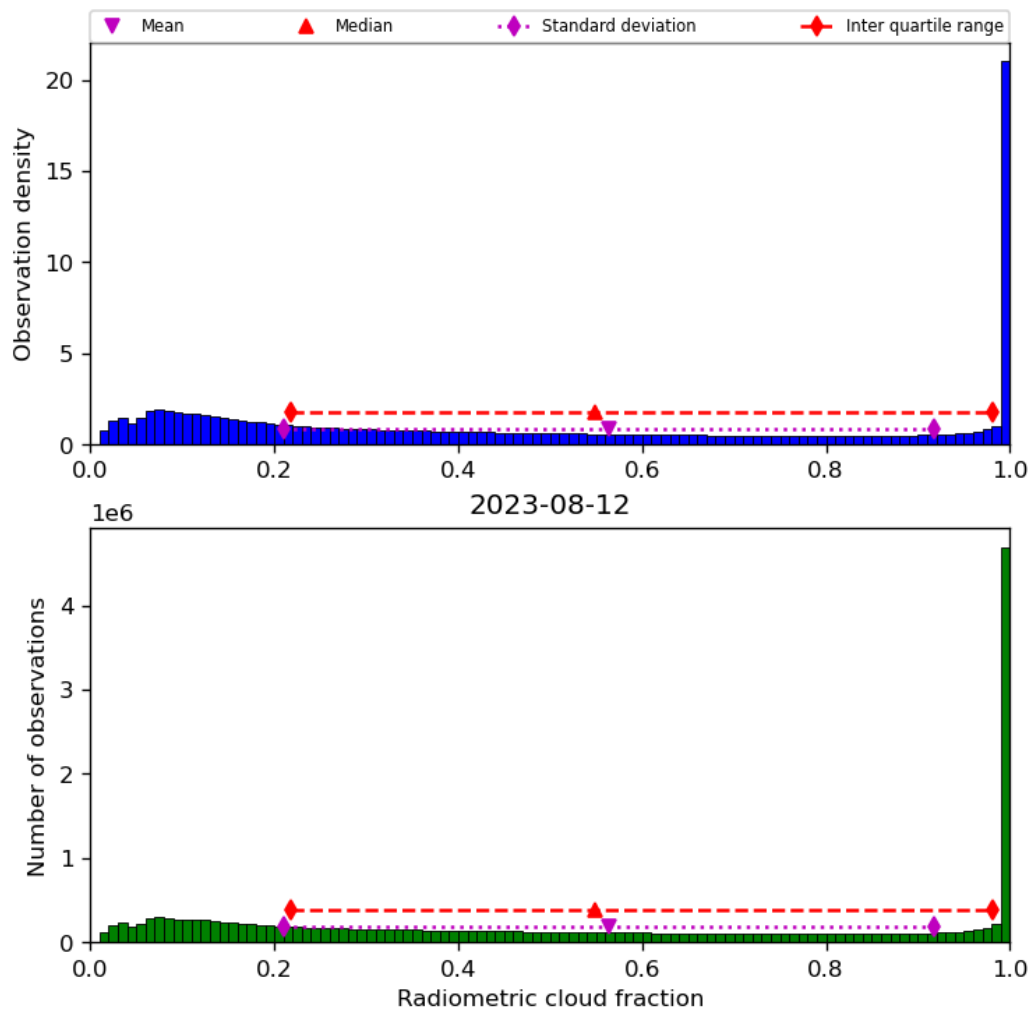
Figure 39: Histogram of “Radiometric cloud fraction” for 2023-08-11 to 2023-08-13
