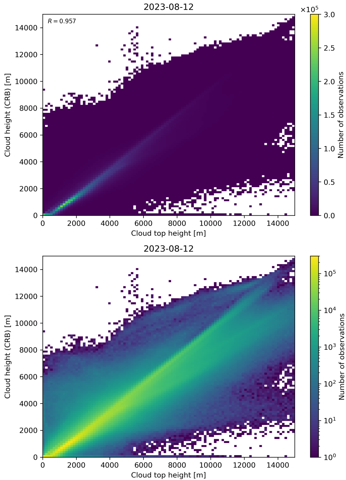
Figure 89: Scatter density plot of “Cloud top height” against “Cloud height (CRB)” for 2023-08-11 to 2023-08-13.
