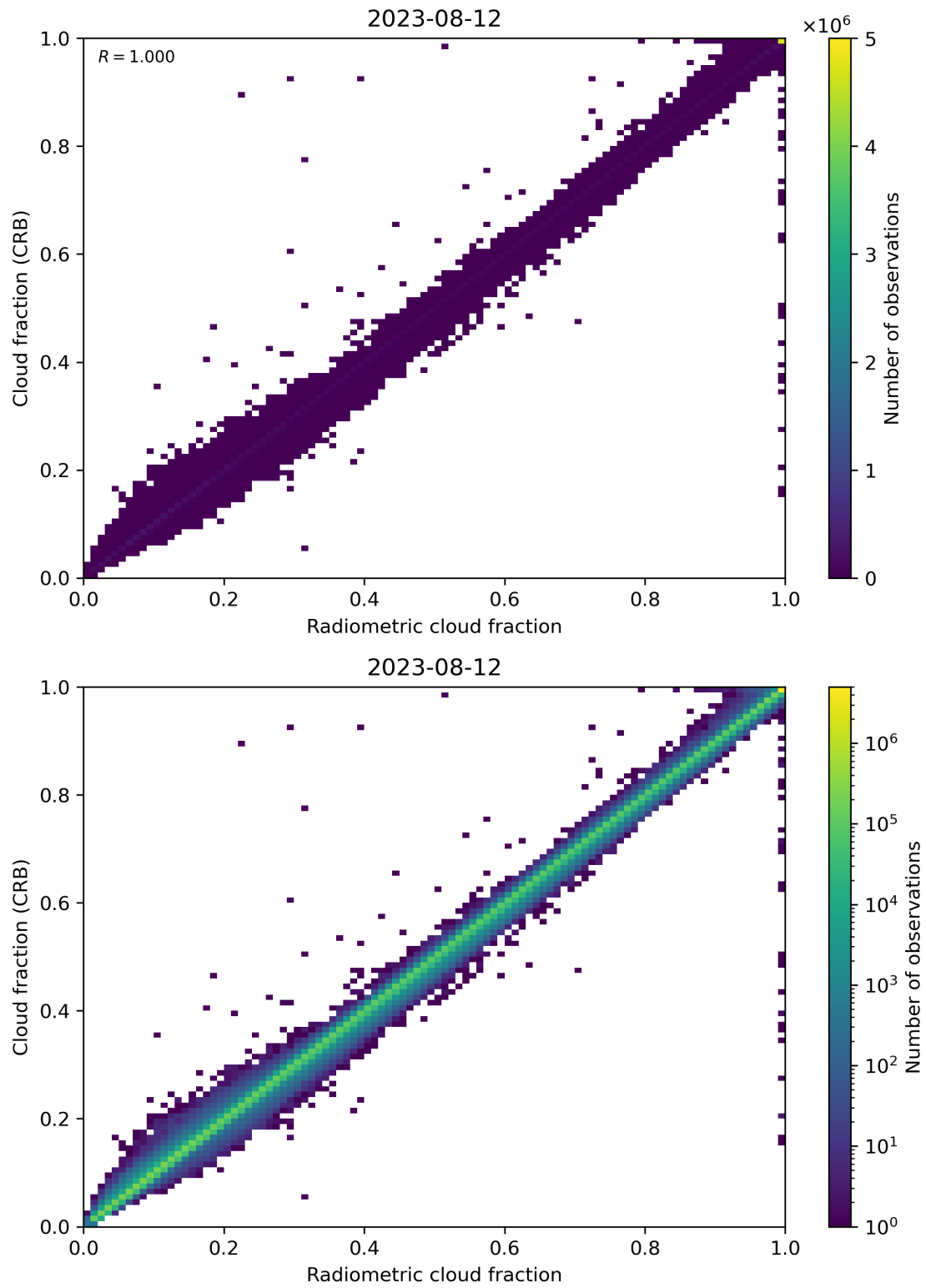
Figure 73: Scatter density plot of “Radiometric cloud fraction” against “Cloud fraction (CRB)” for 2023-08-11 to 2023-08-13.
