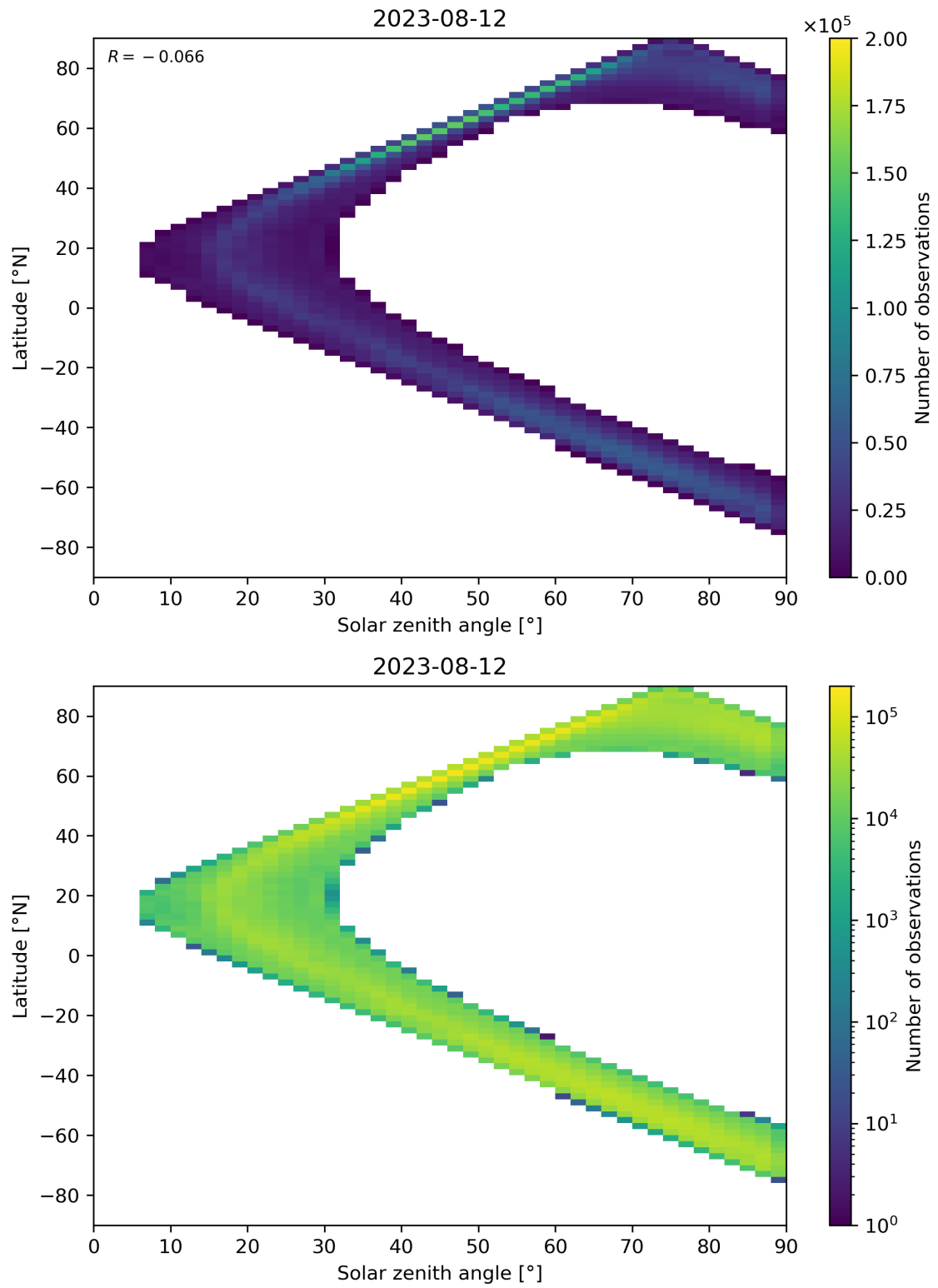
Figure 105: Scatter density plot of “Solar zenith angle” against “Latitude” for 2023-08-11 to 2023-08-13.
