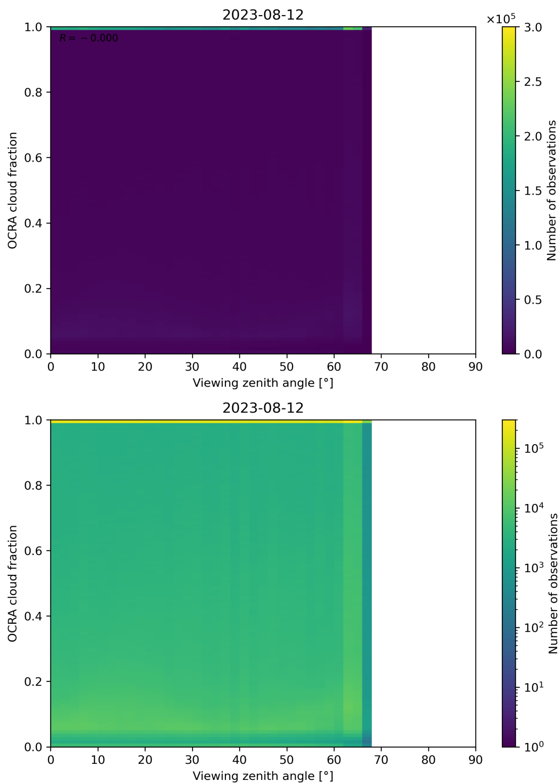
Figure 108: Scatter density plot of “Viewing zenith angle” against “OCRA cloud fraction” for 2023-08-11 to 2023-08-13.
