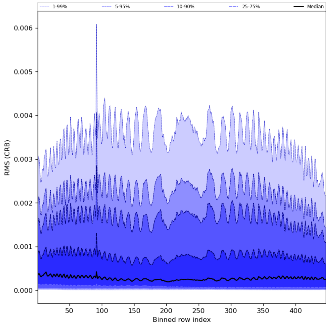
Figure 64: Along track statistics of “RMS (CRB)” for 2023-08-11 to 2023-08-13
