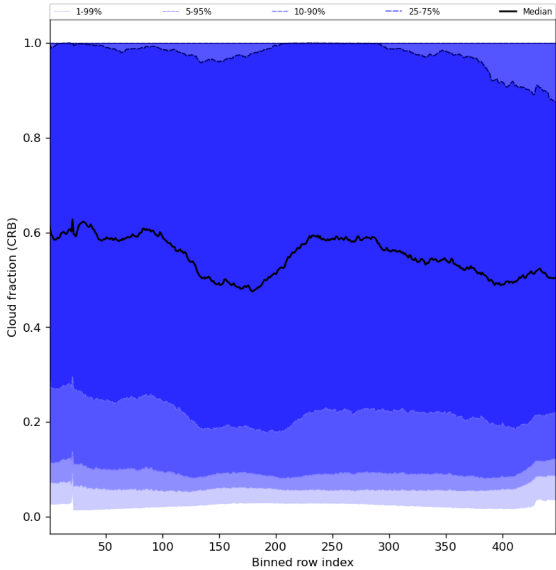
Figure 58: Along track statistics of “Cloud fraction (CRB)” for 2023-08-11 to 2023-08-13
