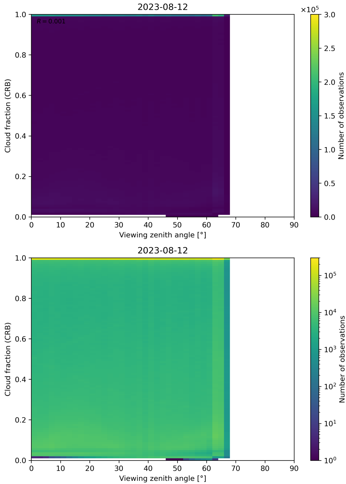
Figure 109: Scatter density plot of “Viewing zenith angle” against “Cloud fraction (CRB)” for 2023-08-11 to 2023-08-13.
