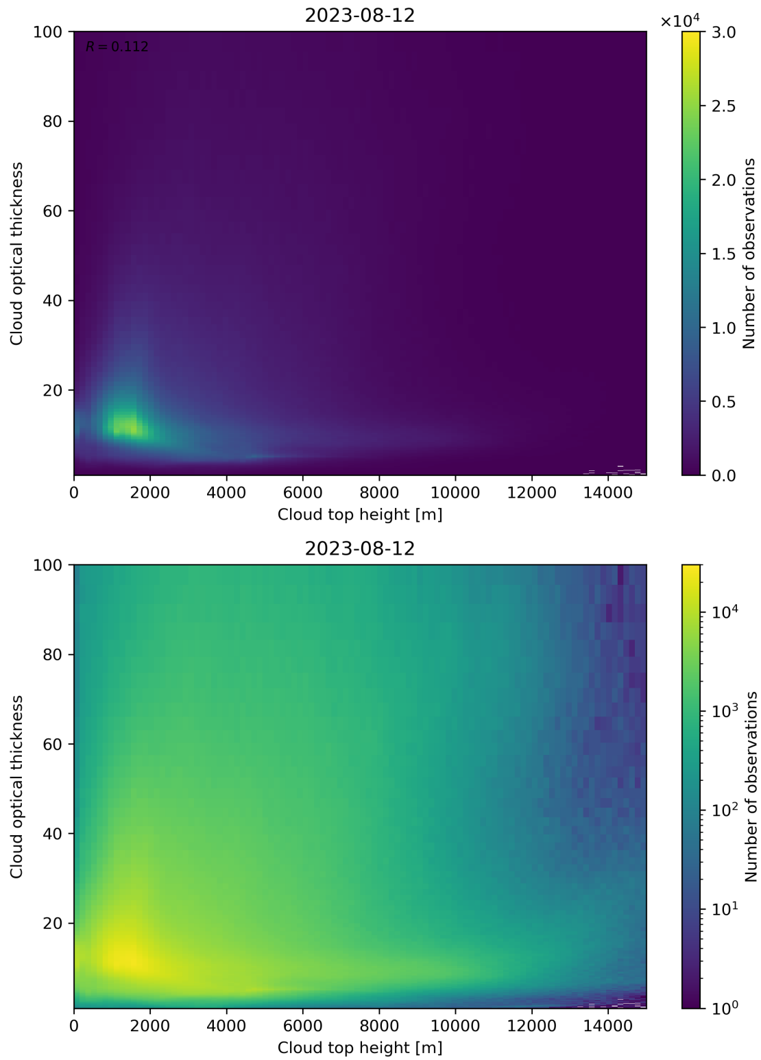
Figure 90: Scatter density plot of “Cloud top height” against “Cloud optical thickness” for 2023-08-11 to 2023-08-13.
