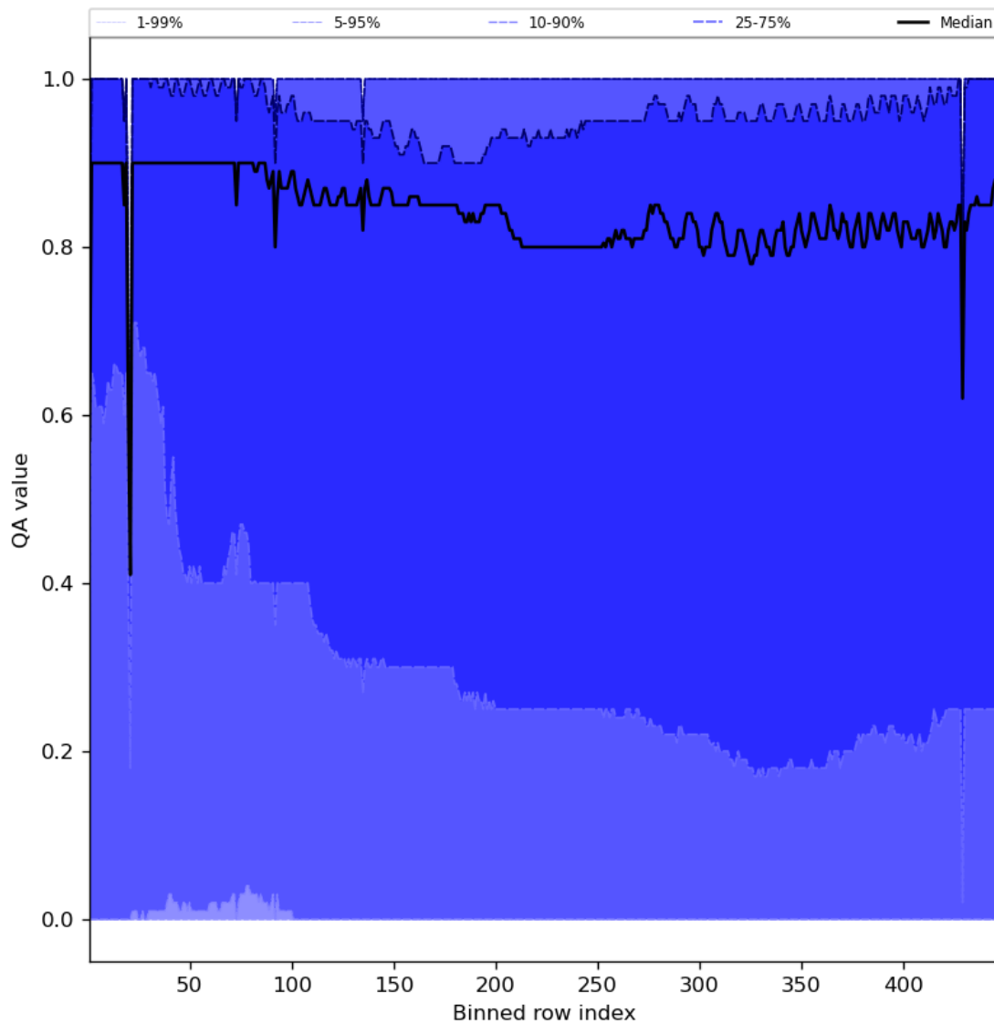
Figure 54: Along track statistics of “QA value” for 2023-08-11 to 2023-08-13
