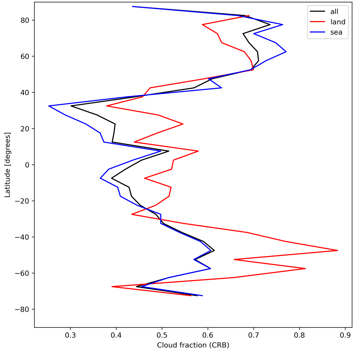
Figure 26: Zonal average of “Cloud fraction (CRB)” for 2023-08-11 to 2023-08-13.
