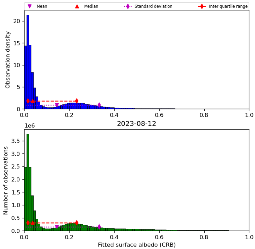
Figure 46: Histogram of “Fitted surface albedo (CRB)” for 2023-08-11 to 2023-08-13
