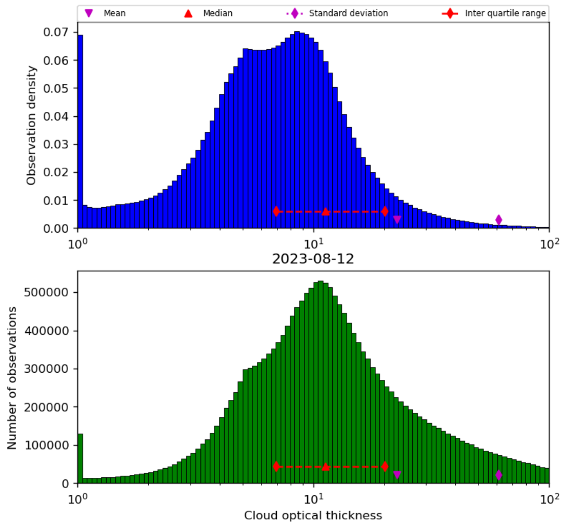
Figure 41: Histogram of “Cloud optical thickness” for 2023-08-11 to 2023-08-13
