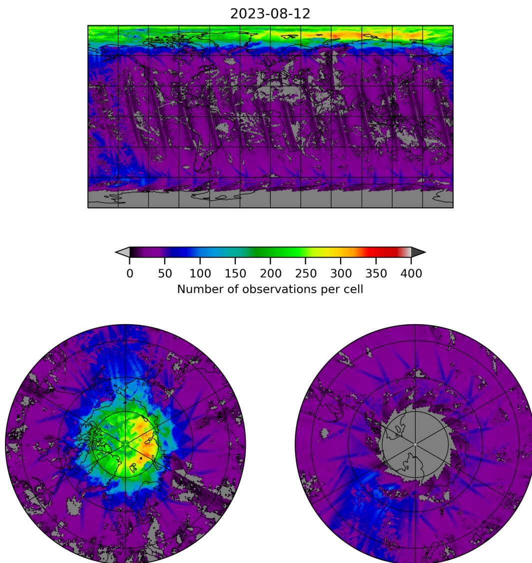
Figure 21: Map of the number of observations for 2023-08-11 to 2023-08-13
