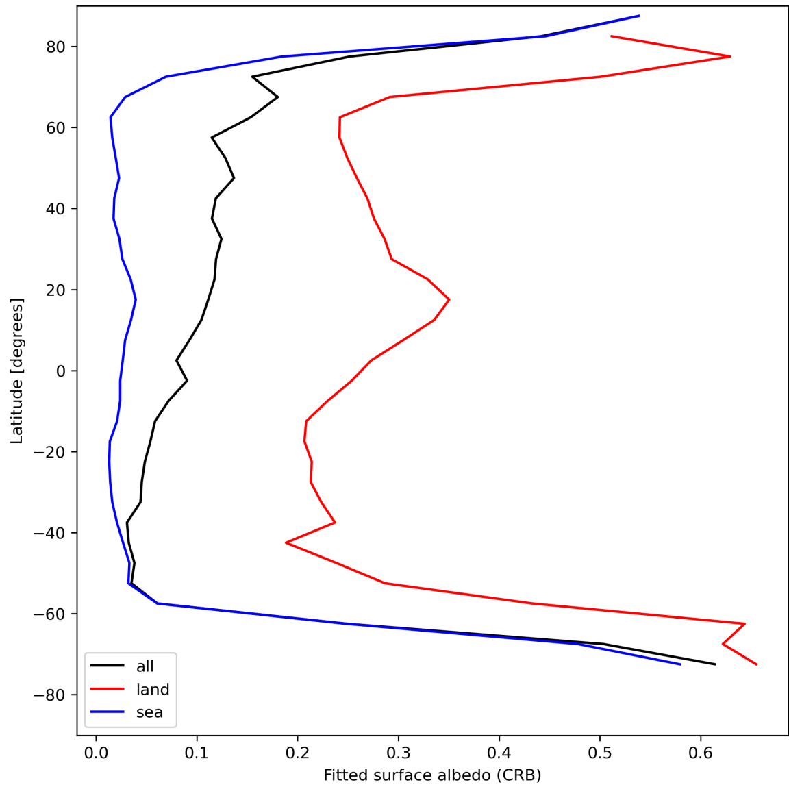
Figure 30: Zonal average of “Fitted surface albedo (CRB)” for 2023-08-11 to 2023-08-13.
