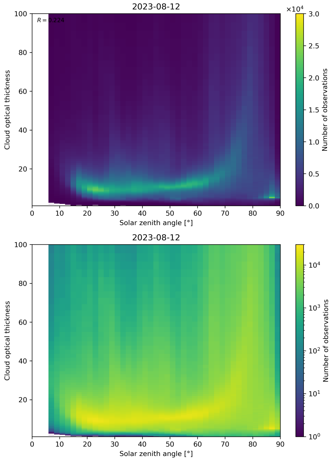
Figure 103: Scatter density plot of “Solar zenith angle” against “Cloud optical thickness” for 2023-08-11 to 2023-08-13.
