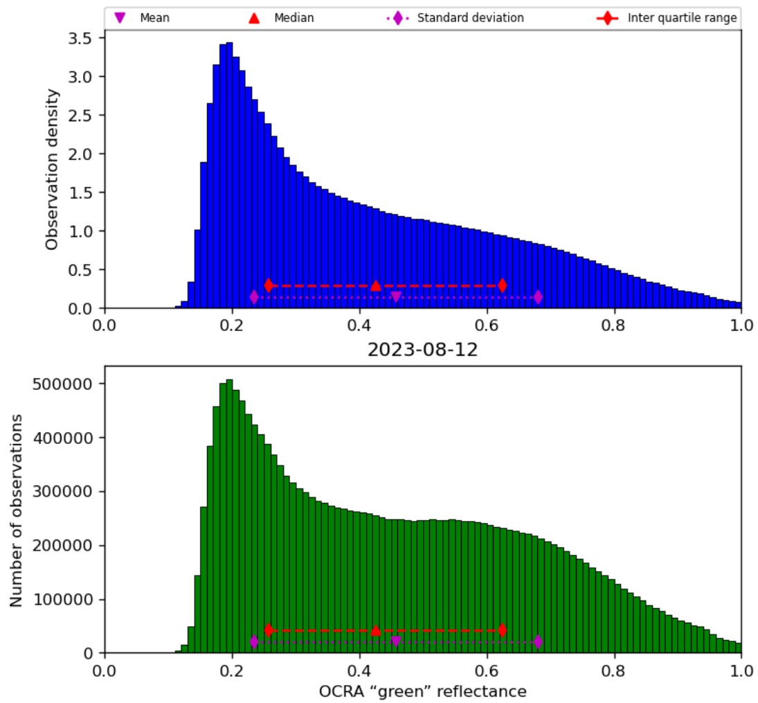
Figure 52: Histogram of “OCRA “green” reflectance” for 2023-08-11 to 2023-08-13
