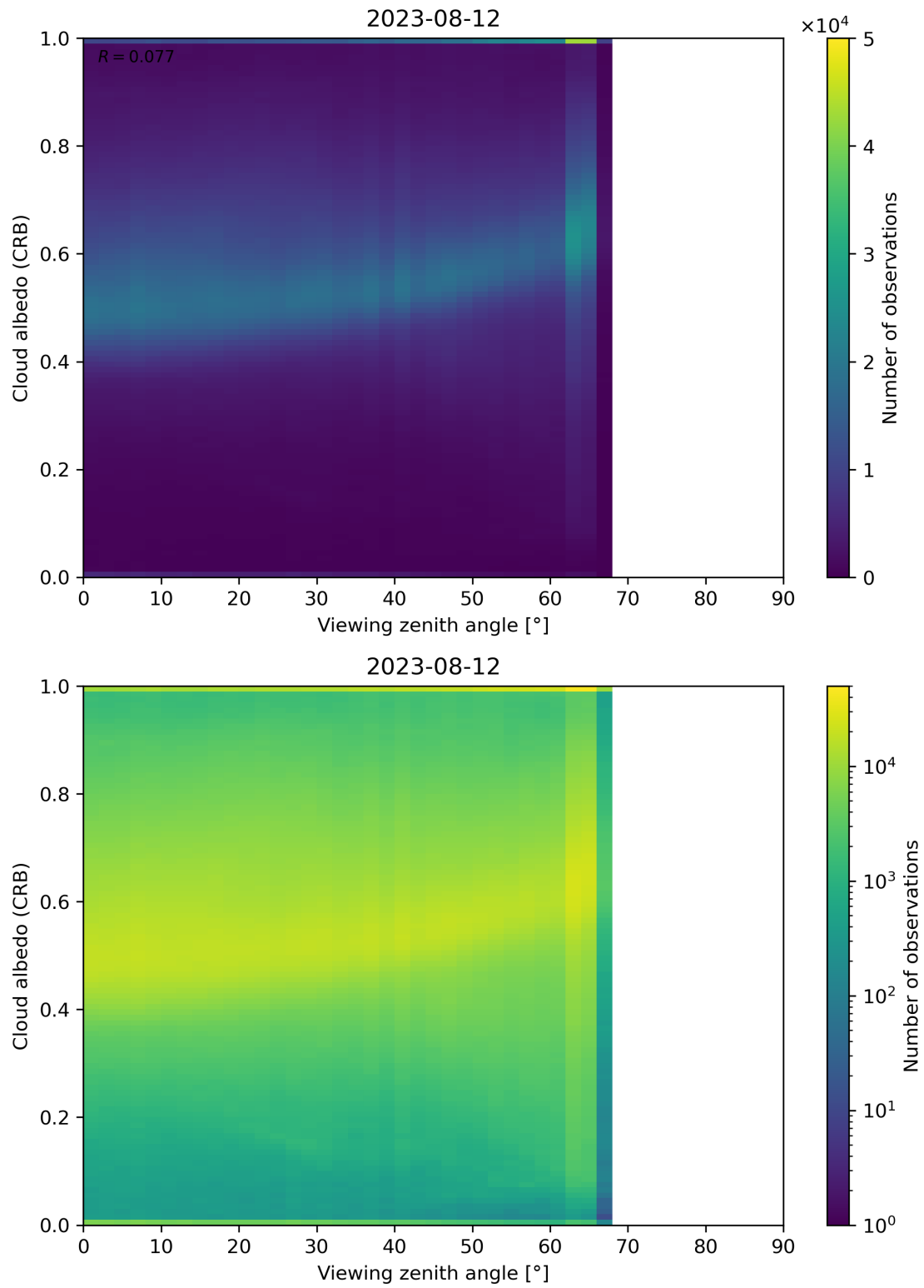
Figure 106: Scatter density plot of “Viewing zenith angle” against “Cloud albedo (CRB)” for 2023-08-11 to 2023-08-13.
