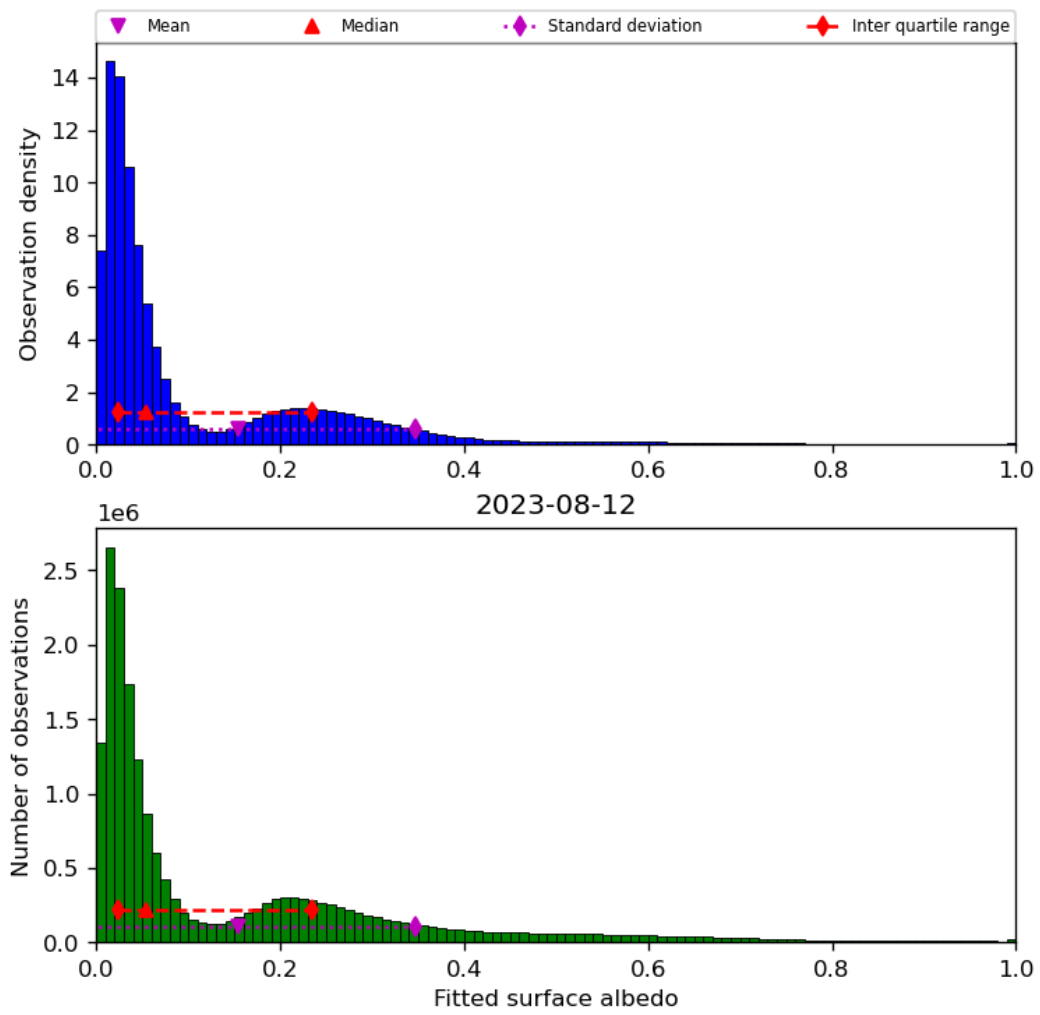
Figure 45: Histogram of “Fitted surface albedo” for 2023-08-11 to 2023-08-13
