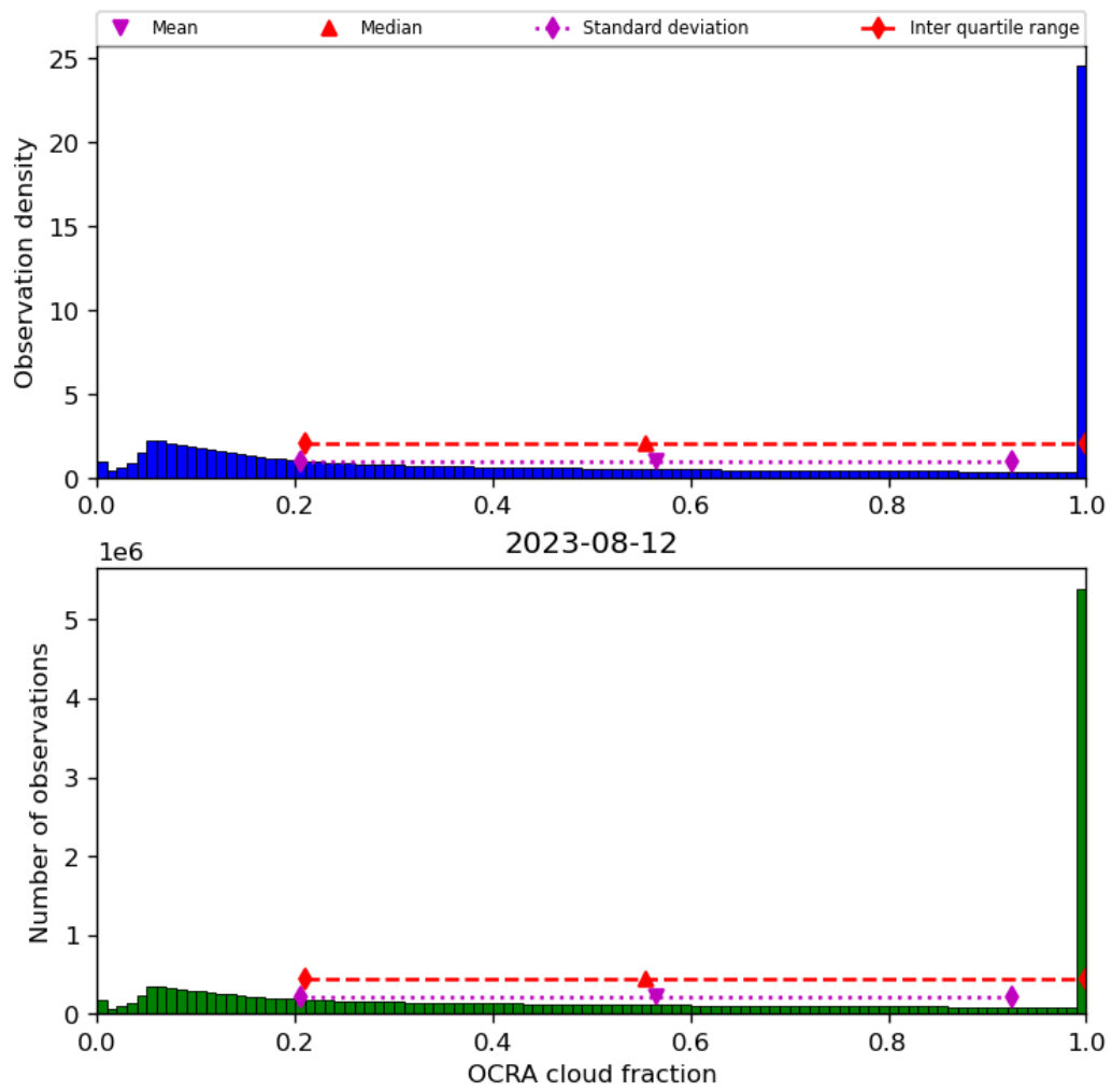
Figure 50: Histogram of “OCRA cloud fraction” for 2023-08-11 to 2023-08-13
