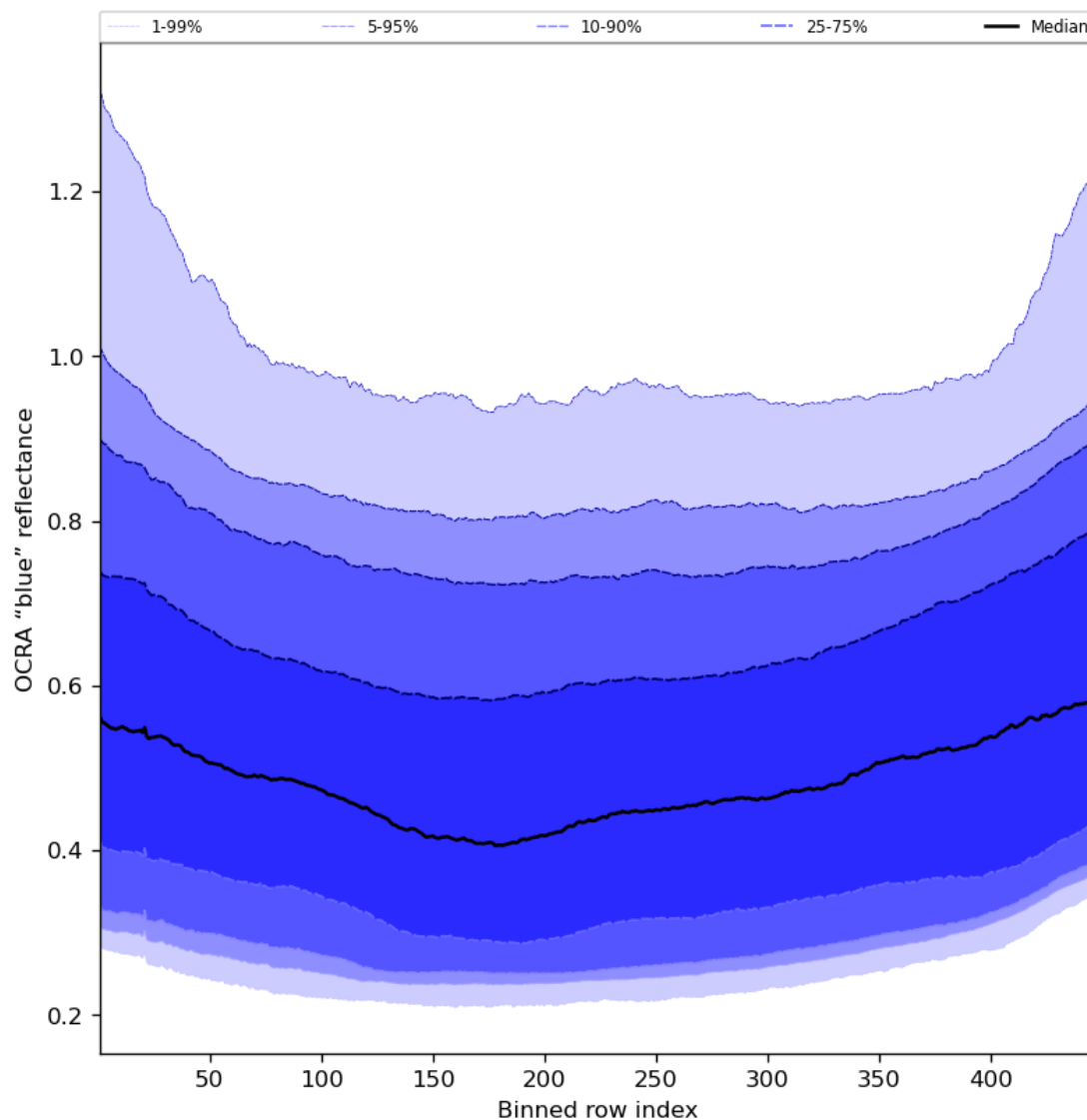
Figure 67: Along track statistics of “OCRA “blue” reflectance” for 2023-08-11 to 2023-08-13
