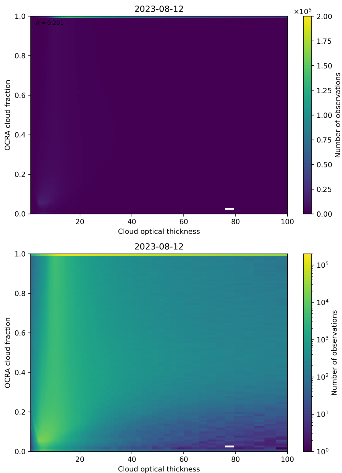
Figure 83: Scatter density plot of “Cloud optical thickness” against “OCRA cloud fraction” for 2023-08-11 to 2023-08-13.
