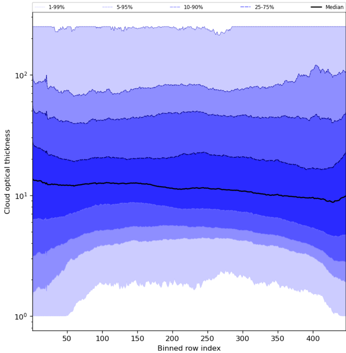
Figure 57: Along track statistics of “Cloud optical thickness” for 2023-08-11 to 2023-08-13
