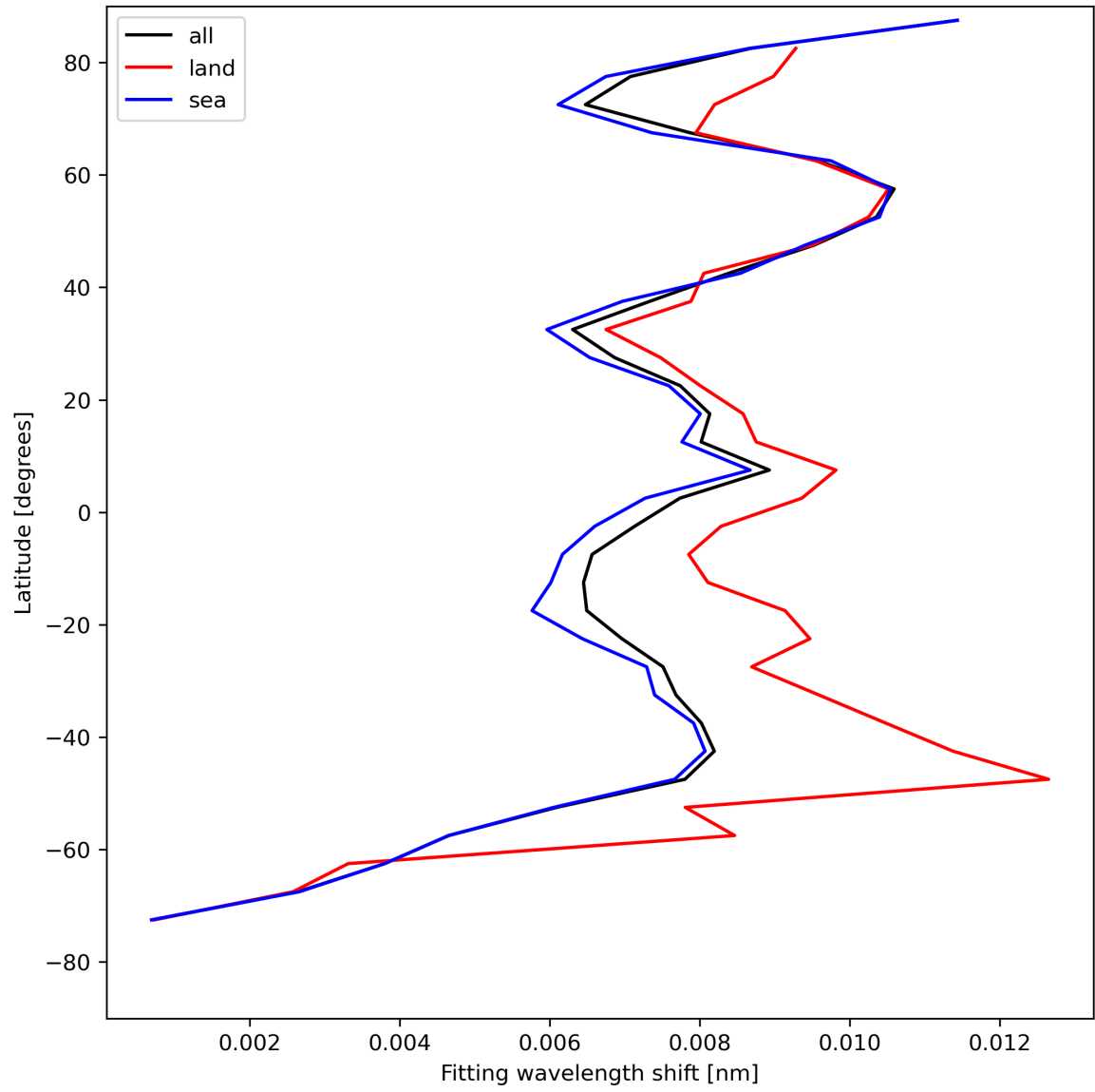
Figure 33: Zonal average of “Fitting wavelength shift” for 2023-08-11 to 2023-08-13.
