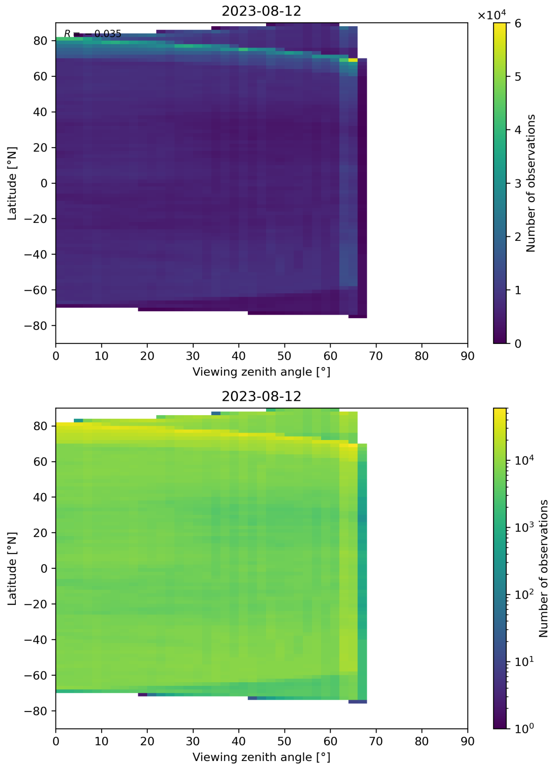
Figure 113: Scatter density plot of “Viewing zenith angle” against “Latitude” for 2023-08-11 to 2023-08-13.
