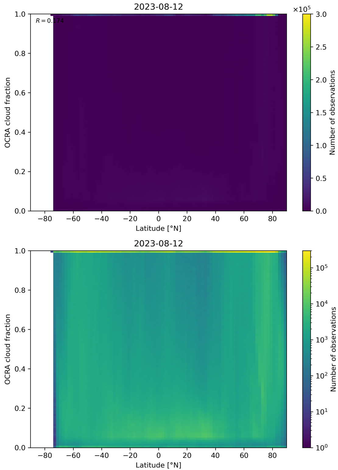
Figure 93: Scatter density plot of “Latitude” against “OCRA cloud fraction” for 2023-08-11 to 2023-08-13.
