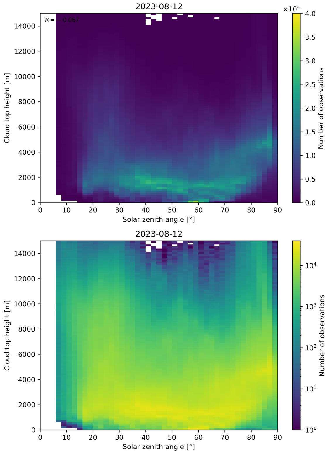
Figure 104: Scatter density plot of “Solar zenith angle” against “Cloud top height” for 2023-08-11 to 2023-08-13.
