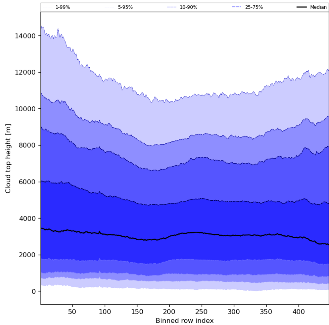
Figure 56: Along track statistics of “Cloud top height” for 2023-08-11 to 2023-08-13
