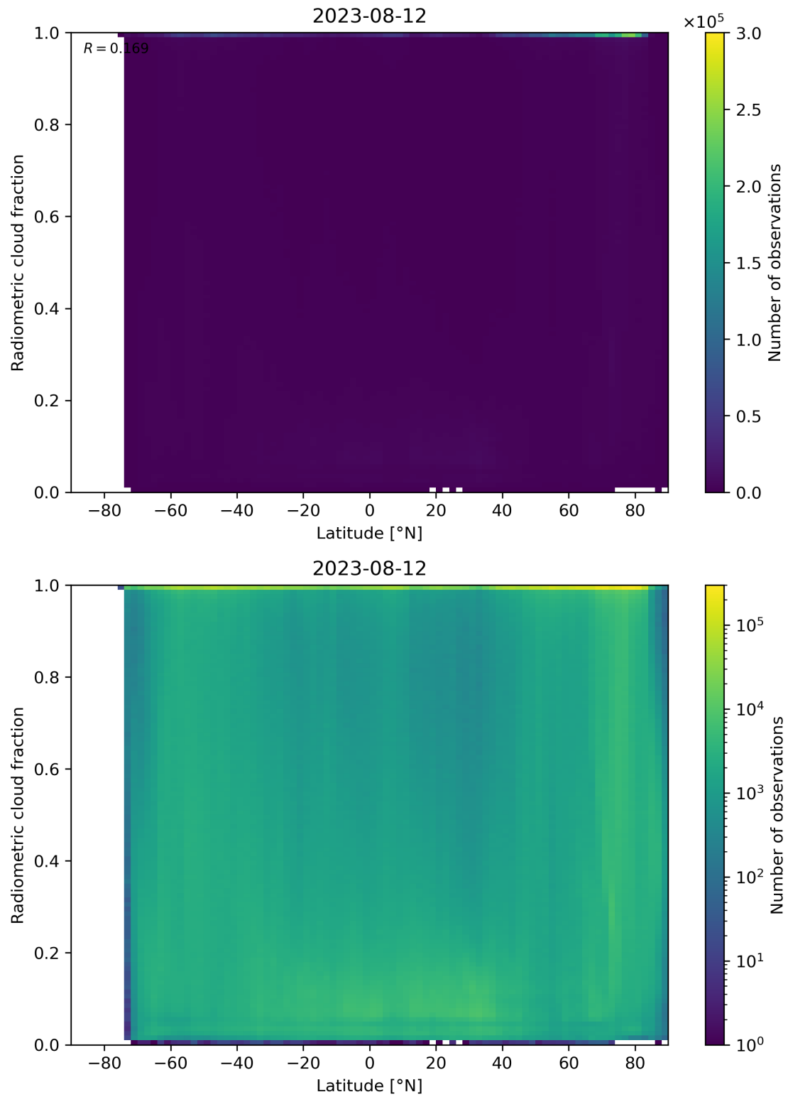
Figure 92: Scatter density plot of “Latitude” against “Radiometric cloud fraction” for 2023-08-11 to 2023-08-13.
