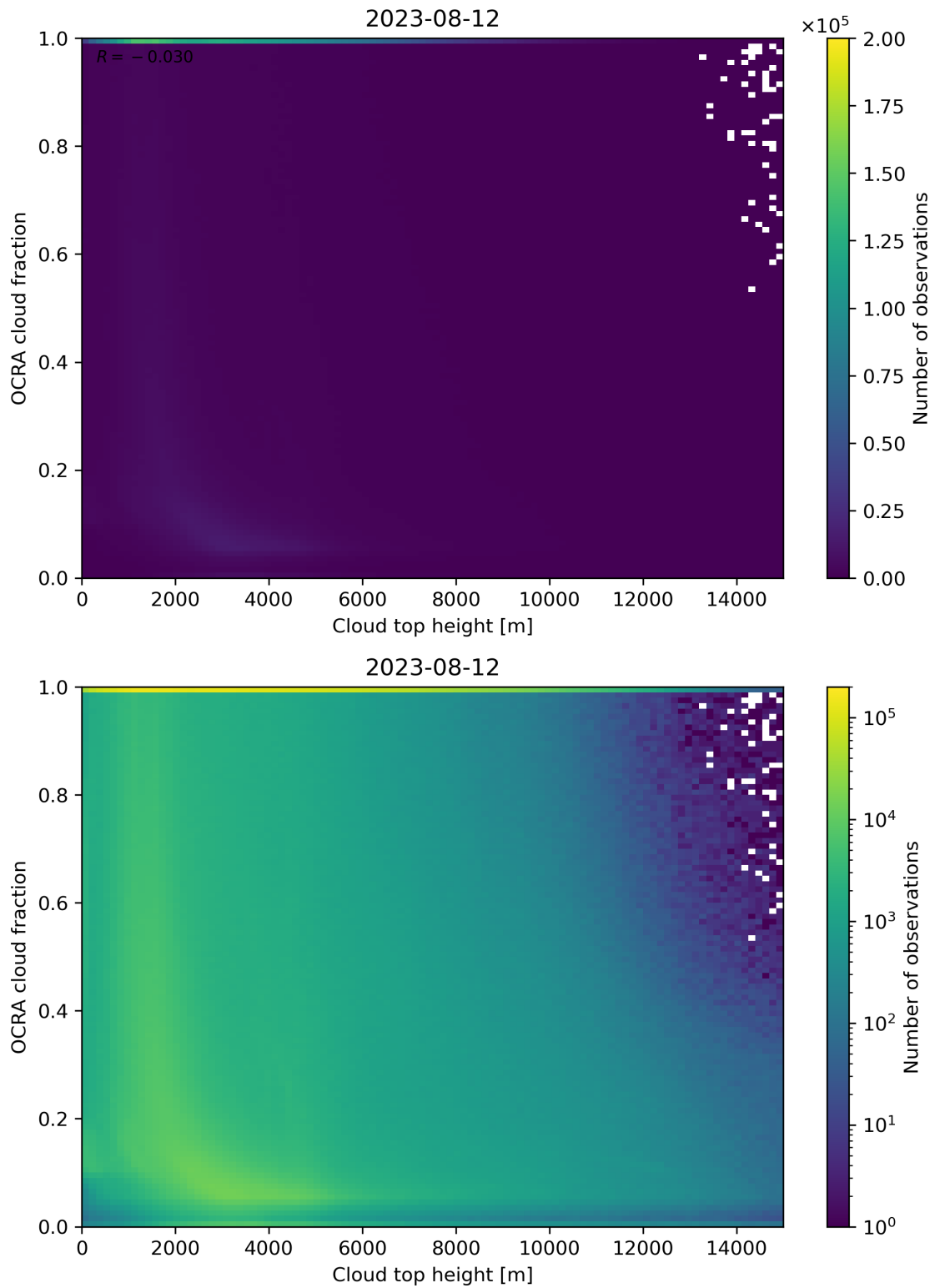
Figure 87: Scatter density plot of “Cloud top height” against “OCRA cloud fraction” for 2023-08-11 to 2023-08-13.
