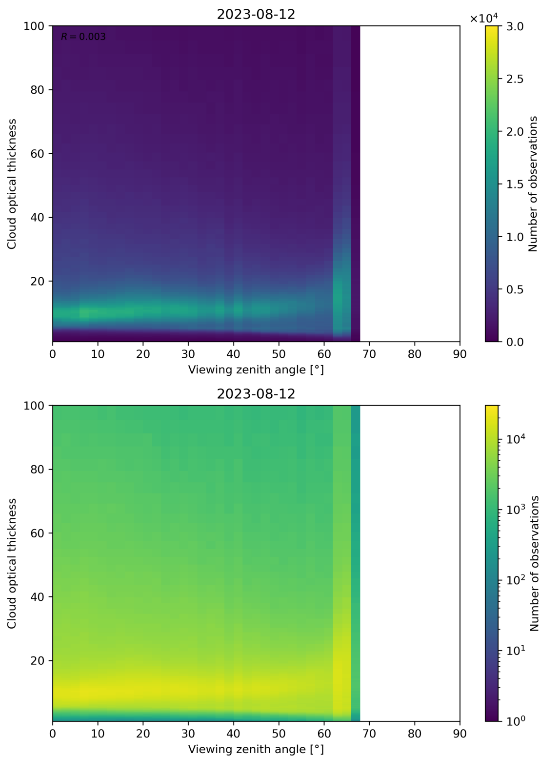
Figure 111: Scatter density plot of “Viewing zenith angle” against “Cloud optical thickness” for 2023-08-11 to 2023-08-13.
