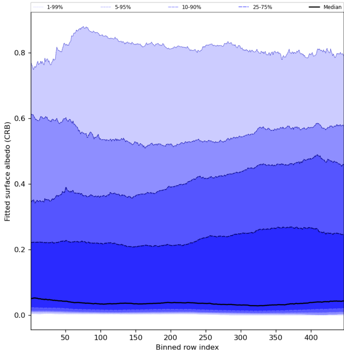
Figure 62: Along track statistics of "Fitted surface albedo (CRB)" for 2023-08-11 to 2023-08-13
