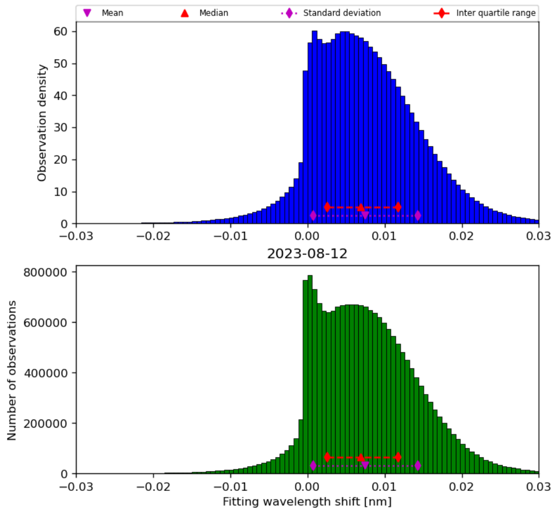
Figure 49: Histogram of “Fitting wavelength shift” for 2023-08-11 to 2023-08-13
