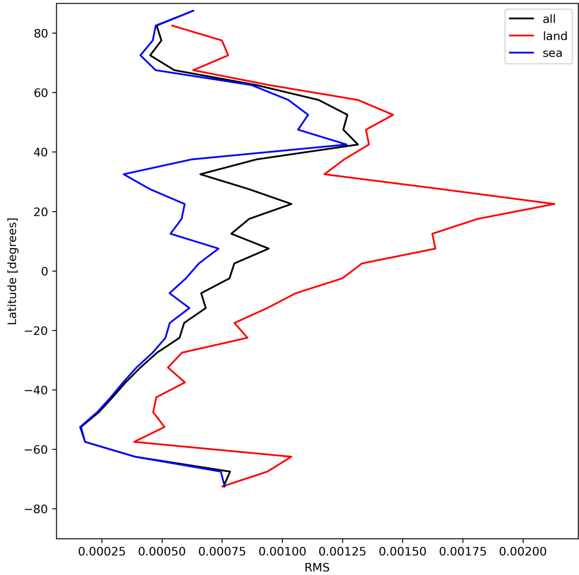
Figure 31: Zonal average of “RMS” for 2023-08-11 to 2023-08-13.
