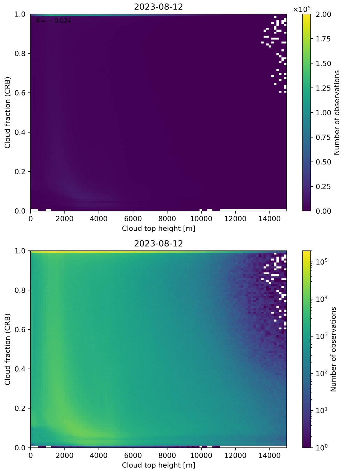
Figure 88: Scatter density plot of “Cloud top height” against “Cloud fraction (CRB)” for 2023-08-11 to 2023-08-13.
