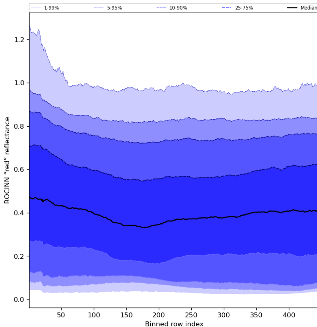
Figure 69: Along track statistics of “ROCINN “red” reflectance” for 2023-08-11 to 2023-08-13
