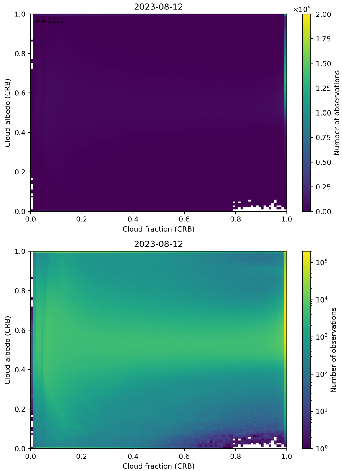
Figure 77: Scatter density plot of “Cloud fraction (CRB)” against “Cloud albedo (CRB)” for 2023-08-11 to 2023-08-13.
