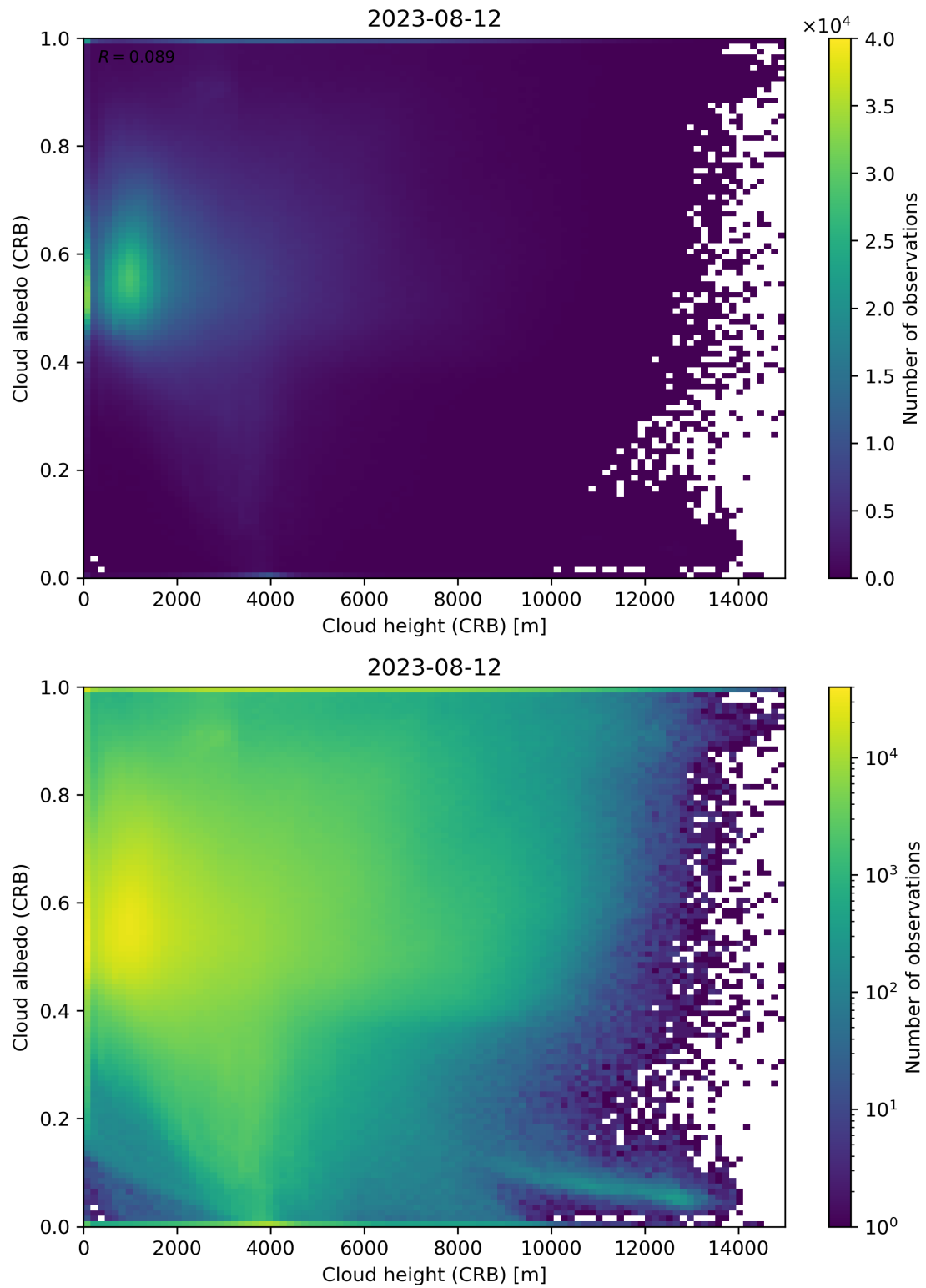
Figure 80: Scatter density plot of “Cloud height (CRB)” against “Cloud albedo (CRB)” for 2023-08-11 to 2023-08-13.
