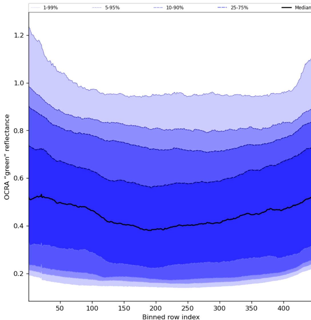
Figure 68: Along track statistics of "OCRA "green" reflectance" for 2023-08-15 to 2023-08-17
