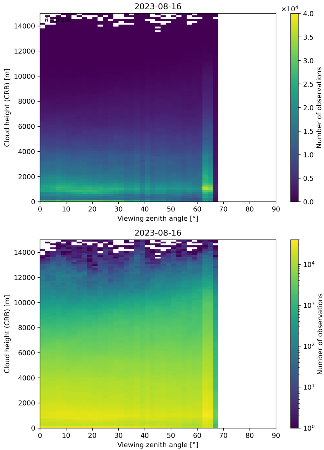
Figure 110: Scatter density plot of “Viewing zenith angle” against “Cloud height (CRB)” for 2023-08-15 to 2023-08-17.
