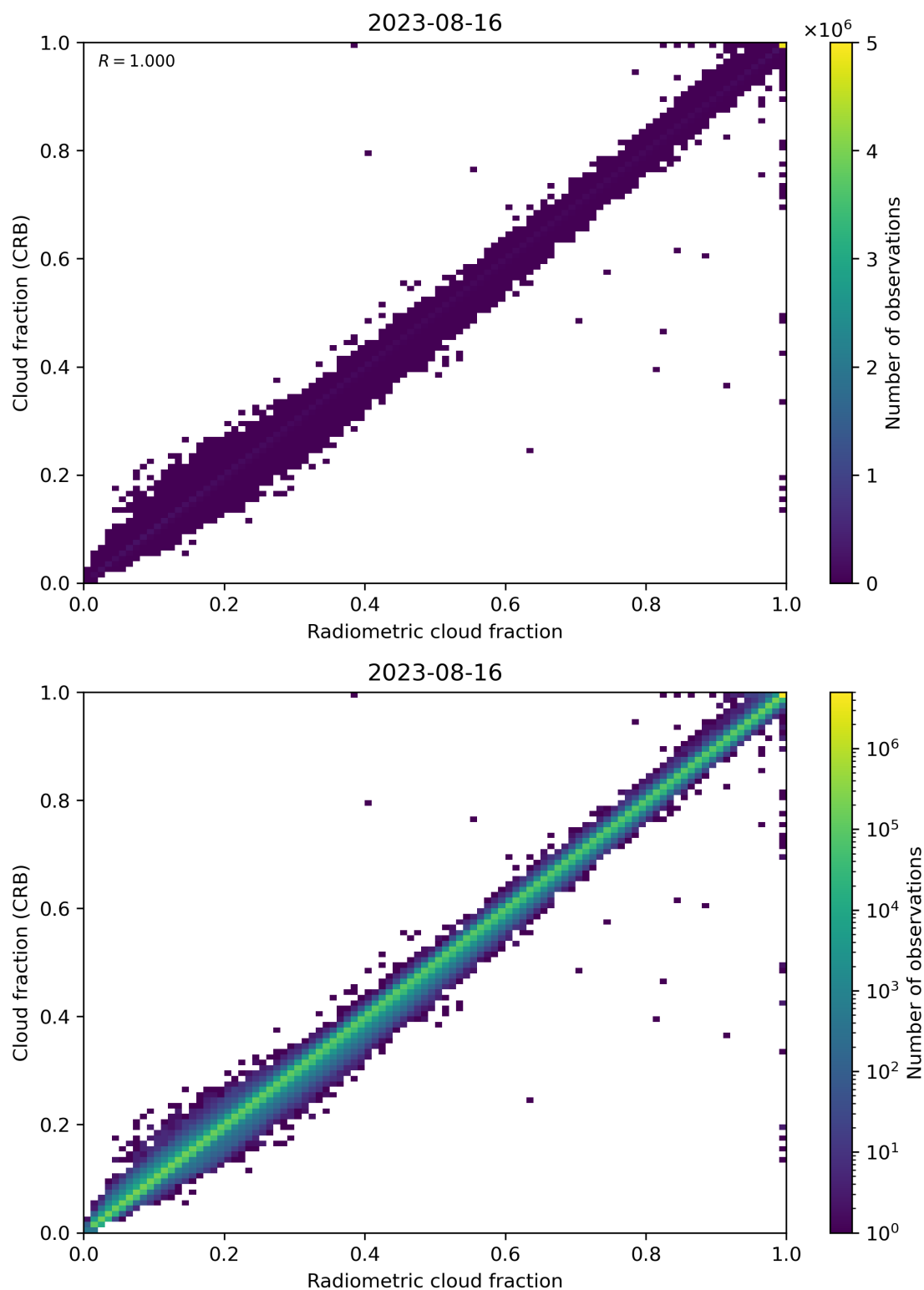
Figure 73: Scatter density plot of “Radiometric cloud fraction” against “Cloud fraction (CRB)” for 2023-08-15 to 2023-08-17.
