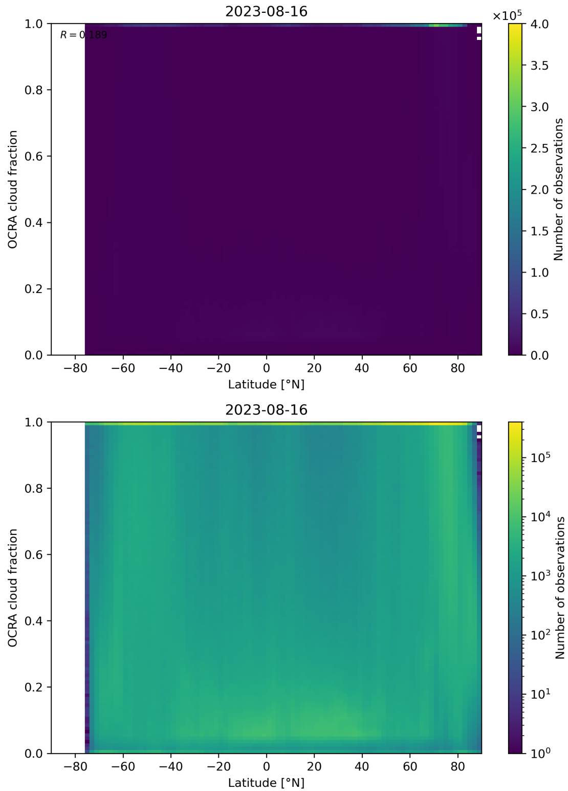
Figure 93: Scatter density plot of “Latitude” against “OCRA cloud fraction” for 2023-08-15 to 2023-08-17.
