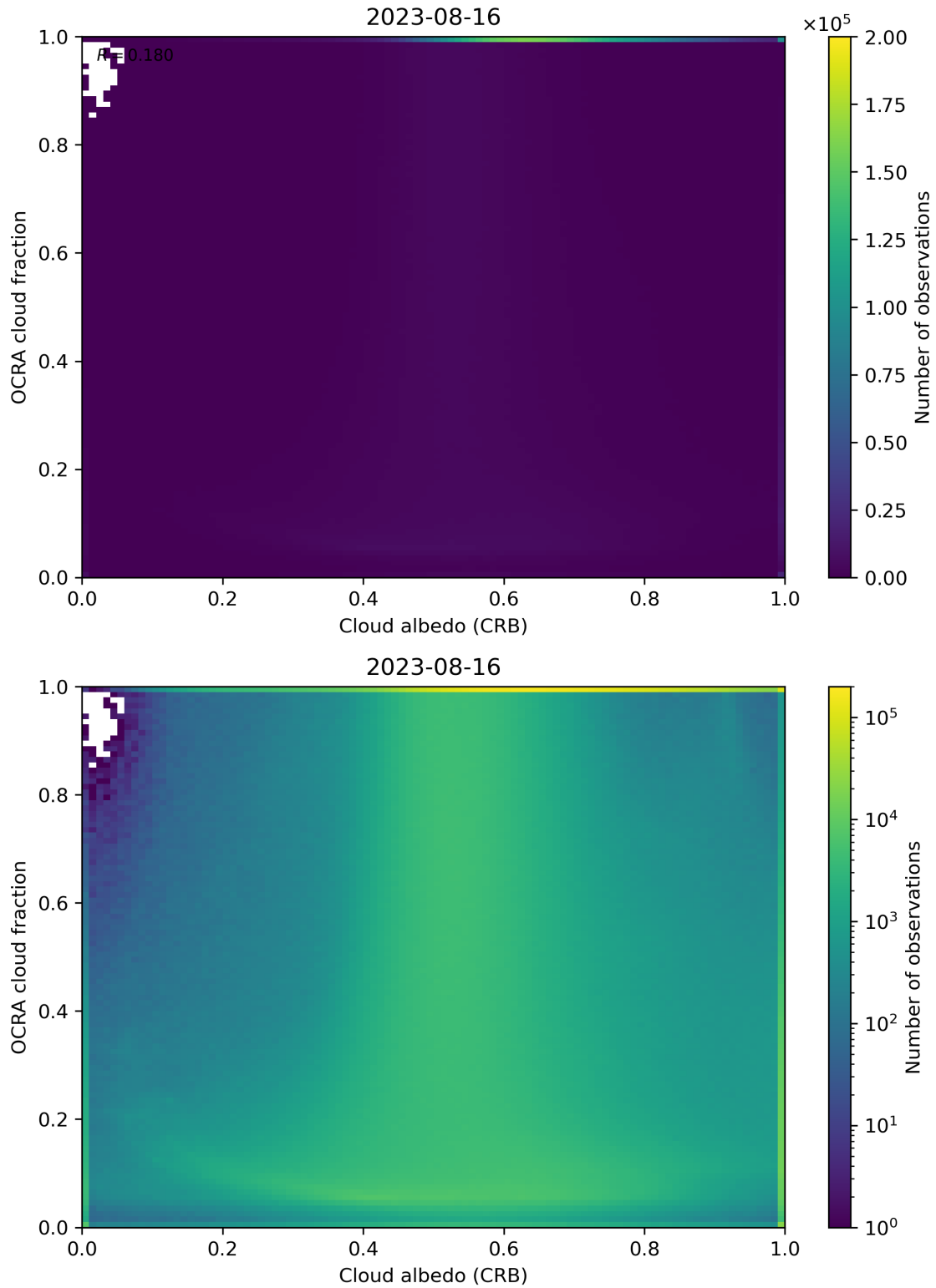
Figure 70: Scatter density plot of “Cloud albedo (CRB)” against “OCRA cloud fraction” for 2023-08-15 to 2023-08-17.
