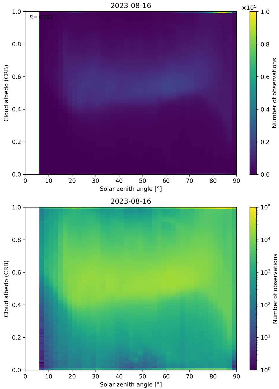
Figure 98: Scatter density plot of “Solar zenith angle” against “Cloud albedo (CRB)” for 2023-08-15 to 2023-08-17.
