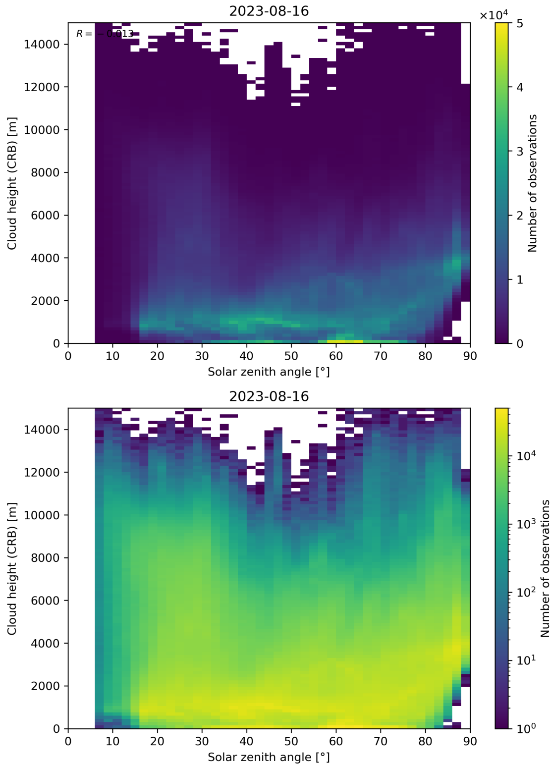
Figure 102: Scatter density plot of “Solar zenith angle” against “Cloud height (CRB)” for 2023-08-15 to 2023-08-17.
