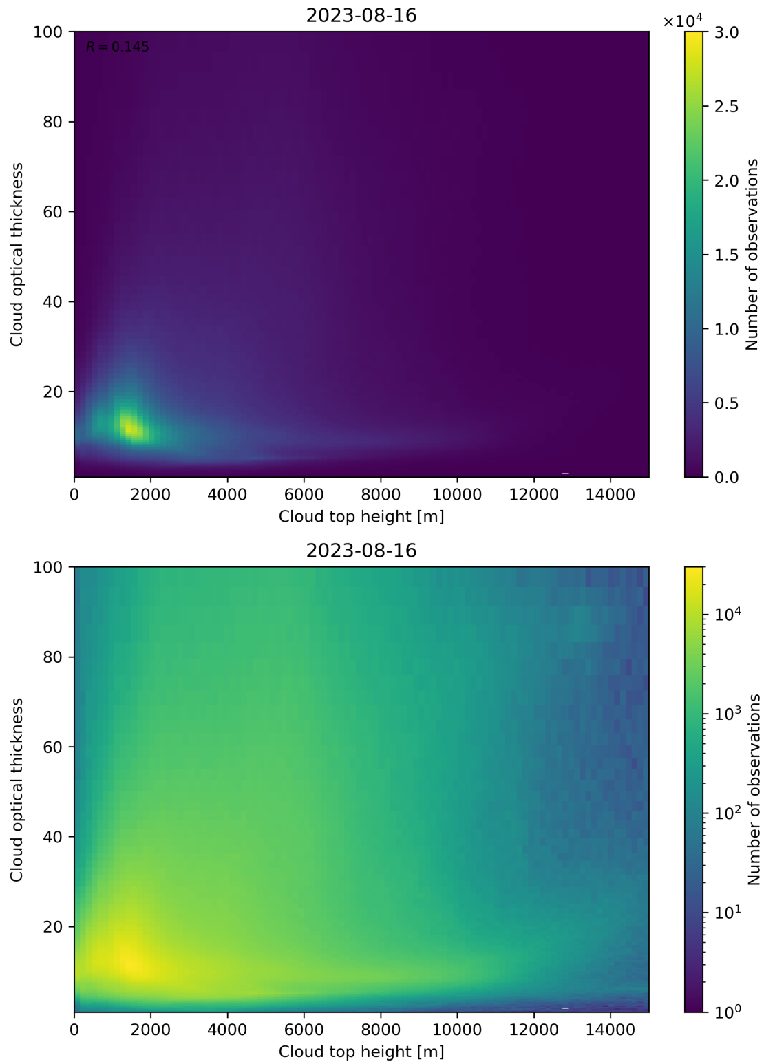
Figure 90: Scatter density plot of “Cloud top height” against “Cloud optical thickness” for 2023-08-15 to 2023-08-17.
