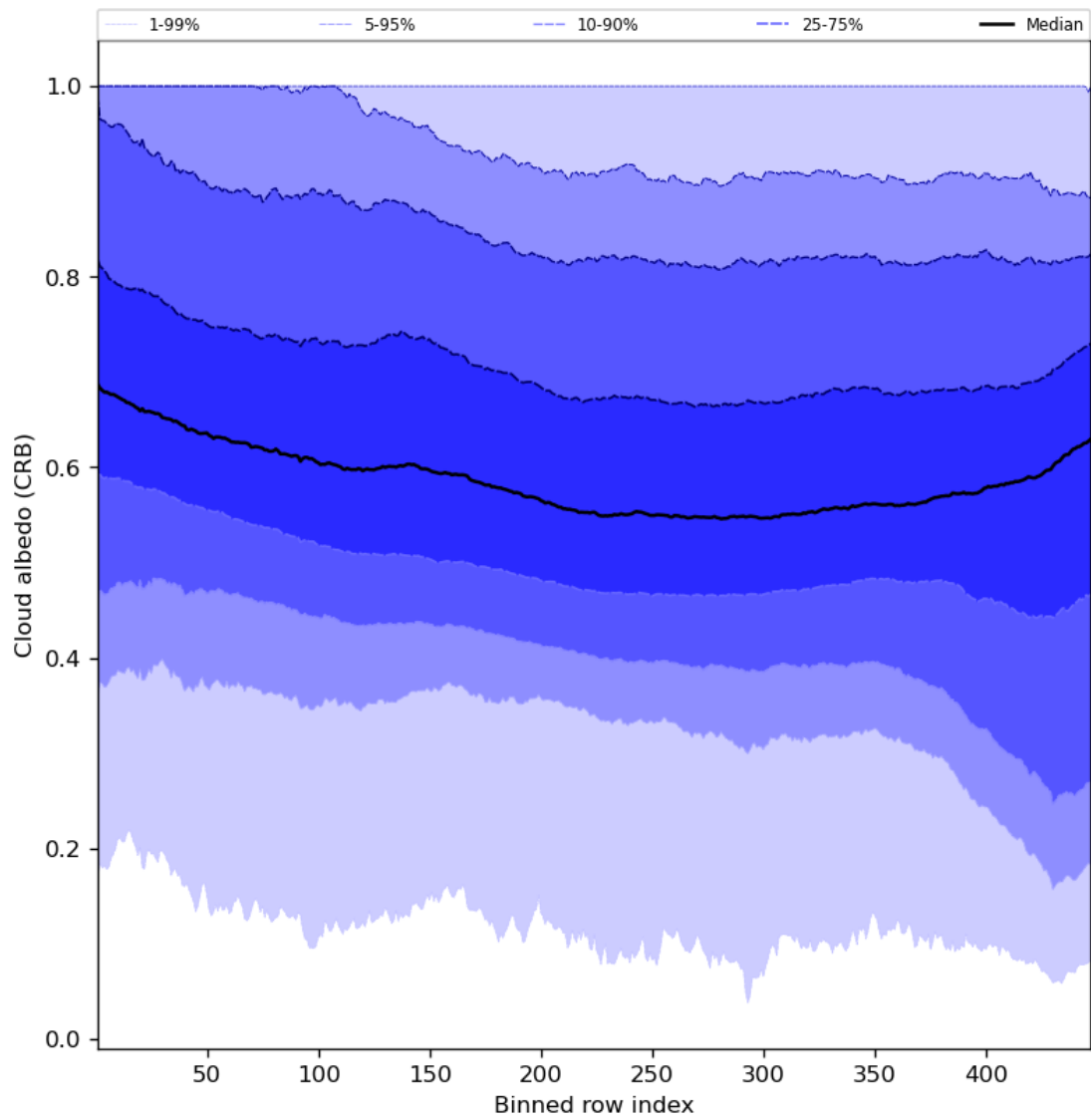
Figure 60: Along track statistics of “Cloud albedo (CRB)” for 2023-08-15 to 2023-08-17
