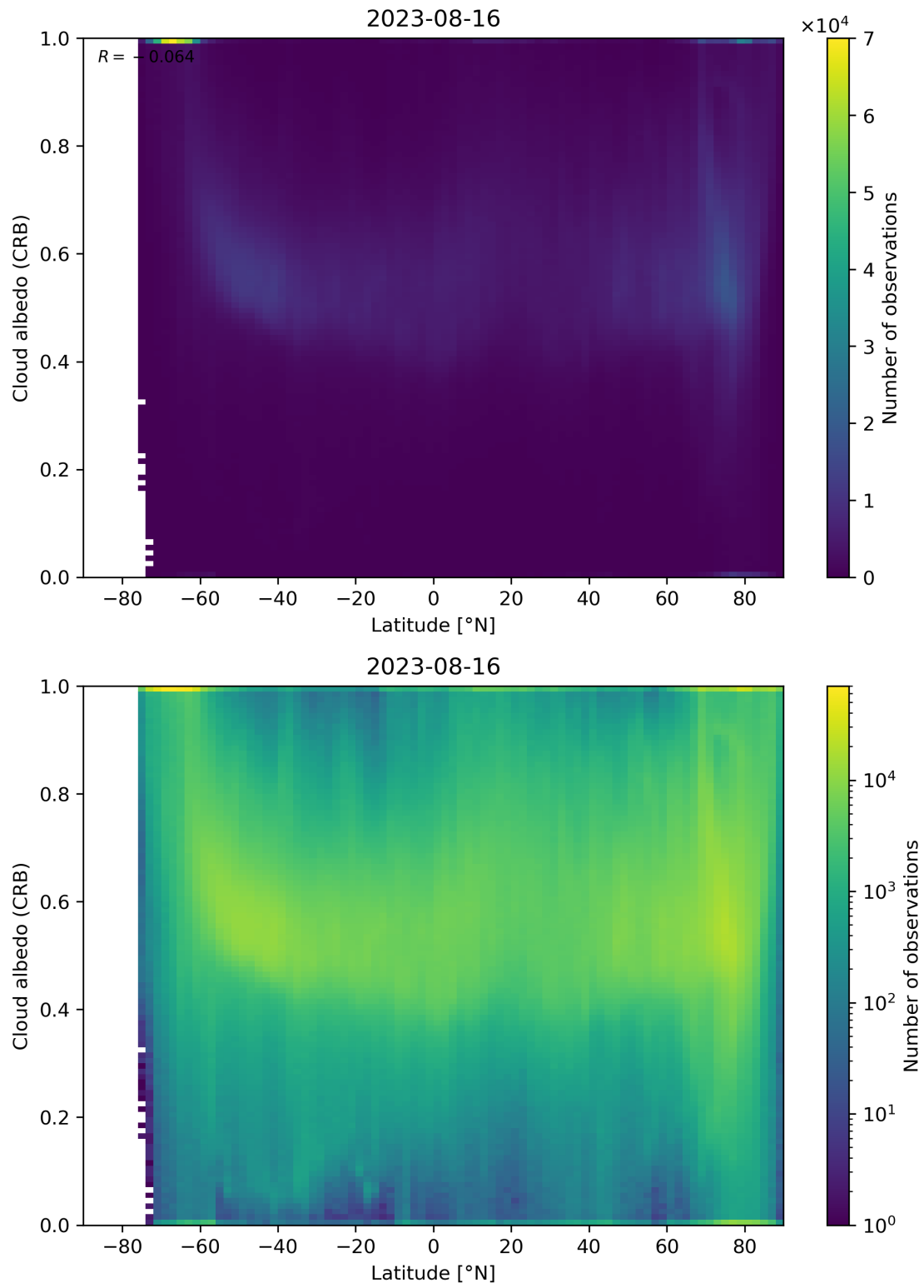
Figure 91: Scatter density plot of “Latitude” against “Cloud albedo (CRB)” for 2023-08-15 to 2023-08-17.
