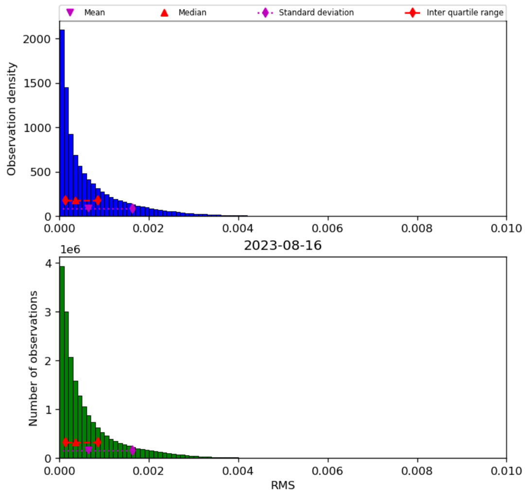
Figure 47: Histogram of “RMS” for 2023-08-15 to 2023-08-17
