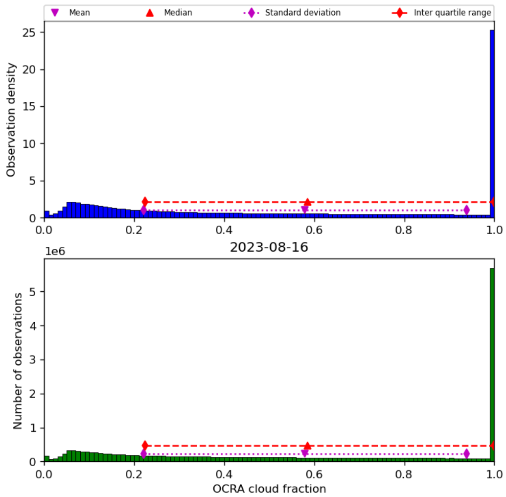
Figure 50: Histogram of “OCRA cloud fraction” for 2023-08-15 to 2023-08-17
