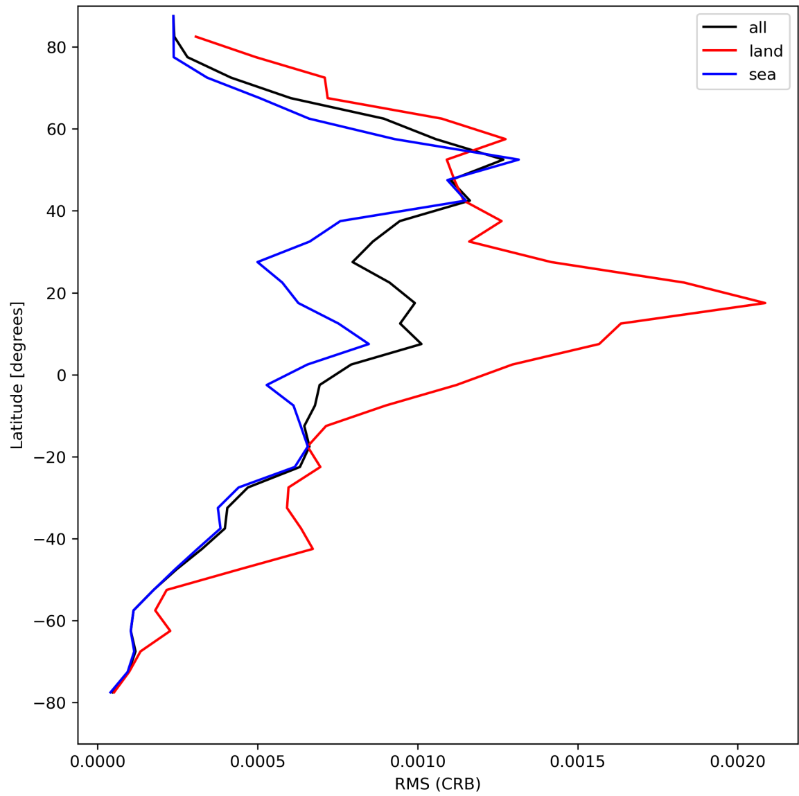
Figure 32: Zonal average of “RMS (CRB)” for 2023-08-15 to 2023-08-17.
