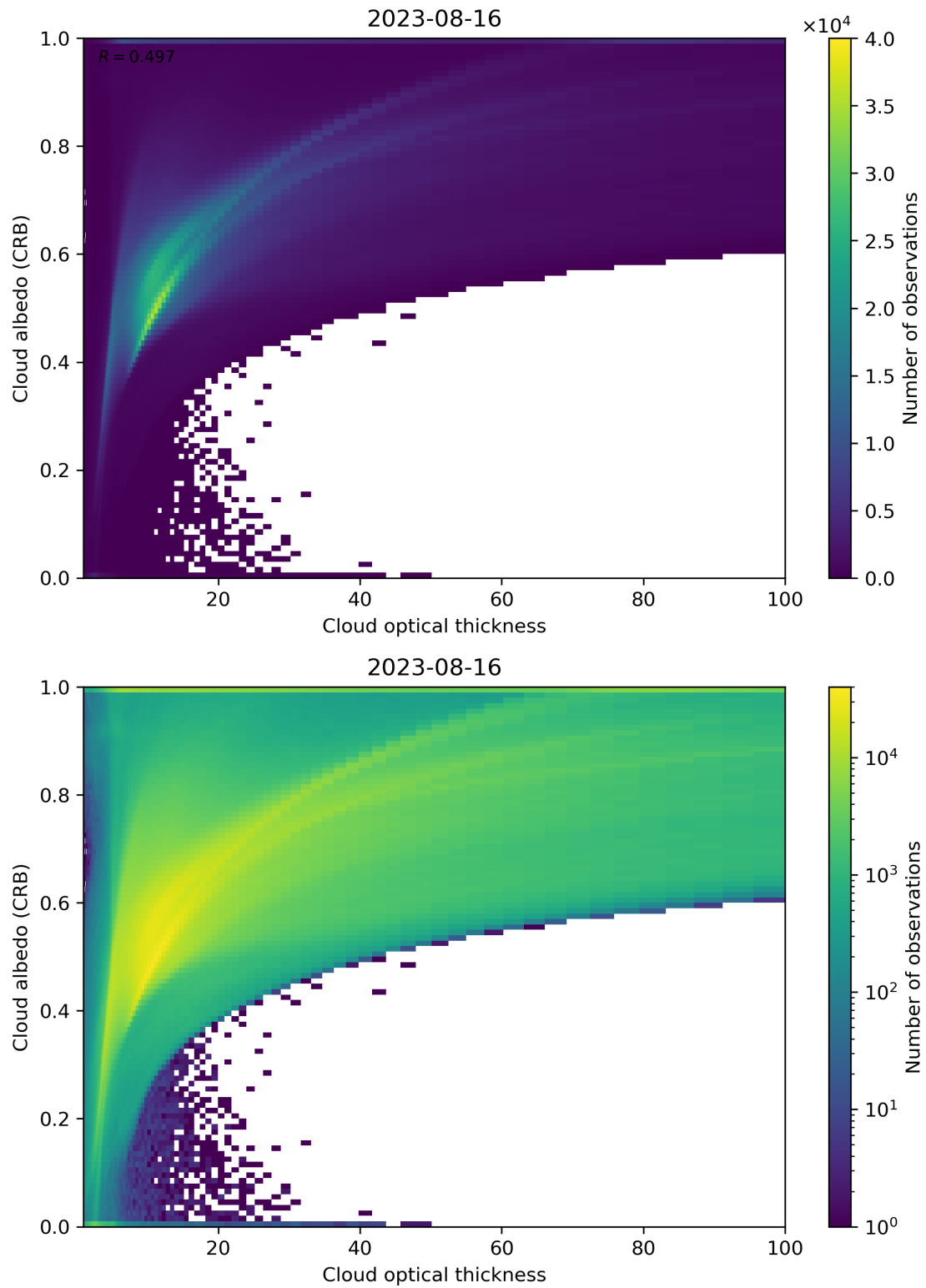
Figure 82: Scatter density plot of “Cloud optical thickness” against “Cloud albedo (CRB)” for 2023-08-15 to 2023-08-17.
