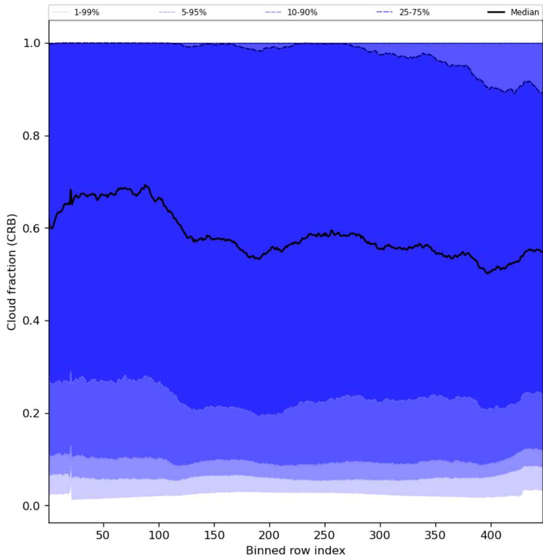
Figure 58: Along track statistics of “Cloud fraction (CRB)” for 2023-08-15 to 2023-08-17
