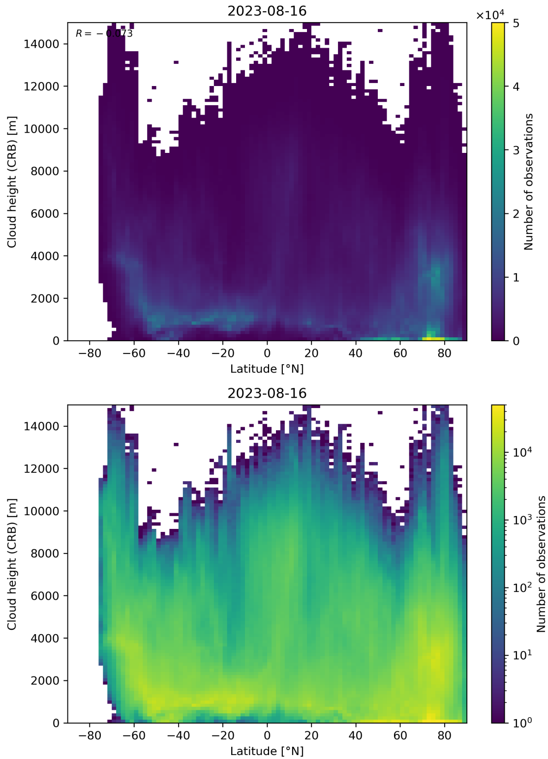
Figure 95: Scatter density plot of “Latitude” against “Cloud height (CRB)” for 2023-08-15 to 2023-08-17.
