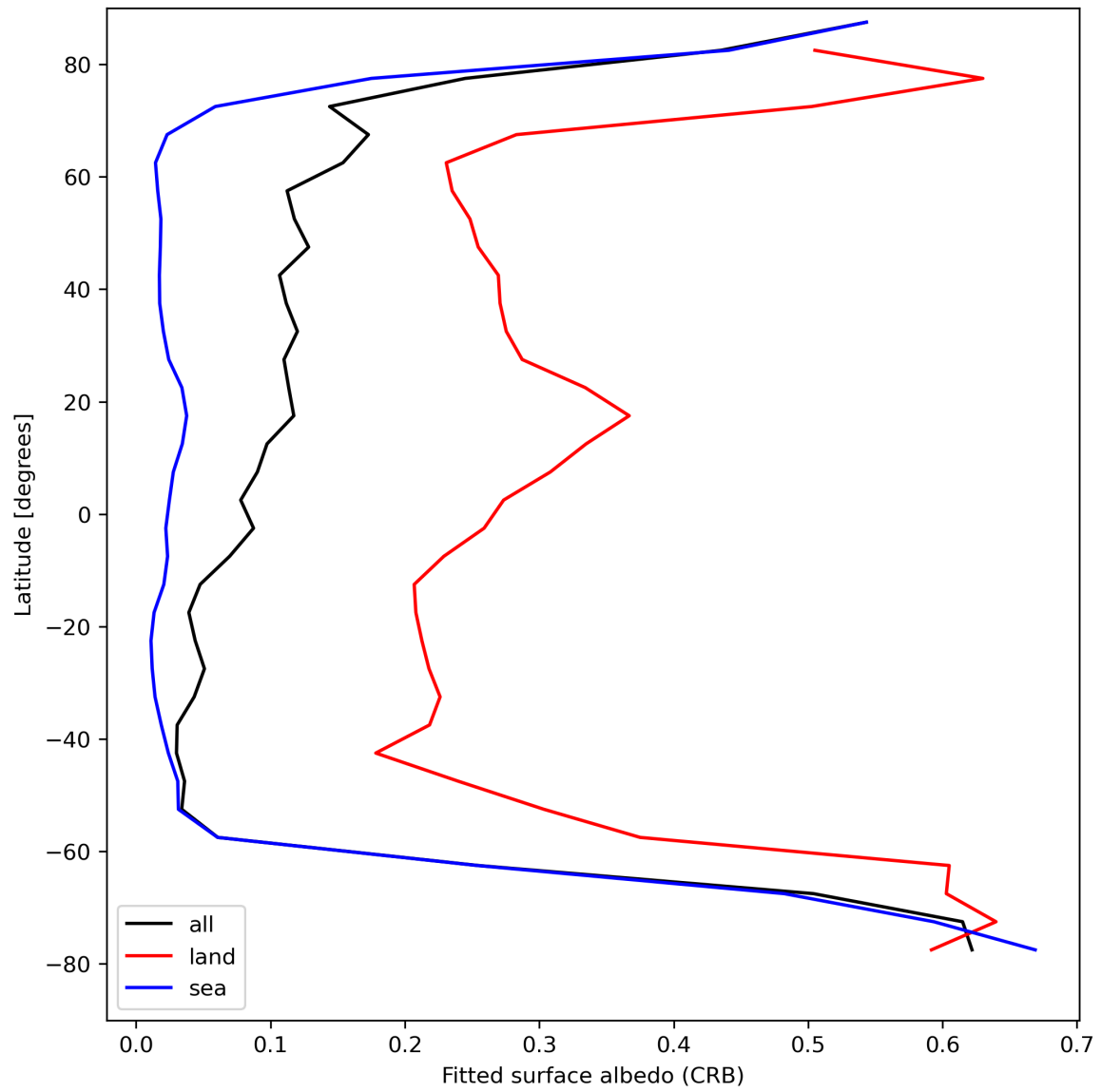
Figure 30: Zonal average of “Fitted surface albedo (CRB)” for 2023-08-15 to 2023-08-17.
