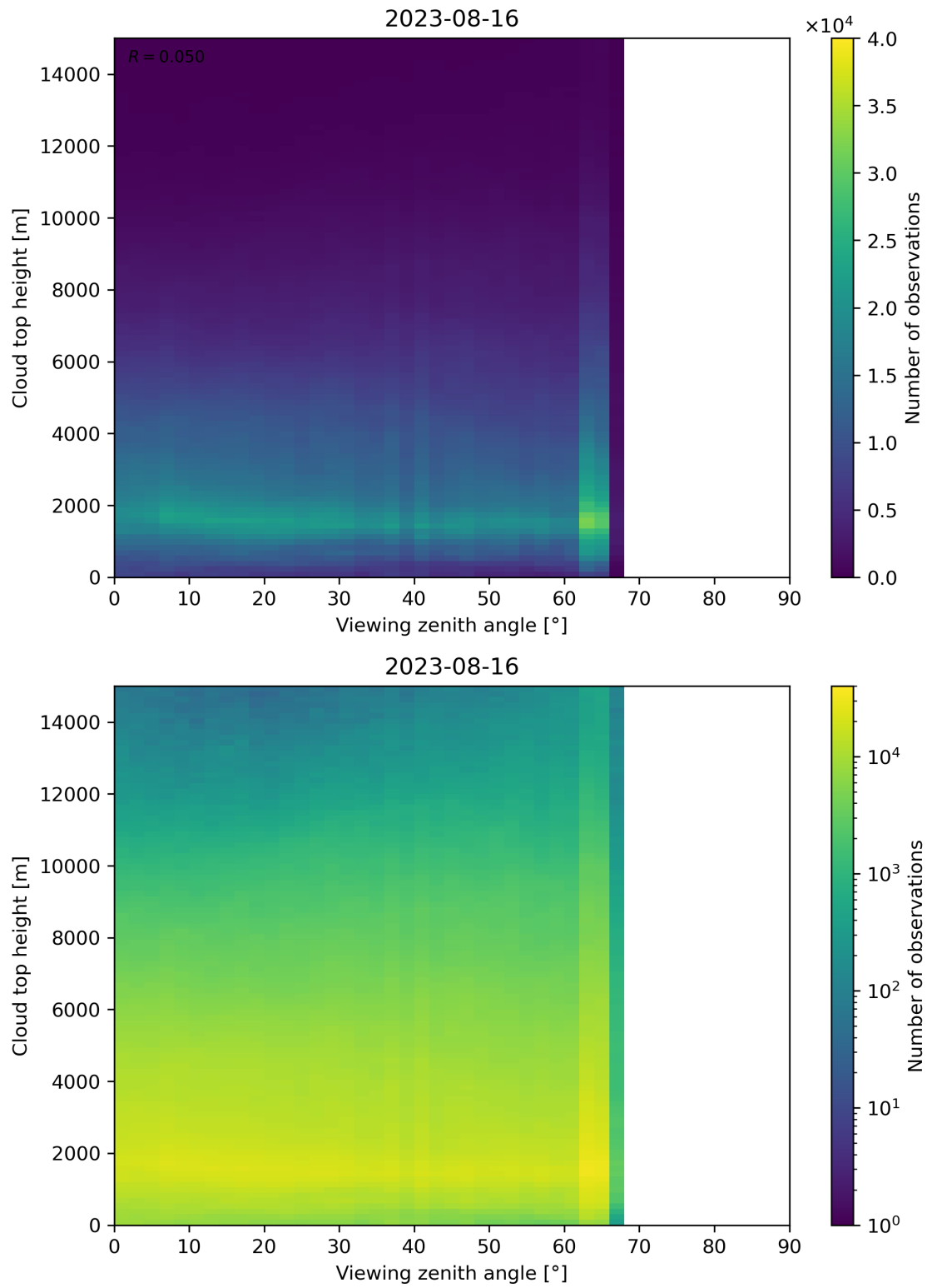
Figure 112: Scatter density plot of “Viewing zenith angle” against “Cloud top height” for 2023-08-15 to 2023-08-17.
