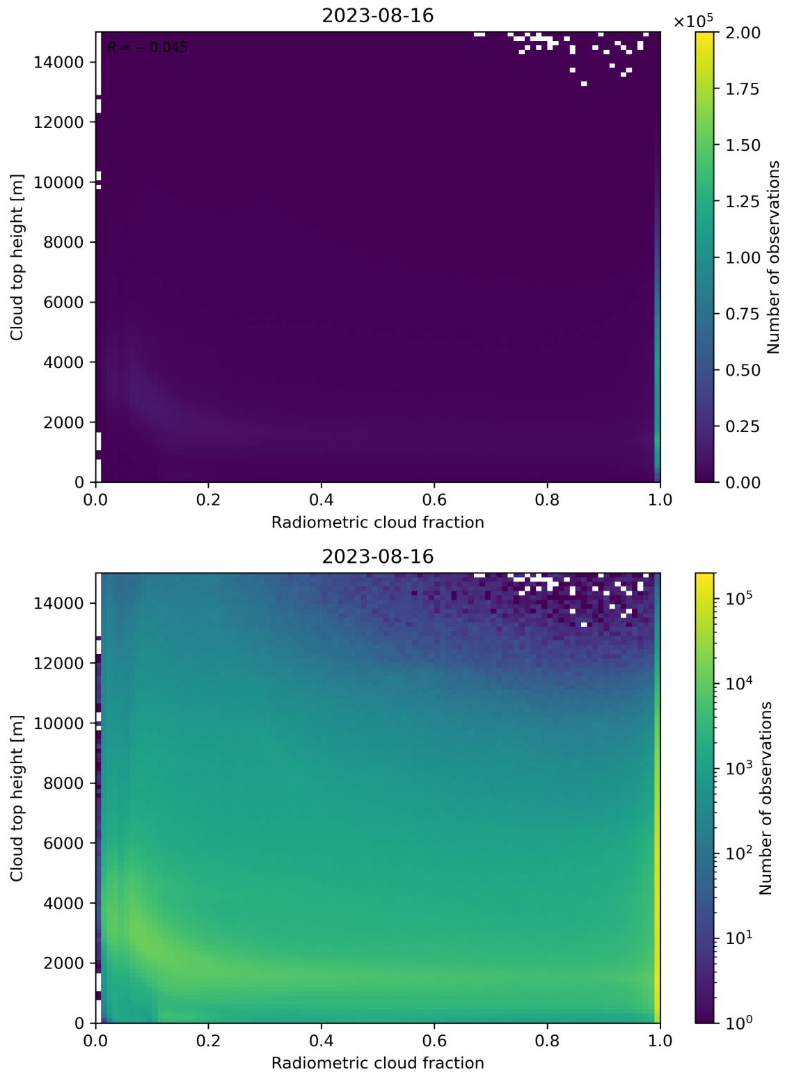
Figure 76: Scatter density plot of “Radiometric cloud fraction” against “Cloud top height” for 2023-08-15 to 2023-08-17.
