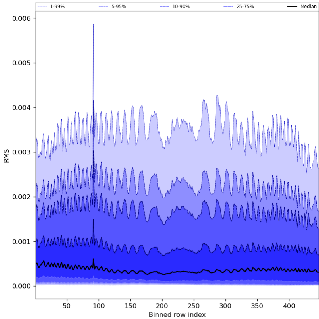
Figure 63: Along track statistics of “RMS” for 2023-08-15 to 2023-08-17
