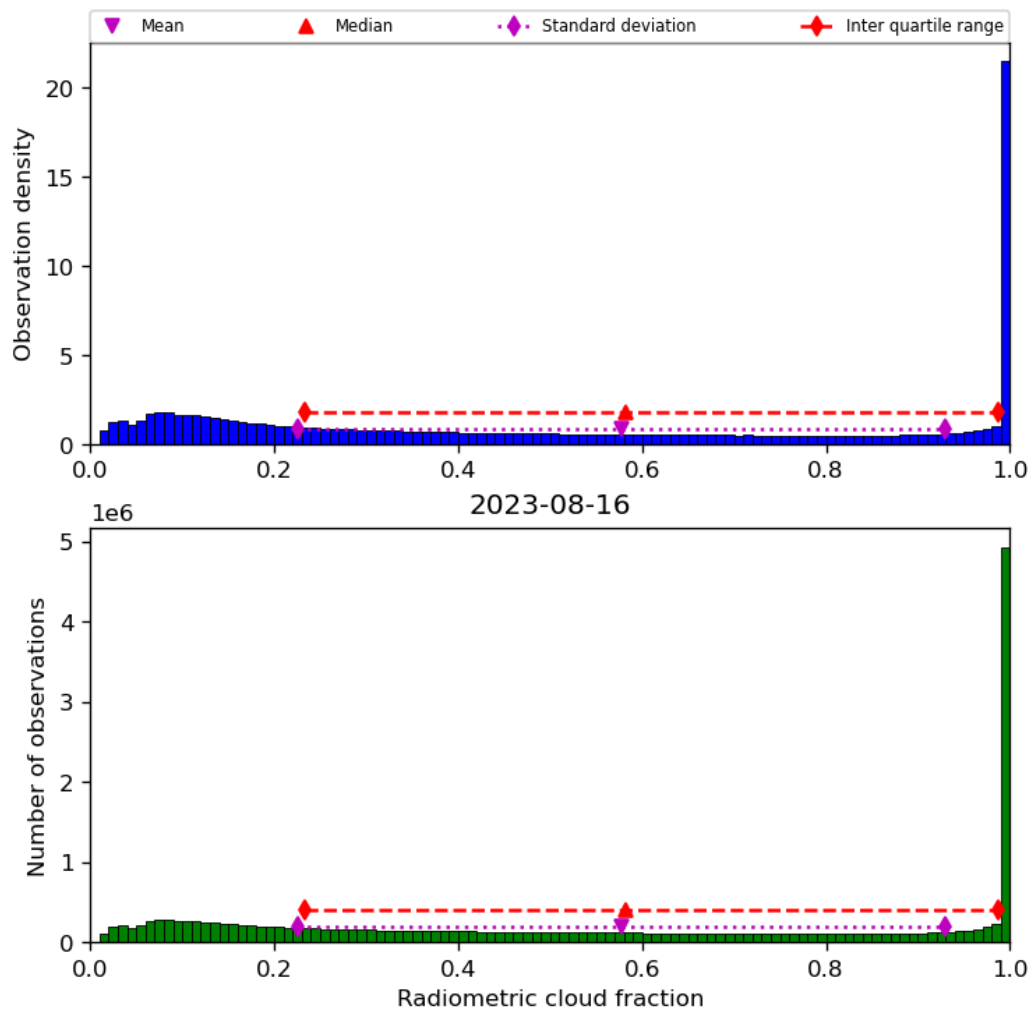
Figure 39: Histogram of “Radiometric cloud fraction” for 2023-08-15 to 2023-08-17
