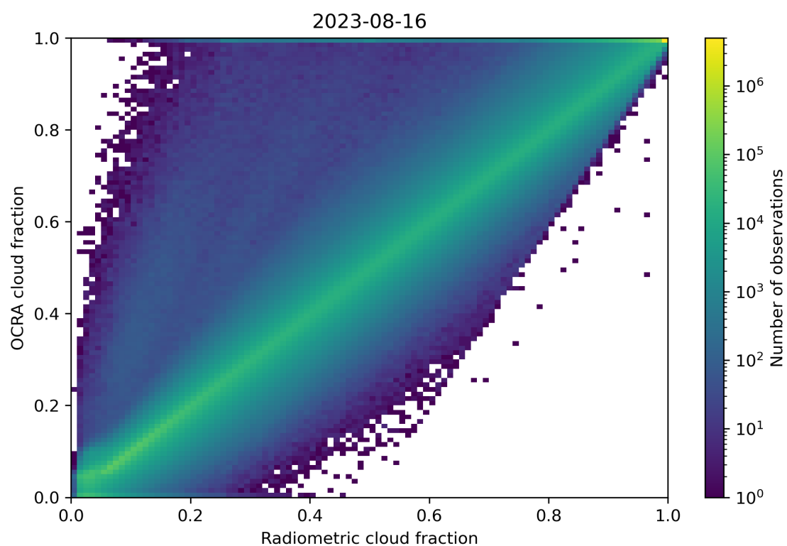
Figure 72: Scatter density plot of “Radiometric cloud fraction” against “OCRA cloud fraction” for 2023-08-15 to 2023-08-17.
