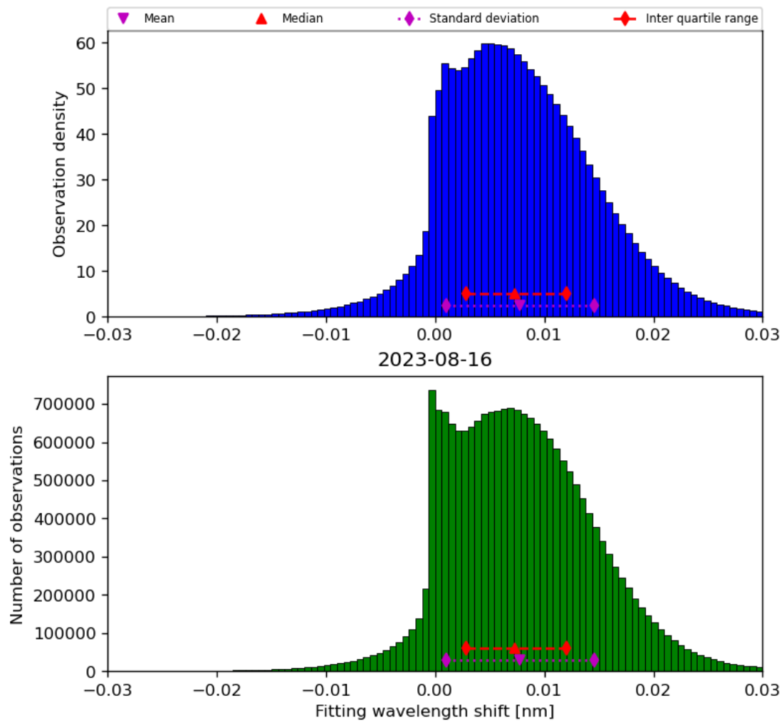
Figure 49: Histogram of “Fitting wavelength shift” for 2023-08-15 to 2023-08-17
