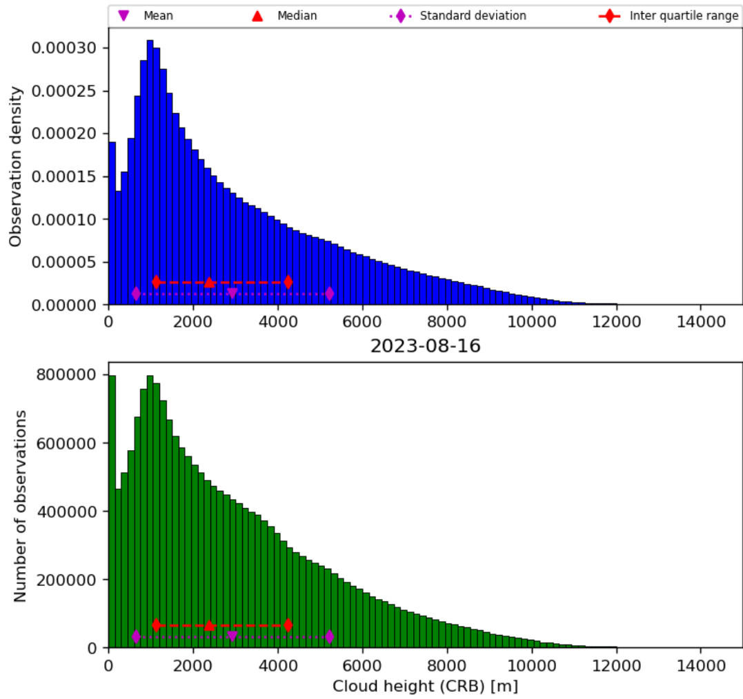
Figure 43: Histogram of “Cloud height (CRB)” for 2023-08-15 to 2023-08-17
