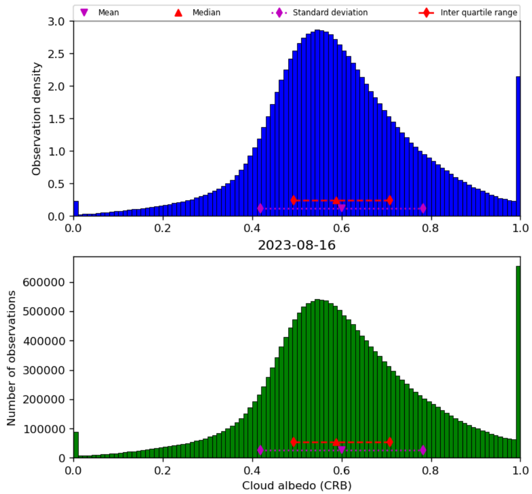
Figure 44: Histogram of “Cloud albedo (CRB)” for 2023-08-15 to 2023-08-17
