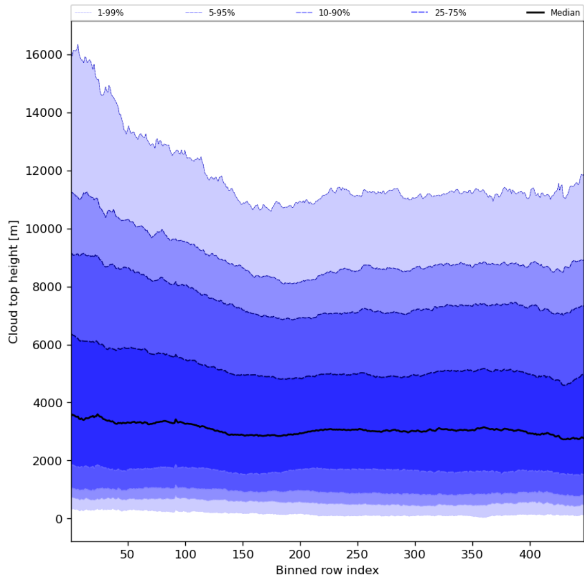
Figure 56: Along track statistics of “Cloud top height” for 2023-08-15 to 2023-08-17
