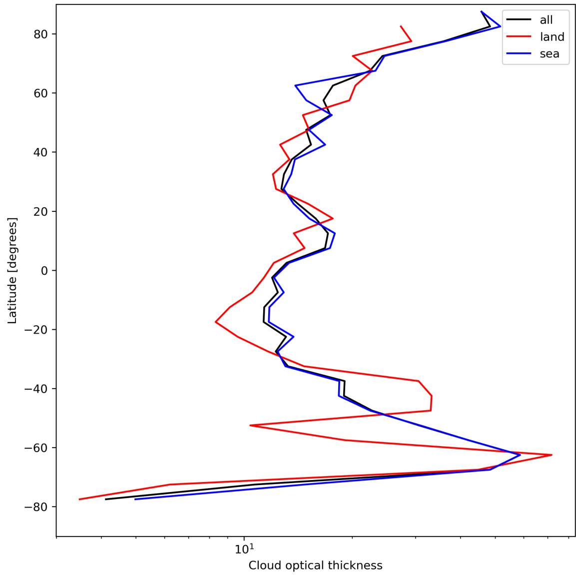
Figure 25: Zonal average of “Cloud optical thickness” for 2023-08-15 to 2023-08-17.
