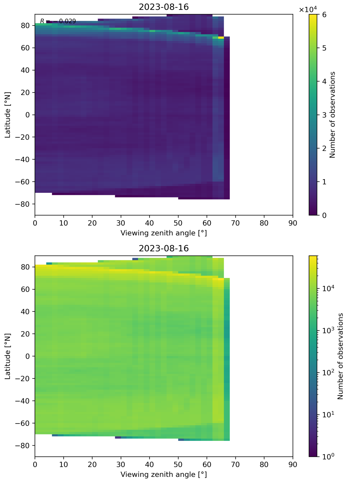
Figure 113: Scatter density plot of “Viewing zenith angle” against “Latitude” for 2023-08-15 to 2023-08-17.
