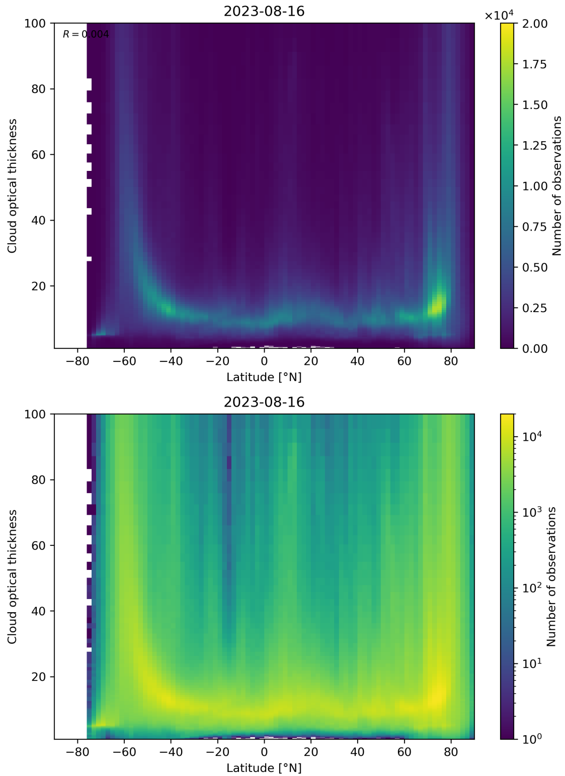
Figure 96: Scatter density plot of “Latitude” against “Cloud optical thickness” for 2023-08-15 to 2023-08-17.
