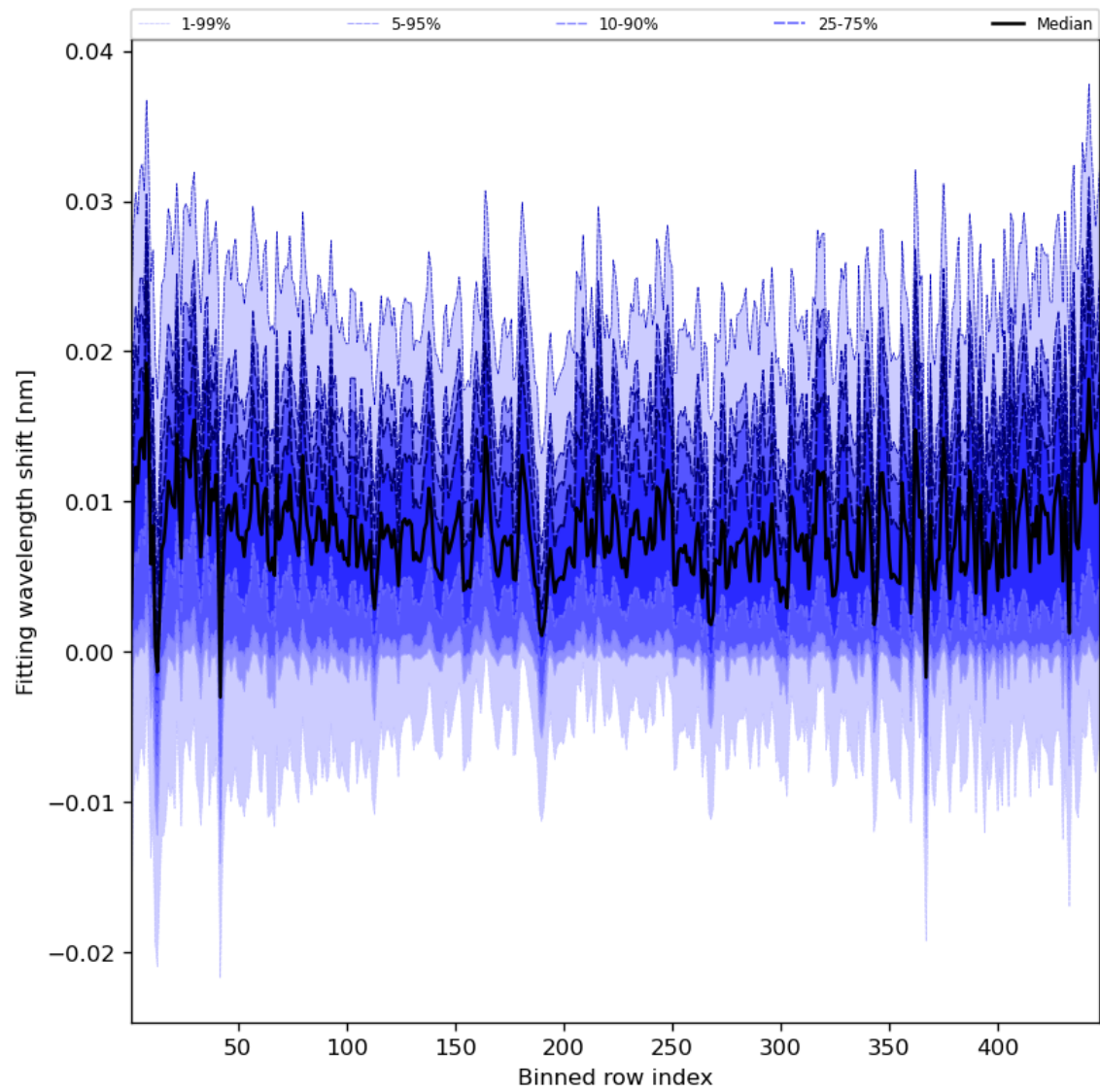
Figure 65: Along track statistics of “Fitting wavelength shift” for 2023-08-15 to 2023-08-17
