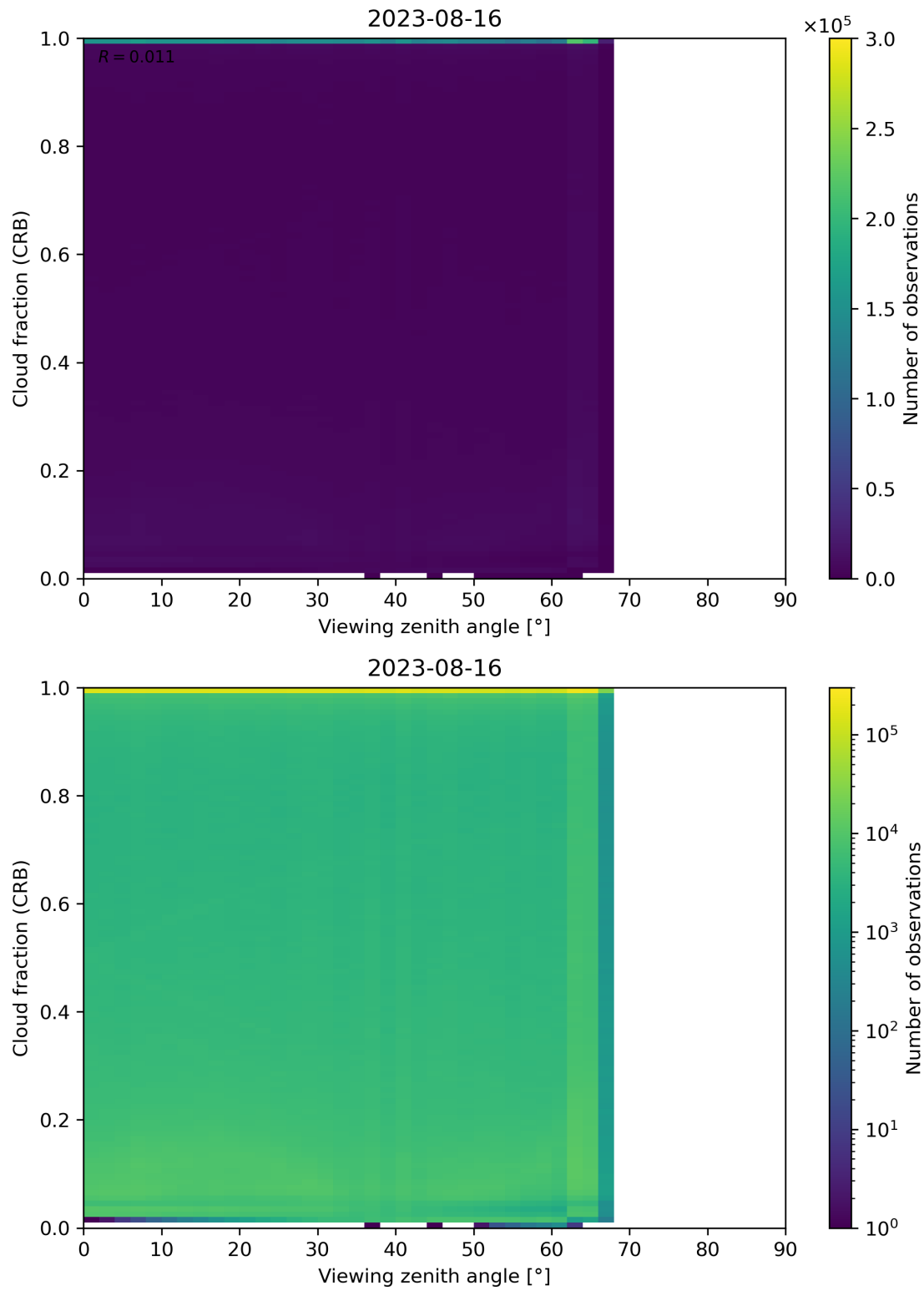
Figure 109: Scatter density plot of “Viewing zenith angle” against “Cloud fraction (CRB)” for 2023-08-15 to 2023-08-17.
