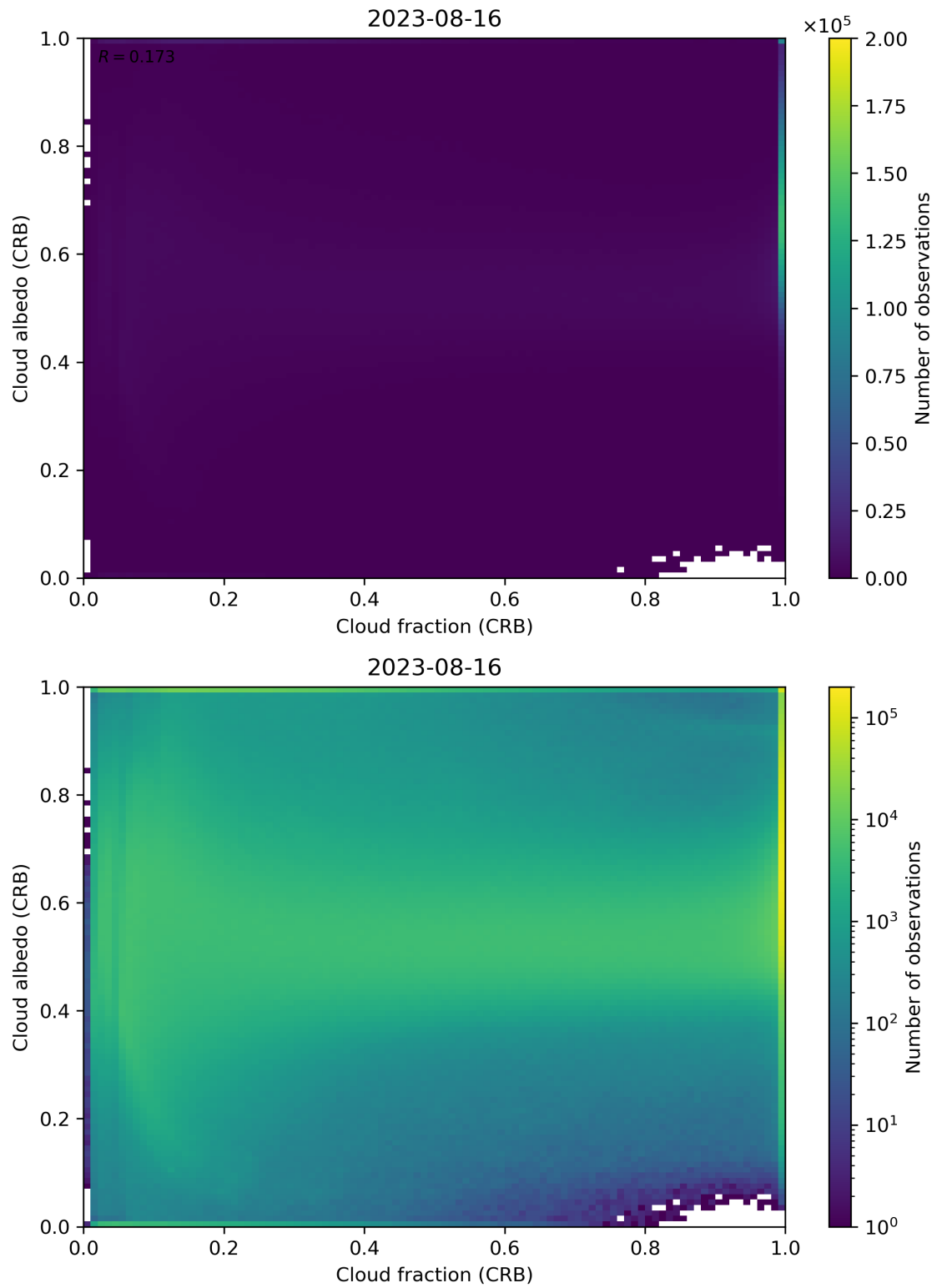
Figure 77: Scatter density plot of “Cloud fraction (CRB)” against “Cloud albedo (CRB)” for 2023-08-15 to 2023-08-17.
