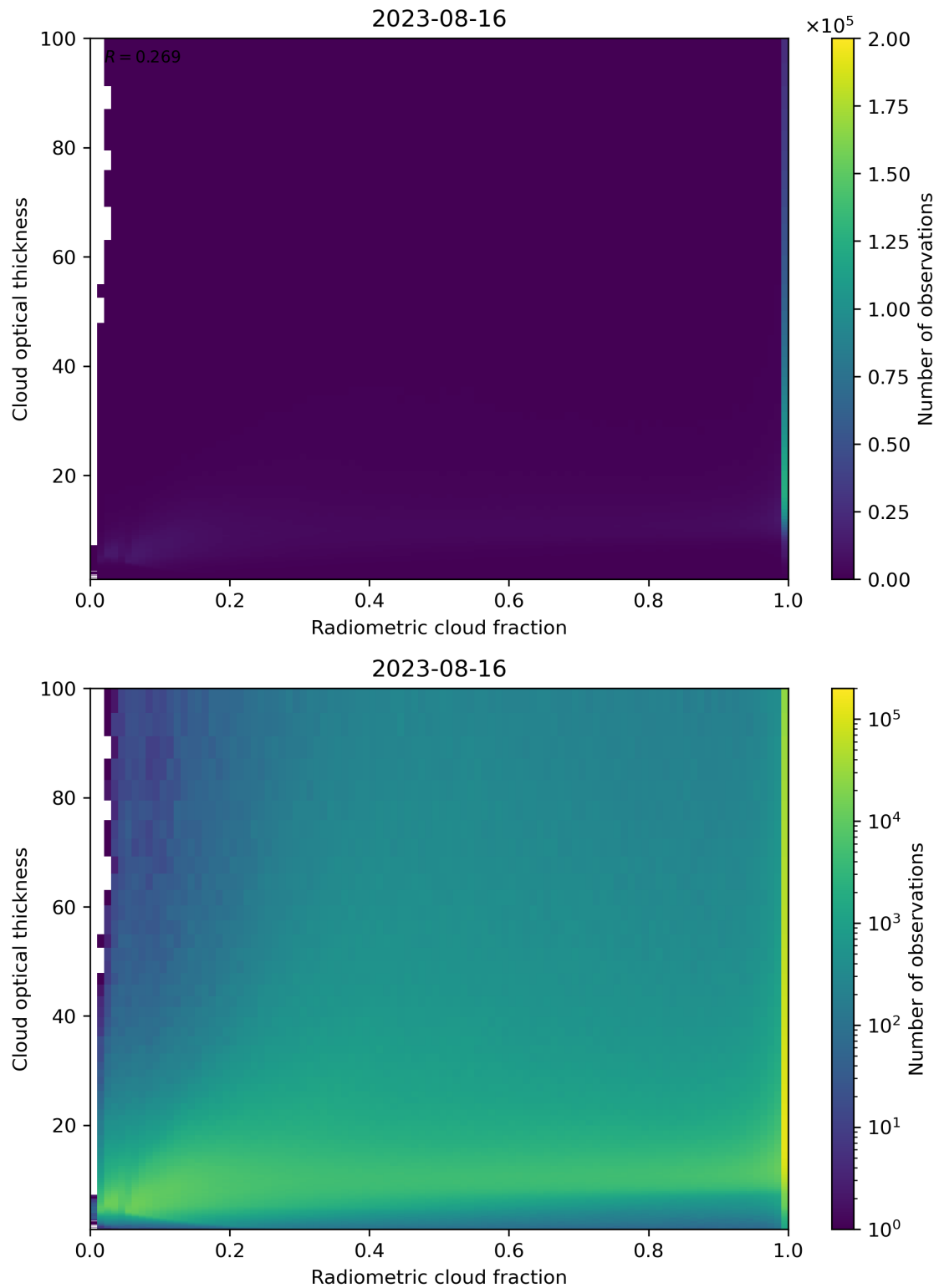
Figure 75: Scatter density plot of “Radiometric cloud fraction” against “Cloud optical thickness” for 2023-08-15 to 2023-08-17.
