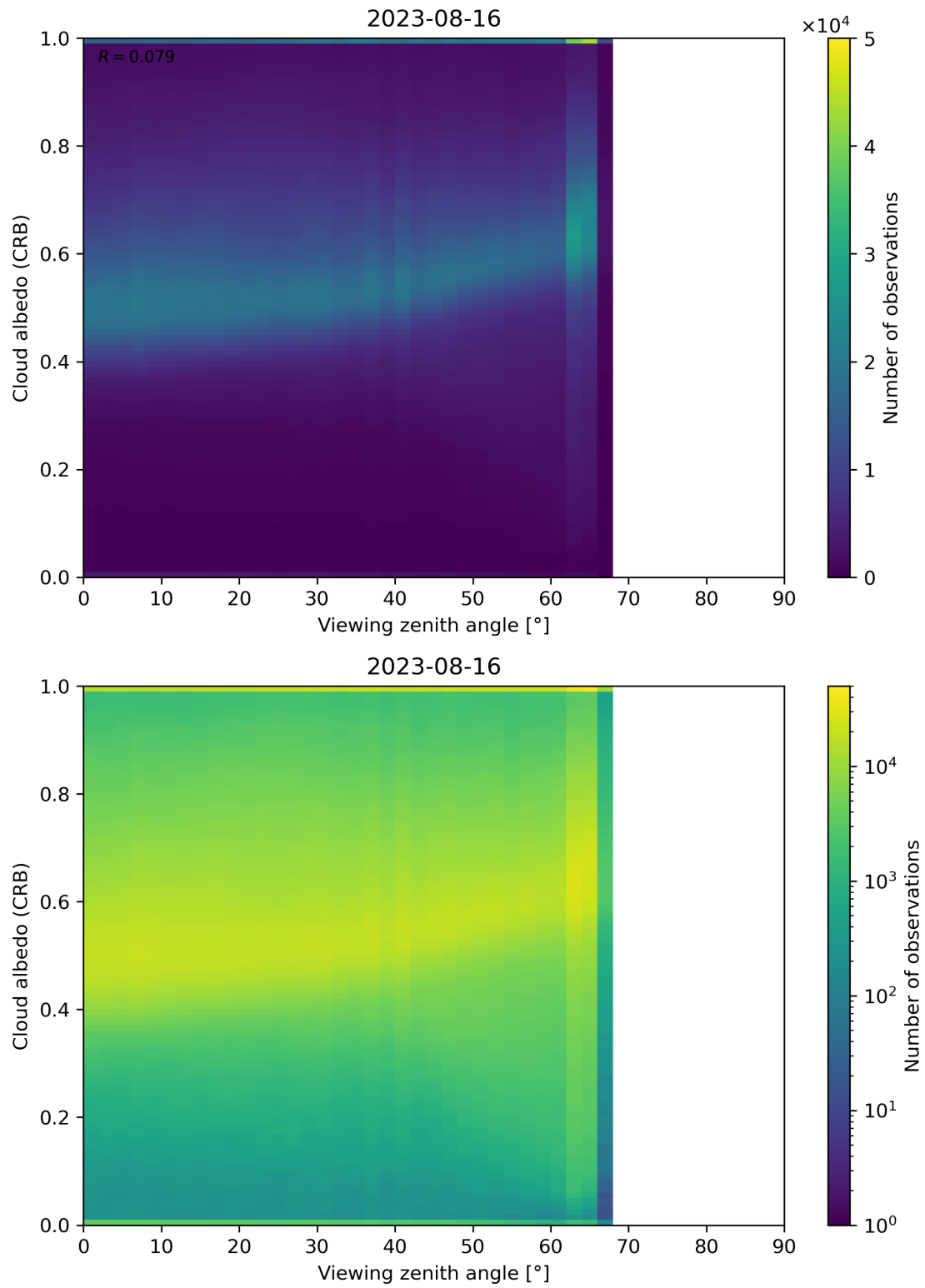
Figure 106: Scatter density plot of “Viewing zenith angle” against “Cloud albedo (CRB)” for 2023-08-15 to 2023-08-17.
