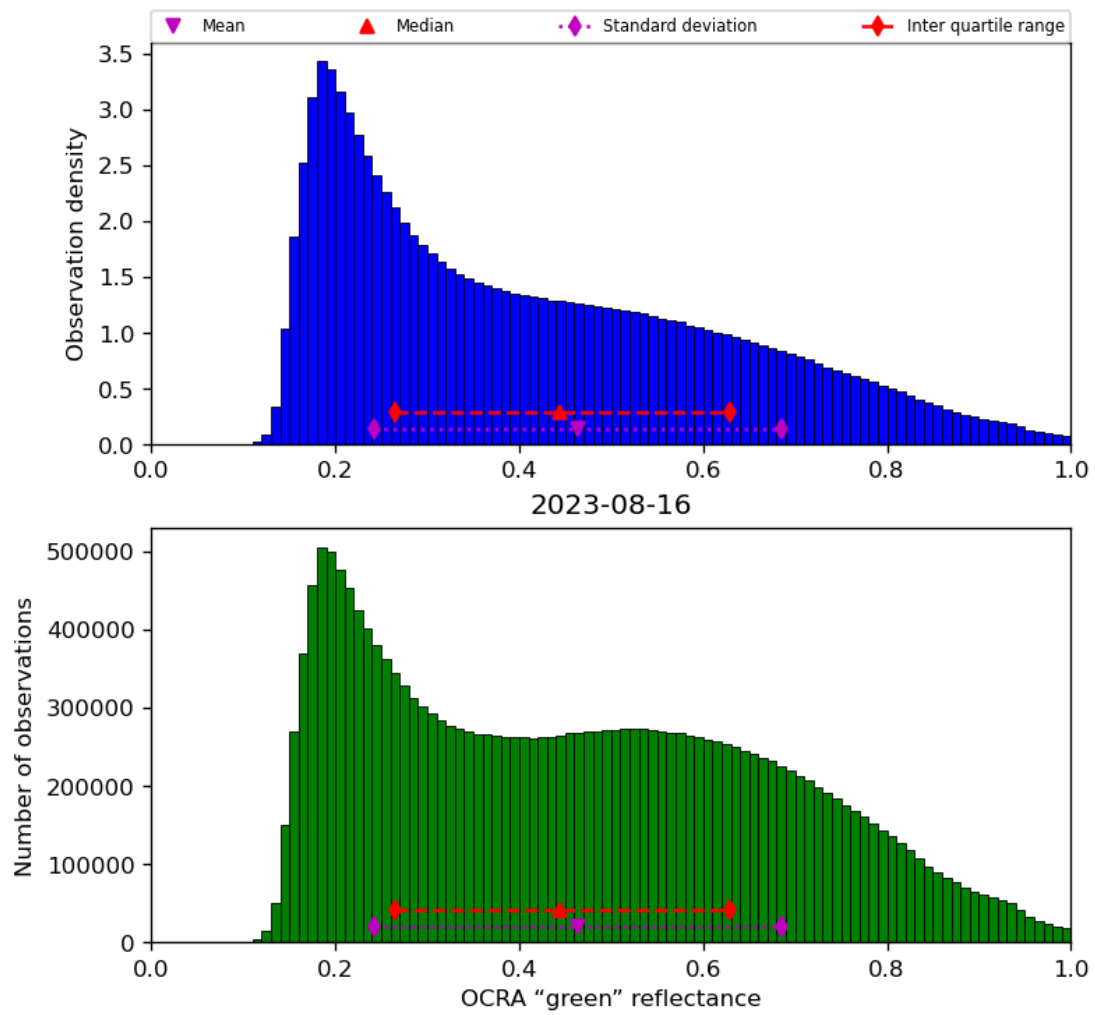
Figure 52: Histogram of “OCRA “green” reflectance” for 2023-08-15 to 2023-08-17
