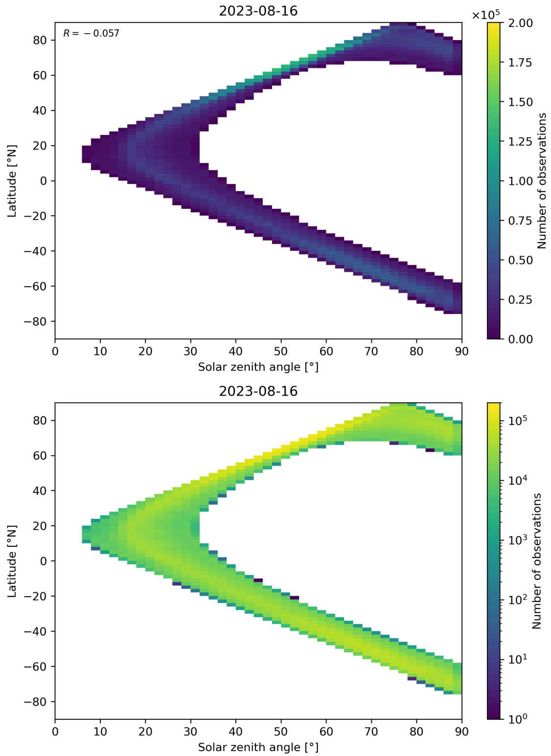
Figure 105: Scatter density plot of “Solar zenith angle” against “Latitude” for 2023-08-15 to 2023-08-17.
