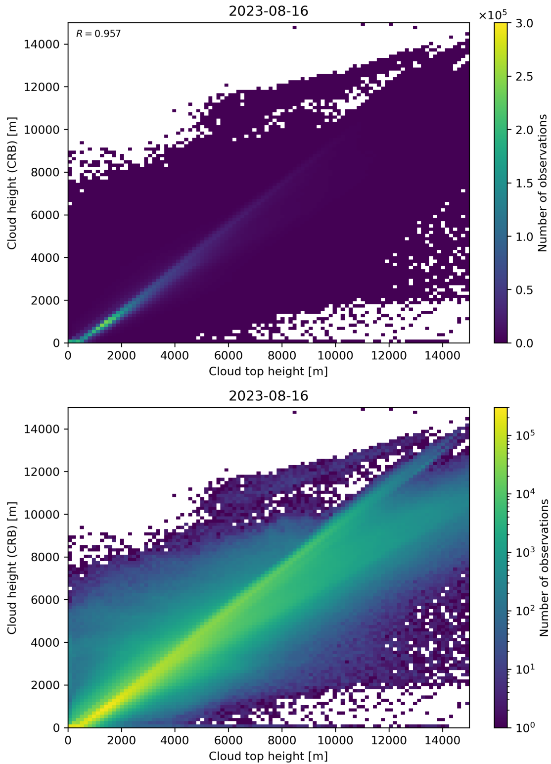
Figure 89: Scatter density plot of “Cloud top height” against “Cloud height (CRB)” for 2023-08-15 to 2023-08-17.
