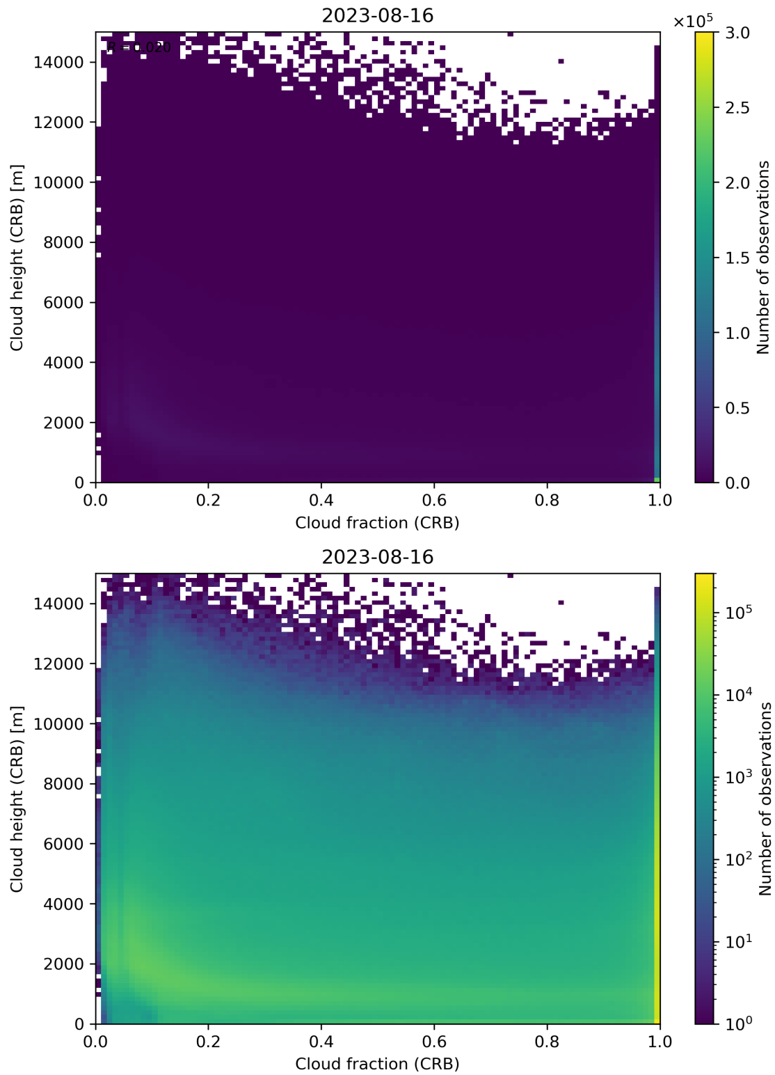
Figure 79: Scatter density plot of “Cloud fraction (CRB)” against “Cloud height (CRB)” for 2023-08-15 to 2023-08-17.
