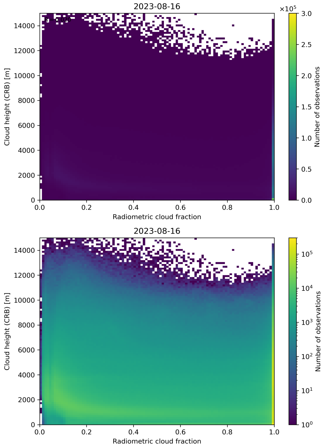
Figure 74: Scatter density plot of “Radiometric cloud fraction” against “Cloud height (CRB)” for 2023-08-15 to 2023-08-17.
