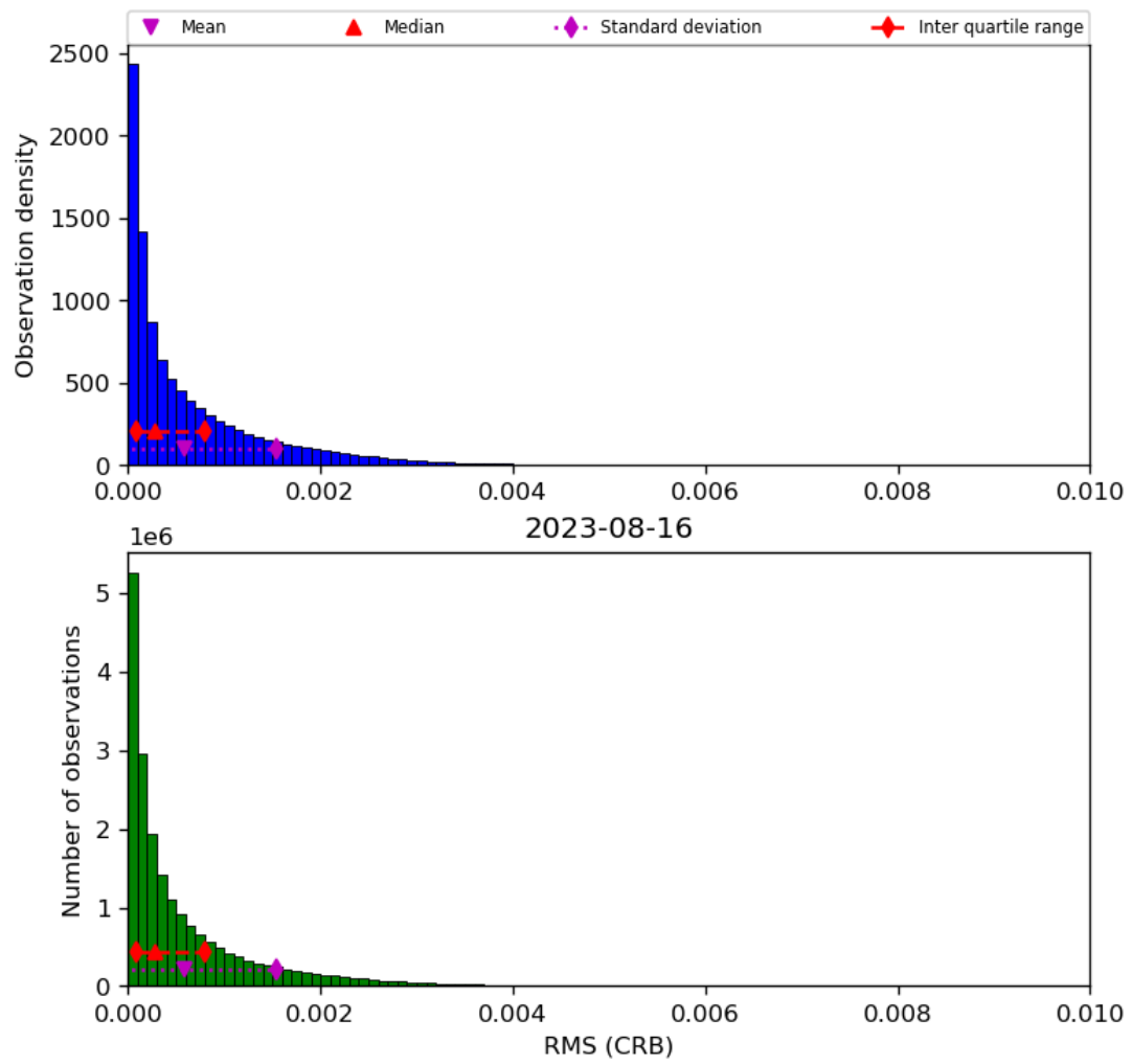
Figure 48: Histogram of “RMS (CRB)” for 2023-08-15 to 2023-08-17
