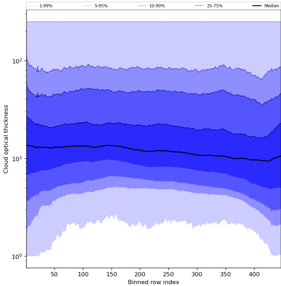
Figure 57: Along track statistics of “Cloud optical thickness” for 2023-08-15 to 2023-08-17
