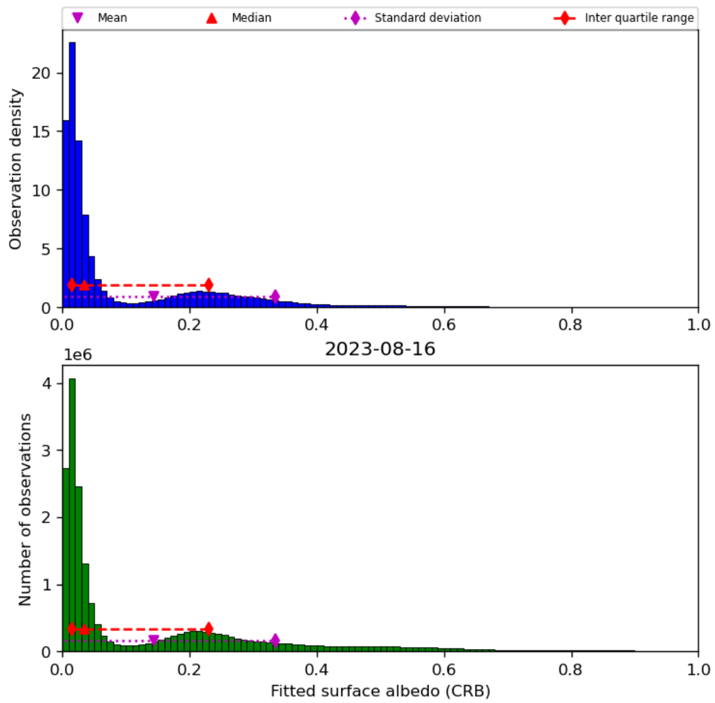
Figure 46: Histogram of “Fitted surface albedo (CRB)” for 2023-08-15 to 2023-08-17
