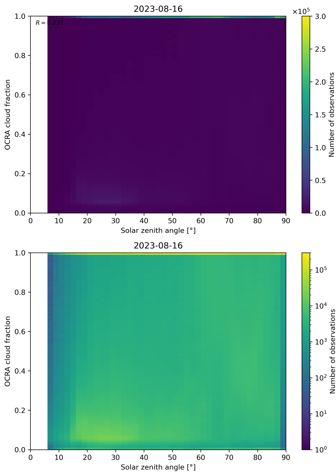
Figure 100: Scatter density plot of “Solar zenith angle” against “OCRA cloud fraction” for 2023-08-15 to 2023-08-17.
