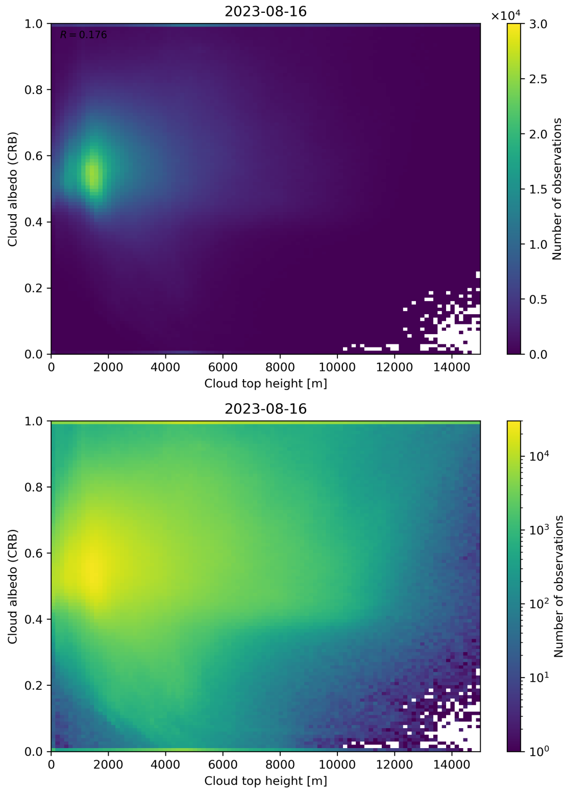
Figure 86: Scatter density plot of “Cloud top height” against “Cloud albedo (CRB)” for 2023-08-15 to 2023-08-17.
