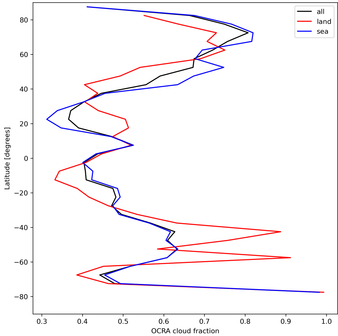
Figure 34: Zonal average of “OCRA cloud fraction” for 2023-08-15 to 2023-08-17.
