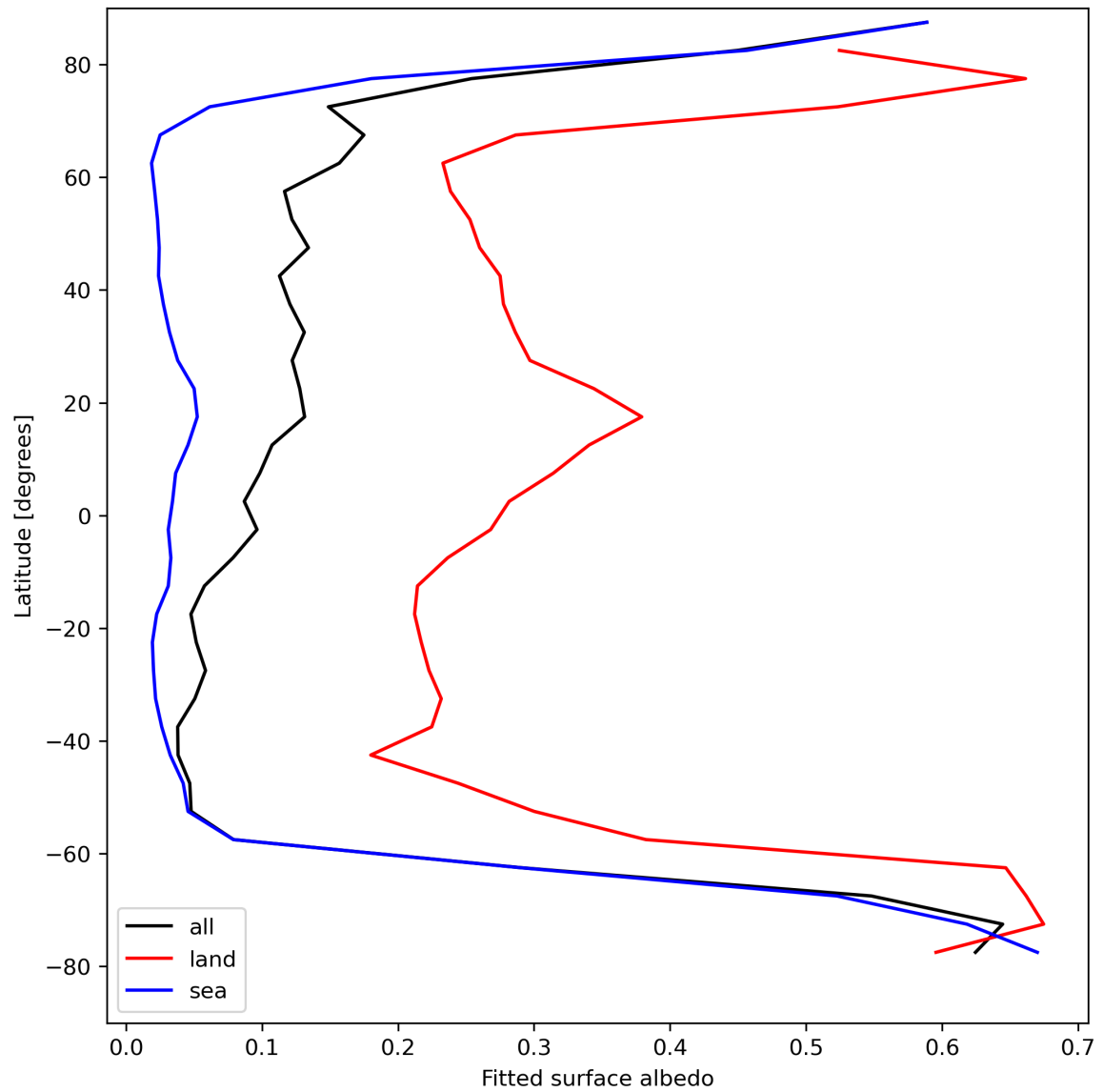
Figure 29: Zonal average of “Fitted surface albedo” for 2023-08-15 to 2023-08-17.
