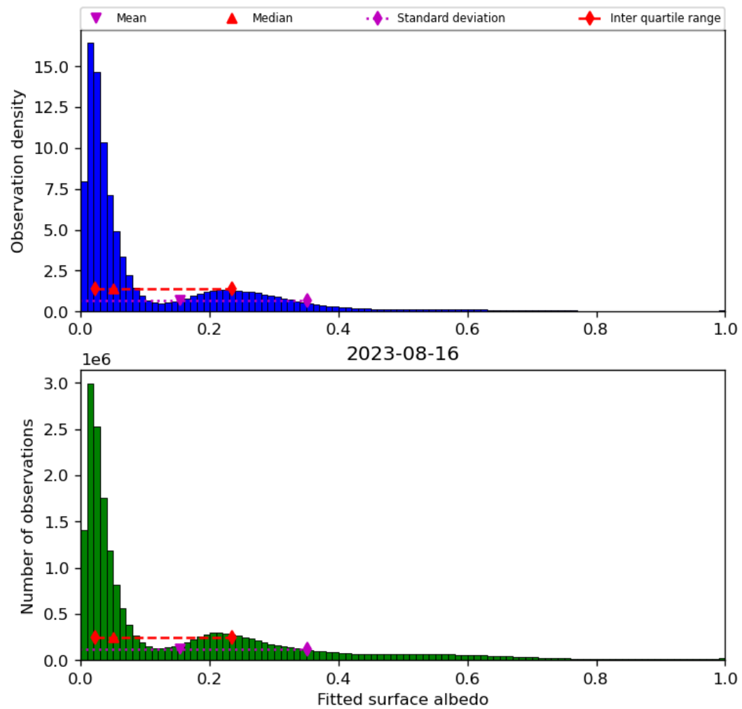
Figure 45: Histogram of “Fitted surface albedo” for 2023-08-15 to 2023-08-17
