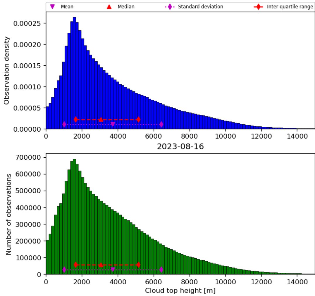
Figure 40: Histogram of “Cloud top height” for 2023-08-15 to 2023-08-17
