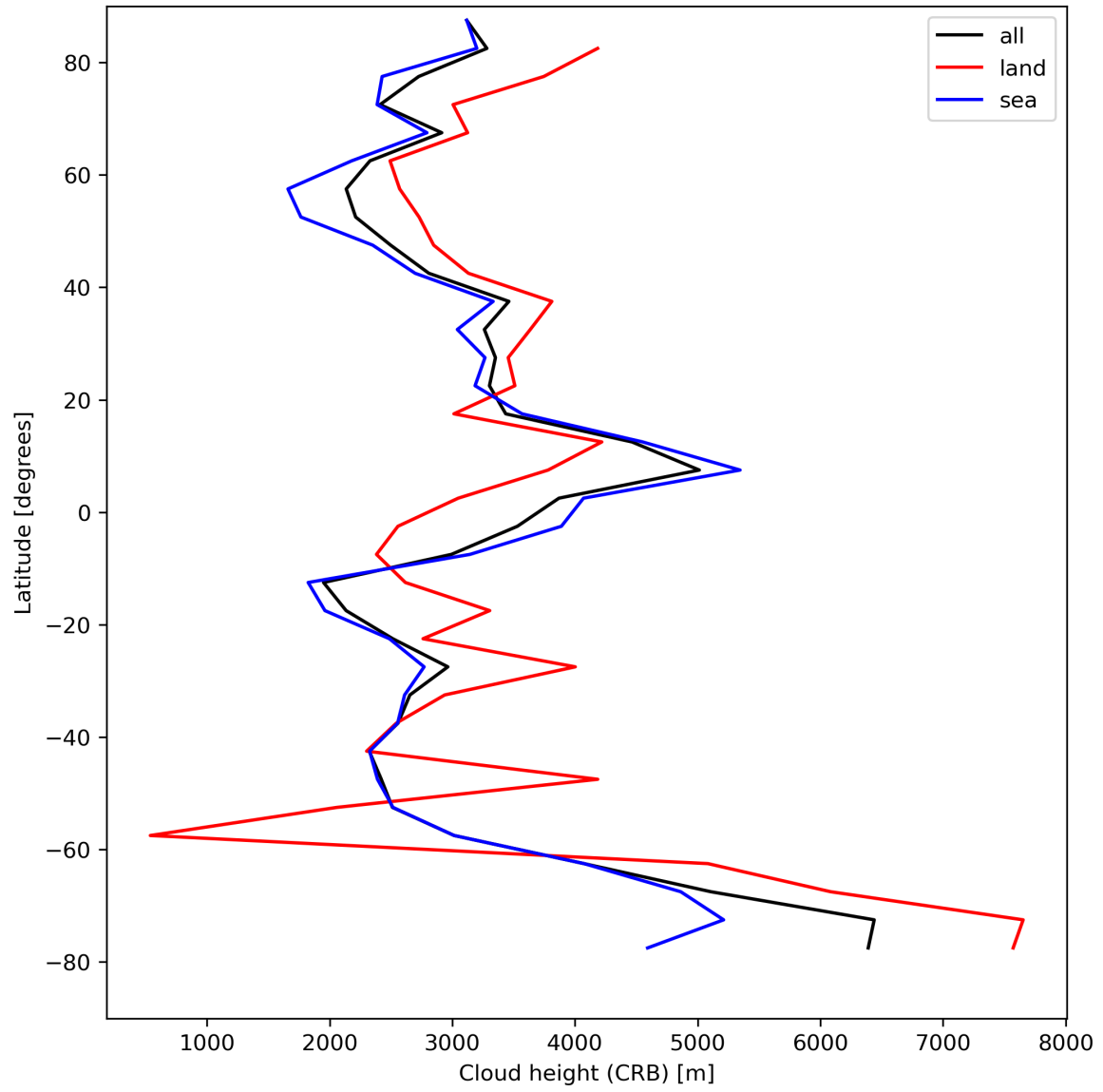
Figure 27: Zonal average of “Cloud height (CRB)” for 2023-08-16 to 2023-08-18.
