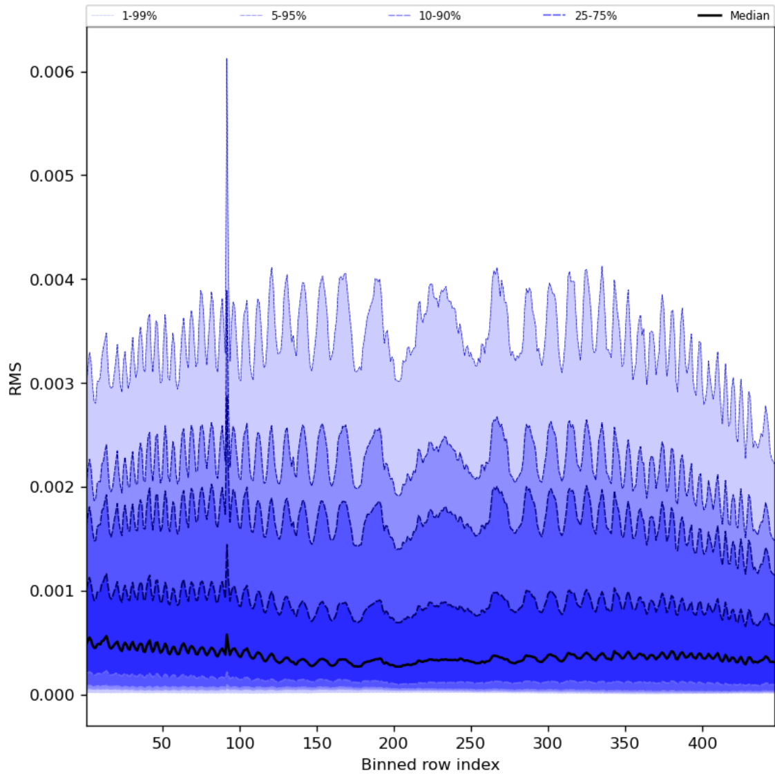
Figure 63: Along track statistics of “RMS” for 2023-08-16 to 2023-08-18
