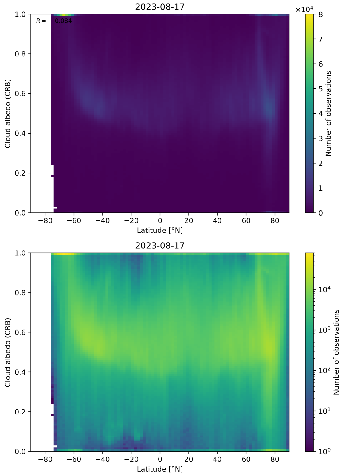
Figure 91: Scatter density plot of “Latitude” against “Cloud albedo (CRB)” for 2023-08-16 to 2023-08-18.
