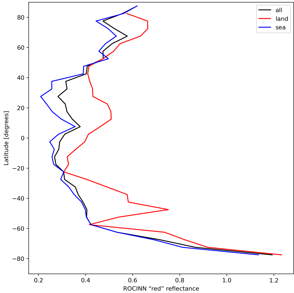
Figure 37: Zonal average of “ROCINN “red” reflectance” for 2023-08-16 to 2023-08-18.
