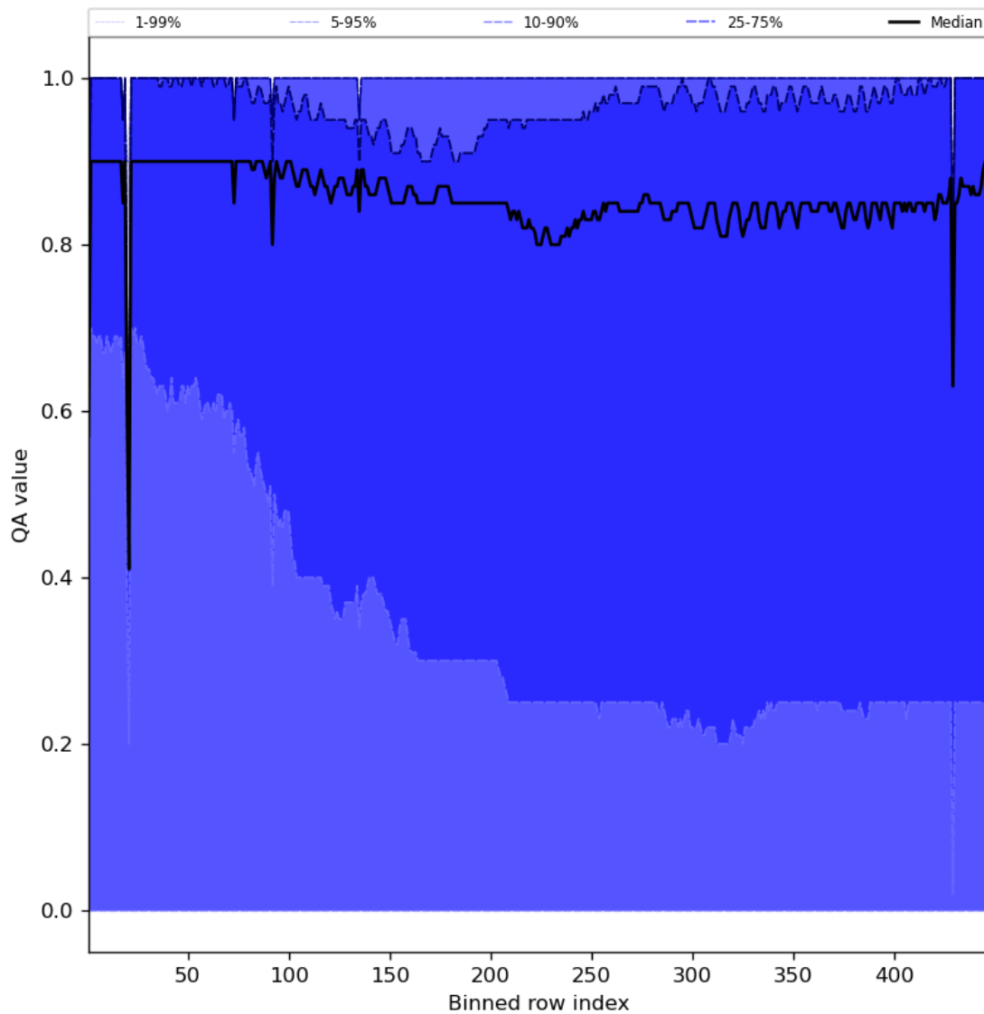
Figure 54: Along track statistics of “QA value” for 2023-08-16 to 2023-08-18
