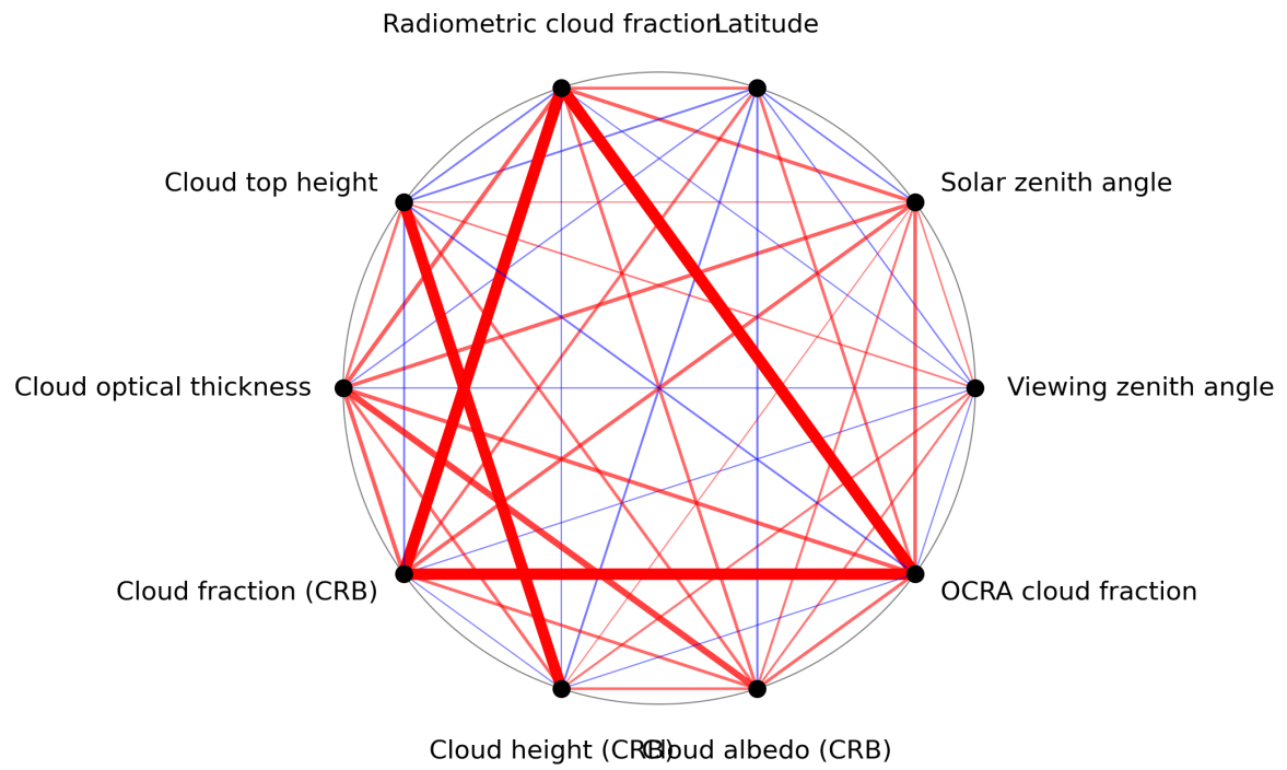
Figure 1: Map of correlation graph for 2023-08-16 to 2023-08-18.
