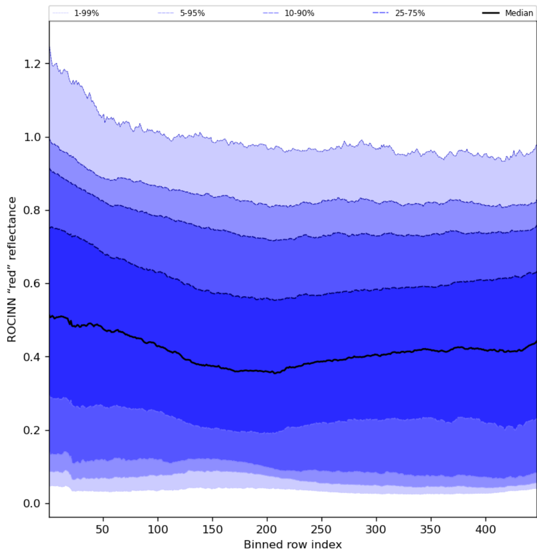
Figure 69: Along track statistics of “ROCINN “red” reflectance” for 2023-08-16 to 2023-08-18
