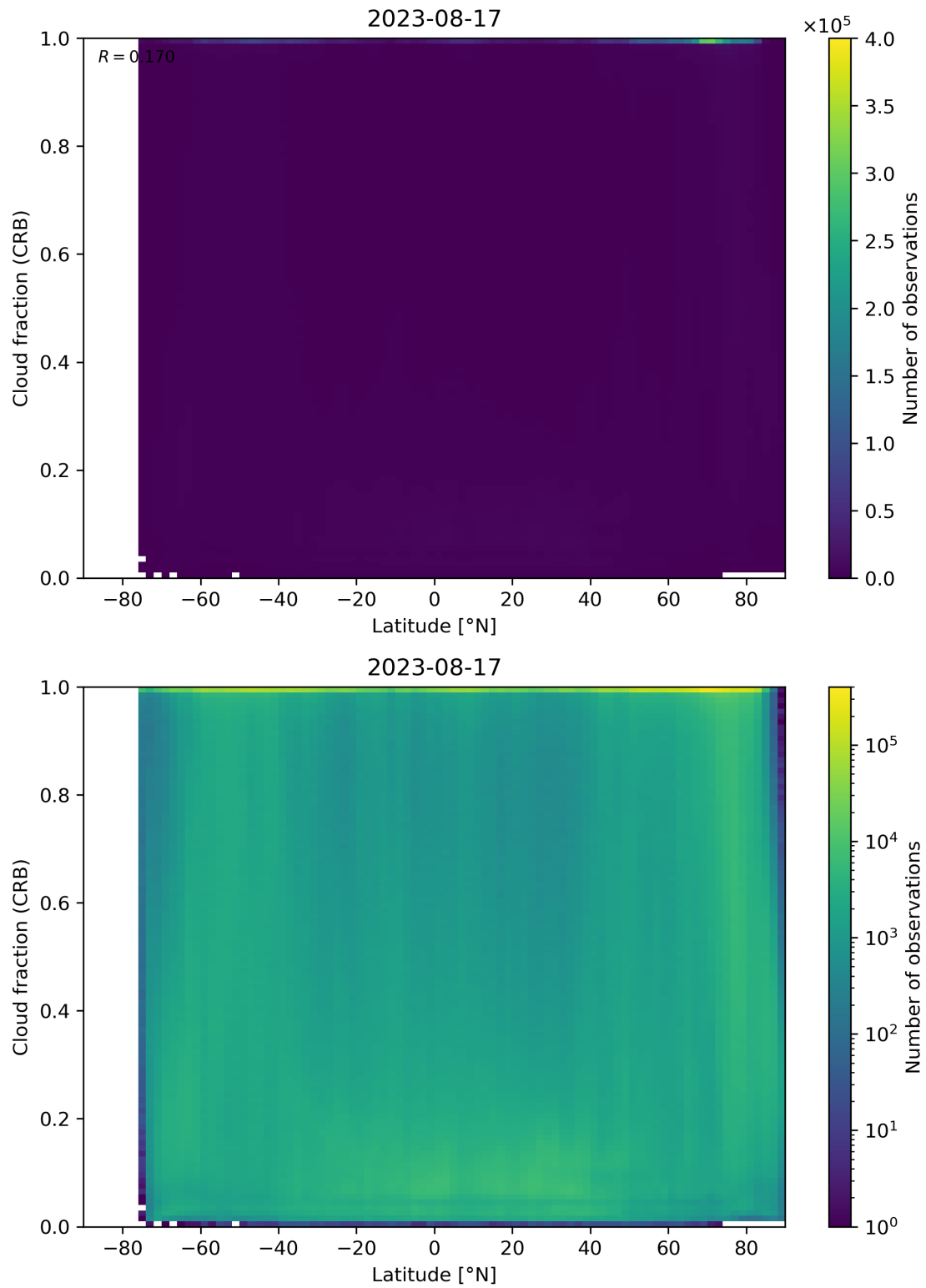
Figure 94: Scatter density plot of “Latitude” against “Cloud fraction (CRB)” for 2023-08-16 to 2023-08-18.
