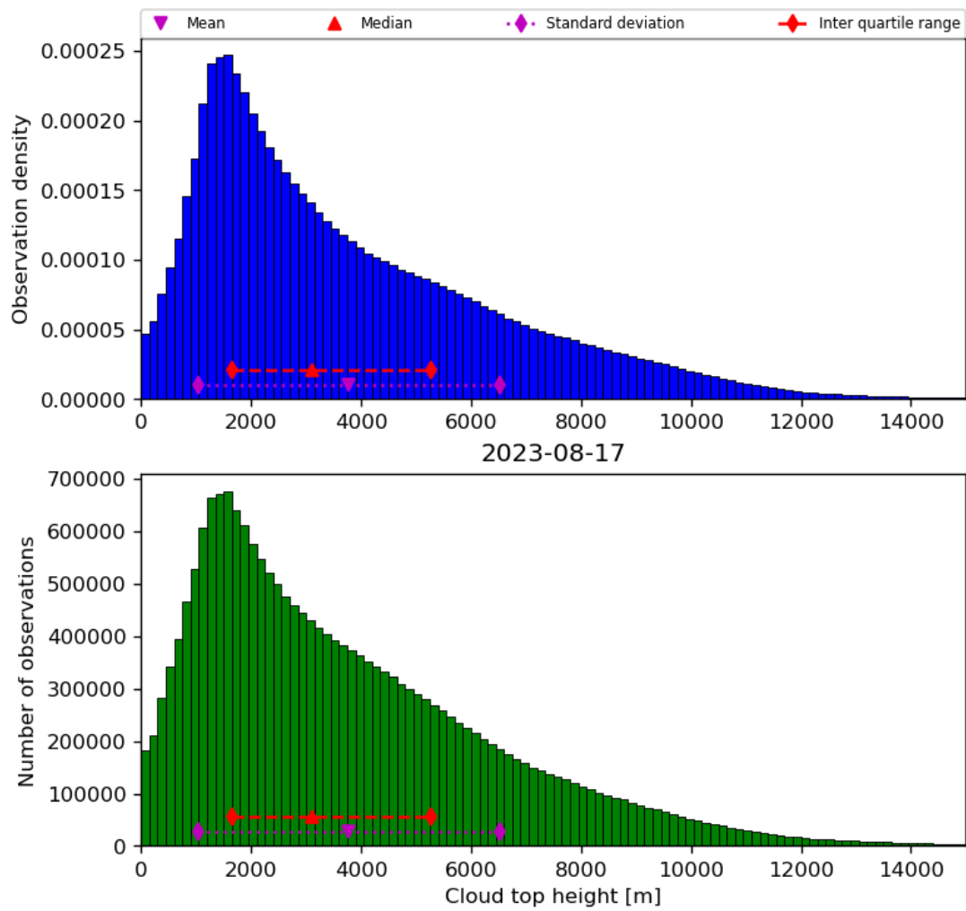
Figure 40: Histogram of “Cloud top height” for 2023-08-16 to 2023-08-18
