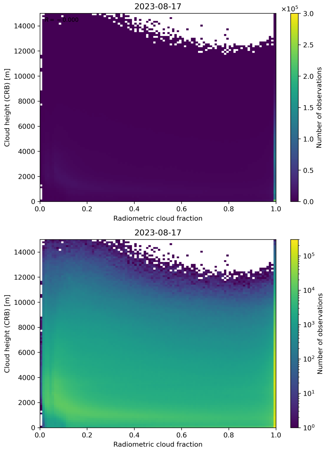
Figure 74: Scatter density plot of “Radiometric cloud fraction” against “Cloud height (CRB)” for 2023-08-16 to 2023-08-18.
