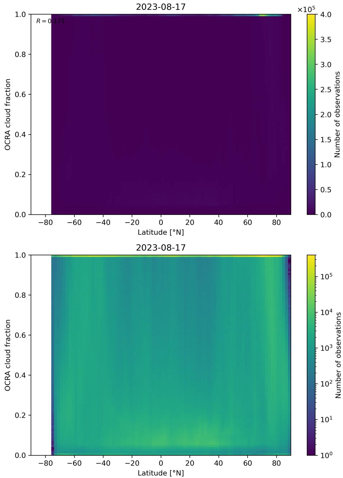
Figure 93: Scatter density plot of “Latitude” against “OCRA cloud fraction” for 2023-08-16 to 2023-08-18.
