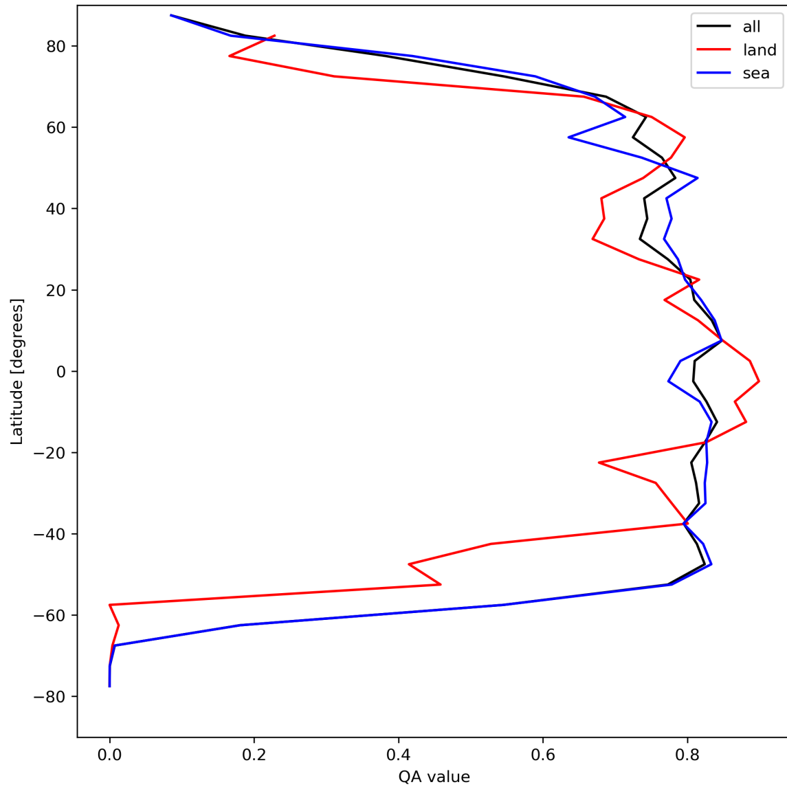
Figure 22: Zonal average of “QA value” for 2023-08-16 to 2023-08-18.
