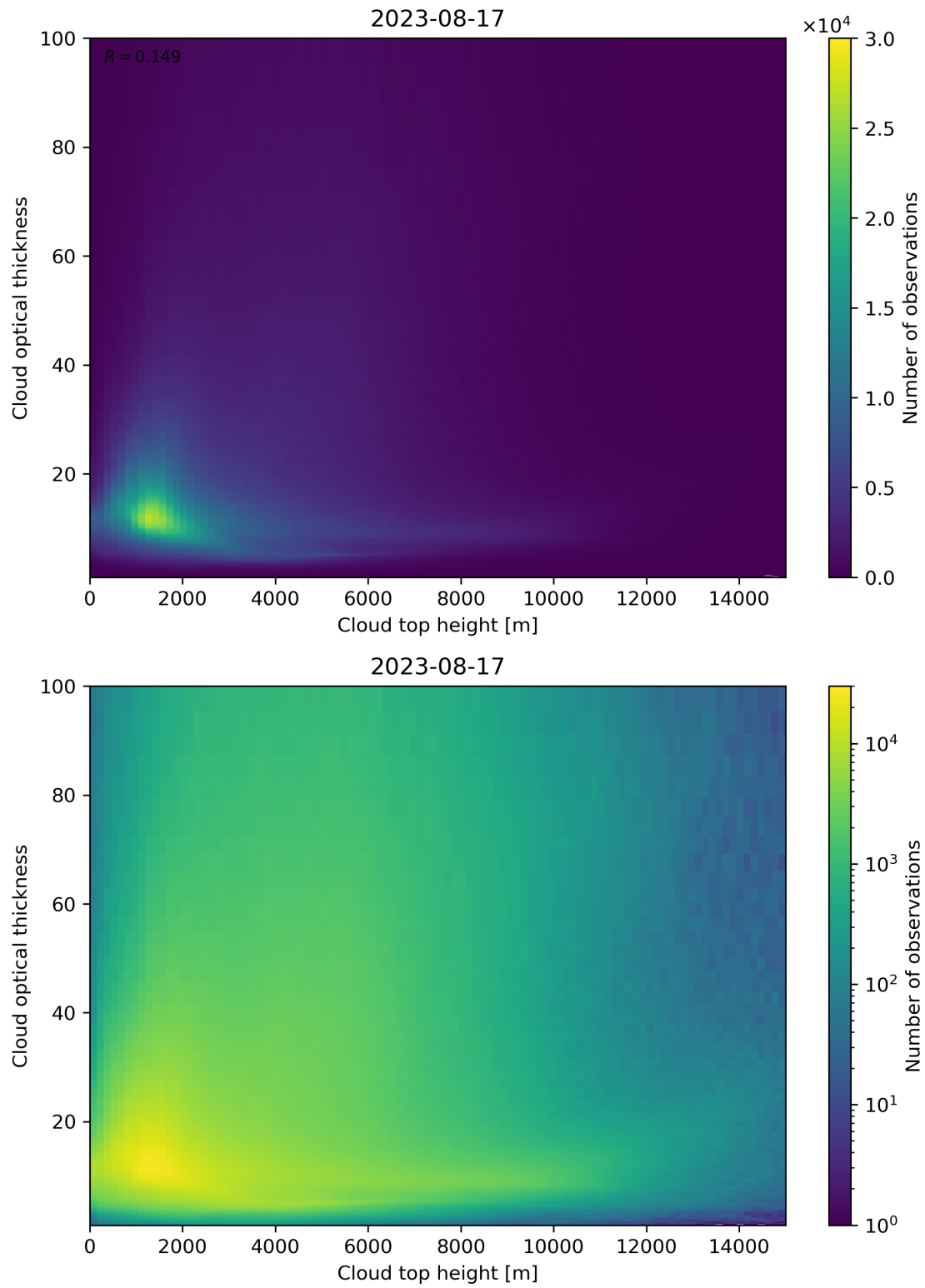
Figure 90: Scatter density plot of “Cloud top height” against “Cloud optical thickness” for 2023-08-16 to 2023-08-18.
