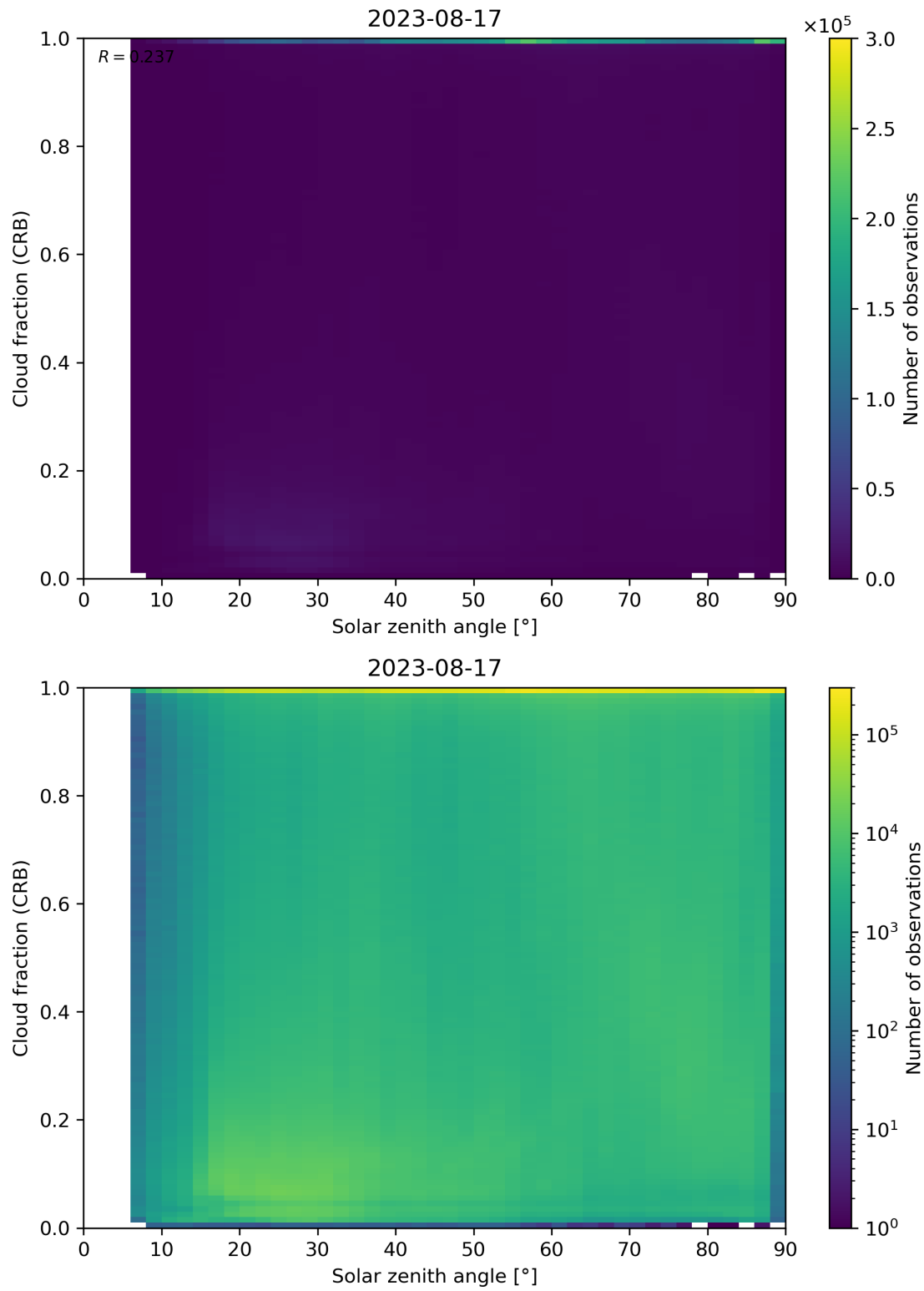
Figure 101: Scatter density plot of “Solar zenith angle” against “Cloud fraction (CRB)” for 2023-08-16 to 2023-08-18.
