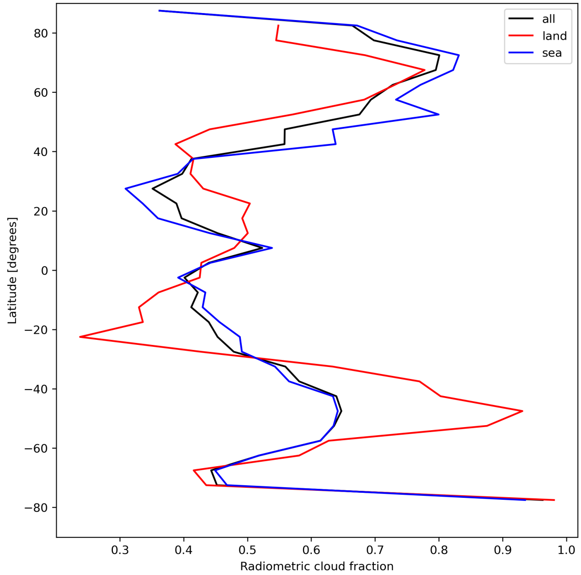
Figure 23: Zonal average of “Radiometric cloud fraction” for 2023-08-16 to 2023-08-18.
