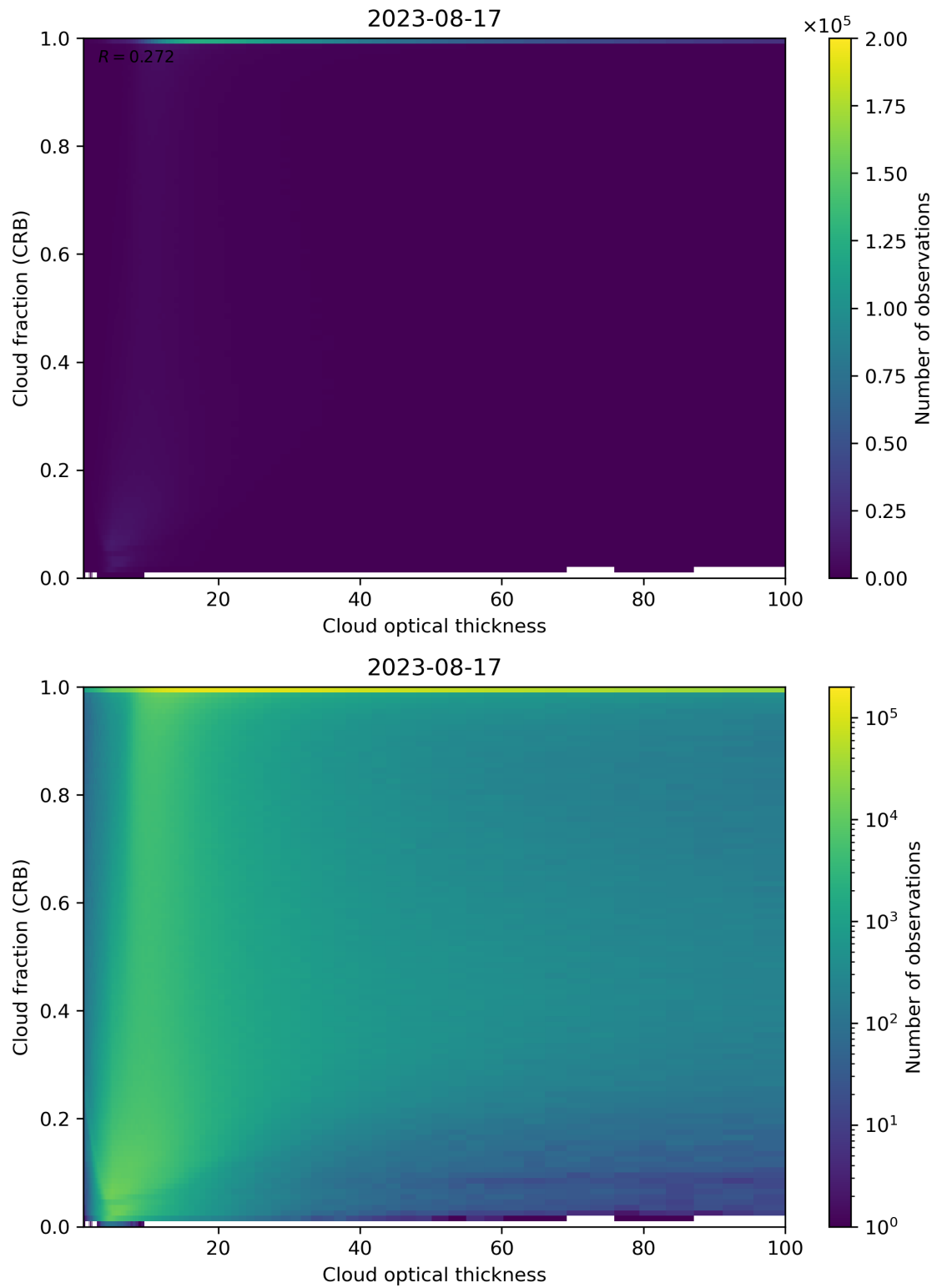
Figure 84: Scatter density plot of “Cloud optical thickness” against “Cloud fraction (CRB)” for 2023-08-16 to 2023-08-18.
