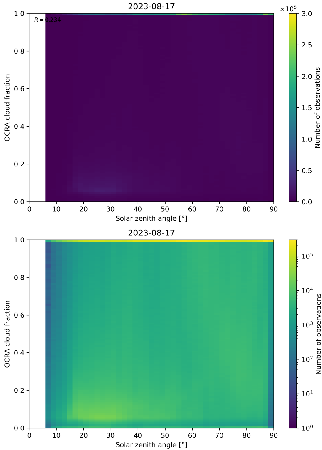
Figure 100: Scatter density plot of “Solar zenith angle” against “OCRA cloud fraction” for 2023-08-16 to 2023-08-18.
