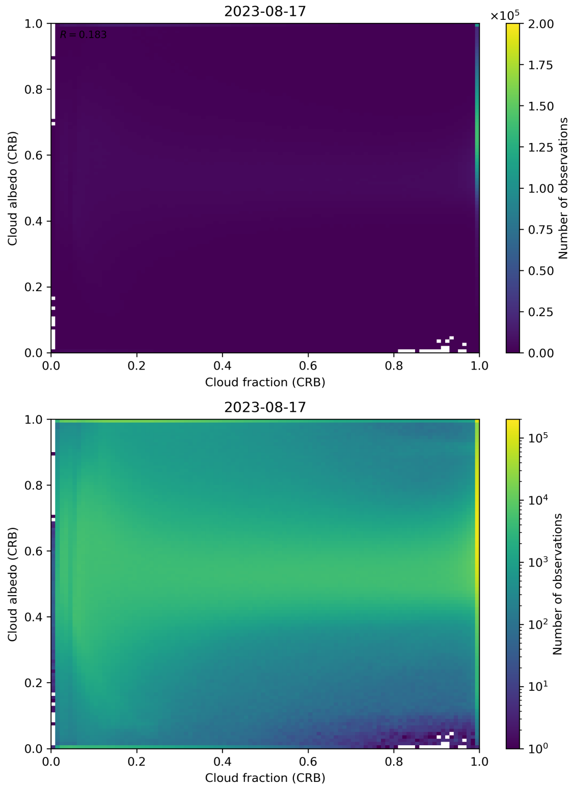
Figure 77: Scatter density plot of “Cloud fraction (CRB)” against “Cloud albedo (CRB)” for 2023-08-16 to 2023-08-18.
