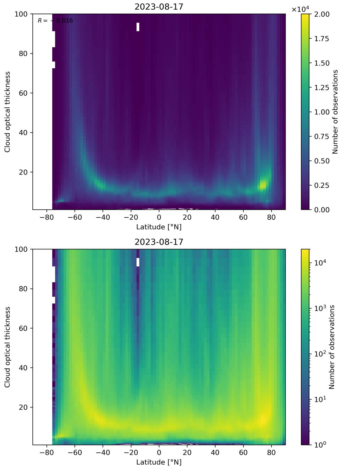
Figure 96: Scatter density plot of “Latitude” against “Cloud optical thickness” for 2023-08-16 to 2023-08-18.
