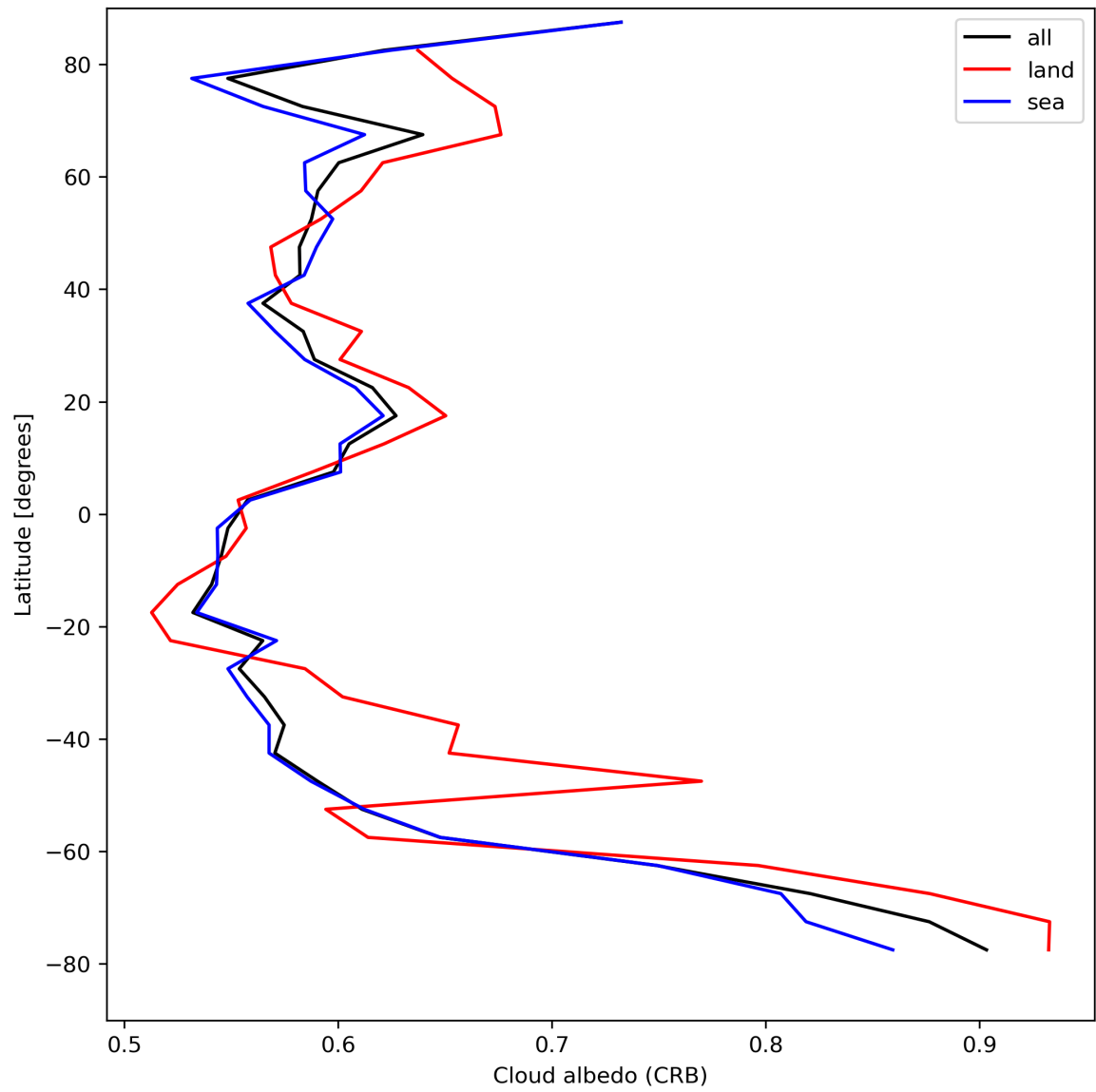
Figure 28: Zonal average of “Cloud albedo (CRB)” for 2023-08-16 to 2023-08-18.
