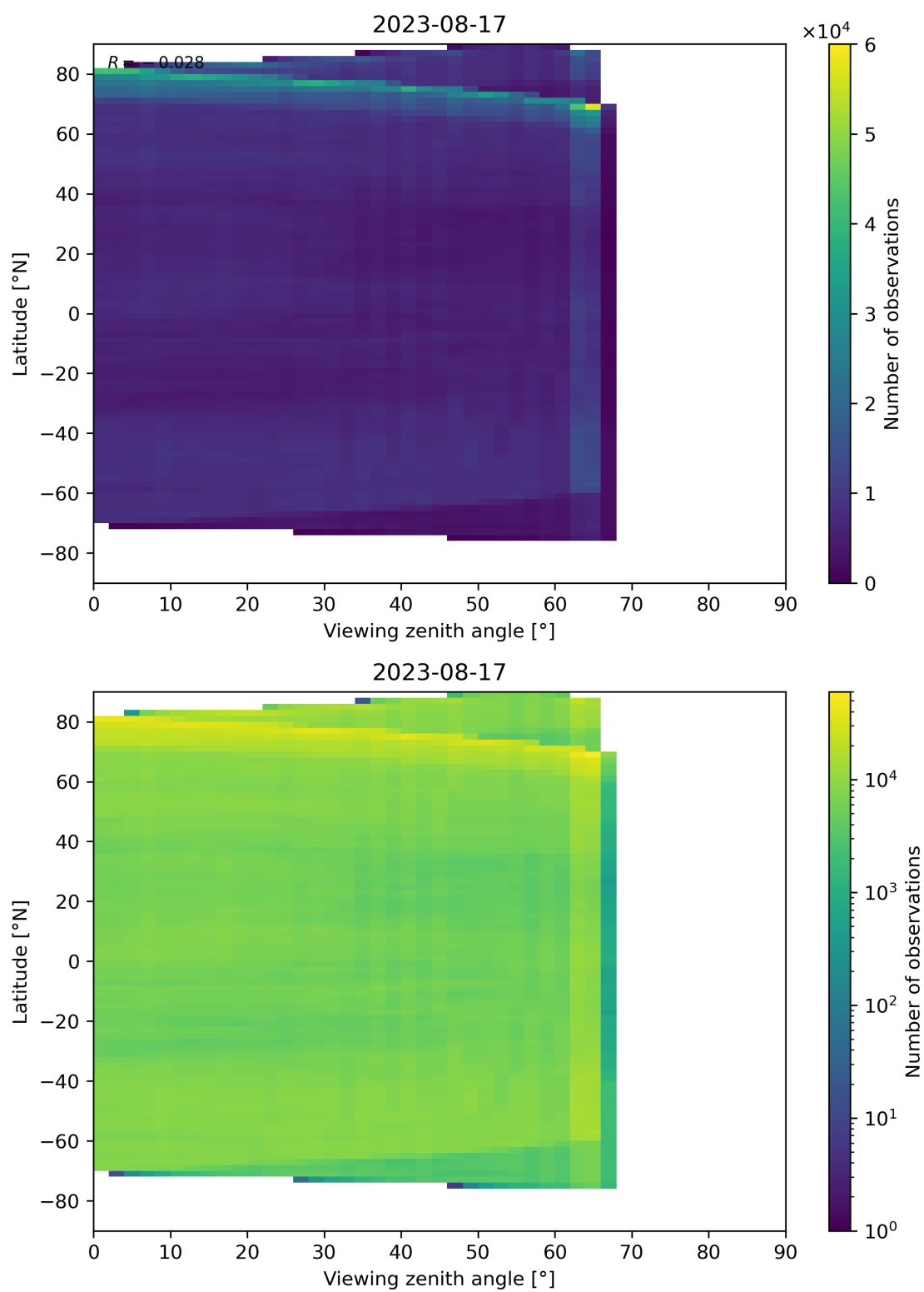
Figure 113: Scatter density plot of “Viewing zenith angle” against “Latitude” for 2023-08-16 to 2023-08-18.
