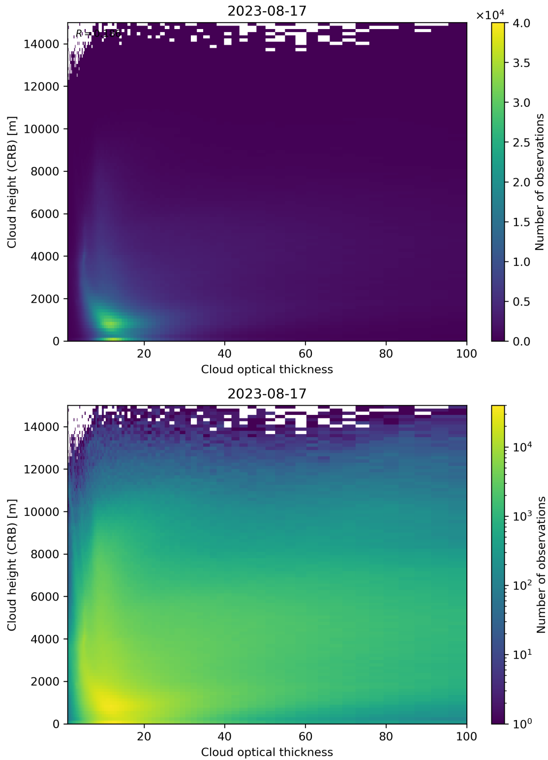
Figure 85: Scatter density plot of “Cloud optical thickness” against “Cloud height (CRB)” for 2023-08-16 to 2023-08-18.
