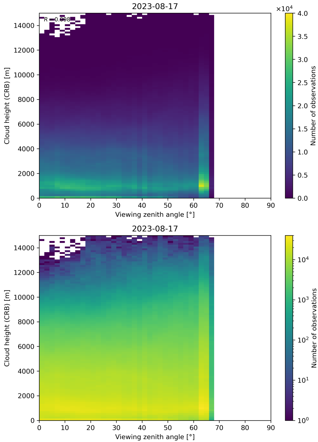
Figure 110: Scatter density plot of “Viewing zenith angle” against “Cloud height (CRB)” for 2023-08-16 to 2023-08-18.
