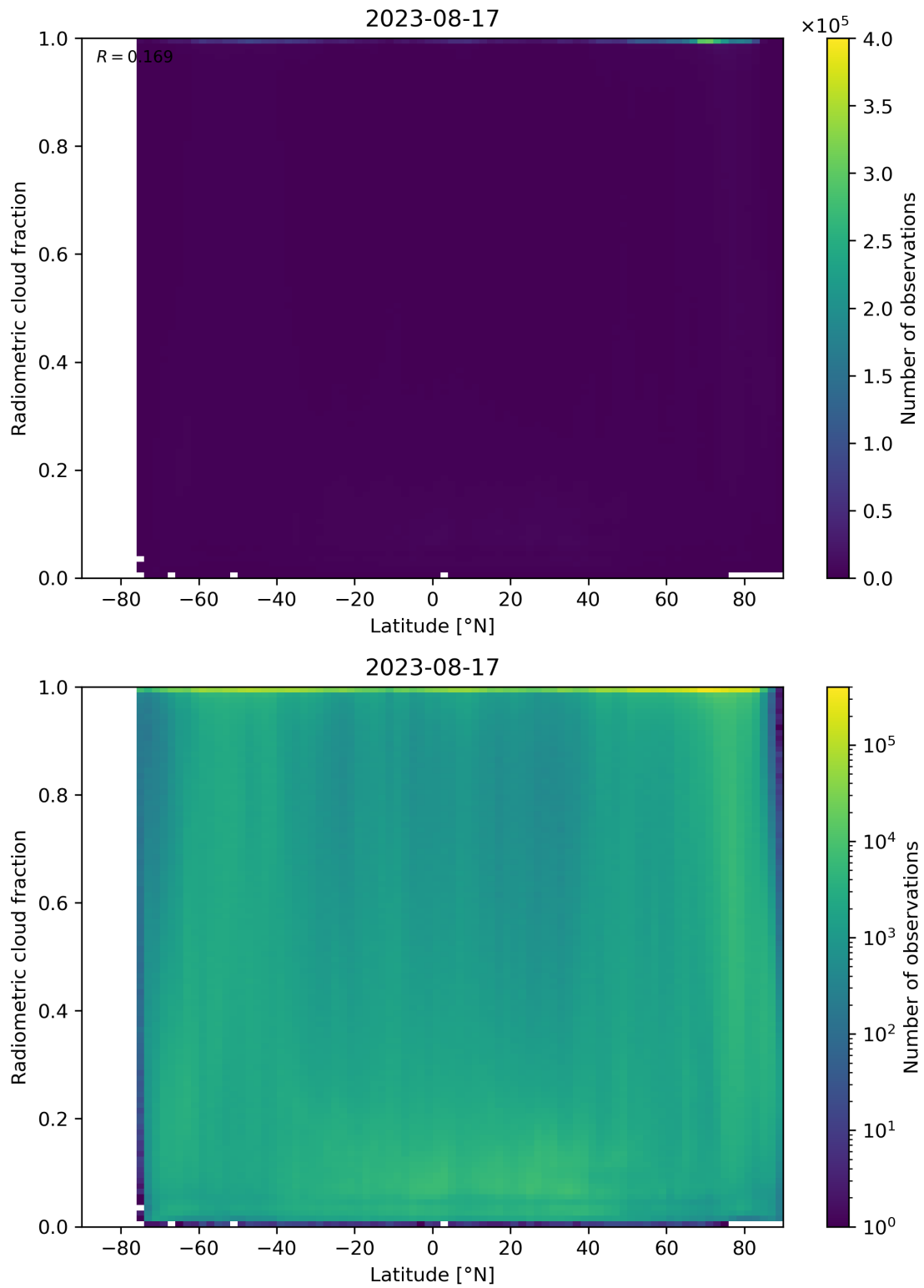
Figure 92: Scatter density plot of “Latitude” against “Radiometric cloud fraction” for 2023-08-16 to 2023-08-18.
