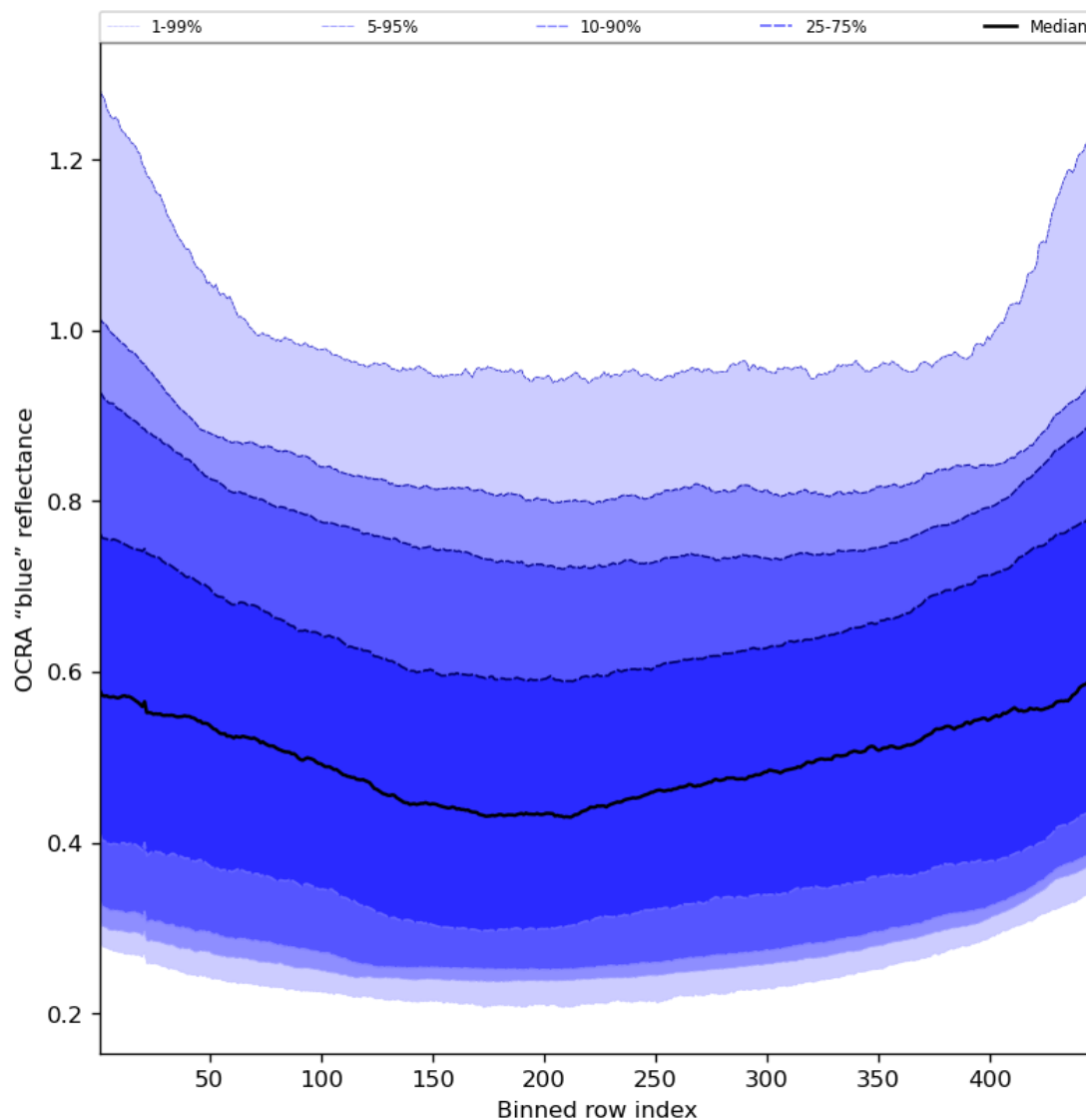
Figure 67: Along track statistics of “OCRA “blue” reflectance” for 2023-08-16 to 2023-08-18
