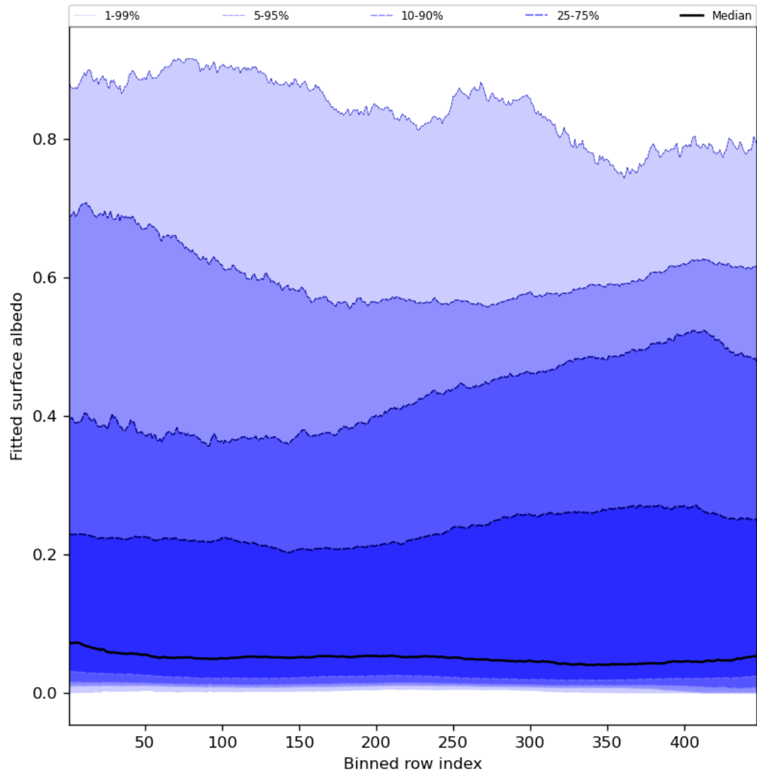
Figure 61: Along track statistics of “Fitted surface albedo” for 2023-08-16 to 2023-08-18
