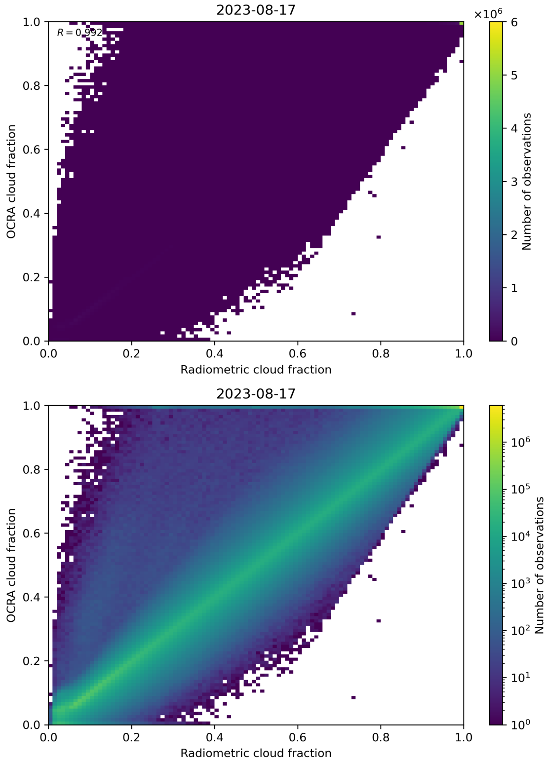
Figure 72: Scatter density plot of “Radiometric cloud fraction” against “OCRA cloud fraction” for 2023-08-16 to 2023-08-18.
