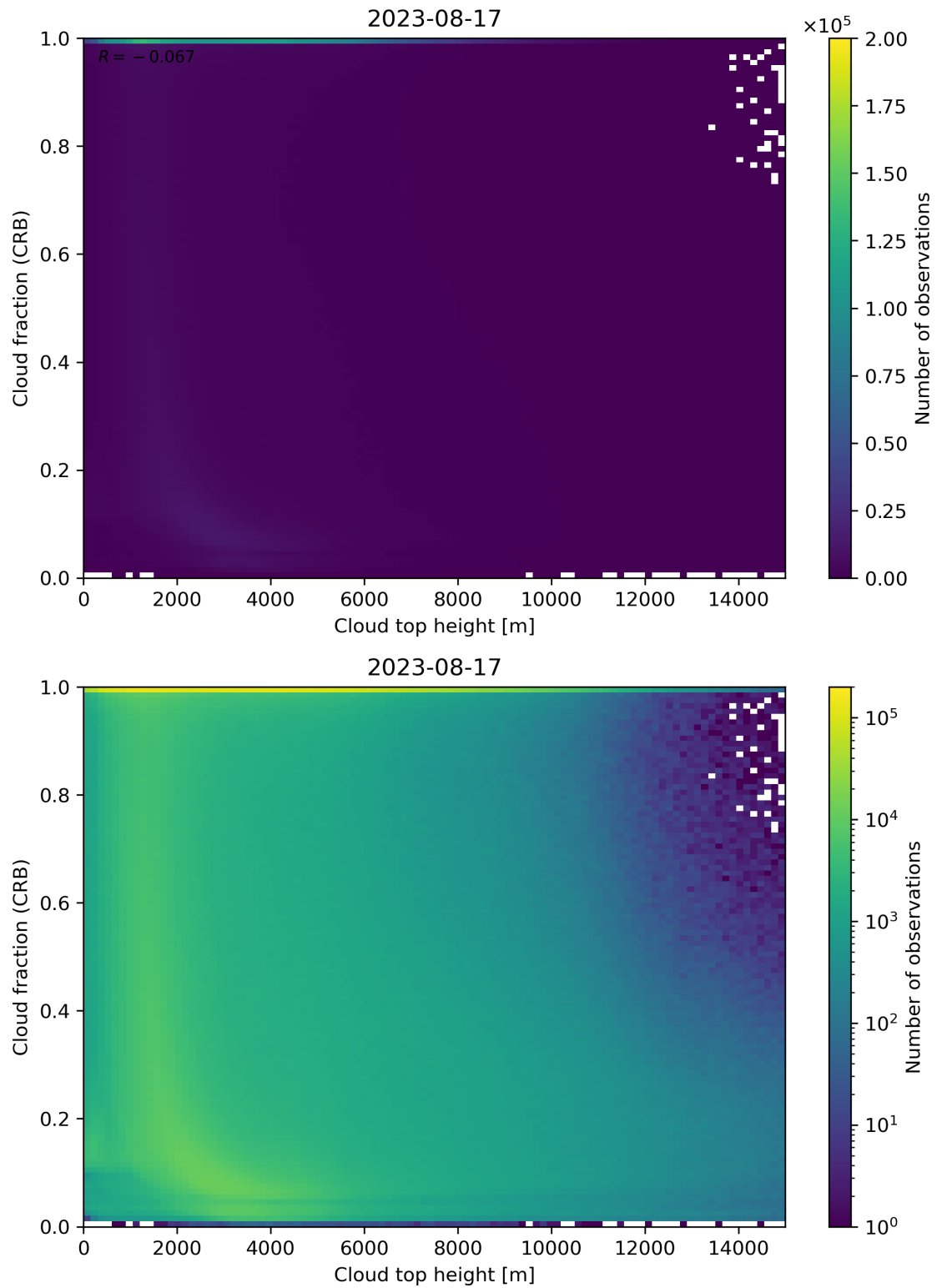
Figure 88: Scatter density plot of “Cloud top height” against “Cloud fraction (CRB)” for 2023-08-16 to 2023-08-18.
