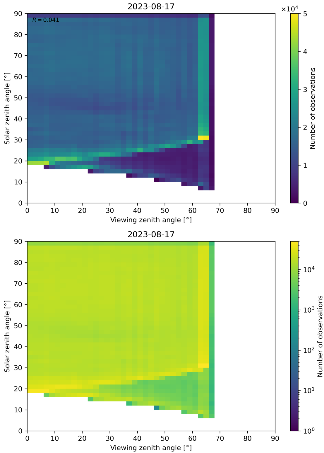
Figure 114: Scatter density plot of “Viewing zenith angle” against “Solar zenith angle” for 2023-08-16 to 2023-08-18.
