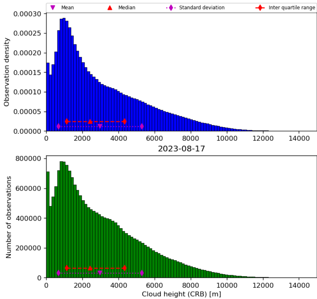
Figure 43: Histogram of “Cloud height (CRB)” for 2023-08-16 to 2023-08-18
