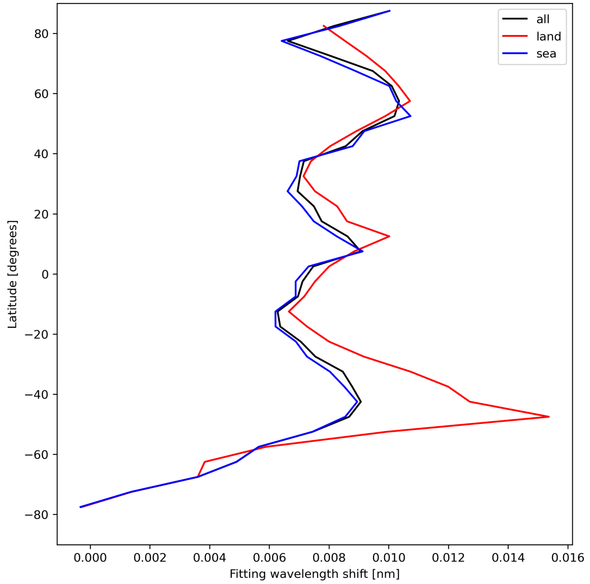
Figure 33: Zonal average of “Fitting wavelength shift” for 2023-08-16 to 2023-08-18.
