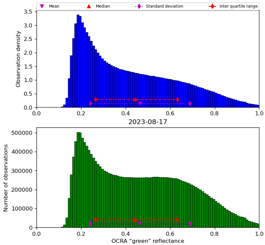
Figure 52: Histogram of “OCRA “green” reflectance” for 2023-08-16 to 2023-08-18
