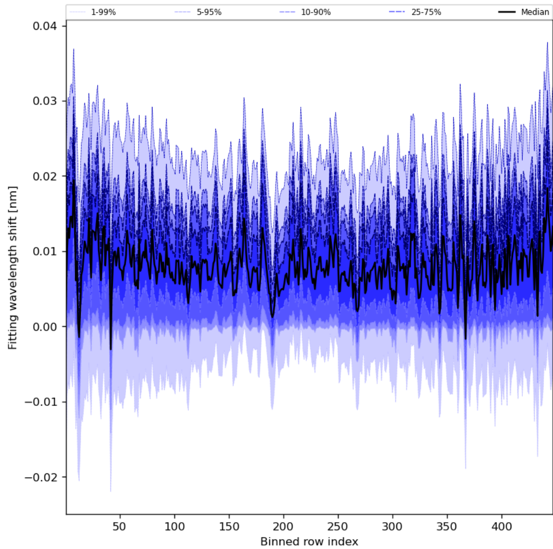
Figure 65: Along track statistics of “Fitting wavelength shift” for 2023-08-16 to 2023-08-18
