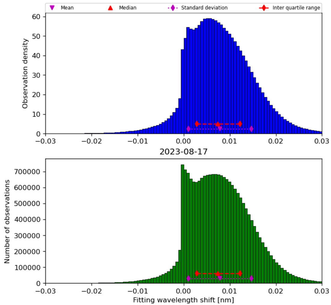
Figure 49: Histogram of “Fitting wavelength shift” for 2023-08-16 to 2023-08-18
