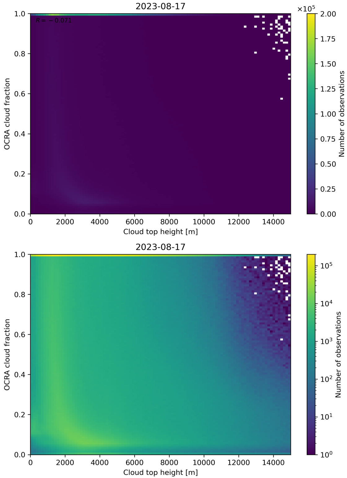
Figure 87: Scatter density plot of “Cloud top height” against “OCRA cloud fraction” for 2023-08-16 to 2023-08-18.
