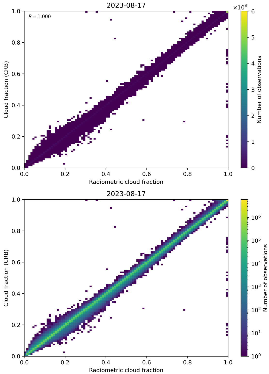
Figure 73: Scatter density plot of “Radiometric cloud fraction” against “Cloud fraction (CRB)” for 2023-08-16 to 2023-08-18.
