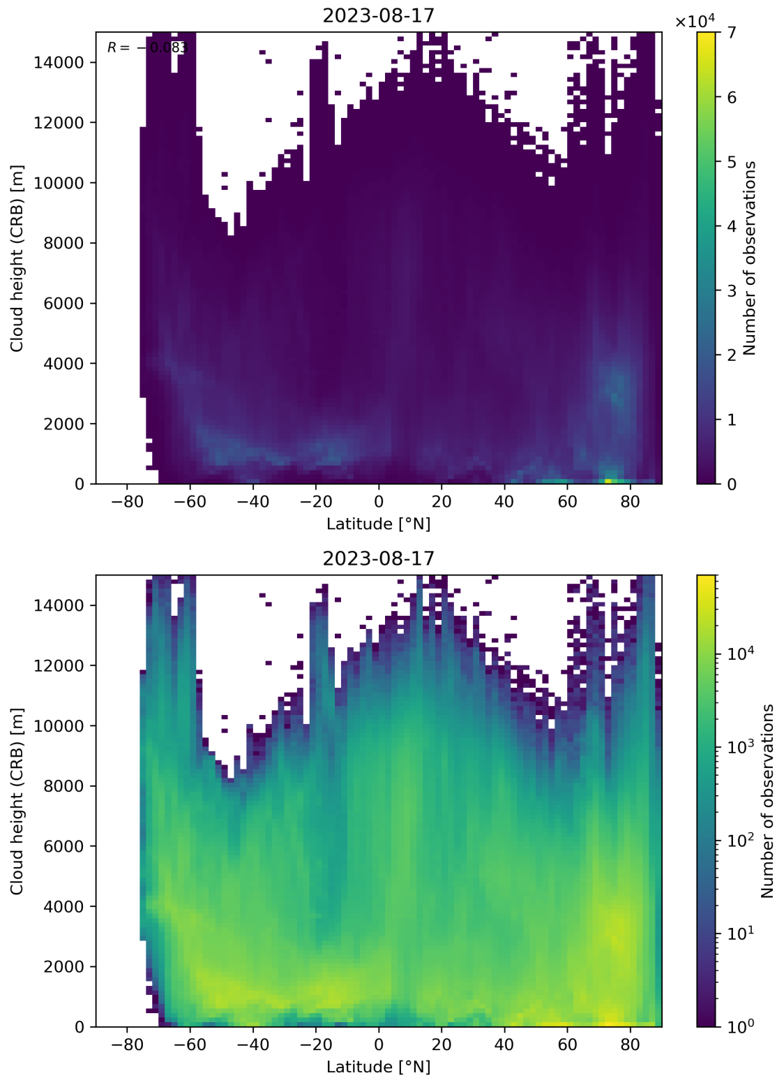
Figure 95: Scatter density plot of “Latitude” against “Cloud height (CRB)” for 2023-08-16 to 2023-08-18.
