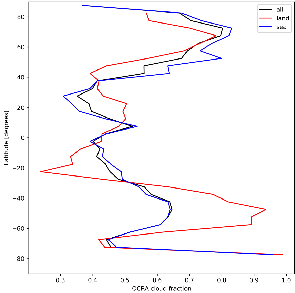
Figure 34: Zonal average of “OCRA cloud fraction” for 2023-08-16 to 2023-08-18.
