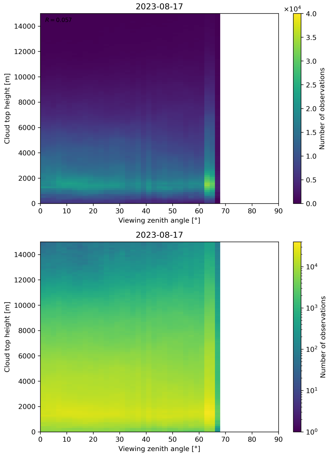
Figure 112: Scatter density plot of “Viewing zenith angle” against “Cloud top height” for 2023-08-16 to 2023-08-18.
