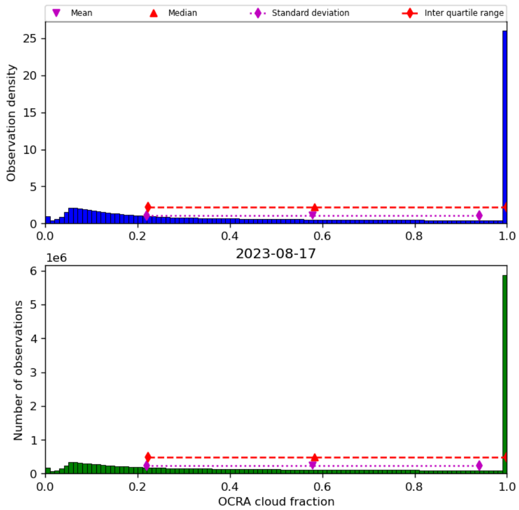
Figure 50: Histogram of “OCRA cloud fraction” for 2023-08-16 to 2023-08-18
