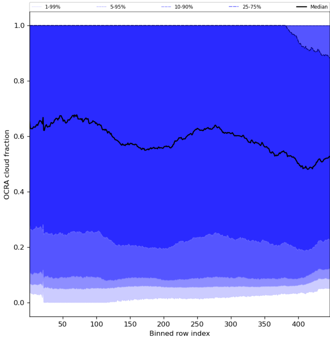
Figure 66: Along track statistics of “OCRA cloud fraction” for 2023-08-16 to 2023-08-18
