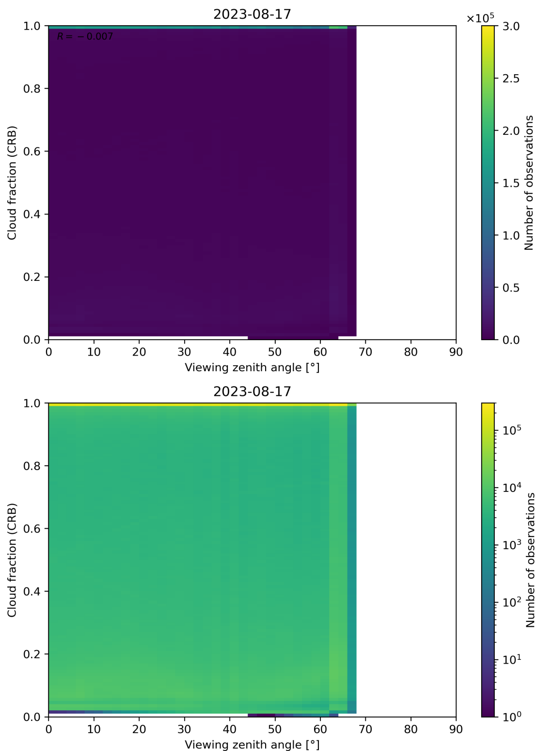
Figure 109: Scatter density plot of “Viewing zenith angle” against “Cloud fraction (CRB)” for 2023-08-16 to 2023-08-18.
