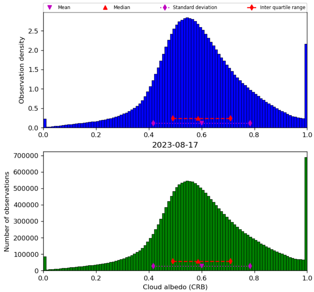
Figure 44: Histogram of “Cloud albedo (CRB)” for 2023-08-16 to 2023-08-18
