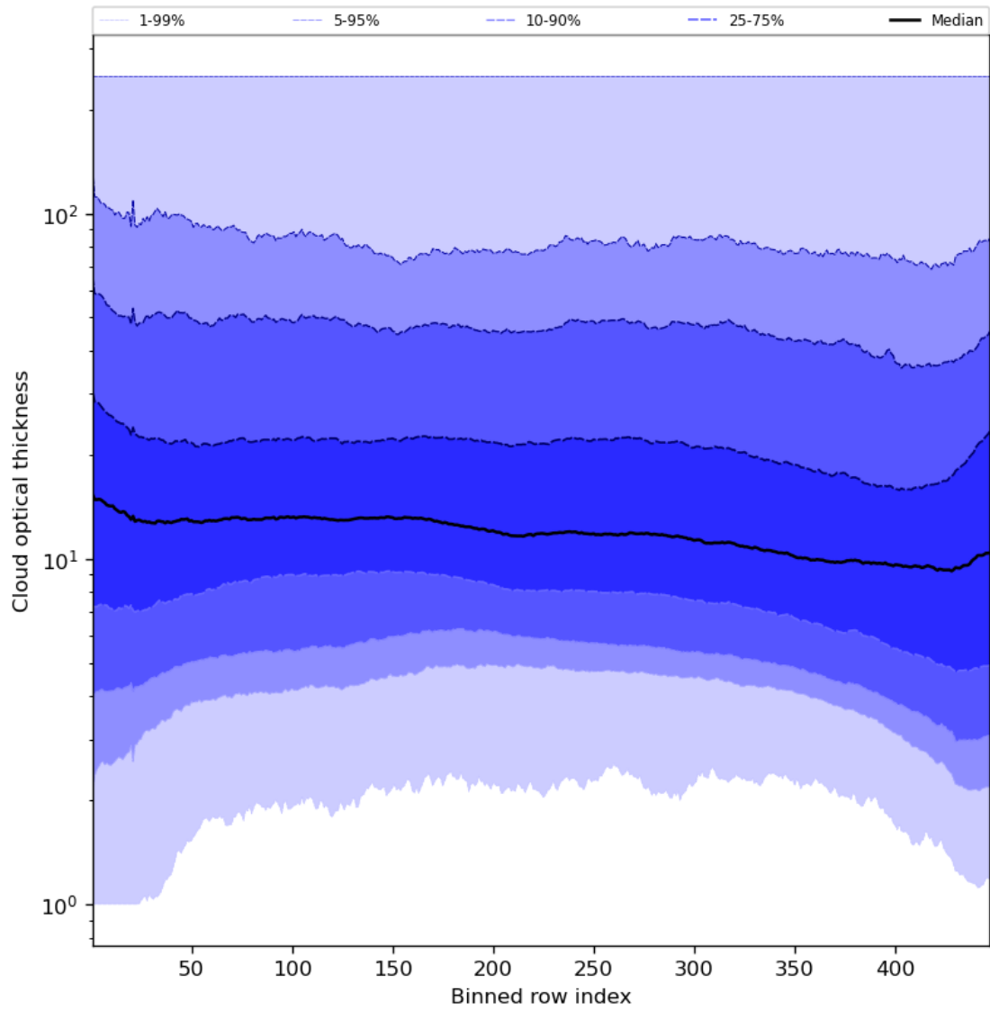
Figure 57: Along track statistics of “Cloud optical thickness” for 2023-08-16 to 2023-08-18
