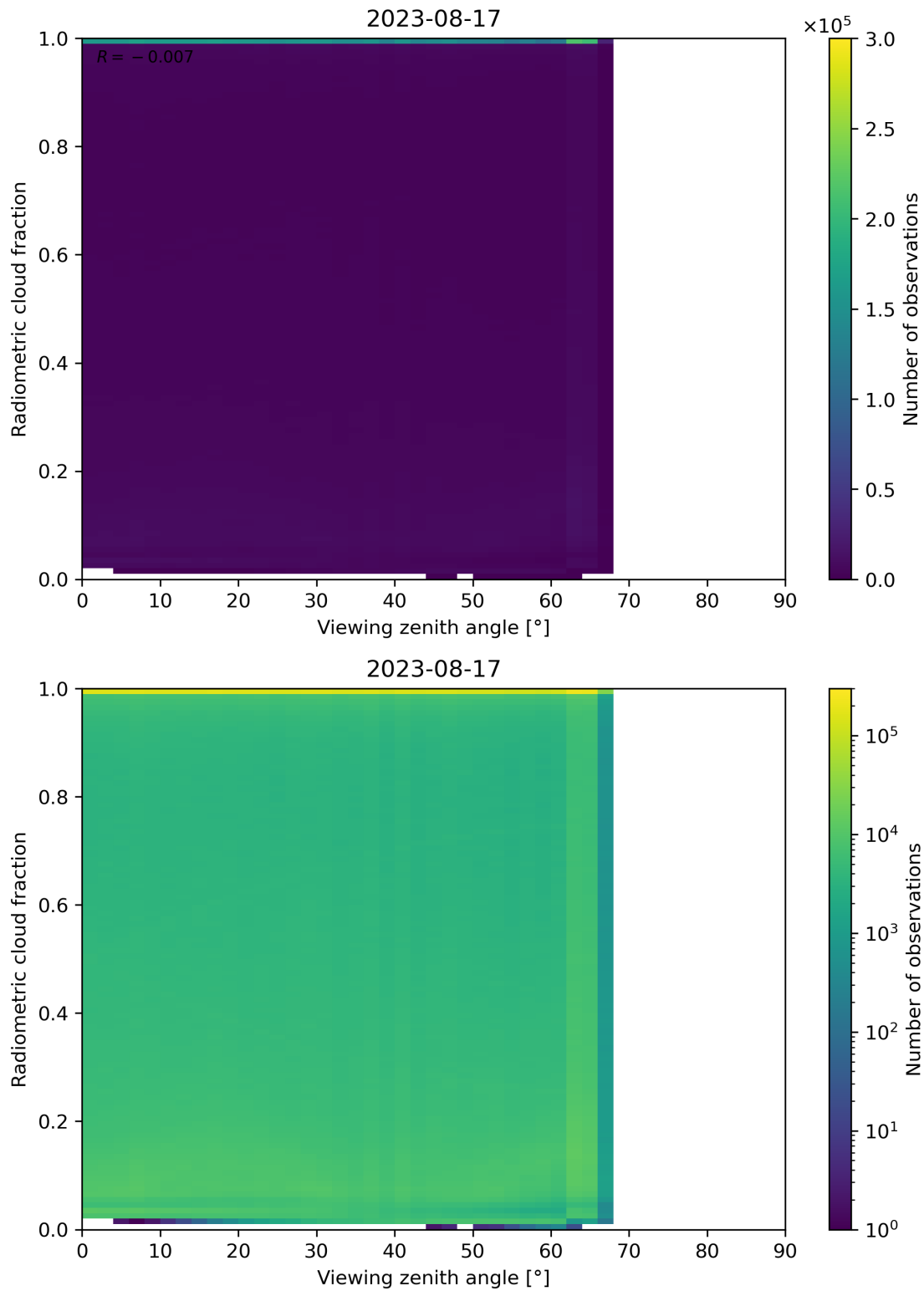
Figure 107: Scatter density plot of “Viewing zenith angle” against “Radiometric cloud fraction” for 2023-08-16 to 2023-08-18.
