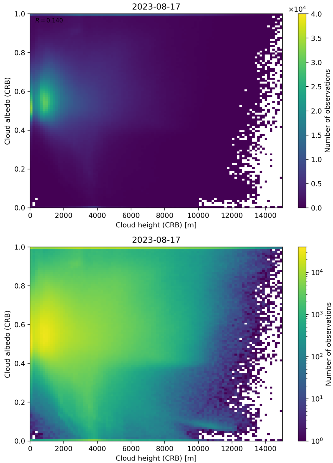
Figure 80: Scatter density plot of “Cloud height (CRB)” against “Cloud albedo (CRB)” for 2023-08-16 to 2023-08-18.
