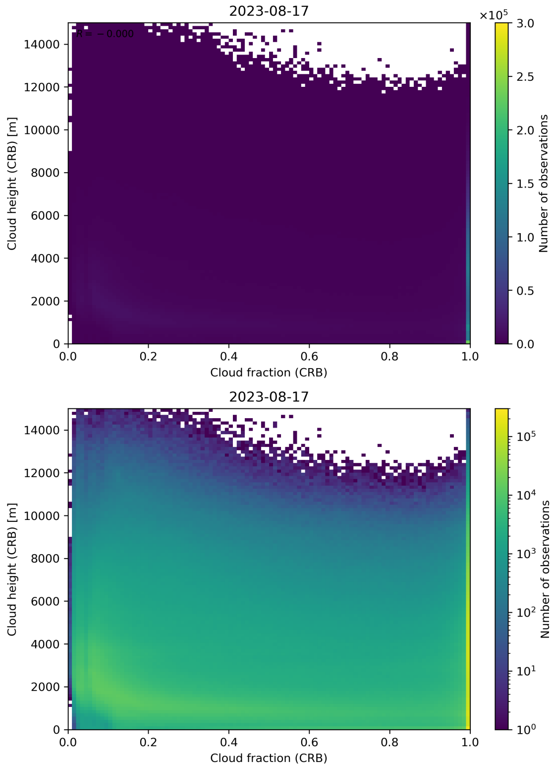
Figure 79: Scatter density plot of “Cloud fraction (CRB)” against “Cloud height (CRB)” for 2023-08-16 to 2023-08-18.
