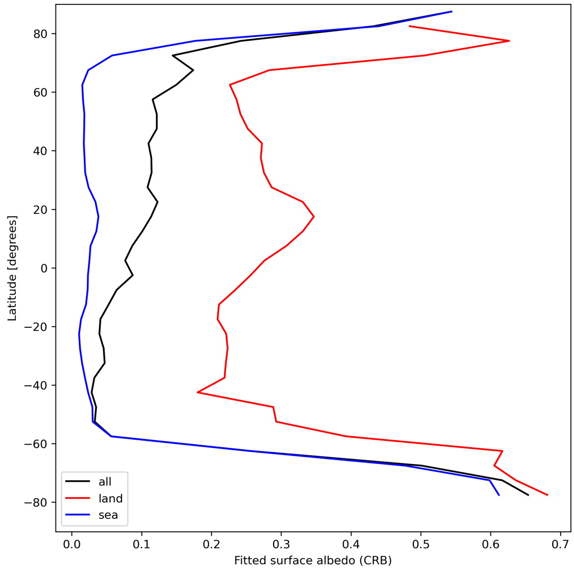
Figure 30: Zonal average of “Fitted surface albedo (CRB)” for 2023-08-16 to 2023-08-18.
