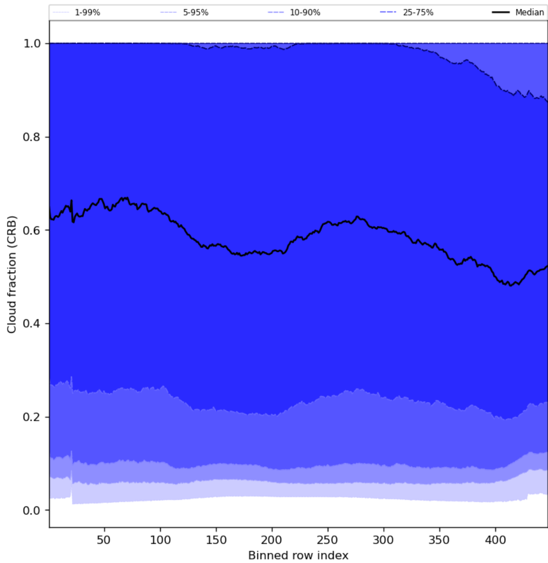
Figure 58: Along track statistics of “Cloud fraction (CRB)” for 2023-08-16 to 2023-08-18
