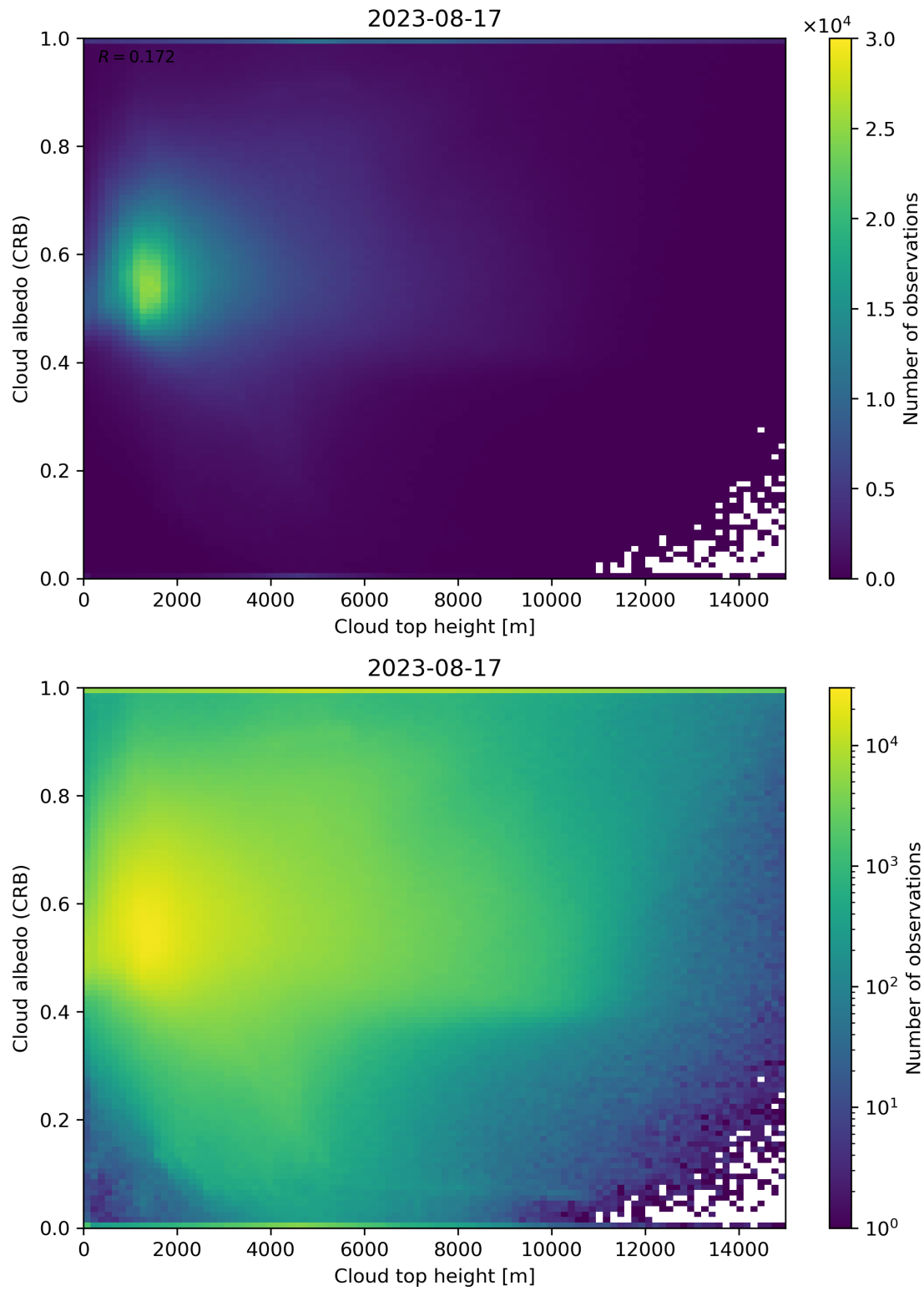
Figure 86: Scatter density plot of “Cloud top height” against “Cloud albedo (CRB)” for 2023-08-16 to 2023-08-18.
