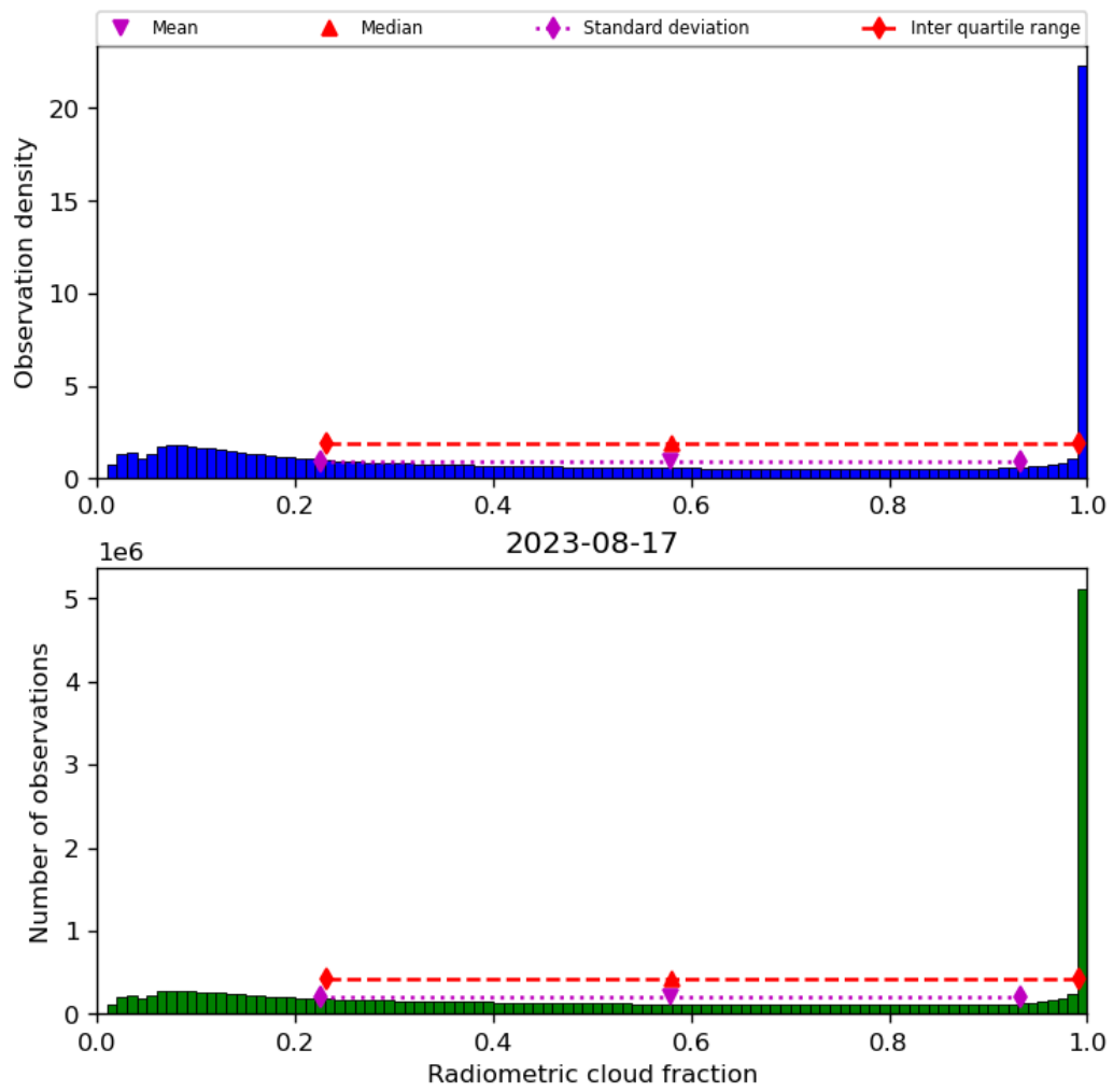
Figure 39: Histogram of “Radiometric cloud fraction” for 2023-08-16 to 2023-08-18
