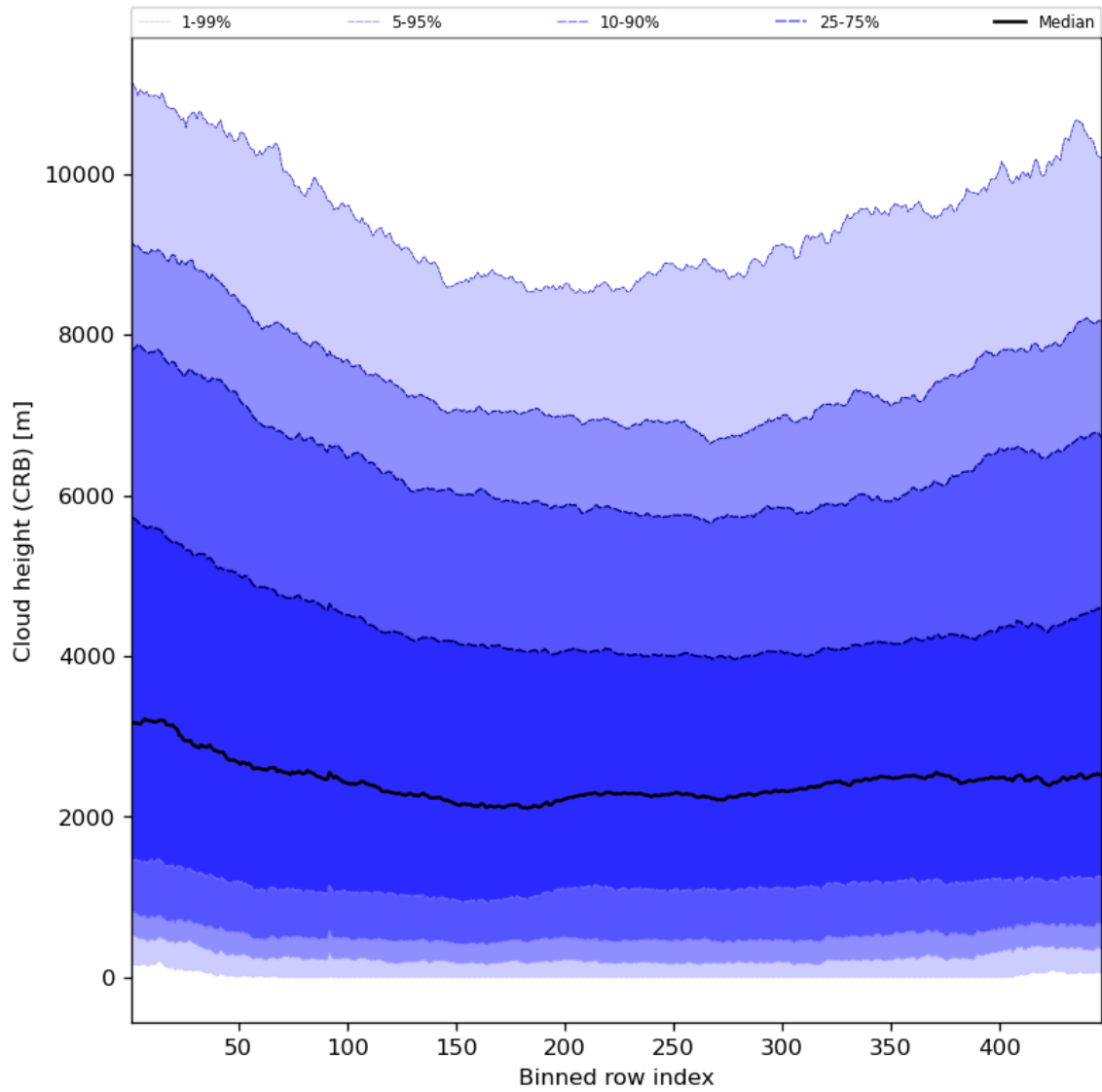
Figure 59: Along track statistics of “Cloud height (CRB)” for 2023-08-16 to 2023-08-18
