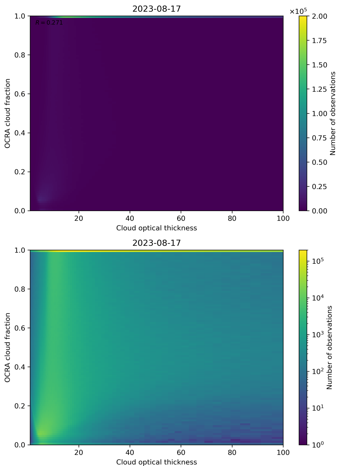
Figure 83: Scatter density plot of “Cloud optical thickness” against “OCRA cloud fraction” for 2023-08-16 to 2023-08-18.
