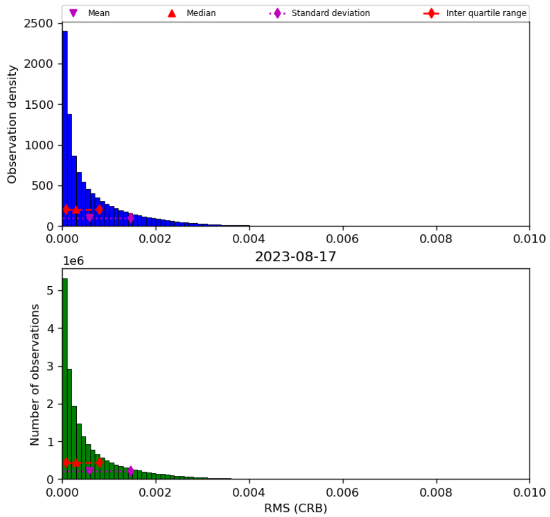
Figure 48: Histogram of “RMS (CRB)” for 2023-08-16 to 2023-08-18
