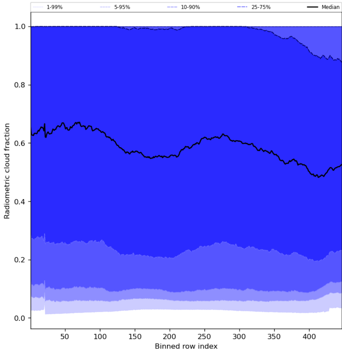
Figure 55: Along track statistics of “Radiometric cloud fraction” for 2023-08-16 to 2023-08-18
