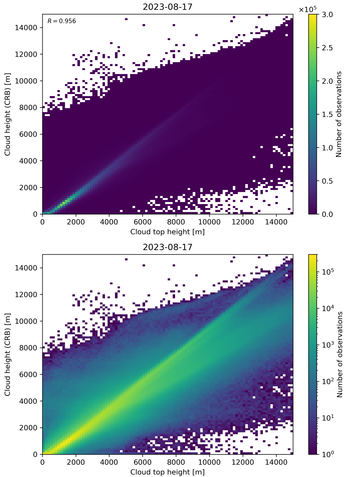
Figure 89: Scatter density plot of “Cloud top height” against “Cloud height (CRB)” for 2023-08-16 to 2023-08-18.
