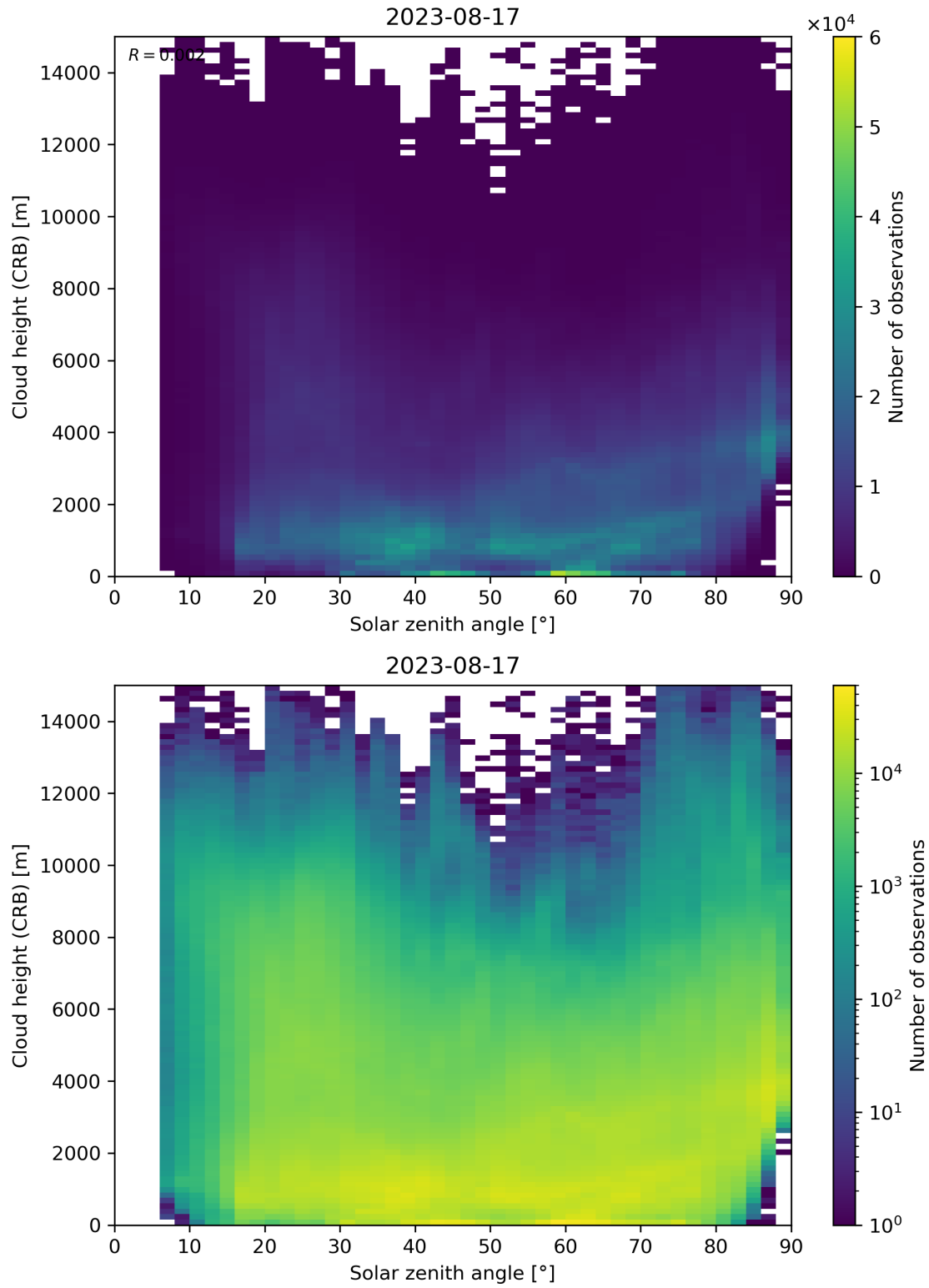
Figure 102: Scatter density plot of “Solar zenith angle” against “Cloud height (CRB)” for 2023-08-16 to 2023-08-18.
