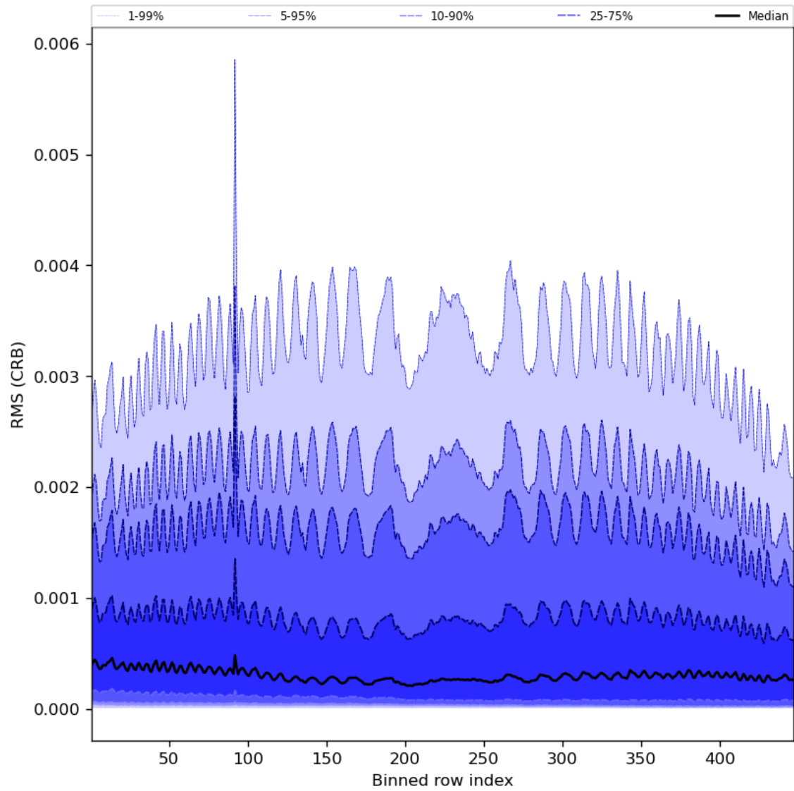
Figure 64: Along track statistics of “RMS (CRB)” for 2023-08-16 to 2023-08-18
