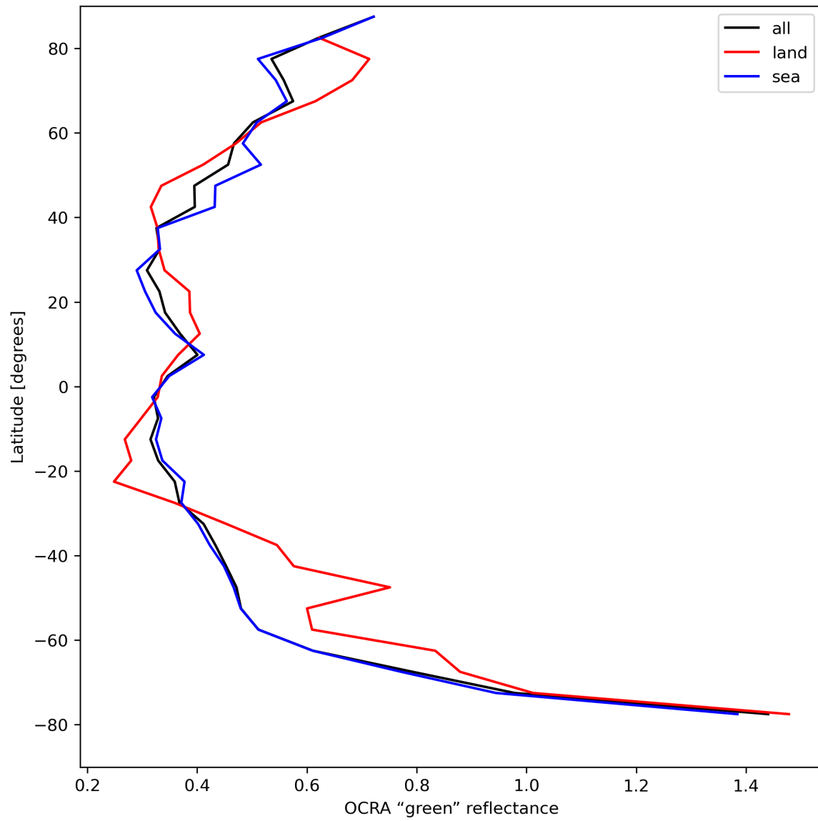
Figure 36: Zonal average of “OCRA “green” reflectance” for 2023-08-16 to 2023-08-18.
