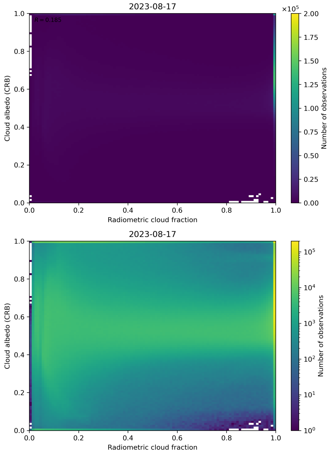
Figure 71: Scatter density plot of “Radiometric cloud fraction” against “Cloud albedo (CRB)” for 2023-08-16 to 2023-08-18.
