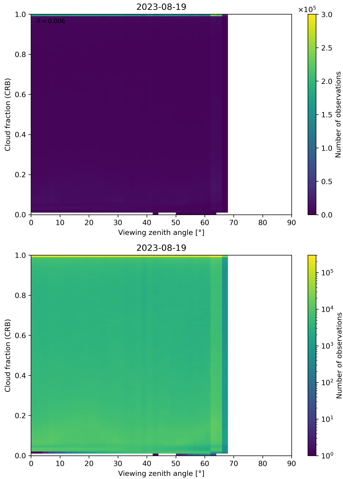
Figure 109: Scatter density plot of “Viewing zenith angle” against “Cloud fraction (CRB)” for 2023-08-18 to 2023-08-20.
