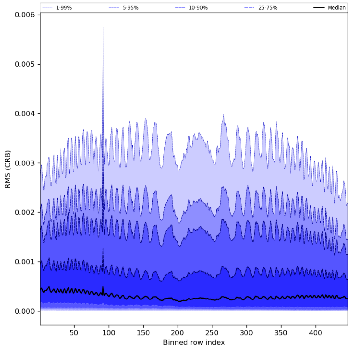
Figure 64: Along track statistics of “RMS (CRB)” for 2023-08-18 to 2023-08-20
