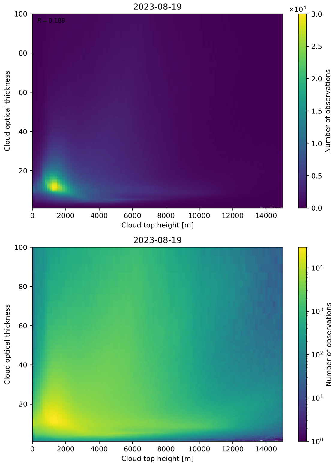
Figure 90: Scatter density plot of “Cloud top height” against “Cloud optical thickness” for 2023-08-18 to 2023-08-20.
