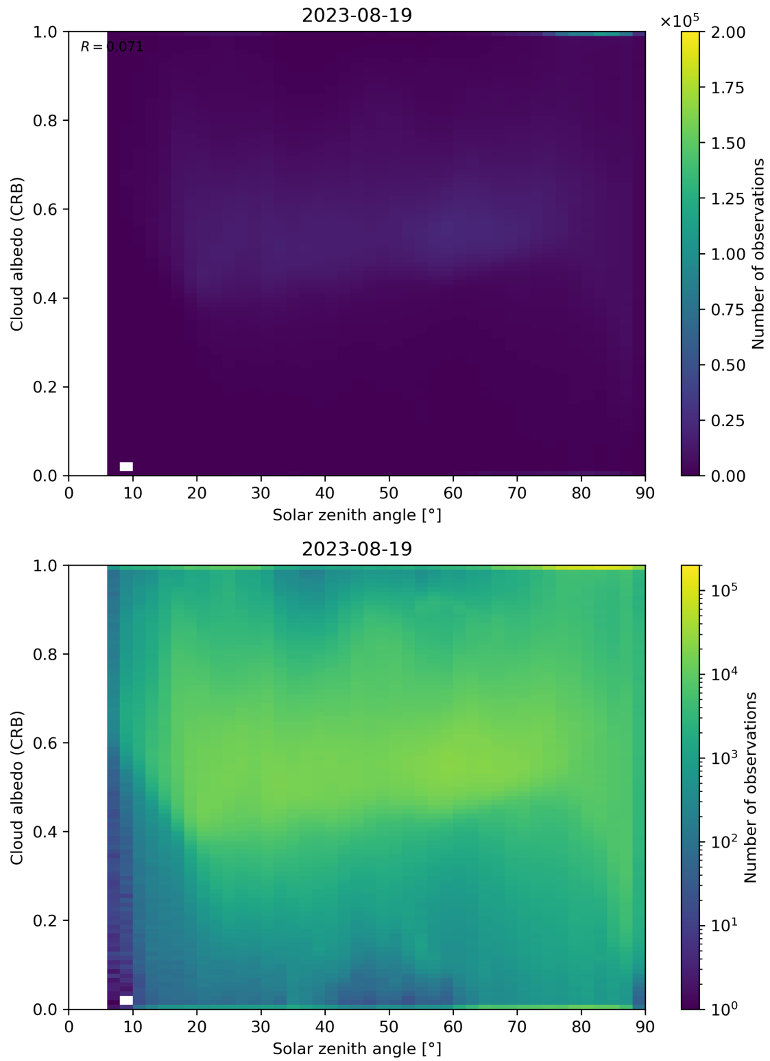
Figure 98: Scatter density plot of “Solar zenith angle” against “Cloud albedo (CRB)” for 2023-08-18 to 2023-08-20.
