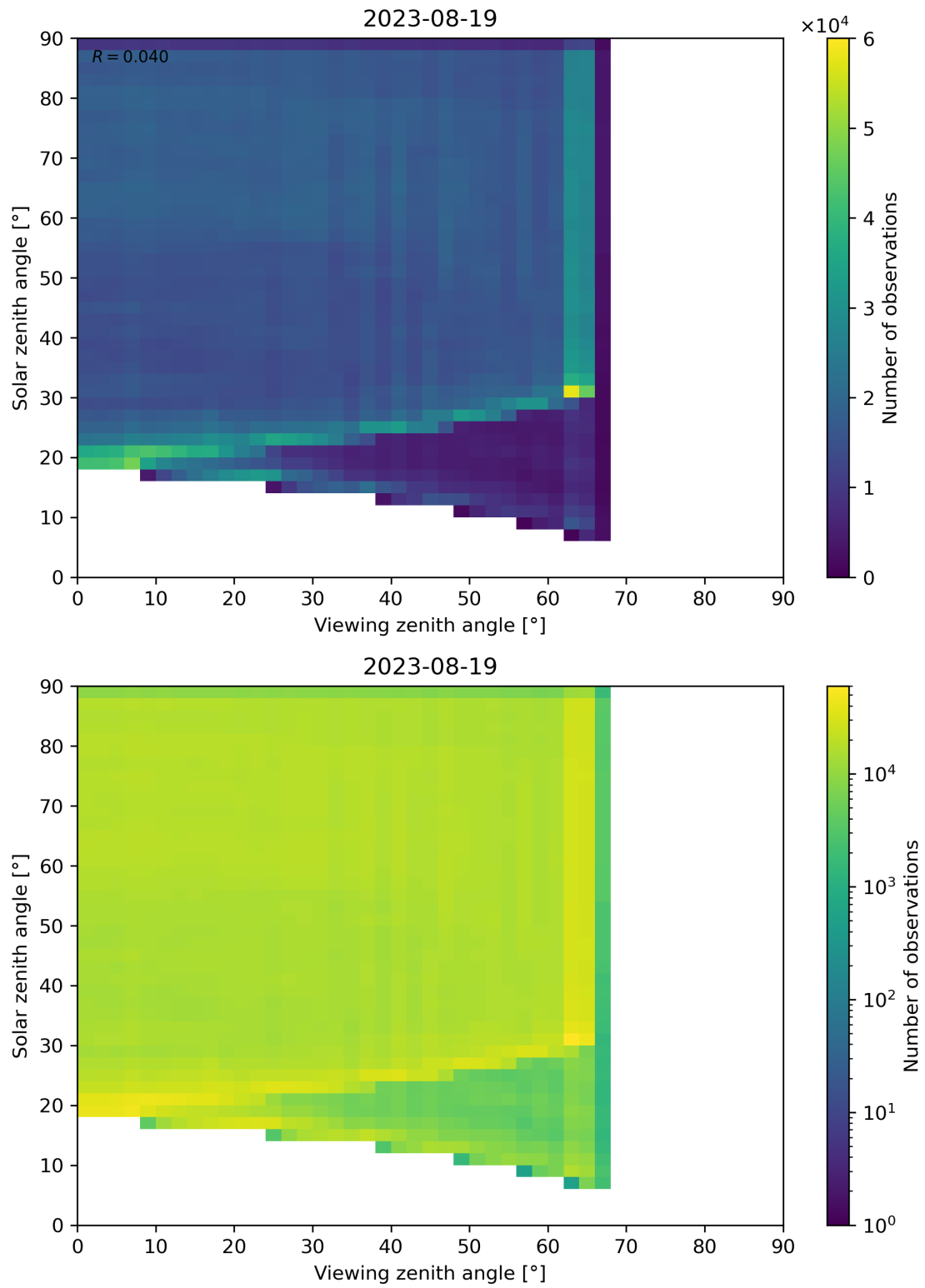
Figure 114: Scatter density plot of “Viewing zenith angle” against “Solar zenith angle” for 2023-08-18 to 2023-08-20.
