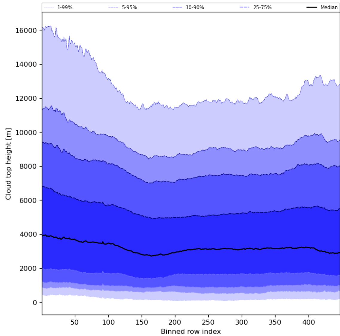
Figure 56: Along track statistics of “Cloud top height” for 2023-08-18 to 2023-08-20
