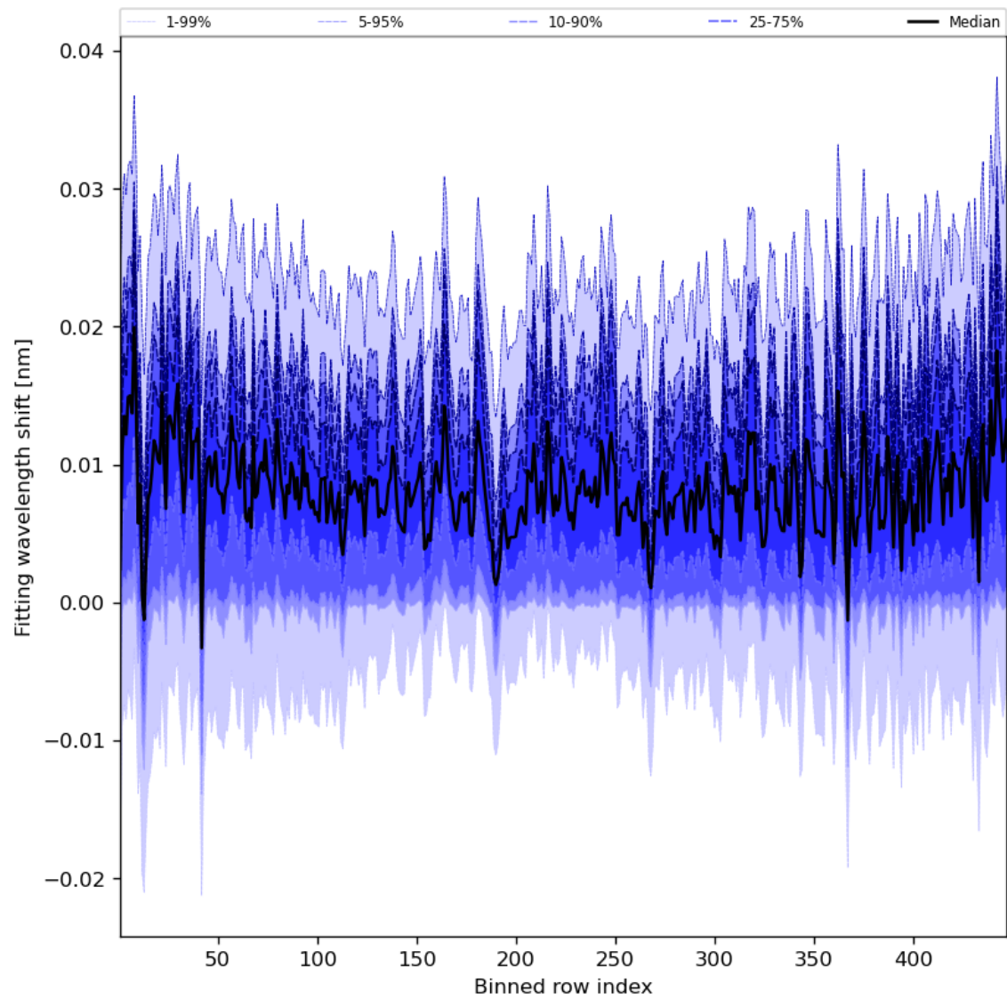
Figure 65: Along track statistics of “Fitting wavelength shift” for 2023-08-18 to 2023-08-20
