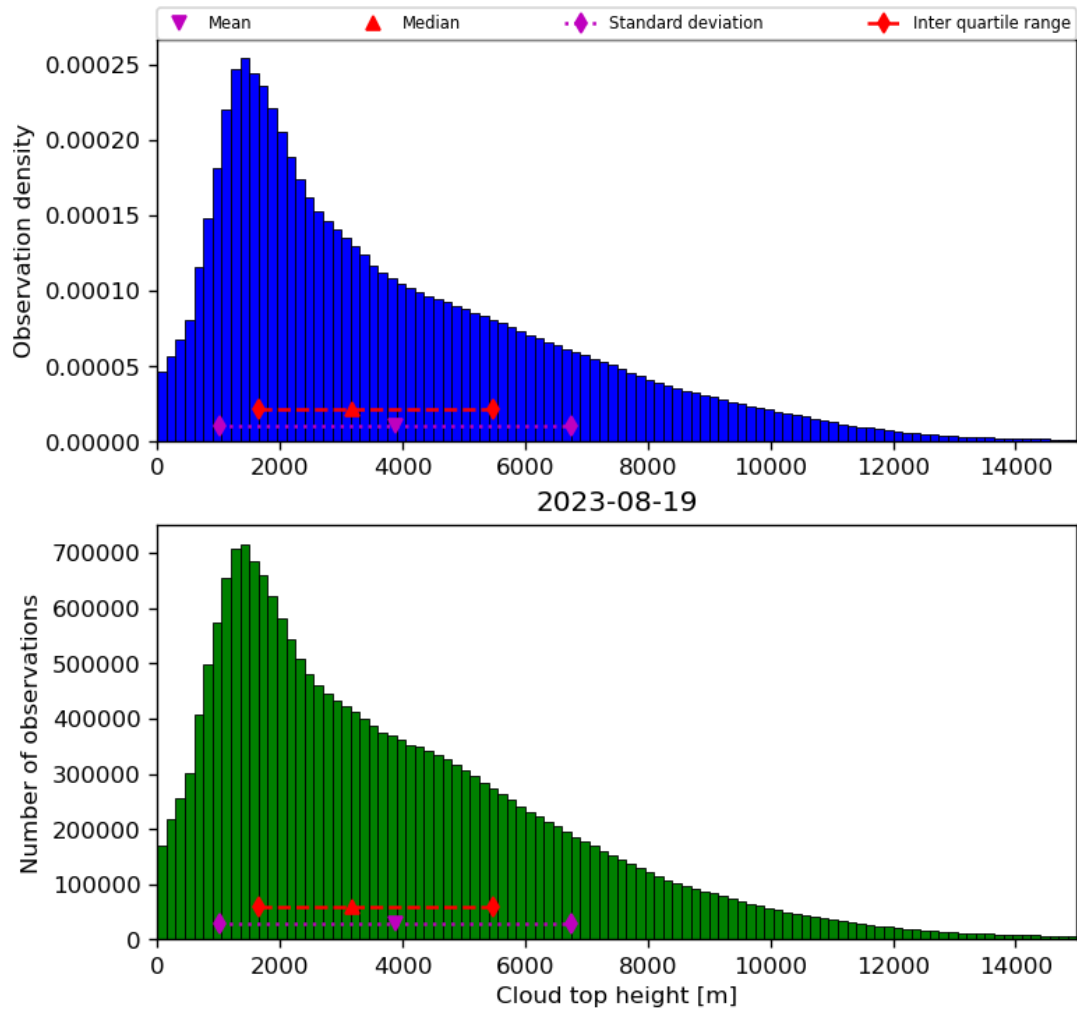
Figure 40: Histogram of “Cloud top height” for 2023-08-18 to 2023-08-20
