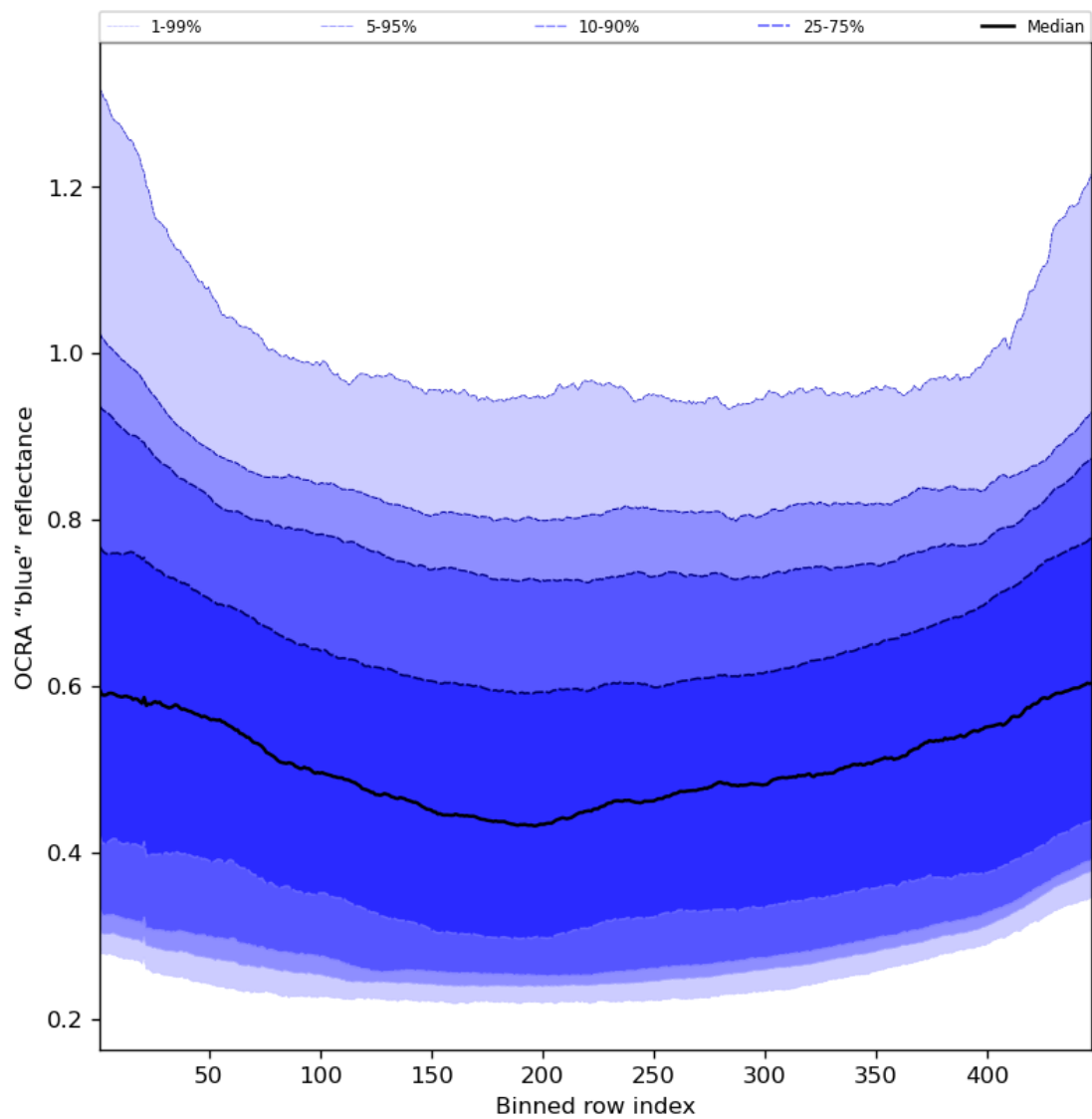
Figure 67: Along track statistics of “OCRA “blue” reflectance” for 2023-08-18 to 2023-08-20
