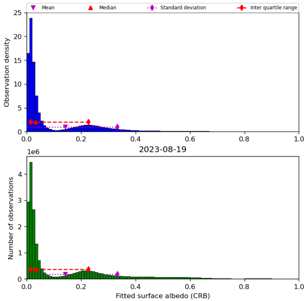
Figure 46: Histogram of “Fitted surface albedo (CRB)” for 2023-08-18 to 2023-08-20
