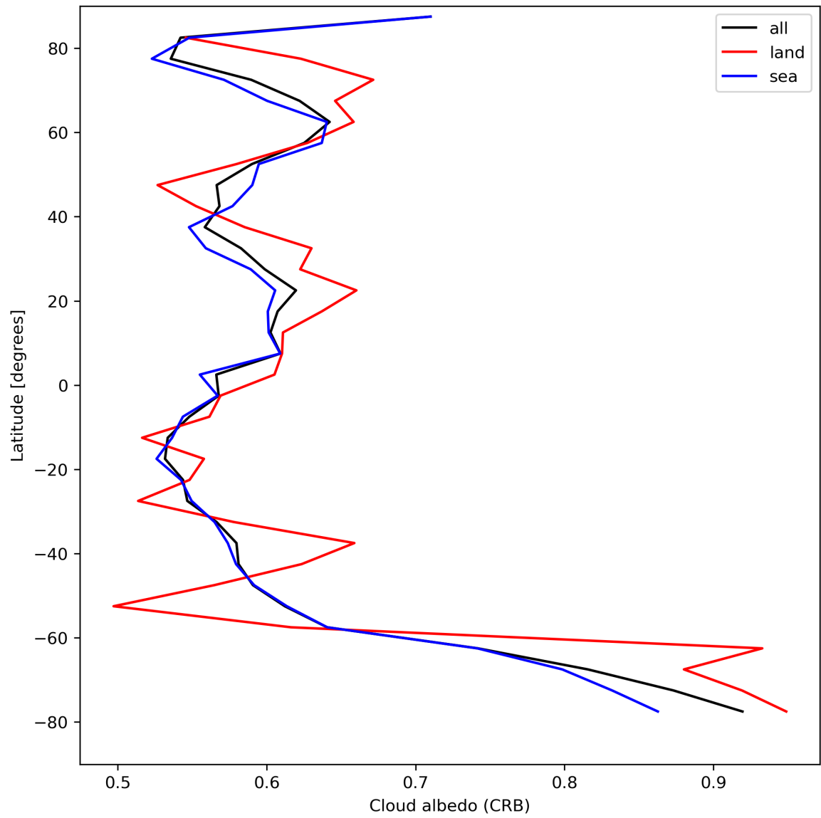
Figure 28: Zonal average of “Cloud albedo (CRB)” for 2023-08-18 to 2023-08-20.
