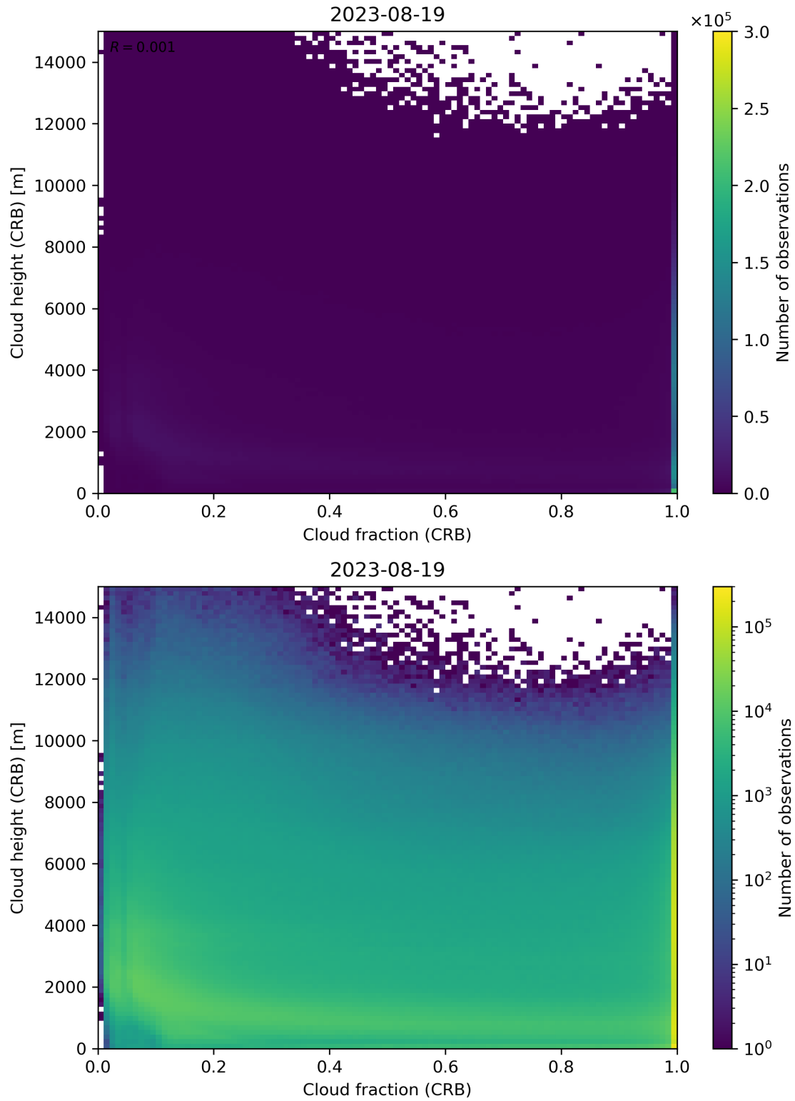
Figure 79: Scatter density plot of “Cloud fraction (CRB)” against “Cloud height (CRB)” for 2023-08-18 to 2023-08-20.
