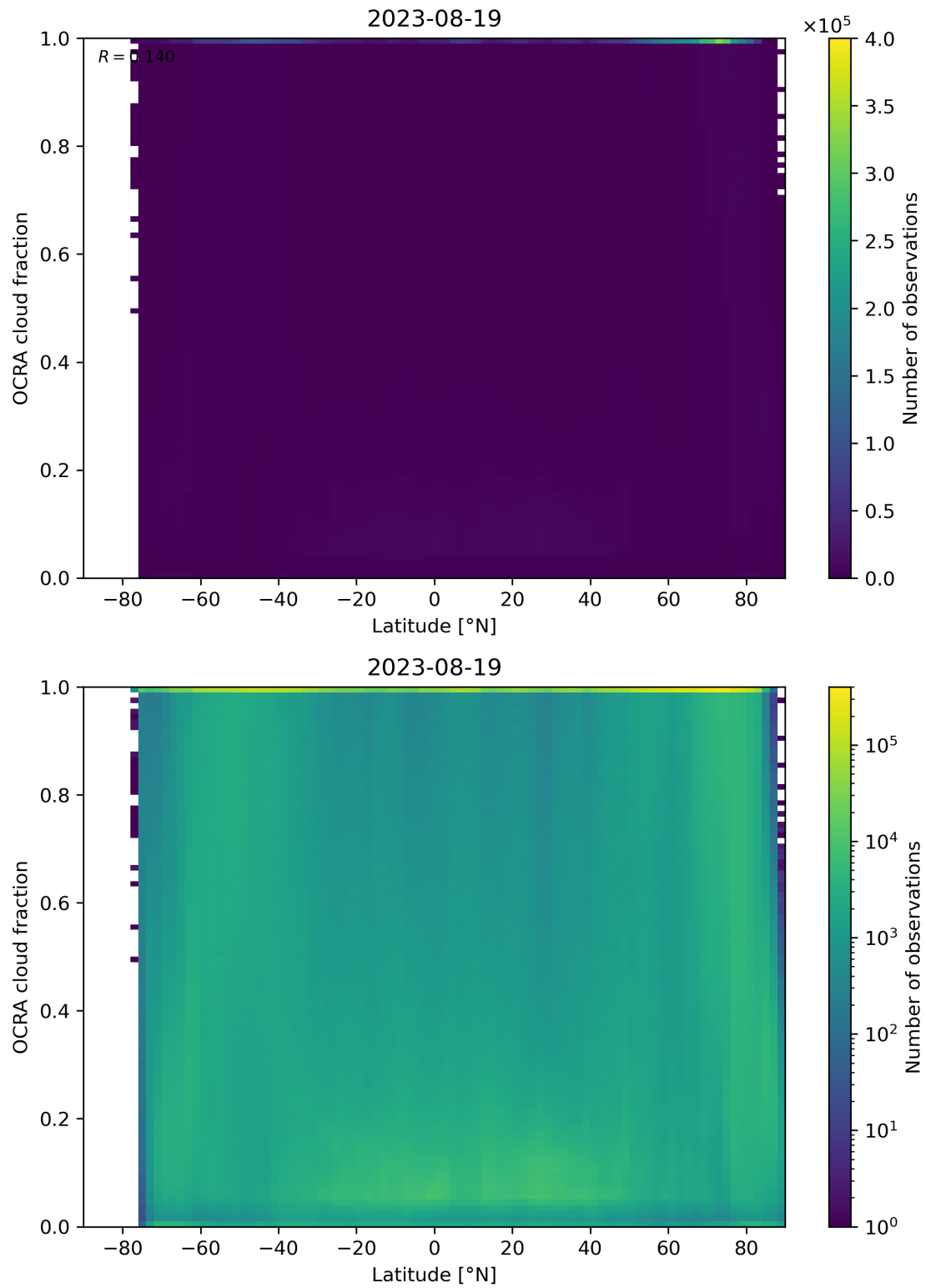
Figure 93: Scatter density plot of “Latitude” against “OCRA cloud fraction” for 2023-08-18 to 2023-08-20.
