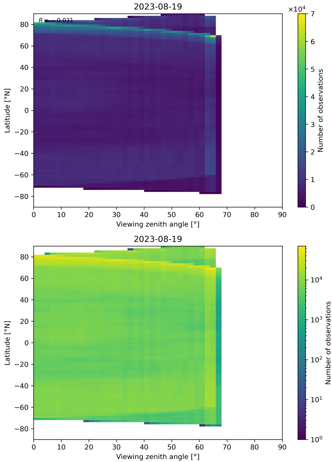
Figure 113: Scatter density plot of “Viewing zenith angle” against “Latitude” for 2023-08-18 to 2023-08-20.
