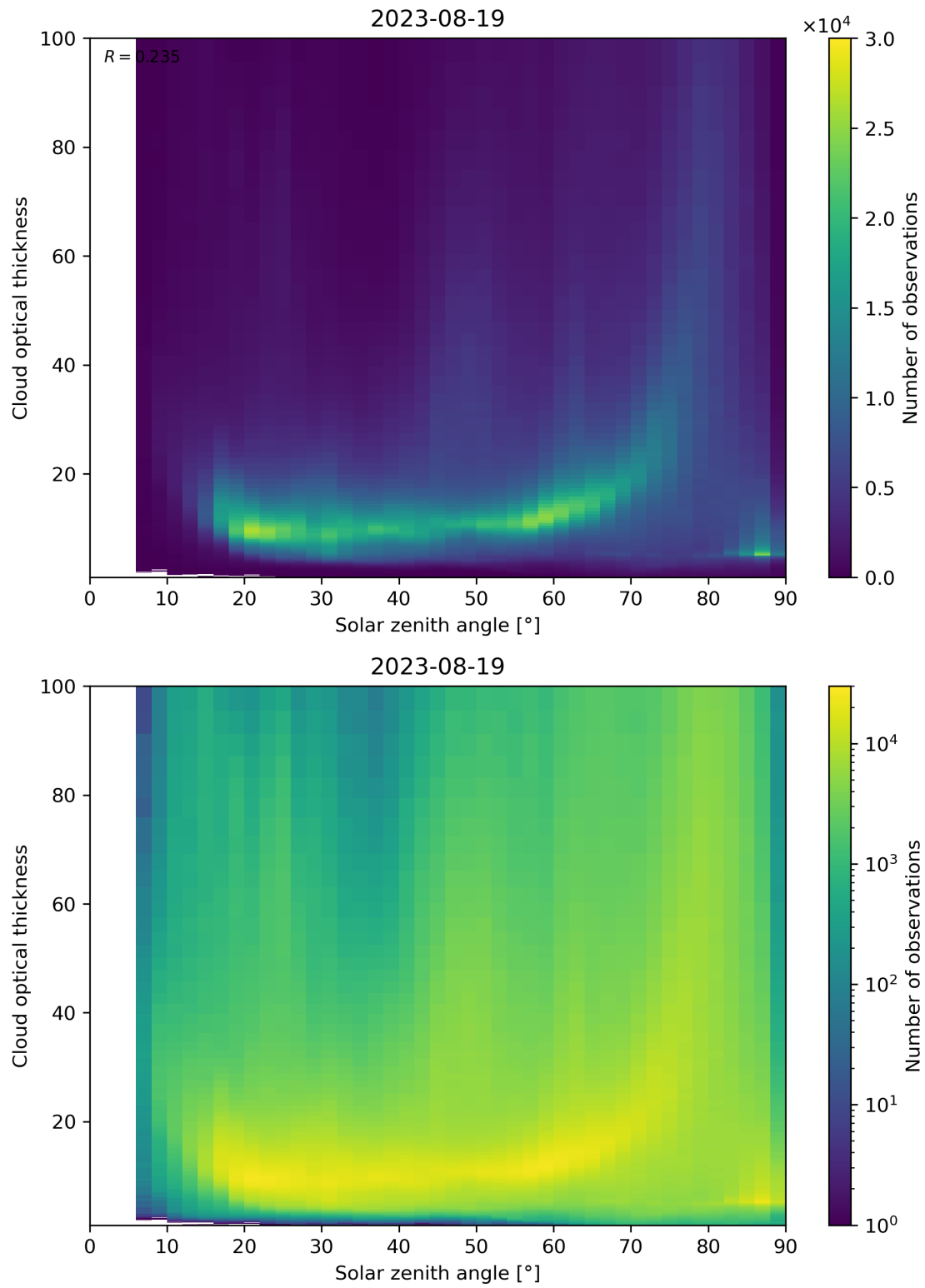
Figure 103: Scatter density plot of “Solar zenith angle” against “Cloud optical thickness” for 2023-08-18 to 2023-08-20.
