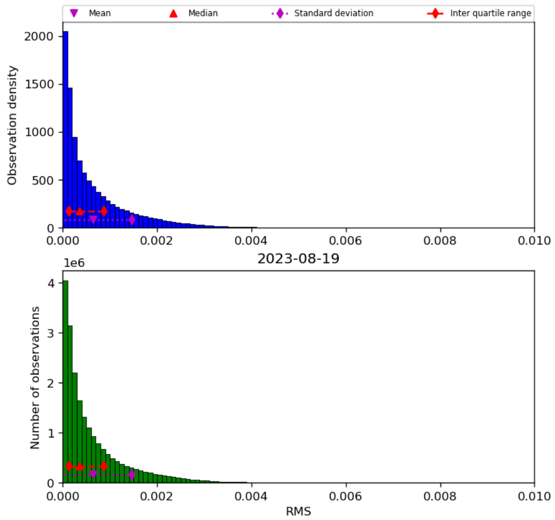
Figure 47: Histogram of “RMS” for 2023-08-18 to 2023-08-20
