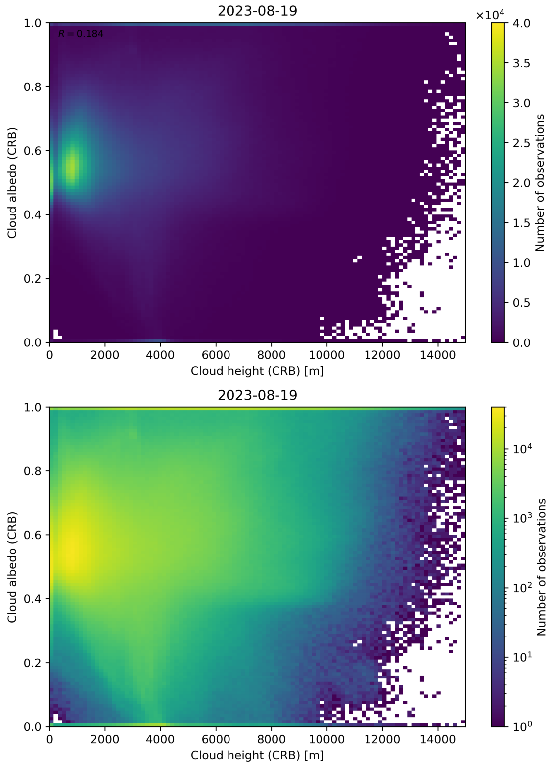
Figure 80: Scatter density plot of “Cloud height (CRB)” against “Cloud albedo (CRB)” for 2023-08-18 to 2023-08-20.
