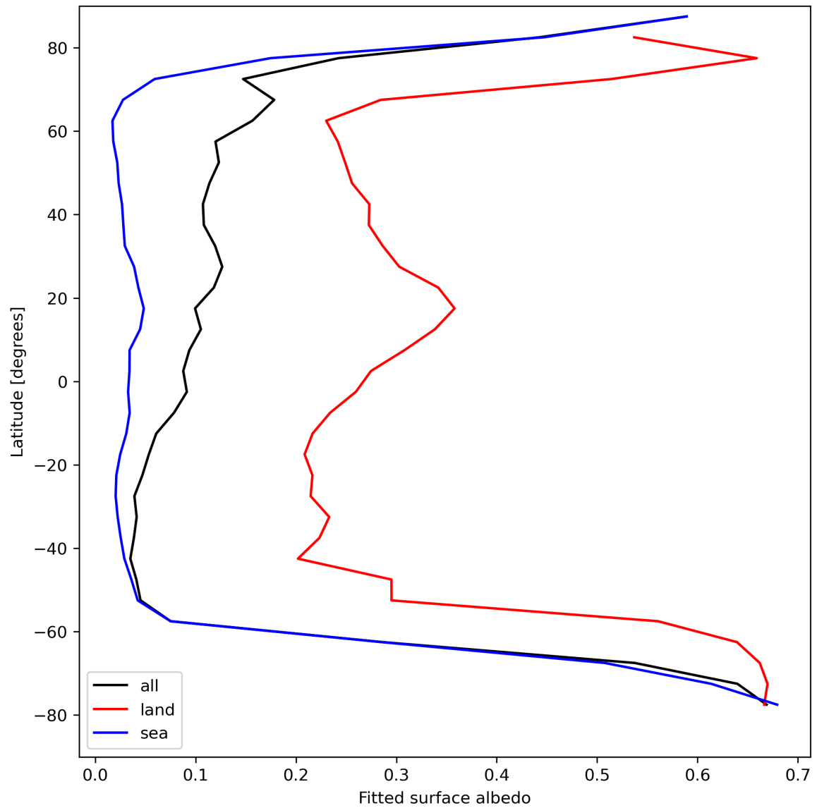
Figure 29: Zonal average of “Fitted surface albedo” for 2023-08-18 to 2023-08-20.
