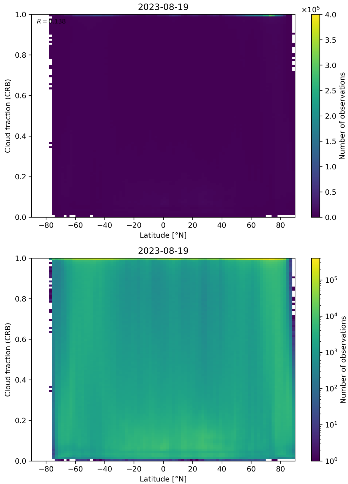
Figure 94: Scatter density plot of “Latitude” against “Cloud fraction (CRB)” for 2023-08-18 to 2023-08-20.
