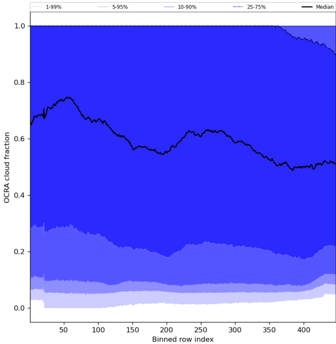
Figure 66: Along track statistics of “OCRA cloud fraction” for 2023-08-18 to 2023-08-20
