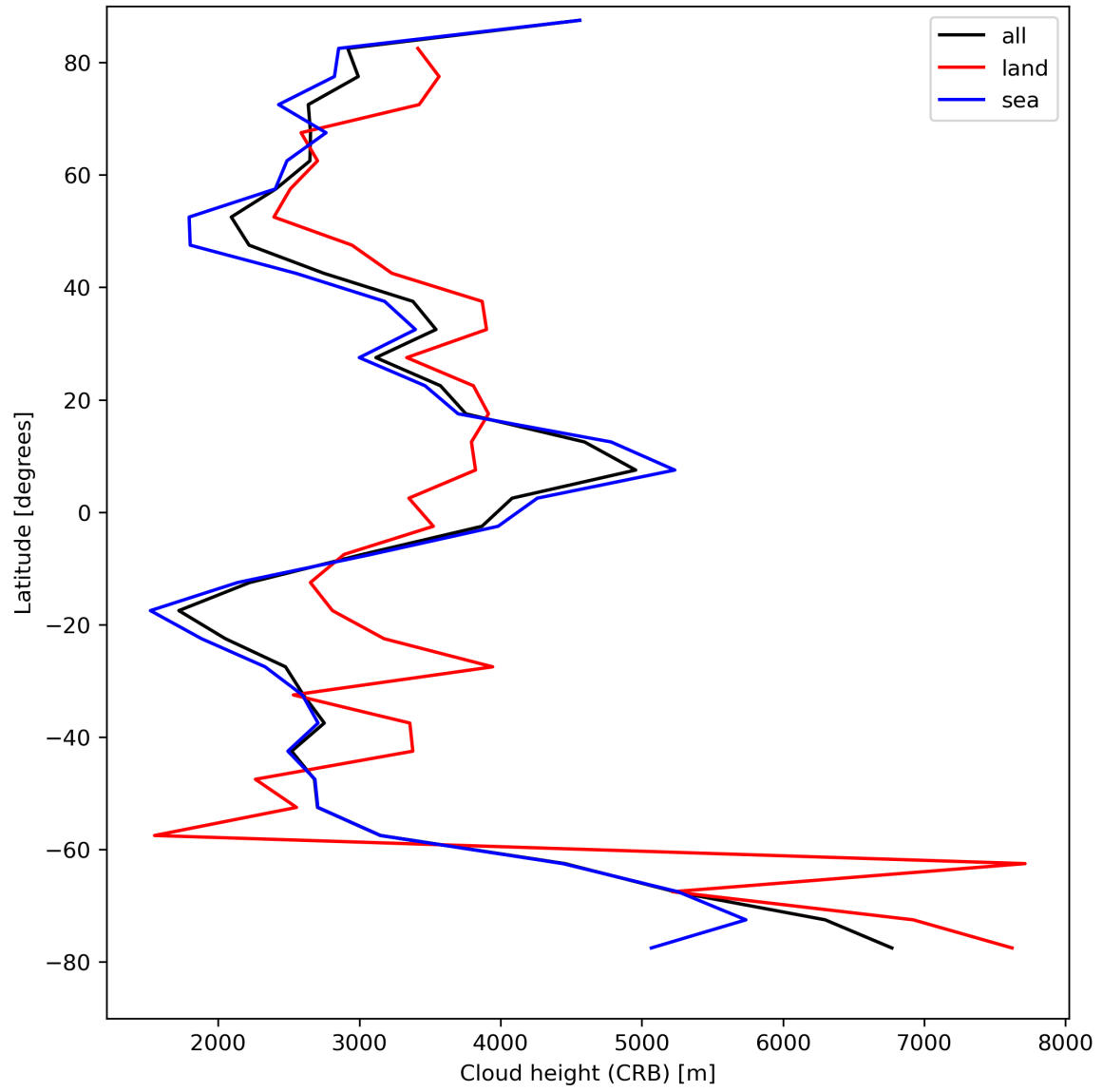
Figure 27: Zonal average of “Cloud height (CRB)” for 2023-08-18 to 2023-08-20.
