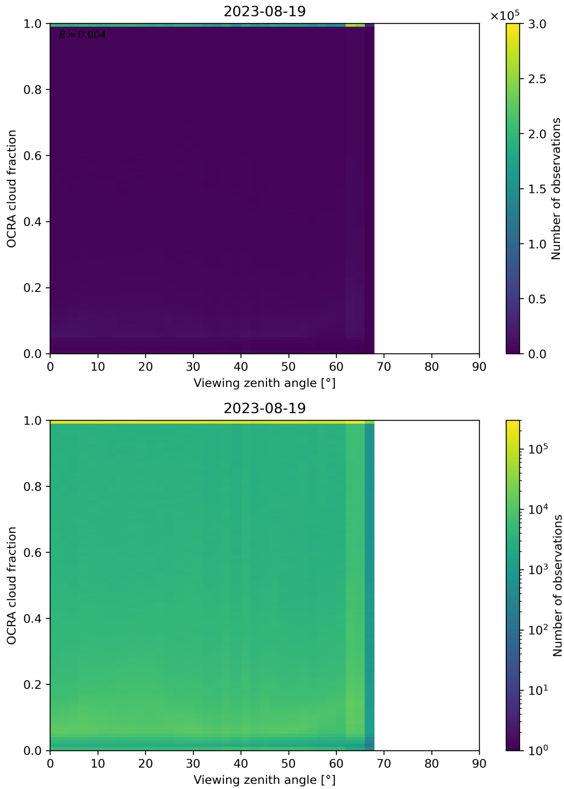
Figure 108: Scatter density plot of “Viewing zenith angle” against “OCRA cloud fraction” for 2023-08-18 to 2023-08-20.
