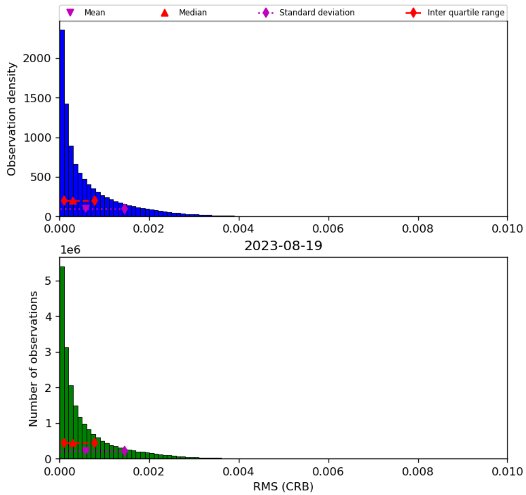
Figure 48: Histogram of "RMS (CRB)" for 2023-08-18 to 2023-08-20
