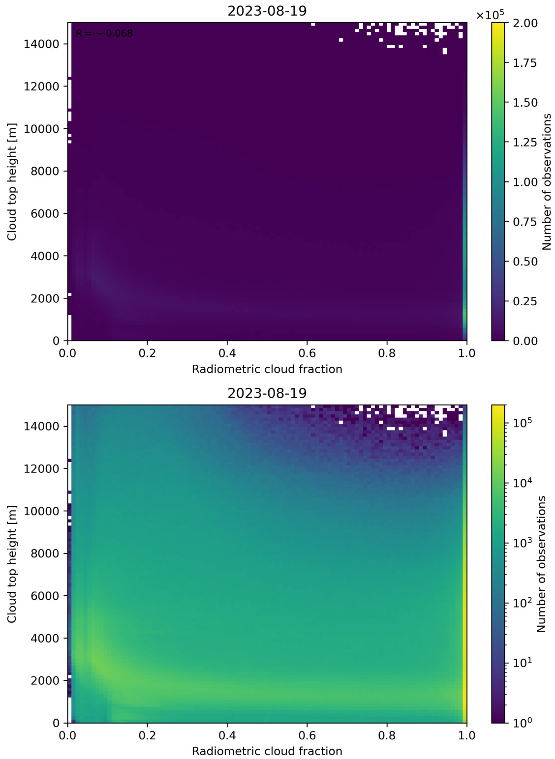
Figure 76: Scatter density plot of “Radiometric cloud fraction” against “Cloud top height” for 2023-08-18 to 2023-08-20.
