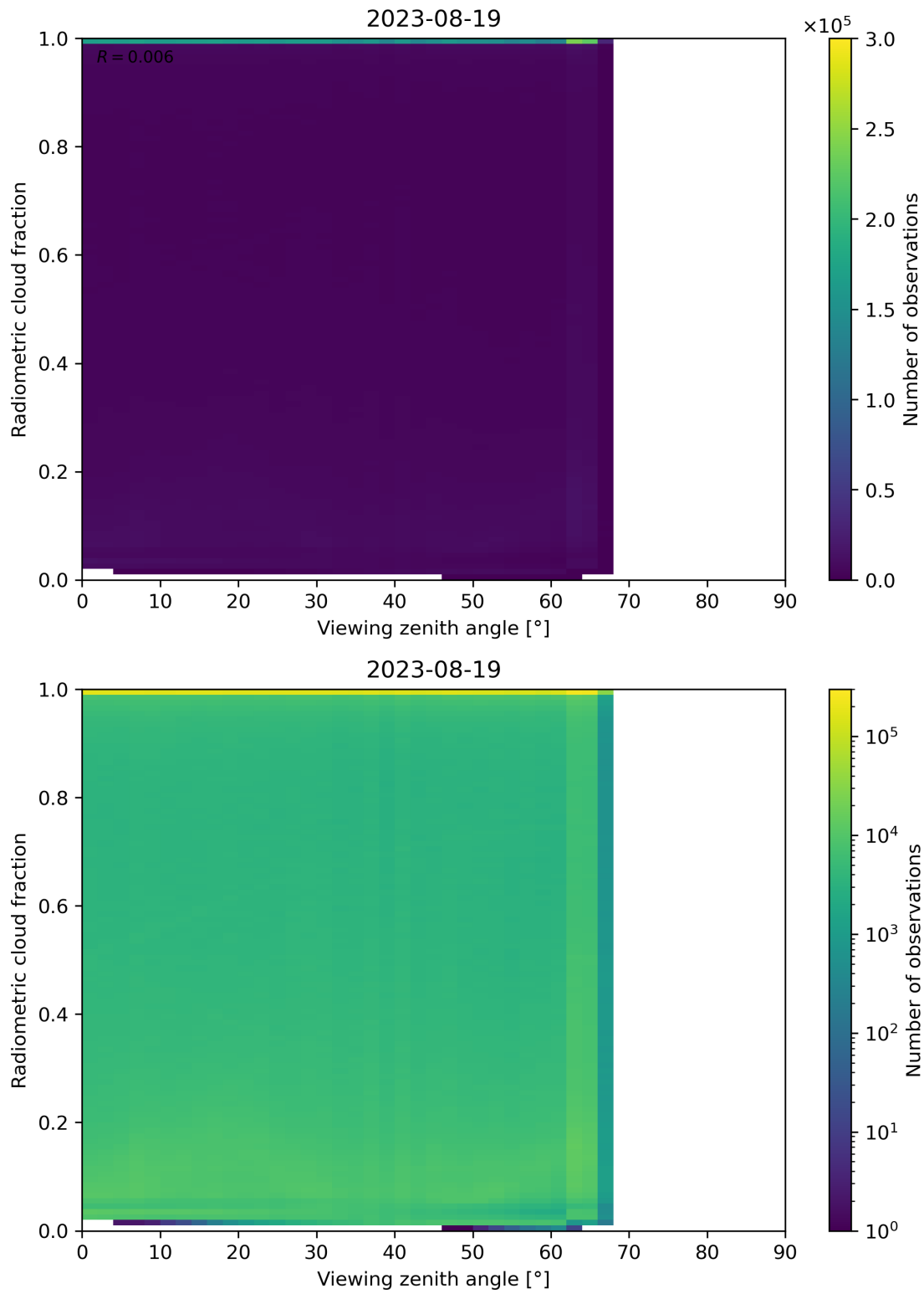
Figure 107: Scatter density plot of “Viewing zenith angle” against “Radiometric cloud fraction” for 2023-08-18 to 2023-08-20.
