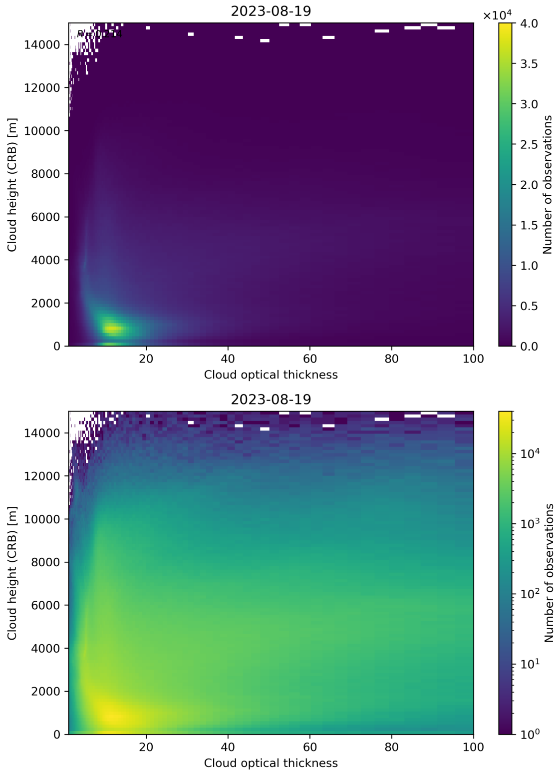
Figure 85: Scatter density plot of “Cloud optical thickness” against “Cloud height (CRB)” for 2023-08-18 to 2023-08-20.
