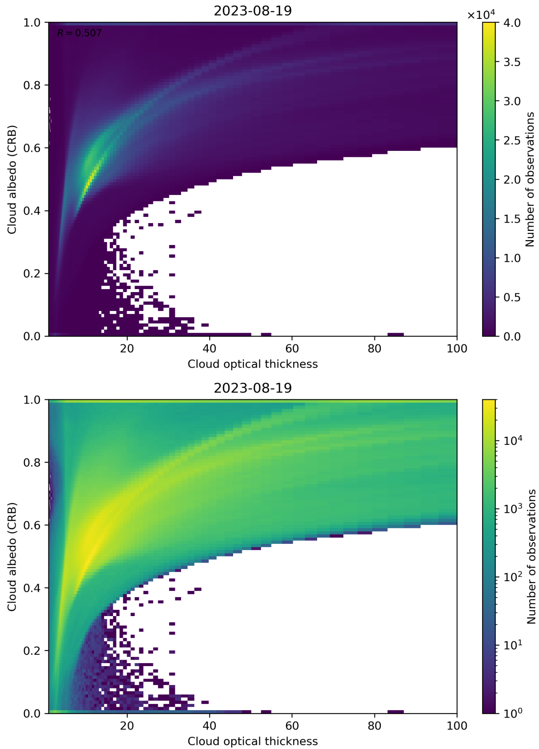
Figure 82: Scatter density plot of “Cloud optical thickness” against “Cloud albedo (CRB)” for 2023-08-18 to 2023-08-20.
