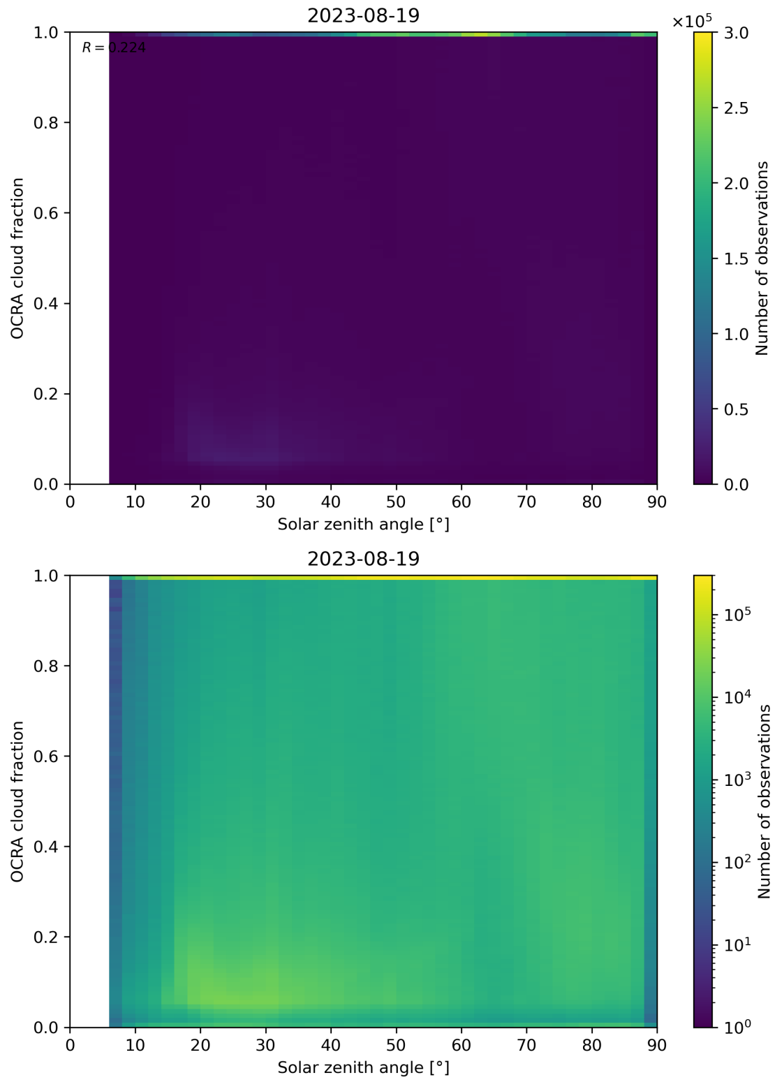
Figure 100: Scatter density plot of “Solar zenith angle” against “OCRA cloud fraction” for 2023-08-18 to 2023-08-20.
