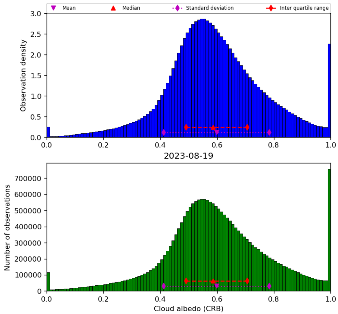
Figure 44: Histogram of “Cloud albedo (CRB)” for 2023-08-18 to 2023-08-20
