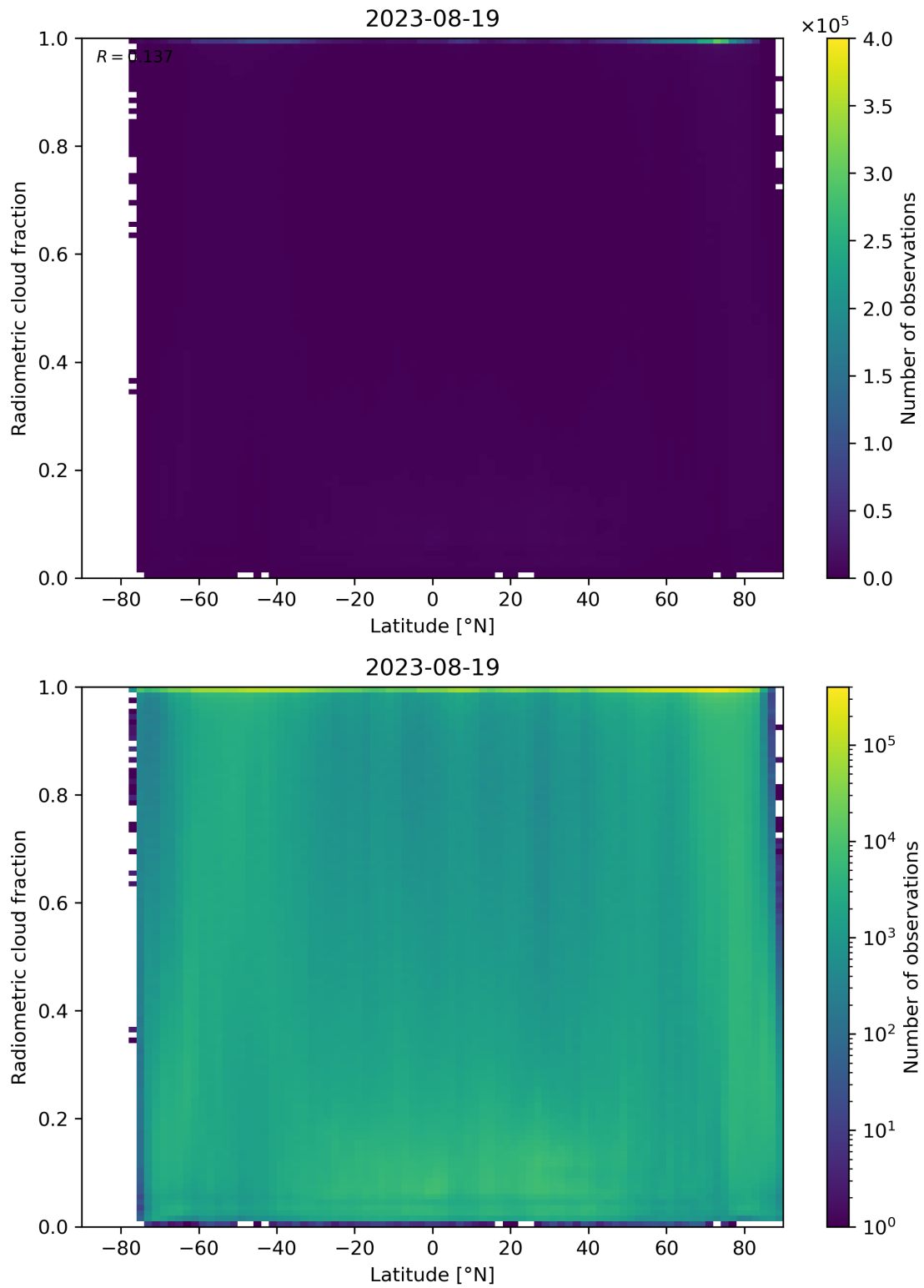
Figure 92: Scatter density plot of “Latitude” against “Radiometric cloud fraction” for 2023-08-18 to 2023-08-20.
