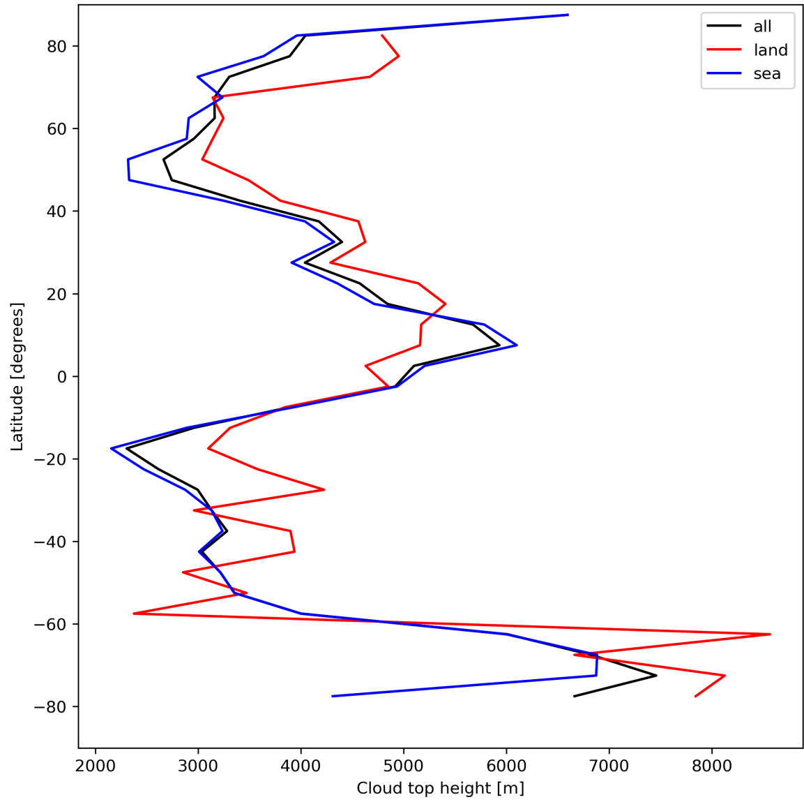
Figure 24: Zonal average of “Cloud top height” for 2023-08-18 to 2023-08-20.
