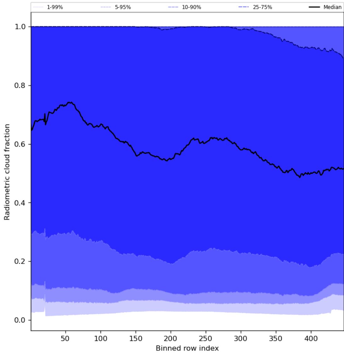
Figure 55: Along track statistics of “Radiometric cloud fraction” for 2023-08-18 to 2023-08-20
