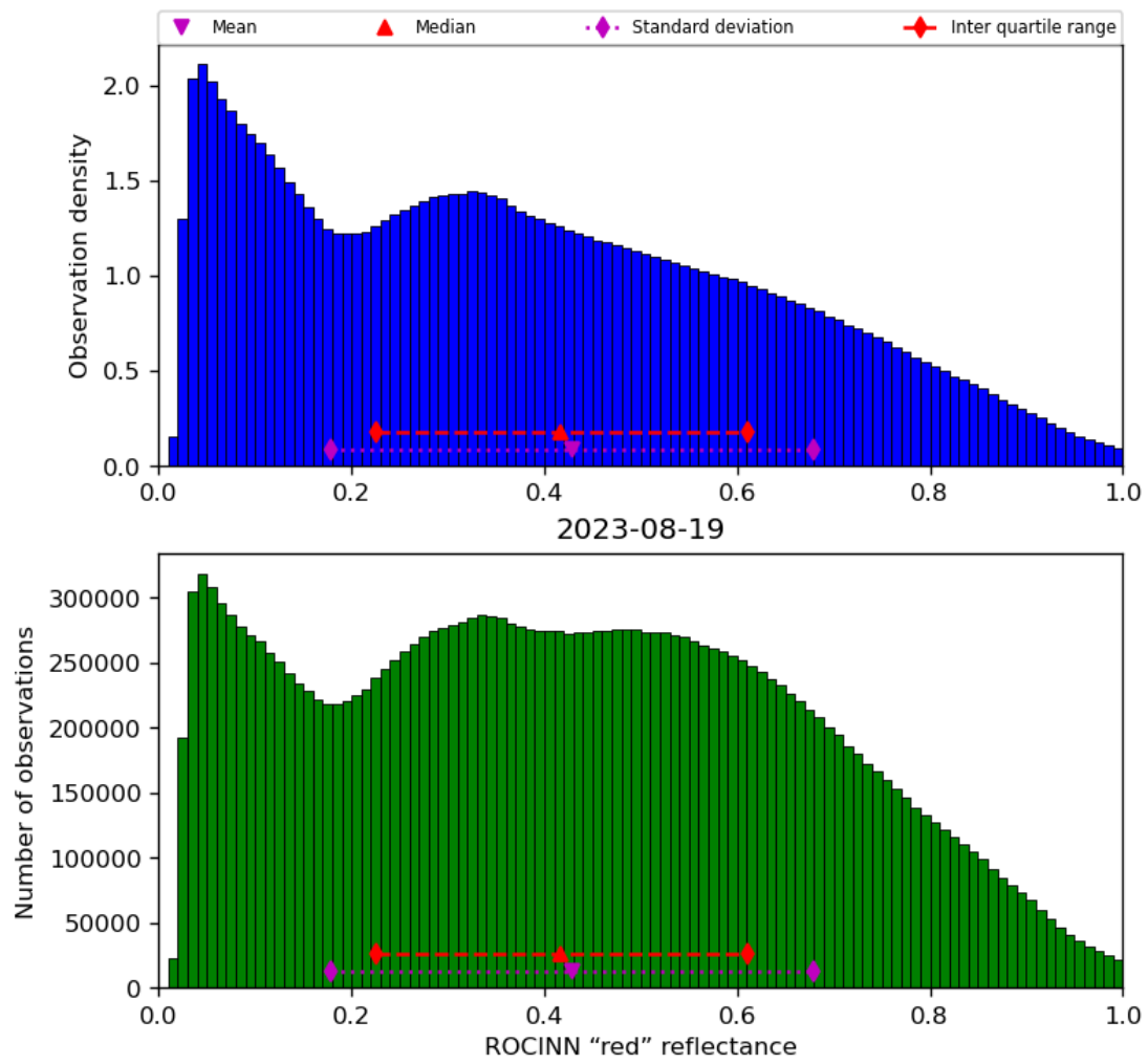
Figure 53: Histogram of “ROCINN “red” reflectance” for 2023-08-18 to 2023-08-20
