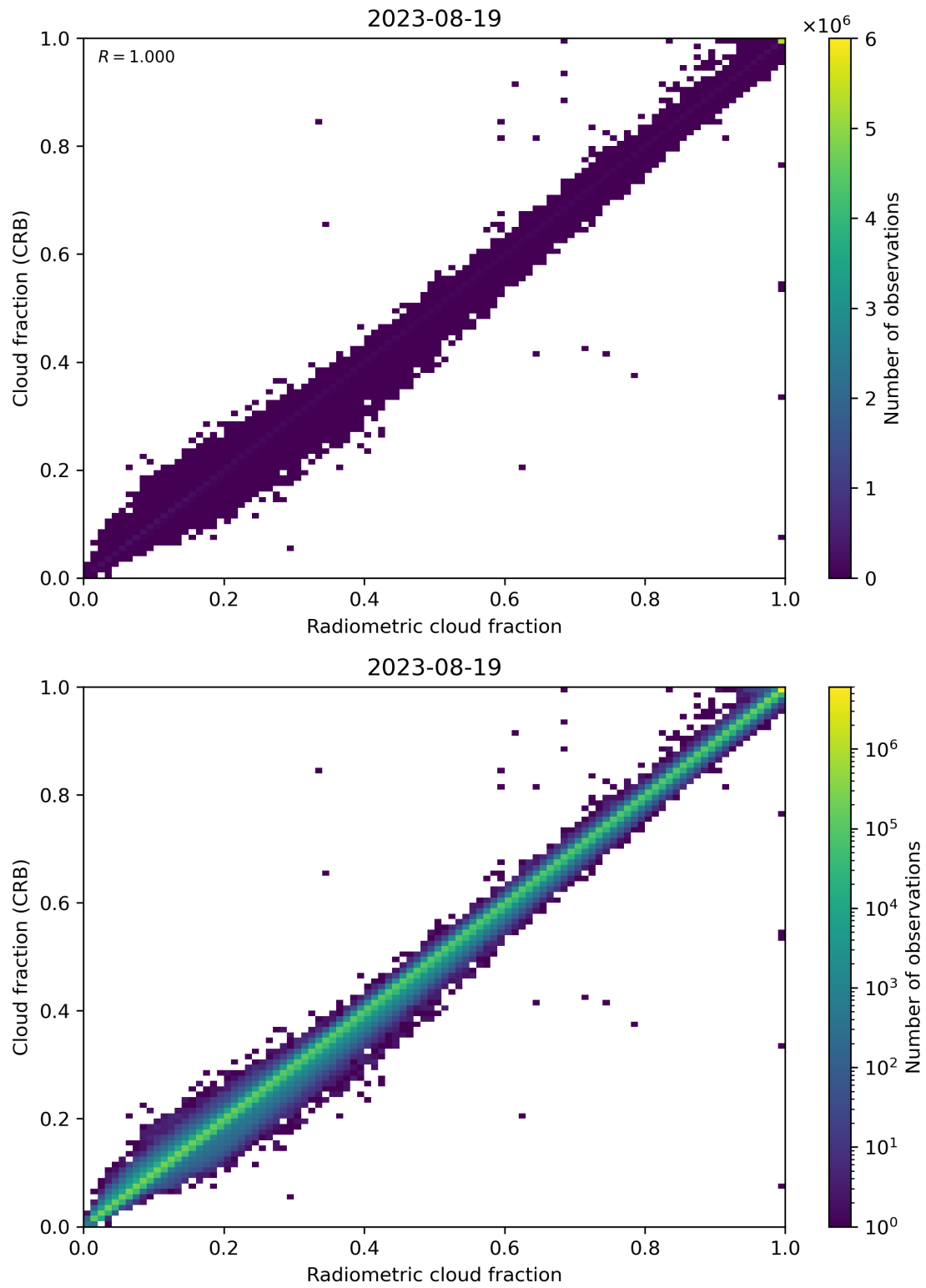
Figure 73: Scatter density plot of “Radiometric cloud fraction” against “Cloud fraction (CRB)” for 2023-08-18 to 2023-08-20.
