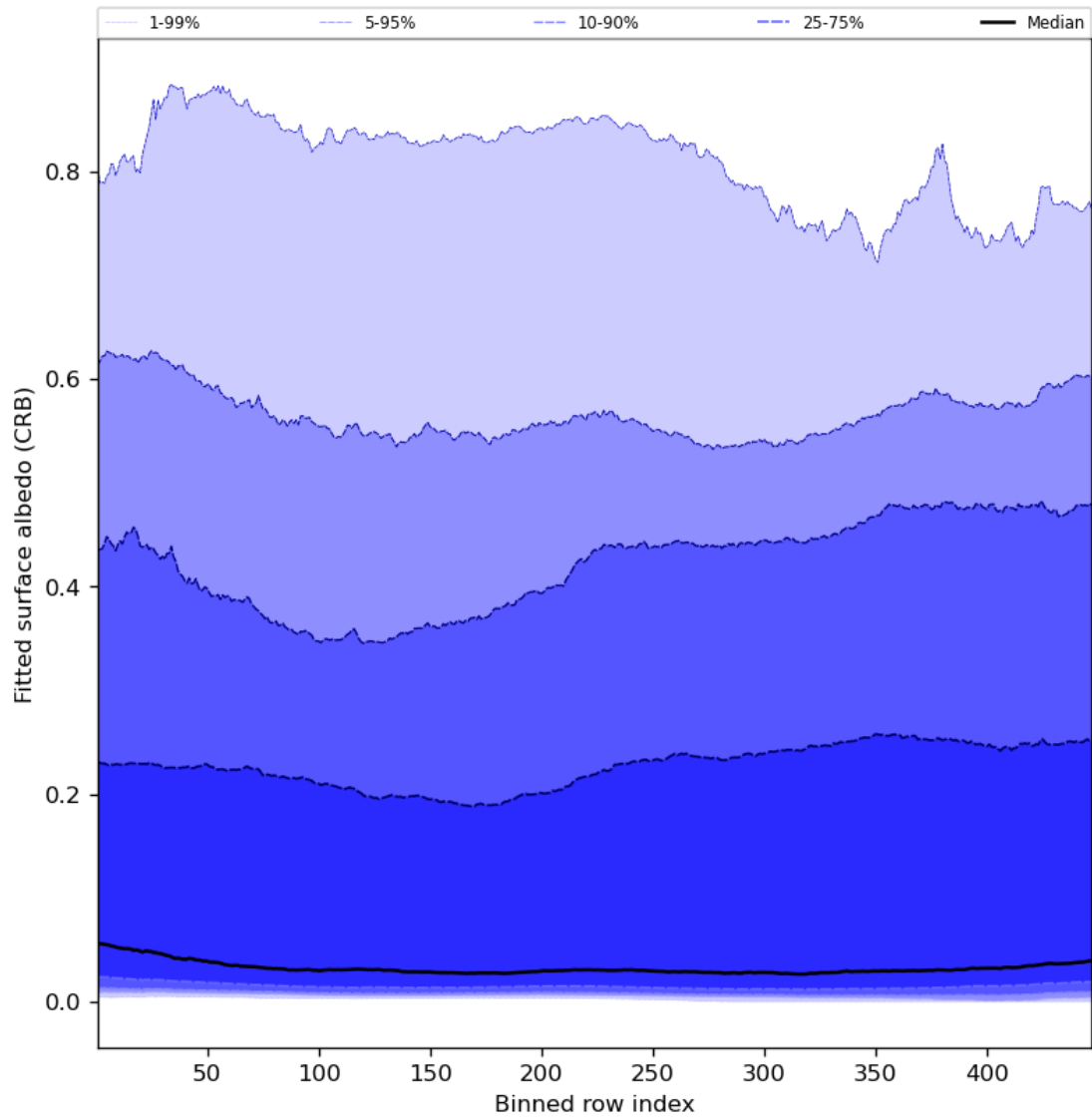
Figure 62: Along track statistics of “Fitted surface albedo (CRB)” for 2023-08-18 to 2023-08-20
