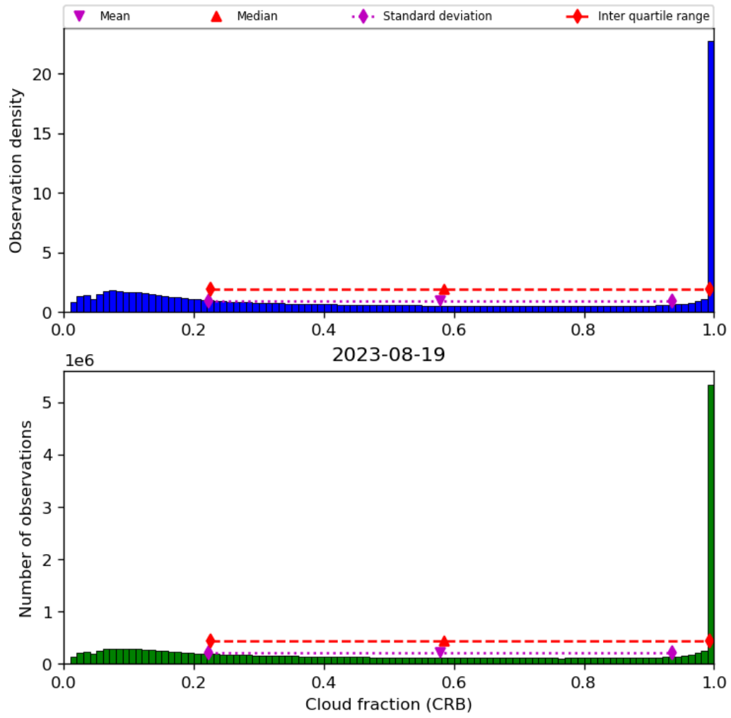
Figure 42: Histogram of “Cloud fraction (CRB)” for 2023-08-18 to 2023-08-20
