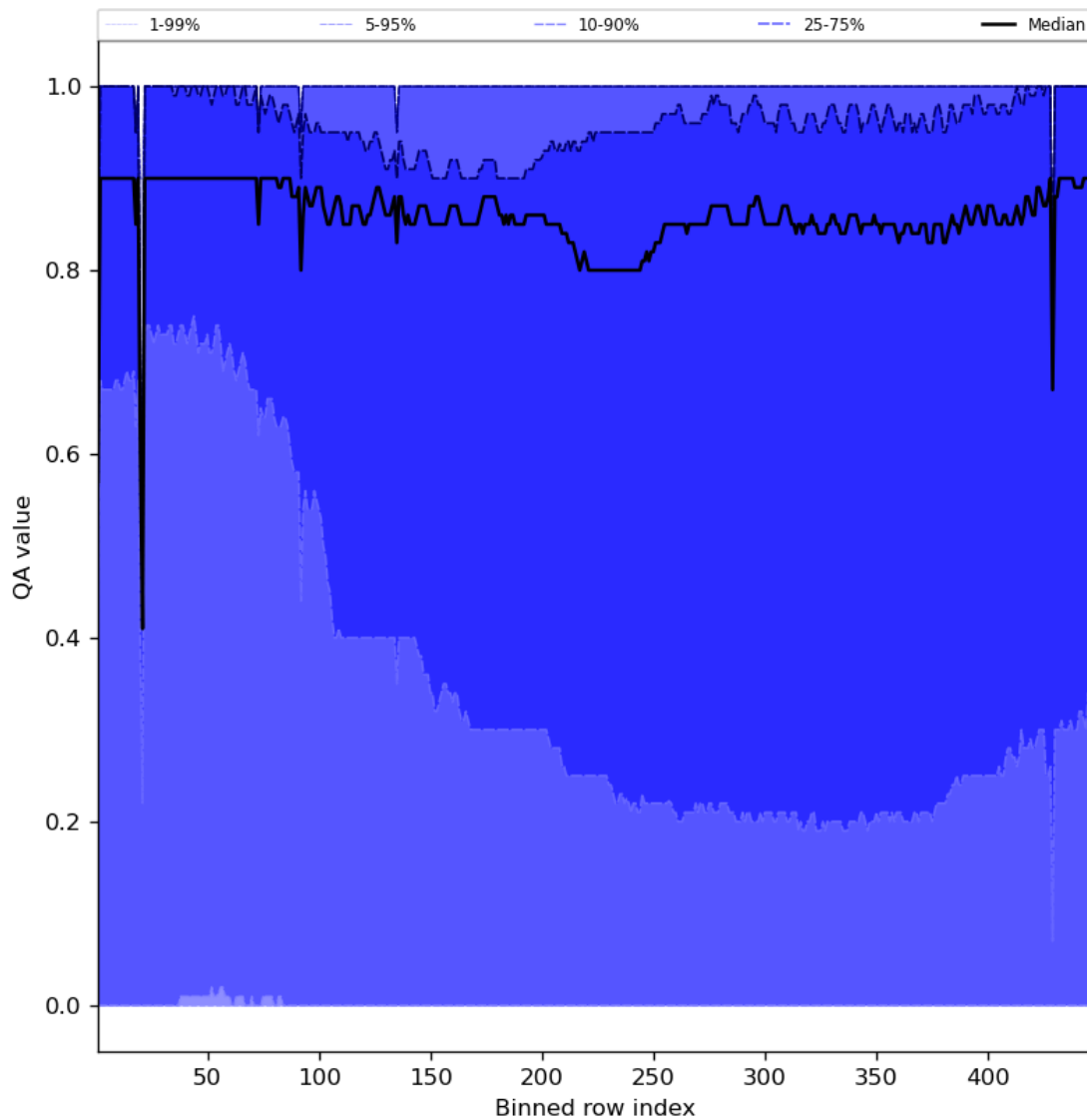
Figure 54: Along track statistics of “QA value” for 2023-08-18 to 2023-08-20
