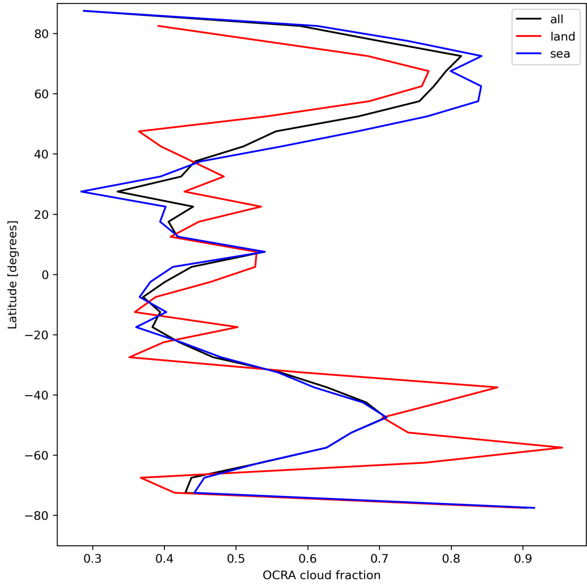
Figure 34: Zonal average of “OCRA cloud fraction” for 2023-08-18 to 2023-08-20.
