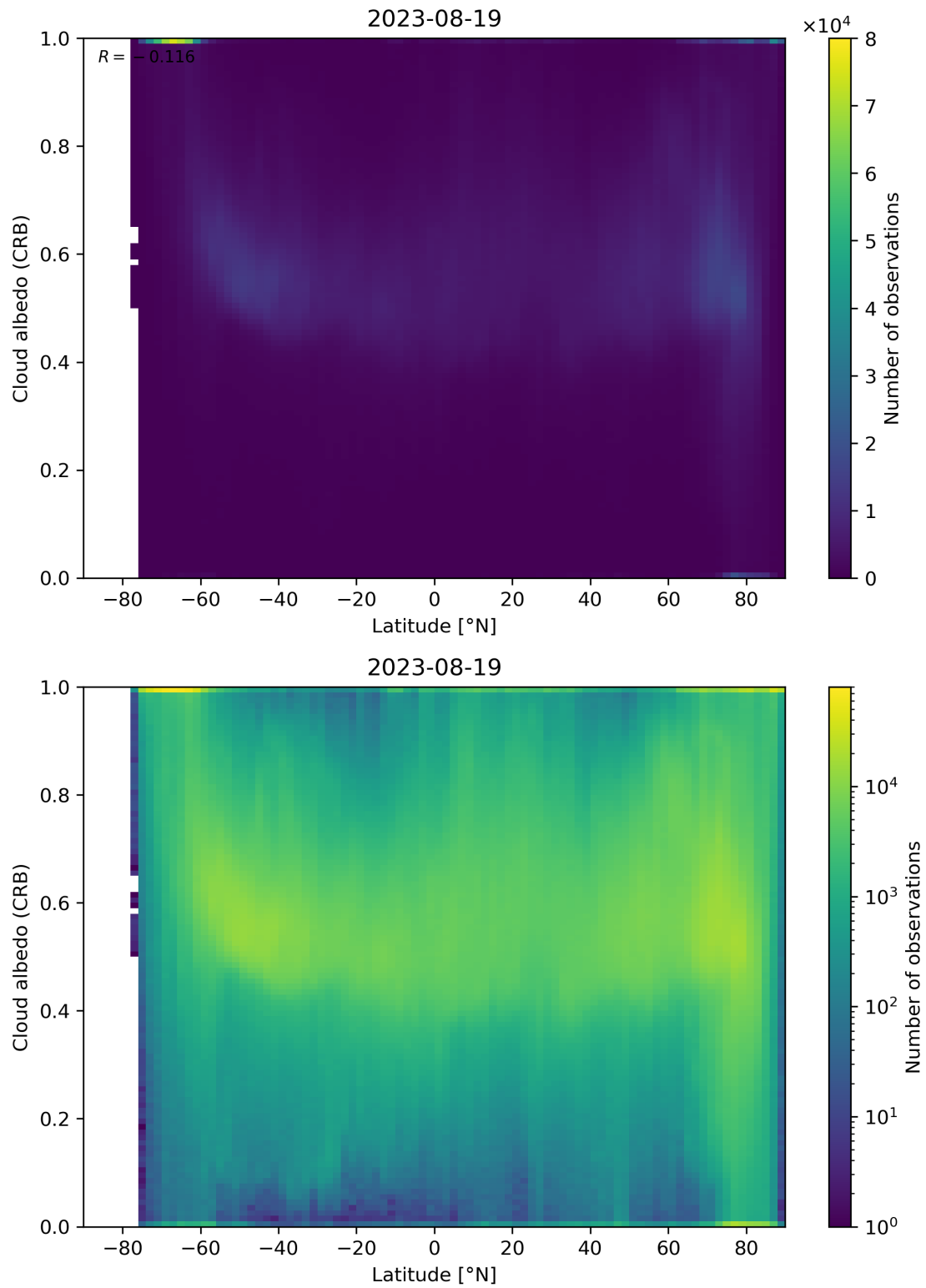
Figure 91: Scatter density plot of “Latitude” against “Cloud albedo (CRB)” for 2023-08-18 to 2023-08-20.
