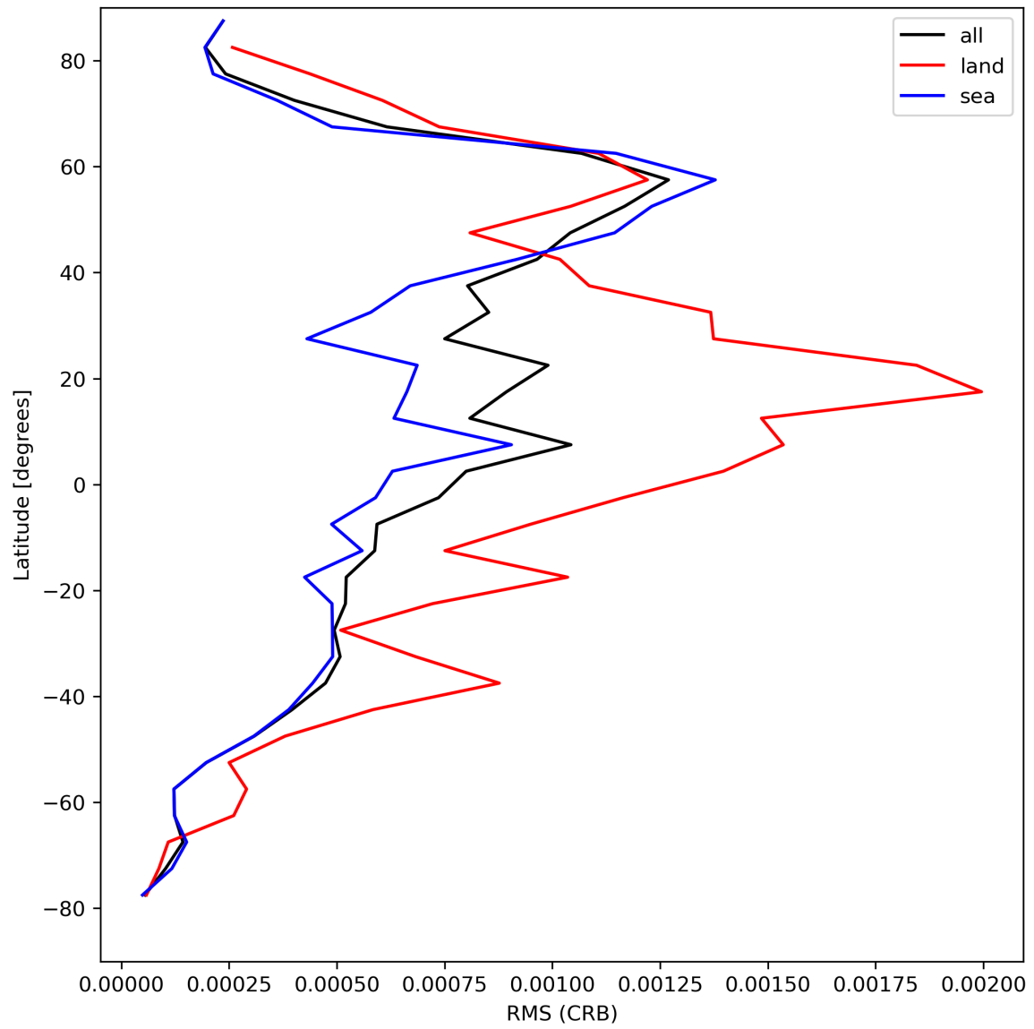
Figure 32: Zonal average of “RMS (CRB)” for 2023-08-18 to 2023-08-20.
