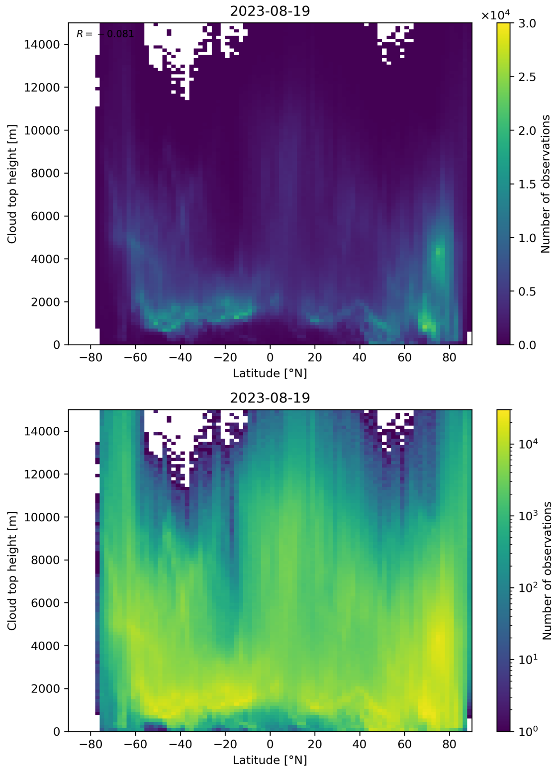
Figure 97: Scatter density plot of “Latitude” against “Cloud top height” for 2023-08-18 to 2023-08-20.
