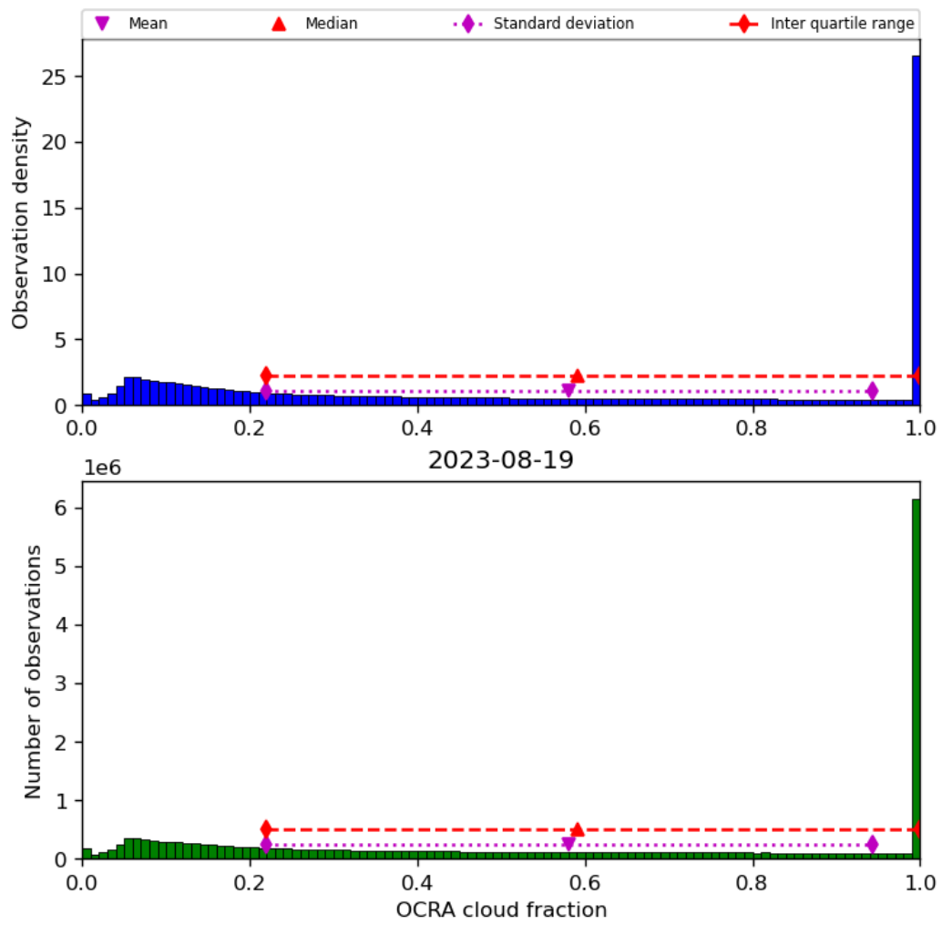
Figure 50: Histogram of “OCRA cloud fraction” for 2023-08-18 to 2023-08-20
