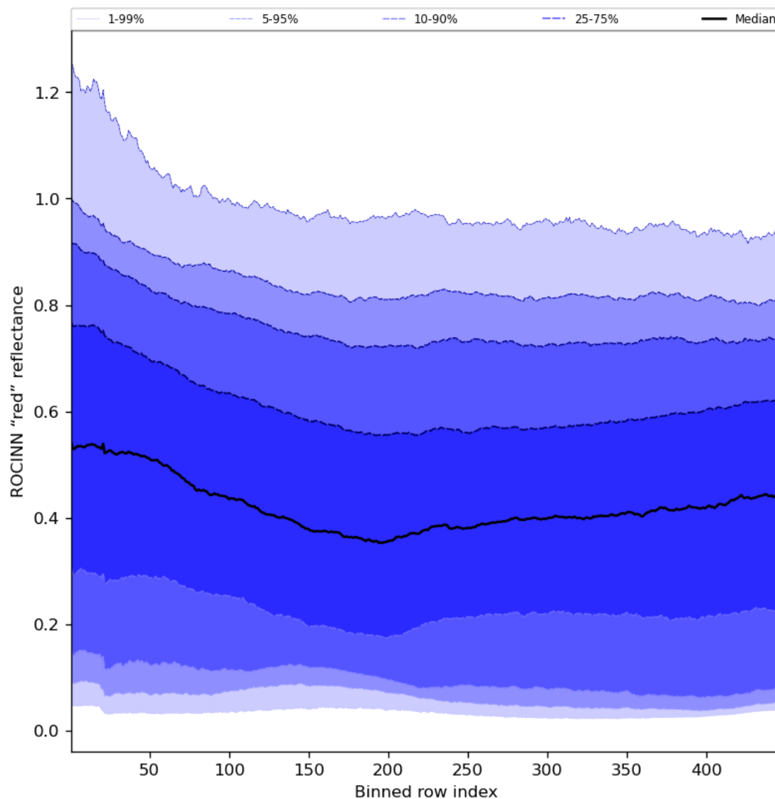
Figure 69: Along track statistics of “ROCINN “red” reflectance” for 2023-08-18 to 2023-08-20
