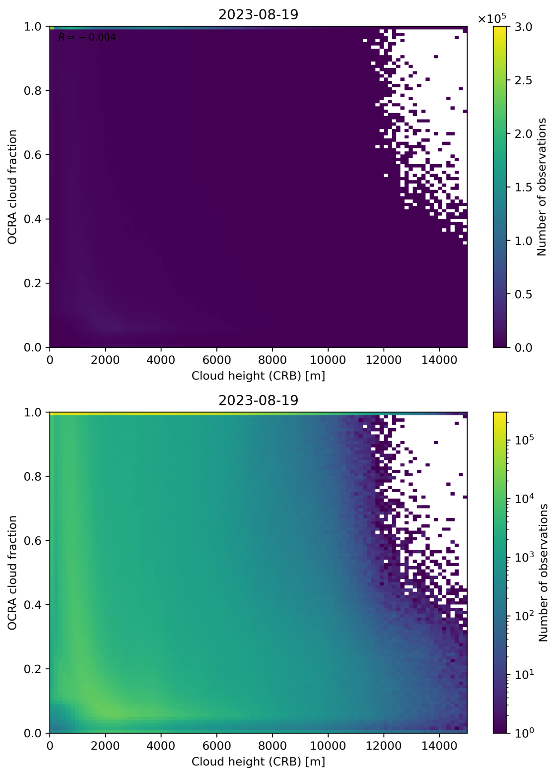
Figure 81: Scatter density plot of “Cloud height (CRB)” against “OCRA cloud fraction” for 2023-08-18 to 2023-08-20.
