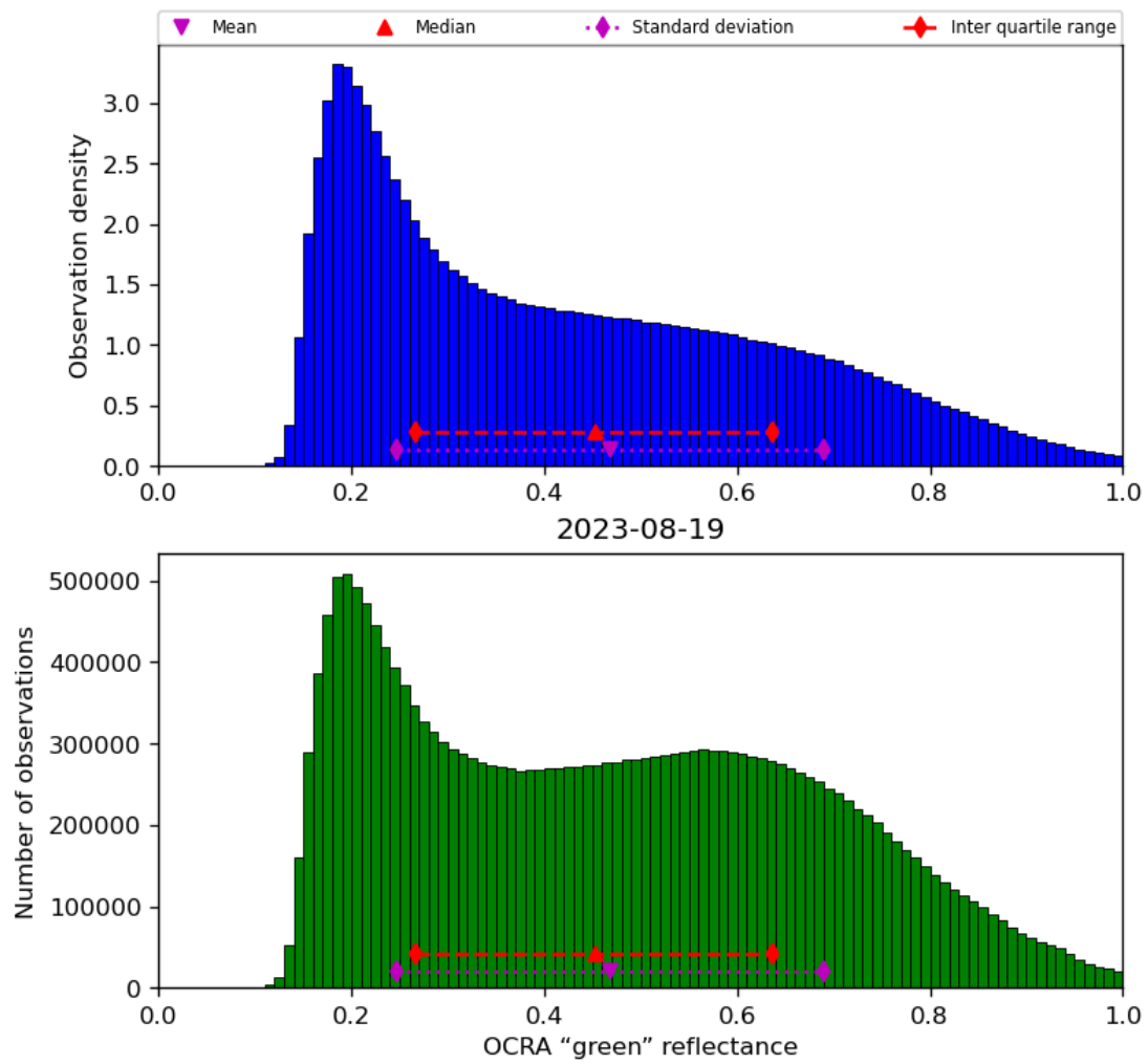
Figure 52: Histogram of “OCRA “green” reflectance” for 2023-08-18 to 2023-08-20
