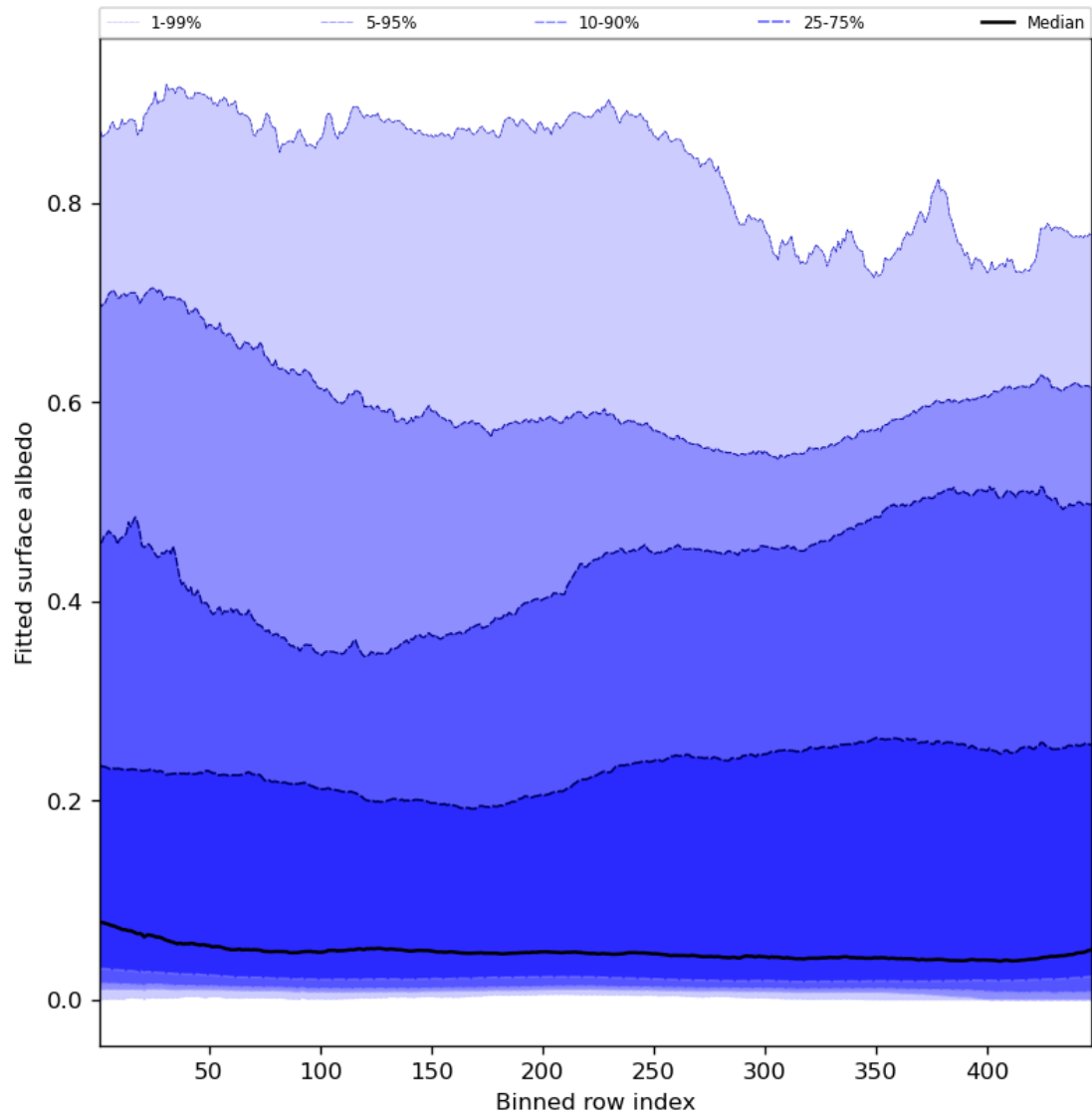
Figure 61: Along track statistics of “Fitted surface albedo” for 2023-08-18 to 2023-08-20
