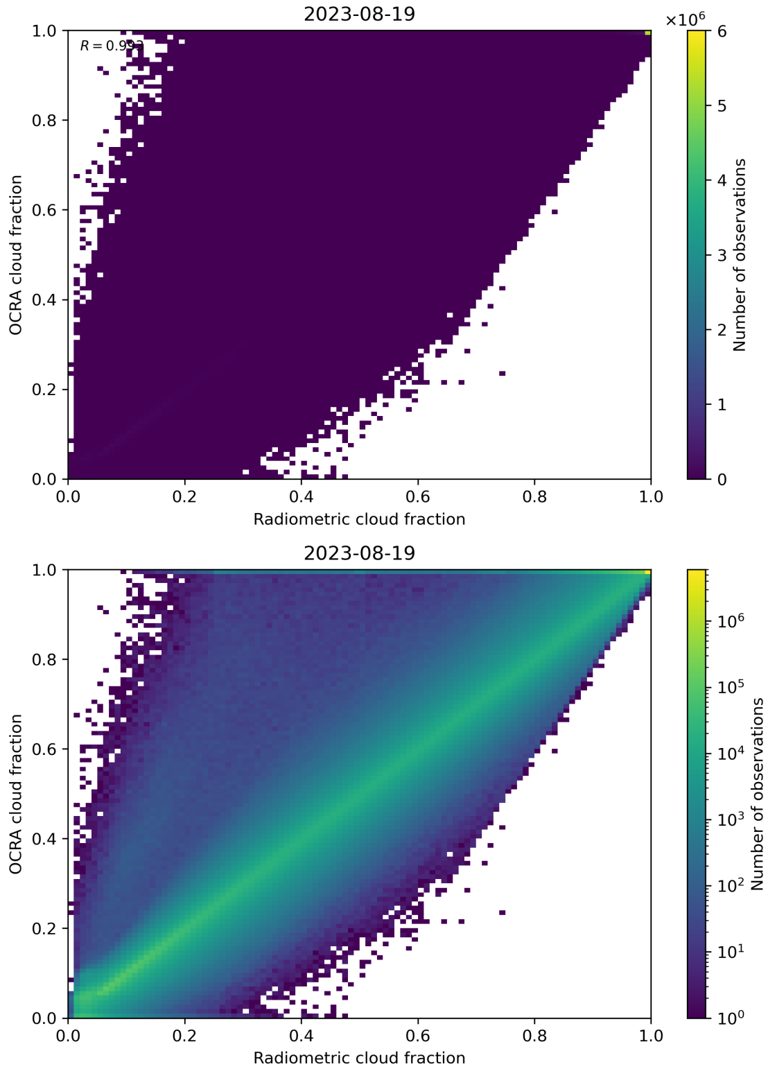
Figure 72: Scatter density plot of “Radiometric cloud fraction” against “OCRA cloud fraction” for 2023-08-18 to 2023-08-20.
