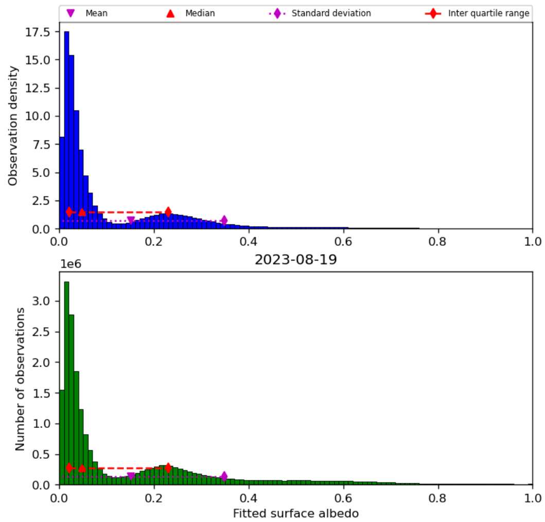
Figure 45: Histogram of “Fitted surface albedo” for 2023-08-18 to 2023-08-20
