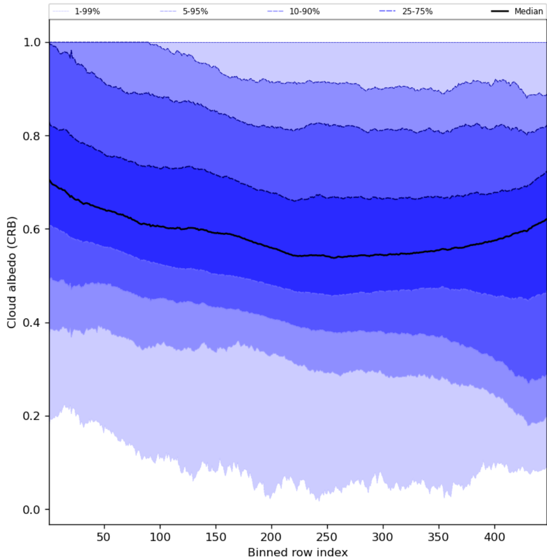
Figure 60: Along track statistics of “Cloud albedo (CRB)” for 2023-08-18 to 2023-08-20
