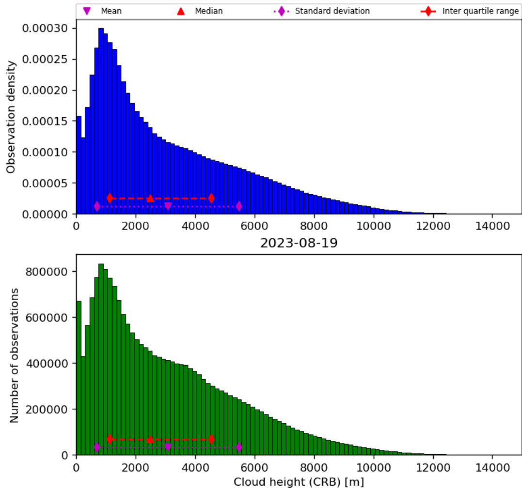
Figure 43: Histogram of “Cloud height (CRB)” for 2023-08-18 to 2023-08-20
