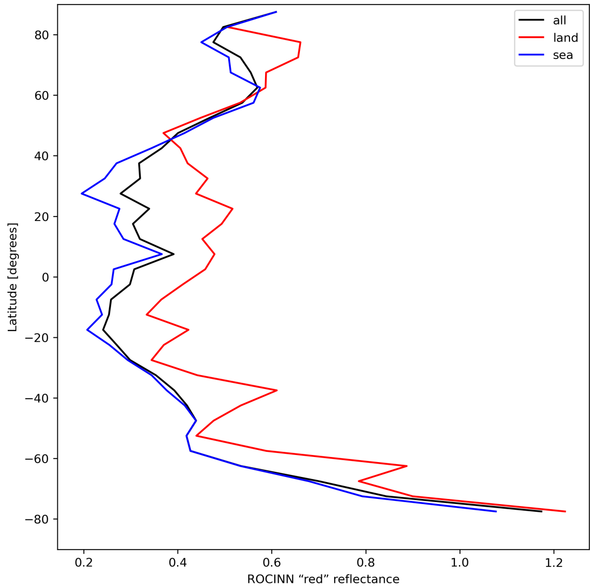
Figure 37: Zonal average of “ROCINN “red” reflectance” for 2023-08-18 to 2023-08-20.
