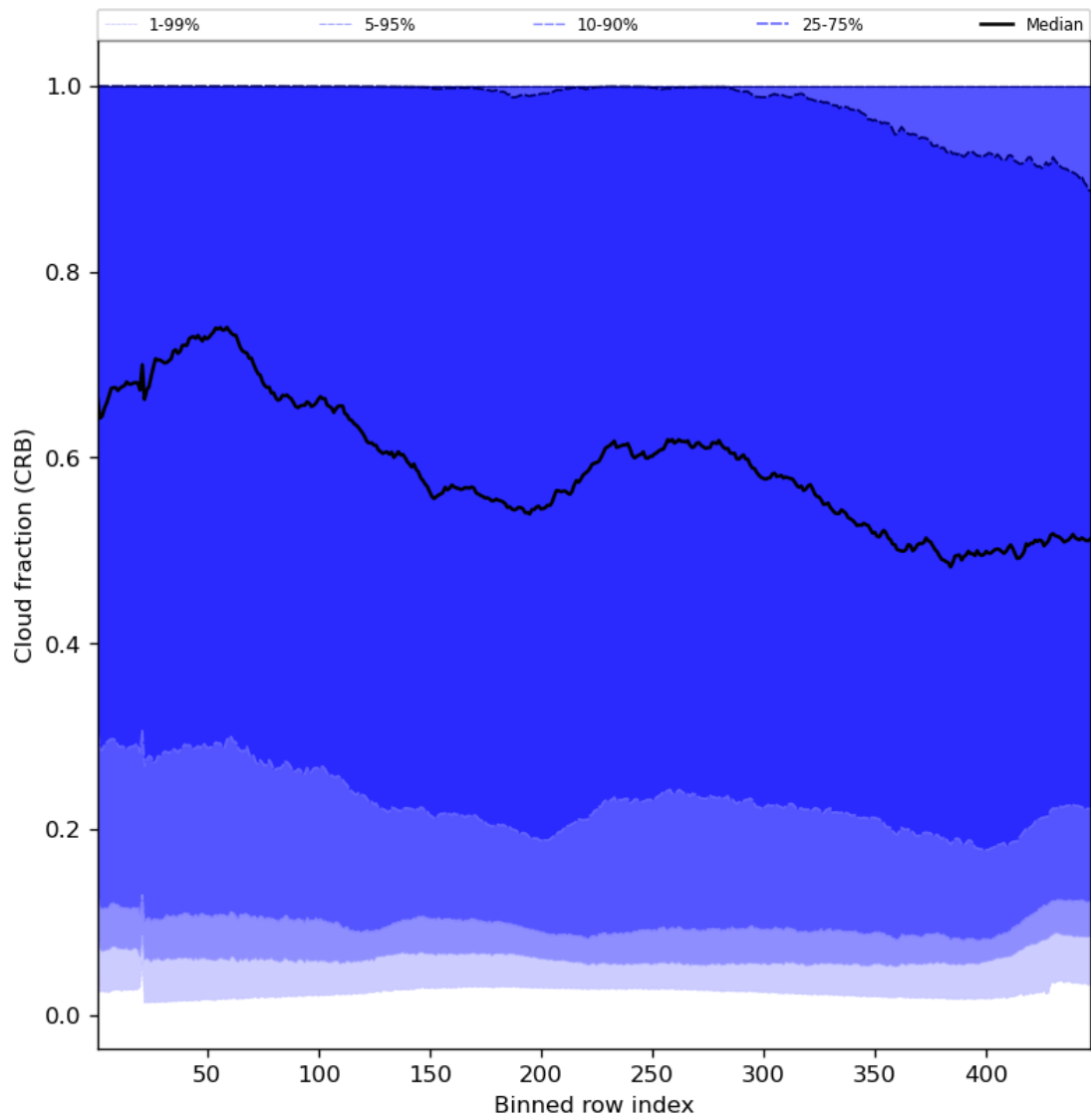
Figure 58: Along track statistics of “Cloud fraction (CRB)” for 2023-08-18 to 2023-08-20
