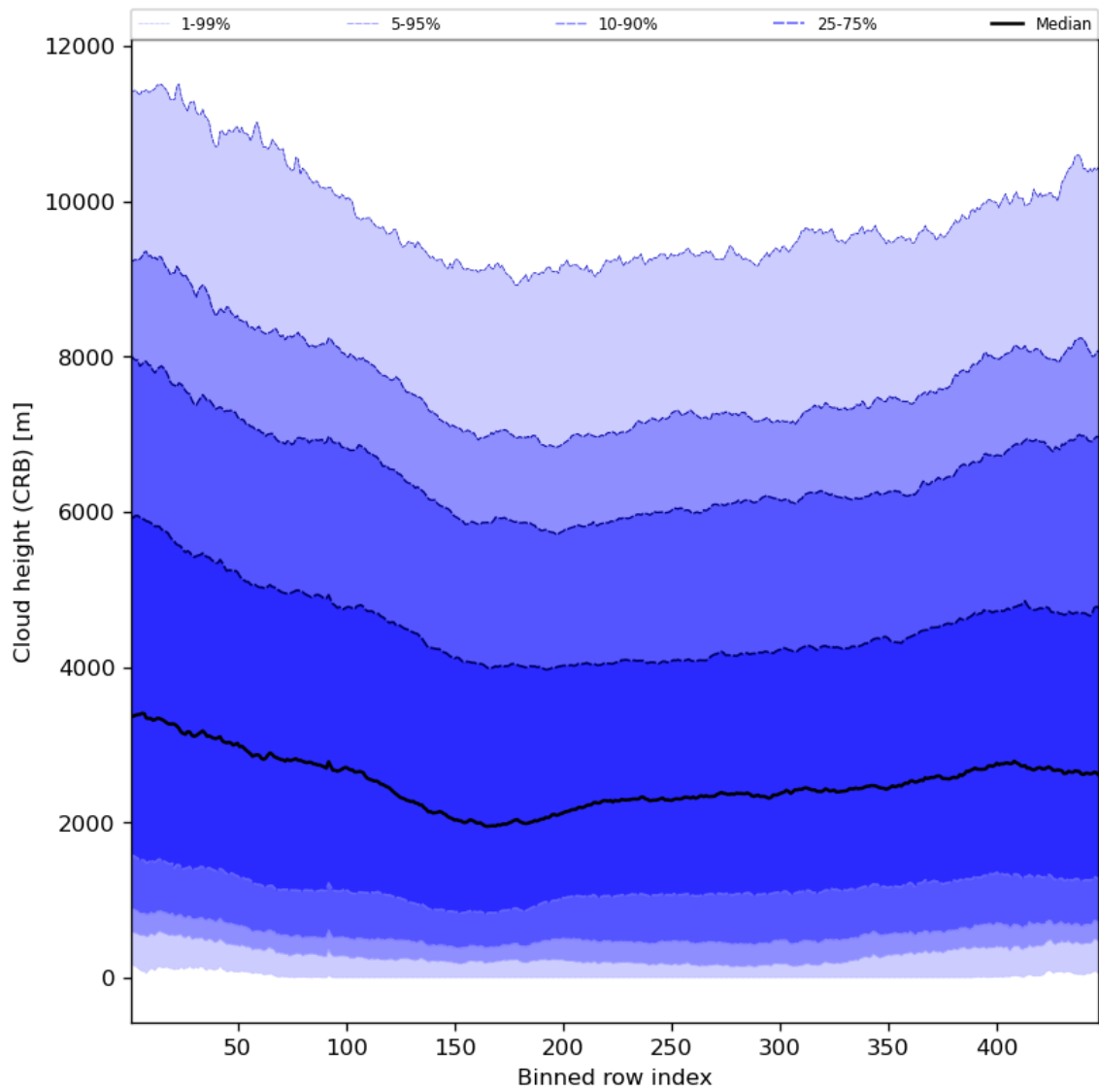
Figure 59: Along track statistics of “Cloud height (CRB)” for 2023-08-18 to 2023-08-20
