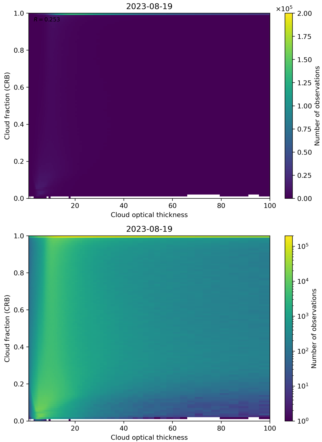
Figure 84: Scatter density plot of “Cloud optical thickness” against “Cloud fraction (CRB)” for 2023-08-18 to 2023-08-20.
