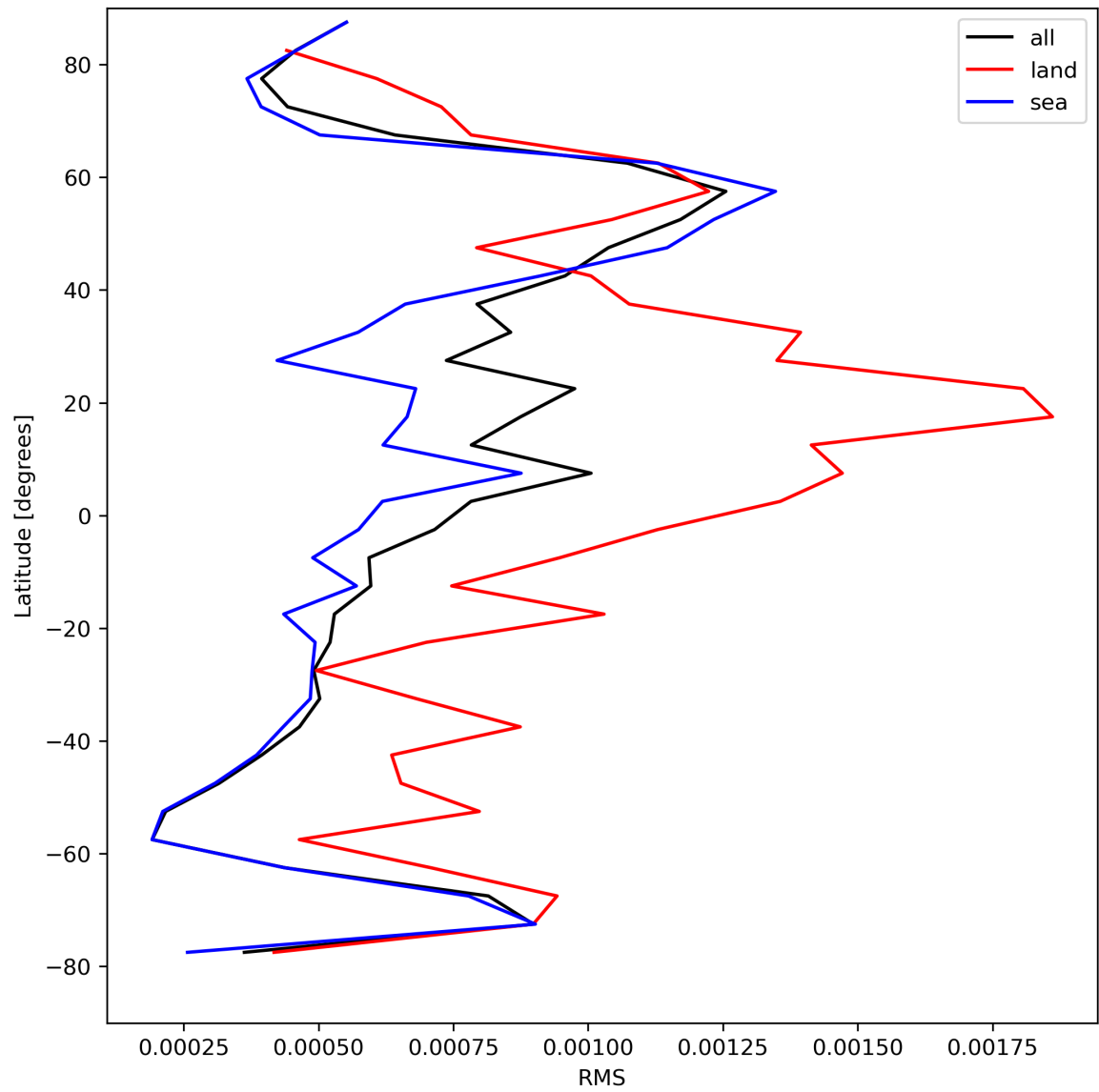
Figure 31: Zonal average of “RMS” for 2023-08-18 to 2023-08-20.
