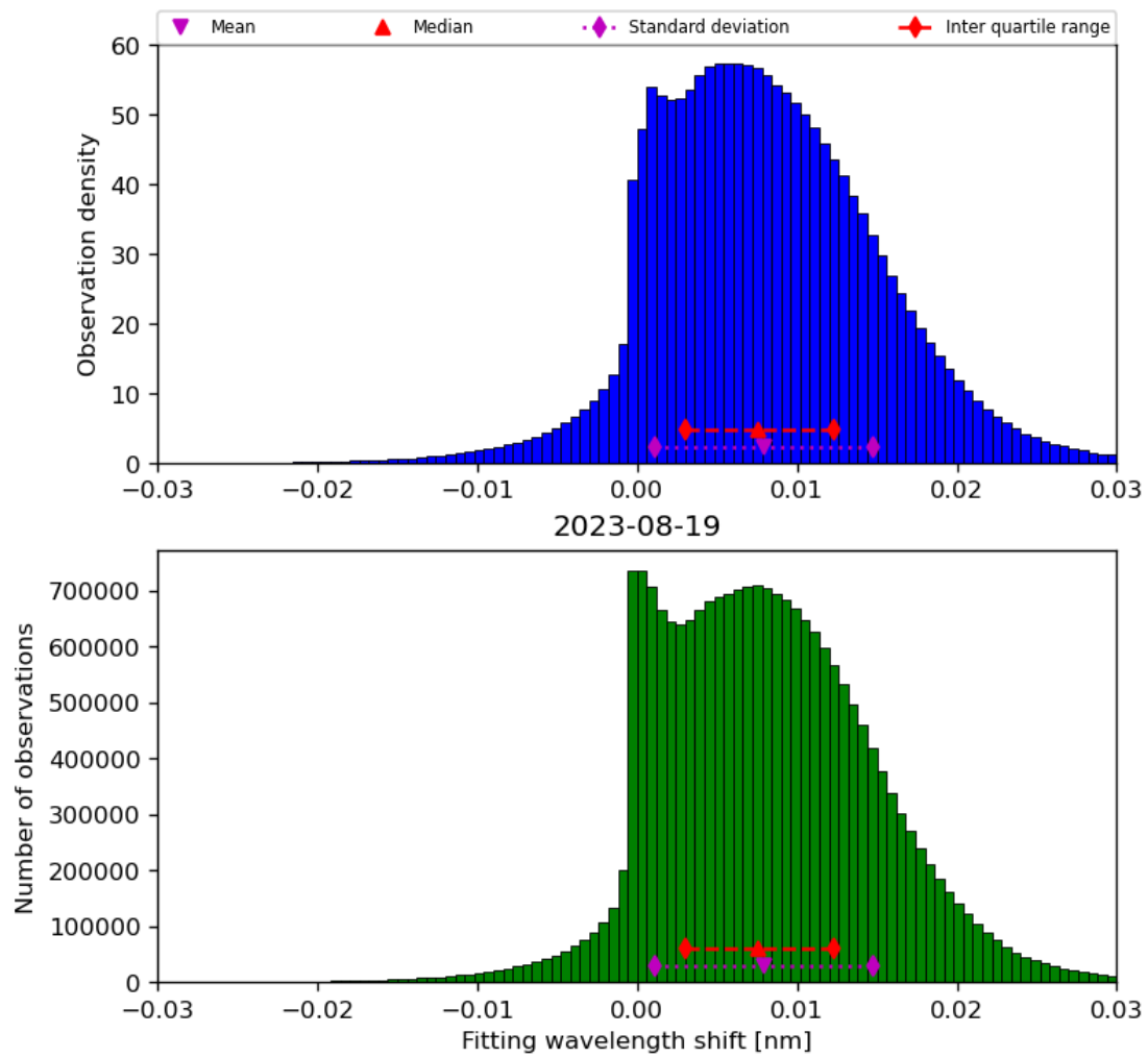
Figure 49: Histogram of “Fitting wavelength shift” for 2023-08-18 to 2023-08-20
