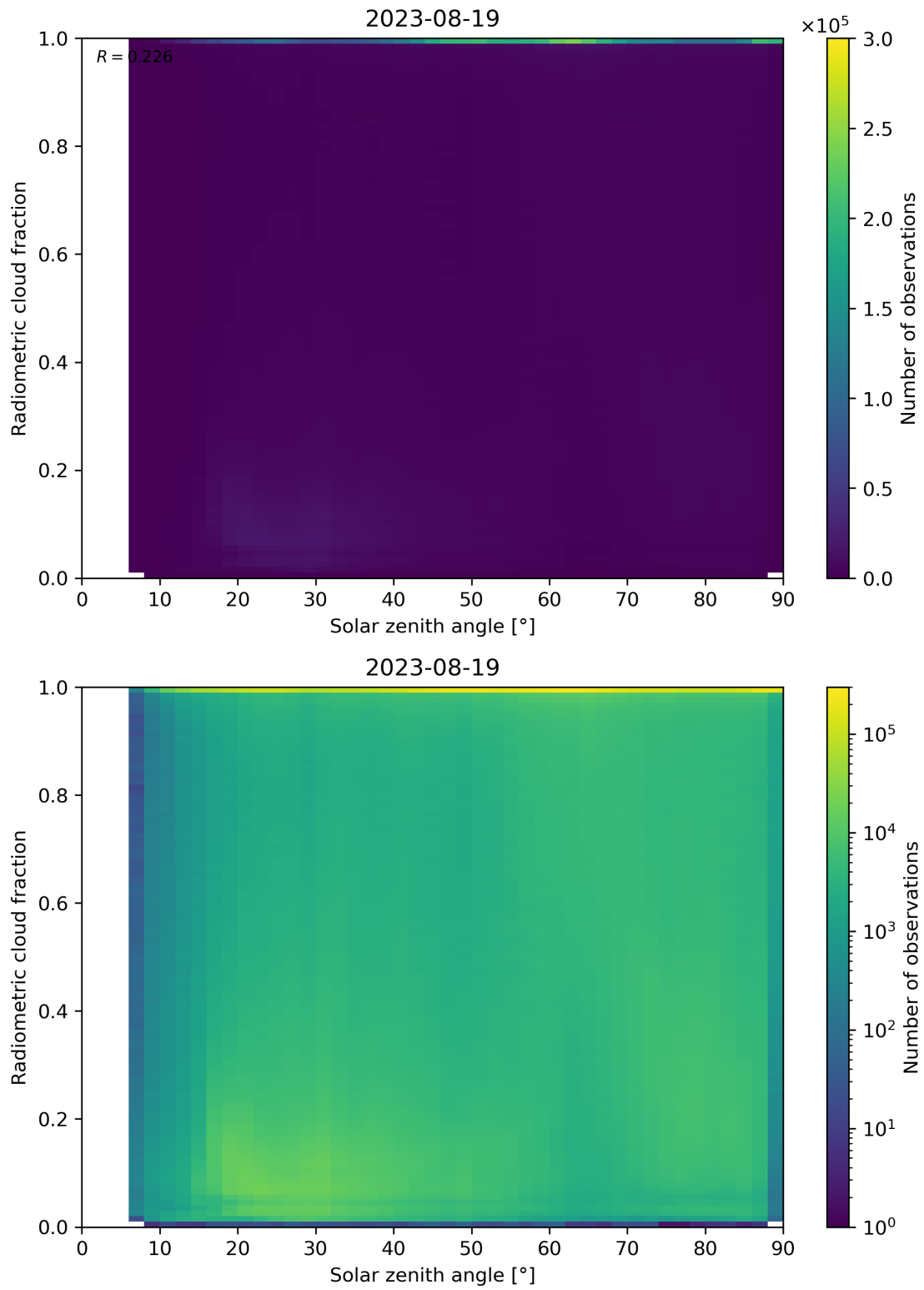
Figure 99: Scatter density plot of “Solar zenith angle” against “Radiometric cloud fraction” for 2023-08-18 to 2023-08-20.
