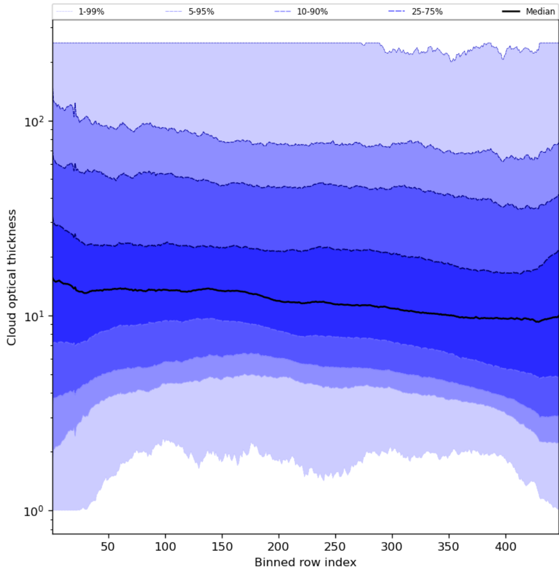
Figure 57: Along track statistics of “Cloud optical thickness” for 2023-08-18 to 2023-08-20
