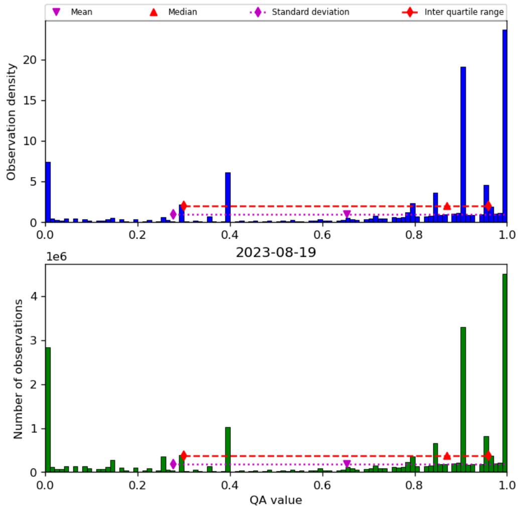
Figure 38: Histogram of “QA value” for 2023-08-18 to 2023-08-20
