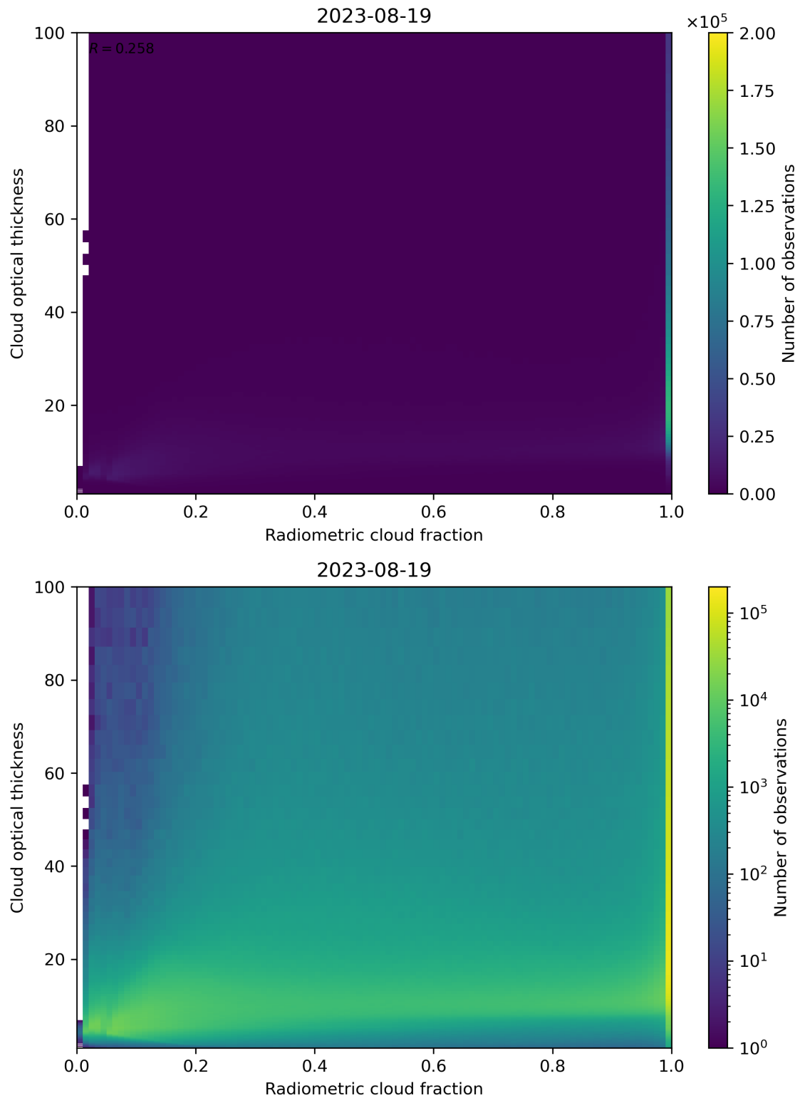
Figure 75: Scatter density plot of “Radiometric cloud fraction” against “Cloud optical thickness” for 2023-08-18 to 2023-08-20.
