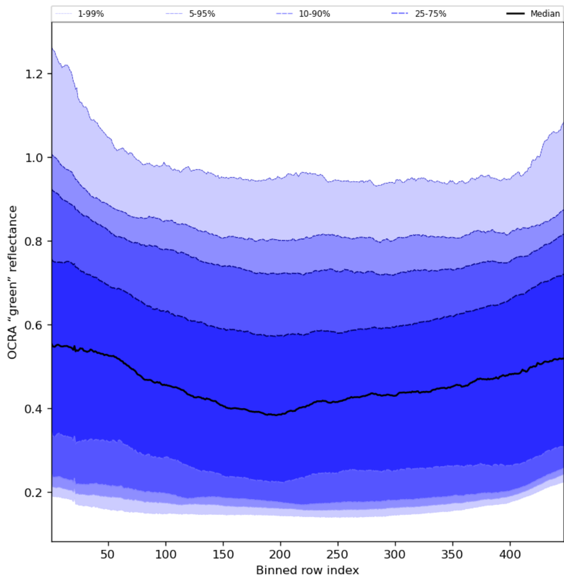
Figure 68: Along track statistics of “OCRA “green” reflectance” for 2023-08-18 to 2023-08-20
