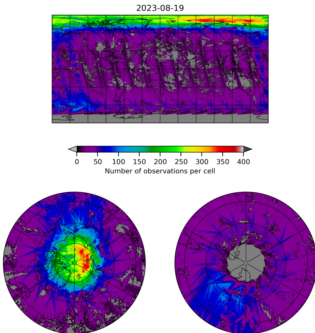
Figure 21: Map of the number of observations for 2023-08-18 to 2023-08-20
