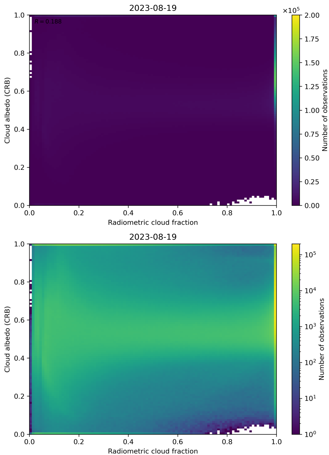
Figure 71: Scatter density plot of “Radiometric cloud fraction” against “Cloud albedo (CRB)” for 2023-08-18 to 2023-08-20.
