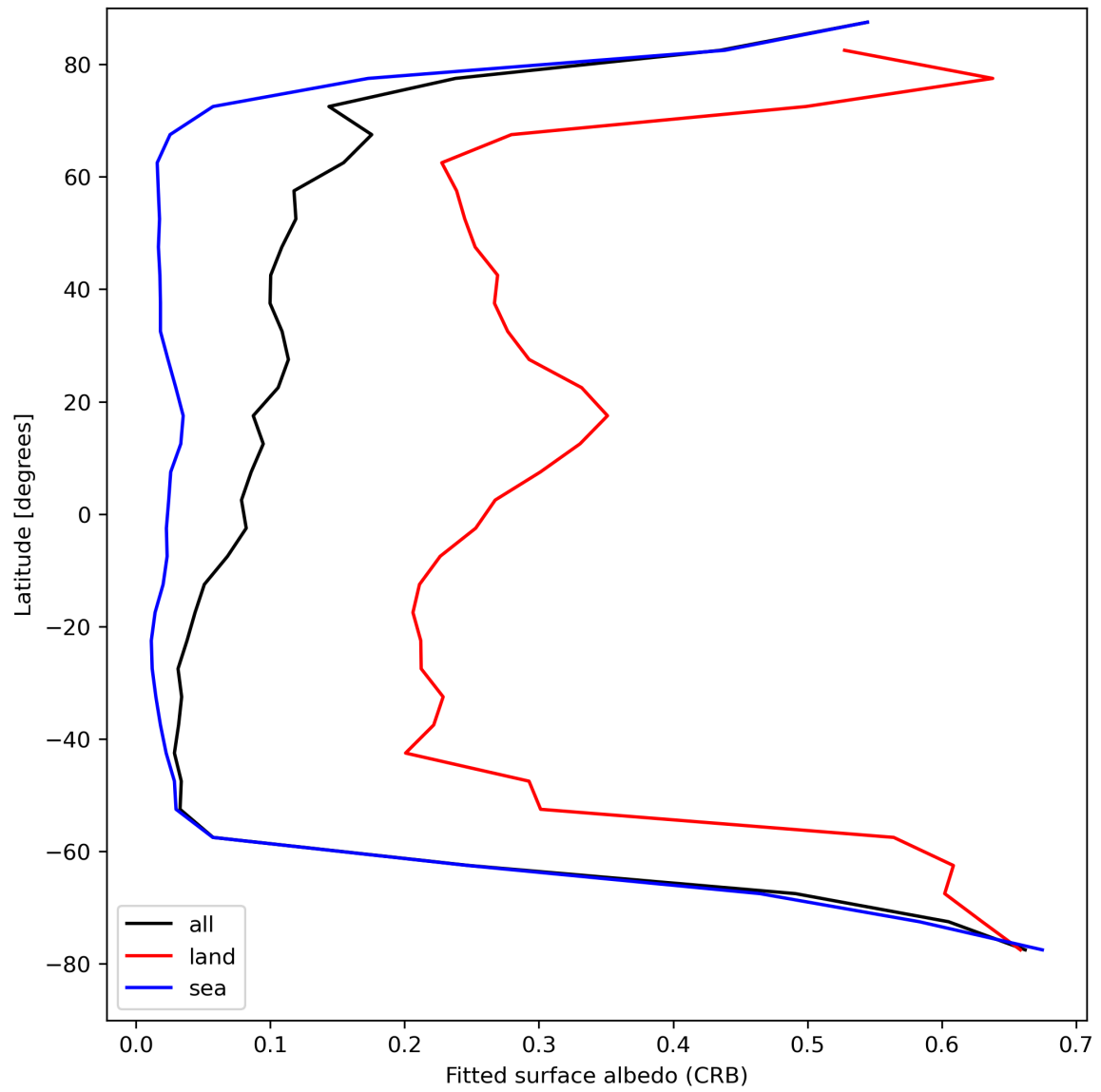
Figure 30: Zonal average of “Fitted surface albedo (CRB)” for 2023-08-18 to 2023-08-20.
