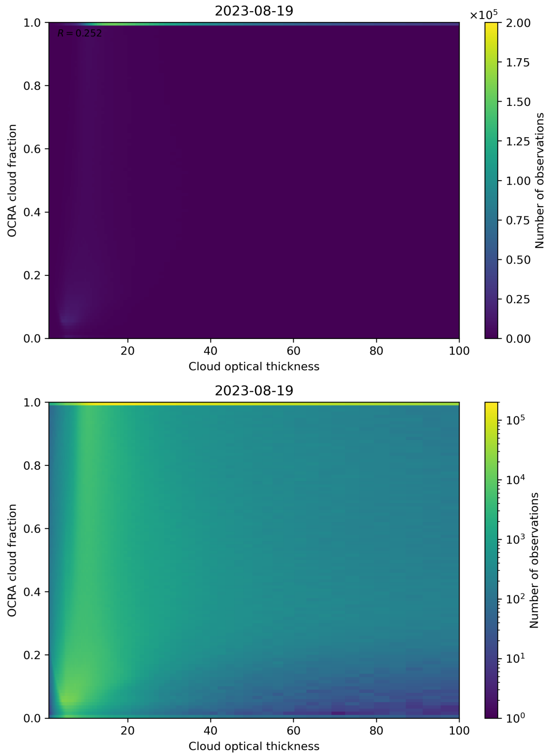
Figure 83: Scatter density plot of “Cloud optical thickness” against “OCRA cloud fraction” for 2023-08-18 to 2023-08-20.
