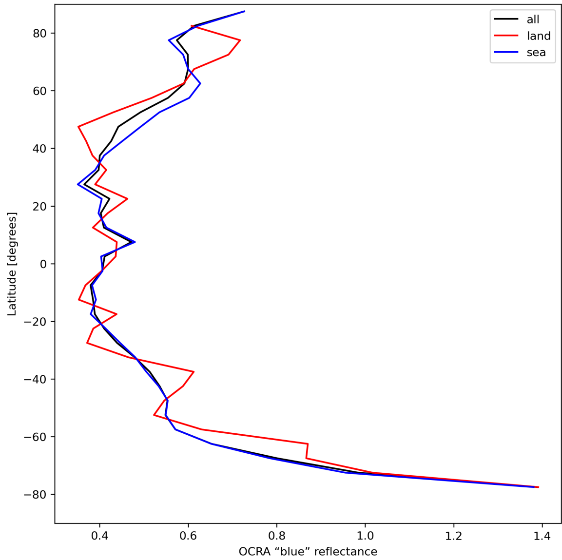
Figure 35: Zonal average of “OCRA “blue” reflectance” for 2023-08-18 to 2023-08-20.
