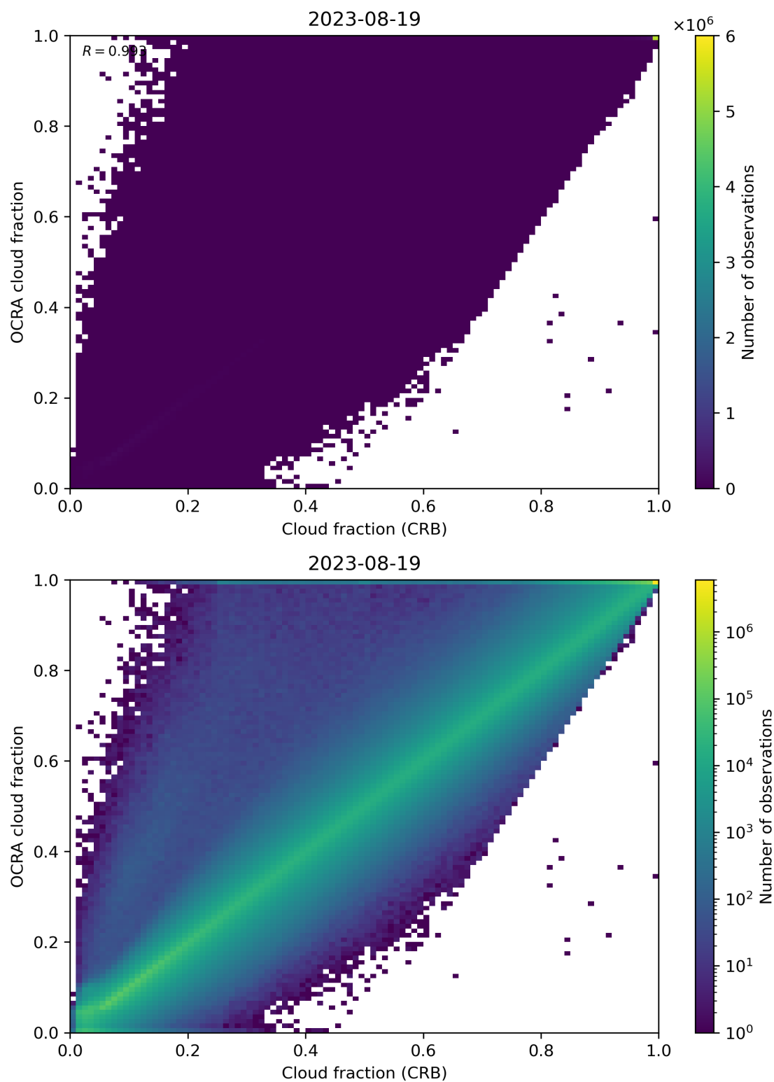
Figure 78: Scatter density plot of “Cloud fraction (CRB)” against “OCRA cloud fraction” for 2023-08-18 to 2023-08-20.
