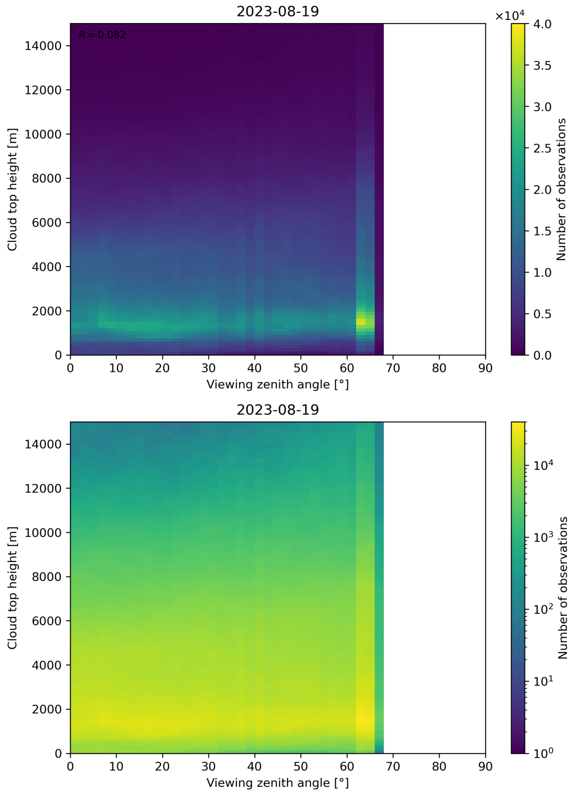
Figure 112: Scatter density plot of “Viewing zenith angle” against “Cloud top height” for 2023-08-18 to 2023-08-20.
