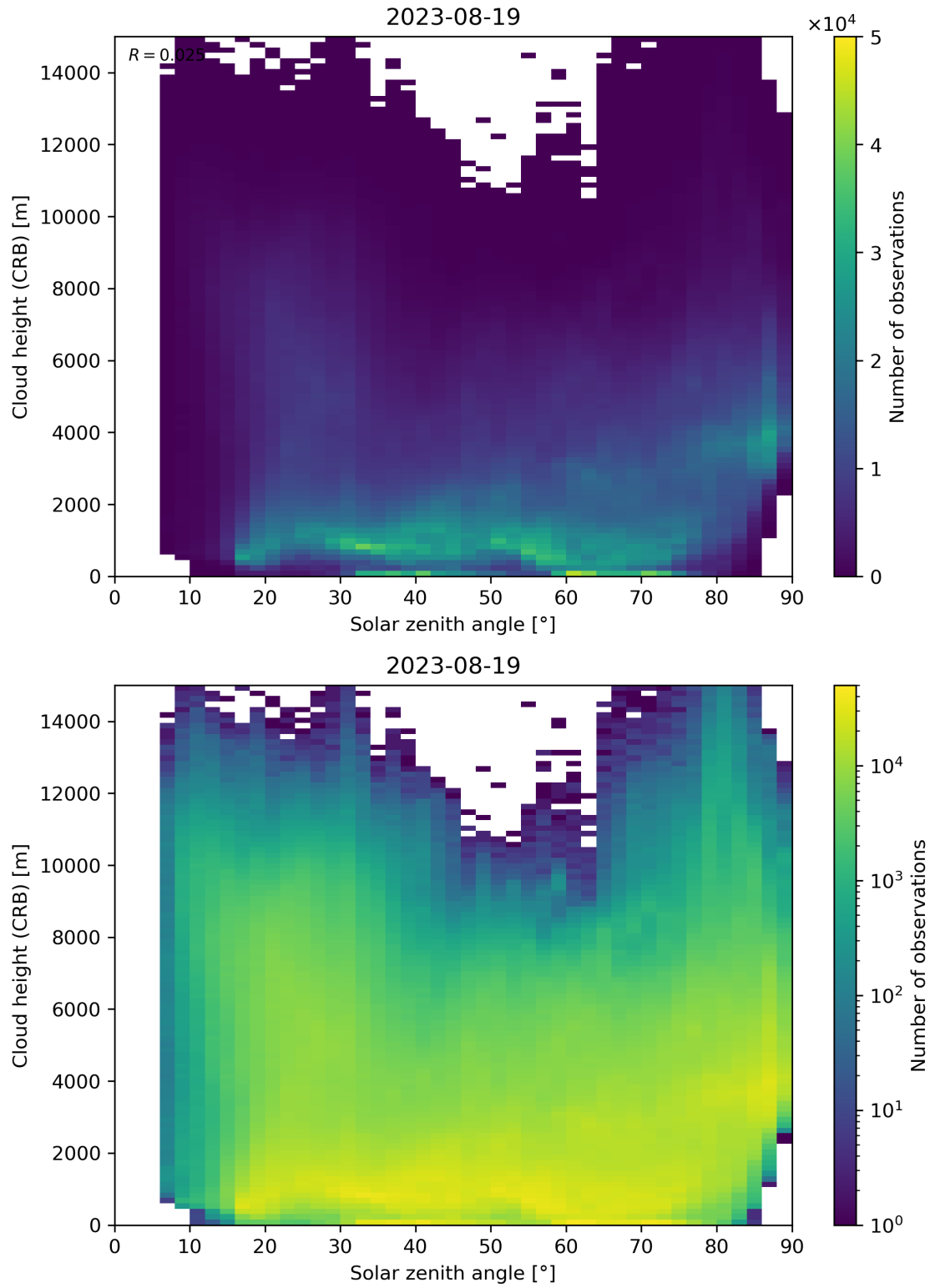
Figure 102: Scatter density plot of “Solar zenith angle” against “Cloud height (CRB)” for 2023-08-18 to 2023-08-20.
