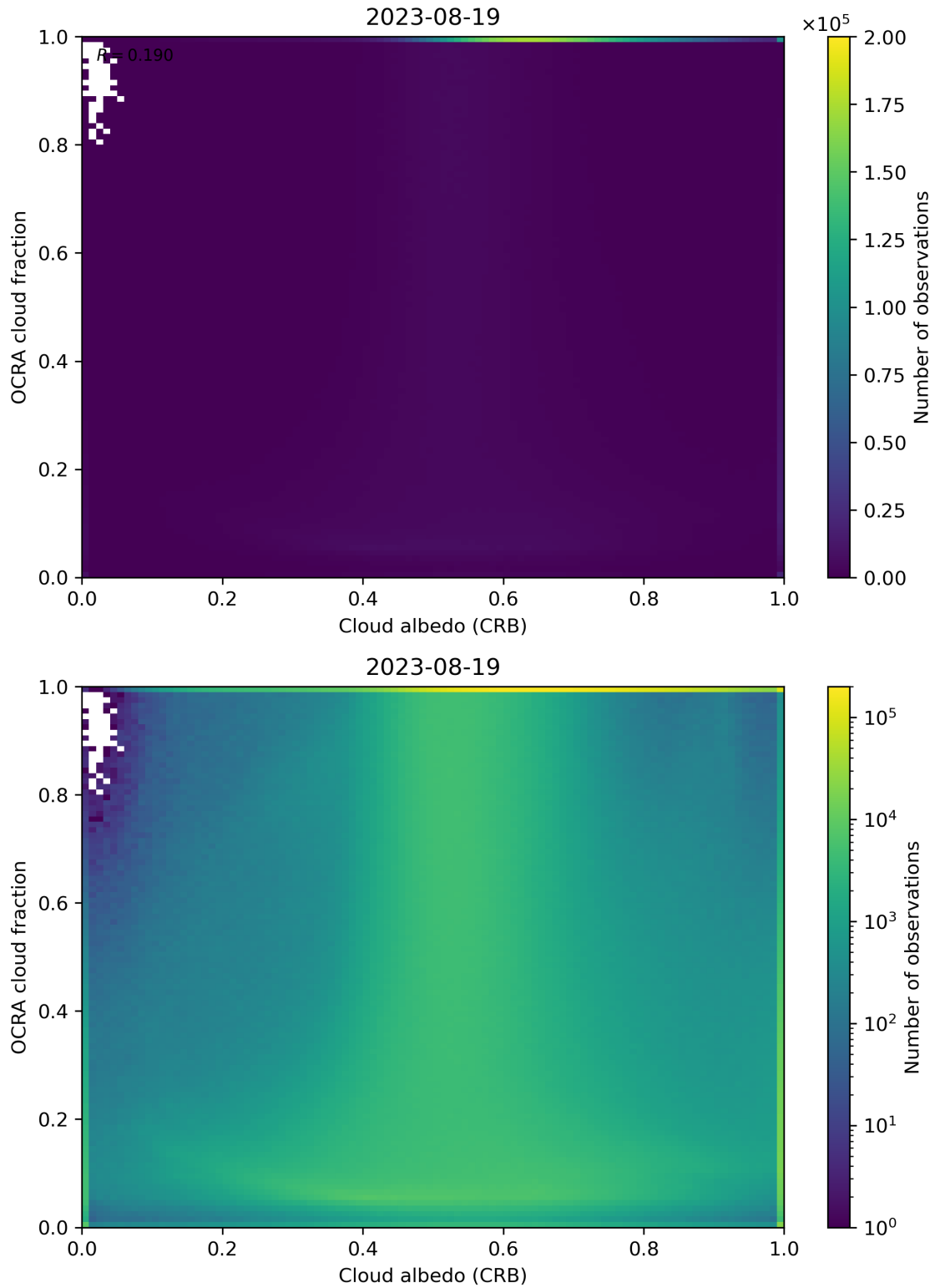
Figure 70: Scatter density plot of “Cloud albedo (CRB)” against “OCRA cloud fraction” for 2023-08-18 to 2023-08-20.
