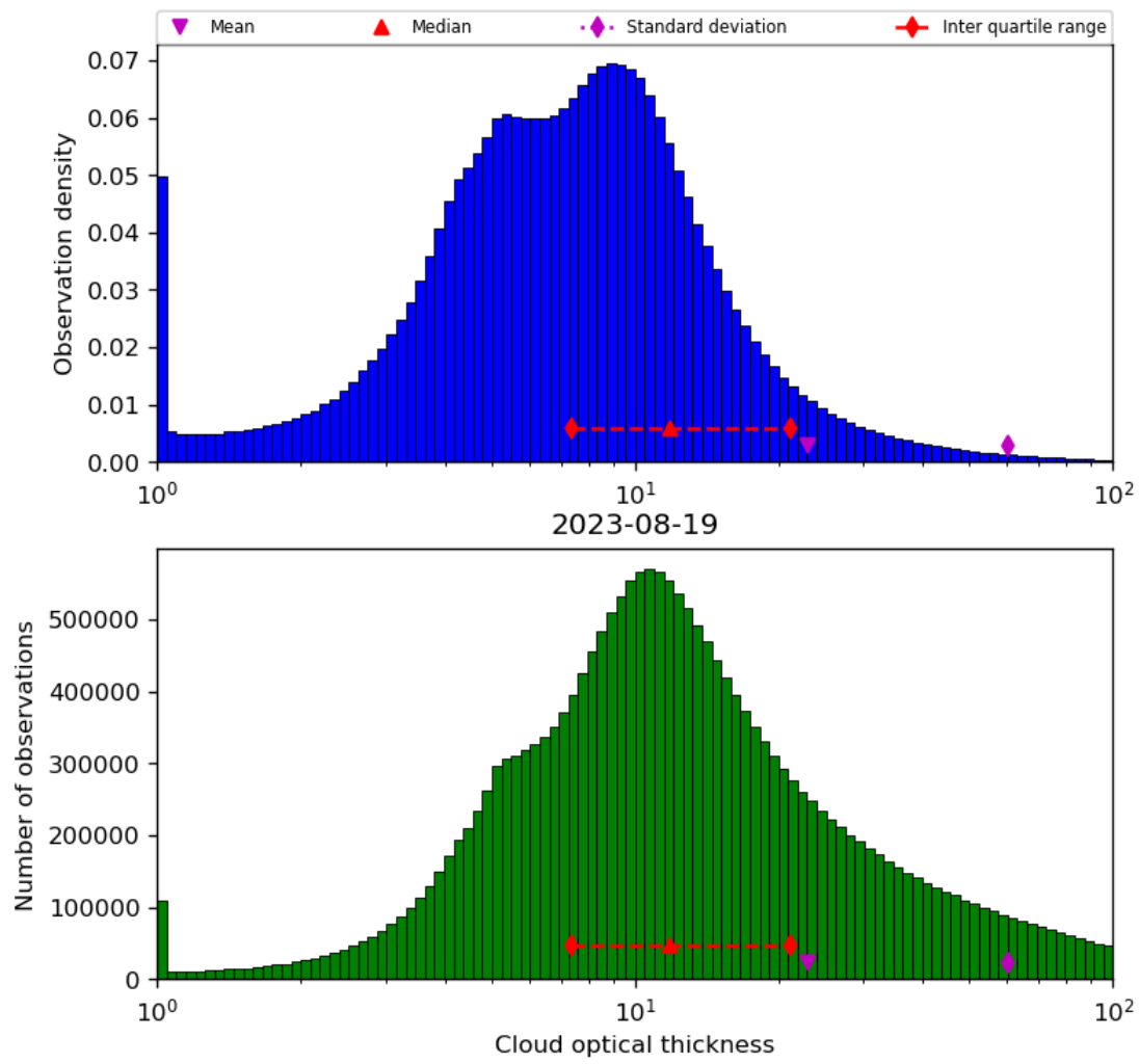
Figure 41: Histogram of “Cloud optical thickness” for 2023-08-18 to 2023-08-20
