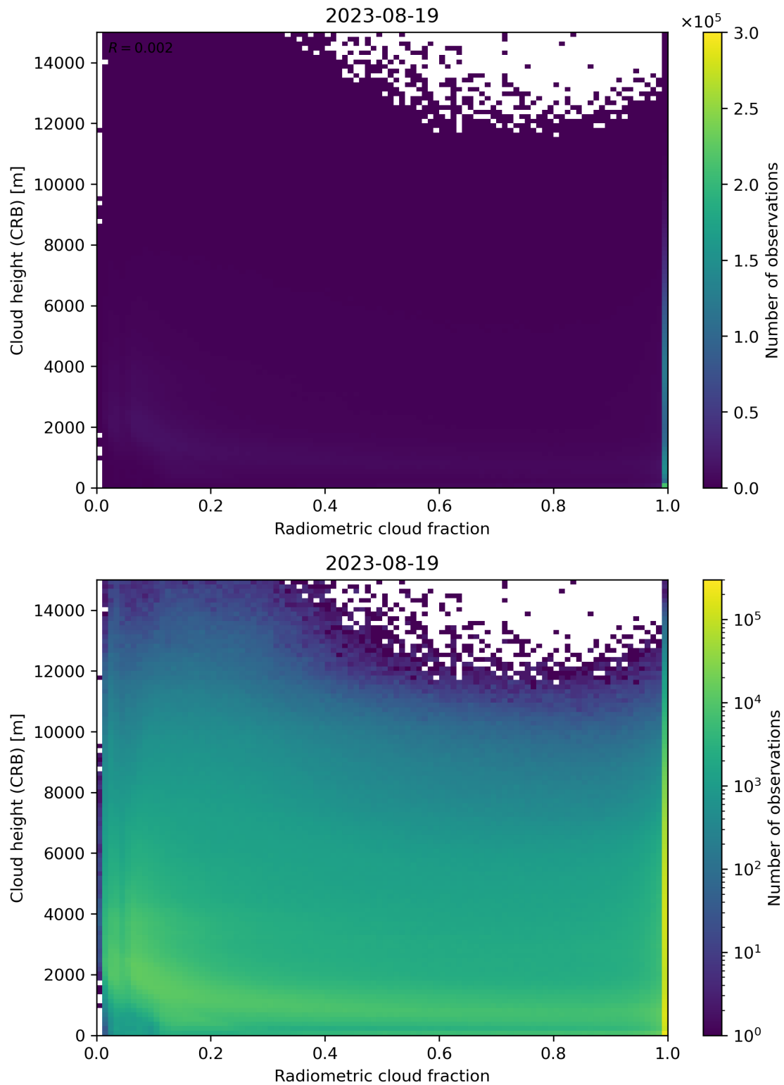
Figure 74: Scatter density plot of “Radiometric cloud fraction” against “Cloud height (CRB)” for 2023-08-18 to 2023-08-20.
