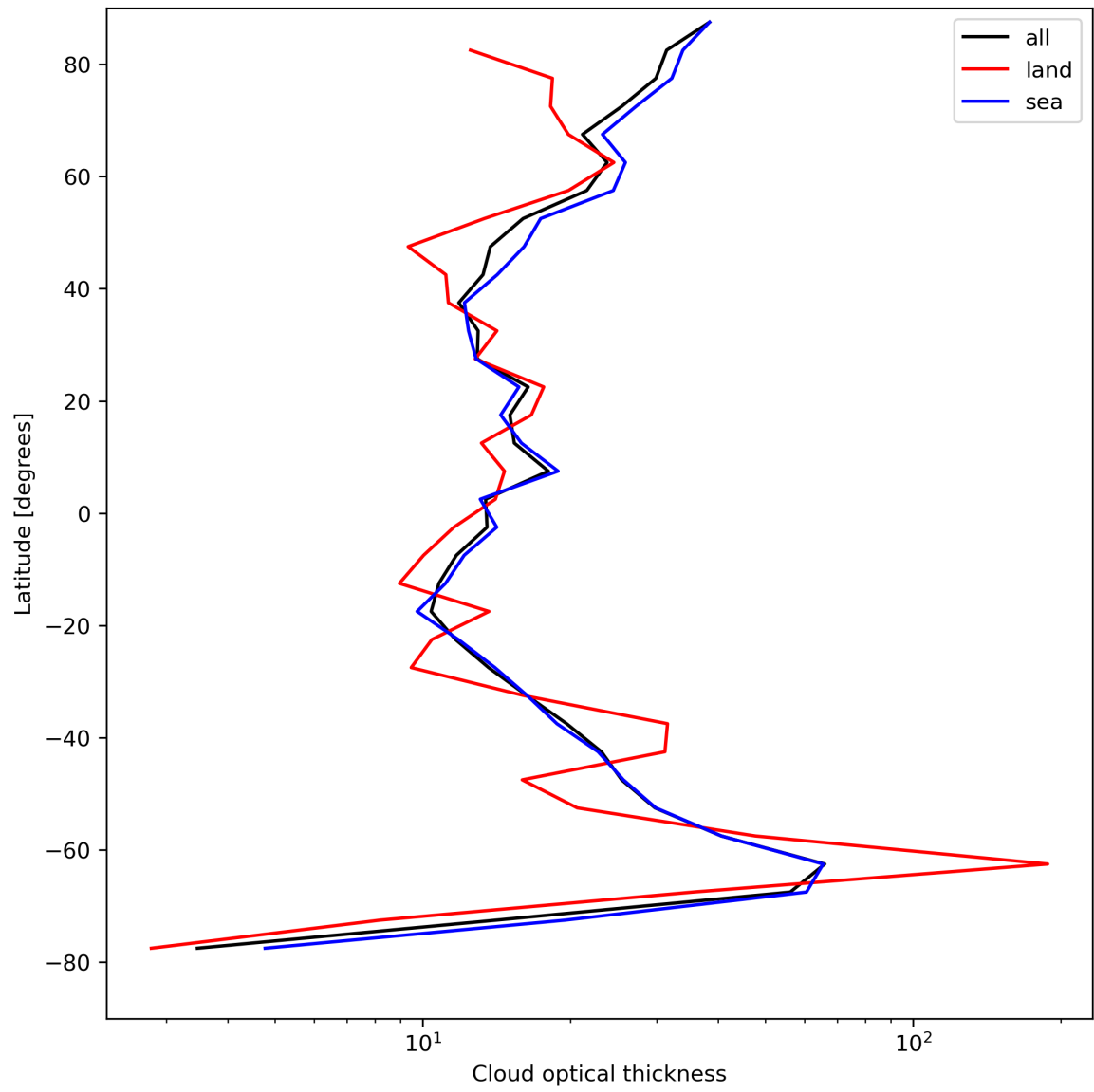
Figure 25: Zonal average of “Cloud optical thickness” for 2023-08-18 to 2023-08-20.
