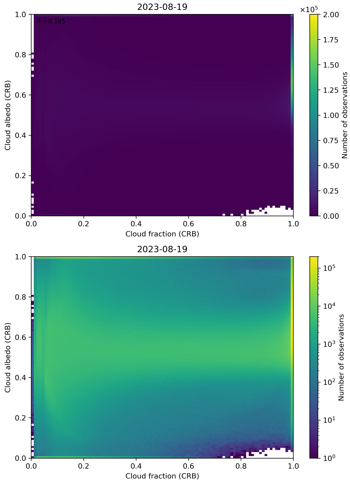
Figure 77: Scatter density plot of “Cloud fraction (CRB)” against “Cloud albedo (CRB)” for 2023-08-18 to 2023-08-20.
