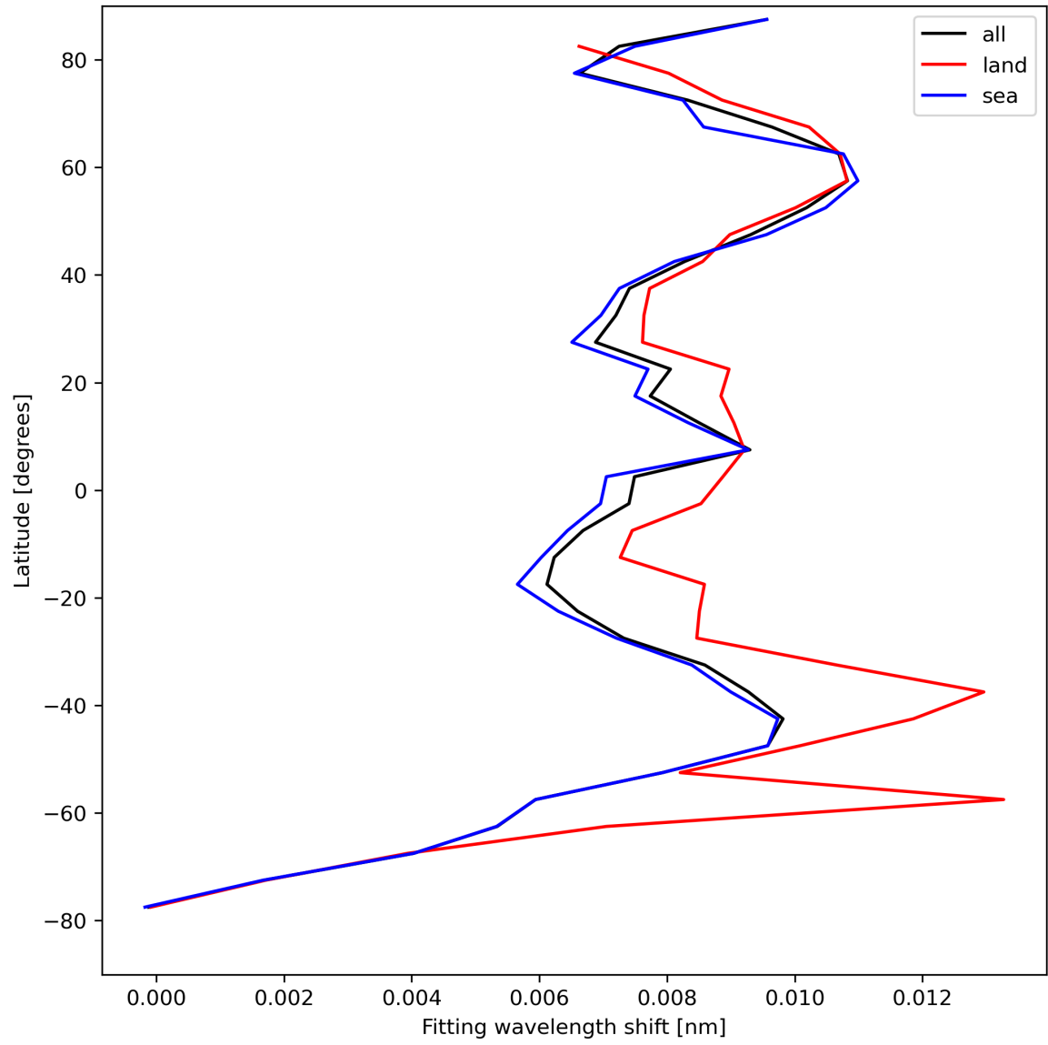
Figure 33: Zonal average of “Fitting wavelength shift” for 2023-08-18 to 2023-08-20.
