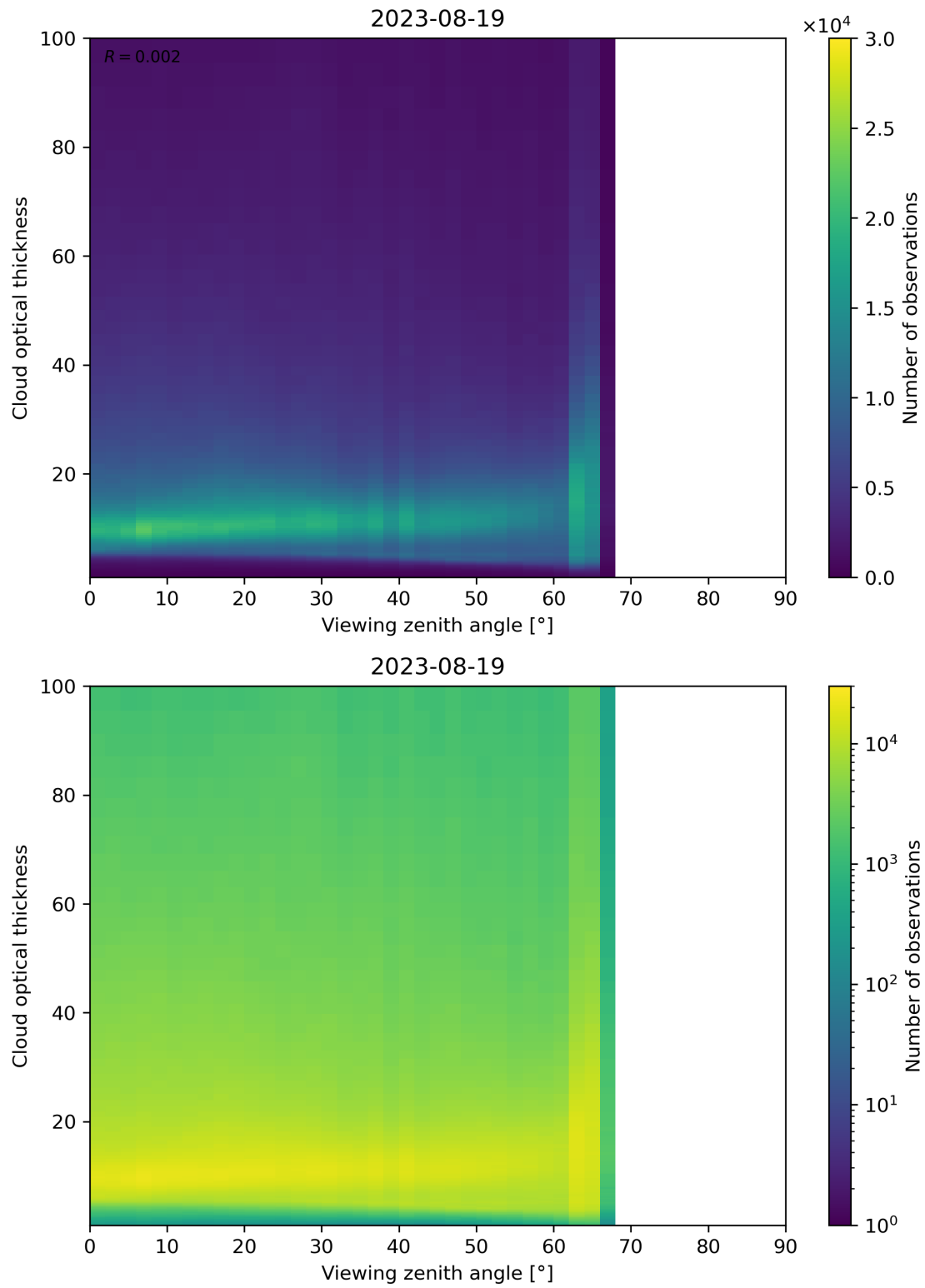
Figure 111: Scatter density plot of “Viewing zenith angle” against “Cloud optical thickness” for 2023-08-18 to 2023-08-20.
