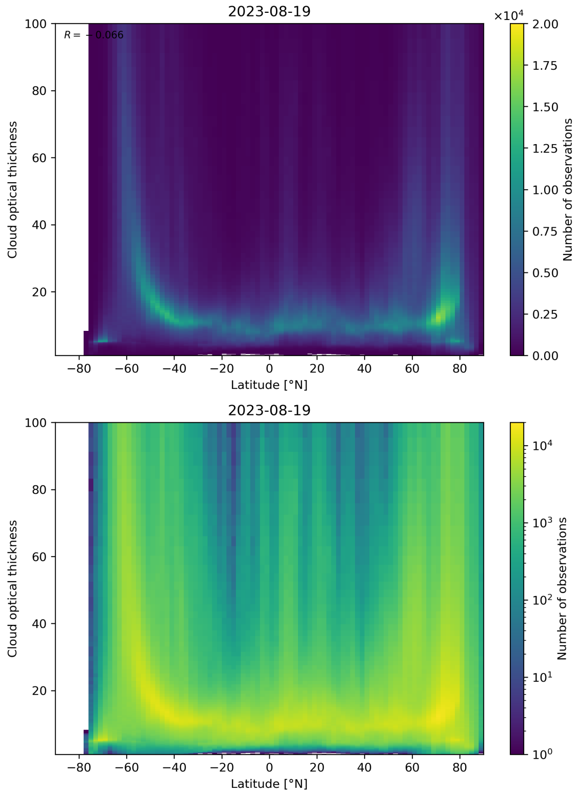
Figure 96: Scatter density plot of “Latitude” against “Cloud optical thickness” for 2023-08-18 to 2023-08-20.
