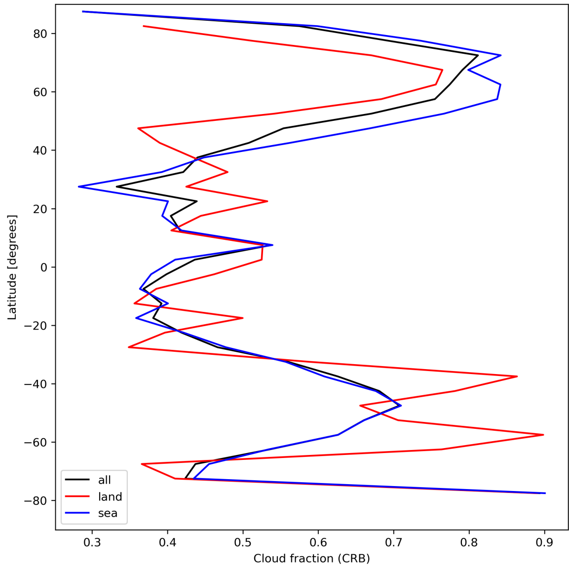
Figure 26: Zonal average of “Cloud fraction (CRB)” for 2023-08-18 to 2023-08-20.
