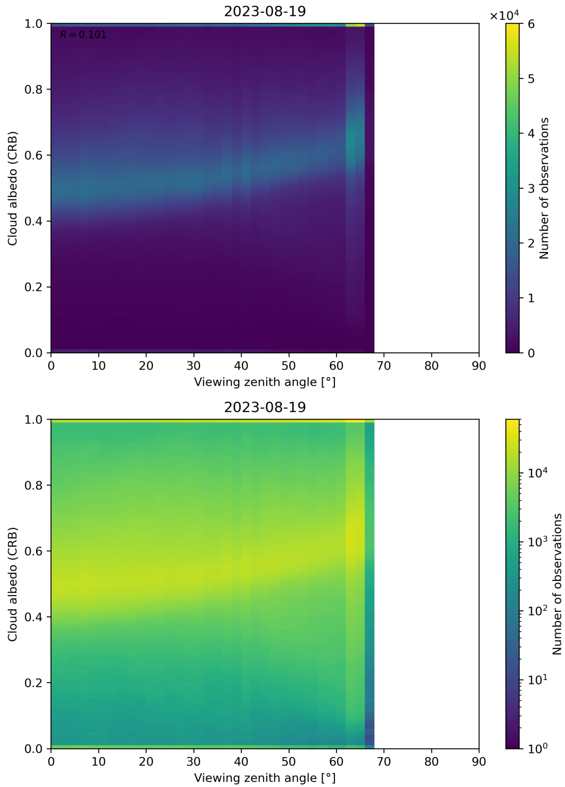
Figure 106: Scatter density plot of “Viewing zenith angle” against “Cloud albedo (CRB)” for 2023-08-18 to 2023-08-20.
