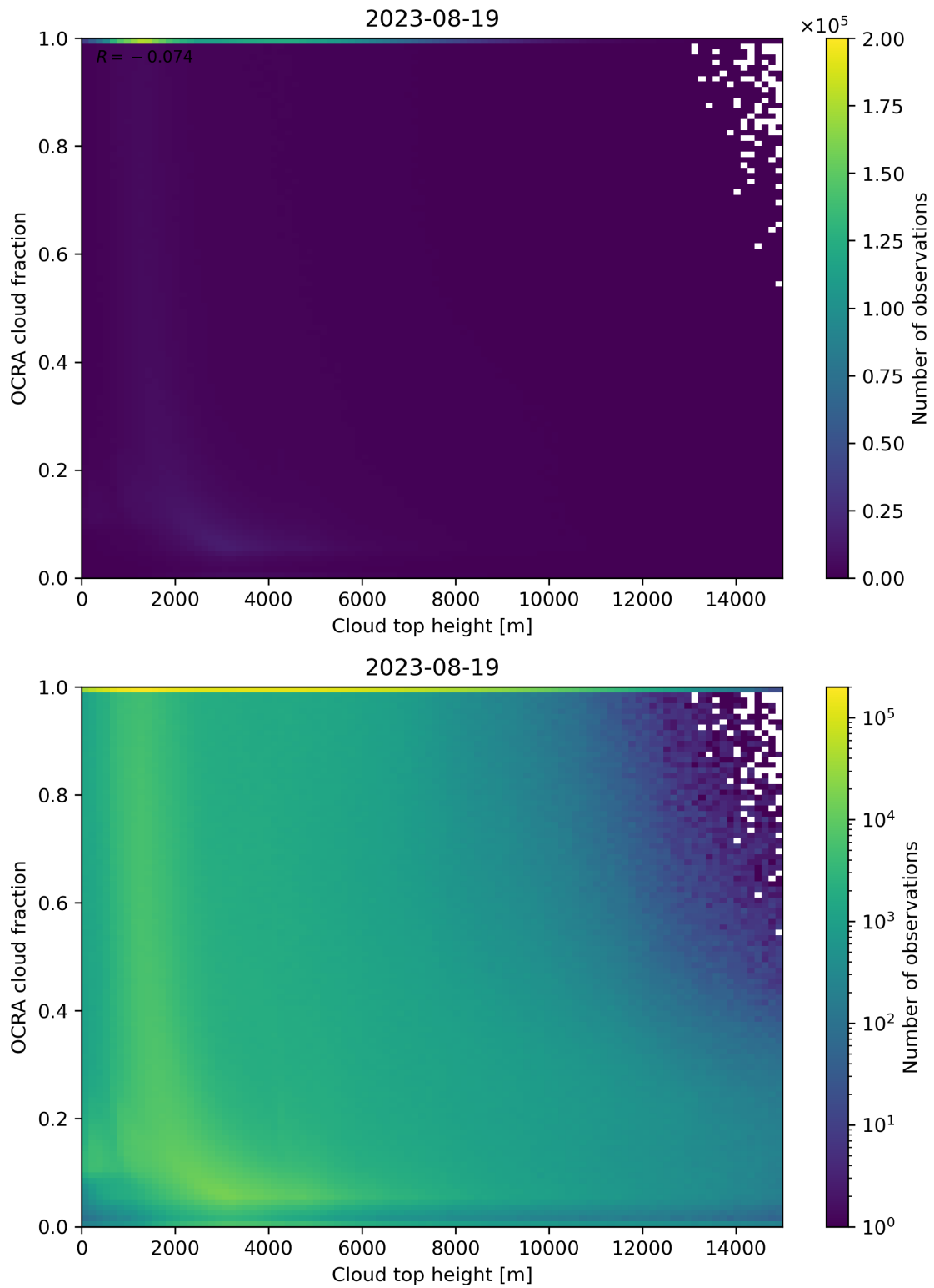
Figure 87: Scatter density plot of “Cloud top height” against “OCRA cloud fraction” for 2023-08-18 to 2023-08-20.
