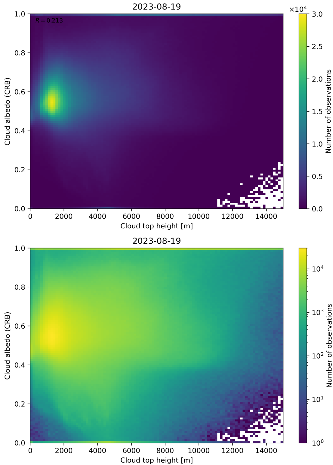
Figure 86: Scatter density plot of “Cloud top height” against “Cloud albedo (CRB)” for 2023-08-18 to 2023-08-20.
