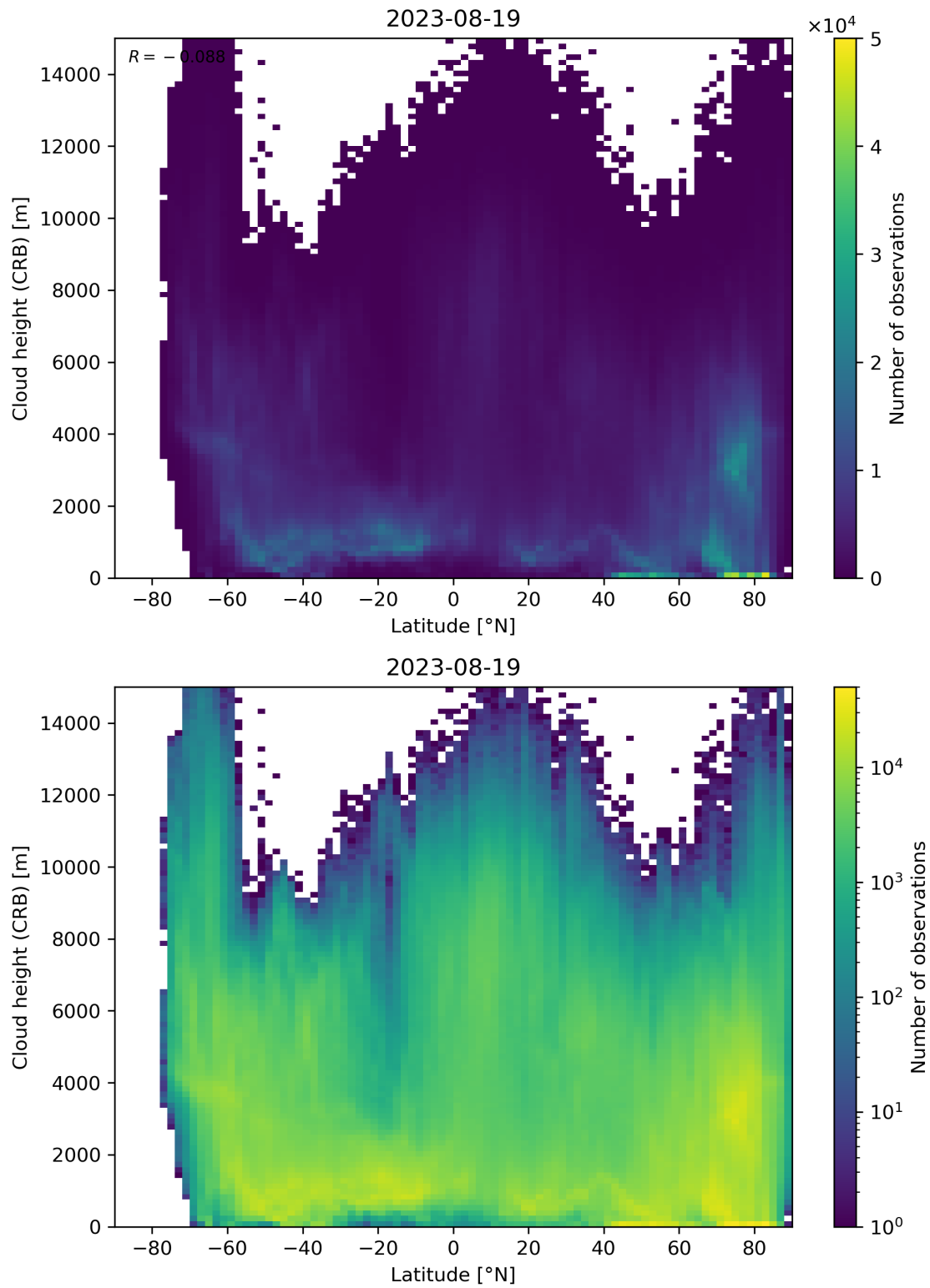
Figure 95: Scatter density plot of “Latitude” against “Cloud height (CRB)” for 2023-08-18 to 2023-08-20.
