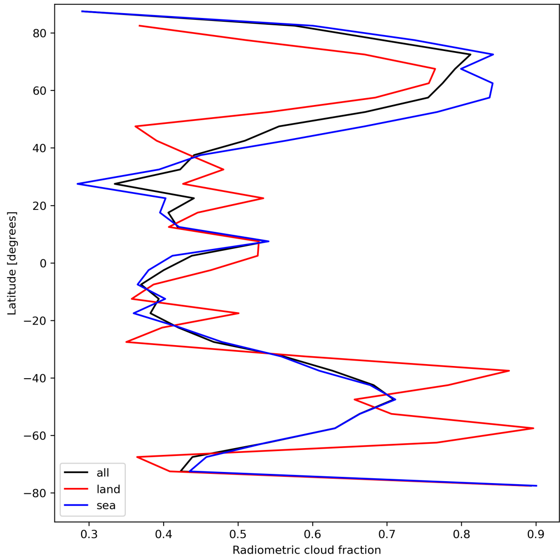
Figure 23: Zonal average of “Radiometric cloud fraction” for 2023-08-18 to 2023-08-20.
