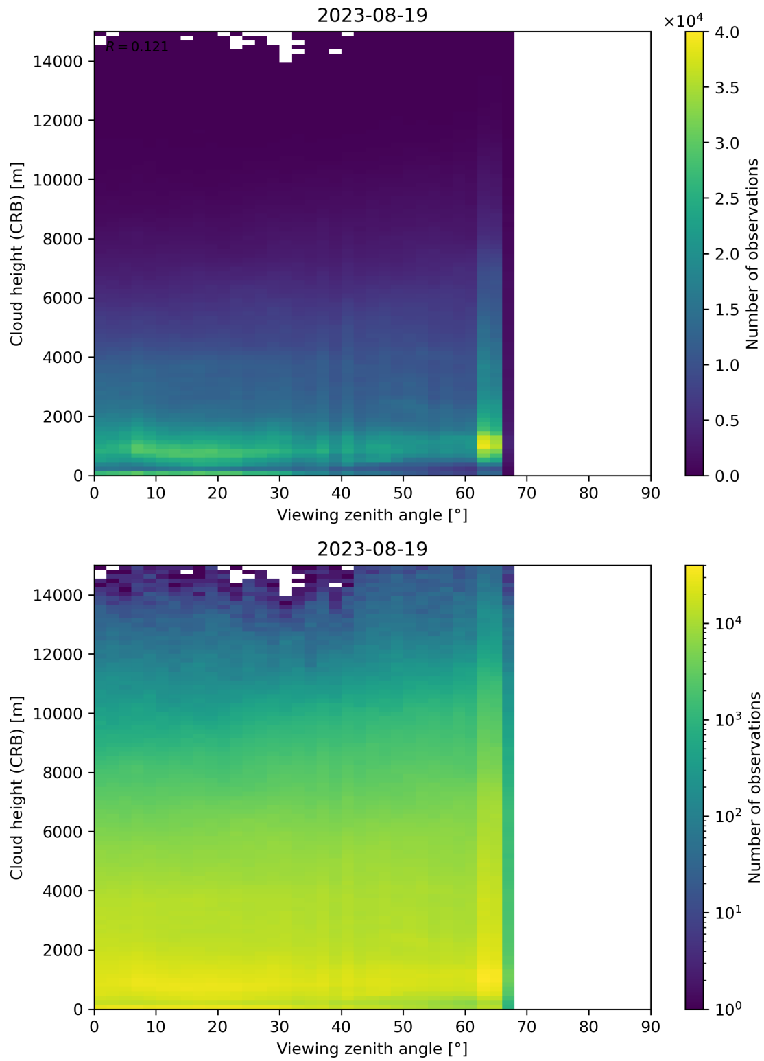
Figure 110: Scatter density plot of “Viewing zenith angle” against “Cloud height (CRB)” for 2023-08-18 to 2023-08-20.
