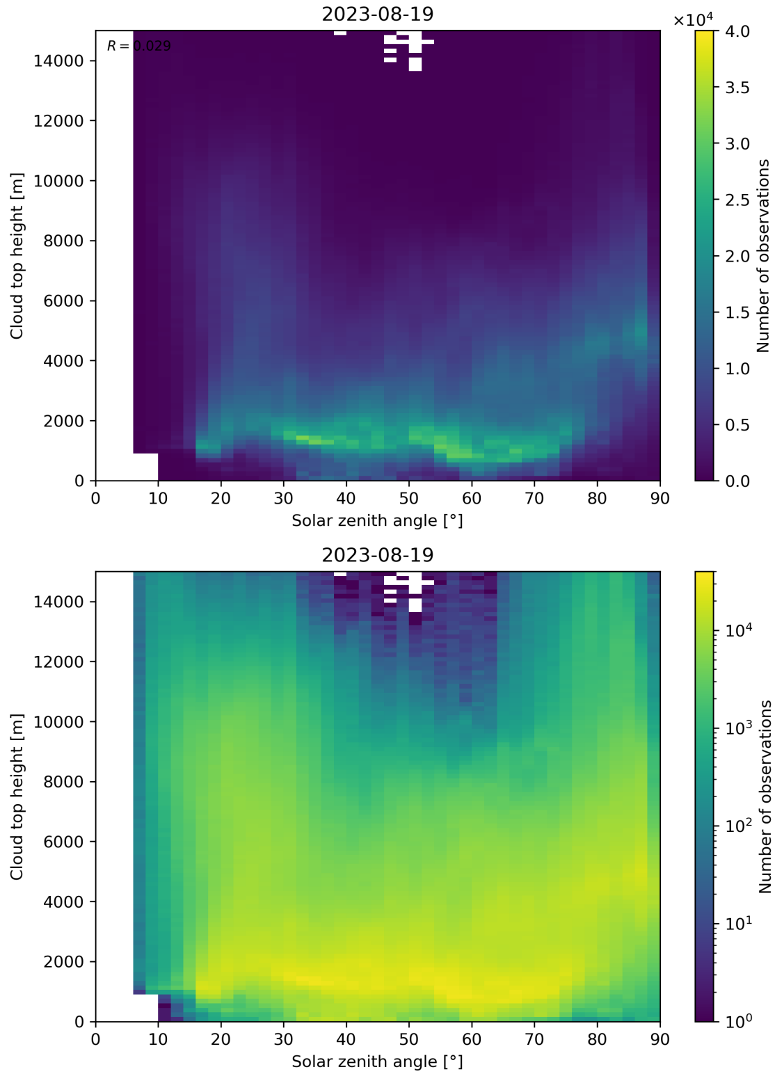
Figure 104: Scatter density plot of “Solar zenith angle” against “Cloud top height” for 2023-08-18 to 2023-08-20.
