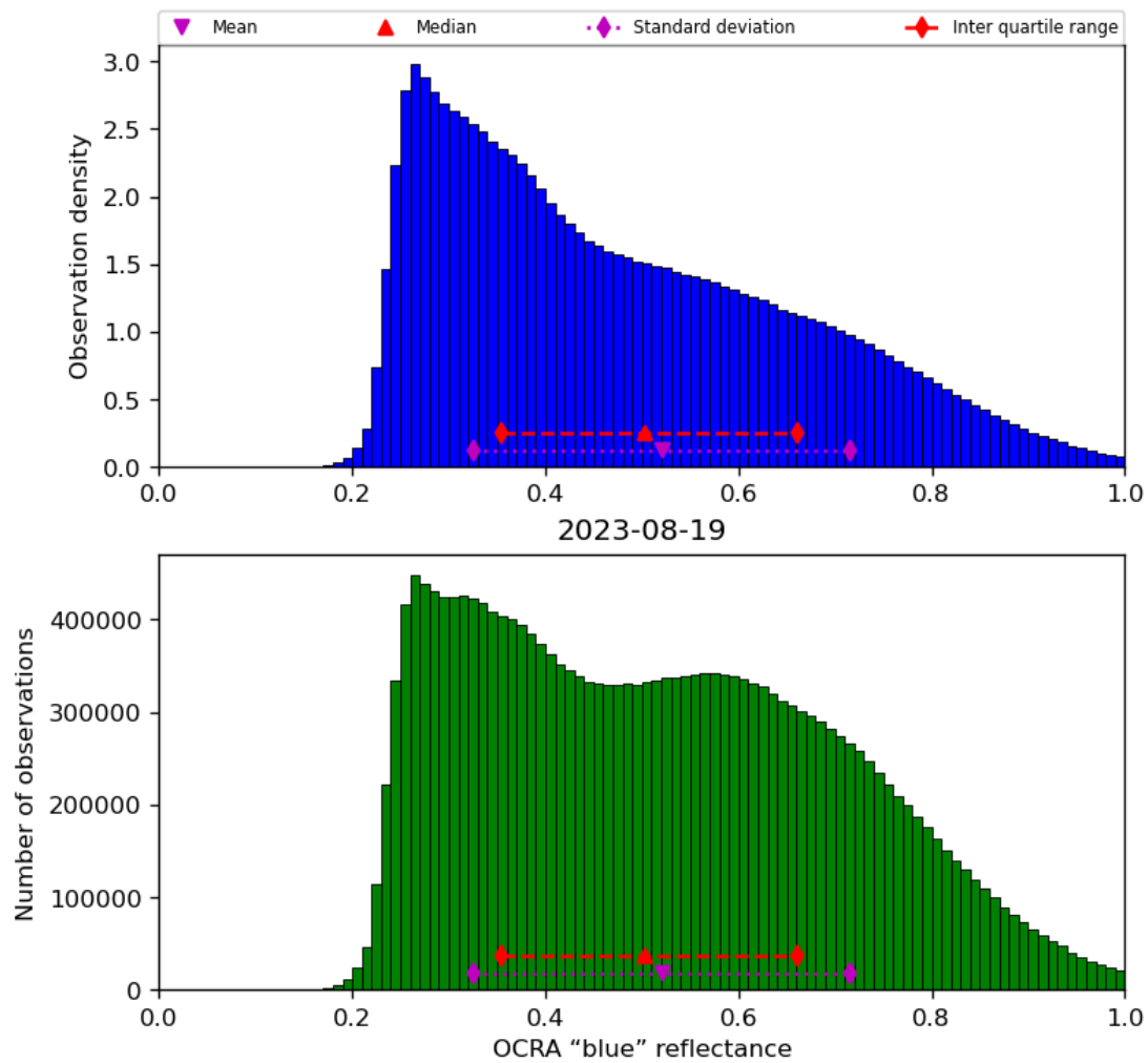
Figure 51: Histogram of “OCRA “blue” reflectance” for 2023-08-18 to 2023-08-20
