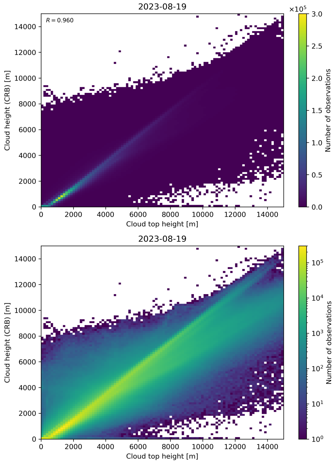
Figure 89: Scatter density plot of “Cloud top height” against “Cloud height (CRB)” for 2023-08-18 to 2023-08-20.
