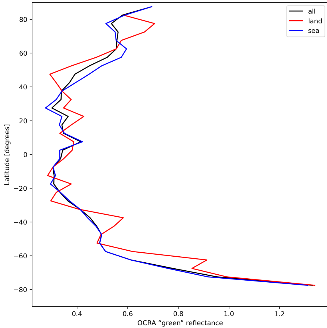
Figure 36: Zonal average of "OCRA "green" reflectance" for 2023-08-18 to 2023-08-20.
