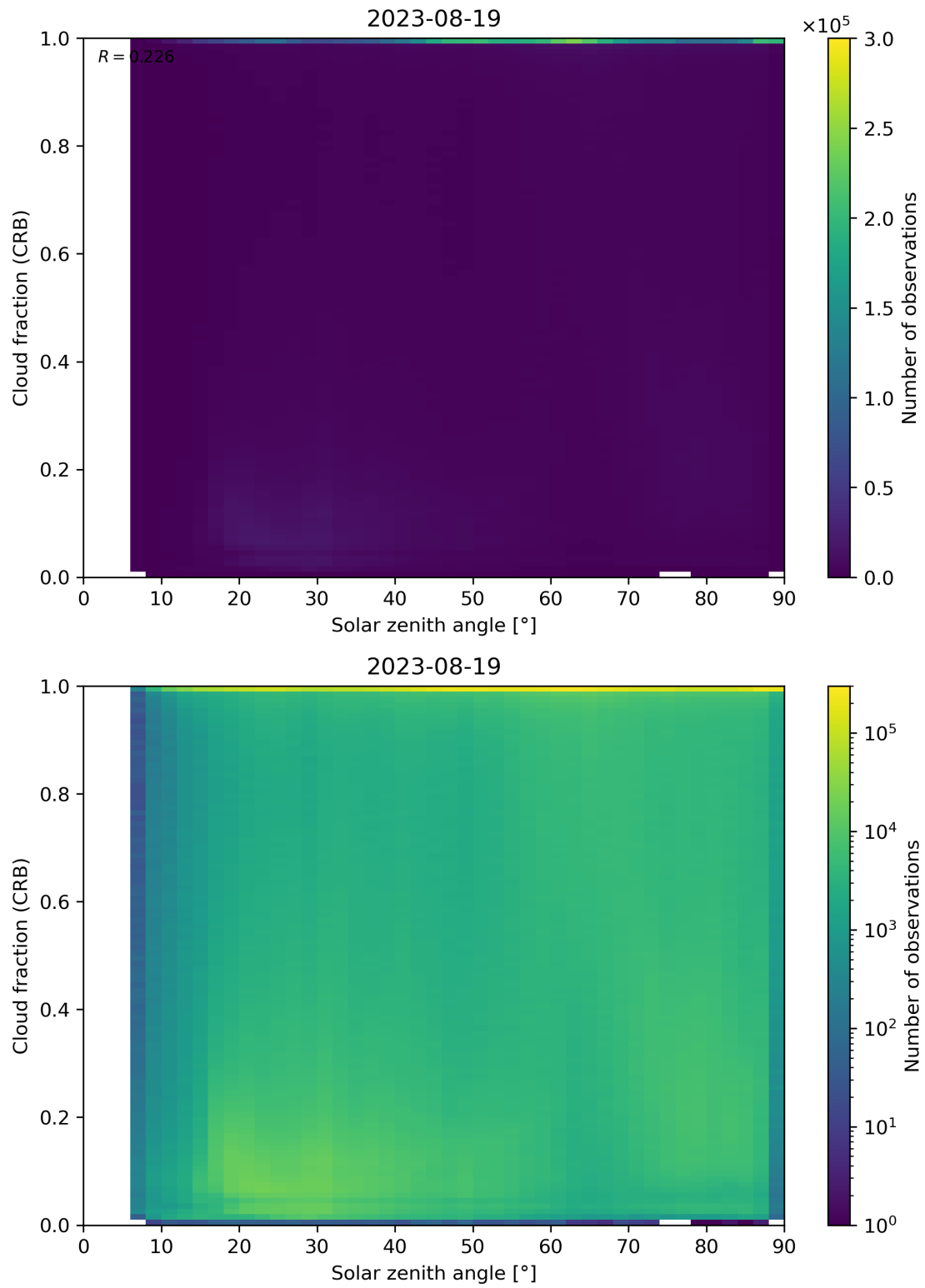
Figure 101: Scatter density plot of “Solar zenith angle” against “Cloud fraction (CRB)” for 2023-08-18 to 2023-08-20.
