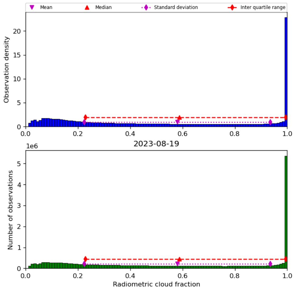
Figure 39: Histogram of “Radiometric cloud fraction” for 2023-08-18 to 2023-08-20
