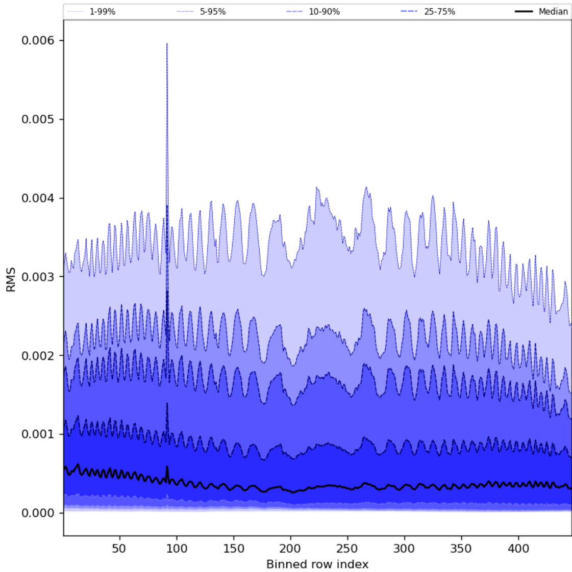
Figure 63: Along track statistics of “RMS” for 2023-08-18 to 2023-08-20
