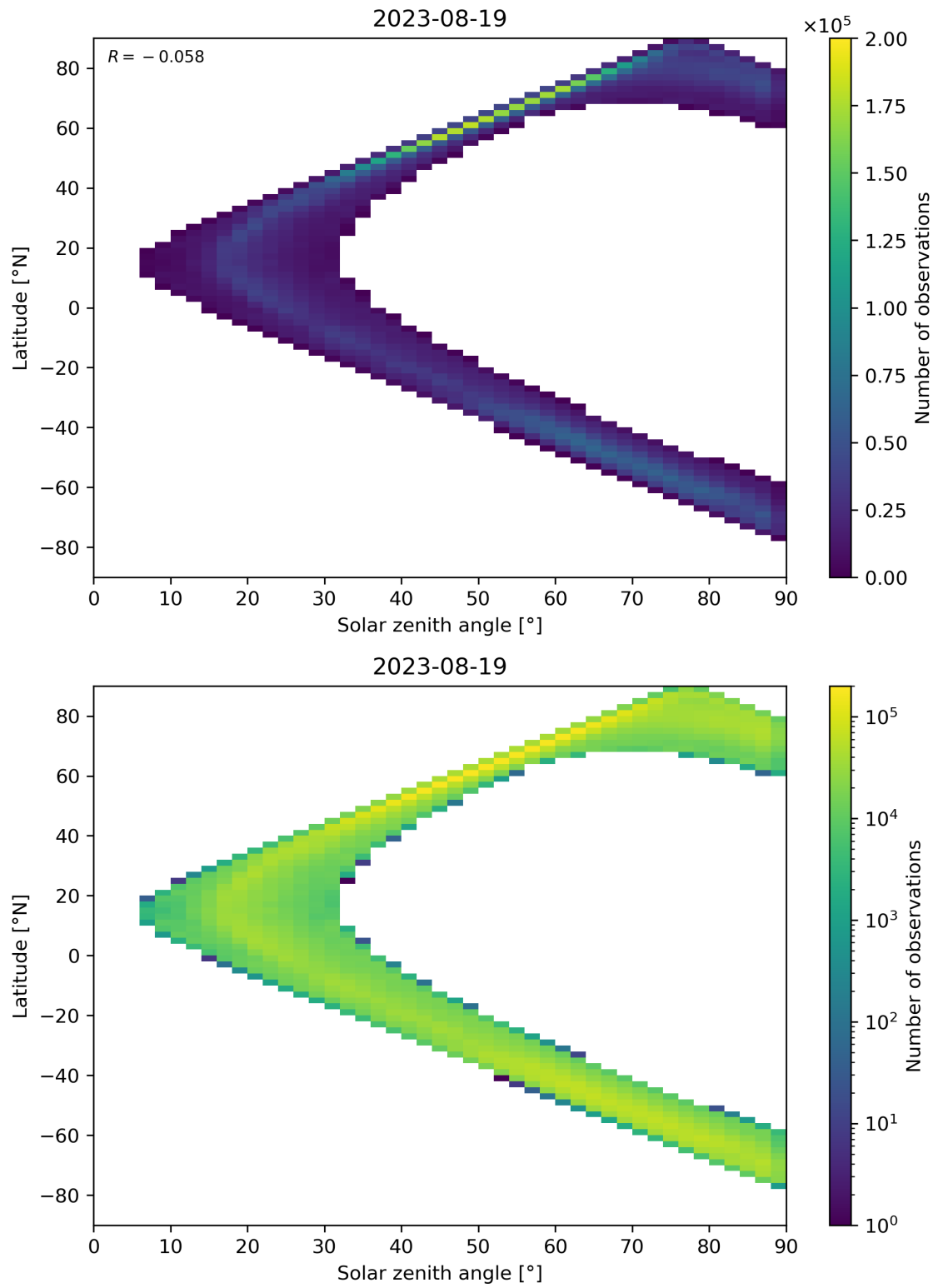
Figure 105: Scatter density plot of “Solar zenith angle” against “Latitude” for 2023-08-18 to 2023-08-20.
