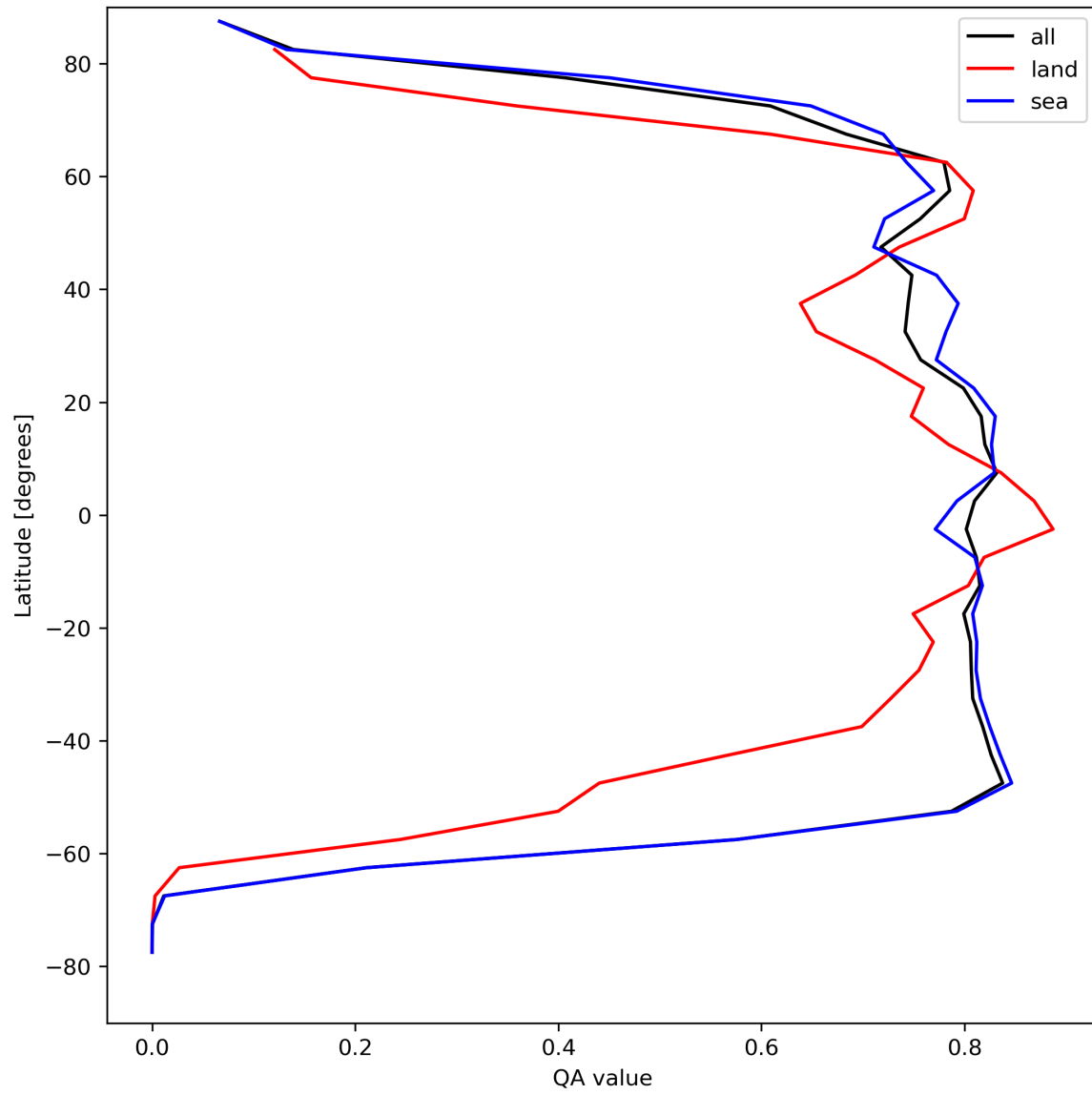
Figure 22: Zonal average of “QA value” for 2023-08-18 to 2023-08-20.
