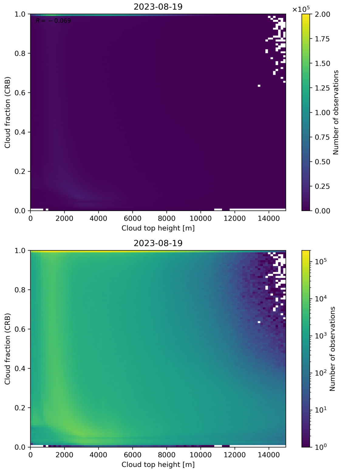
Figure 88: Scatter density plot of “Cloud top height” against “Cloud fraction (CRB)” for 2023-08-18 to 2023-08-20.
