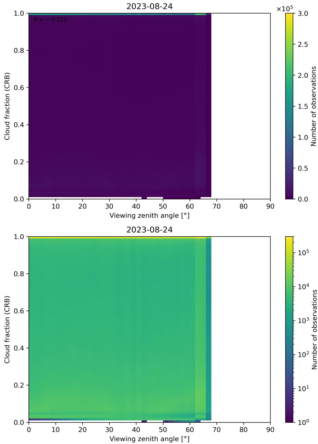
Figure 109: Scatter density plot of “Viewing zenith angle” against “Cloud fraction (CRB)” for 2023-08-23 to 2023-08-25.
