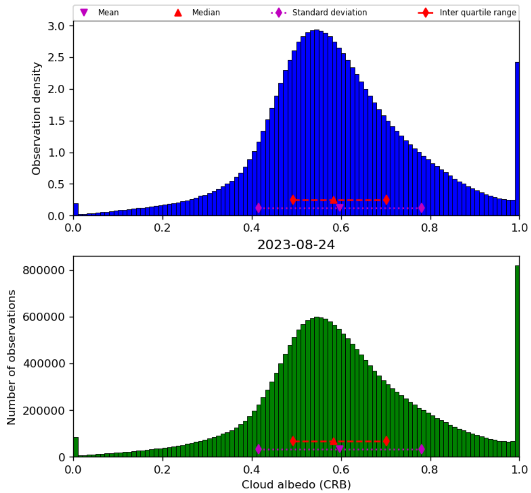
Figure 44: Histogram of “Cloud albedo (CRB)” for 2023-08-23 to 2023-08-25
