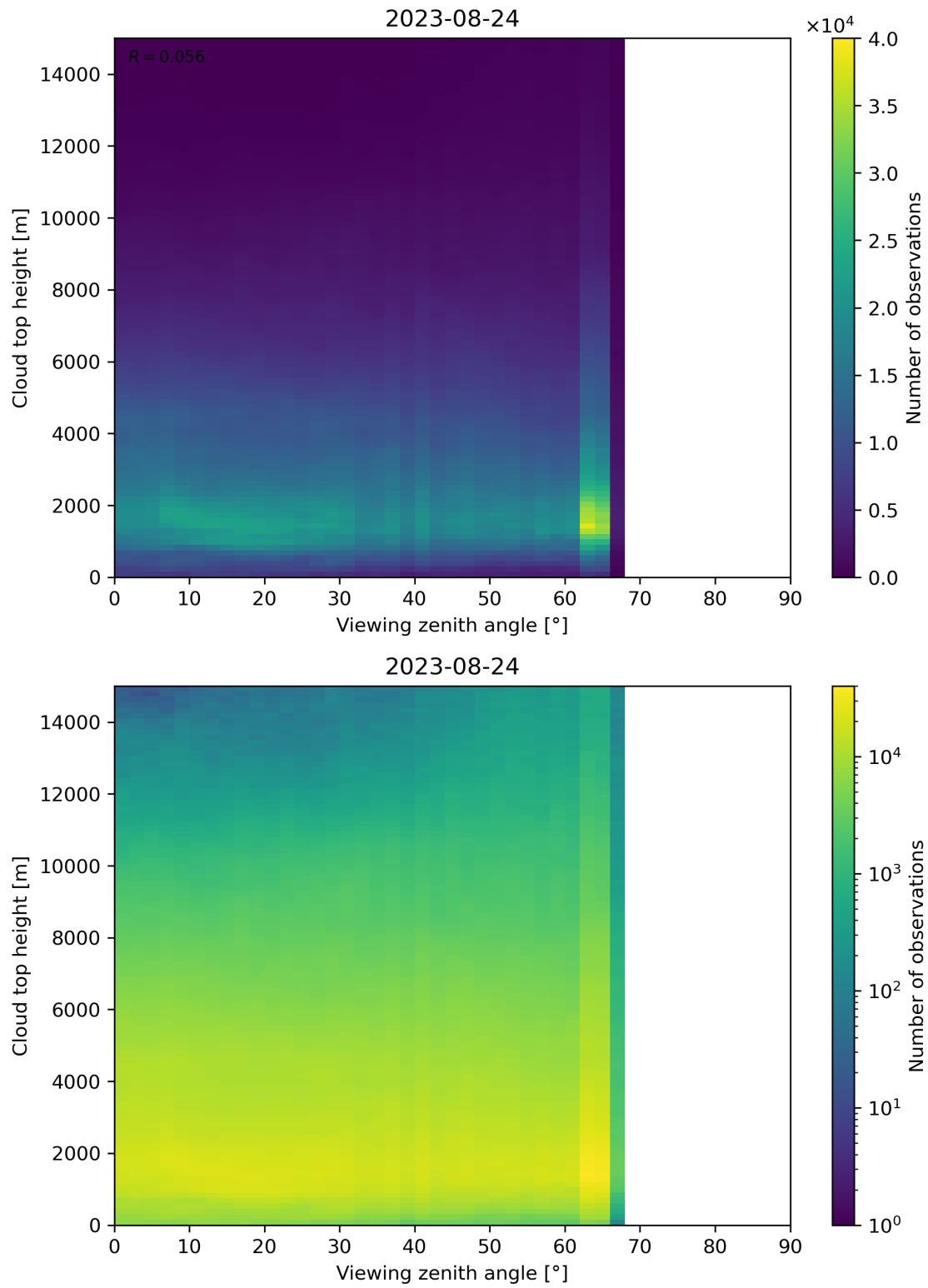
Figure 112: Scatter density plot of “Viewing zenith angle” against “Cloud top height” for 2023-08-23 to 2023-08-25.
