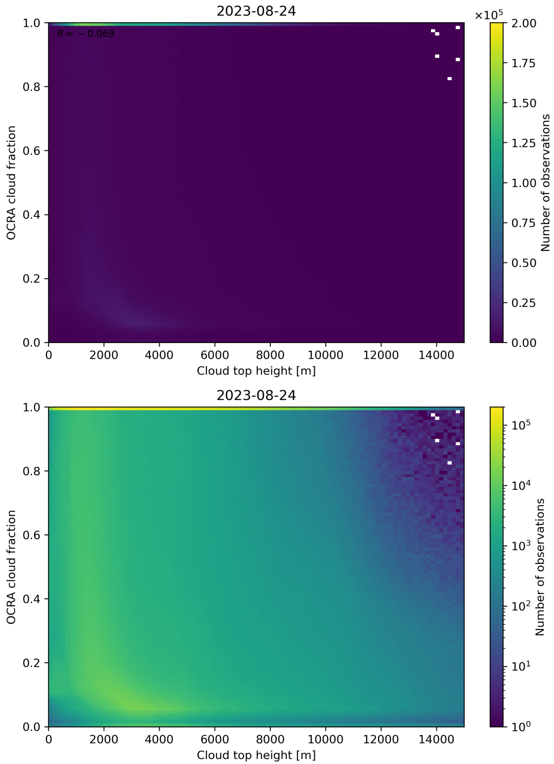
Figure 87: Scatter density plot of “Cloud top height” against “OCRA cloud fraction” for 2023-08-23 to 2023-08-25.
