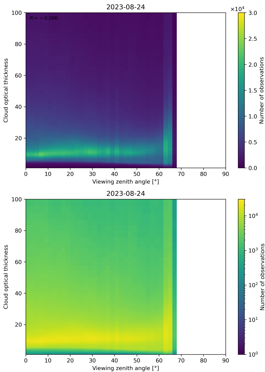
Figure 111: Scatter density plot of “Viewing zenith angle” against “Cloud optical thickness” for 2023-08-23 to 2023-08-25.
