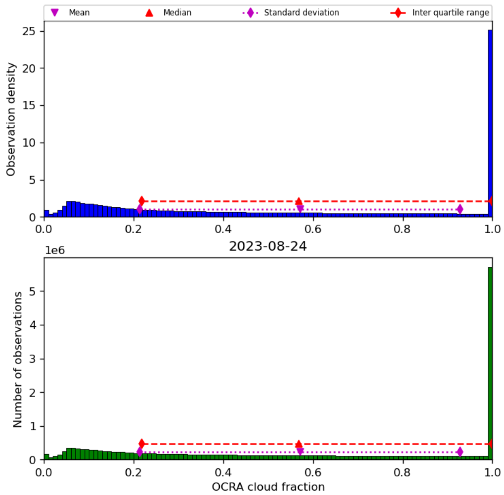
Figure 50: Histogram of “OCRA cloud fraction” for 2023-08-23 to 2023-08-25
