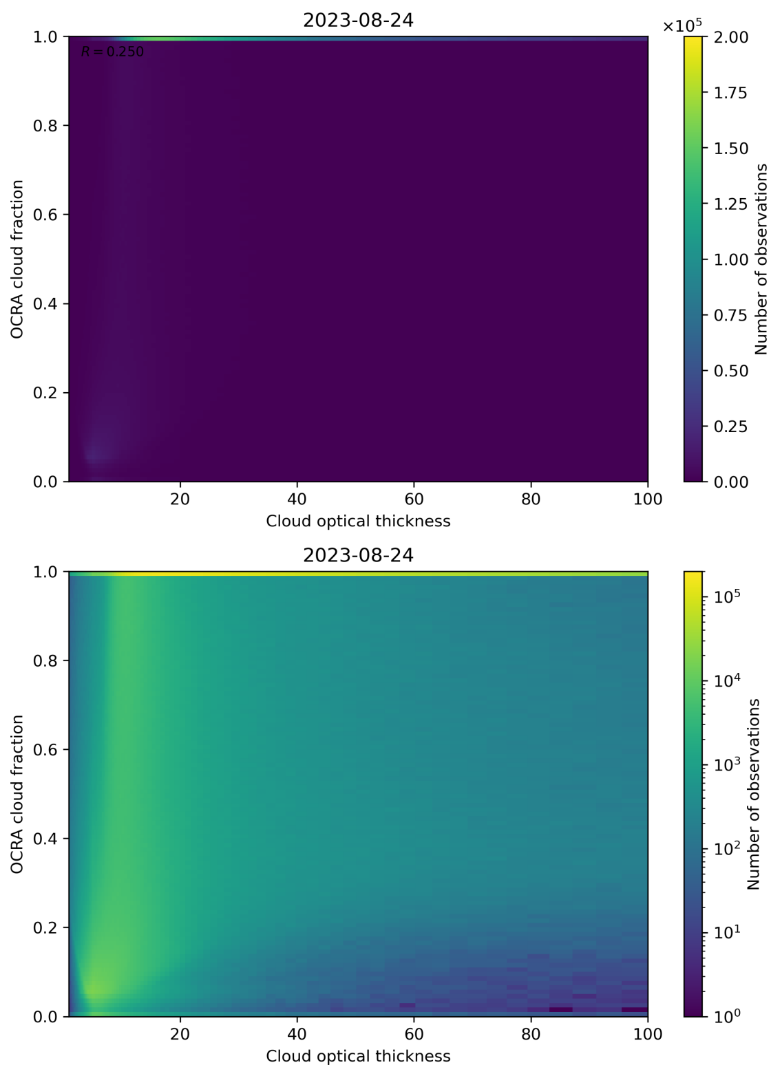
Figure 83: Scatter density plot of “Cloud optical thickness” against “OCRA cloud fraction” for 2023-08-23 to 2023-08-25.
