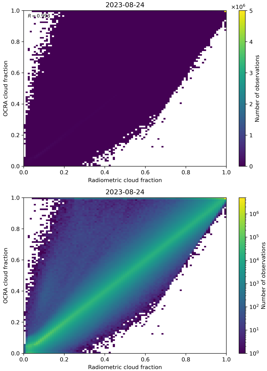
Figure 72: Scatter density plot of “Radiometric cloud fraction” against “OCRA cloud fraction” for 2023-08-23 to 2023-08-25.
