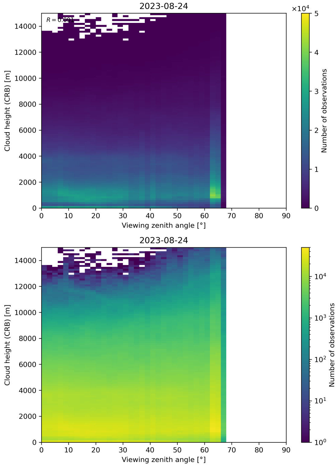
Figure 110: Scatter density plot of “Viewing zenith angle” against “Cloud height (CRB)” for 2023-08-23 to 2023-08-25.
