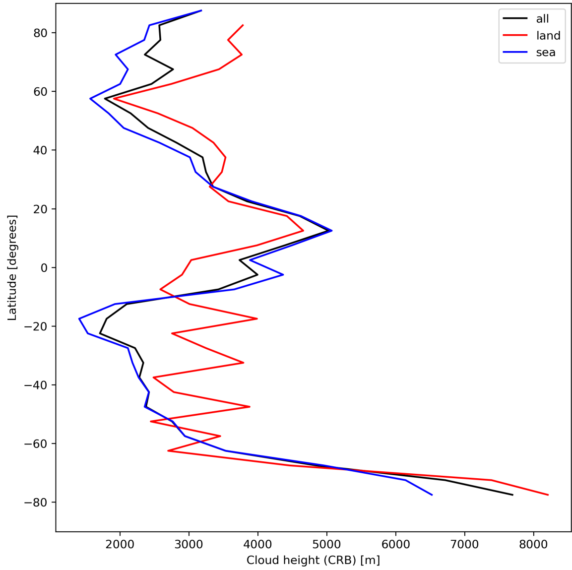
Figure 27: Zonal average of “Cloud height (CRB)” for 2023-08-23 to 2023-08-25.
