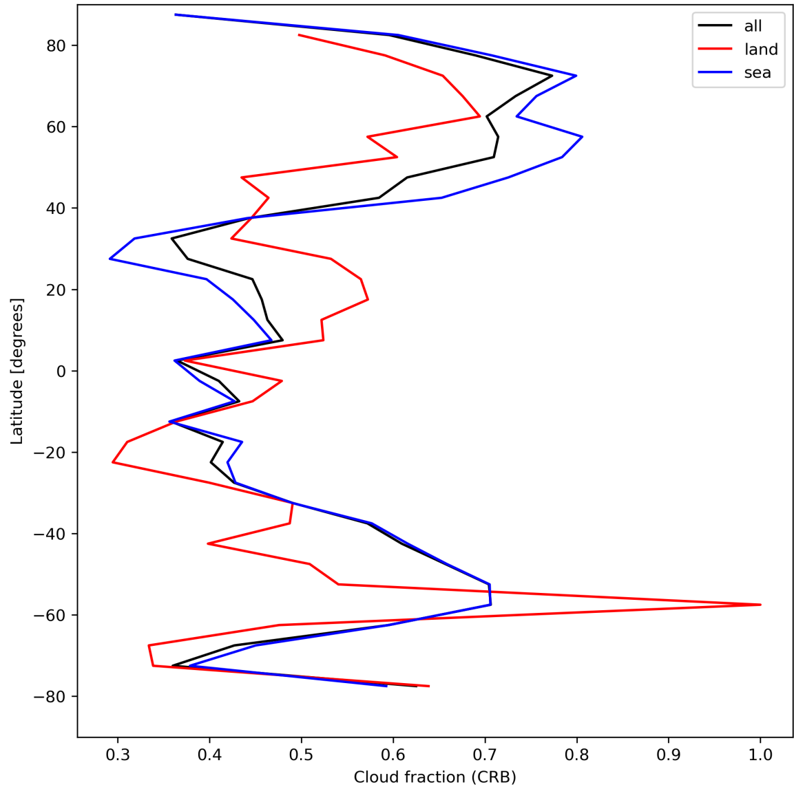
Figure 26: Zonal average of “Cloud fraction (CRB)” for 2023-08-23 to 2023-08-25.
