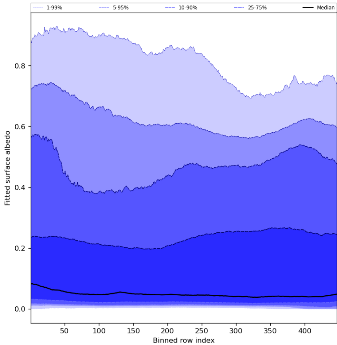
Figure 61: Along track statistics of “Fitted surface albedo” for 2023-08-23 to 2023-08-25
