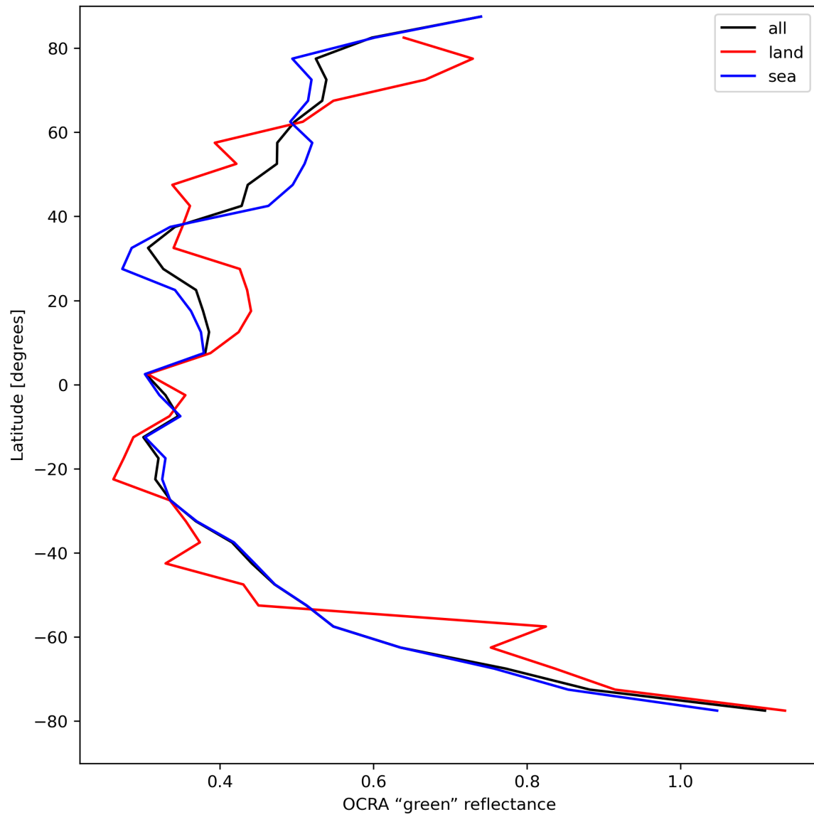
Figure 36: Zonal average of “OCRA “green” reflectance” for 2023-08-23 to 2023-08-25.
