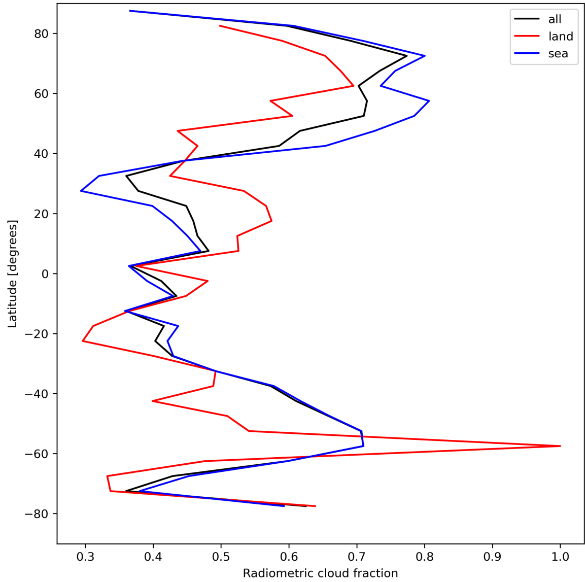
Figure 23: Zonal average of “Radiometric cloud fraction” for 2023-08-23 to 2023-08-25.
