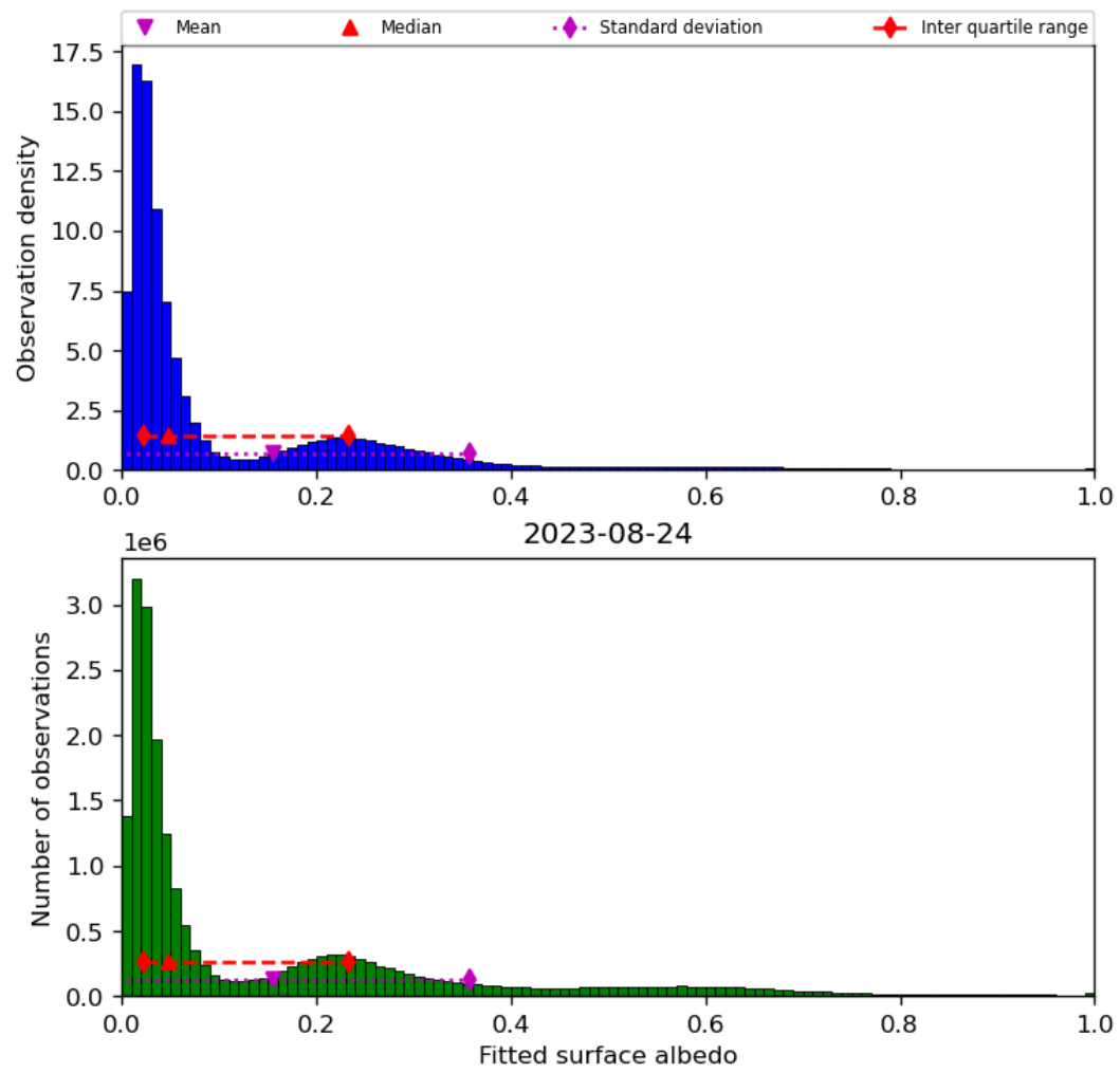
Figure 45: Histogram of “Fitted surface albedo” for 2023-08-23 to 2023-08-25
