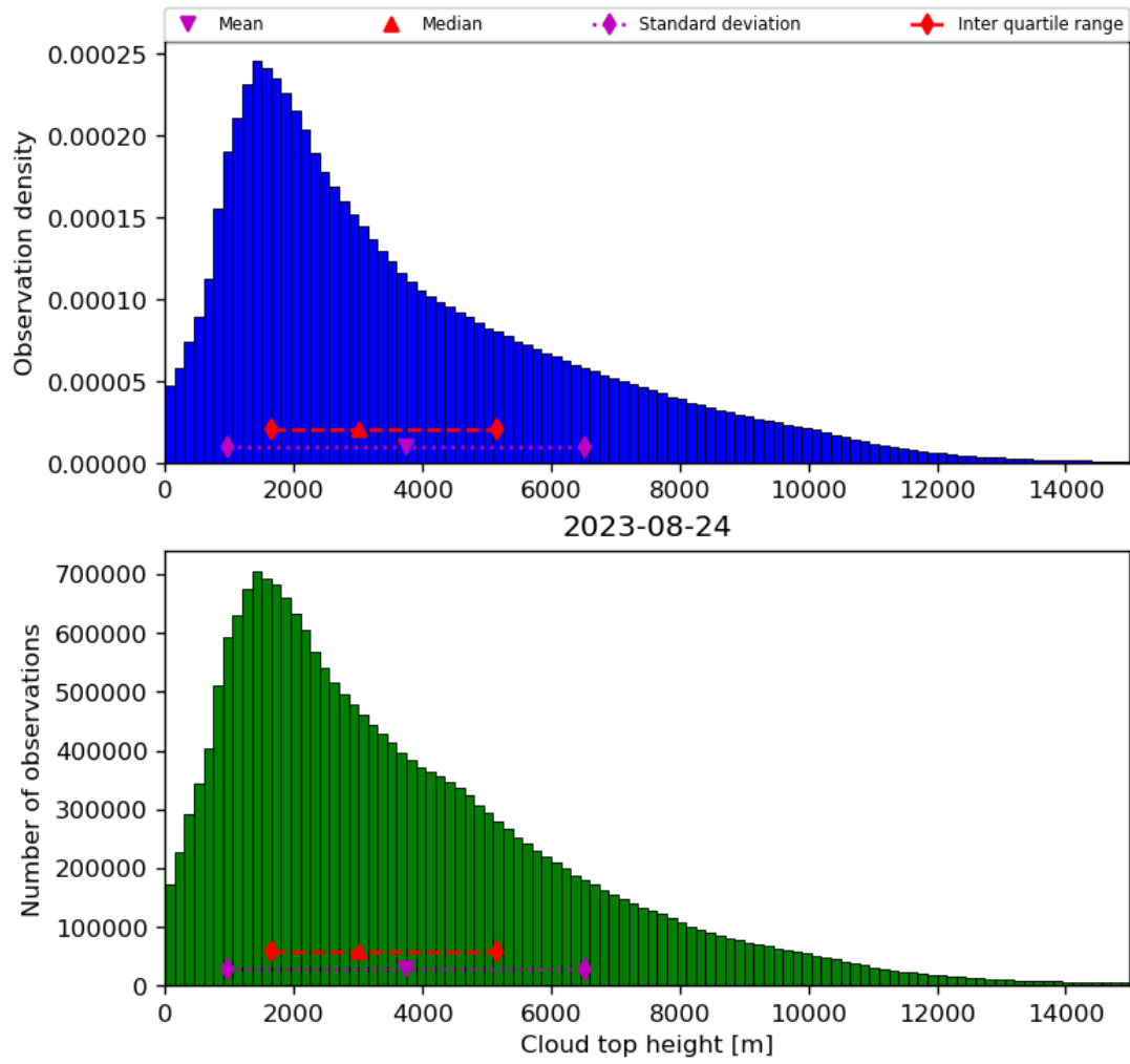
Figure 40: Histogram of “Cloud top height” for 2023-08-23 to 2023-08-25
