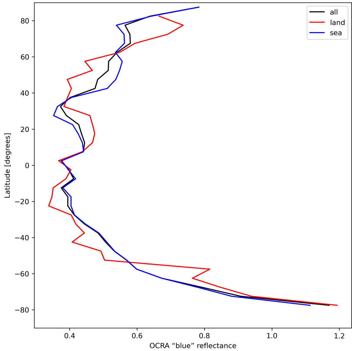
Figure 35: Zonal average of "OCRA "blue" reflectance" for 2023-08-23 to 2023-08-25.
