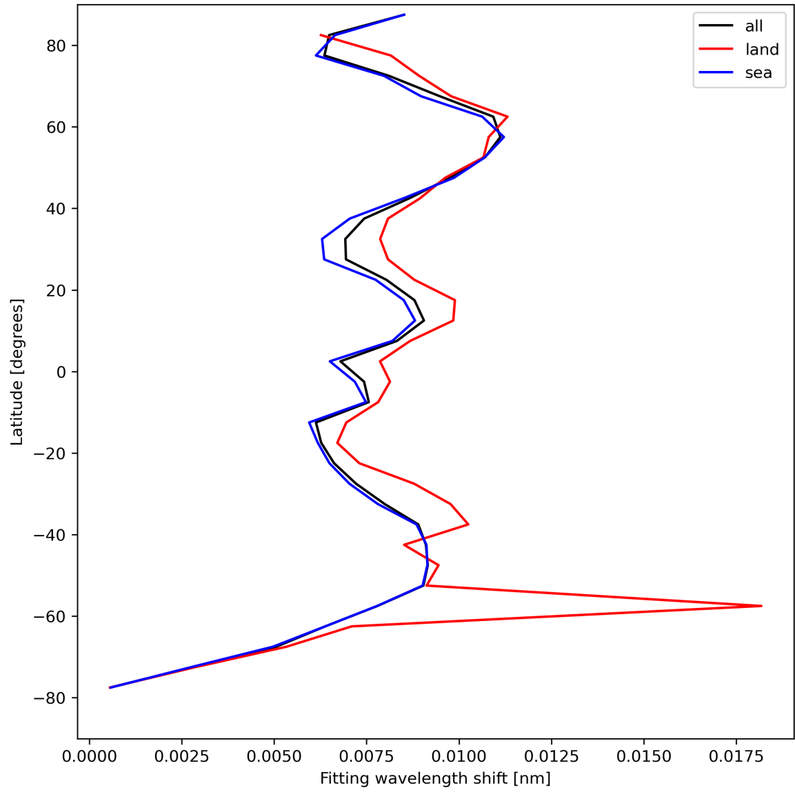
Figure 33: Zonal average of “Fitting wavelength shift” for 2023-08-23 to 2023-08-25.
