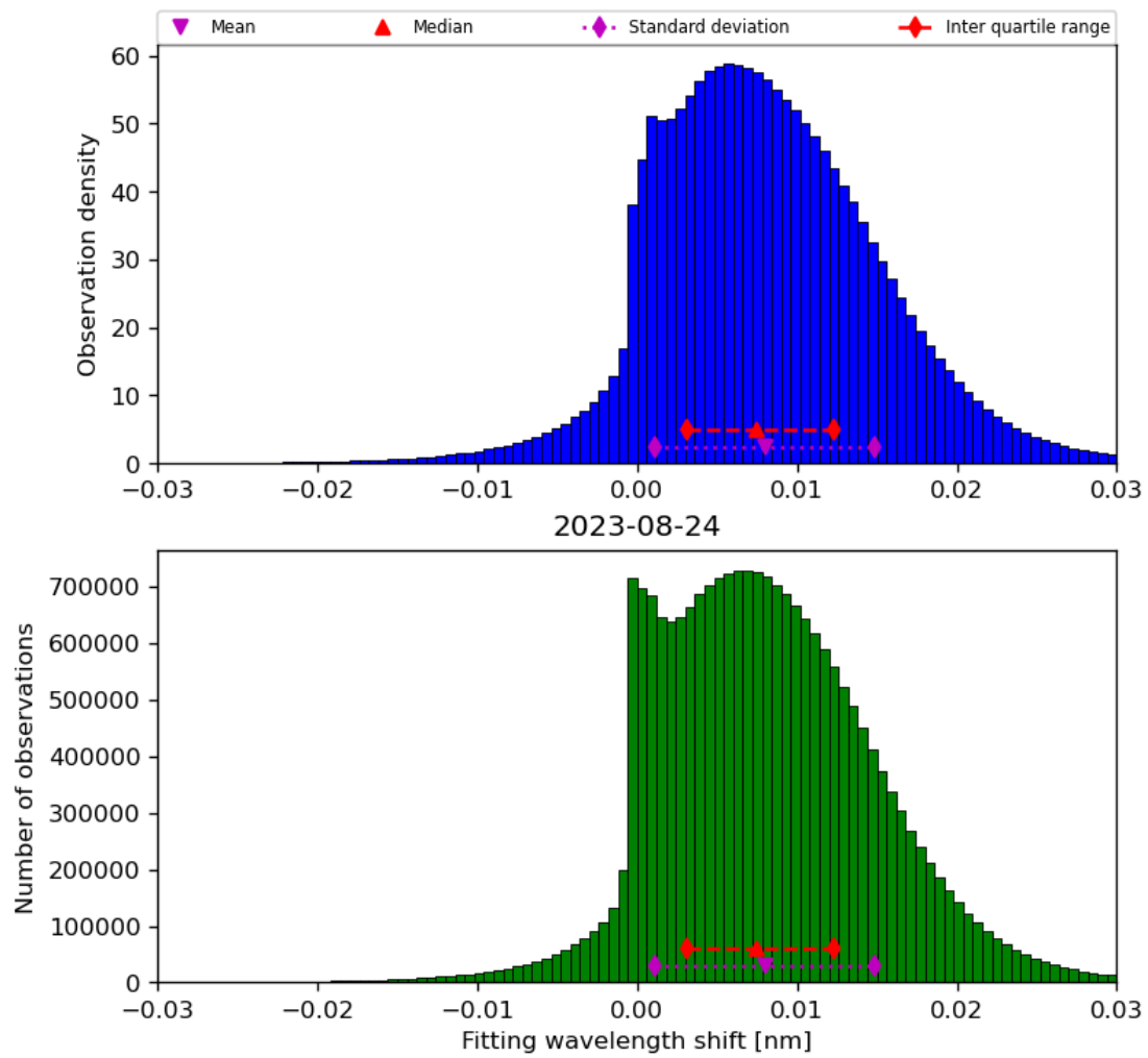
Figure 49: Histogram of “Fitting wavelength shift” for 2023-08-23 to 2023-08-25
