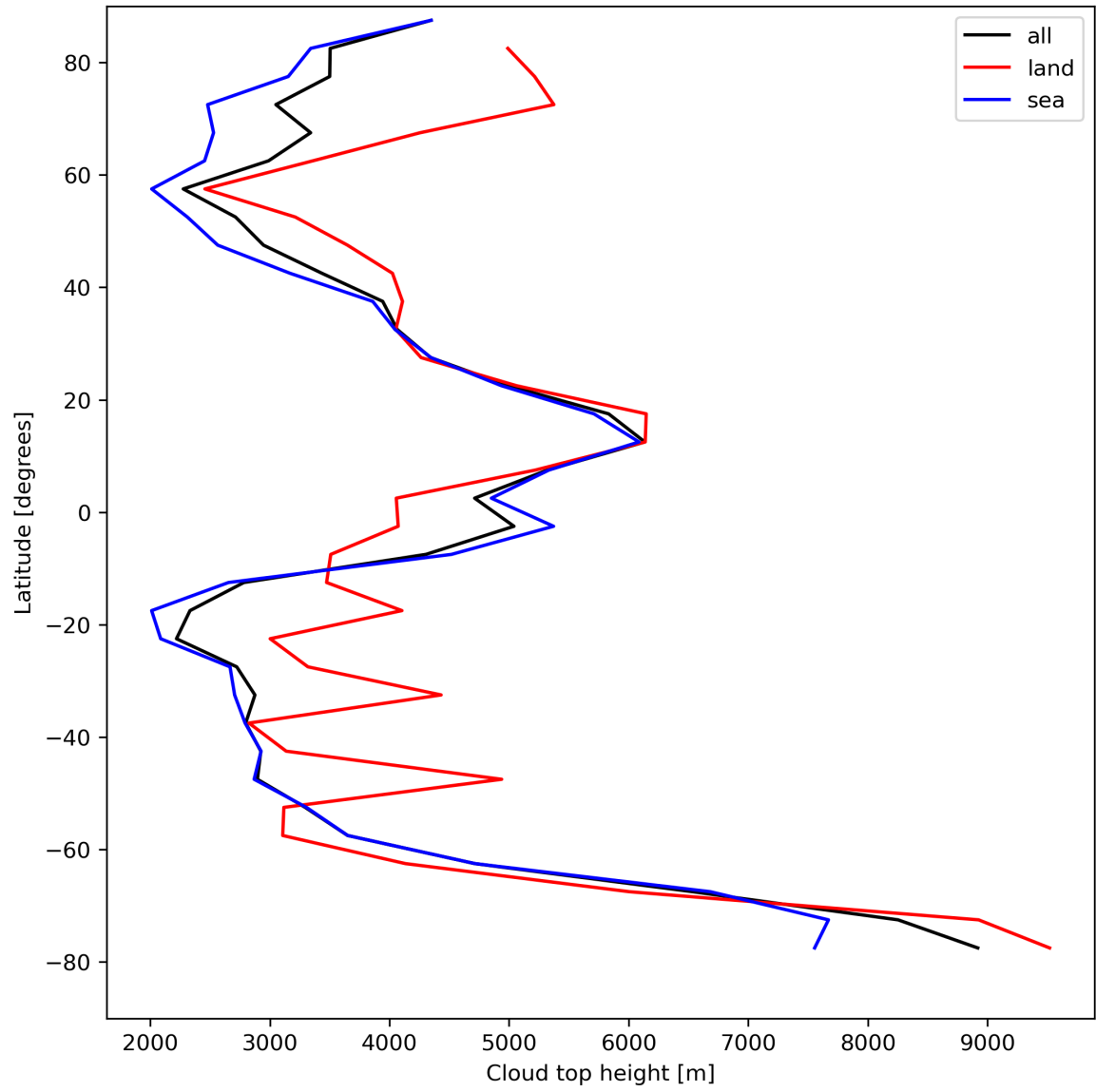
Figure 24: Zonal average of “Cloud top height” for 2023-08-23 to 2023-08-25.
