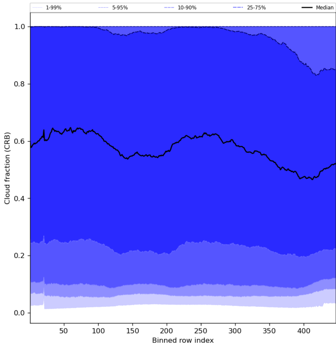
Figure 58: Along track statistics of “Cloud fraction (CRB)” for 2023-08-23 to 2023-08-25
