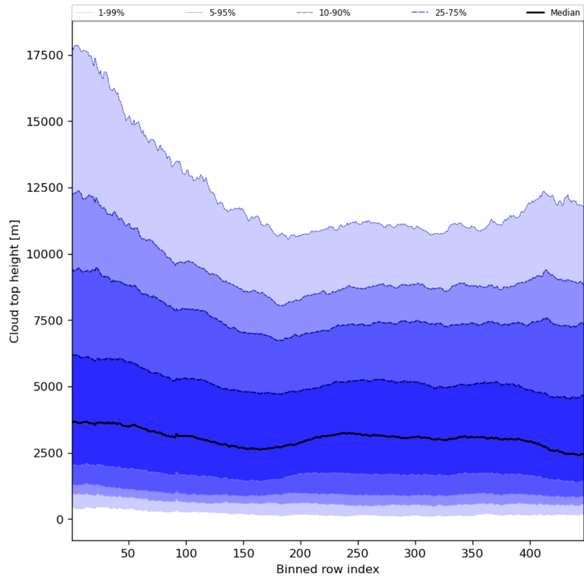
Figure 56: Along track statistics of “Cloud top height” for 2023-08-23 to 2023-08-25
