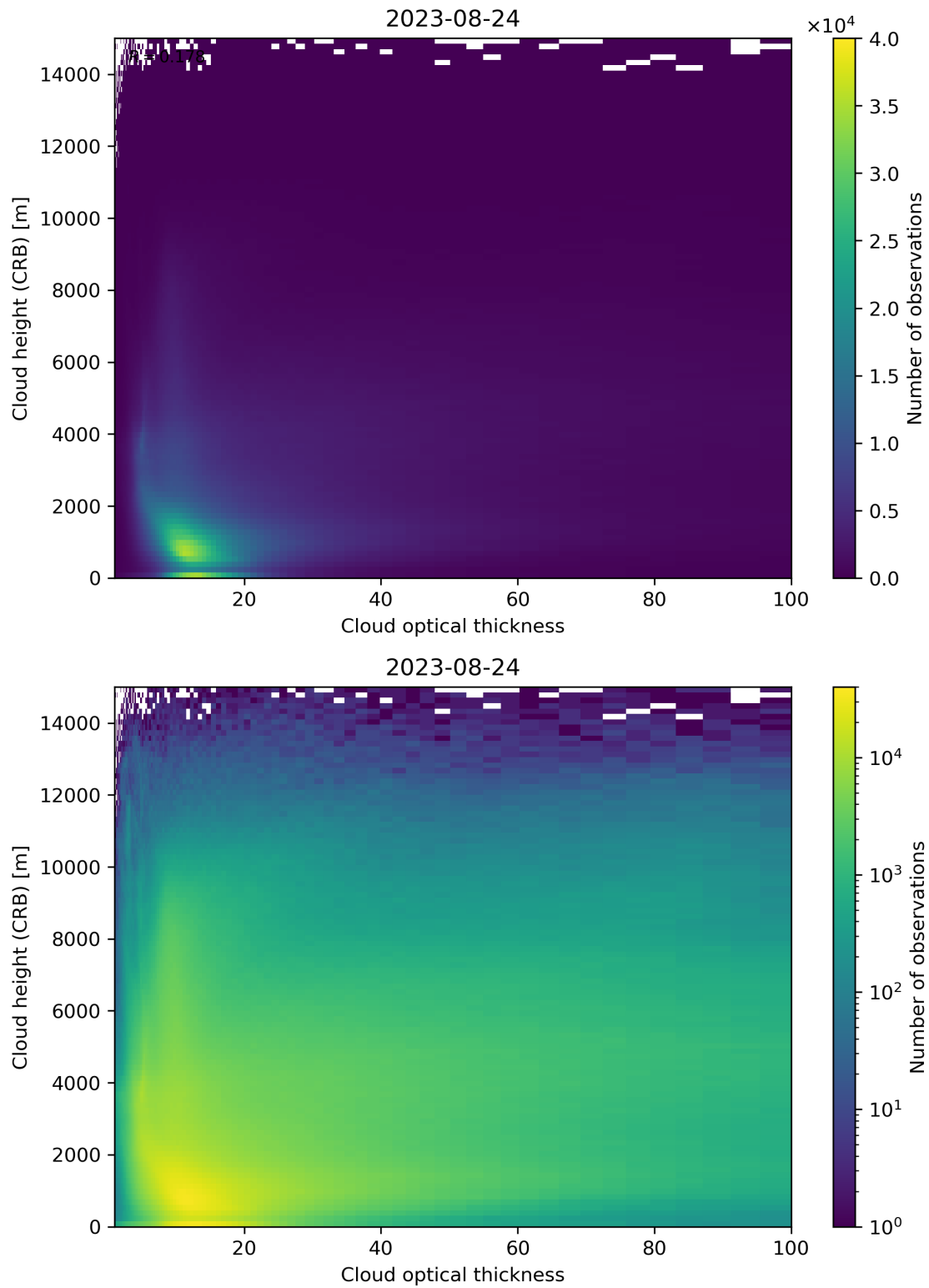
Figure 85: Scatter density plot of “Cloud optical thickness” against “Cloud height (CRB)” for 2023-08-23 to 2023-08-25.
