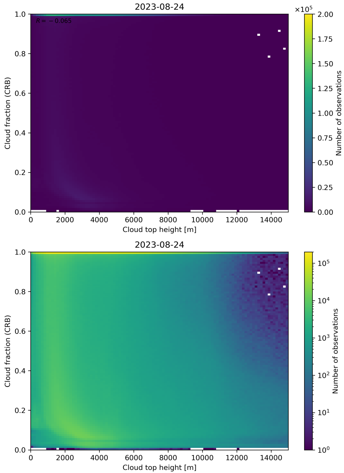
Figure 88: Scatter density plot of “Cloud top height” against “Cloud fraction (CRB)” for 2023-08-23 to 2023-08-25.
