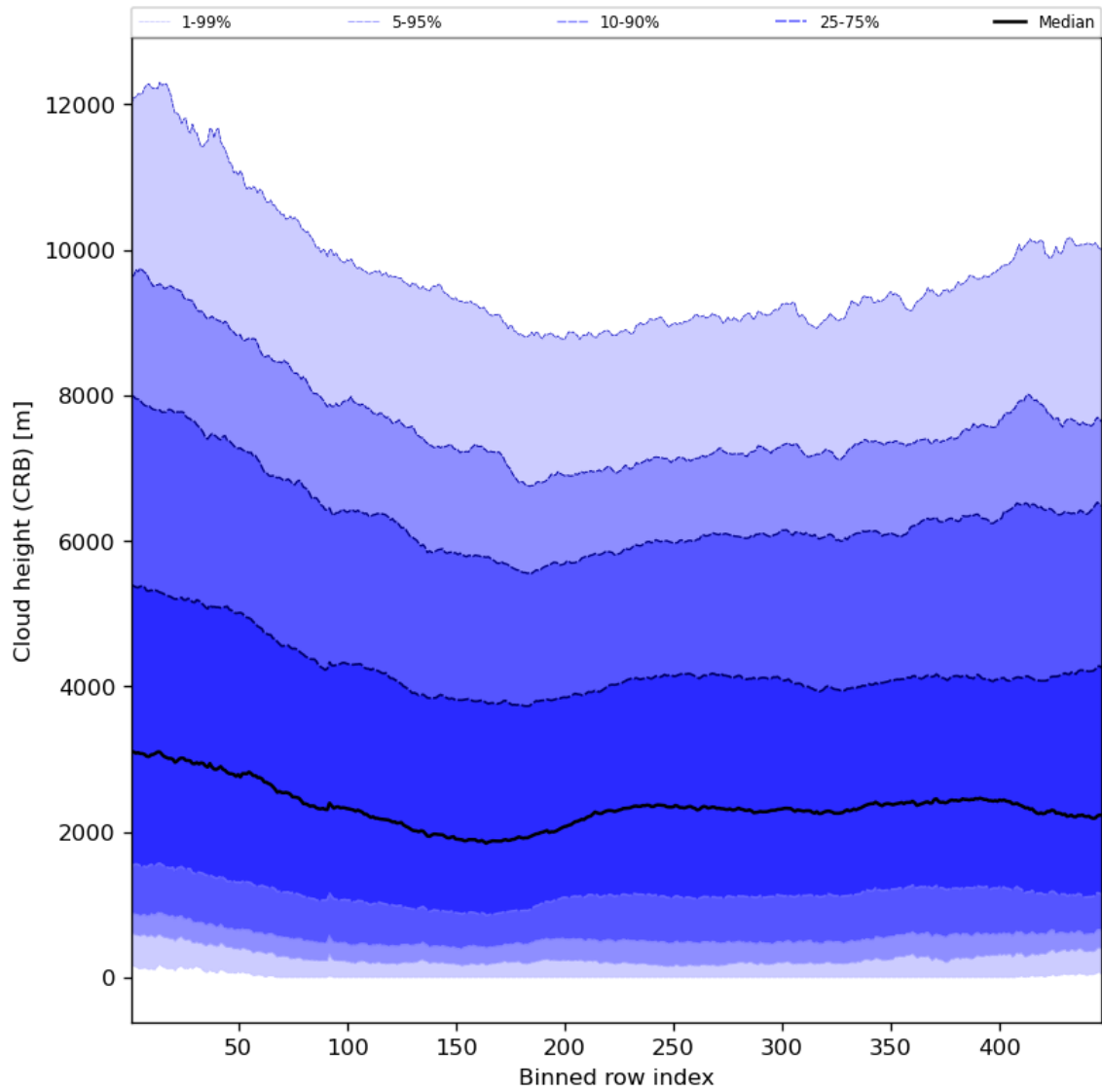
Figure 59: Along track statistics of “Cloud height (CRB)” for 2023-08-23 to 2023-08-25
