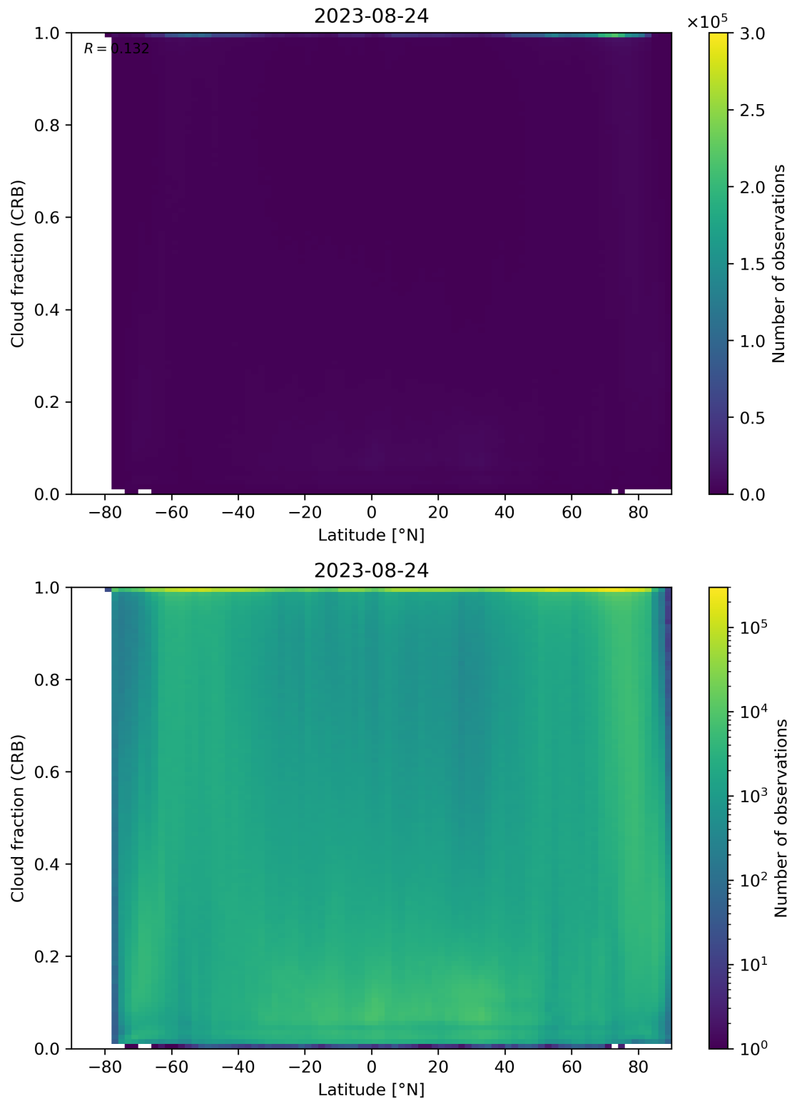
Figure 94: Scatter density plot of “Latitude” against “Cloud fraction (CRB)” for 2023-08-23 to 2023-08-25.
