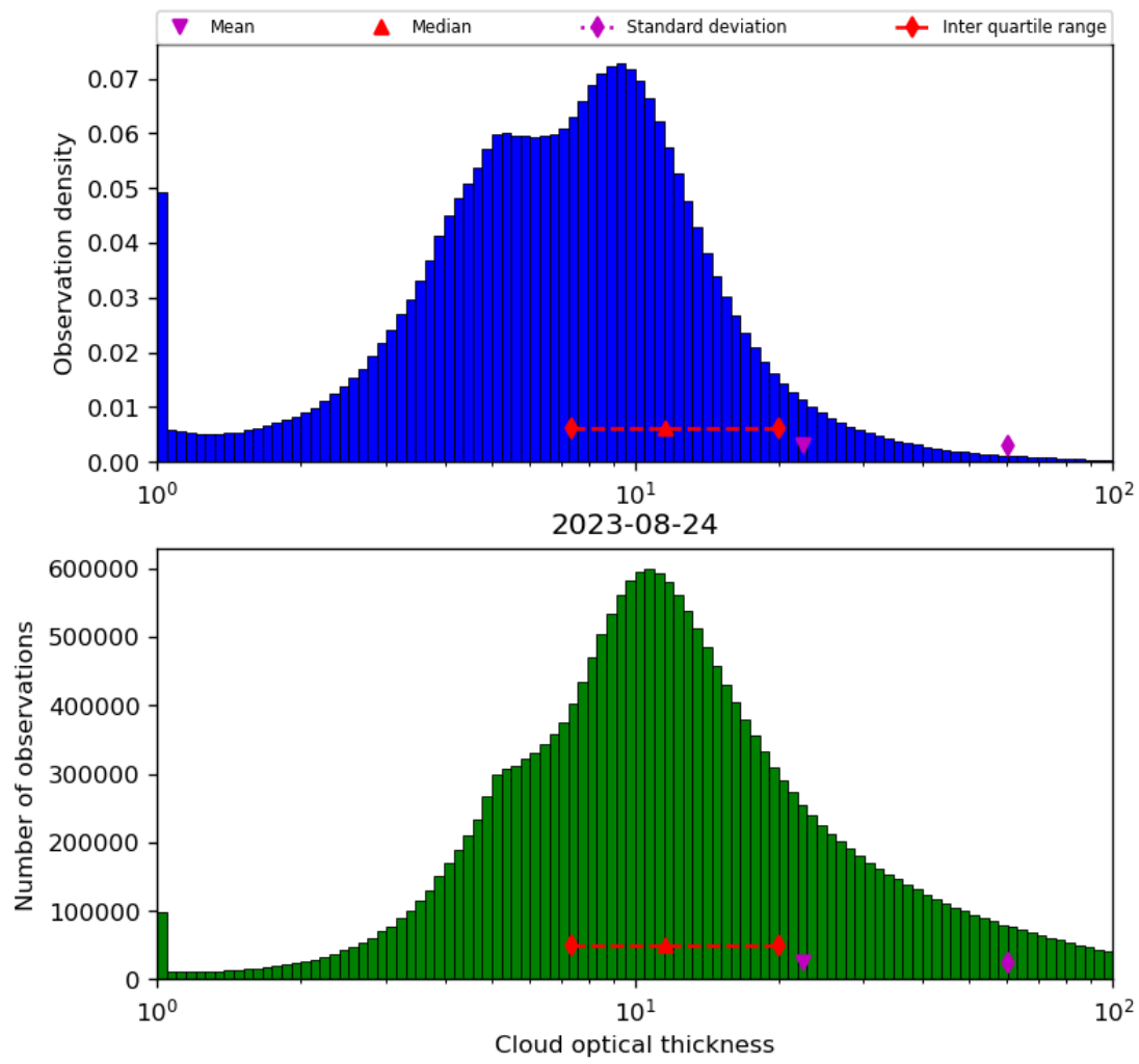
Figure 41: Histogram of “Cloud optical thickness” for 2023-08-23 to 2023-08-25
