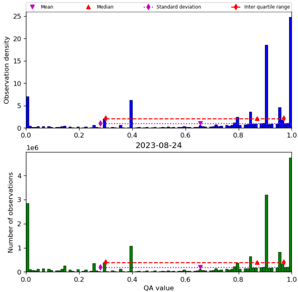
Figure 38: Histogram of “QA value” for 2023-08-23 to 2023-08-25
