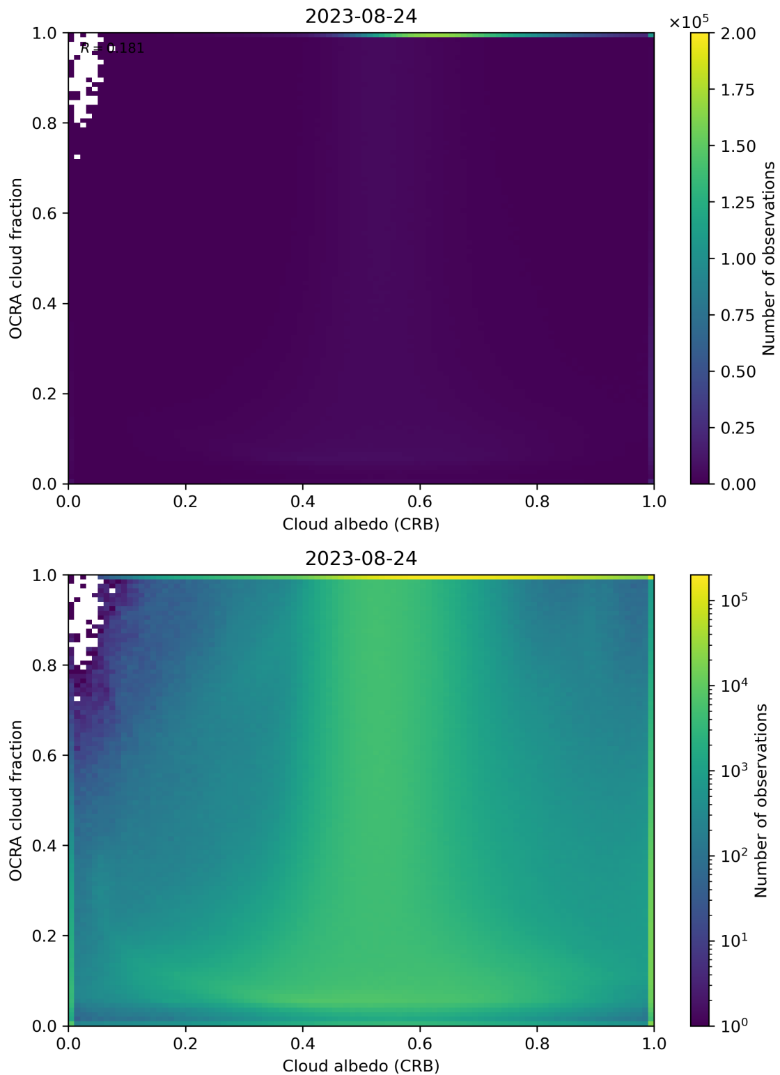
Figure 70: Scatter density plot of “Cloud albedo (CRB)” against “OCRA cloud fraction” for 2023-08-23 to 2023-08-25.
