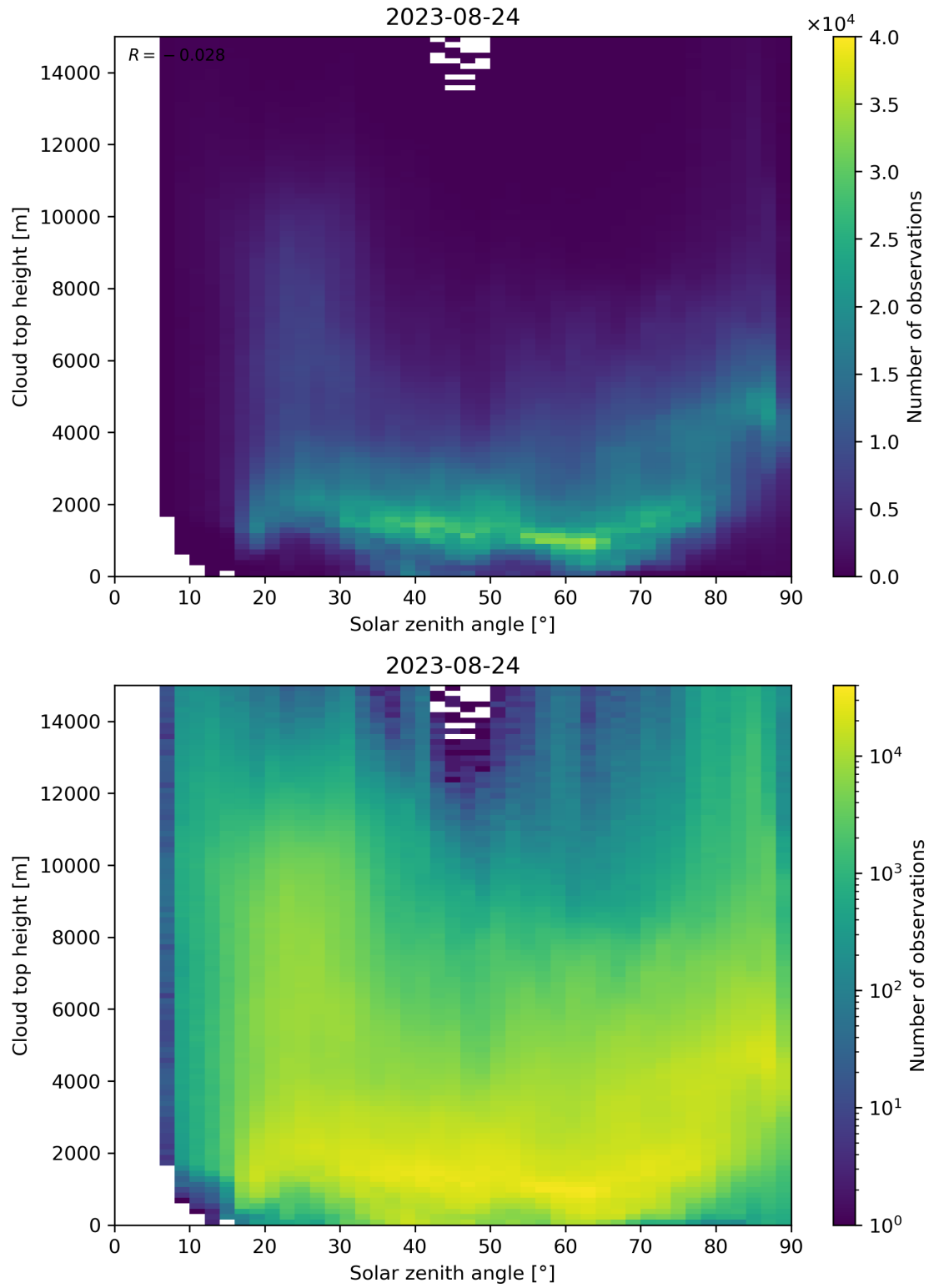
Figure 104: Scatter density plot of “Solar zenith angle” against “Cloud top height” for 2023-08-23 to 2023-08-25.
