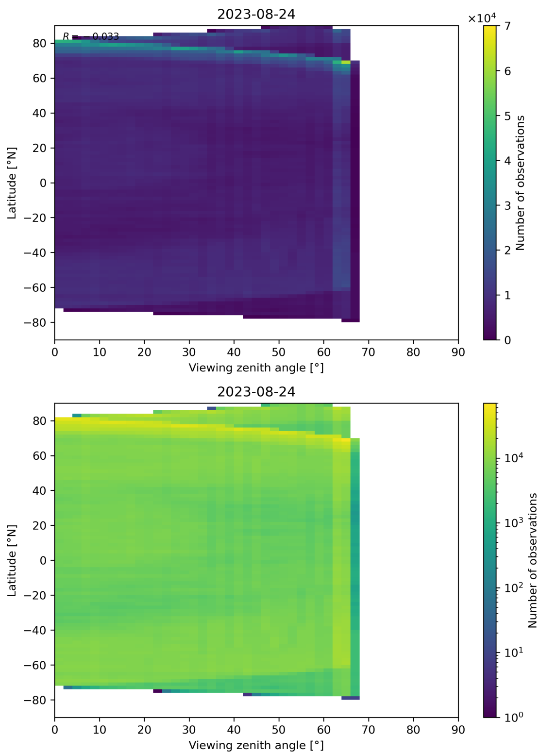
Figure 113: Scatter density plot of “Viewing zenith angle” against “Latitude” for 2023-08-23 to 2023-08-25.
