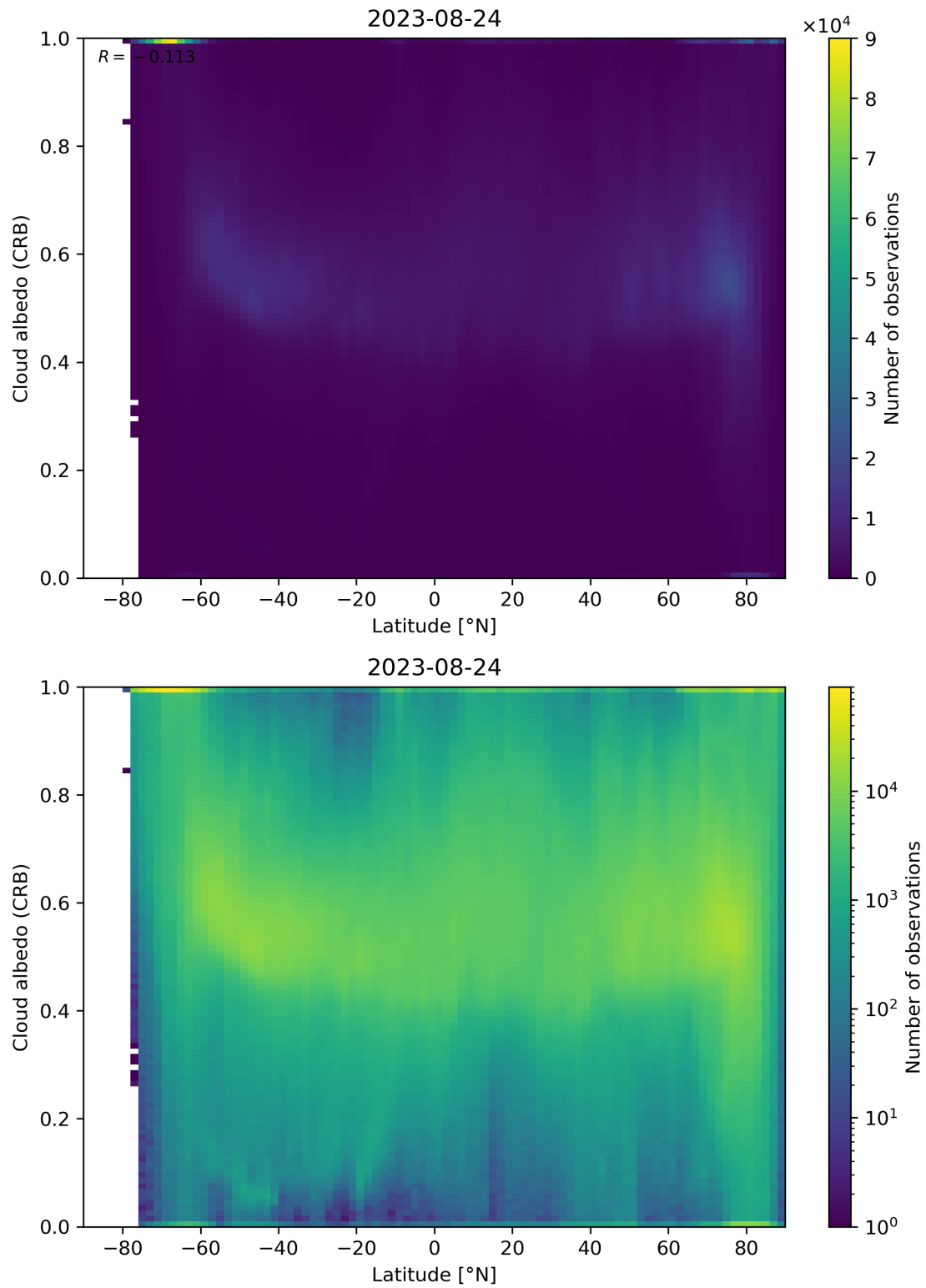
Figure 91: Scatter density plot of “Latitude” against “Cloud albedo (CRB)” for 2023-08-23 to 2023-08-25.
