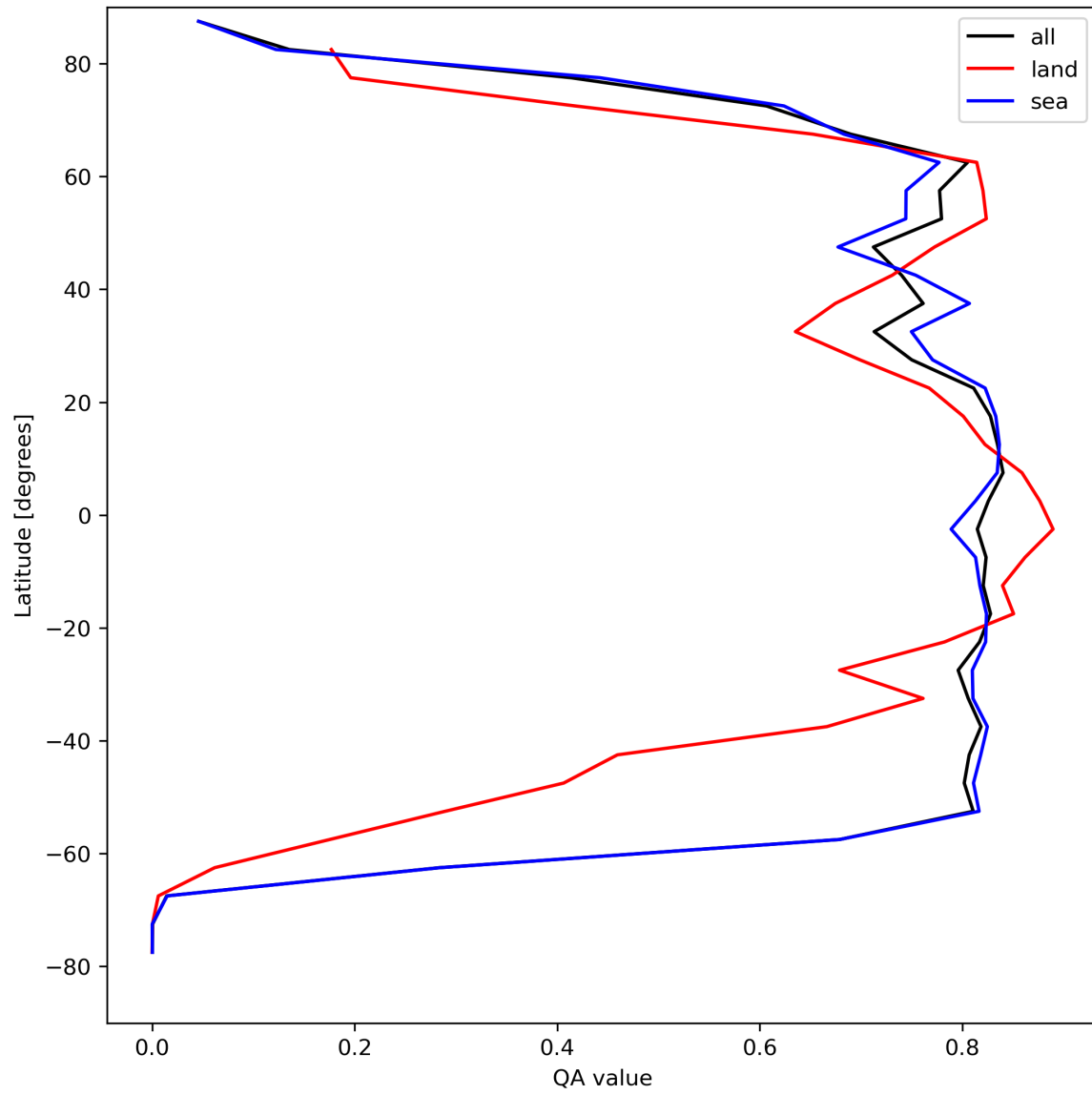
Figure 22: Zonal average of “QA value” for 2023-08-23 to 2023-08-25.
