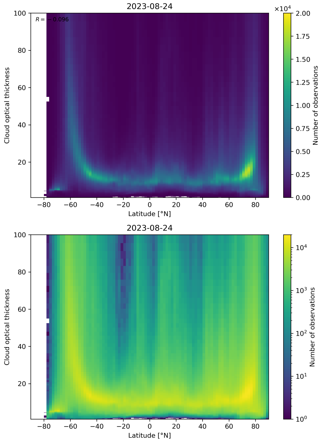
Figure 96: Scatter density plot of “Latitude” against “Cloud optical thickness” for 2023-08-23 to 2023-08-25.
