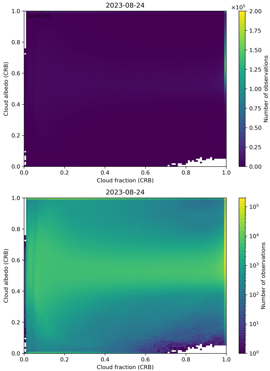
Figure 77: Scatter density plot of “Cloud fraction (CRB)” against “Cloud albedo (CRB)” for 2023-08-23 to 2023-08-25.
