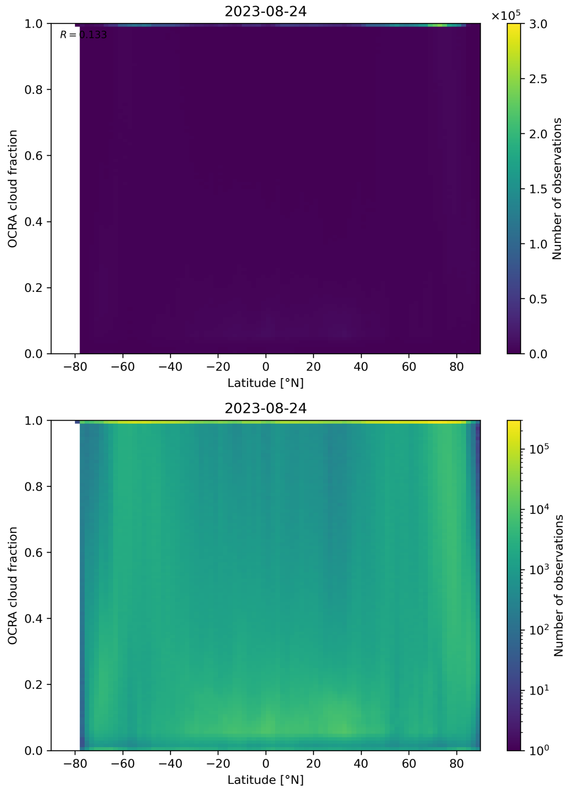
Figure 93: Scatter density plot of “Latitude” against “OCRA cloud fraction” for 2023-08-23 to 2023-08-25.
