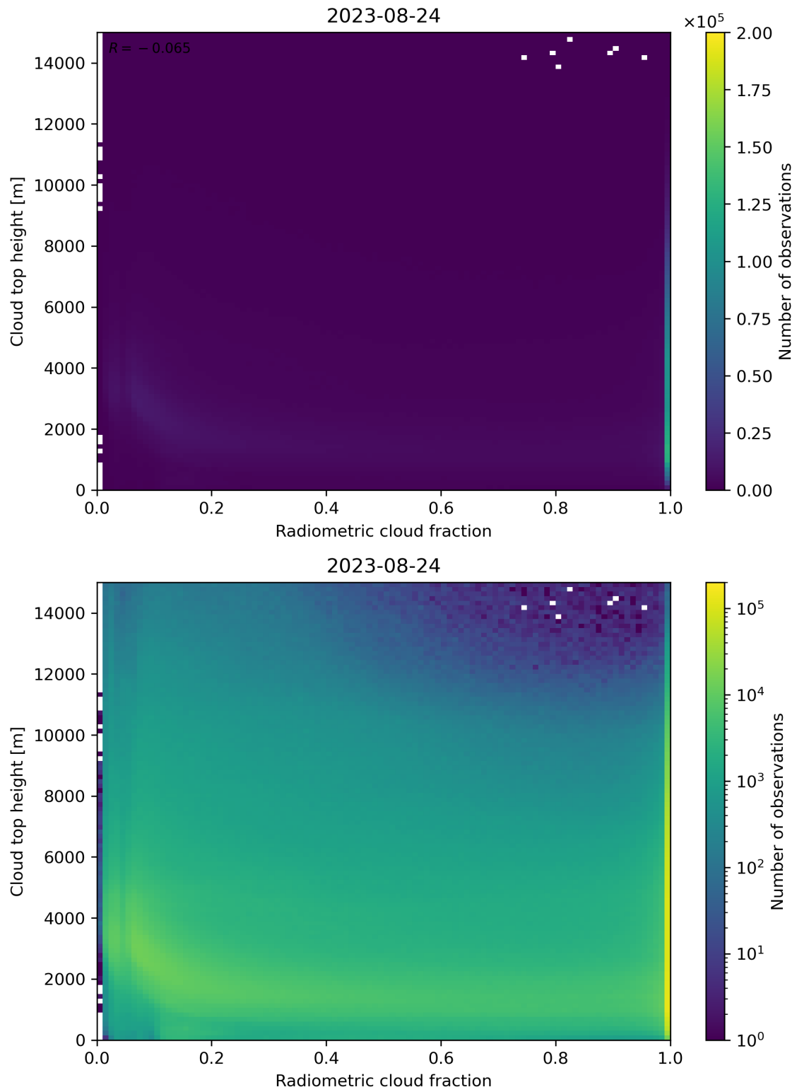
Figure 76: Scatter density plot of “Radiometric cloud fraction” against “Cloud top height” for 2023-08-23 to 2023-08-25.
