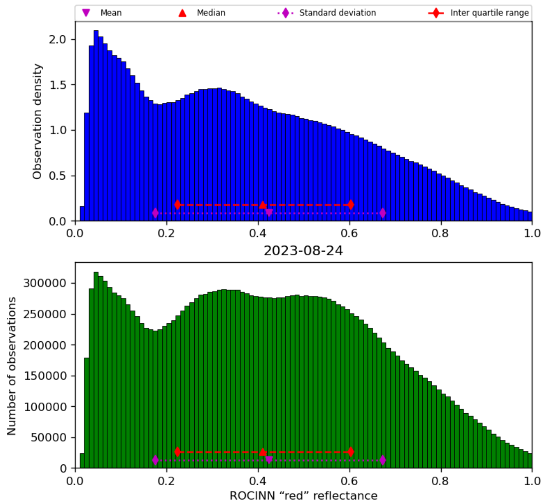
Figure 53: Histogram of "ROCINN "red" reflectance" for 2023-08-23 to 2023-08-25
