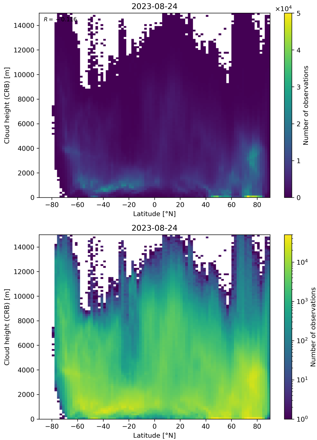
Figure 95: Scatter density plot of “Latitude” against “Cloud height (CRB)” for 2023-08-23 to 2023-08-25.
