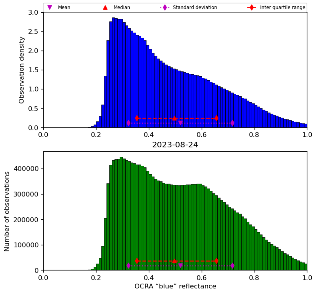
Figure 51: Histogram of “OCRA “blue” reflectance” for 2023-08-23 to 2023-08-25
