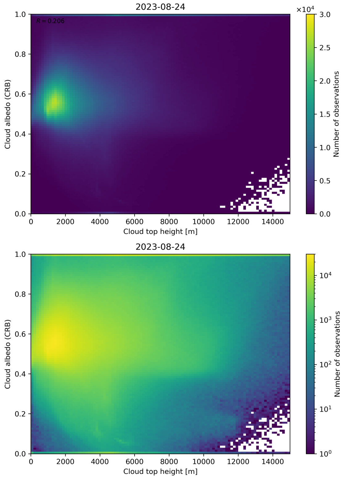
Figure 86: Scatter density plot of “Cloud top height” against “Cloud albedo (CRB)” for 2023-08-23 to 2023-08-25.
