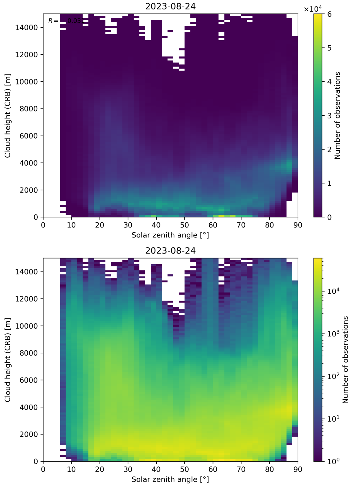
Figure 102: Scatter density plot of “Solar zenith angle” against “Cloud height (CRB)” for 2023-08-23 to 2023-08-25.
