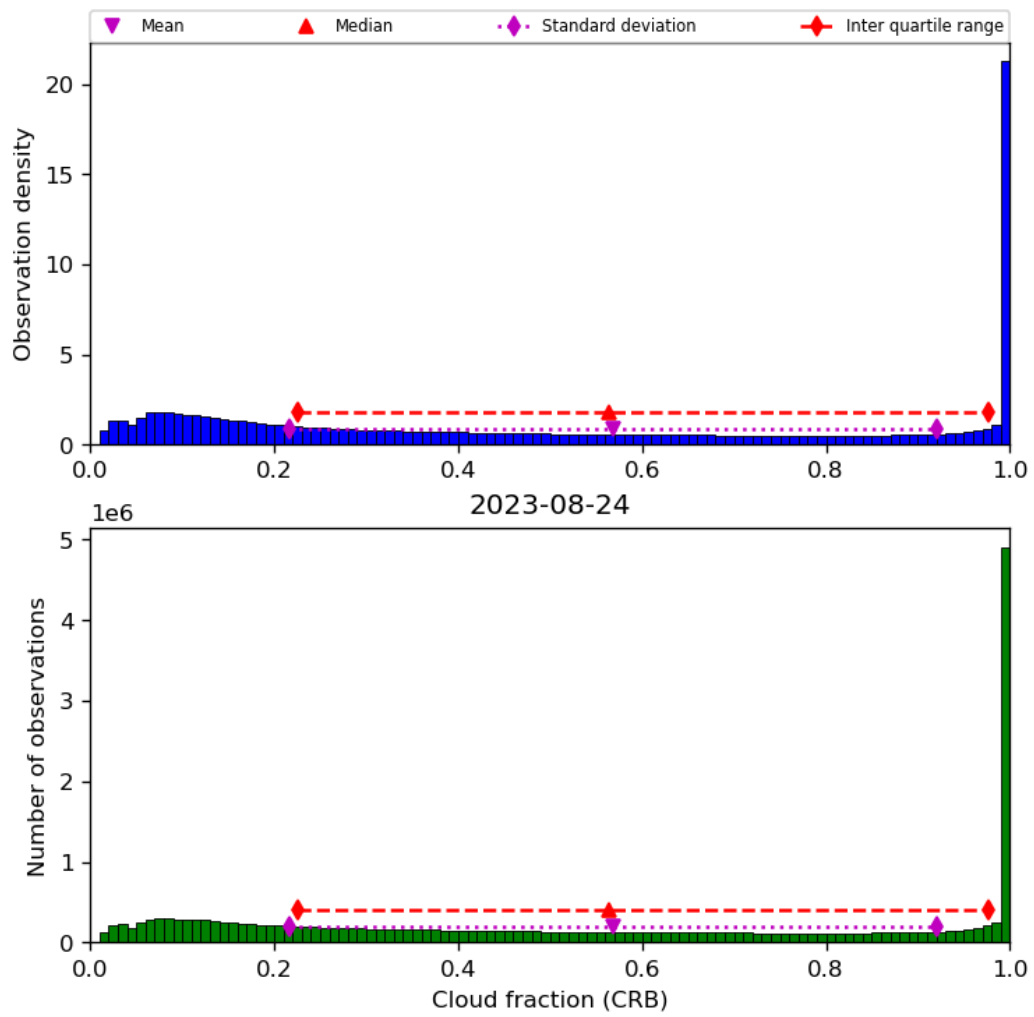
Figure 42: Histogram of “Cloud fraction (CRB)” for 2023-08-23 to 2023-08-25
