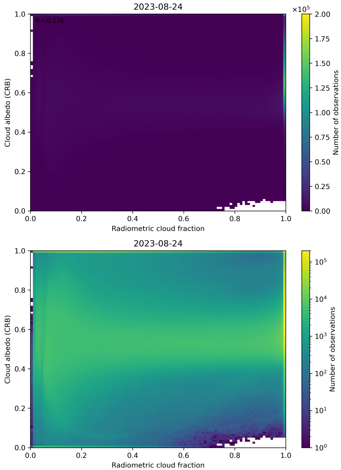
Figure 71: Scatter density plot of “Radiometric cloud fraction” against “Cloud albedo (CRB)” for 2023-08-23 to 2023-08-25.
