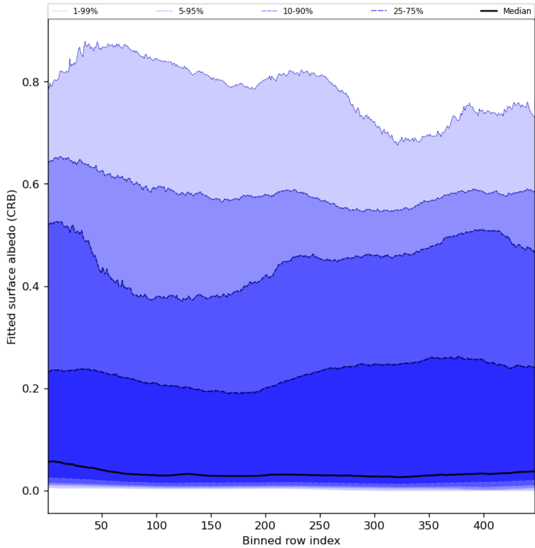
Figure 62: Along track statistics of “Fitted surface albedo (CRB)” for 2023-08-23 to 2023-08-25
