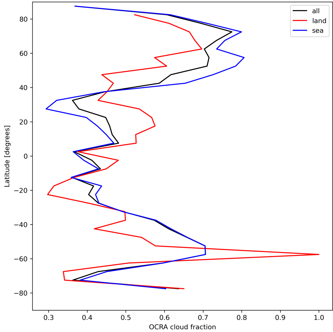
Figure 34: Zonal average of “OCRA cloud fraction” for 2023-08-23 to 2023-08-25.
