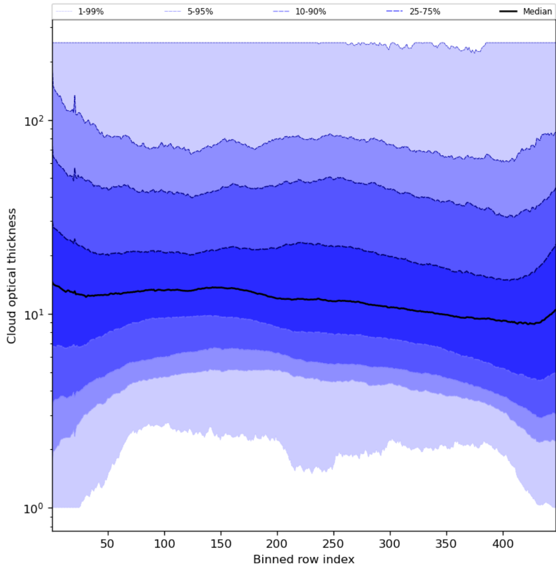
Figure 57: Along track statistics of “Cloud optical thickness” for 2023-08-23 to 2023-08-25
