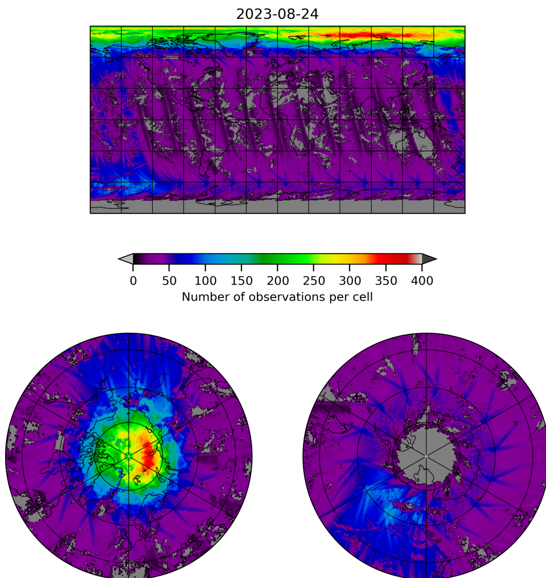
Figure 21: Map of the number of observations for 2023-08-23 to 2023-08-25
