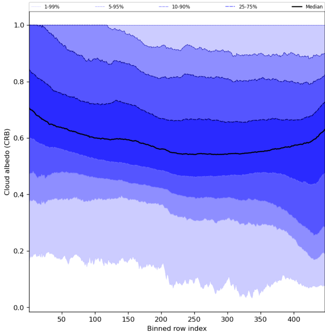
Figure 60: Along track statistics of “Cloud albedo (CRB)” for 2023-08-23 to 2023-08-25
