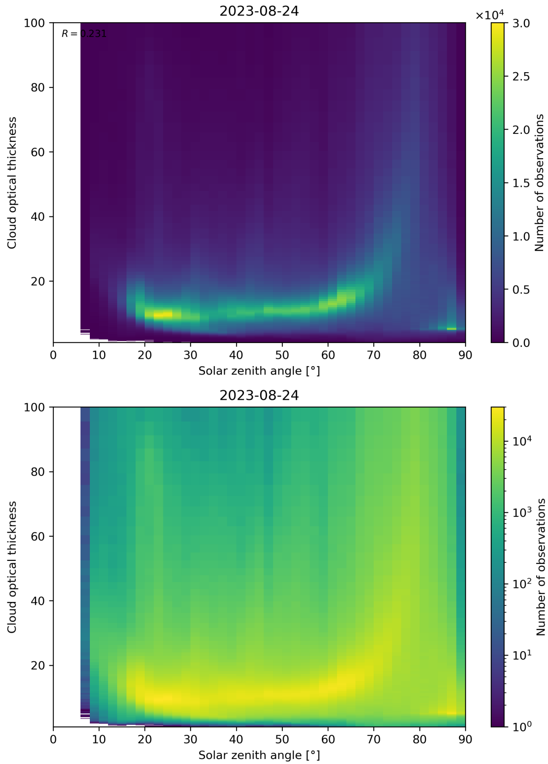
Figure 103: Scatter density plot of “Solar zenith angle” against “Cloud optical thickness” for 2023-08-23 to 2023-08-25.
