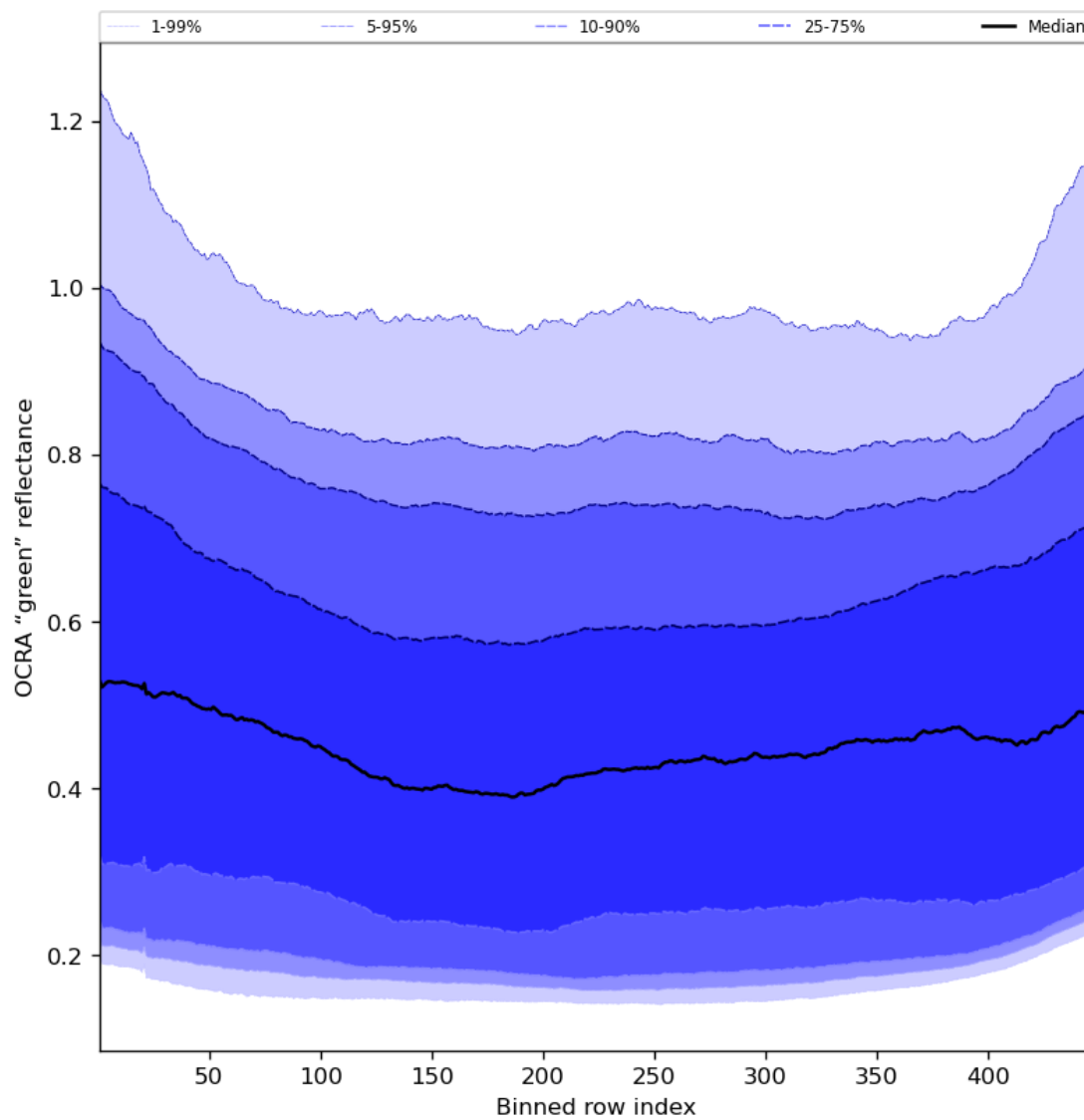
Figure 68: Along track statistics of “OCRA “green” reflectance” for 2023-08-23 to 2023-08-25
