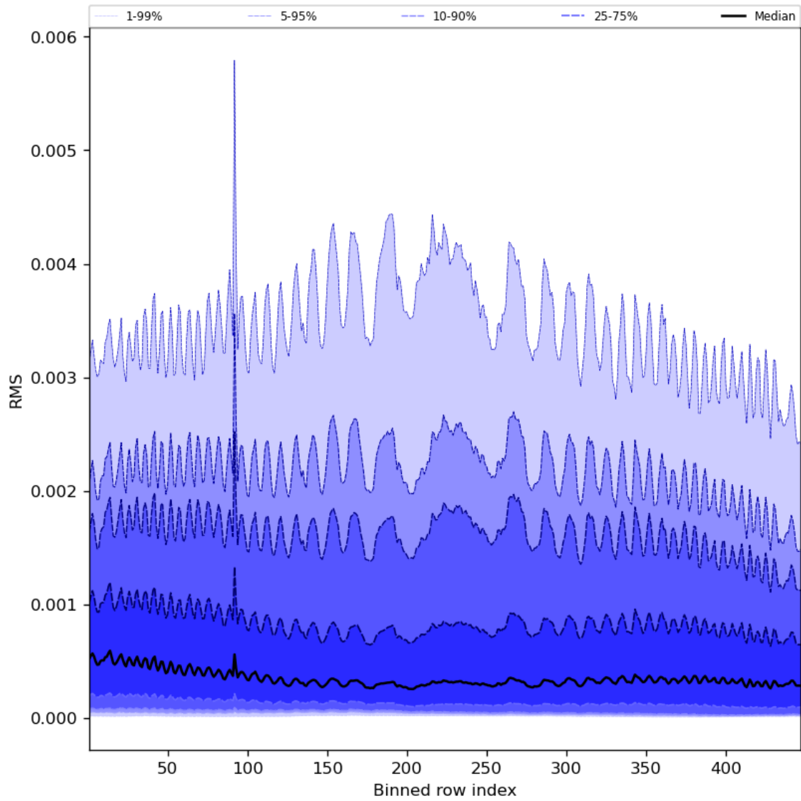
Figure 63: Along track statistics of “RMS” for 2023-08-23 to 2023-08-25
