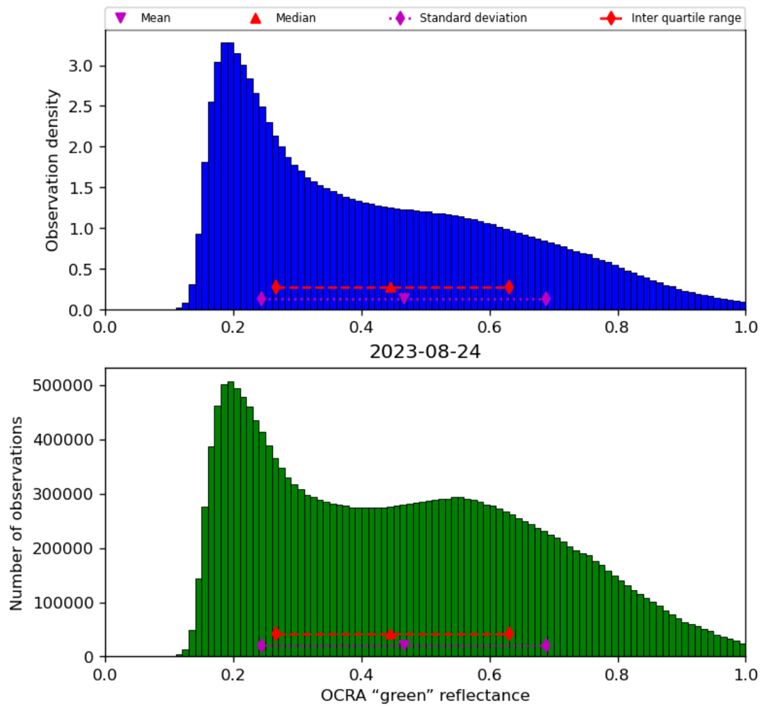
Figure 52: Histogram of “OCRA “green” reflectance” for 2023-08-23 to 2023-08-25
