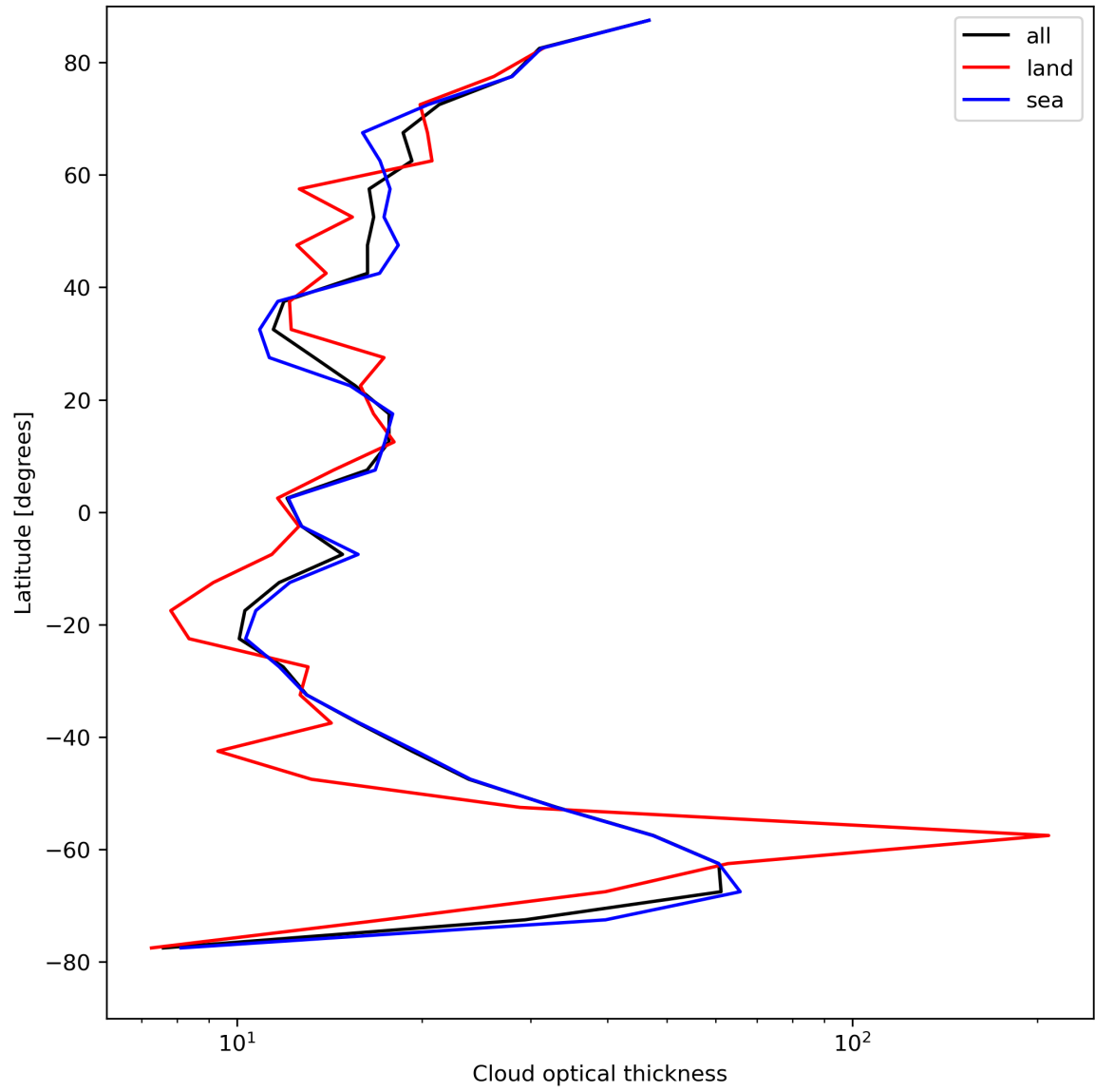
Figure 25: Zonal average of “Cloud optical thickness” for 2023-08-23 to 2023-08-25.
