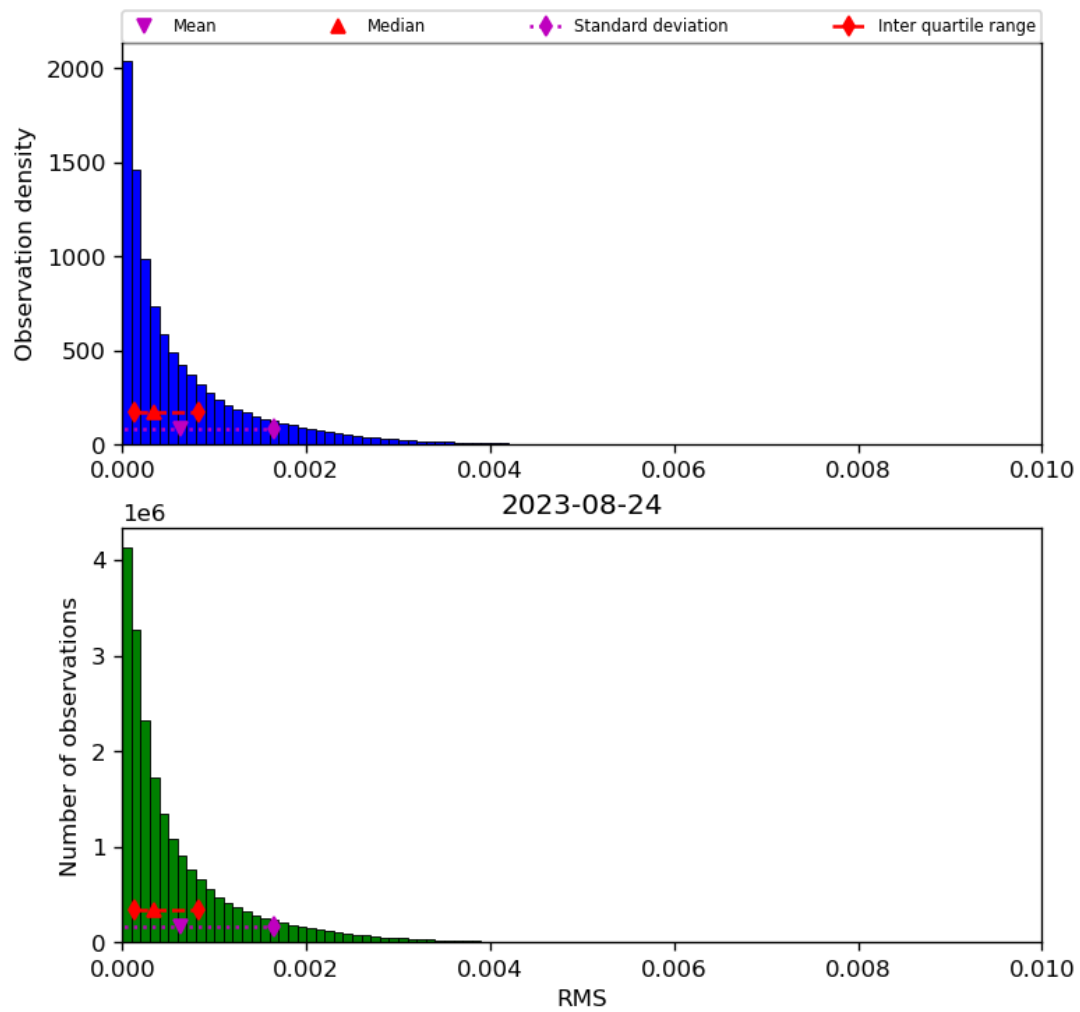
Figure 47: Histogram of “RMS” for 2023-08-23 to 2023-08-25
