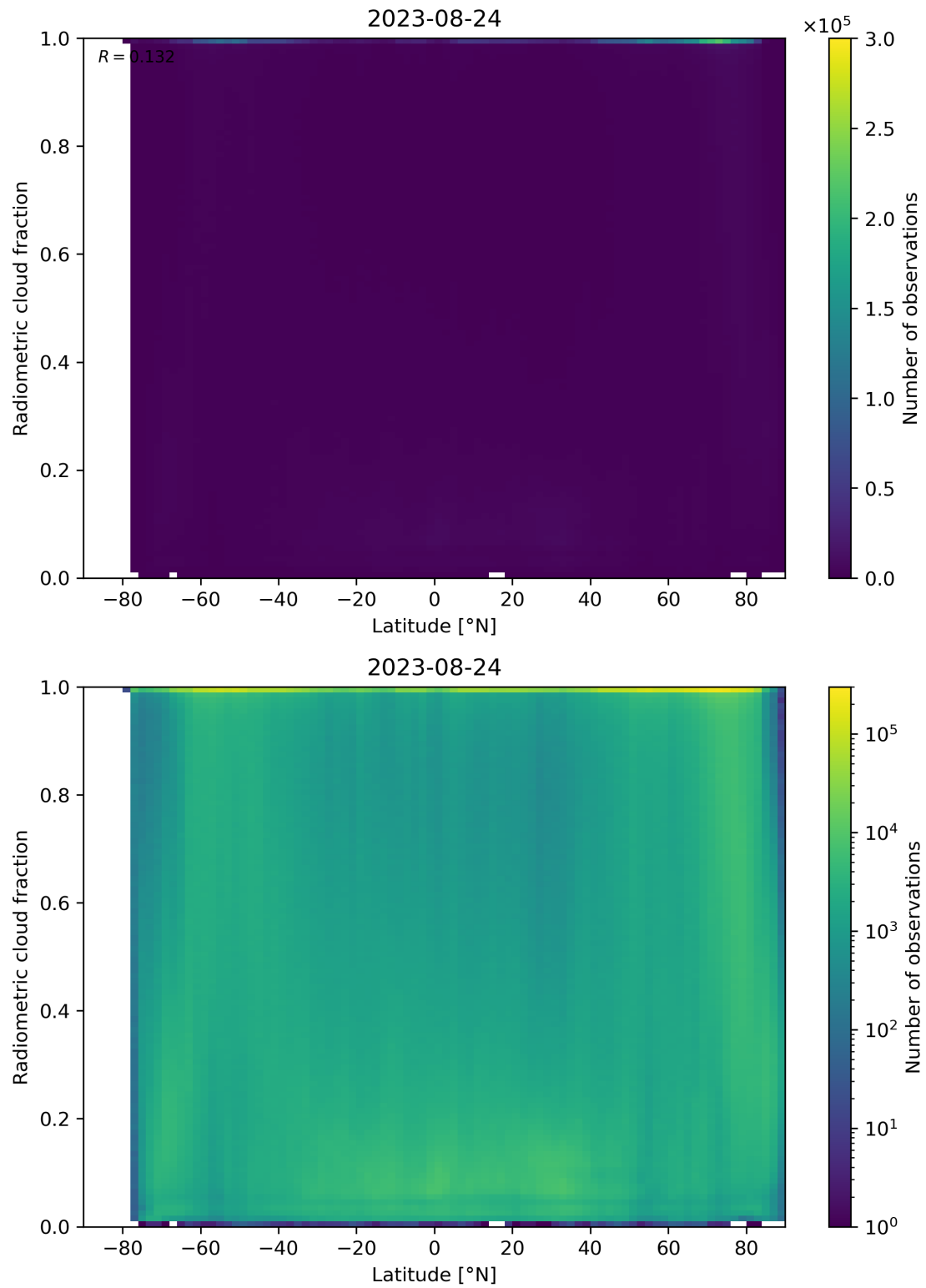
Figure 92: Scatter density plot of “Latitude” against “Radiometric cloud fraction” for 2023-08-23 to 2023-08-25.
