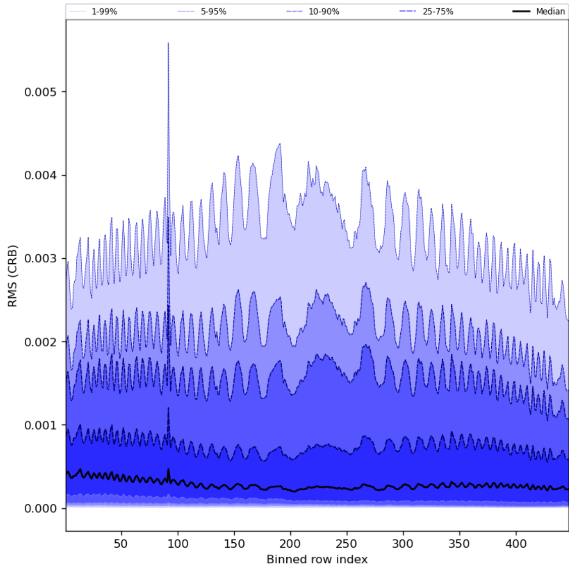
Figure 64: Along track statistics of “RMS (CRB)” for 2023-08-23 to 2023-08-25
