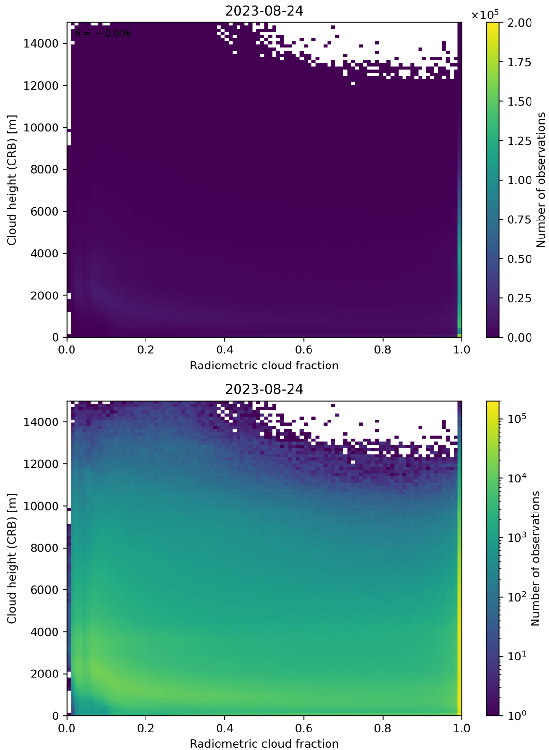
Figure 74: Scatter density plot of “Radiometric cloud fraction” against “Cloud height (CRB)” for 2023-08-23 to 2023-08-25.
