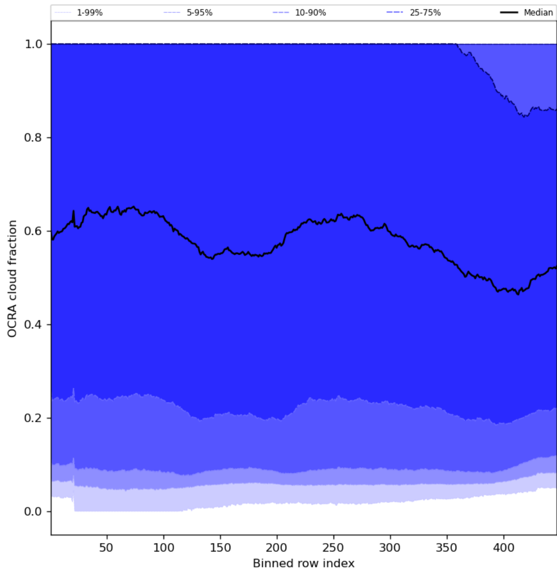
Figure 66: Along track statistics of “OCRA cloud fraction” for 2023-08-23 to 2023-08-25
