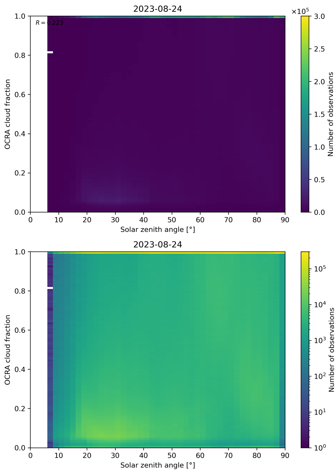
Figure 100: Scatter density plot of “Solar zenith angle” against “OCRA cloud fraction” for 2023-08-23 to 2023-08-25.
