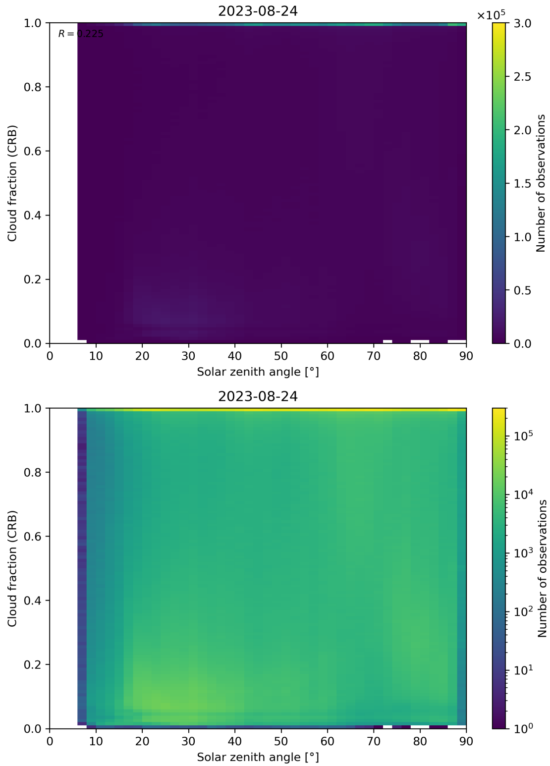
Figure 101: Scatter density plot of “Solar zenith angle” against “Cloud fraction (CRB)” for 2023-08-23 to 2023-08-25.
