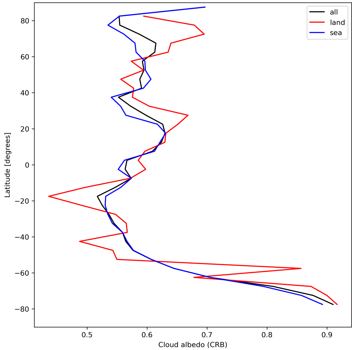
Figure 28: Zonal average of “Cloud albedo (CRB)” for 2023-08-23 to 2023-08-25.
