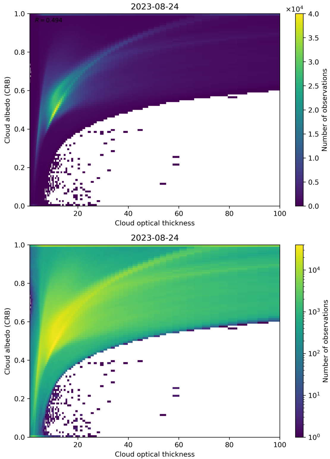
Figure 82: Scatter density plot of “Cloud optical thickness” against “Cloud albedo (CRB)” for 2023-08-23 to 2023-08-25.
