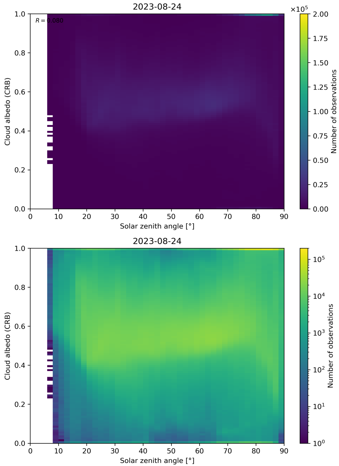
Figure 98: Scatter density plot of “Solar zenith angle” against “Cloud albedo (CRB)” for 2023-08-23 to 2023-08-25.
