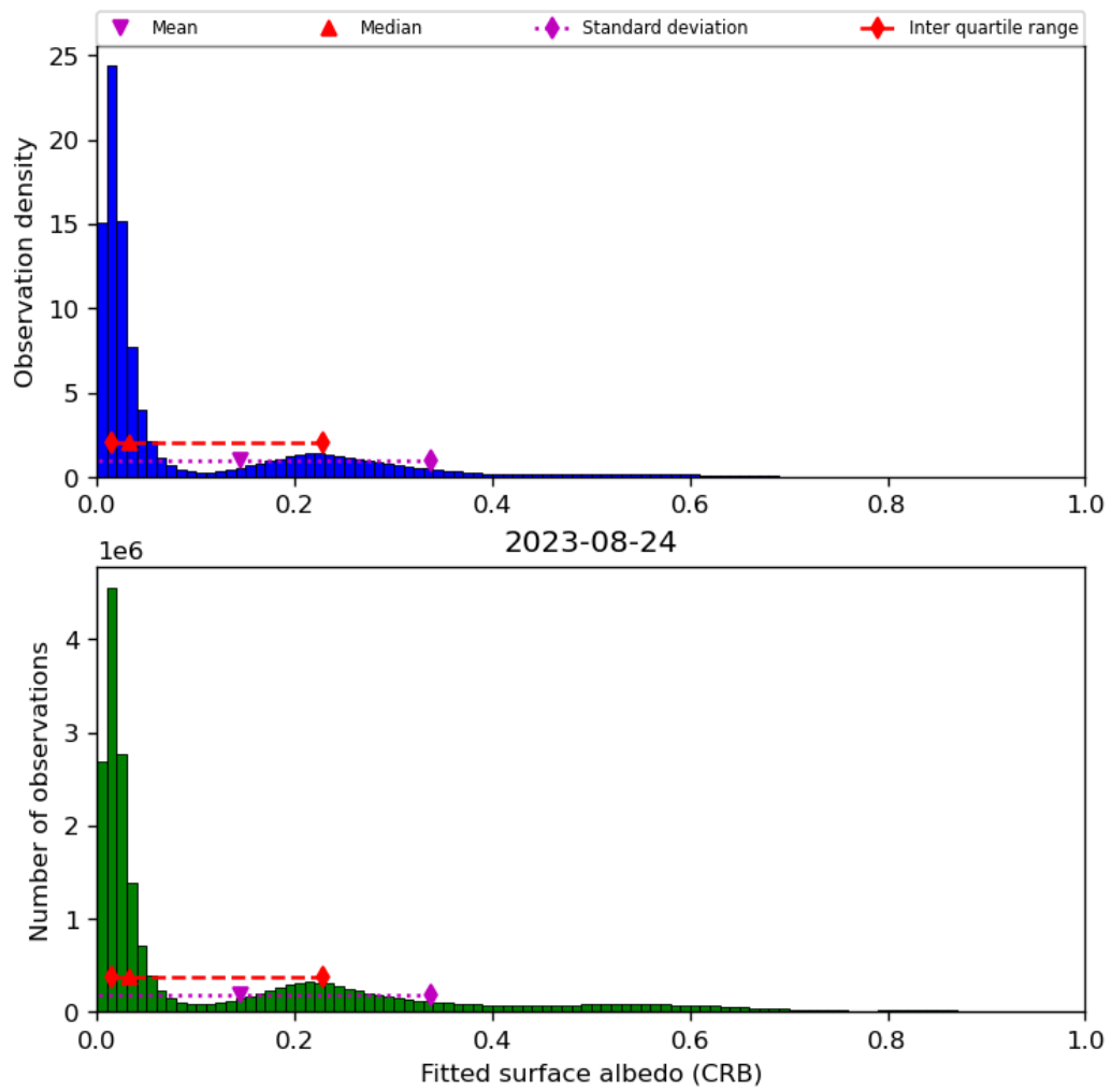
Figure 46: Histogram of “Fitted surface albedo (CRB)” for 2023-08-23 to 2023-08-25
