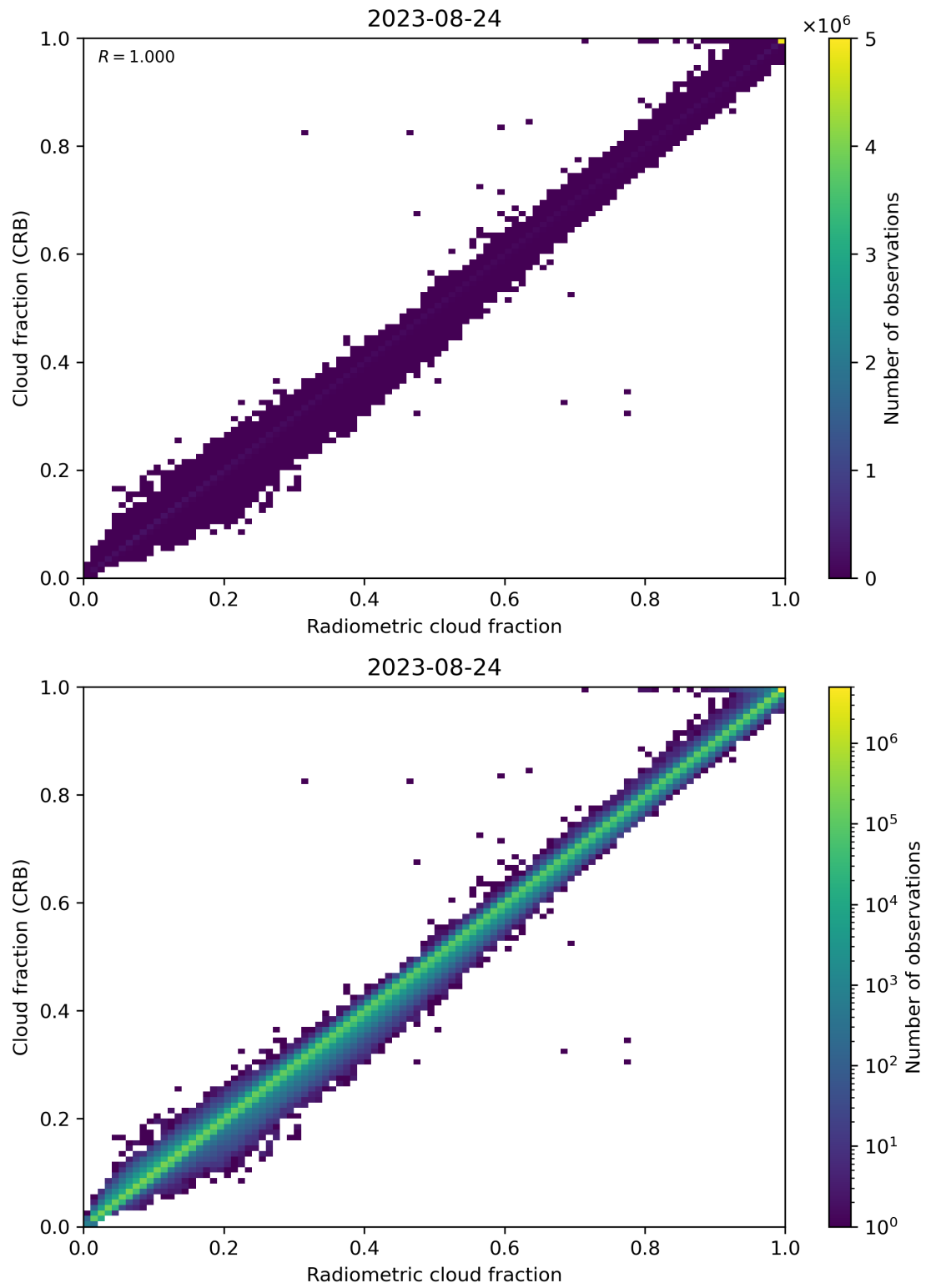
Figure 73: Scatter density plot of “Radiometric cloud fraction” against “Cloud fraction (CRB)” for 2023-08-23 to 2023-08-25.
