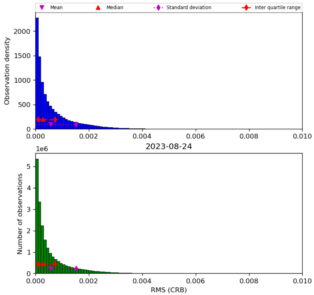
Figure 48: Histogram of “RMS (CRB)” for 2023-08-23 to 2023-08-25
