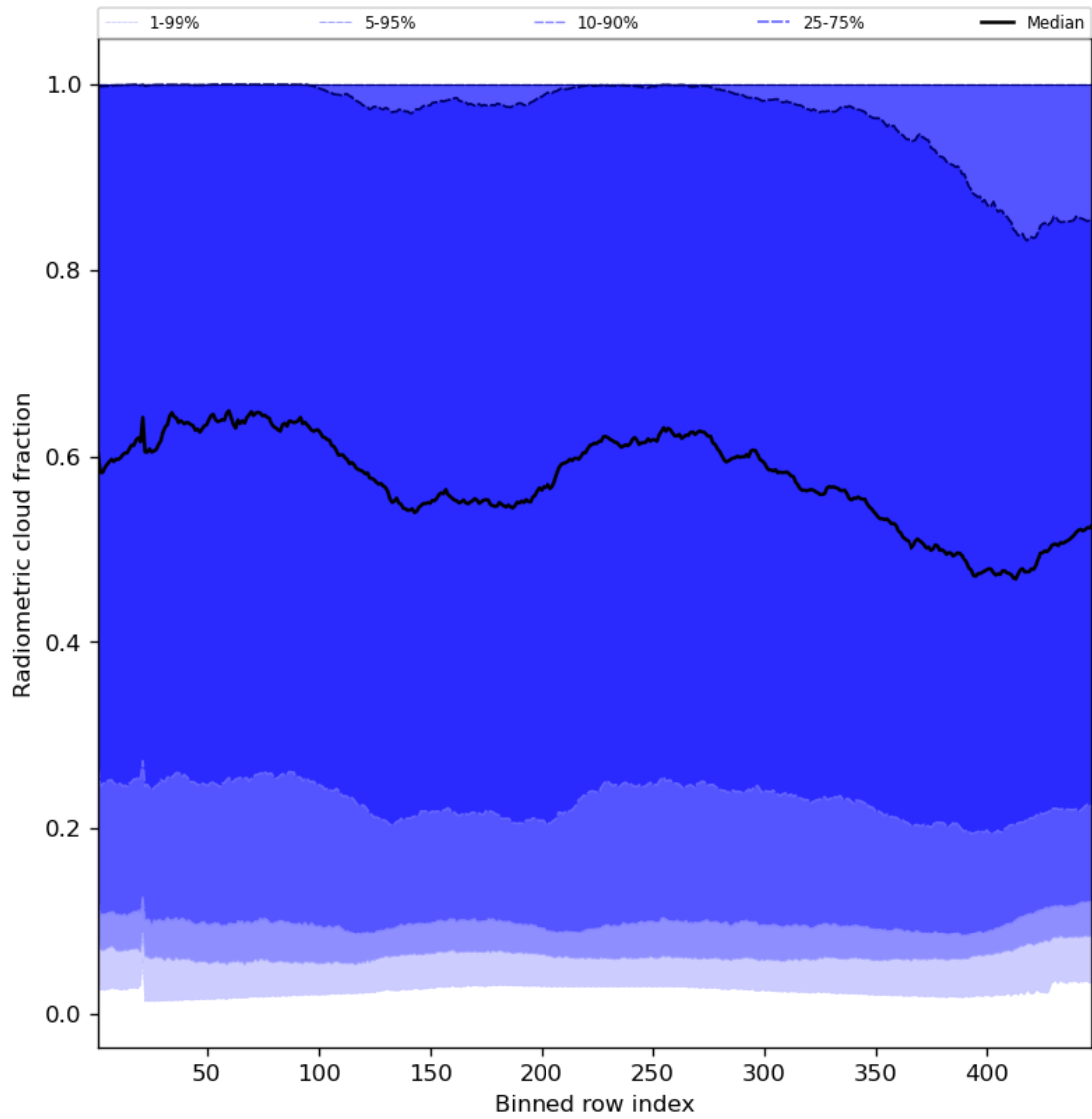
Figure 55: Along track statistics of “Radiometric cloud fraction” for 2023-08-23 to 2023-08-25
