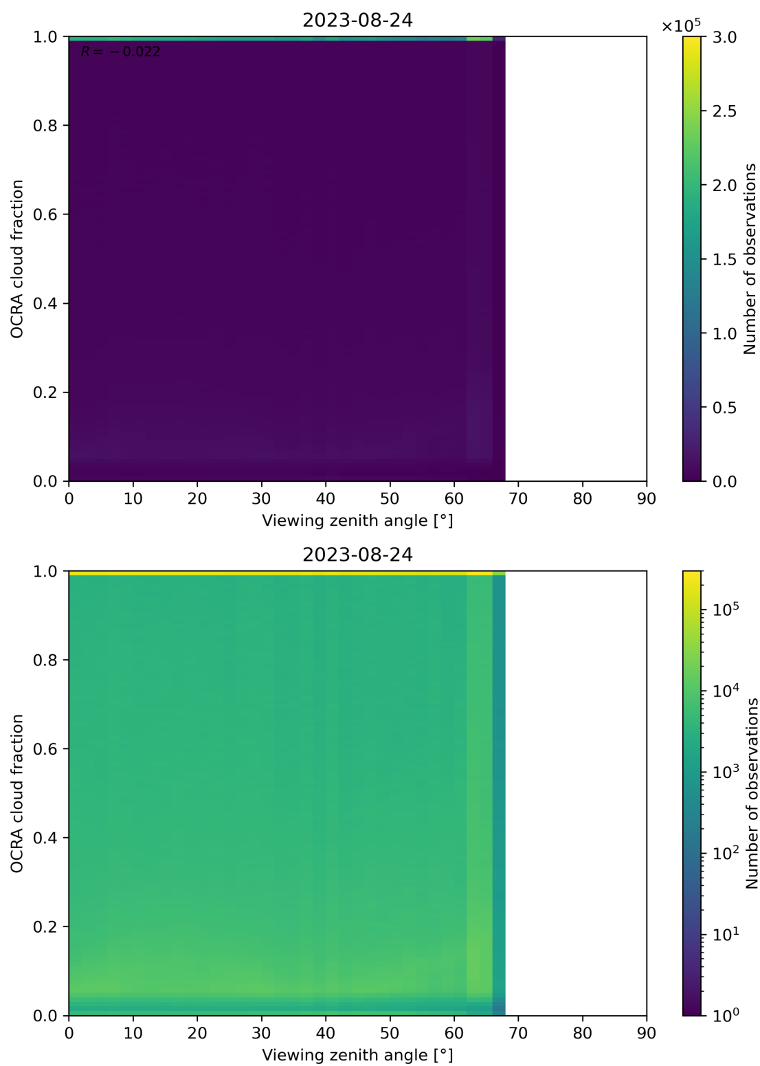
Figure 108: Scatter density plot of “Viewing zenith angle” against “OCRA cloud fraction” for 2023-08-23 to 2023-08-25.
