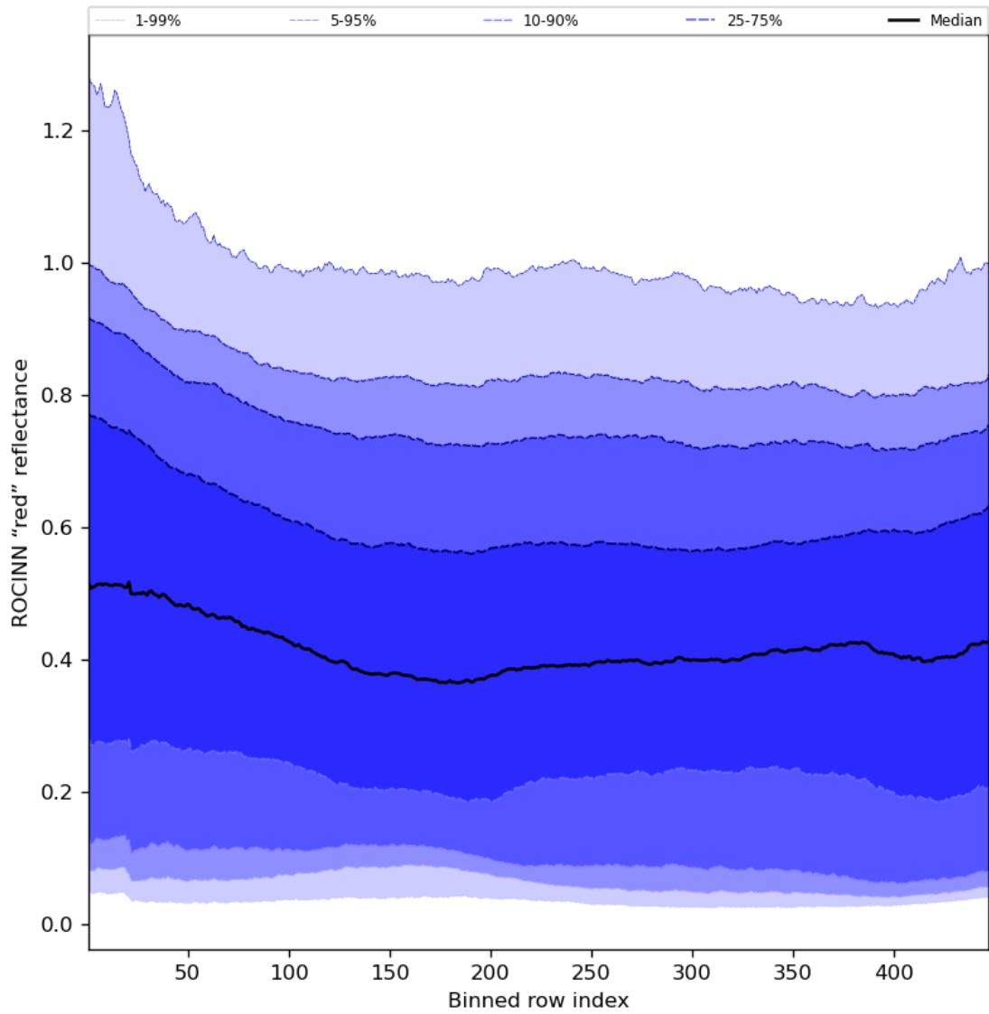
Figure 69: Along track statistics of “ROCINN “red” reflectance” for 2023-08-23 to 2023-08-25
