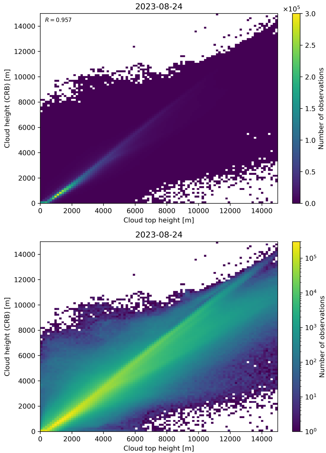
Figure 89: Scatter density plot of “Cloud top height” against “Cloud height (CRB)” for 2023-08-23 to 2023-08-25.
