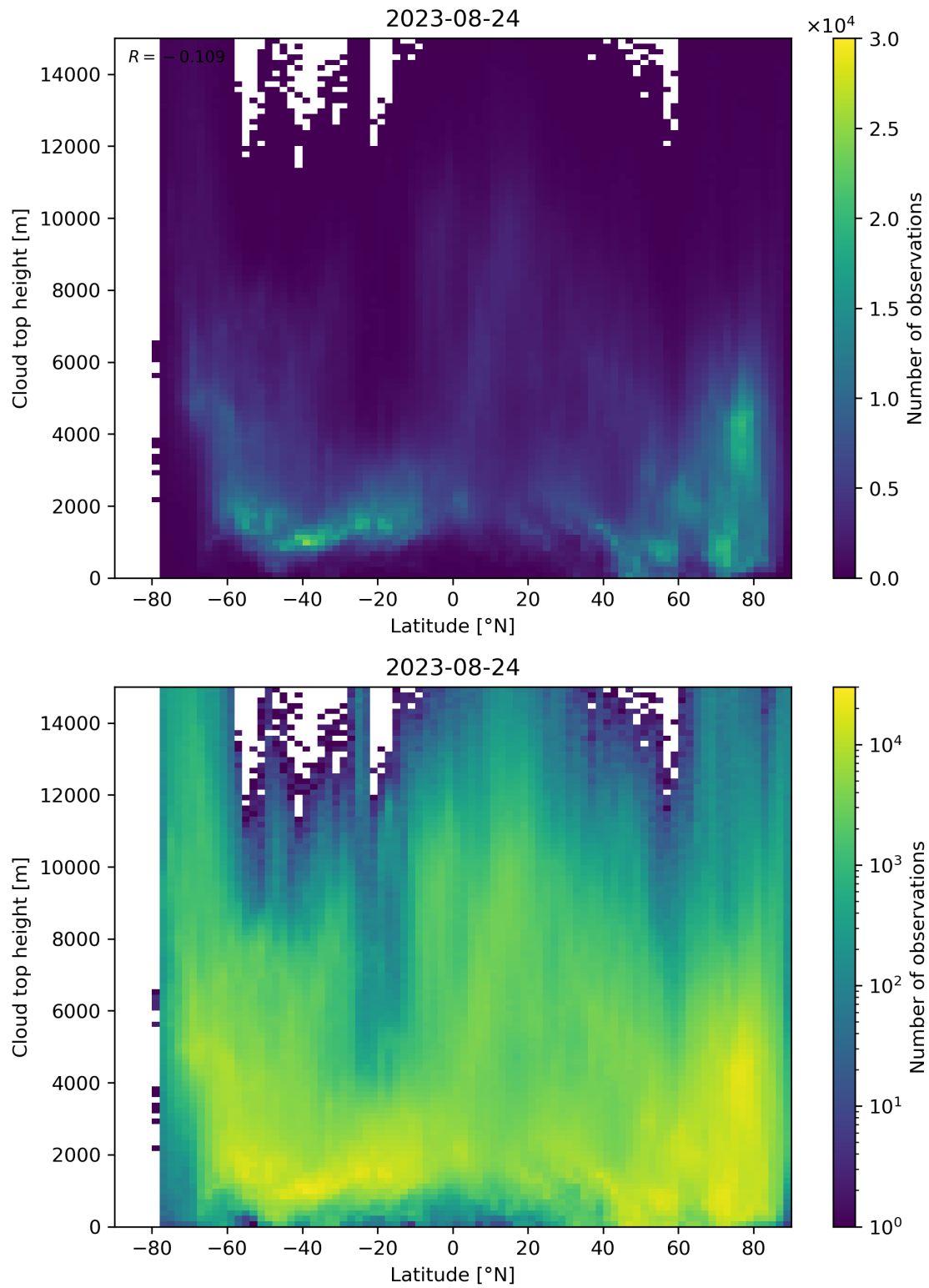
Figure 97: Scatter density plot of “Latitude” against “Cloud top height” for 2023-08-23 to 2023-08-25.
