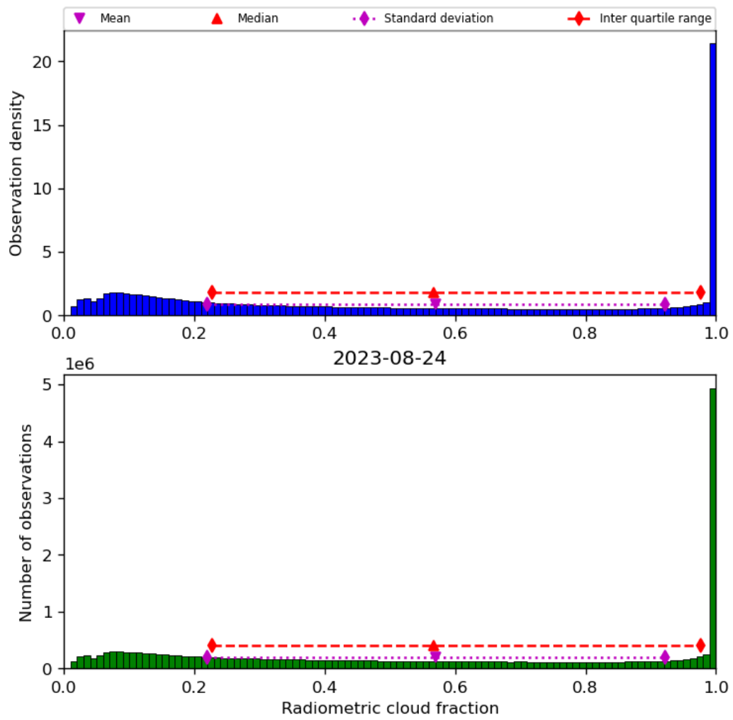
Figure 39: Histogram of “Radiometric cloud fraction” for 2023-08-23 to 2023-08-25
