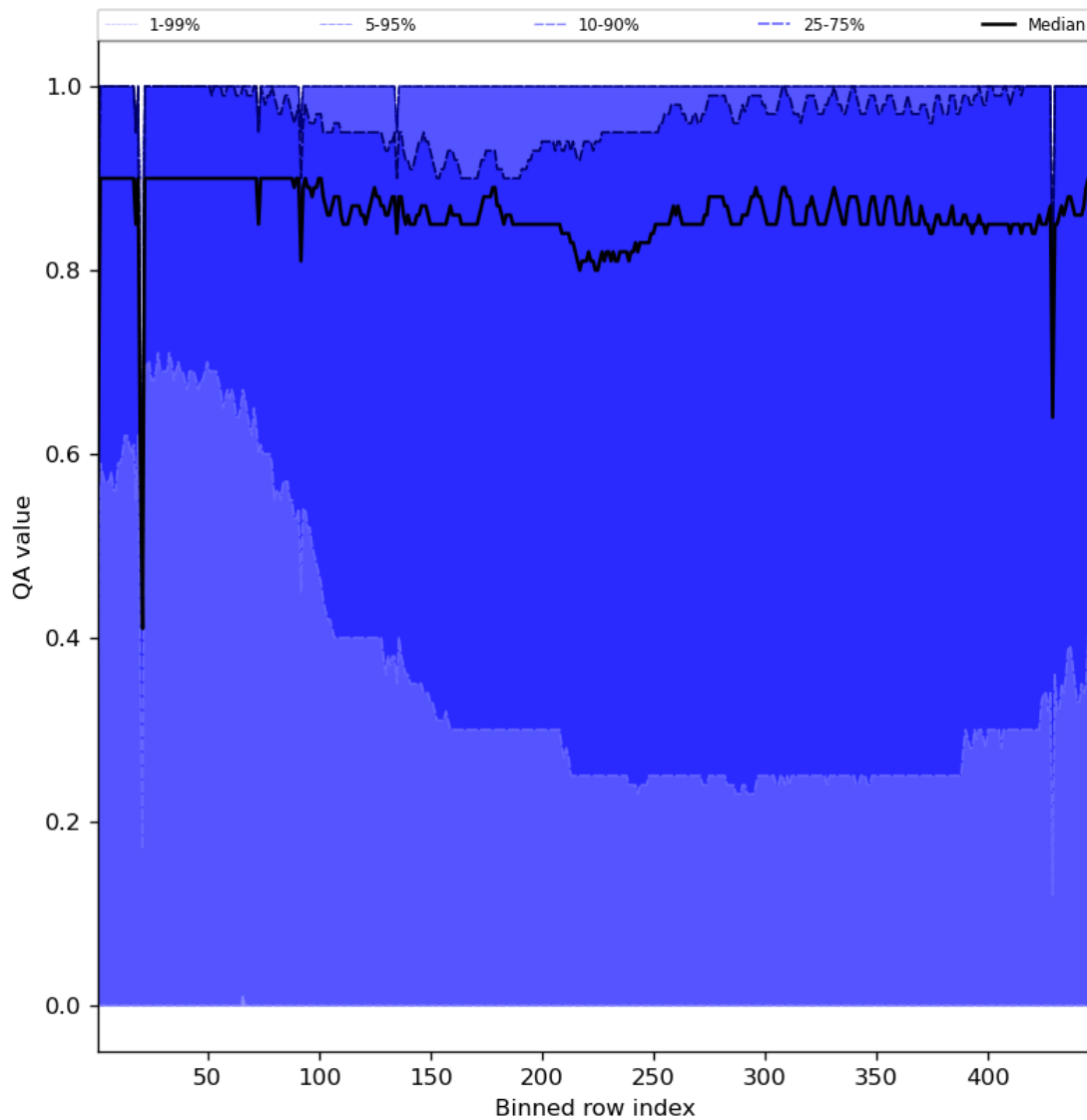
Figure 54: Along track statistics of “QA value” for 2023-08-23 to 2023-08-25
