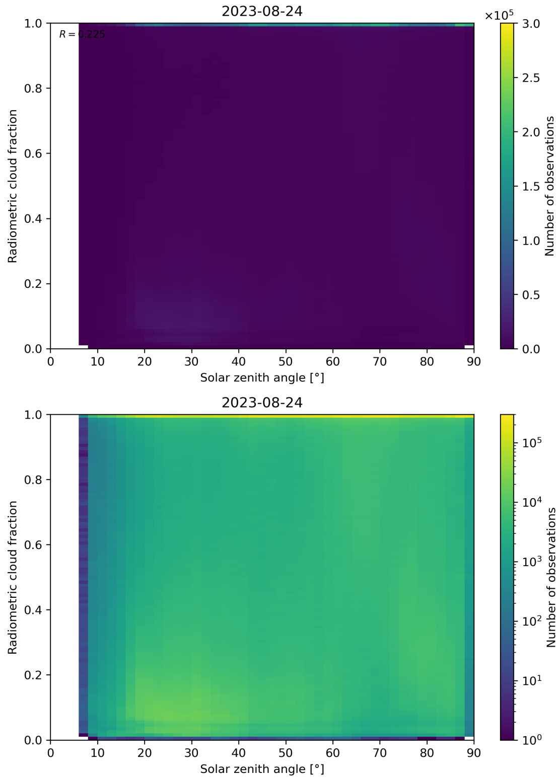
Figure 99: Scatter density plot of “Solar zenith angle” against “Radiometric cloud fraction” for 2023-08-23 to 2023-08-25.
