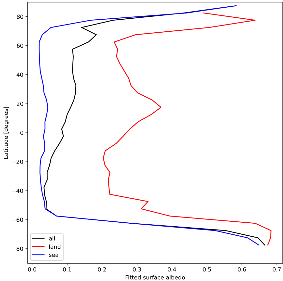
Figure 29: Zonal average of “Fitted surface albedo” for 2023-08-23 to 2023-08-25.
