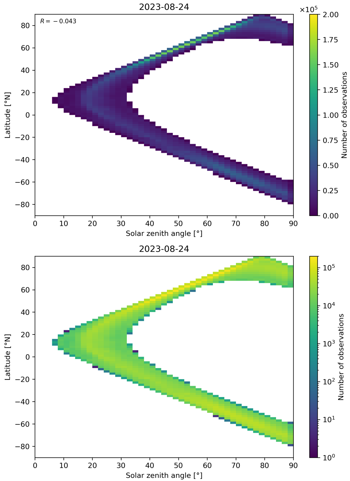
Figure 105: Scatter density plot of “Solar zenith angle” against “Latitude” for 2023-08-23 to 2023-08-25.
