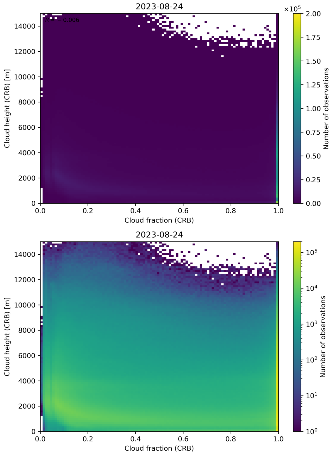
Figure 79: Scatter density plot of “Cloud fraction (CRB)” against “Cloud height (CRB)” for 2023-08-23 to 2023-08-25.
