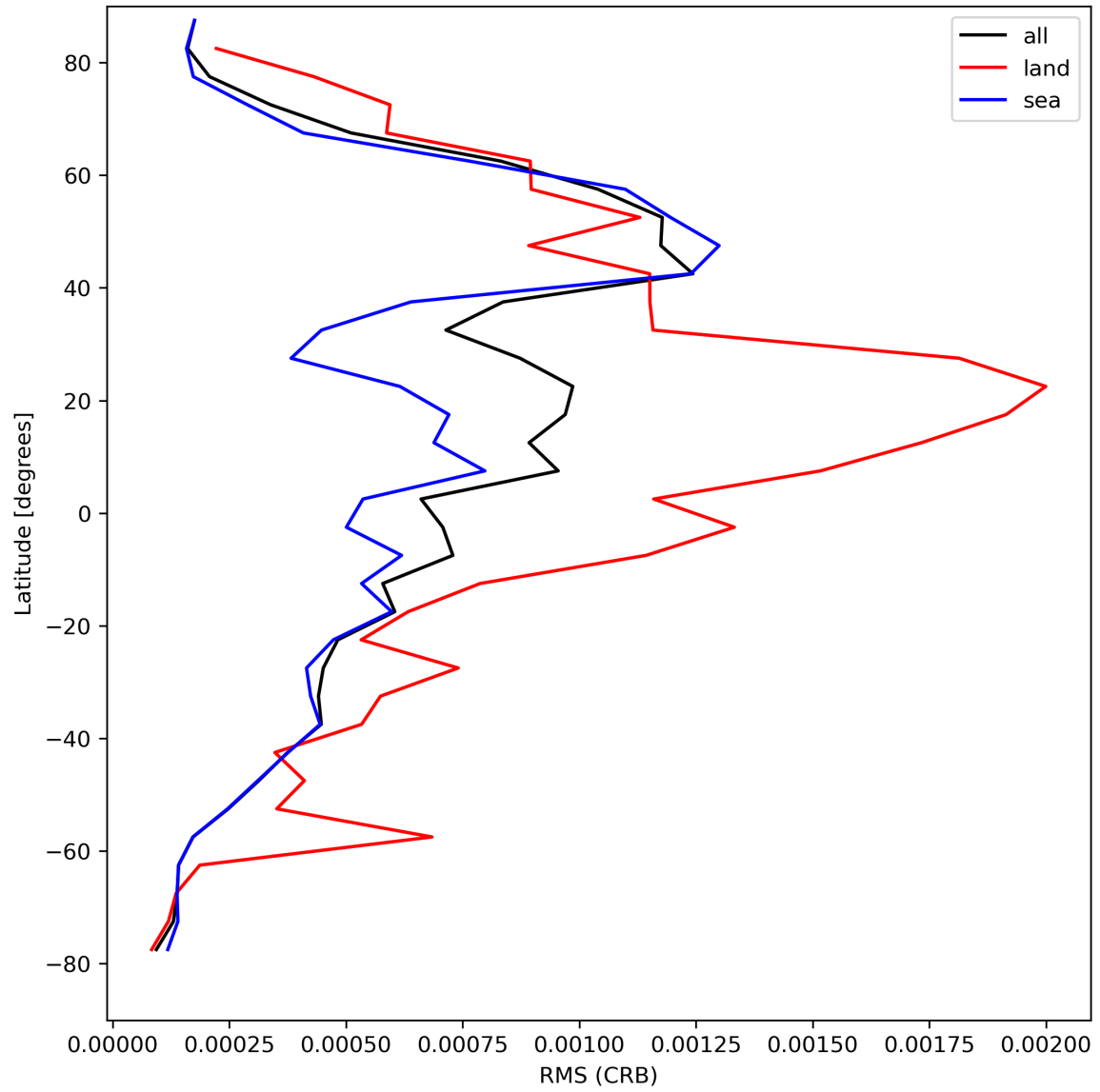
Figure 32: Zonal average of “RMS (CRB)” for 2023-08-23 to 2023-08-25.
