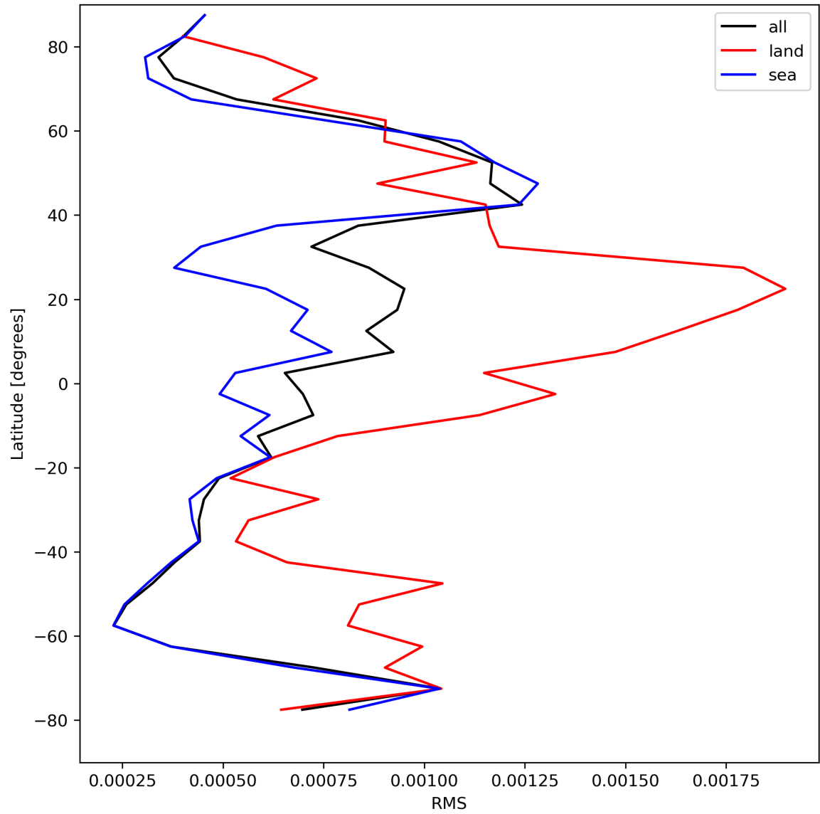
Figure 31: Zonal average of “RMS” for 2023-08-23 to 2023-08-25.
