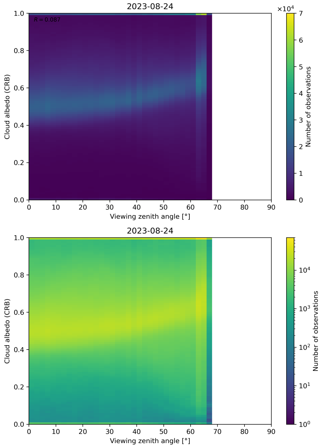
Figure 106: Scatter density plot of “Viewing zenith angle” against “Cloud albedo (CRB)” for 2023-08-23 to 2023-08-25.
