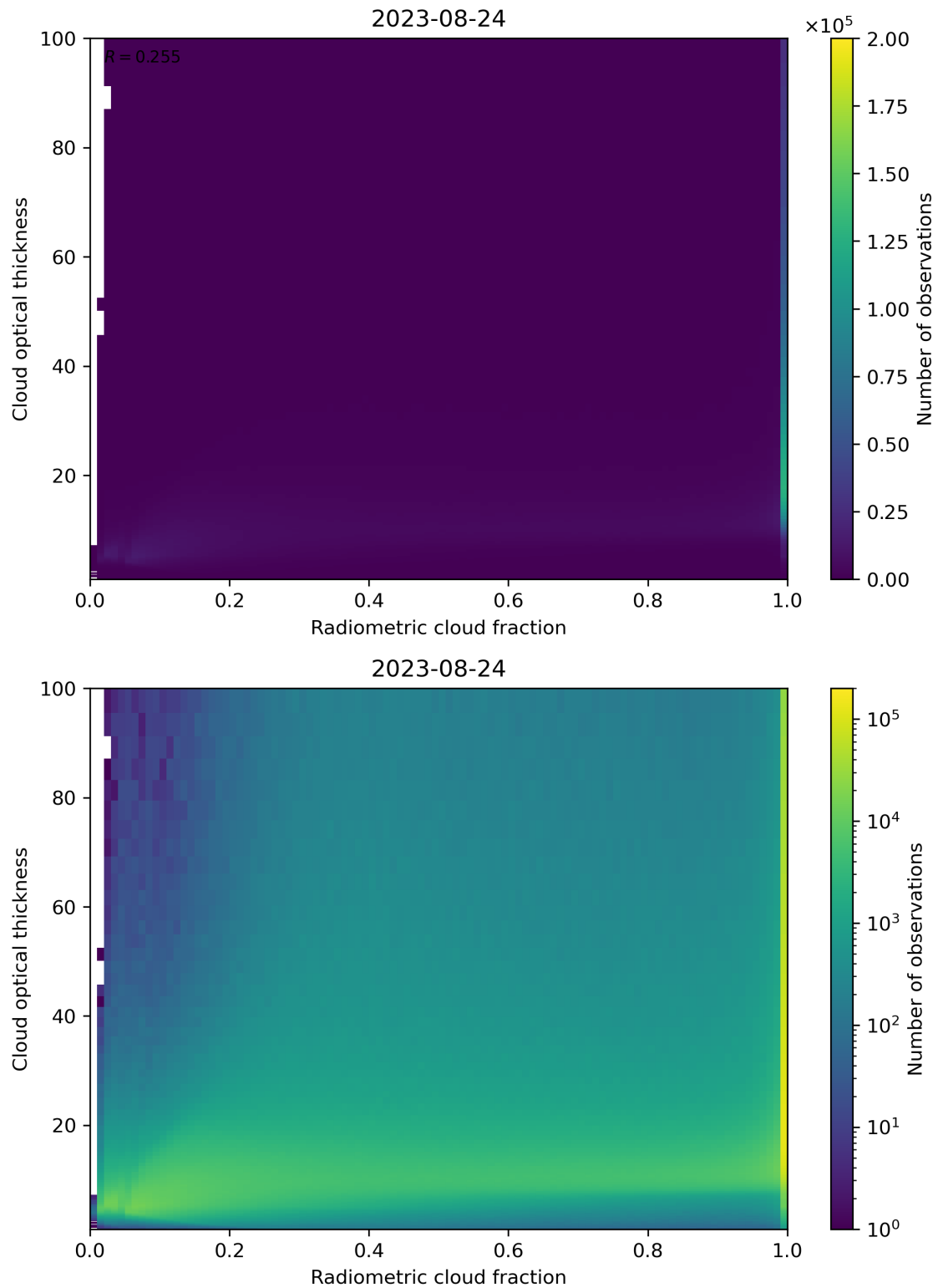
Figure 75: Scatter density plot of “Radiometric cloud fraction” against “Cloud optical thickness” for 2023-08-23 to 2023-08-25.
