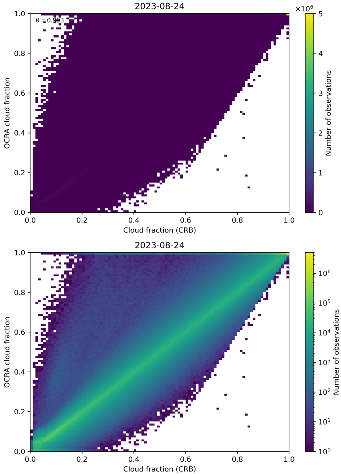
Figure 78: Scatter density plot of “Cloud fraction (CRB)” against “OCRA cloud fraction” for 2023-08-23 to 2023-08-25.
