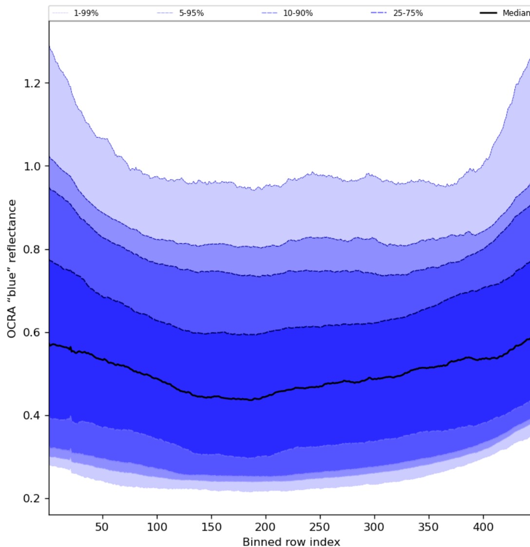
Figure 67: Along track statistics of “OCRA “blue” reflectance” for 2023-08-23 to 2023-08-25
