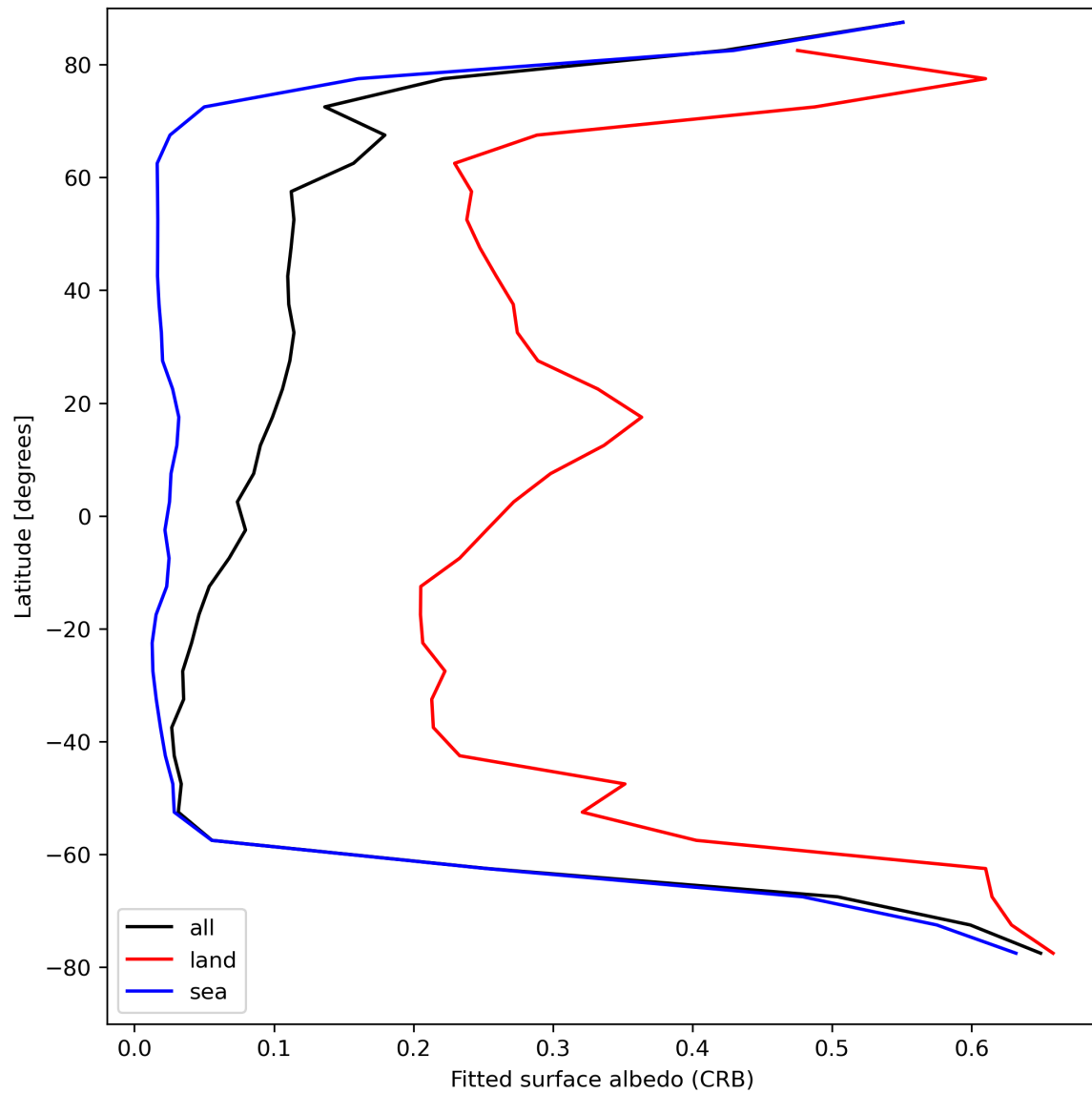
Figure 30: Zonal average of “Fitted surface albedo (CRB)” for 2023-08-23 to 2023-08-25.
