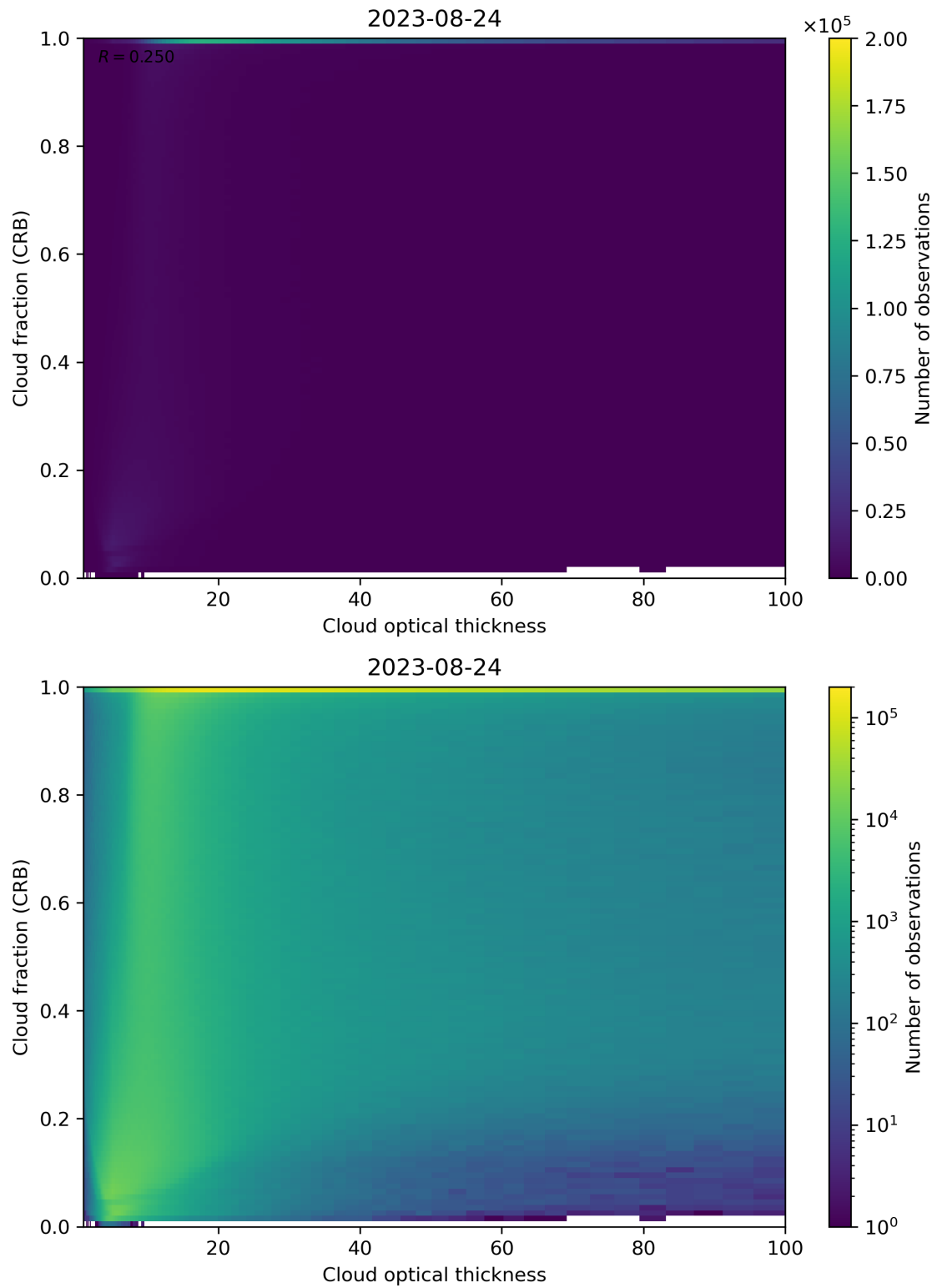
Figure 84: Scatter density plot of “Cloud optical thickness” against “Cloud fraction (CRB)” for 2023-08-23 to 2023-08-25.
