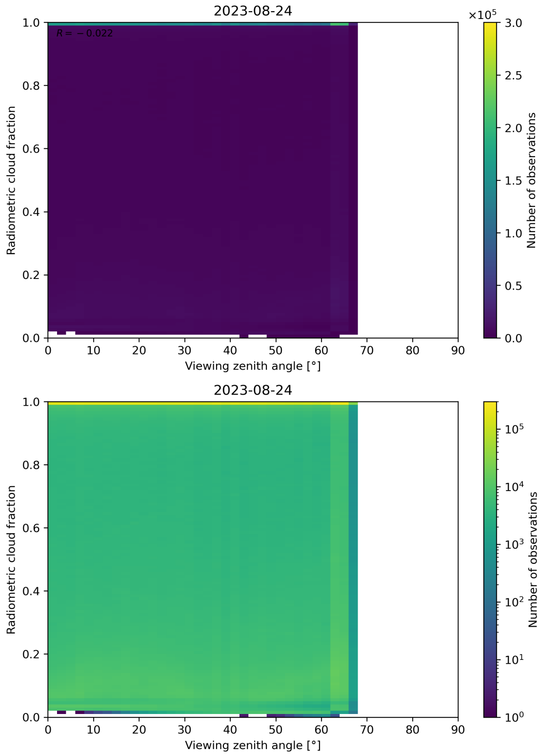
Figure 107: Scatter density plot of “Viewing zenith angle” against “Radiometric cloud fraction” for 2023-08-23 to 2023-08-25.
