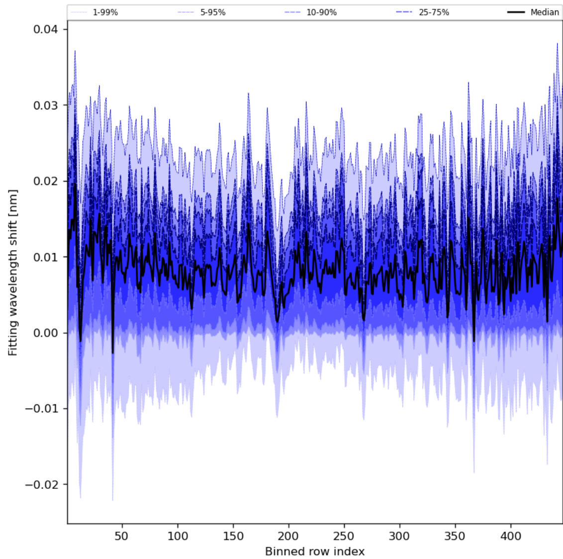
Figure 65: Along track statistics of “Fitting wavelength shift” for 2023-08-23 to 2023-08-25
