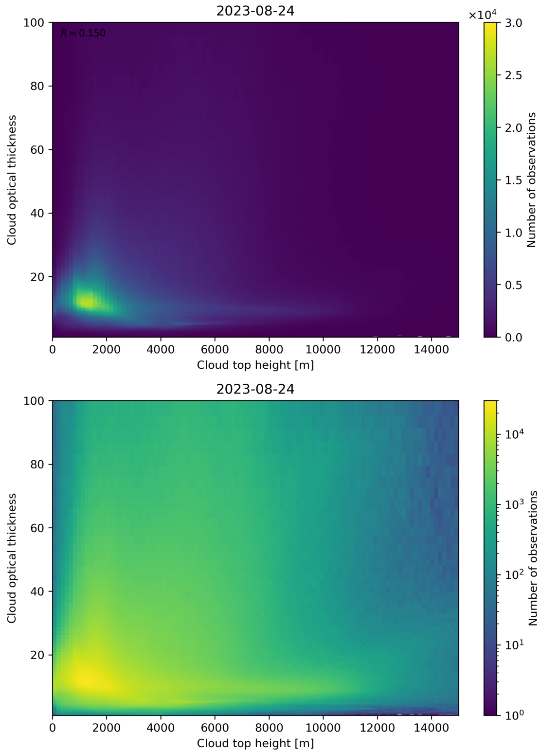
Figure 90: Scatter density plot of “Cloud top height” against “Cloud optical thickness” for 2023-08-23 to 2023-08-25.
