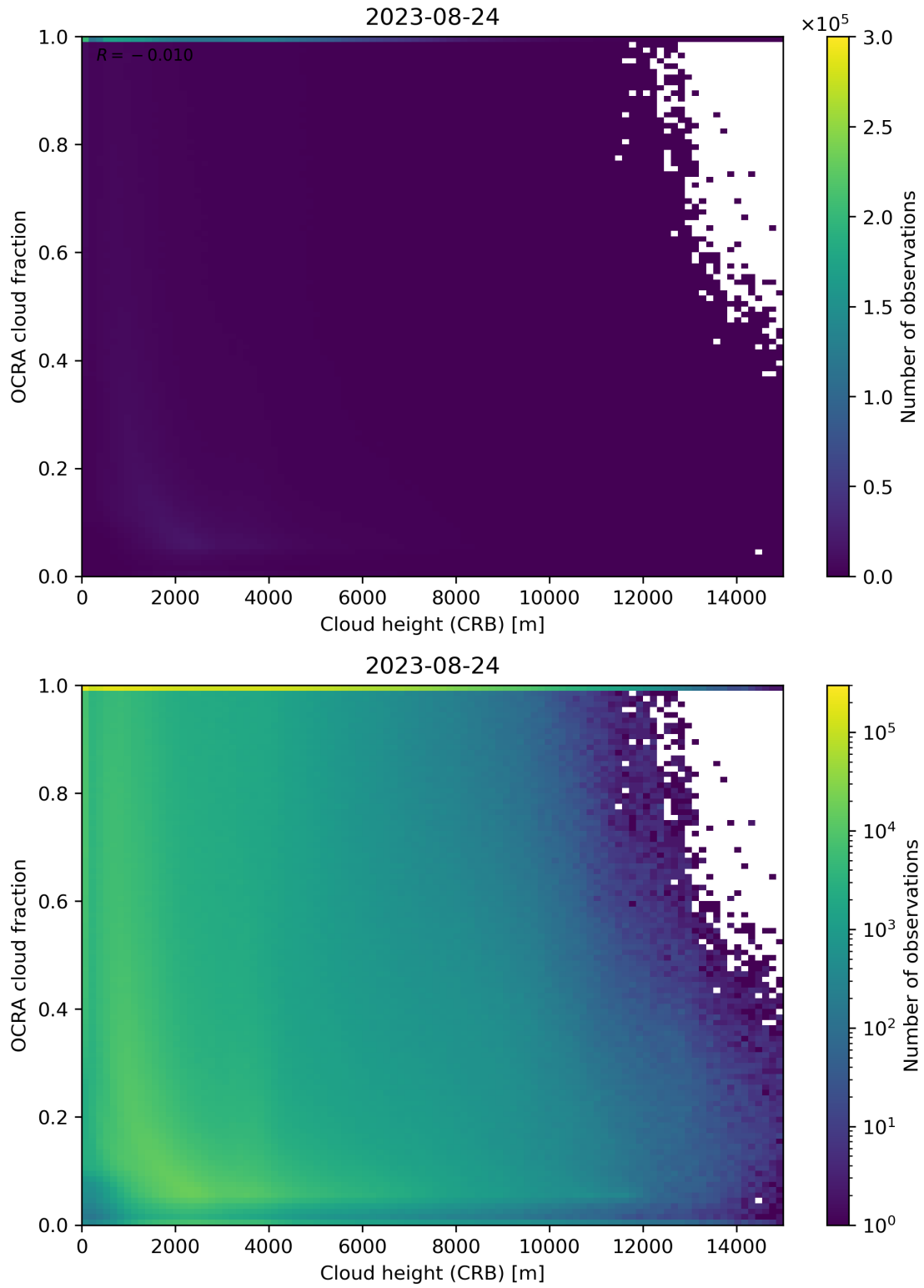
Figure 81: Scatter density plot of “Cloud height (CRB)” against “OCRA cloud fraction” for 2023-08-23 to 2023-08-25.
