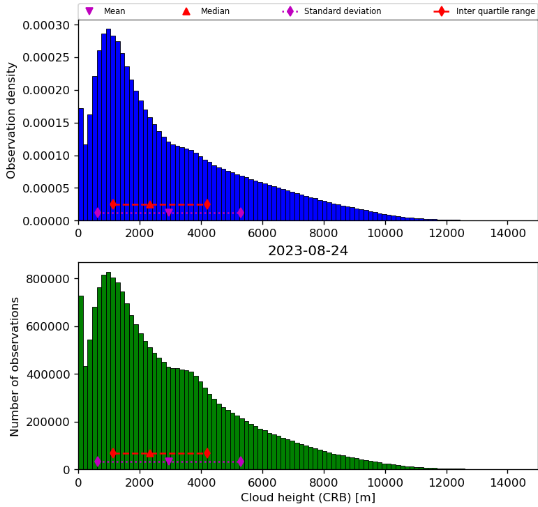
Figure 43: Histogram of “Cloud height (CRB)” for 2023-08-23 to 2023-08-25
