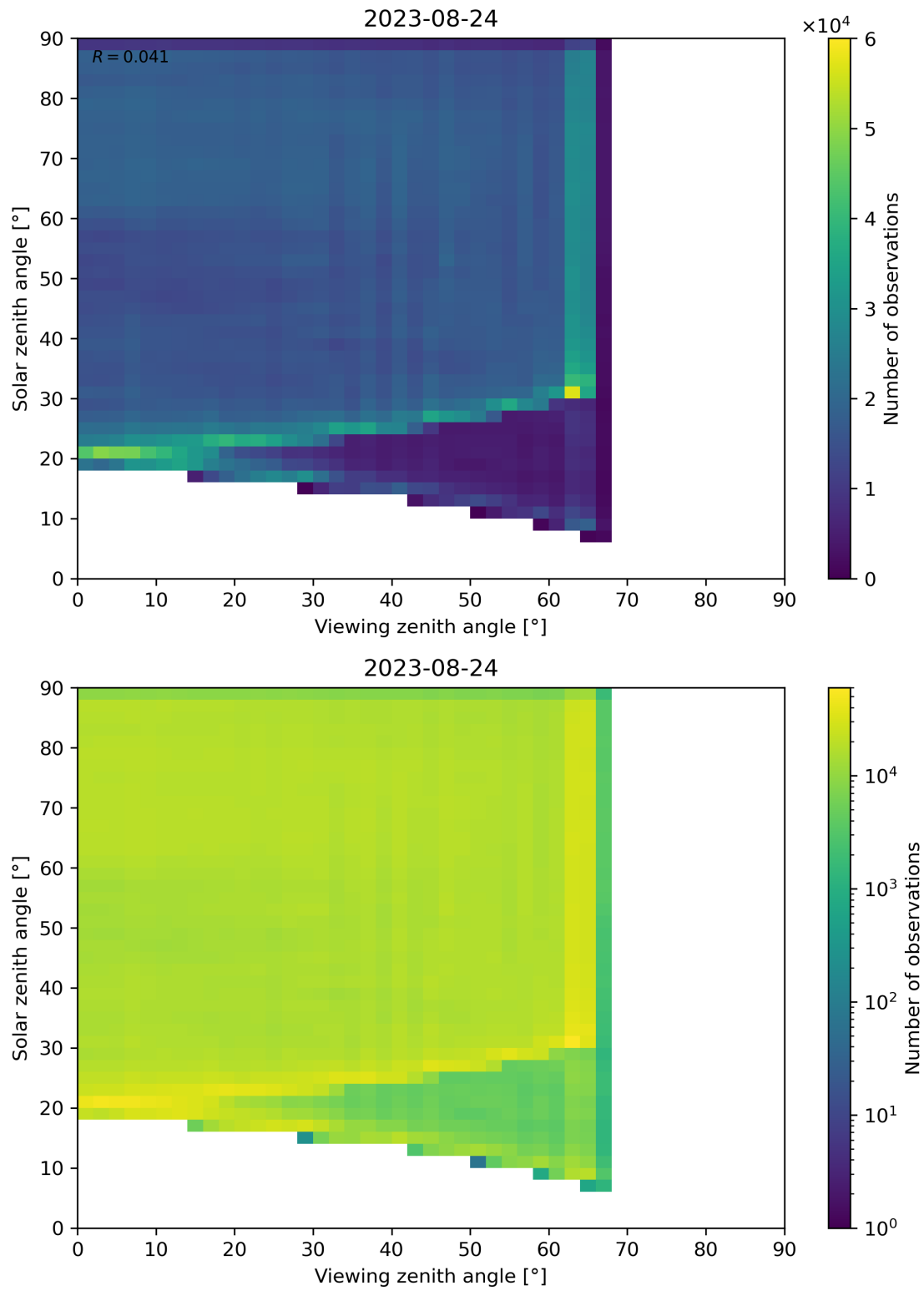
Figure 114: Scatter density plot of “Viewing zenith angle” against “Solar zenith angle” for 2023-08-23 to 2023-08-25.
