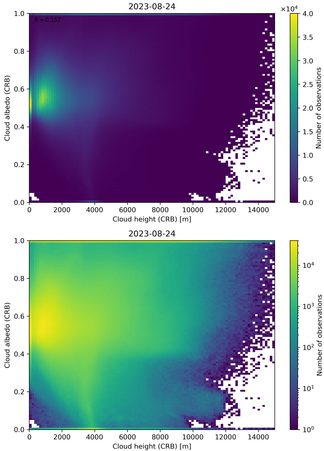
Figure 80: Scatter density plot of “Cloud height (CRB)” against “Cloud albedo (CRB)” for 2023-08-23 to 2023-08-25.
