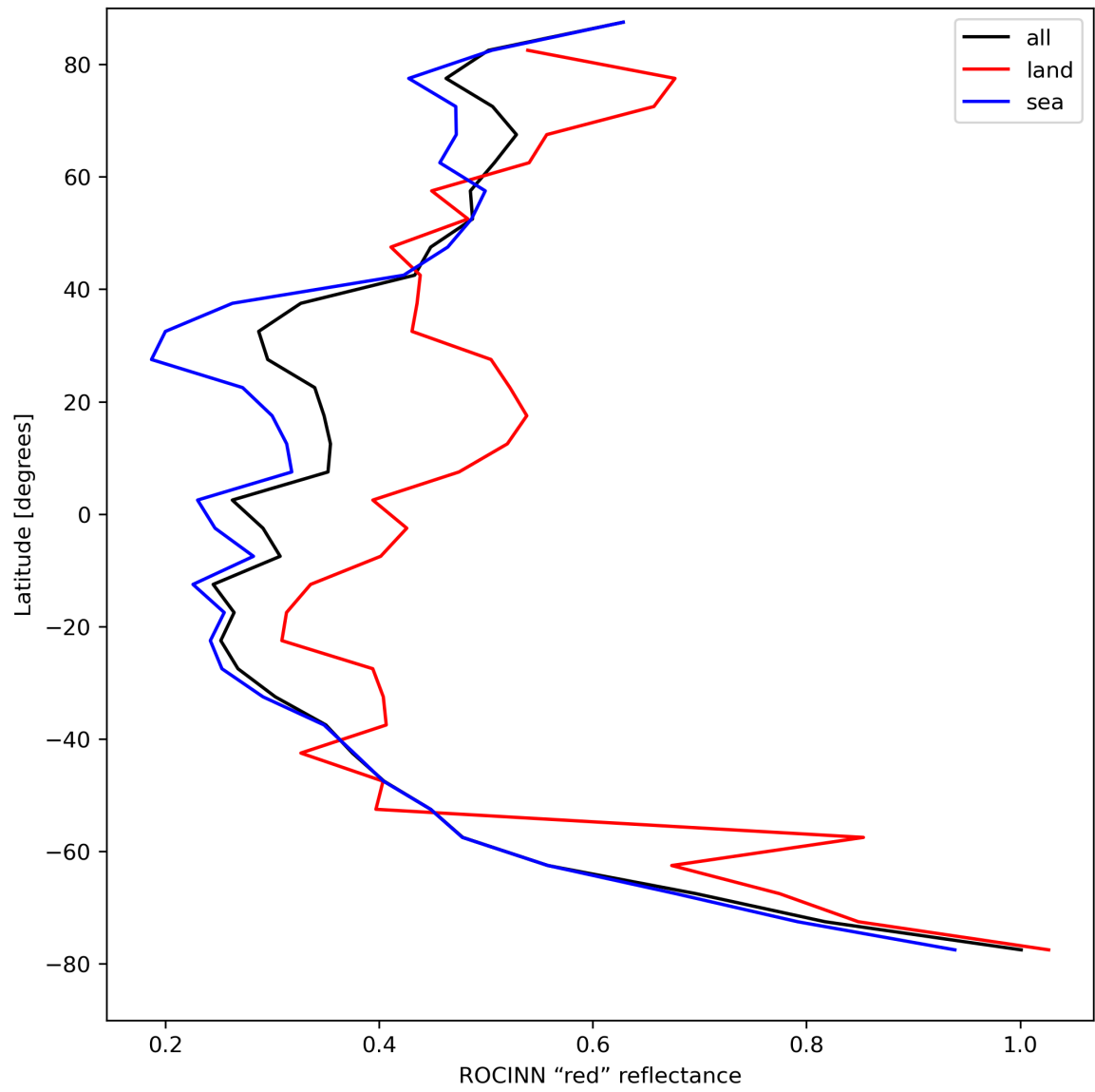
Figure 37: Zonal average of “ROCINN “red” reflectance” for 2023-08-23 to 2023-08-25.
