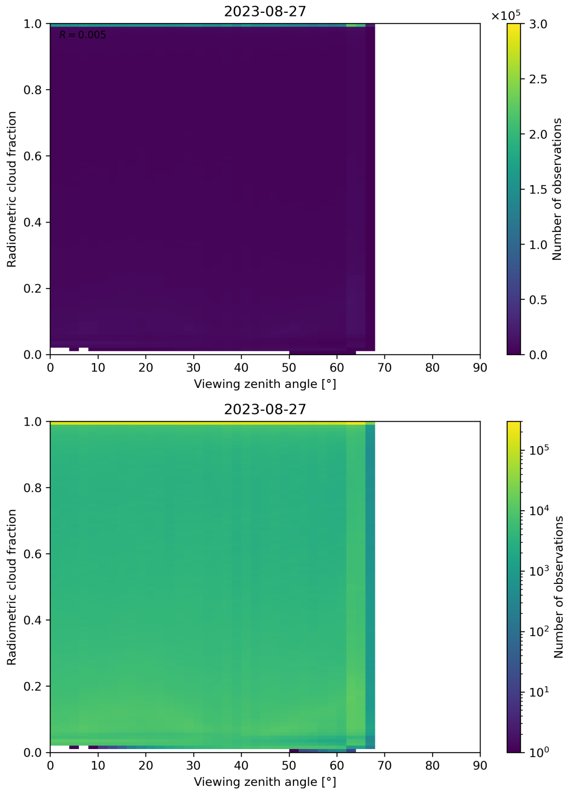
Figure 107: Scatter density plot of “Viewing zenith angle” against “Radiometric cloud fraction” for 2023-08-26 to 2023-08-28.
