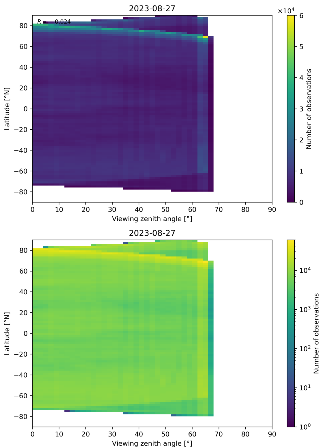
Figure 113: Scatter density plot of “Viewing zenith angle” against “Latitude” for 2023-08-26 to 2023-08-28.
