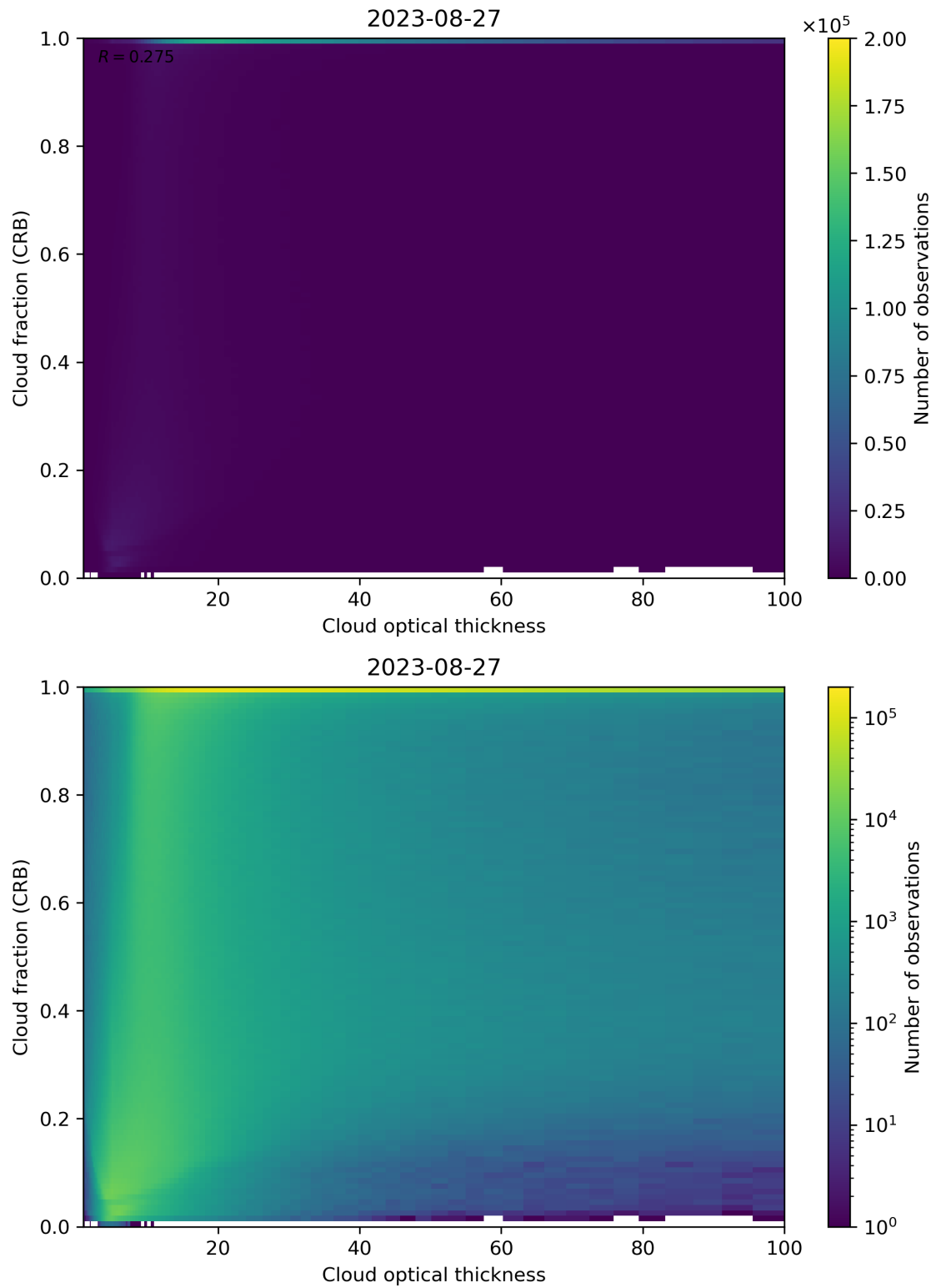
Figure 84: Scatter density plot of “Cloud optical thickness” against “Cloud fraction (CRB)” for 2023-08-26 to 2023-08-28.
