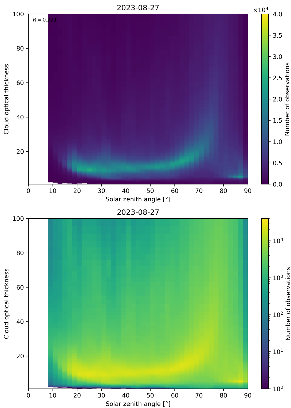
Figure 103: Scatter density plot of “Solar zenith angle” against “Cloud optical thickness” for 2023-08-26 to 2023-08-28.
