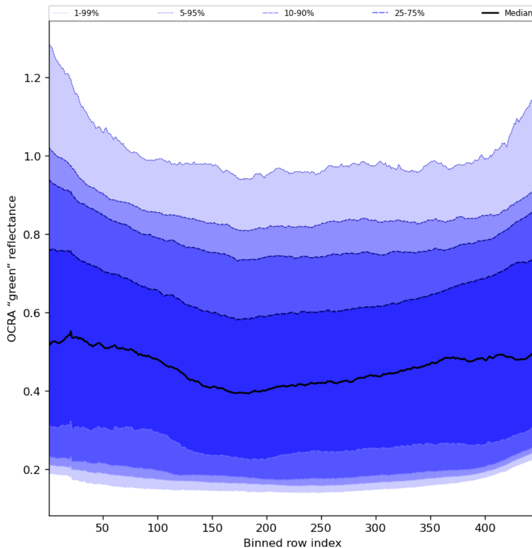
Figure 68: Along track statistics of “OCRA “green” reflectance” for 2023-08-26 to 2023-08-28
