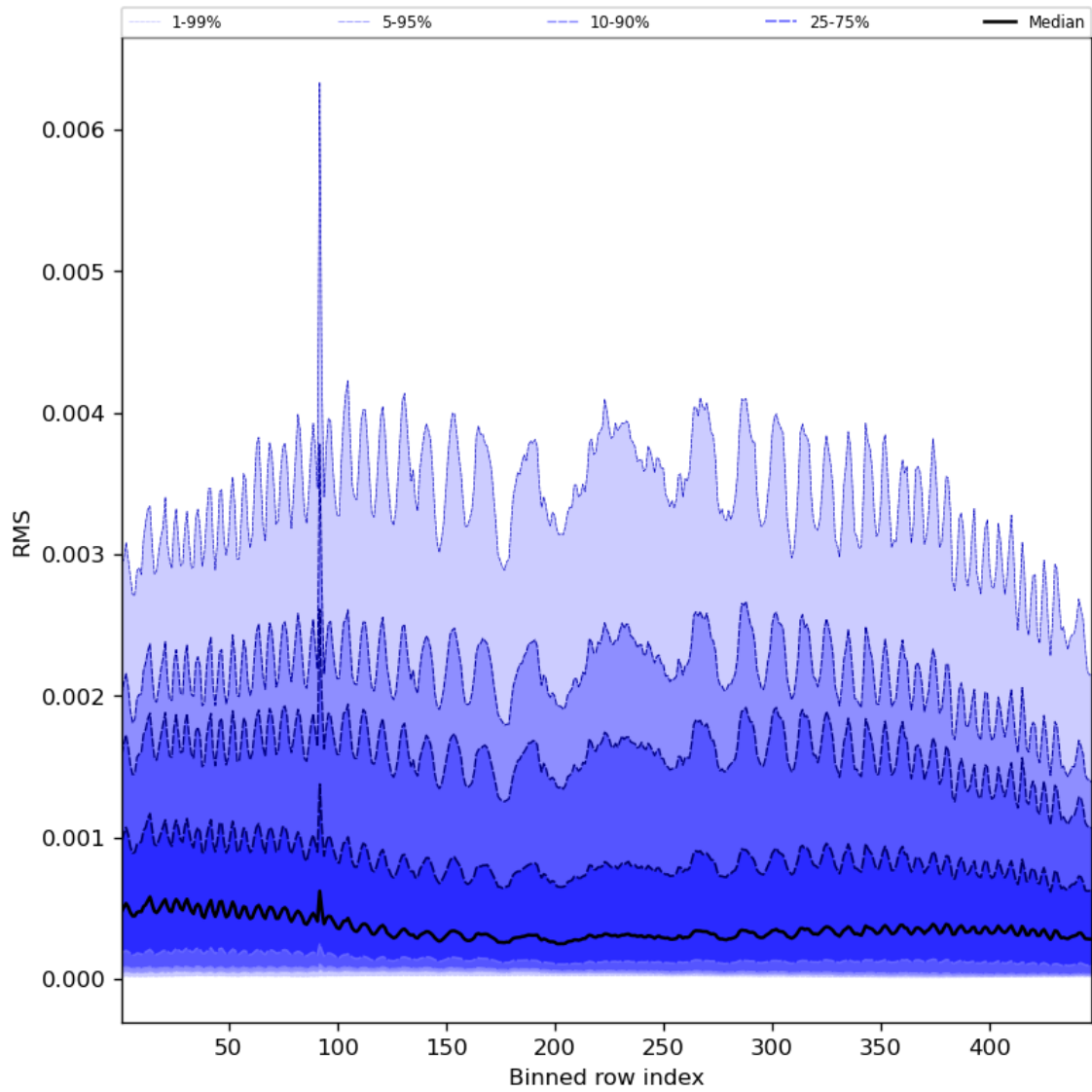
Figure 63: Along track statistics of “RMS” for 2023-08-26 to 2023-08-28
