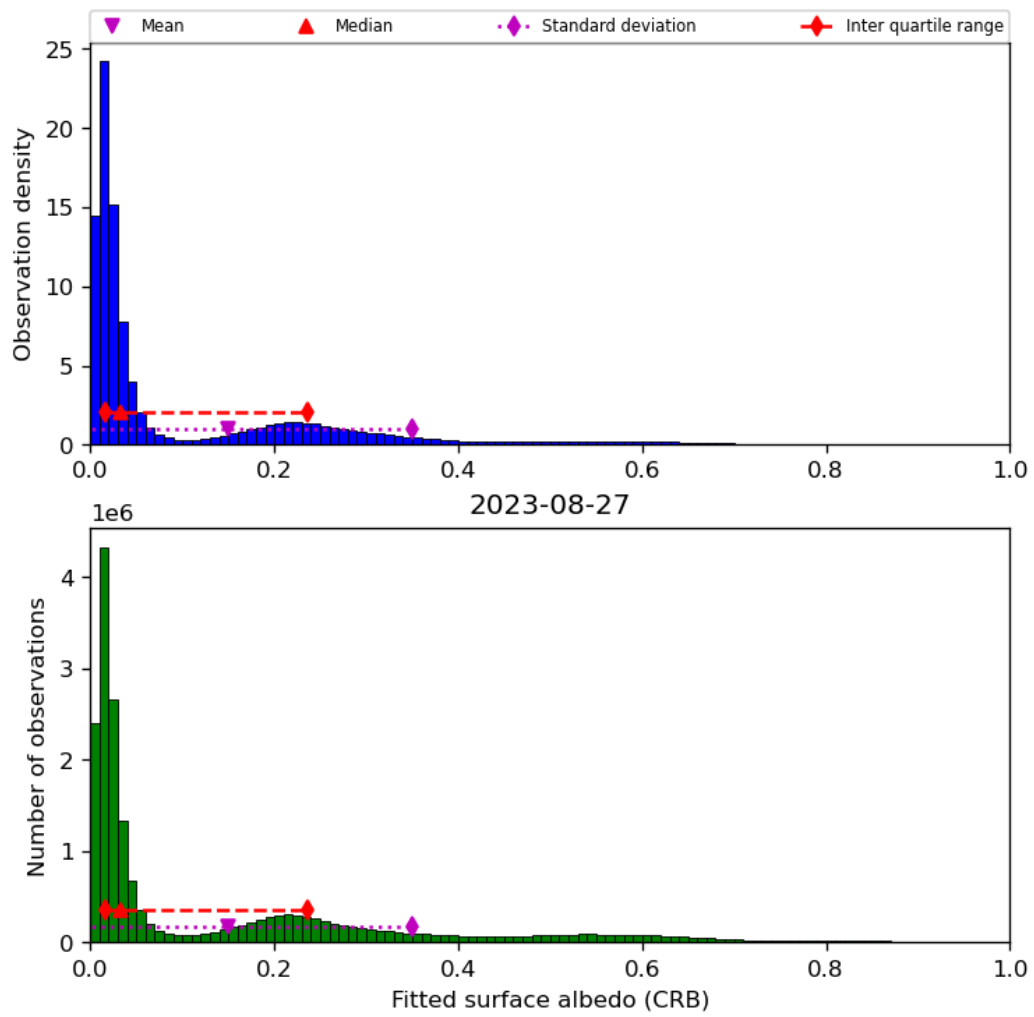
Figure 46: Histogram of “Fitted surface albedo (CRB)” for 2023-08-26 to 2023-08-28
