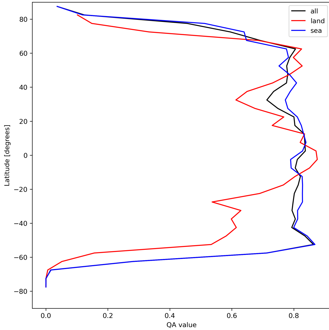
Figure 22: Zonal average of “QA value” for 2023-08-26 to 2023-08-28.
