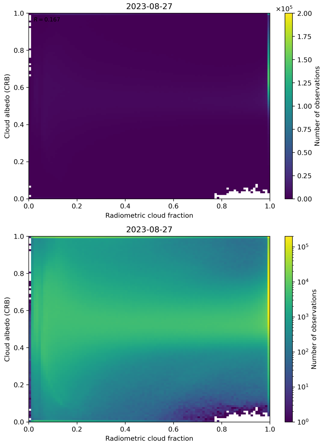
Figure 71: Scatter density plot of “Radiometric cloud fraction” against “Cloud albedo (CRB)” for 2023-08-26 to 2023-08-28.
