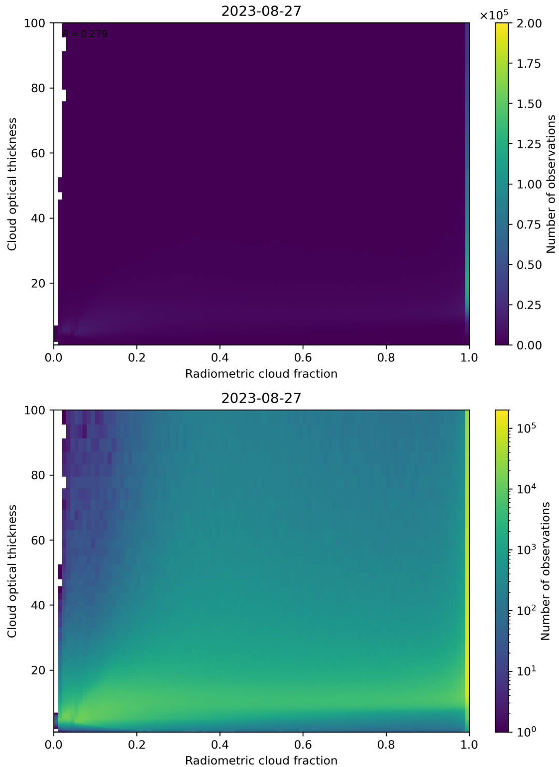
Figure 75: Scatter density plot of “Radiometric cloud fraction” against “Cloud optical thickness” for 2023-08-26 to 2023-08-28.
