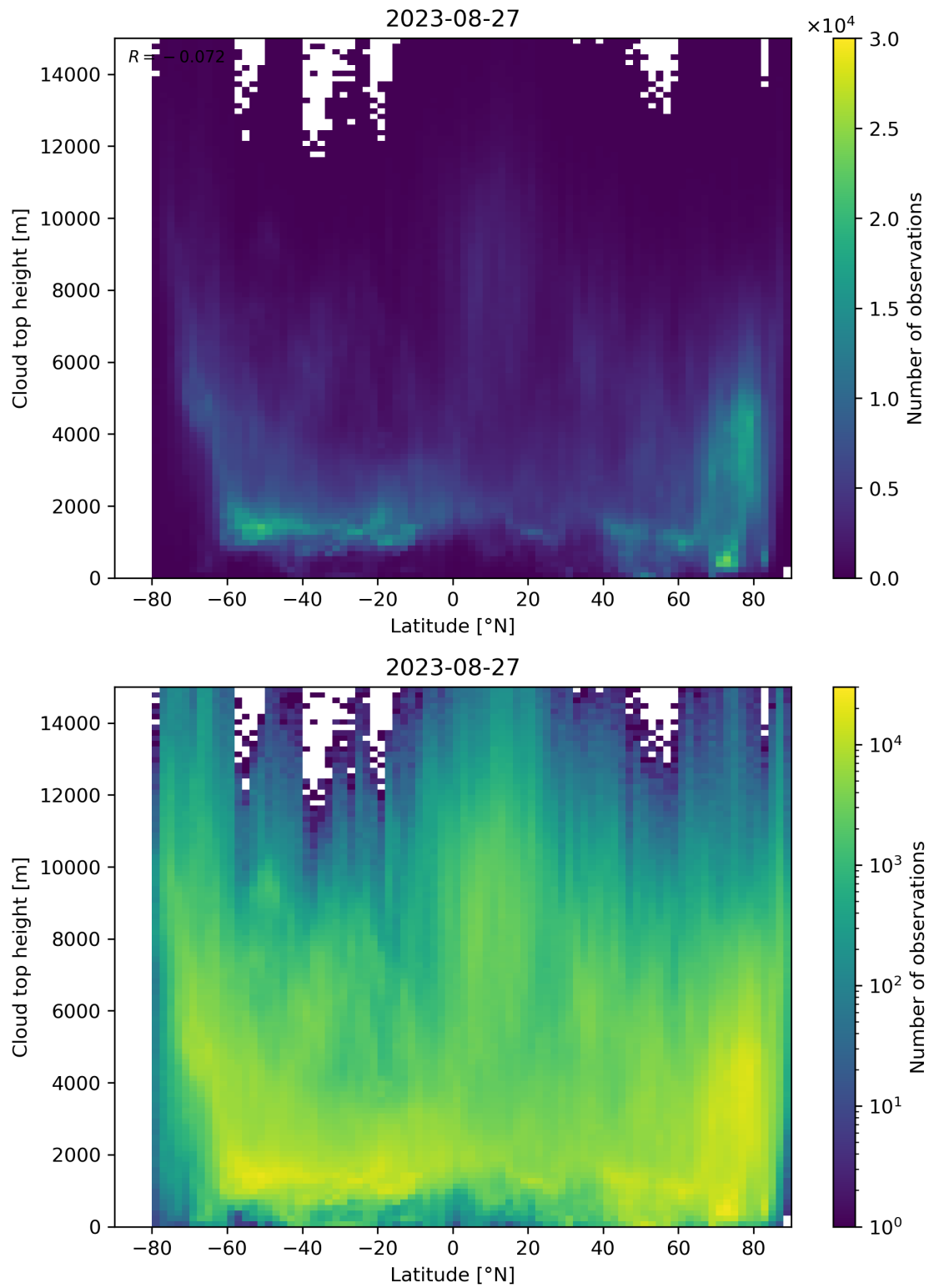
Figure 97: Scatter density plot of “Latitude” against “Cloud top height” for 2023-08-26 to 2023-08-28.
