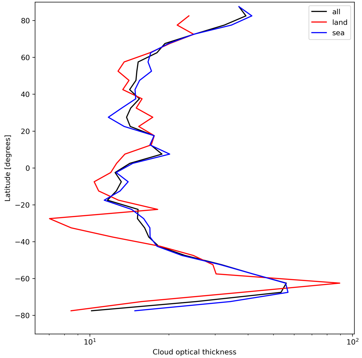
Figure 25: Zonal average of “Cloud optical thickness” for 2023-08-26 to 2023-08-28.
