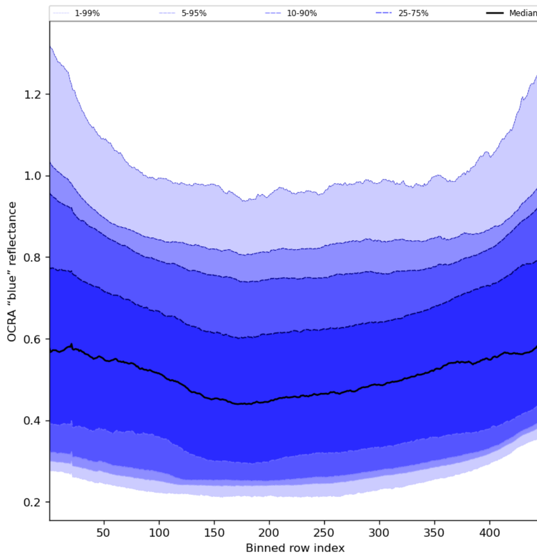
Figure 67: Along track statistics of “OCRA “blue” reflectance” for 2023-08-26 to 2023-08-28
