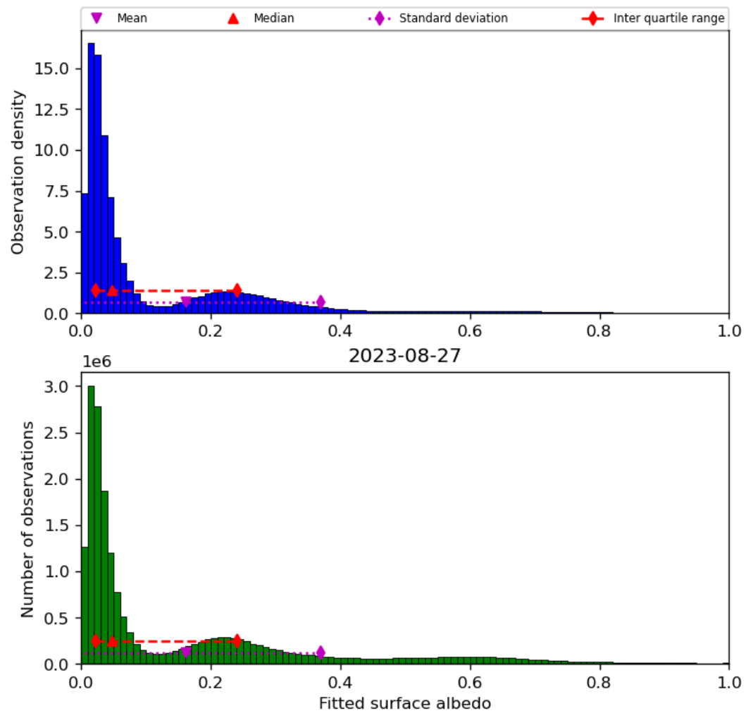
Figure 45: Histogram of “Fitted surface albedo” for 2023-08-26 to 2023-08-28
