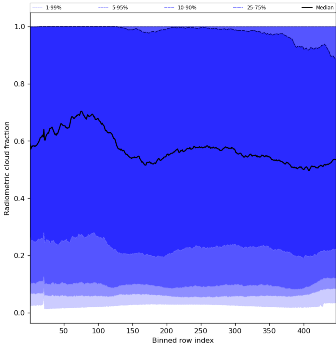
Figure 55: Along track statistics of “Radiometric cloud fraction” for 2023-08-26 to 2023-08-28
