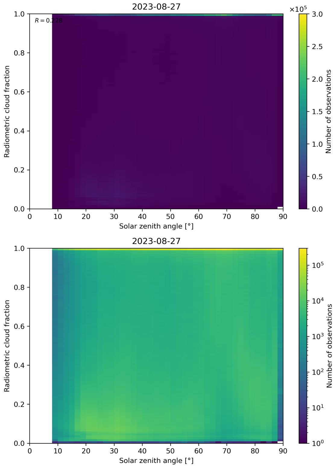
Figure 99: Scatter density plot of “Solar zenith angle” against “Radiometric cloud fraction” for 2023-08-26 to 2023-08-28.
