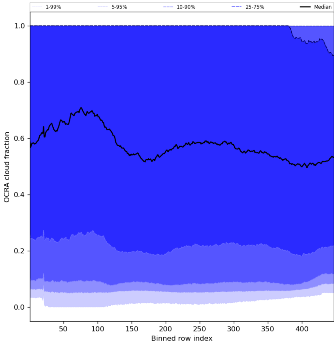
Figure 66: Along track statistics of “OCRA cloud fraction” for 2023-08-26 to 2023-08-28
