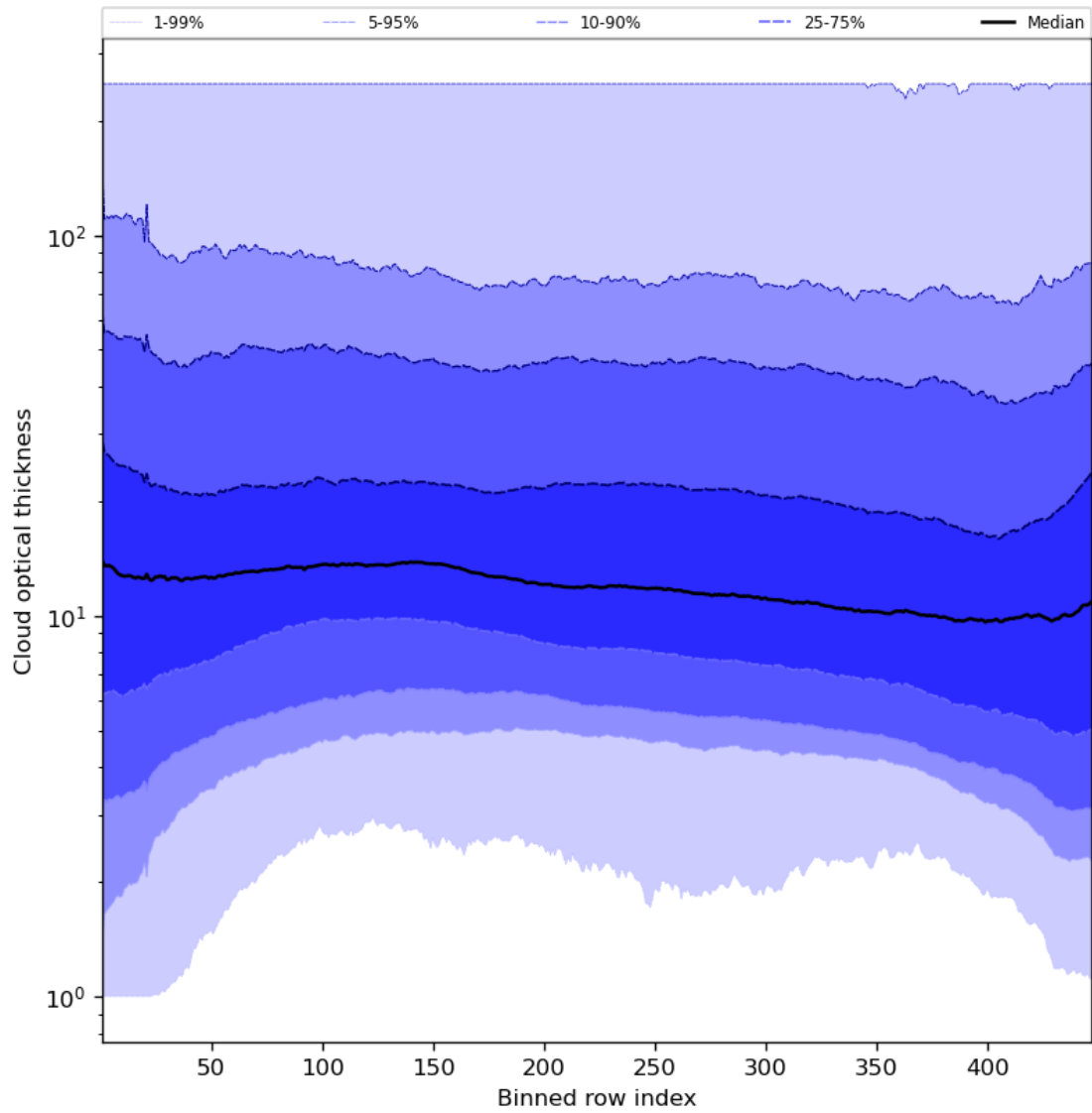
Figure 57: Along track statistics of “Cloud optical thickness” for 2023-08-26 to 2023-08-28
