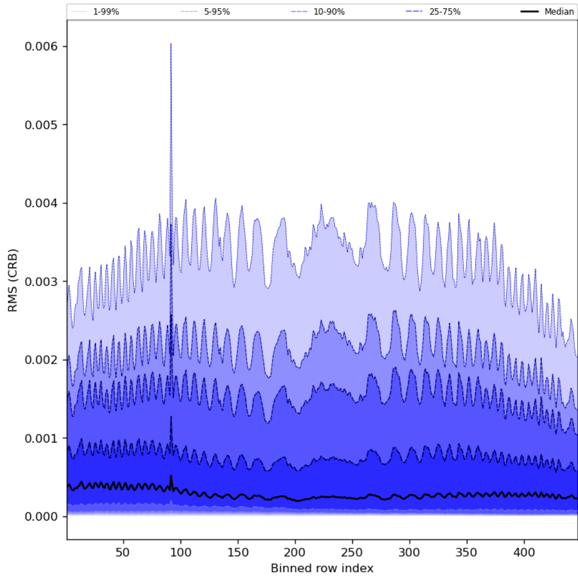
Figure 64: Along track statistics of “RMS (CRB)” for 2023-08-26 to 2023-08-28
