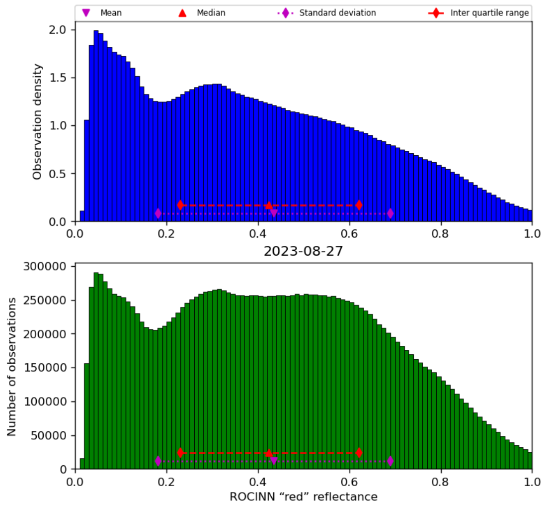
Figure 53: Histogram of “ROCINN “red” reflectance” for 2023-08-26 to 2023-08-28
