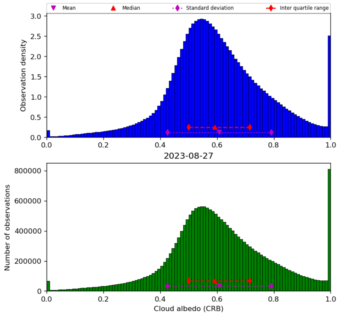
Figure 44: Histogram of “Cloud albedo (CRB)” for 2023-08-26 to 2023-08-28
