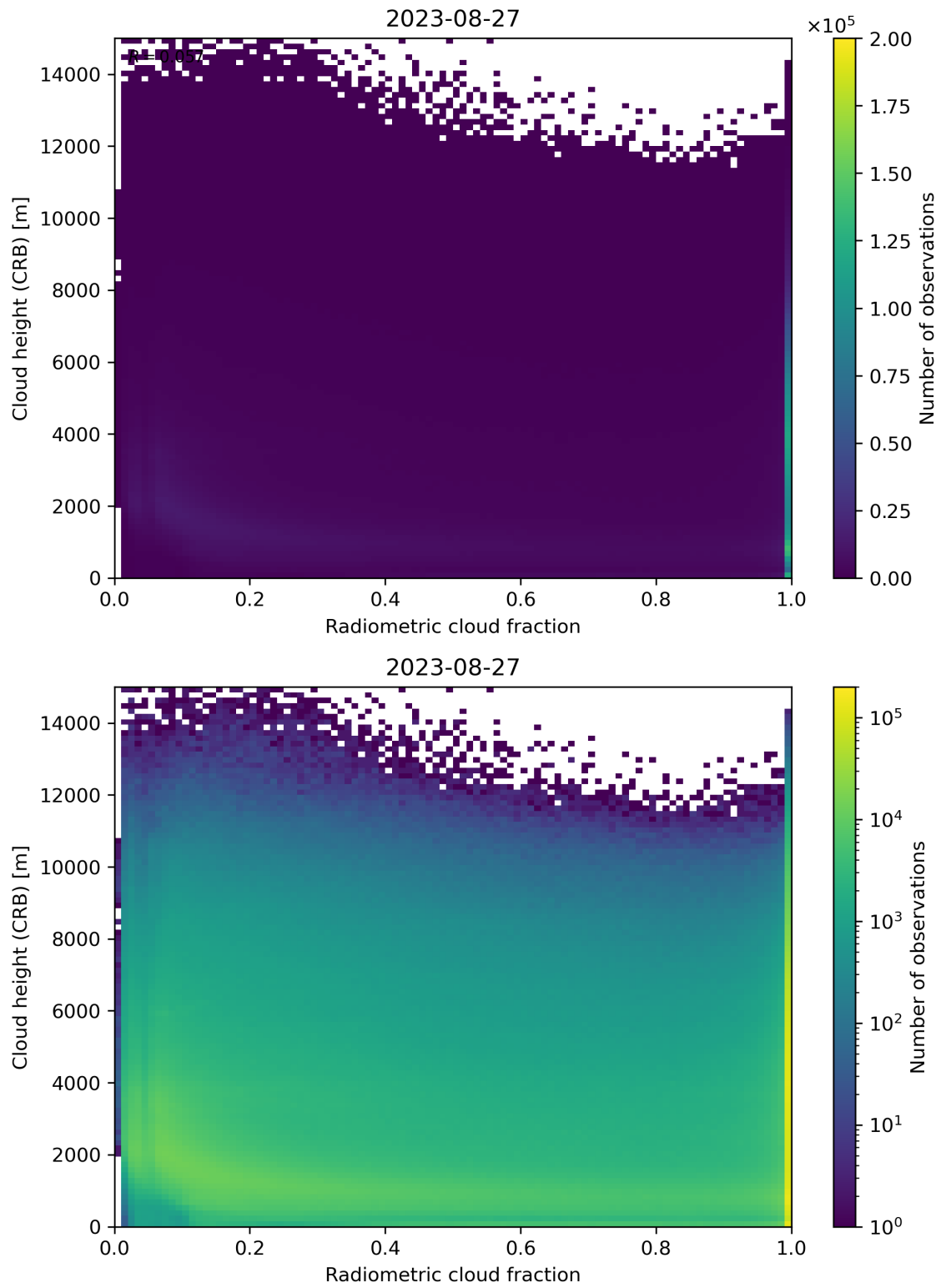
Figure 74: Scatter density plot of “Radiometric cloud fraction” against “Cloud height (CRB)” for 2023-08-26 to 2023-08-28.
