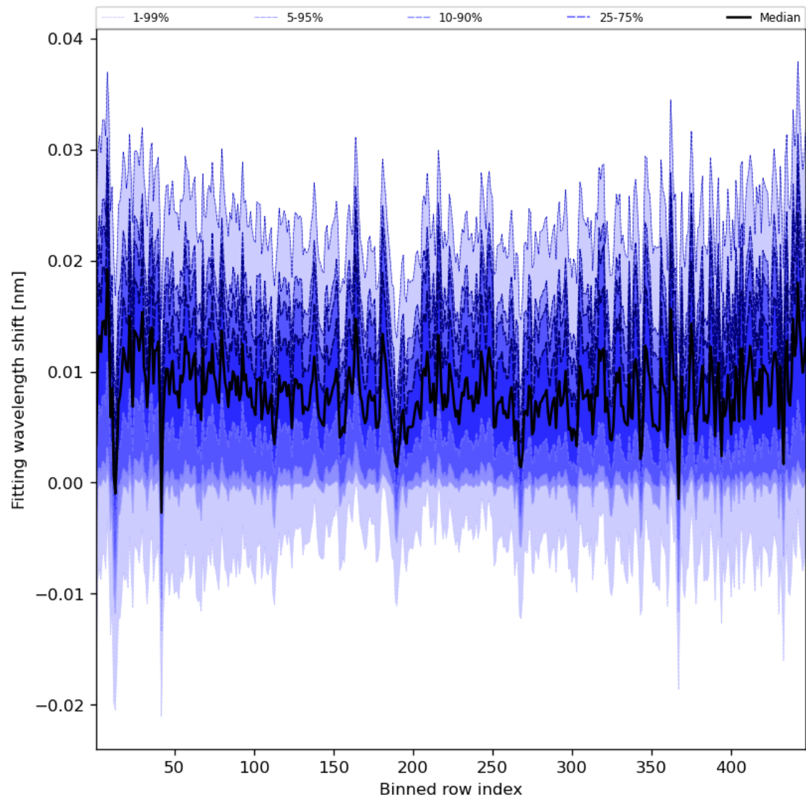
Figure 65: Along track statistics of “Fitting wavelength shift” for 2023-08-26 to 2023-08-28
