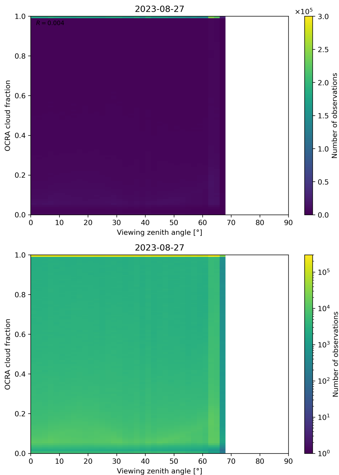
Figure 108: Scatter density plot of “Viewing zenith angle” against “OCRA cloud fraction” for 2023-08-26 to 2023-08-28.
