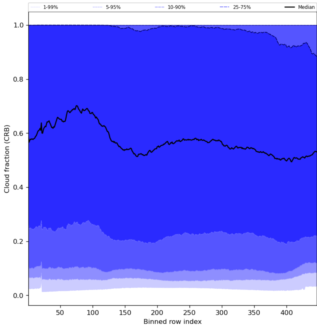
Figure 58: Along track statistics of “Cloud fraction (CRB)” for 2023-08-26 to 2023-08-28
