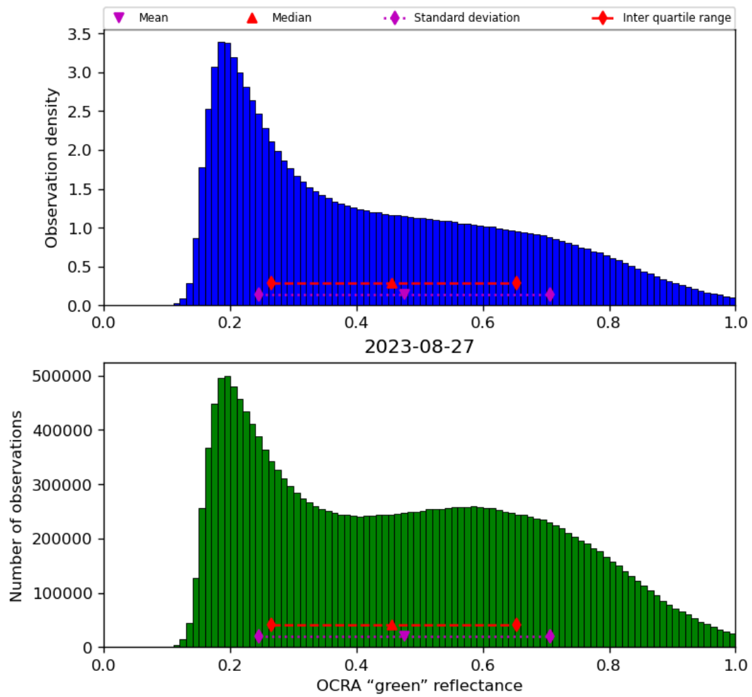
Figure 52: Histogram of “OCRA “green” reflectance” for 2023-08-26 to 2023-08-28
