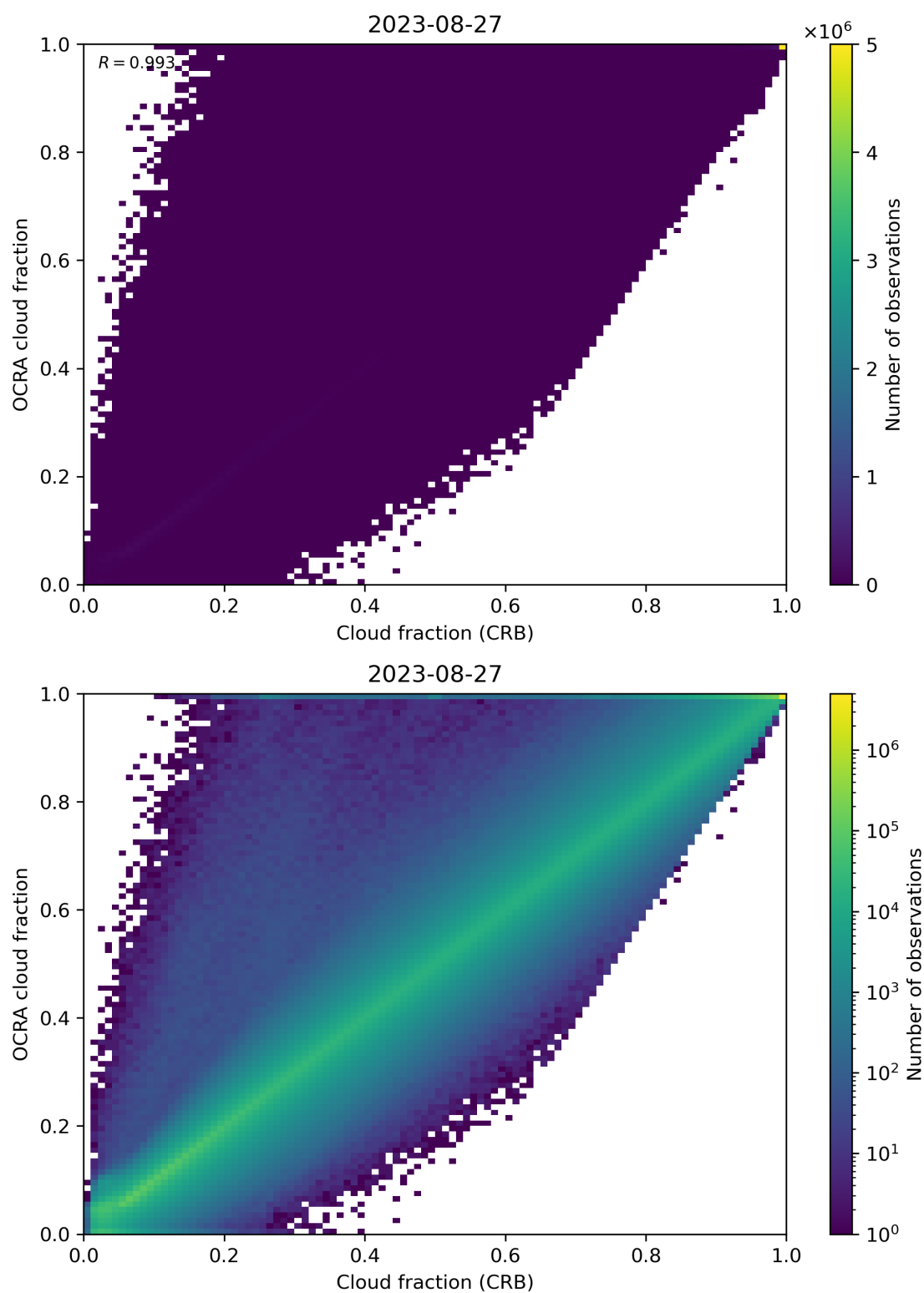
Figure 78: Scatter density plot of “Cloud fraction (CRB)” against “OCRA cloud fraction” for 2023-08-26 to 2023-08-28.
