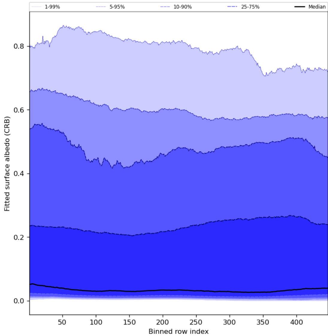
Figure 62: Along track statistics of “Fitted surface albedo (CRB)” for 2023-08-26 to 2023-08-28
