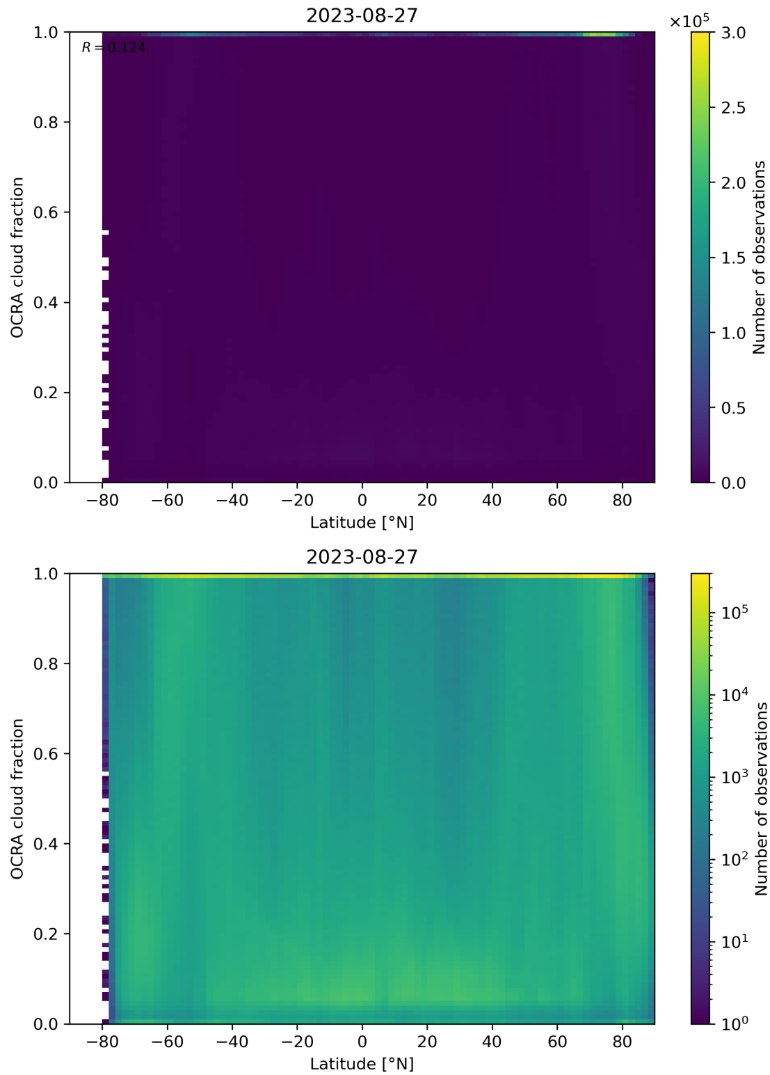
Figure 93: Scatter density plot of “Latitude” against “OCRA cloud fraction” for 2023-08-26 to 2023-08-28.
