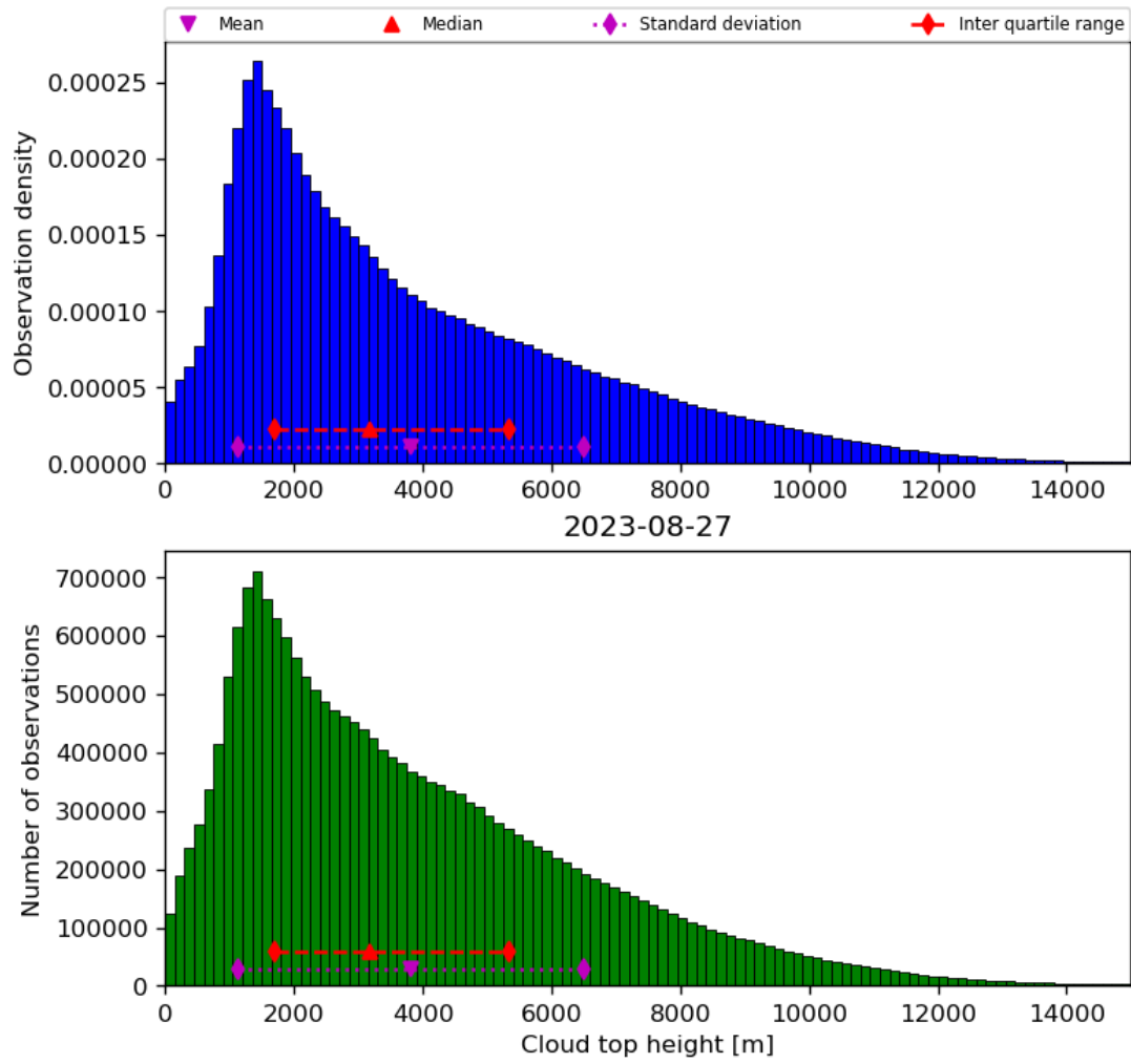
Figure 40: Histogram of “Cloud top height” for 2023-08-26 to 2023-08-28
