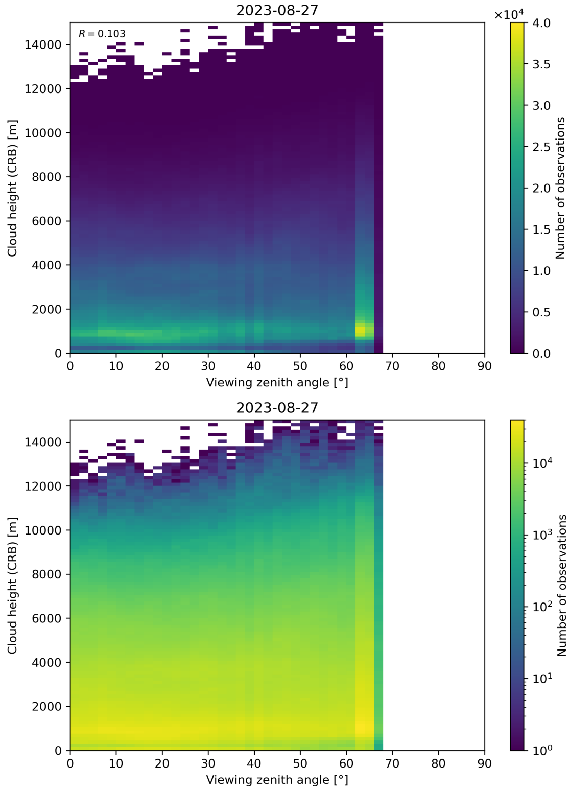
Figure 110: Scatter density plot of “Viewing zenith angle” against “Cloud height (CRB)” for 2023-08-26 to 2023-08-28.
