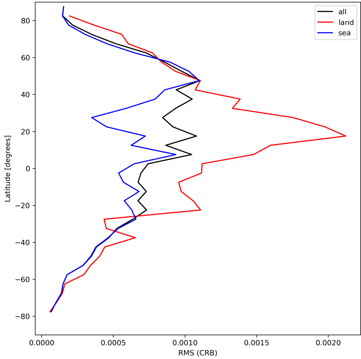
Figure 32: Zonal average of “RMS (CRB)” for 2023-08-26 to 2023-08-28.
