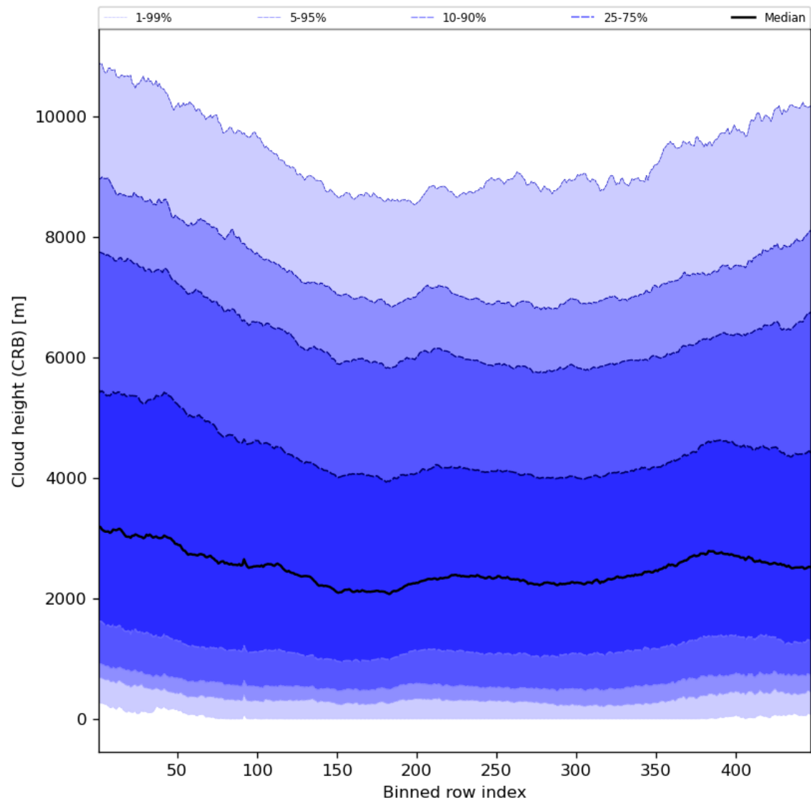
Figure 59: Along track statistics of “Cloud height (CRB)” for 2023-08-26 to 2023-08-28
