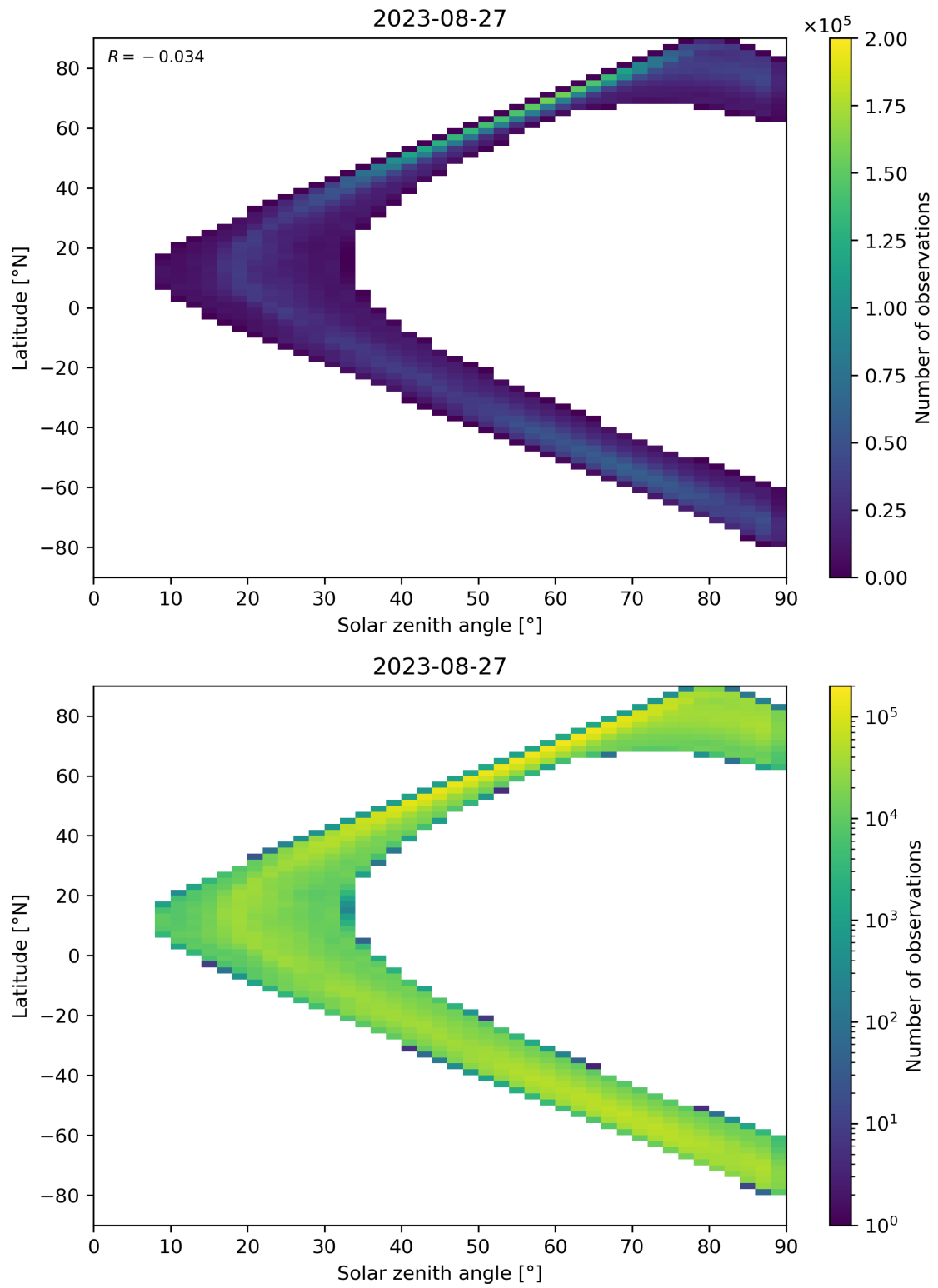
Figure 105: Scatter density plot of “Solar zenith angle” against “Latitude” for 2023-08-26 to 2023-08-28.
