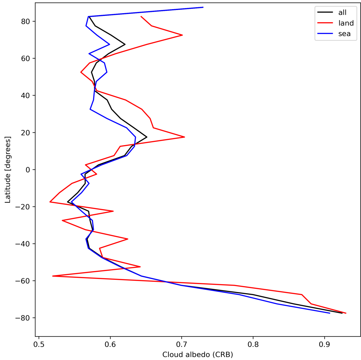
Figure 28: Zonal average of “Cloud albedo (CRB)” for 2023-08-26 to 2023-08-28.
