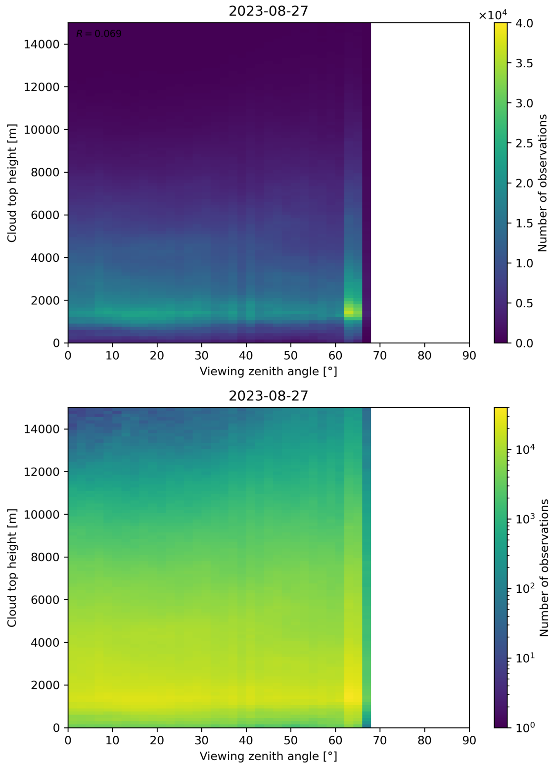
Figure 112: Scatter density plot of “Viewing zenith angle” against “Cloud top height” for 2023-08-26 to 2023-08-28.
