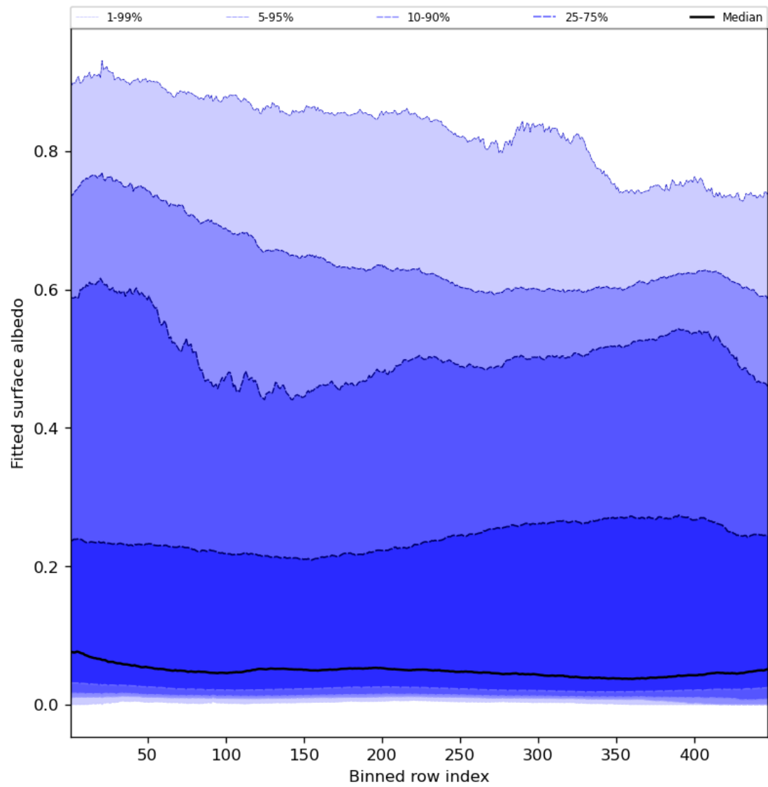
Figure 61: Along track statistics of “Fitted surface albedo” for 2023-08-26 to 2023-08-28
