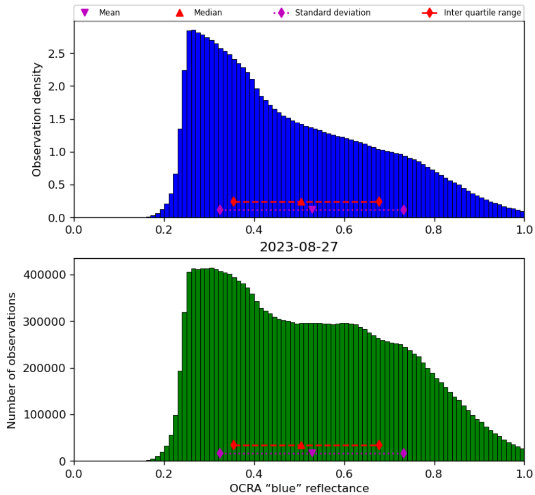
Figure 51: Histogram of “OCRA “blue” reflectance” for 2023-08-26 to 2023-08-28
