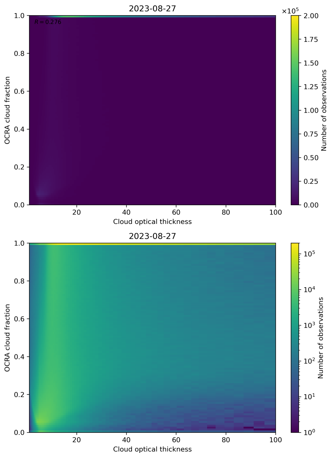
Figure 83: Scatter density plot of “Cloud optical thickness” against “OCRA cloud fraction” for 2023-08-26 to 2023-08-28.
