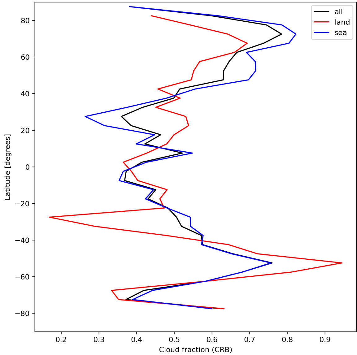
Figure 26: Zonal average of “Cloud fraction (CRB)” for 2023-08-26 to 2023-08-28.
