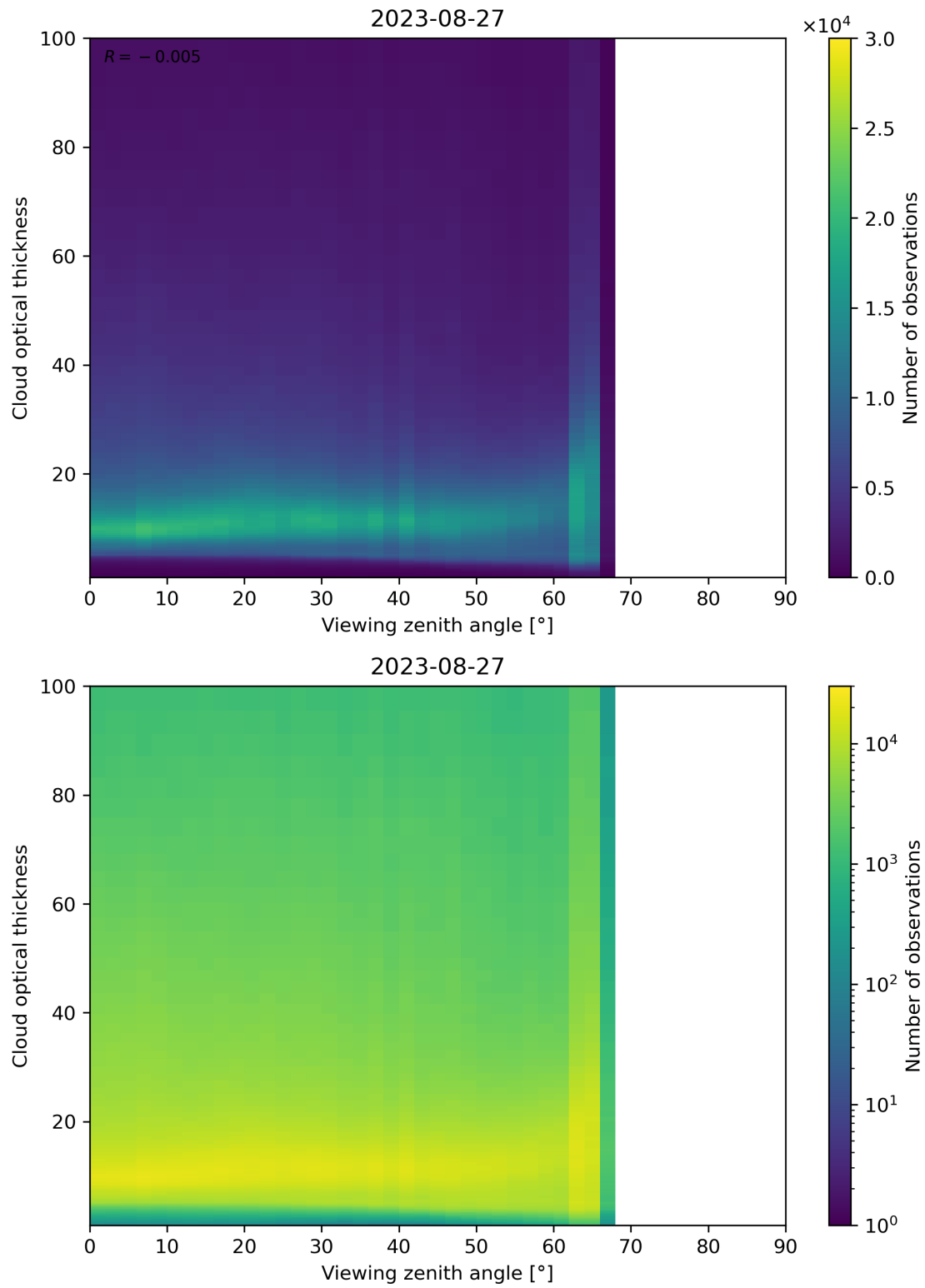
Figure 111: Scatter density plot of “Viewing zenith angle” against “Cloud optical thickness” for 2023-08-26 to 2023-08-28.
