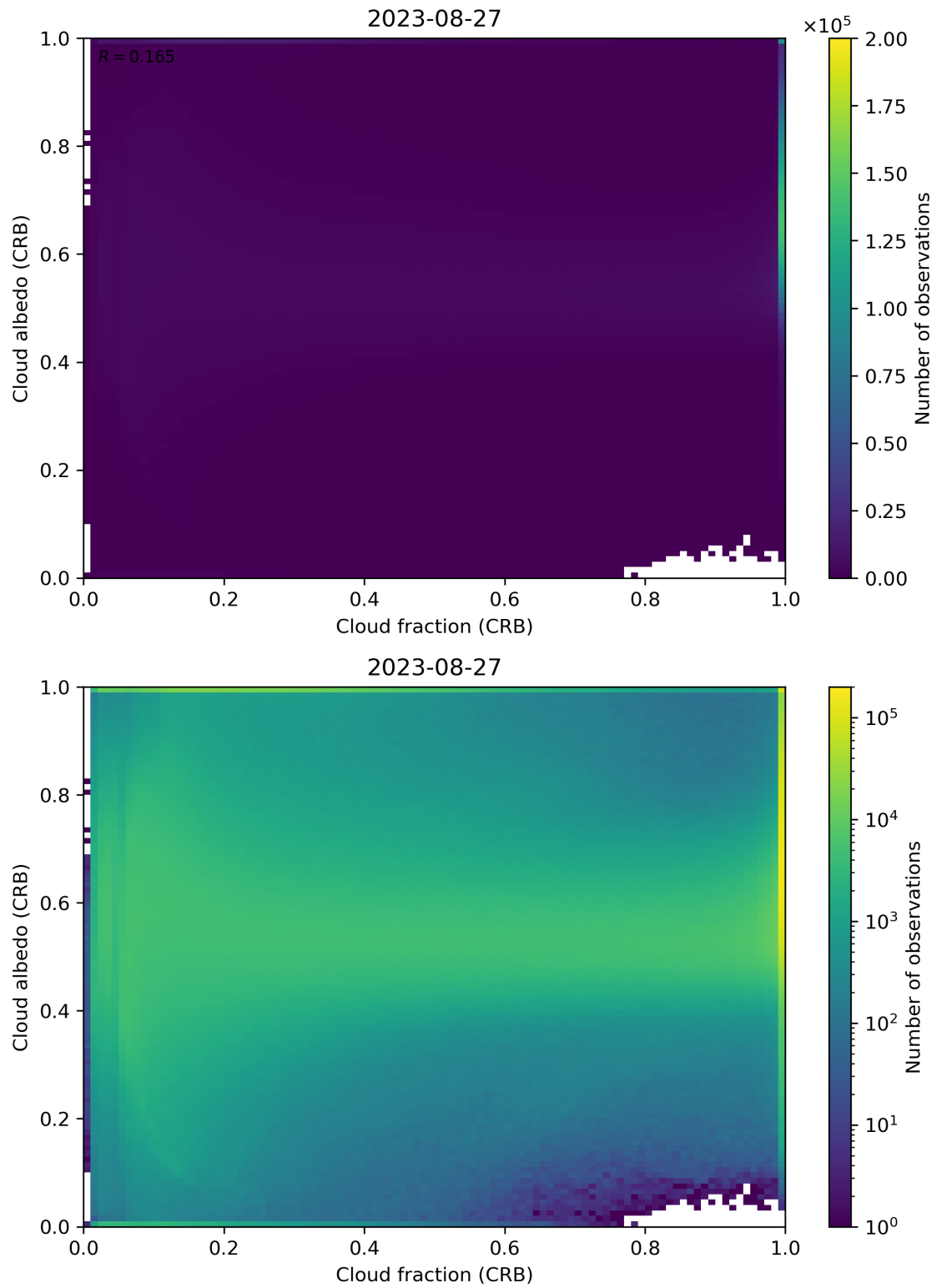
Figure 77: Scatter density plot of “Cloud fraction (CRB)” against “Cloud albedo (CRB)” for 2023-08-26 to 2023-08-28.
