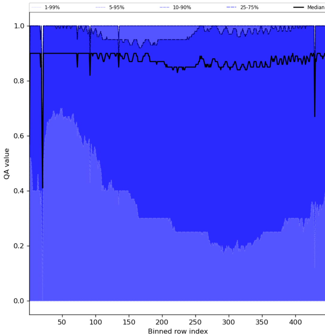
Figure 54: Along track statistics of “QA value” for 2023-08-26 to 2023-08-28
