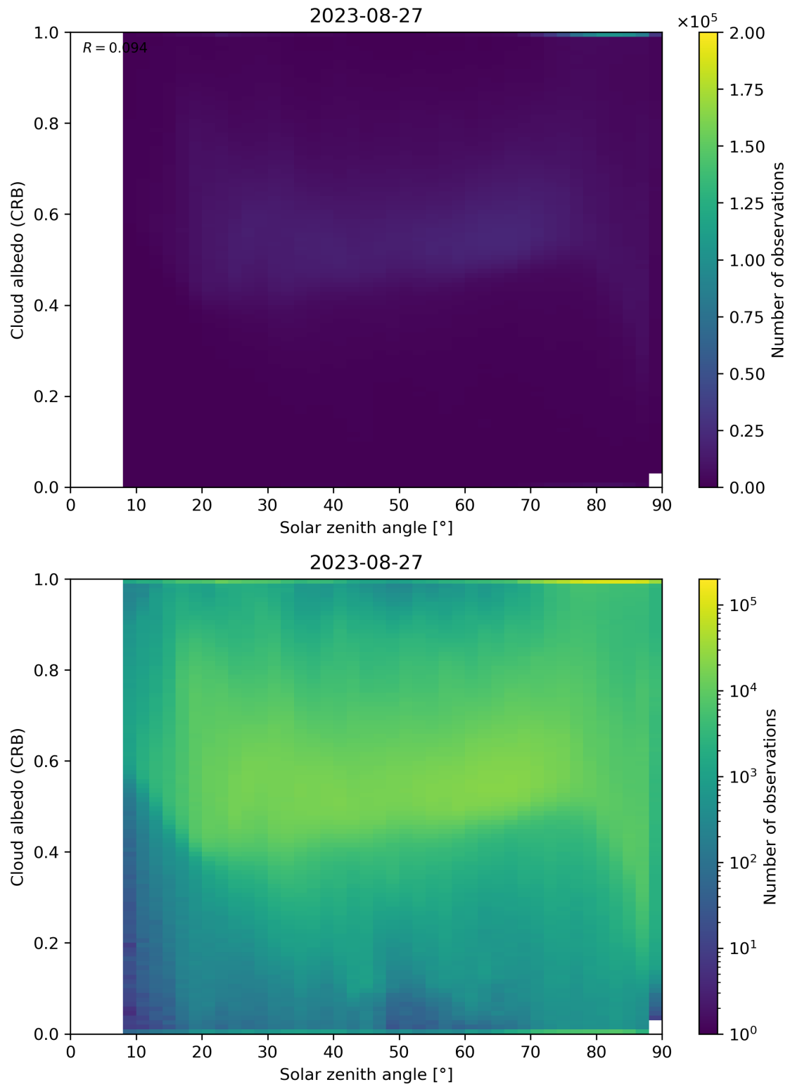
Figure 98: Scatter density plot of “Solar zenith angle” against “Cloud albedo (CRB)” for 2023-08-26 to 2023-08-28.
