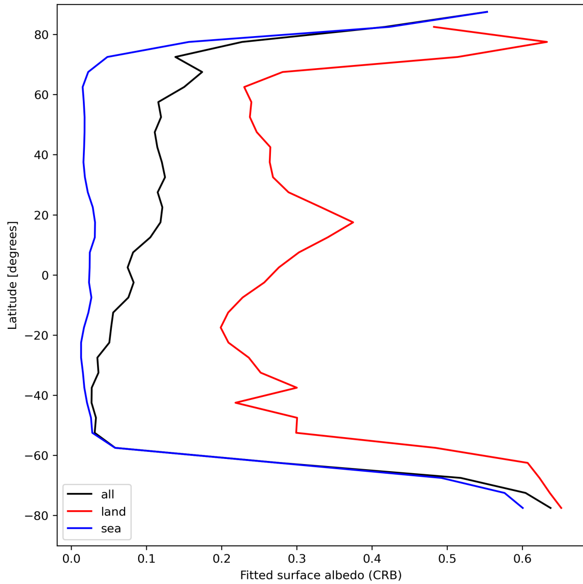
Figure 30: Zonal average of “Fitted surface albedo (CRB)” for 2023-08-26 to 2023-08-28.
