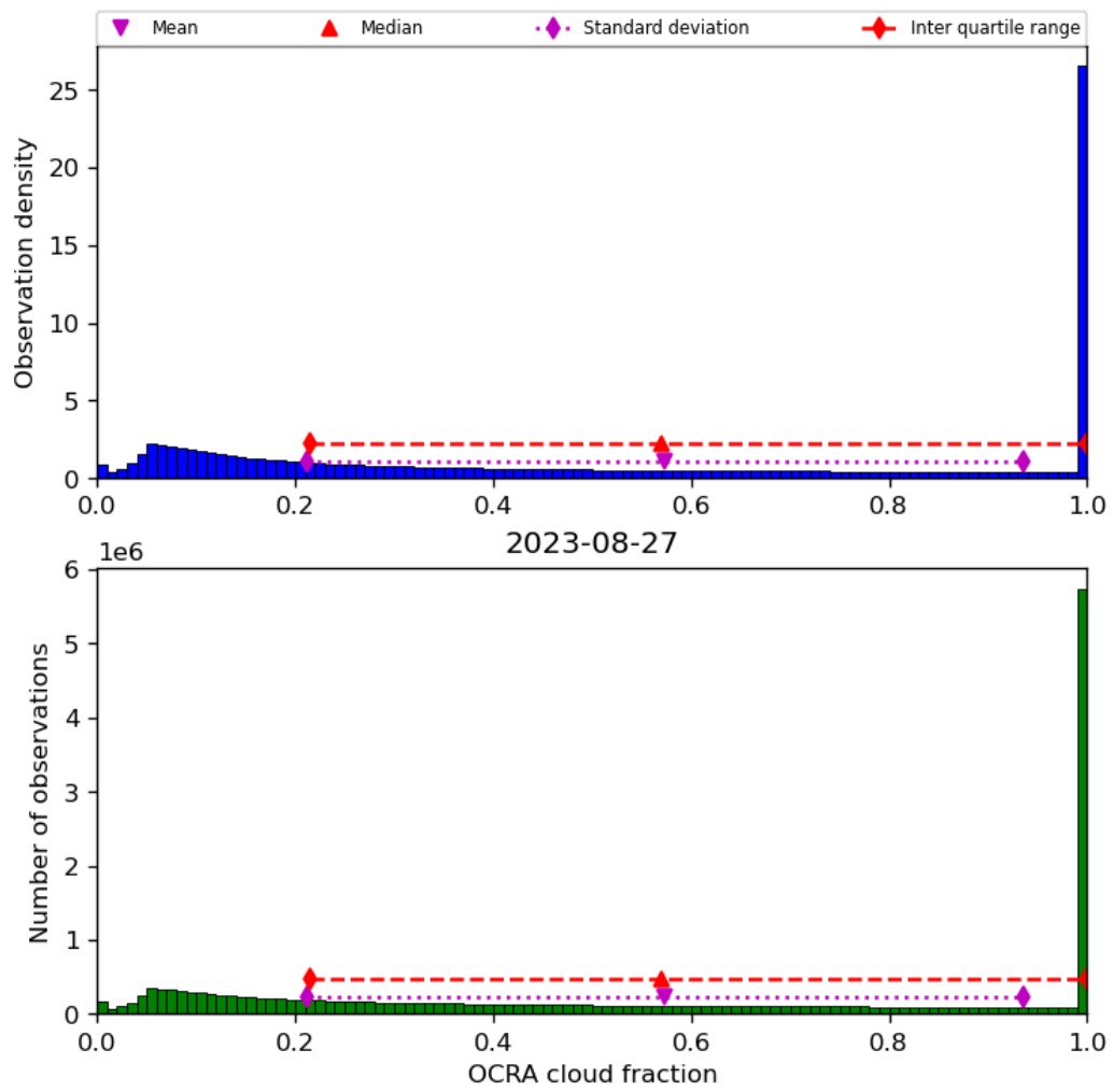
Figure 50: Histogram of “OCRA cloud fraction” for 2023-08-26 to 2023-08-28
