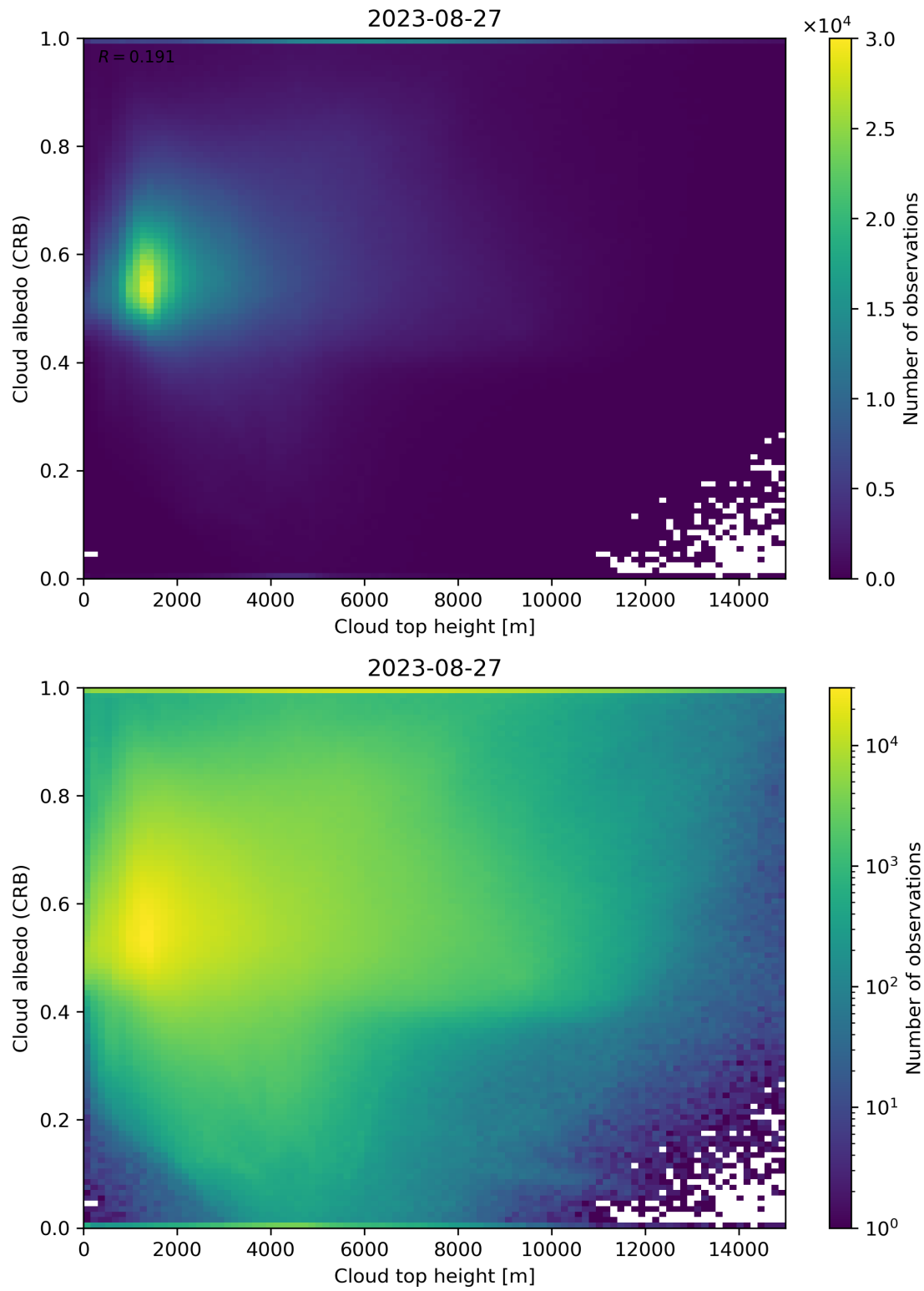
Figure 86: Scatter density plot of “Cloud top height” against “Cloud albedo (CRB)” for 2023-08-26 to 2023-08-28.
