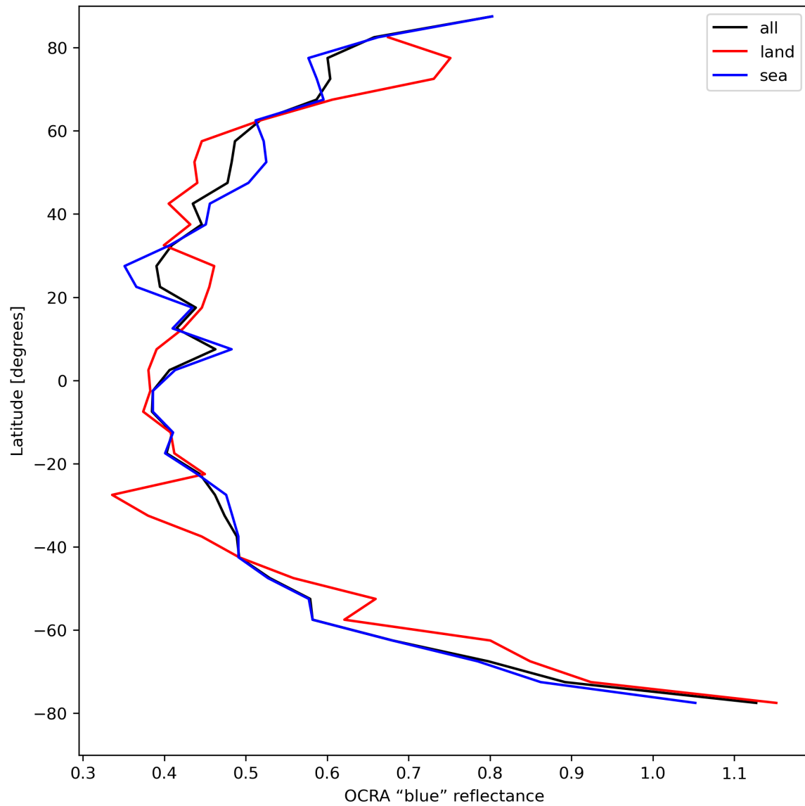
Figure 35: Zonal average of “OCRA “blue” reflectance” for 2023-08-26 to 2023-08-28.
