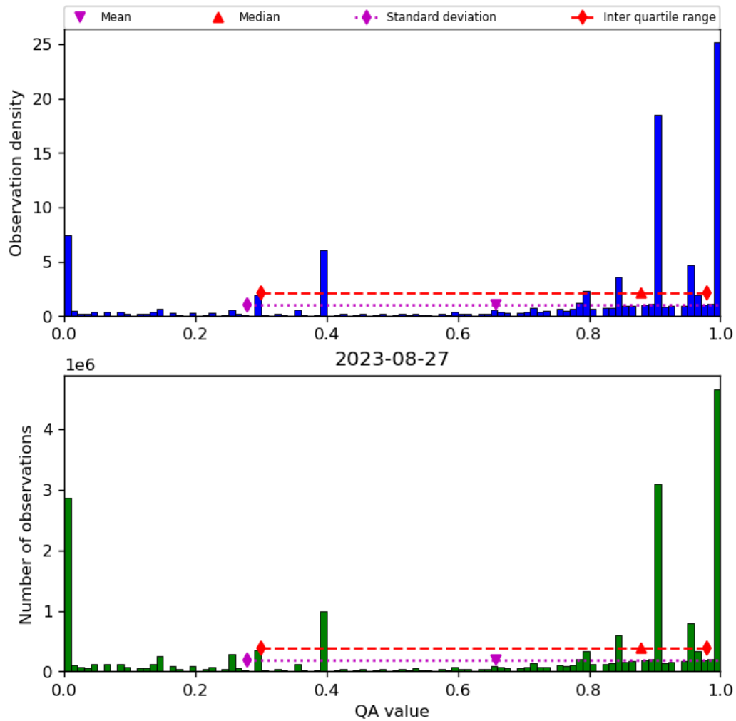
Figure 38: Histogram of “QA value” for 2023-08-26 to 2023-08-28
