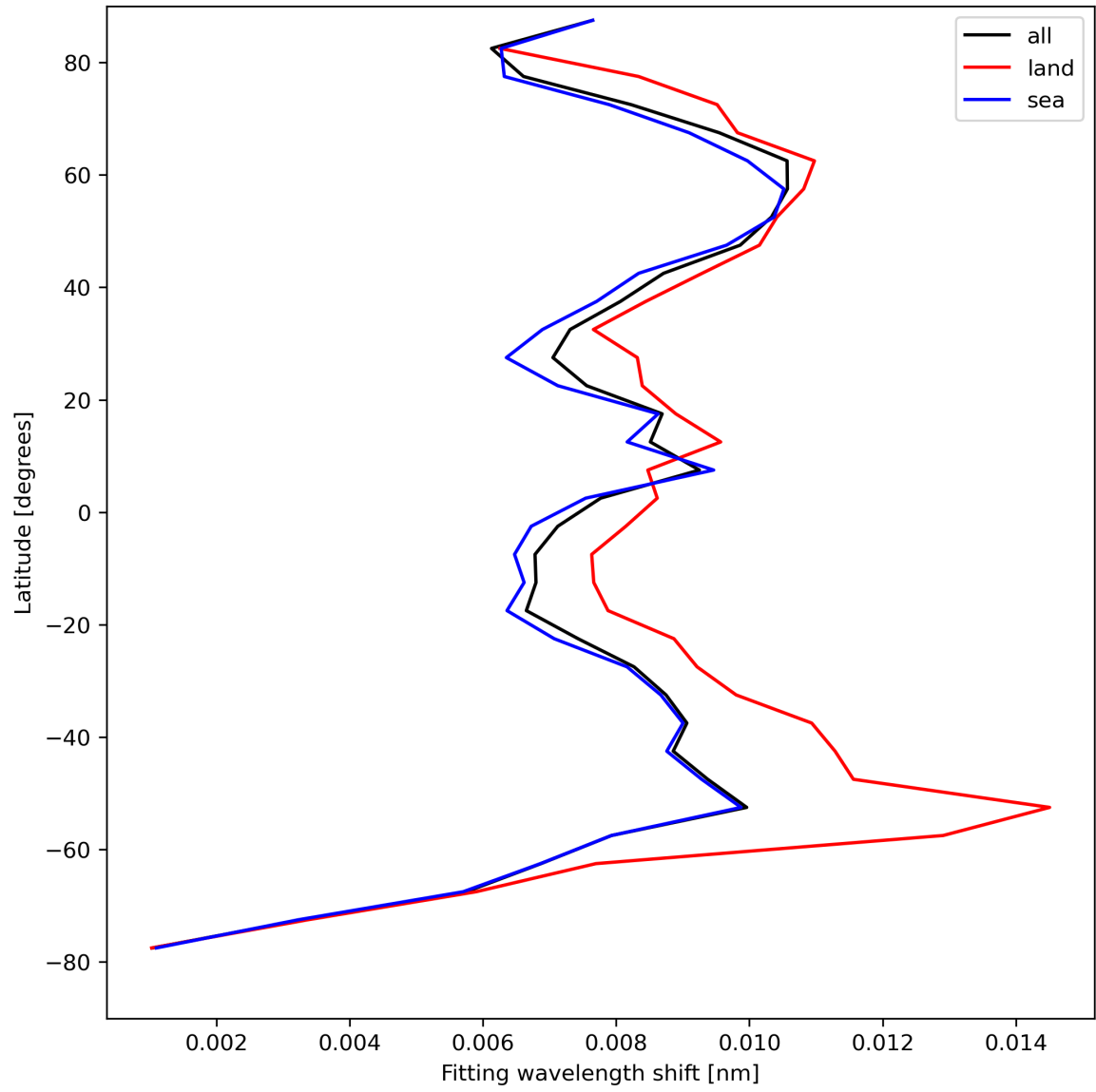
Figure 33: Zonal average of “Fitting wavelength shift” for 2023-08-26 to 2023-08-28.
