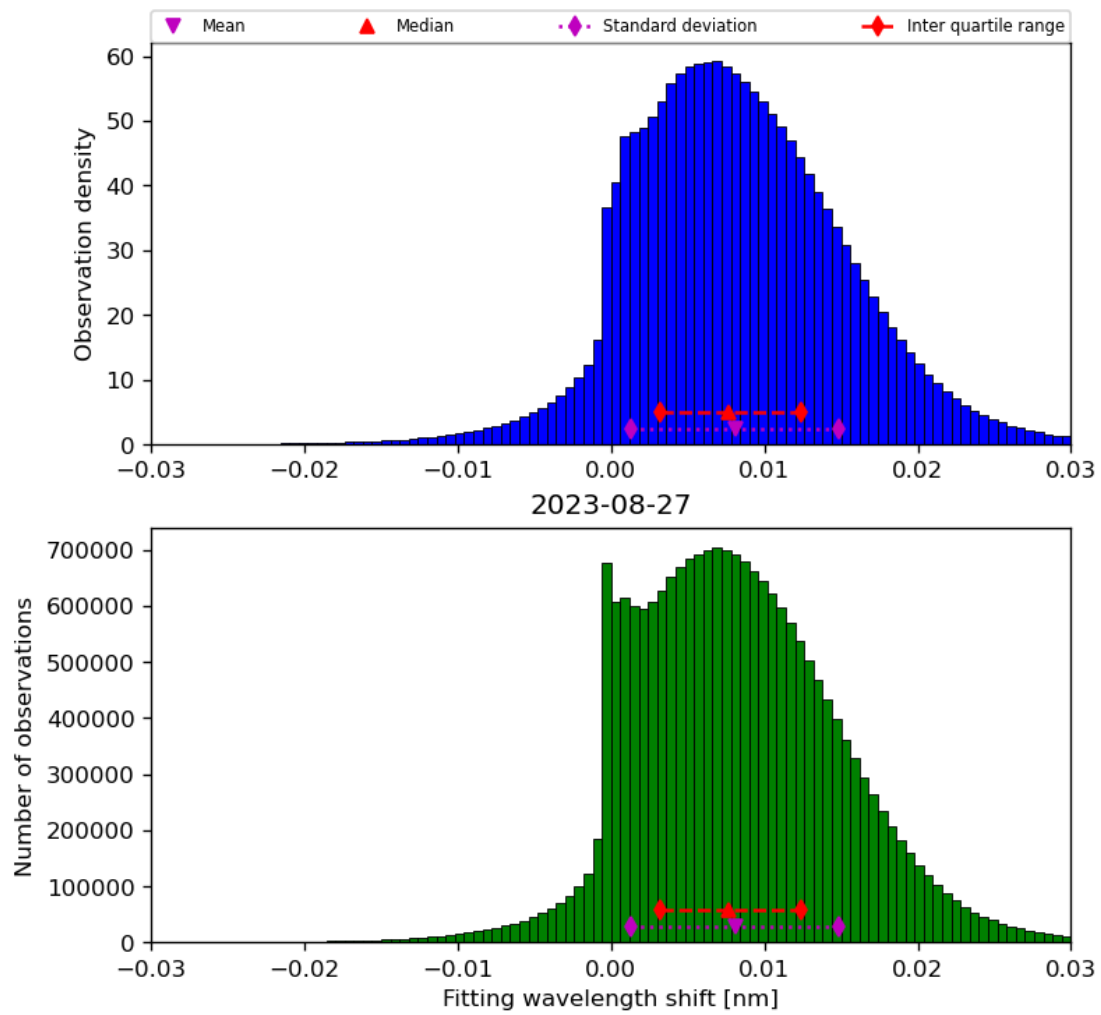
Figure 49: Histogram of “Fitting wavelength shift” for 2023-08-26 to 2023-08-28
