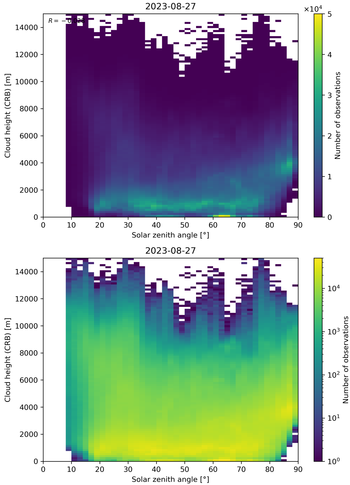
Figure 102: Scatter density plot of “Solar zenith angle” against “Cloud height (CRB)” for 2023-08-26 to 2023-08-28.
