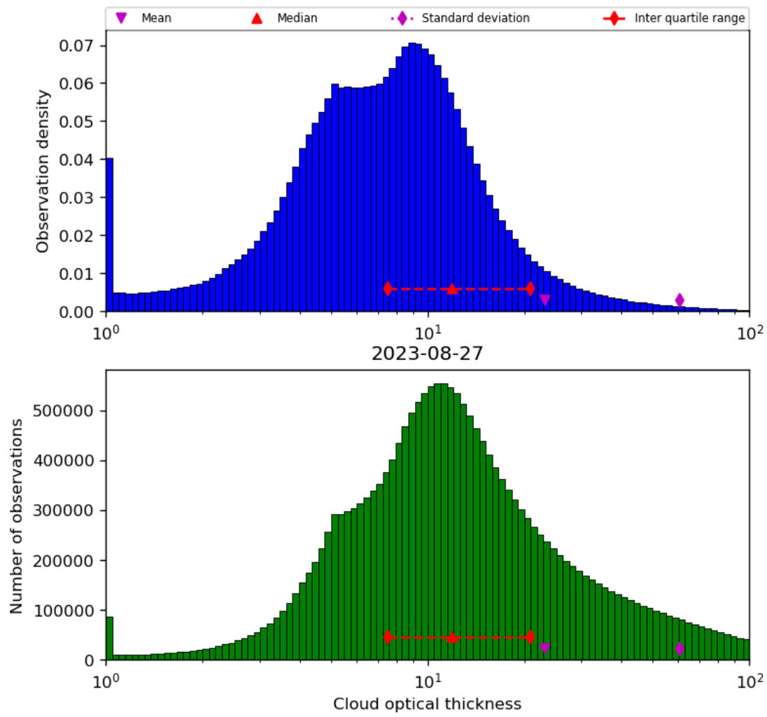
Figure 41: Histogram of “Cloud optical thickness” for 2023-08-26 to 2023-08-28
