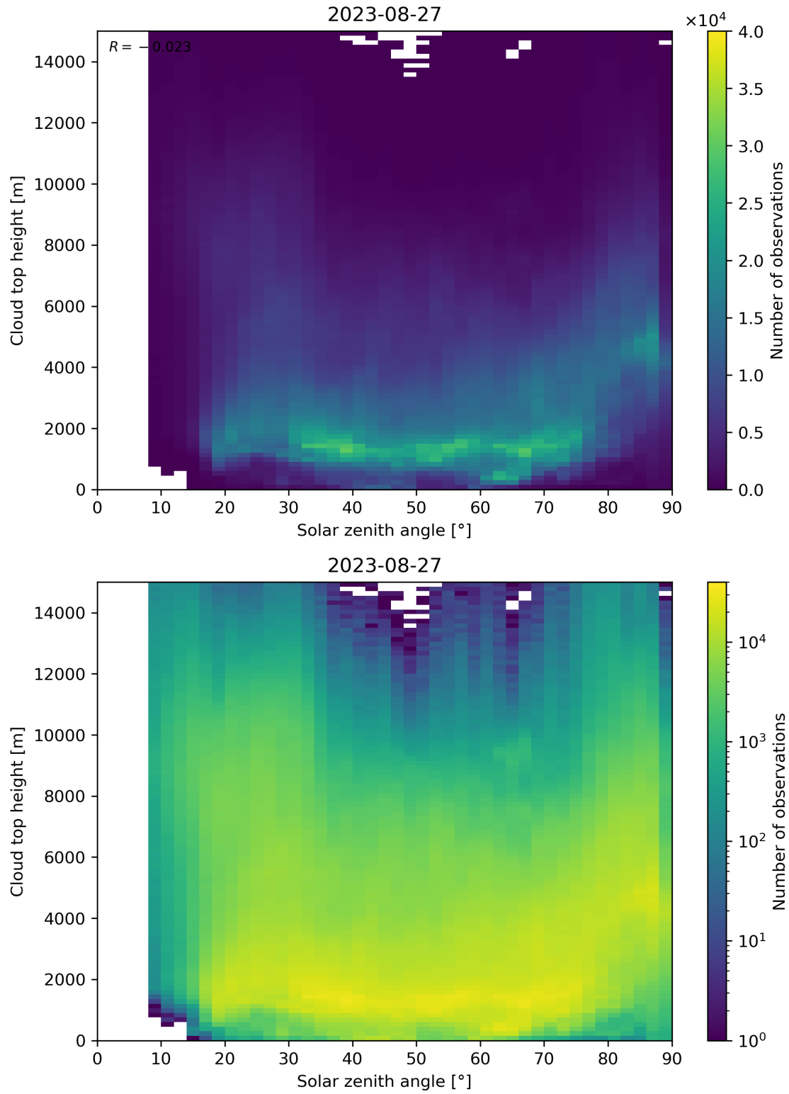
Figure 104: Scatter density plot of “Solar zenith angle” against “Cloud top height” for 2023-08-26 to 2023-08-28.
