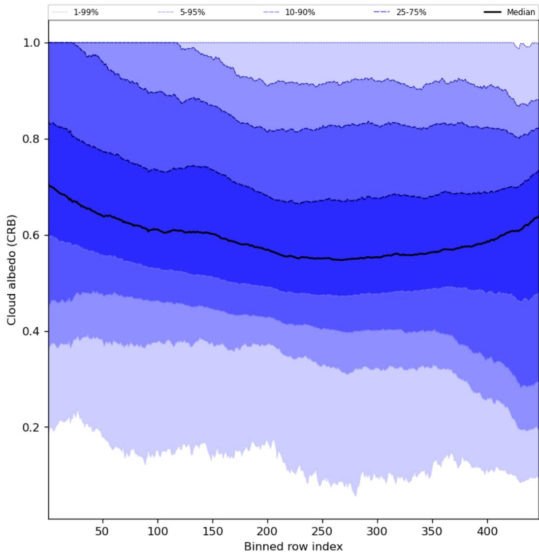
Figure 60: Along track statistics of “Cloud albedo (CRB)” for 2023-08-26 to 2023-08-28
