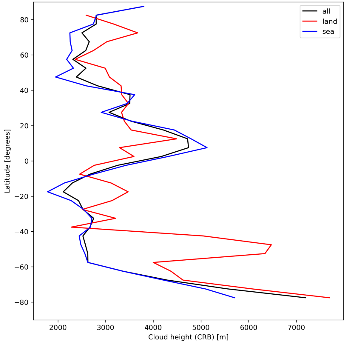
Figure 27: Zonal average of “Cloud height (CRB)” for 2023-08-26 to 2023-08-28.
