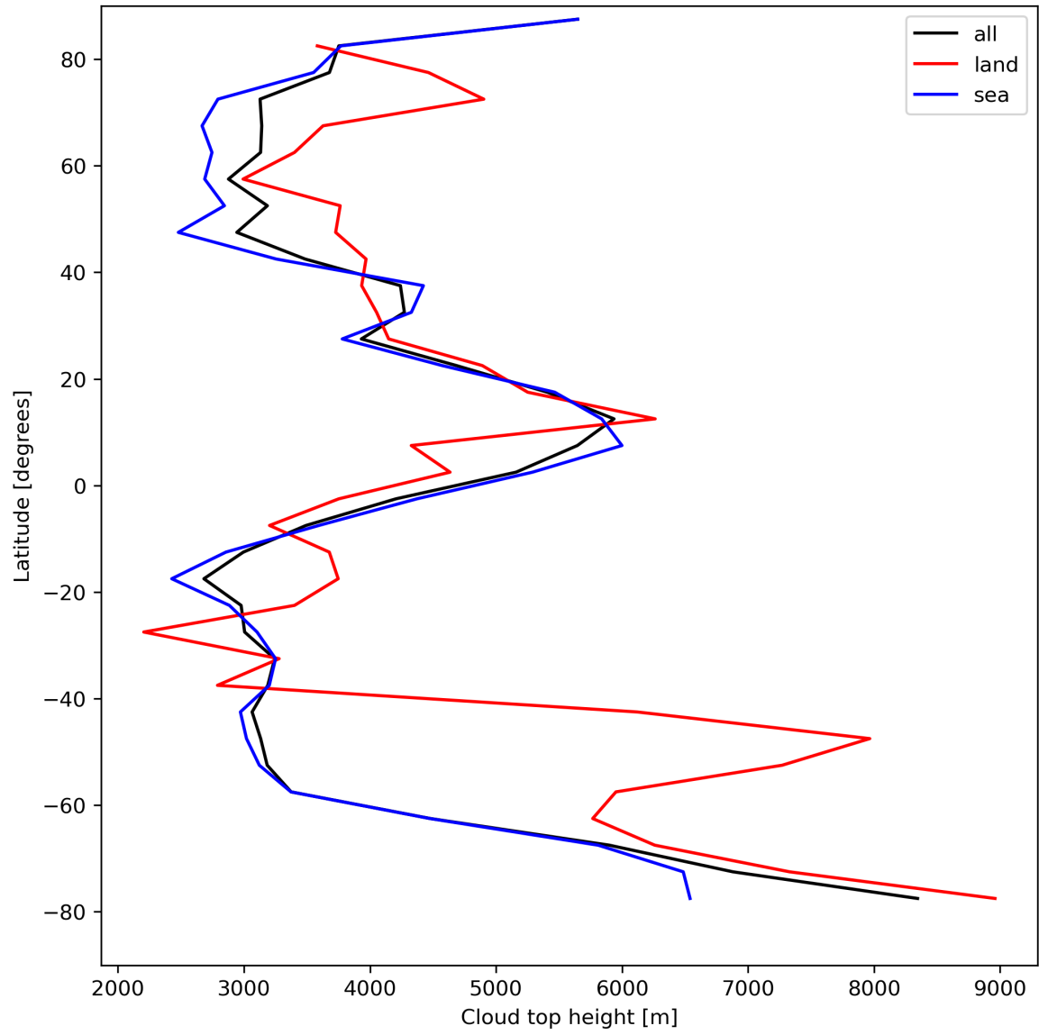
Figure 24: Zonal average of “Cloud top height” for 2023-08-26 to 2023-08-28.
