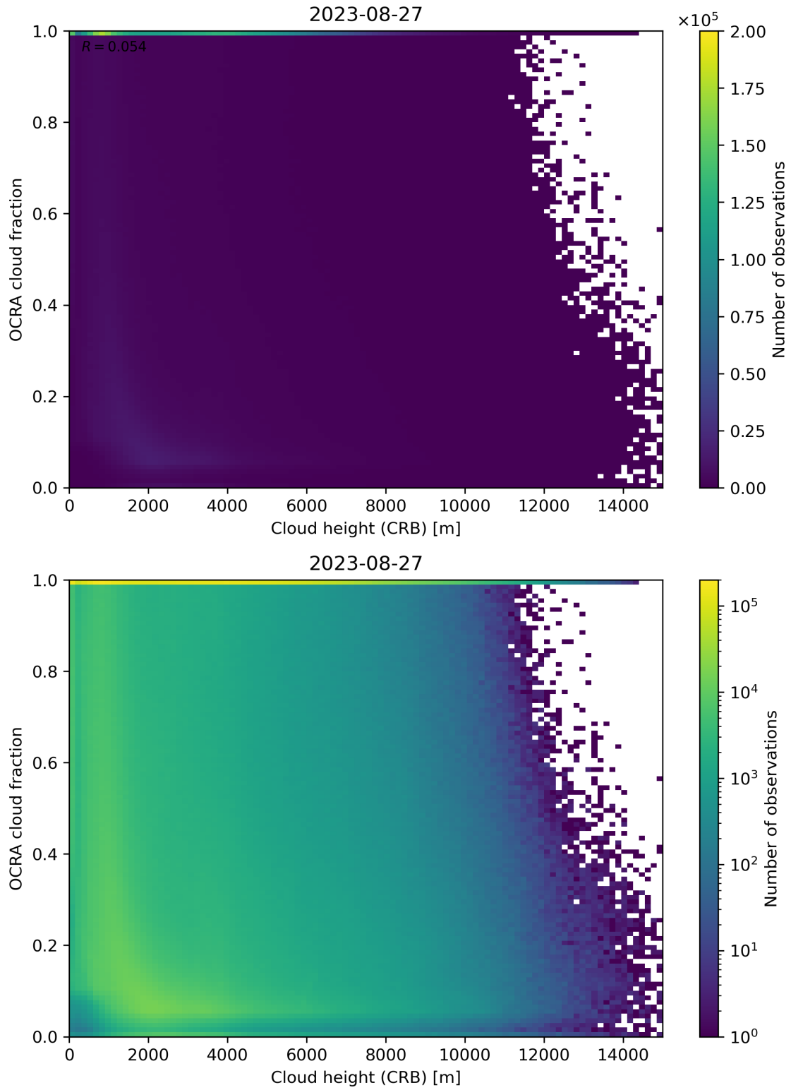
Figure 81: Scatter density plot of “Cloud height (CRB)” against “OCRA cloud fraction” for 2023-08-26 to 2023-08-28.
