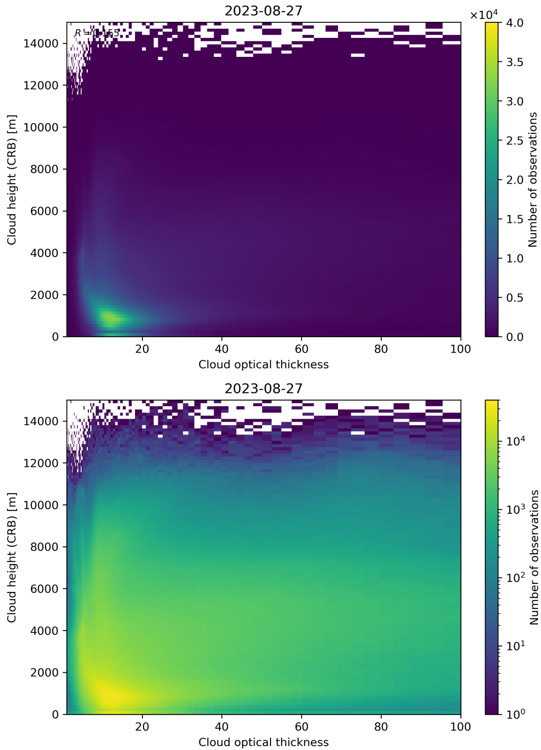
Figure 85: Scatter density plot of “Cloud optical thickness” against “Cloud height (CRB)” for 2023-08-26 to 2023-08-28.
