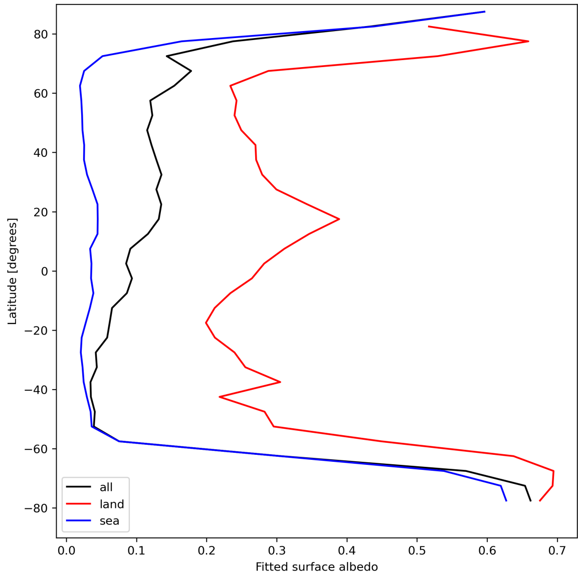
Figure 29: Zonal average of “Fitted surface albedo” for 2023-08-26 to 2023-08-28.
