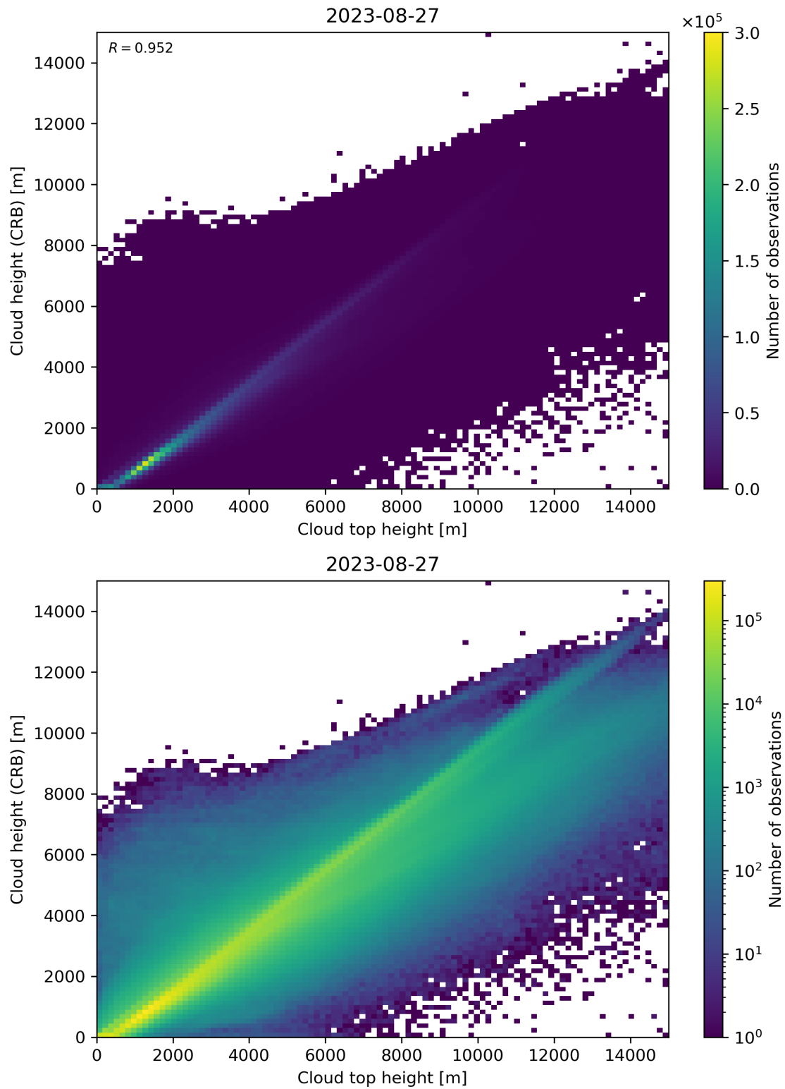
Figure 89: Scatter density plot of “Cloud top height” against “Cloud height (CRB)” for 2023-08-26 to 2023-08-28.
