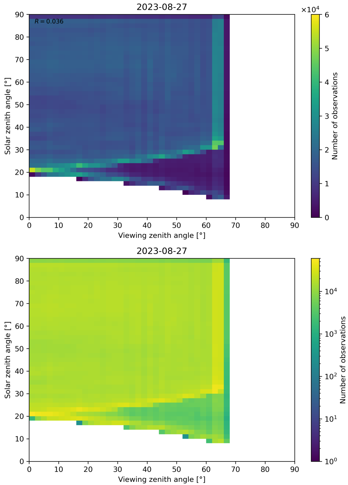
Figure 114: Scatter density plot of “Viewing zenith angle” against “Solar zenith angle” for 2023-08-26 to 2023-08-28.
