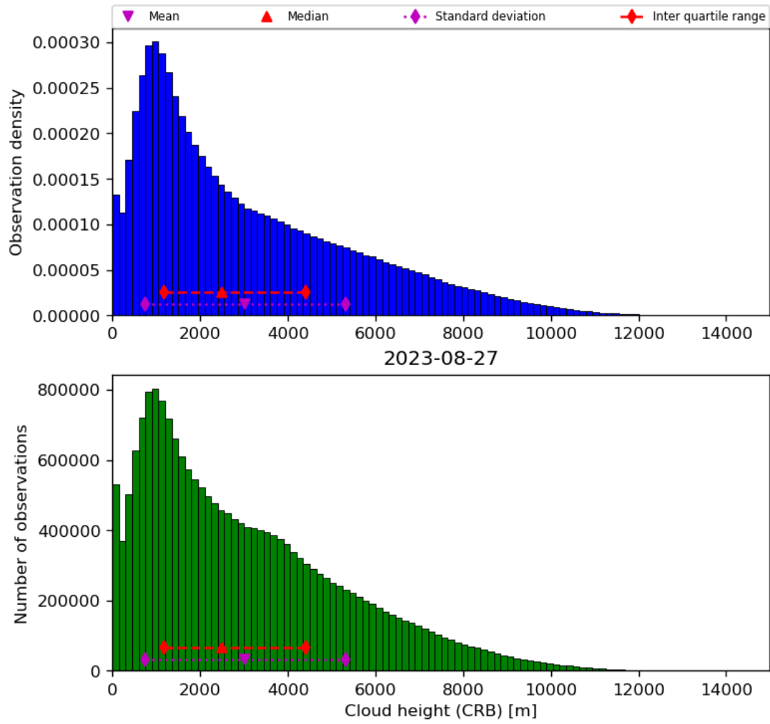
Figure 43: Histogram of “Cloud height (CRB)” for 2023-08-26 to 2023-08-28
