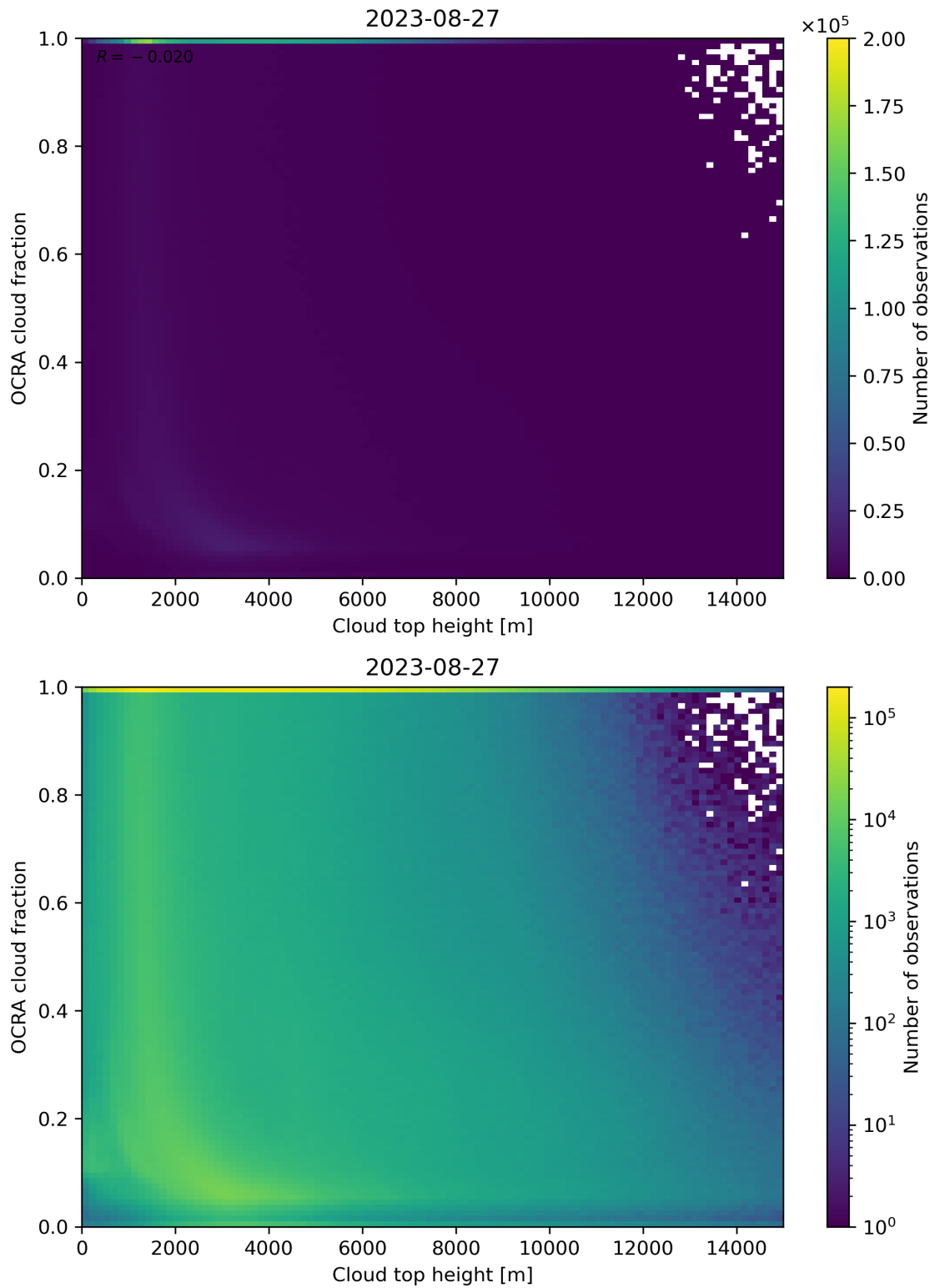
Figure 87: Scatter density plot of “Cloud top height” against “OCRA cloud fraction” for 2023-08-26 to 2023-08-28.
