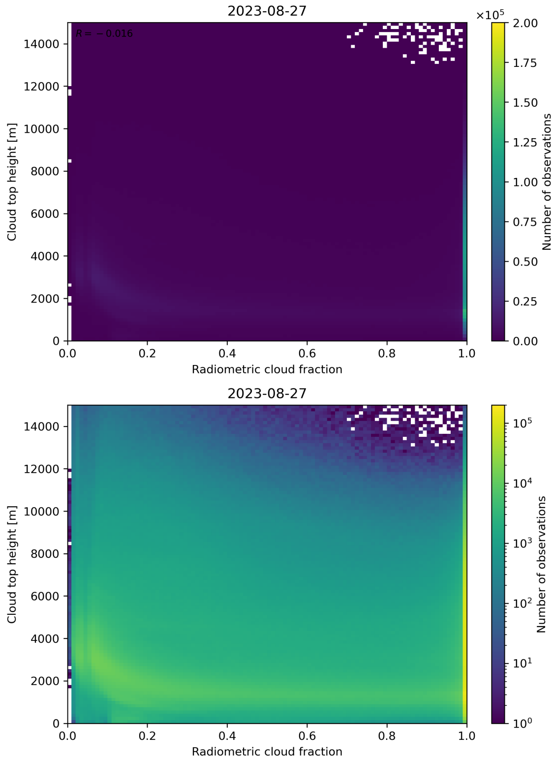
Figure 76: Scatter density plot of “Radiometric cloud fraction” against “Cloud top height” for 2023-08-26 to 2023-08-28.
