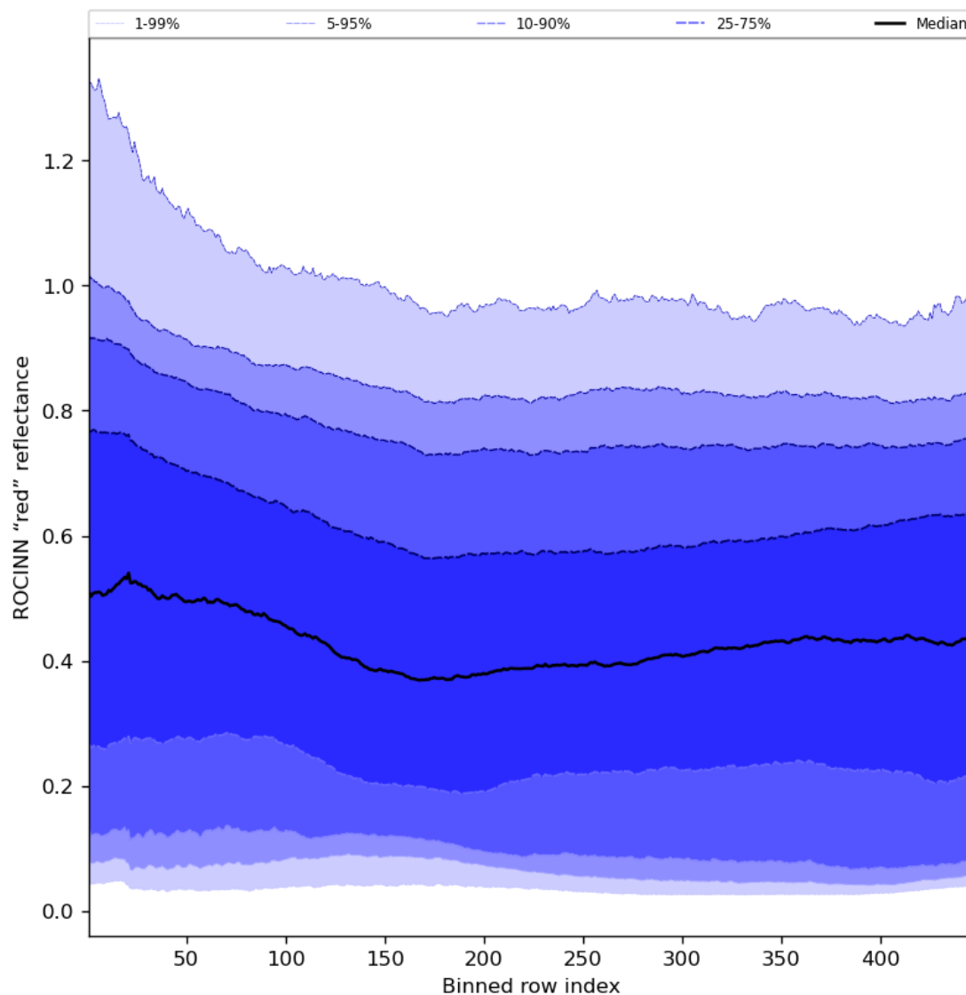
Figure 69: Along track statistics of “ROCINN “red” reflectance” for 2023-08-26 to 2023-08-28
