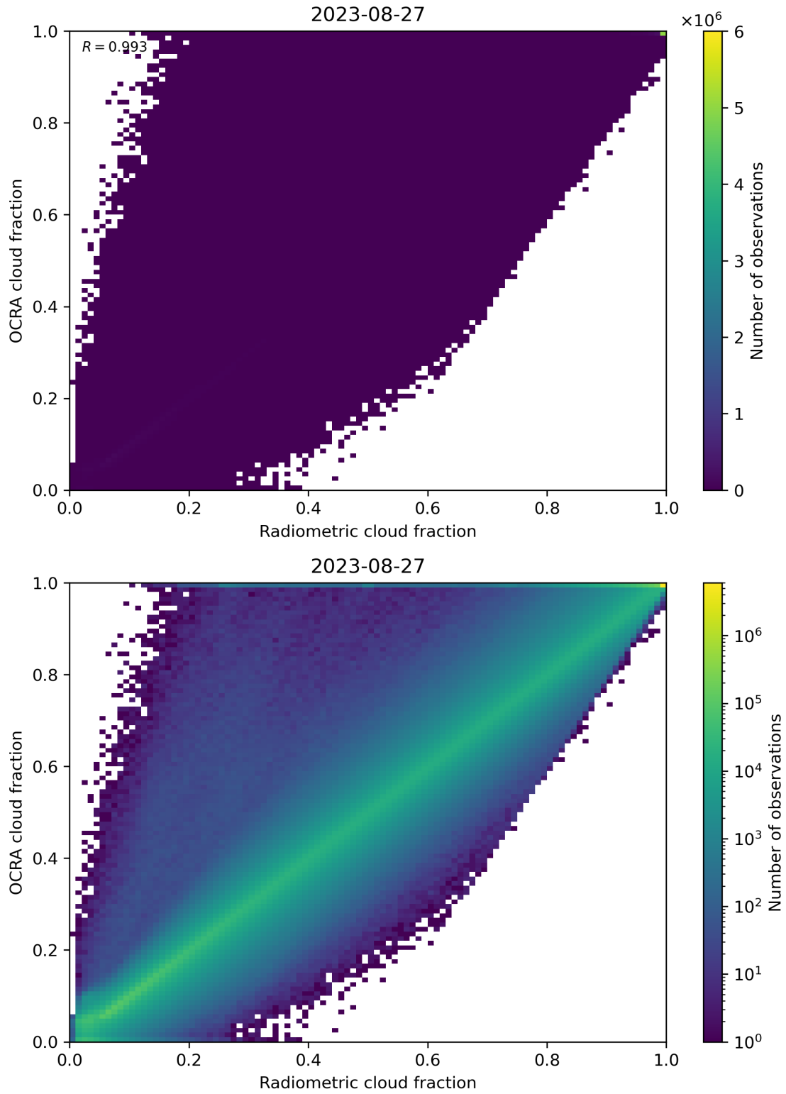
Figure 72: Scatter density plot of “Radiometric cloud fraction” against “OCRA cloud fraction” for 2023-08-26 to 2023-08-28.
