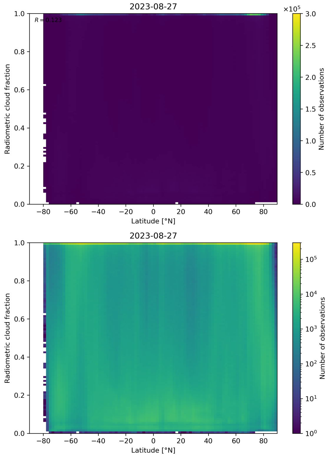
Figure 92: Scatter density plot of “Latitude” against “Radiometric cloud fraction” for 2023-08-26 to 2023-08-28.
