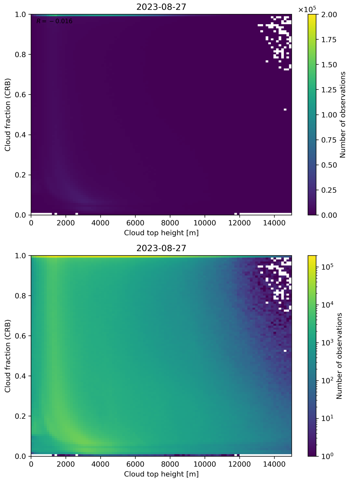
Figure 88: Scatter density plot of “Cloud top height” against “Cloud fraction (CRB)” for 2023-08-26 to 2023-08-28.
