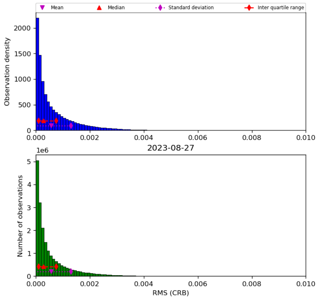
Figure 48: Histogram of “RMS (CRB)” for 2023-08-26 to 2023-08-28
