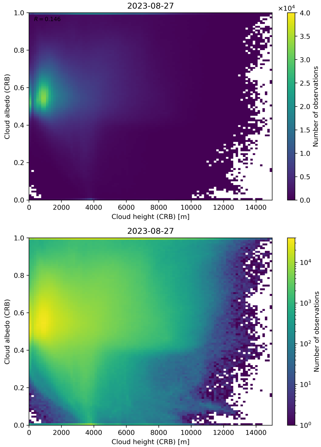
Figure 80: Scatter density plot of “Cloud height (CRB)” against “Cloud albedo (CRB)” for 2023-08-26 to 2023-08-28.
