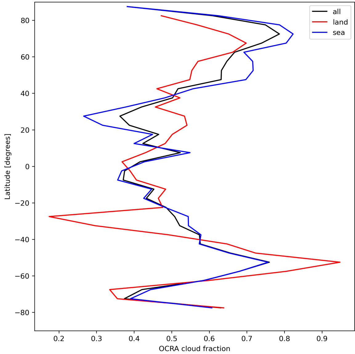
Figure 34: Zonal average of “OCRA cloud fraction” for 2023-08-26 to 2023-08-28.
