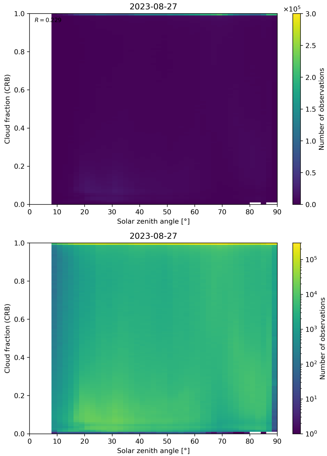
Figure 101: Scatter density plot of “Solar zenith angle” against “Cloud fraction (CRB)” for 2023-08-26 to 2023-08-28.
