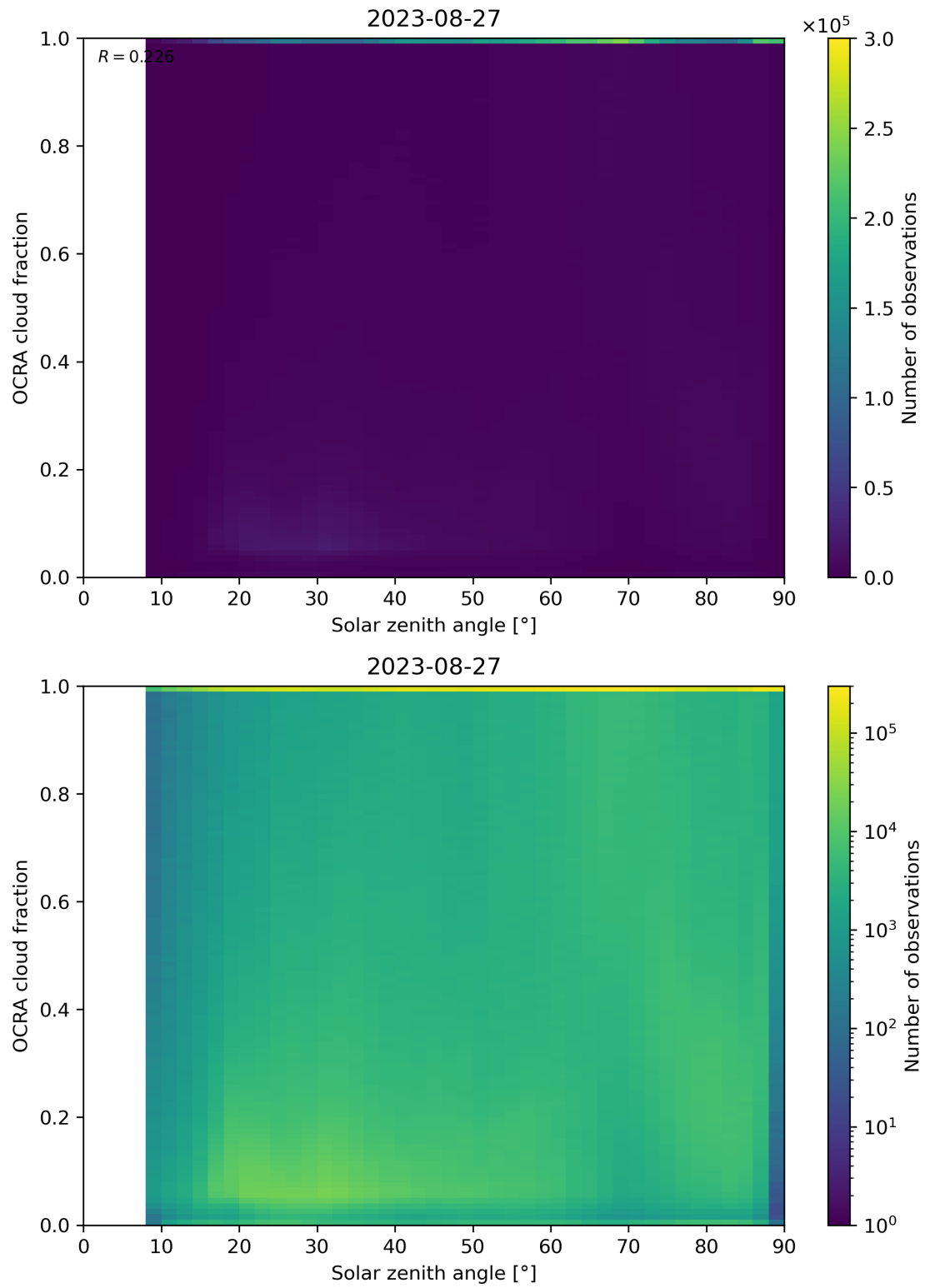
Figure 100: Scatter density plot of “Solar zenith angle” against “OCRA cloud fraction” for 2023-08-26 to 2023-08-28.
