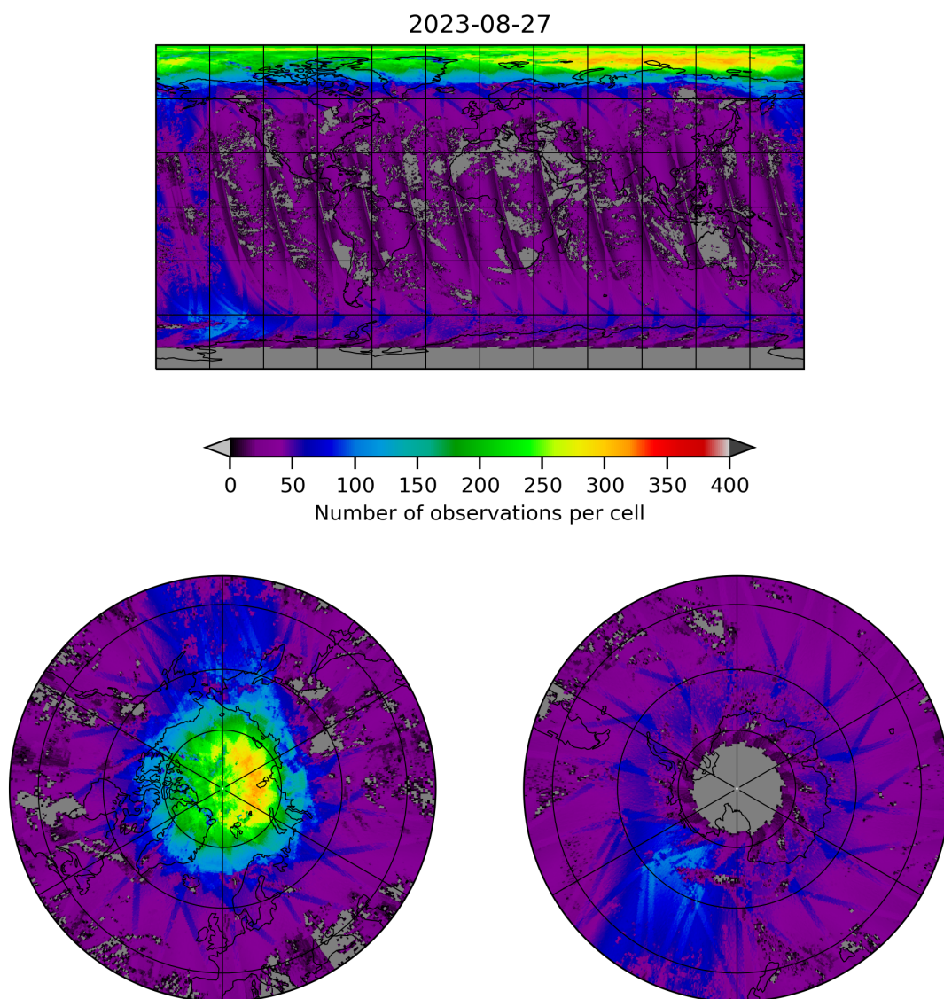
Figure 21: Map of the number of observations for 2023-08-26 to 2023-08-28
