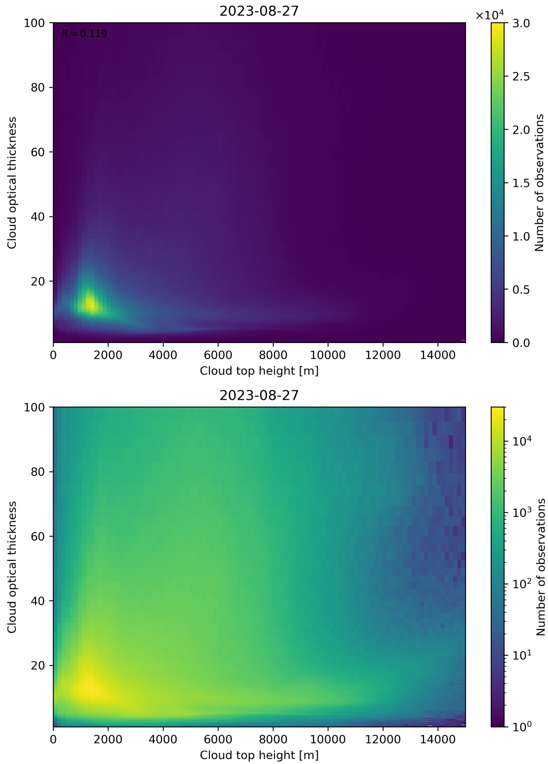
Figure 90: Scatter density plot of “Cloud top height” against “Cloud optical thickness” for 2023-08-26 to 2023-08-28.
