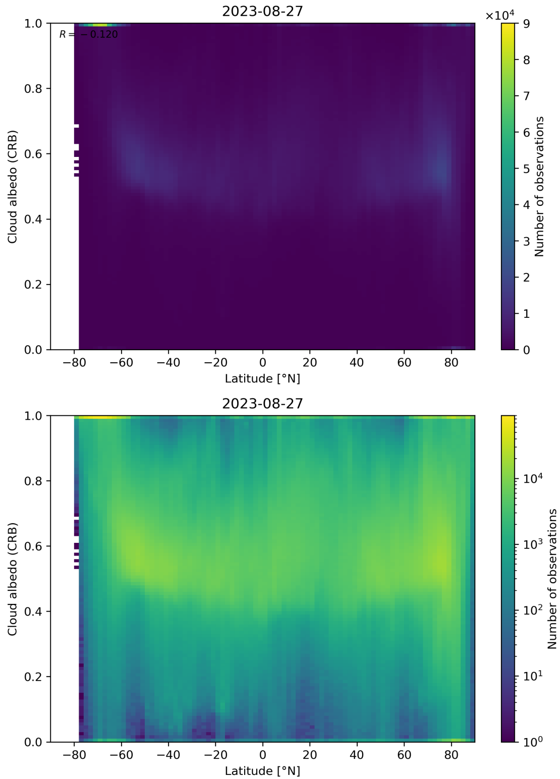
Figure 91: Scatter density plot of “Latitude” against “Cloud albedo (CRB)” for 2023-08-26 to 2023-08-28.
