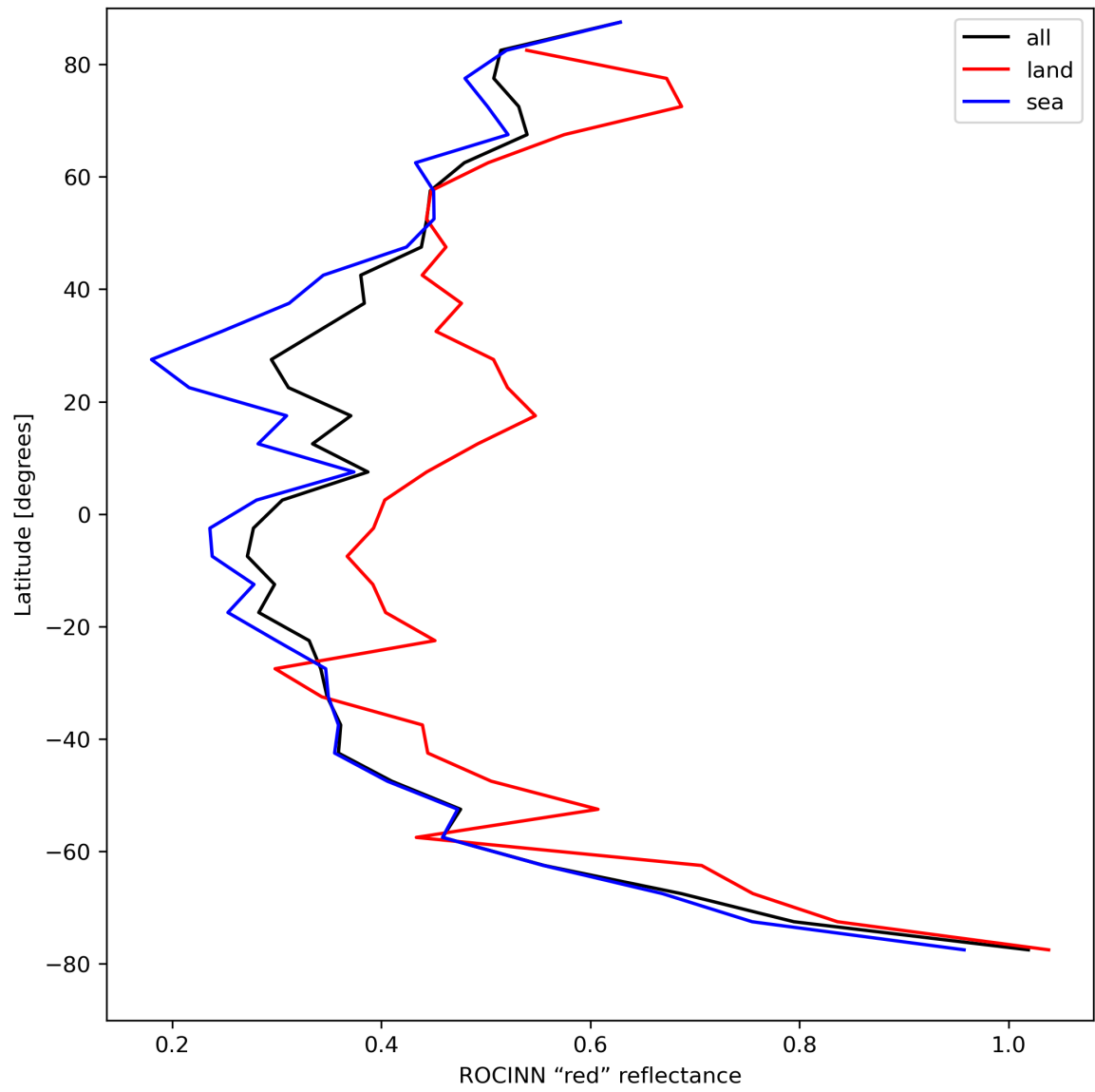
Figure 37: Zonal average of “ROCINN “red” reflectance” for 2023-08-26 to 2023-08-28.
