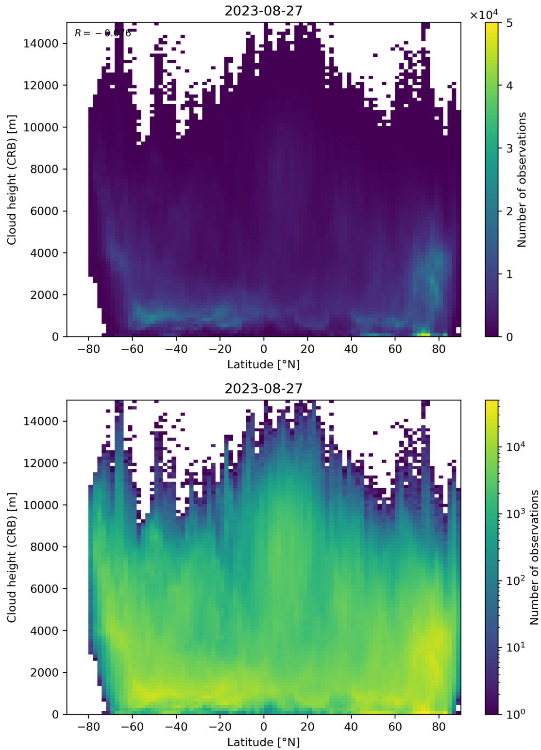
Figure 95: Scatter density plot of “Latitude” against “Cloud height (CRB)” for 2023-08-26 to 2023-08-28.
