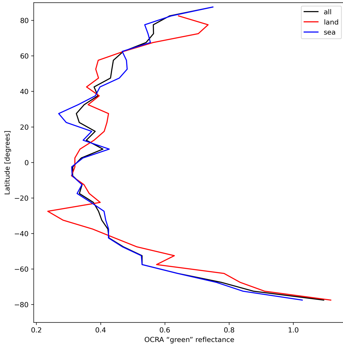
Figure 36: Zonal average of “OCRA “green” reflectance” for 2023-08-26 to 2023-08-28.
