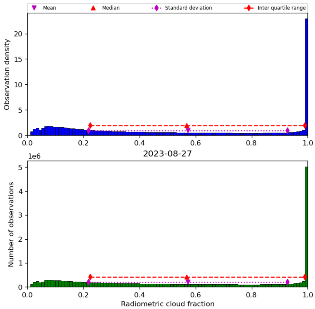
Figure 39: Histogram of “Radiometric cloud fraction” for 2023-08-26 to 2023-08-28
