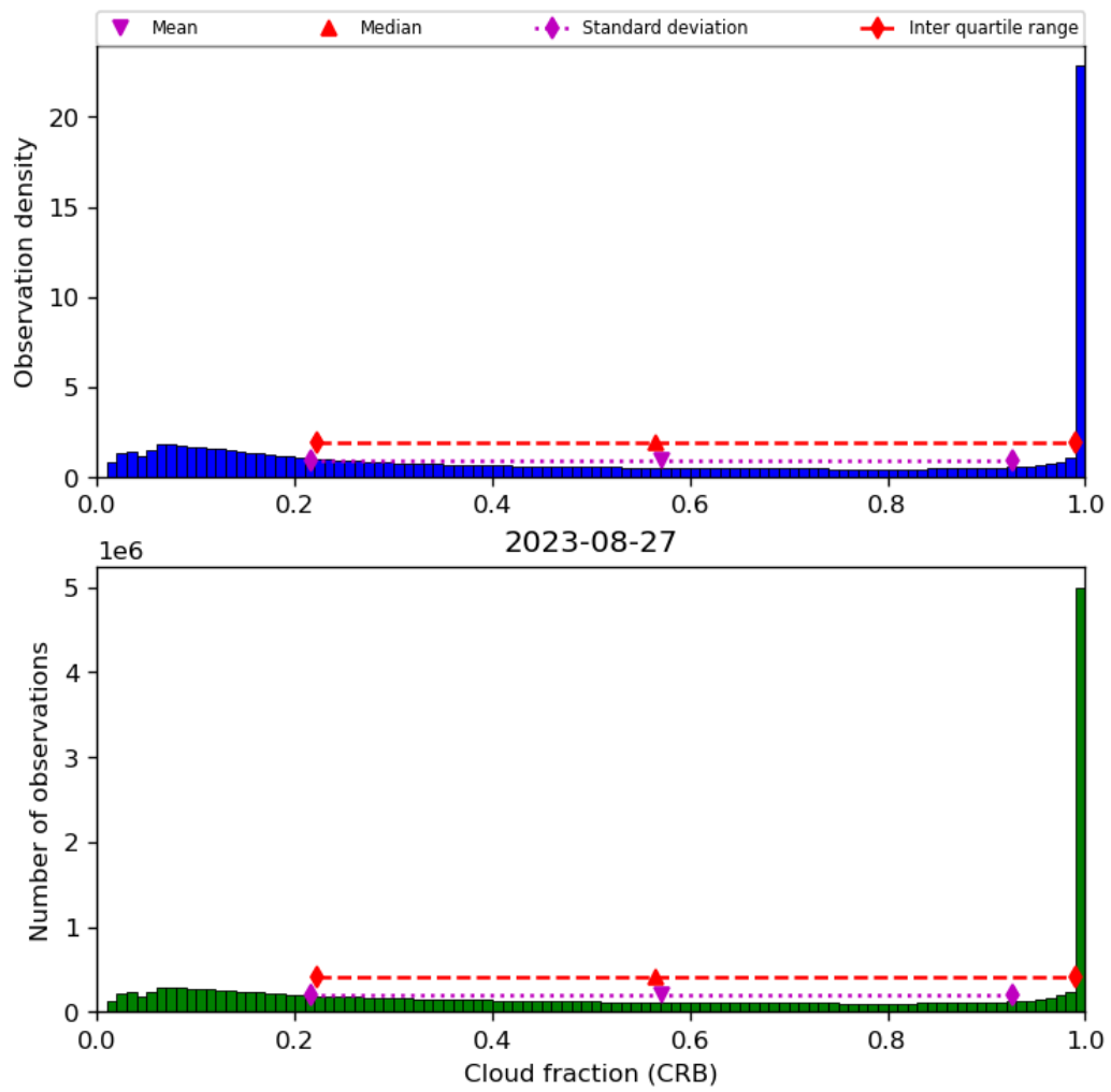
Figure 42: Histogram of “Cloud fraction (CRB)” for 2023-08-26 to 2023-08-28
