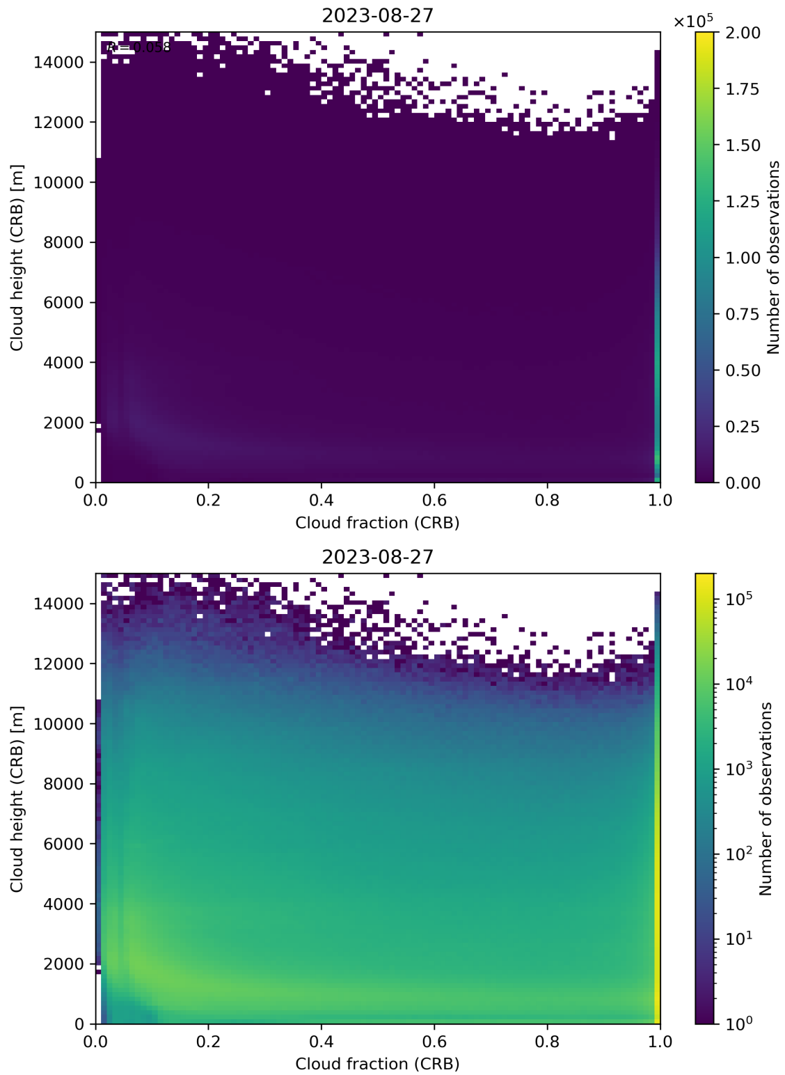
Figure 79: Scatter density plot of “Cloud fraction (CRB)” against “Cloud height (CRB)” for 2023-08-26 to 2023-08-28.
