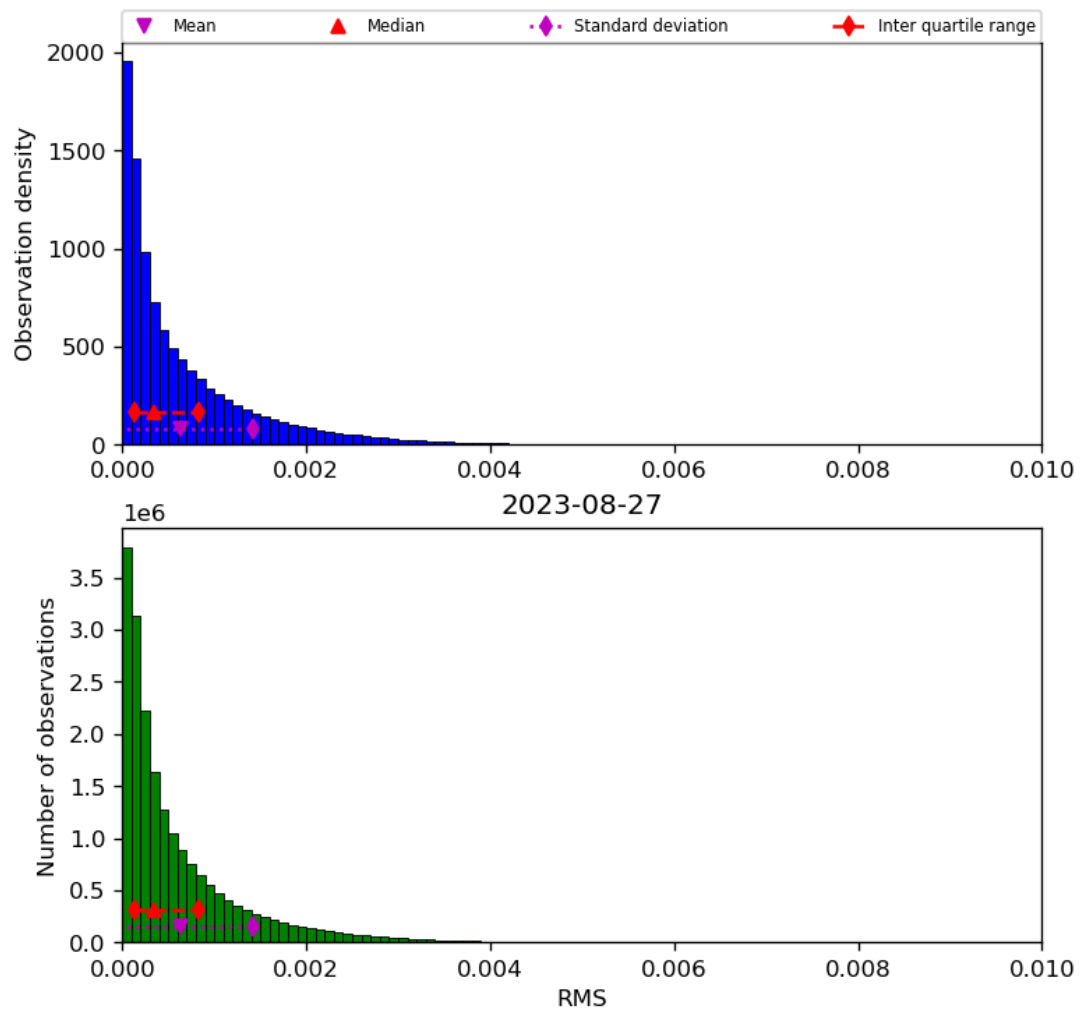
Figure 47: Histogram of “RMS” for 2023-08-26 to 2023-08-28
