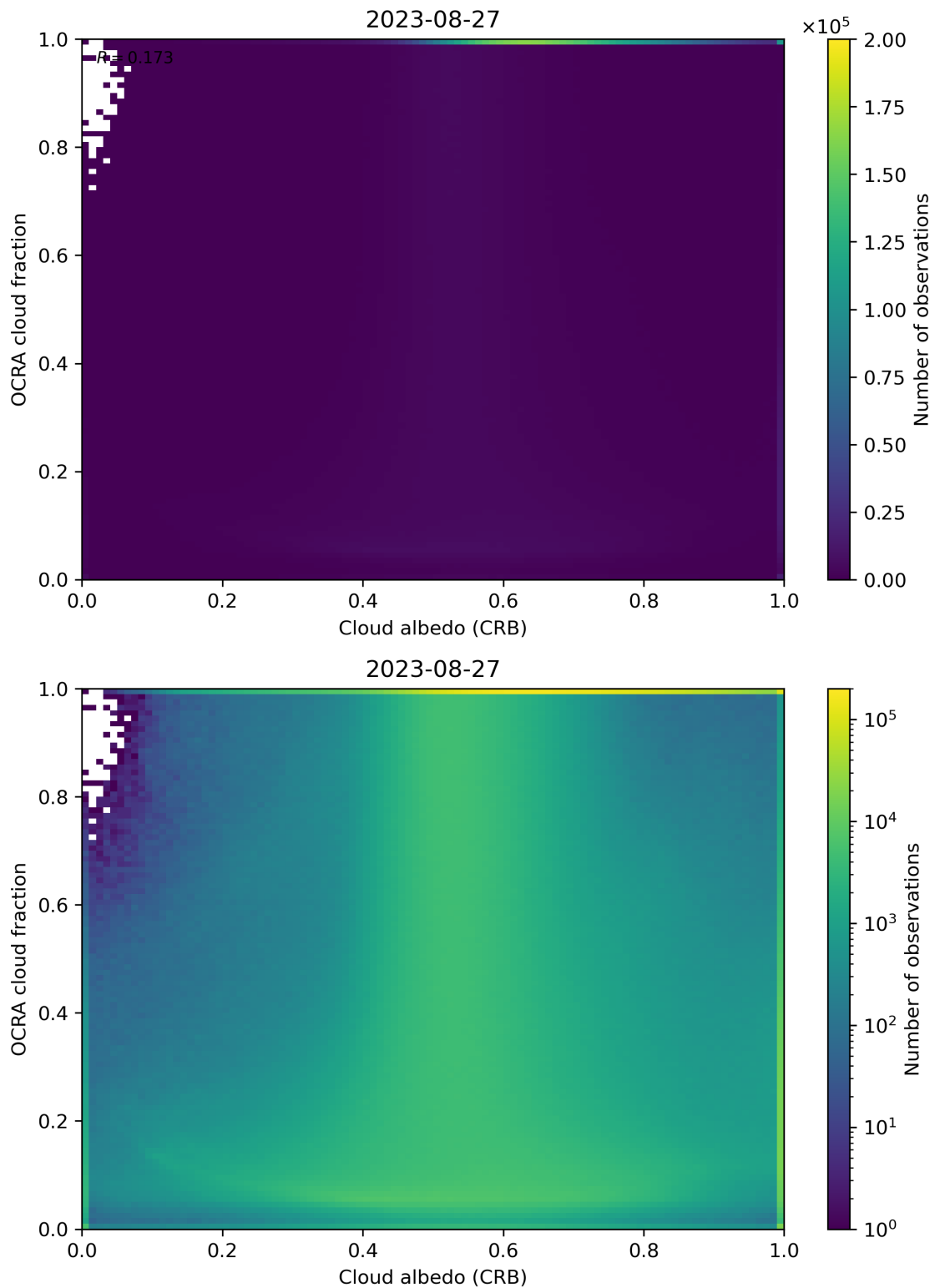
Figure 70: Scatter density plot of “Cloud albedo (CRB)” against “OCRA cloud fraction” for 2023-08-26 to 2023-08-28.
