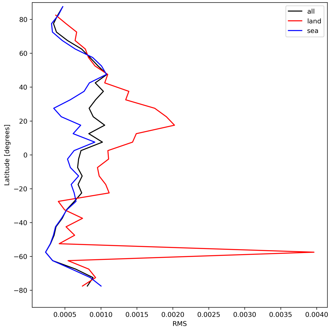
Figure 31: Zonal average of “RMS” for 2023-08-26 to 2023-08-28.
