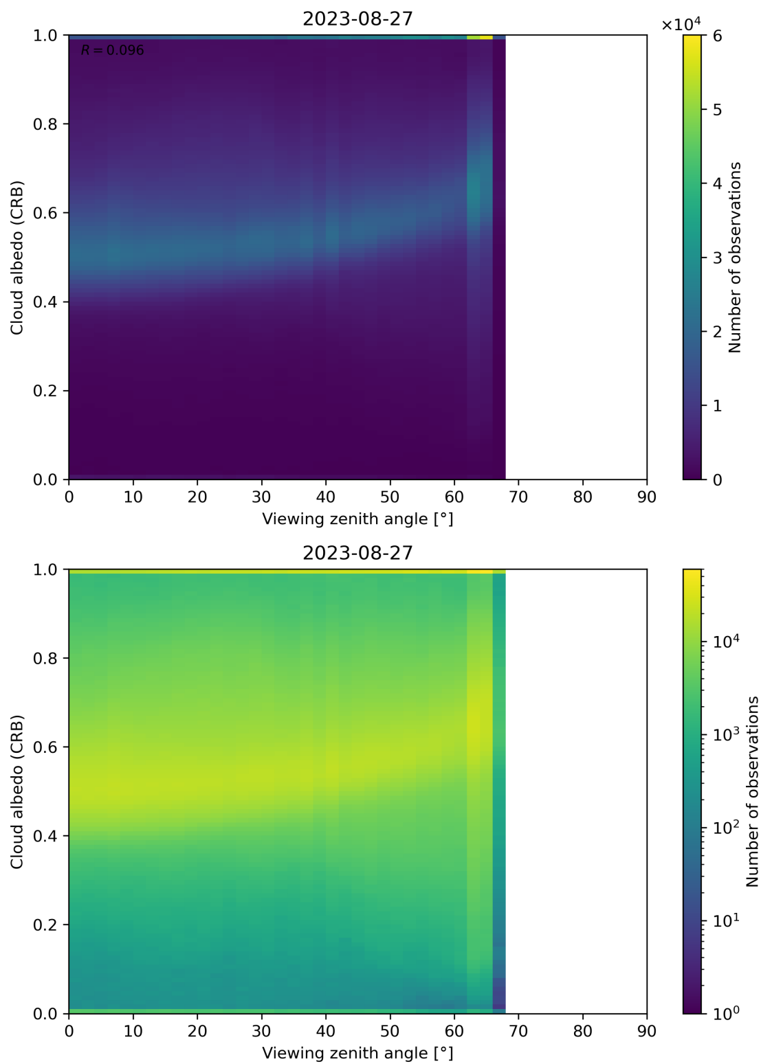
Figure 106: Scatter density plot of “Viewing zenith angle” against “Cloud albedo (CRB)” for 2023-08-26 to 2023-08-28.
