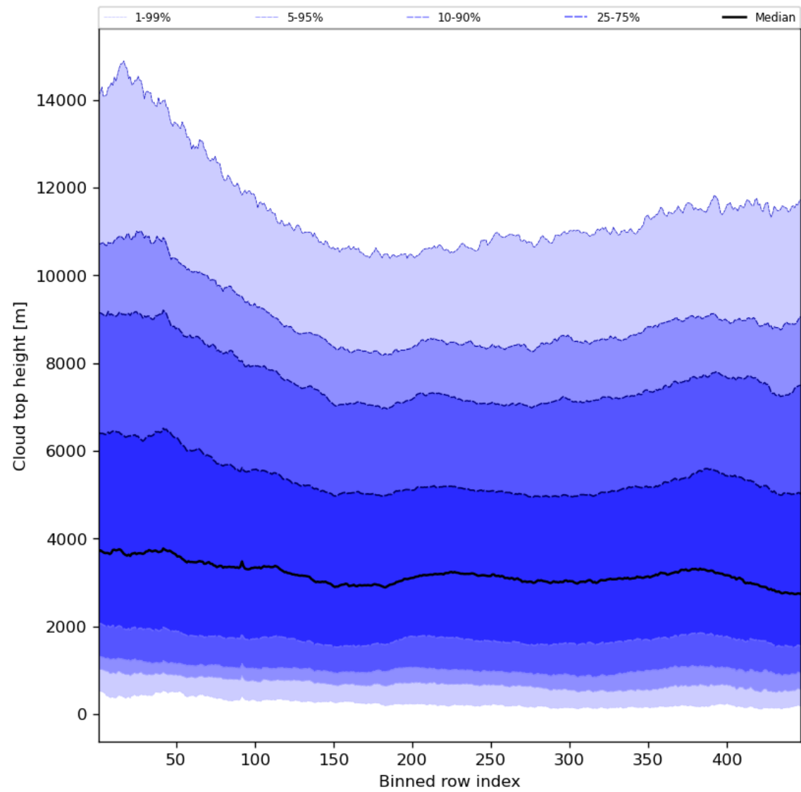
Figure 56: Along track statistics of “Cloud top height” for 2023-08-26 to 2023-08-28
