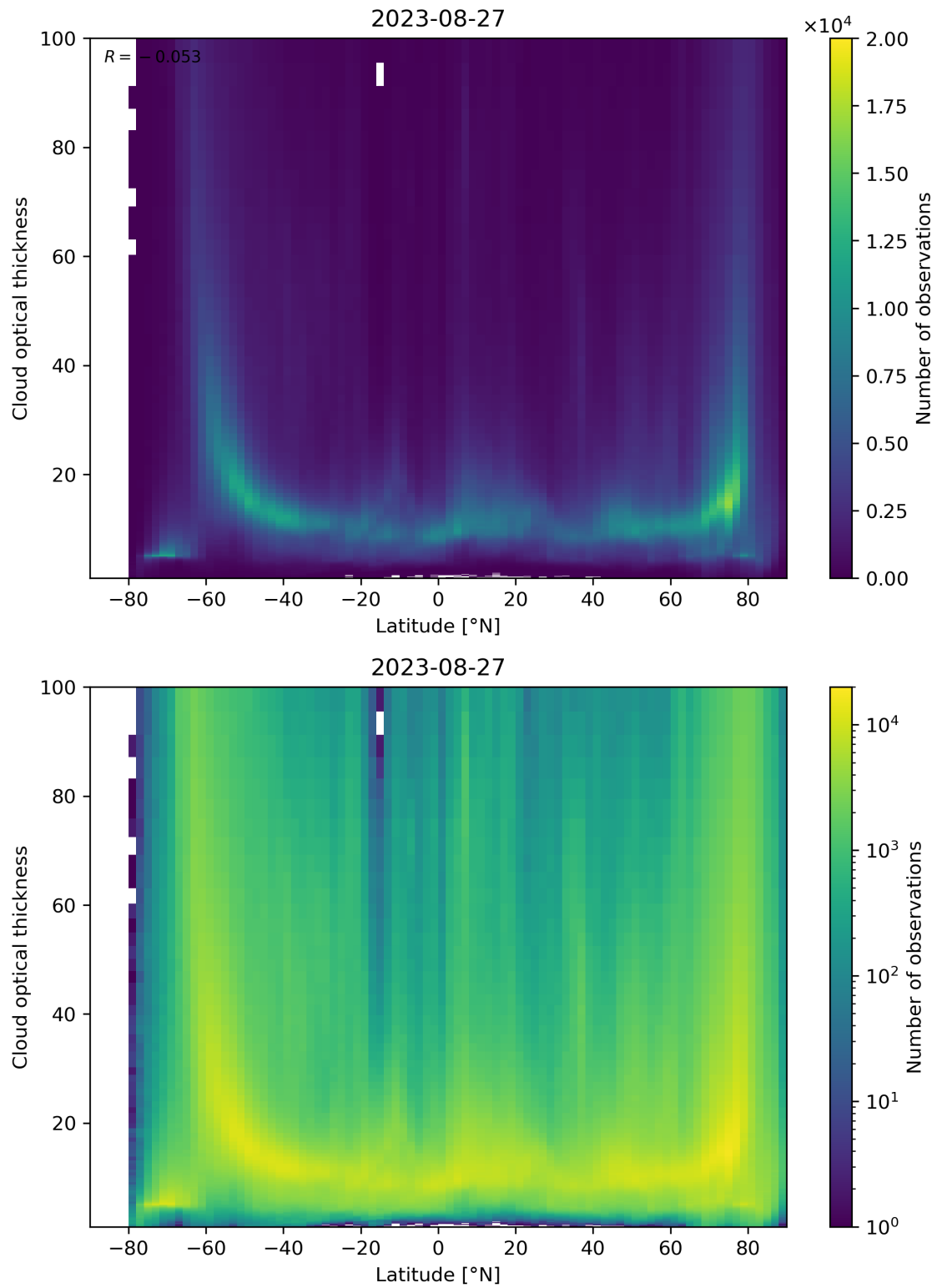
Figure 96: Scatter density plot of “Latitude” against “Cloud optical thickness” for 2023-08-26 to 2023-08-28.
