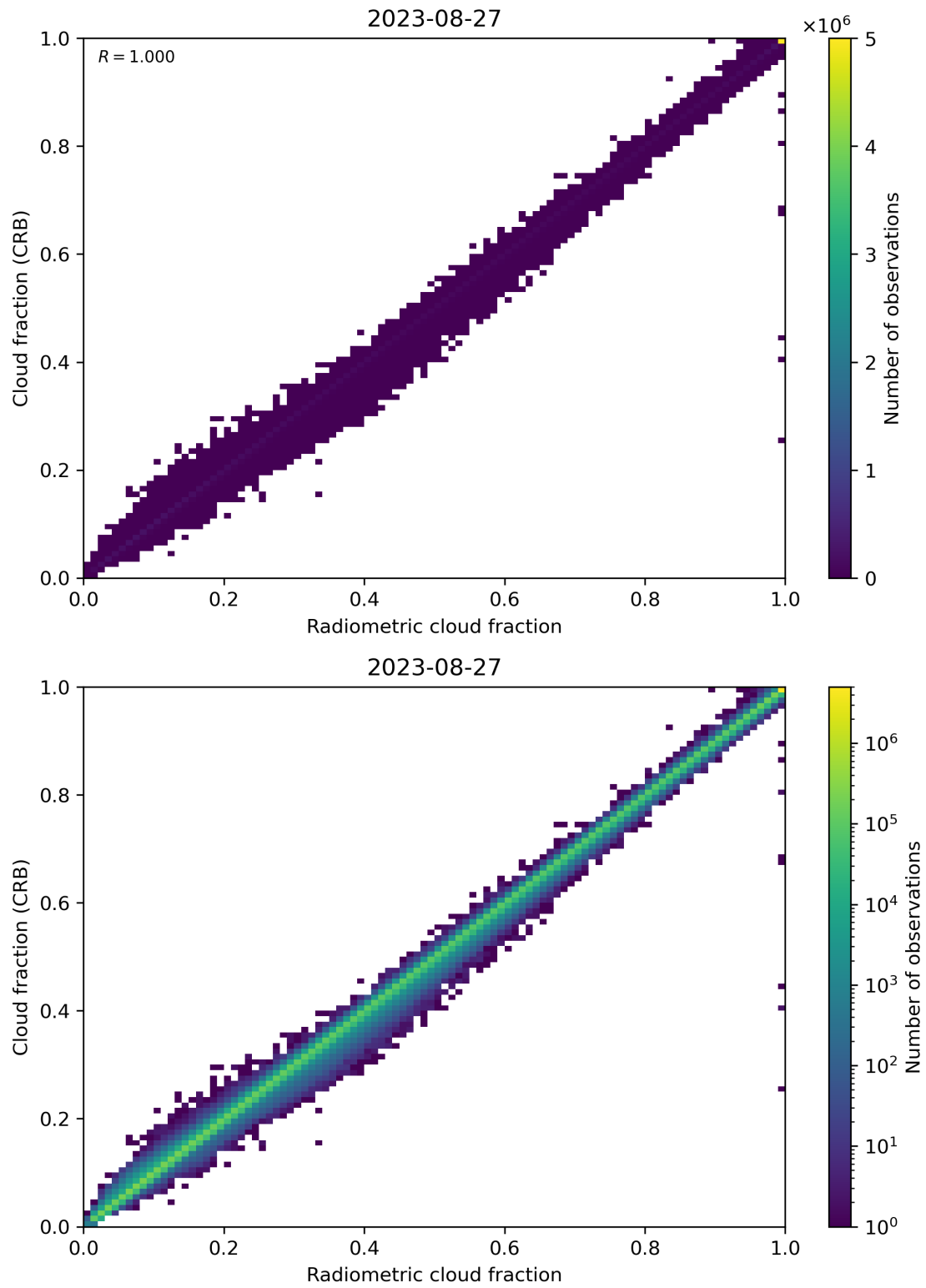
Figure 73: Scatter density plot of “Radiometric cloud fraction” against “Cloud fraction (CRB)” for 2023-08-26 to 2023-08-28.
