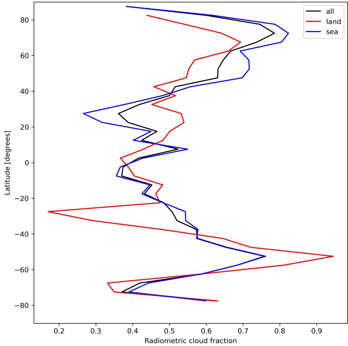
Figure 23: Zonal average of “Radiometric cloud fraction” for 2023-08-26 to 2023-08-28.
