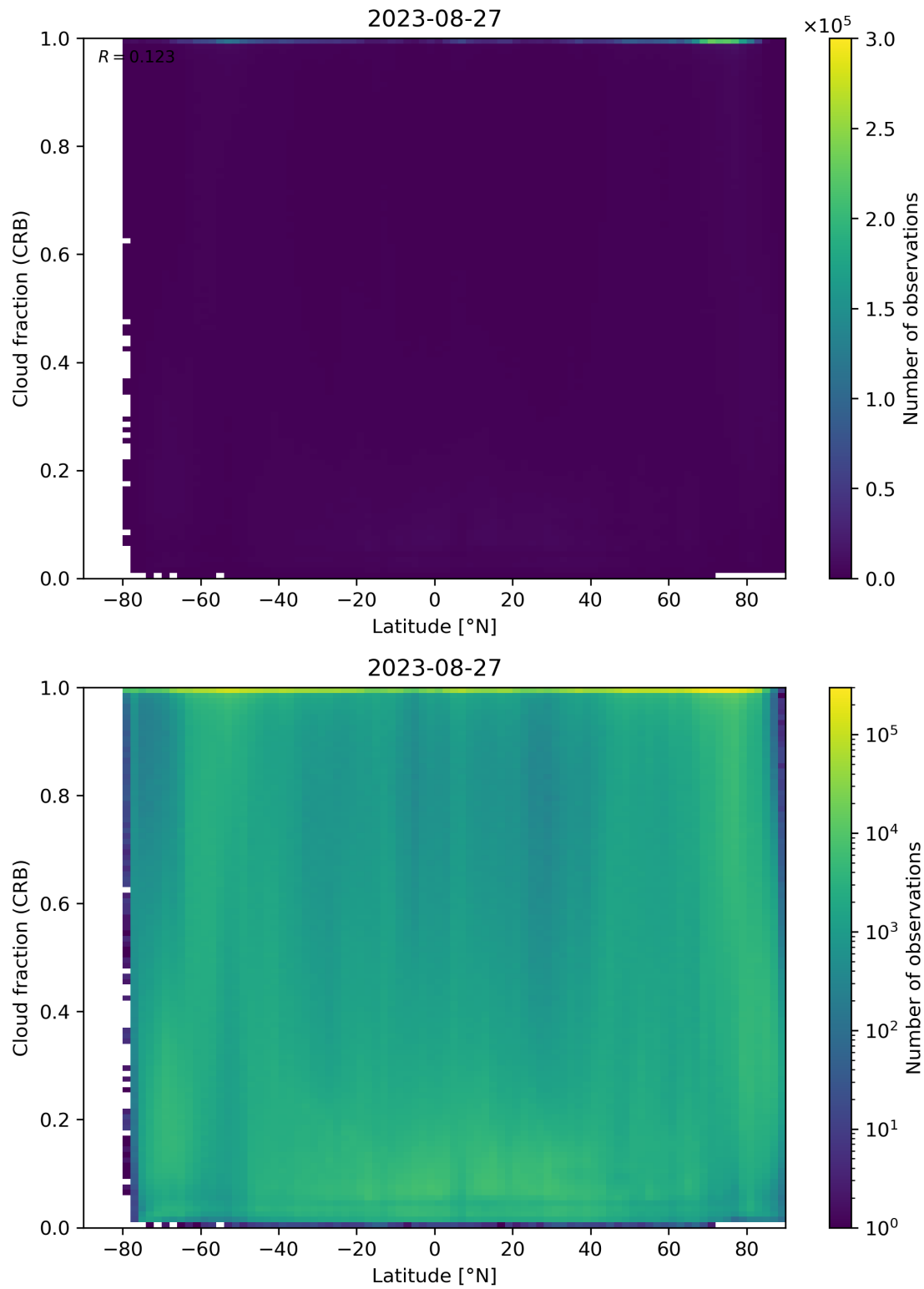
Figure 94: Scatter density plot of “Latitude” against “Cloud fraction (CRB)” for 2023-08-26 to 2023-08-28.
