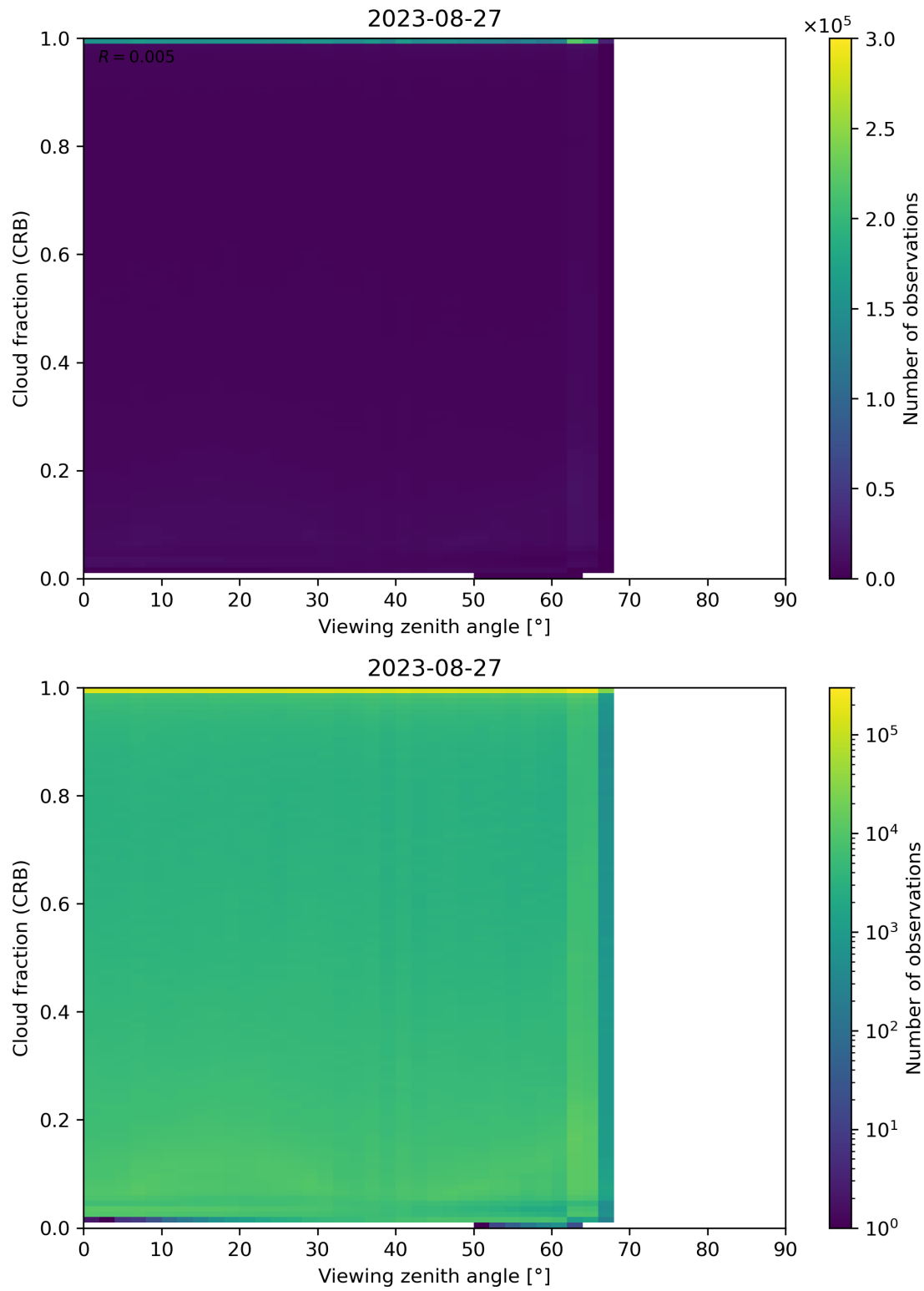
Figure 109: Scatter density plot of “Viewing zenith angle” against “Cloud fraction (CRB)” for 2023-08-26 to 2023-08-28.
