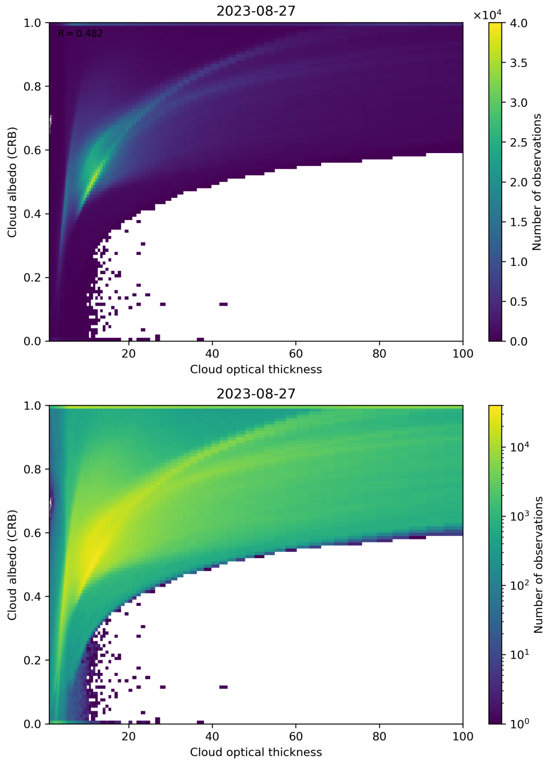
Figure 82: Scatter density plot of “Cloud optical thickness” against “Cloud albedo (CRB)” for 2023-08-26 to 2023-08-28.
