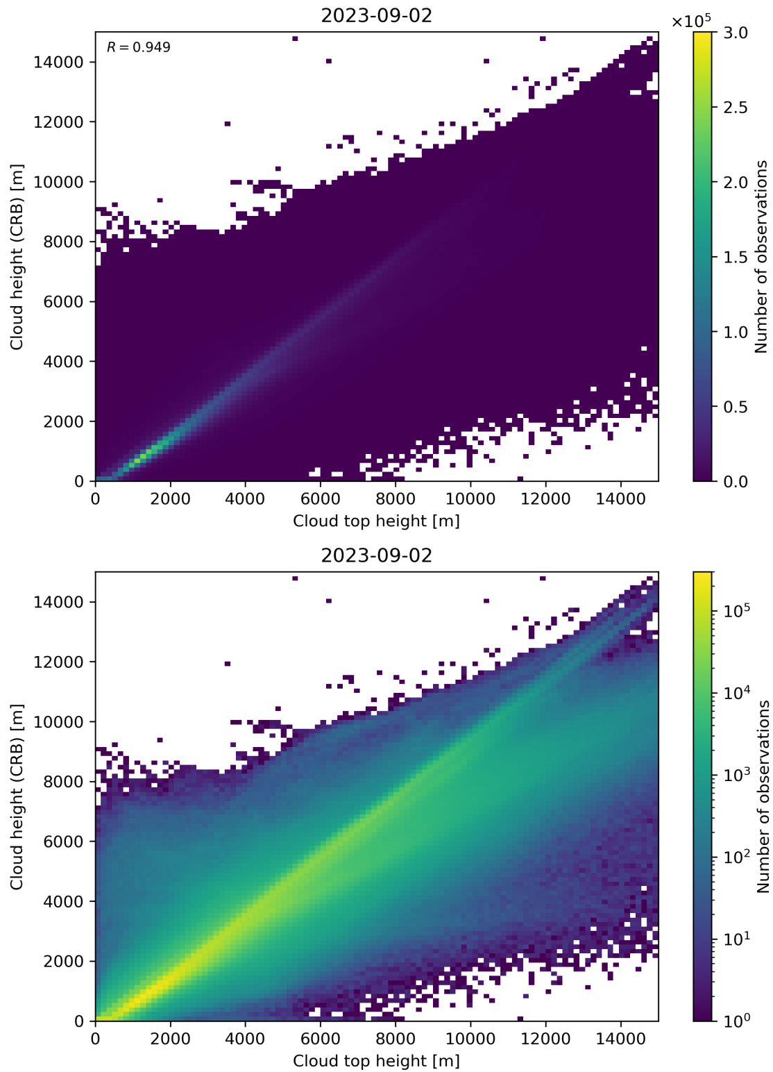
Figure 89: Scatter density plot of “Cloud top height” against “Cloud height (CRB)” for 2023-09-01 to 2023-09-03.
