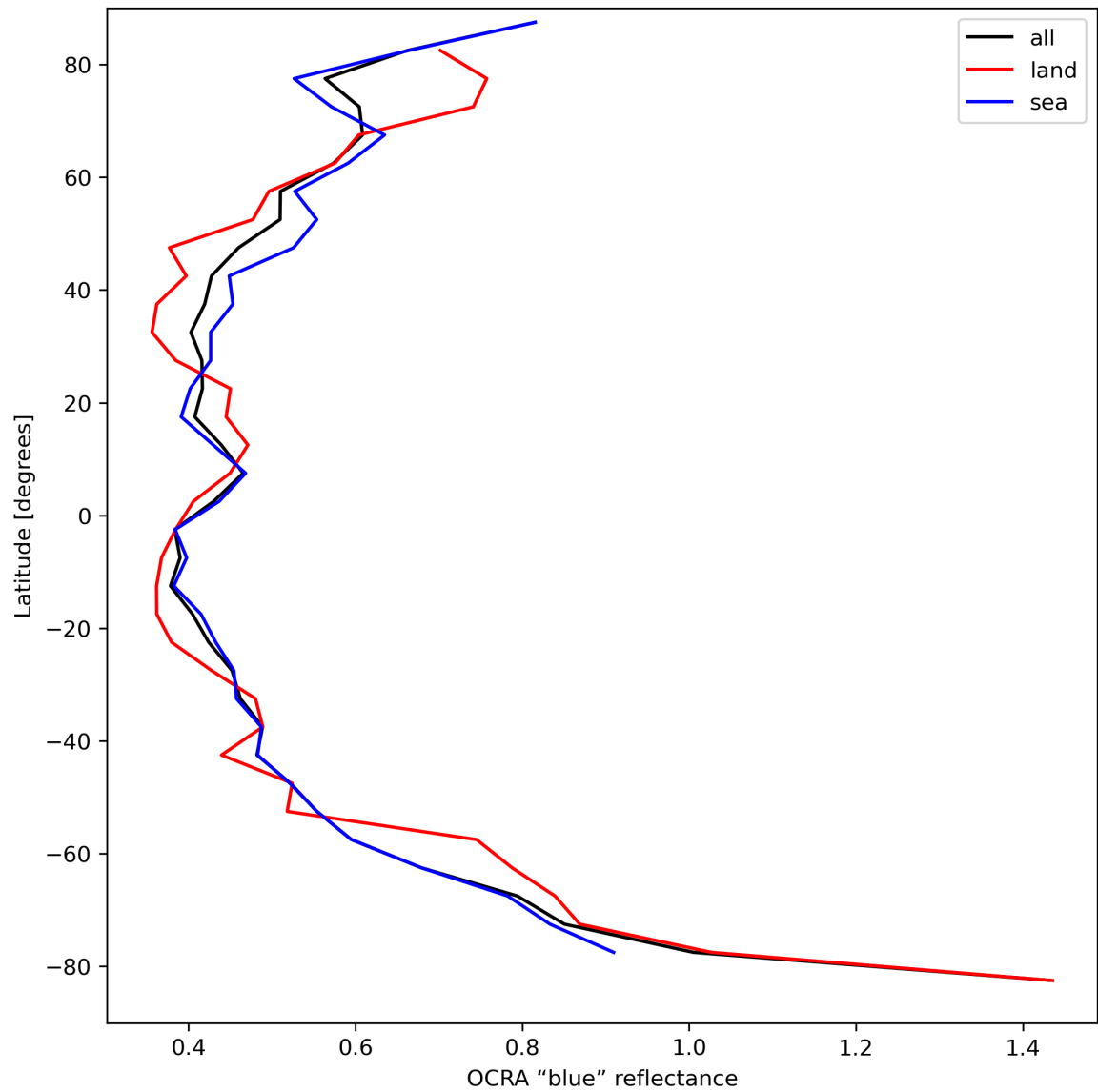
Figure 35: Zonal average of “OCRA “blue” reflectance” for 2023-09-01 to 2023-09-03.
