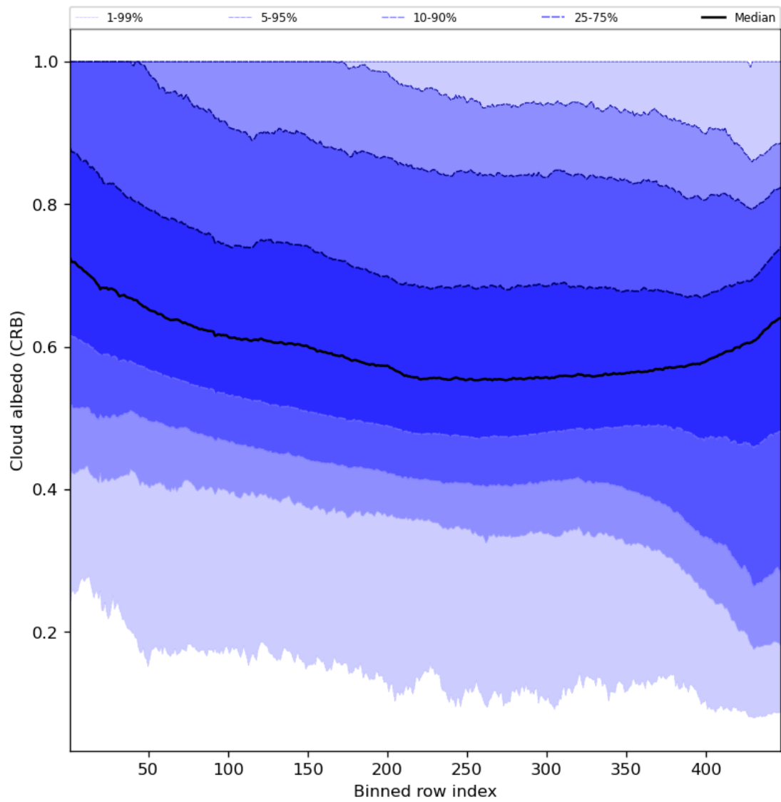
Figure 60: Along track statistics of “Cloud albedo (CRB)” for 2023-09-01 to 2023-09-03
