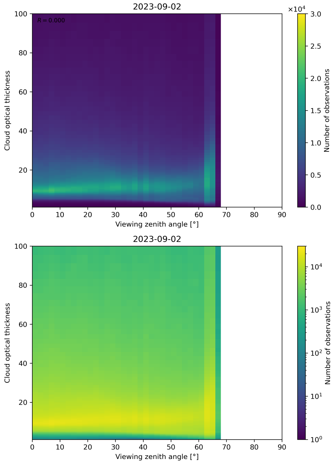
Figure 111: Scatter density plot of “Viewing zenith angle” against “Cloud optical thickness” for 2023-09-01 to 2023-09-03.
