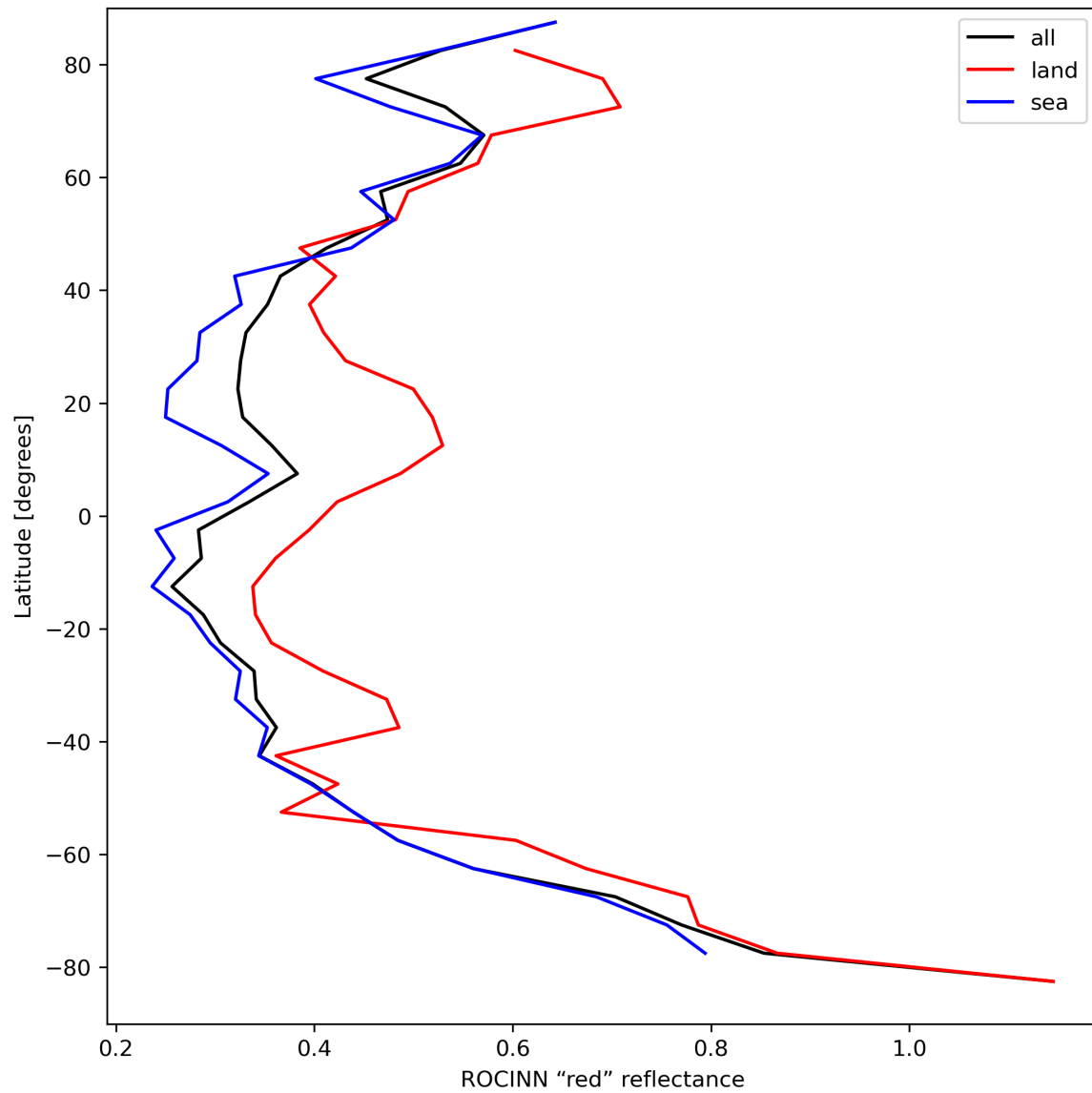
Figure 37: Zonal average of “ROCINN “red” reflectance” for 2023-09-01 to 2023-09-03.
