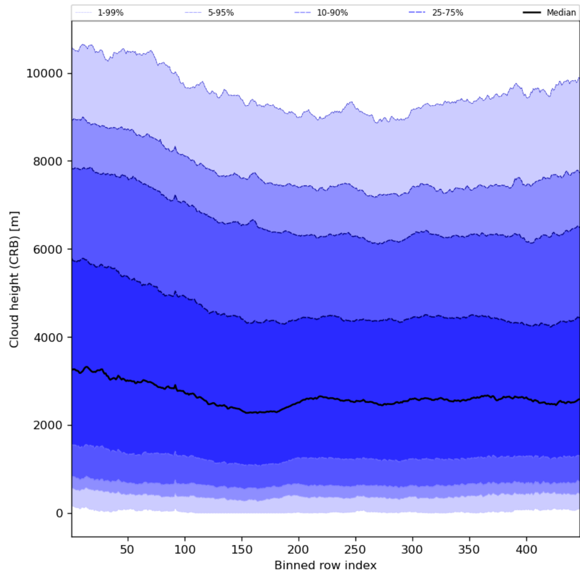
Figure 59: Along track statistics of “Cloud height (CRB)” for 2023-09-01 to 2023-09-03
