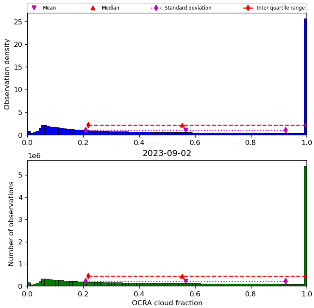
Figure 50: Histogram of “OCRA cloud fraction” for 2023-09-01 to 2023-09-03
