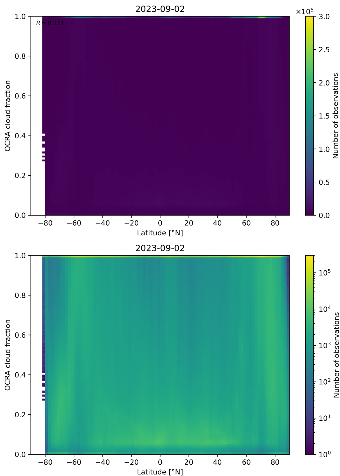
Figure 93: Scatter density plot of “Latitude” against “OCRA cloud fraction” for 2023-09-01 to 2023-09-03.
