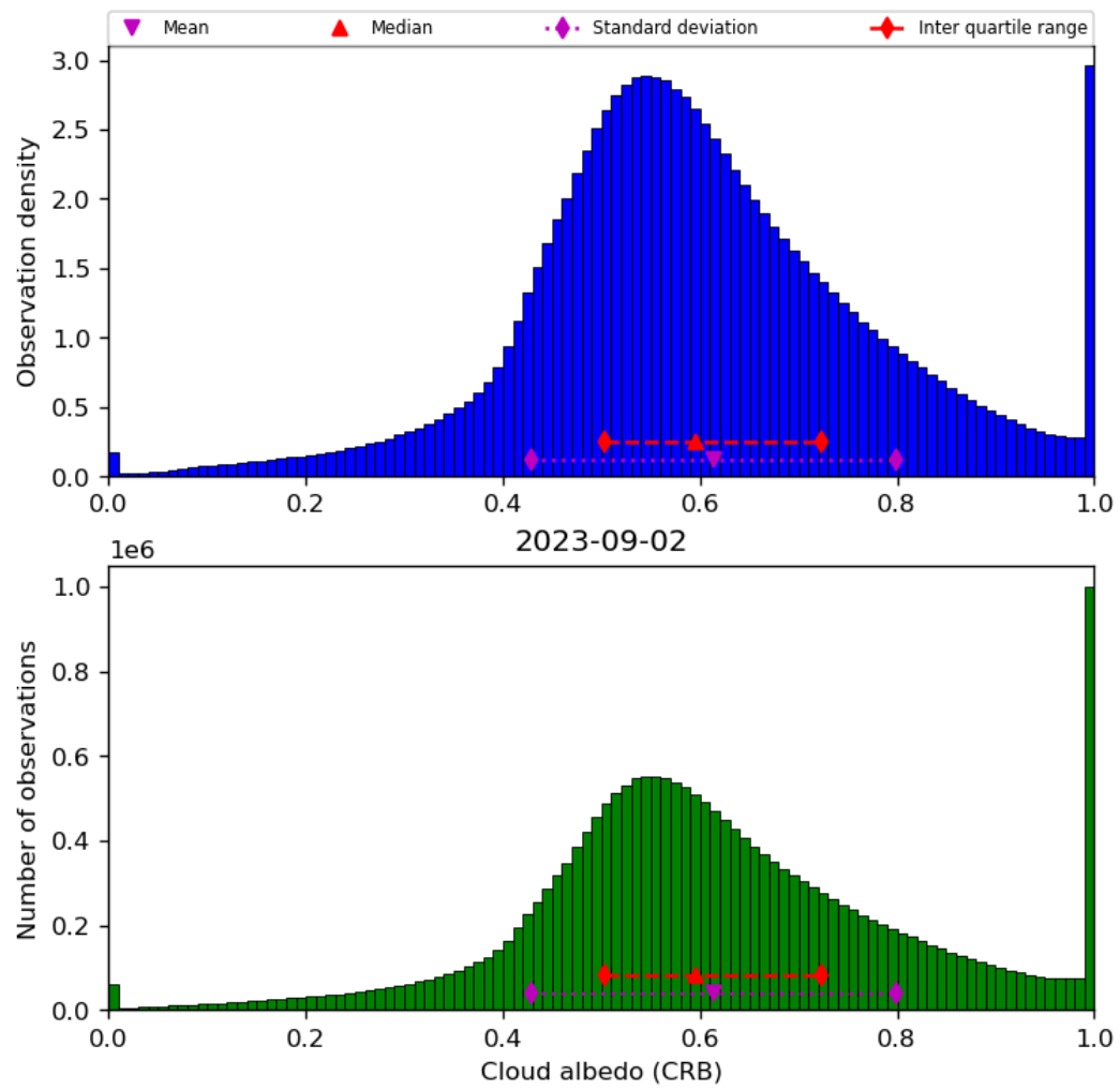
Figure 44: Histogram of “Cloud albedo (CRB)” for 2023-09-01 to 2023-09-03
