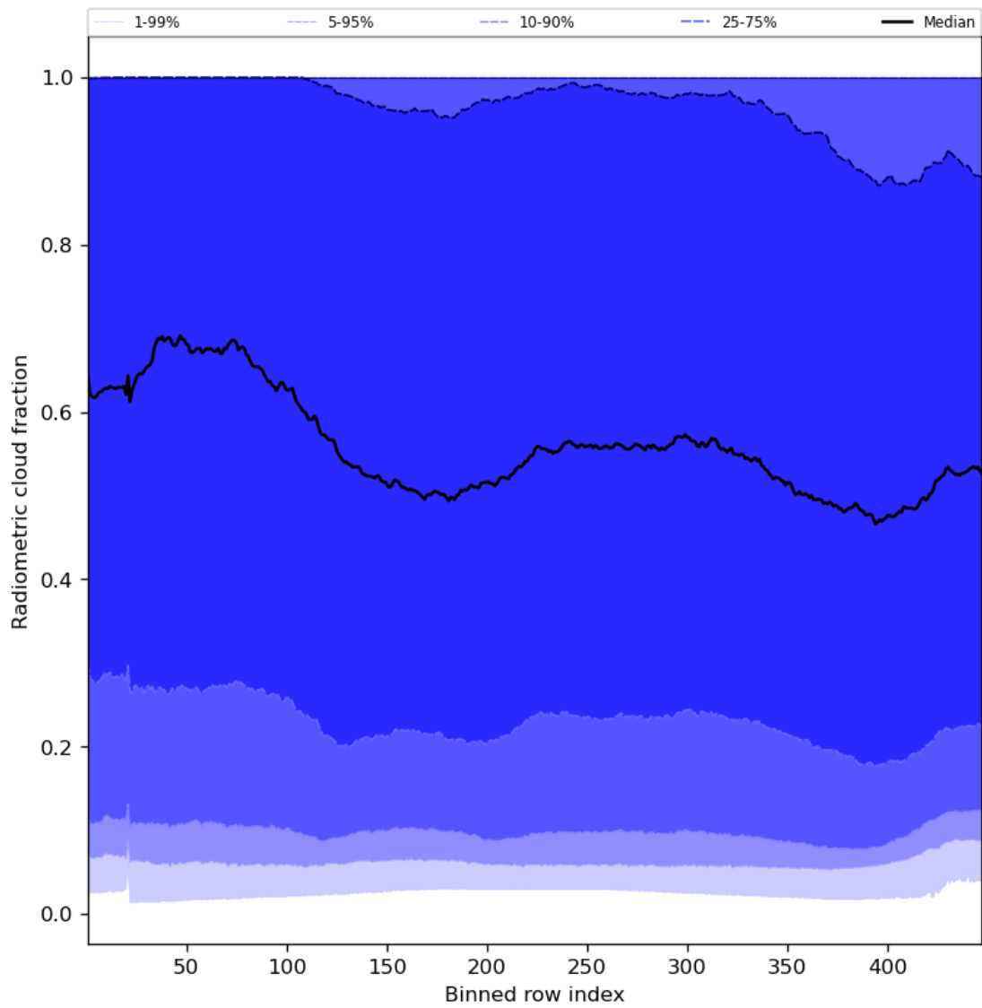
Figure 55: Along track statistics of “Radiometric cloud fraction” for 2023-09-01 to 2023-09-03
