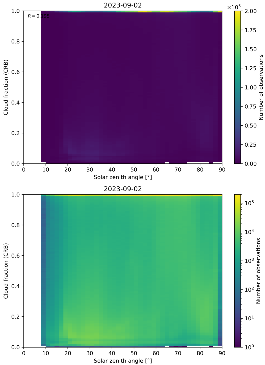
Figure 101: Scatter density plot of “Solar zenith angle” against “Cloud fraction (CRB)” for 2023-09-01 to 2023-09-03.
