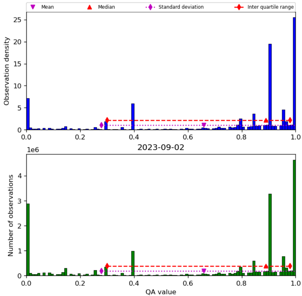
Figure 38: Histogram of “QA value” for 2023-09-01 to 2023-09-03
