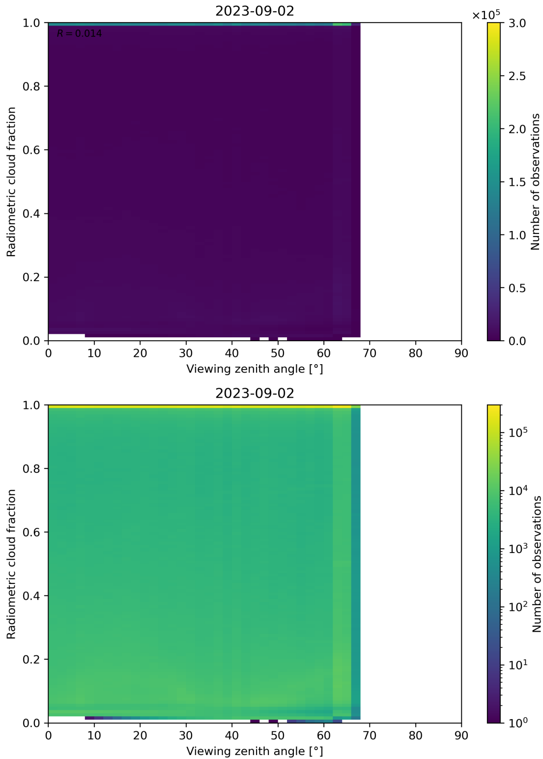
Figure 107: Scatter density plot of “Viewing zenith angle” against “Radiometric cloud fraction” for 2023-09-01 to 2023-09-03.
