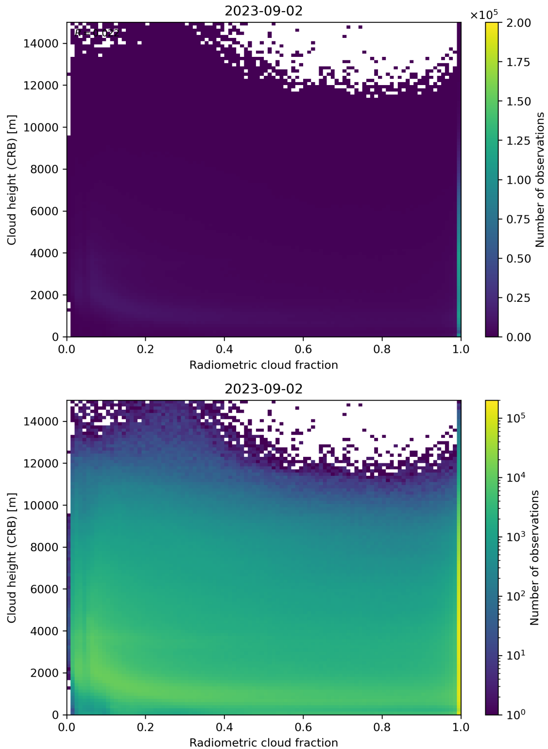
Figure 74: Scatter density plot of “Radiometric cloud fraction” against “Cloud height (CRB)” for 2023-09-01 to 2023-09-03.
