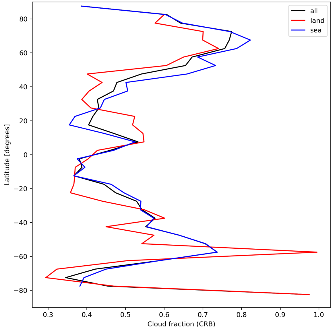
Figure 26: Zonal average of “Cloud fraction (CRB)” for 2023-09-01 to 2023-09-03.
