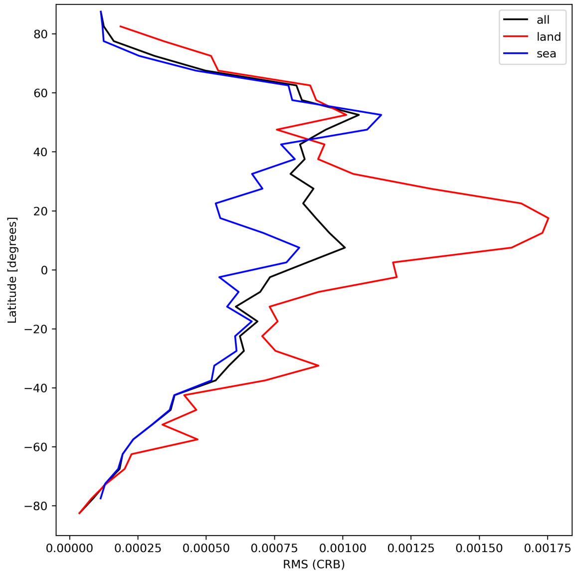
Figure 32: Zonal average of “RMS (CRB)” for 2023-09-01 to 2023-09-03.
