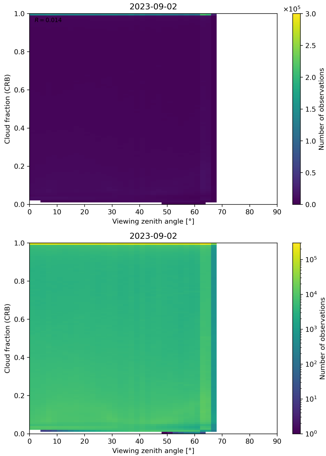
Figure 109: Scatter density plot of “Viewing zenith angle” against “Cloud fraction (CRB)” for 2023-09-01 to 2023-09-03.
