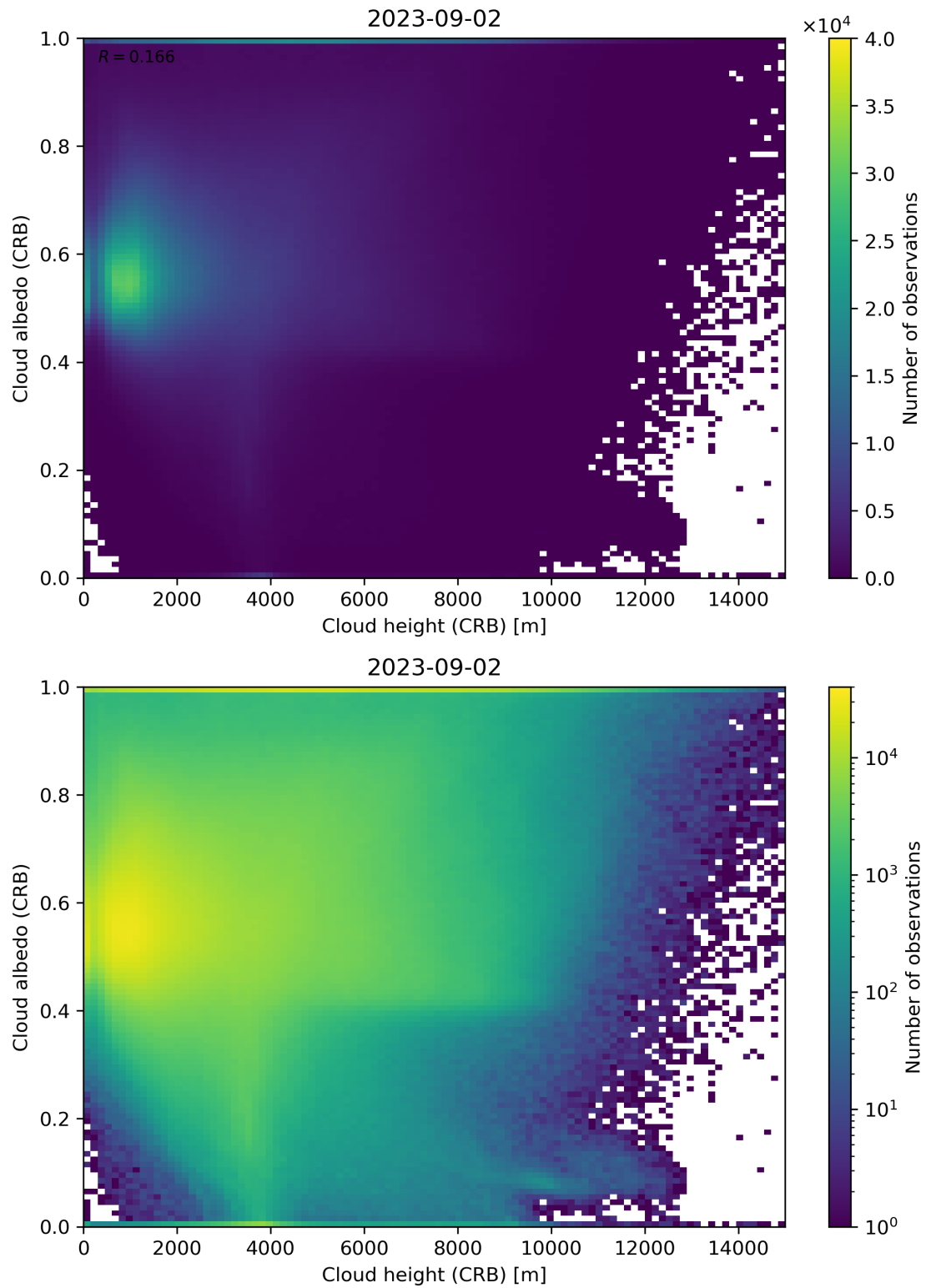
Figure 80: Scatter density plot of “Cloud height (CRB)” against “Cloud albedo (CRB)” for 2023-09-01 to 2023-09-03.
