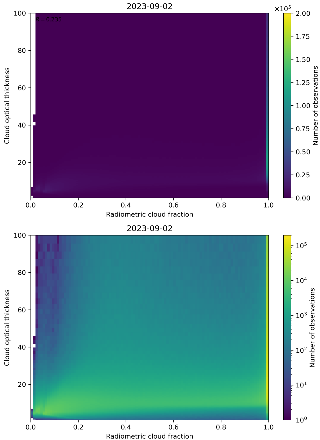
Figure 75: Scatter density plot of “Radiometric cloud fraction” against “Cloud optical thickness” for 2023-09-01 to 2023-09-03.
