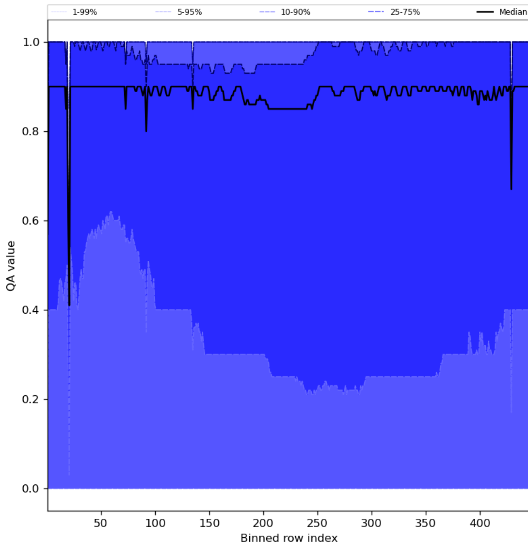
Figure 54: Along track statistics of “QA value” for 2023-09-01 to 2023-09-03
