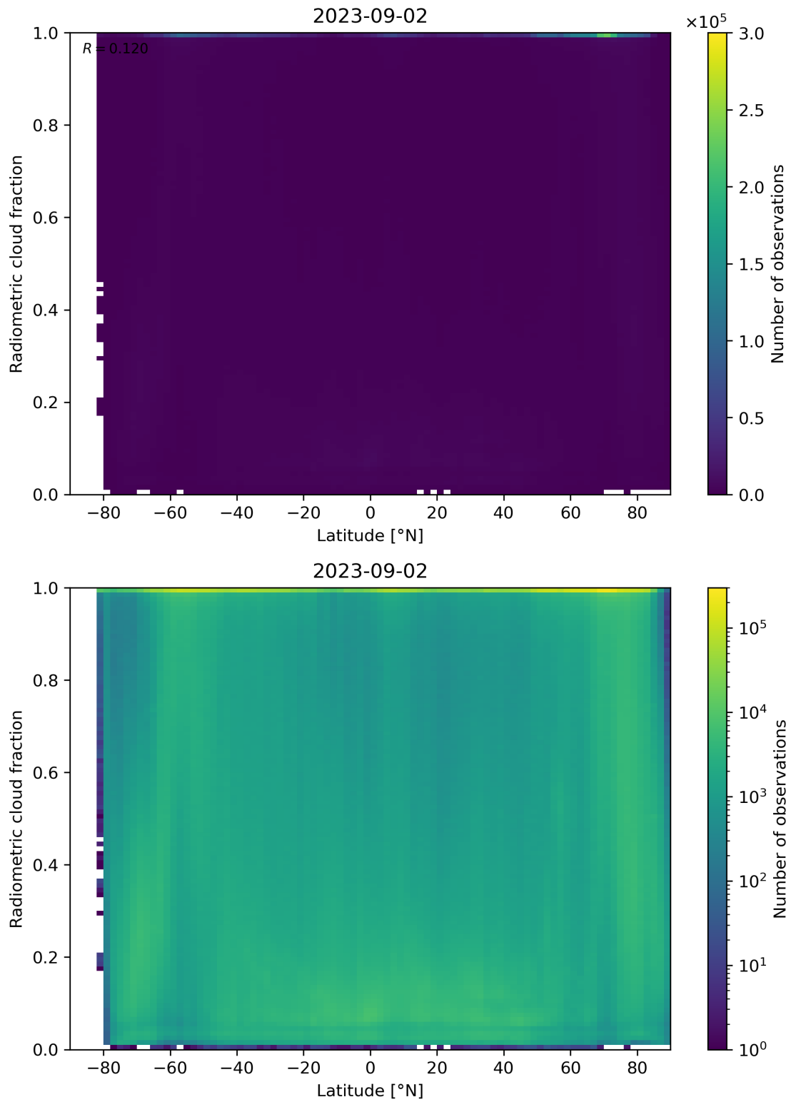
Figure 92: Scatter density plot of “Latitude” against “Radiometric cloud fraction” for 2023-09-01 to 2023-09-03.
