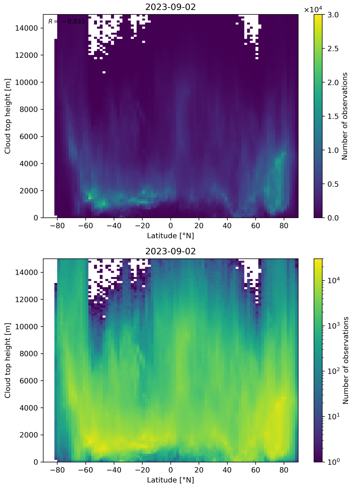
Figure 97: Scatter density plot of “Latitude” against “Cloud top height” for 2023-09-01 to 2023-09-03.
