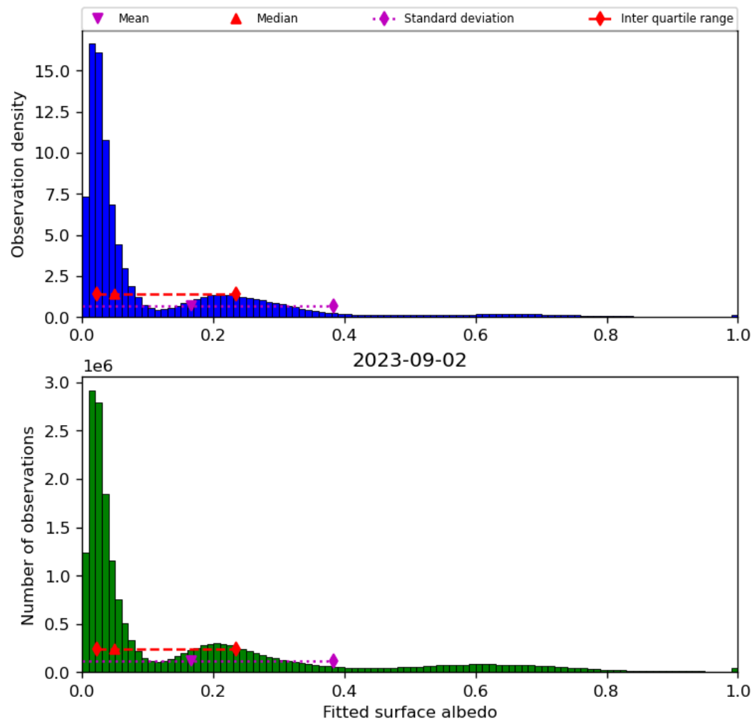
Figure 45: Histogram of “Fitted surface albedo” for 2023-09-01 to 2023-09-03
