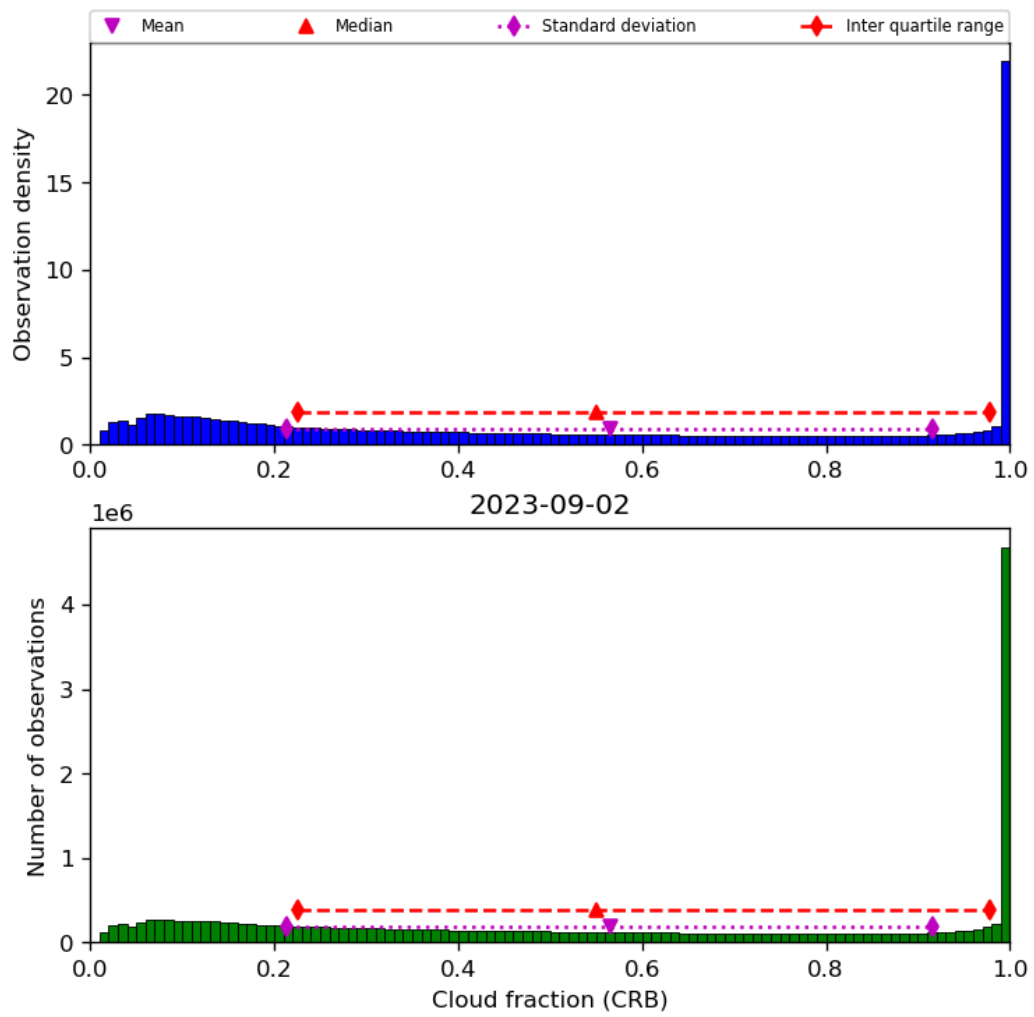
Figure 42: Histogram of “Cloud fraction (CRB)” for 2023-09-01 to 2023-09-03
