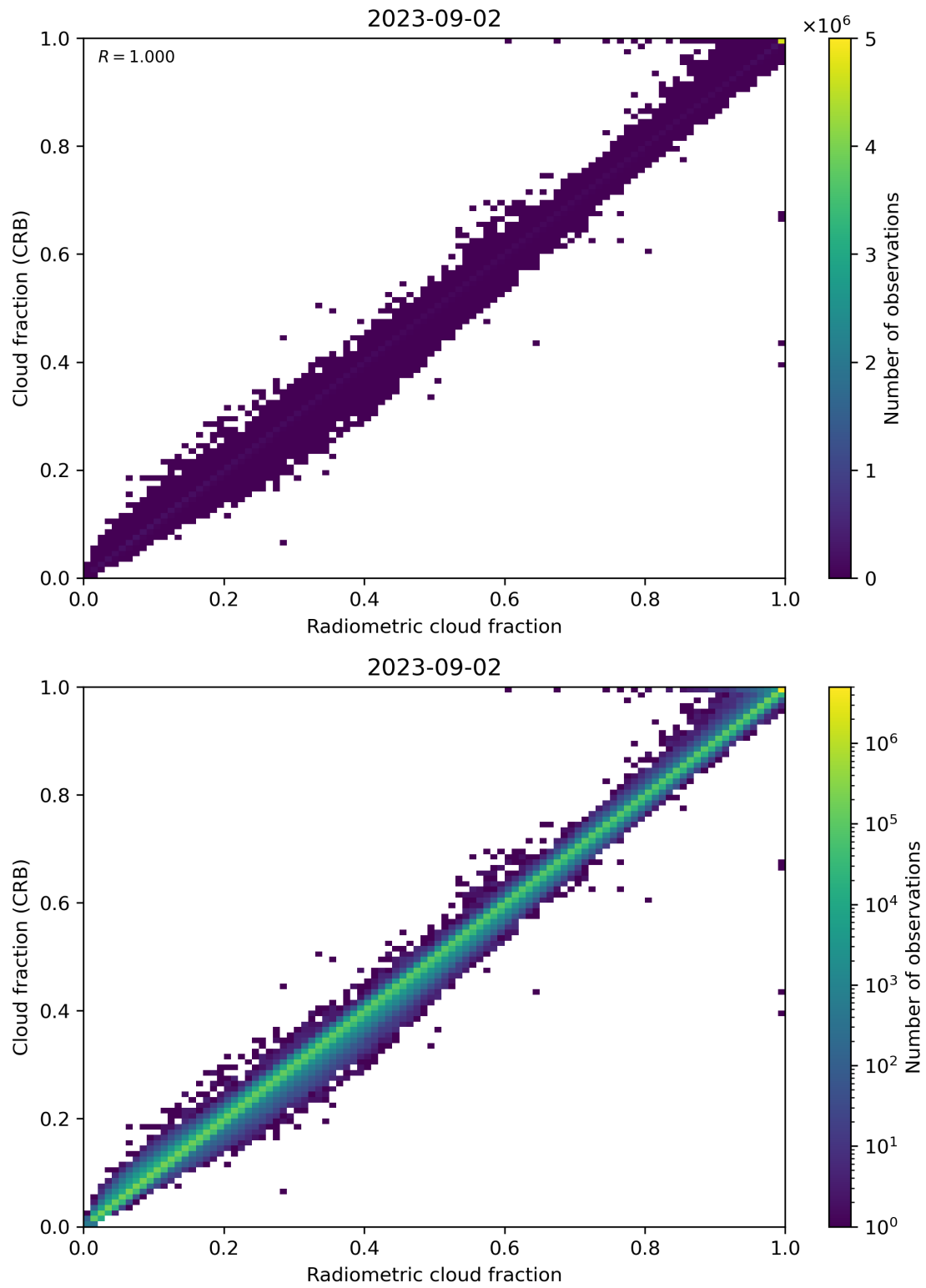
Figure 73: Scatter density plot of “Radiometric cloud fraction” against “Cloud fraction (CRB)” for 2023-09-01 to 2023-09-03.
