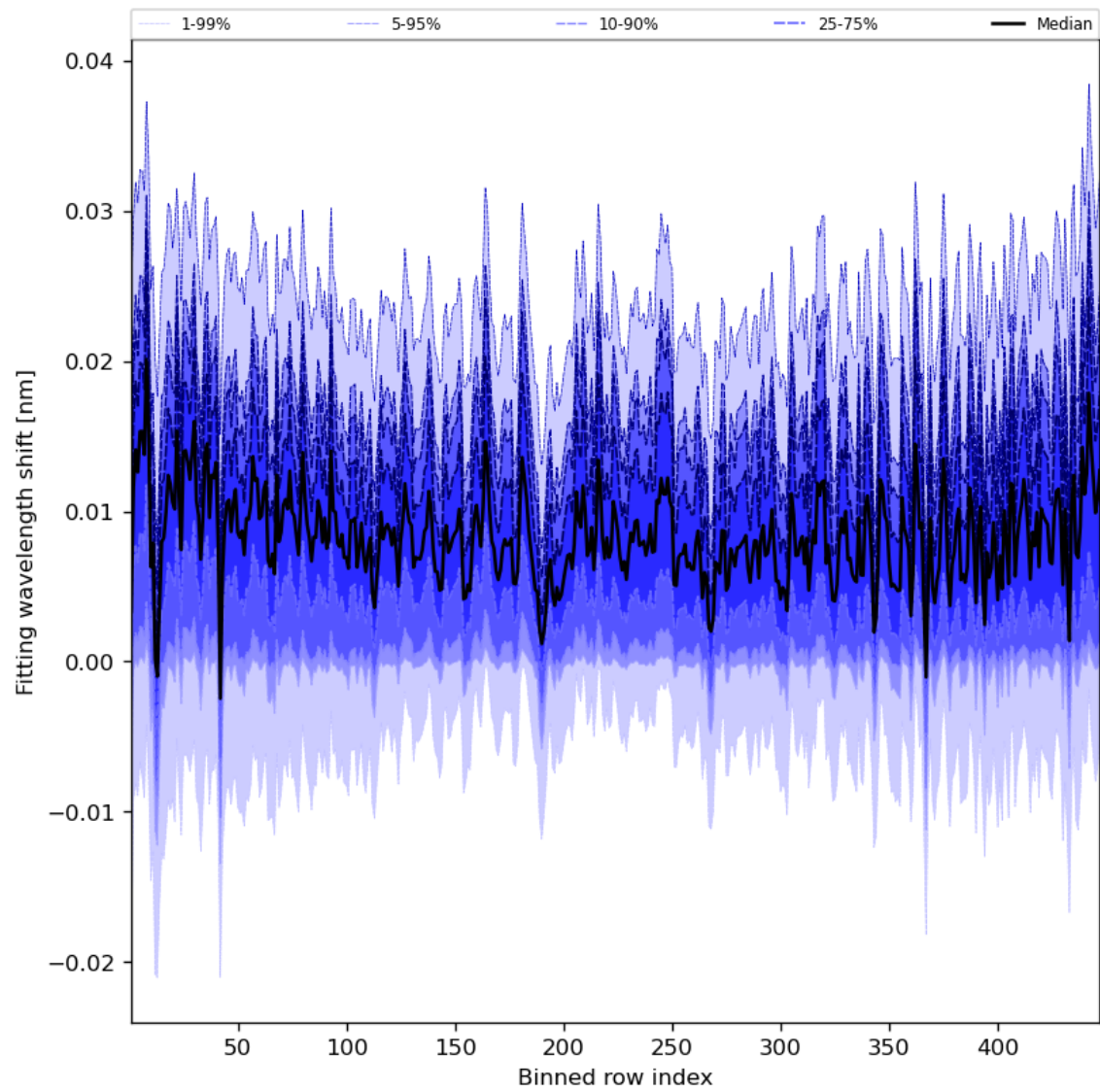
Figure 65: Along track statistics of “Fitting wavelength shift” for 2023-09-01 to 2023-09-03
