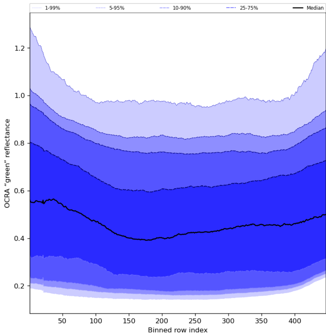
Figure 68: Along track statistics of “OCRA “green” reflectance” for 2023-09-01 to 2023-09-03
