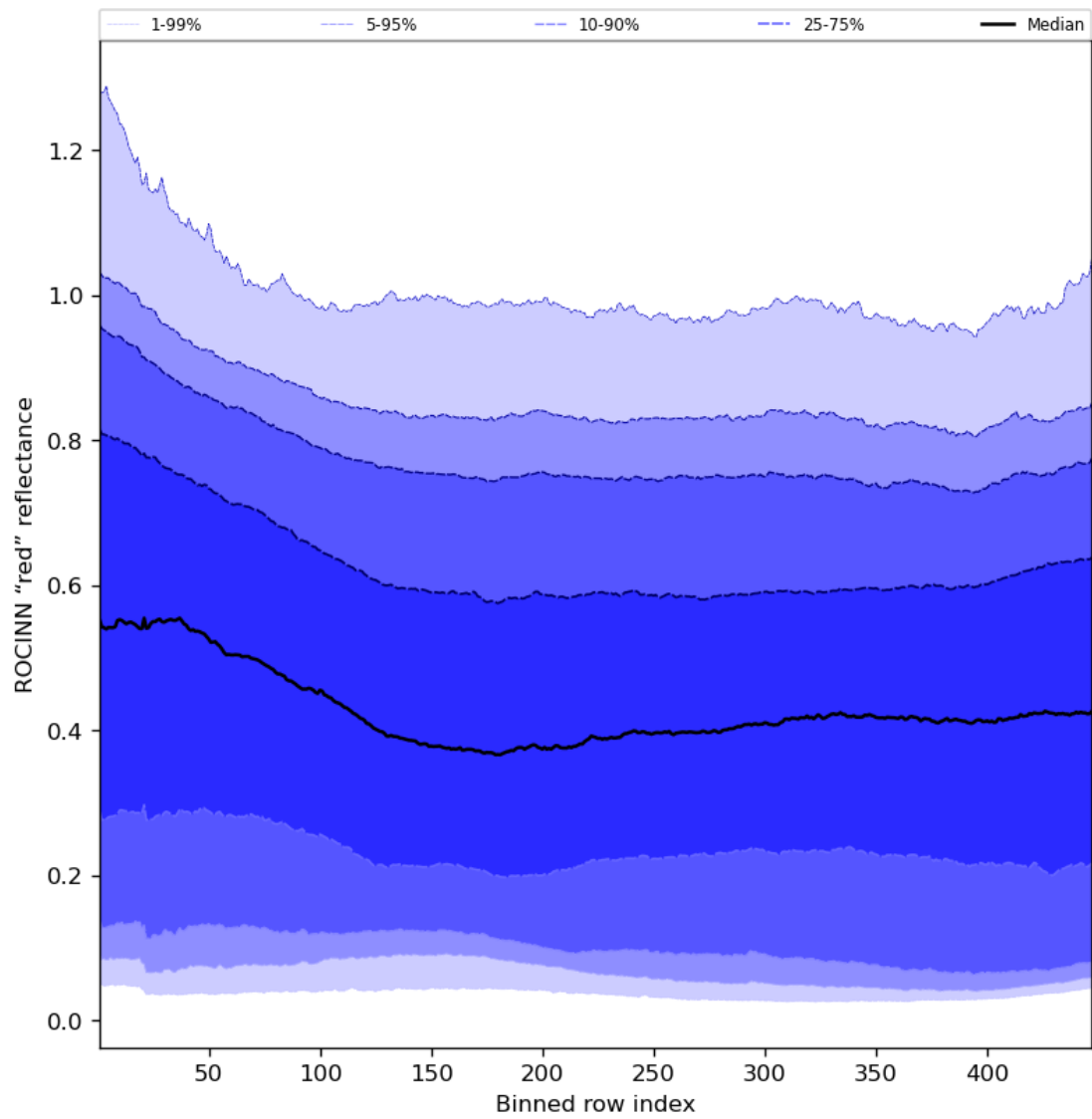
Figure 69: Along track statistics of “ROCINN “red” reflectance” for 2023-09-01 to 2023-09-03
