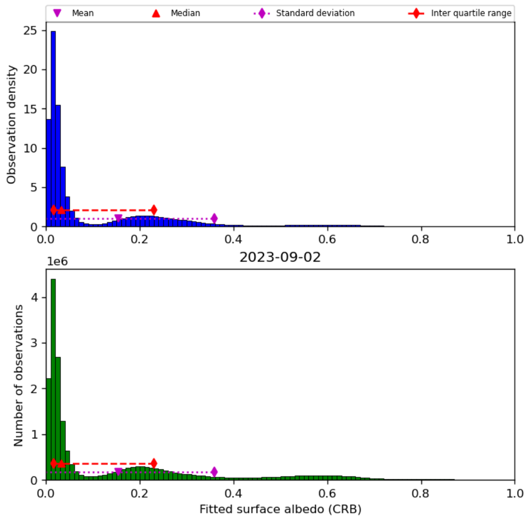
Figure 46: Histogram of “Fitted surface albedo (CRB)” for 2023-09-01 to 2023-09-03
