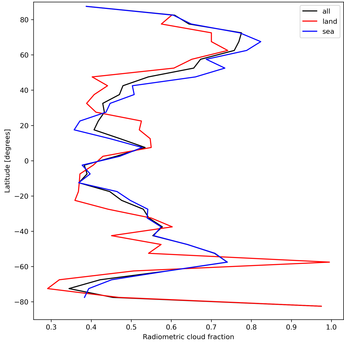
Figure 23: Zonal average of “Radiometric cloud fraction” for 2023-09-01 to 2023-09-03.
