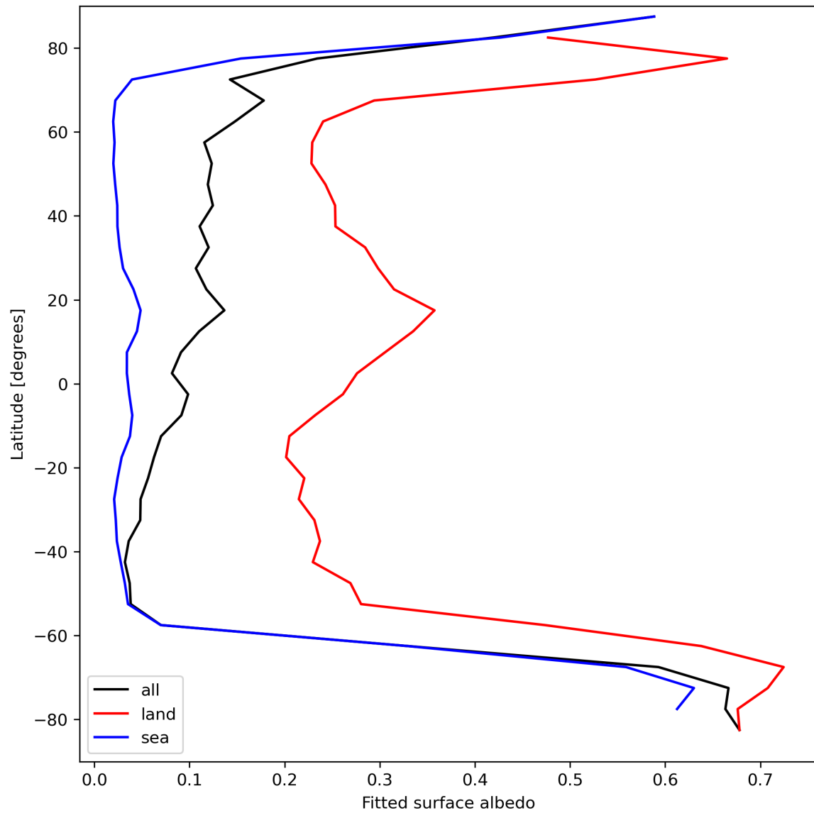
Figure 29: Zonal average of “Fitted surface albedo” for 2023-09-01 to 2023-09-03.
