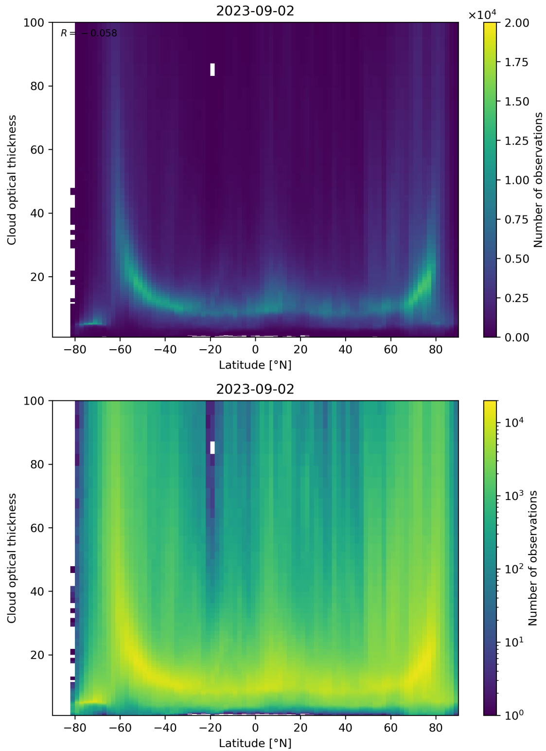
Figure 96: Scatter density plot of “Latitude” against “Cloud optical thickness” for 2023-09-01 to 2023-09-03.
