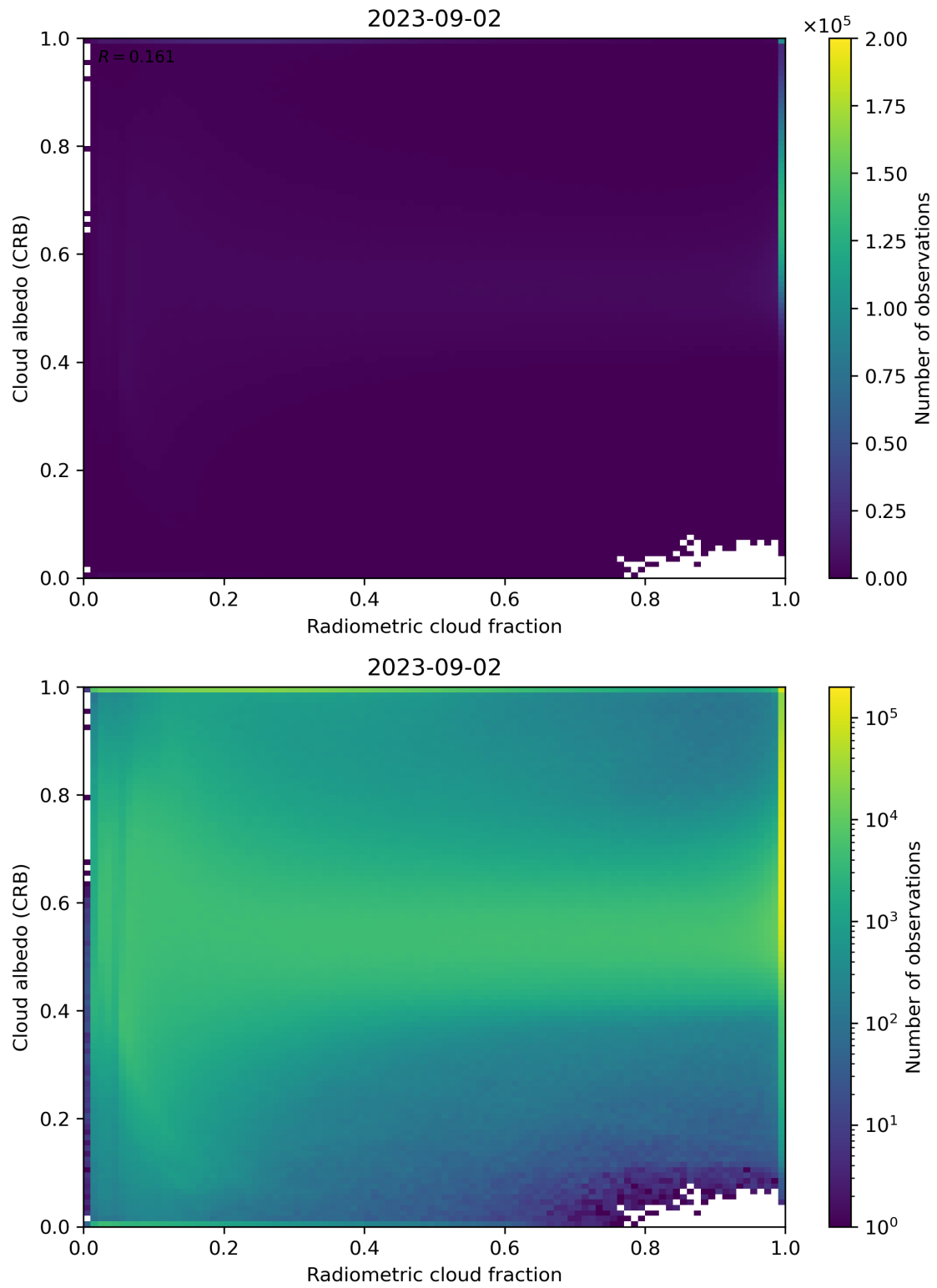
Figure 71: Scatter density plot of “Radiometric cloud fraction” against “Cloud albedo (CRB)” for 2023-09-01 to 2023-09-03.
