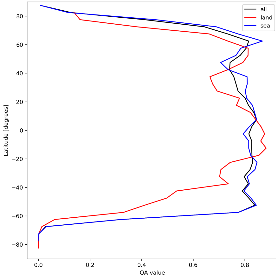
Figure 22: Zonal average of “QA value” for 2023-09-01 to 2023-09-03.
