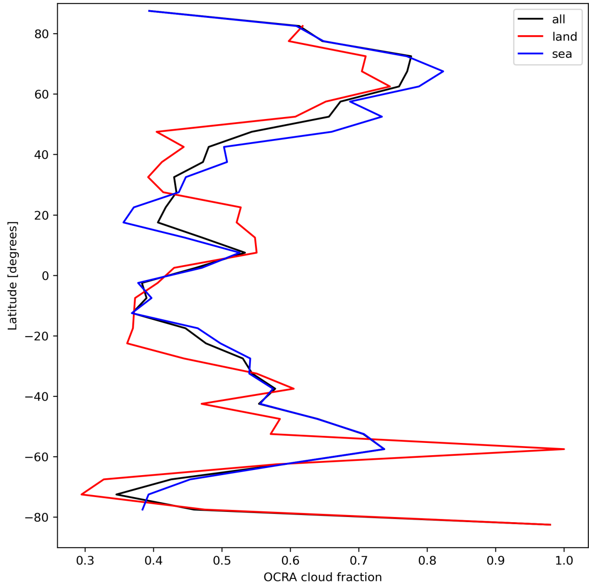
Figure 34: Zonal average of “OCRA cloud fraction” for 2023-09-01 to 2023-09-03.
