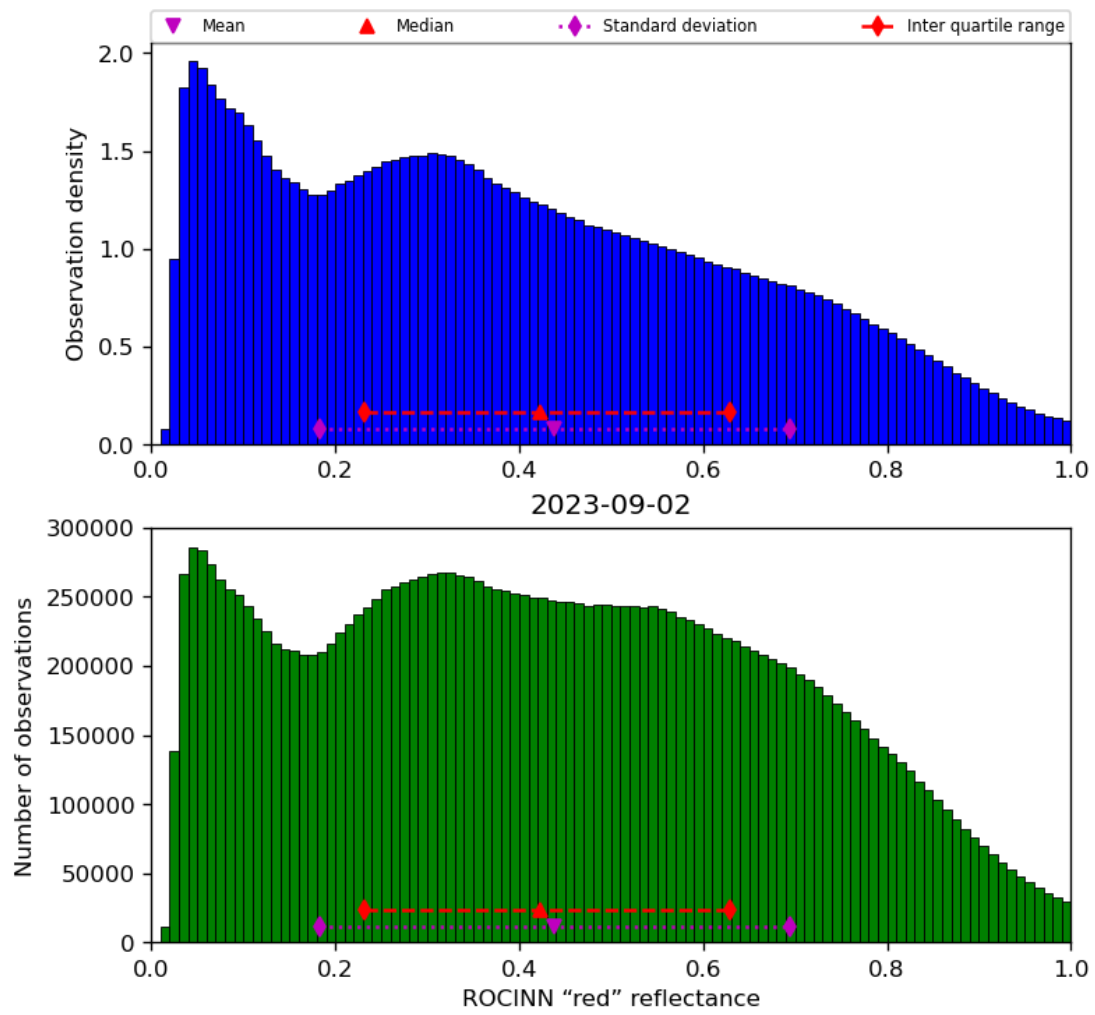
Figure 53: Histogram of “ROCINN “red” reflectance” for 2023-09-01 to 2023-09-03
