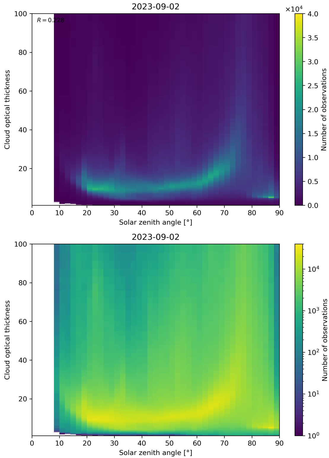
Figure 103: Scatter density plot of “Solar zenith angle” against “Cloud optical thickness” for 2023-09-01 to 2023-09-03.
