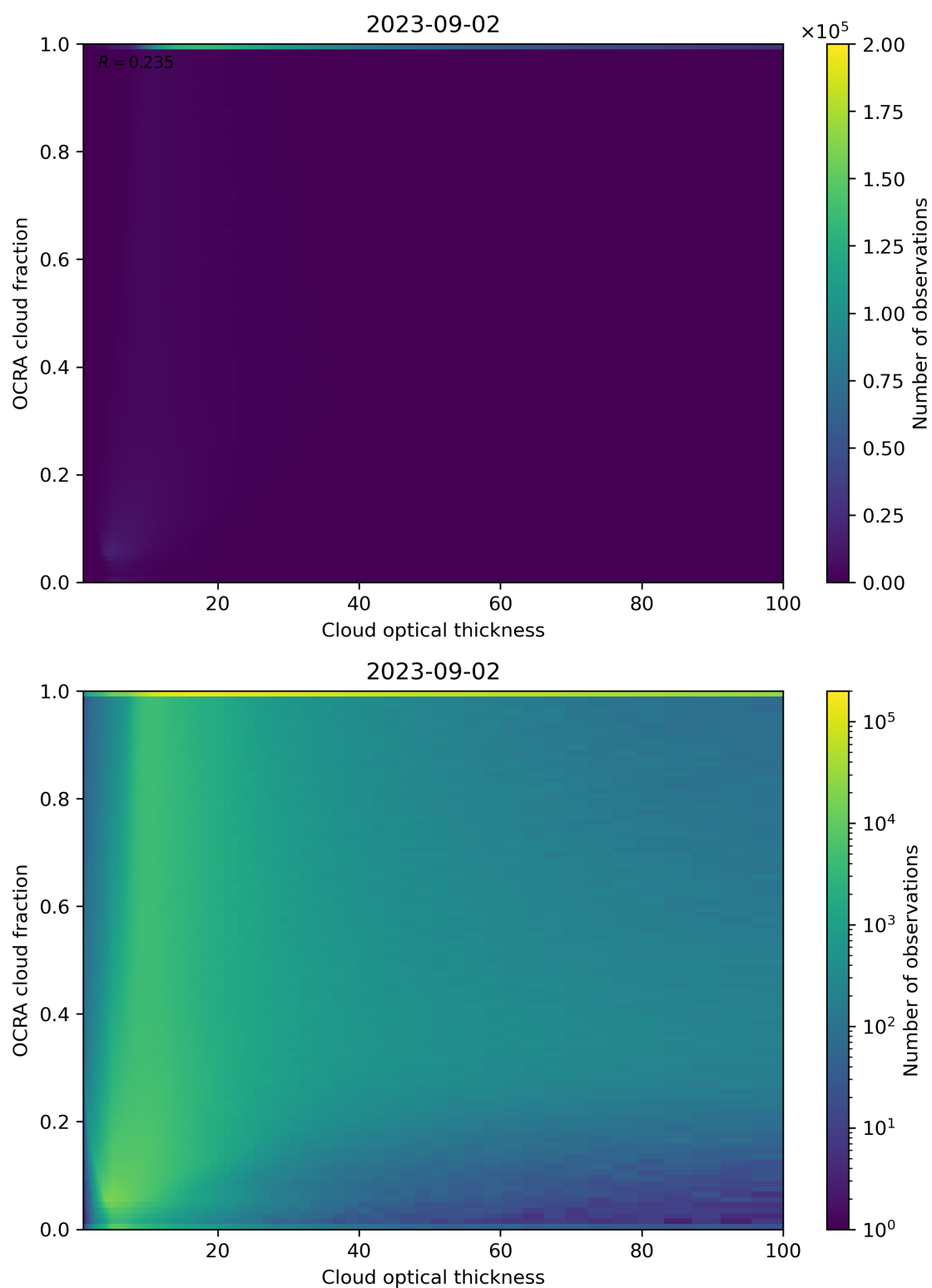
Figure 83: Scatter density plot of “Cloud optical thickness” against “OCRA cloud fraction” for 2023-09-01 to 2023-09-03.
