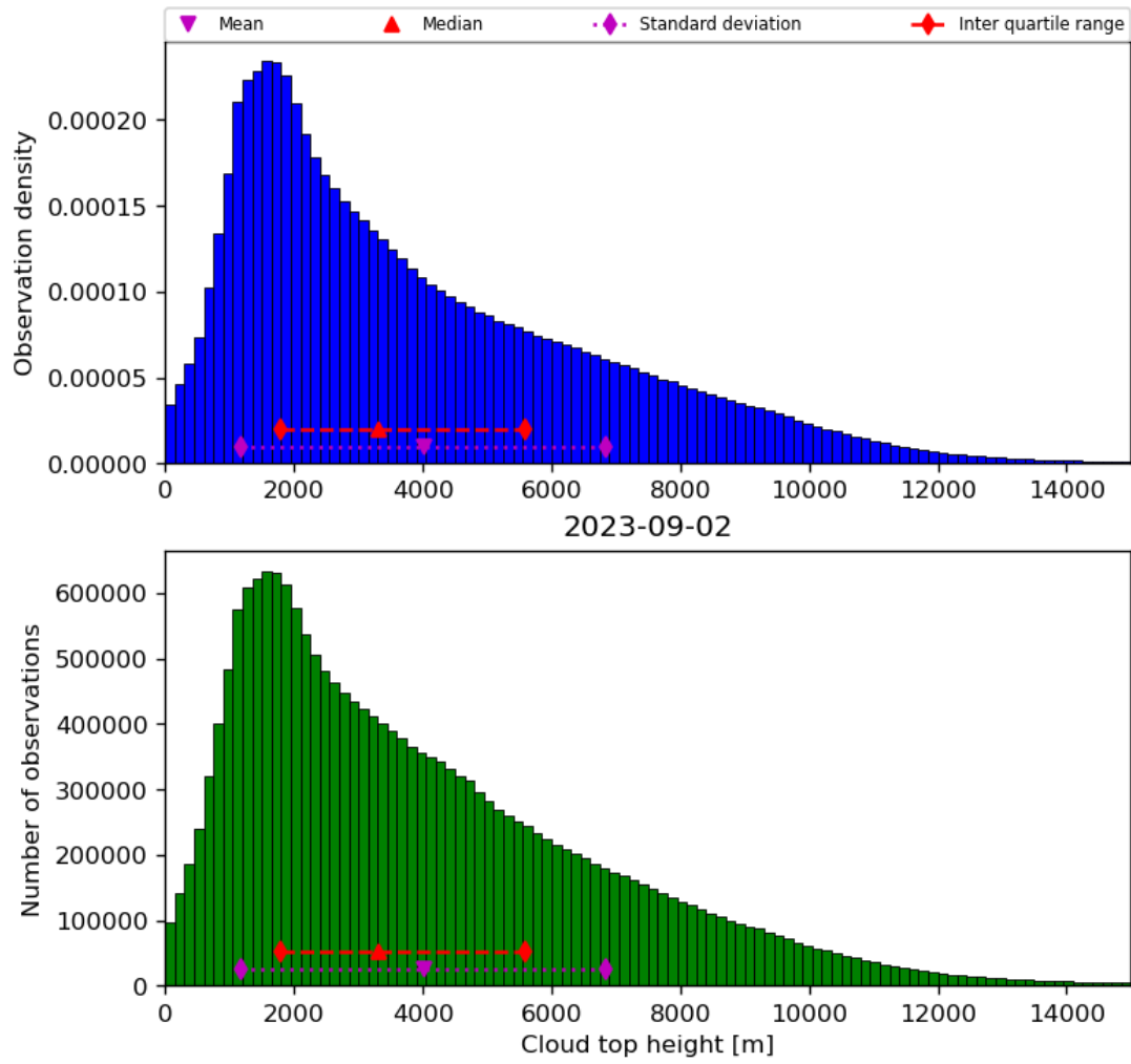
Figure 40: Histogram of “Cloud top height” for 2023-09-01 to 2023-09-03
