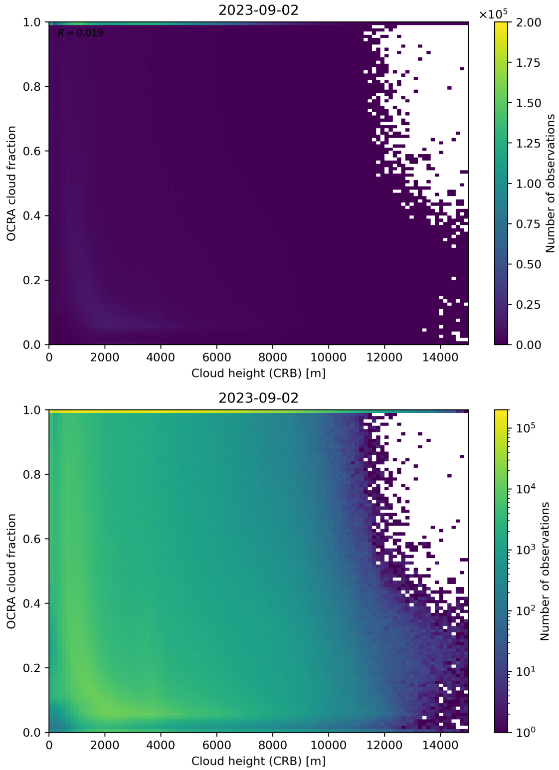
Figure 81: Scatter density plot of “Cloud height (CRB)” against “OCRA cloud fraction” for 2023-09-01 to 2023-09-03.
