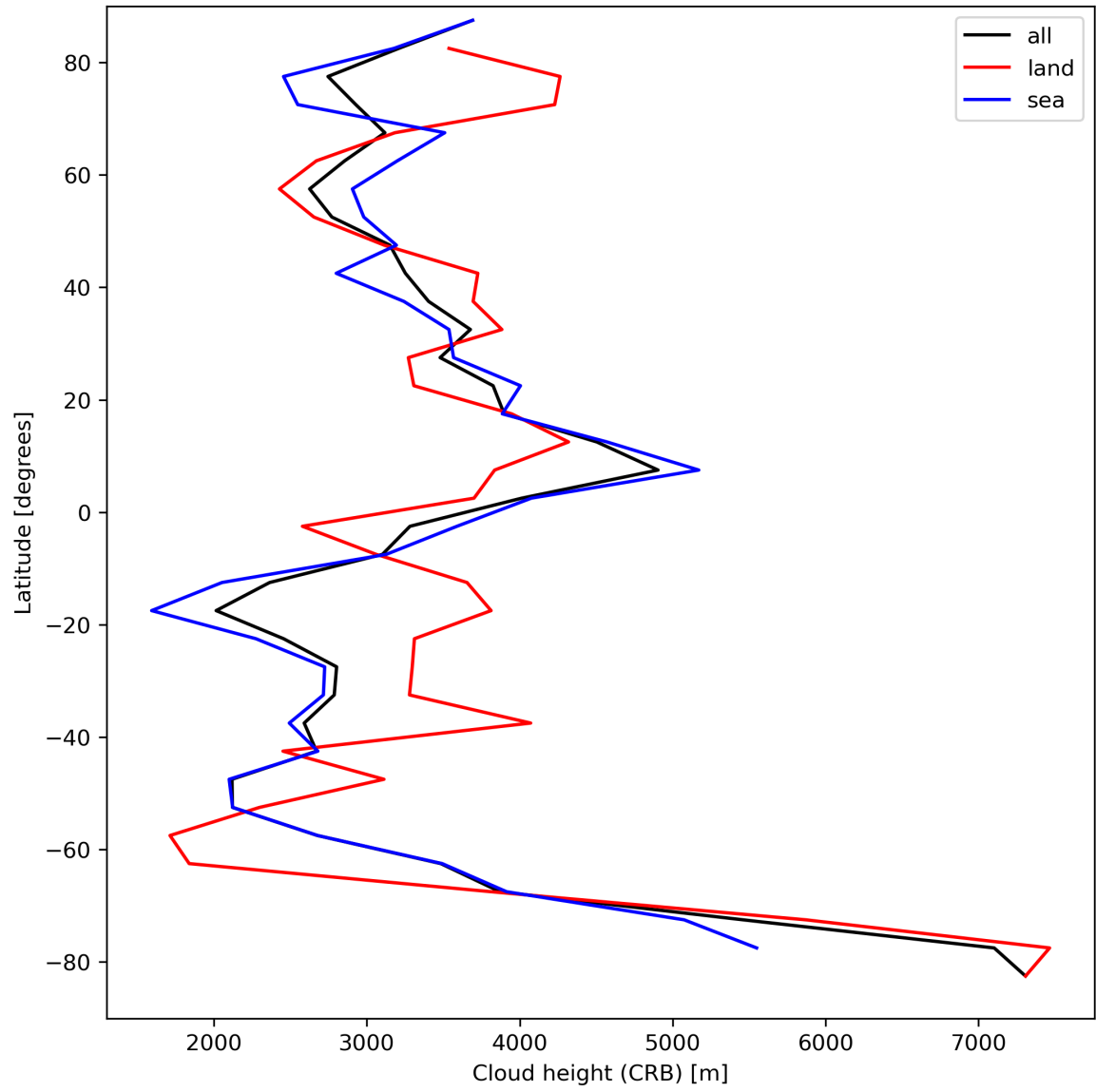
Figure 27: Zonal average of “Cloud height (CRB)” for 2023-09-01 to 2023-09-03.
