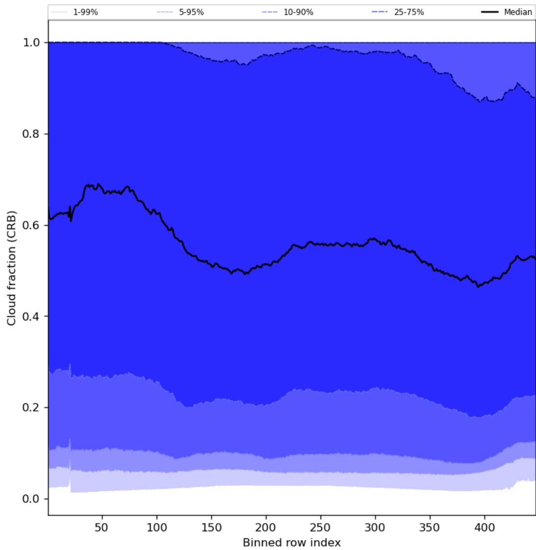
Figure 58: Along track statistics of “Cloud fraction (CRB)” for 2023-09-01 to 2023-09-03
