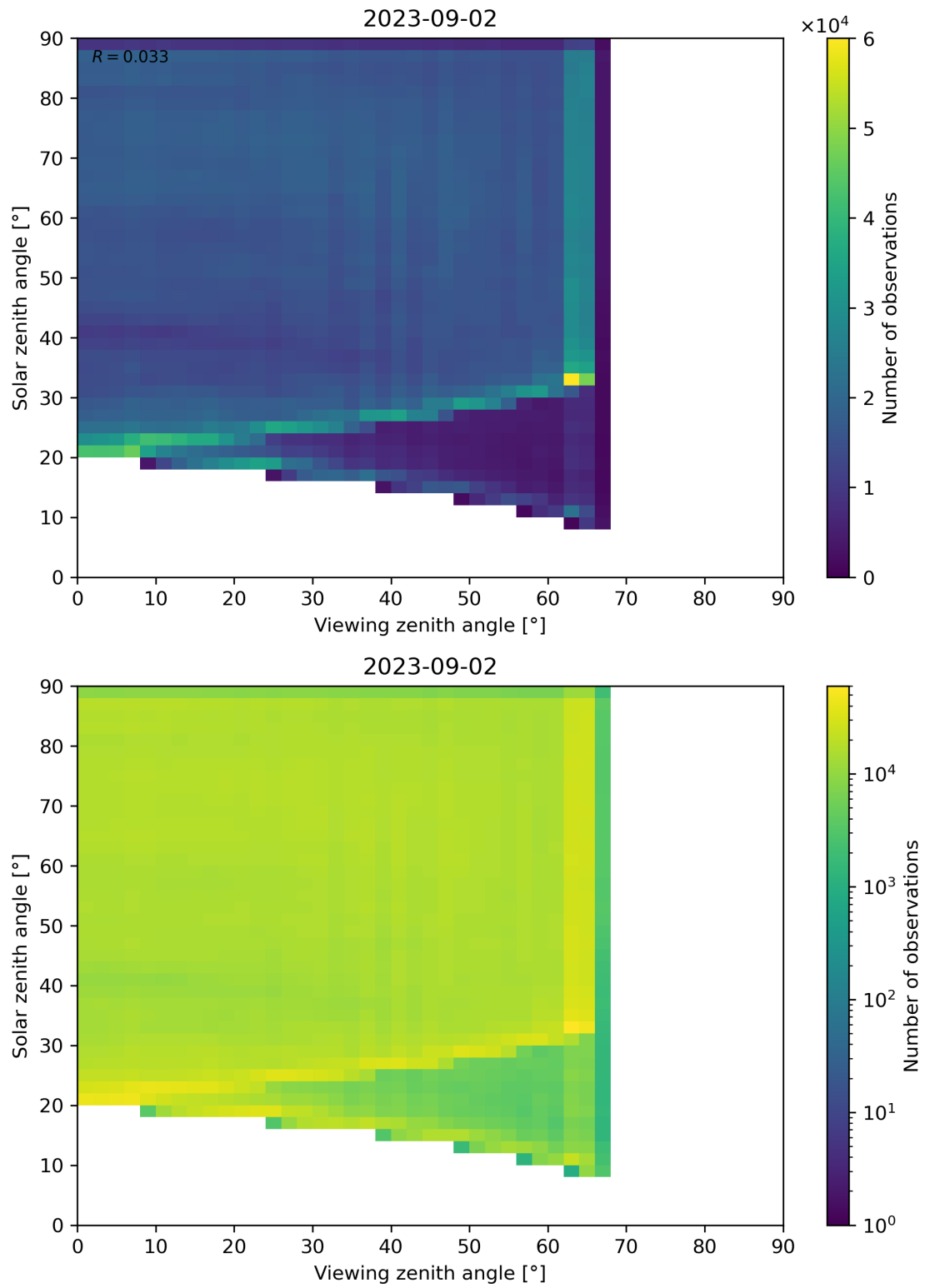
Figure 114: Scatter density plot of “Viewing zenith angle” against “Solar zenith angle” for 2023-09-01 to 2023-09-03.
