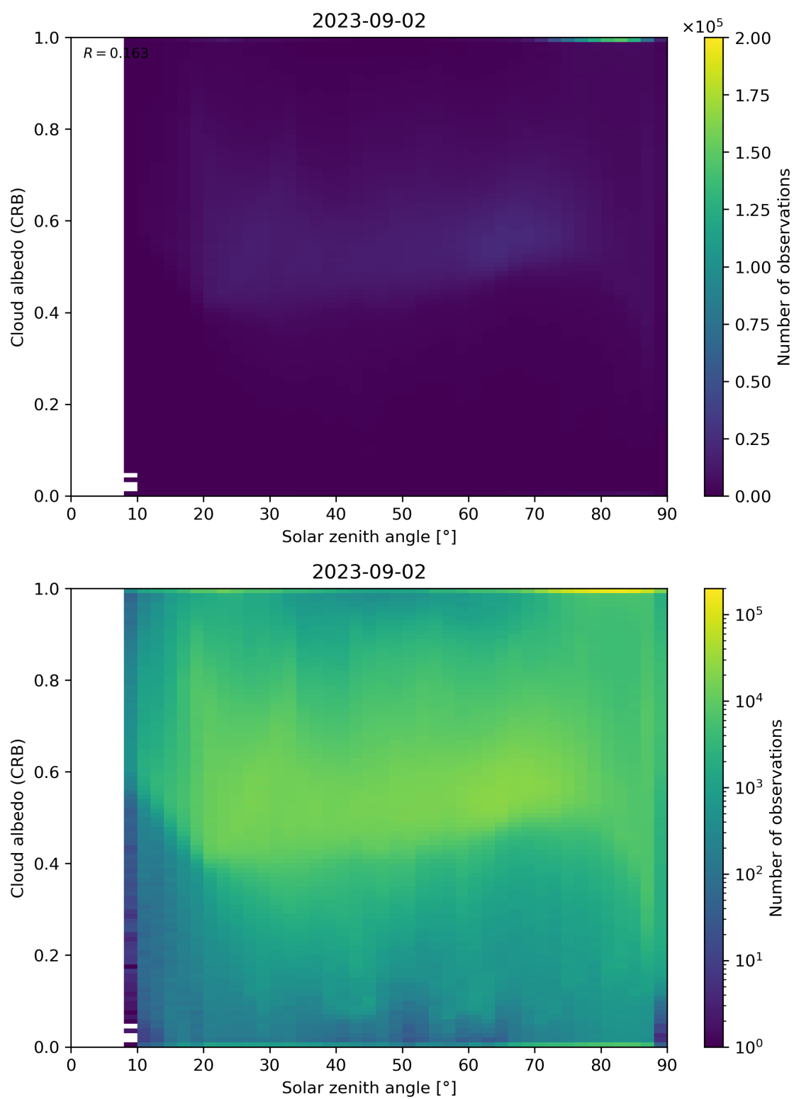
Figure 98: Scatter density plot of “Solar zenith angle” against “Cloud albedo (CRB)” for 2023-09-01 to 2023-09-03.
