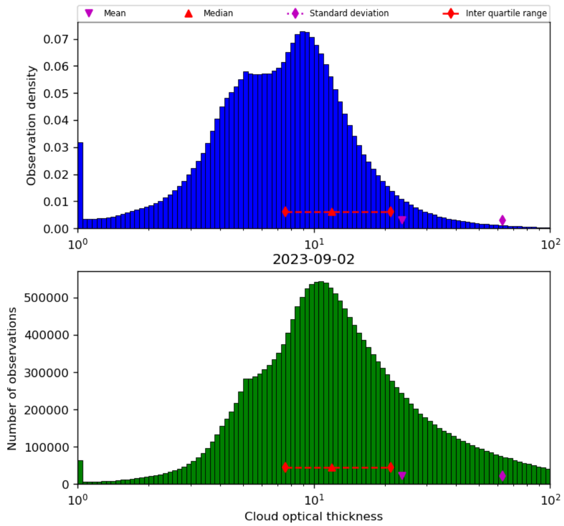
Figure 41: Histogram of “Cloud optical thickness” for 2023-09-01 to 2023-09-03
