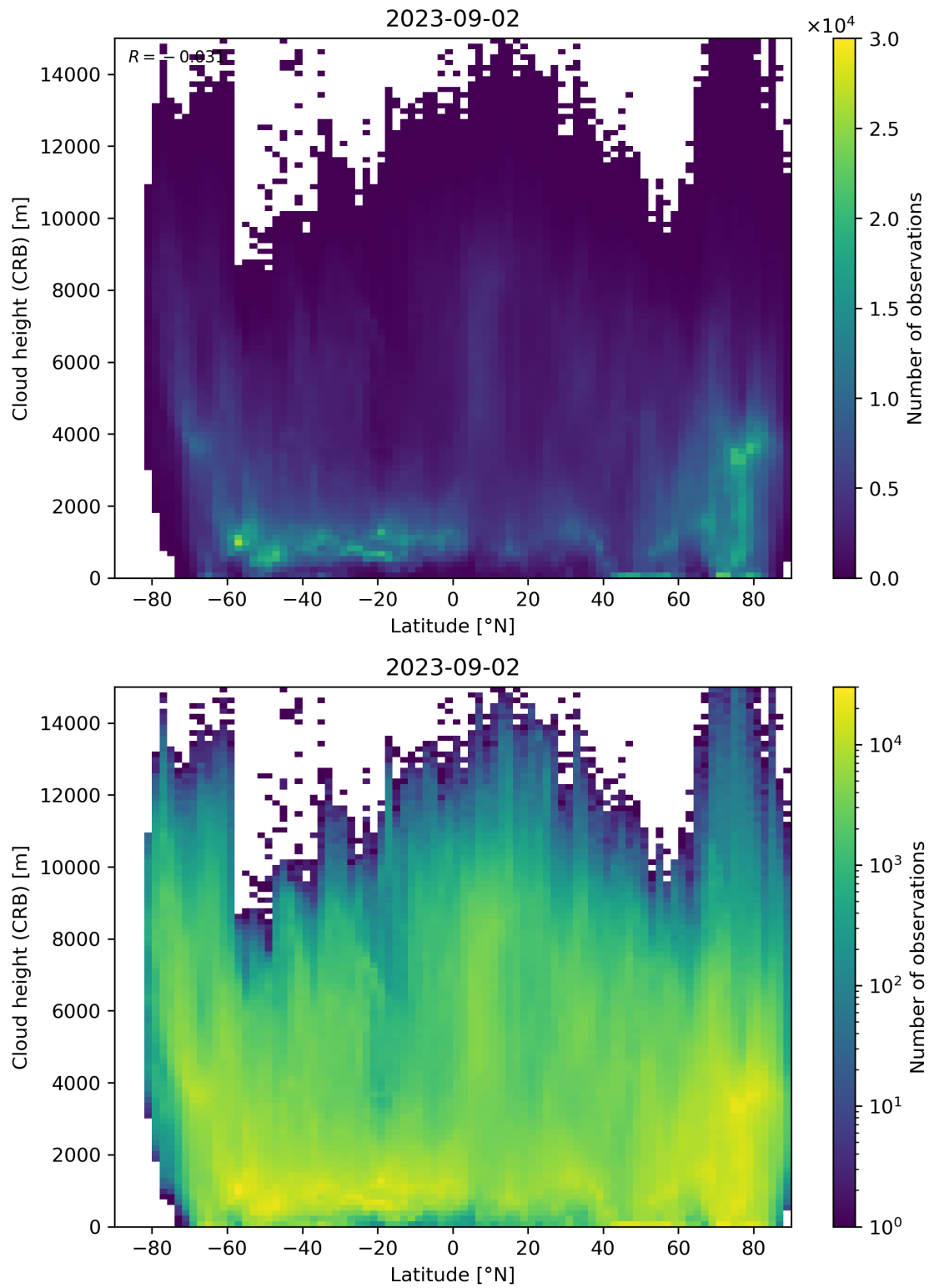
Figure 95: Scatter density plot of “Latitude” against “Cloud height (CRB)” for 2023-09-01 to 2023-09-03.
