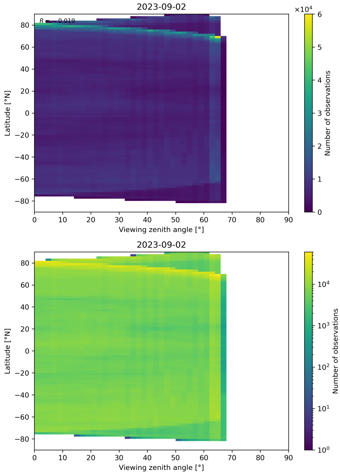
Figure 113: Scatter density plot of “Viewing zenith angle” against “Latitude” for 2023-09-01 to 2023-09-03.
