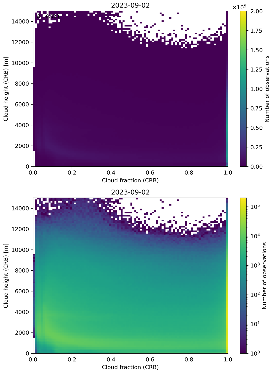
Figure 79: Scatter density plot of “Cloud fraction (CRB)” against “Cloud height (CRB)” for 2023-09-01 to 2023-09-03.
