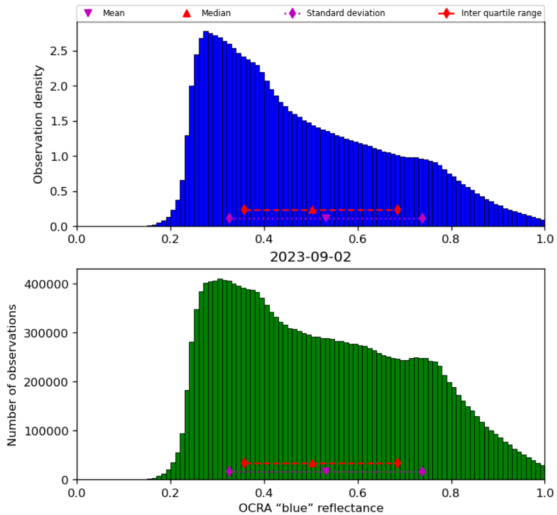
Figure 51: Histogram of “OCRA “blue” reflectance” for 2023-09-01 to 2023-09-03
