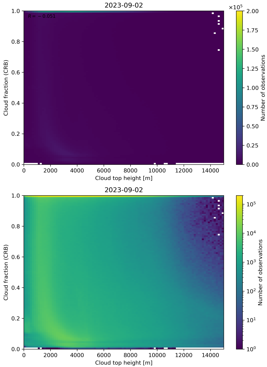
Figure 88: Scatter density plot of “Cloud top height” against “Cloud fraction (CRB)” for 2023-09-01 to 2023-09-03.
