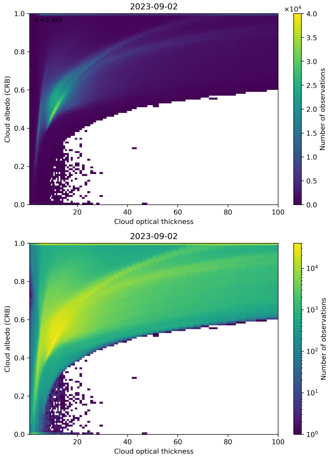
Figure 82: Scatter density plot of “Cloud optical thickness” against “Cloud albedo (CRB)” for 2023-09-01 to 2023-09-03.
