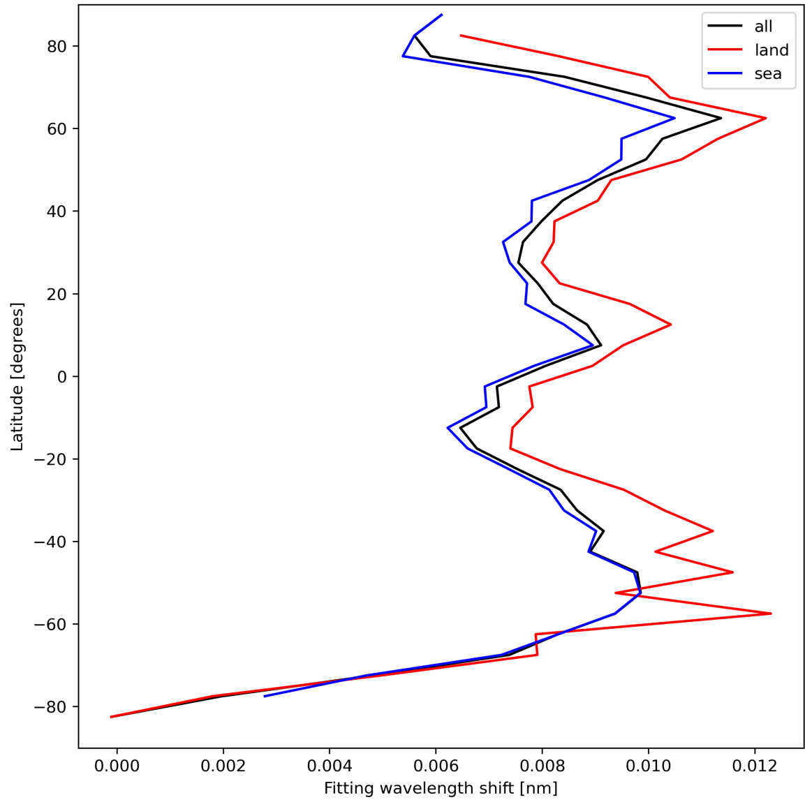
Figure 33: Zonal average of “Fitting wavelength shift” for 2023-09-01 to 2023-09-03.
