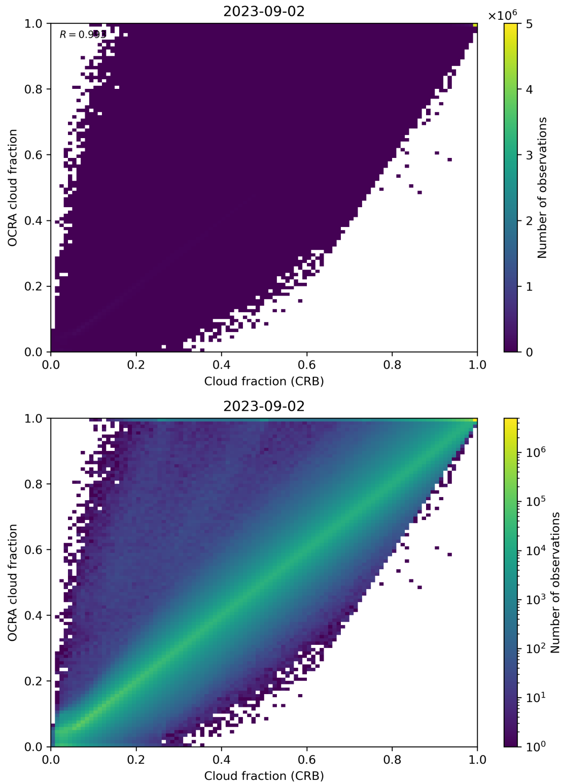
Figure 78: Scatter density plot of “Cloud fraction (CRB)” against “OCRA cloud fraction” for 2023-09-01 to 2023-09-03.
