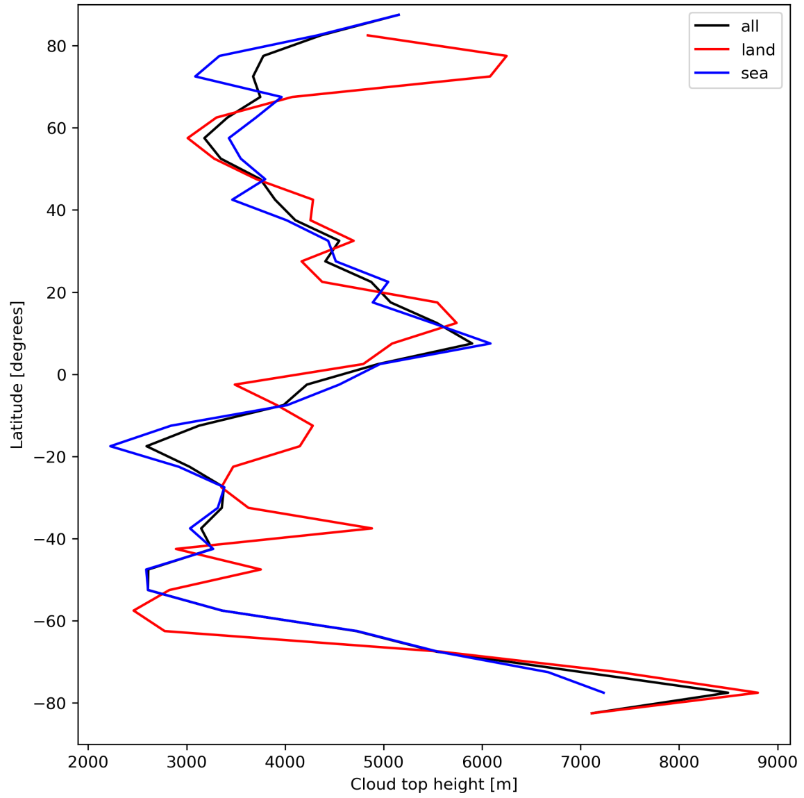
Figure 24: Zonal average of “Cloud top height” for 2023-09-01 to 2023-09-03.
