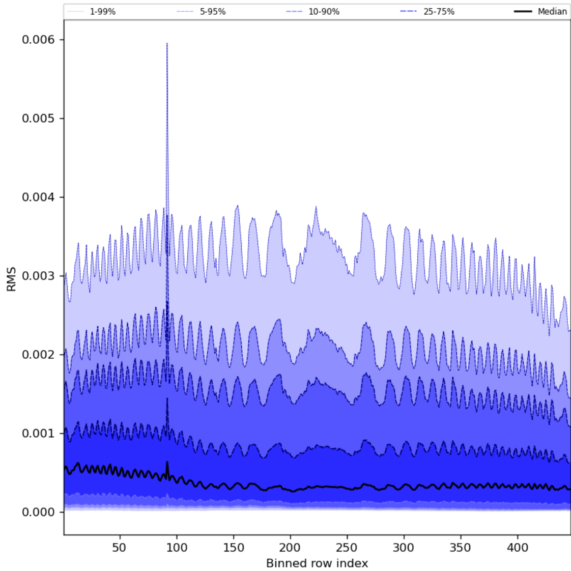
Figure 63: Along track statistics of “RMS” for 2023-09-01 to 2023-09-03
