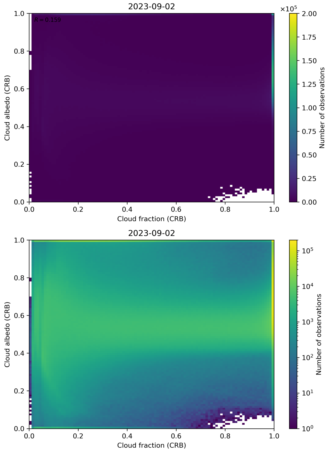
Figure 77: Scatter density plot of “Cloud fraction (CRB)” against “Cloud albedo (CRB)” for 2023-09-01 to 2023-09-03.
