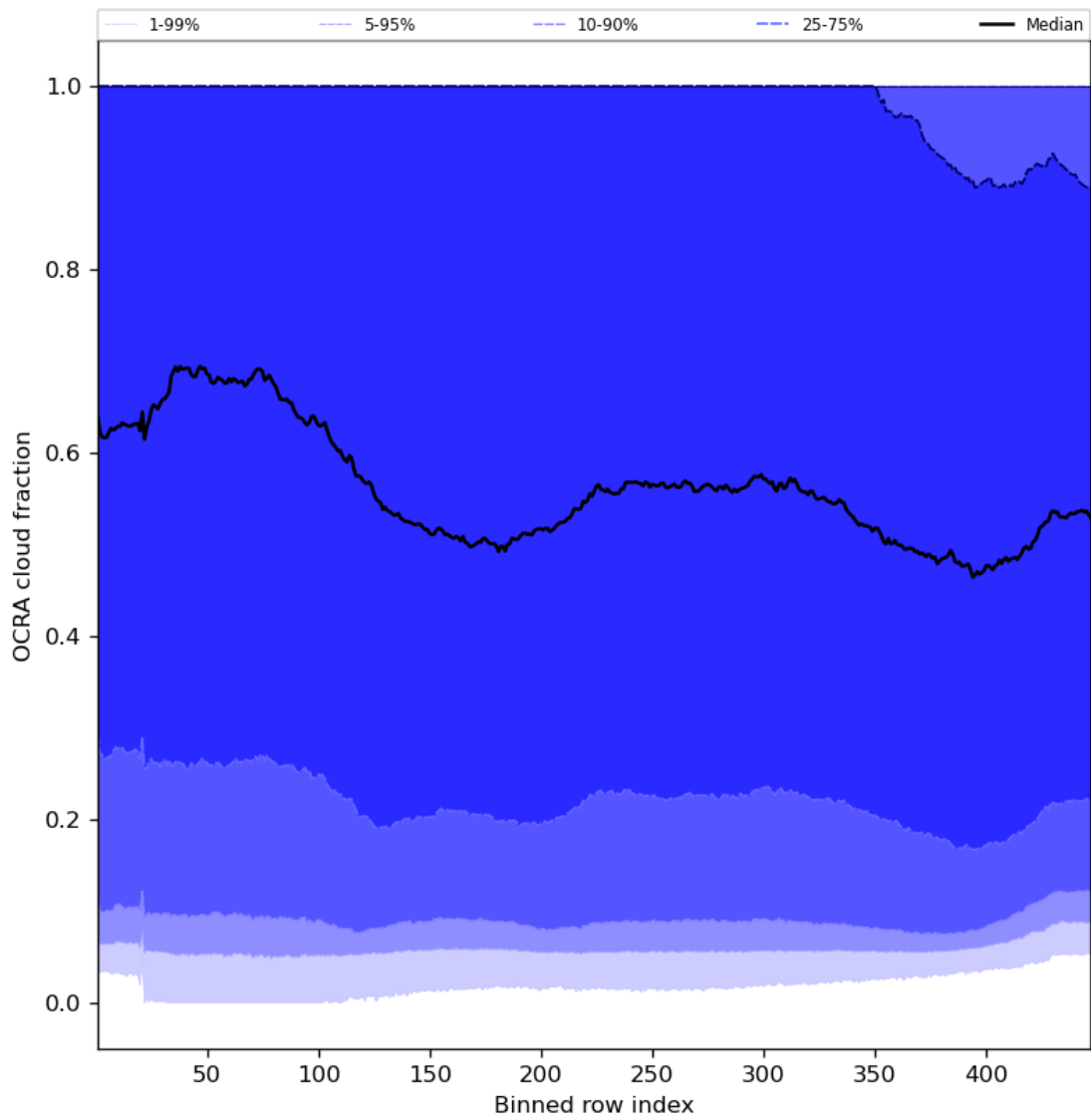
Figure 66: Along track statistics of “OCRA cloud fraction” for 2023-09-01 to 2023-09-03
