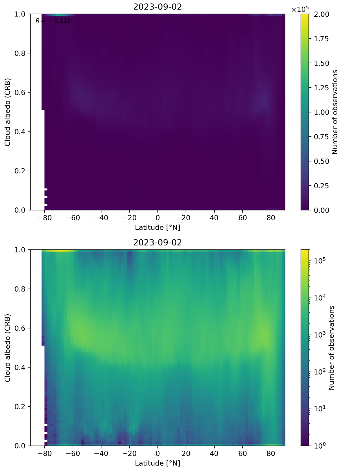
Figure 91: Scatter density plot of “Latitude” against “Cloud albedo (CRB)” for 2023-09-01 to 2023-09-03.
