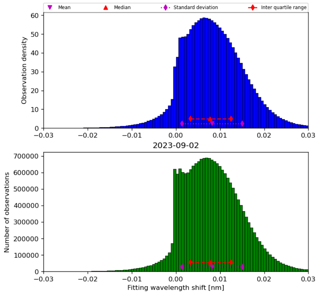
Figure 49: Histogram of “Fitting wavelength shift” for 2023-09-01 to 2023-09-03
