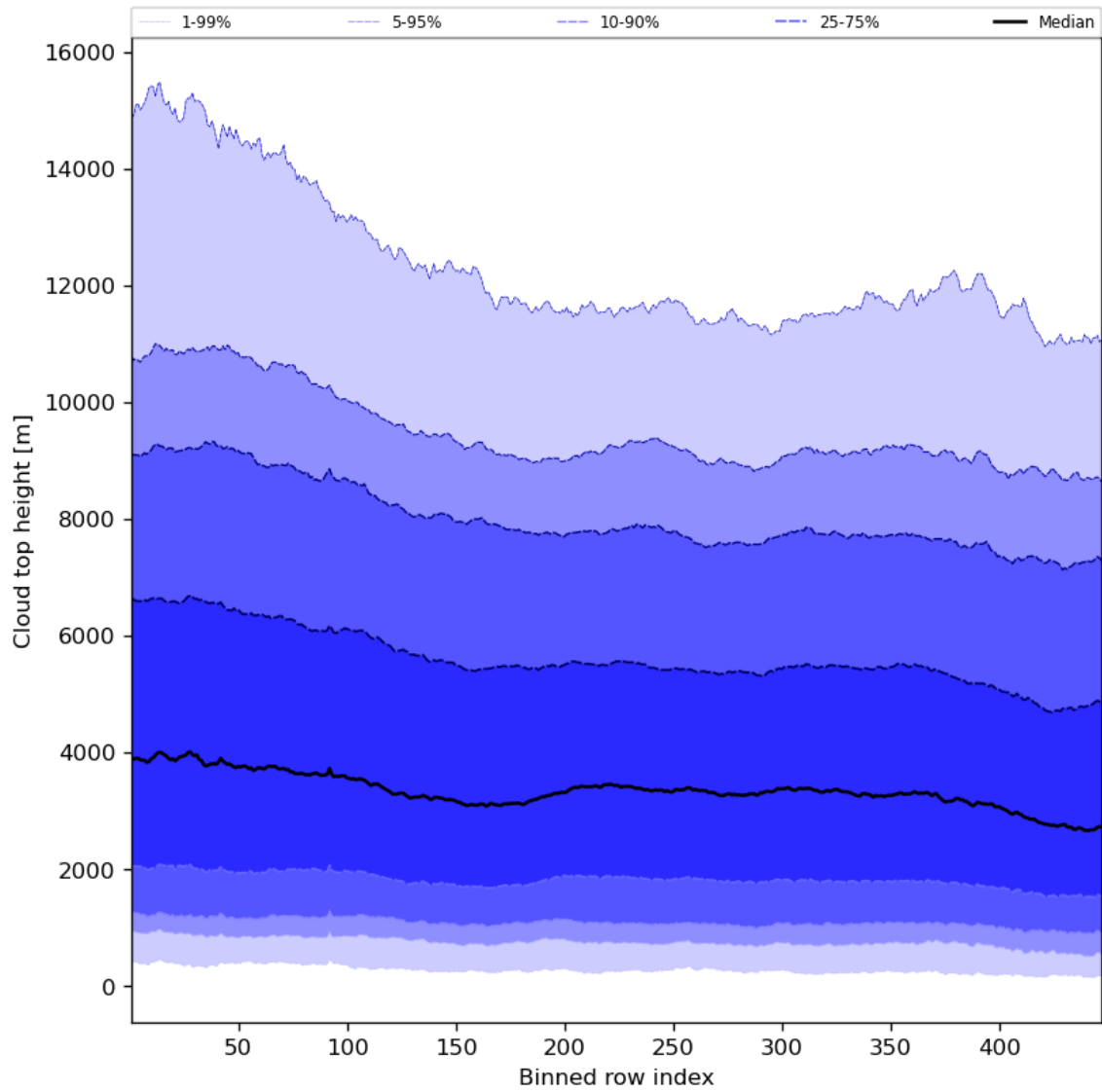
Figure 56: Along track statistics of “Cloud top height” for 2023-09-01 to 2023-09-03
