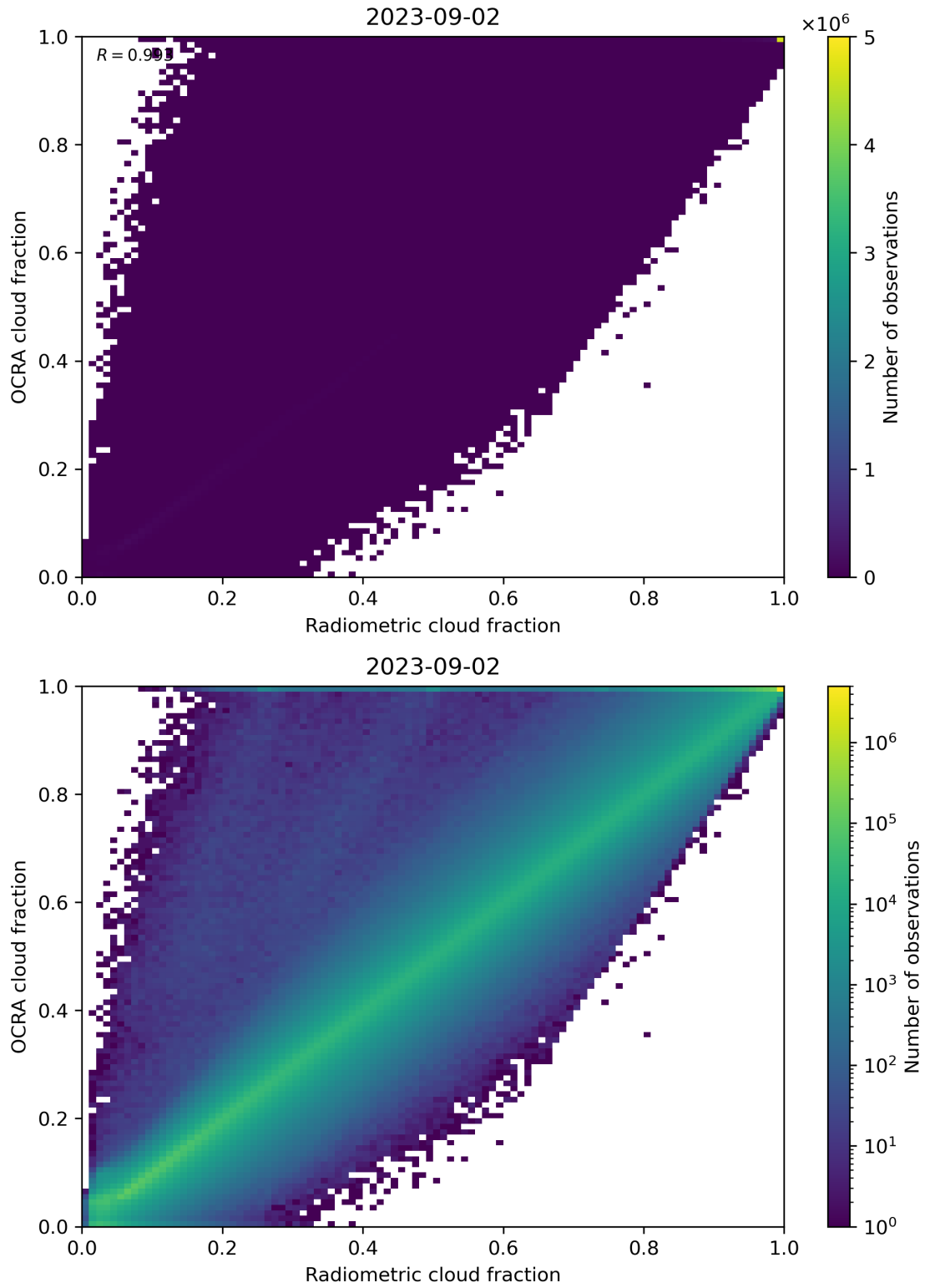
Figure 72: Scatter density plot of “Radiometric cloud fraction” against “OCRA cloud fraction” for 2023-09-01 to 2023-09-03.
