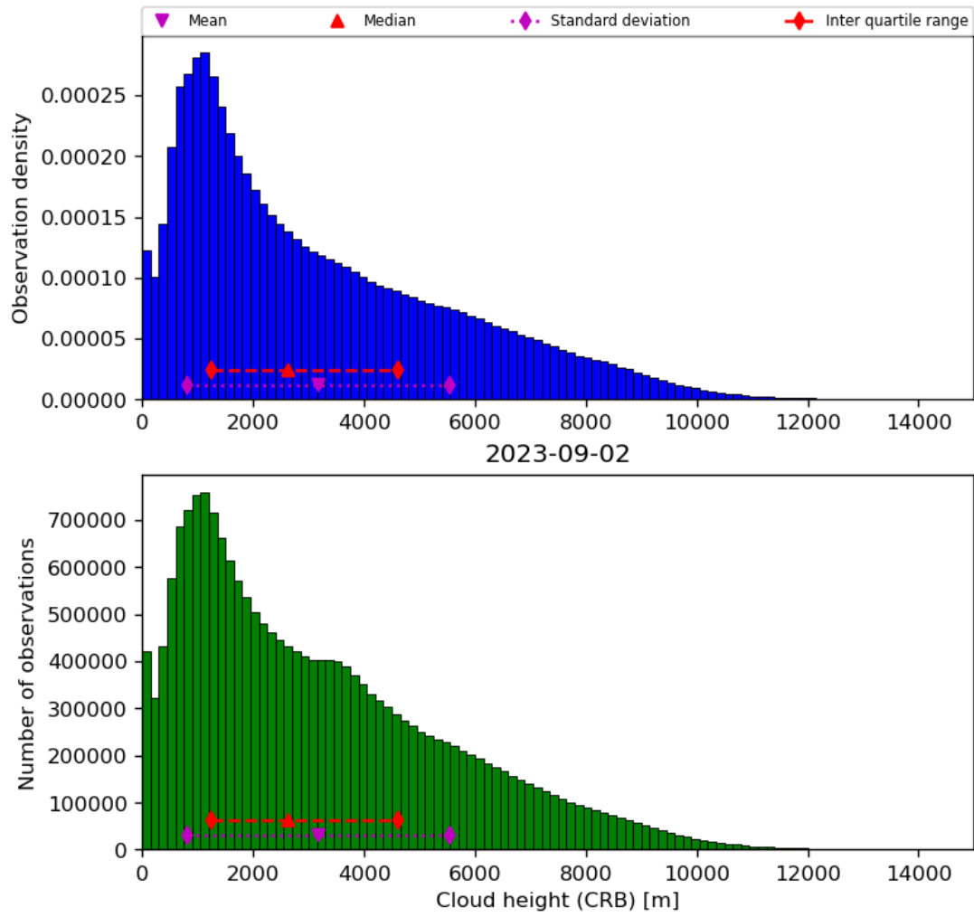
Figure 43: Histogram of “Cloud height (CRB)” for 2023-09-01 to 2023-09-03
