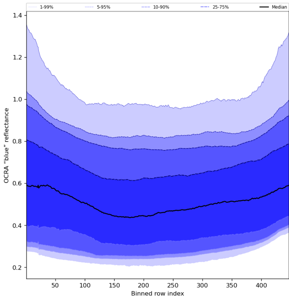
Figure 67: Along track statistics of “OCRA “blue” reflectance” for 2023-09-01 to 2023-09-03
