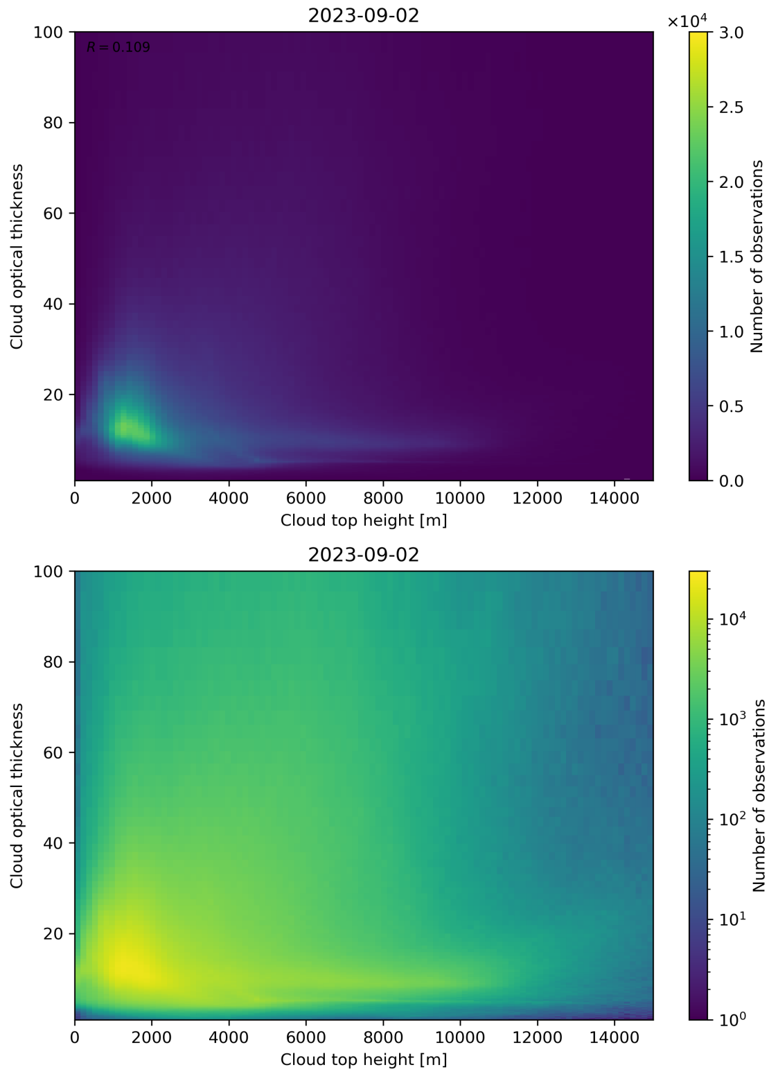
Figure 90: Scatter density plot of “Cloud top height” against “Cloud optical thickness” for 2023-09-01 to 2023-09-03.
