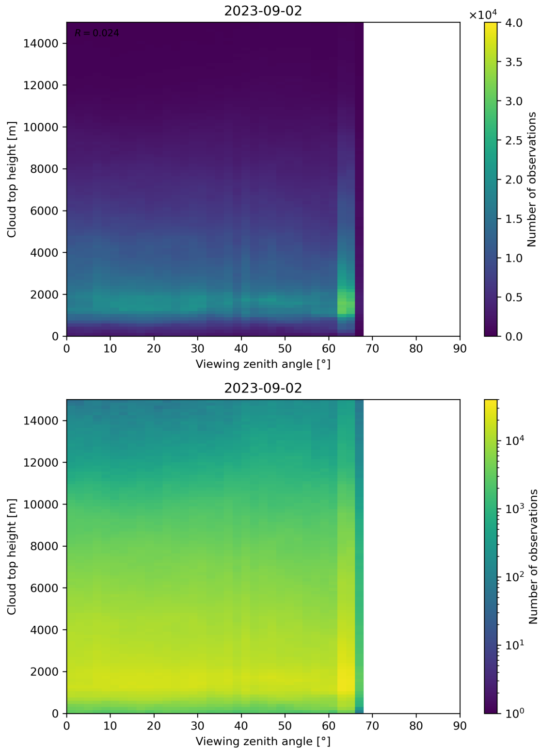
Figure 112: Scatter density plot of “Viewing zenith angle” against “Cloud top height” for 2023-09-01 to 2023-09-03.
