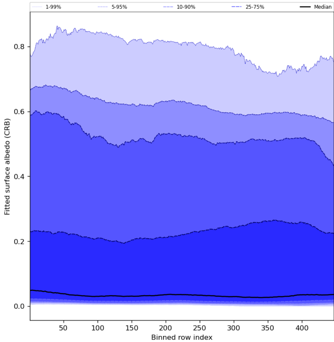
Figure 62: Along track statistics of “Fitted surface albedo (CRB)” for 2023-09-01 to 2023-09-03
