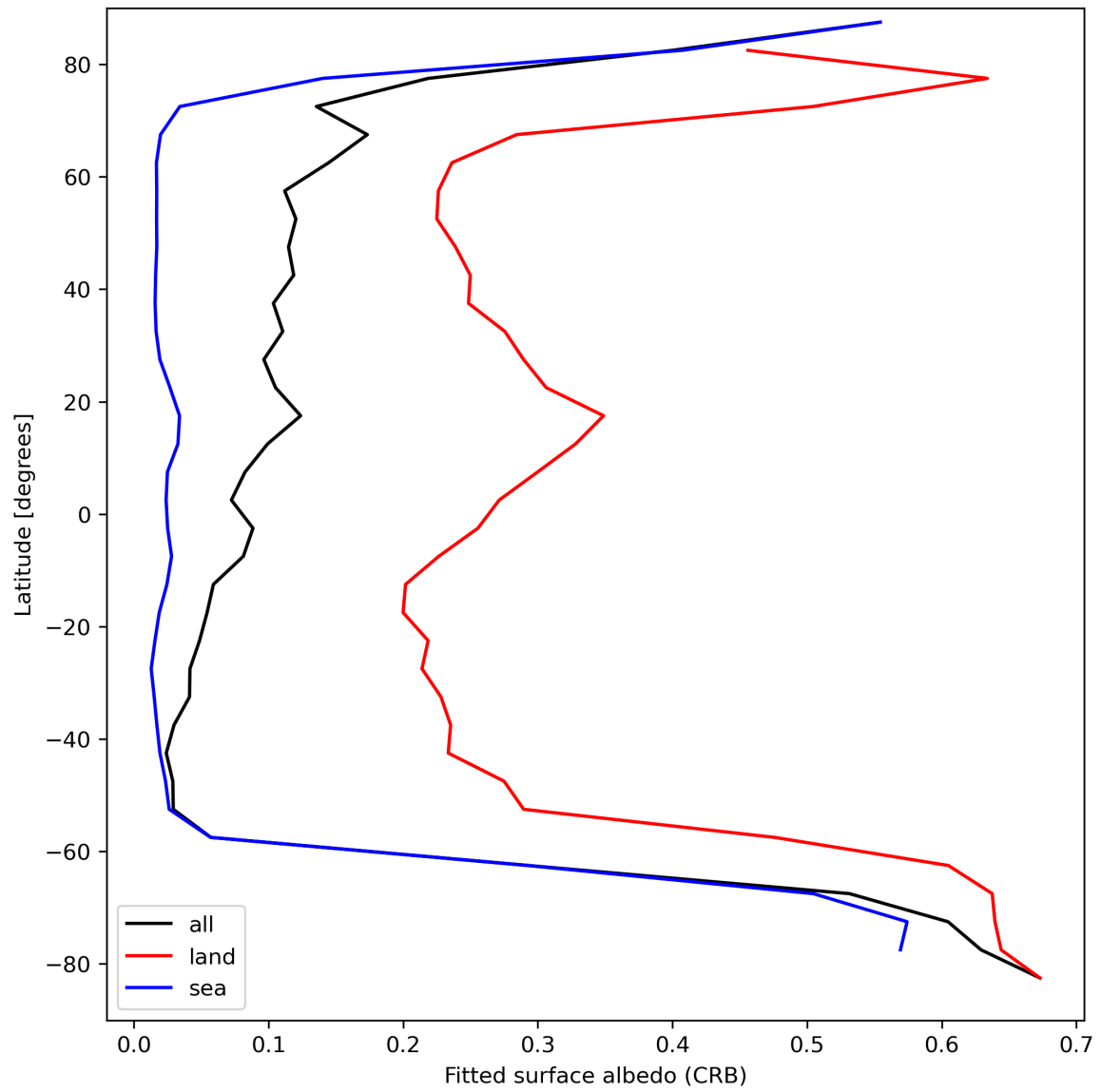
Figure 30: Zonal average of “Fitted surface albedo (CRB)” for 2023-09-01 to 2023-09-03.
