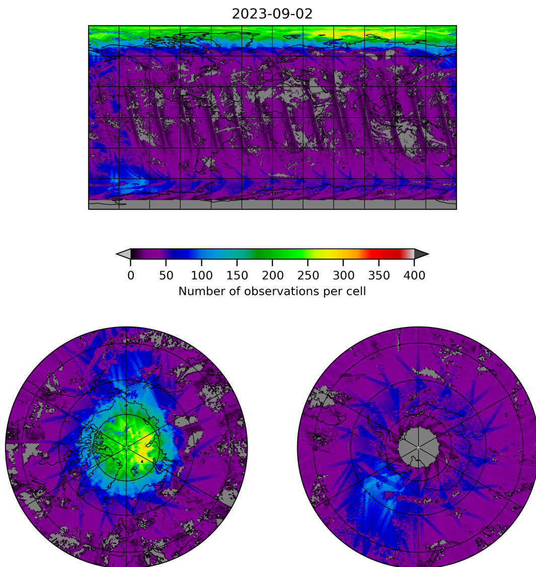
Figure 21: Map of the number of observations for 2023-09-01 to 2023-09-03
