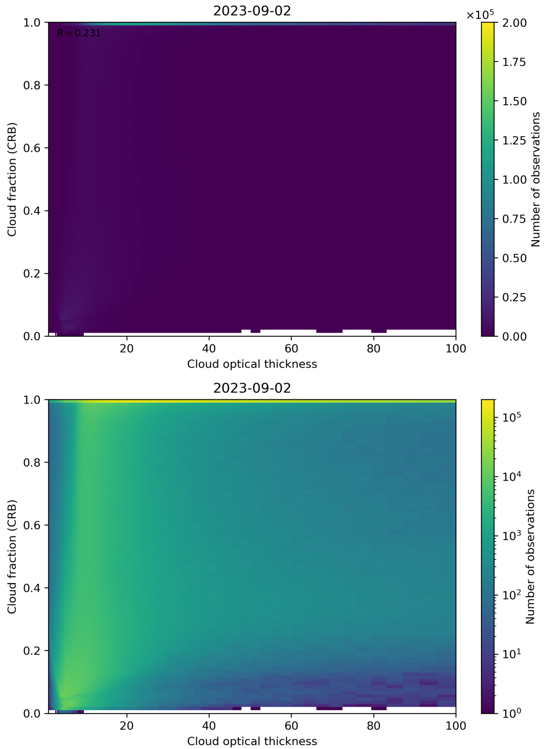
Figure 84: Scatter density plot of “Cloud optical thickness” against “Cloud fraction (CRB)” for 2023-09-01 to 2023-09-03.
