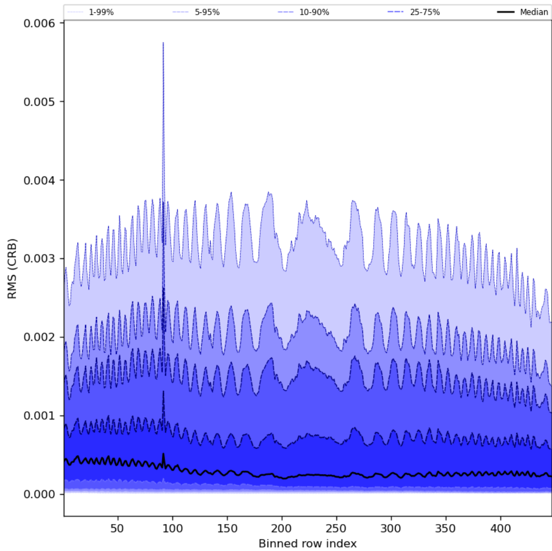
Figure 64: Along track statistics of “RMS (CRB)” for 2023-09-01 to 2023-09-03
