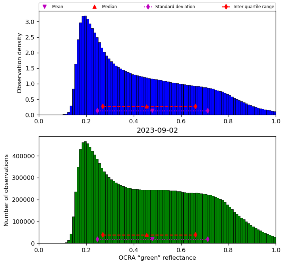
Figure 52: Histogram of “OCRA “green” reflectance” for 2023-09-01 to 2023-09-03
