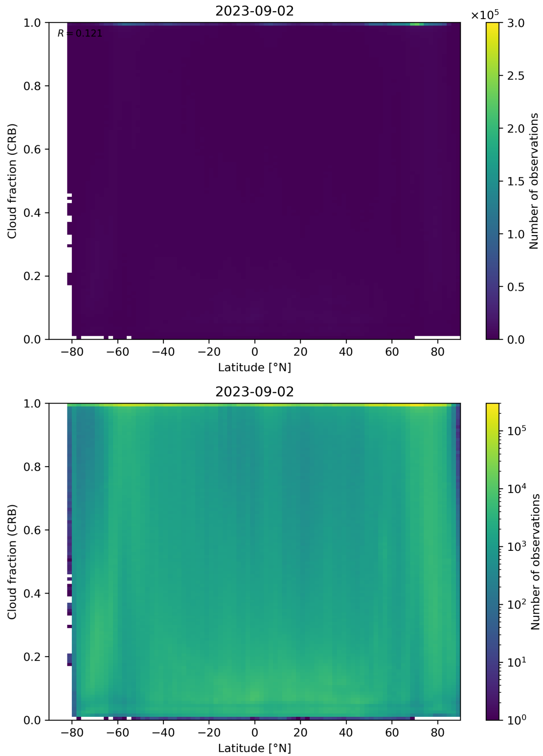
Figure 94: Scatter density plot of “Latitude” against “Cloud fraction (CRB)” for 2023-09-01 to 2023-09-03.
