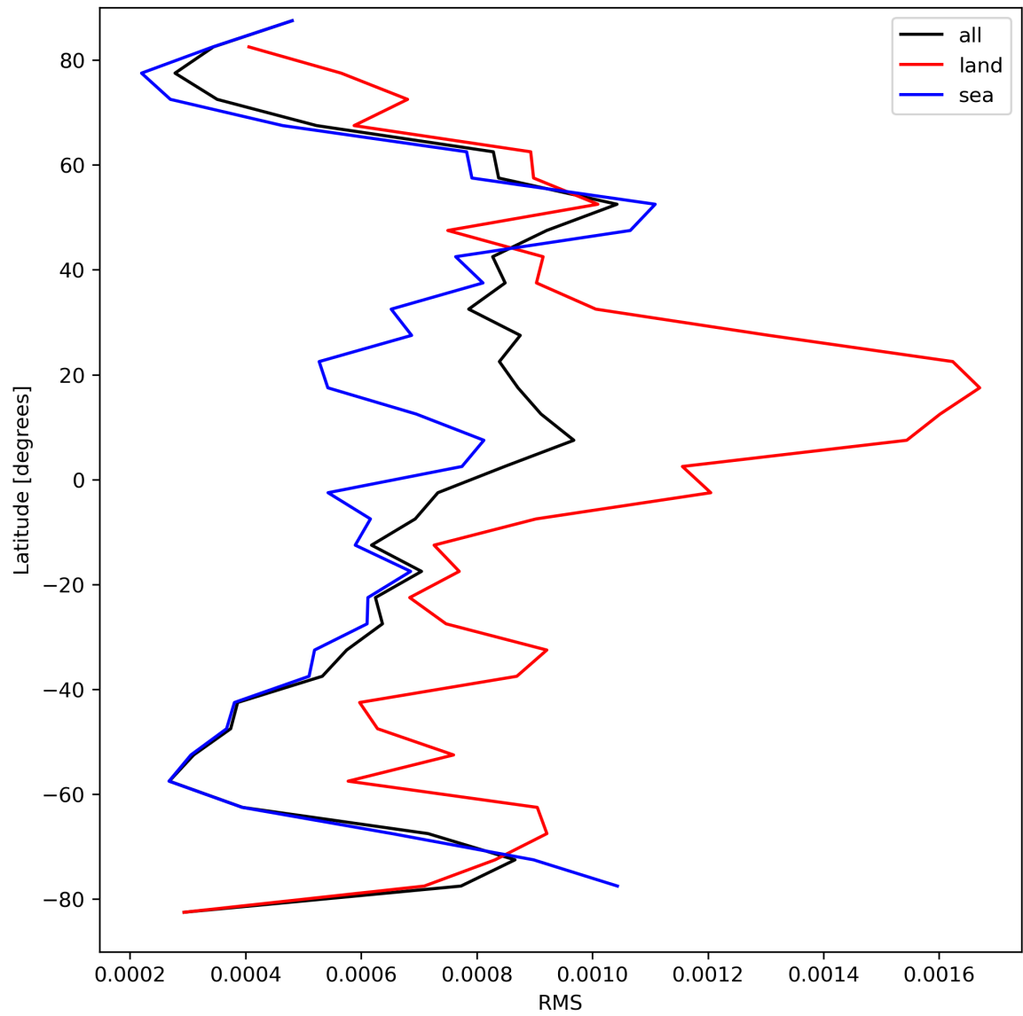
Figure 31: Zonal average of “RMS” for 2023-09-01 to 2023-09-03.
