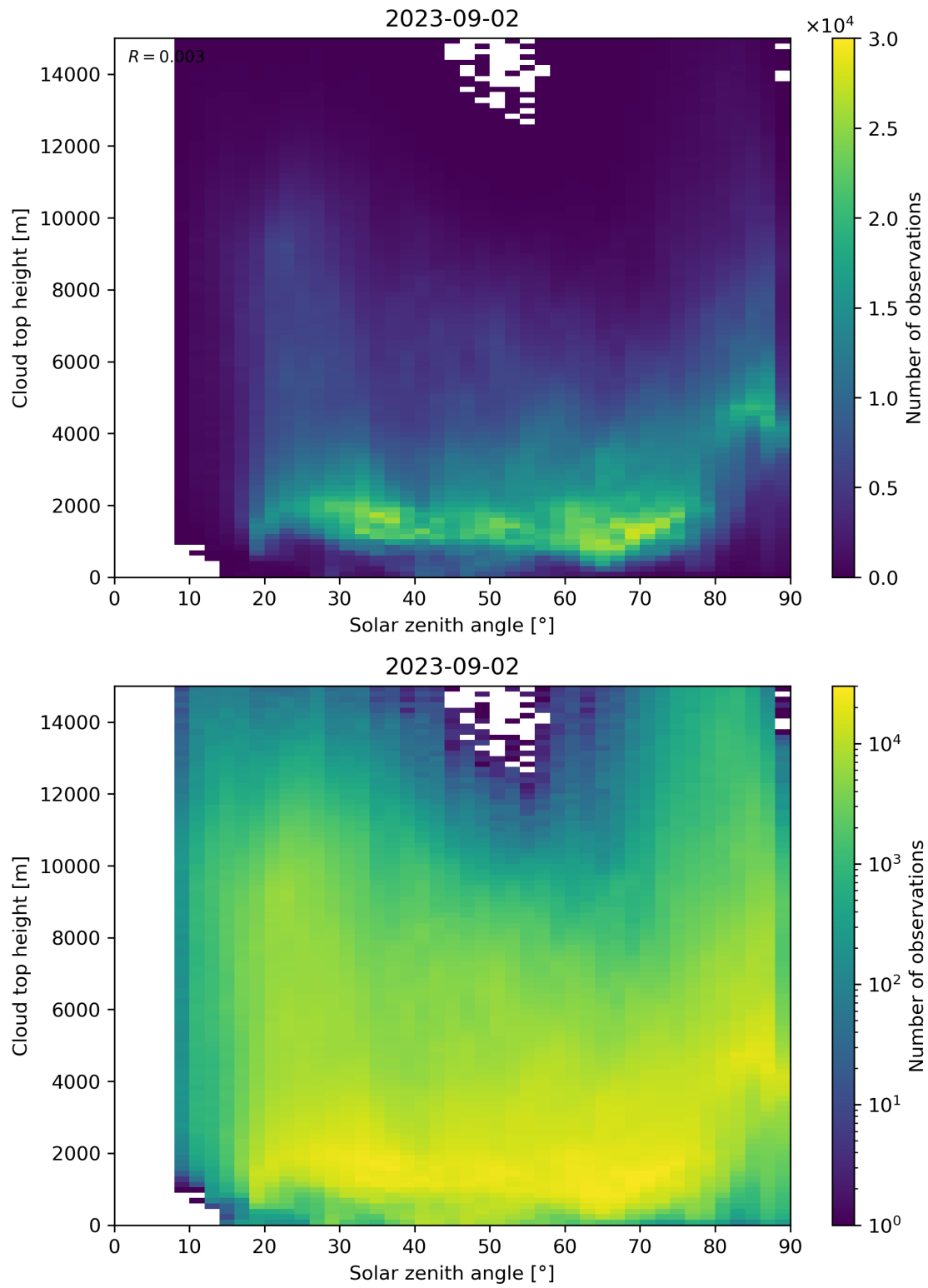
Figure 104: Scatter density plot of “Solar zenith angle” against “Cloud top height” for 2023-09-01 to 2023-09-03.
