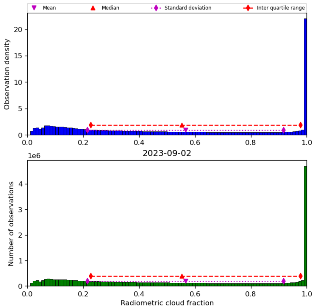
Figure 39: Histogram of “Radiometric cloud fraction” for 2023-09-01 to 2023-09-03
