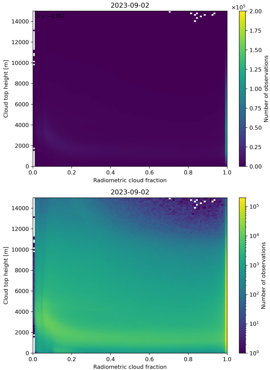
Figure 76: Scatter density plot of “Radiometric cloud fraction” against “Cloud top height” for 2023-09-01 to 2023-09-03.
