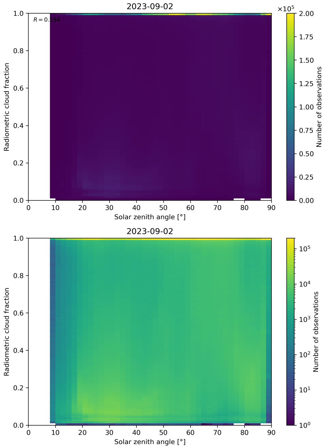
Figure 99: Scatter density plot of “Solar zenith angle” against “Radiometric cloud fraction” for 2023-09-01 to 2023-09-03.
