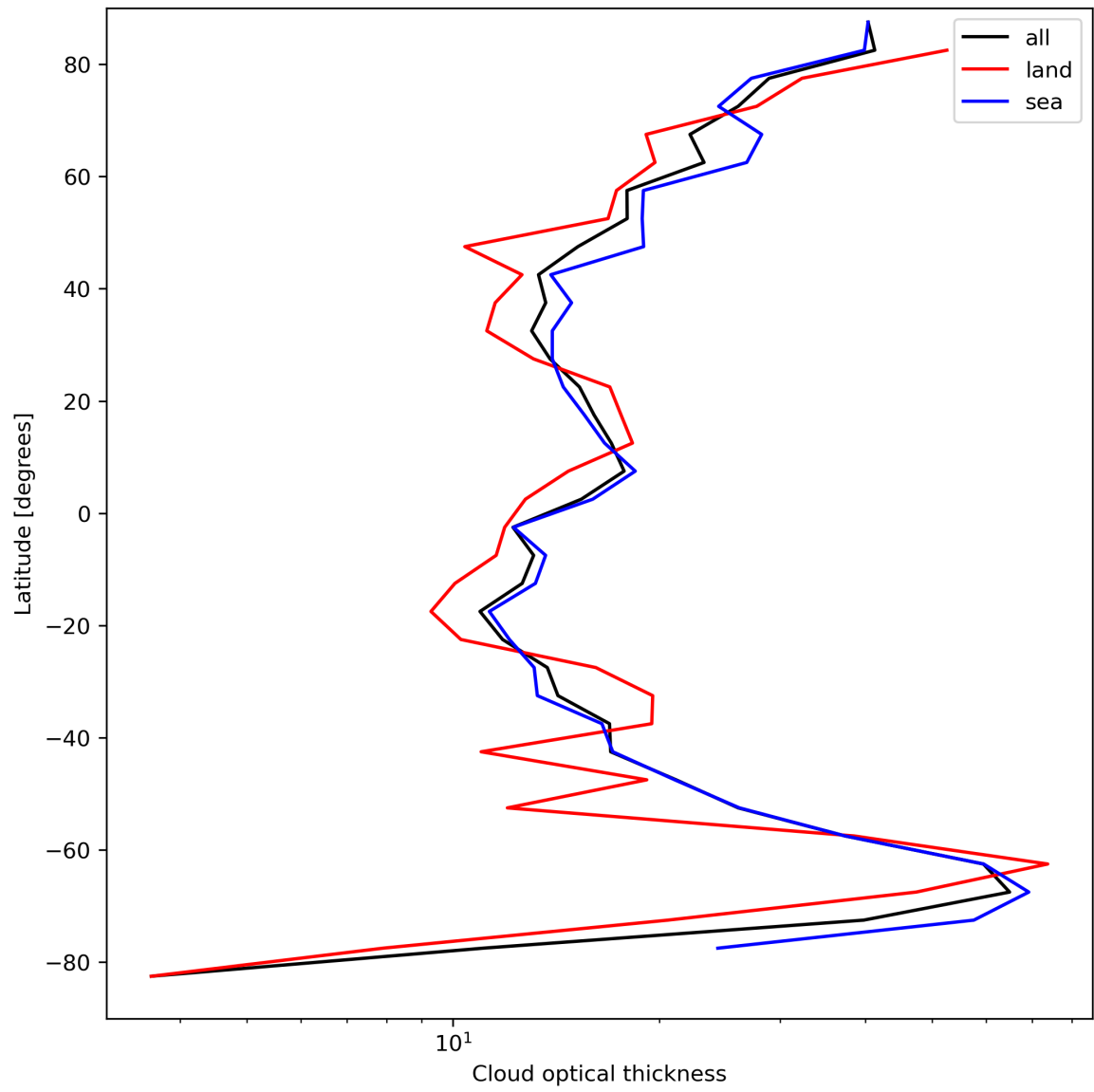
Figure 25: Zonal average of “Cloud optical thickness” for 2023-09-01 to 2023-09-03.
