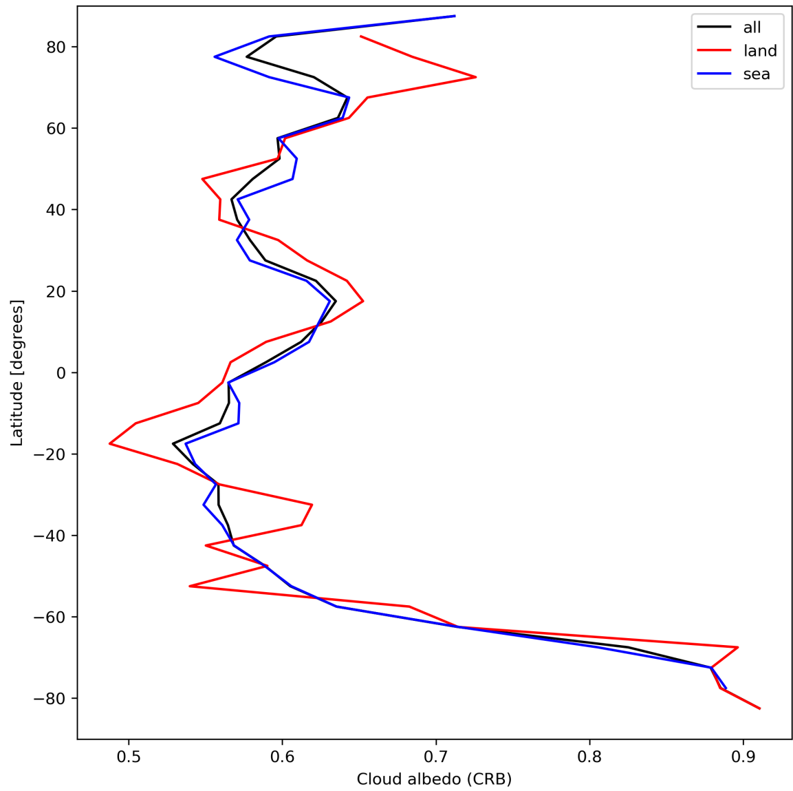
Figure 28: Zonal average of “Cloud albedo (CRB)” for 2023-09-01 to 2023-09-03.
