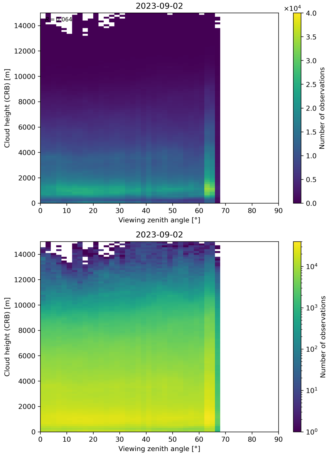
Figure 110: Scatter density plot of “Viewing zenith angle” against “Cloud height (CRB)” for 2023-09-01 to 2023-09-03.
