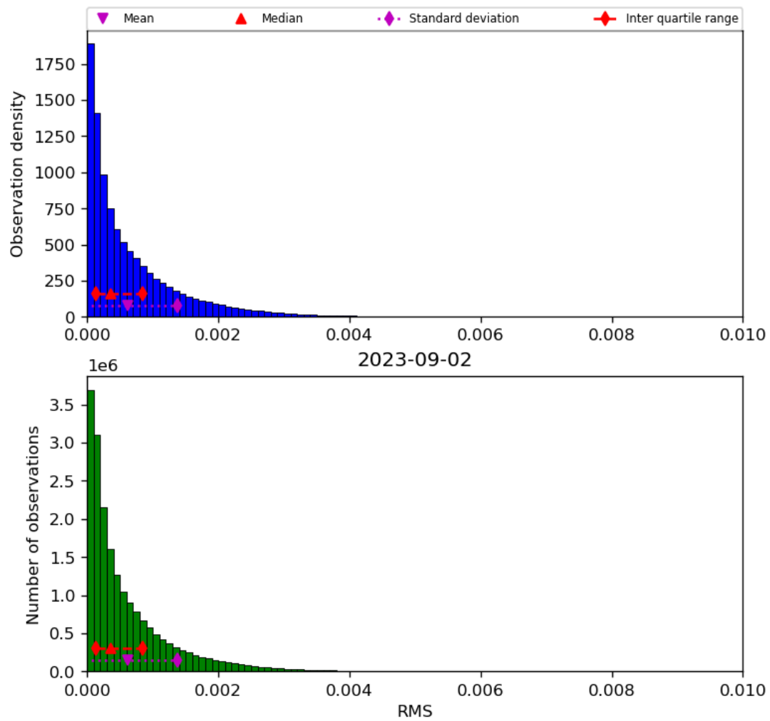
Figure 47: Histogram of “RMS” for 2023-09-01 to 2023-09-03
