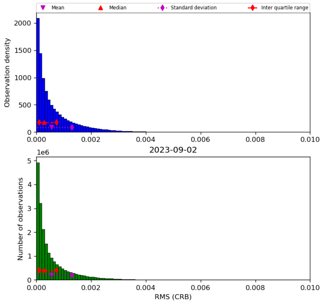
Figure 48: Histogram of “RMS (CRB)” for 2023-09-01 to 2023-09-03
