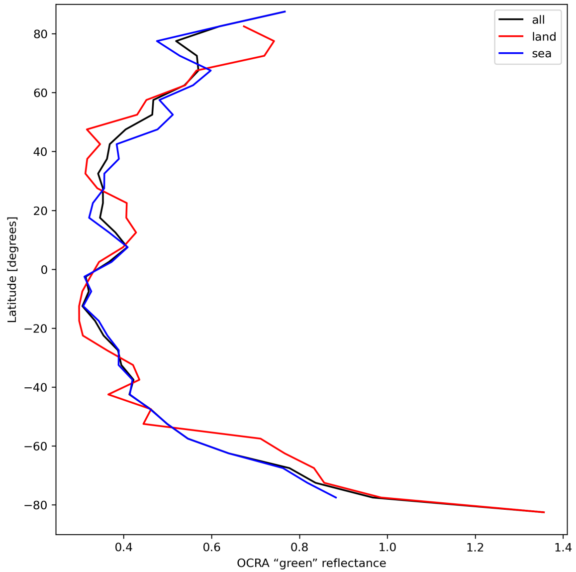
Figure 36: Zonal average of “OCRA “green” reflectance” for 2023-09-01 to 2023-09-03.
