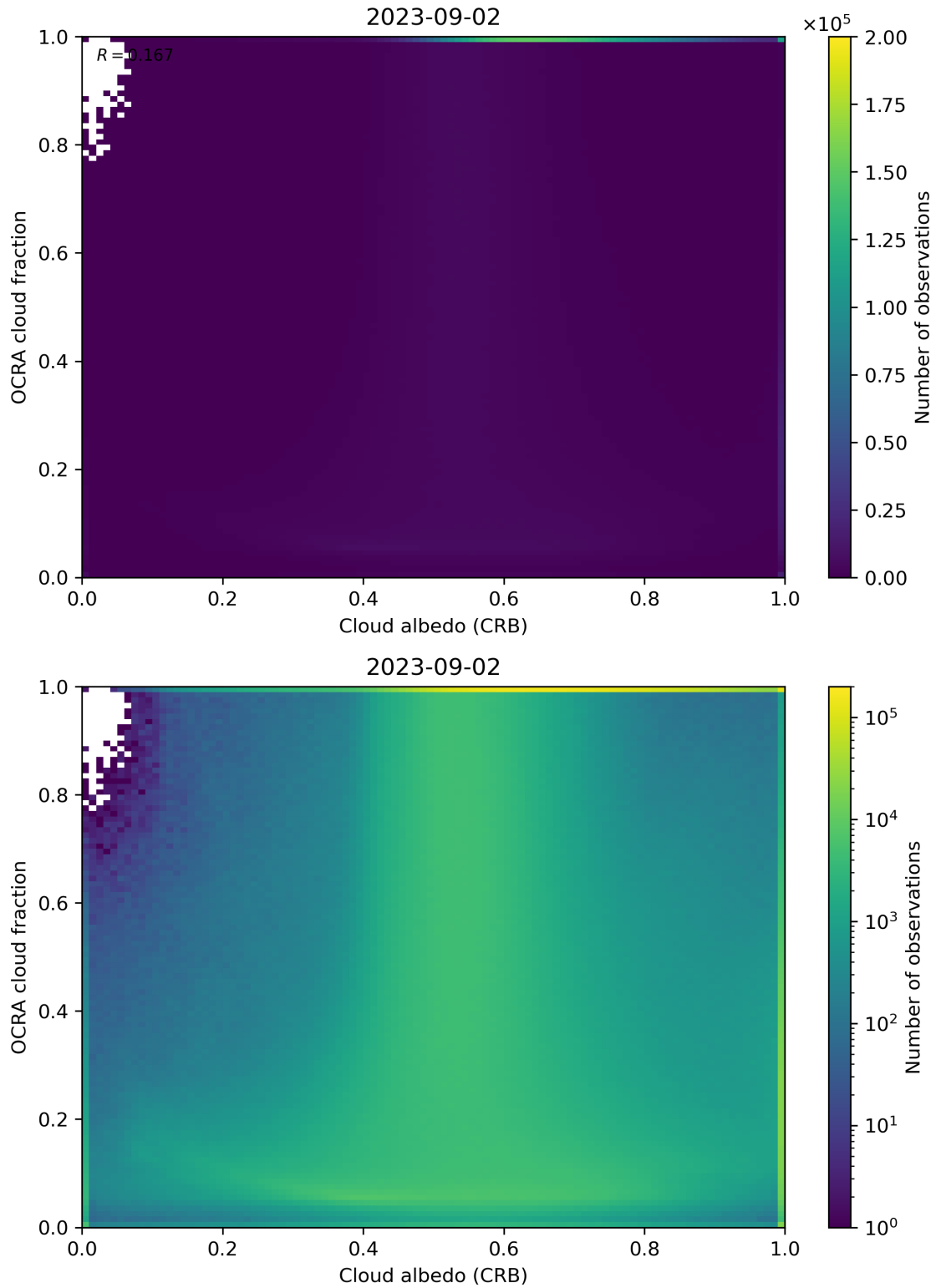
Figure 70: Scatter density plot of “Cloud albedo (CRB)” against “OCRA cloud fraction” for 2023-09-01 to 2023-09-03.
