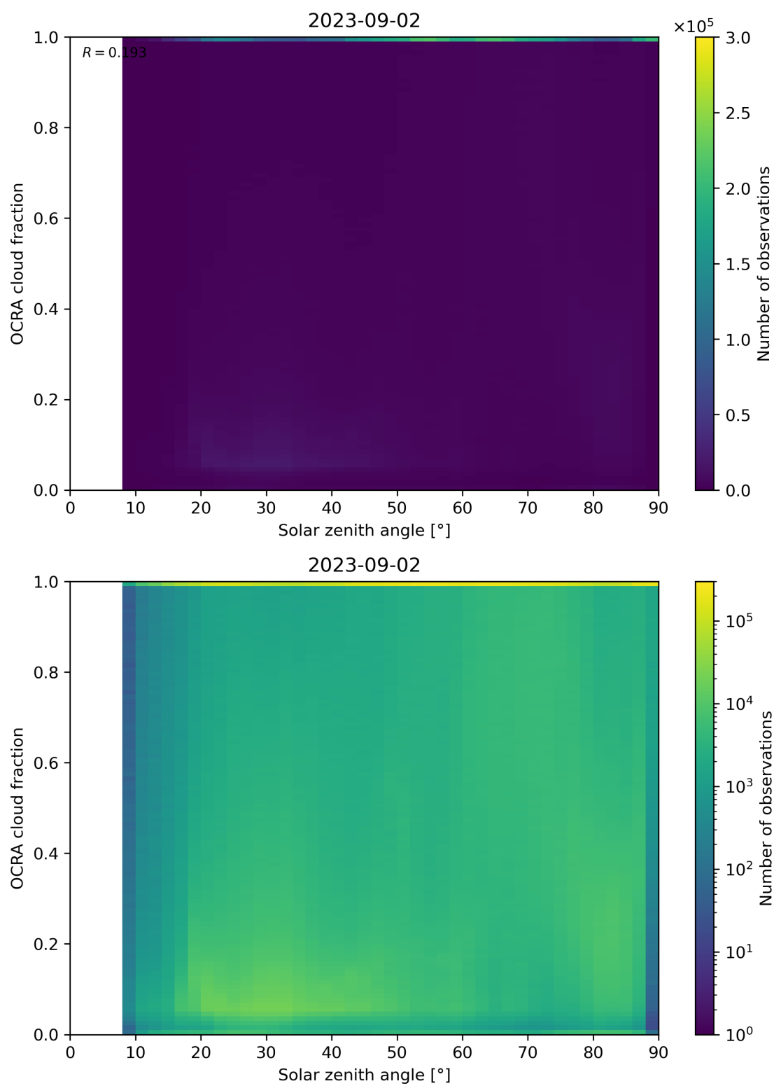
Figure 100: Scatter density plot of “Solar zenith angle” against “OCRA cloud fraction” for 2023-09-01 to 2023-09-03.
