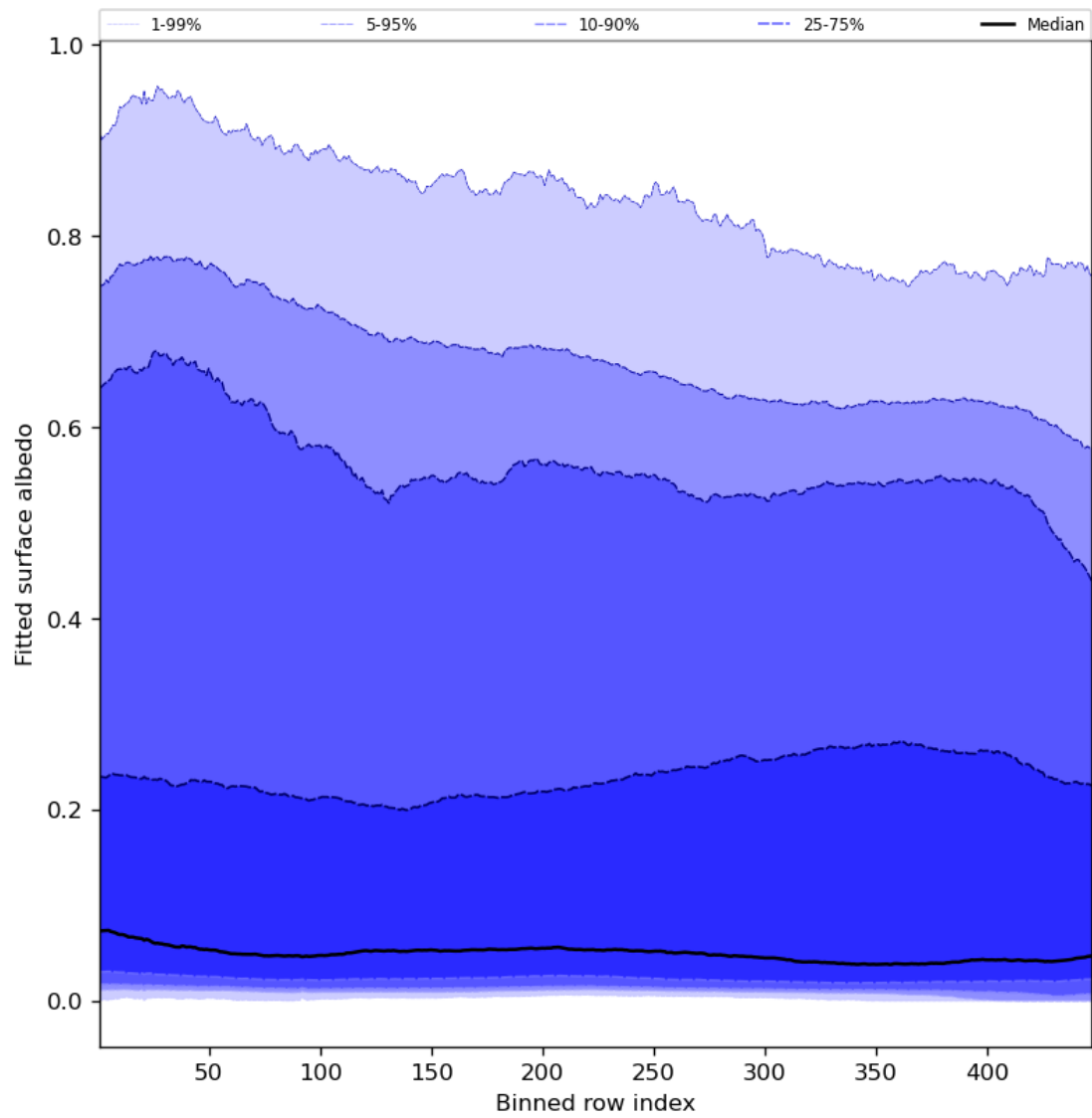
Figure 61: Along track statistics of “Fitted surface albedo” for 2023-09-01 to 2023-09-03
