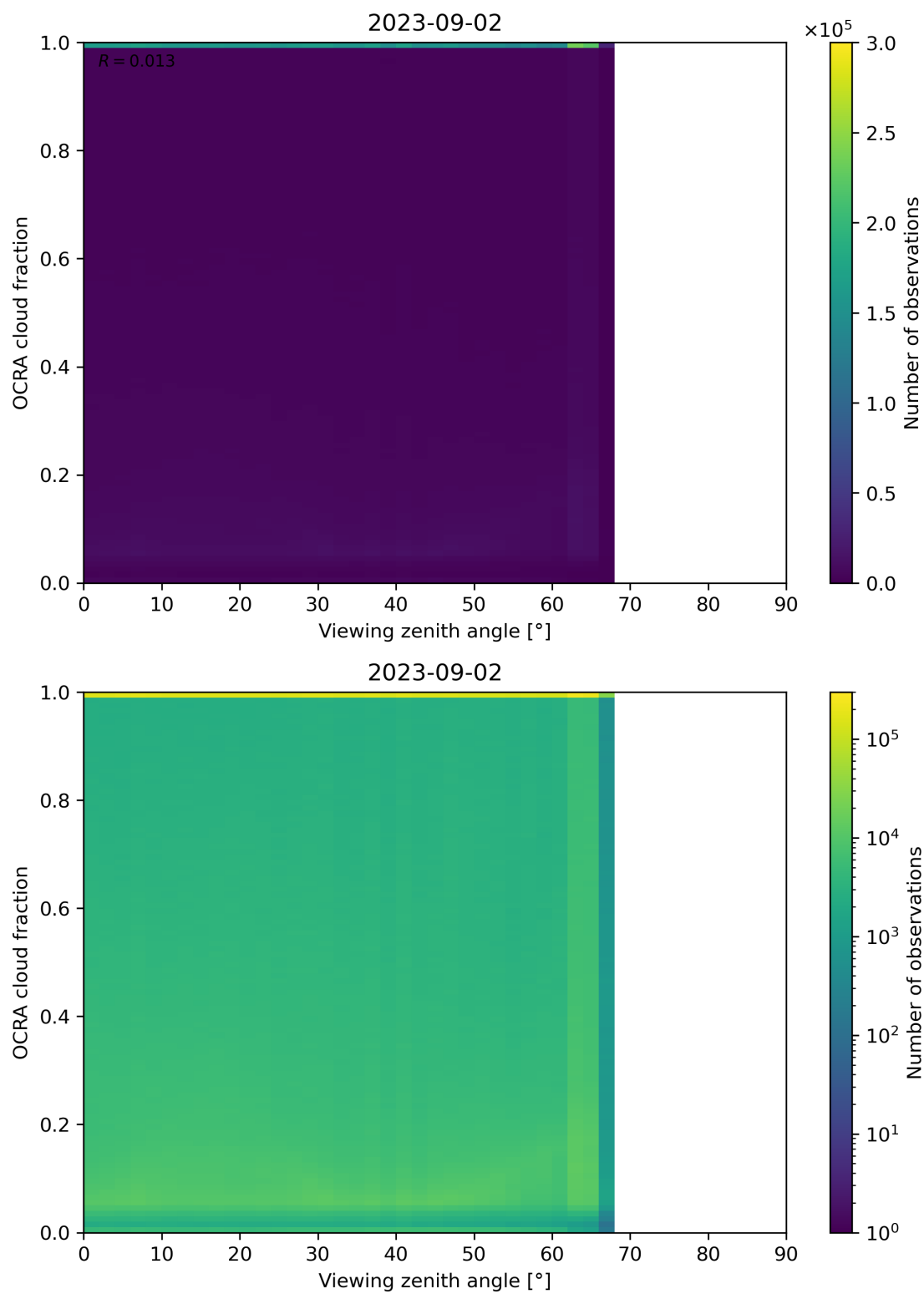
Figure 108: Scatter density plot of “Viewing zenith angle” against “OCRA cloud fraction” for 2023-09-01 to 2023-09-03.
