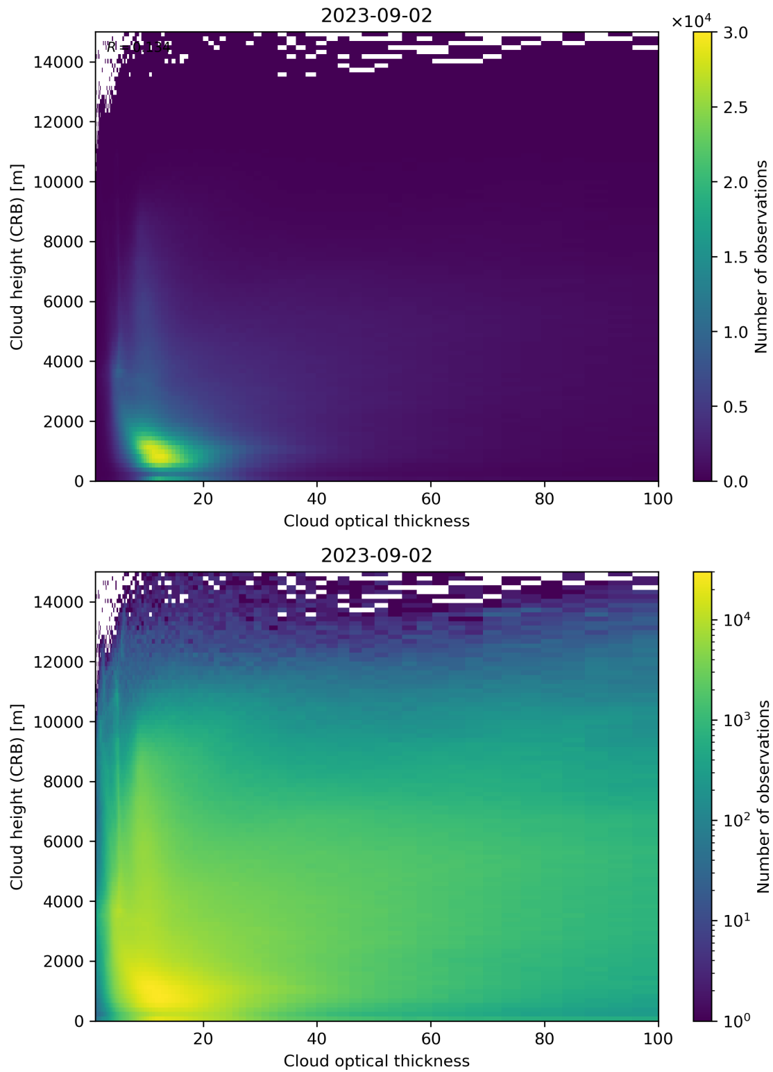
Figure 85: Scatter density plot of “Cloud optical thickness” against “Cloud height (CRB)” for 2023-09-01 to 2023-09-03.
