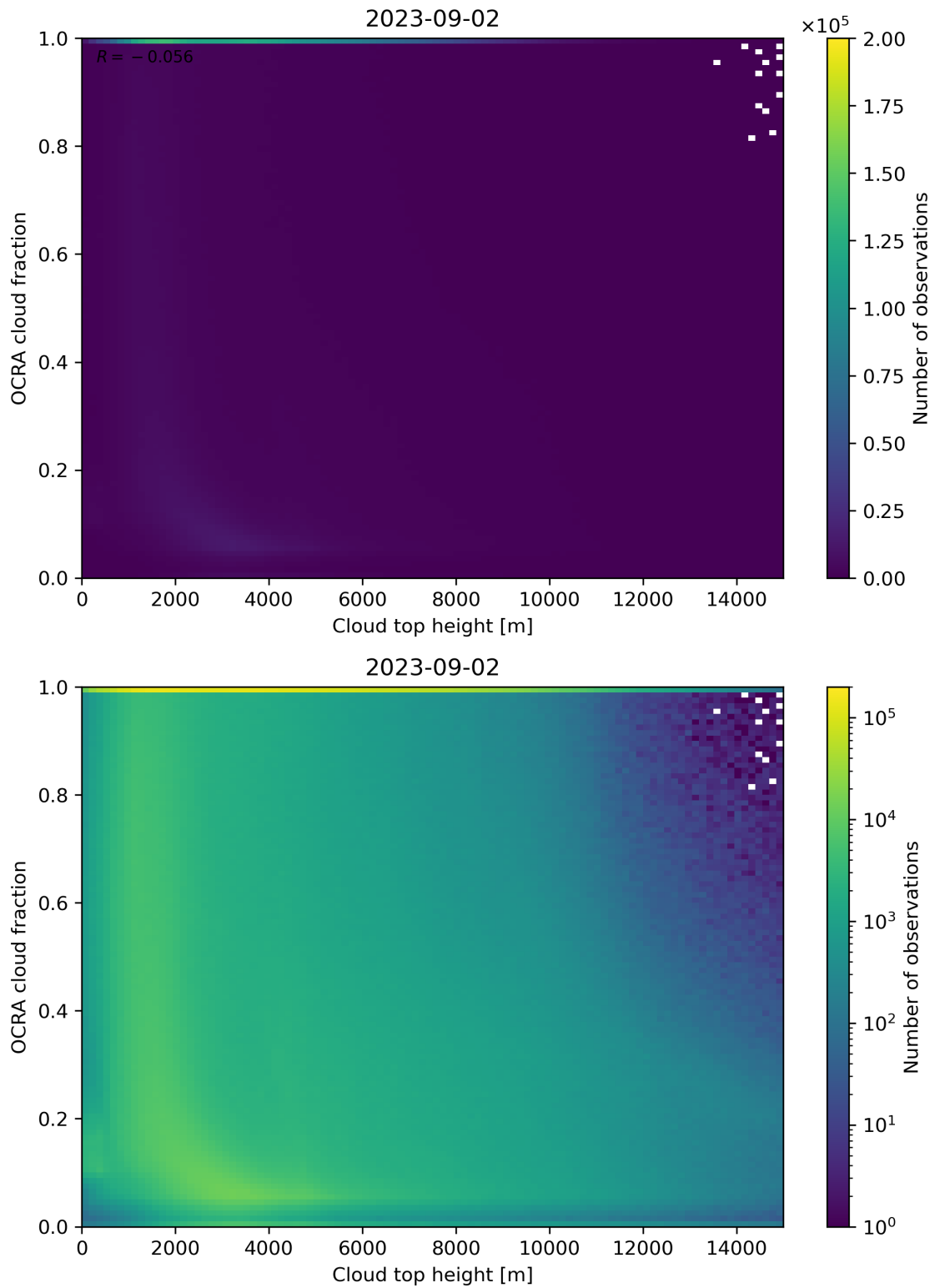
Figure 87: Scatter density plot of “Cloud top height” against “OCRA cloud fraction” for 2023-09-01 to 2023-09-03.
