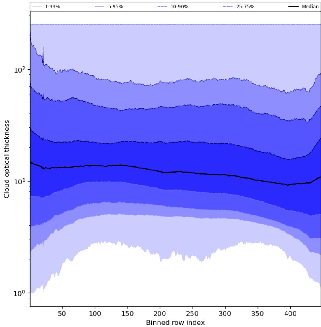
Figure 57: Along track statistics of “Cloud optical thickness” for 2023-09-01 to 2023-09-03
