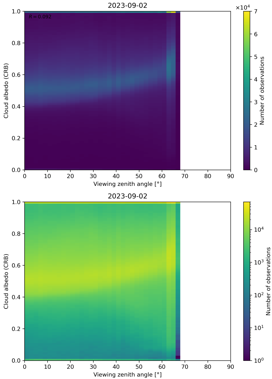
Figure 106: Scatter density plot of “Viewing zenith angle” against “Cloud albedo (CRB)” for 2023-09-01 to 2023-09-03.
