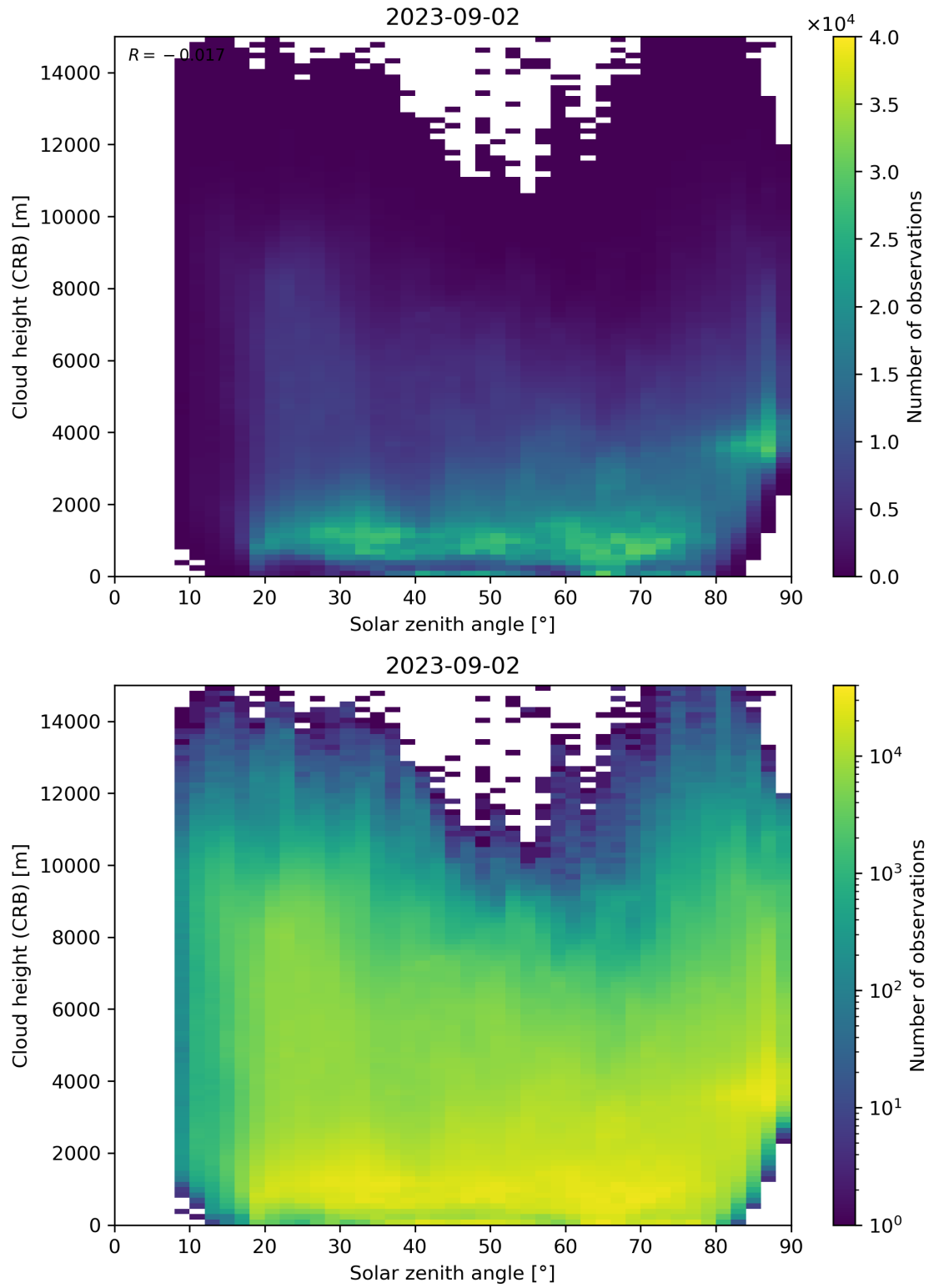
Figure 102: Scatter density plot of “Solar zenith angle” against “Cloud height (CRB)” for 2023-09-01 to 2023-09-03.
