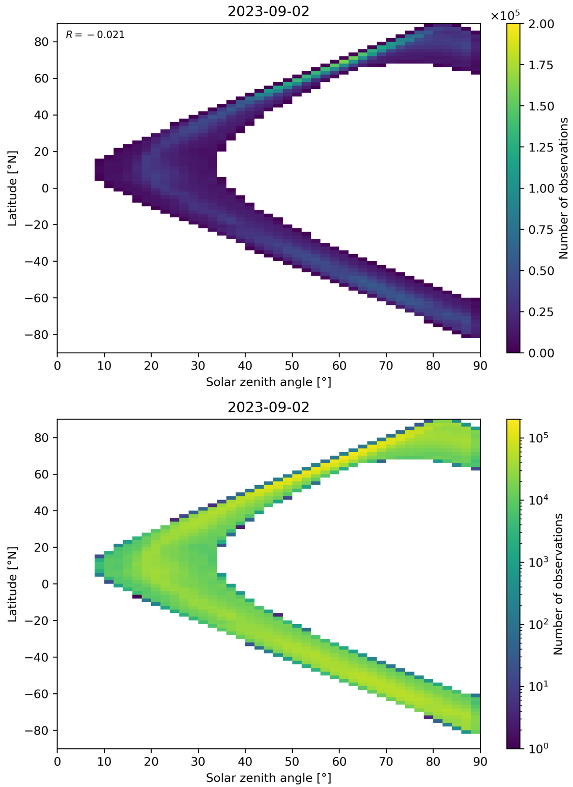
Figure 105: Scatter density plot of “Solar zenith angle” against “Latitude” for 2023-09-01 to 2023-09-03.
