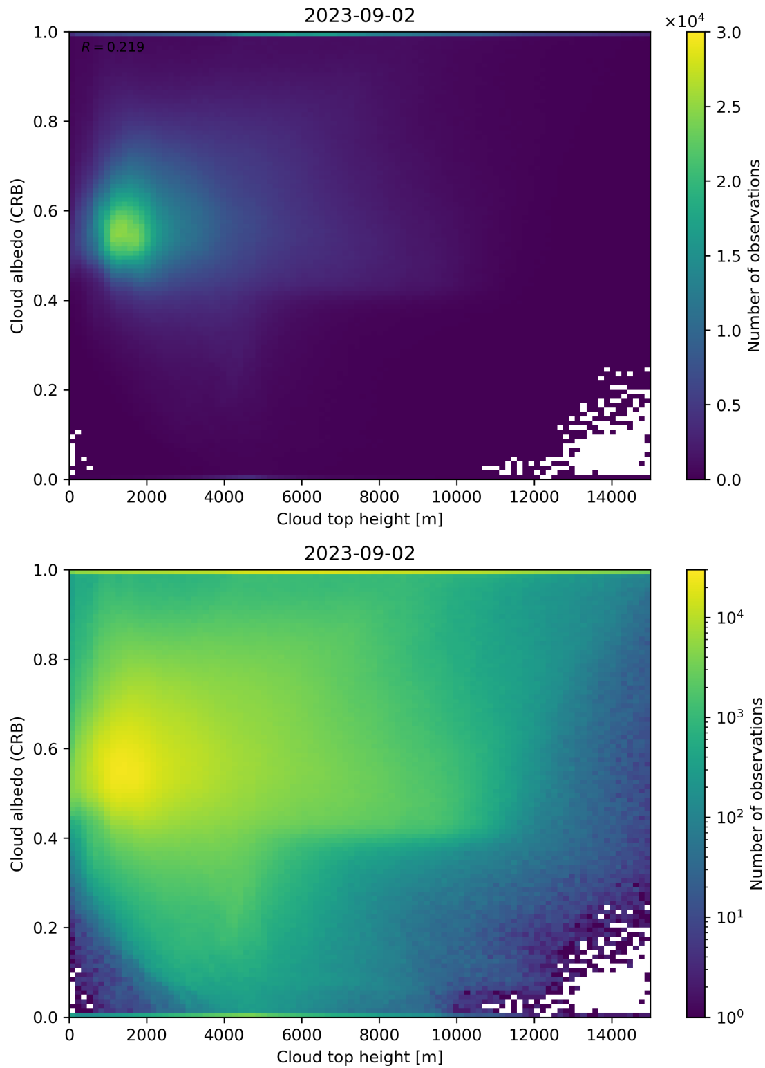
Figure 86: Scatter density plot of “Cloud top height” against “Cloud albedo (CRB)” for 2023-09-01 to 2023-09-03.
