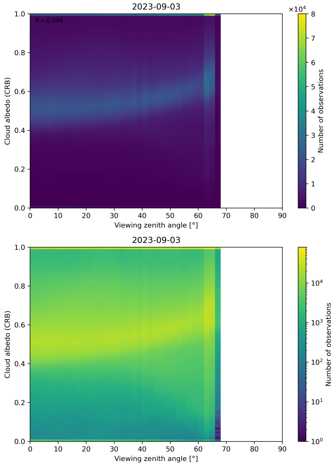
Figure 106: Scatter density plot of “Viewing zenith angle” against “Cloud albedo (CRB)” for 2023-09-02 to 2023-09-04.
