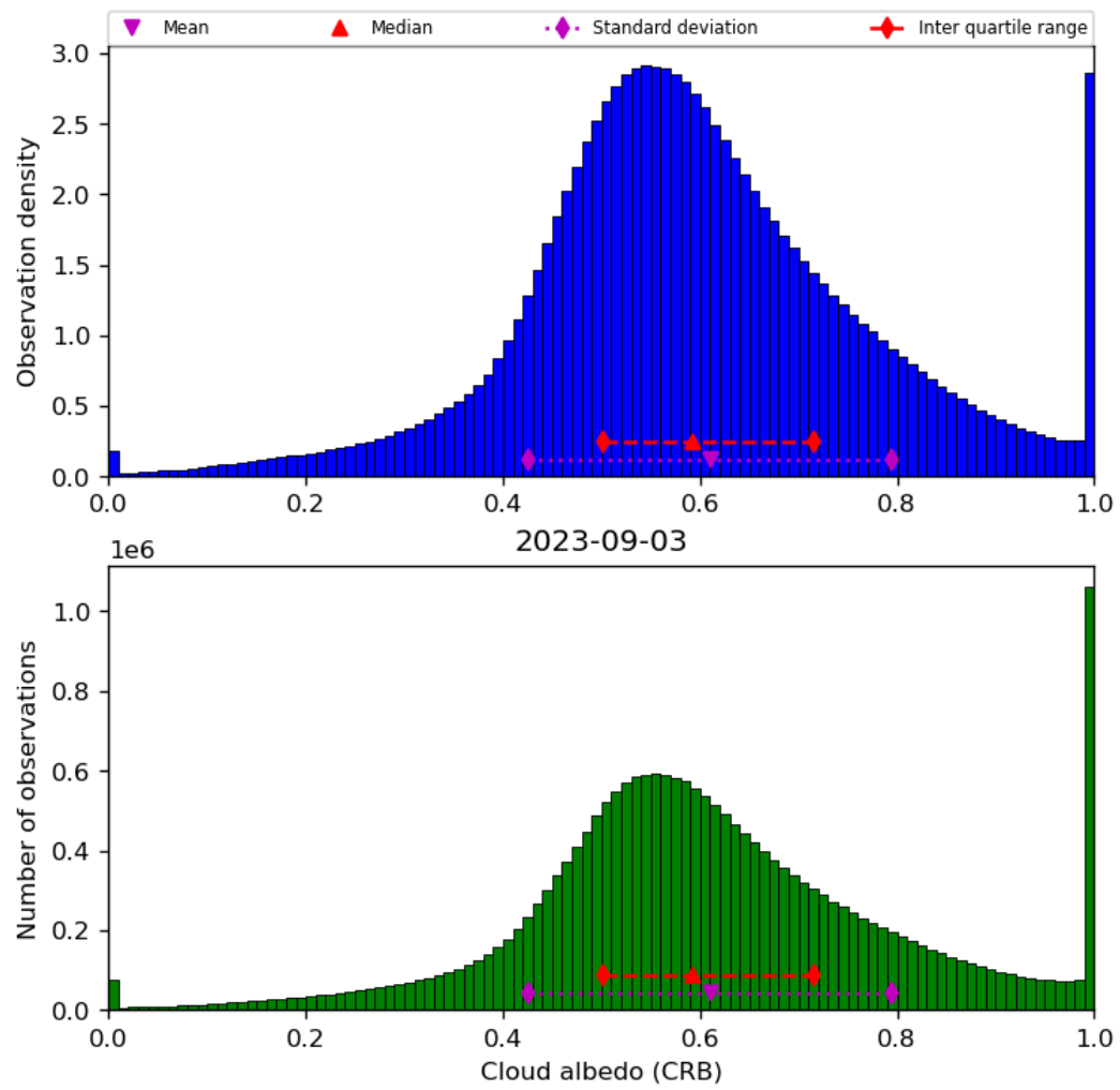
Figure 44: Histogram of “Cloud albedo (CRB)” for 2023-09-02 to 2023-09-04
