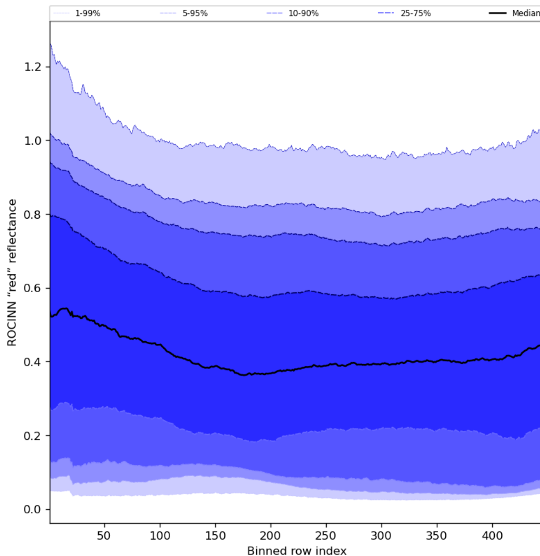
Figure 69: Along track statistics of “ROCINN “red” reflectance” for 2023-09-02 to 2023-09-04
