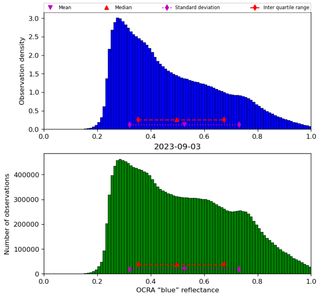
Figure 51: Histogram of “OCRA “blue” reflectance” for 2023-09-02 to 2023-09-04
