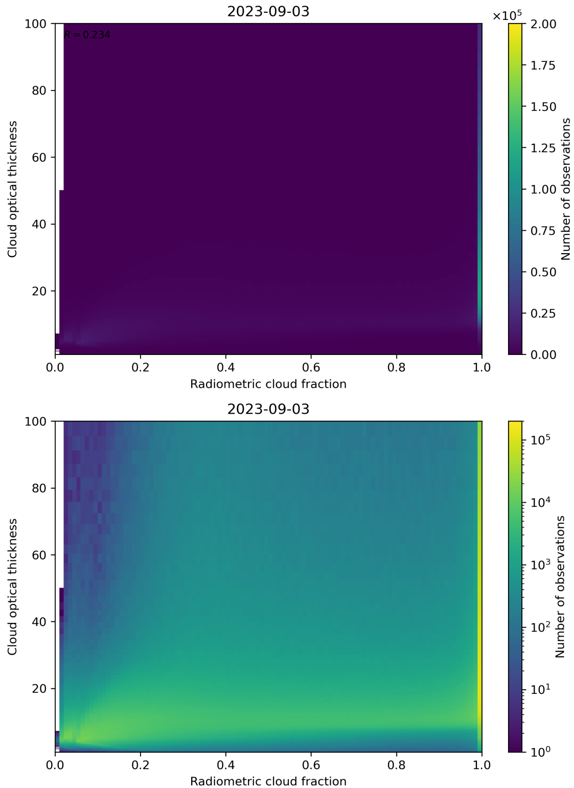
Figure 75: Scatter density plot of “Radiometric cloud fraction” against “Cloud optical thickness” for 2023-09-02 to 2023-09-04.
