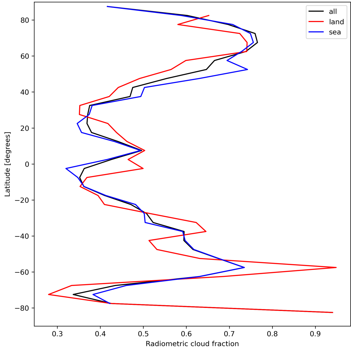
Figure 23: Zonal average of “Radiometric cloud fraction” for 2023-09-02 to 2023-09-04.
