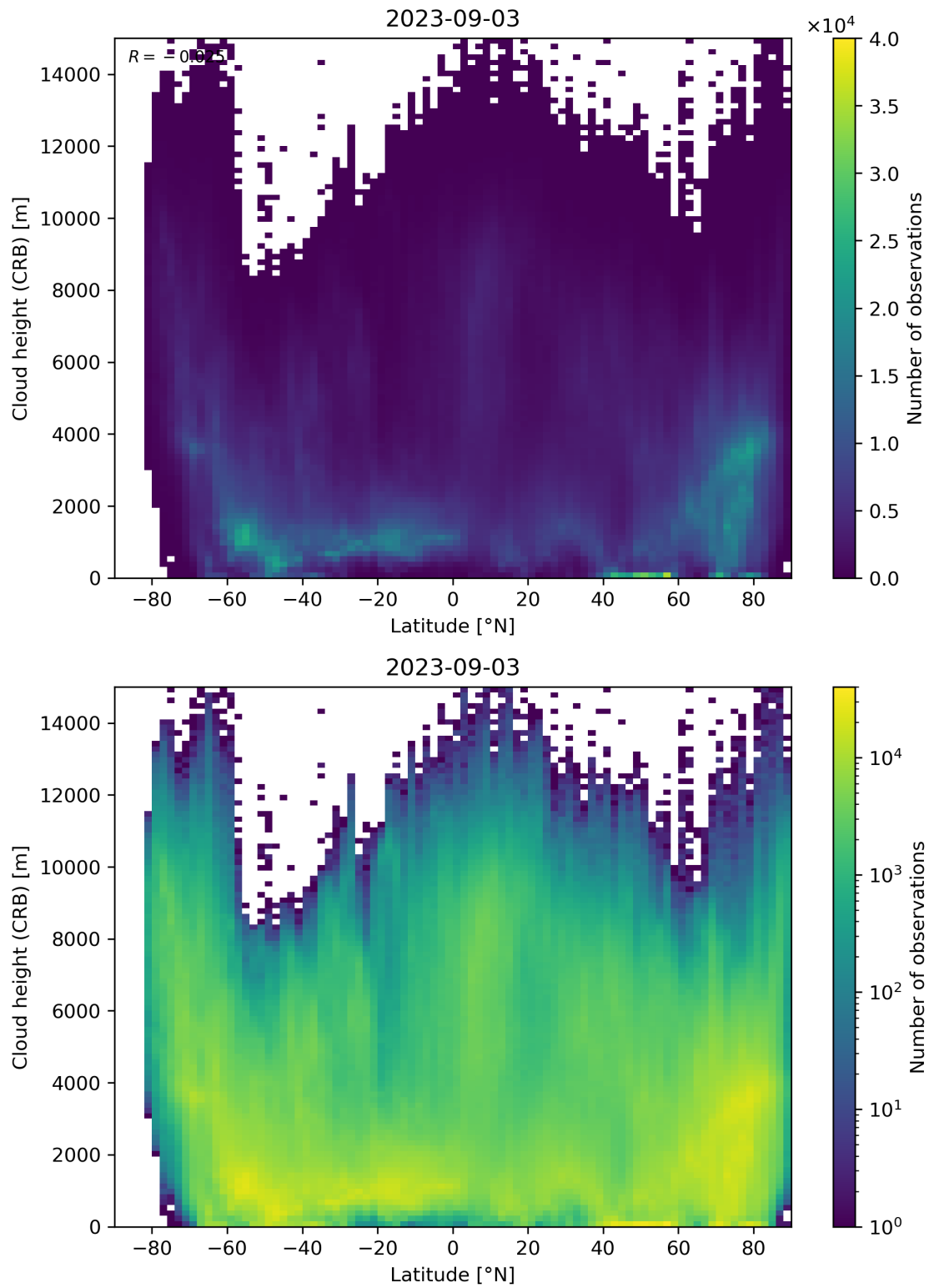
Figure 95: Scatter density plot of “Latitude” against “Cloud height (CRB)” for 2023-09-02 to 2023-09-04.
