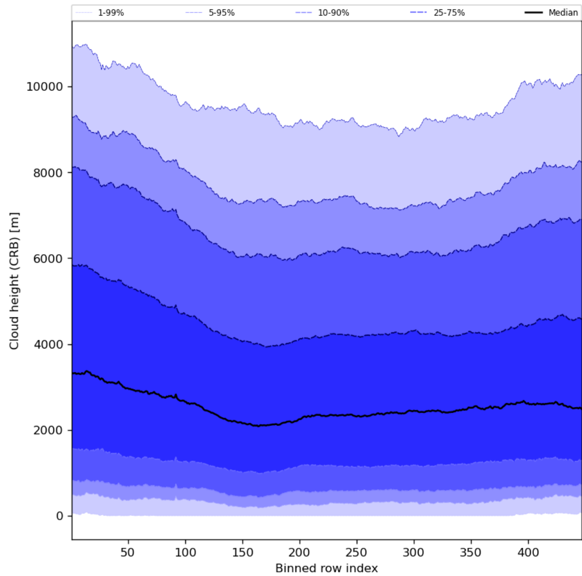
Figure 59: Along track statistics of “Cloud height (CRB)” for 2023-09-02 to 2023-09-04
