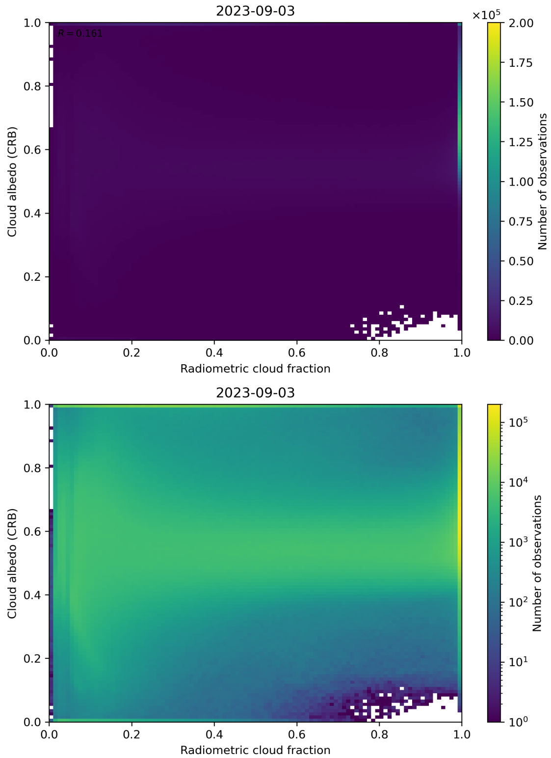
Figure 71: Scatter density plot of “Radiometric cloud fraction” against “Cloud albedo (CRB)” for 2023-09-02 to 2023-09-04.
