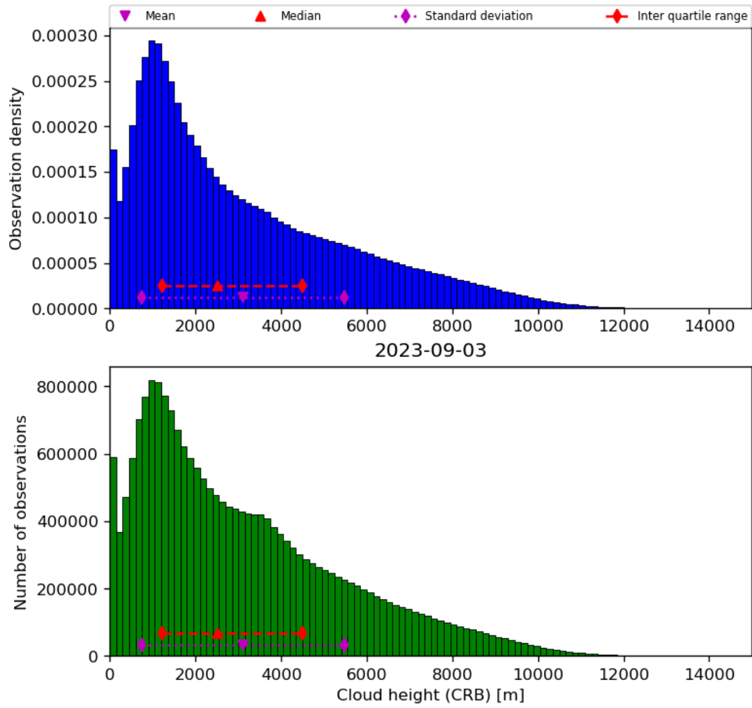
Figure 43: Histogram of “Cloud height (CRB)” for 2023-09-02 to 2023-09-04
