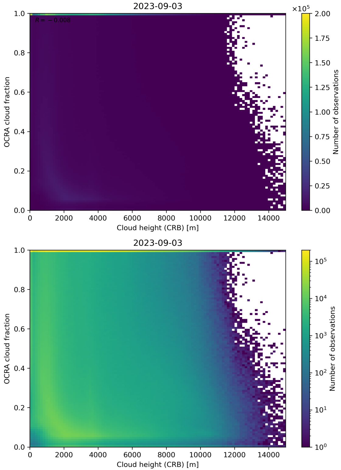
Figure 81: Scatter density plot of “Cloud height (CRB)” against “OCRA cloud fraction” for 2023-09-02 to 2023-09-04.
