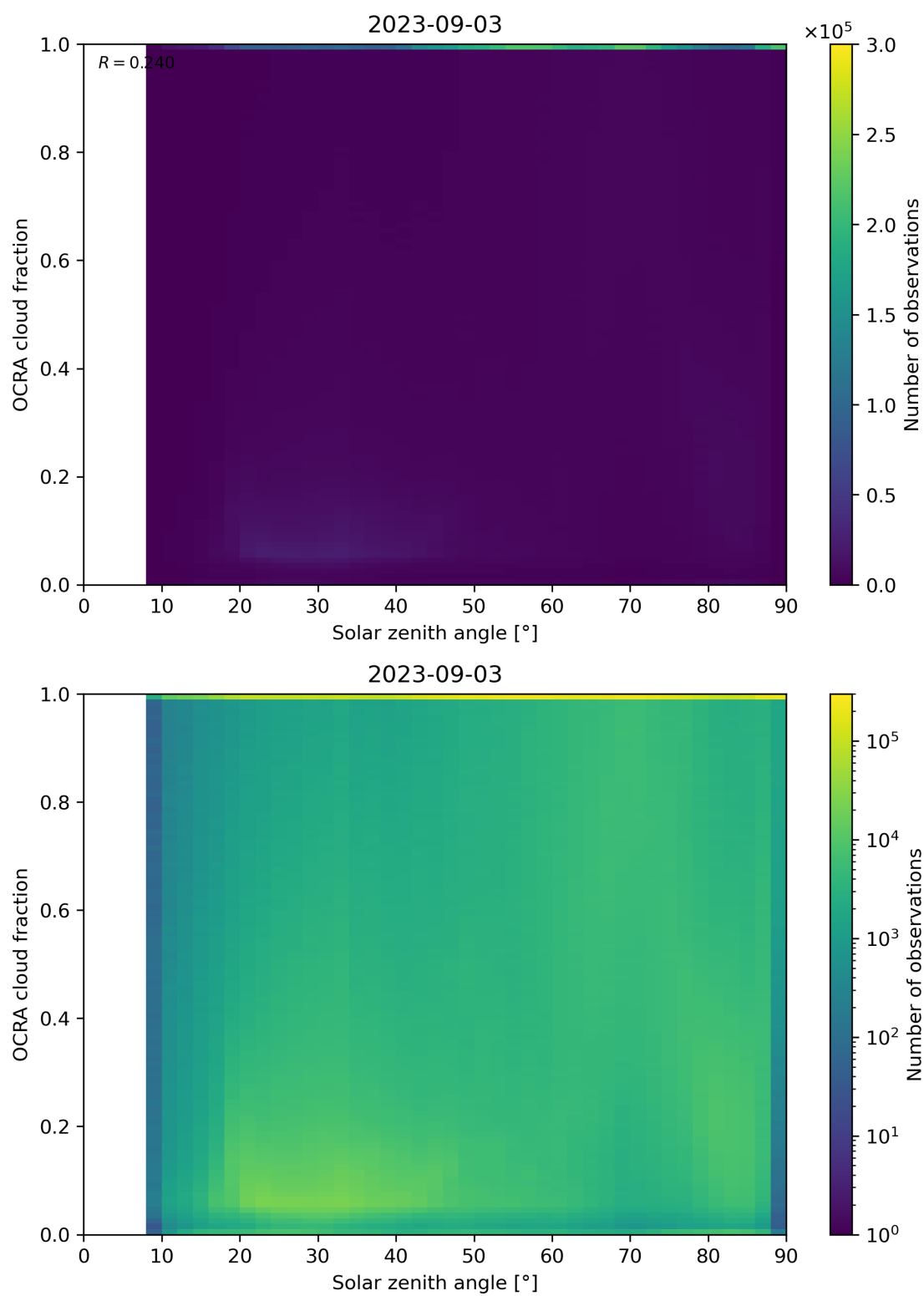
Figure 100: Scatter density plot of “Solar zenith angle” against “OCRA cloud fraction” for 2023-09-02 to 2023-09-04.
