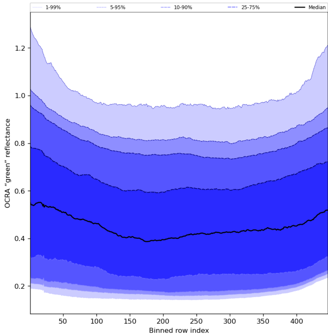
Figure 68: Along track statistics of “OCRA “green” reflectance” for 2023-09-02 to 2023-09-04
