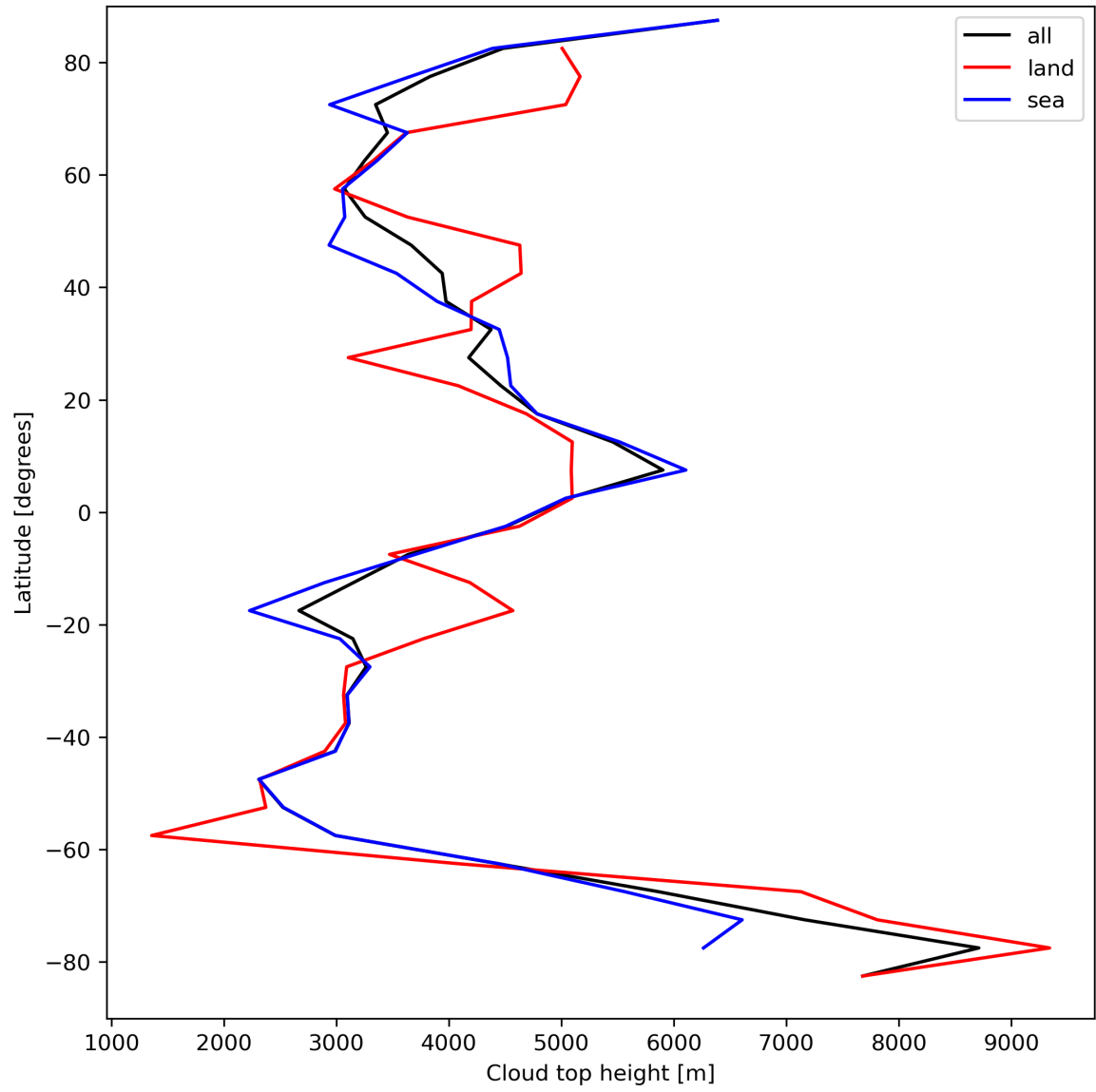
Figure 24: Zonal average of “Cloud top height” for 2023-09-02 to 2023-09-04.
