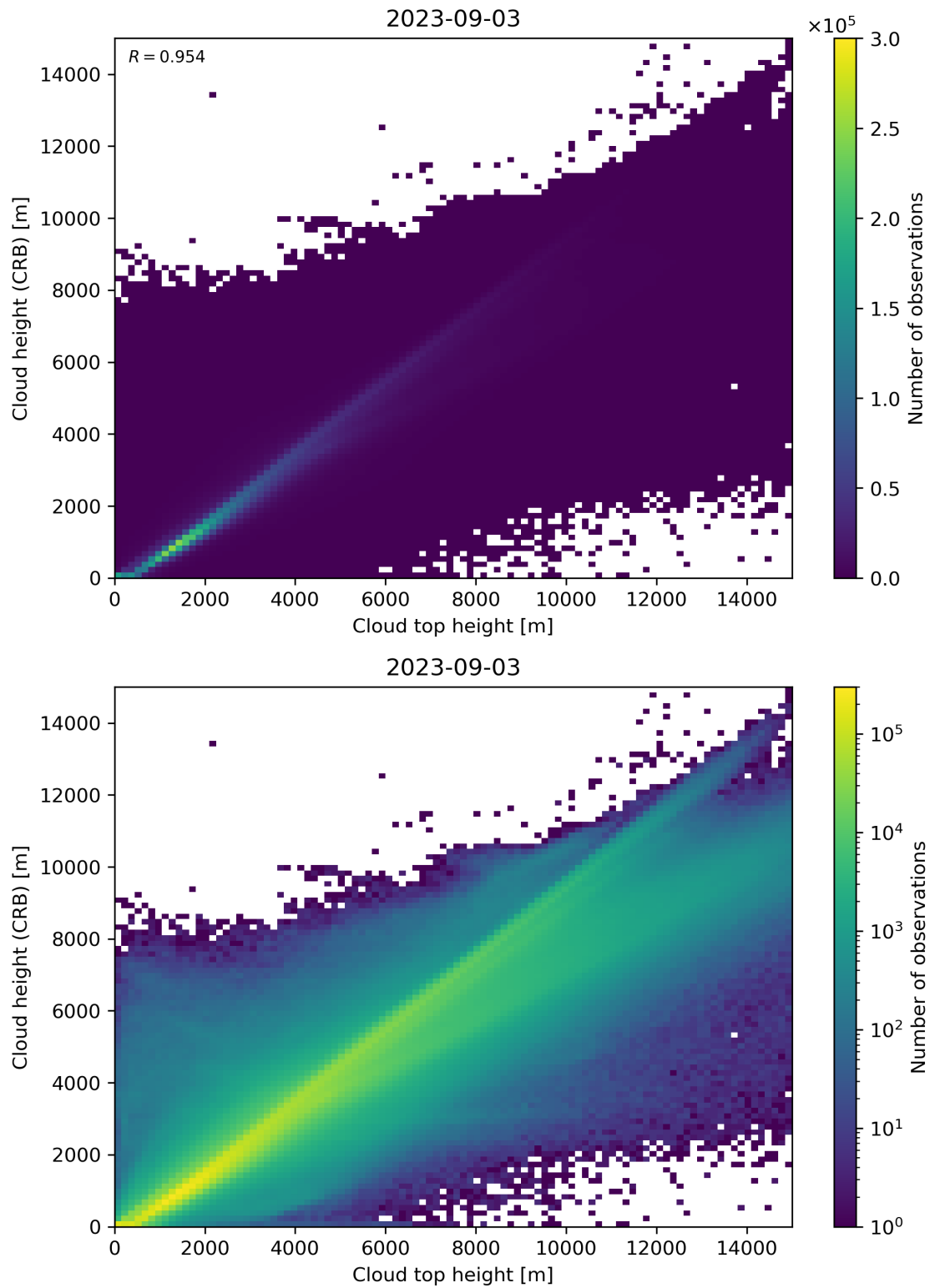
Figure 89: Scatter density plot of “Cloud top height” against “Cloud height (CRB)” for 2023-09-02 to 2023-09-04.
