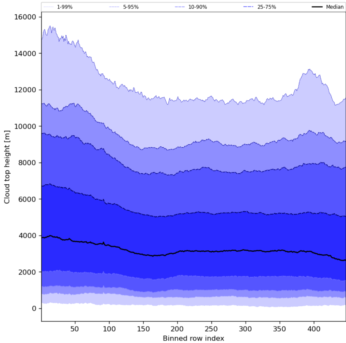
Figure 56: Along track statistics of “Cloud top height” for 2023-09-02 to 2023-09-04
