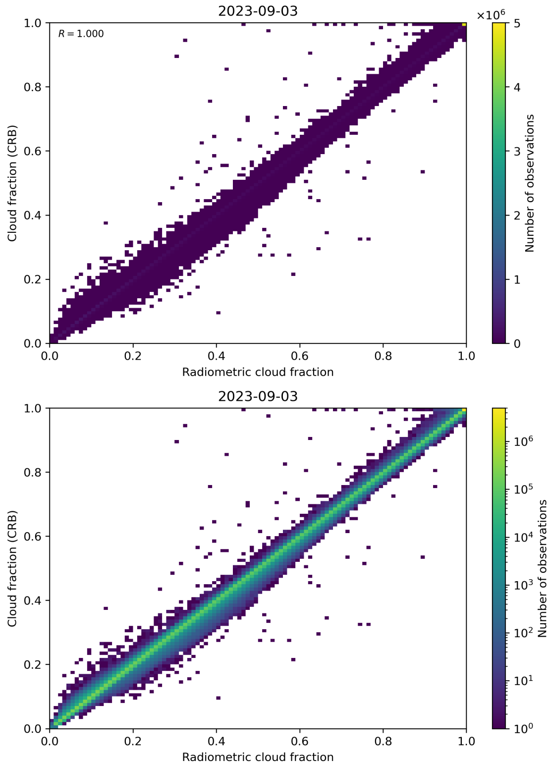
Figure 73: Scatter density plot of “Radiometric cloud fraction” against “Cloud fraction (CRB)” for 2023-09-02 to 2023-09-04.
