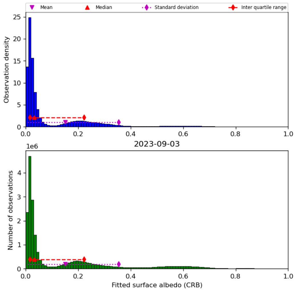
Figure 46: Histogram of “Fitted surface albedo (CRB)” for 2023-09-02 to 2023-09-04
