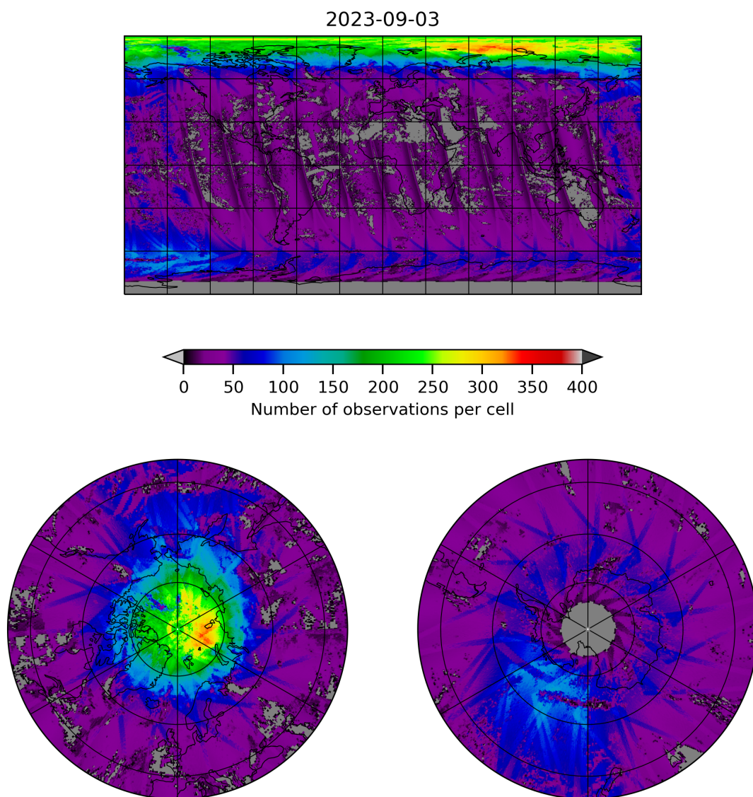
Figure 21: Map of the number of observations for 2023-09-02 to 2023-09-04
