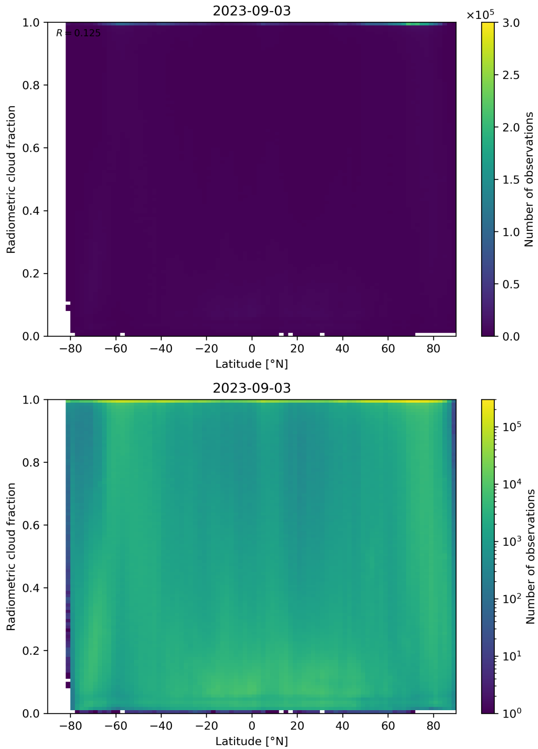
Figure 92: Scatter density plot of “Latitude” against “Radiometric cloud fraction” for 2023-09-02 to 2023-09-04.
