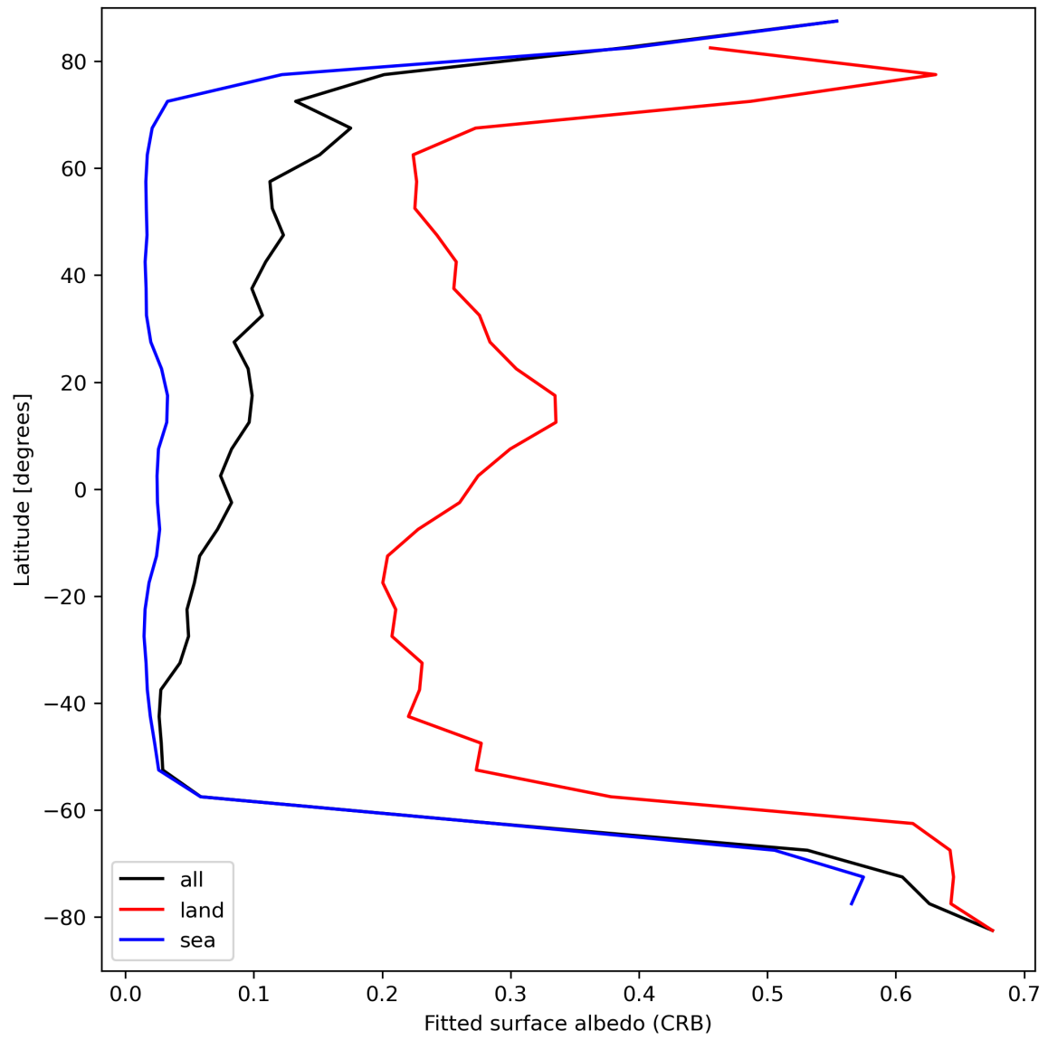
Figure 30: Zonal average of “Fitted surface albedo (CRB)” for 2023-09-02 to 2023-09-04.
