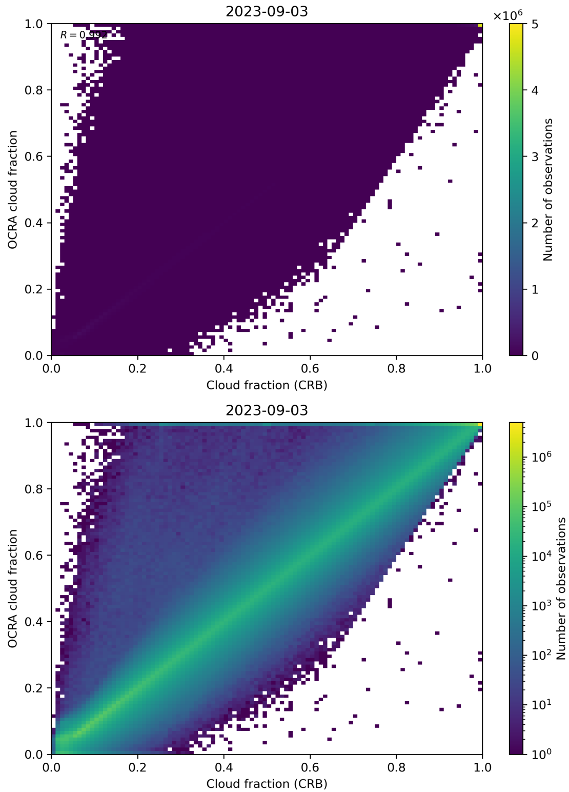
Figure 78: Scatter density plot of “Cloud fraction (CRB)” against “OCRA cloud fraction” for 2023-09-02 to 2023-09-04.
