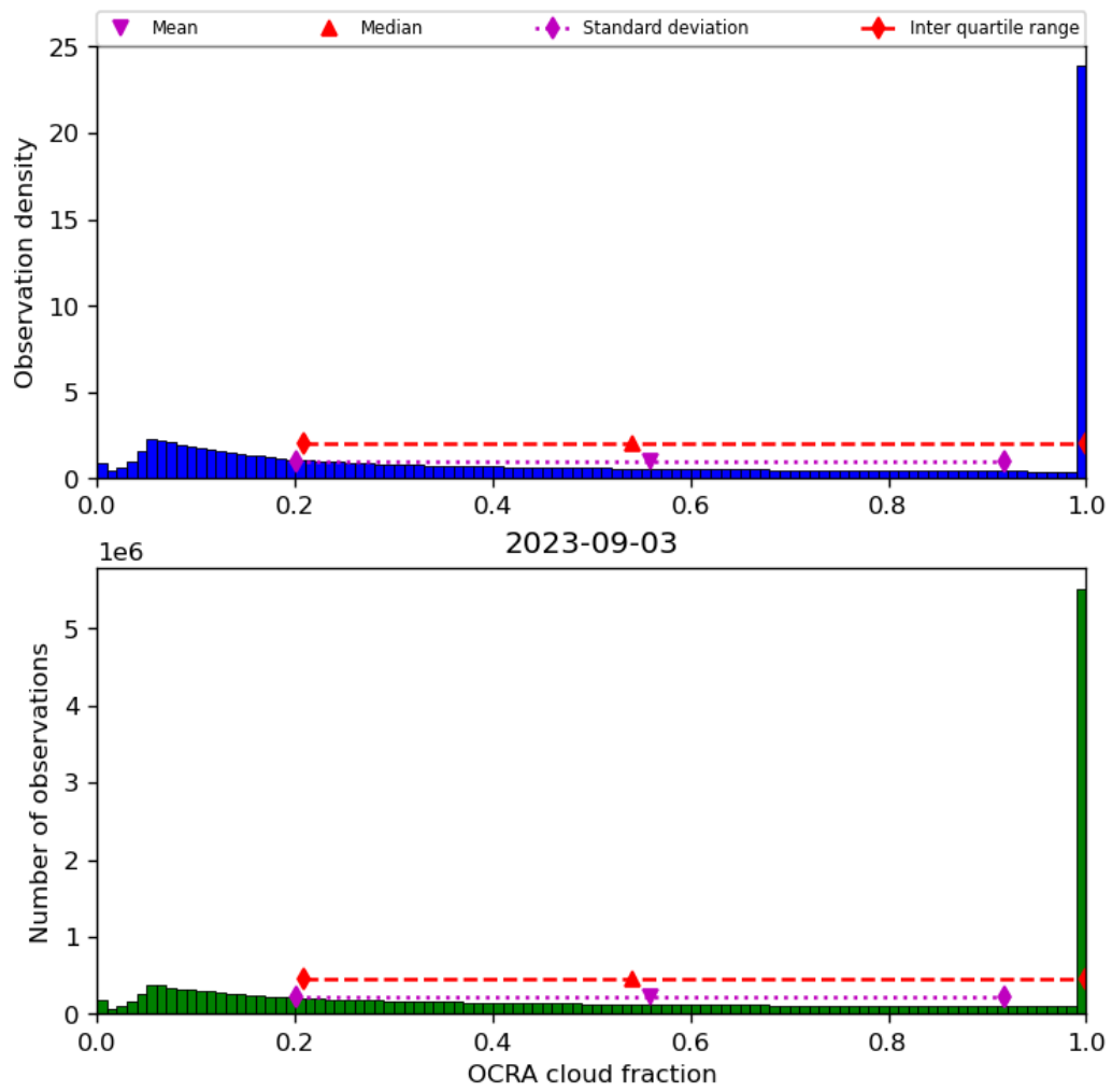
Figure 50: Histogram of “OCRA cloud fraction” for 2023-09-02 to 2023-09-04
