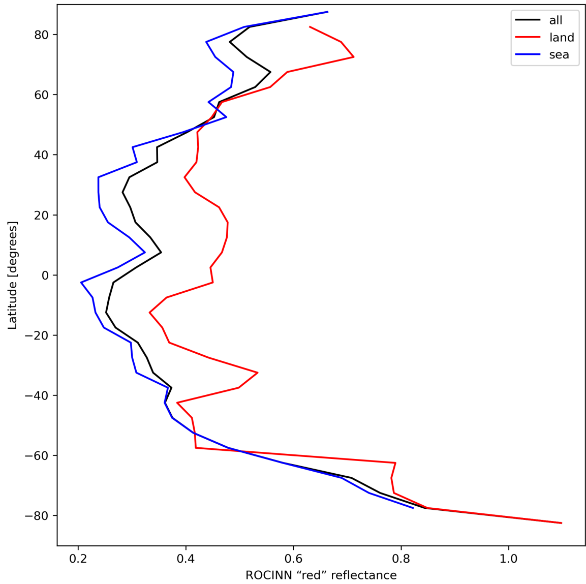
Figure 37: Zonal average of “ROCINN “red” reflectance” for 2023-09-02 to 2023-09-04.
