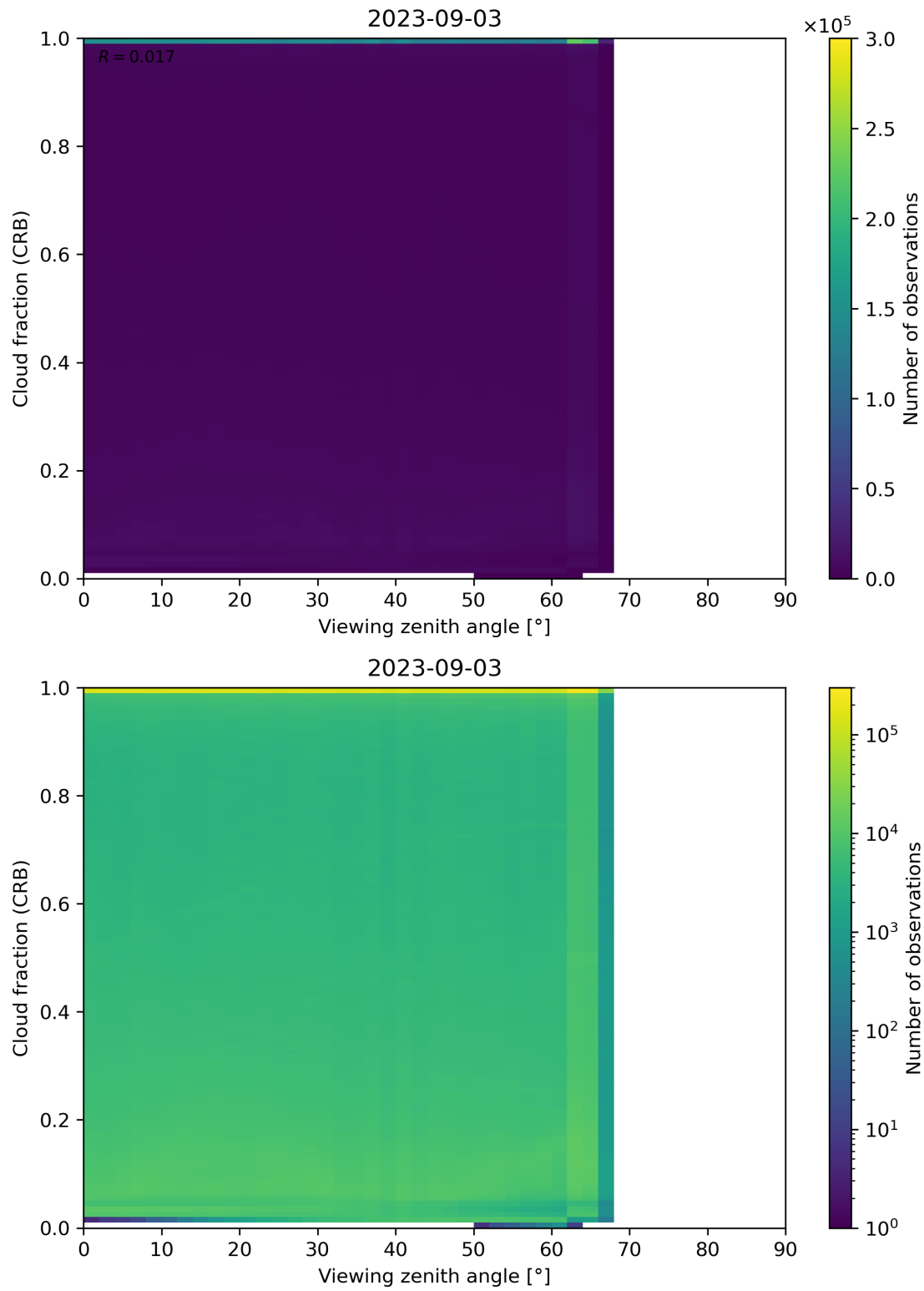
Figure 109: Scatter density plot of “Viewing zenith angle” against “Cloud fraction (CRB)” for 2023-09-02 to 2023-09-04.
