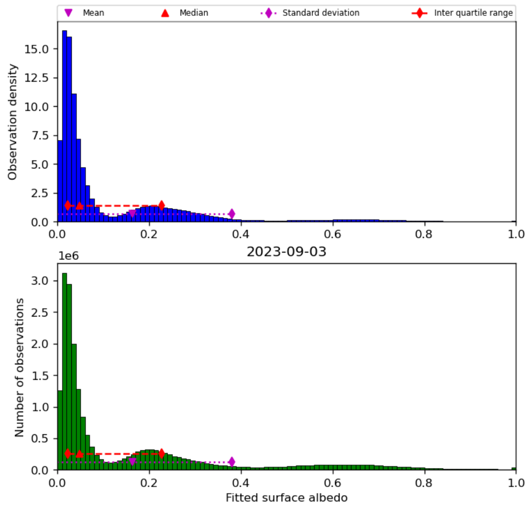
Figure 45: Histogram of “Fitted surface albedo” for 2023-09-02 to 2023-09-04
