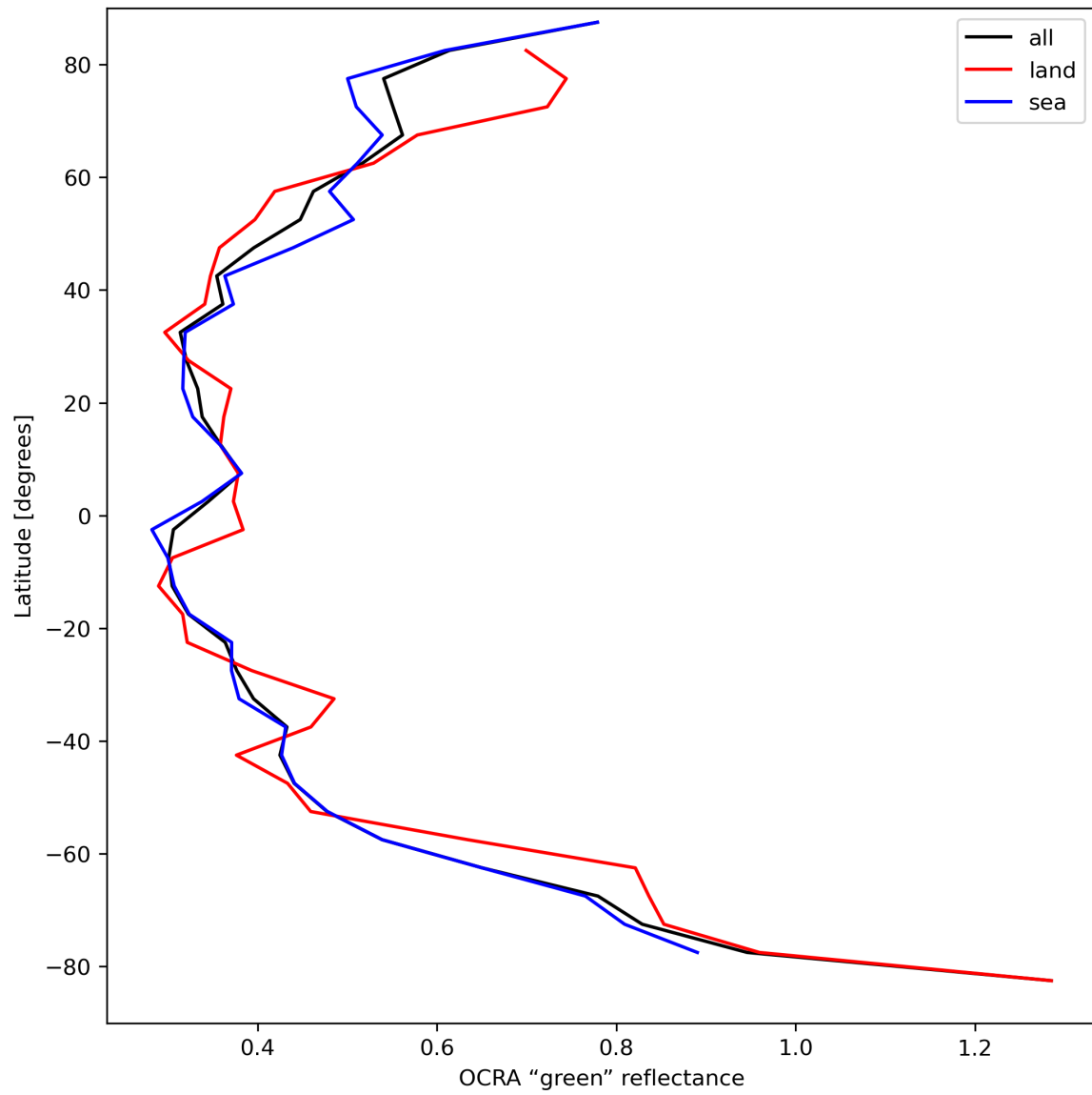
Figure 36: Zonal average of “OCRA “green” reflectance” for 2023-09-02 to 2023-09-04.
