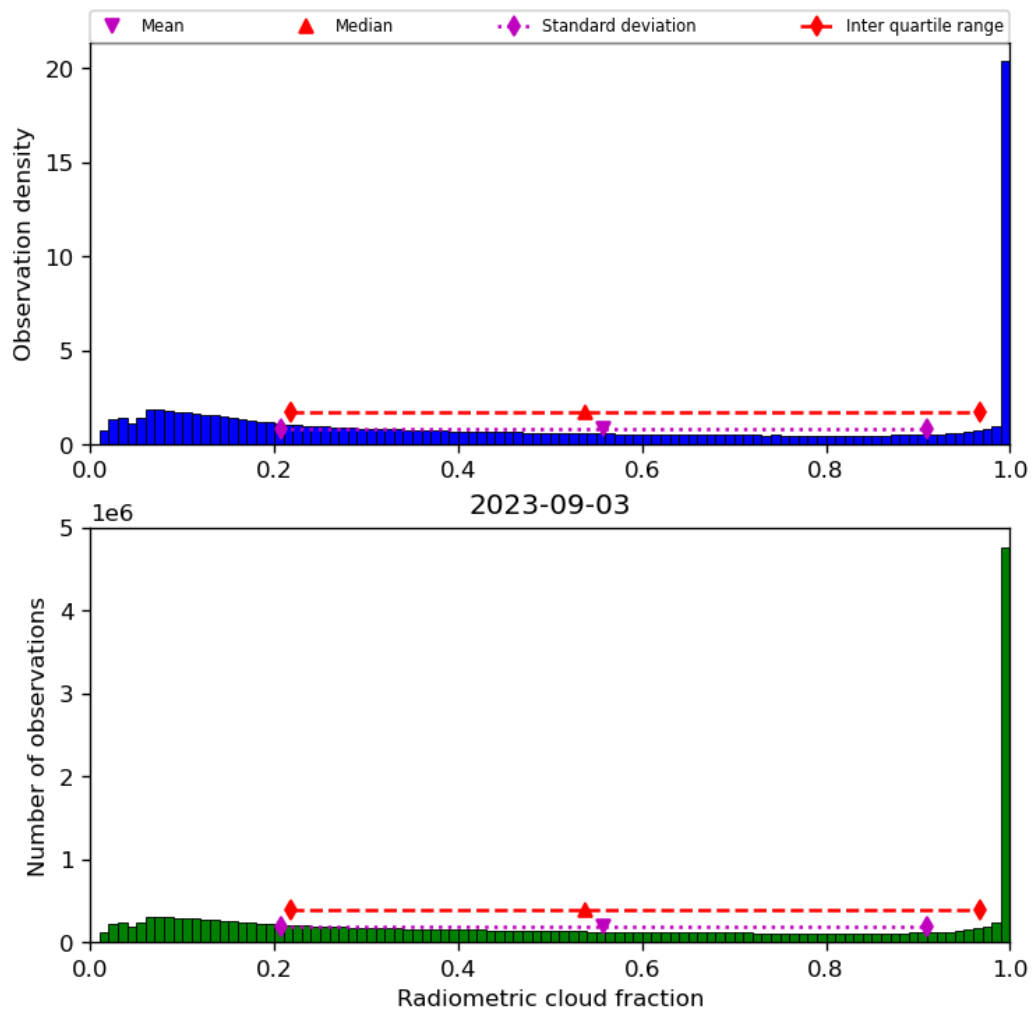
Figure 39: Histogram of “Radiometric cloud fraction” for 2023-09-02 to 2023-09-04
