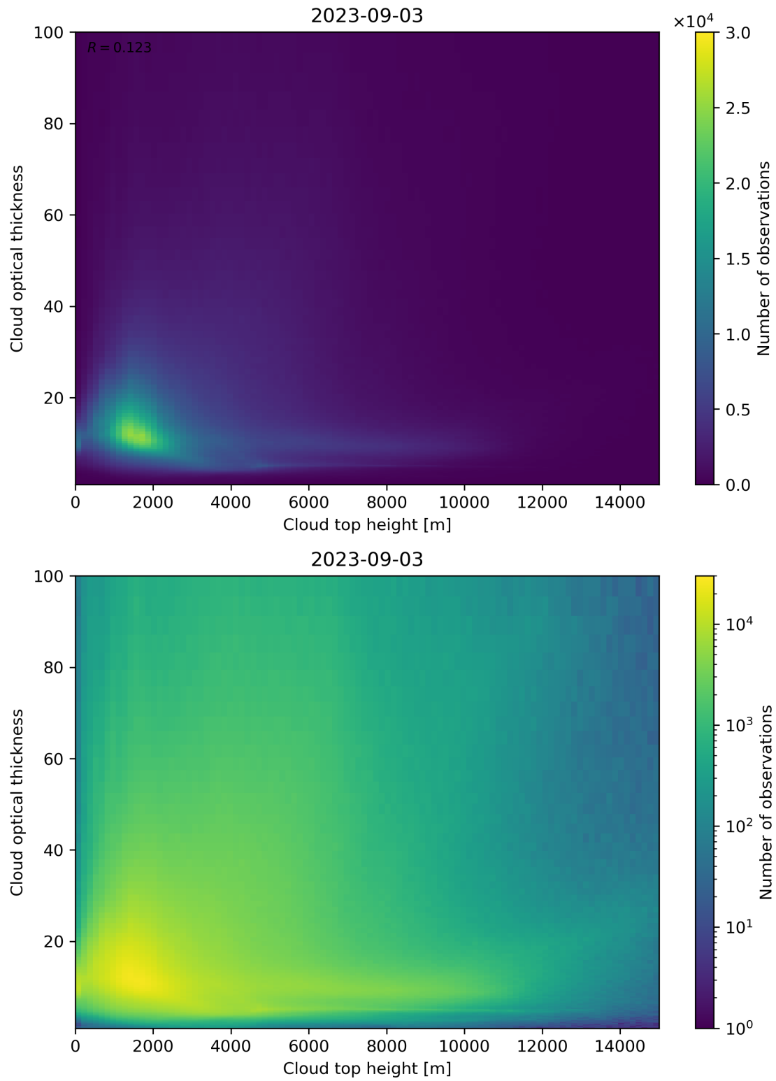
Figure 90: Scatter density plot of “Cloud top height” against “Cloud optical thickness” for 2023-09-02 to 2023-09-04.
