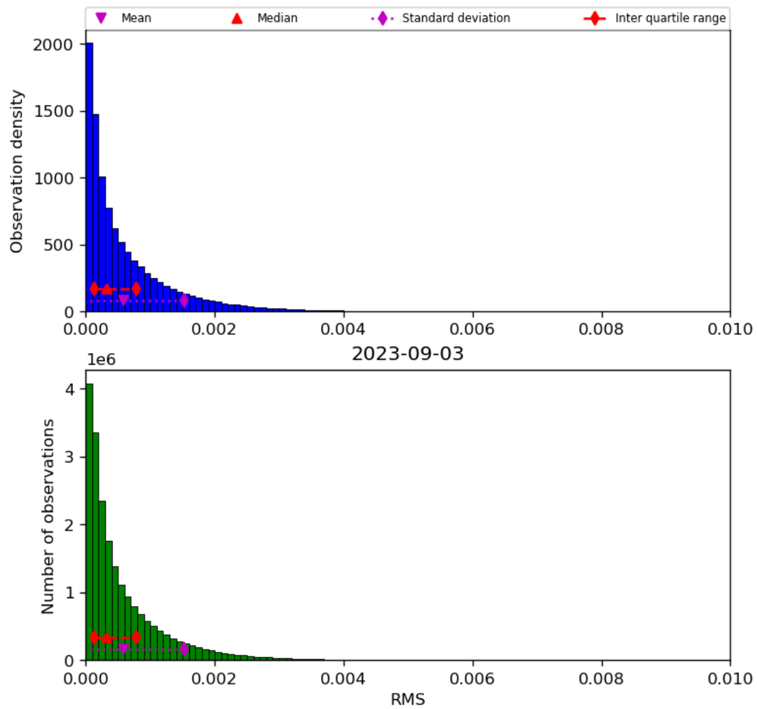
Figure 47: Histogram of “RMS” for 2023-09-02 to 2023-09-04
