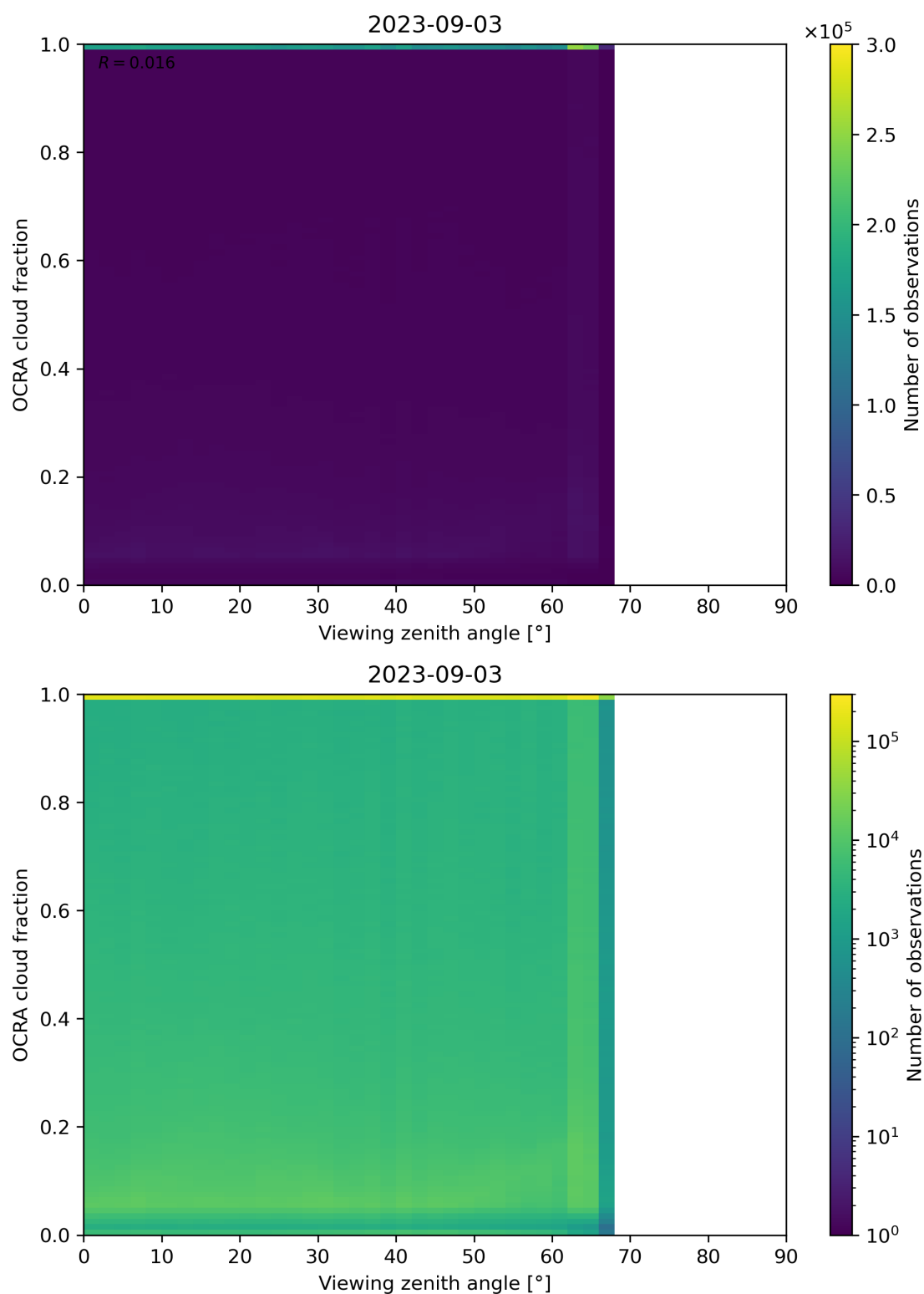
Figure 108: Scatter density plot of “Viewing zenith angle” against “OCRA cloud fraction” for 2023-09-02 to 2023-09-04.
