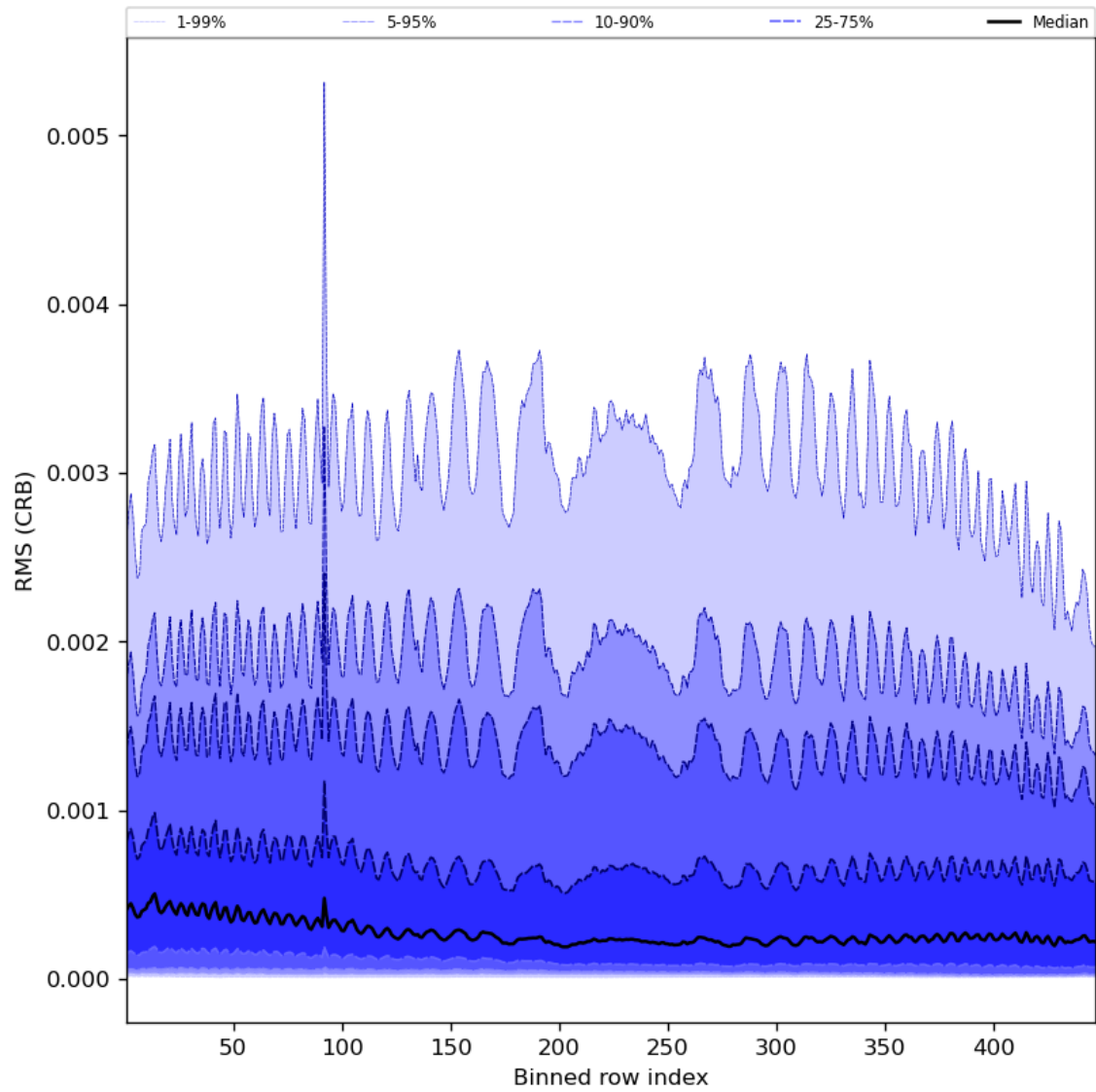
Figure 64: Along track statistics of “RMS (CRB)” for 2023-09-02 to 2023-09-04
