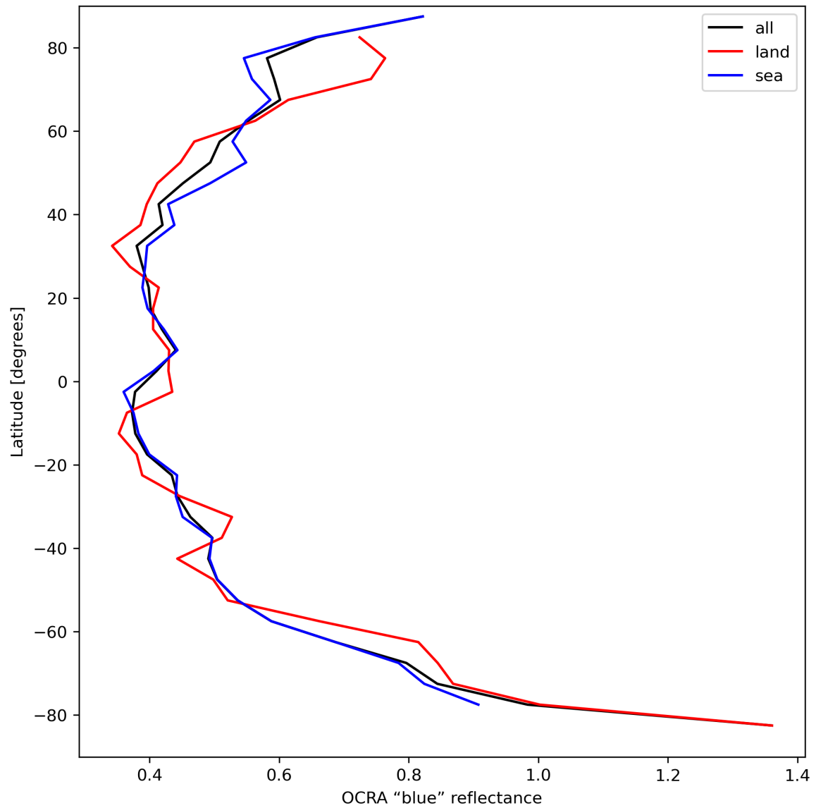
Figure 35: Zonal average of “OCRA “blue” reflectance” for 2023-09-02 to 2023-09-04.
