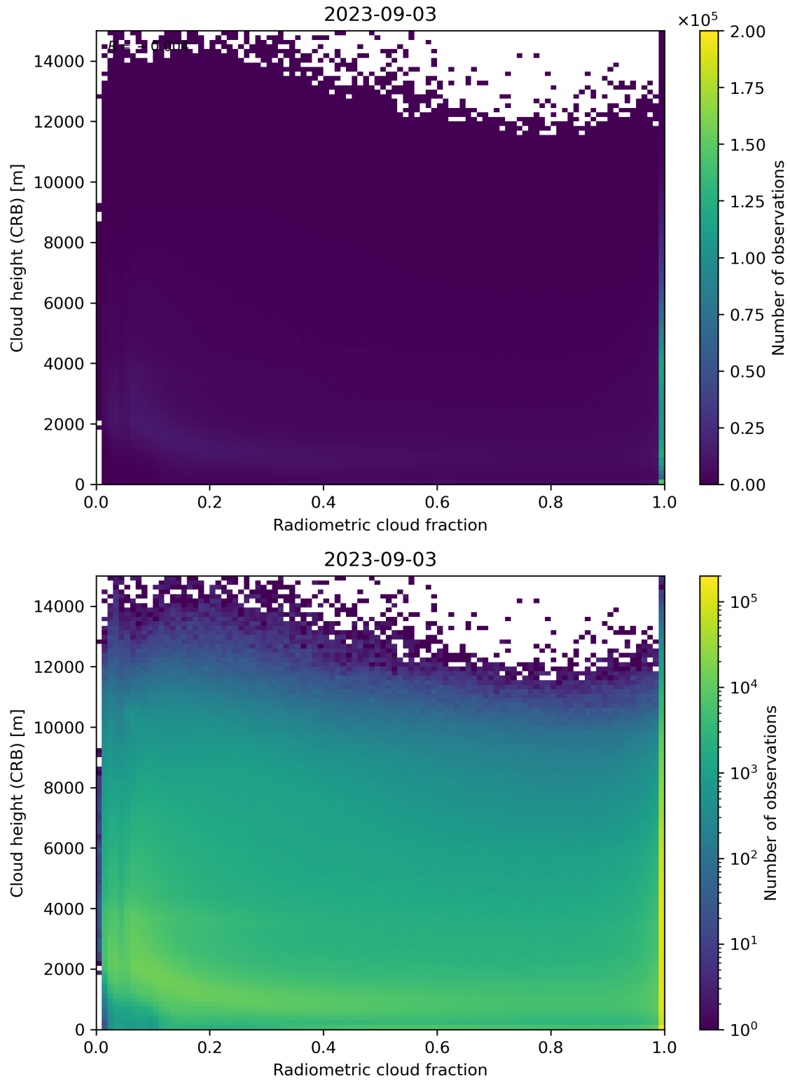
Figure 74: Scatter density plot of “Radiometric cloud fraction” against “Cloud height (CRB)” for 2023-09-02 to 2023-09-04.
