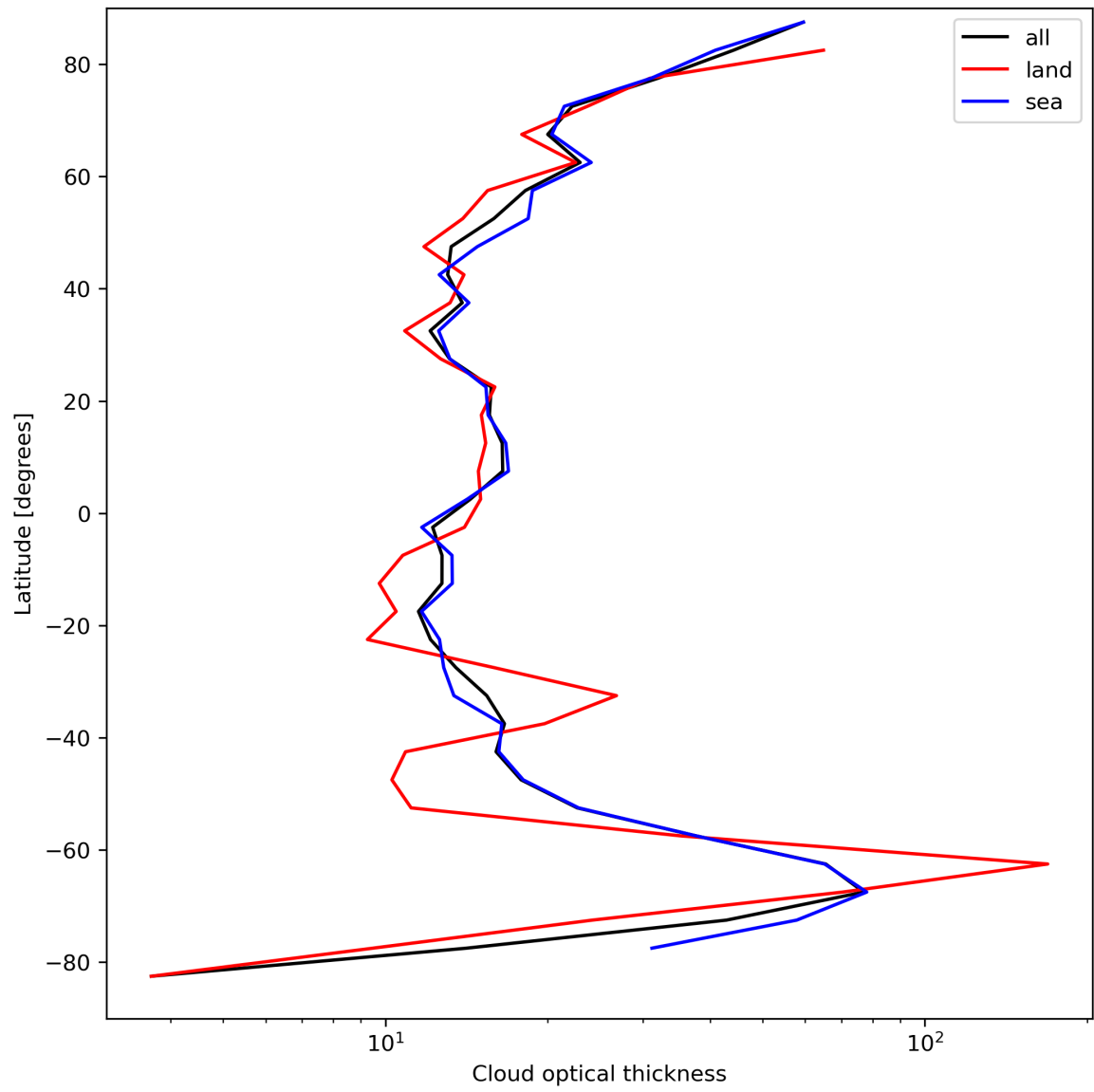
Figure 25: Zonal average of “Cloud optical thickness” for 2023-09-02 to 2023-09-04.
