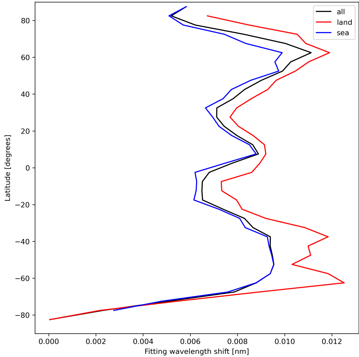
Figure 33: Zonal average of “Fitting wavelength shift” for 2023-09-02 to 2023-09-04.
