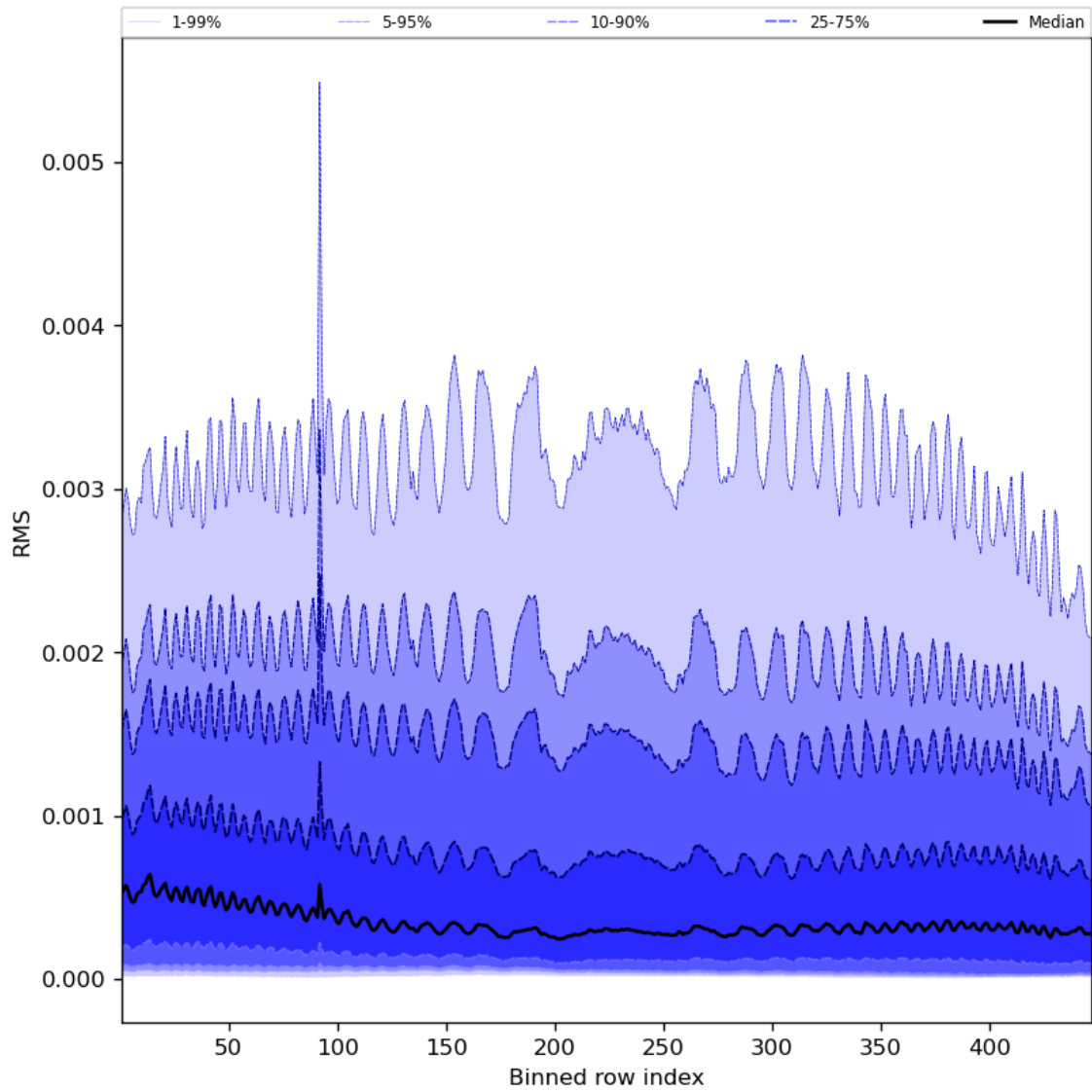
Figure 63: Along track statistics of “RMS” for 2023-09-02 to 2023-09-04
