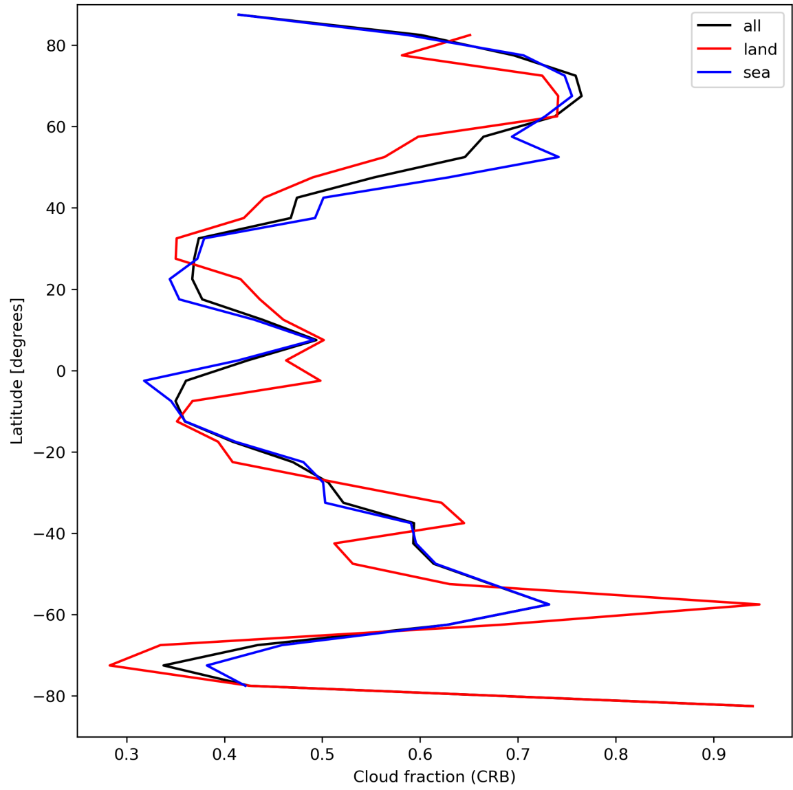
Figure 26: Zonal average of “Cloud fraction (CRB)” for 2023-09-02 to 2023-09-04.
