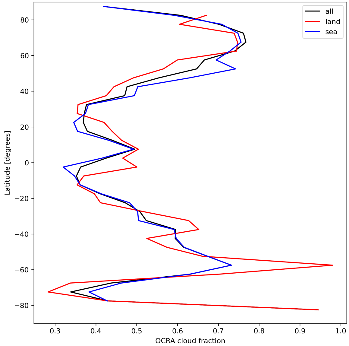
Figure 34: Zonal average of “OCRA cloud fraction” for 2023-09-02 to 2023-09-04.
