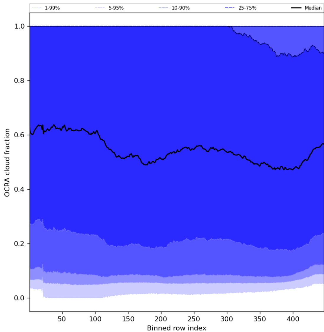
Figure 66: Along track statistics of “OCRA cloud fraction” for 2023-09-02 to 2023-09-04
