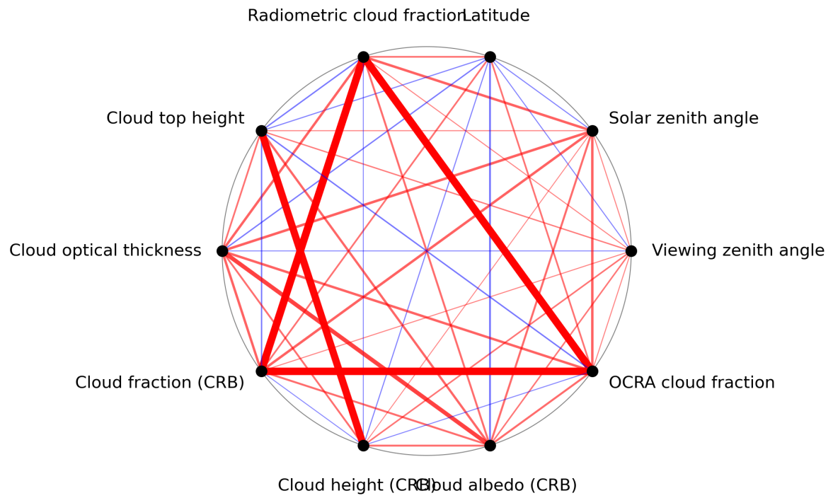
Figure 1: Map of correlation graph for 2023-09-02 to 2023-09-04.
