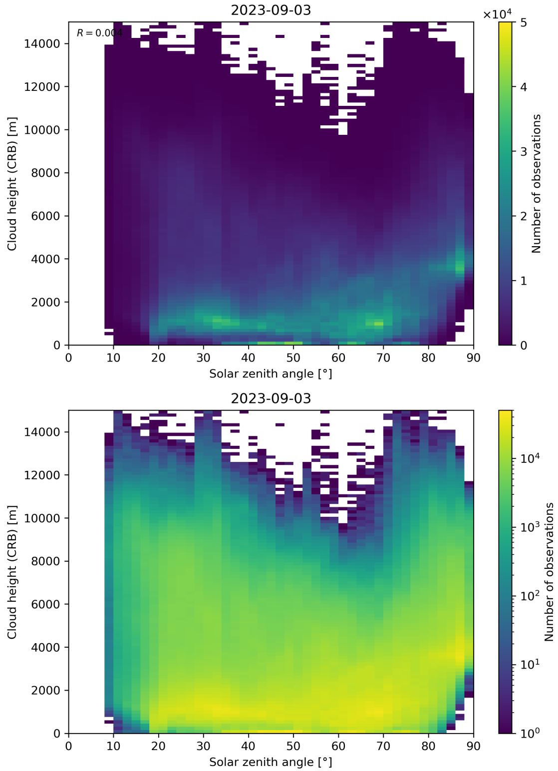
Figure 102: Scatter density plot of “Solar zenith angle” against “Cloud height (CRB)” for 2023-09-02 to 2023-09-04.
