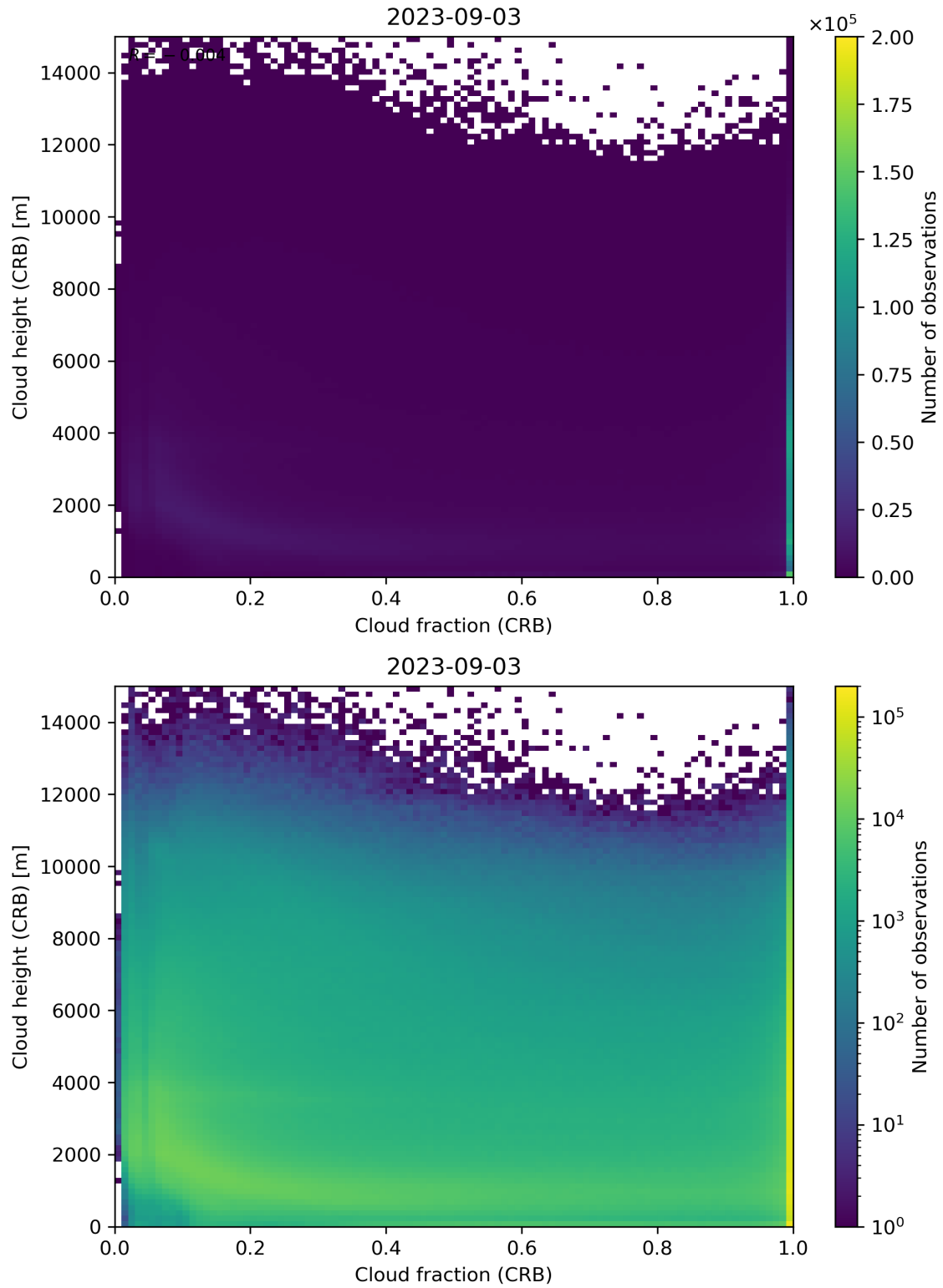
Figure 79: Scatter density plot of “Cloud fraction (CRB)” against “Cloud height (CRB)” for 2023-09-02 to 2023-09-04.
