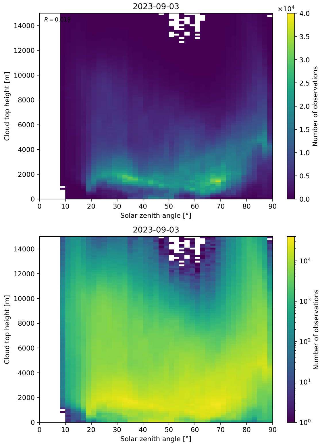
Figure 104: Scatter density plot of “Solar zenith angle” against “Cloud top height” for 2023-09-02 to 2023-09-04.
