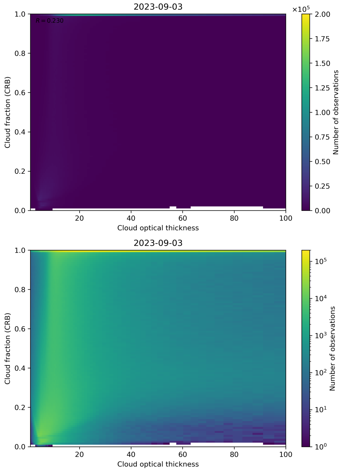
Figure 84: Scatter density plot of “Cloud optical thickness” against “Cloud fraction (CRB)” for 2023-09-02 to 2023-09-04.
