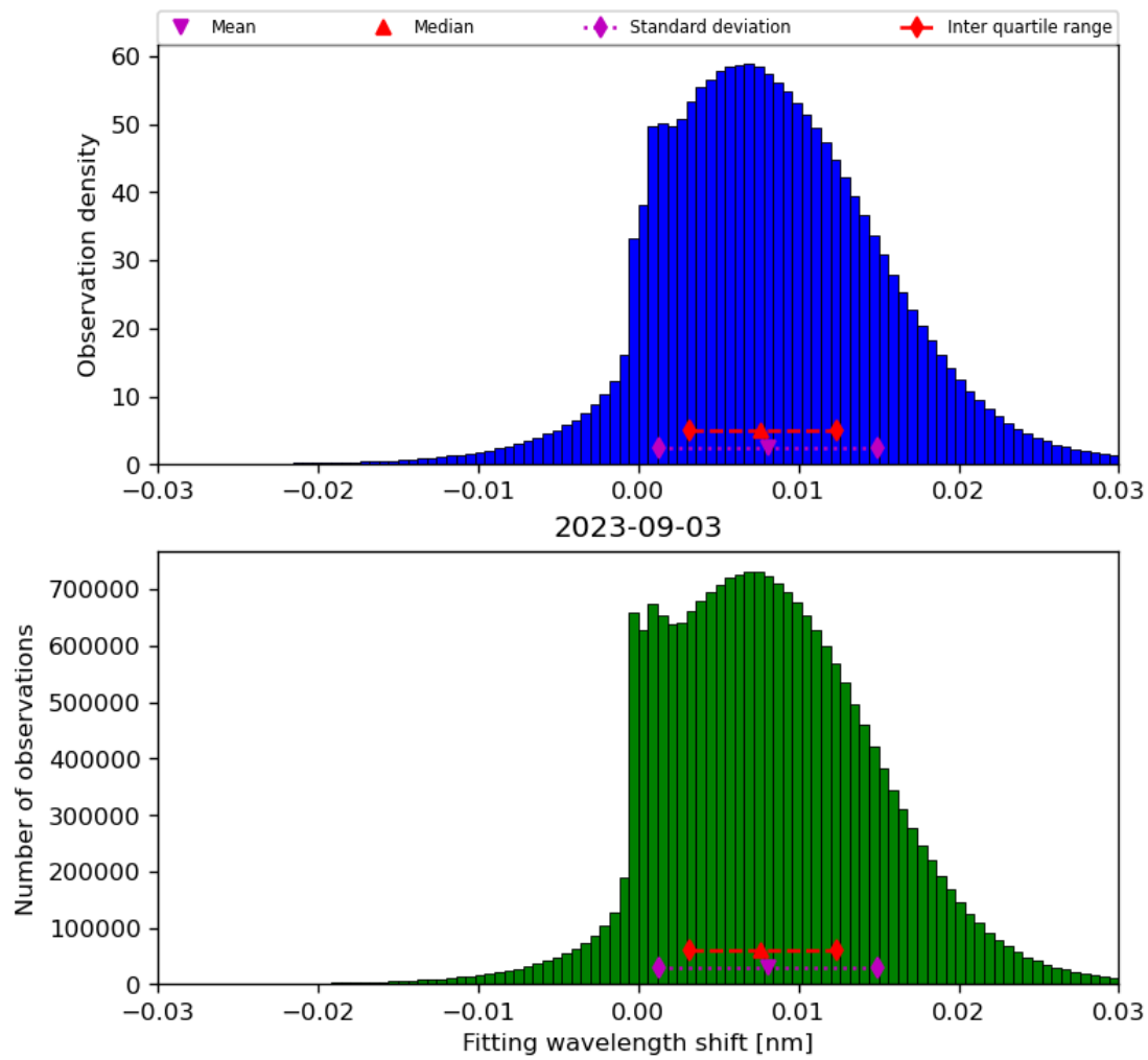
Figure 49: Histogram of “Fitting wavelength shift” for 2023-09-02 to 2023-09-04
