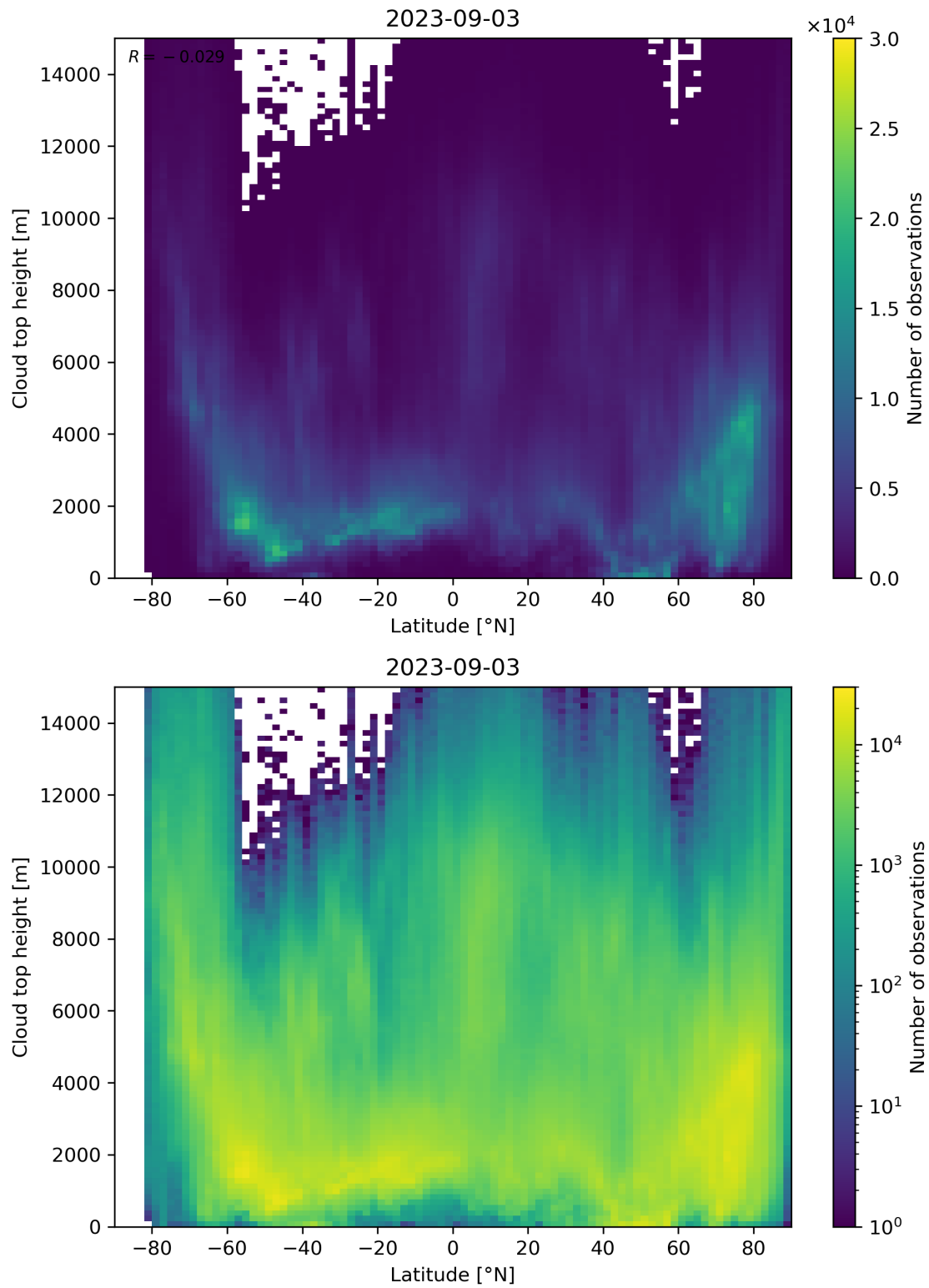
Figure 97: Scatter density plot of “Latitude” against “Cloud top height” for 2023-09-02 to 2023-09-04.
