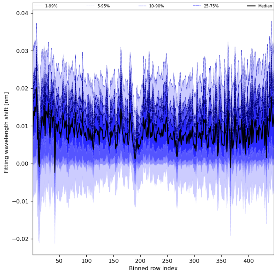
Figure 65: Along track statistics of “Fitting wavelength shift” for 2023-09-02 to 2023-09-04
