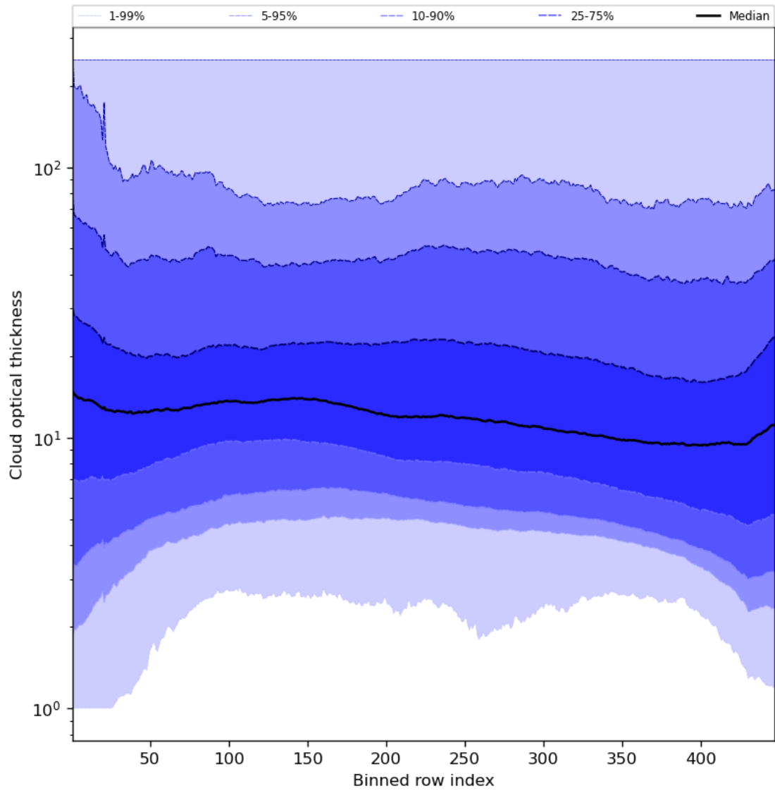
Figure 57: Along track statistics of “Cloud optical thickness” for 2023-09-02 to 2023-09-04
