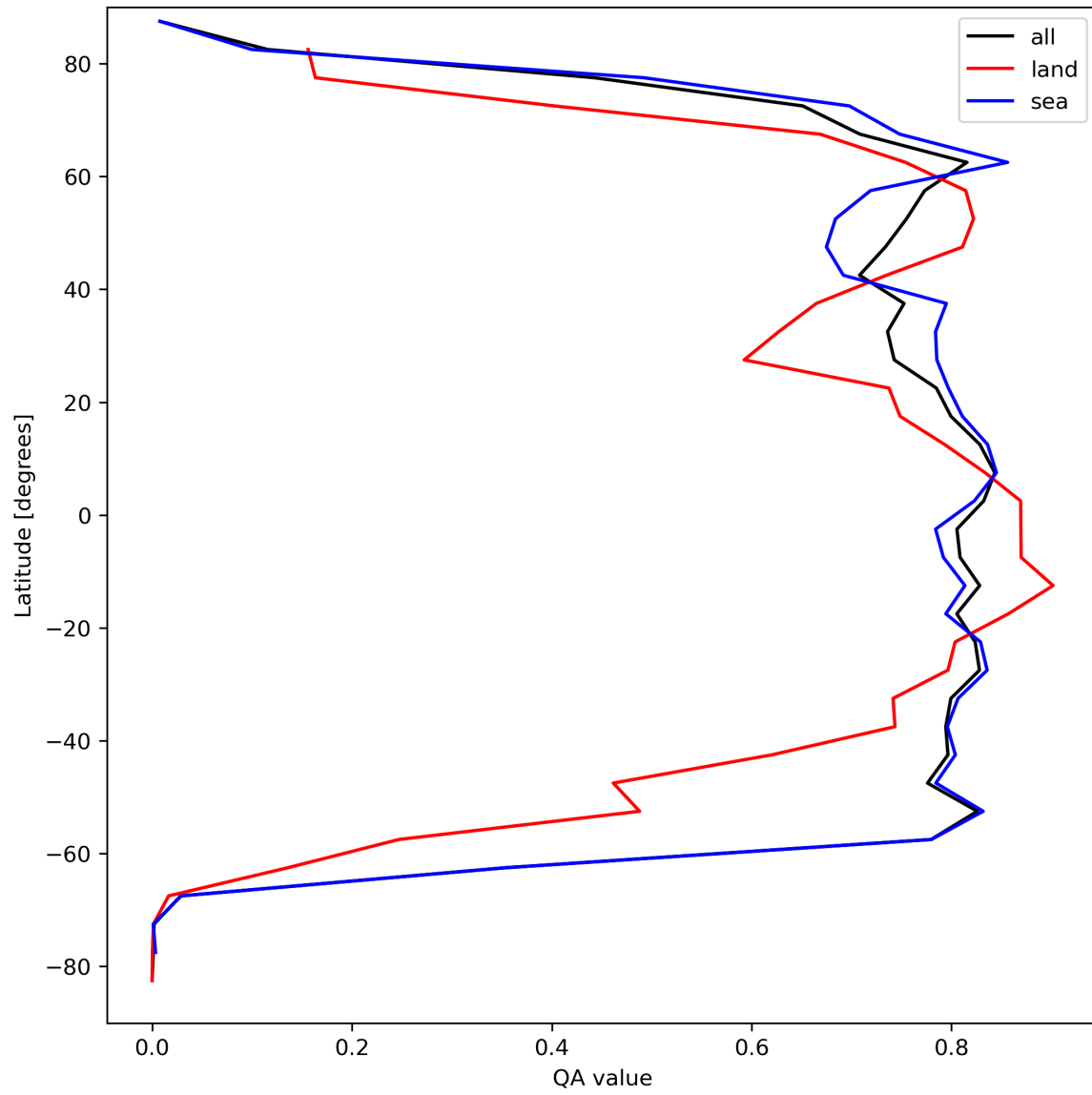
Figure 22: Zonal average of “QA value” for 2023-09-02 to 2023-09-04.
