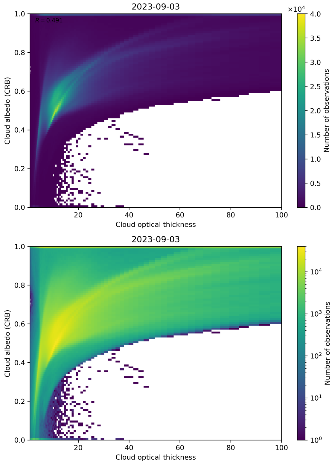
Figure 82: Scatter density plot of “Cloud optical thickness” against “Cloud albedo (CRB)” for 2023-09-02 to 2023-09-04.
