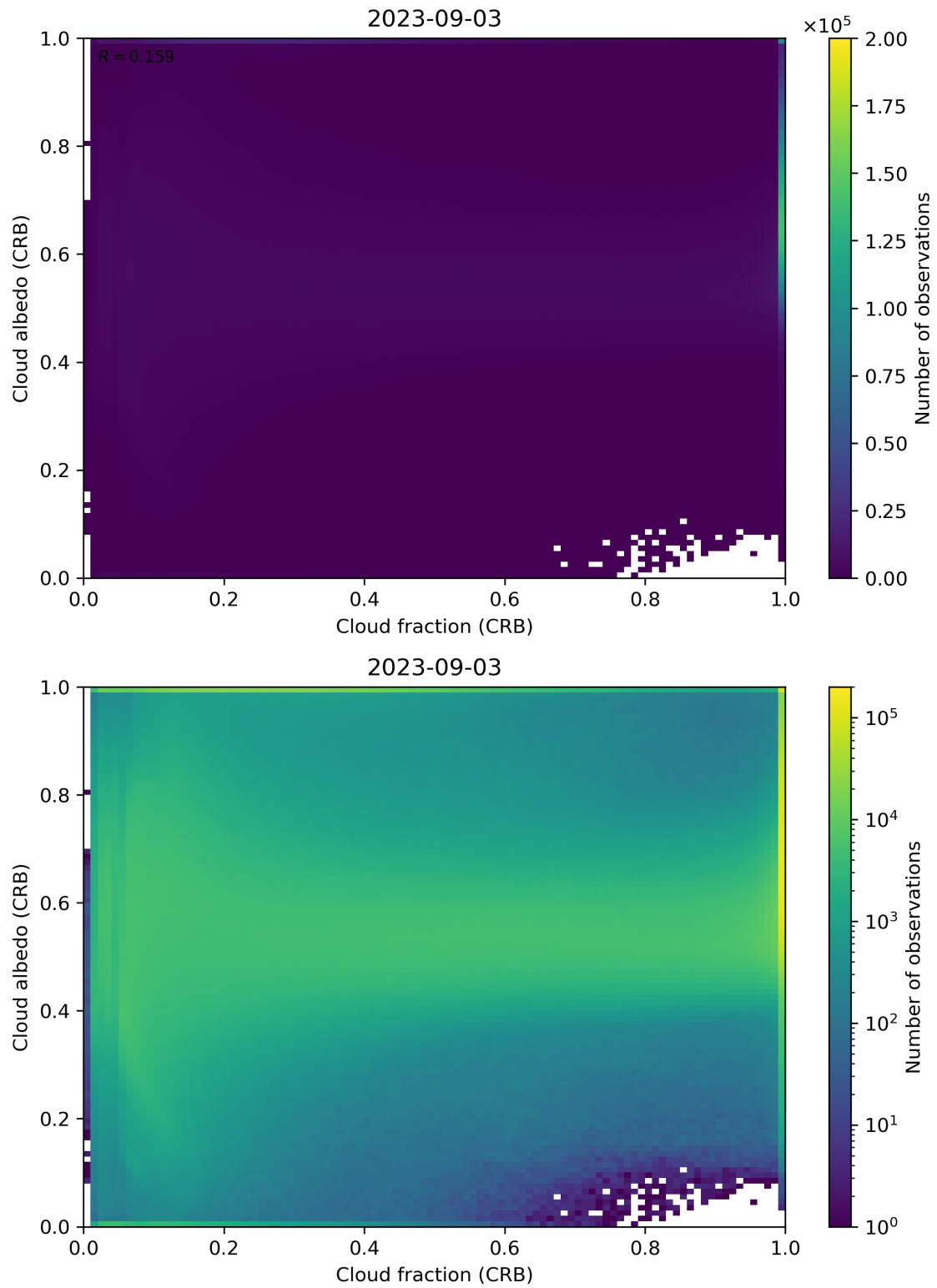
Figure 77: Scatter density plot of “Cloud fraction (CRB)” against “Cloud albedo (CRB)” for 2023-09-02 to 2023-09-04.
