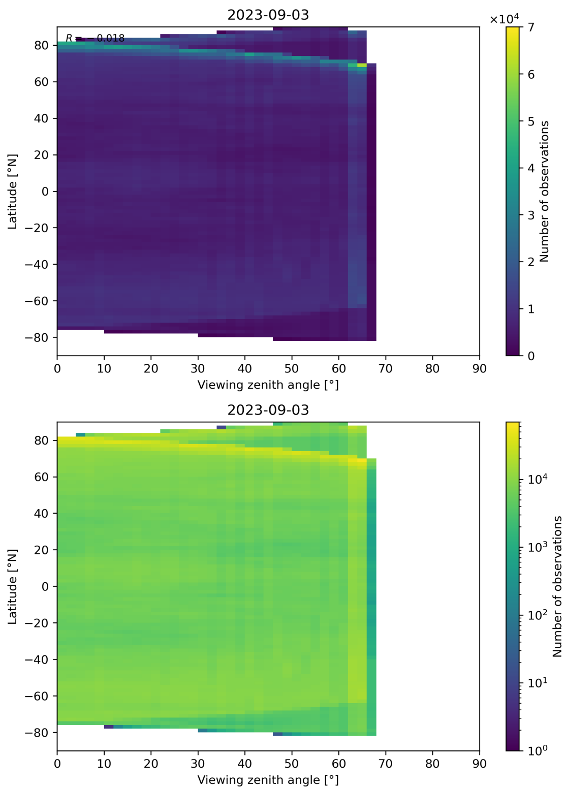
Figure 113: Scatter density plot of “Viewing zenith angle” against “Latitude” for 2023-09-02 to 2023-09-04.
