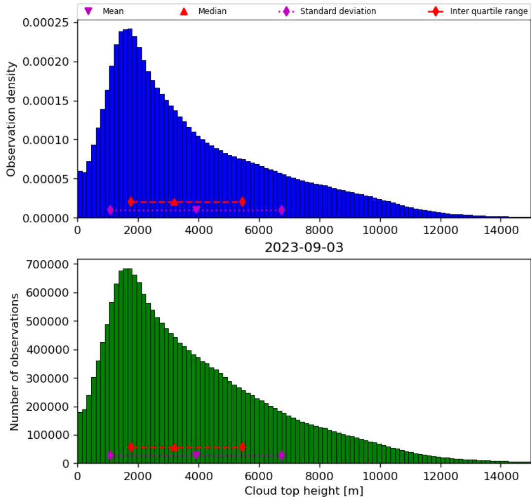
Figure 40: Histogram of “Cloud top height” for 2023-09-02 to 2023-09-04
