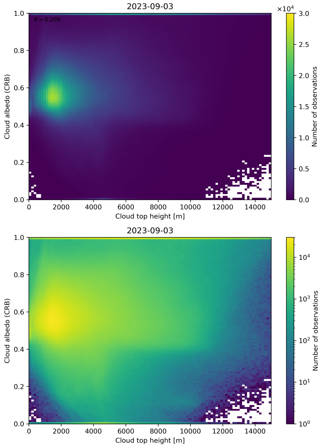
Figure 86: Scatter density plot of “Cloud top height” against “Cloud albedo (CRB)” for 2023-09-02 to 2023-09-04.
