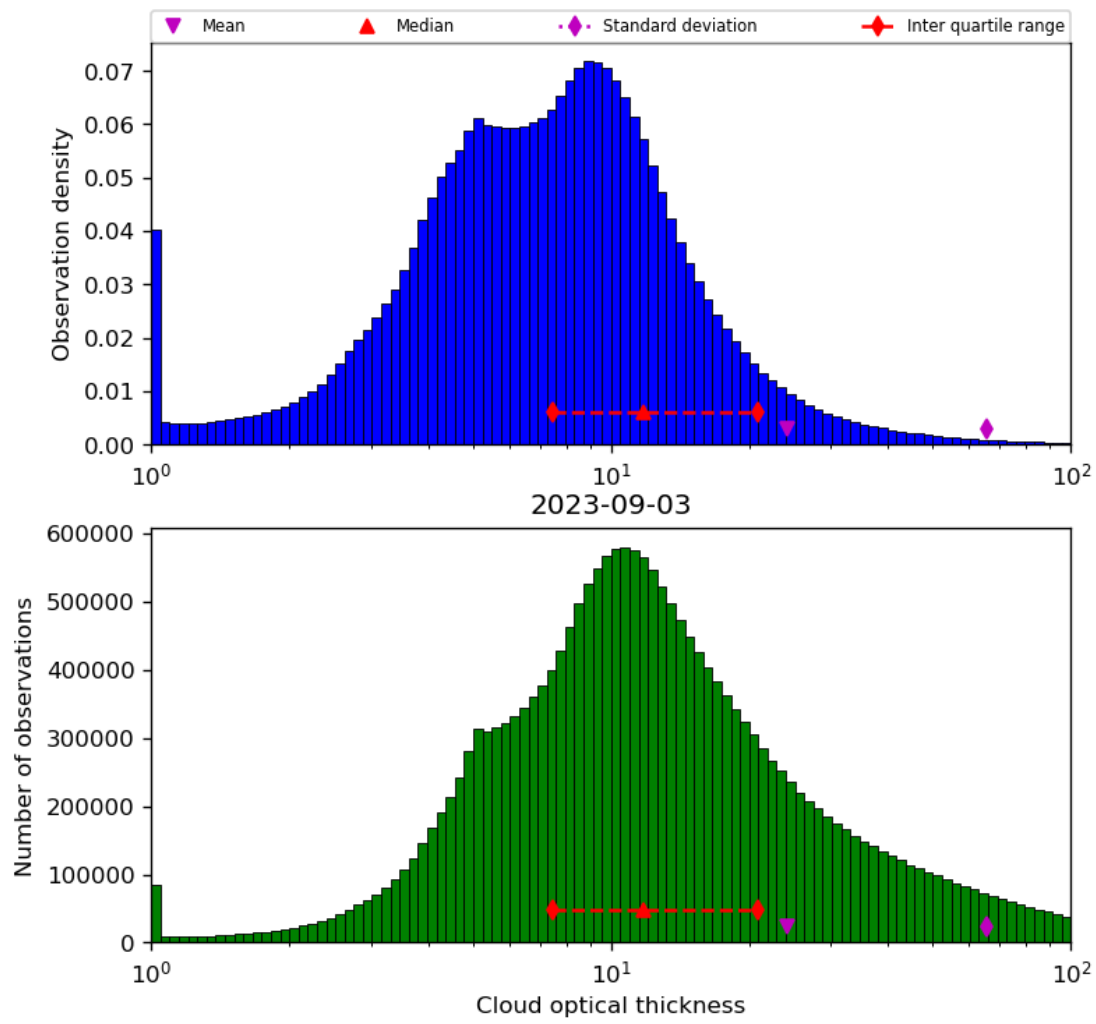
Figure 41: Histogram of “Cloud optical thickness” for 2023-09-02 to 2023-09-04
