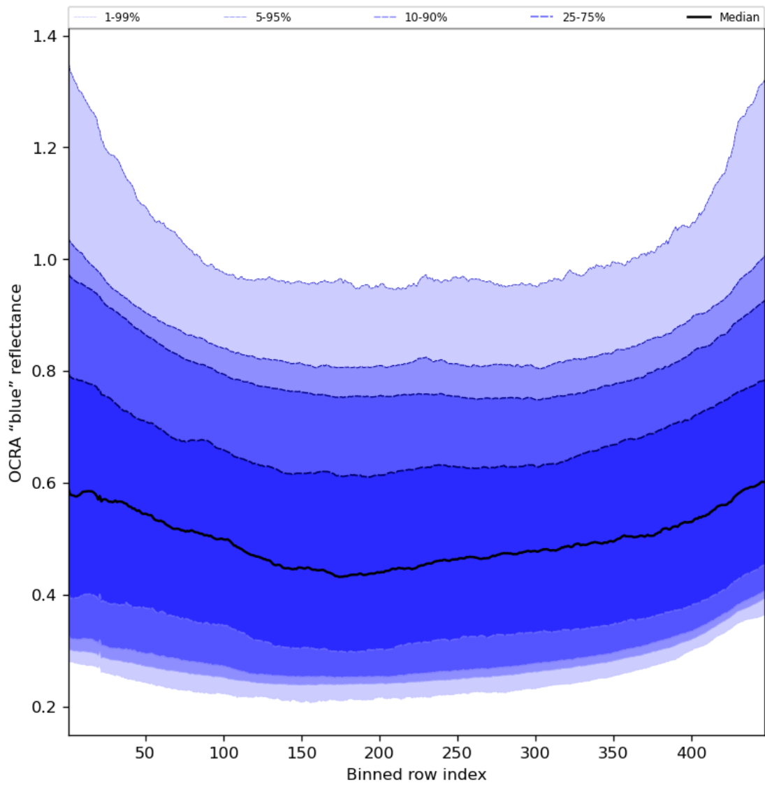
Figure 67: Along track statistics of “OCRA “blue” reflectance” for 2023-09-02 to 2023-09-04
