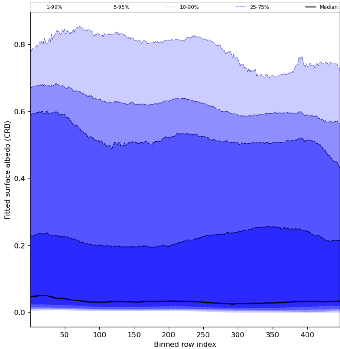
Figure 62: Along track statistics of “Fitted surface albedo (CRB)” for 2023-09-02 to 2023-09-04
