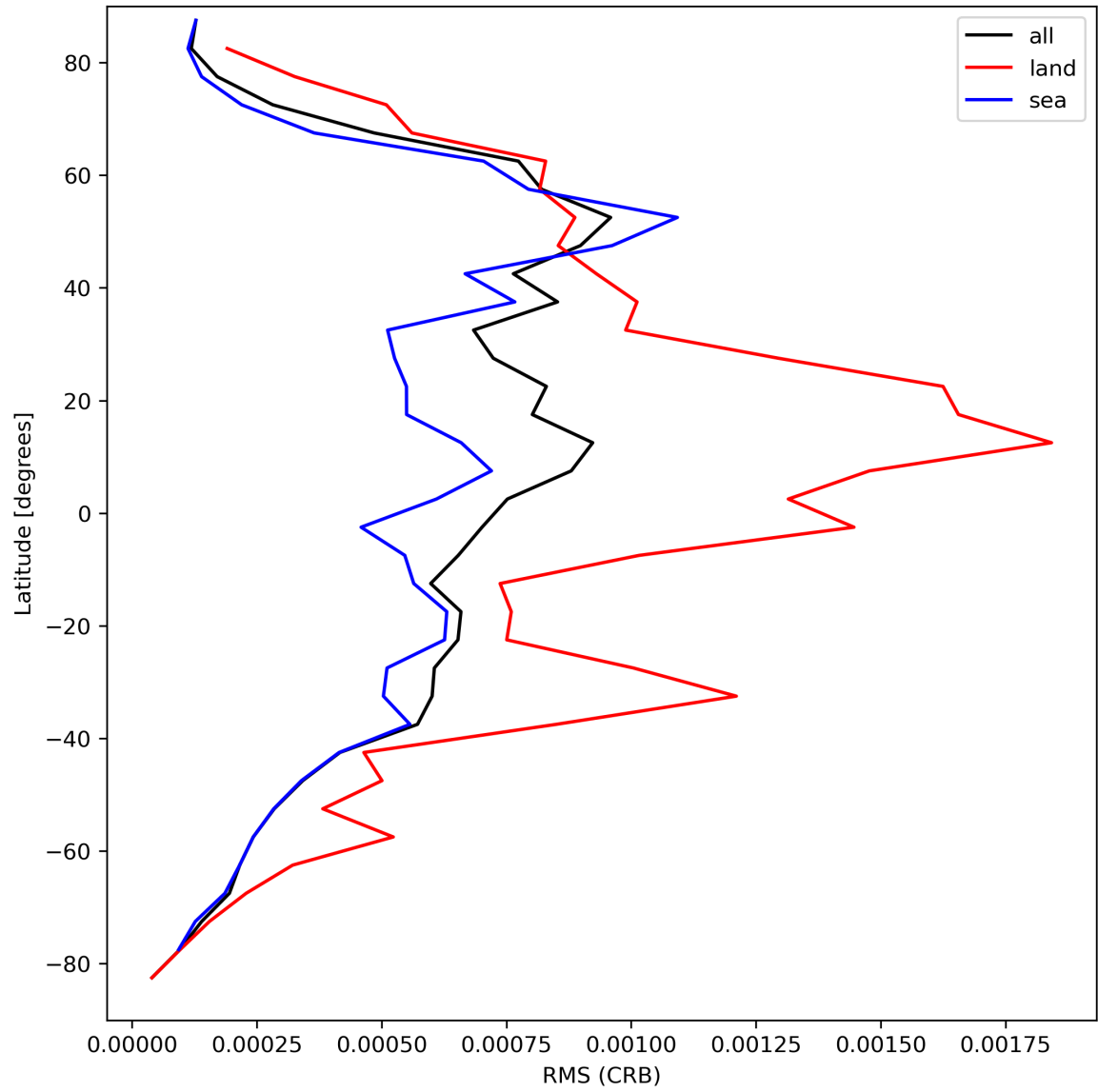
Figure 32: Zonal average of “RMS (CRB)” for 2023-09-02 to 2023-09-04.
