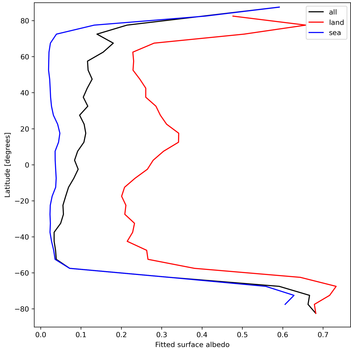
Figure 29: Zonal average of “Fitted surface albedo” for 2023-09-02 to 2023-09-04.
