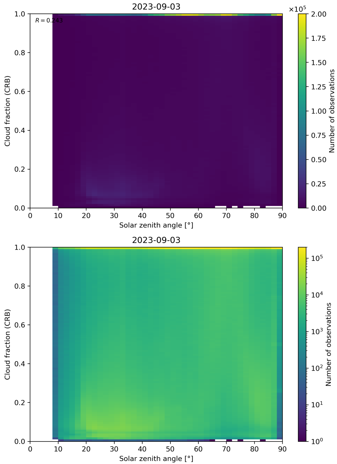
Figure 101: Scatter density plot of “Solar zenith angle” against “Cloud fraction (CRB)” for 2023-09-02 to 2023-09-04.
