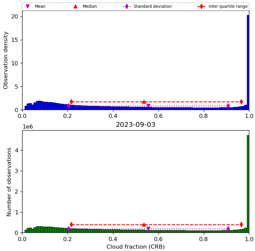
Figure 42: Histogram of “Cloud fraction (CRB)” for 2023-09-02 to 2023-09-04
