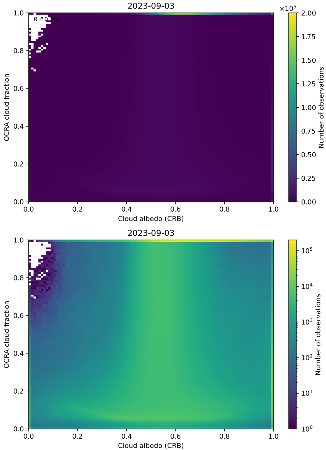
Figure 70: Scatter density plot of “Cloud albedo (CRB)” against “OCRA cloud fraction” for 2023-09-02 to 2023-09-04.
