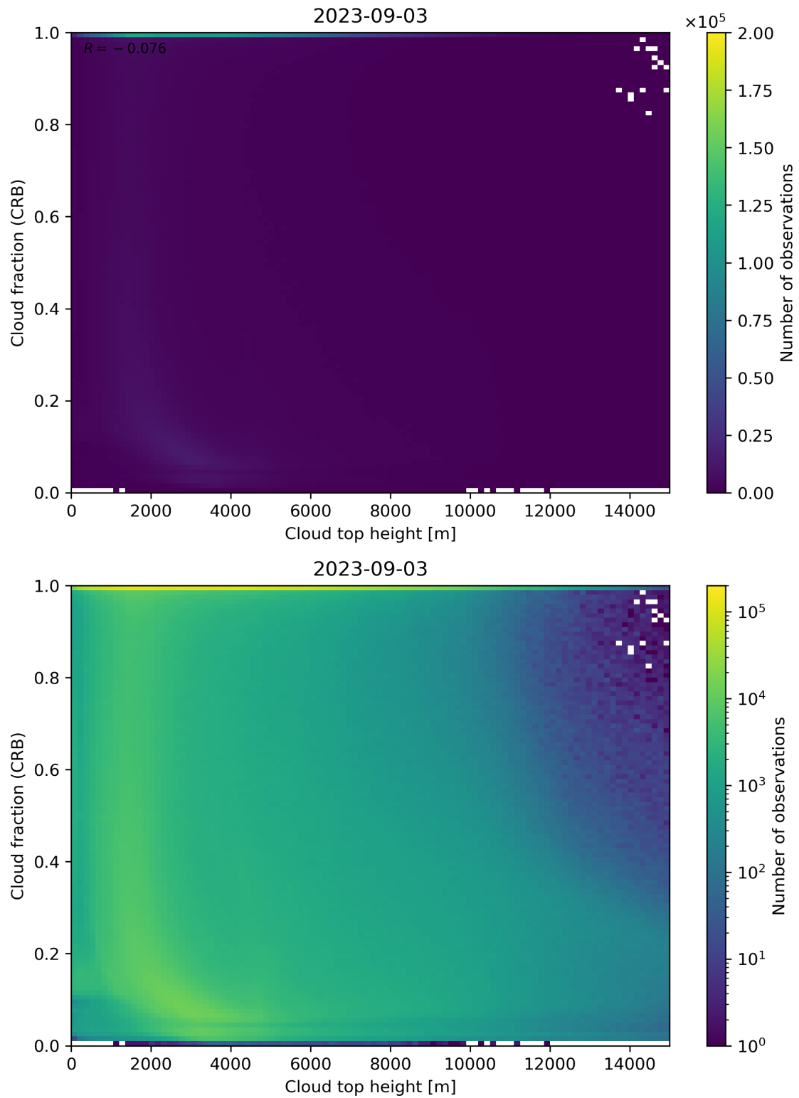
Figure 88: Scatter density plot of “Cloud top height” against “Cloud fraction (CRB)” for 2023-09-02 to 2023-09-04.
