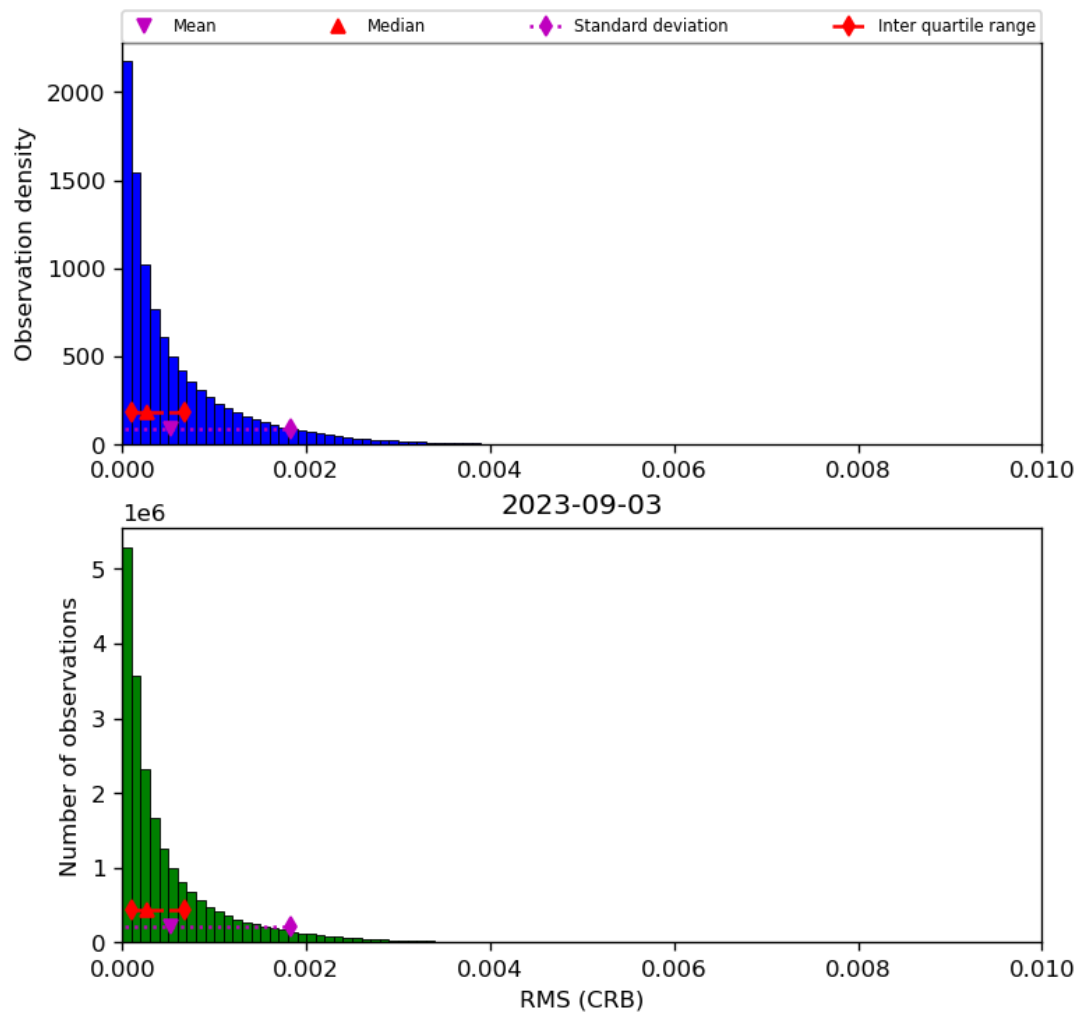
Figure 48: Histogram of “RMS (CRB)” for 2023-09-02 to 2023-09-04
