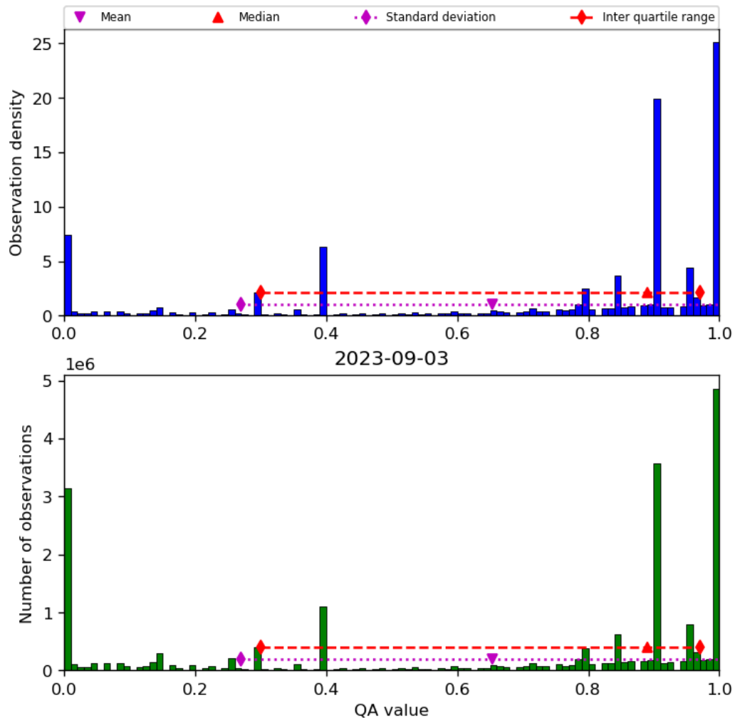
Figure 38: Histogram of “QA value” for 2023-09-02 to 2023-09-04
