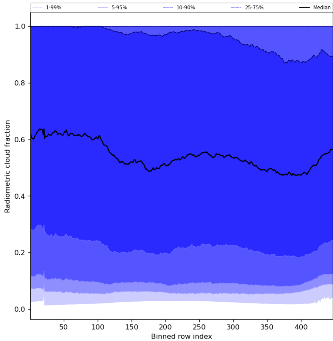
Figure 55: Along track statistics of “Radiometric cloud fraction” for 2023-09-02 to 2023-09-04
