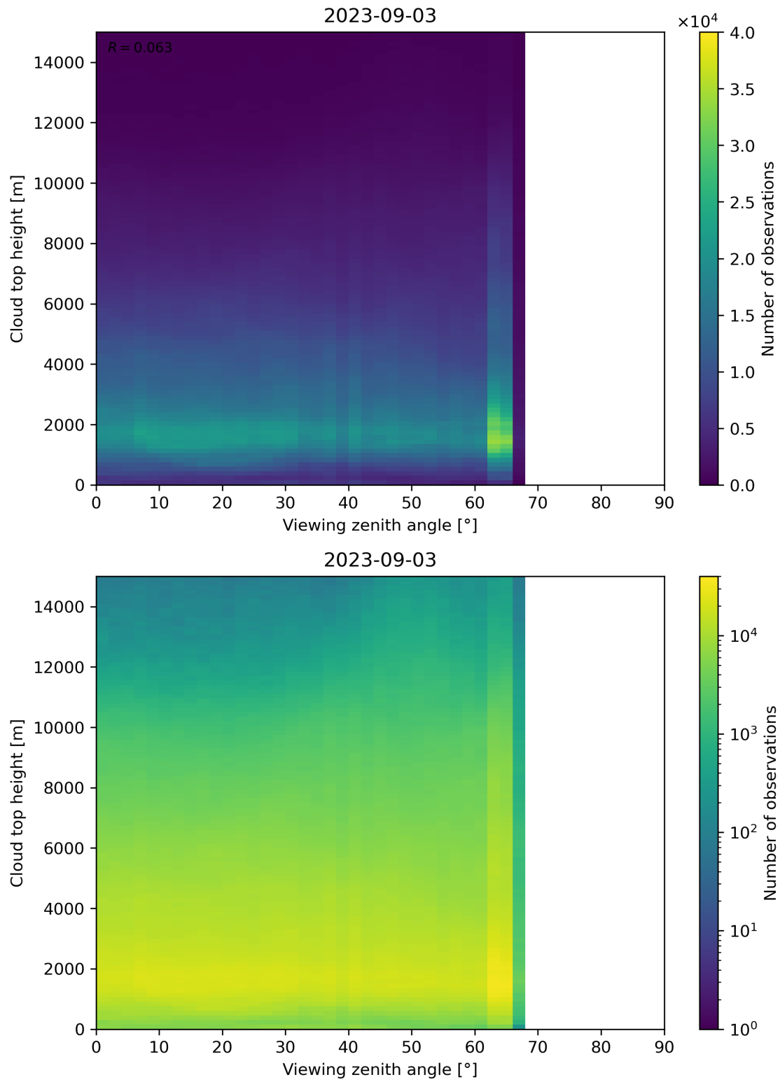
Figure 112: Scatter density plot of “Viewing zenith angle” against “Cloud top height” for 2023-09-02 to 2023-09-04.
