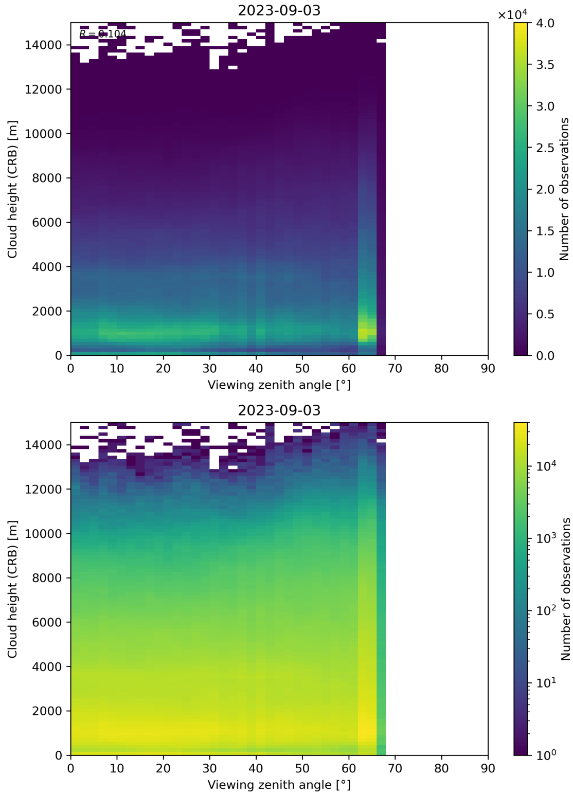
Figure 110: Scatter density plot of “Viewing zenith angle” against “Cloud height (CRB)” for 2023-09-02 to 2023-09-04.
