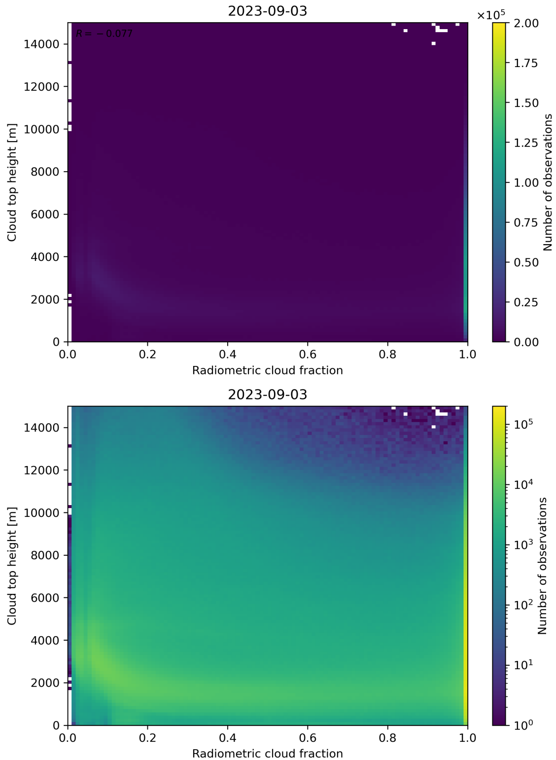
Figure 76: Scatter density plot of “Radiometric cloud fraction” against “Cloud top height” for 2023-09-02 to 2023-09-04.
