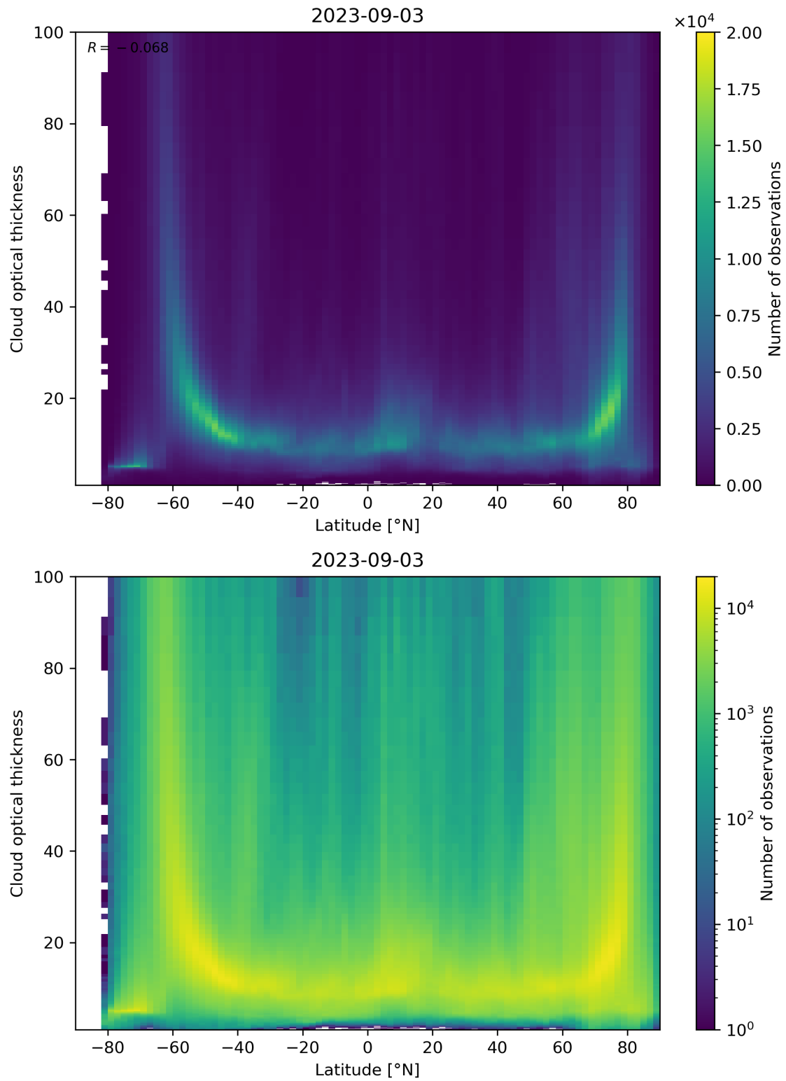
Figure 96: Scatter density plot of “Latitude” against “Cloud optical thickness” for 2023-09-02 to 2023-09-04.
