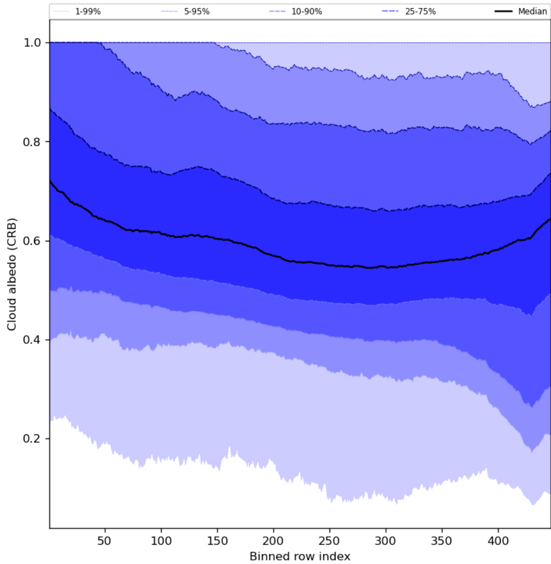
Figure 60: Along track statistics of “Cloud albedo (CRB)” for 2023-09-02 to 2023-09-04
