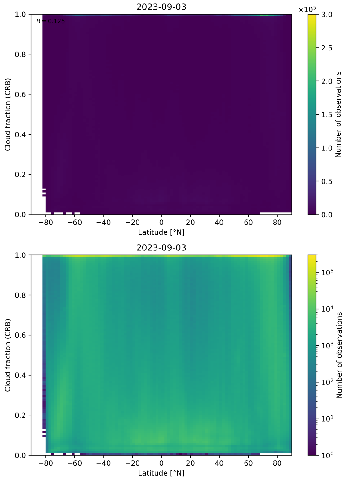
Figure 94: Scatter density plot of “Latitude” against “Cloud fraction (CRB)” for 2023-09-02 to 2023-09-04.
