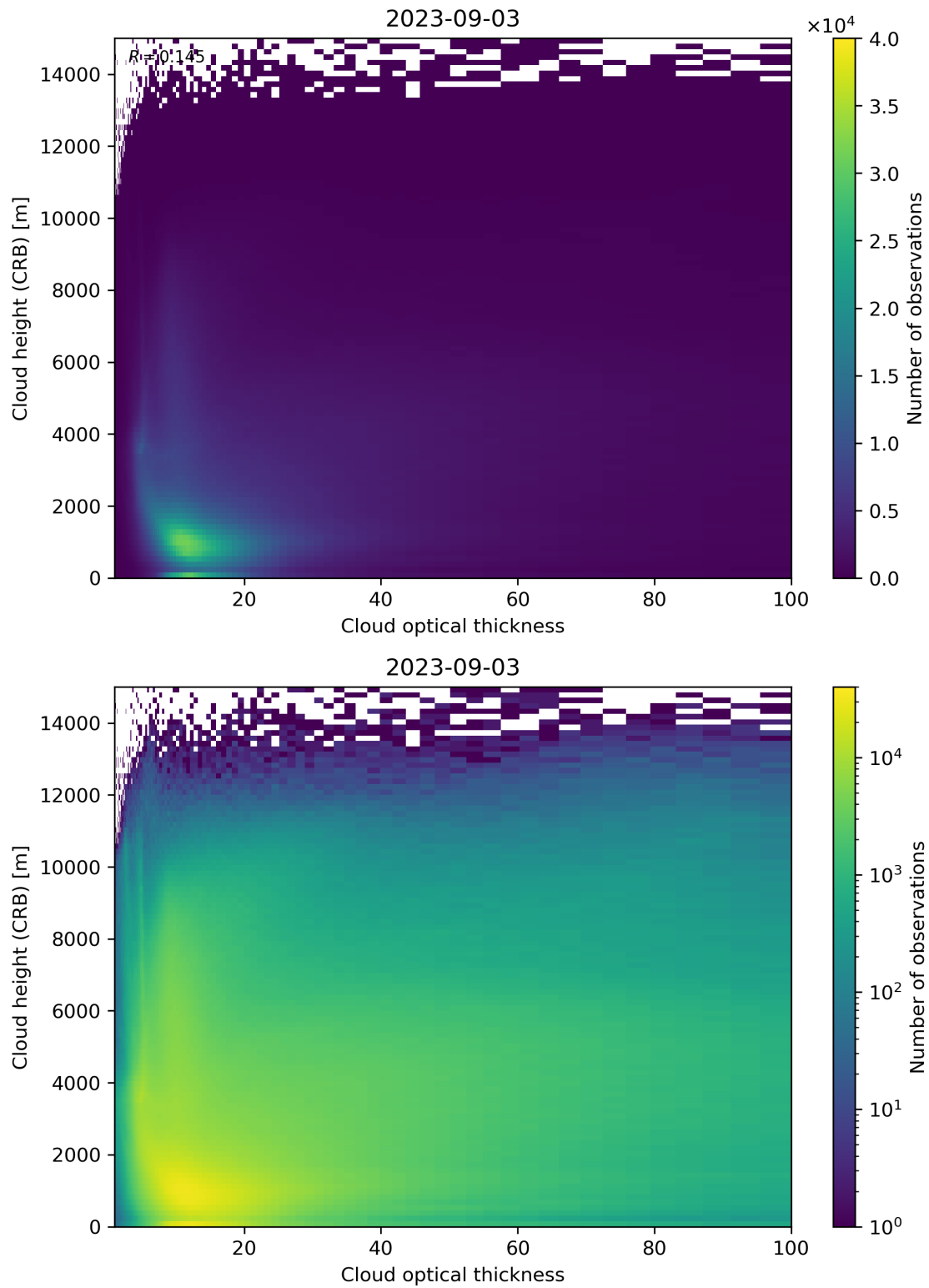
Figure 85: Scatter density plot of “Cloud optical thickness” against “Cloud height (CRB)” for 2023-09-02 to 2023-09-04.
