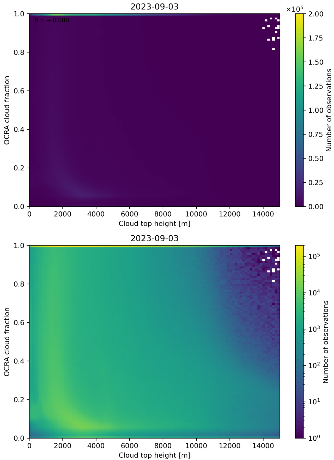
Figure 87: Scatter density plot of “Cloud top height” against “OCRA cloud fraction” for 2023-09-02 to 2023-09-04.
