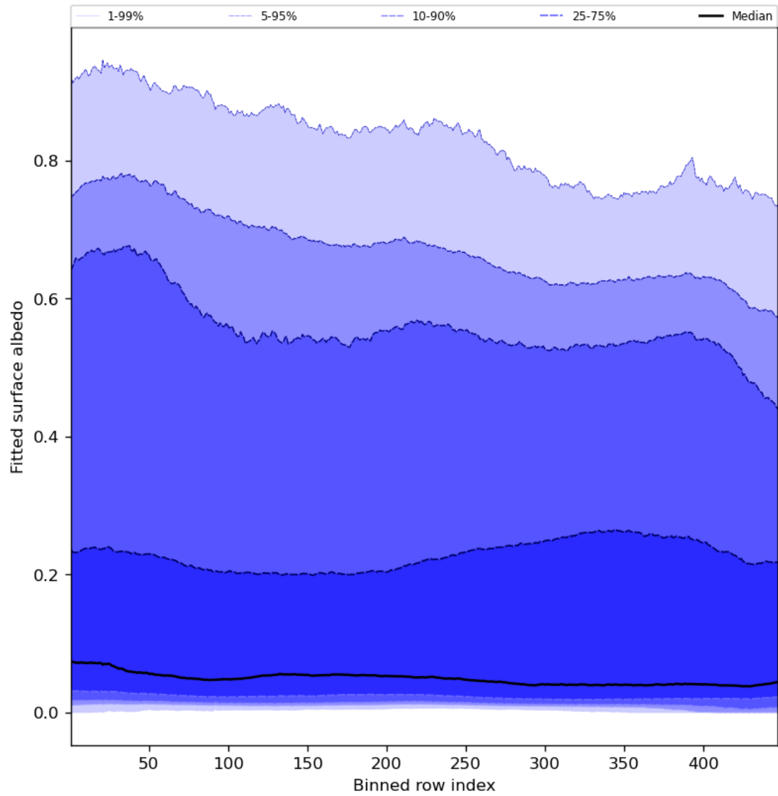
Figure 61: Along track statistics of “Fitted surface albedo” for 2023-09-02 to 2023-09-04
