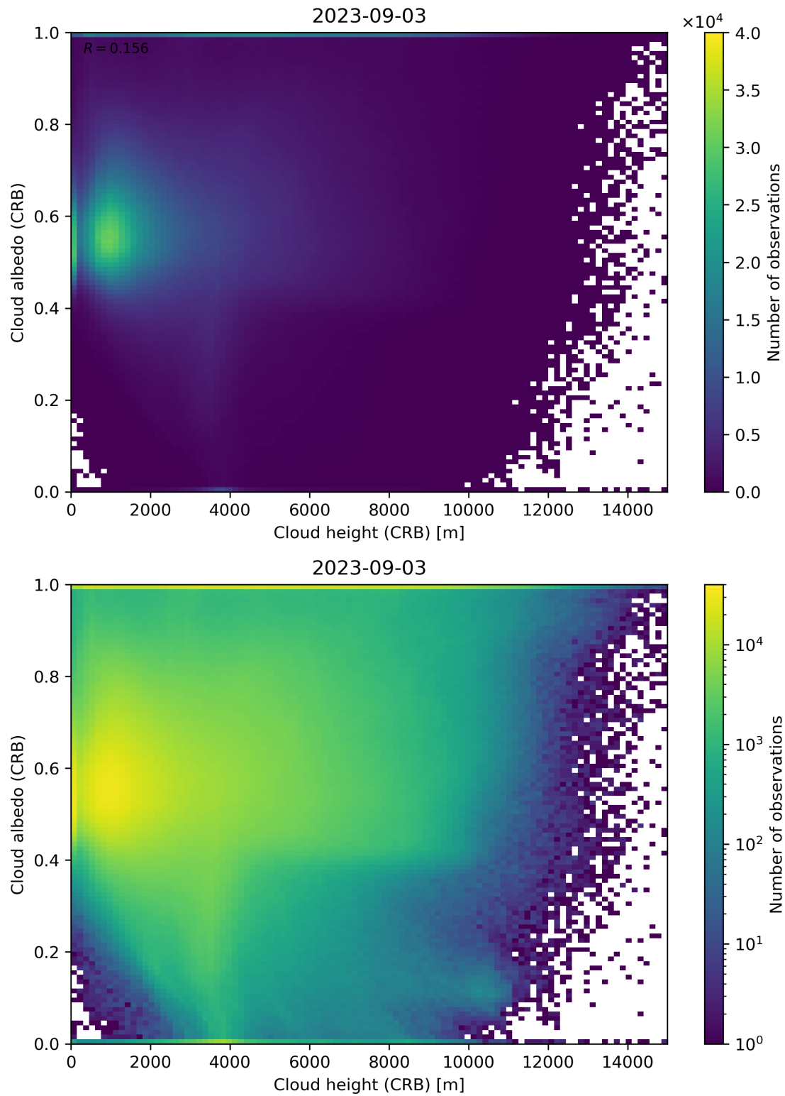
Figure 80: Scatter density plot of “Cloud height (CRB)” against “Cloud albedo (CRB)” for 2023-09-02 to 2023-09-04.
