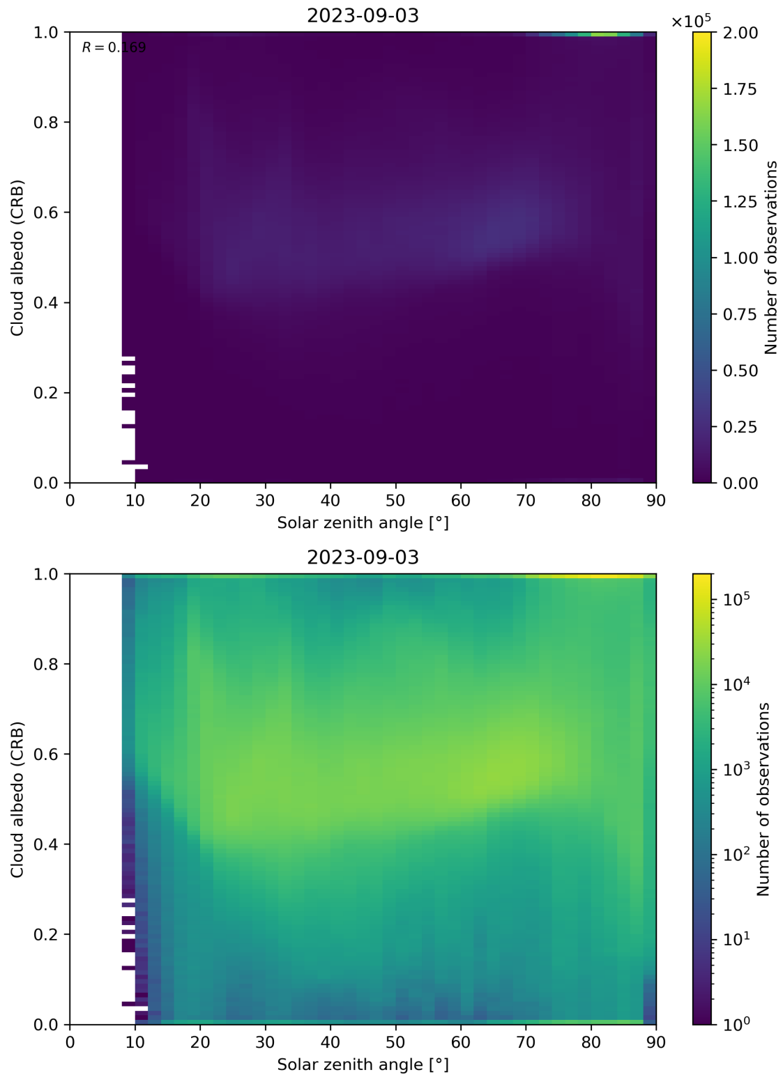
Figure 98: Scatter density plot of “Solar zenith angle” against “Cloud albedo (CRB)” for 2023-09-02 to 2023-09-04.
