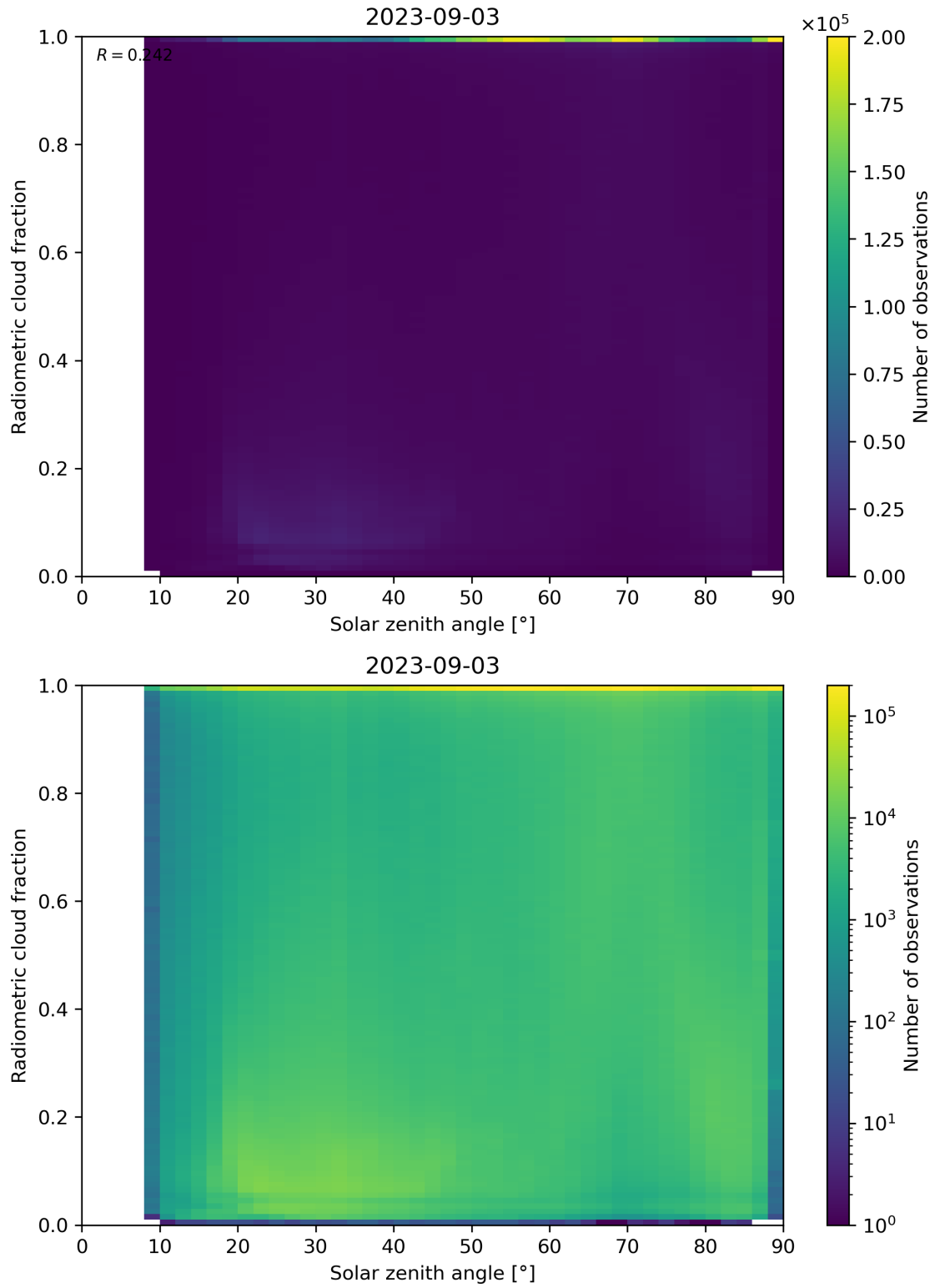
Figure 99: Scatter density plot of “Solar zenith angle” against “Radiometric cloud fraction” for 2023-09-02 to 2023-09-04.
