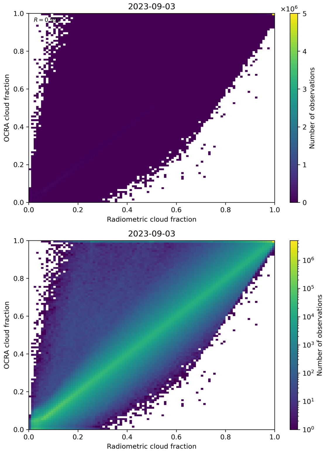
Figure 72: Scatter density plot of “Radiometric cloud fraction” against “OCRA cloud fraction” for 2023-09-02 to 2023-09-04.
