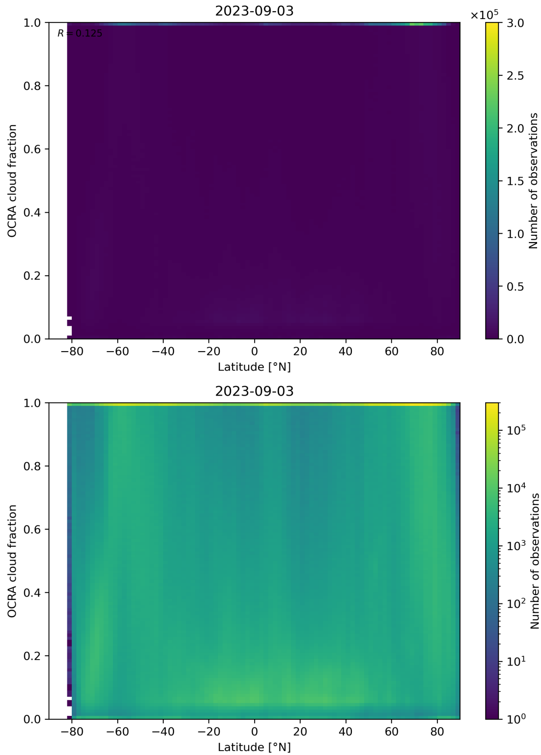
Figure 93: Scatter density plot of “Latitude” against “OCRA cloud fraction” for 2023-09-02 to 2023-09-04.
