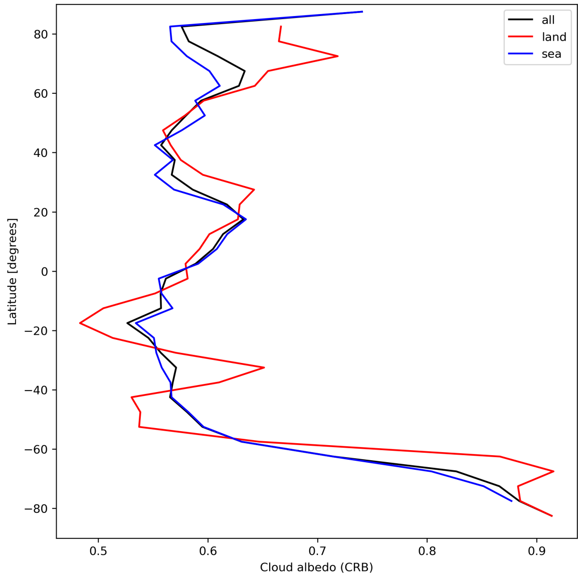
Figure 28: Zonal average of “Cloud albedo (CRB)” for 2023-09-02 to 2023-09-04.
