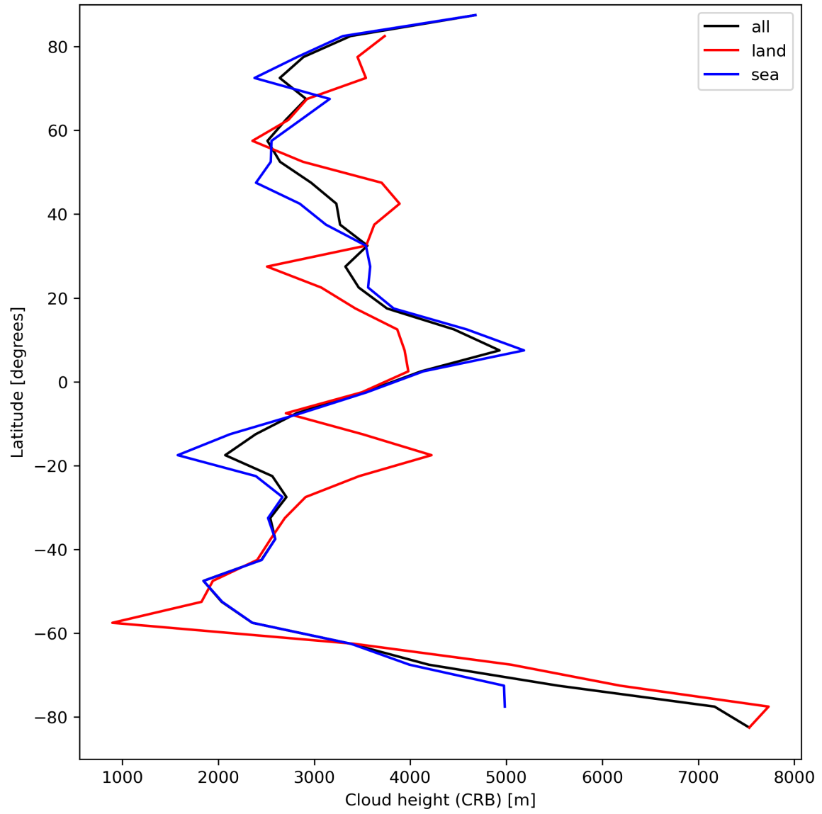
Figure 27: Zonal average of “Cloud height (CRB)” for 2023-09-02 to 2023-09-04.
