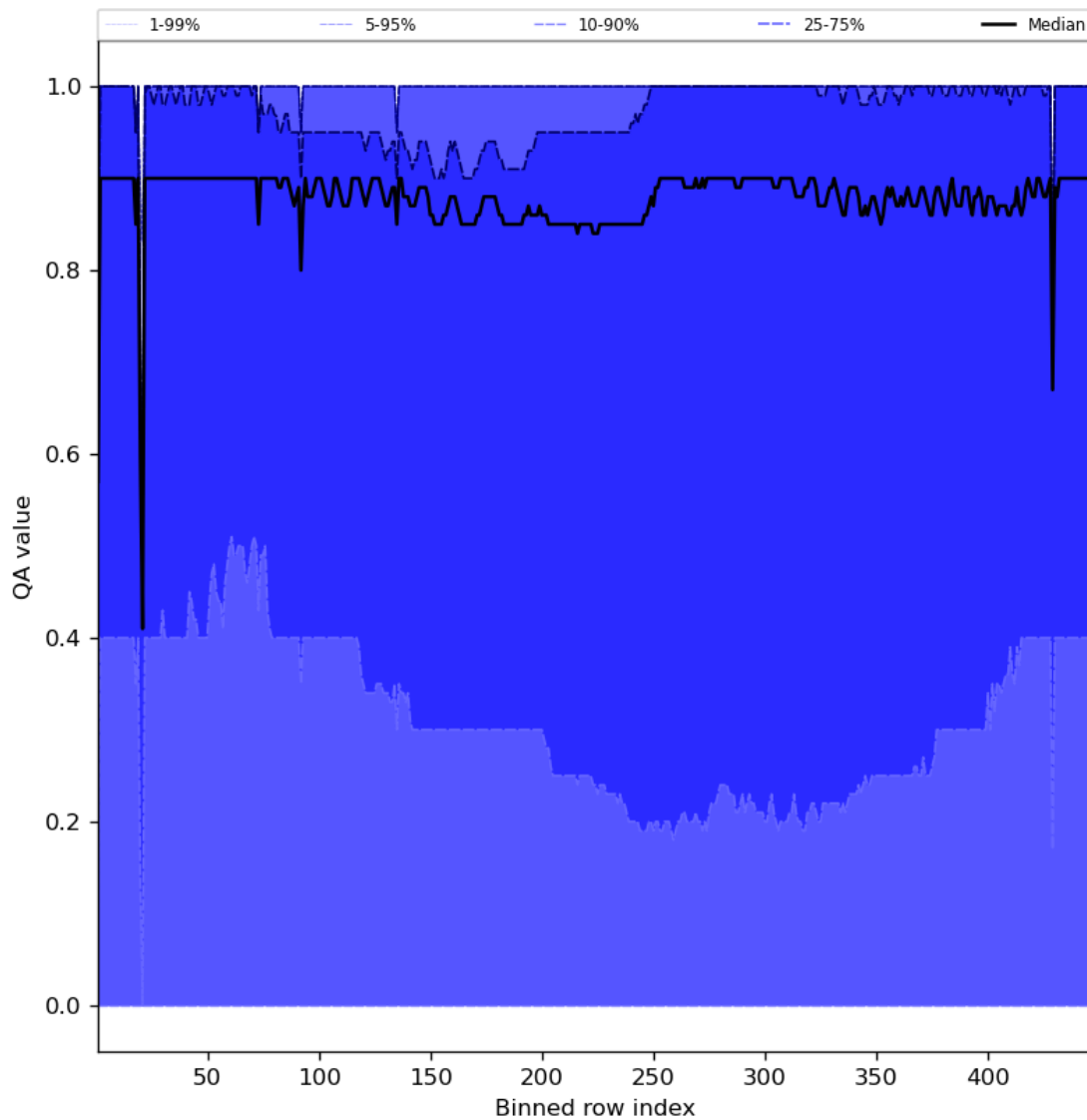
Figure 54: Along track statistics of “QA value” for 2023-09-02 to 2023-09-04
