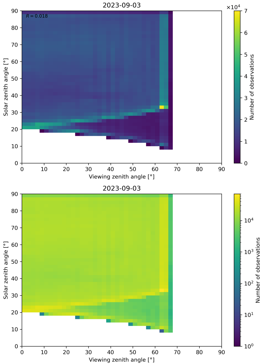
Figure 114: Scatter density plot of “Viewing zenith angle” against “Solar zenith angle” for 2023-09-02 to 2023-09-04.
