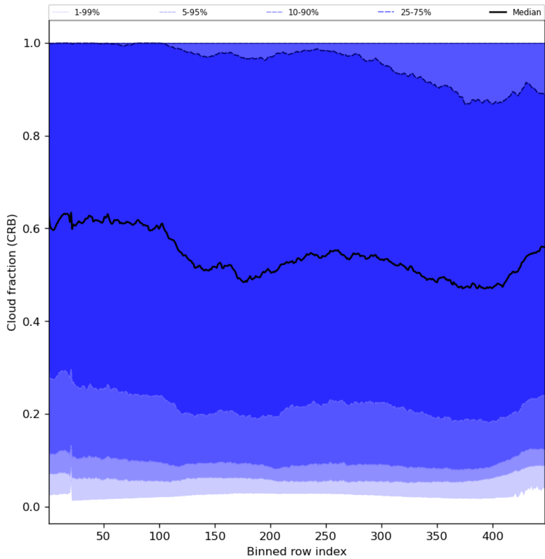
Figure 58: Along track statistics of “Cloud fraction (CRB)” for 2023-09-02 to 2023-09-04
