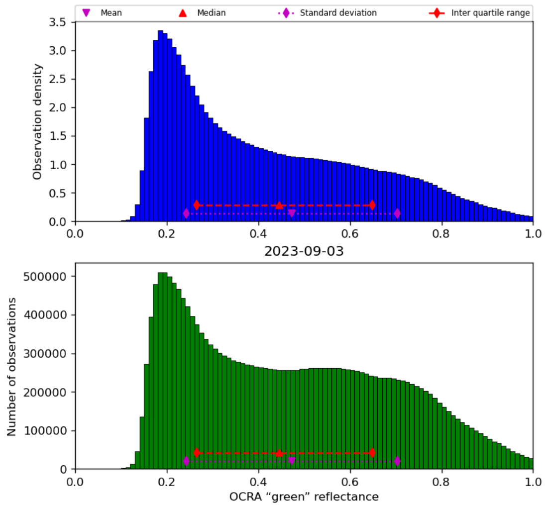
Figure 52: Histogram of “OCRA “green” reflectance” for 2023-09-02 to 2023-09-04
