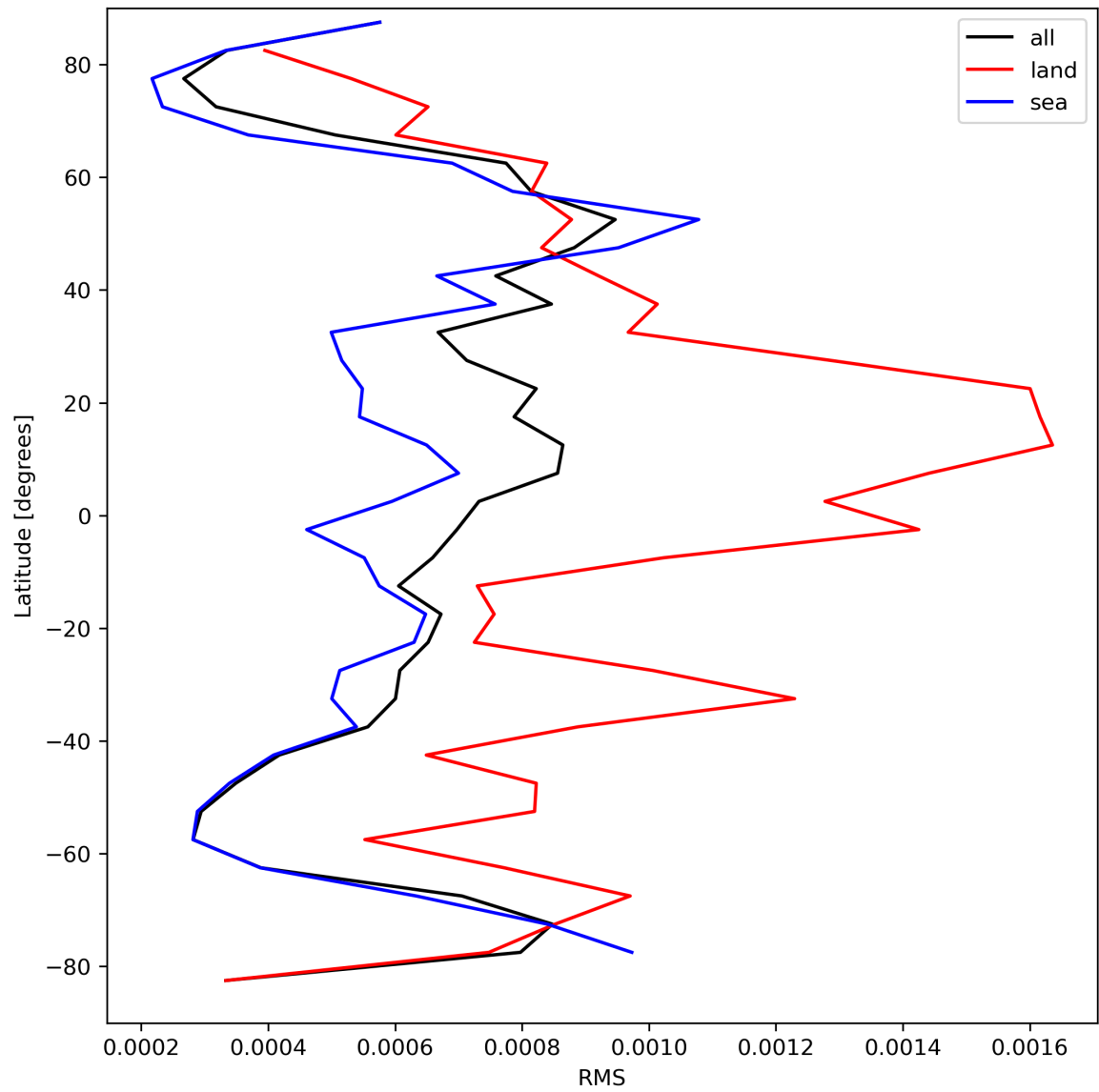
Figure 31: Zonal average of “RMS” for 2023-09-02 to 2023-09-04.
