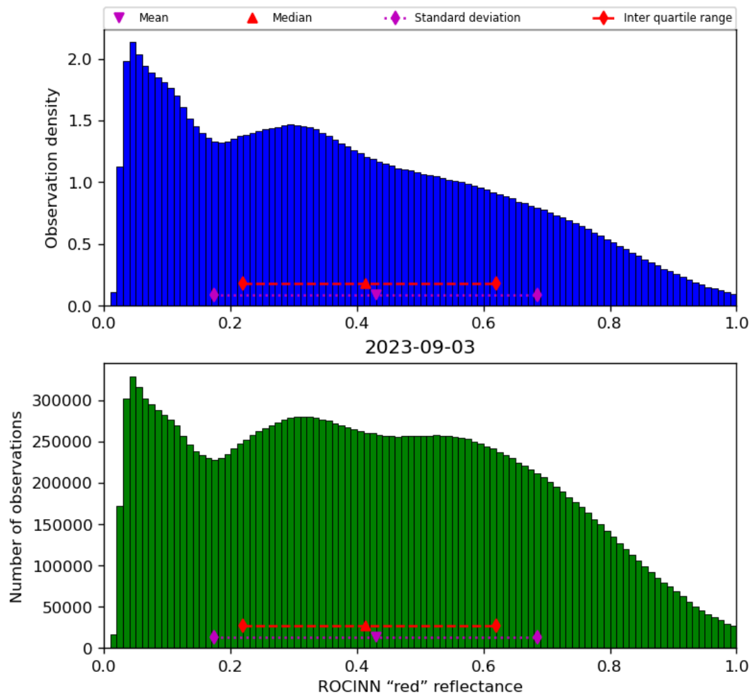
Figure 53: Histogram of “ROCINN “red” reflectance” for 2023-09-02 to 2023-09-04
