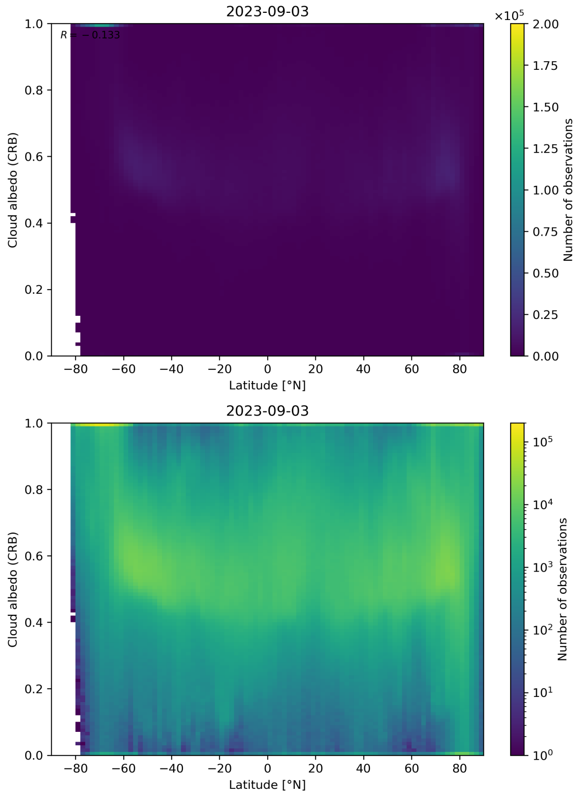
Figure 91: Scatter density plot of “Latitude” against “Cloud albedo (CRB)” for 2023-09-02 to 2023-09-04.
