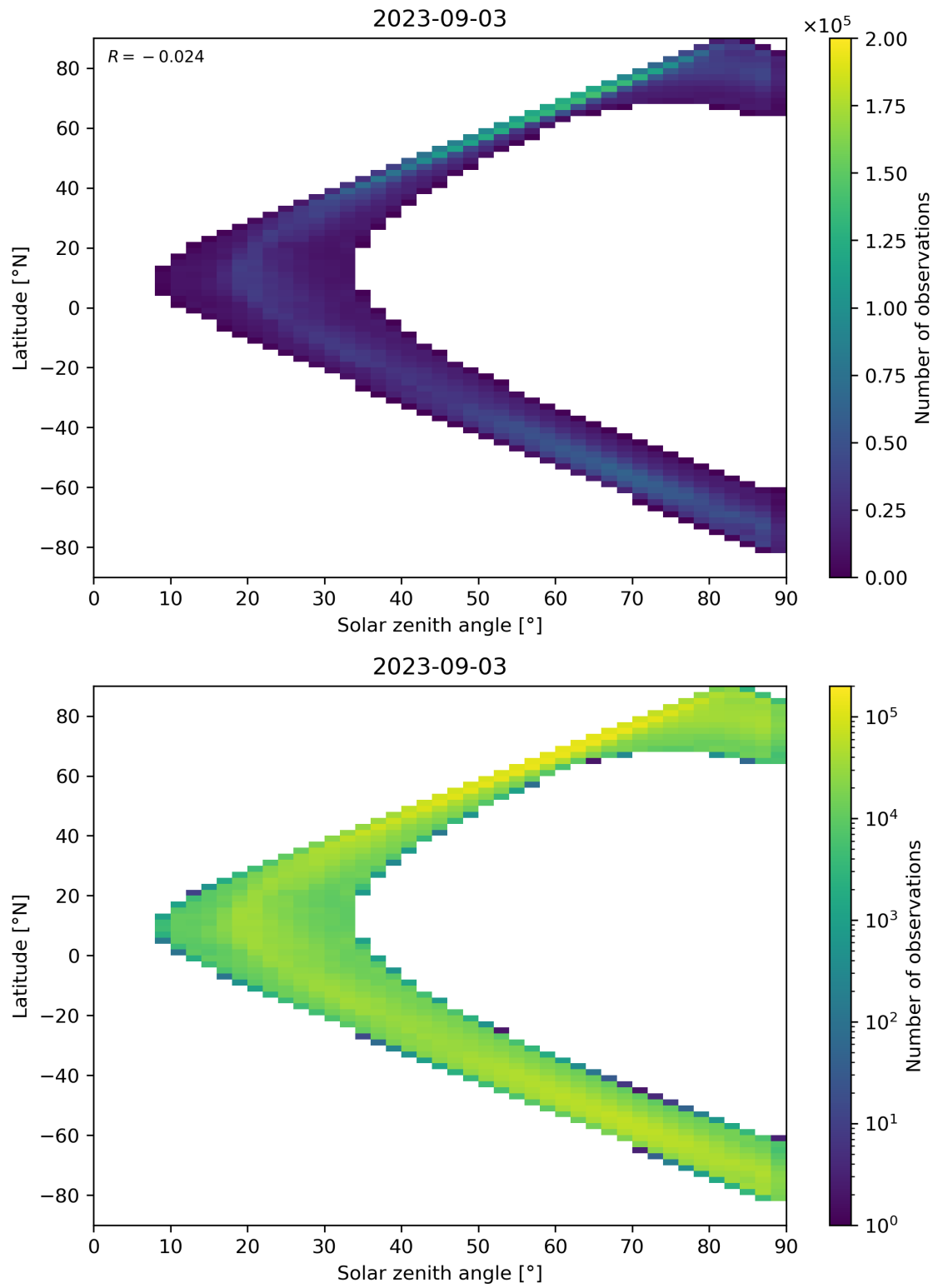
Figure 105: Scatter density plot of “Solar zenith angle” against “Latitude” for 2023-09-02 to 2023-09-04.
