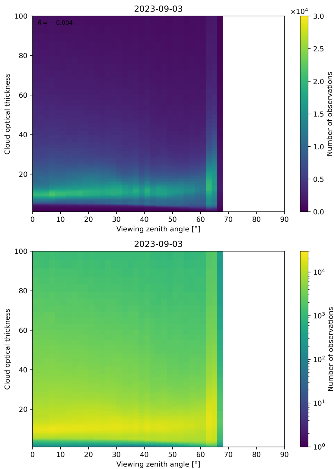
Figure 111: Scatter density plot of “Viewing zenith angle” against “Cloud optical thickness” for 2023-09-02 to 2023-09-04.
