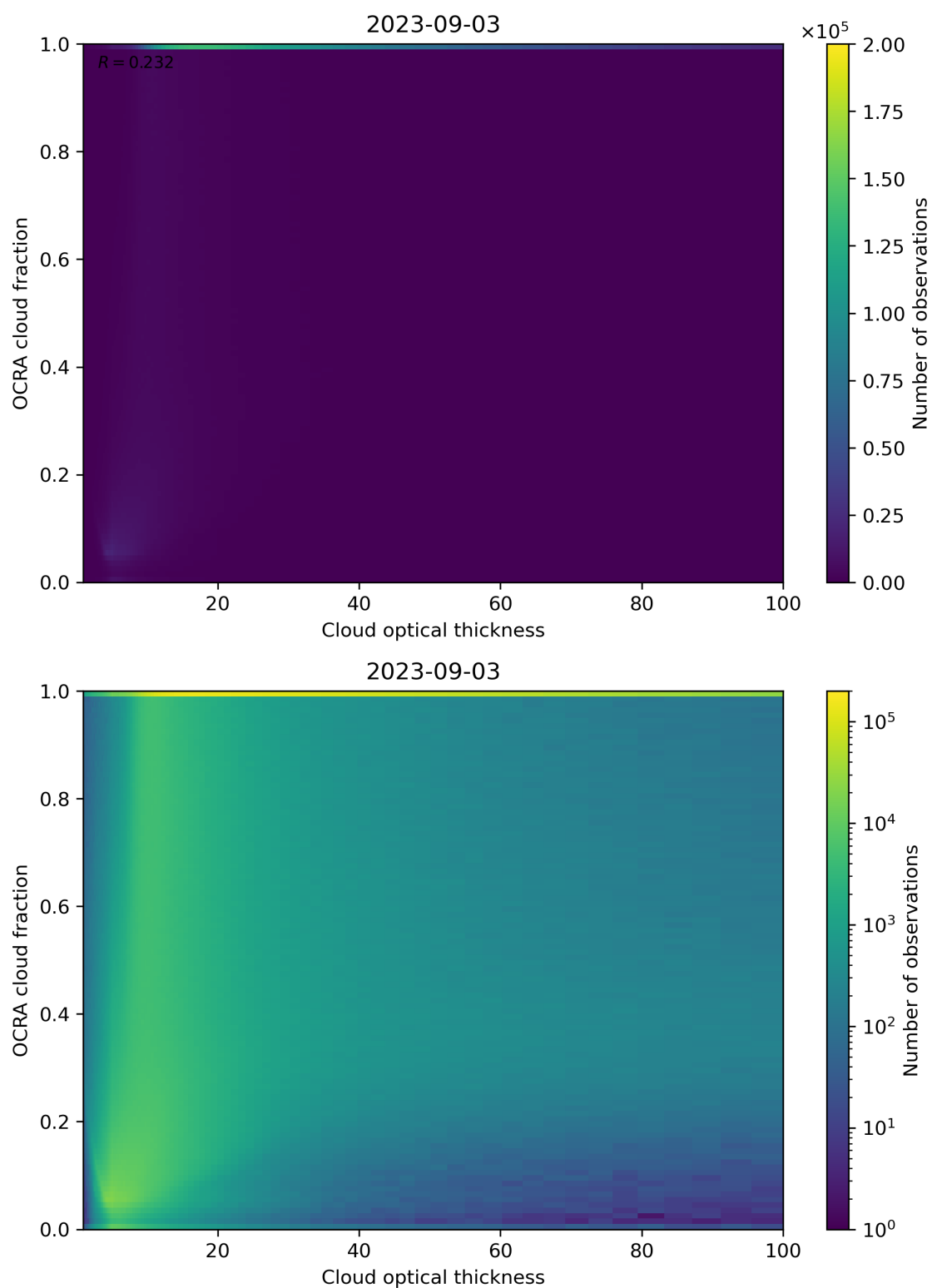
Figure 83: Scatter density plot of “Cloud optical thickness” against “OCRA cloud fraction” for 2023-09-02 to 2023-09-04.
