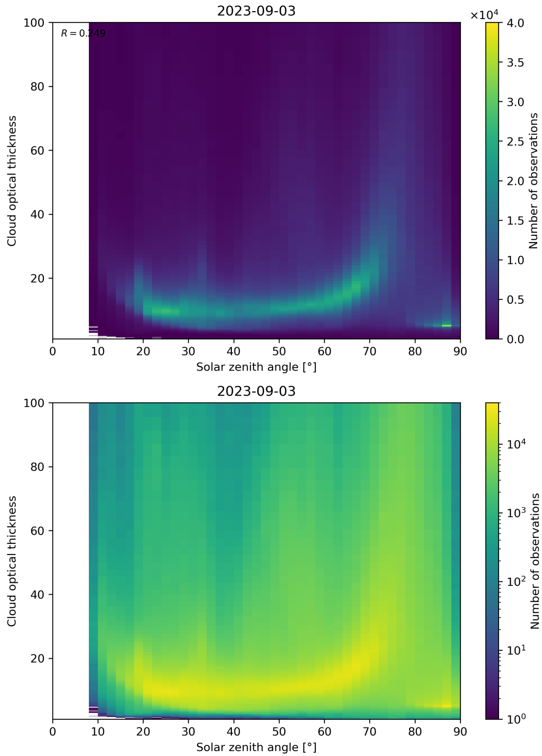
Figure 103: Scatter density plot of “Solar zenith angle” against “Cloud optical thickness” for 2023-09-02 to 2023-09-04.
