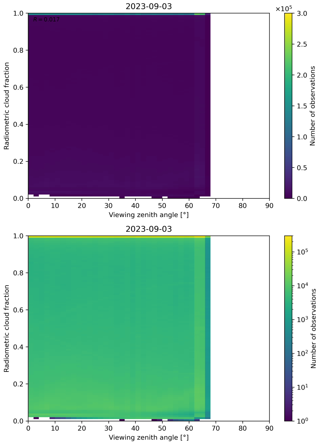
Figure 107: Scatter density plot of “Viewing zenith angle” against “Radiometric cloud fraction” for 2023-09-02 to 2023-09-04.
