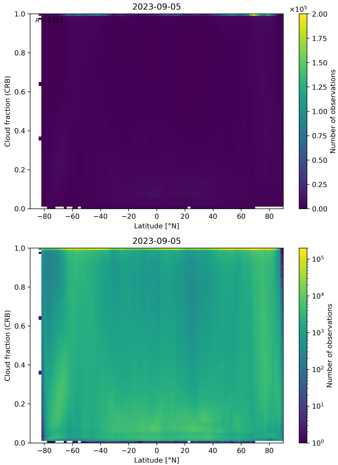
Figure 94: Scatter density plot of “Latitude” against “Cloud fraction (CRB)” for 2023-09-05 to 2023-09-06.
