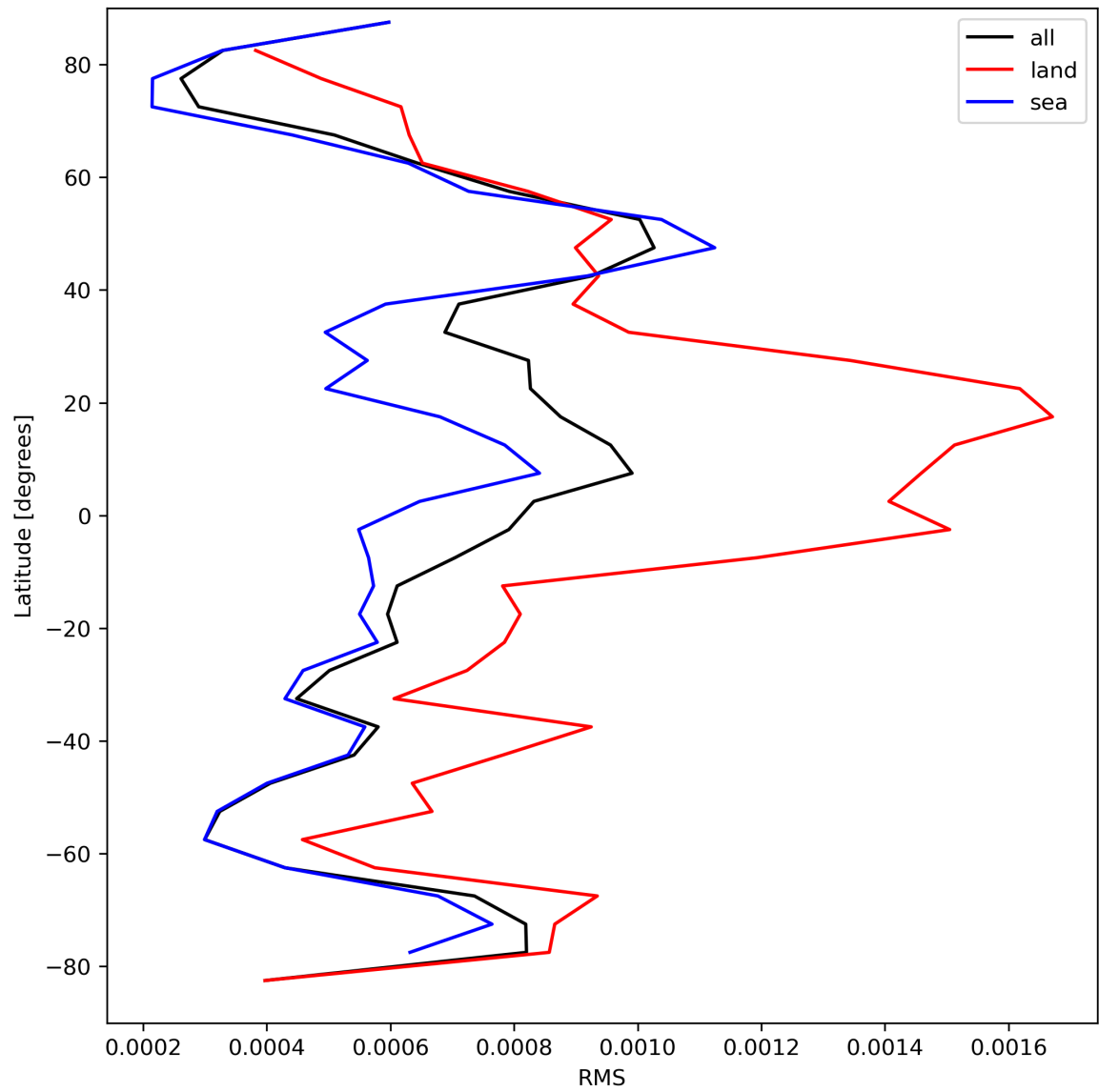
Figure 31: Zonal average of “RMS” for 2023-09-05 to 2023-09-06.
