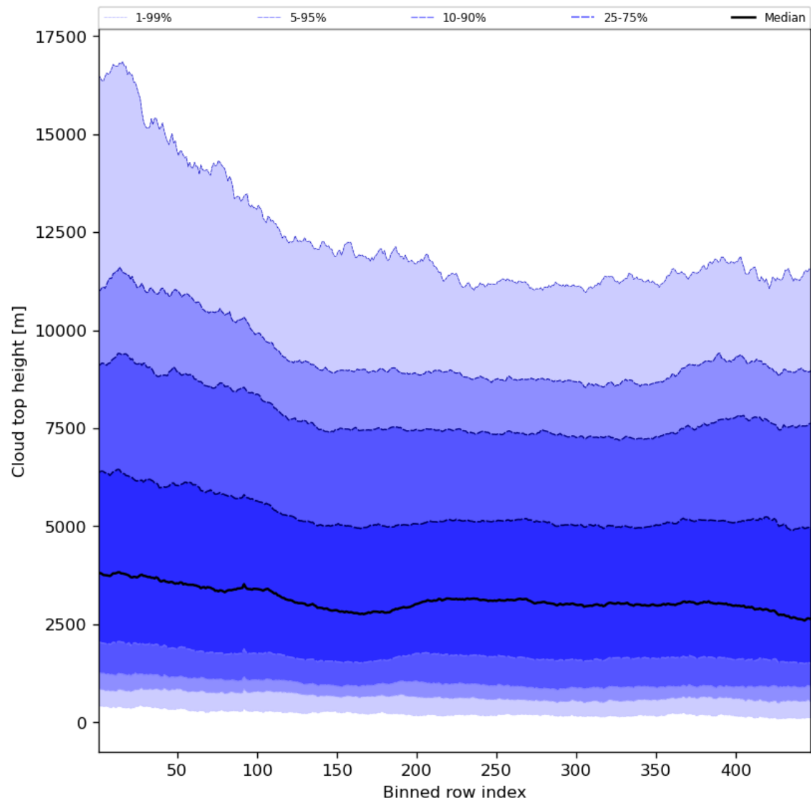
Figure 56: Along track statistics of “Cloud top height” for 2023-09-05 to 2023-09-06
