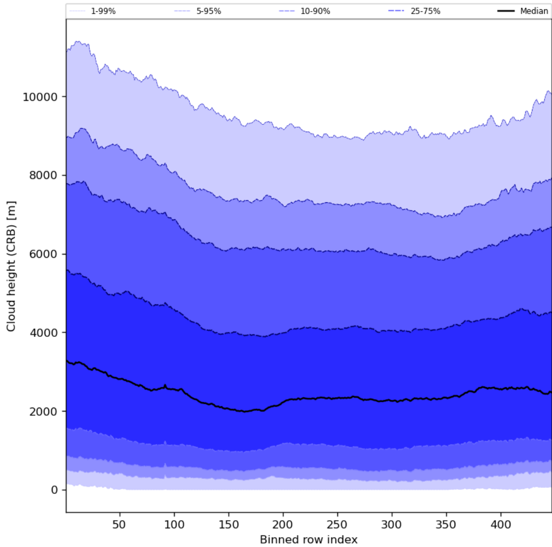
Figure 59: Along track statistics of “Cloud height (CRB)” for 2023-09-05 to 2023-09-06
