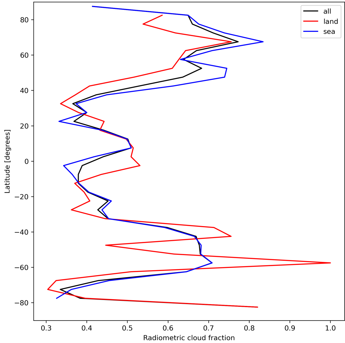
Figure 23: Zonal average of “Radiometric cloud fraction” for 2023-09-05 to 2023-09-06.
