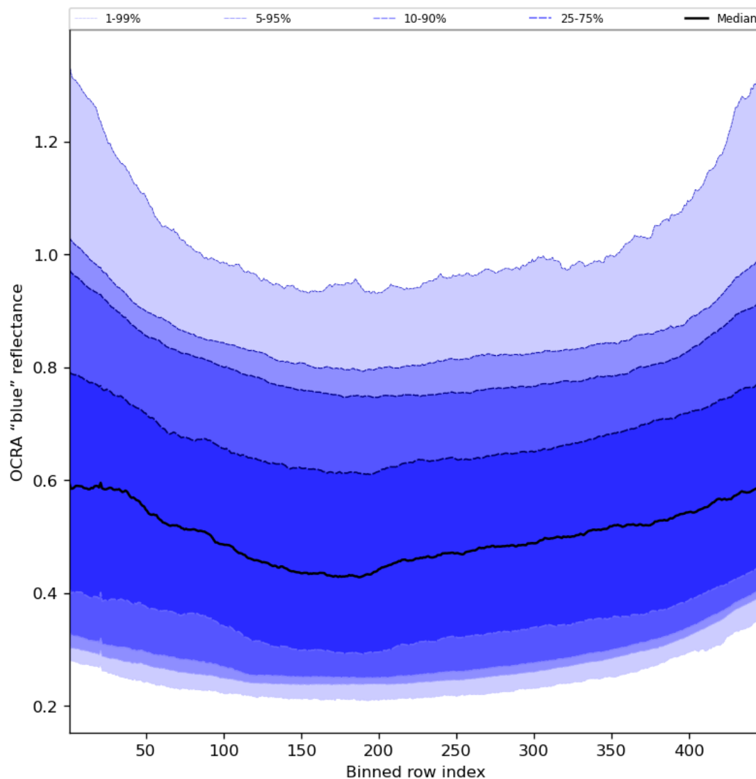
Figure 67: Along track statistics of “OCRA “blue” reflectance” for 2023-09-05 to 2023-09-06
