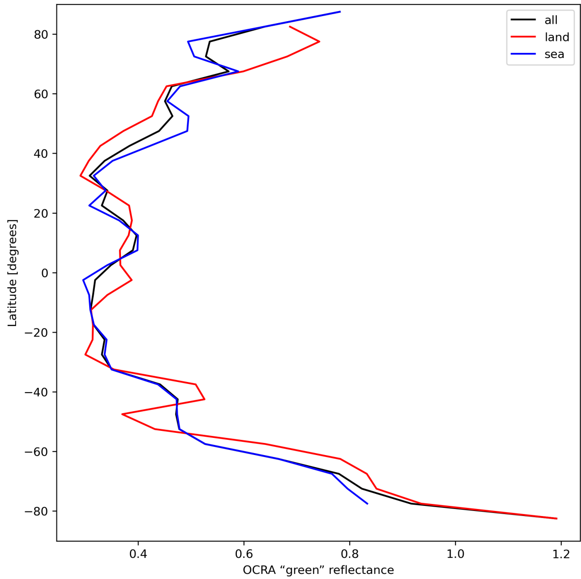
Figure 36: Zonal average of “OCRA “green” reflectance” for 2023-09-05 to 2023-09-06.
