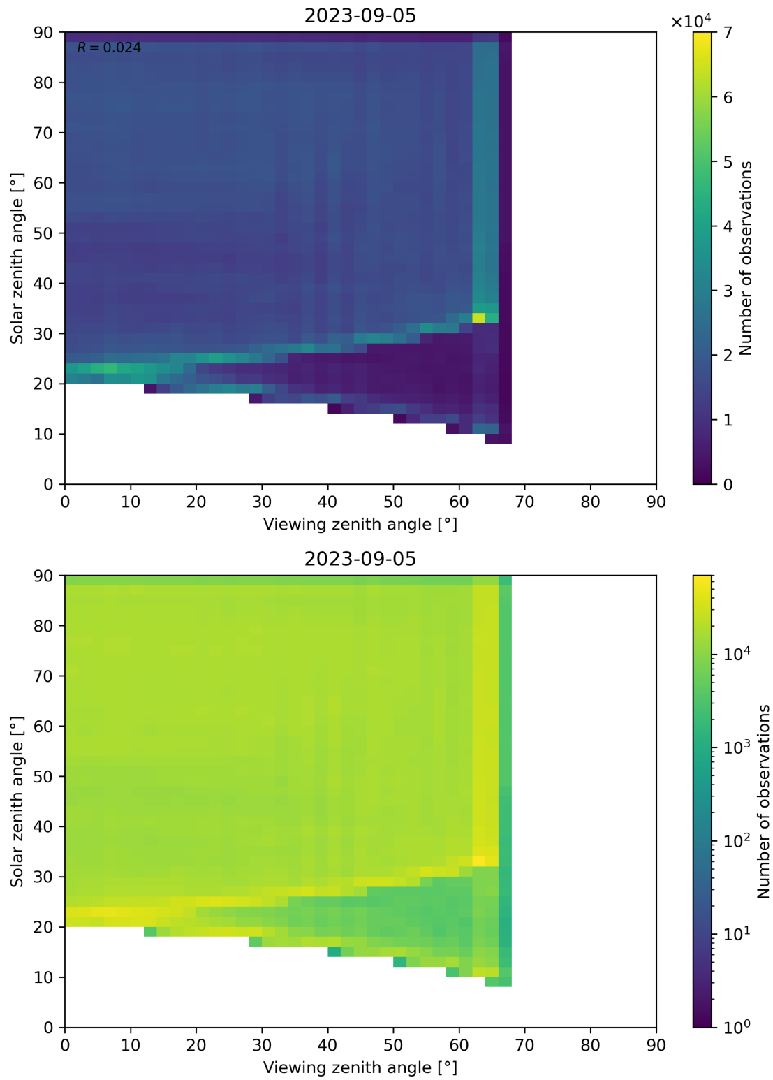
Figure 114: Scatter density plot of “Viewing zenith angle” against “Solar zenith angle” for 2023-09-05 to 2023-09-06.
