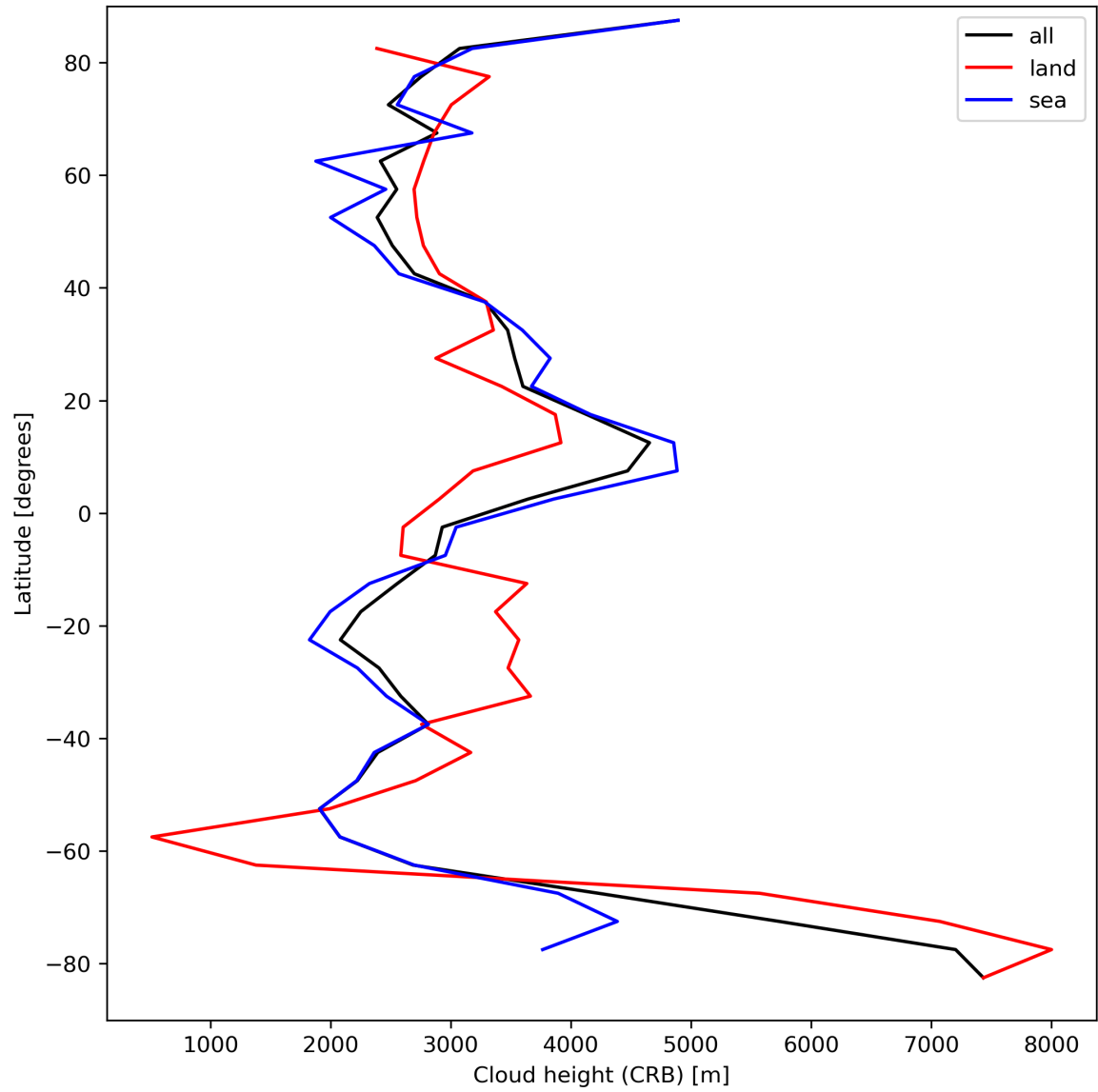
Figure 27: Zonal average of “Cloud height (CRB)” for 2023-09-05 to 2023-09-06.
