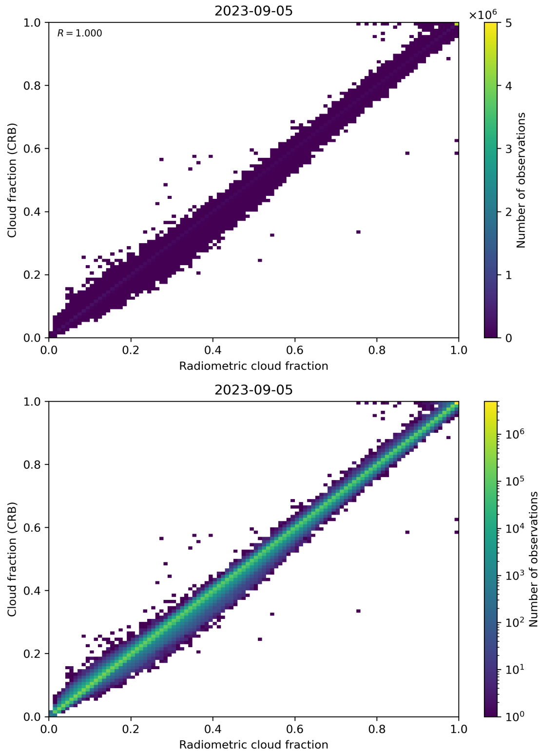
Figure 73: Scatter density plot of “Radiometric cloud fraction” against “Cloud fraction (CRB)” for 2023-09-05 to 2023-09-06.
