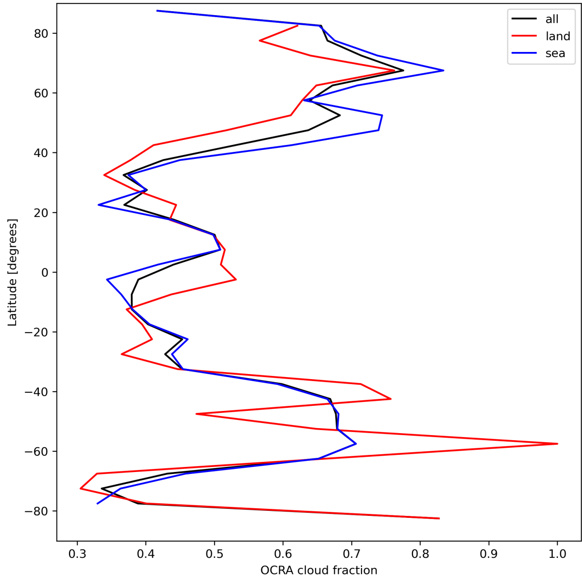
Figure 34: Zonal average of “OCRA cloud fraction” for 2023-09-05 to 2023-09-06.
