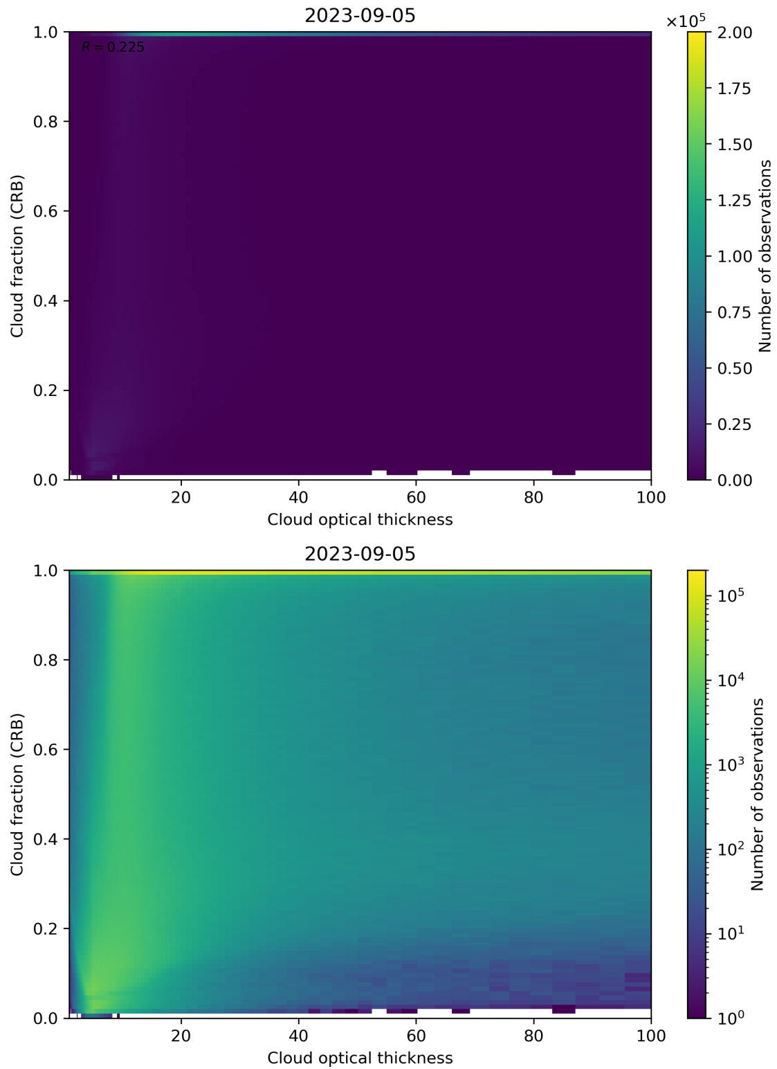
Figure 84: Scatter density plot of “Cloud optical thickness” against “Cloud fraction (CRB)” for 2023-09-05 to 2023-09-06.
