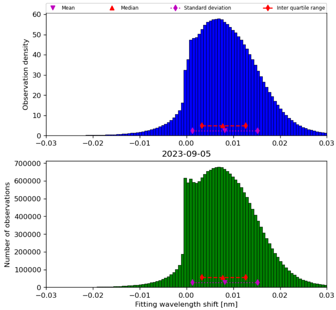
Figure 49: Histogram of “Fitting wavelength shift” for 2023-09-05 to 2023-09-06
