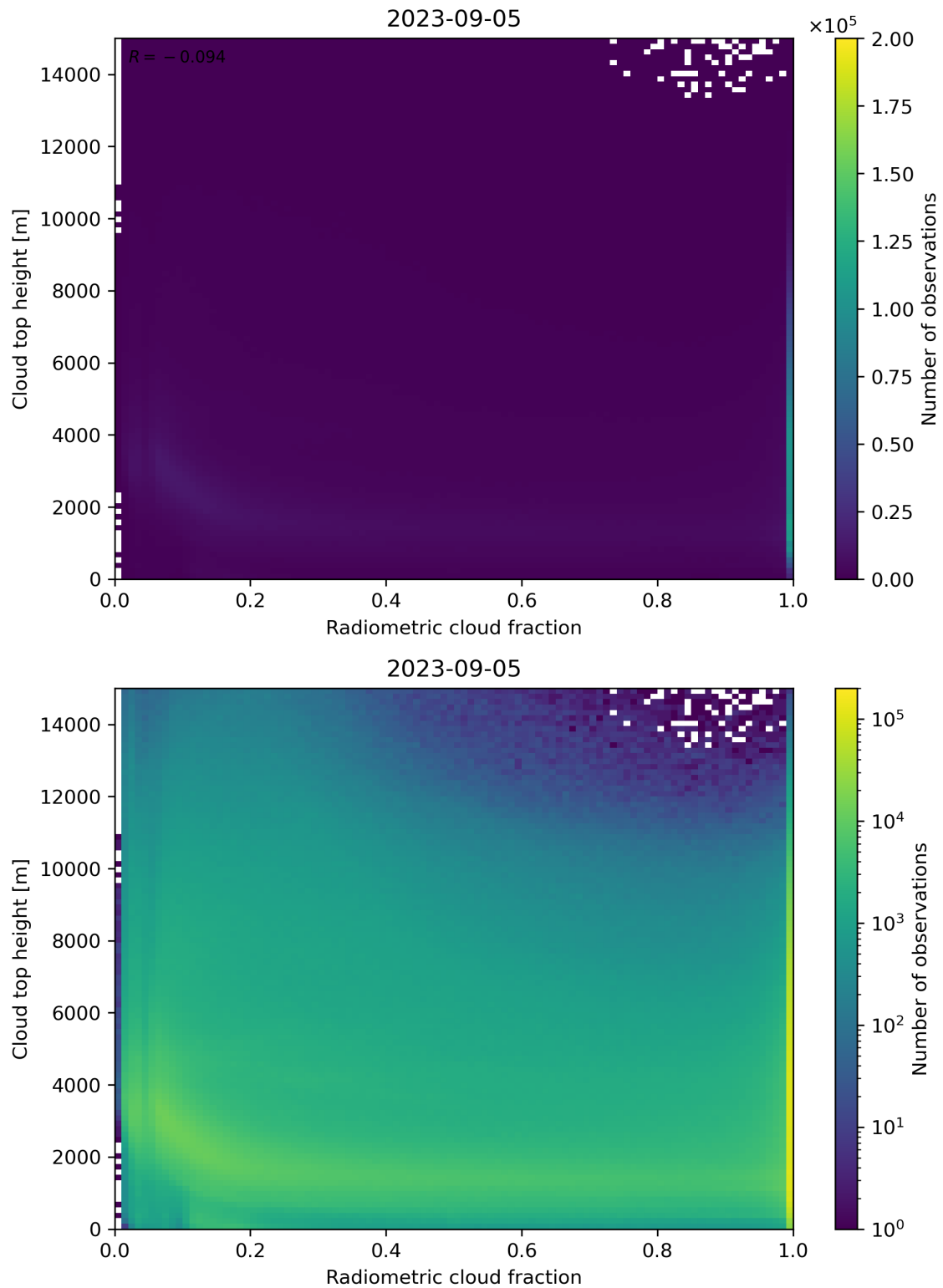
Figure 76: Scatter density plot of “Radiometric cloud fraction” against “Cloud top height” for 2023-09-05 to 2023-09-06.
