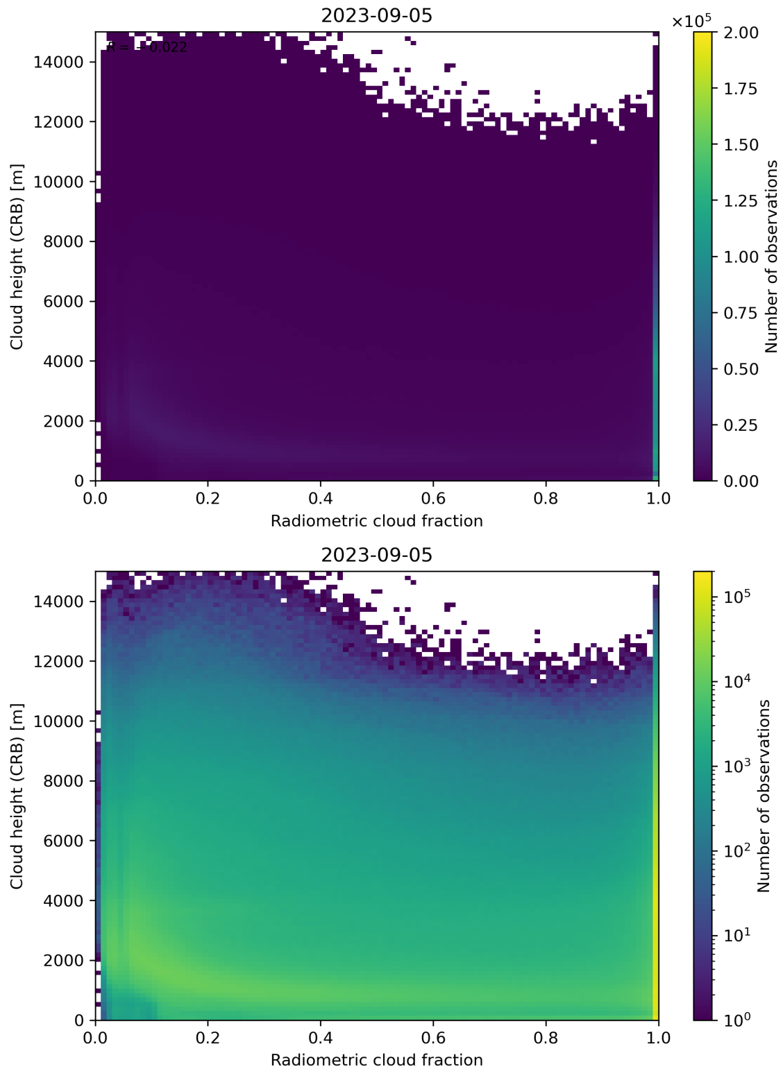
Figure 74: Scatter density plot of “Radiometric cloud fraction” against “Cloud height (CRB)” for 2023-09-05 to 2023-09-06.
