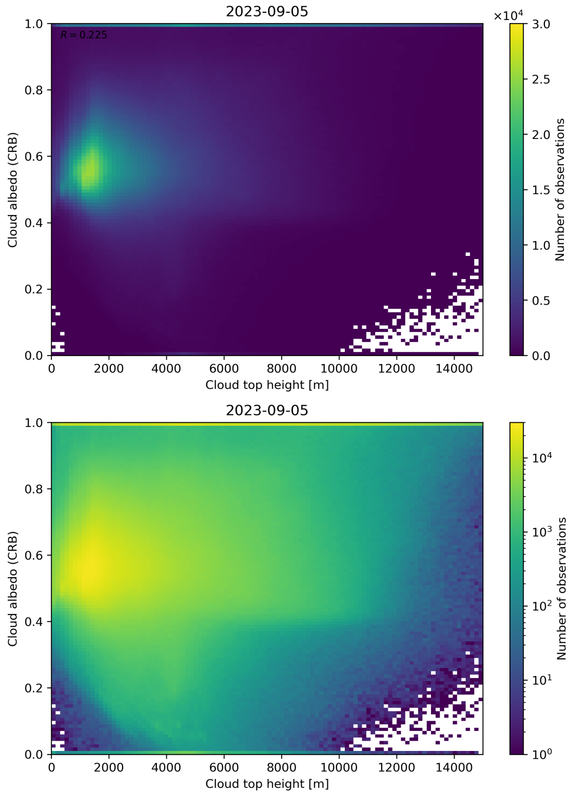
Figure 86: Scatter density plot of “Cloud top height” against “Cloud albedo (CRB)” for 2023-09-05 to 2023-09-06.
