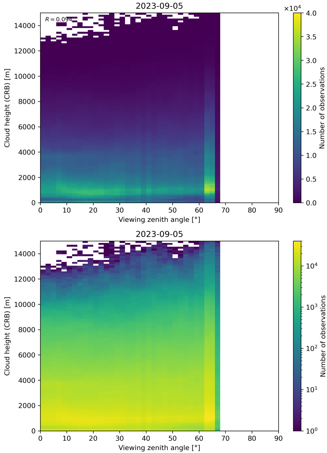
Figure 110: Scatter density plot of “Viewing zenith angle” against “Cloud height (CRB)” for 2023-09-05 to 2023-09-06.
