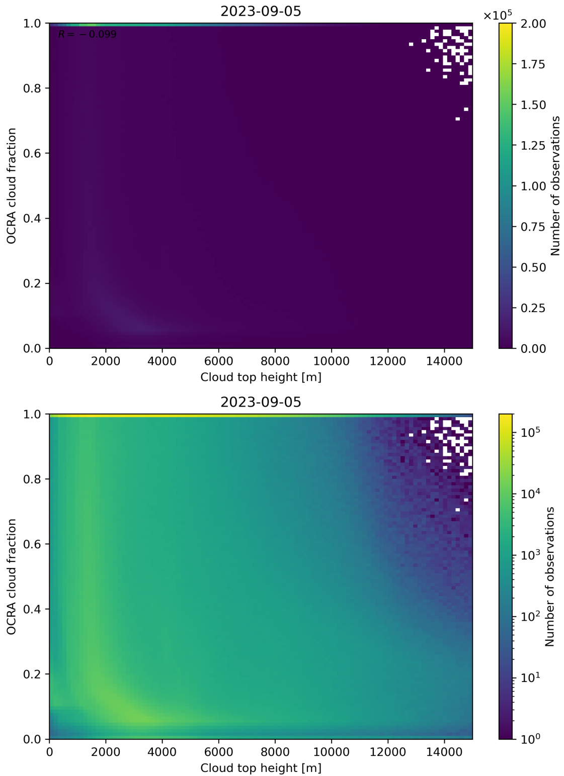
Figure 87: Scatter density plot of “Cloud top height” against “OCRA cloud fraction” for 2023-09-05 to 2023-09-06.
