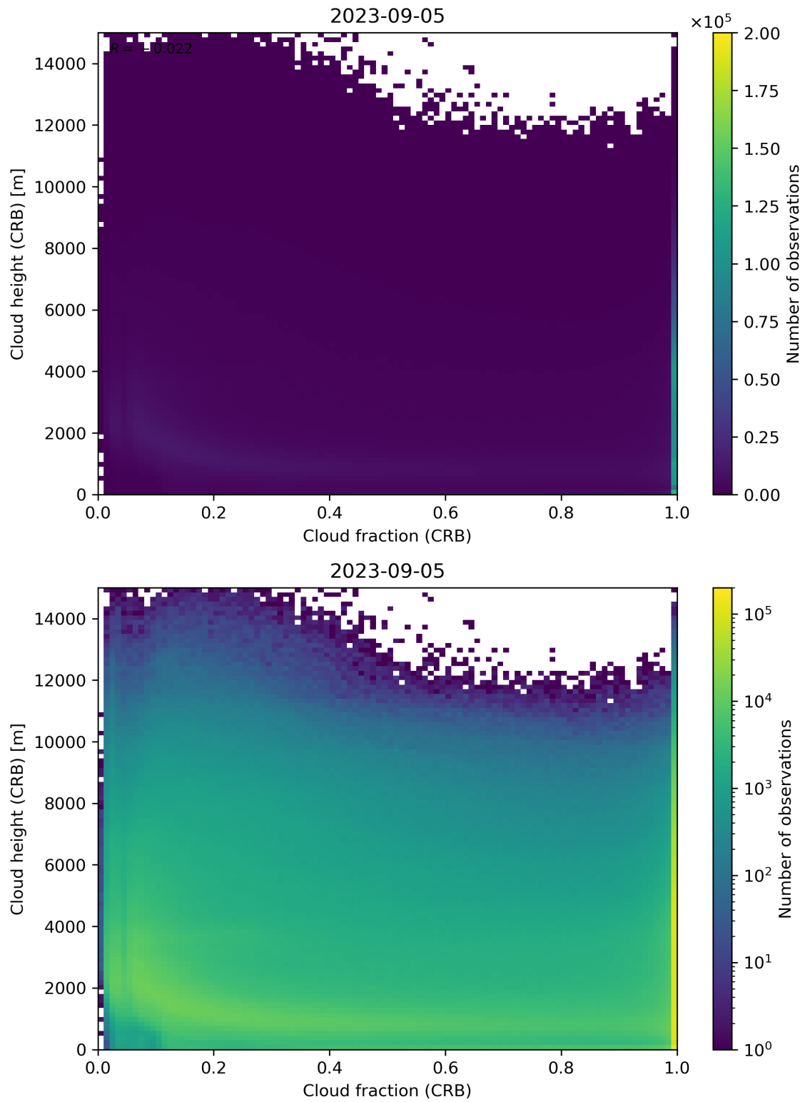
Figure 79: Scatter density plot of “Cloud fraction (CRB)” against “Cloud height (CRB)” for 2023-09-05 to 2023-09-06.
