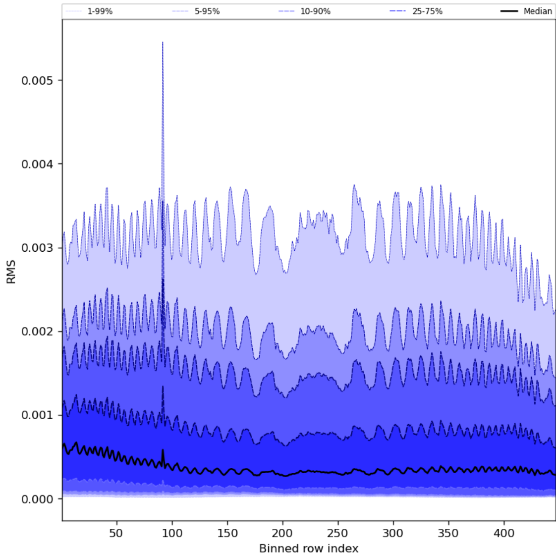
Figure 63: Along track statistics of “RMS” for 2023-09-05 to 2023-09-06
