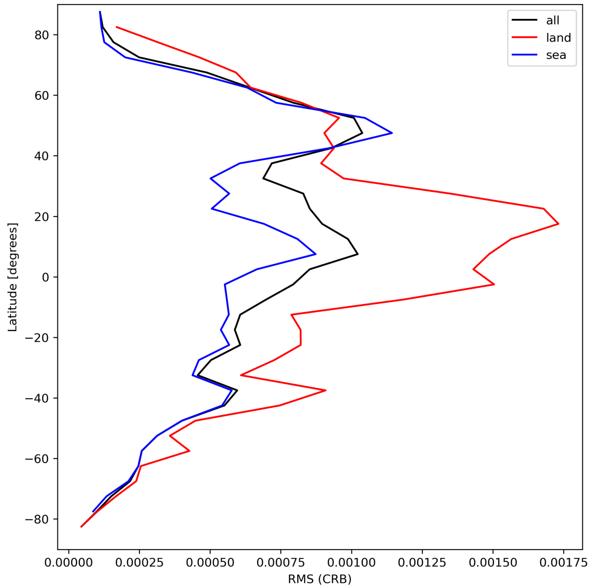
Figure 32: Zonal average of “RMS (CRB)” for 2023-09-05 to 2023-09-06.
