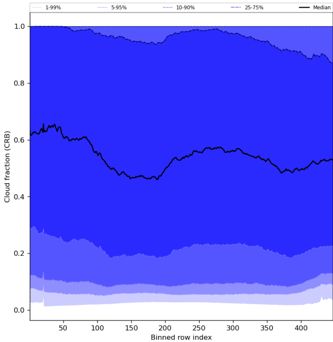
Figure 58: Along track statistics of “Cloud fraction (CRB)” for 2023-09-05 to 2023-09-06
