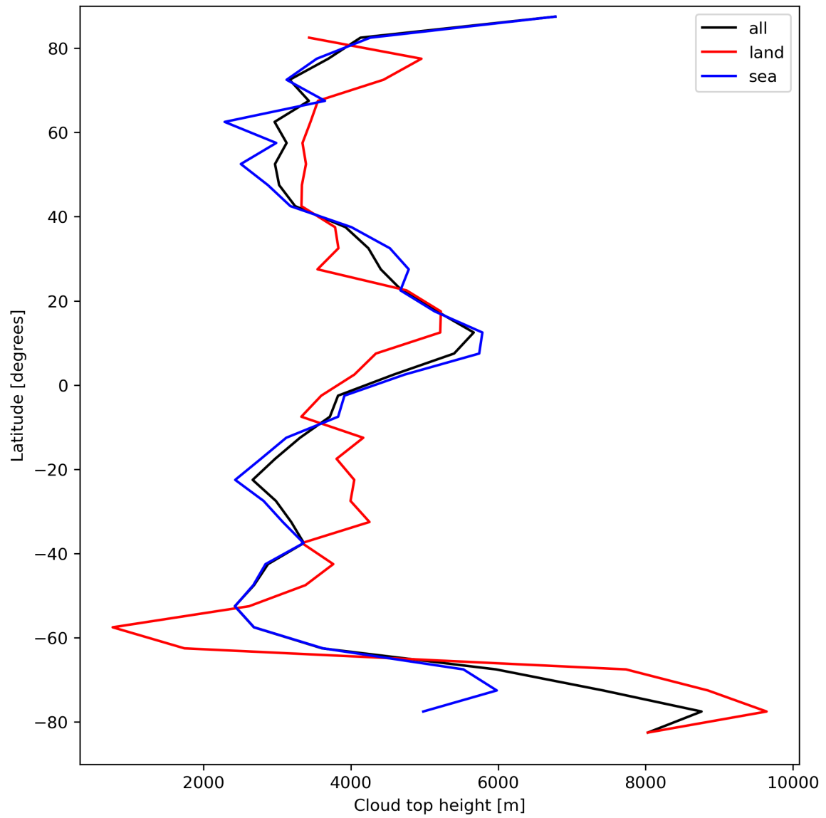
Figure 24: Zonal average of “Cloud top height” for 2023-09-05 to 2023-09-06.
