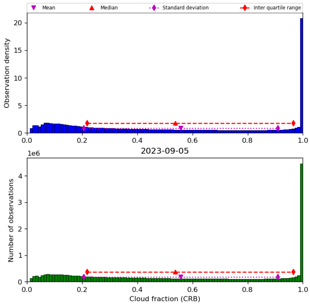
Figure 42: Histogram of “Cloud fraction (CRB)” for 2023-09-05 to 2023-09-06
