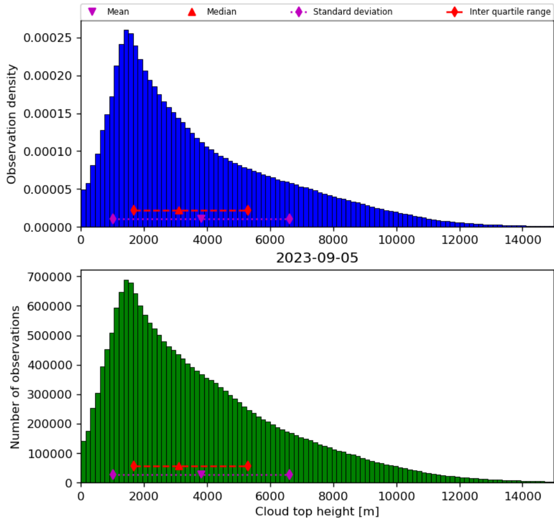
Figure 40: Histogram of “Cloud top height” for 2023-09-05 to 2023-09-06
