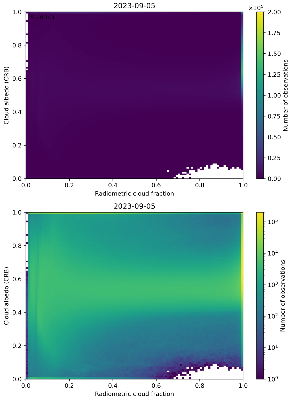
Figure 71: Scatter density plot of “Radiometric cloud fraction” against “Cloud albedo (CRB)” for 2023-09-05 to 2023-09-06.
