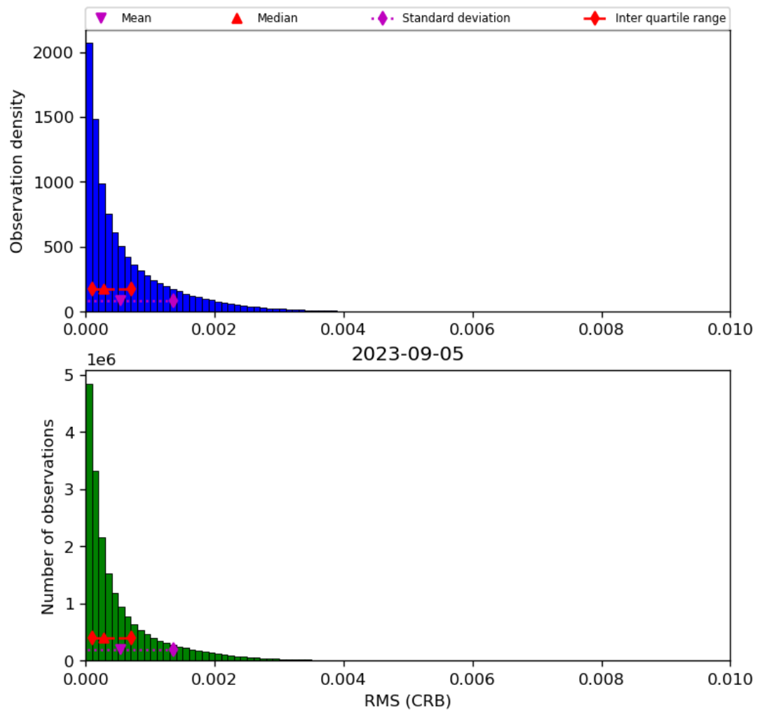
Figure 48: Histogram of "RMS (CRB)" for 2023-09-05 to 2023-09-06
