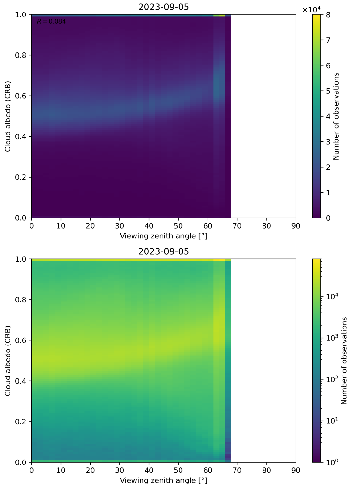
Figure 106: Scatter density plot of “Viewing zenith angle” against “Cloud albedo (CRB)” for 2023-09-05 to 2023-09-06.
