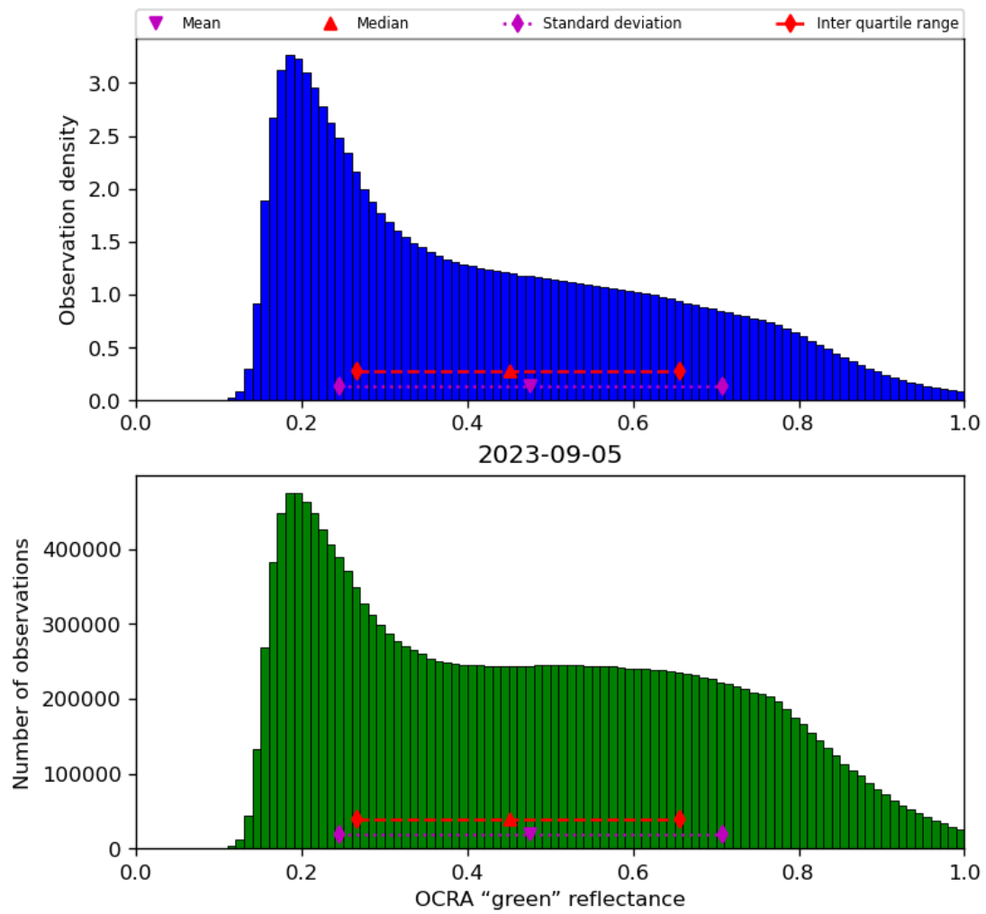
Figure 52: Histogram of “OCRA “green” reflectance” for 2023-09-05 to 2023-09-06
