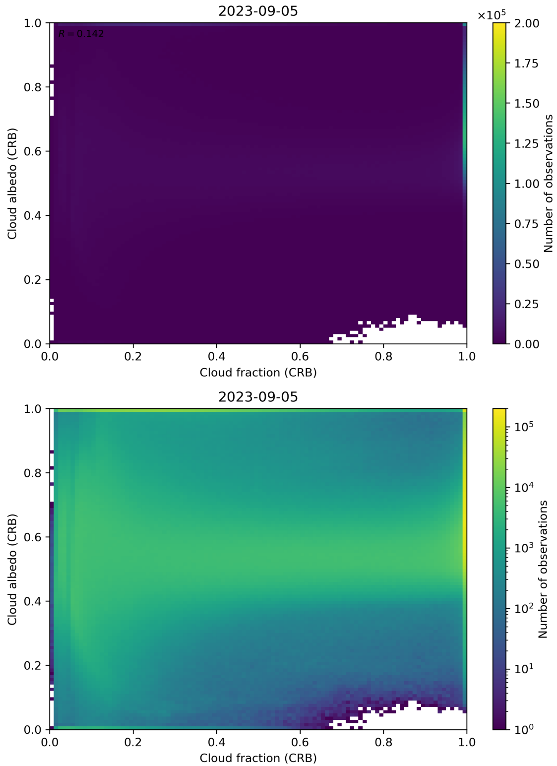
Figure 77: Scatter density plot of “Cloud fraction (CRB)” against “Cloud albedo (CRB)” for 2023-09-05 to 2023-09-06.
