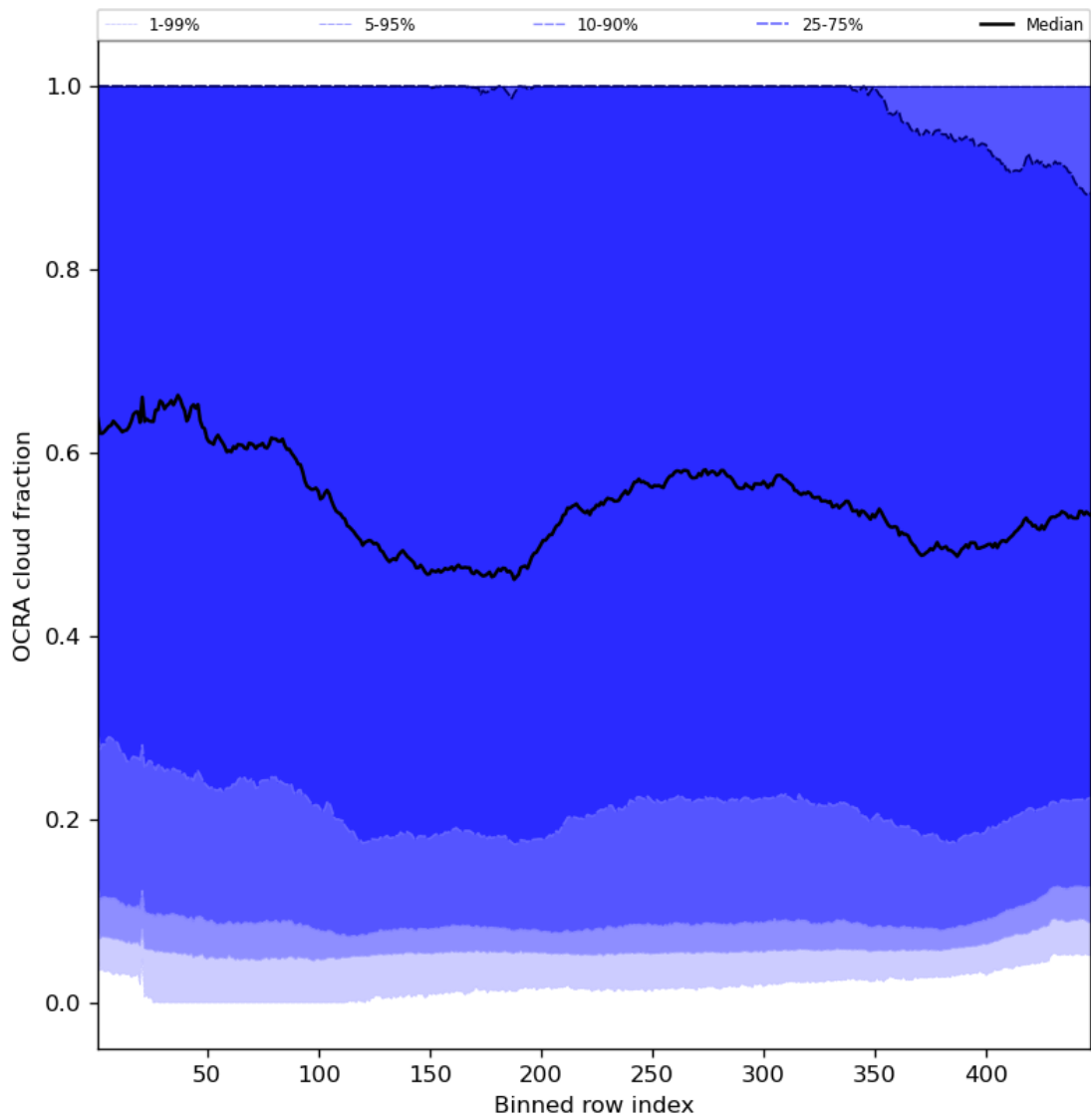
Figure 66: Along track statistics of “OCRA cloud fraction” for 2023-09-05 to 2023-09-06
