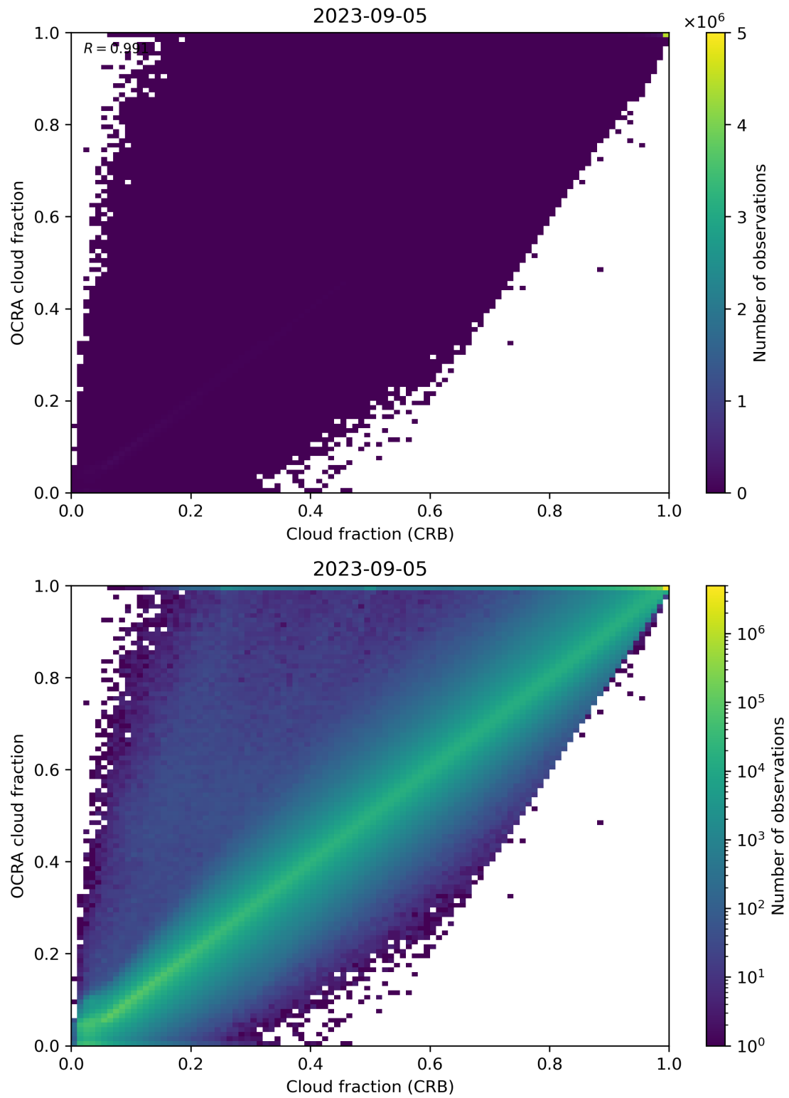
Figure 78: Scatter density plot of “Cloud fraction (CRB)” against “OCRA cloud fraction” for 2023-09-05 to 2023-09-06.
