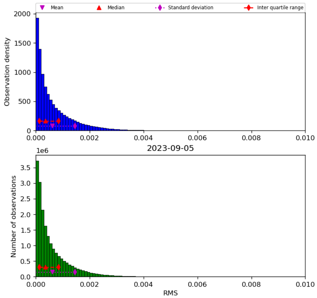
Figure 47: Histogram of “RMS” for 2023-09-05 to 2023-09-06
