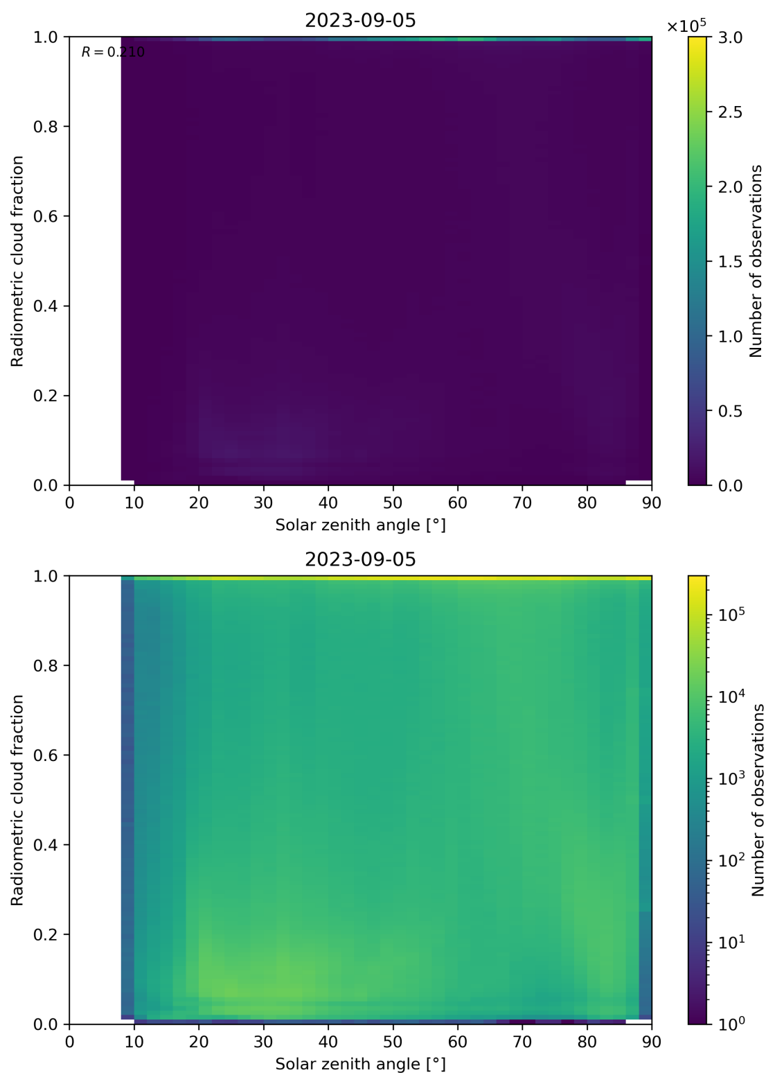
Figure 99: Scatter density plot of “Solar zenith angle” against “Radiometric cloud fraction” for 2023-09-05 to 2023-09-06.
