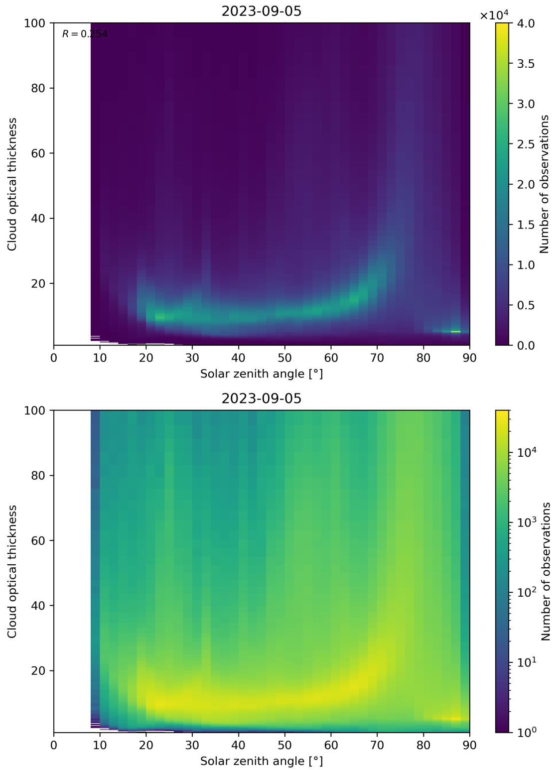
Figure 103: Scatter density plot of “Solar zenith angle” against “Cloud optical thickness” for 2023-09-05 to 2023-09-06.
