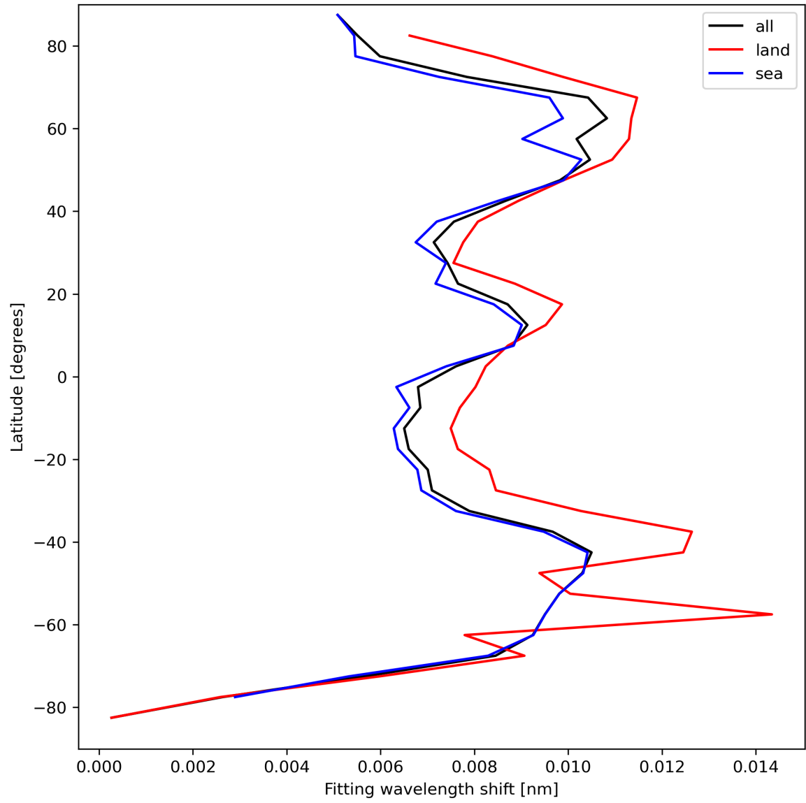
Figure 33: Zonal average of “Fitting wavelength shift” for 2023-09-05 to 2023-09-06.
