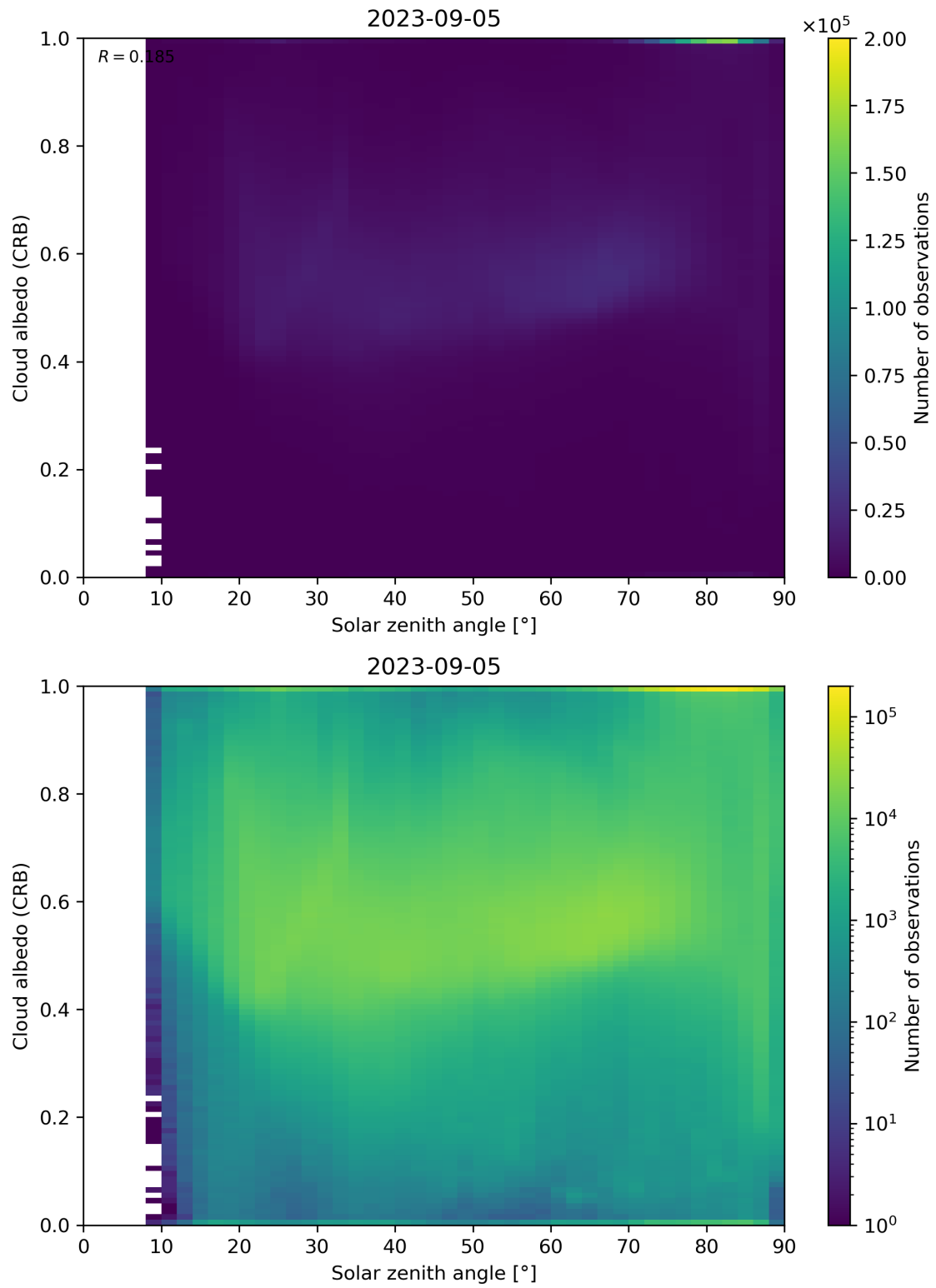
Figure 98: Scatter density plot of “Solar zenith angle” against “Cloud albedo (CRB)” for 2023-09-05 to 2023-09-06.
