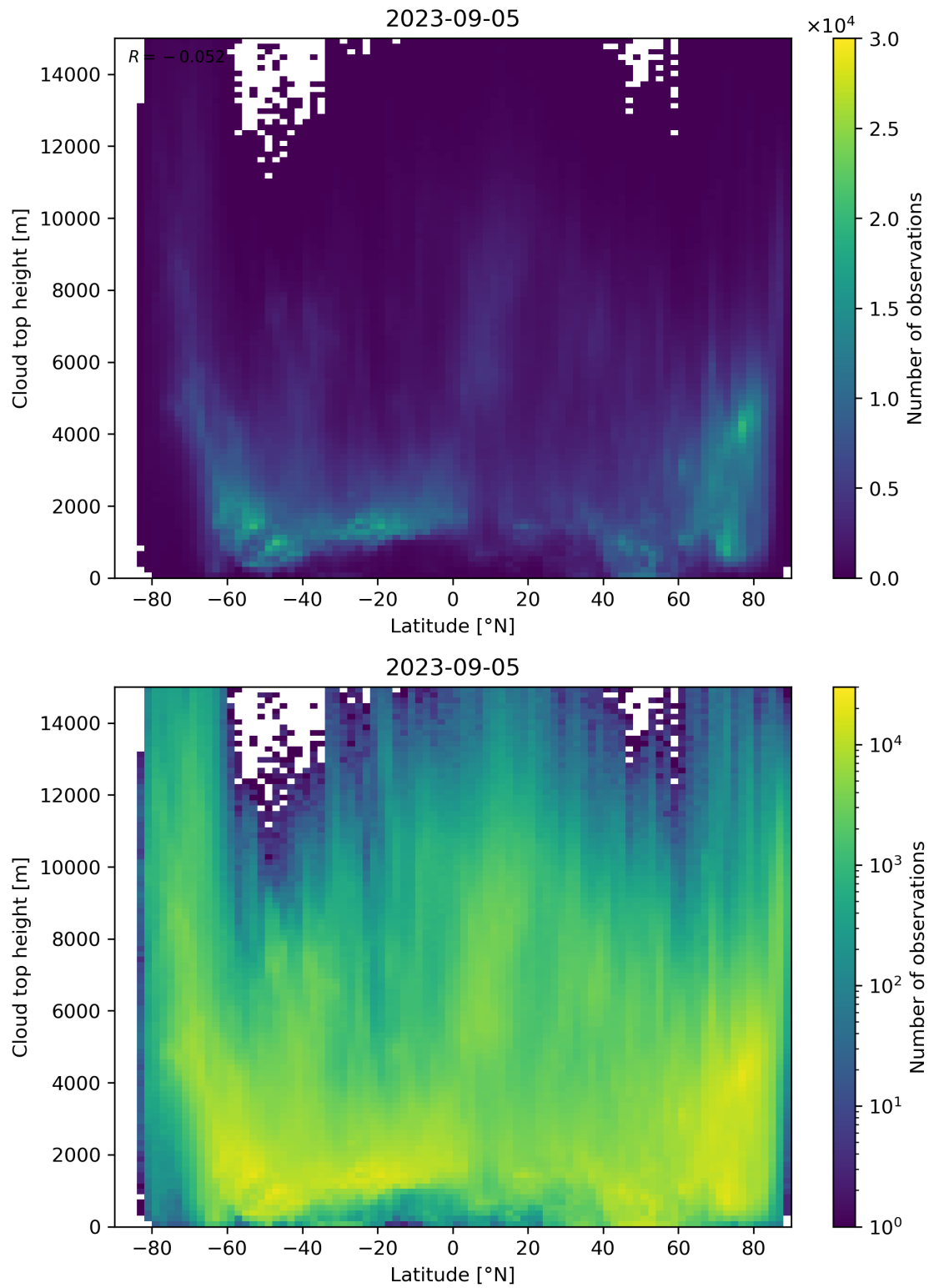
Figure 97: Scatter density plot of “Latitude” against “Cloud top height” for 2023-09-05 to 2023-09-06.
