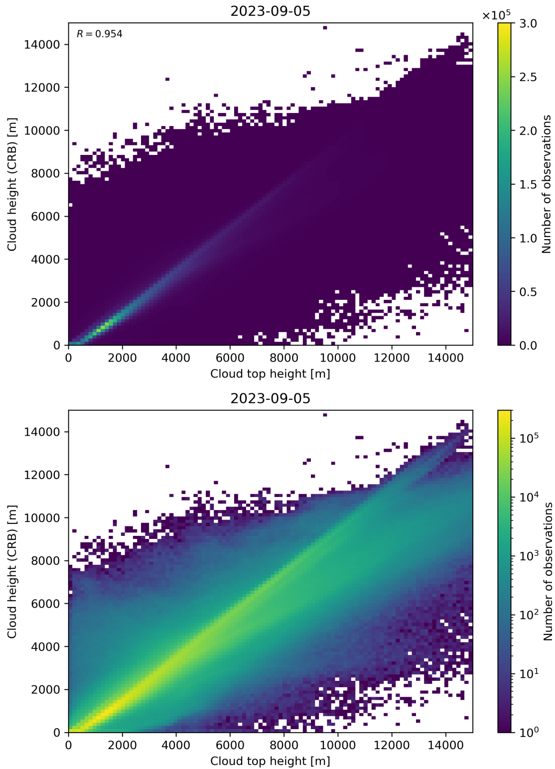
Figure 89: Scatter density plot of “Cloud top height” against “Cloud height (CRB)” for 2023-09-05 to 2023-09-06.
