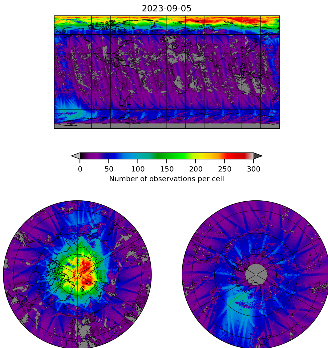
Figure 21: Map of the number of observations for 2023-09-05 to 2023-09-06
