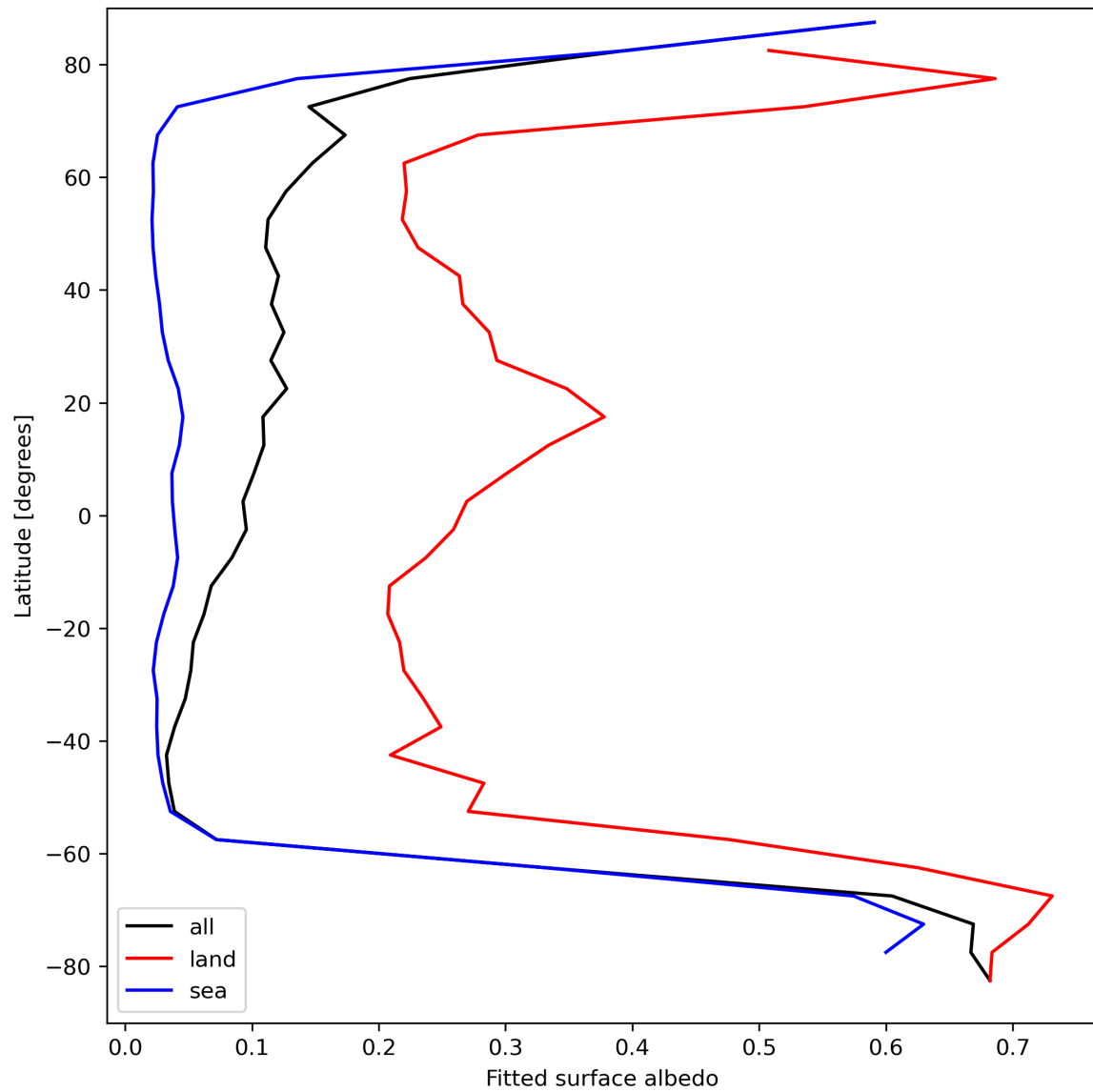
Figure 29: Zonal average of “Fitted surface albedo” for 2023-09-05 to 2023-09-06.
