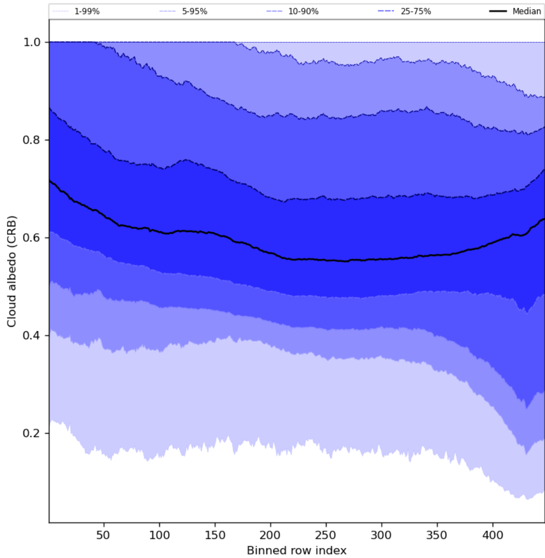
Figure 60: Along track statistics of “Cloud albedo (CRB)” for 2023-09-05 to 2023-09-06
