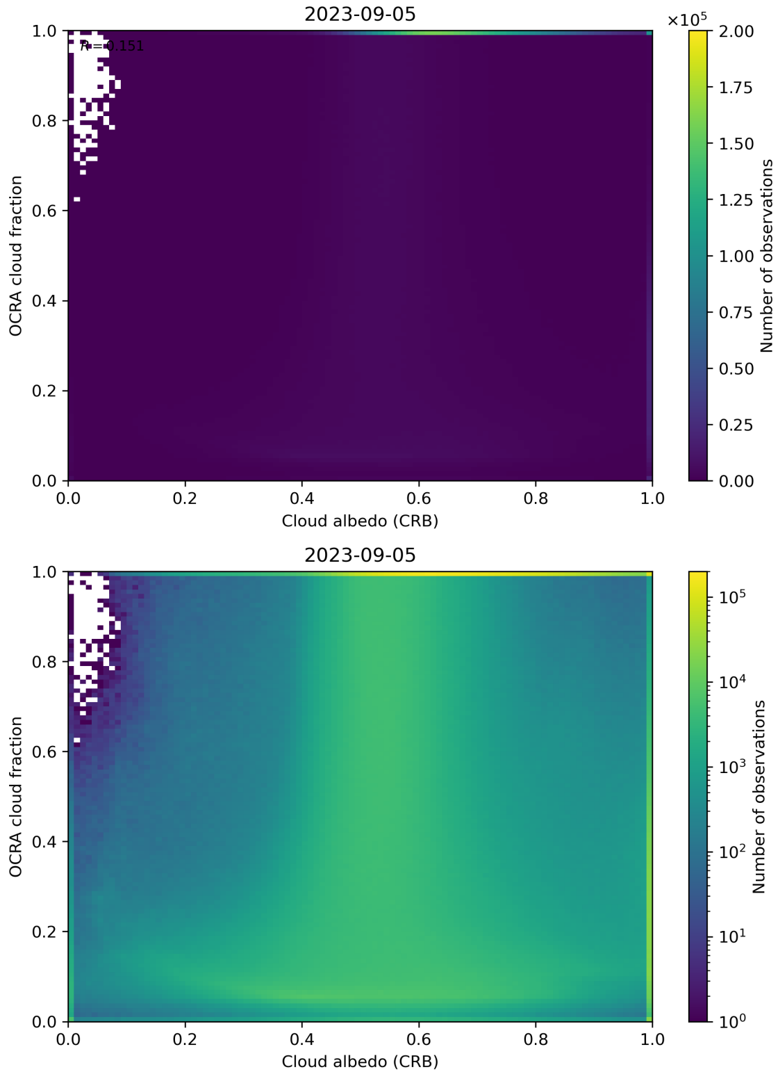
Figure 70: Scatter density plot of “Cloud albedo (CRB)” against “OCRA cloud fraction” for 2023-09-05 to 2023-09-06.
