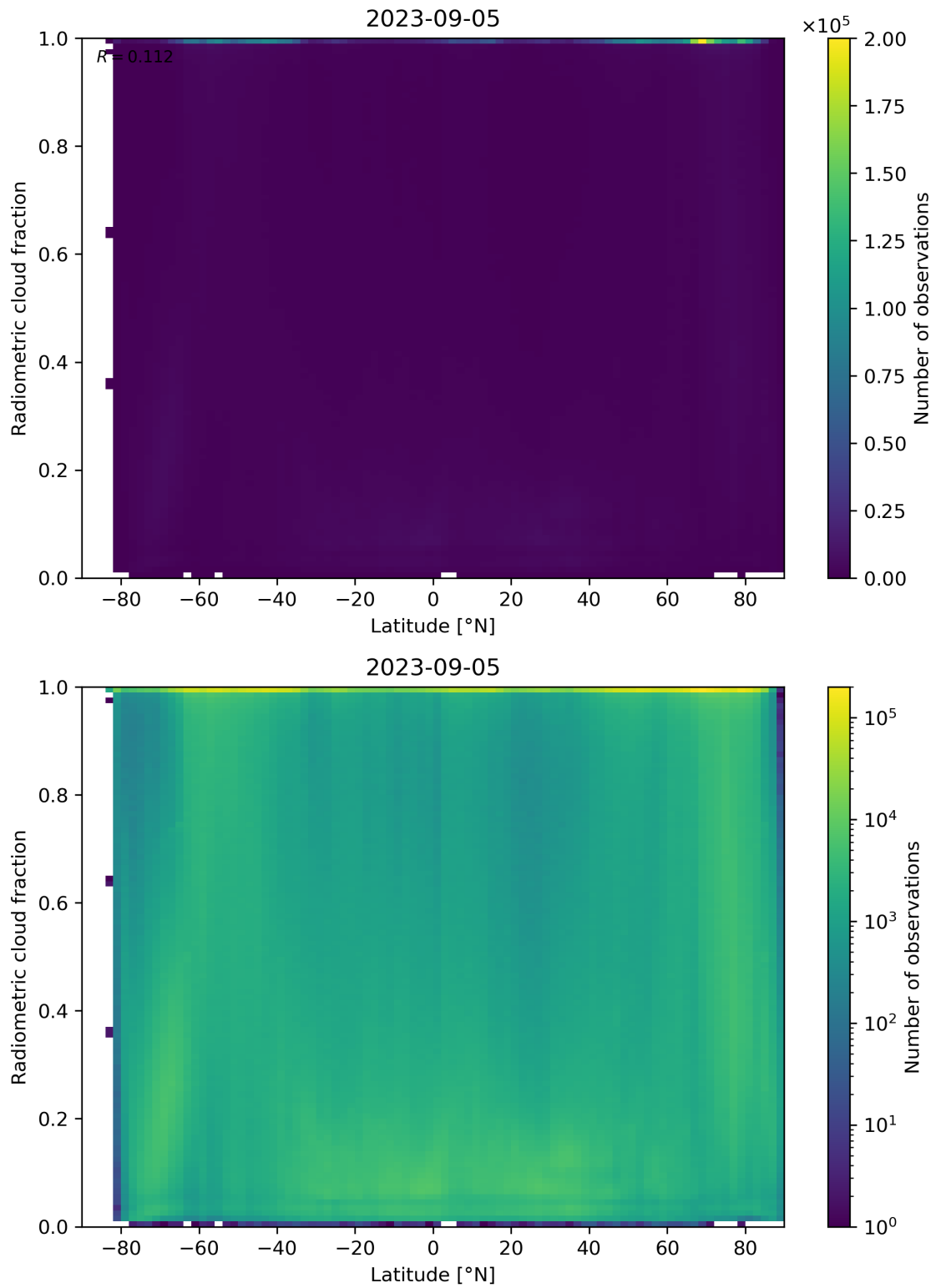
Figure 92: Scatter density plot of “Latitude” against “Radiometric cloud fraction” for 2023-09-05 to 2023-09-06.
