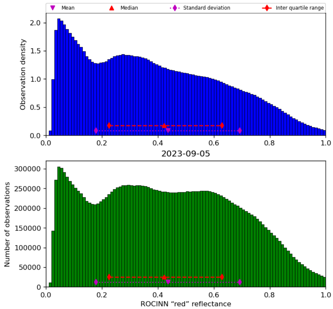
Figure 53: Histogram of “ROCINN “red” reflectance” for 2023-09-05 to 2023-09-06
