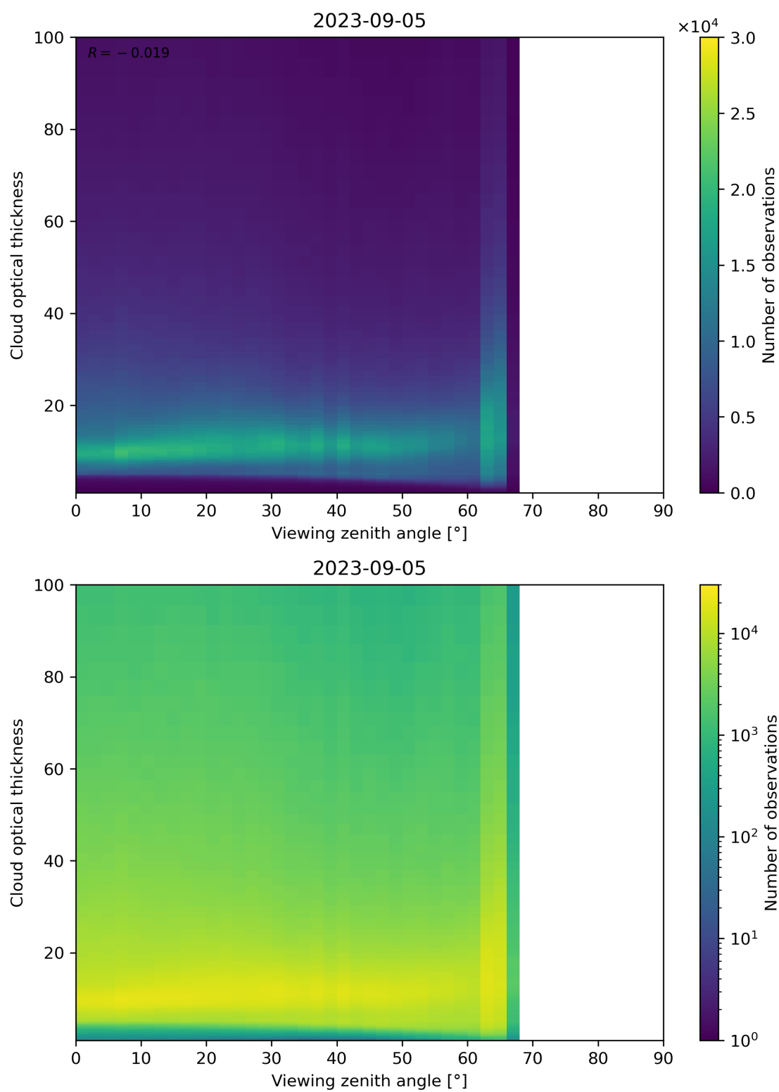
Figure 111: Scatter density plot of “Viewing zenith angle” against “Cloud optical thickness” for 2023-09-05 to 2023-09-06.
