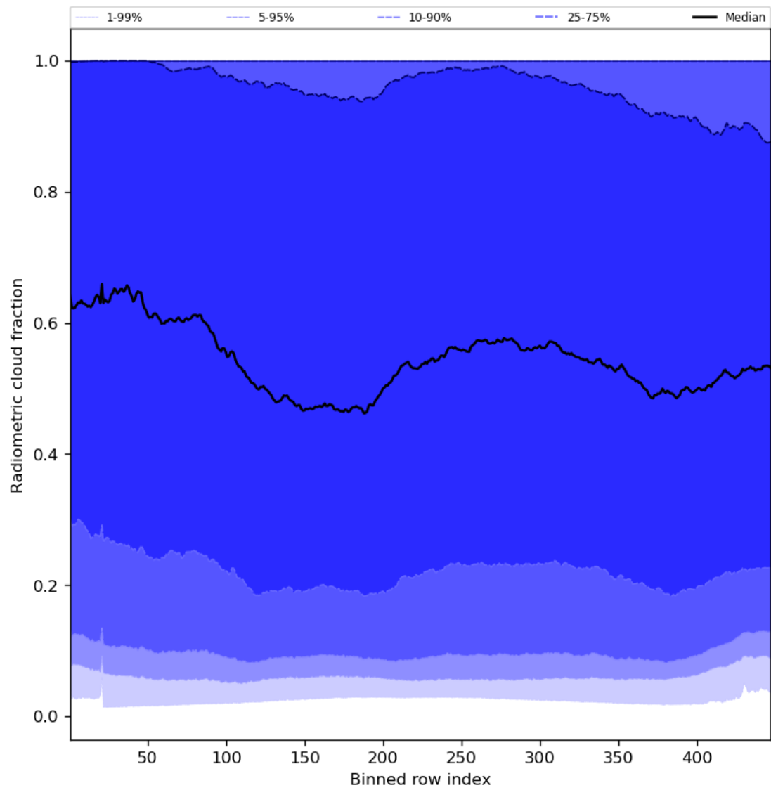
Figure 55: Along track statistics of “Radiometric cloud fraction” for 2023-09-05 to 2023-09-06
