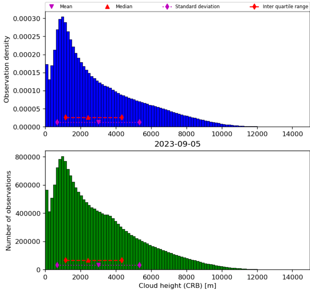
Figure 43: Histogram of “Cloud height (CRB)” for 2023-09-05 to 2023-09-06
