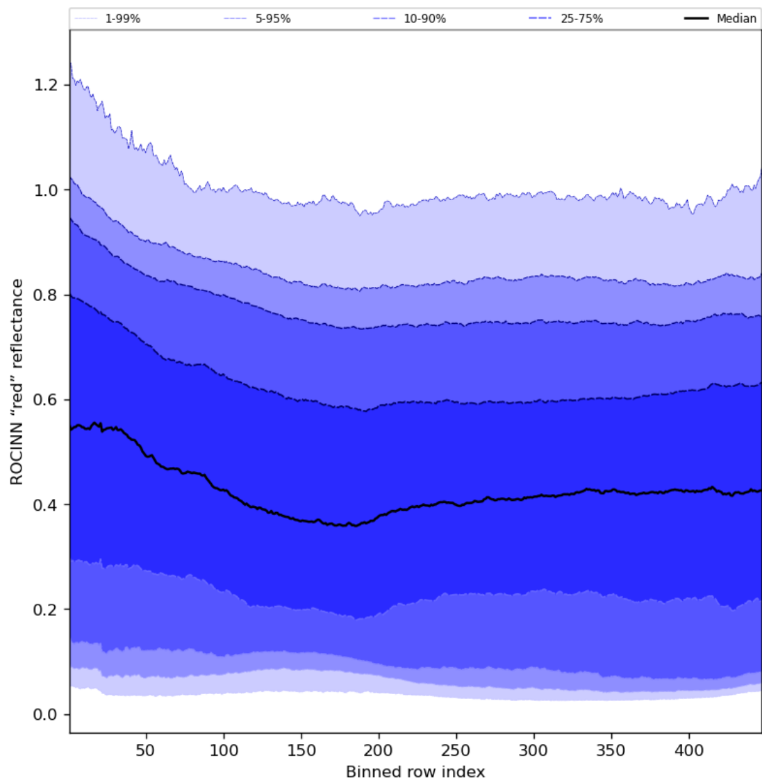
Figure 69: Along track statistics of “ROCINN “red” reflectance” for 2023-09-05 to 2023-09-06
