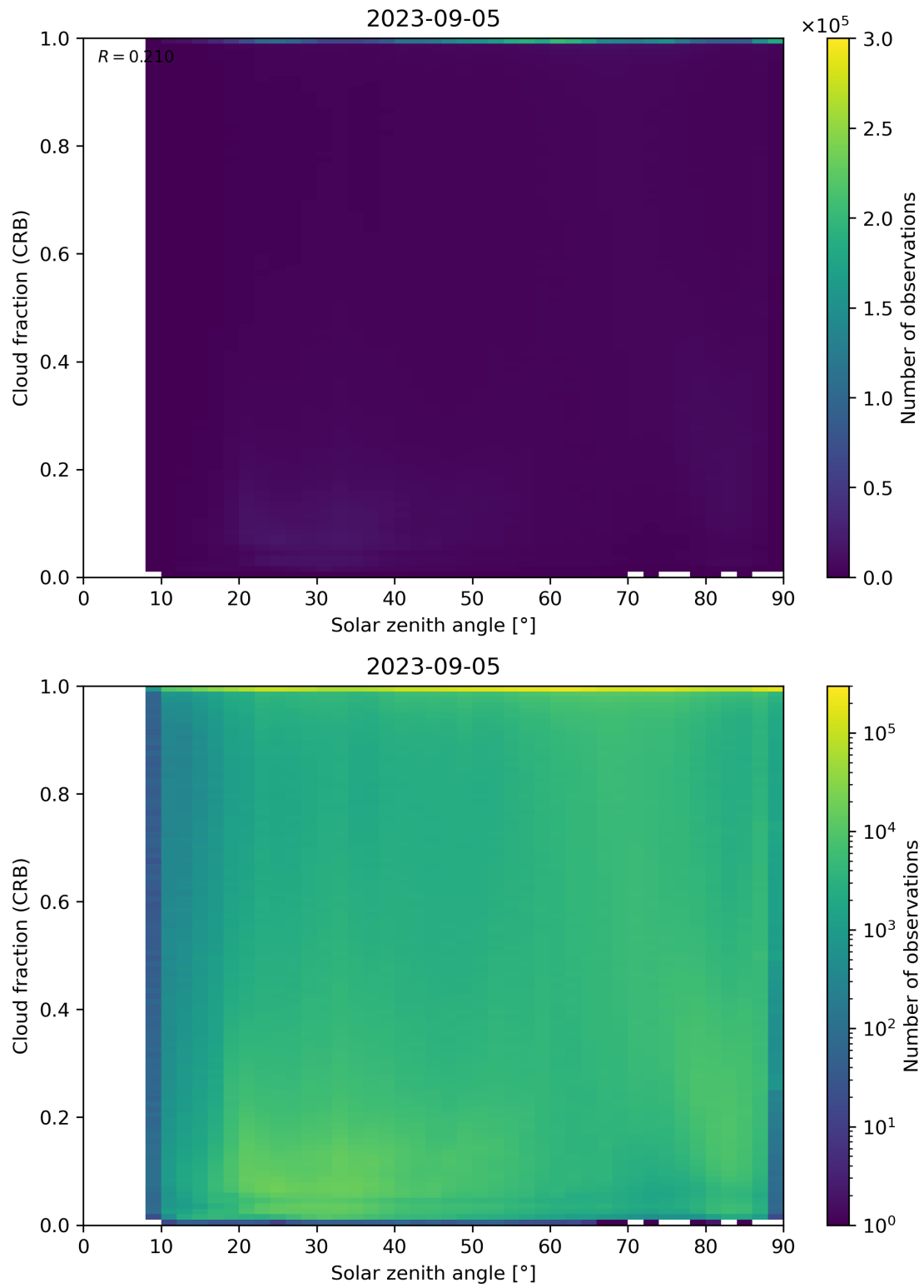
Figure 101: Scatter density plot of “Solar zenith angle” against “Cloud fraction (CRB)” for 2023-09-05 to 2023-09-06.
