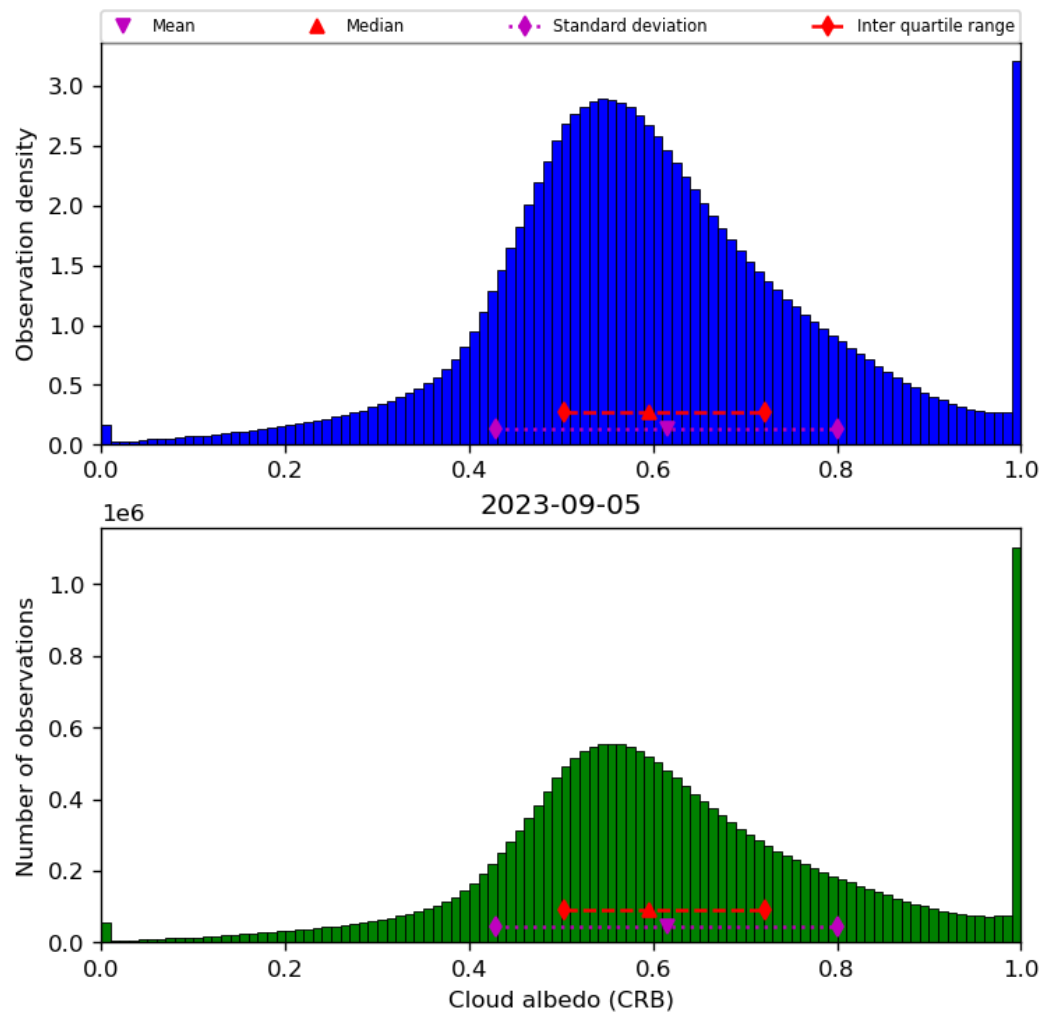
Figure 44: Histogram of “Cloud albedo (CRB)” for 2023-09-05 to 2023-09-06
