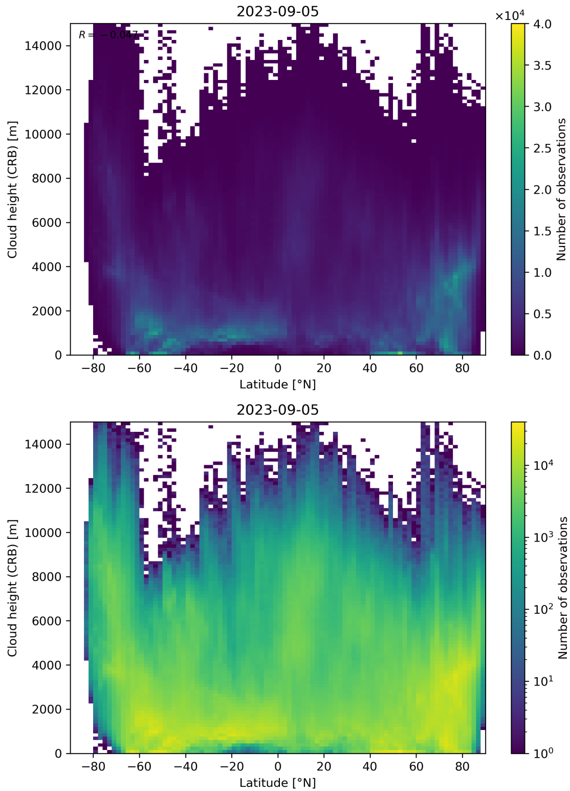
Figure 95: Scatter density plot of “Latitude” against “Cloud height (CRB)” for 2023-09-05 to 2023-09-06.
