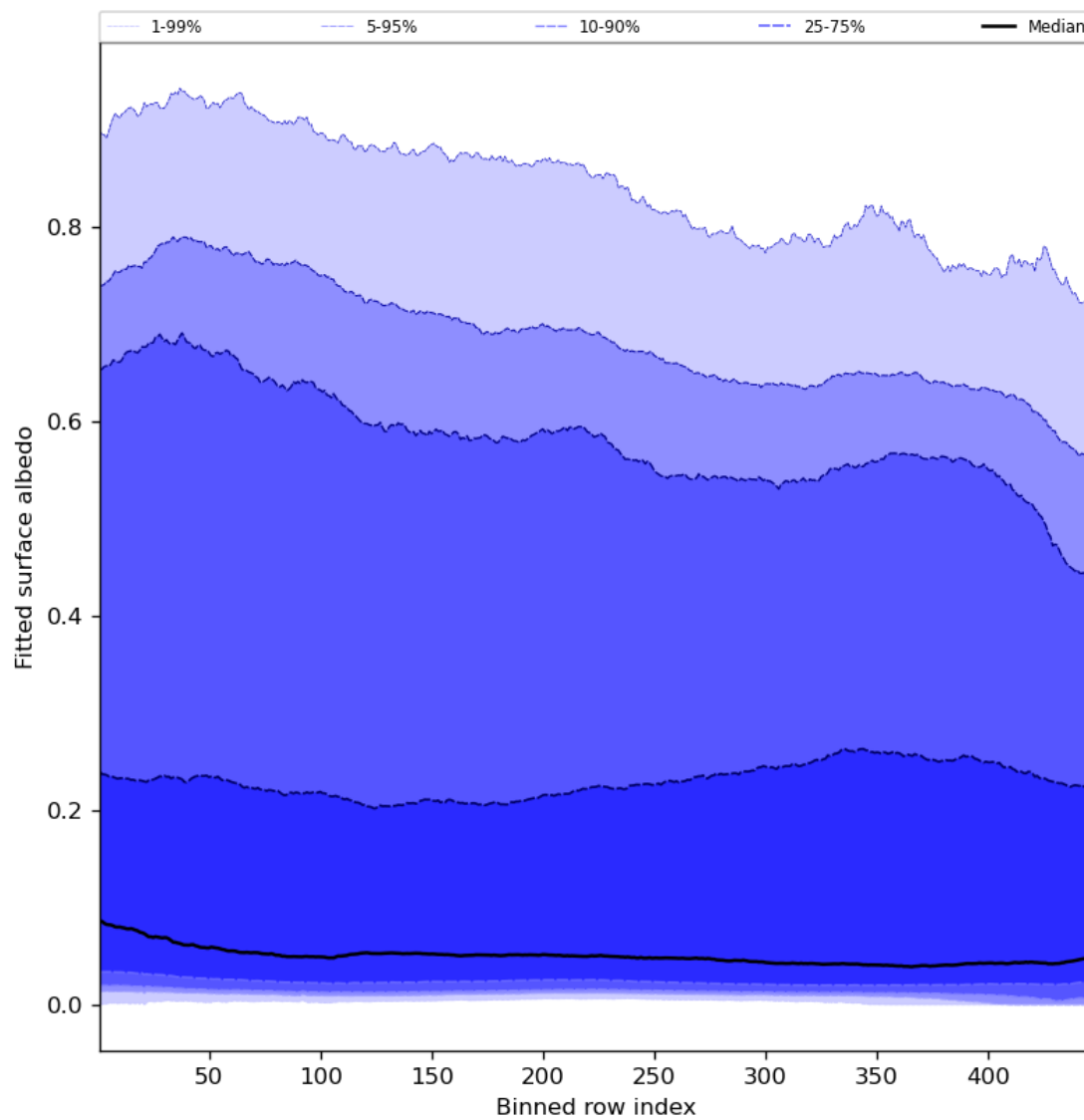
Figure 61: Along track statistics of “Fitted surface albedo” for 2023-09-05 to 2023-09-06
