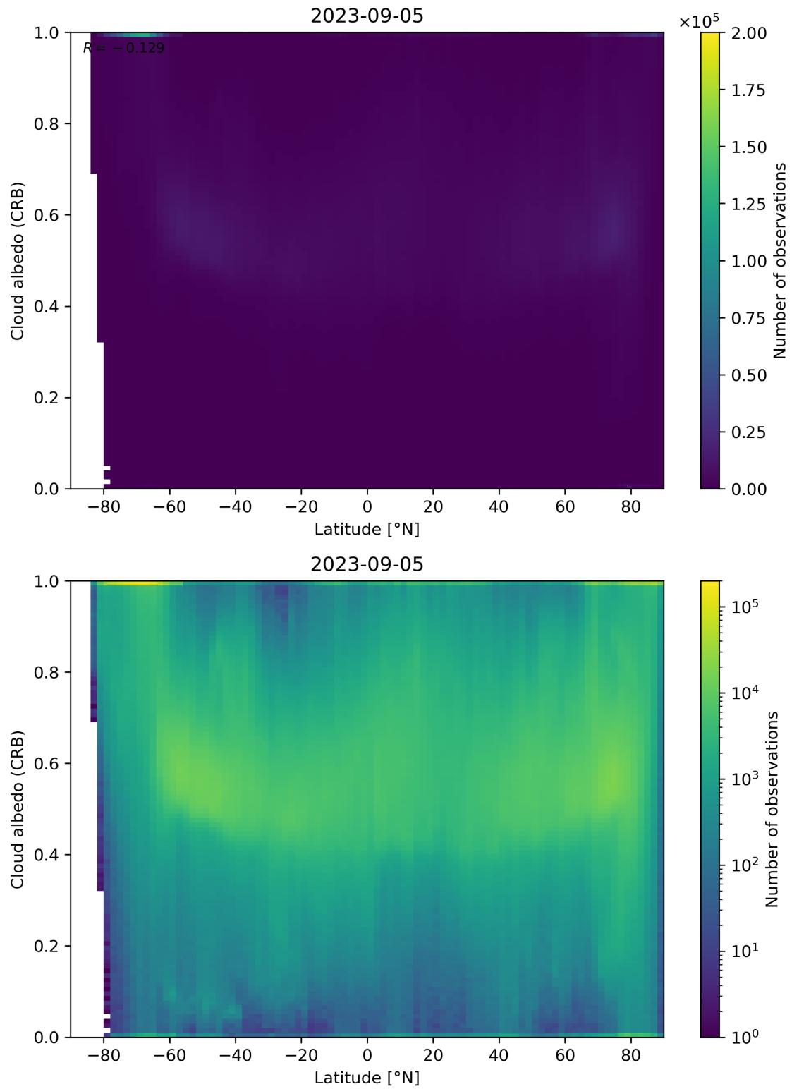
Figure 91: Scatter density plot of “Latitude” against “Cloud albedo (CRB)” for 2023-09-05 to 2023-09-06.
