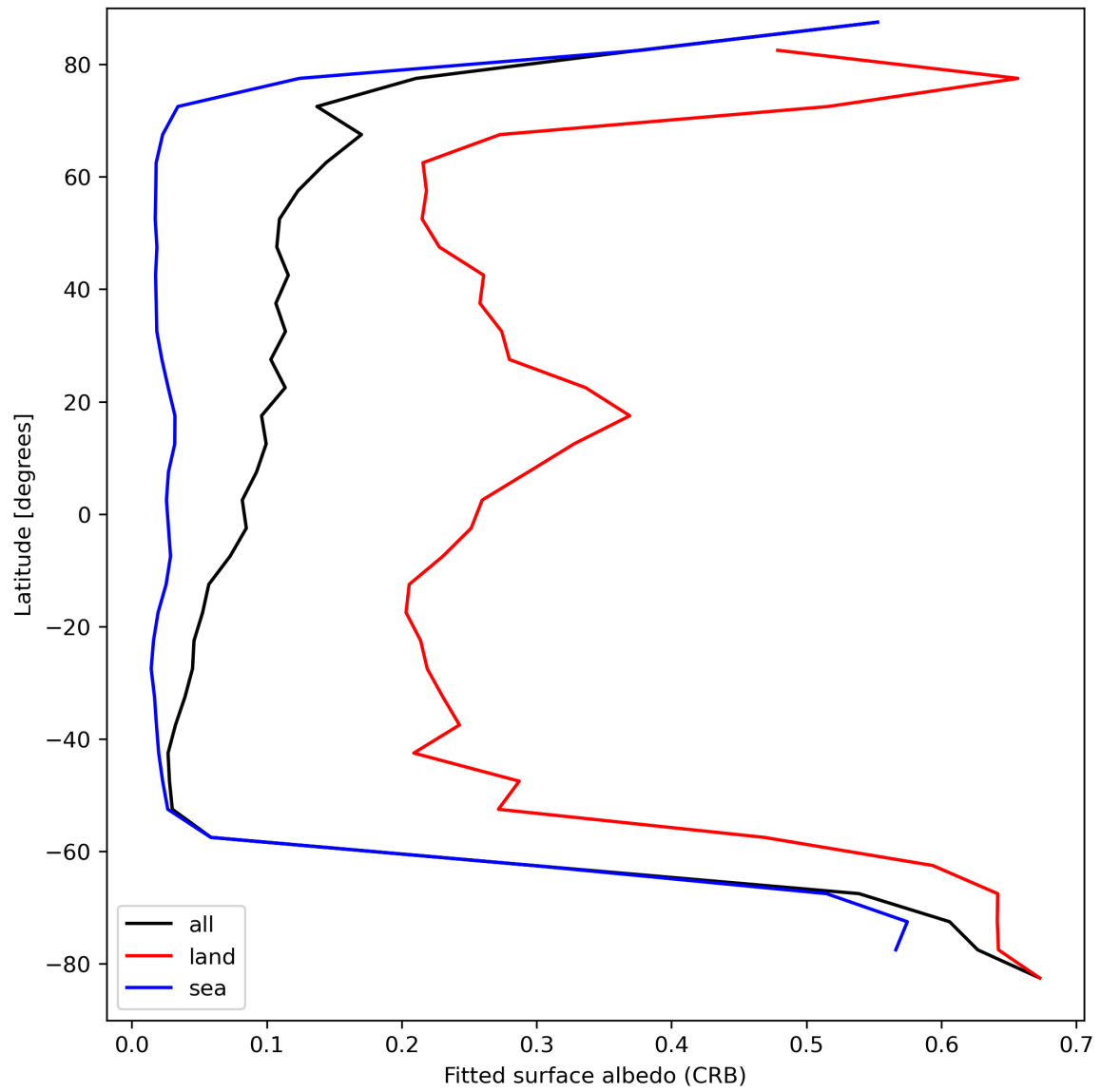
Figure 30: Zonal average of “Fitted surface albedo (CRB)” for 2023-09-05 to 2023-09-06.
