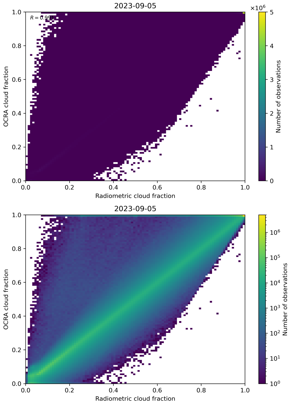
Figure 72: Scatter density plot of “Radiometric cloud fraction” against “OCRA cloud fraction” for 2023-09-05 to 2023-09-06.
