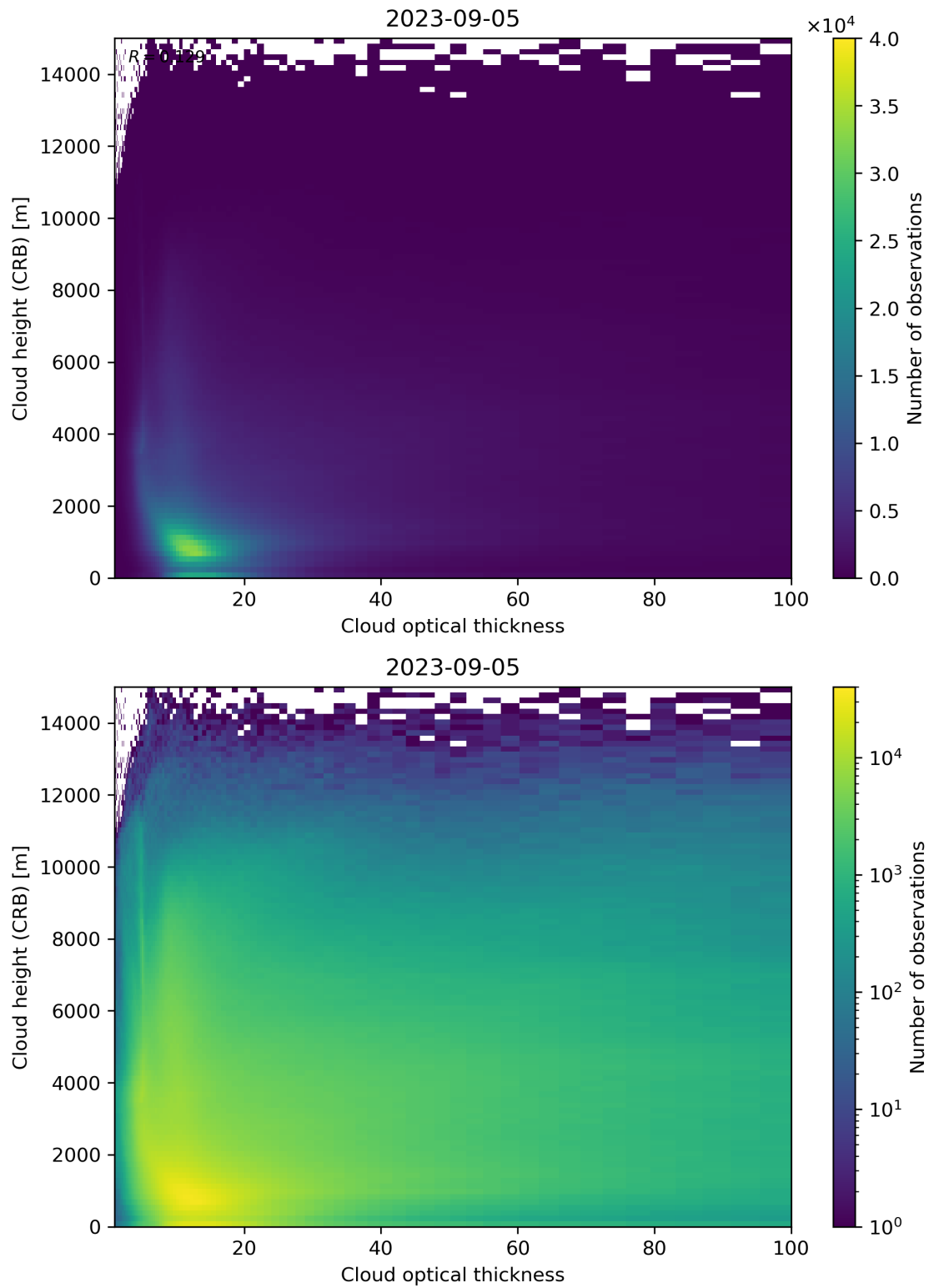
Figure 85: Scatter density plot of “Cloud optical thickness” against “Cloud height (CRB)” for 2023-09-05 to 2023-09-06.
