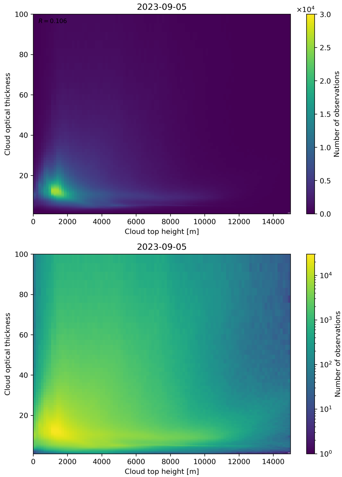
Figure 90: Scatter density plot of “Cloud top height” against “Cloud optical thickness” for 2023-09-05 to 2023-09-06.
