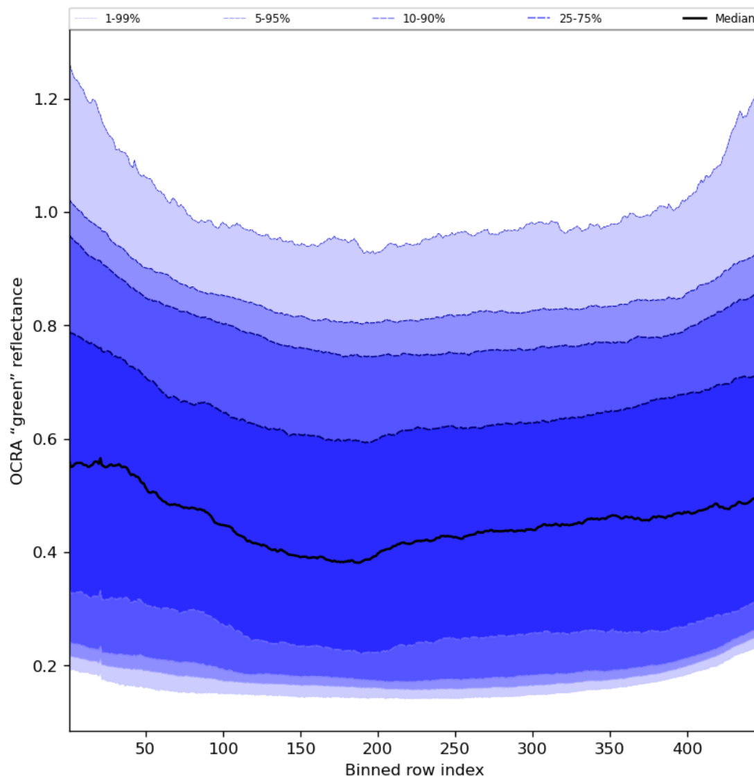
Figure 68: Along track statistics of “OCRA “green” reflectance” for 2023-09-05 to 2023-09-06
