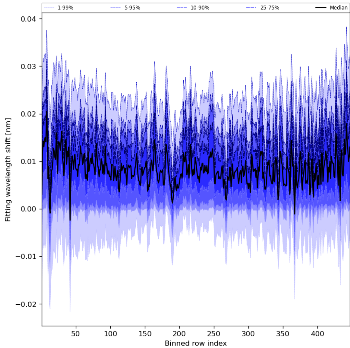
Figure 65: Along track statistics of “Fitting wavelength shift” for 2023-09-05 to 2023-09-06
