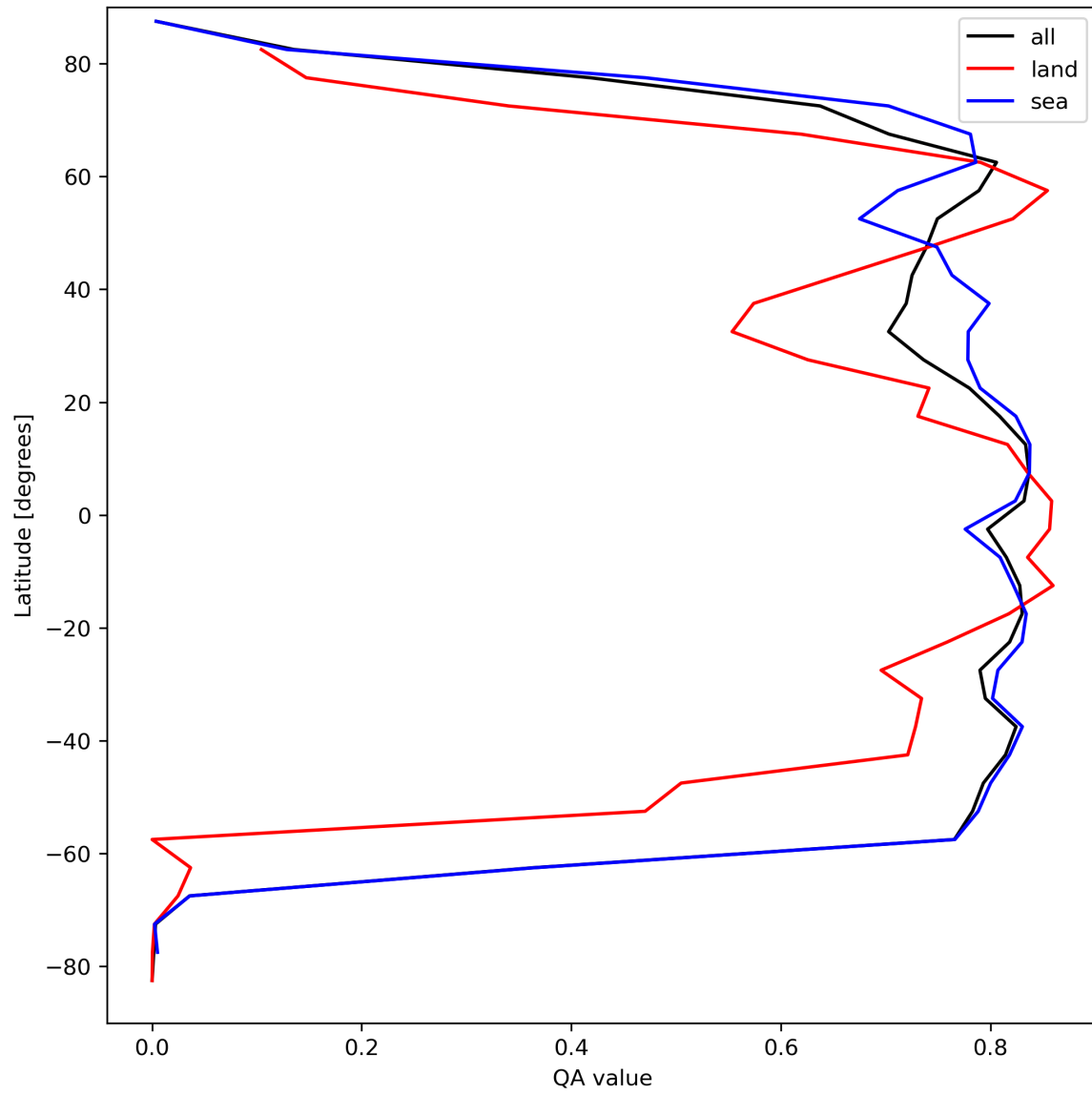
Figure 22: Zonal average of “QA value” for 2023-09-05 to 2023-09-06.
