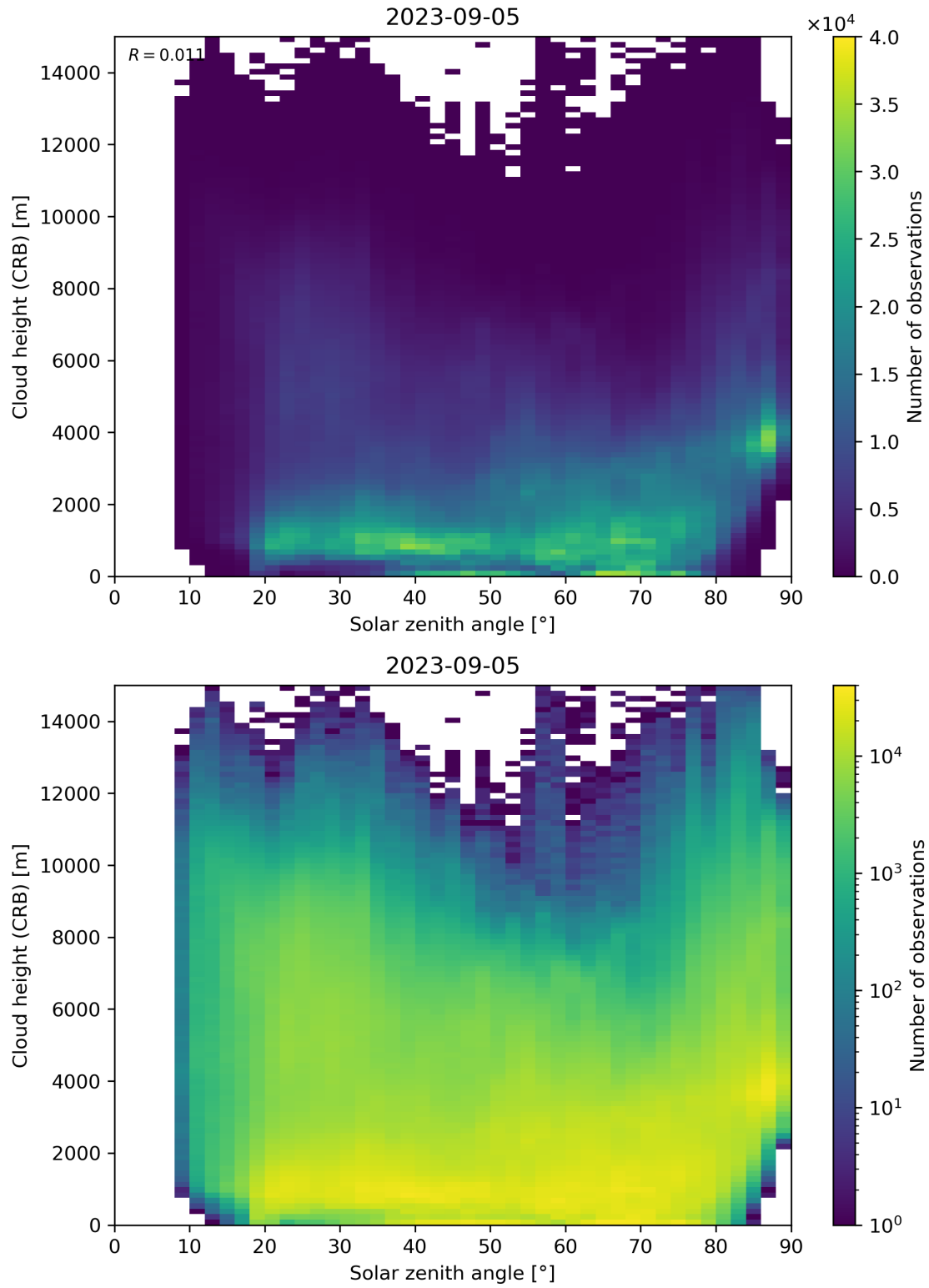
Figure 102: Scatter density plot of “Solar zenith angle” against “Cloud height (CRB)” for 2023-09-05 to 2023-09-06.
