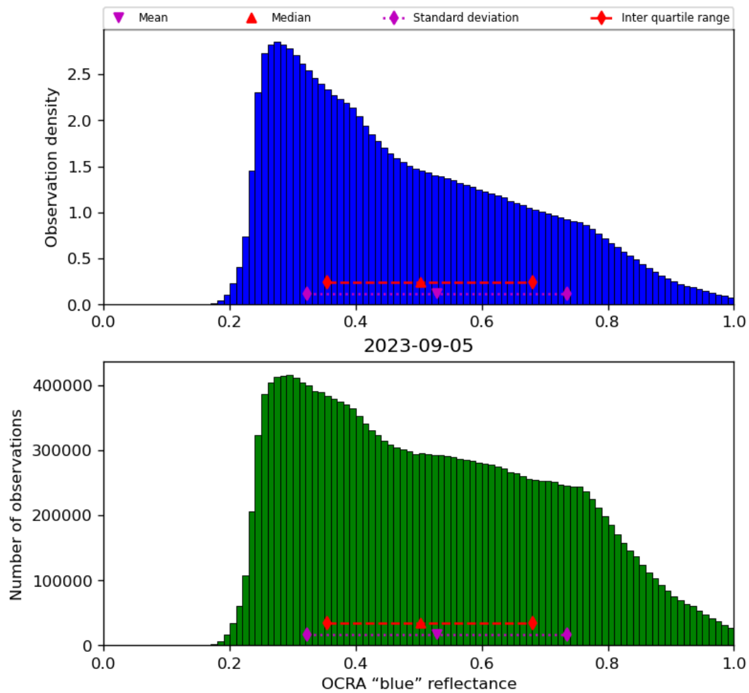
Figure 51: Histogram of “OCRA “blue” reflectance” for 2023-09-05 to 2023-09-06
