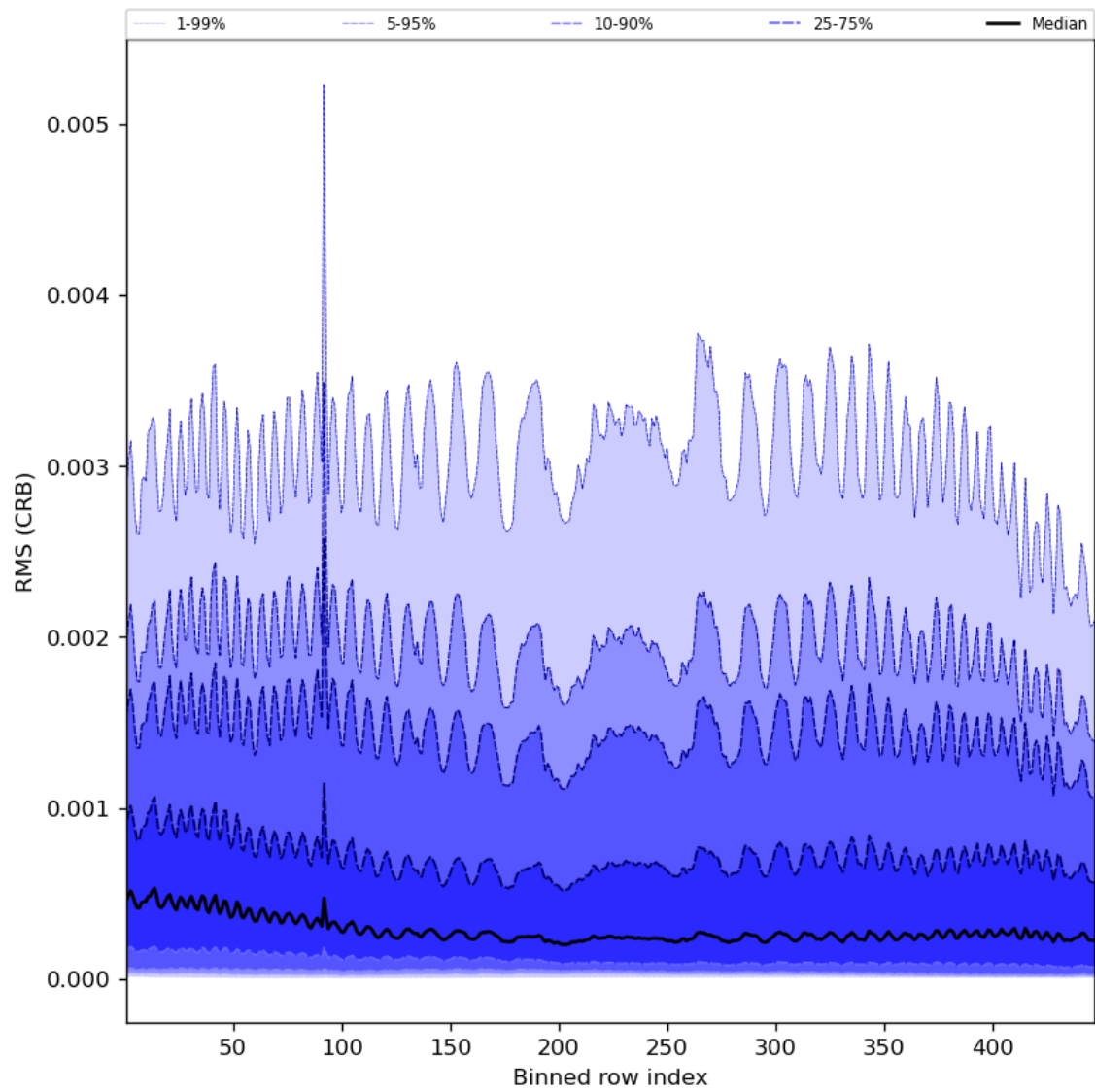
Figure 64: Along track statistics of “RMS (CRB)” for 2023-09-05 to 2023-09-06
