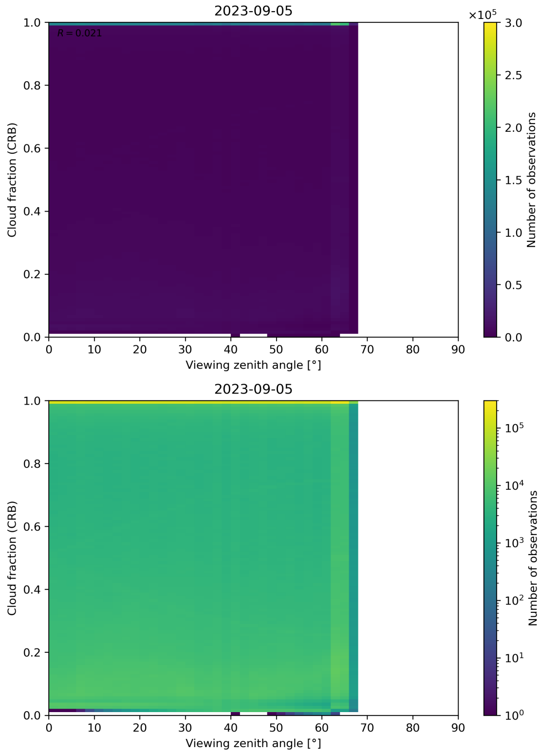
Figure 109: Scatter density plot of “Viewing zenith angle” against “Cloud fraction (CRB)” for 2023-09-05 to 2023-09-06.
