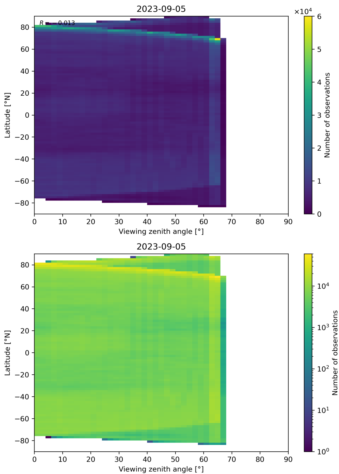
Figure 113: Scatter density plot of “Viewing zenith angle” against “Latitude” for 2023-09-05 to 2023-09-06.
