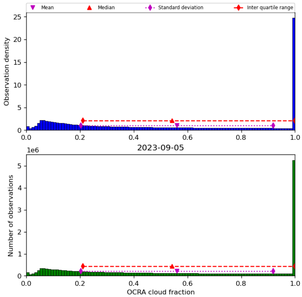
Figure 50: Histogram of “OCRA cloud fraction” for 2023-09-05 to 2023-09-06
