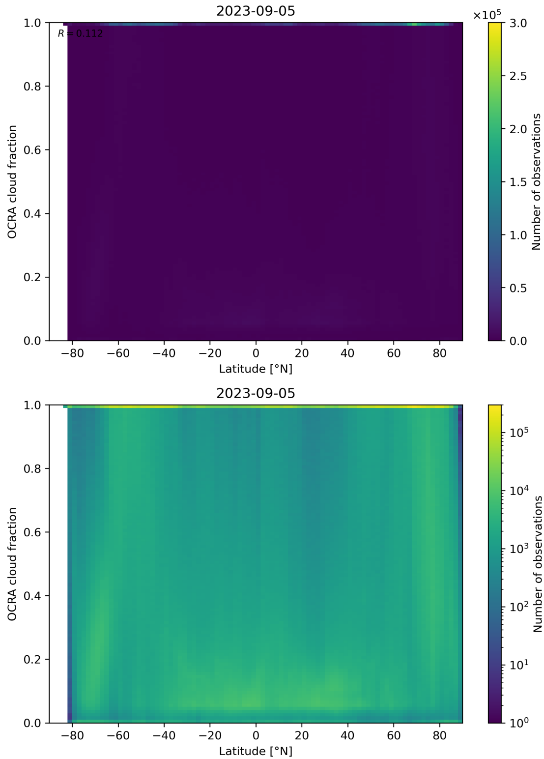
Figure 93: Scatter density plot of “Latitude” against “OCRA cloud fraction” for 2023-09-05 to 2023-09-06.
