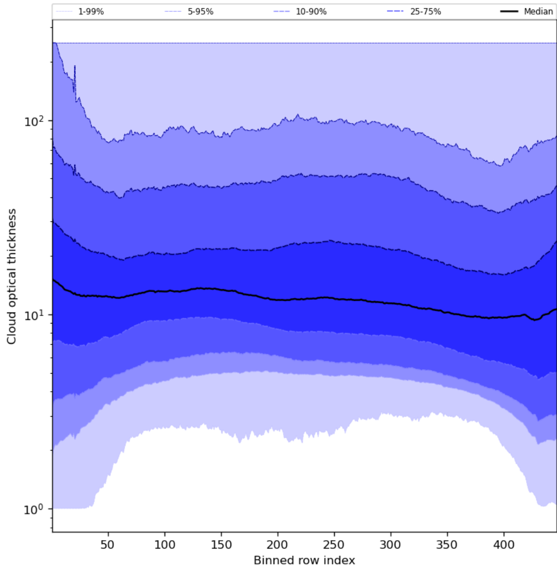
Figure 57: Along track statistics of “Cloud optical thickness” for 2023-09-05 to 2023-09-06
