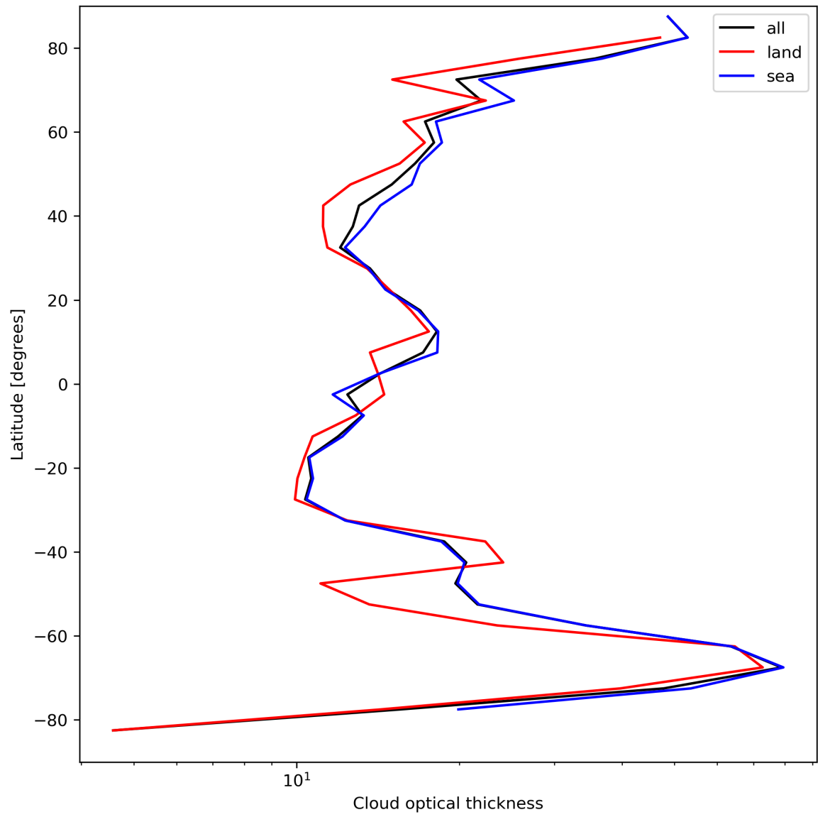
Figure 25: Zonal average of “Cloud optical thickness” for 2023-09-05 to 2023-09-06.
