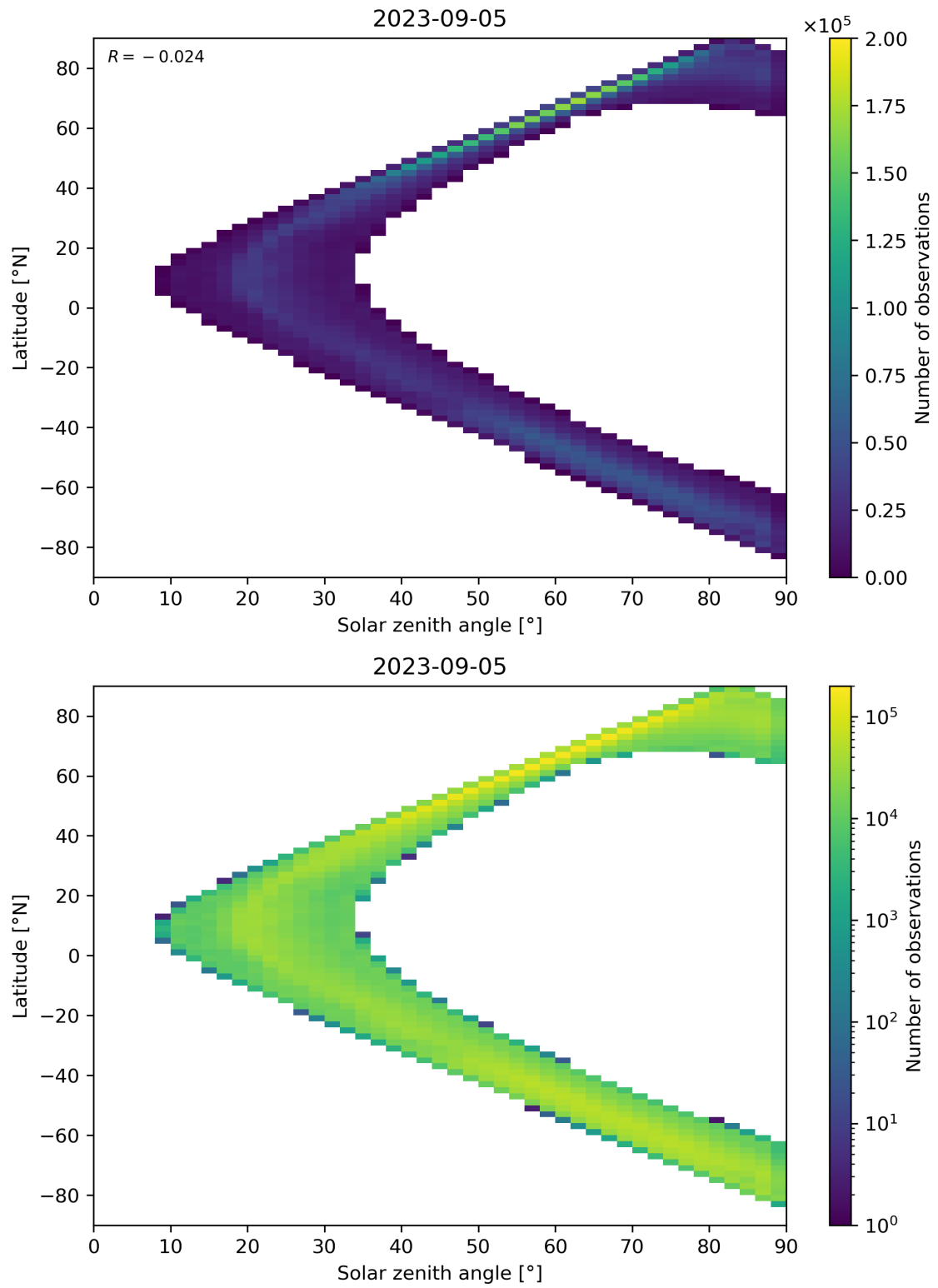
Figure 105: Scatter density plot of “Solar zenith angle” against “Latitude” for 2023-09-05 to 2023-09-06.
