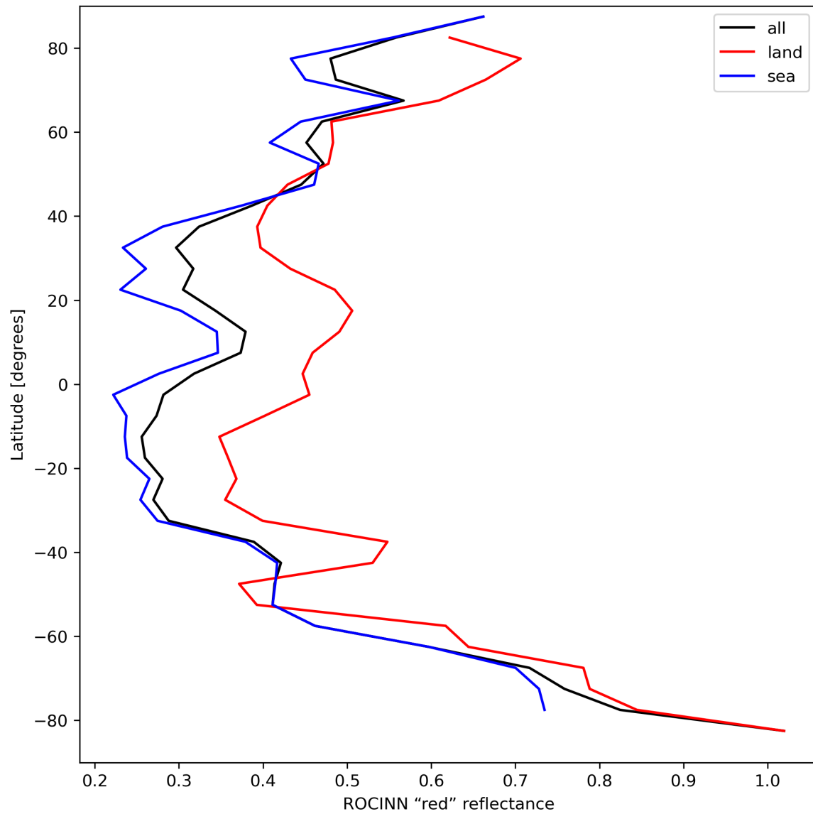
Figure 37: Zonal average of “ROCINN “red” reflectance” for 2023-09-05 to 2023-09-06.
