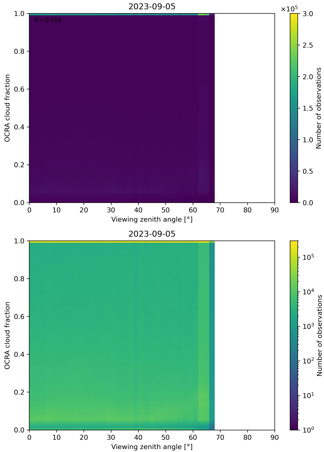
Figure 108: Scatter density plot of “Viewing zenith angle” against “OCRA cloud fraction” for 2023-09-05 to 2023-09-06.
