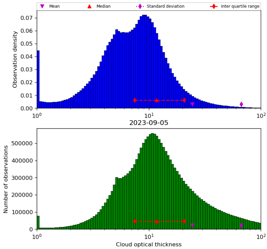
Figure 41: Histogram of “Cloud optical thickness” for 2023-09-05 to 2023-09-06
