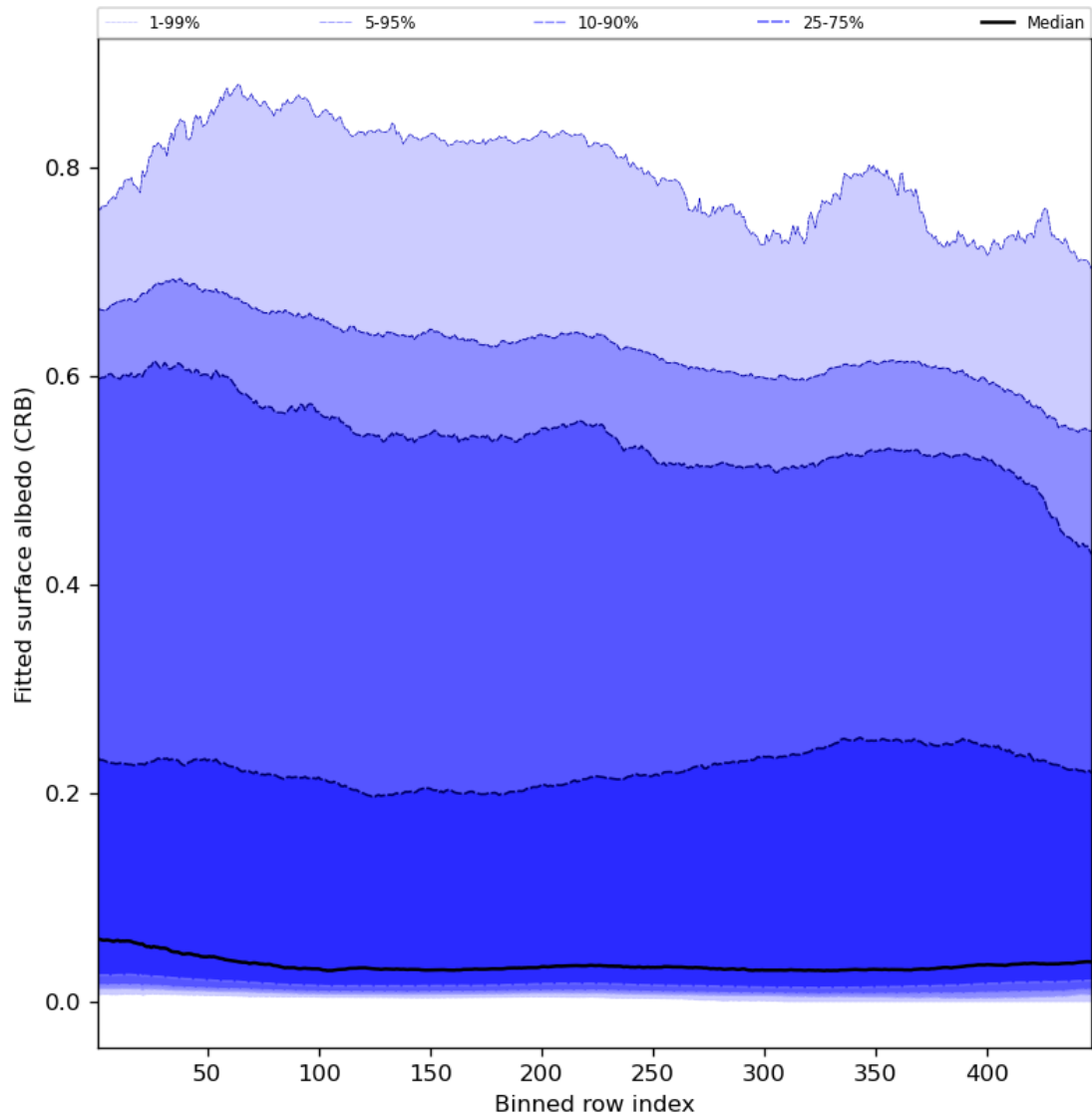
Figure 62: Along track statistics of “Fitted surface albedo (CRB)” for 2023-09-05 to 2023-09-06
