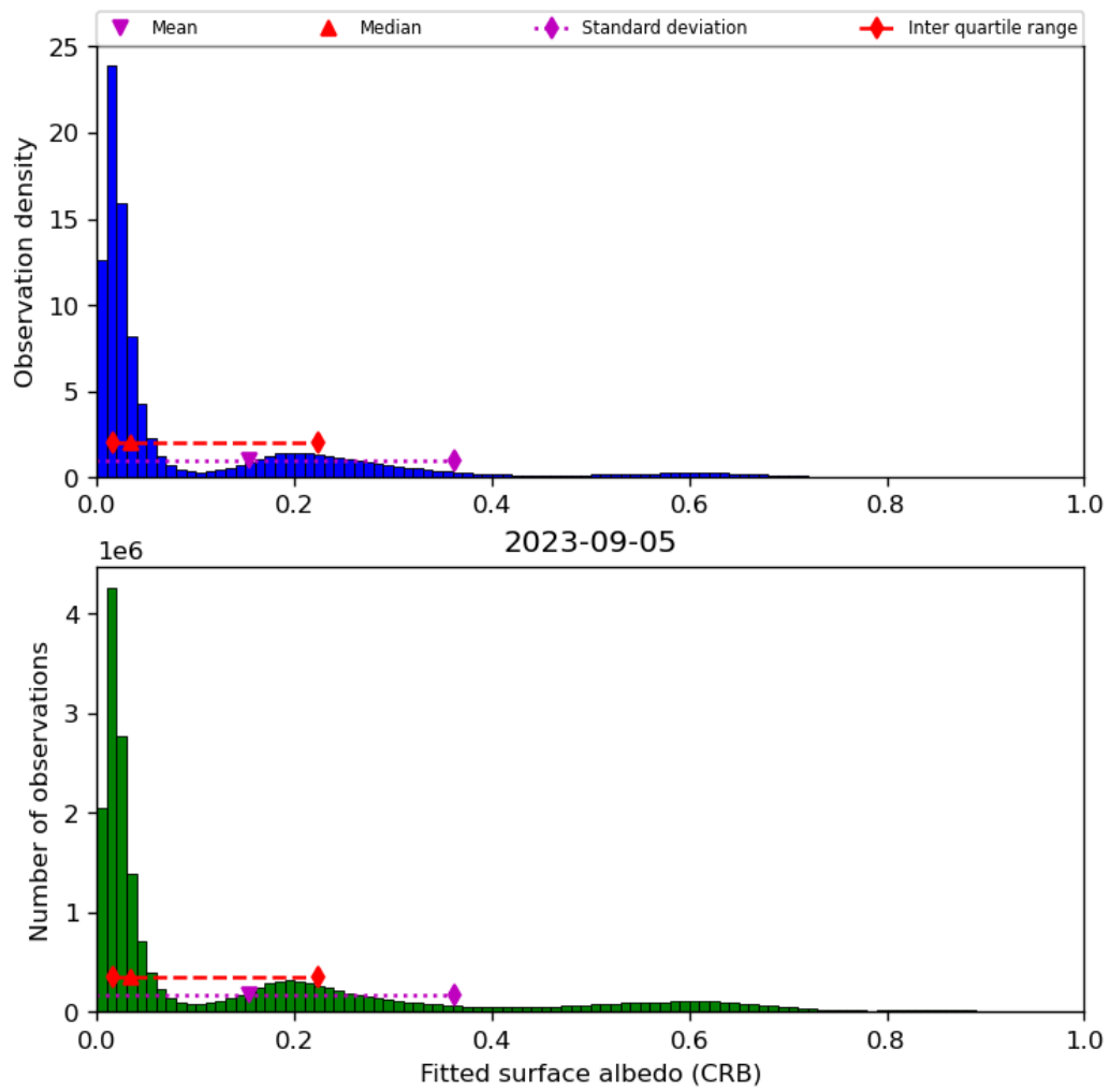
Figure 46: Histogram of “Fitted surface albedo (CRB)” for 2023-09-05 to 2023-09-06
