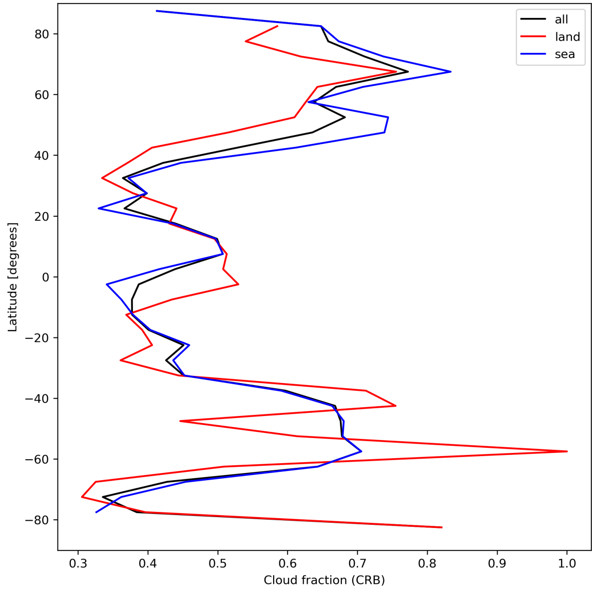
Figure 26: Zonal average of “Cloud fraction (CRB)” for 2023-09-05 to 2023-09-06.
