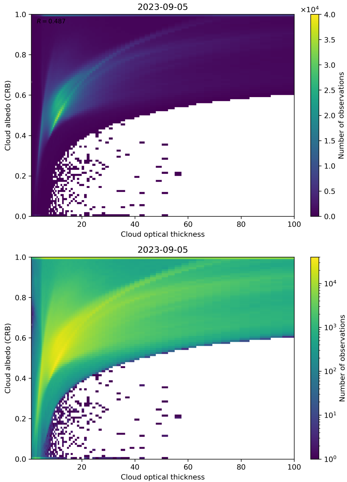
Figure 82: Scatter density plot of “Cloud optical thickness” against “Cloud albedo (CRB)” for 2023-09-05 to 2023-09-06.
