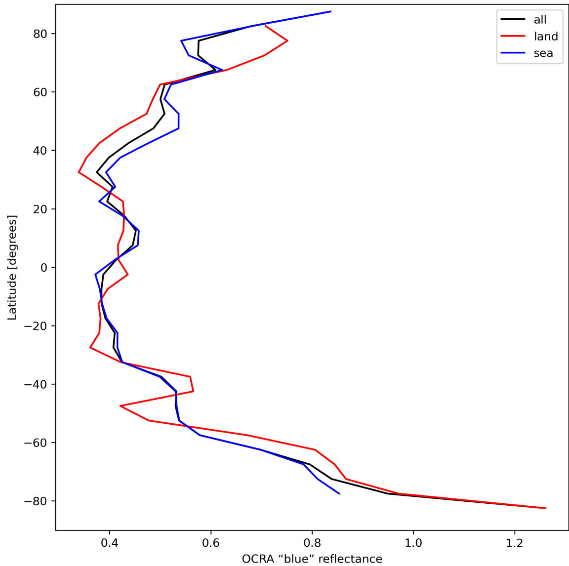
Figure 35: Zonal average of “OCRA “blue” reflectance” for 2023-09-05 to 2023-09-06.
