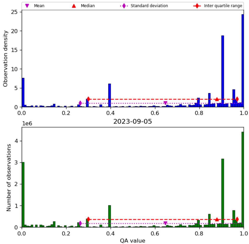
Figure 38: Histogram of “QA value” for 2023-09-05 to 2023-09-06
