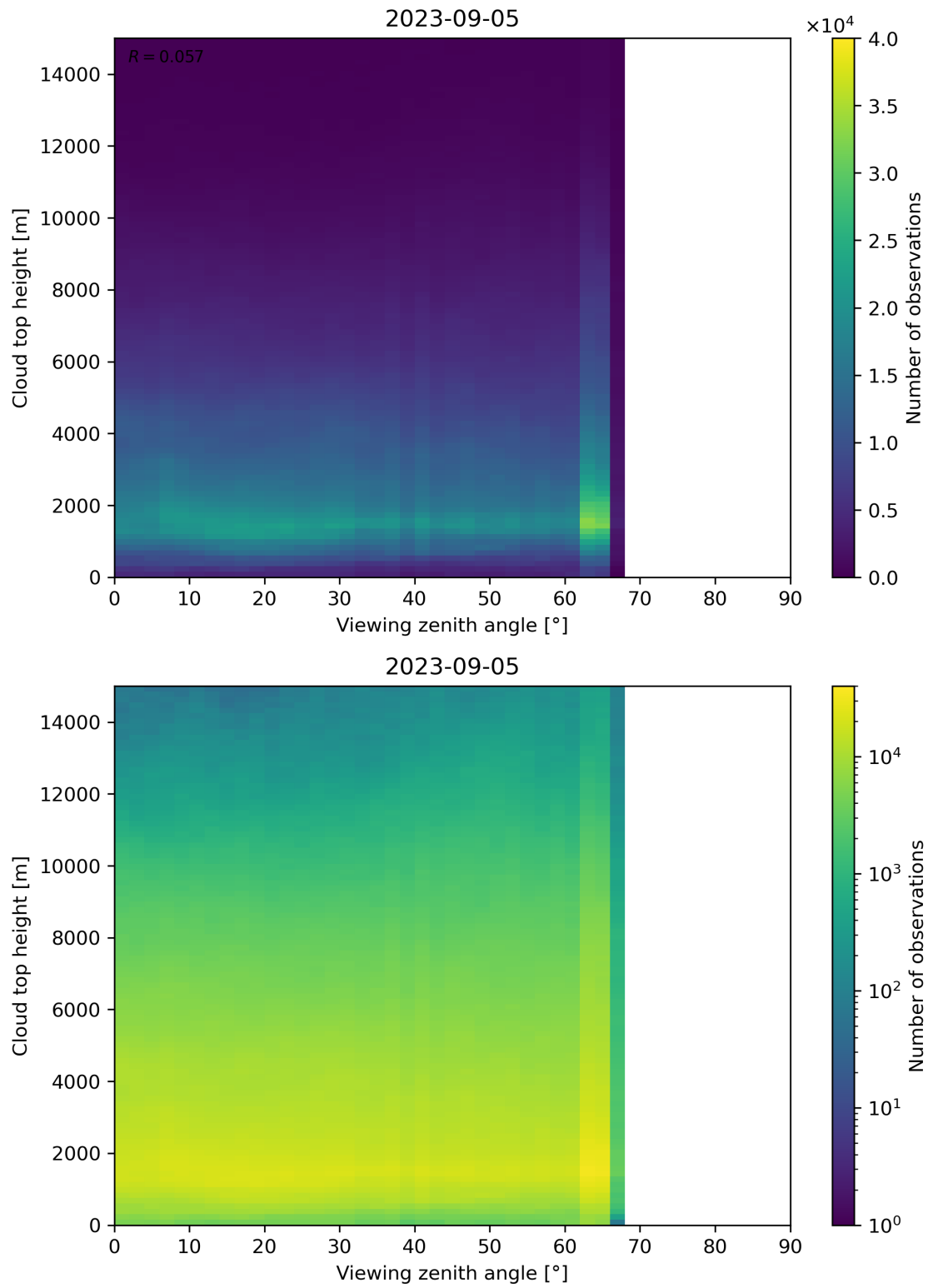
Figure 112: Scatter density plot of “Viewing zenith angle” against “Cloud top height” for 2023-09-05 to 2023-09-06.
