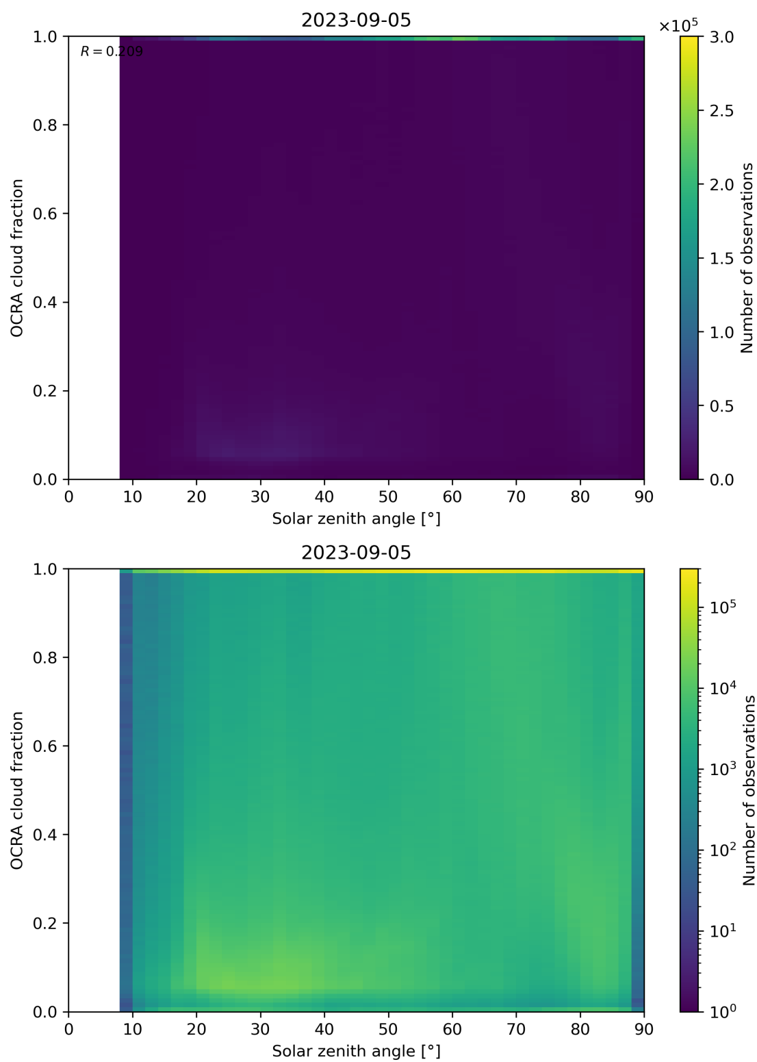
Figure 100: Scatter density plot of “Solar zenith angle” against “OCRA cloud fraction” for 2023-09-05 to 2023-09-06.
