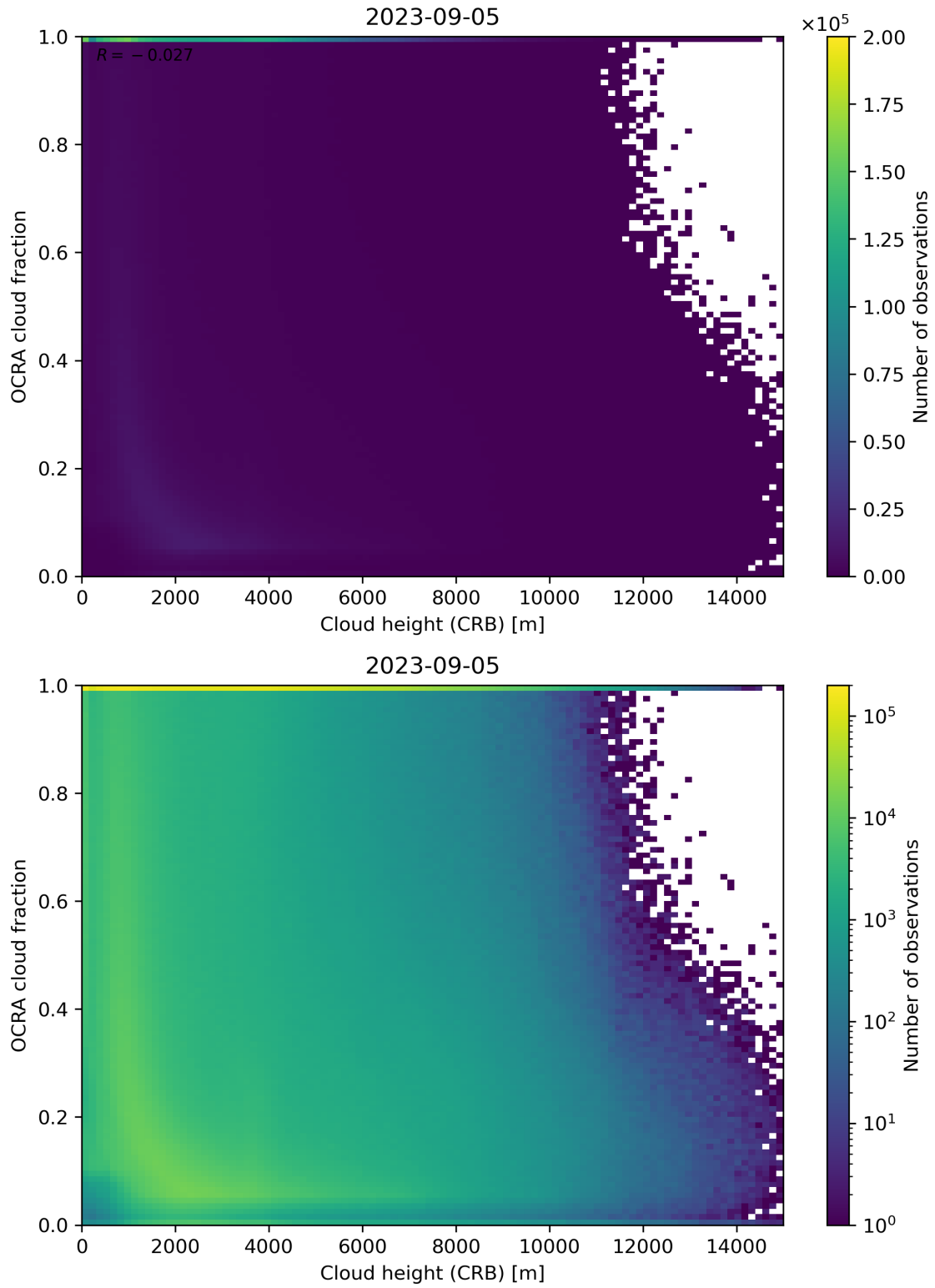
Figure 81: Scatter density plot of “Cloud height (CRB)” against “OCRA cloud fraction” for 2023-09-05 to 2023-09-06.
