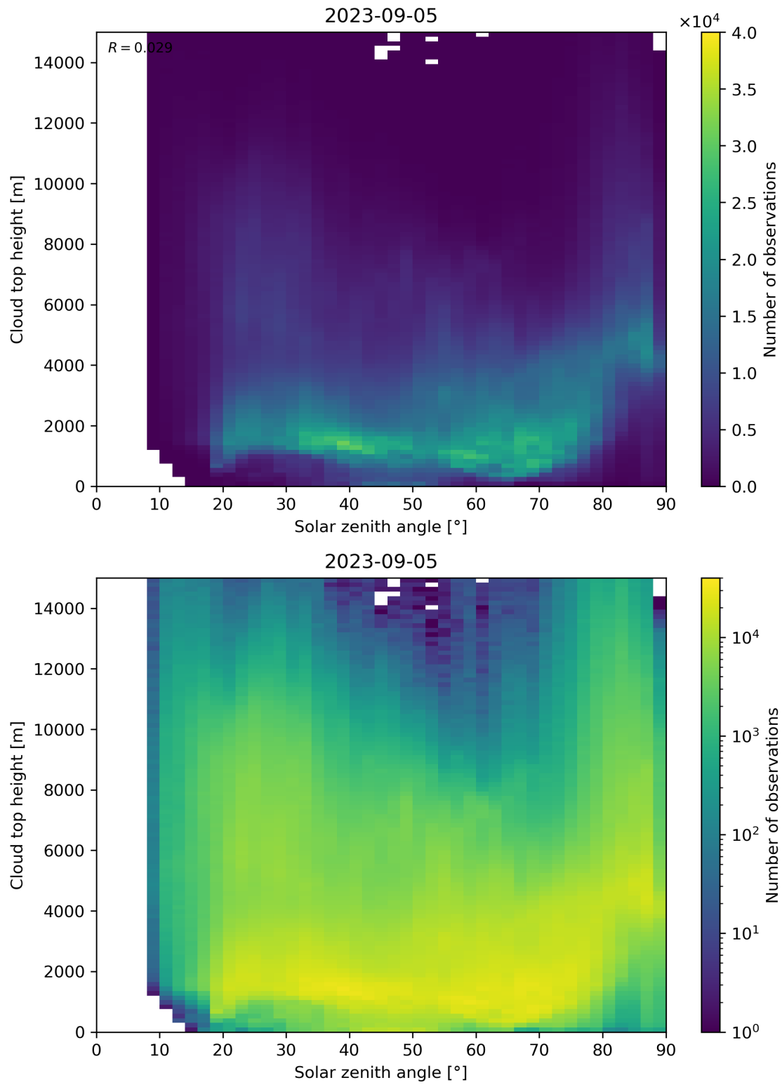
Figure 104: Scatter density plot of “Solar zenith angle” against “Cloud top height” for 2023-09-05 to 2023-09-06.
