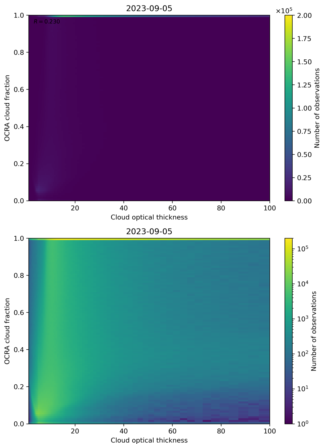
Figure 83: Scatter density plot of “Cloud optical thickness” against “OCRA cloud fraction” for 2023-09-05 to 2023-09-06.
