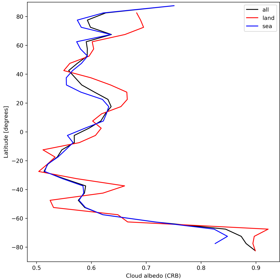
Figure 28: Zonal average of “Cloud albedo (CRB)” for 2023-09-05 to 2023-09-06.
