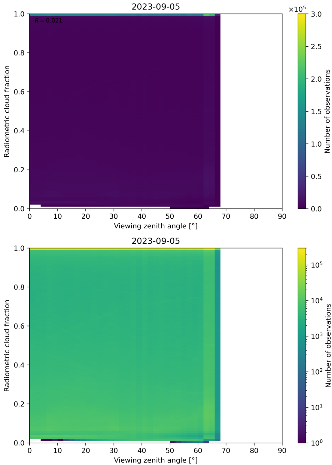
Figure 107: Scatter density plot of “Viewing zenith angle” against “Radiometric cloud fraction” for 2023-09-05 to 2023-09-06.
