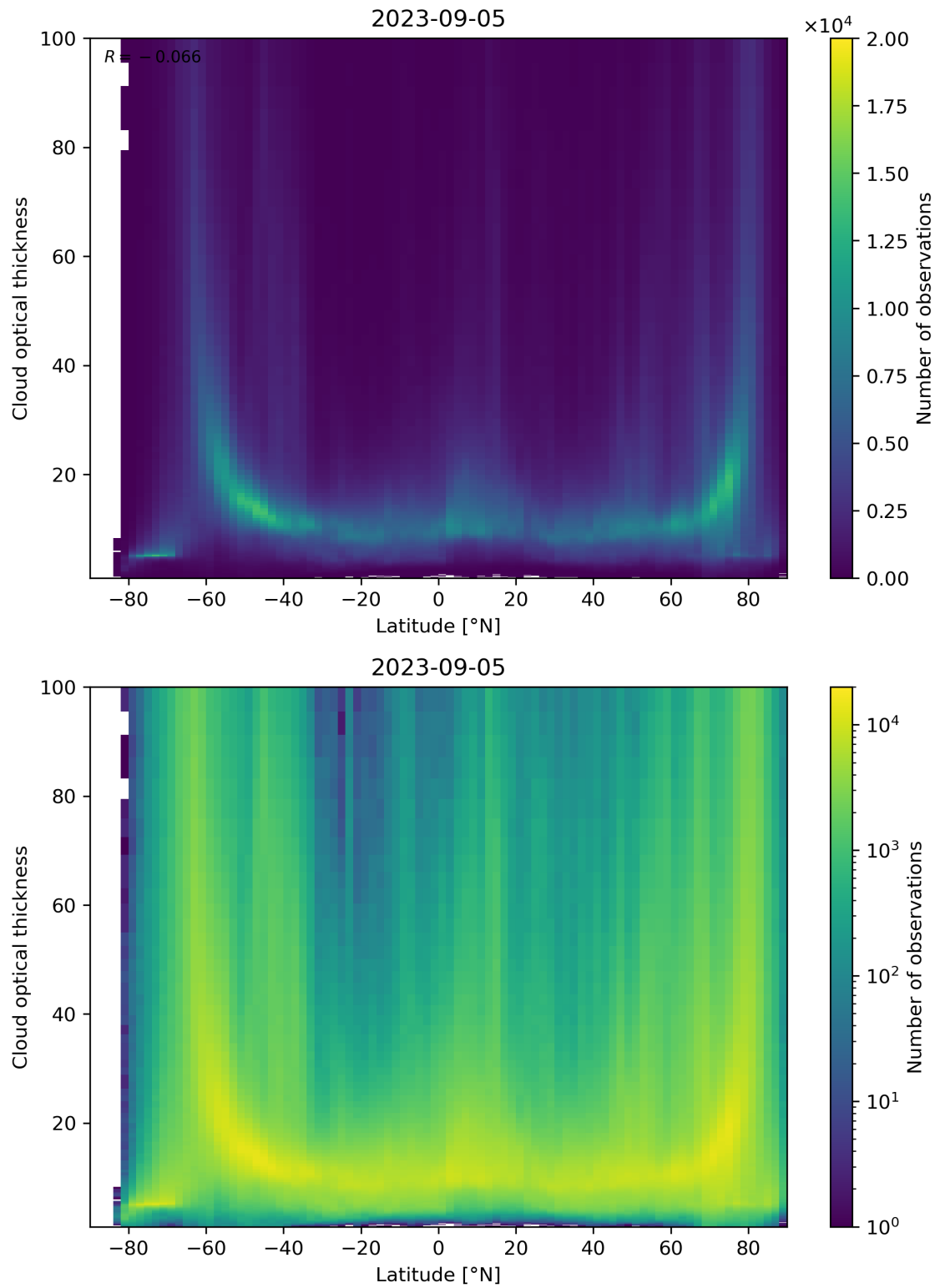
Figure 96: Scatter density plot of “Latitude” against “Cloud optical thickness” for 2023-09-05 to 2023-09-06.
