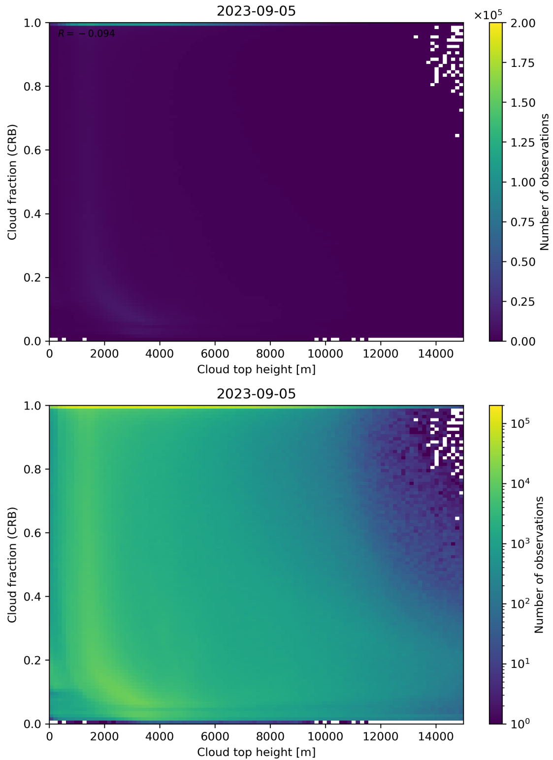
Figure 88: Scatter density plot of “Cloud top height” against “Cloud fraction (CRB)” for 2023-09-05 to 2023-09-06.
