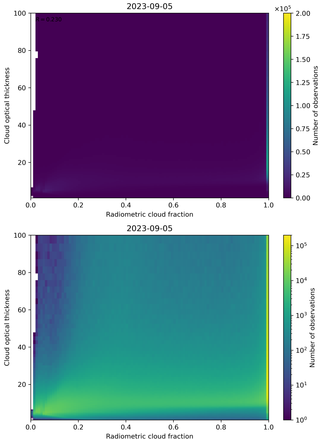
Figure 75: Scatter density plot of “Radiometric cloud fraction” against “Cloud optical thickness” for 2023-09-05 to 2023-09-06.
