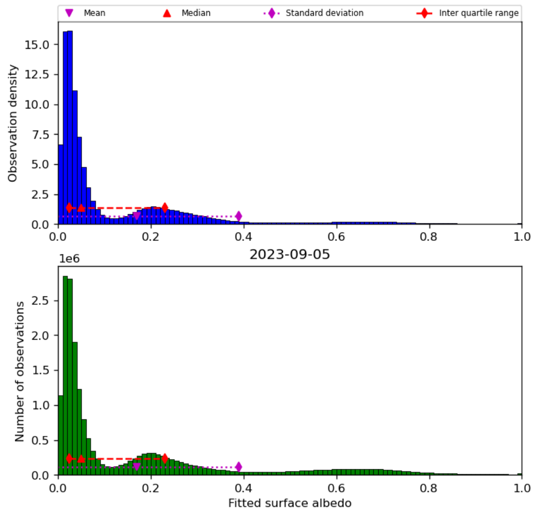
Figure 45: Histogram of “Fitted surface albedo” for 2023-09-05 to 2023-09-06
