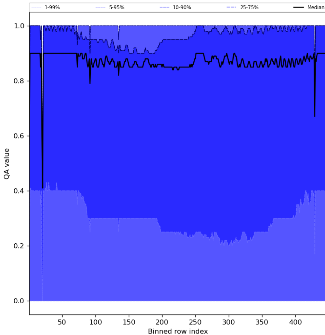
Figure 54: Along track statistics of “QA value” for 2023-09-05 to 2023-09-06
