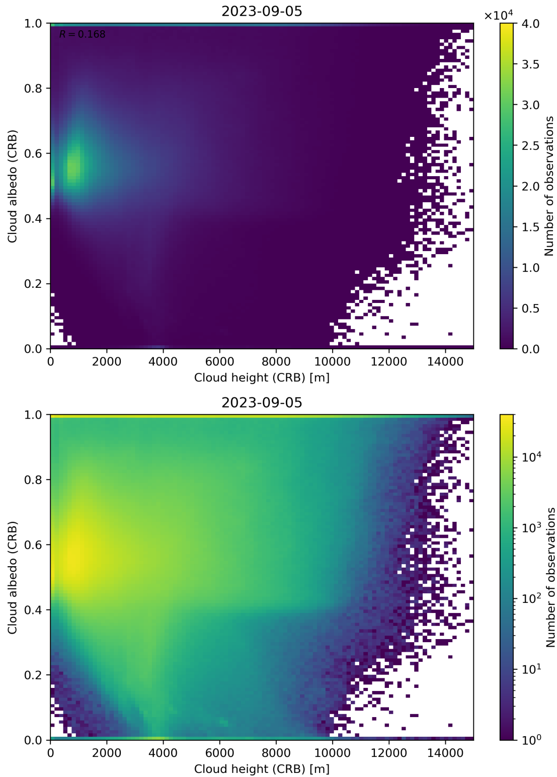
Figure 80: Scatter density plot of “Cloud height (CRB)” against “Cloud albedo (CRB)” for 2023-09-05 to 2023-09-06.
