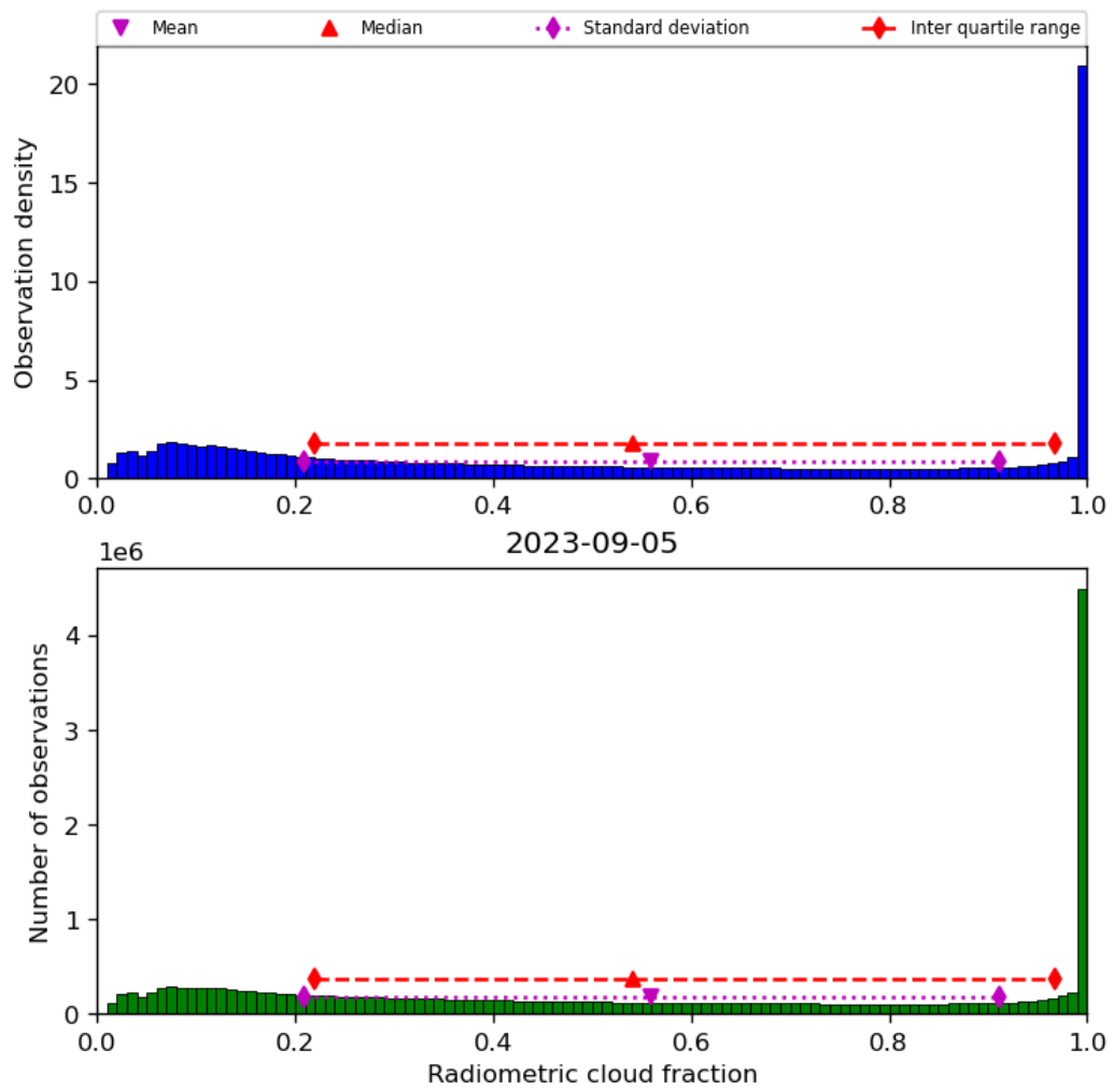
Figure 39: Histogram of “Radiometric cloud fraction” for 2023-09-05 to 2023-09-06
