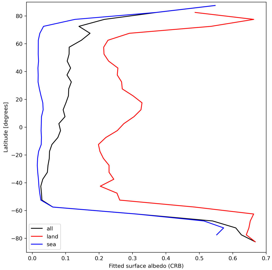
Figure 30: Zonal average of “Fitted surface albedo (CRB)” for 2023-09-06 to 2023-09-08.
