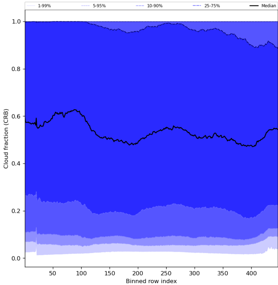
Figure 58: Along track statistics of “Cloud fraction (CRB)” for 2023-09-06 to 2023-09-08
