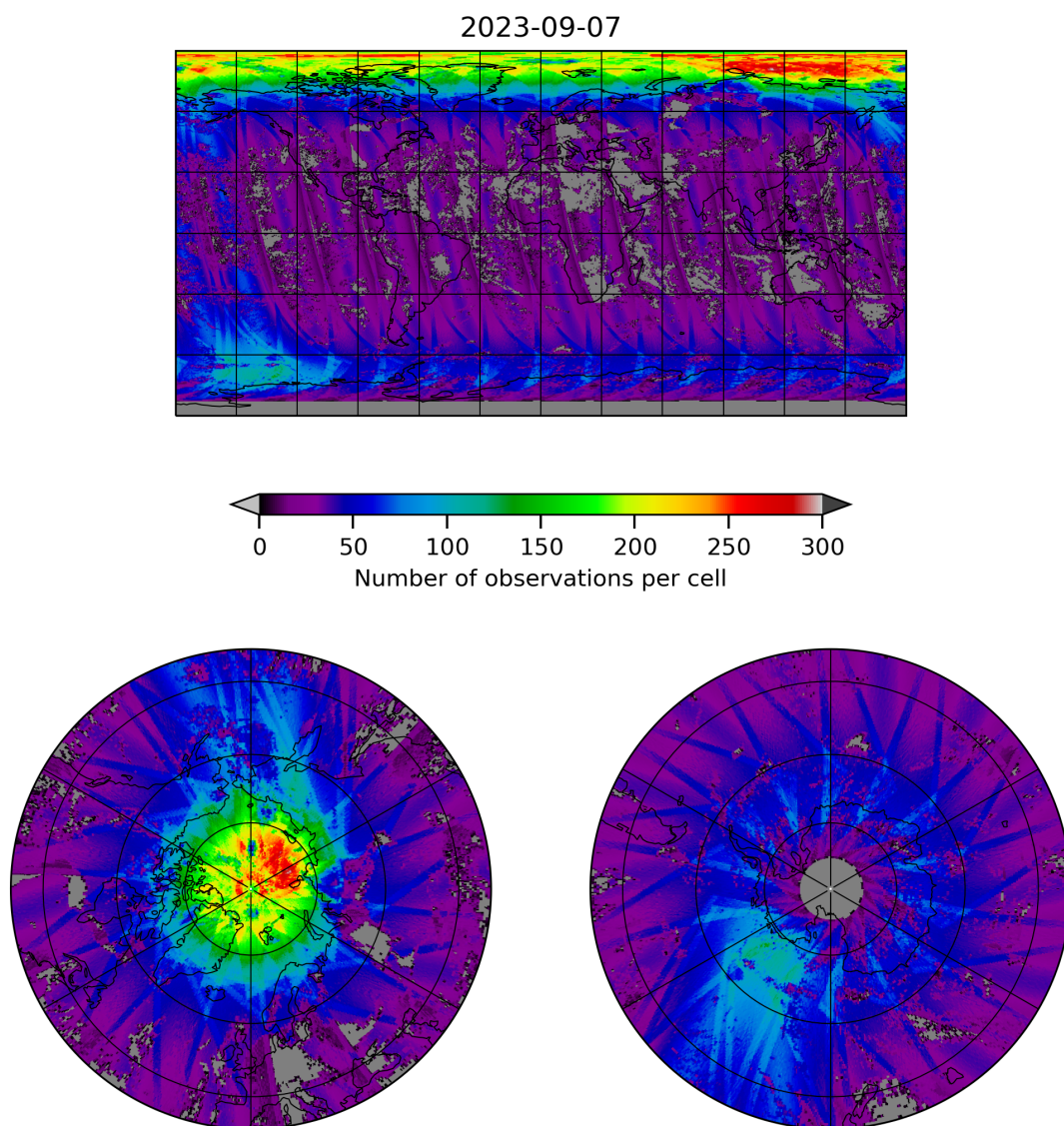
Figure 21: Map of the number of observations for 2023-09-06 to 2023-09-08
