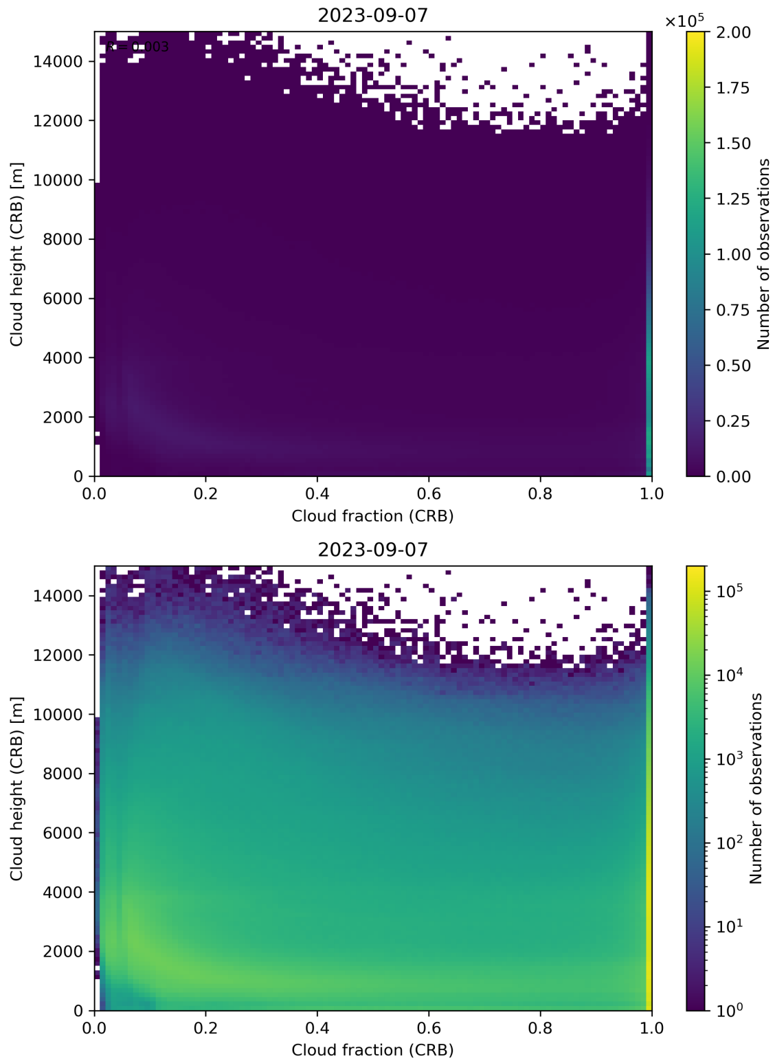
Figure 79: Scatter density plot of “Cloud fraction (CRB)” against “Cloud height (CRB)” for 2023-09-06 to 2023-09-08.
