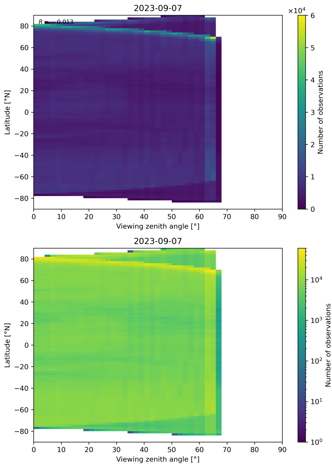
Figure 113: Scatter density plot of “Viewing zenith angle” against “Latitude” for 2023-09-06 to 2023-09-08.
