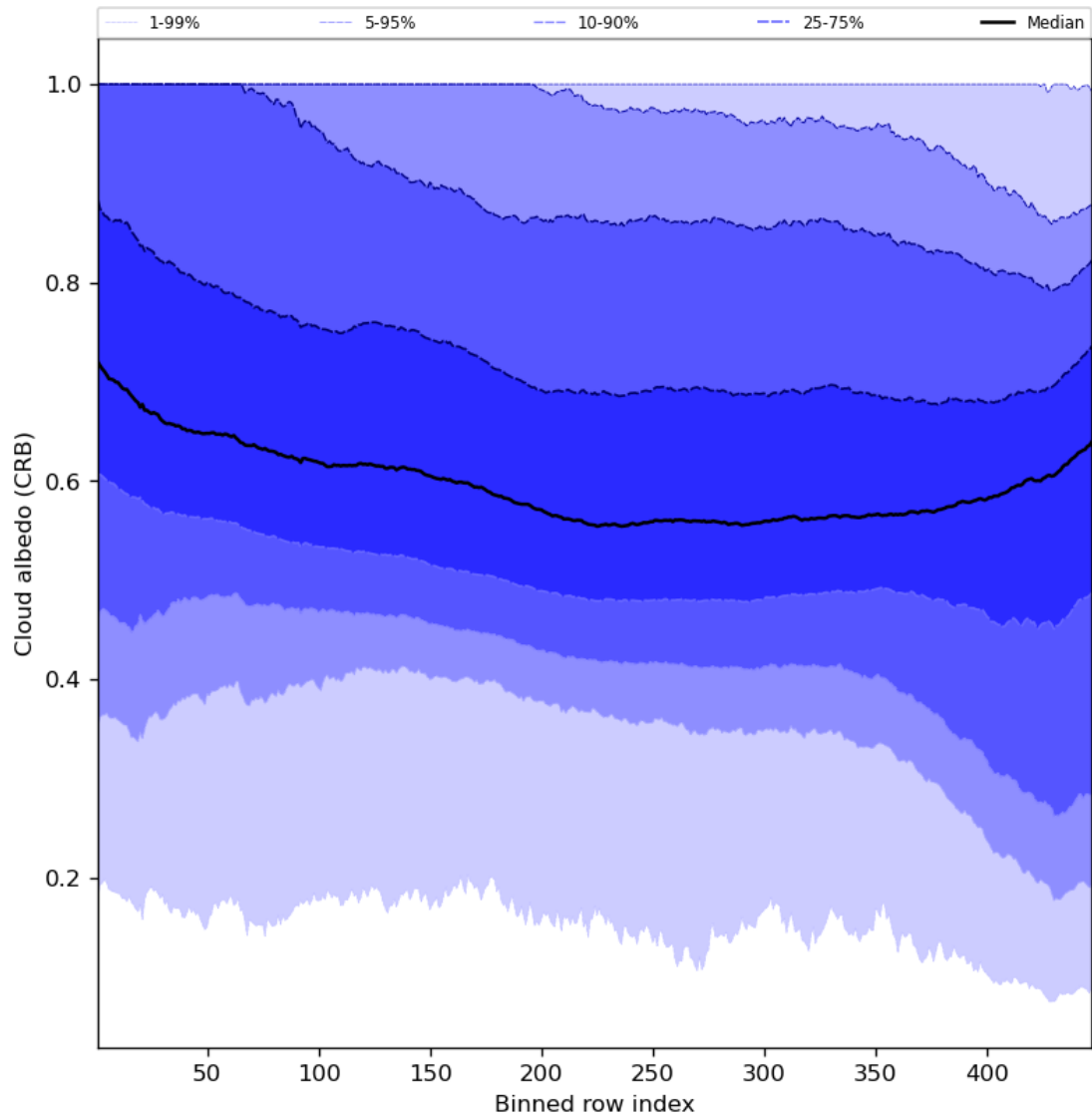
Figure 60: Along track statistics of “Cloud albedo (CRB)” for 2023-09-06 to 2023-09-08
