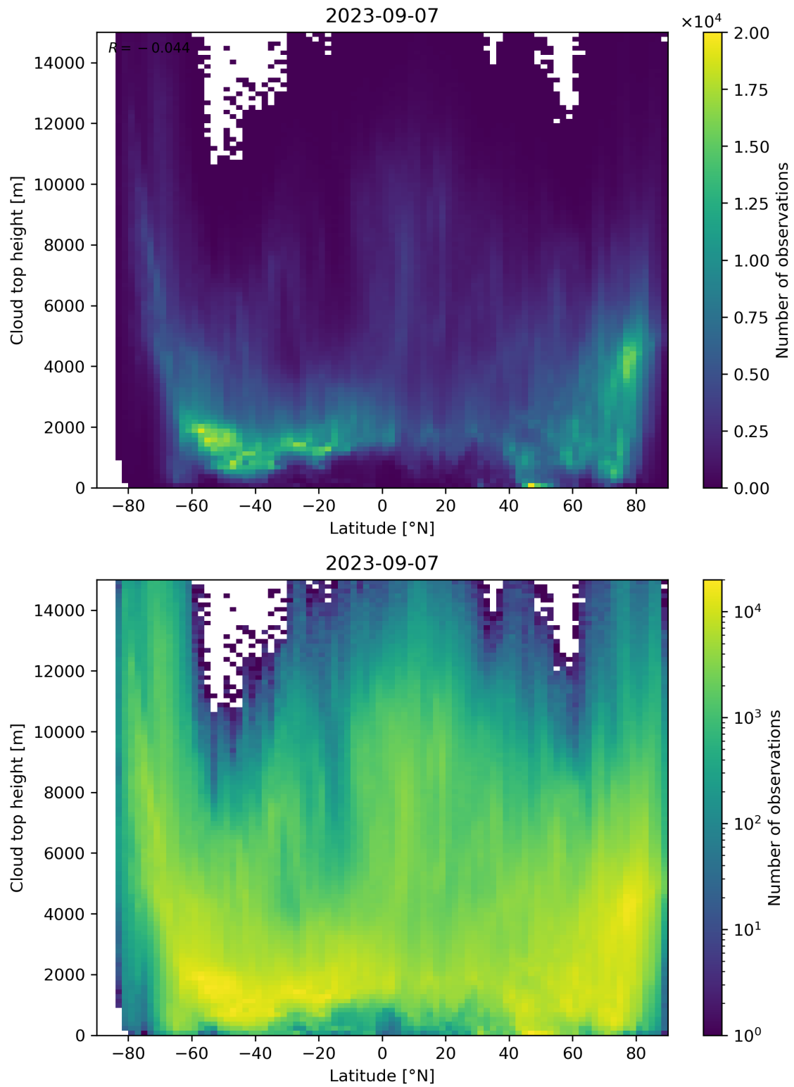
Figure 97: Scatter density plot of “Latitude” against “Cloud top height” for 2023-09-06 to 2023-09-08.
