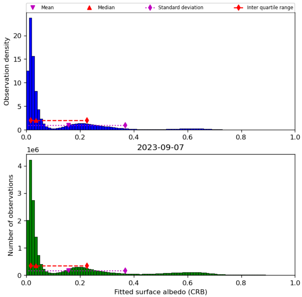
Figure 46: Histogram of “Fitted surface albedo (CRB)” for 2023-09-06 to 2023-09-08
