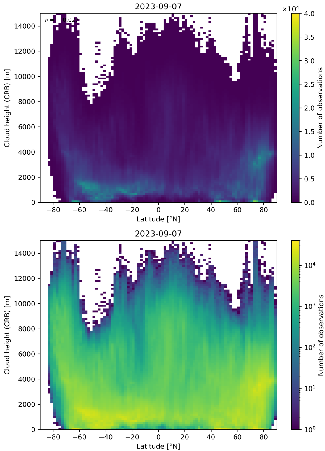
Figure 95: Scatter density plot of “Latitude” against “Cloud height (CRB)” for 2023-09-06 to 2023-09-08.
