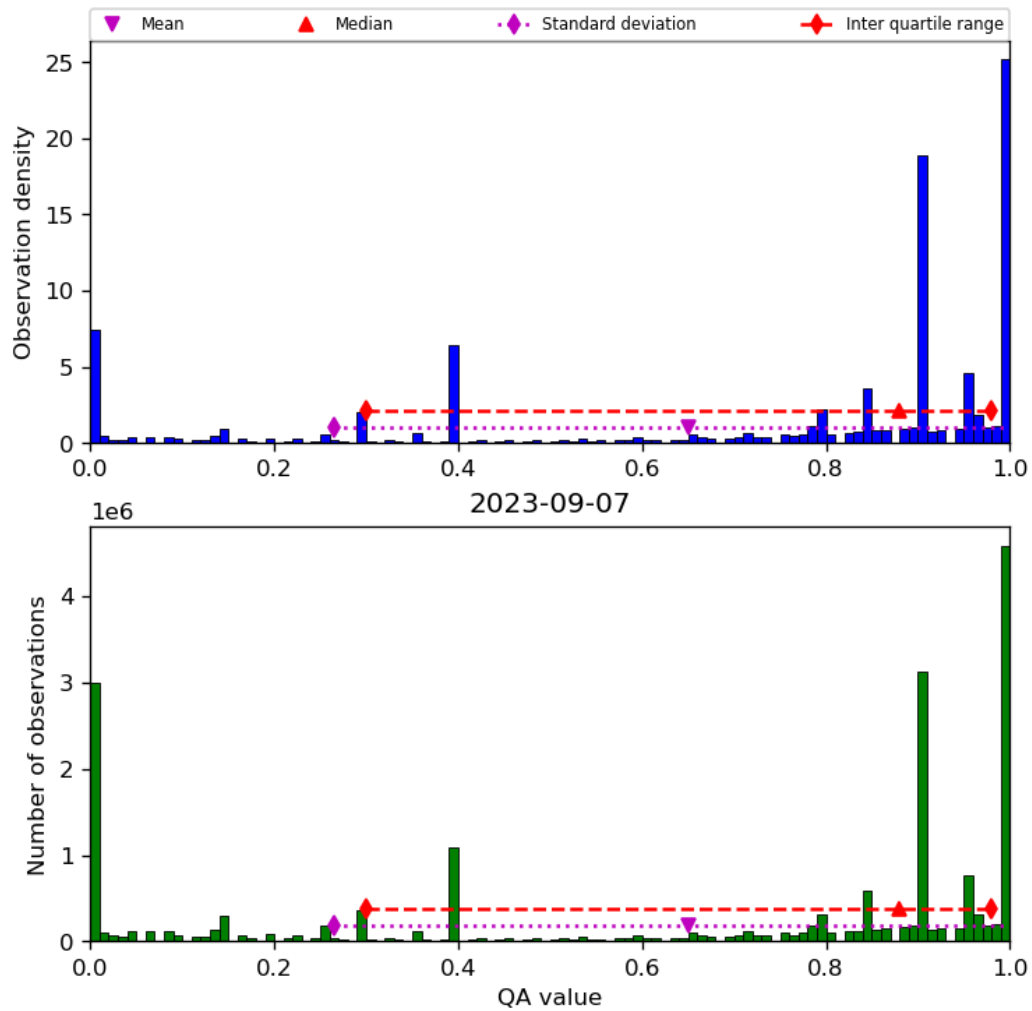
Figure 38: Histogram of “QA value” for 2023-09-06 to 2023-09-08
