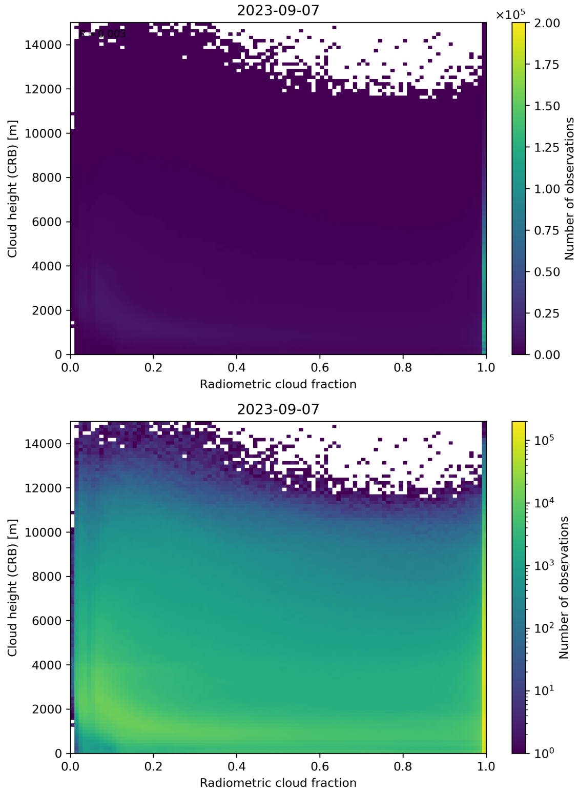
Figure 74: Scatter density plot of “Radiometric cloud fraction” against “Cloud height (CRB)” for 2023-09-06 to 2023-09-08.
