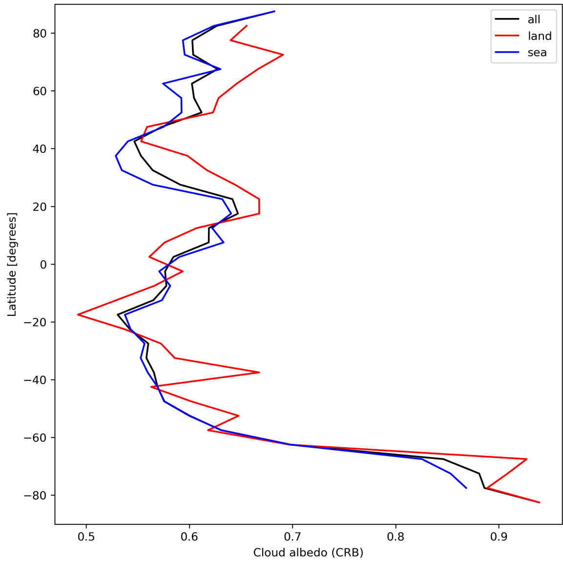
Figure 28: Zonal average of “Cloud albedo (CRB)” for 2023-09-06 to 2023-09-08.
