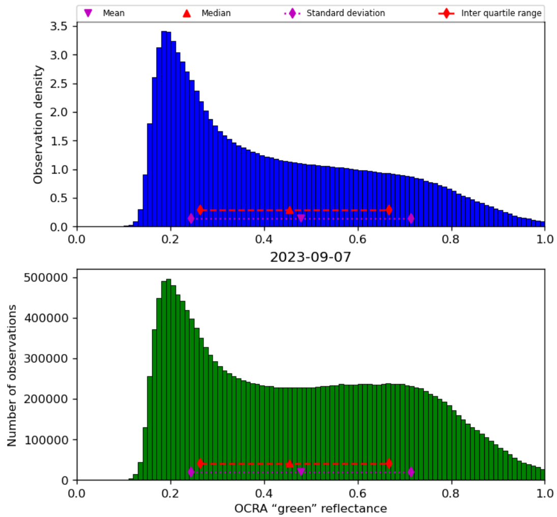
Figure 52: Histogram of “OCRA “green” reflectance” for 2023-09-06 to 2023-09-08
