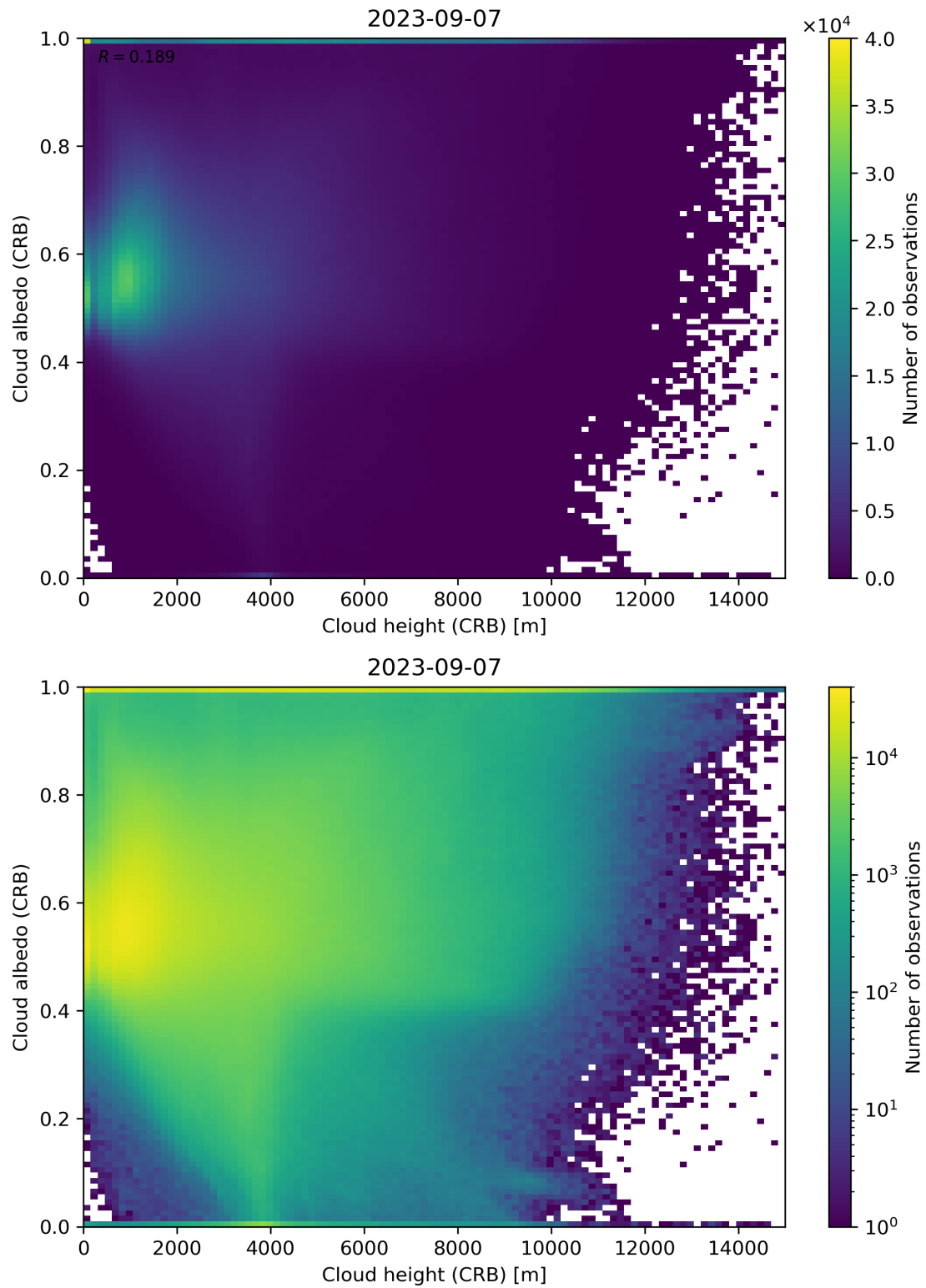
Figure 80: Scatter density plot of “Cloud height (CRB)” against “Cloud albedo (CRB)” for 2023-09-06 to 2023-09-08.
