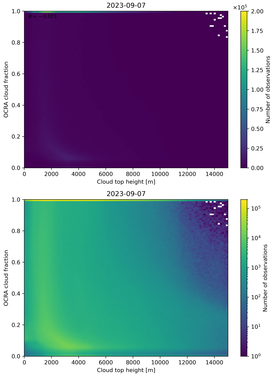
Figure 87: Scatter density plot of “Cloud top height” against “OCRA cloud fraction” for 2023-09-06 to 2023-09-08.
