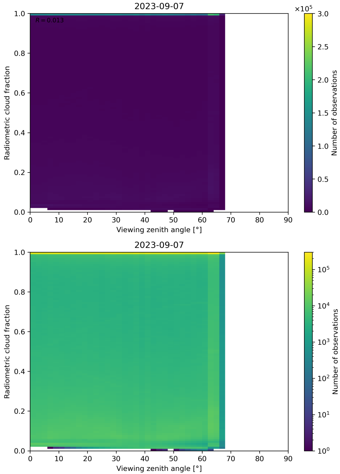
Figure 107: Scatter density plot of “Viewing zenith angle” against “Radiometric cloud fraction” for 2023-09-06 to 2023-09-08.
