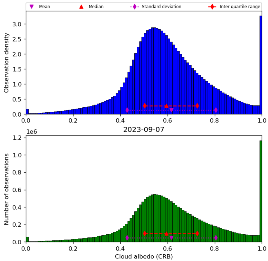
Figure 44: Histogram of “Cloud albedo (CRB)” for 2023-09-06 to 2023-09-08
