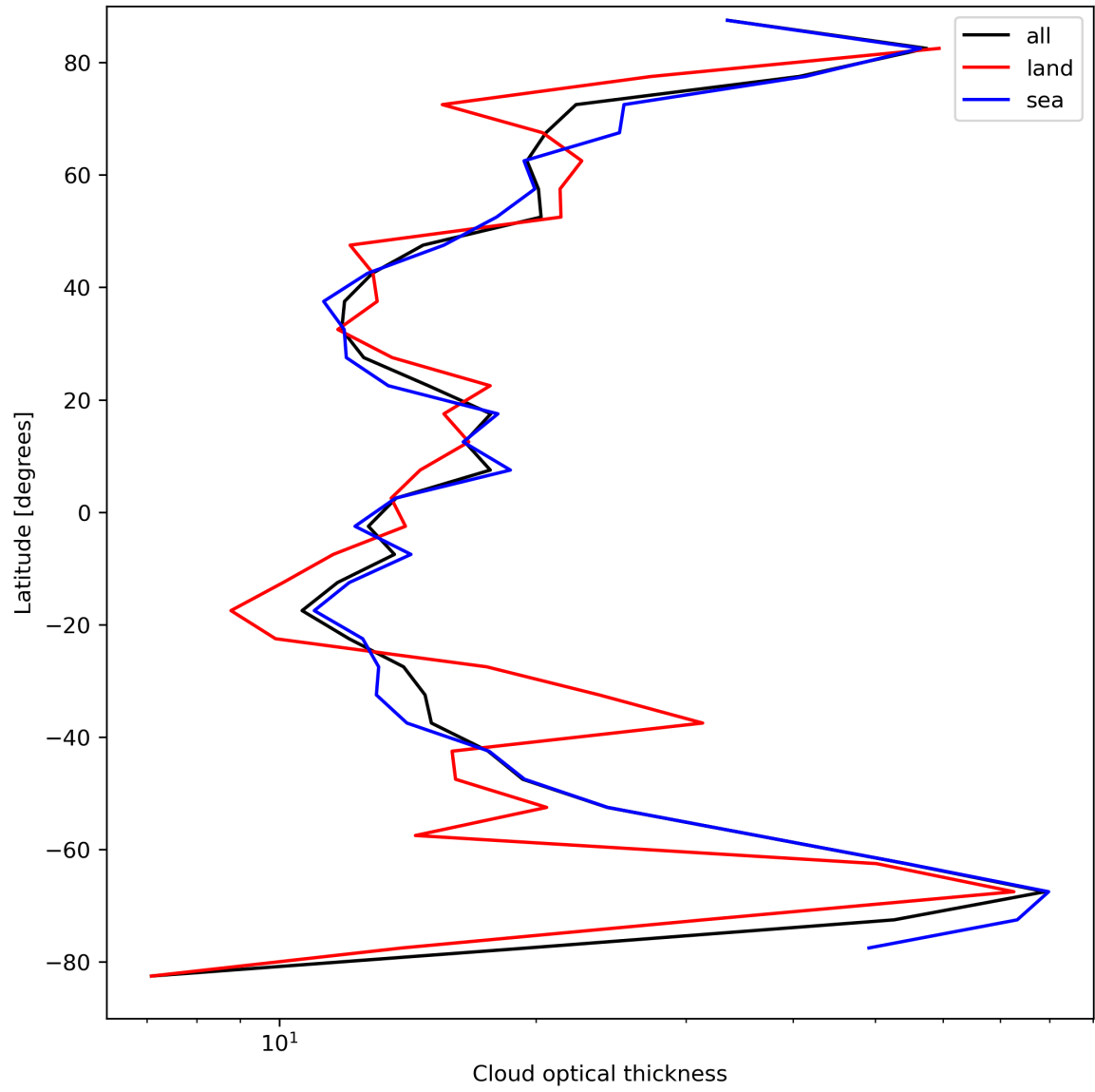
Figure 25: Zonal average of “Cloud optical thickness” for 2023-09-06 to 2023-09-08.
