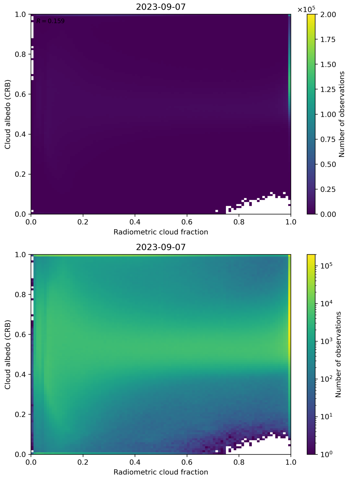
Figure 71: Scatter density plot of “Radiometric cloud fraction” against “Cloud albedo (CRB)” for 2023-09-06 to 2023-09-08.
