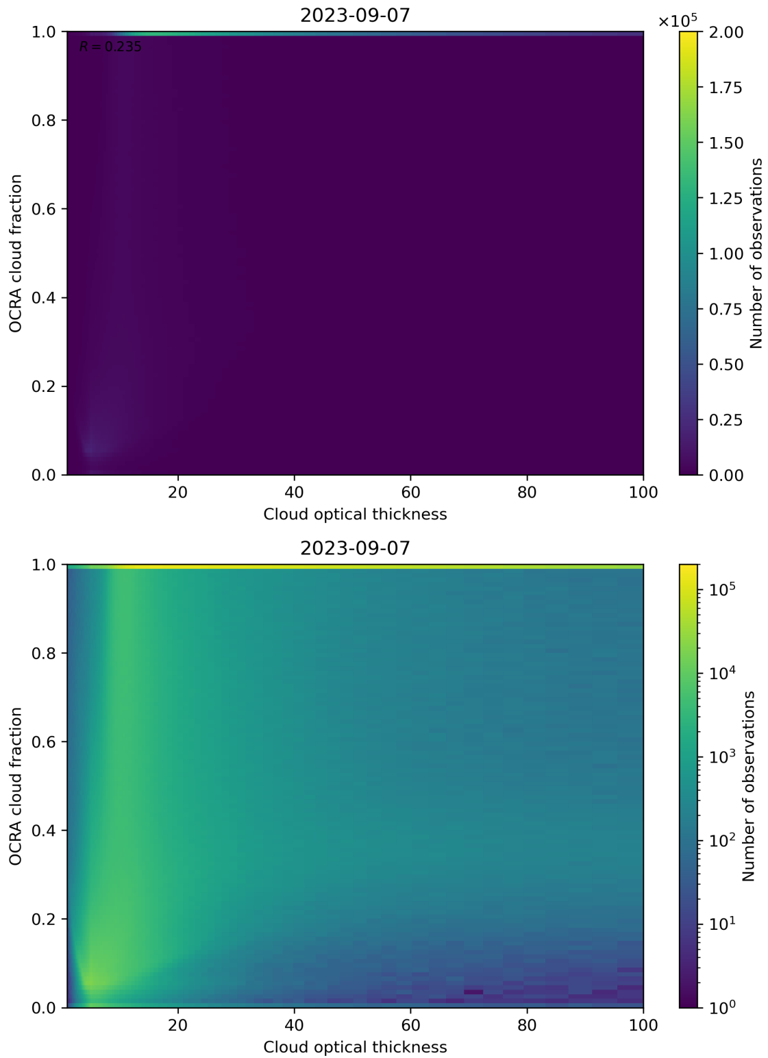
Figure 83: Scatter density plot of “Cloud optical thickness” against “OCRA cloud fraction” for 2023-09-06 to 2023-09-08.
