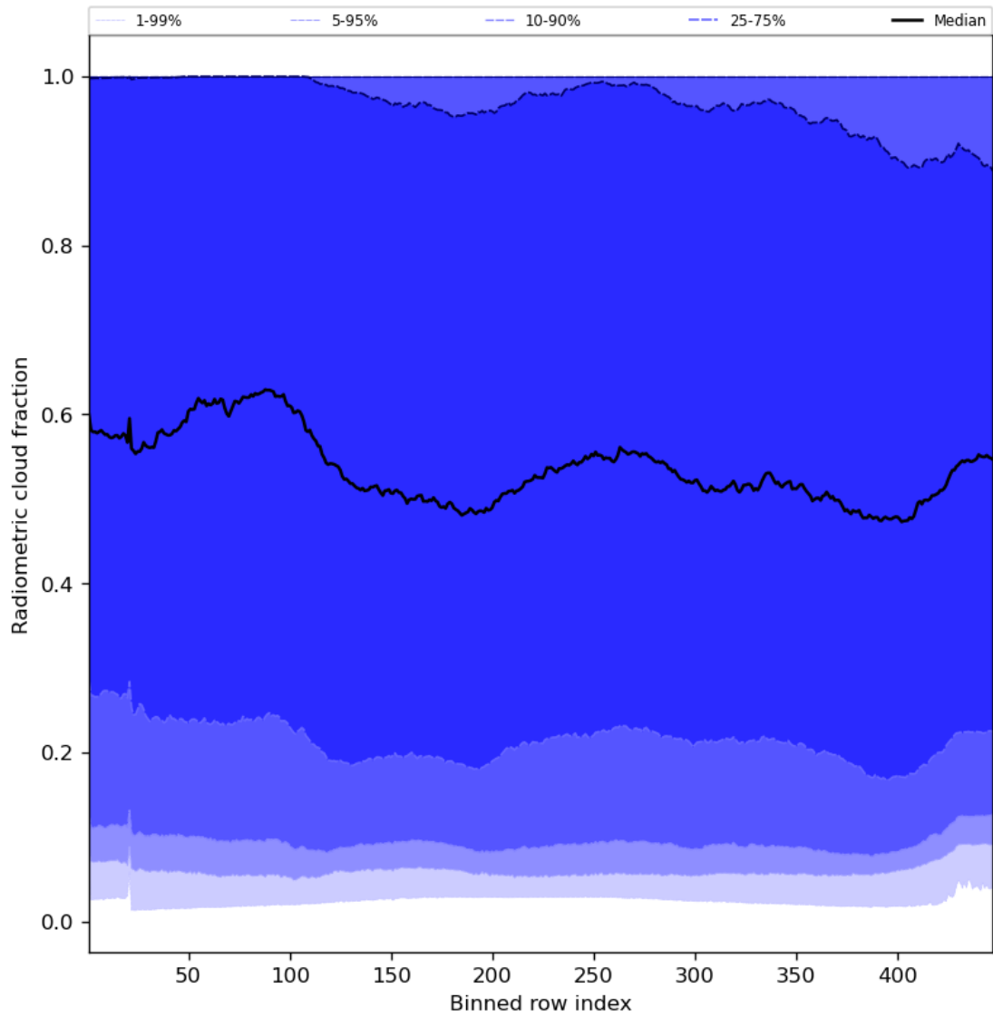
Figure 55: Along track statistics of “Radiometric cloud fraction” for 2023-09-06 to 2023-09-08
