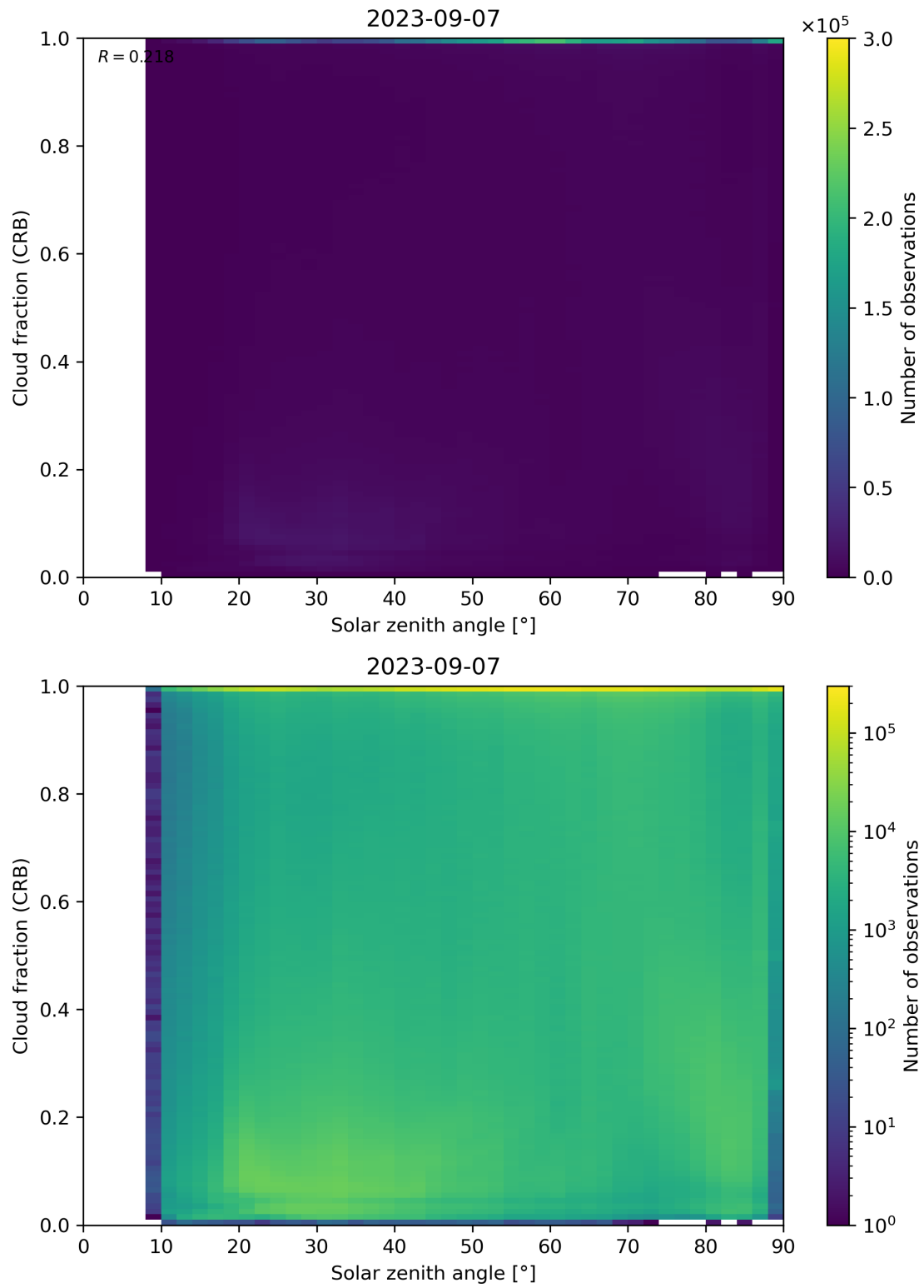
Figure 101: Scatter density plot of “Solar zenith angle” against “Cloud fraction (CRB)” for 2023-09-06 to 2023-09-08.
