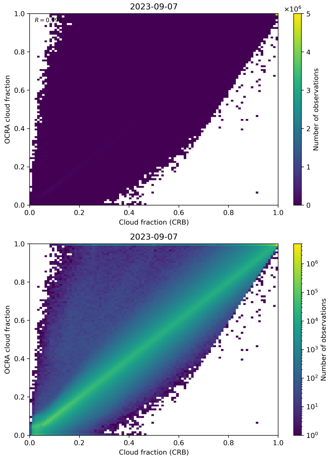
Figure 78: Scatter density plot of “Cloud fraction (CRB)” against “OCRA cloud fraction” for 2023-09-06 to 2023-09-08.
