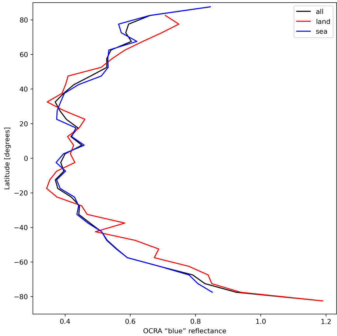
Figure 35: Zonal average of “OCRA “blue” reflectance” for 2023-09-06 to 2023-09-08.
