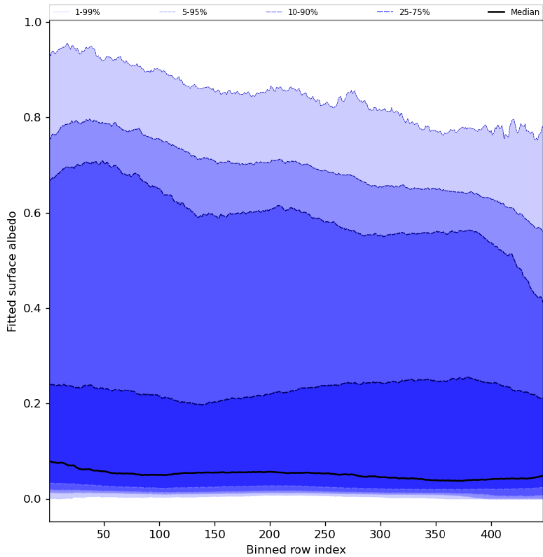
Figure 61: Along track statistics of “Fitted surface albedo” for 2023-09-06 to 2023-09-08
