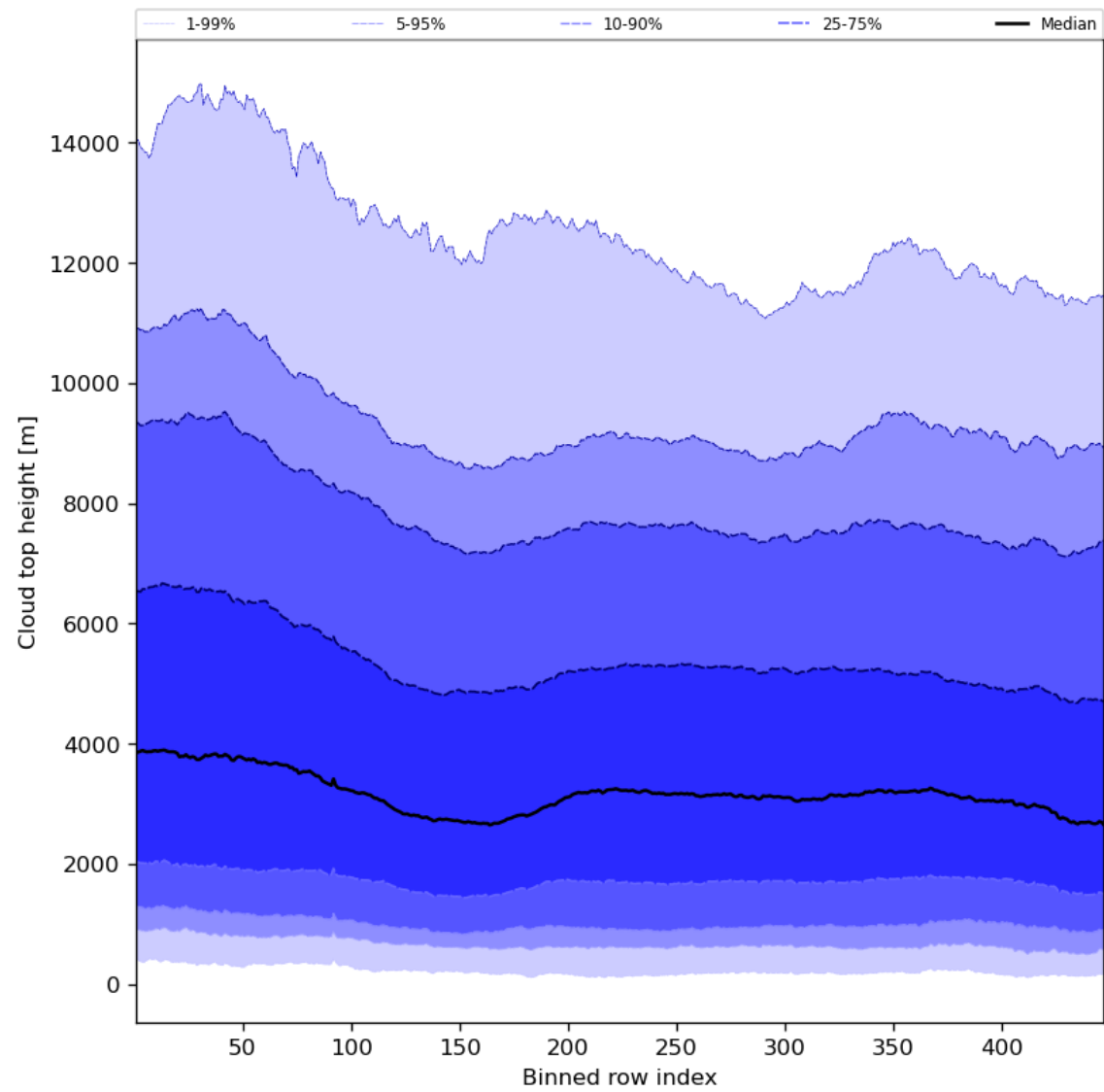
Figure 56: Along track statistics of “Cloud top height” for 2023-09-06 to 2023-09-08
