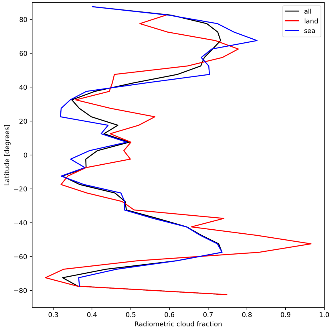
Figure 23: Zonal average of “Radiometric cloud fraction” for 2023-09-06 to 2023-09-08.
