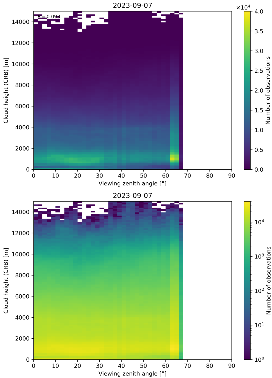
Figure 110: Scatter density plot of “Viewing zenith angle” against “Cloud height (CRB)” for 2023-09-06 to 2023-09-08.
