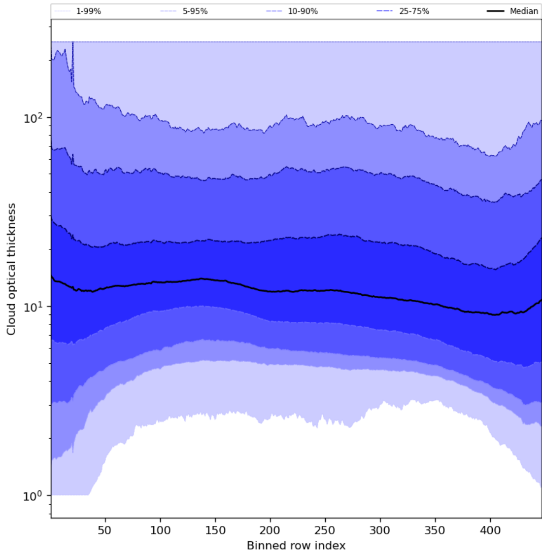
Figure 57: Along track statistics of “Cloud optical thickness” for 2023-09-06 to 2023-09-08
