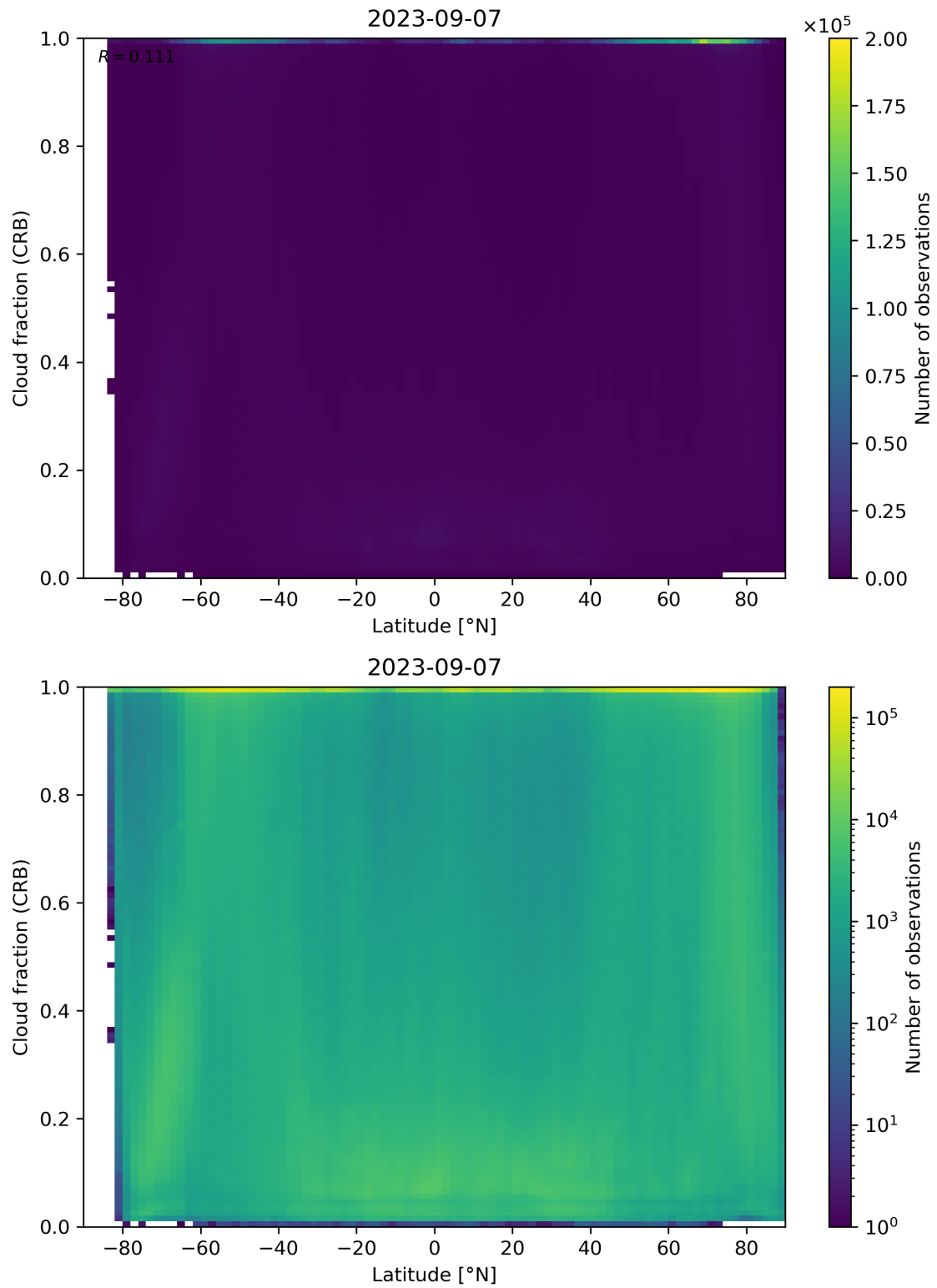
Figure 94: Scatter density plot of “Latitude” against “Cloud fraction (CRB)” for 2023-09-06 to 2023-09-08.
