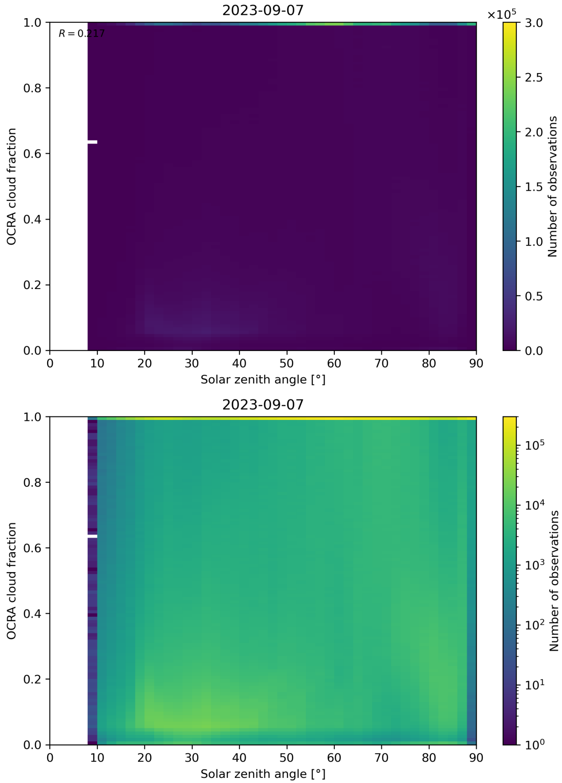
Figure 100: Scatter density plot of “Solar zenith angle” against “OCRA cloud fraction” for 2023-09-06 to 2023-09-08.
