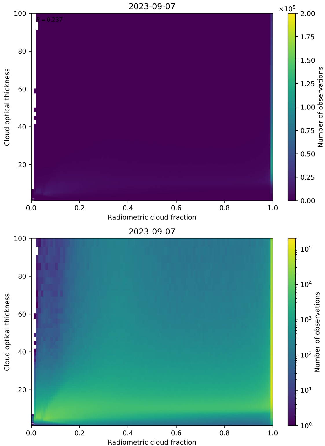
Figure 75: Scatter density plot of “Radiometric cloud fraction” against “Cloud optical thickness” for 2023-09-06 to 2023-09-08.
