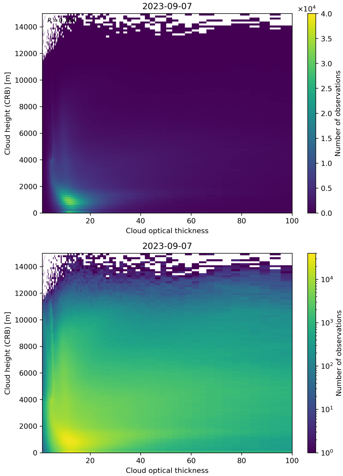
Figure 85: Scatter density plot of “Cloud optical thickness” against “Cloud height (CRB)” for 2023-09-06 to 2023-09-08.
