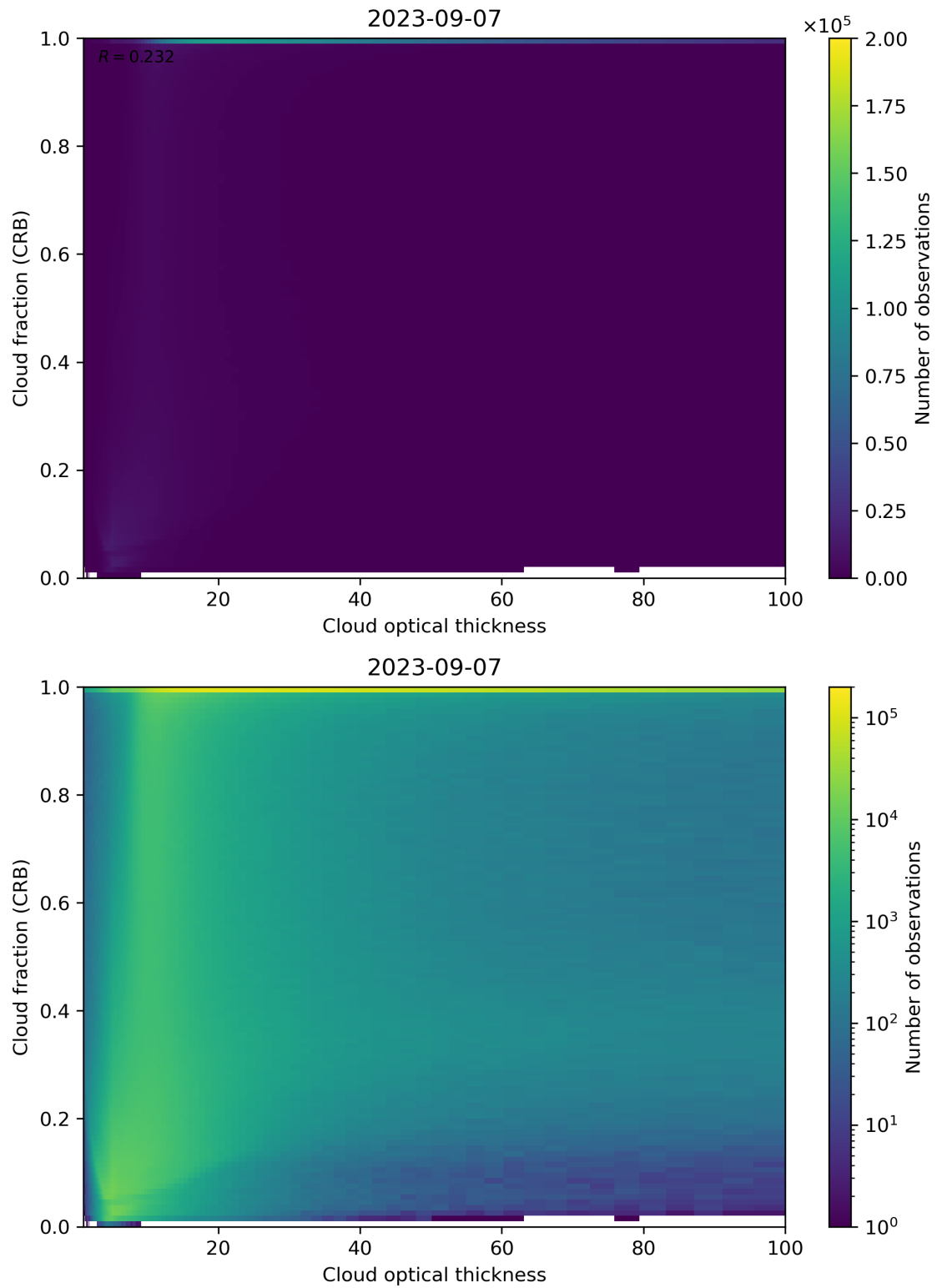
Figure 84: Scatter density plot of “Cloud optical thickness” against “Cloud fraction (CRB)” for 2023-09-06 to 2023-09-08.
