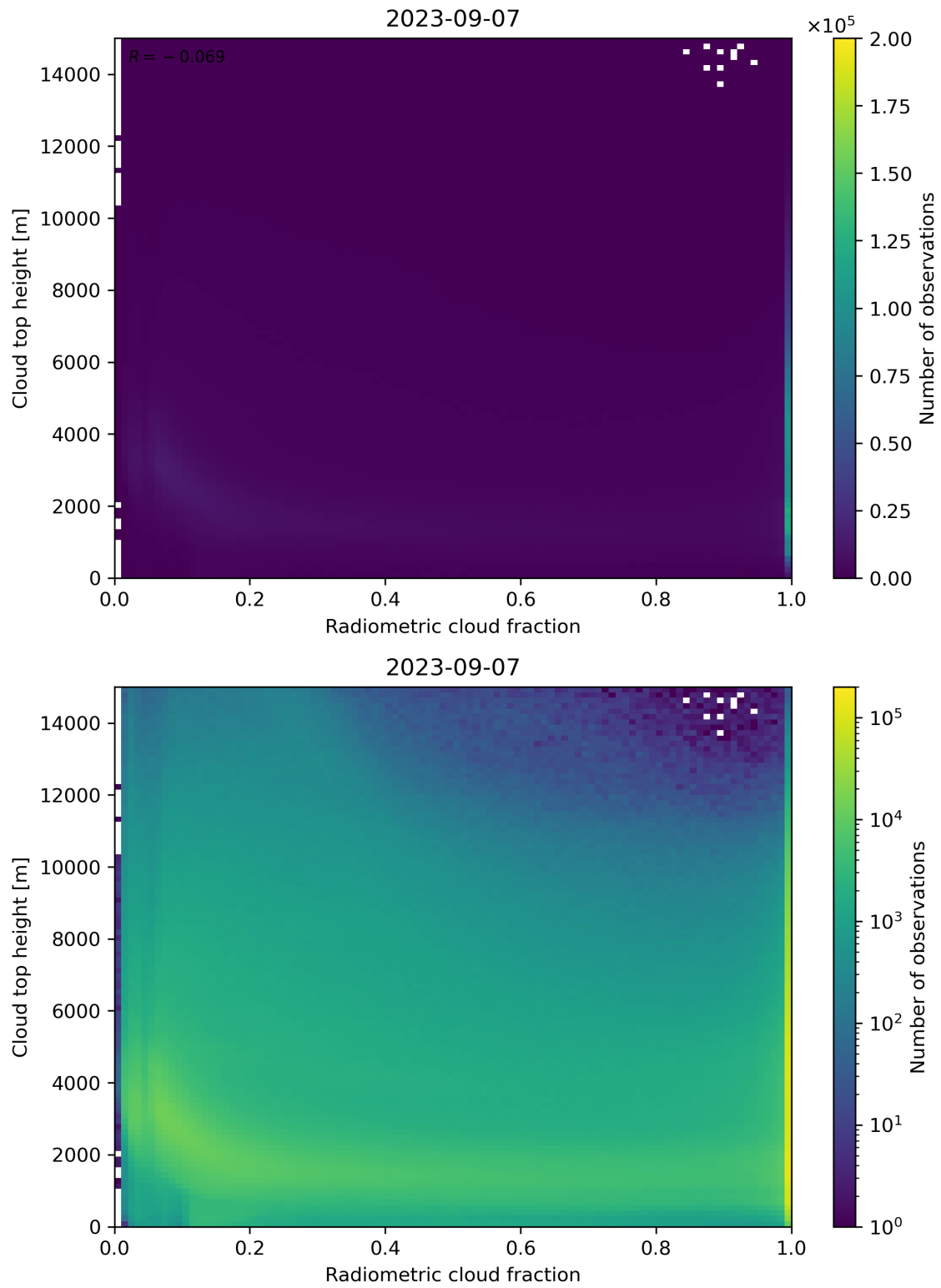
Figure 76: Scatter density plot of “Radiometric cloud fraction” against “Cloud top height” for 2023-09-06 to 2023-09-08.
