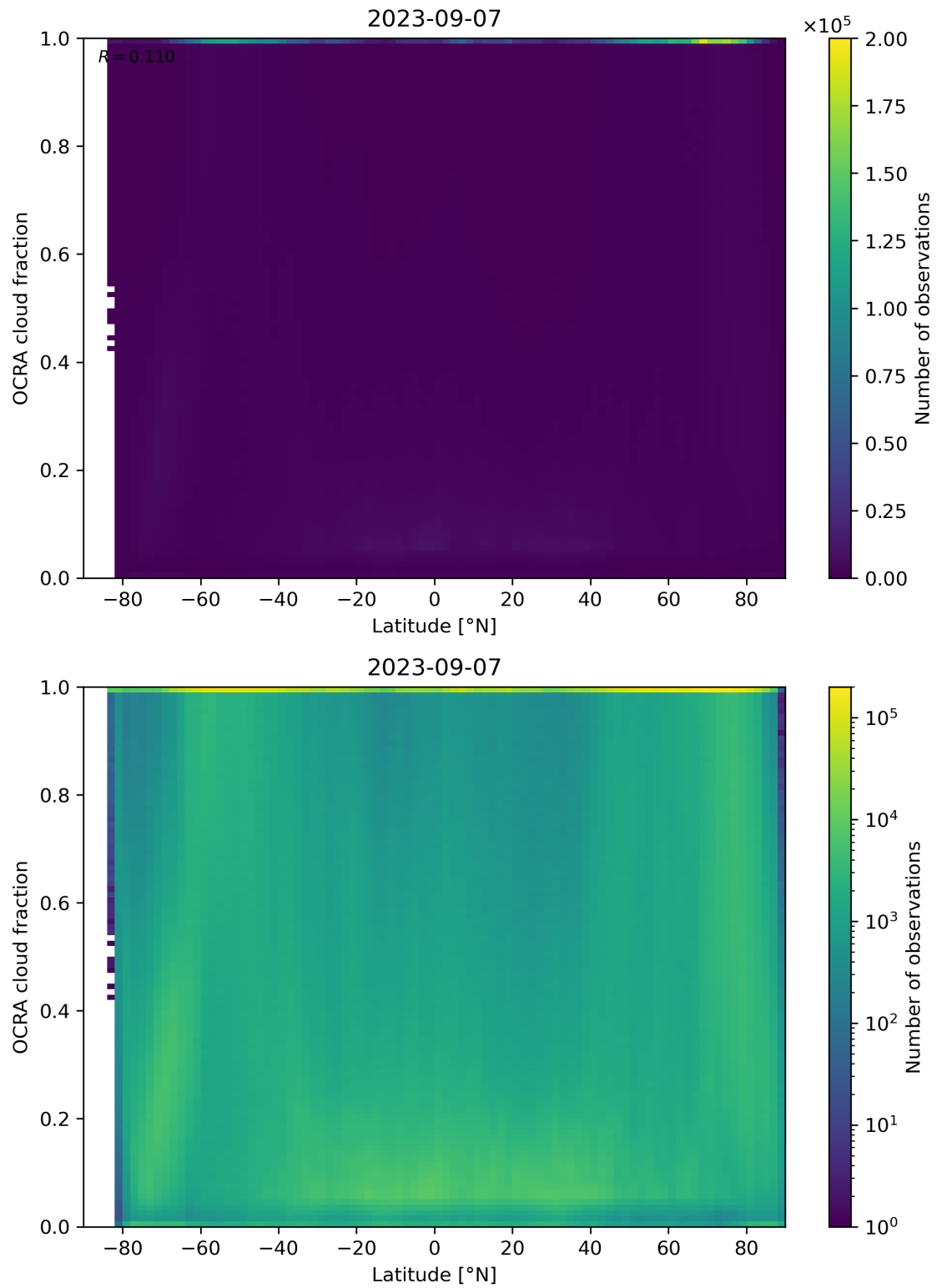
Figure 93: Scatter density plot of “Latitude” against “OCRA cloud fraction” for 2023-09-06 to 2023-09-08.
