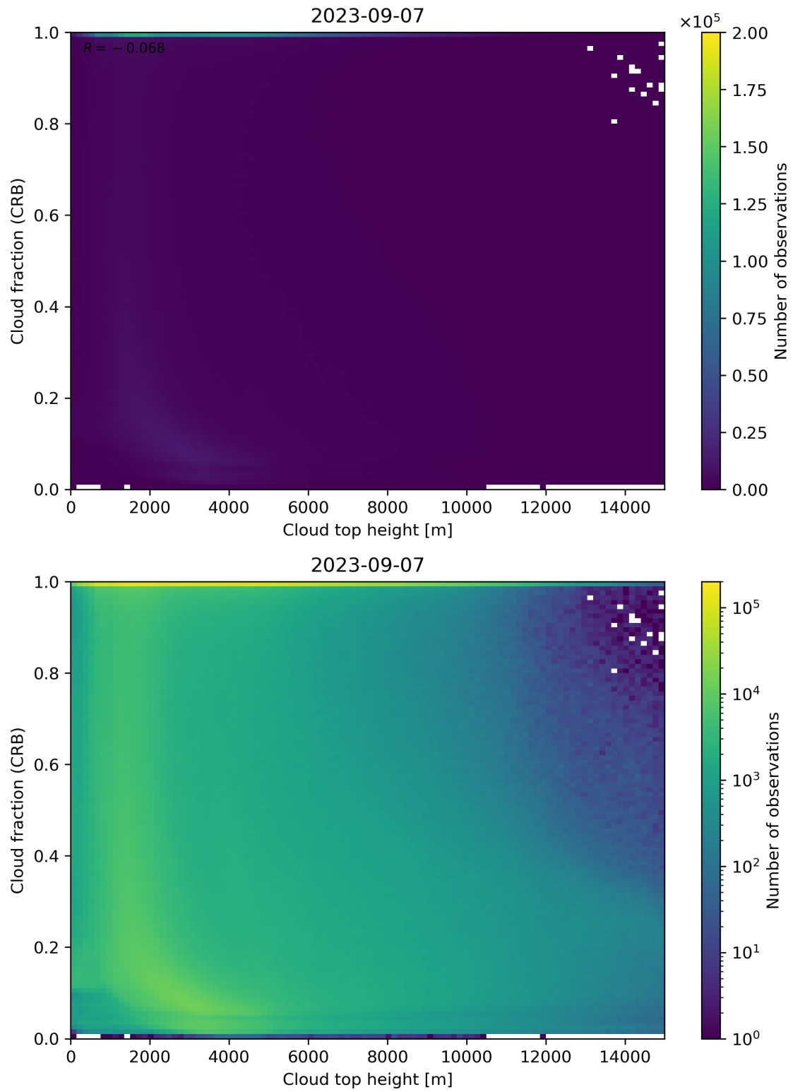
Figure 88: Scatter density plot of “Cloud top height” against “Cloud fraction (CRB)” for 2023-09-06 to 2023-09-08.
