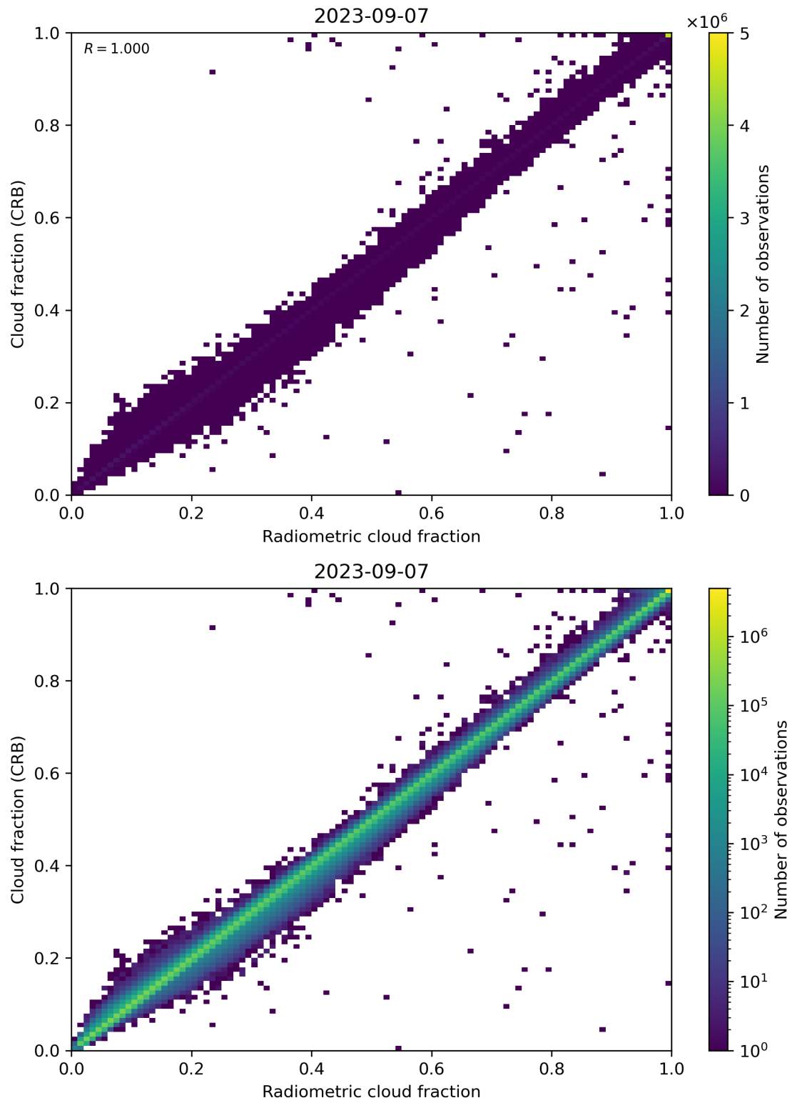
Figure 73: Scatter density plot of “Radiometric cloud fraction” against “Cloud fraction (CRB)” for 2023-09-06 to 2023-09-08.
