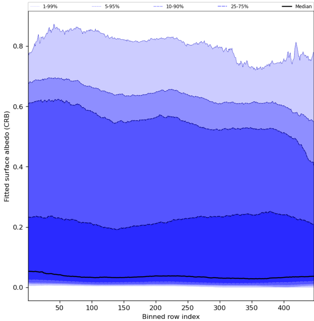
Figure 62: Along track statistics of “Fitted surface albedo (CRB)” for 2023-09-06 to 2023-09-08
