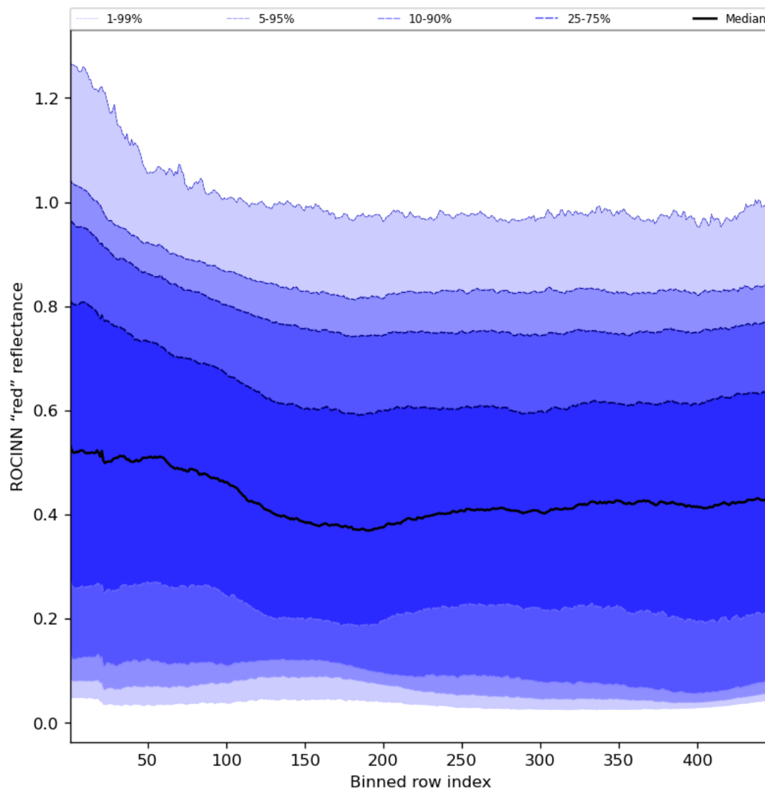
Figure 69: Along track statistics of “ROCINN “red” reflectance” for 2023-09-06 to 2023-09-08
