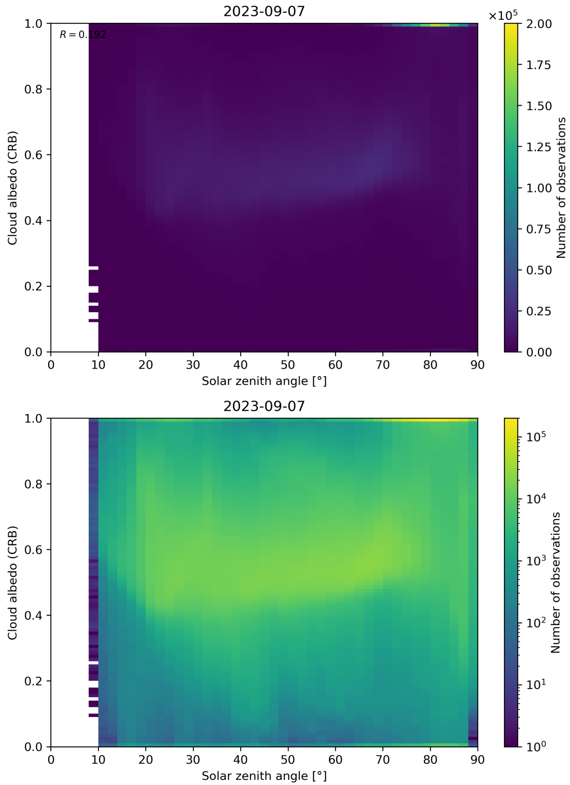
Figure 98: Scatter density plot of “Solar zenith angle” against “Cloud albedo (CRB)” for 2023-09-06 to 2023-09-08.
