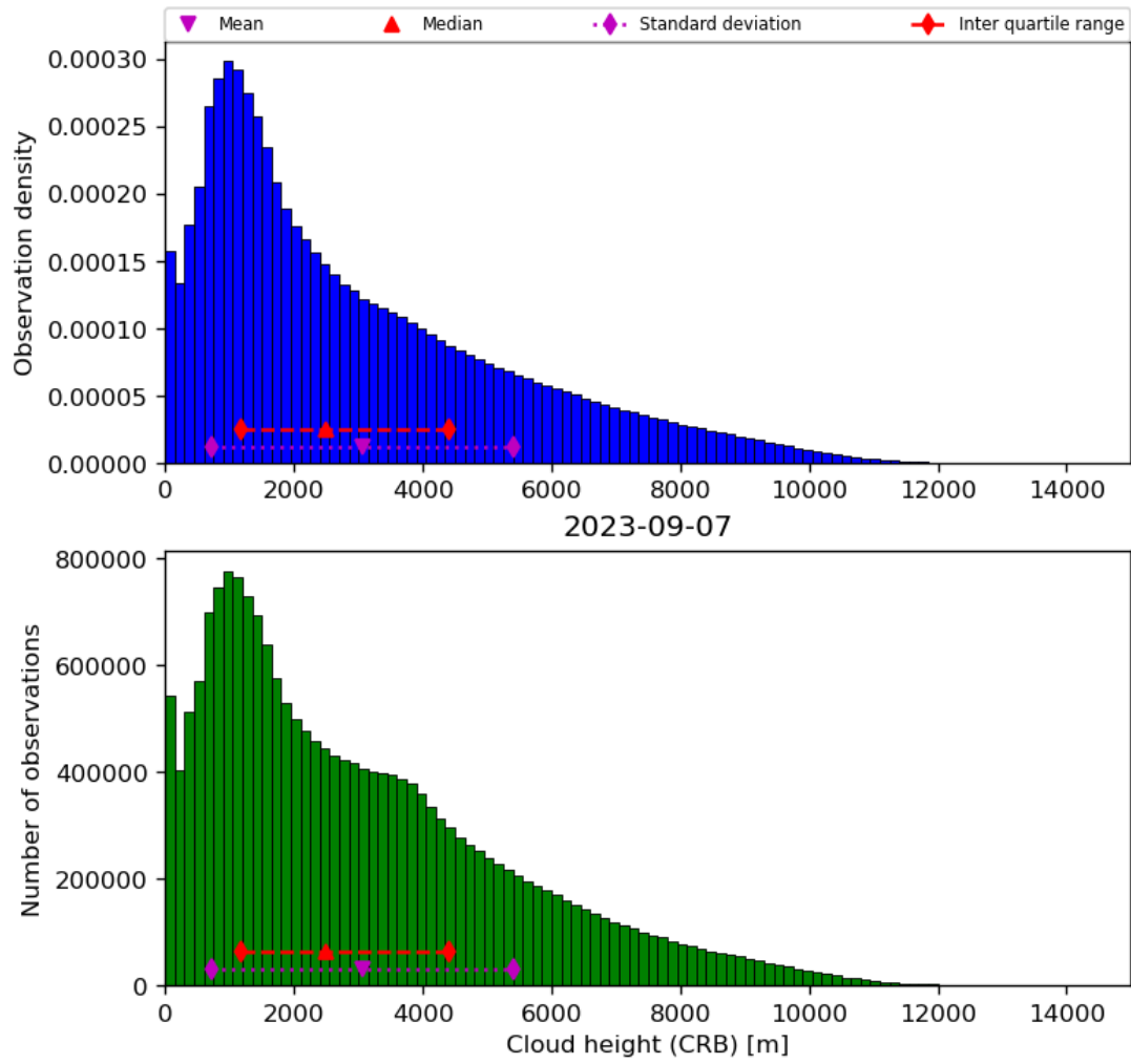
Figure 43: Histogram of “Cloud height (CRB)” for 2023-09-06 to 2023-09-08
