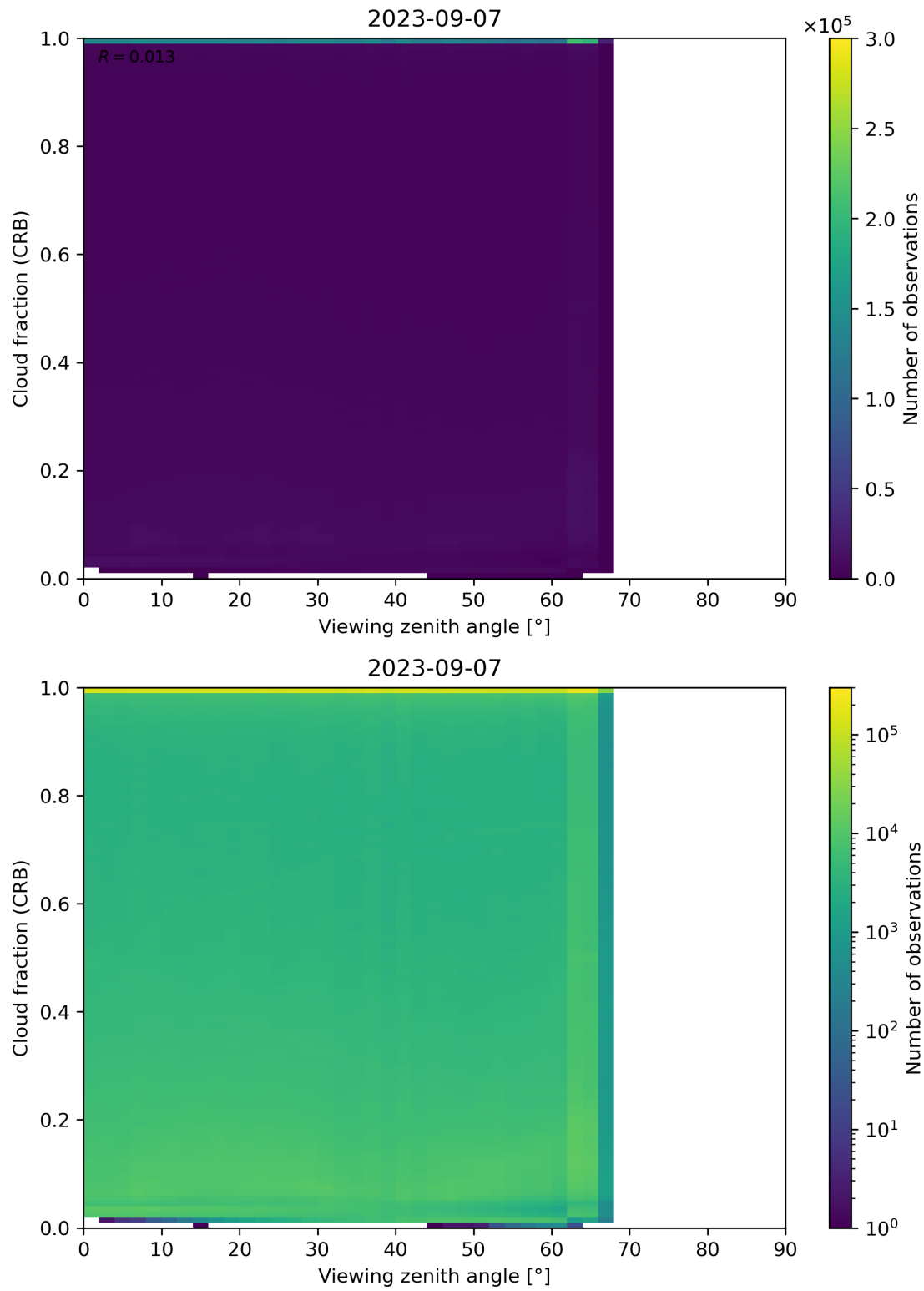
Figure 109: Scatter density plot of “Viewing zenith angle” against “Cloud fraction (CRB)” for 2023-09-06 to 2023-09-08.
