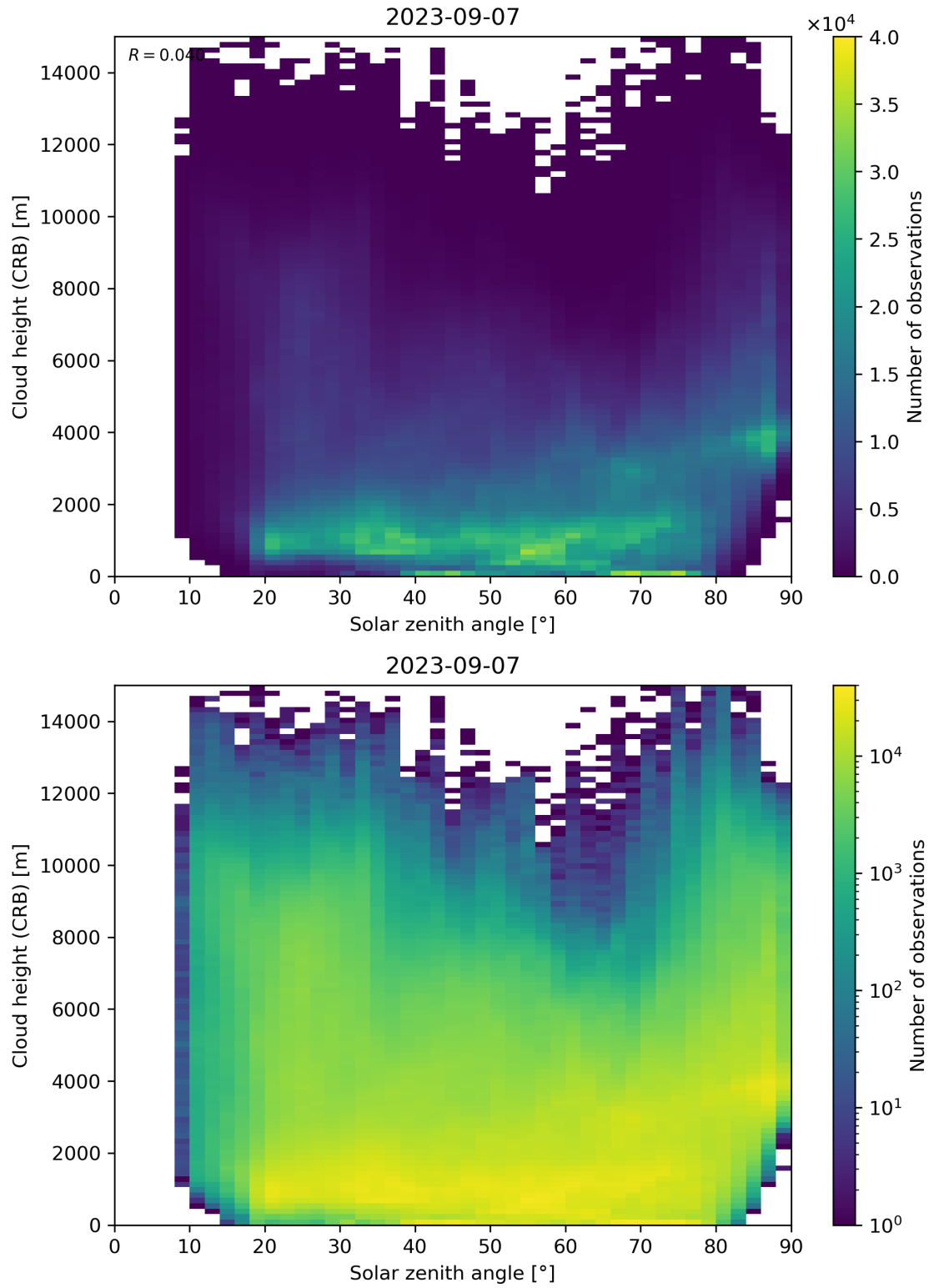
Figure 102: Scatter density plot of “Solar zenith angle” against “Cloud height (CRB)” for 2023-09-06 to 2023-09-08.
