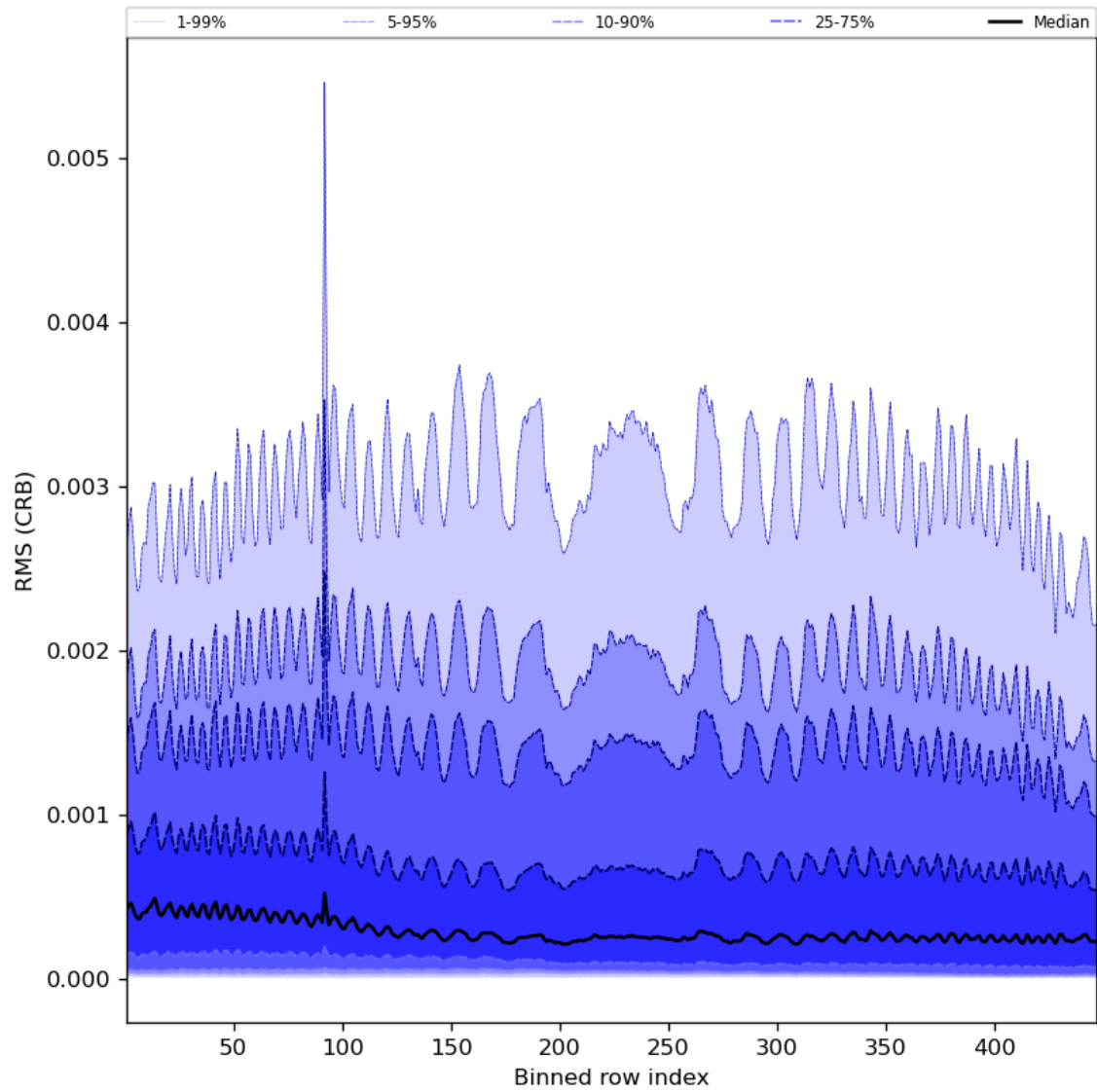
Figure 64: Along track statistics of “RMS (CRB)” for 2023-09-06 to 2023-09-08
