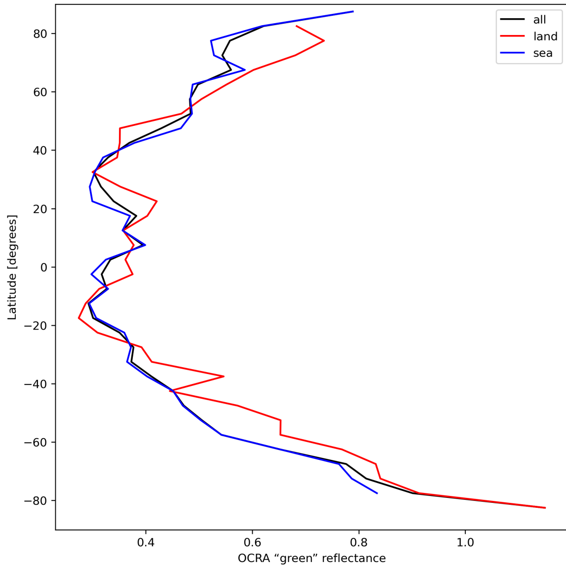
Figure 36: Zonal average of “OCRA “green” reflectance” for 2023-09-06 to 2023-09-08.
