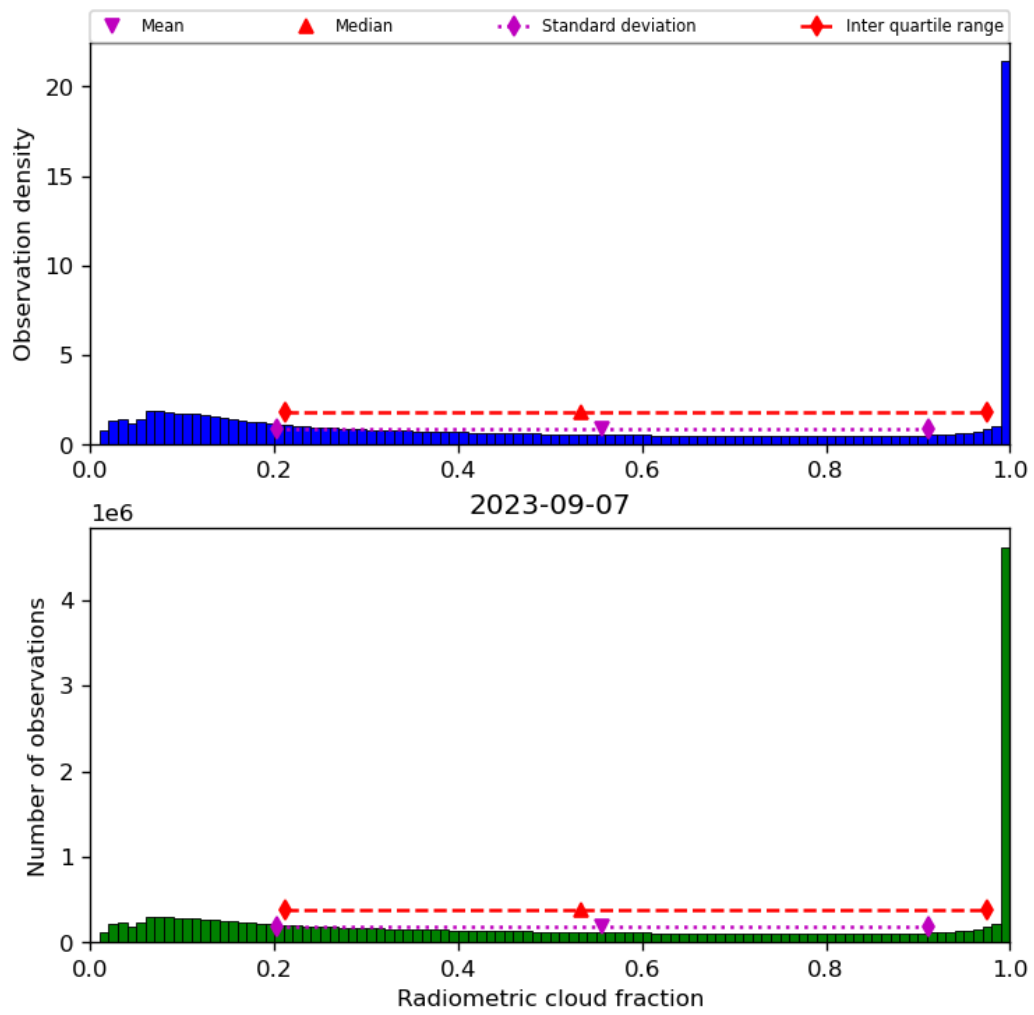
Figure 39: Histogram of “Radiometric cloud fraction” for 2023-09-06 to 2023-09-08
