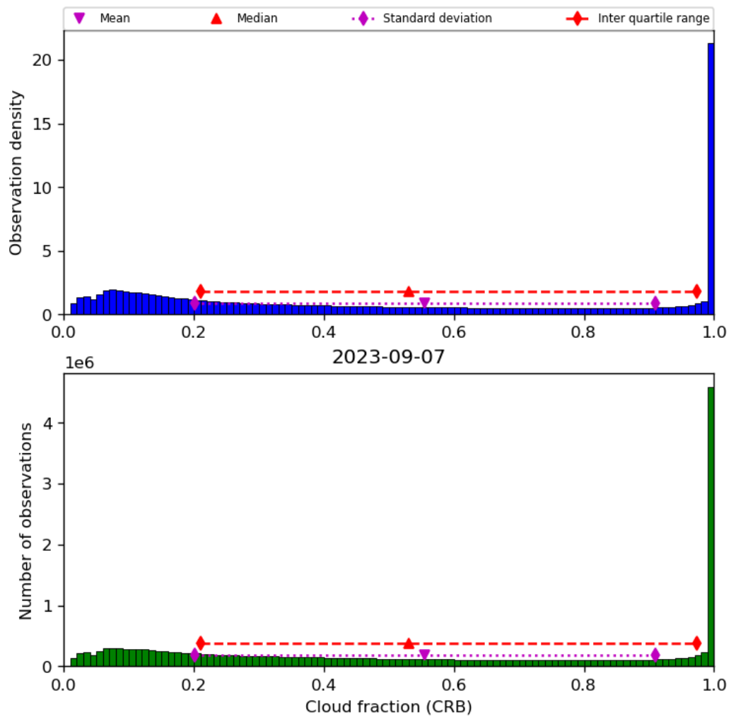
Figure 42: Histogram of “Cloud fraction (CRB)” for 2023-09-06 to 2023-09-08
