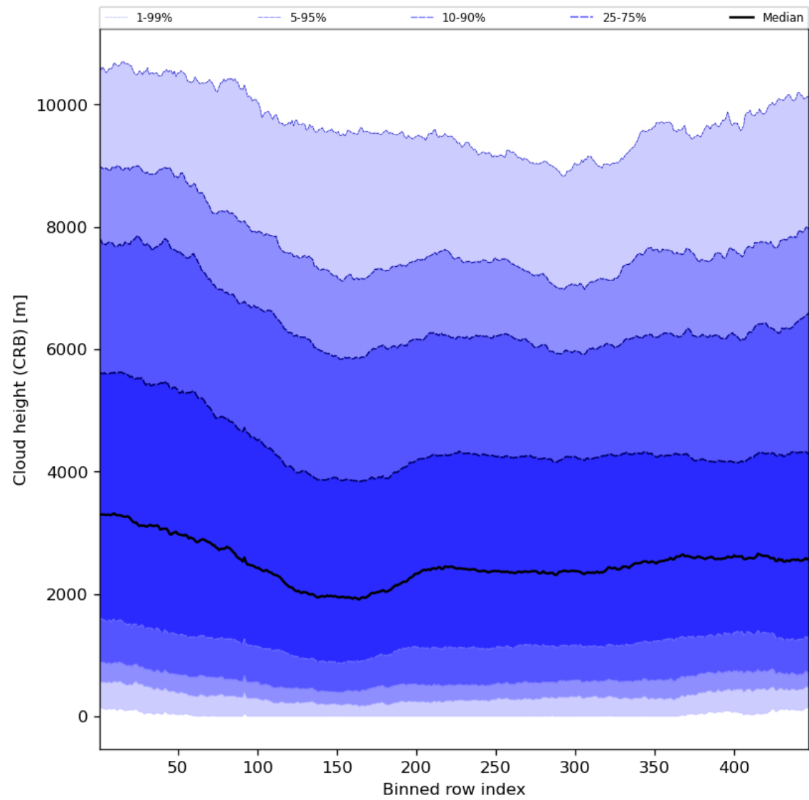
Figure 59: Along track statistics of “Cloud height (CRB)” for 2023-09-06 to 2023-09-08
