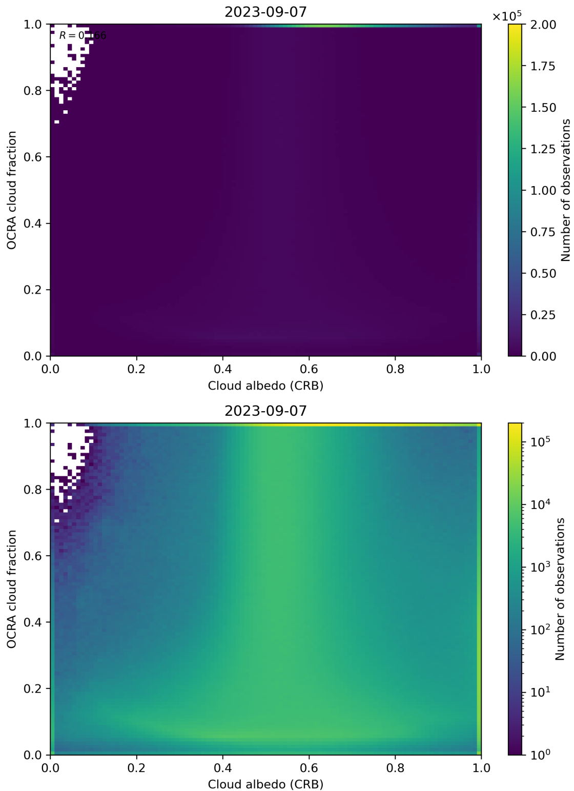
Figure 70: Scatter density plot of “Cloud albedo (CRB)” against “OCRA cloud fraction” for 2023-09-06 to 2023-09-08.
