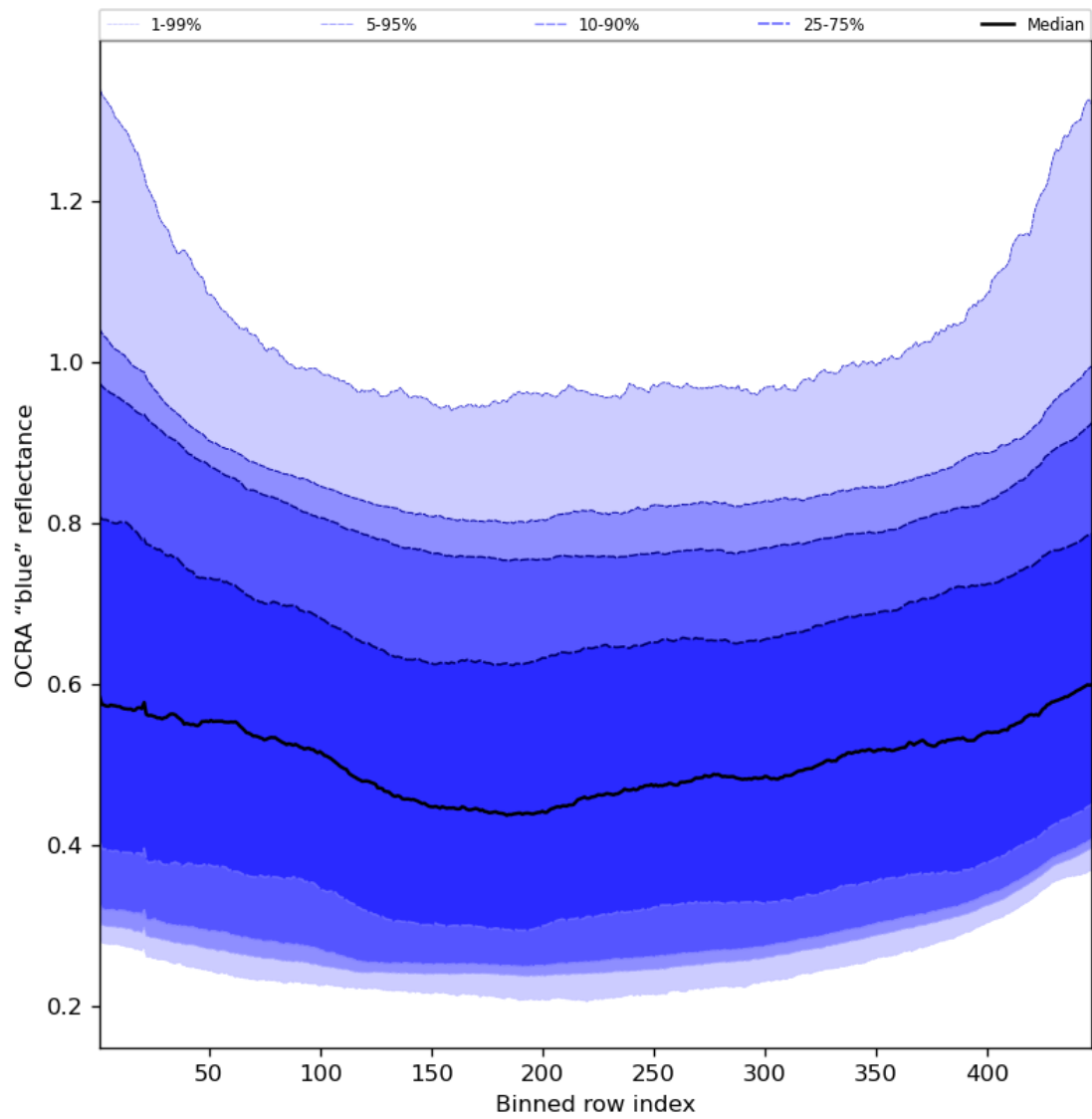
Figure 67: Along track statistics of “OCRA “blue” reflectance” for 2023-09-06 to 2023-09-08
