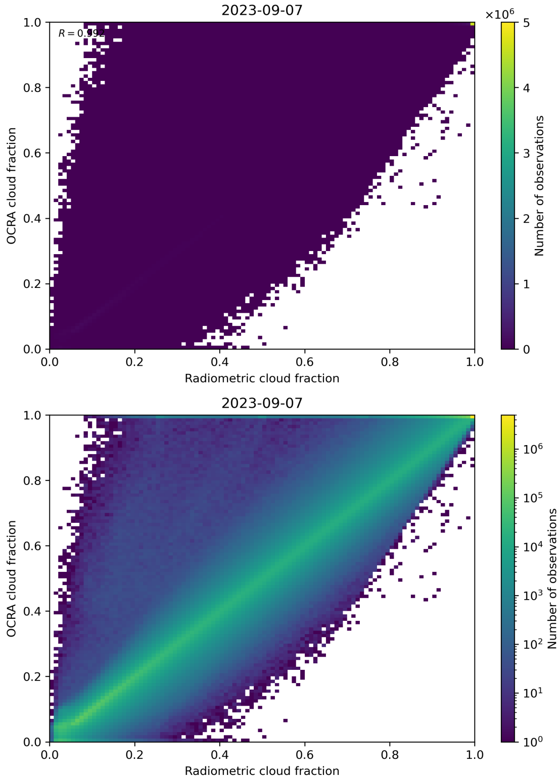
Figure 72: Scatter density plot of “Radiometric cloud fraction” against “OCRA cloud fraction” for 2023-09-06 to 2023-09-08.
