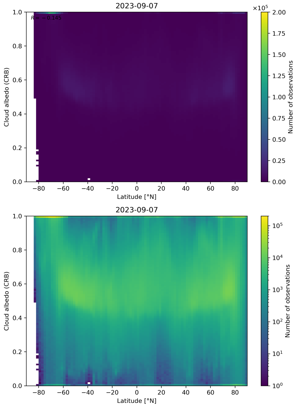
Figure 91: Scatter density plot of “Latitude” against “Cloud albedo (CRB)” for 2023-09-06 to 2023-09-08.
