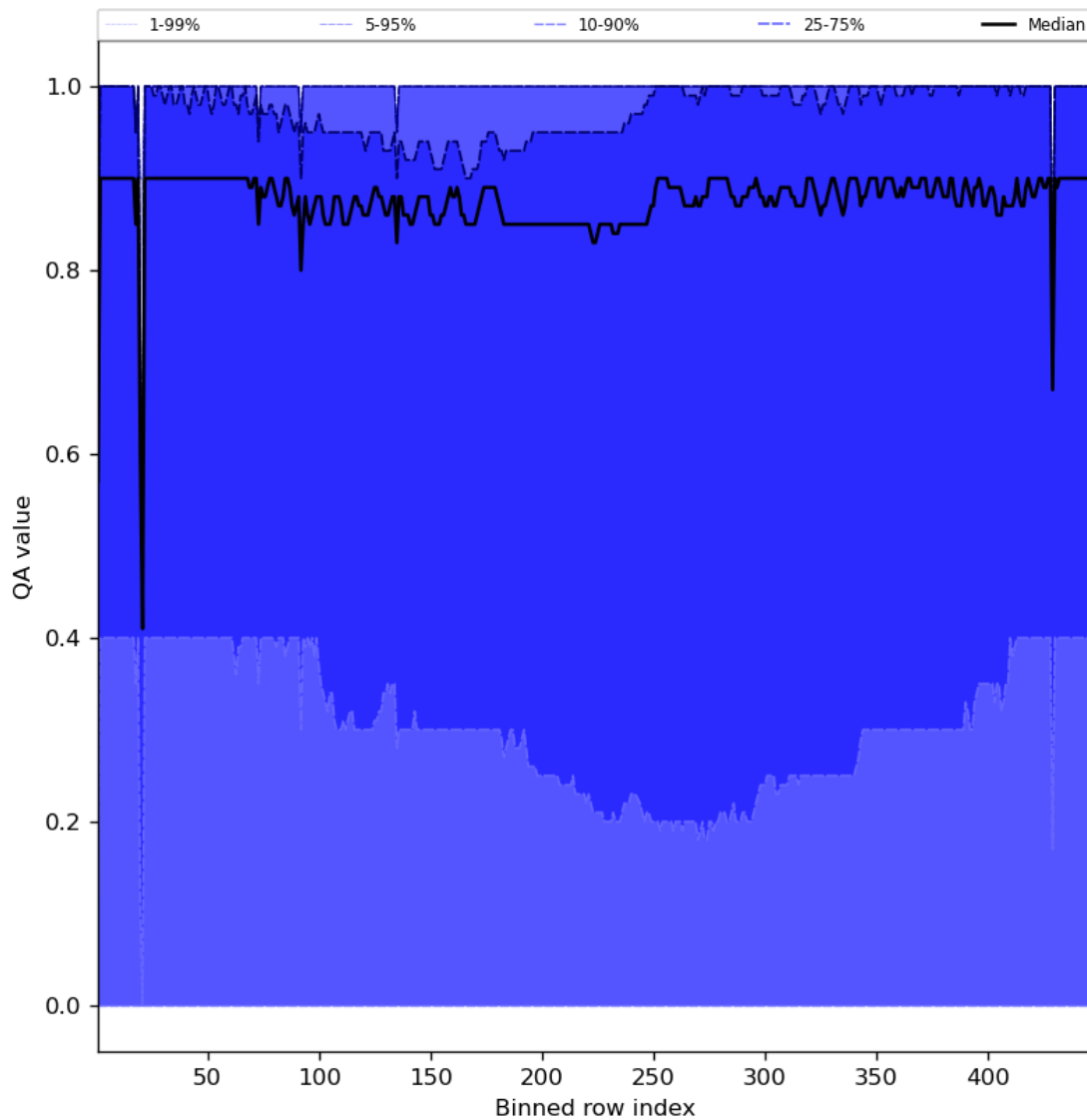
Figure 54: Along track statistics of “QA value” for 2023-09-06 to 2023-09-08
