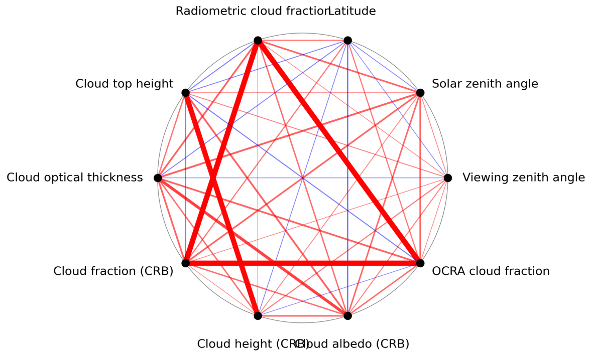
Figure 1: Map of correlation graph for 2023-09-06 to 2023-09-08.
