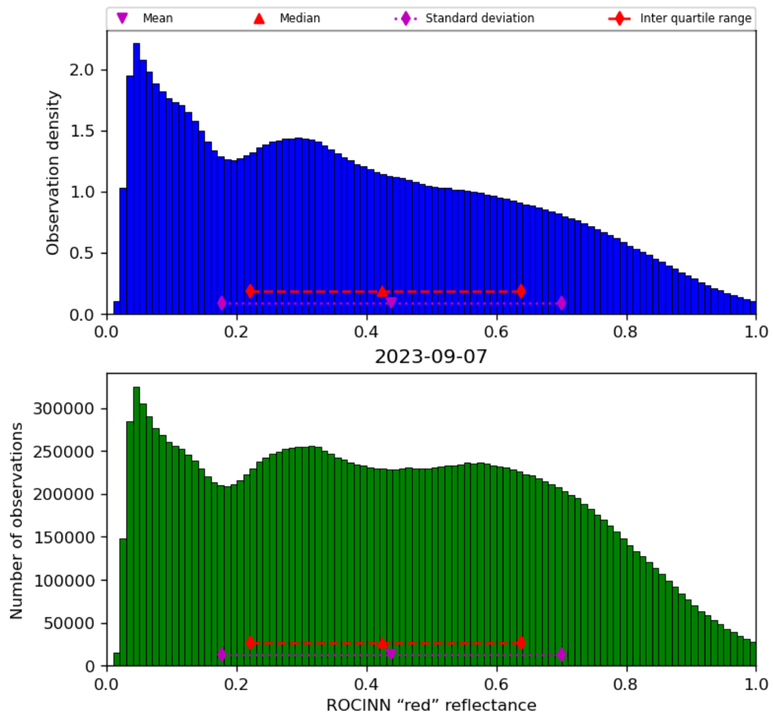
Figure 53: Histogram of “ROCINN “red” reflectance” for 2023-09-06 to 2023-09-08
