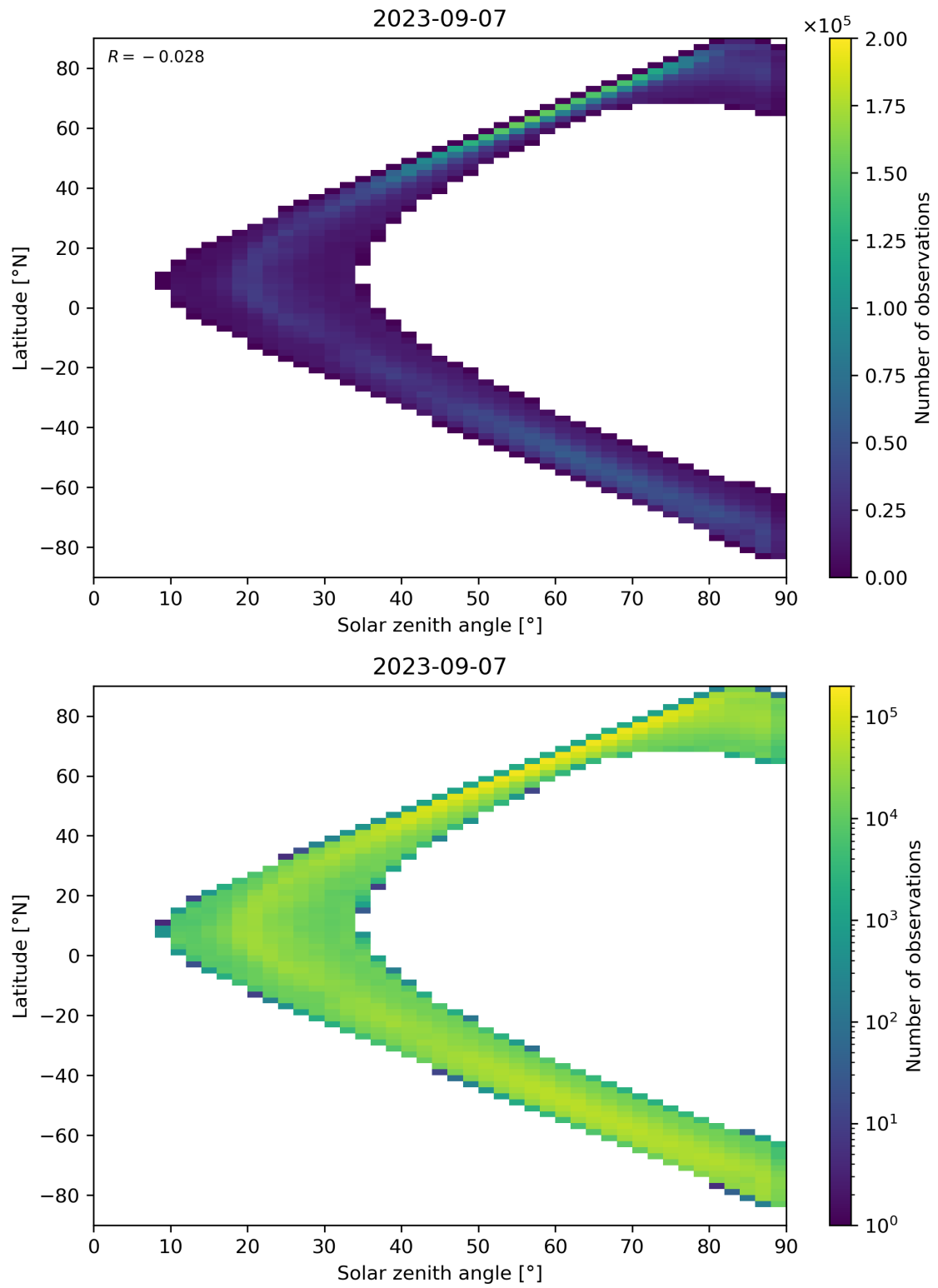
Figure 105: Scatter density plot of “Solar zenith angle” against “Latitude” for 2023-09-06 to 2023-09-08.
