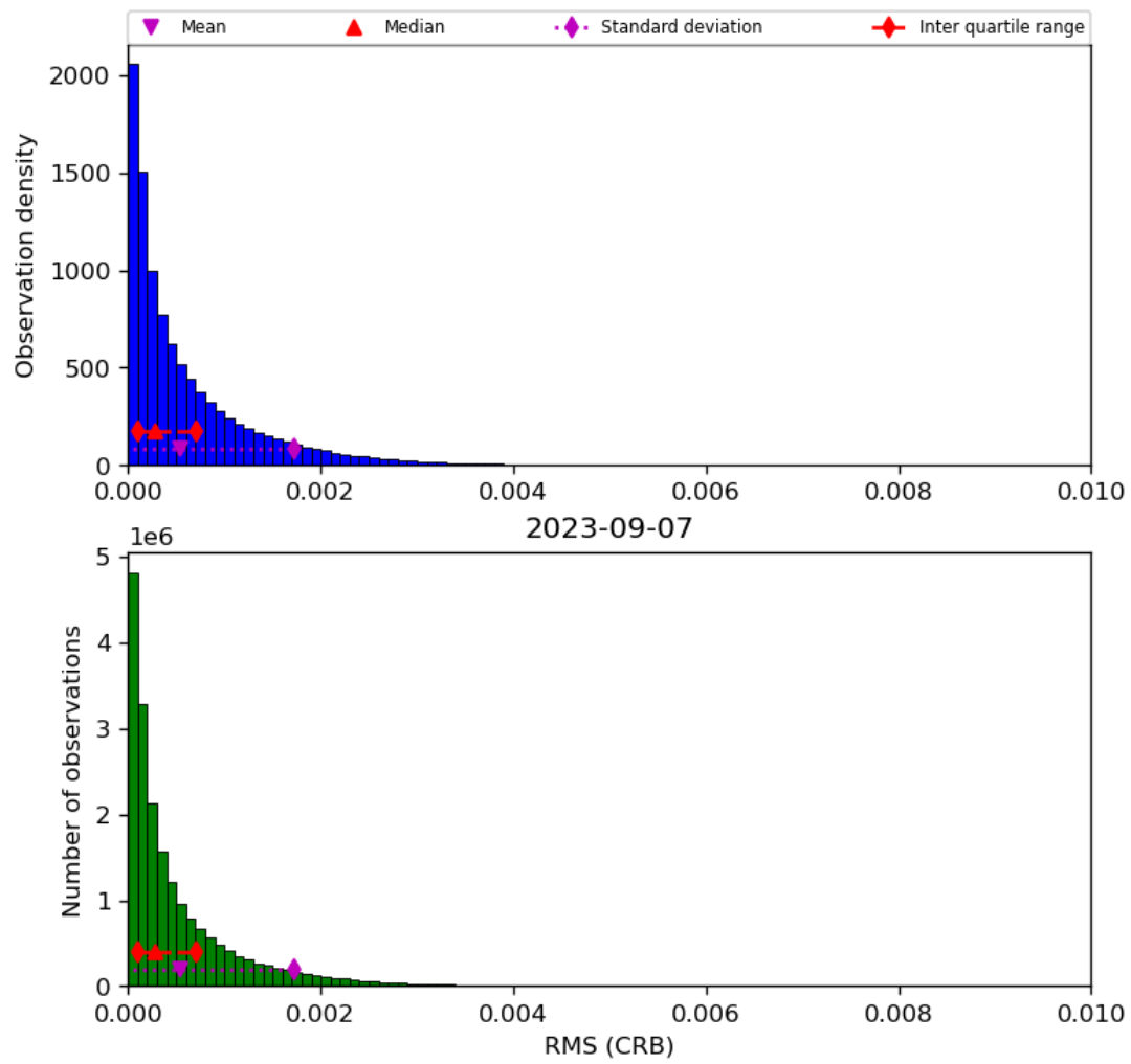
Figure 48: Histogram of “RMS (CRB)” for 2023-09-06 to 2023-09-08
