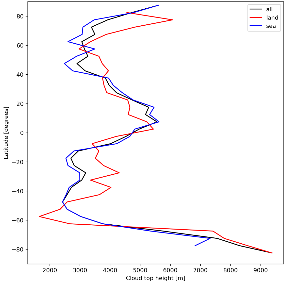
Figure 24: Zonal average of “Cloud top height” for 2023-09-06 to 2023-09-08.
