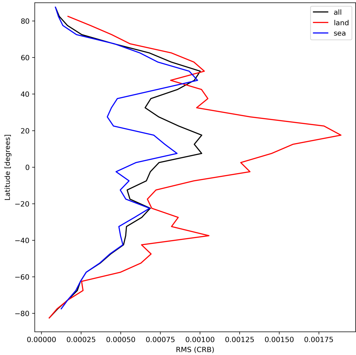
Figure 32: Zonal average of “RMS (CRB)” for 2023-09-06 to 2023-09-08.
