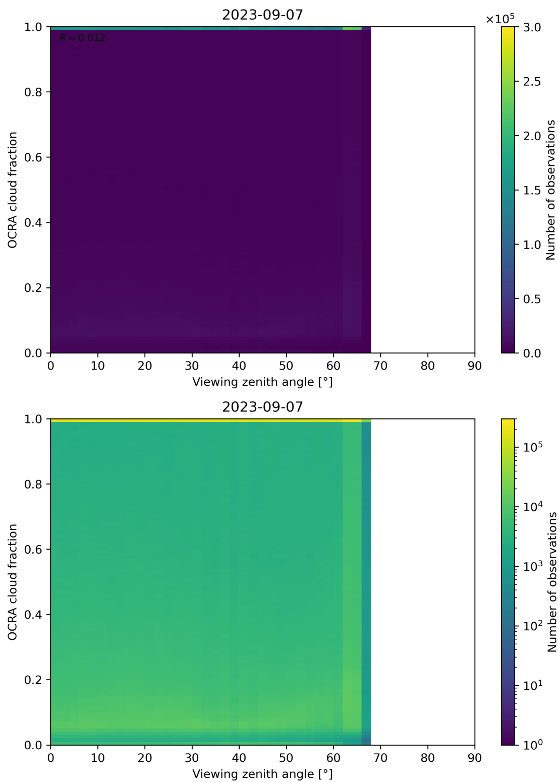
Figure 108: Scatter density plot of “Viewing zenith angle” against “OCRA cloud fraction” for 2023-09-06 to 2023-09-08.
