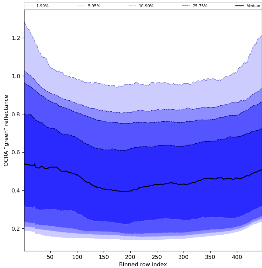
Figure 68: Along track statistics of “OCRA “green” reflectance” for 2023-09-06 to 2023-09-08
