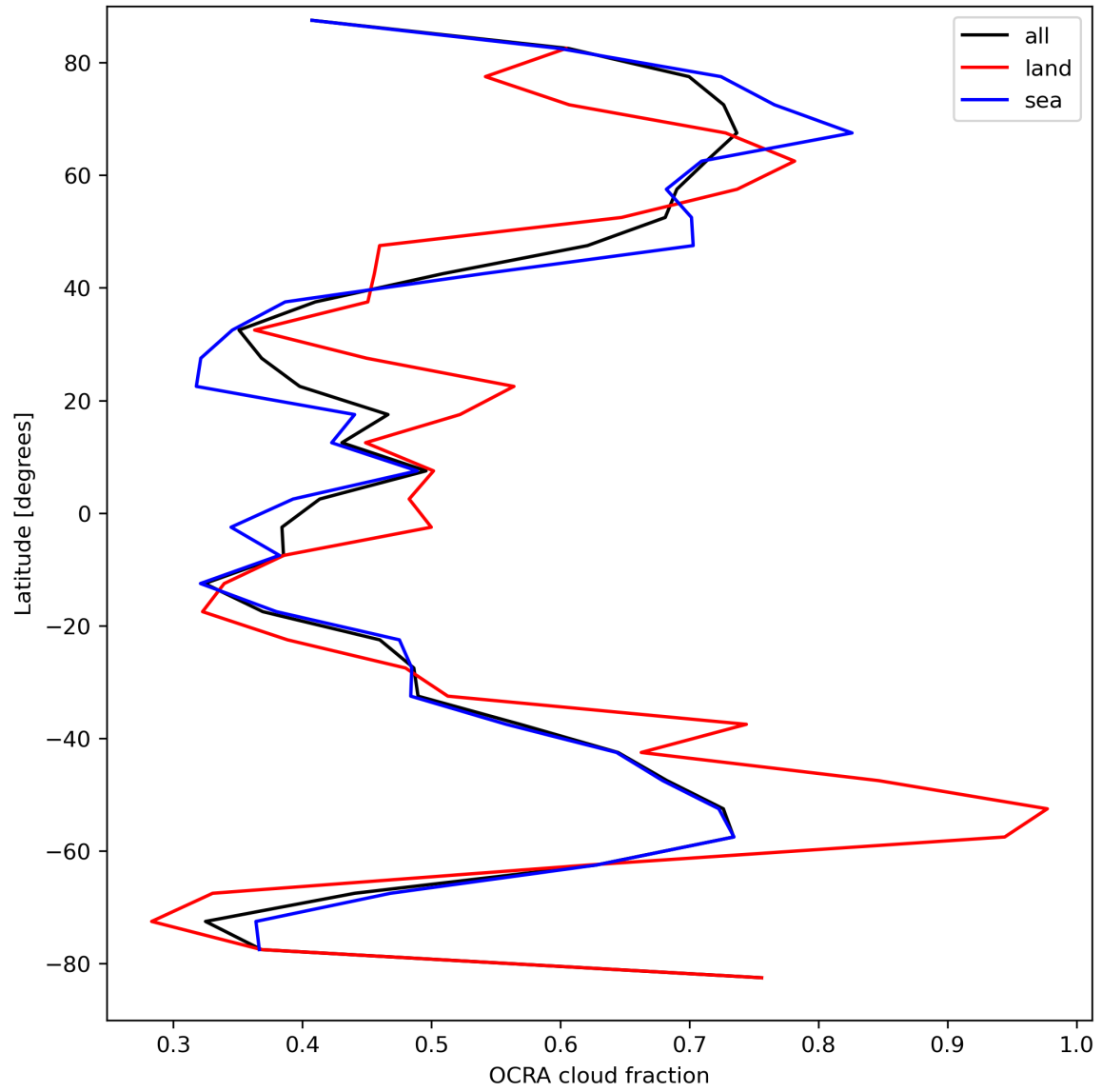
Figure 34: Zonal average of “OCRA cloud fraction” for 2023-09-06 to 2023-09-08.
