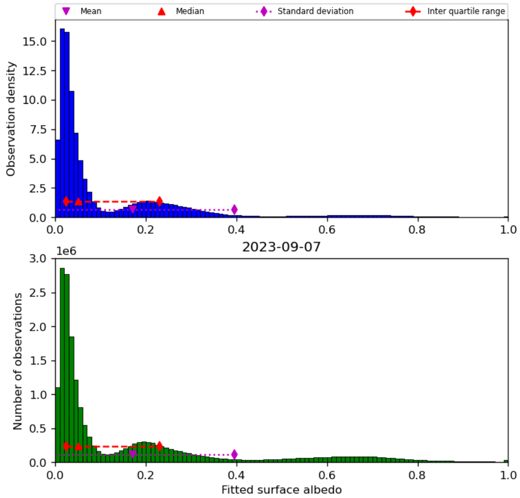
Figure 45: Histogram of “Fitted surface albedo” for 2023-09-06 to 2023-09-08
