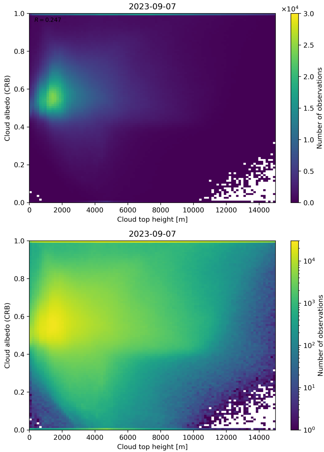
Figure 86: Scatter density plot of “Cloud top height” against “Cloud albedo (CRB)” for 2023-09-06 to 2023-09-08.
