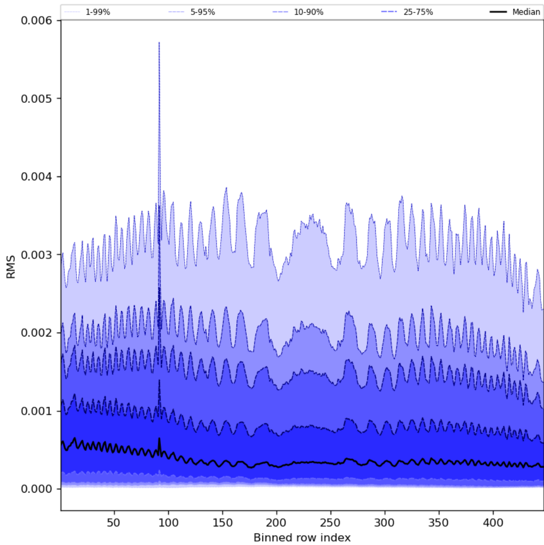
Figure 63: Along track statistics of “RMS” for 2023-09-06 to 2023-09-08
