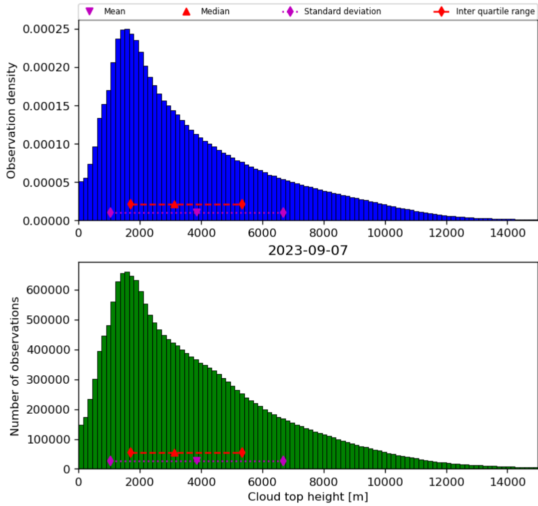
Figure 40: Histogram of “Cloud top height” for 2023-09-06 to 2023-09-08
