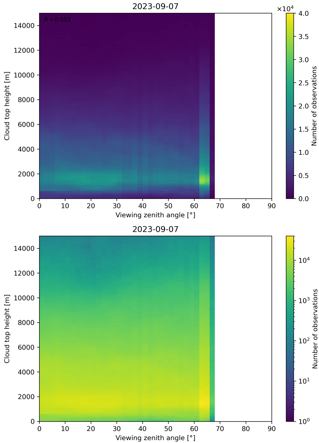
Figure 112: Scatter density plot of “Viewing zenith angle” against “Cloud top height” for 2023-09-06 to 2023-09-08.
