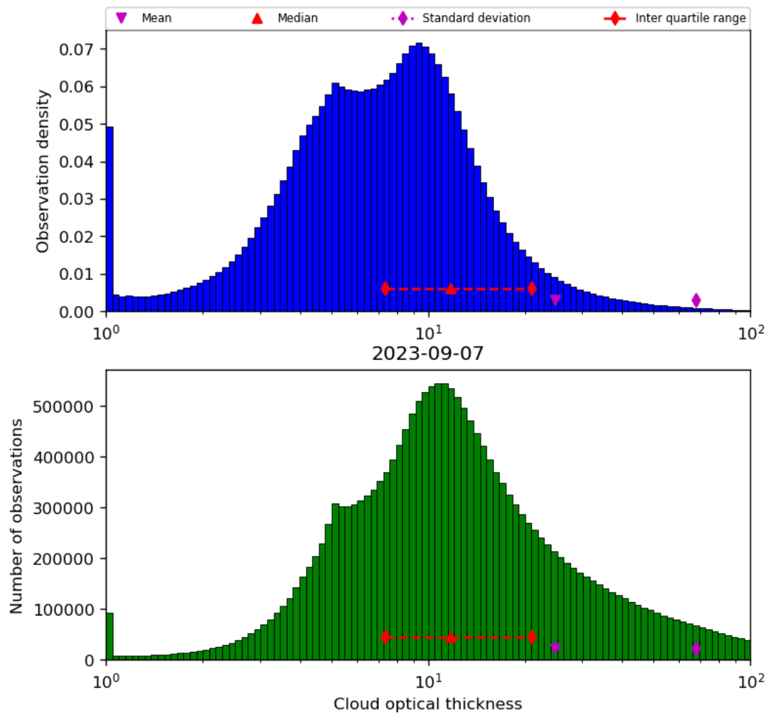
Figure 41: Histogram of “Cloud optical thickness” for 2023-09-06 to 2023-09-08
