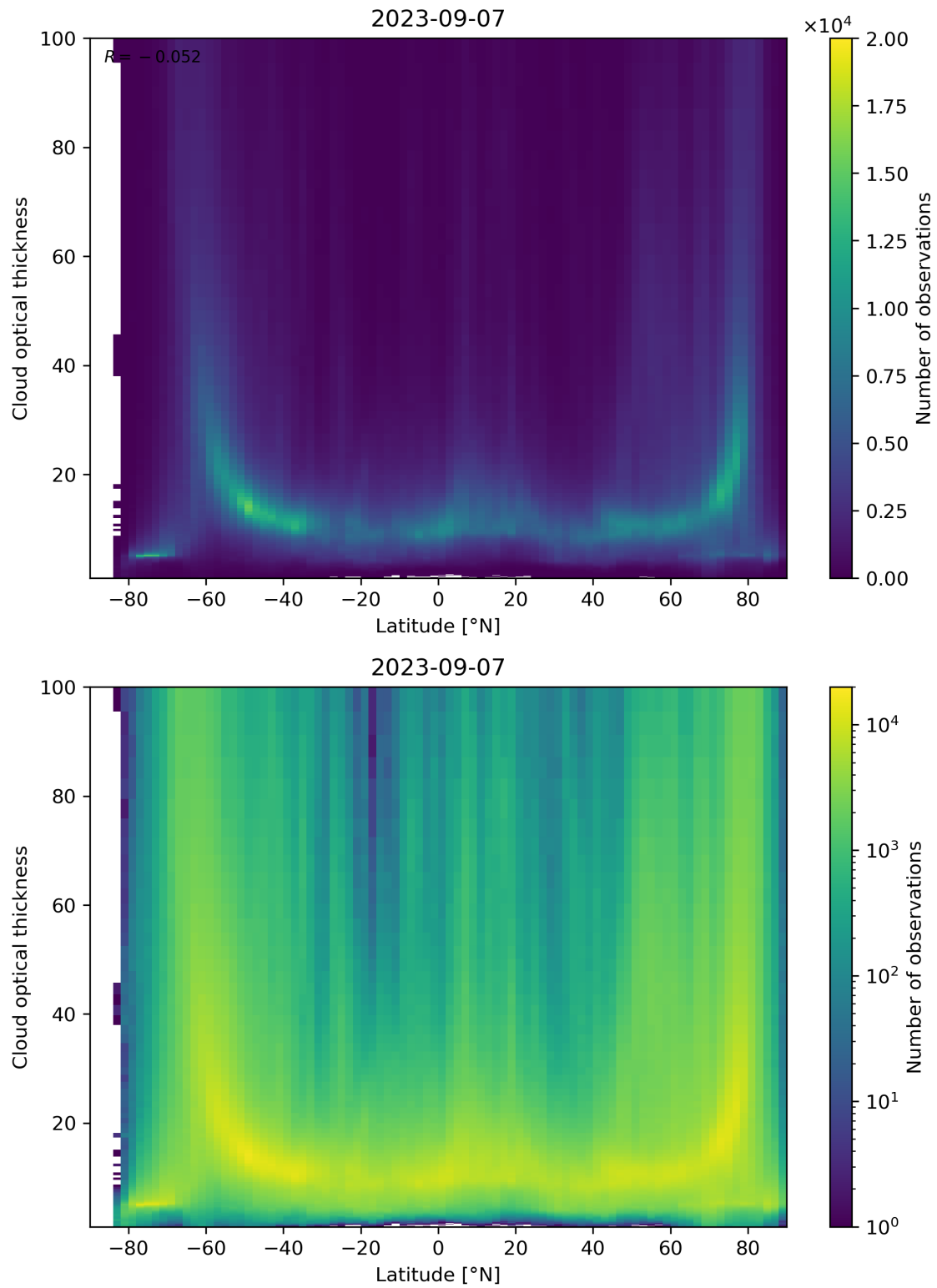
Figure 96: Scatter density plot of “Latitude” against “Cloud optical thickness” for 2023-09-06 to 2023-09-08.
