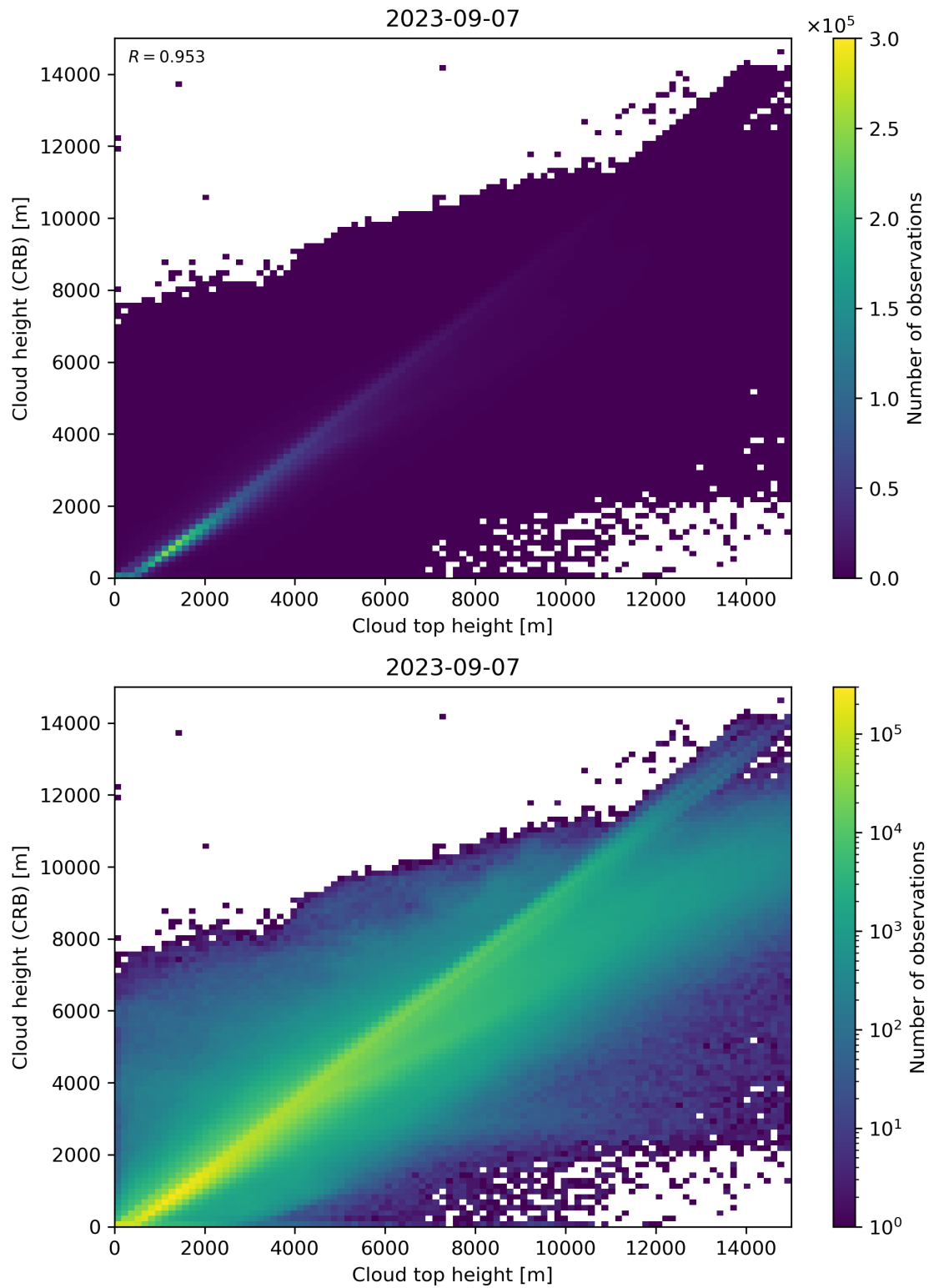
Figure 89: Scatter density plot of “Cloud top height” against “Cloud height (CRB)” for 2023-09-06 to 2023-09-08.
