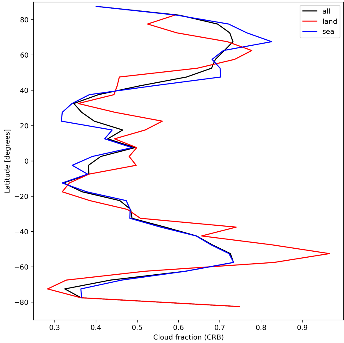
Figure 26: Zonal average of “Cloud fraction (CRB)” for 2023-09-06 to 2023-09-08.
