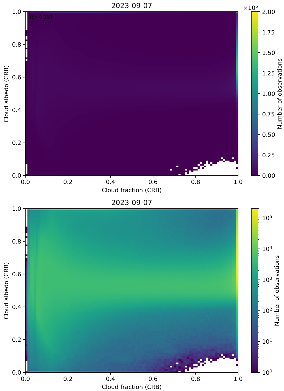
Figure 77: Scatter density plot of “Cloud fraction (CRB)” against “Cloud albedo (CRB)” for 2023-09-06 to 2023-09-08.
