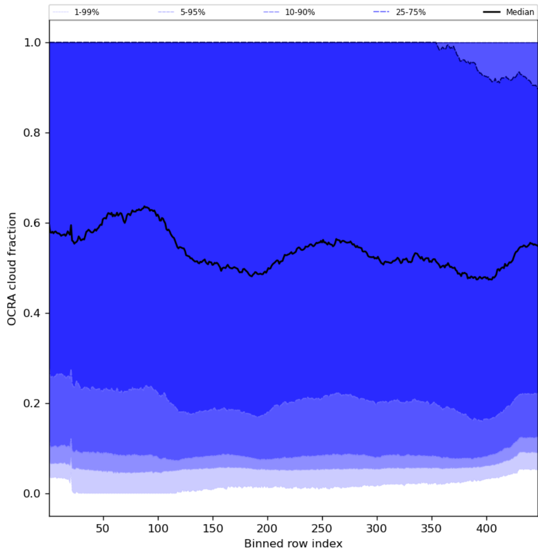
Figure 66: Along track statistics of “OCRA cloud fraction” for 2023-09-06 to 2023-09-08
