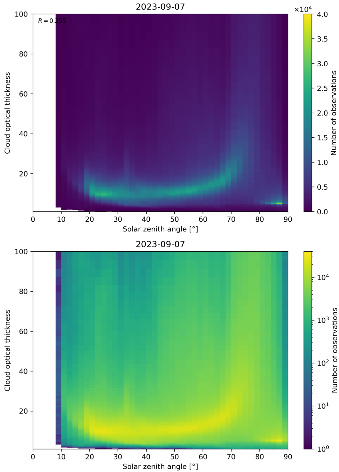
Figure 103: Scatter density plot of “Solar zenith angle” against “Cloud optical thickness” for 2023-09-06 to 2023-09-08.
