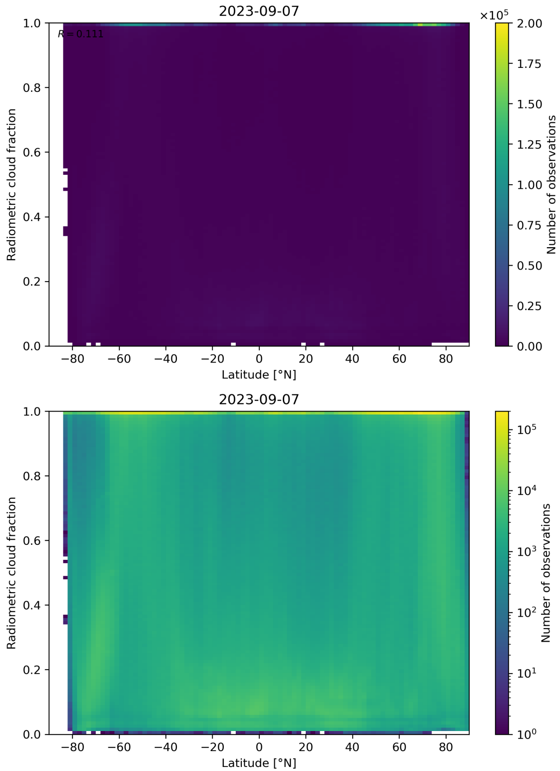
Figure 92: Scatter density plot of “Latitude” against “Radiometric cloud fraction” for 2023-09-06 to 2023-09-08.
