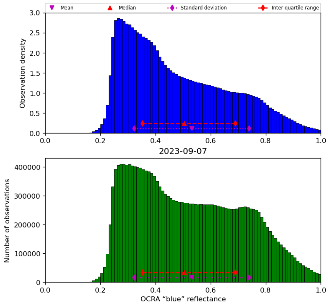
Figure 51: Histogram of “OCRA “blue” reflectance” for 2023-09-06 to 2023-09-08
