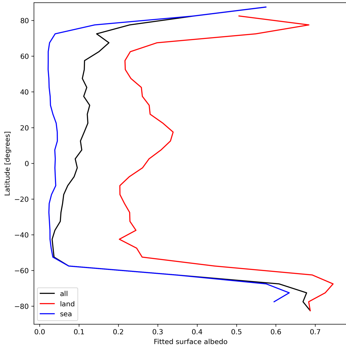
Figure 29: Zonal average of “Fitted surface albedo” for 2023-09-06 to 2023-09-08.
