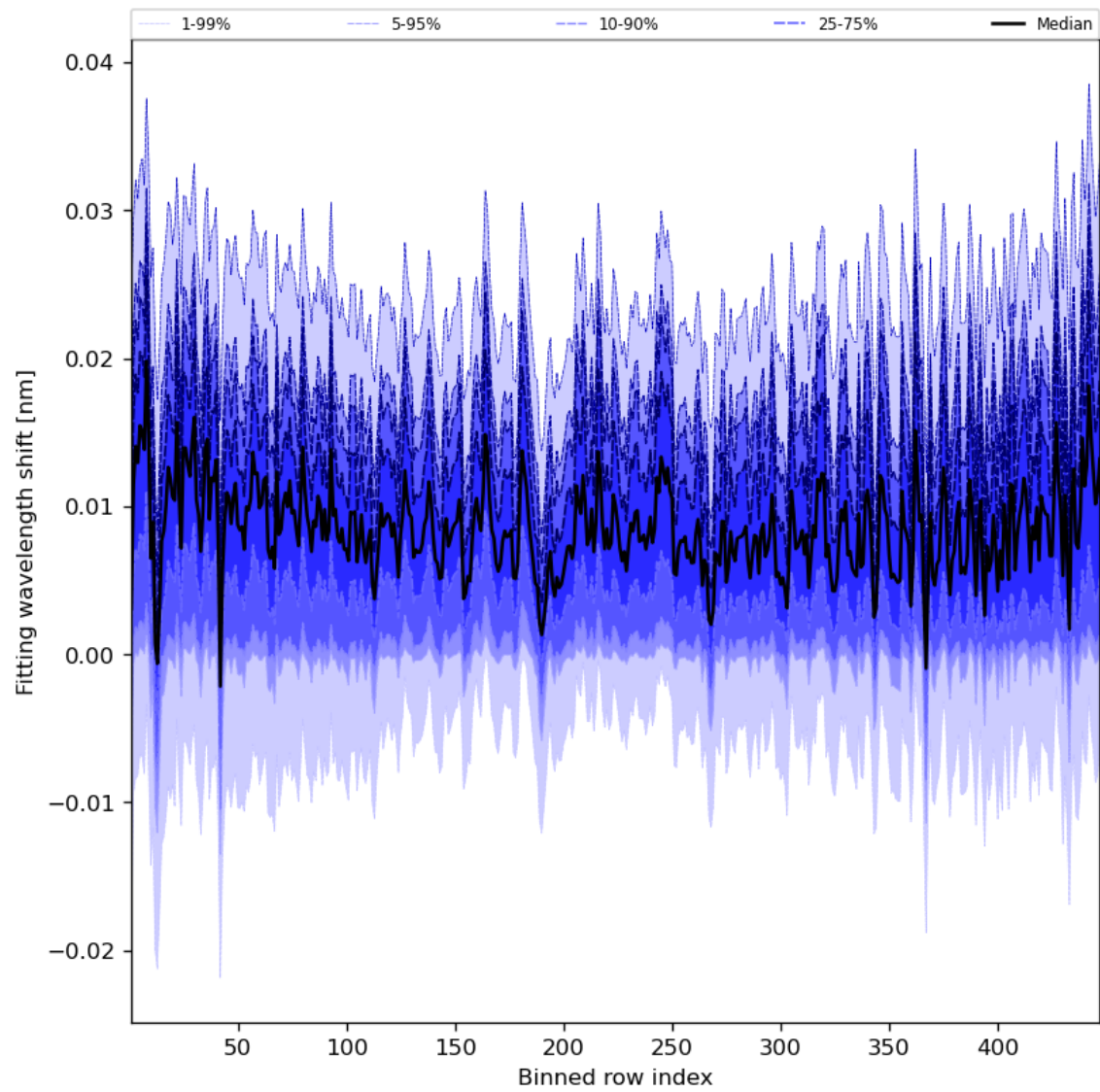
Figure 65: Along track statistics of “Fitting wavelength shift” for 2023-09-06 to 2023-09-08
