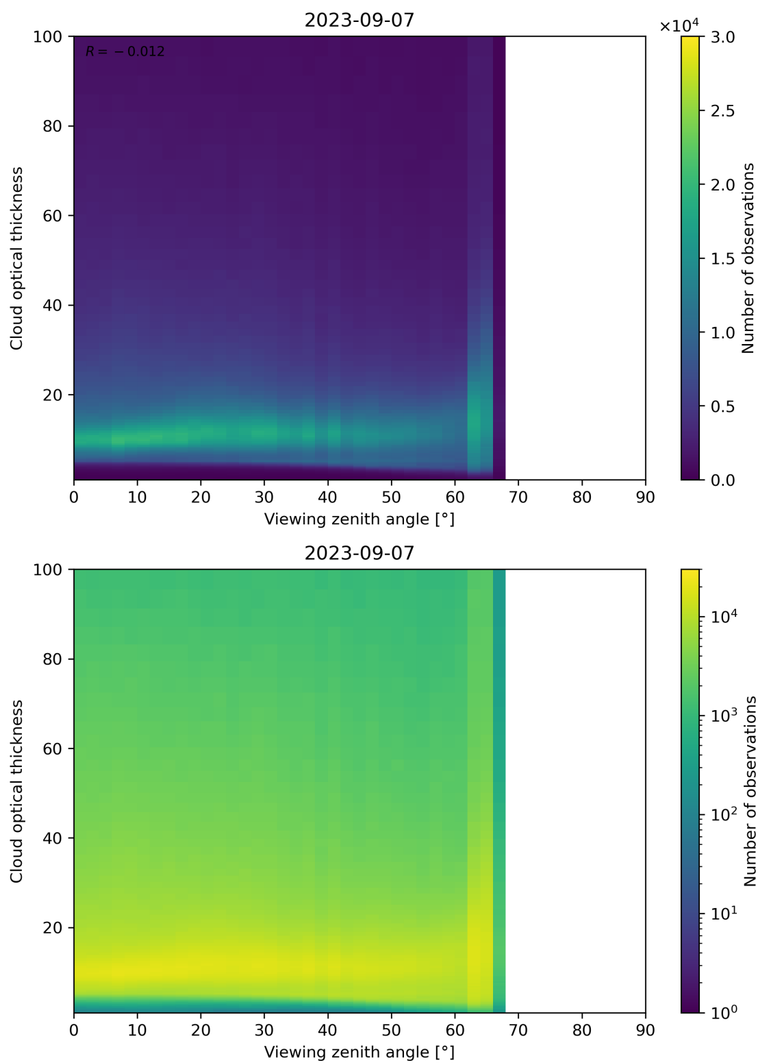
Figure 111: Scatter density plot of “Viewing zenith angle” against “Cloud optical thickness” for 2023-09-06 to 2023-09-08.
