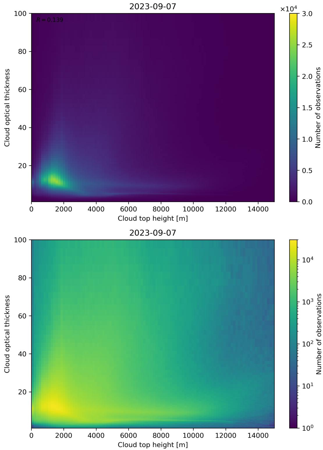
Figure 90: Scatter density plot of “Cloud top height” against “Cloud optical thickness” for 2023-09-06 to 2023-09-08.
