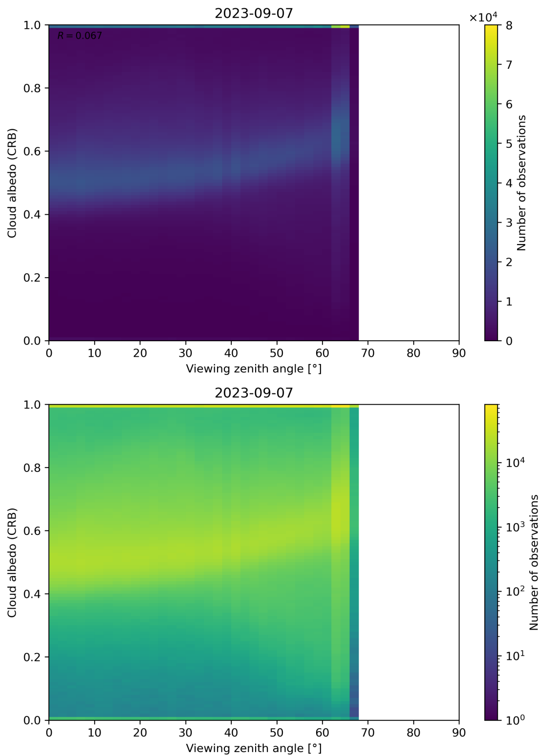
Figure 106: Scatter density plot of “Viewing zenith angle” against “Cloud albedo (CRB)” for 2023-09-06 to 2023-09-08.
