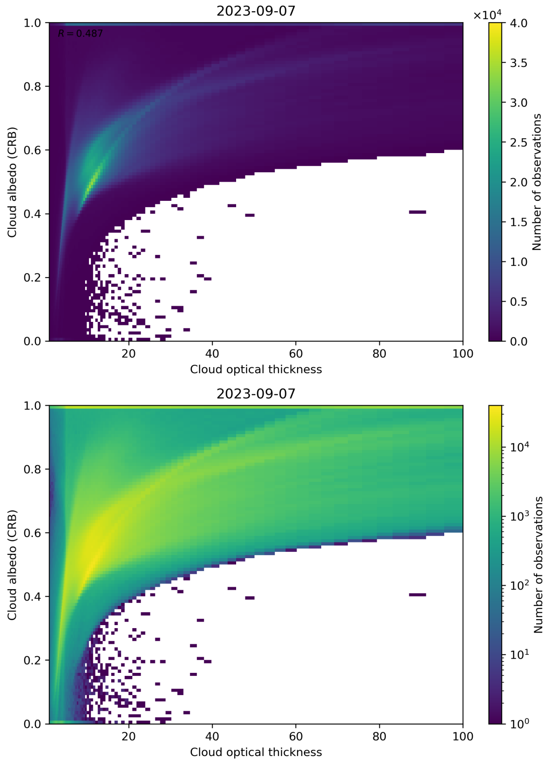
Figure 82: Scatter density plot of “Cloud optical thickness” against “Cloud albedo (CRB)” for 2023-09-06 to 2023-09-08.
