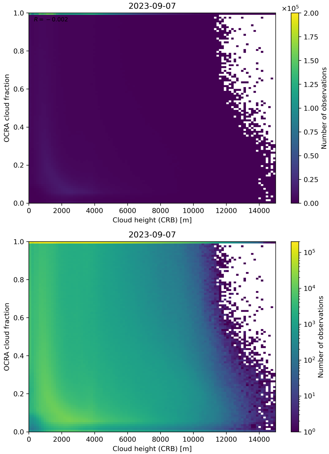
Figure 81: Scatter density plot of “Cloud height (CRB)” against “OCRA cloud fraction” for 2023-09-06 to 2023-09-08.
