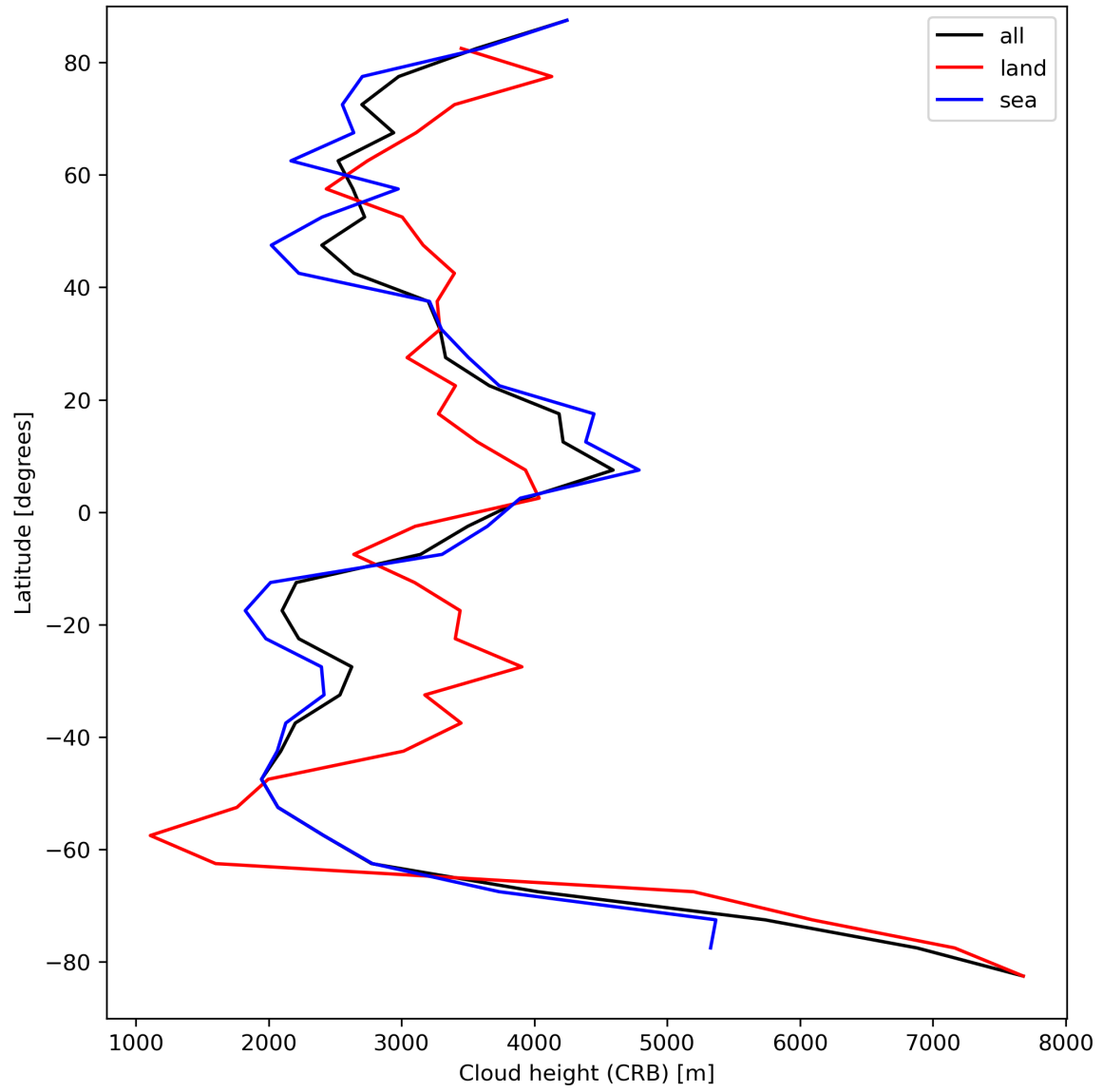
Figure 27: Zonal average of “Cloud height (CRB)” for 2023-09-06 to 2023-09-08.
