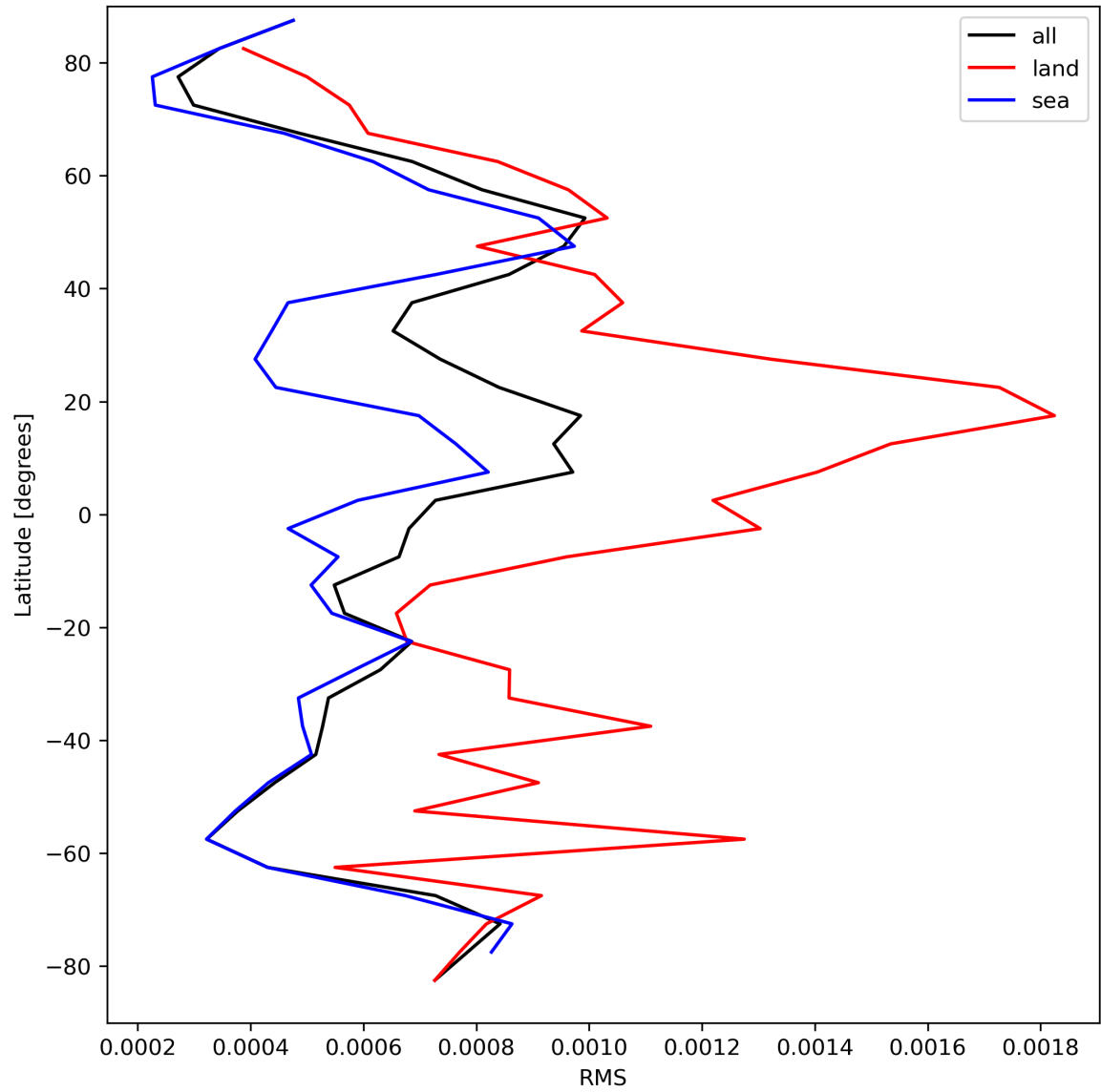
Figure 31: Zonal average of “RMS” for 2023-09-06 to 2023-09-08.
