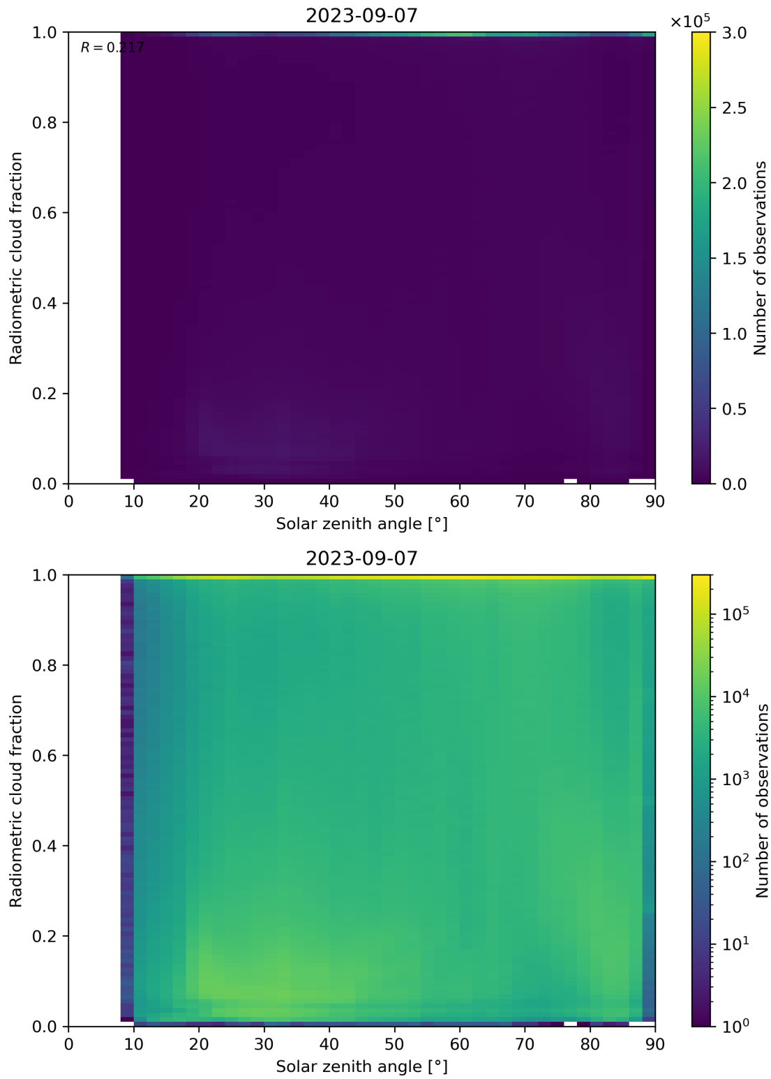
Figure 99: Scatter density plot of “Solar zenith angle” against “Radiometric cloud fraction” for 2023-09-06 to 2023-09-08.
