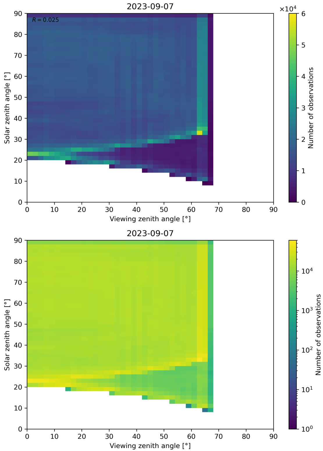
Figure 114: Scatter density plot of “Viewing zenith angle” against “Solar zenith angle” for 2023-09-06 to 2023-09-08.
