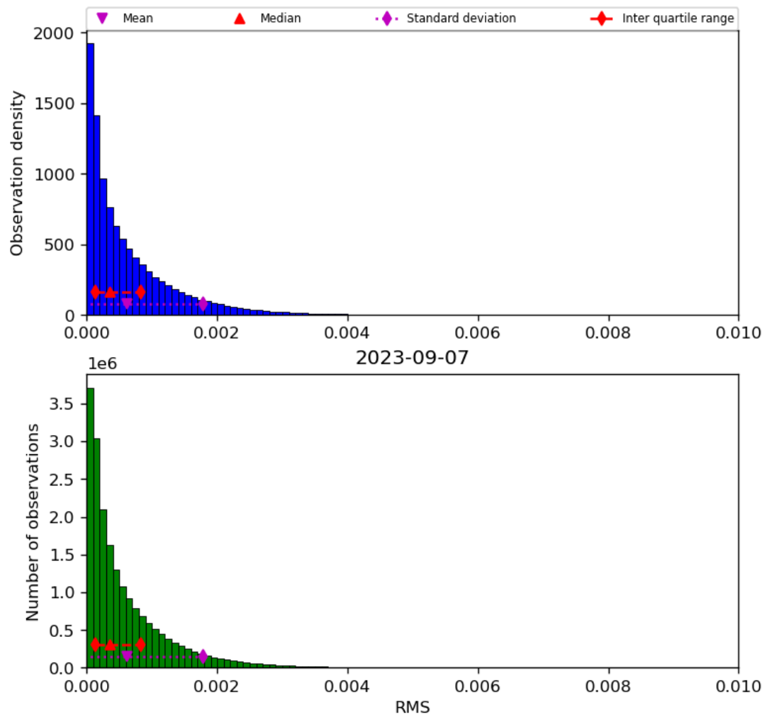
Figure 47: Histogram of “RMS” for 2023-09-06 to 2023-09-08
