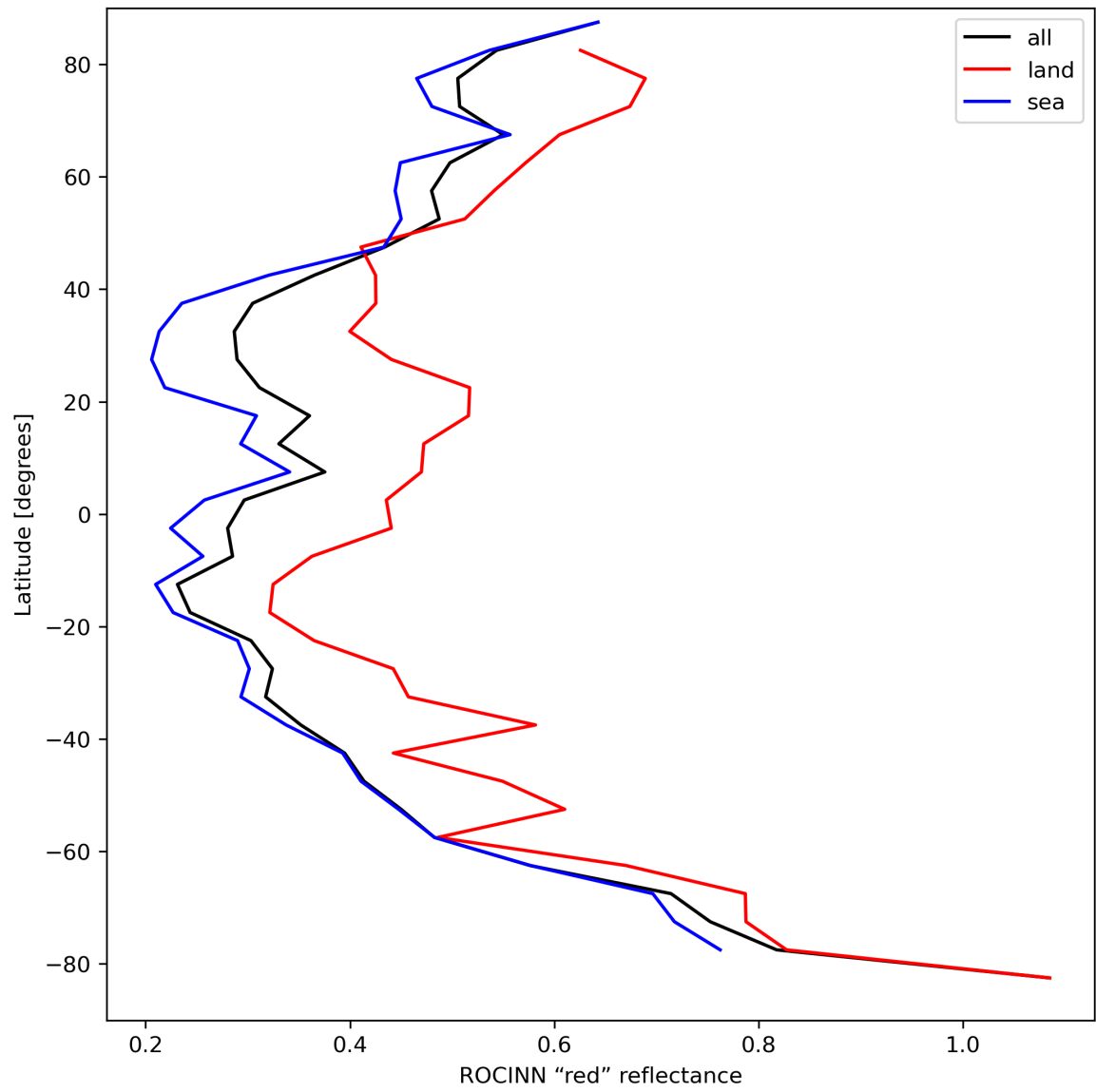
Figure 37: Zonal average of “ROCINN “red” reflectance” for 2023-09-06 to 2023-09-08.
