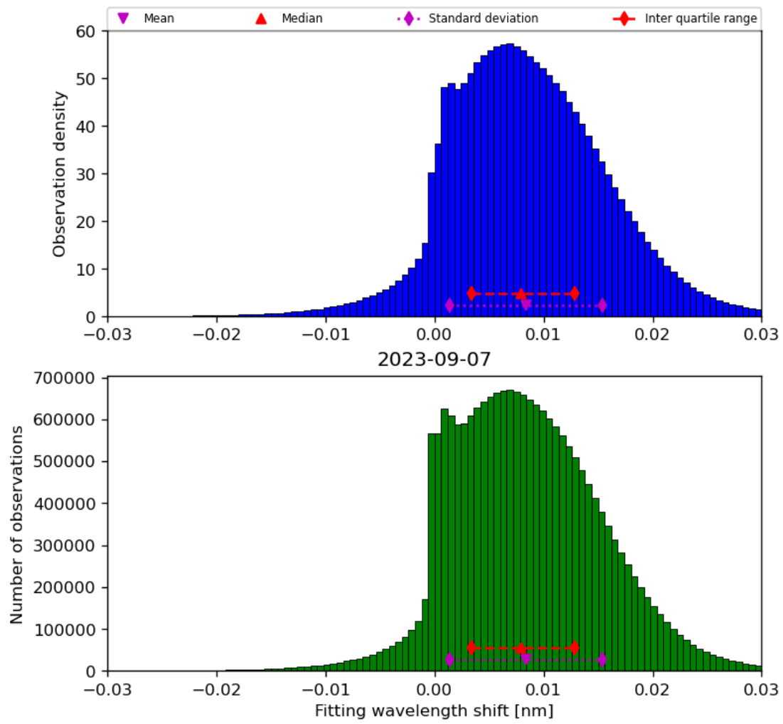
Figure 49: Histogram of “Fitting wavelength shift” for 2023-09-06 to 2023-09-08
