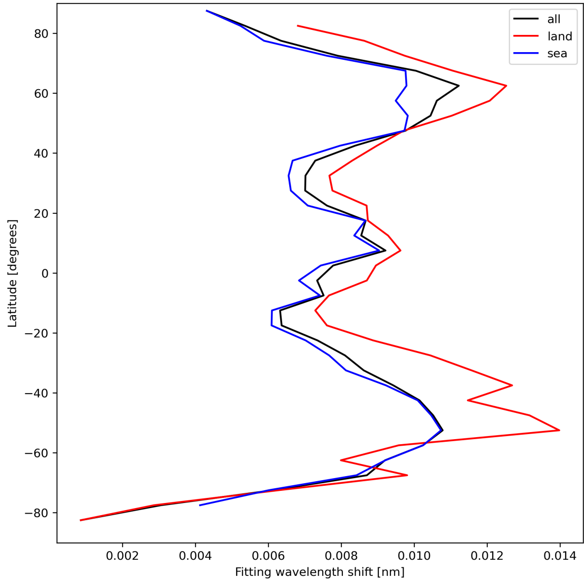
Figure 33: Zonal average of “Fitting wavelength shift” for 2023-09-06 to 2023-09-08.
