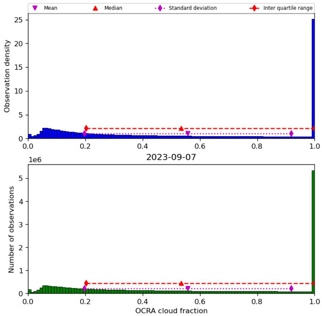
Figure 50: Histogram of “OCRA cloud fraction” for 2023-09-06 to 2023-09-08
