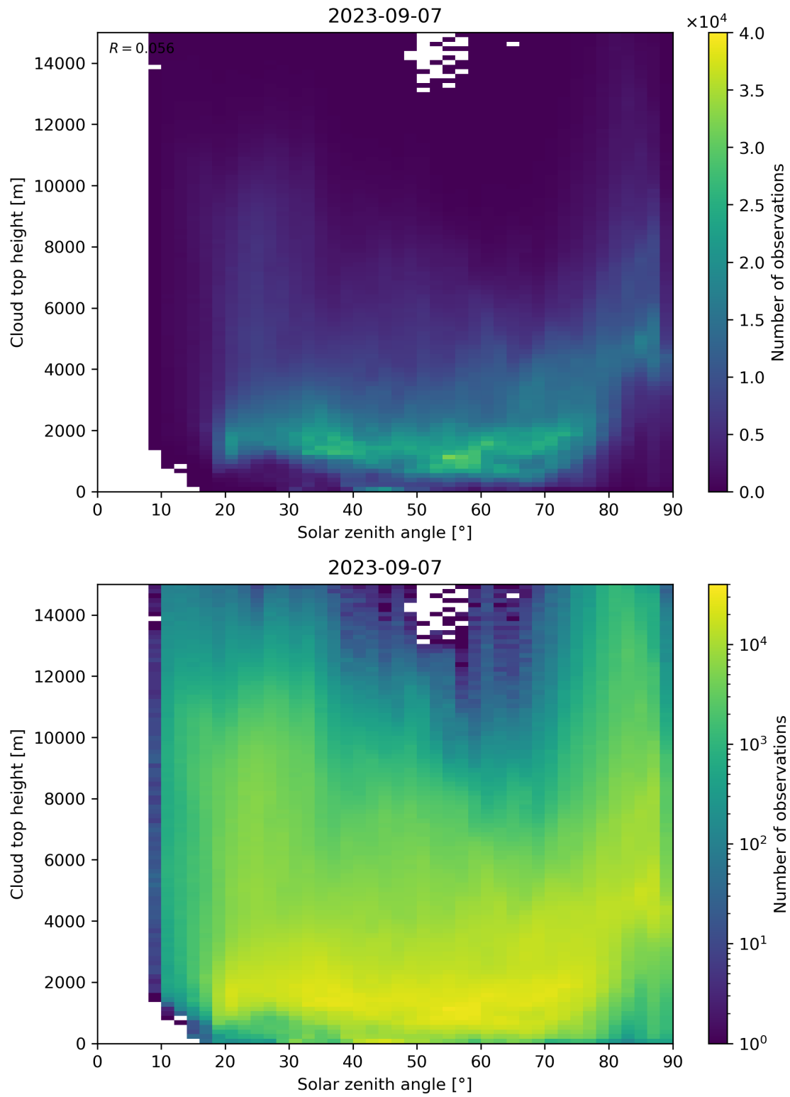
Figure 104: Scatter density plot of “Solar zenith angle” against “Cloud top height” for 2023-09-06 to 2023-09-08.
