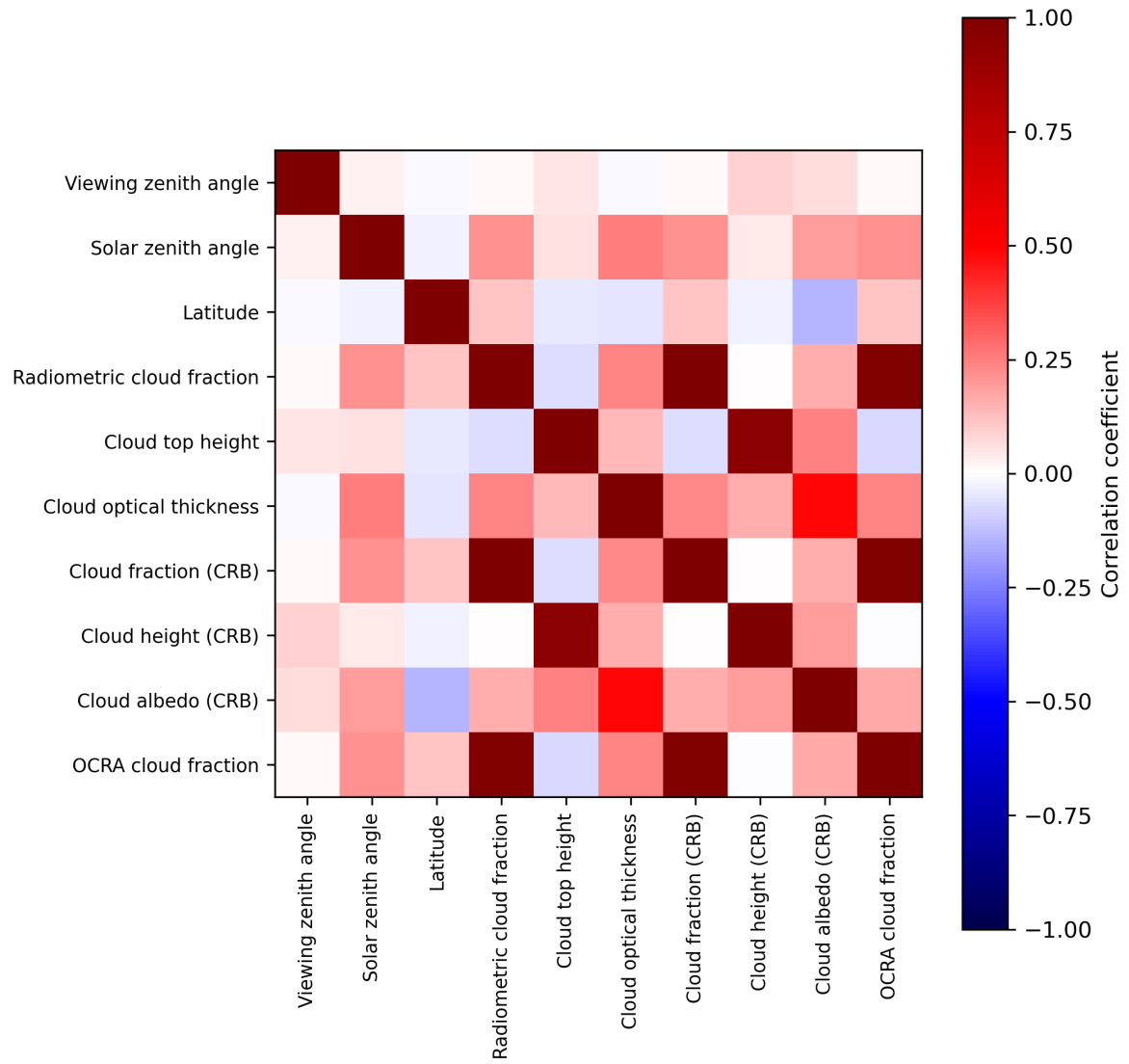
Figure 2: Map of correlation matrix for 2023-09-06 to 2023-09-08.
