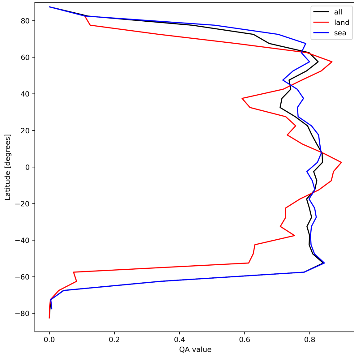
Figure 22: Zonal average of “QA value” for 2023-09-06 to 2023-09-08.
