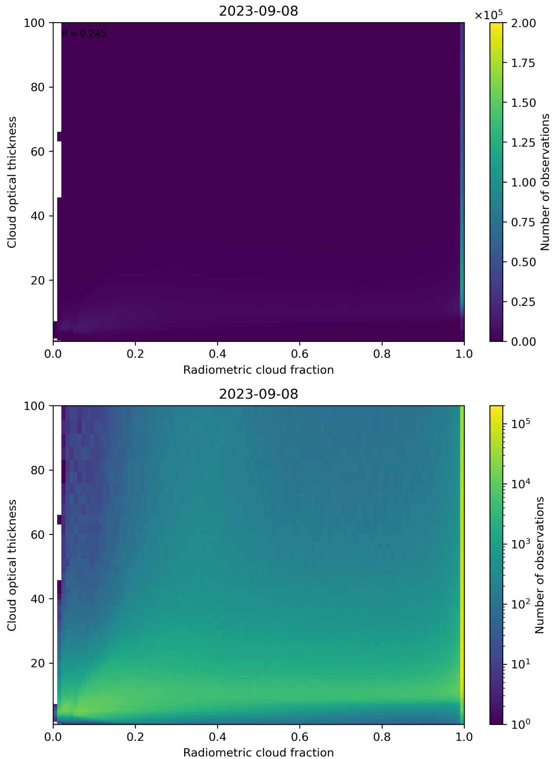
Figure 75: Scatter density plot of “Radiometric cloud fraction” against “Cloud optical thickness” for 2023-09-07 to 2023-09-09.
