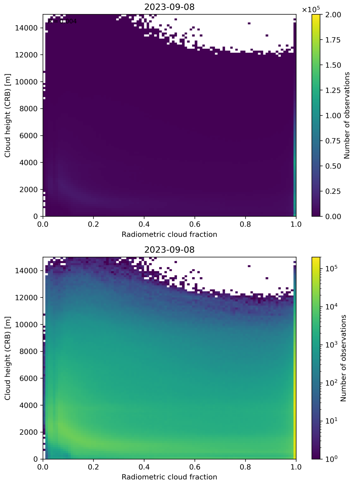
Figure 74: Scatter density plot of “Radiometric cloud fraction” against “Cloud height (CRB)” for 2023-09-07 to 2023-09-09.
