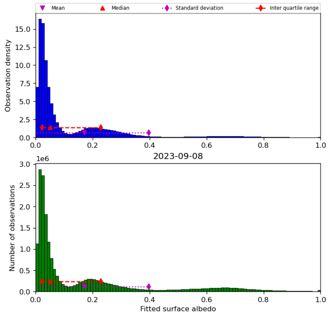
Figure 45: Histogram of “Fitted surface albedo” for 2023-09-07 to 2023-09-09
