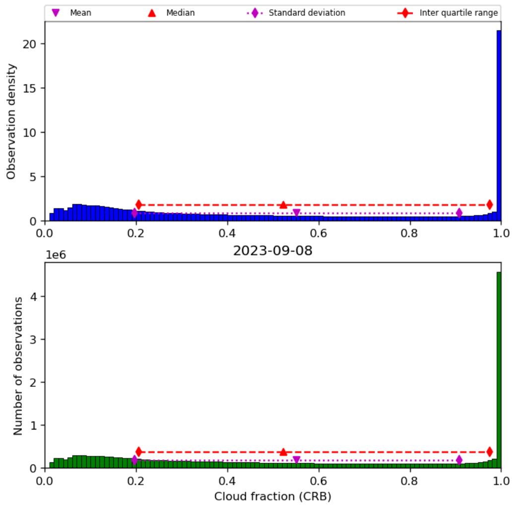
Figure 42: Histogram of “Cloud fraction (CRB)” for 2023-09-07 to 2023-09-09
