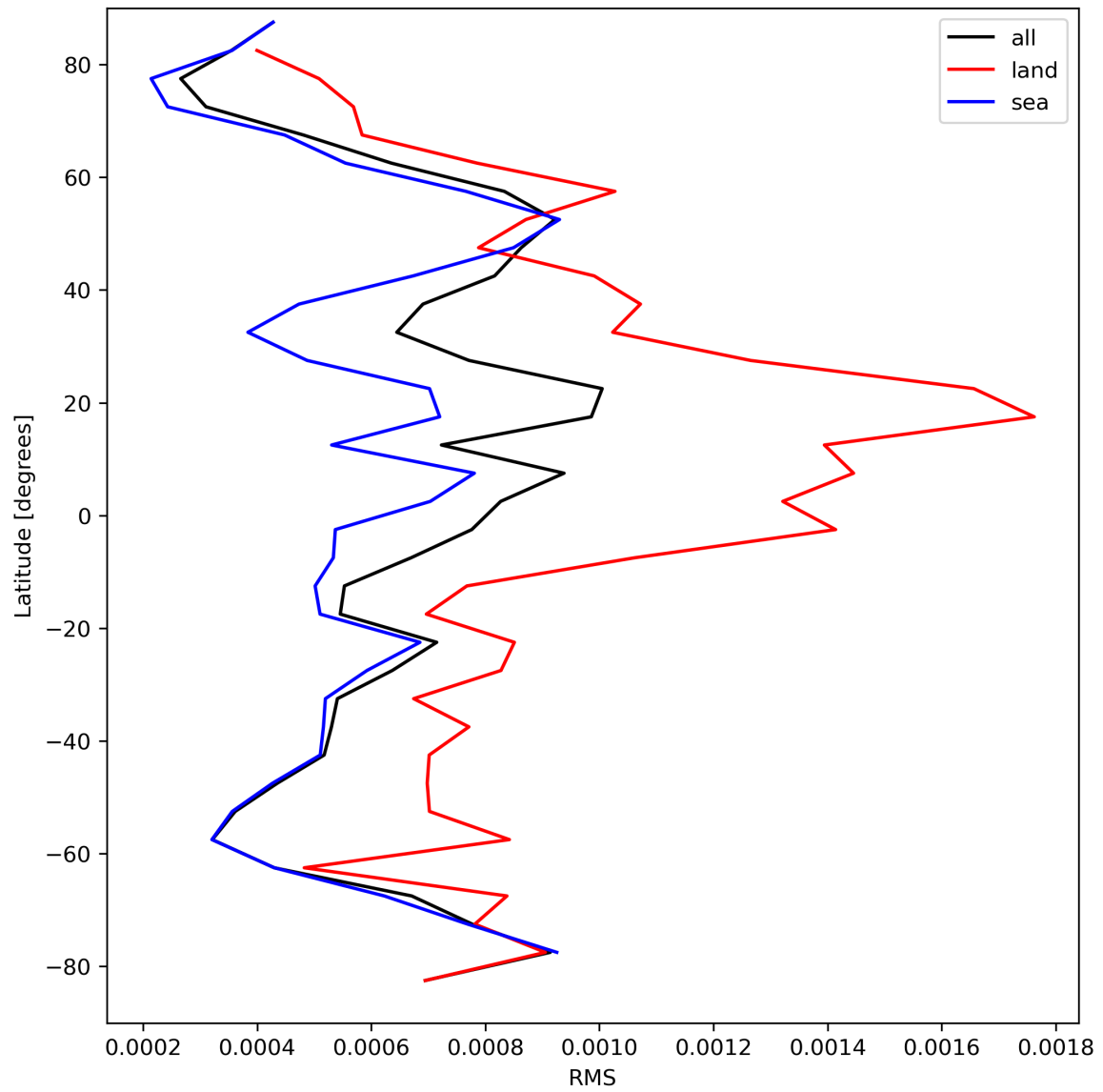
Figure 31: Zonal average of “RMS” for 2023-09-07 to 2023-09-09.
