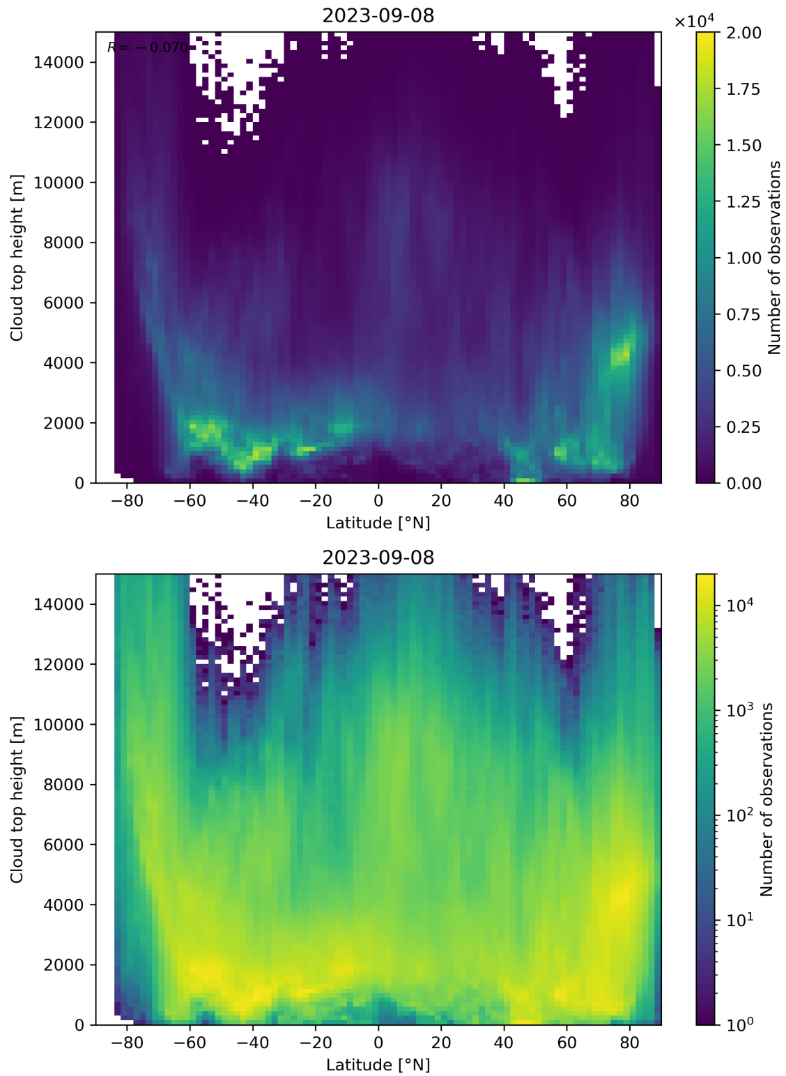
Figure 97: Scatter density plot of “Latitude” against “Cloud top height” for 2023-09-07 to 2023-09-09.
