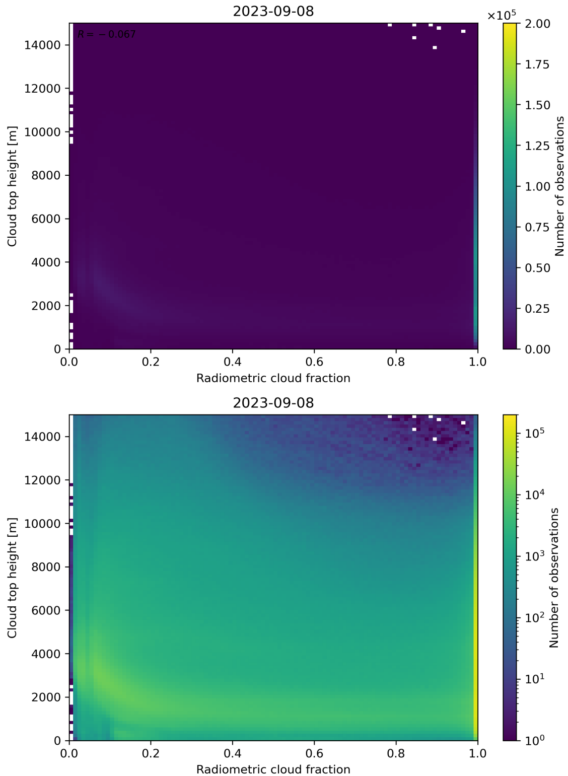
Figure 76: Scatter density plot of “Radiometric cloud fraction” against “Cloud top height” for 2023-09-07 to 2023-09-09.
