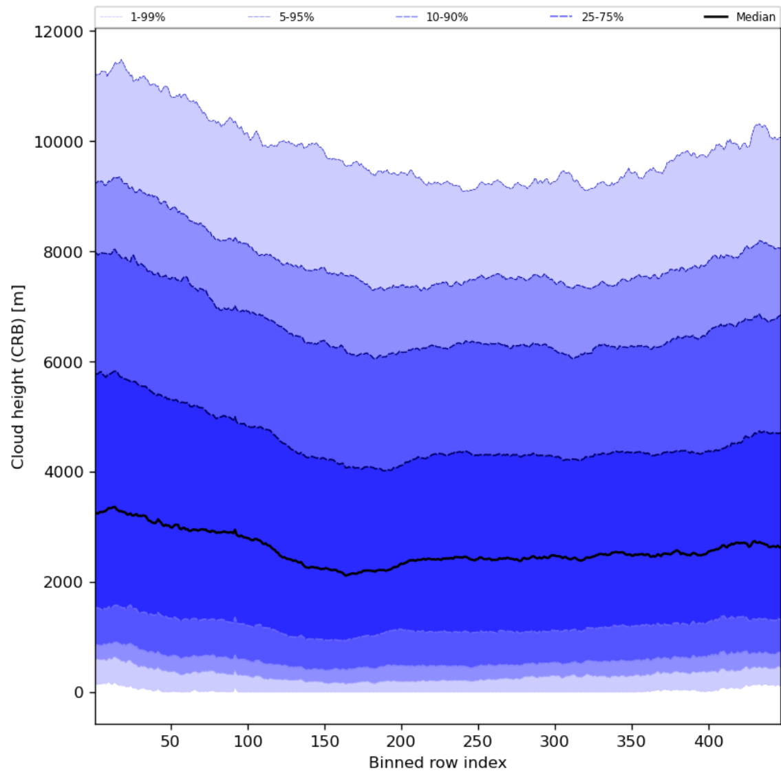
Figure 59: Along track statistics of “Cloud height (CRB)” for 2023-09-07 to 2023-09-09
