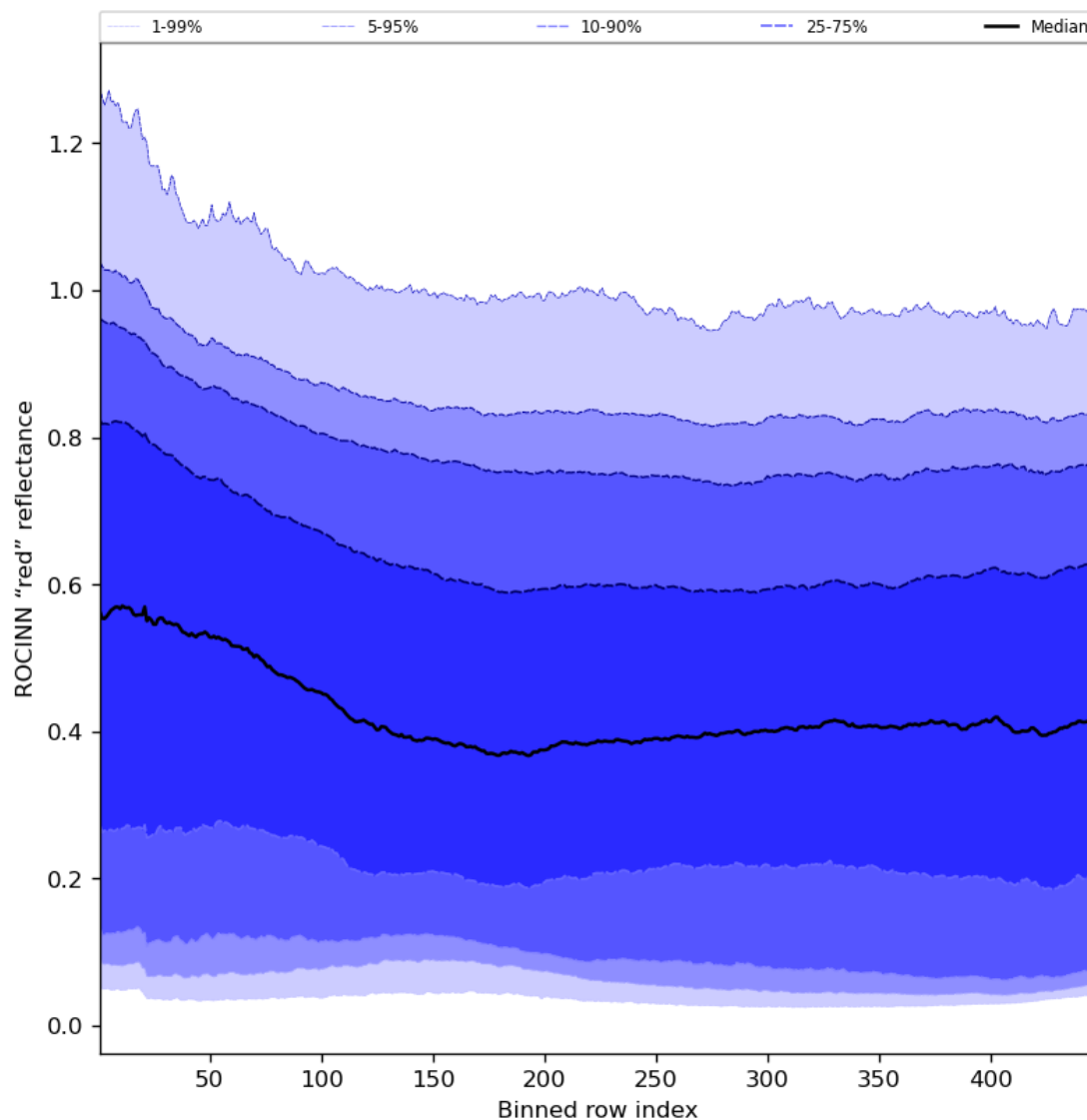
Figure 69: Along track statistics of “ROCINN “red” reflectance” for 2023-09-07 to 2023-09-09
