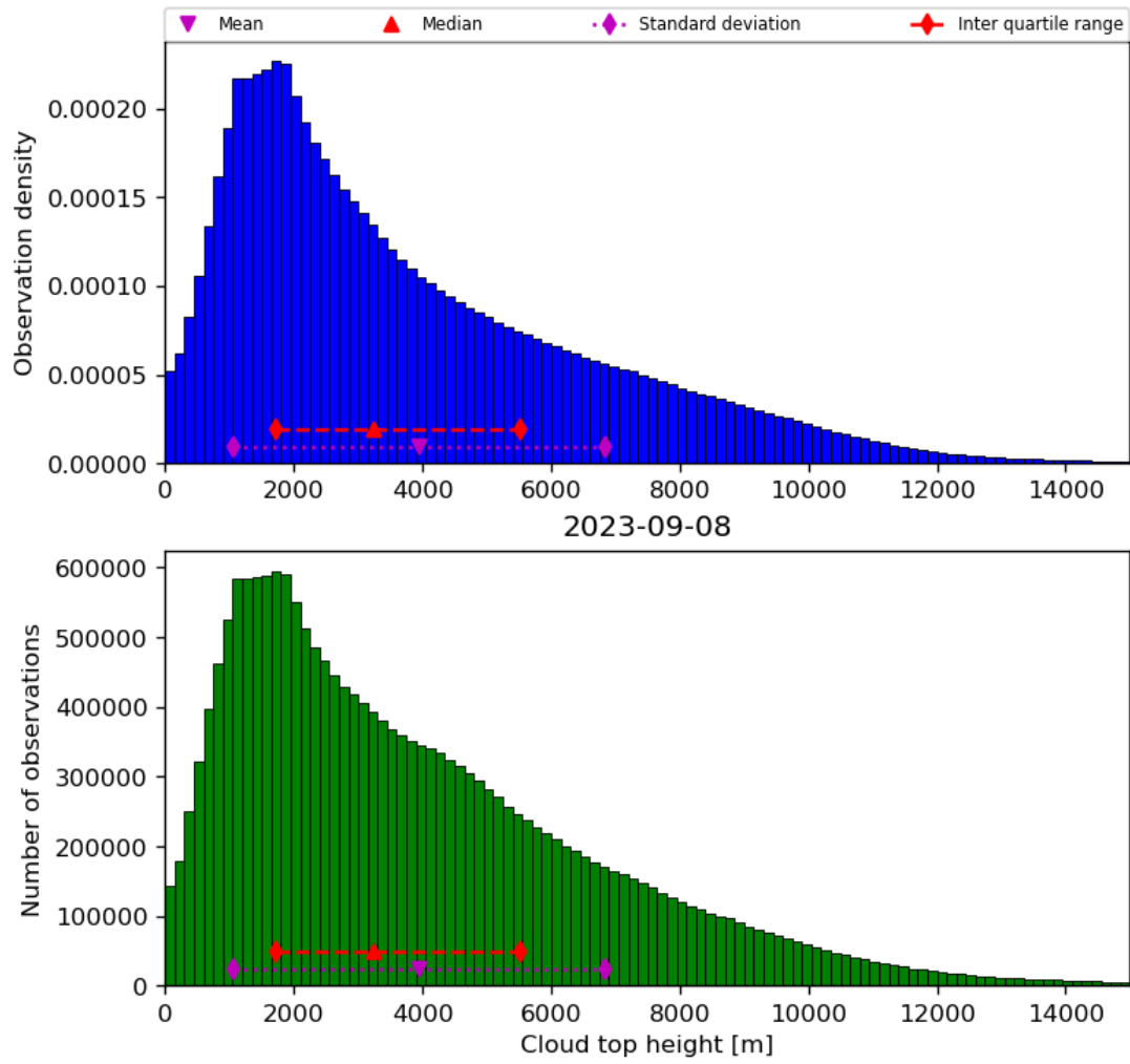
Figure 40: Histogram of “Cloud top height” for 2023-09-07 to 2023-09-09
