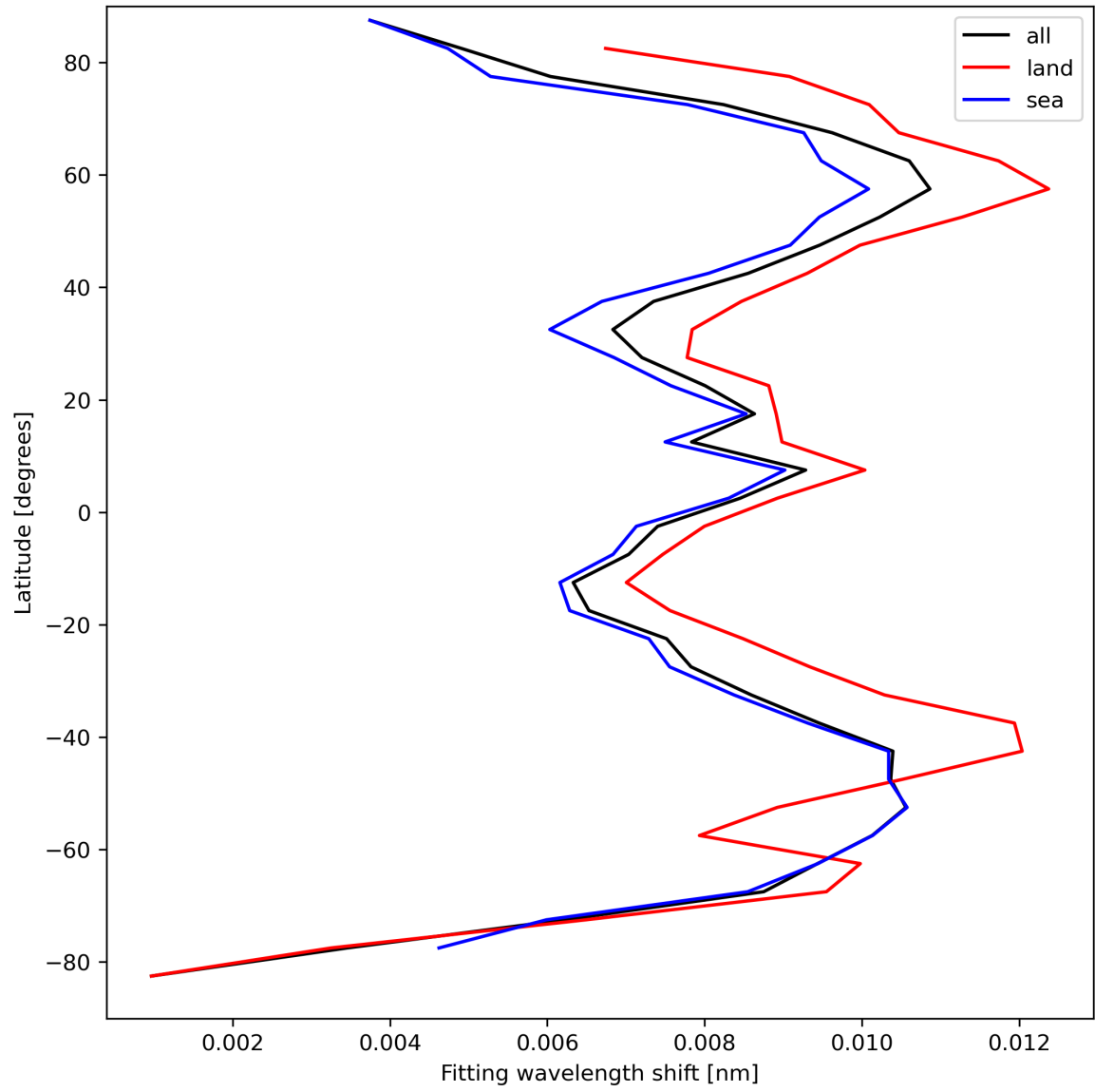
Figure 33: Zonal average of “Fitting wavelength shift” for 2023-09-07 to 2023-09-09.
