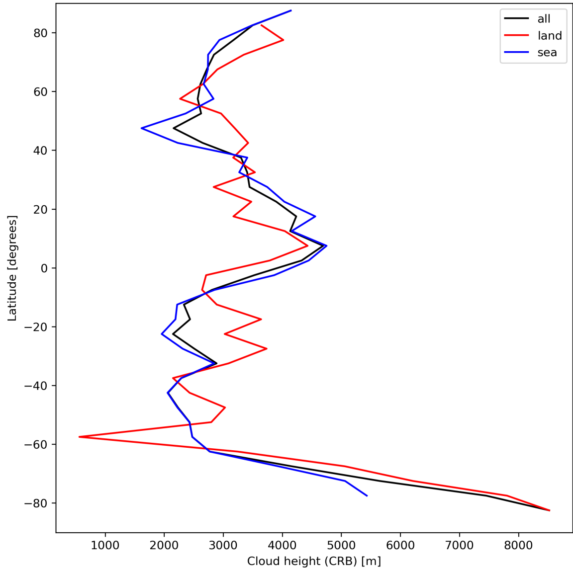
Figure 27: Zonal average of “Cloud height (CRB)” for 2023-09-07 to 2023-09-09.
