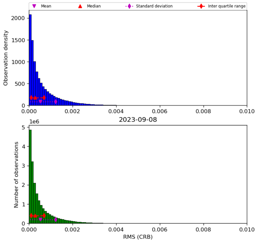
Figure 48: Histogram of “RMS (CRB)” for 2023-09-07 to 2023-09-09
