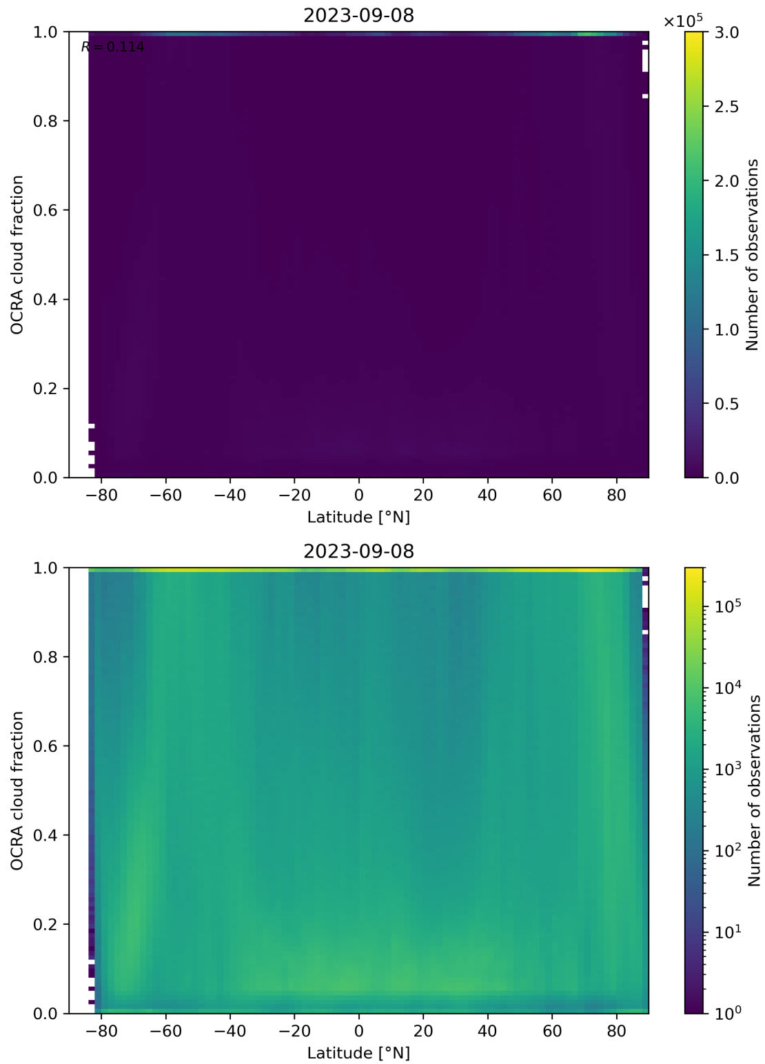
Figure 93: Scatter density plot of “Latitude” against “OCRA cloud fraction” for 2023-09-07 to 2023-09-09.
