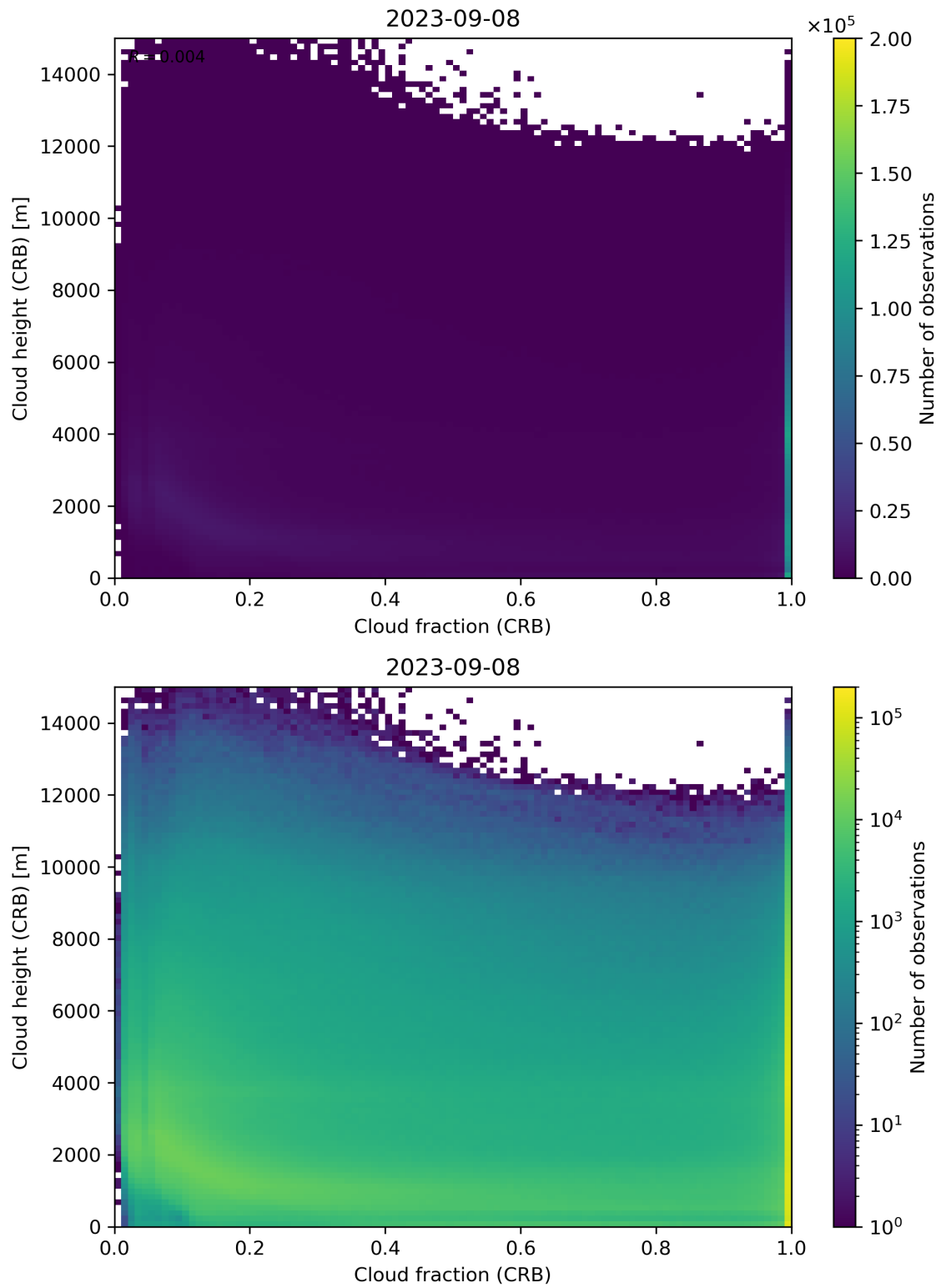
Figure 79: Scatter density plot of “Cloud fraction (CRB)” against “Cloud height (CRB)” for 2023-09-07 to 2023-09-09.
