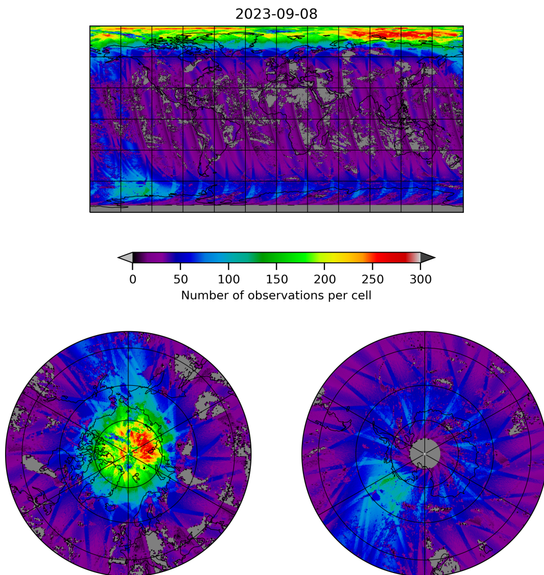
Figure 21: Map of the number of observations for 2023-09-07 to 2023-09-09
