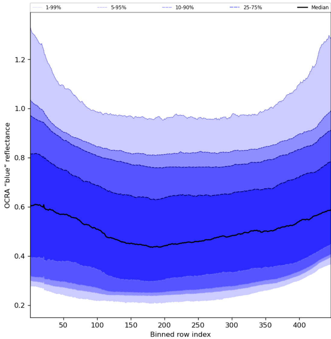
Figure 67: Along track statistics of “OCRA “blue” reflectance” for 2023-09-07 to 2023-09-09
