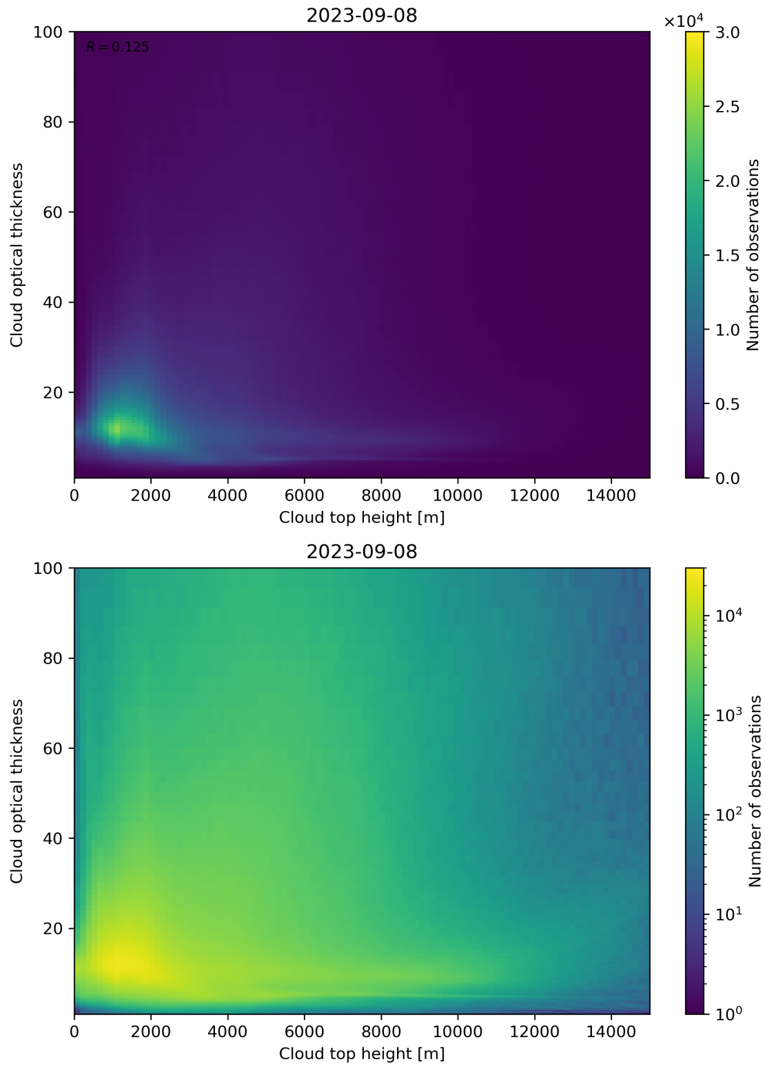
Figure 90: Scatter density plot of “Cloud top height” against “Cloud optical thickness” for 2023-09-07 to 2023-09-09.
