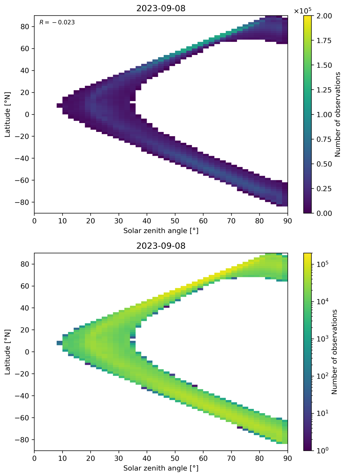
Figure 105: Scatter density plot of “Solar zenith angle” against “Latitude” for 2023-09-07 to 2023-09-09.
