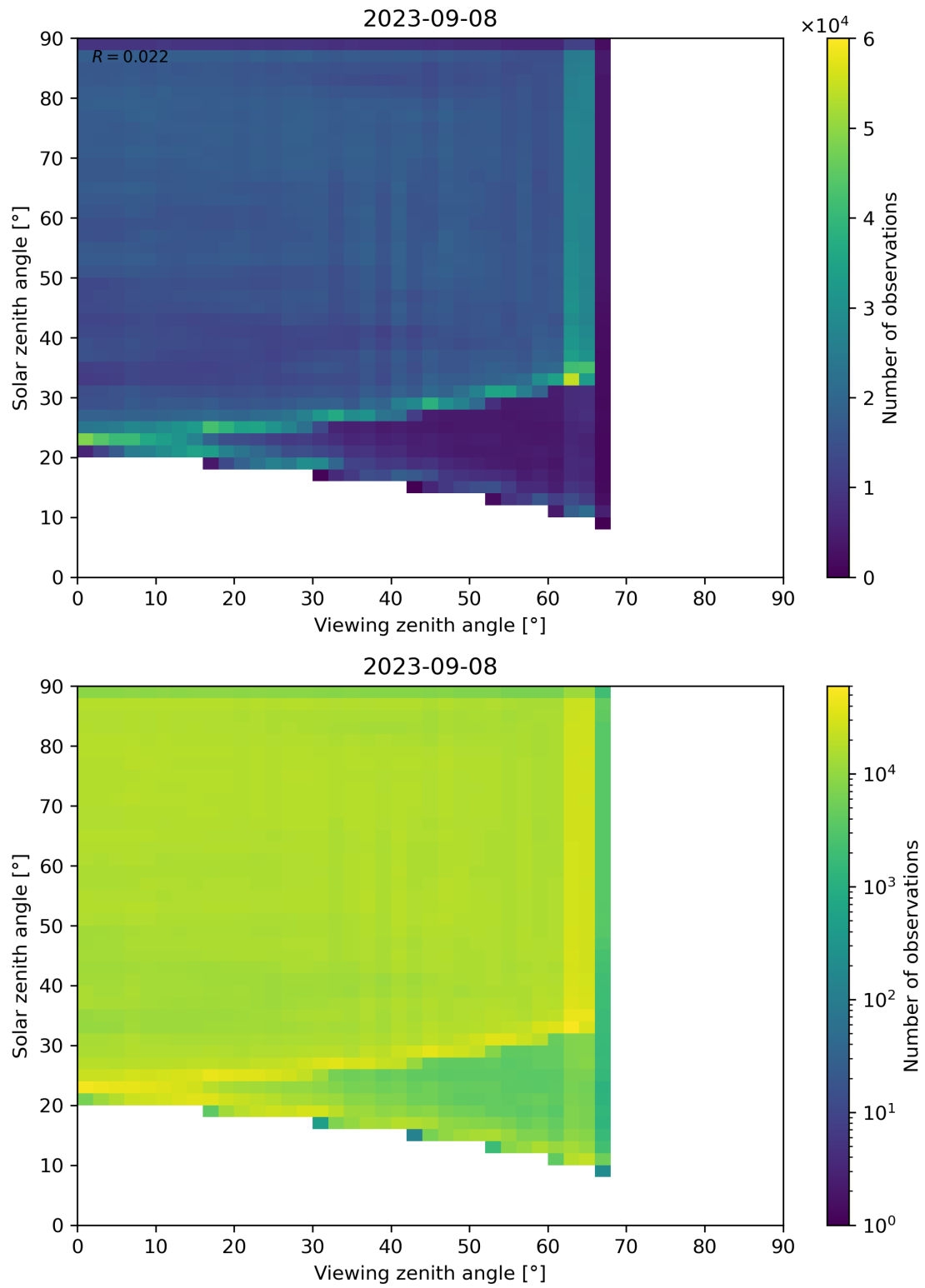
Figure 114: Scatter density plot of “Viewing zenith angle” against “Solar zenith angle” for 2023-09-07 to 2023-09-09.
