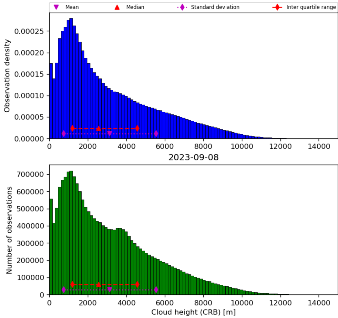
Figure 43: Histogram of “Cloud height (CRB)” for 2023-09-07 to 2023-09-09
