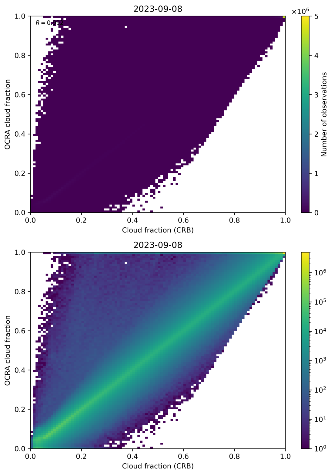
Figure 78: Scatter density plot of “Cloud fraction (CRB)” against “OCRA cloud fraction” for 2023-09-07 to 2023-09-09.
