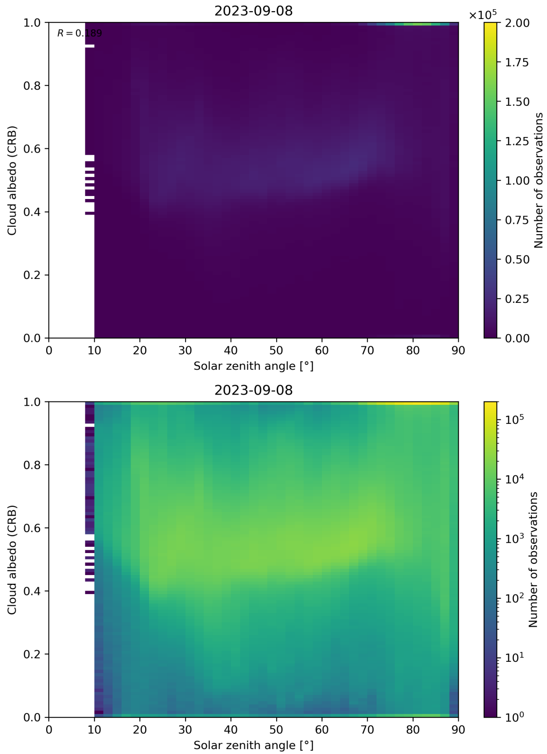
Figure 98: Scatter density plot of “Solar zenith angle” against “Cloud albedo (CRB)” for 2023-09-07 to 2023-09-09.
