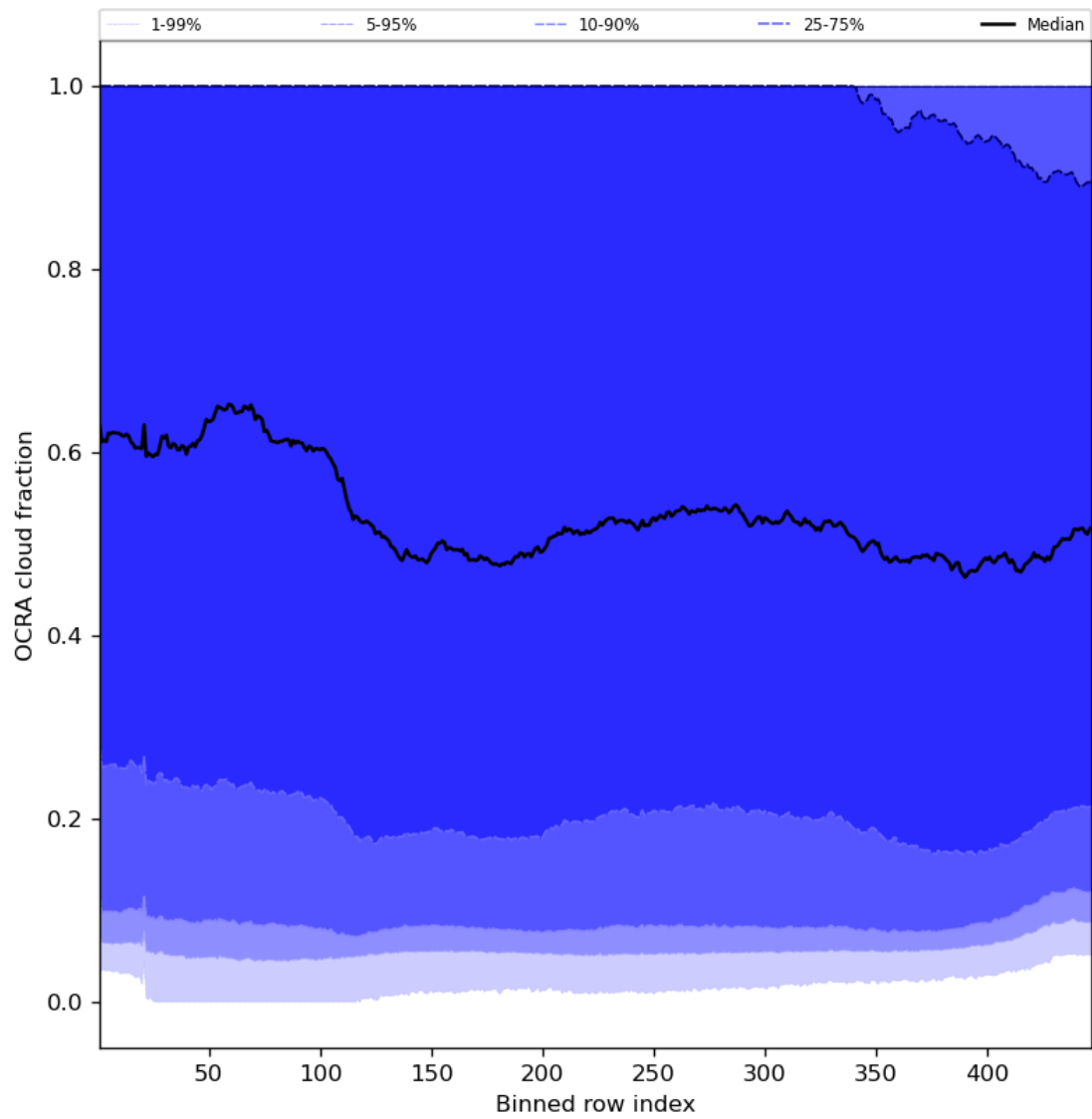
Figure 66: Along track statistics of “OCRA cloud fraction” for 2023-09-07 to 2023-09-09
