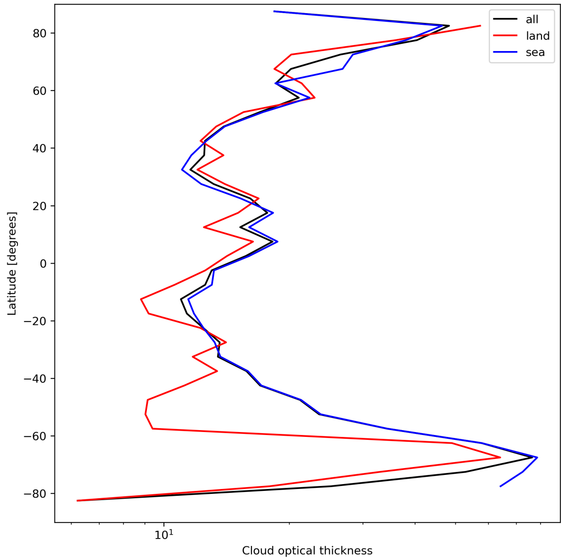
Figure 25: Zonal average of “Cloud optical thickness” for 2023-09-07 to 2023-09-09.
