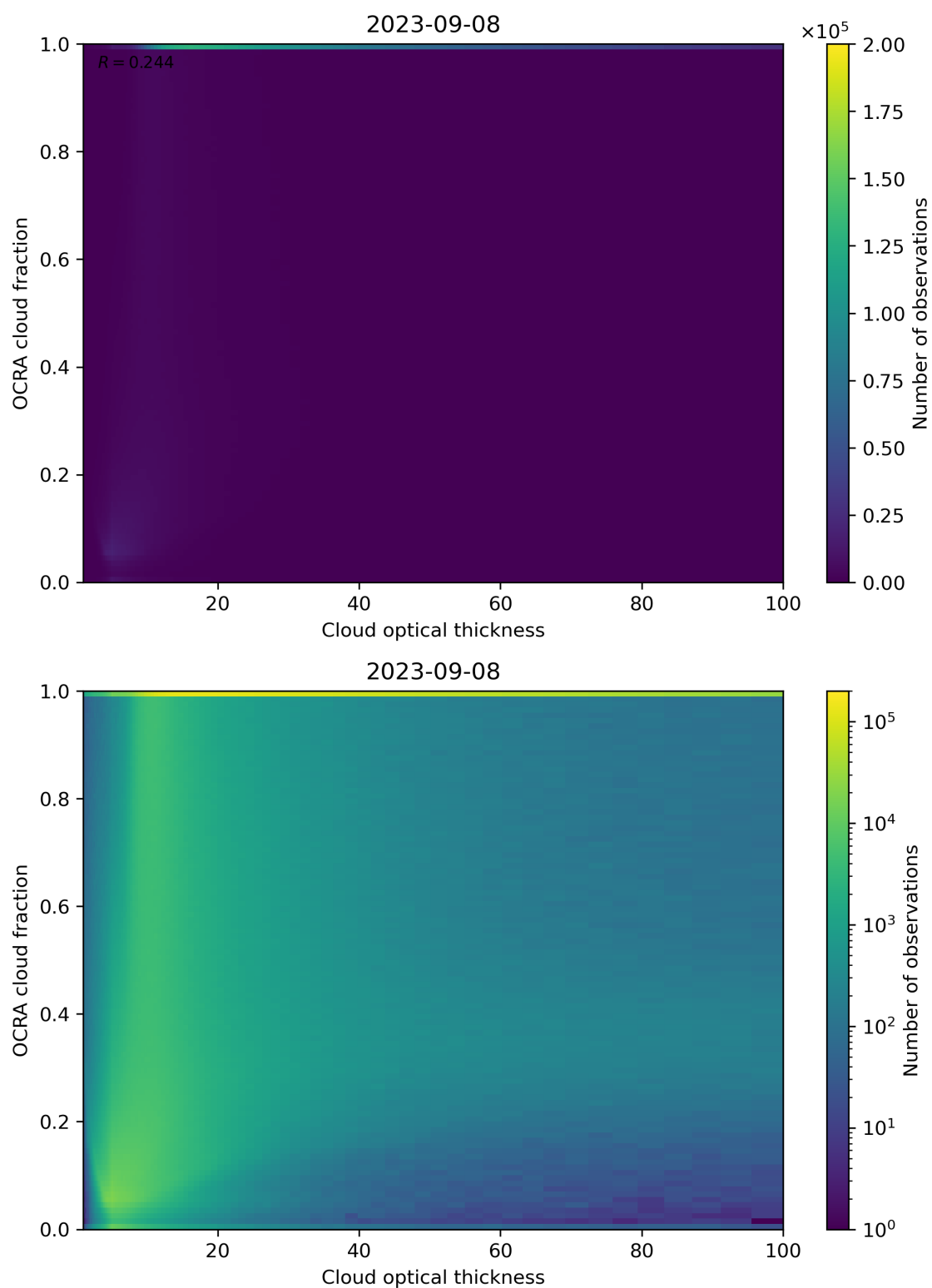
Figure 83: Scatter density plot of “Cloud optical thickness” against “OCRA cloud fraction” for 2023-09-07 to 2023-09-09.
