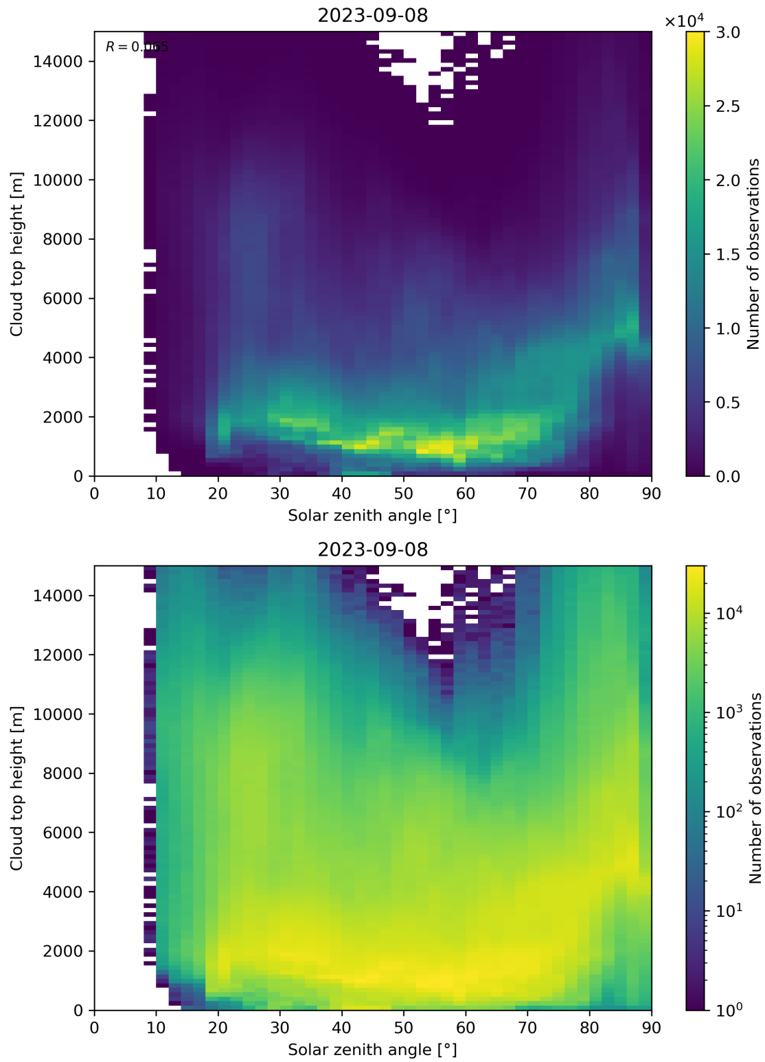
Figure 104: Scatter density plot of “Solar zenith angle” against “Cloud top height” for 2023-09-07 to 2023-09-09.
