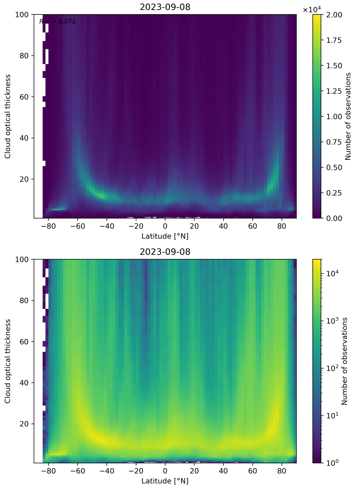
Figure 96: Scatter density plot of “Latitude” against “Cloud optical thickness” for 2023-09-07 to 2023-09-09.
