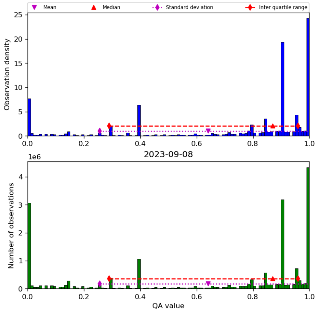
Figure 38: Histogram of “QA value” for 2023-09-07 to 2023-09-09
