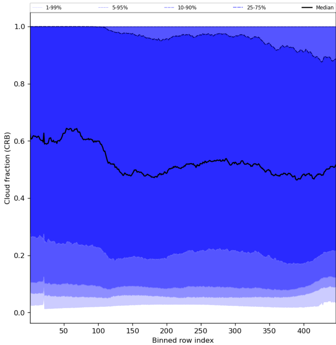
Figure 58: Along track statistics of “Cloud fraction (CRB)” for 2023-09-07 to 2023-09-09
