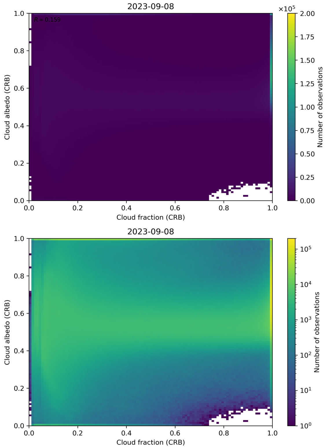
Figure 77: Scatter density plot of “Cloud fraction (CRB)” against “Cloud albedo (CRB)” for 2023-09-07 to 2023-09-09.
