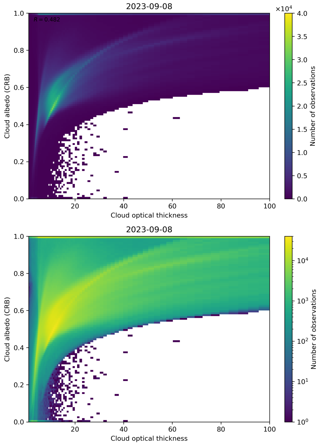
Figure 82: Scatter density plot of “Cloud optical thickness” against “Cloud albedo (CRB)” for 2023-09-07 to 2023-09-09.
