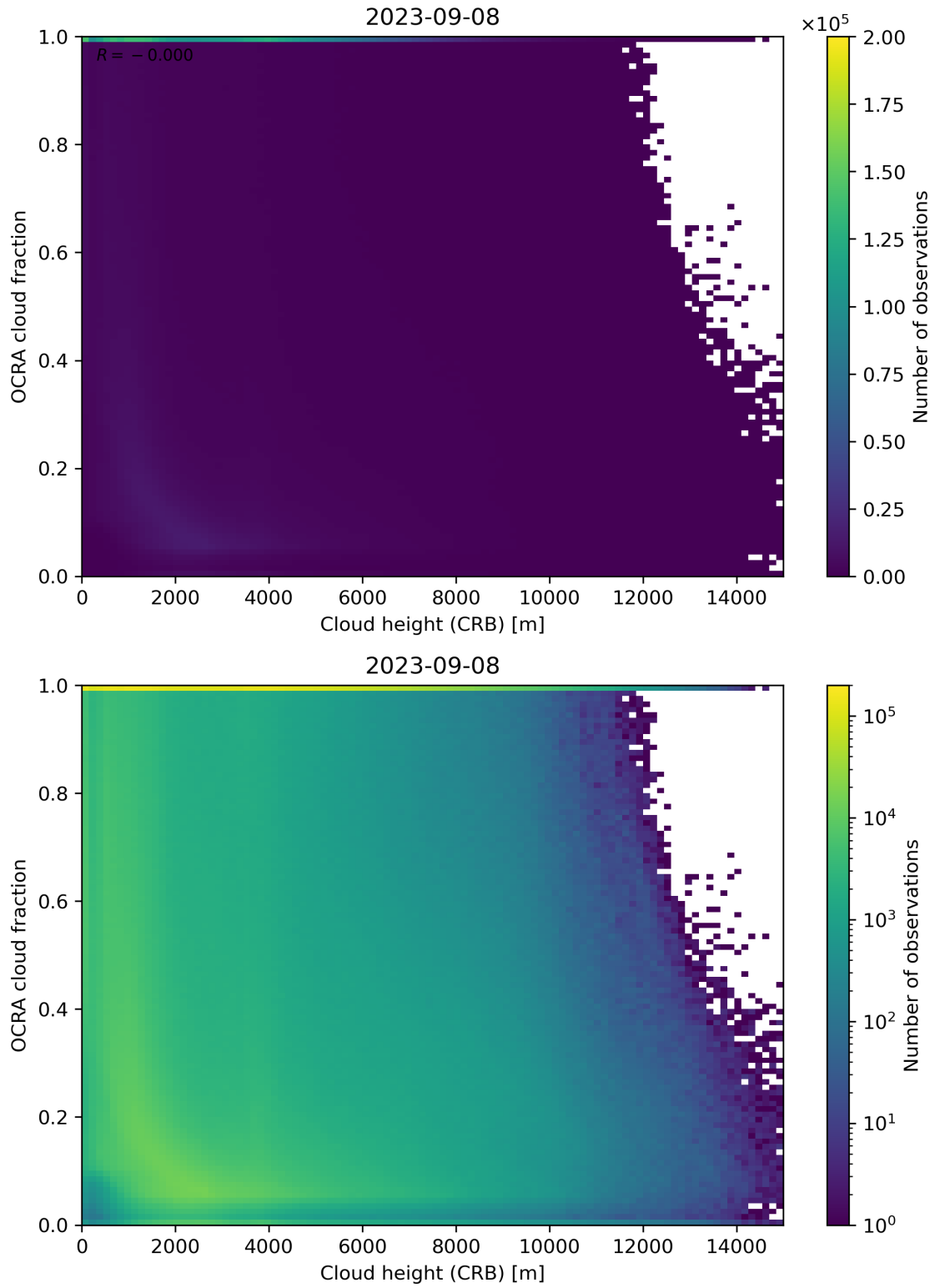
Figure 81: Scatter density plot of “Cloud height (CRB)” against “OCRA cloud fraction” for 2023-09-07 to 2023-09-09.
