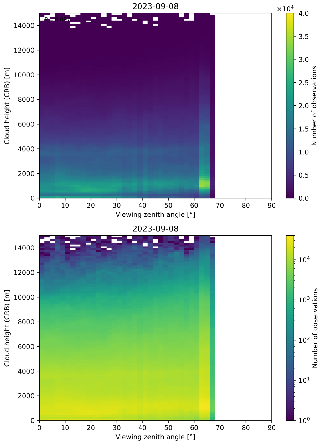
Figure 110: Scatter density plot of “Viewing zenith angle” against “Cloud height (CRB)” for 2023-09-07 to 2023-09-09.
