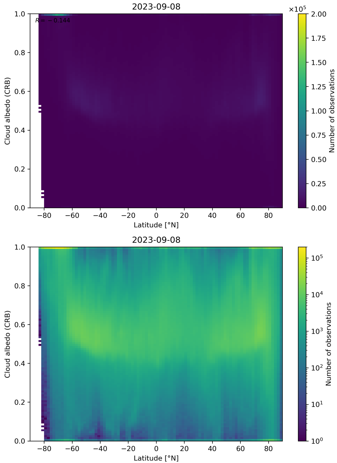
Figure 91: Scatter density plot of “Latitude” against “Cloud albedo (CRB)” for 2023-09-07 to 2023-09-09.
