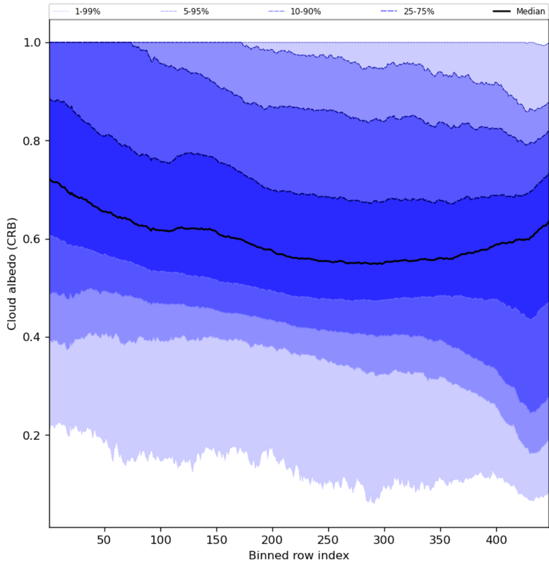
Figure 60: Along track statistics of “Cloud albedo (CRB)” for 2023-09-07 to 2023-09-09
