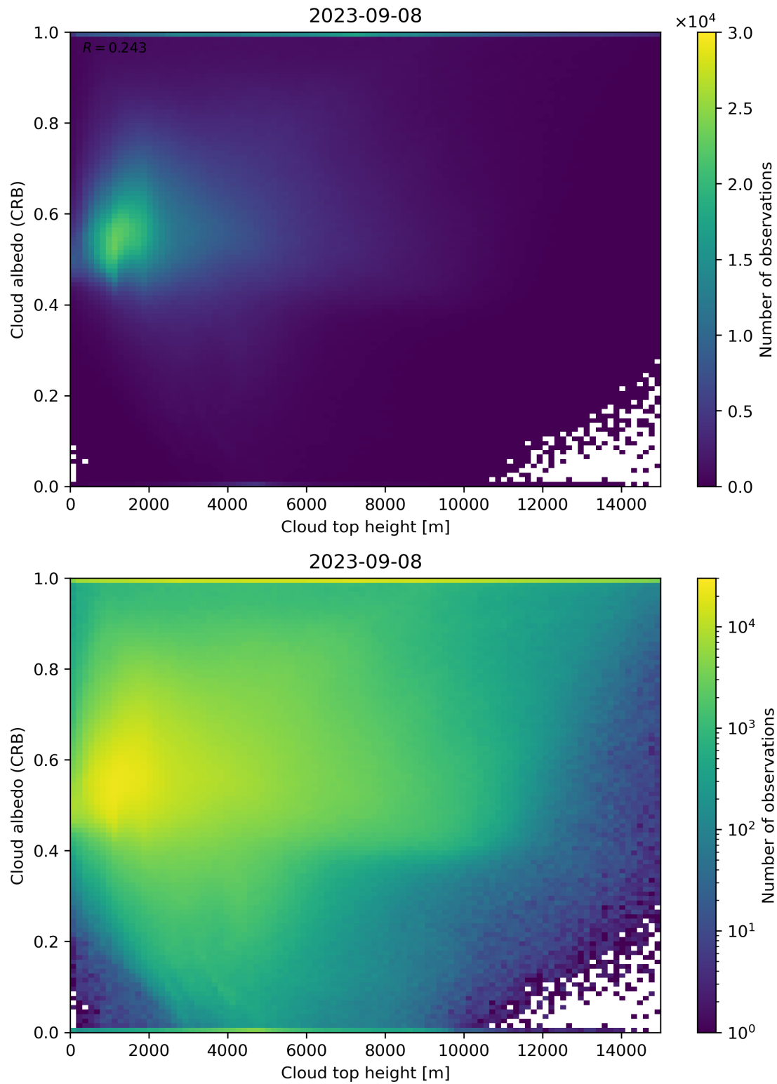
Figure 86: Scatter density plot of “Cloud top height” against “Cloud albedo (CRB)” for 2023-09-07 to 2023-09-09.
