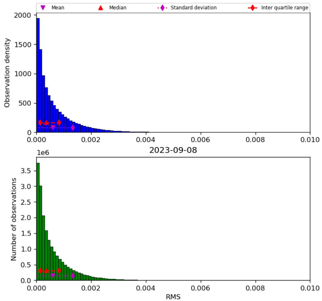
Figure 47: Histogram of “RMS” for 2023-09-07 to 2023-09-09
