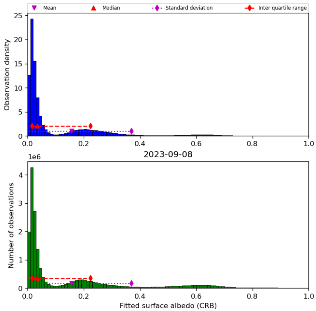
Figure 46: Histogram of “Fitted surface albedo (CRB)” for 2023-09-07 to 2023-09-09
