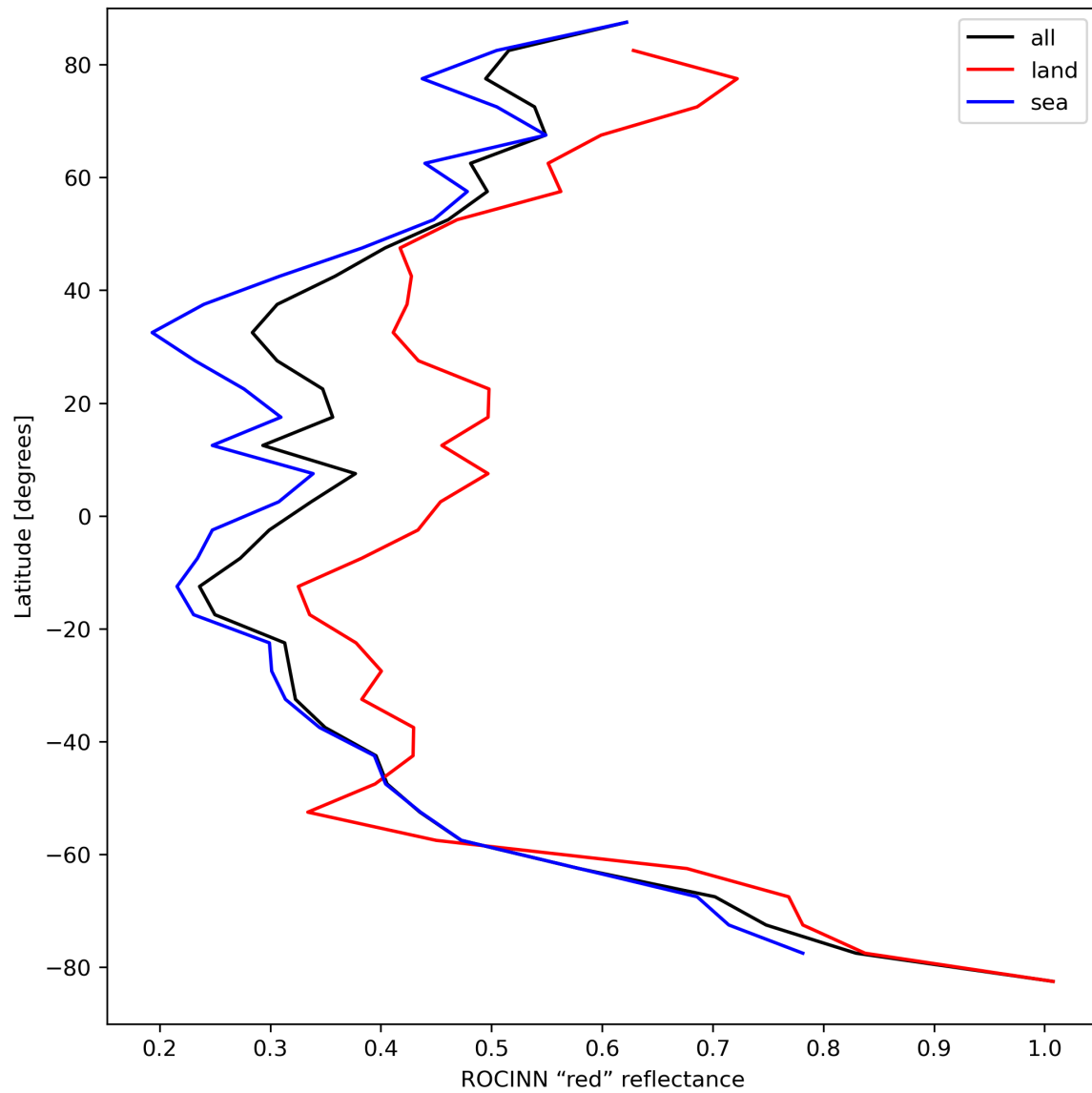
Figure 37: Zonal average of “ROCINN “red” reflectance” for 2023-09-07 to 2023-09-09.
