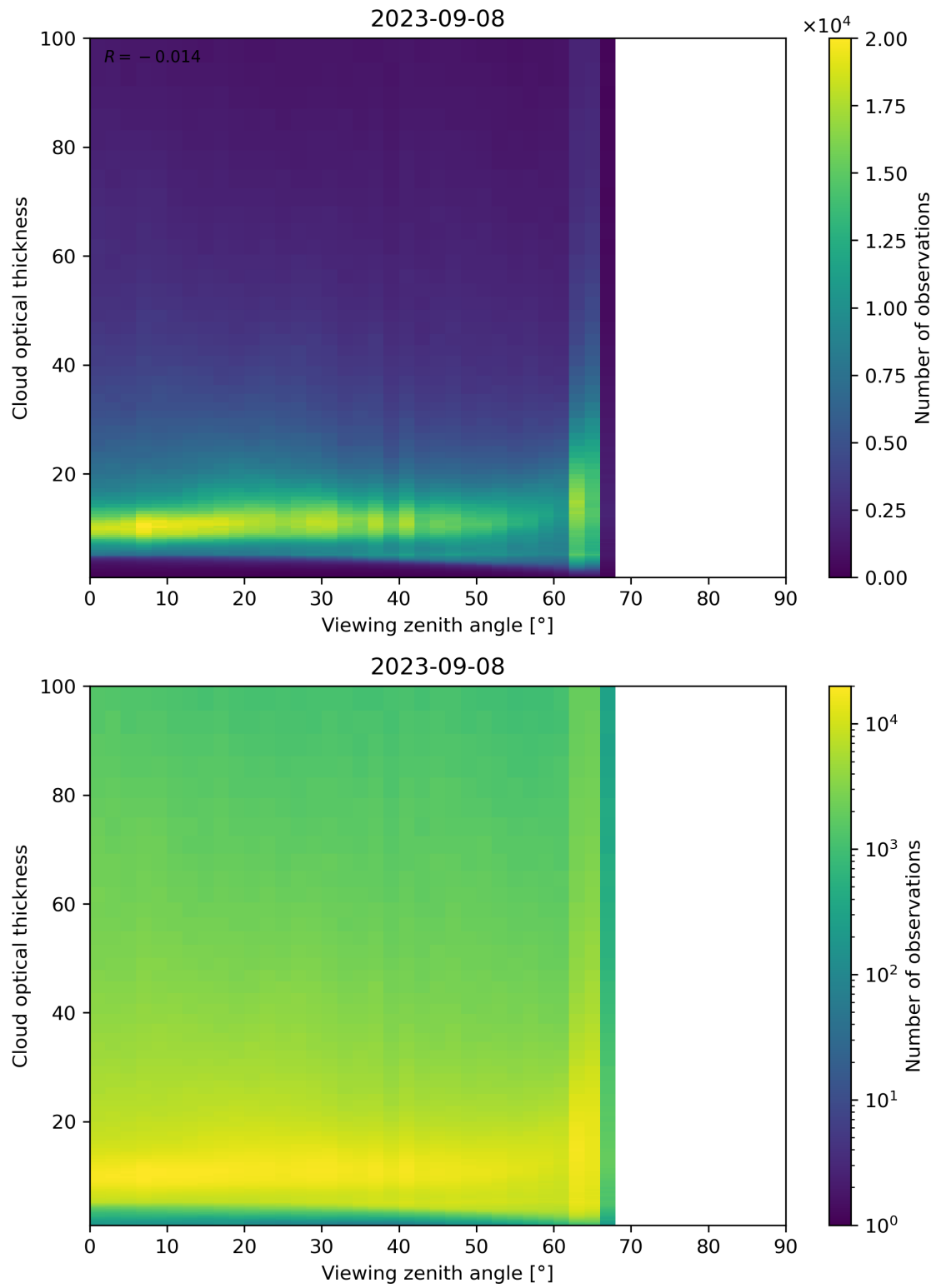
Figure 111: Scatter density plot of “Viewing zenith angle” against “Cloud optical thickness” for 2023-09-07 to 2023-09-09.
