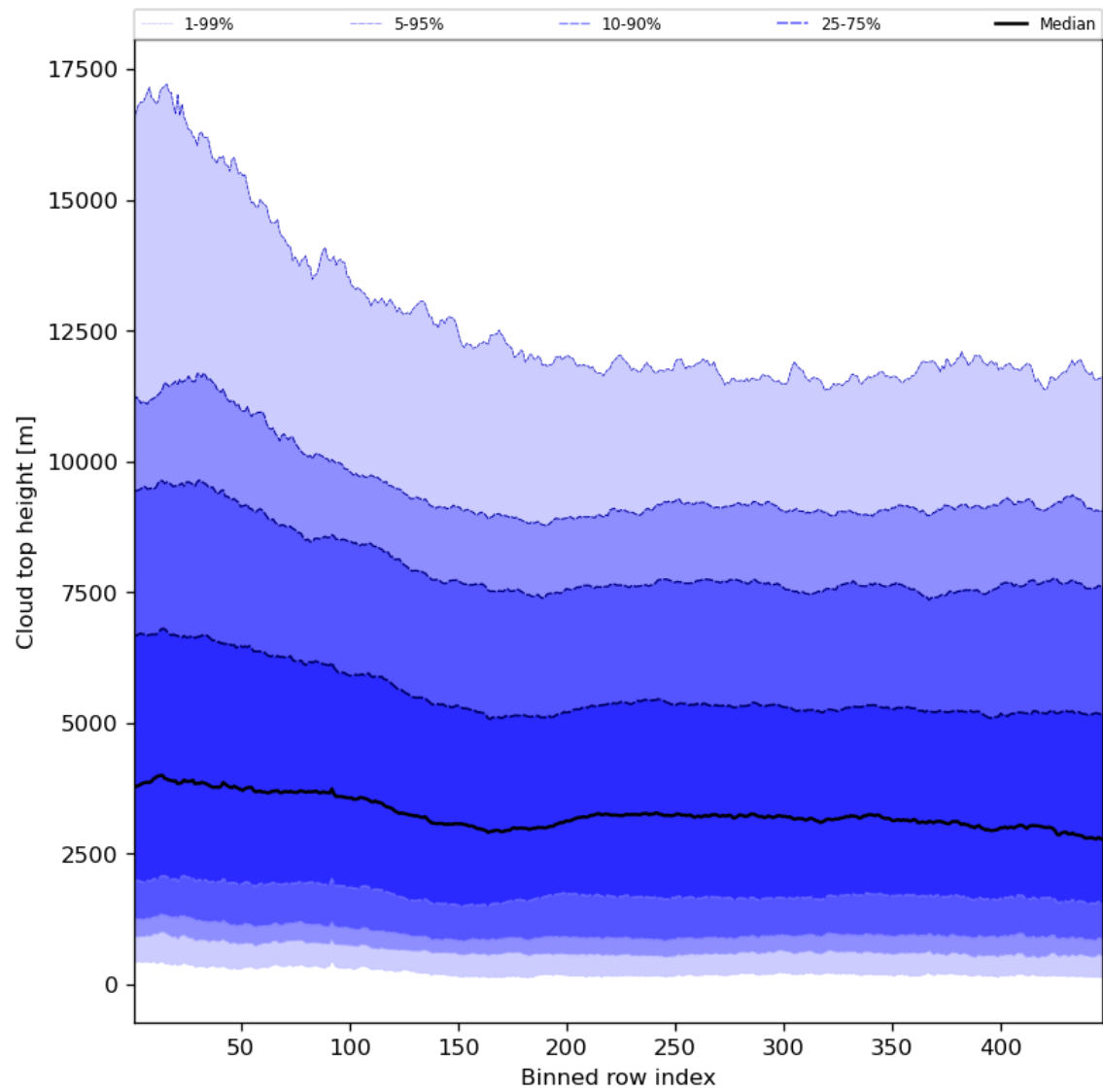
Figure 56: Along track statistics of “Cloud top height” for 2023-09-07 to 2023-09-09
