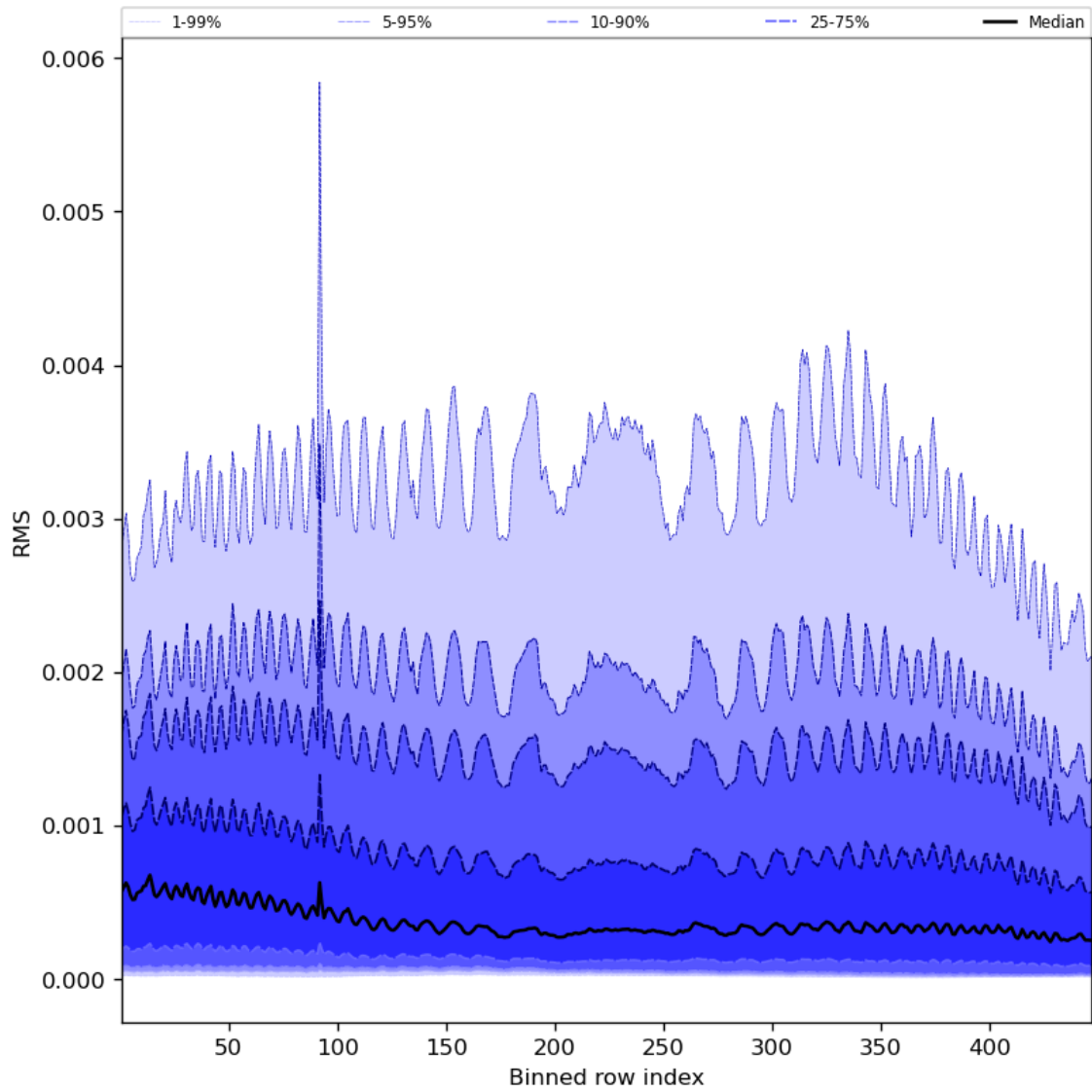
Figure 63: Along track statistics of “RMS” for 2023-09-07 to 2023-09-09
