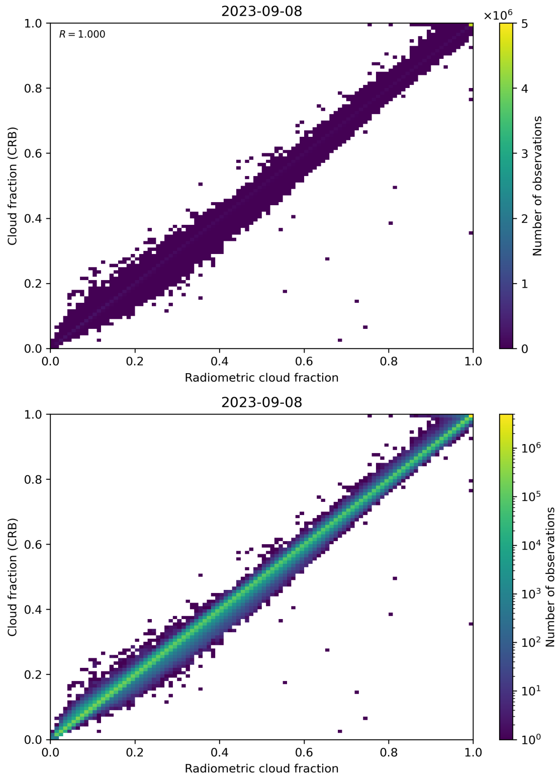
Figure 73: Scatter density plot of “Radiometric cloud fraction” against “Cloud fraction (CRB)” for 2023-09-07 to 2023-09-09.
