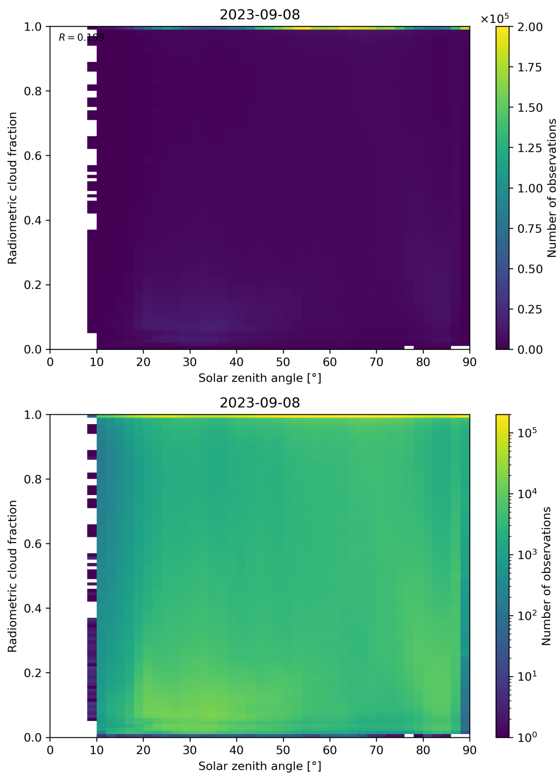
Figure 99: Scatter density plot of “Solar zenith angle” against “Radiometric cloud fraction” for 2023-09-07 to 2023-09-09.
