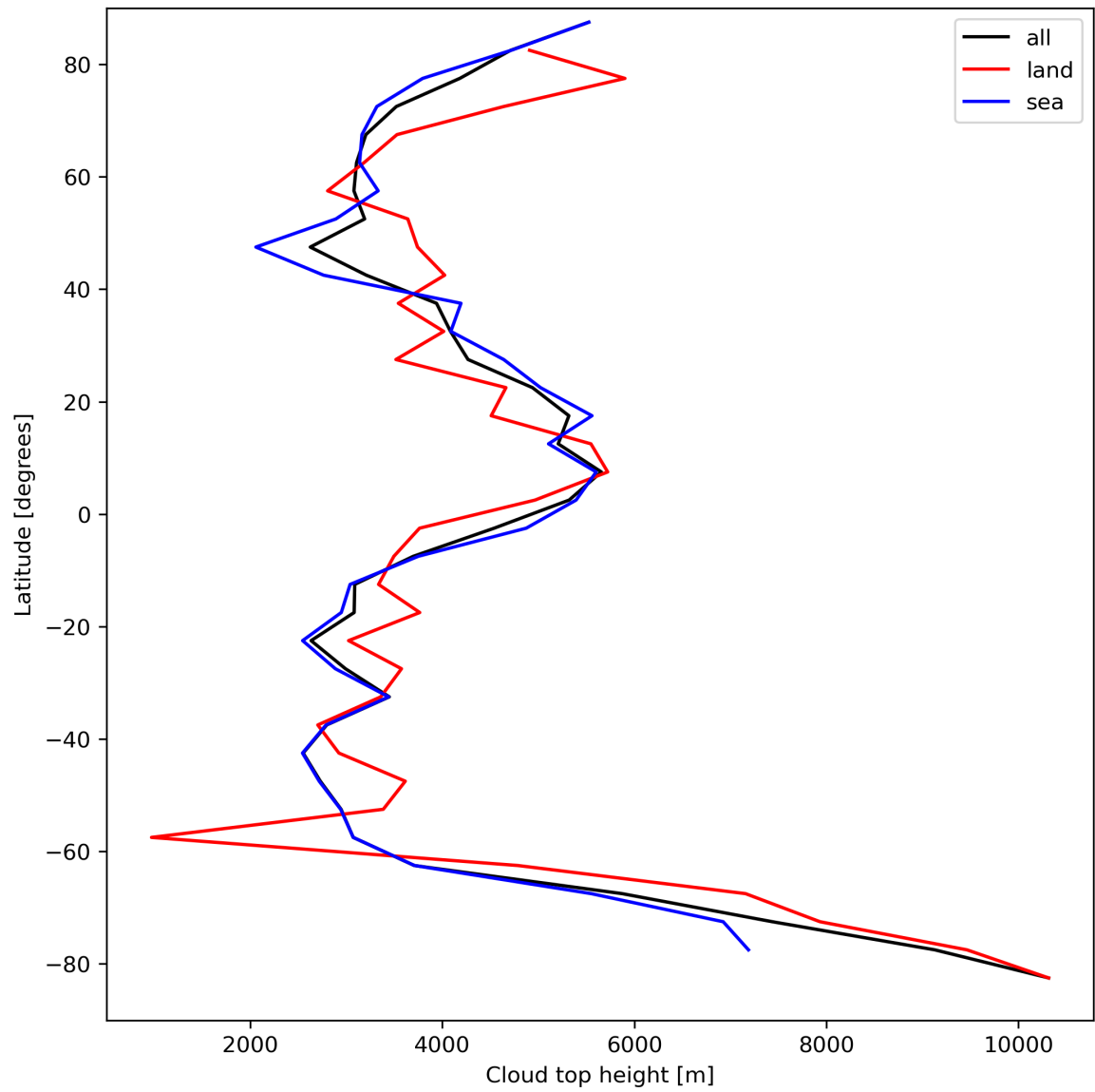
Figure 24: Zonal average of “Cloud top height” for 2023-09-07 to 2023-09-09.
