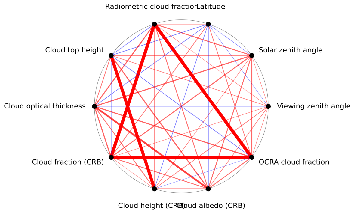
Figure 1: Map of correlation graph for 2023-09-07 to 2023-09-09.
