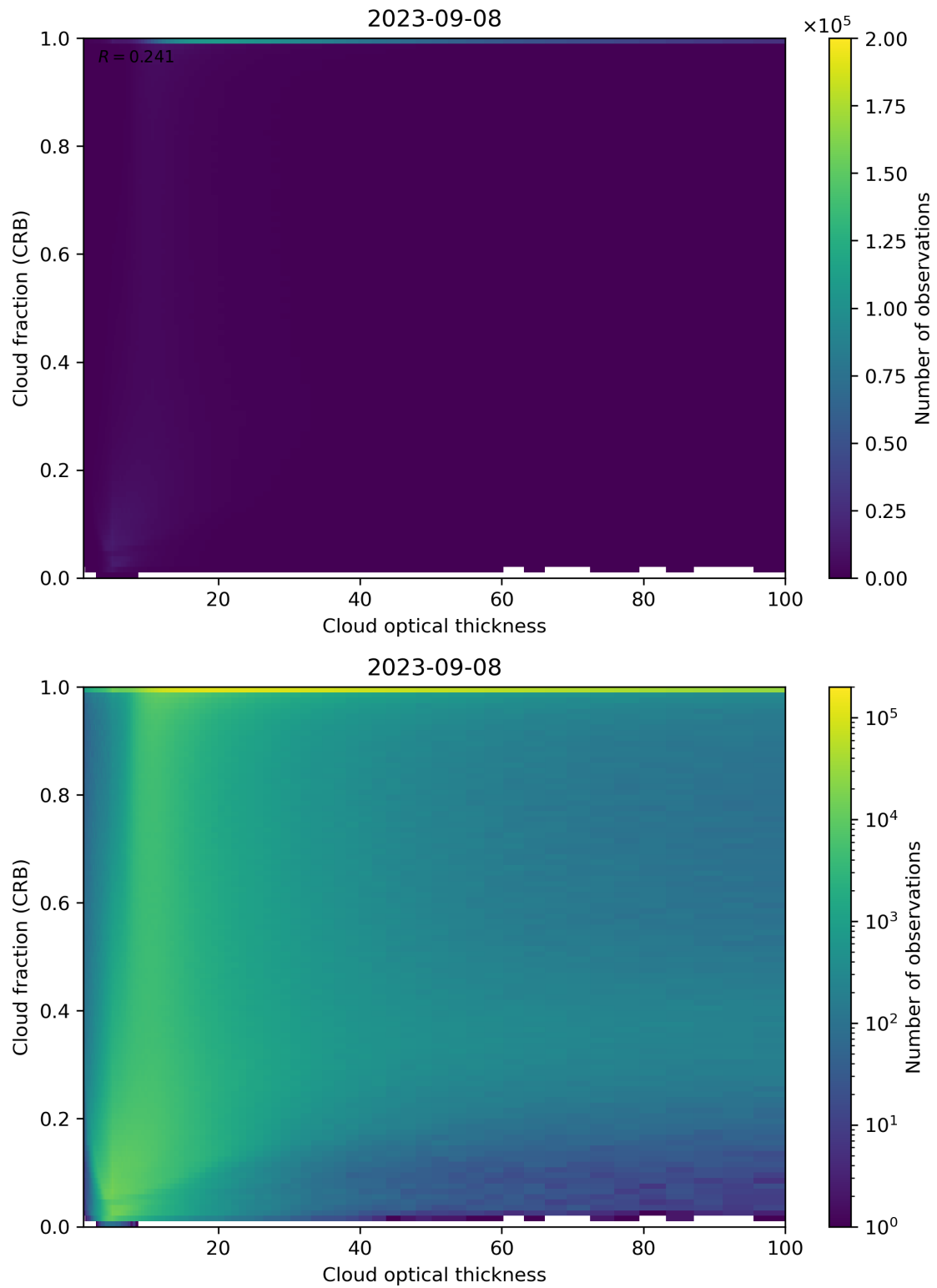
Figure 84: Scatter density plot of “Cloud optical thickness” against “Cloud fraction (CRB)” for 2023-09-07 to 2023-09-09.
