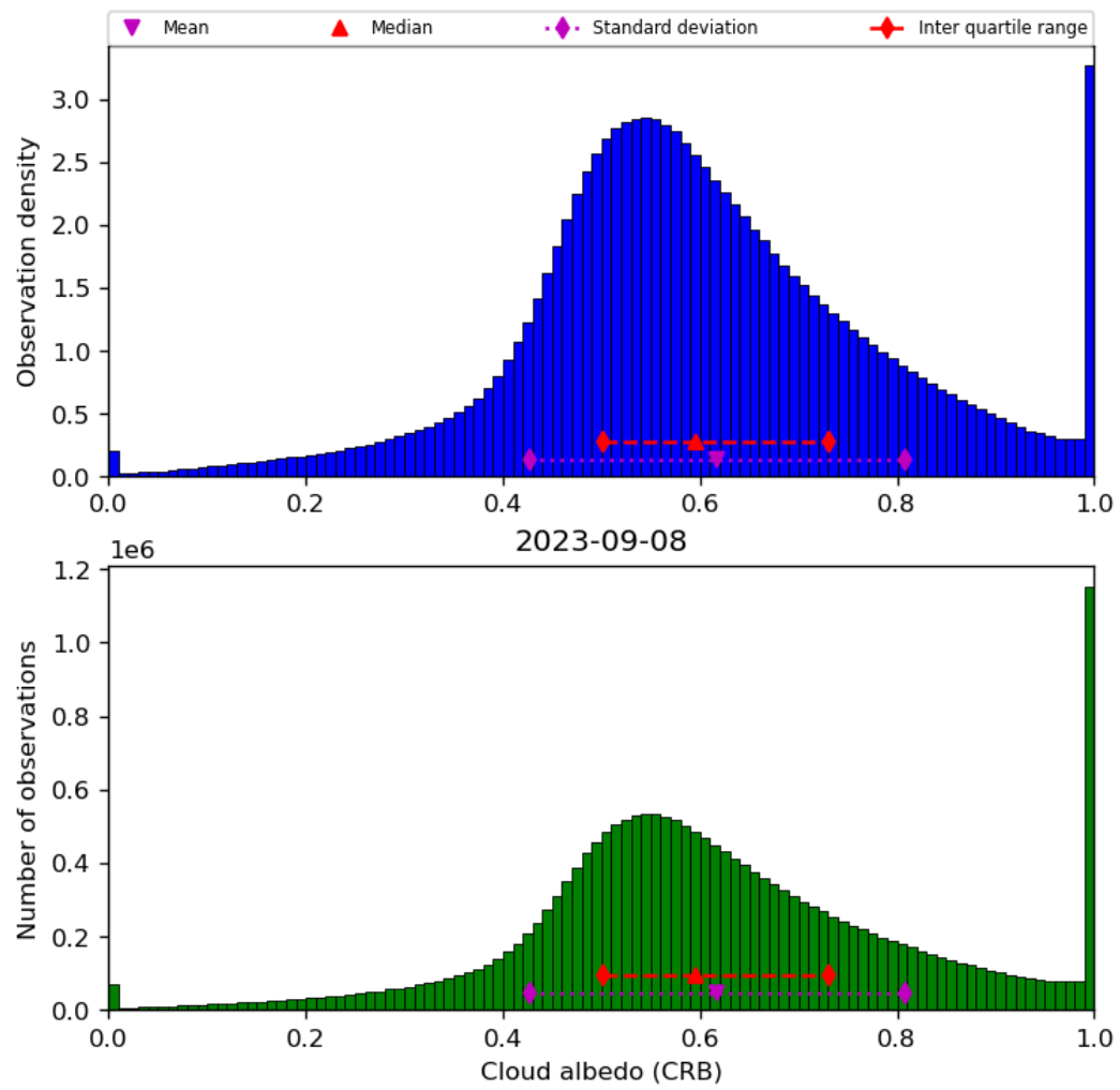
Figure 44: Histogram of “Cloud albedo (CRB)” for 2023-09-07 to 2023-09-09
