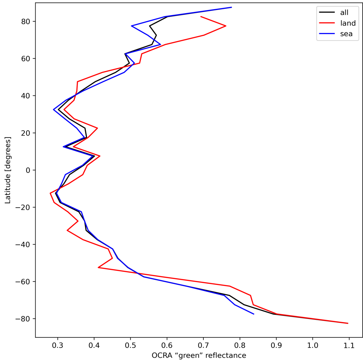
Figure 36: Zonal average of “OCRA “green” reflectance” for 2023-09-07 to 2023-09-09.
