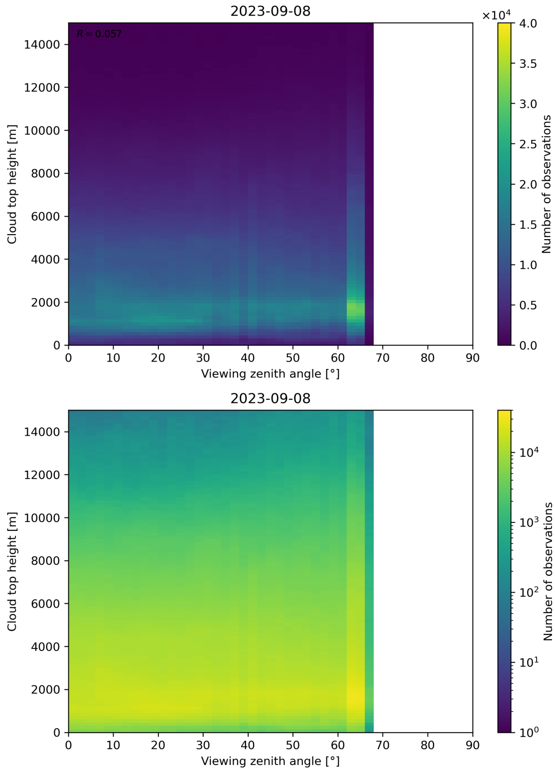
Figure 112: Scatter density plot of “Viewing zenith angle” against “Cloud top height” for 2023-09-07 to 2023-09-09.
