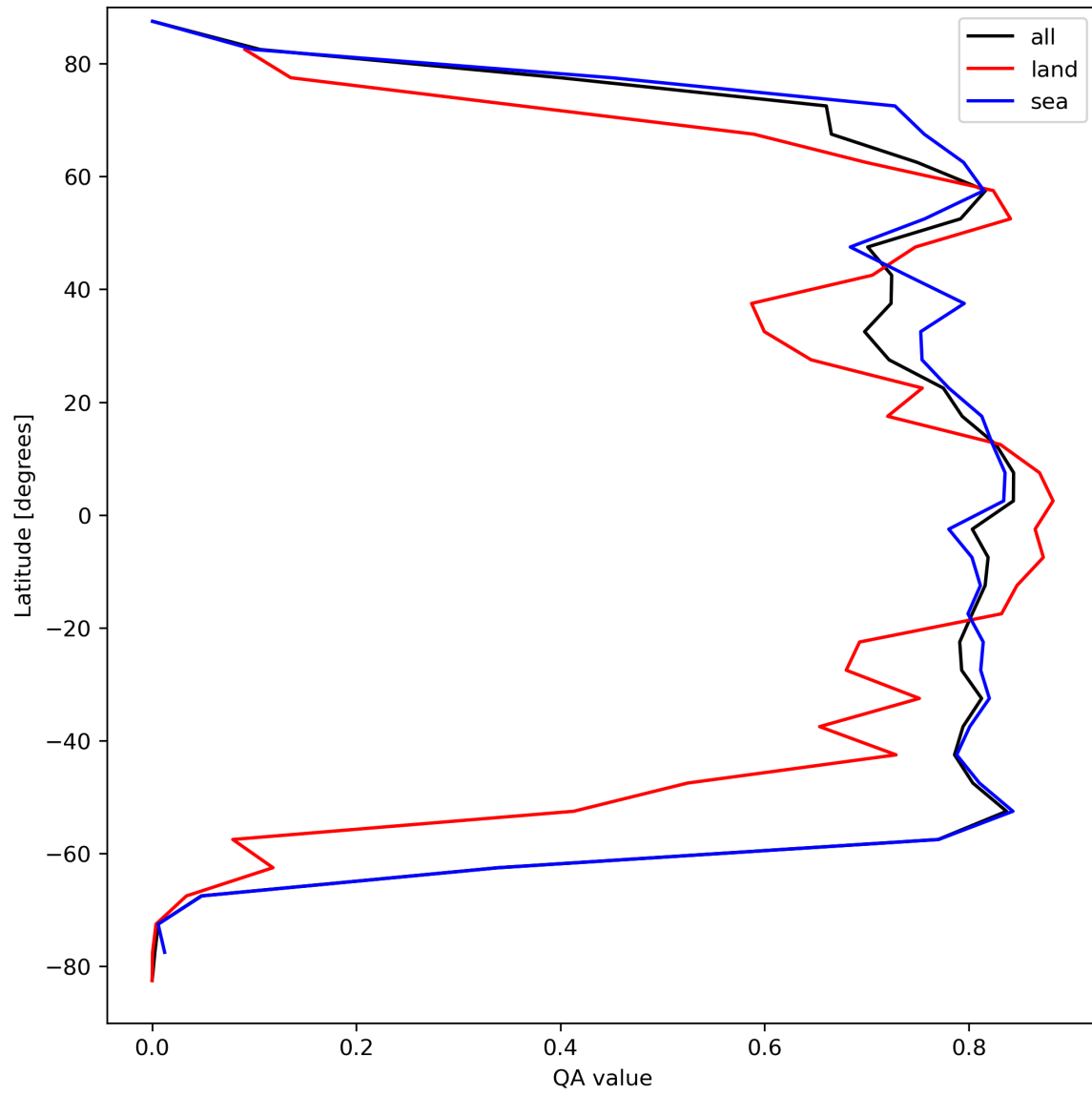
Figure 22: Zonal average of “QA value” for 2023-09-07 to 2023-09-09.
