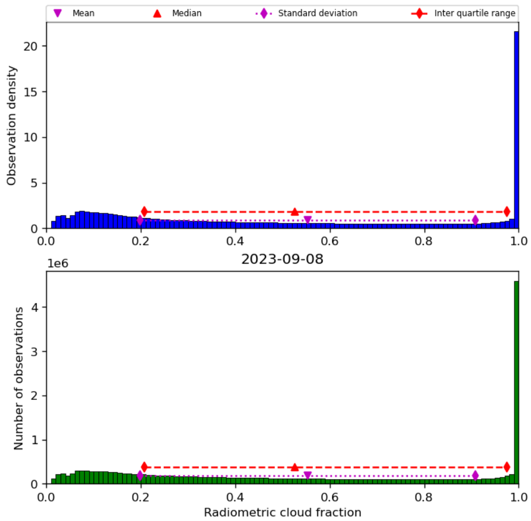
Figure 39: Histogram of “Radiometric cloud fraction” for 2023-09-07 to 2023-09-09
