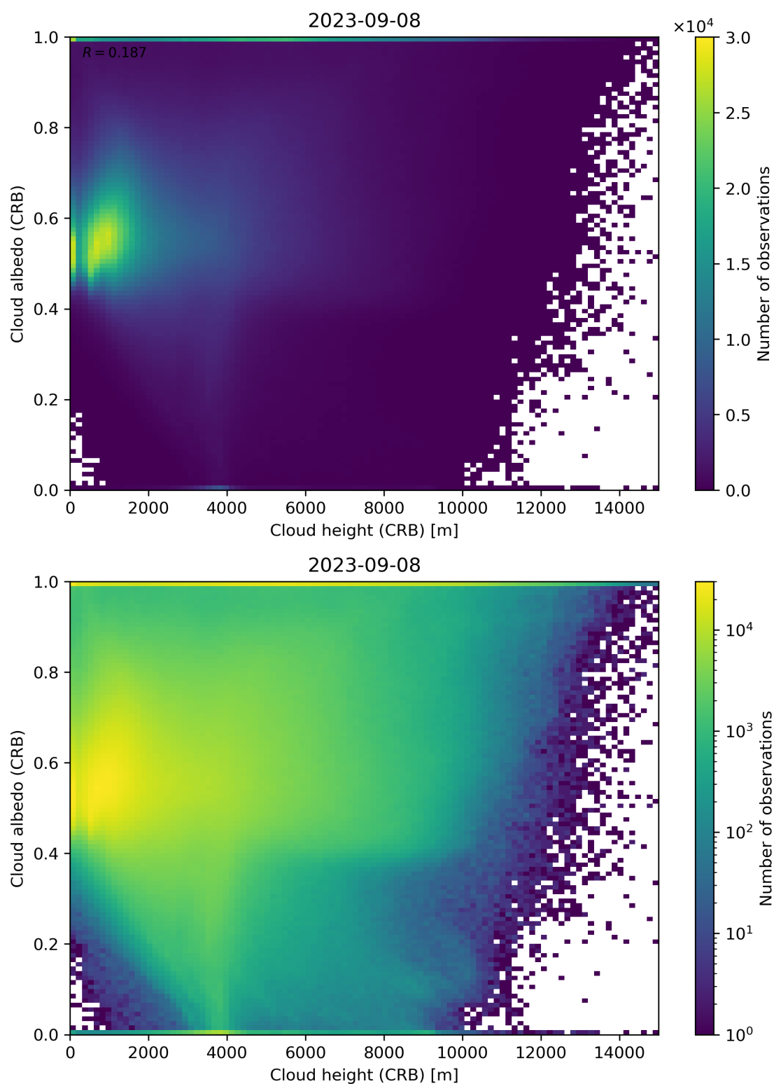
Figure 80: Scatter density plot of “Cloud height (CRB)” against “Cloud albedo (CRB)” for 2023-09-07 to 2023-09-09.
