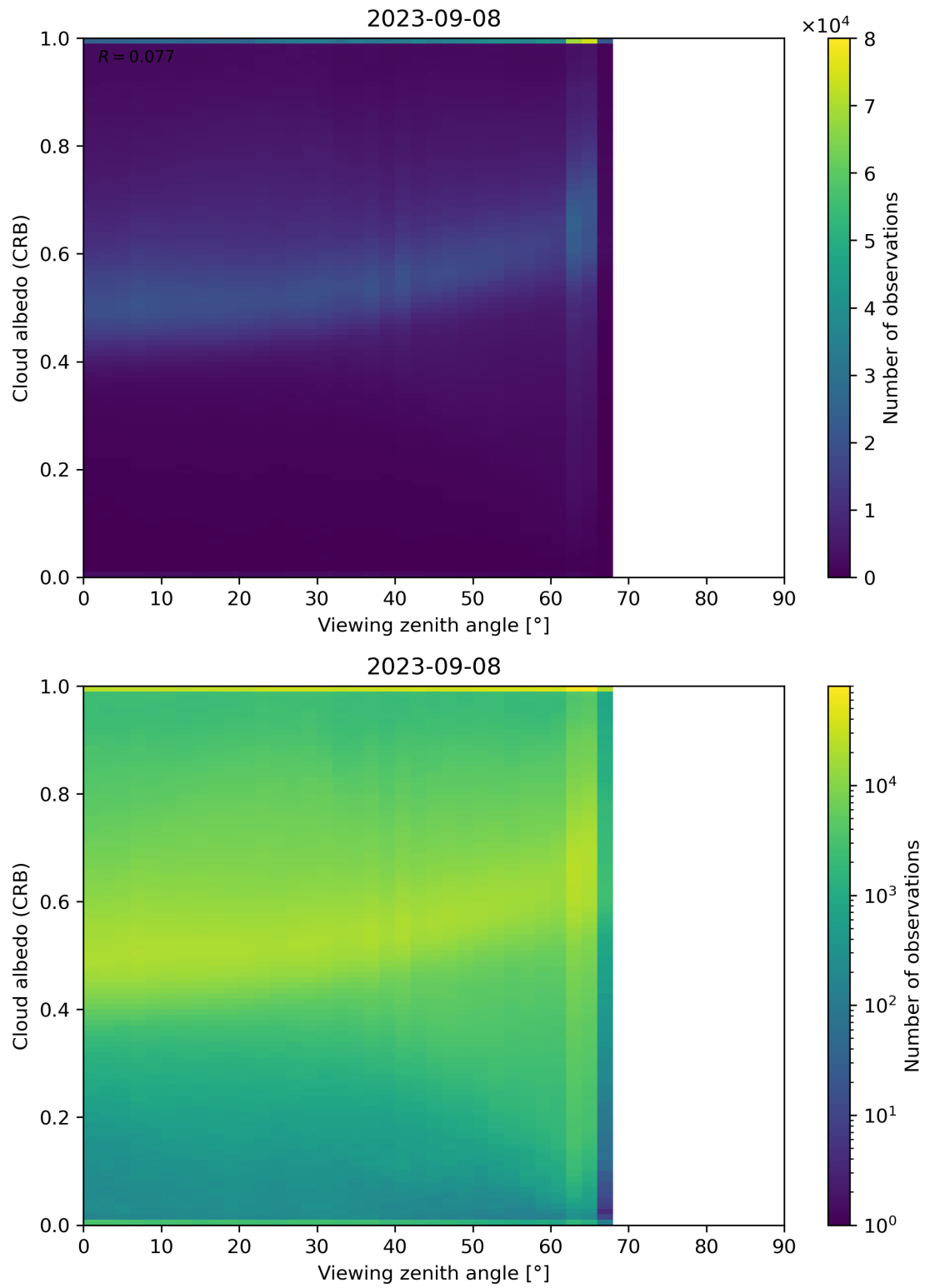
Figure 106: Scatter density plot of “Viewing zenith angle” against “Cloud albedo (CRB)” for 2023-09-07 to 2023-09-09.
