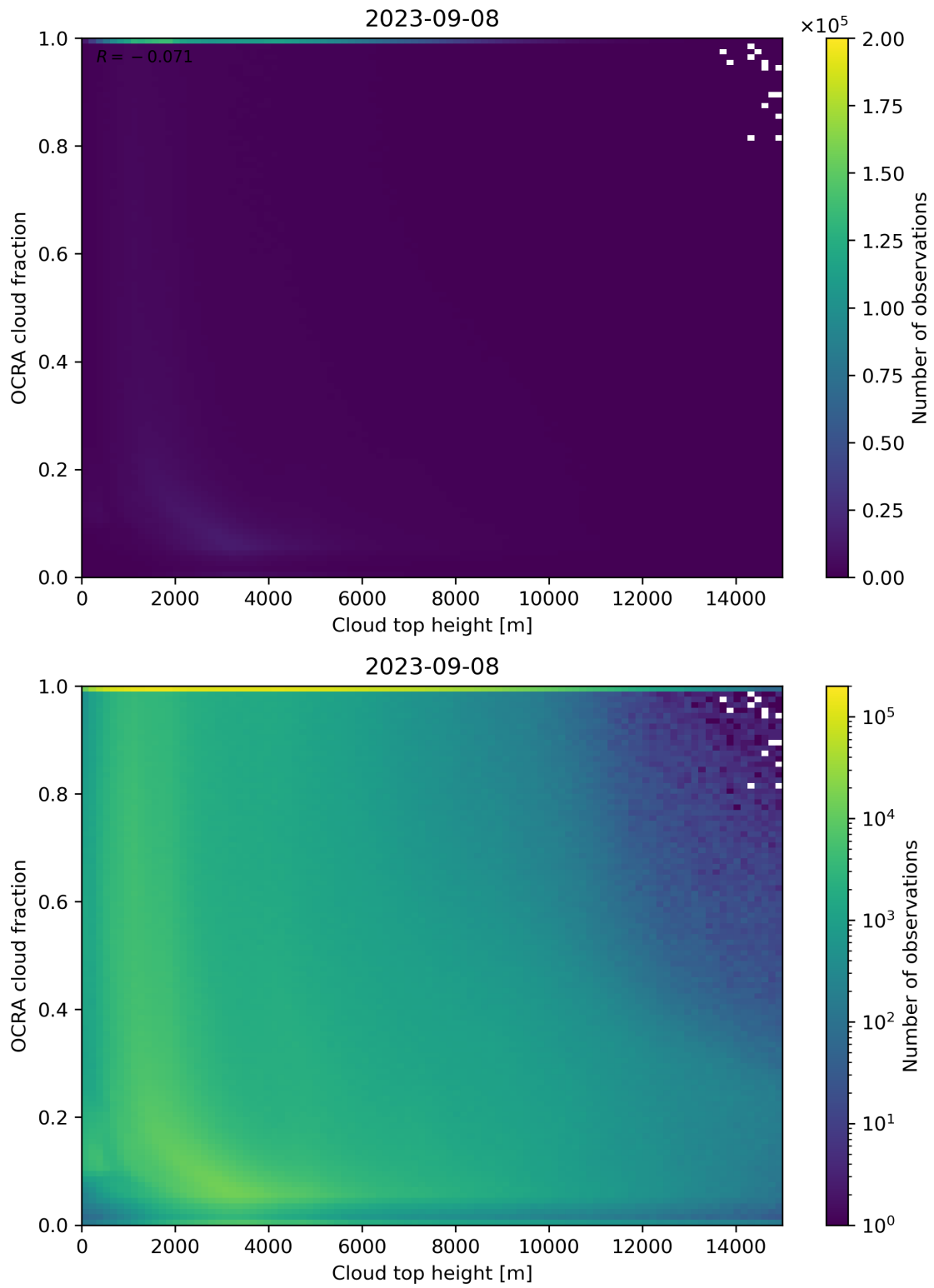
Figure 87: Scatter density plot of “Cloud top height” against “OCRA cloud fraction” for 2023-09-07 to 2023-09-09.
