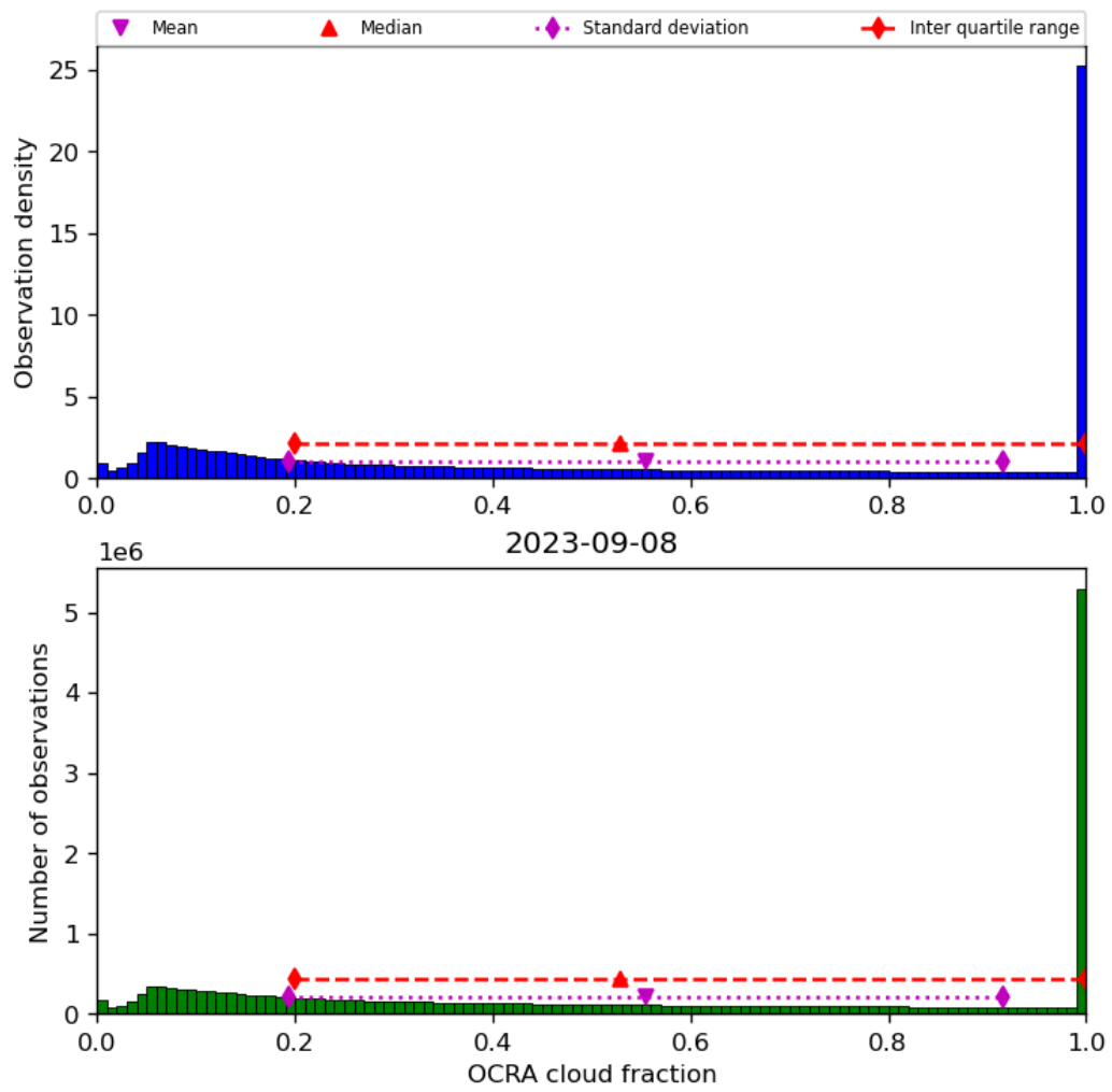
Figure 50: Histogram of “OCRA cloud fraction” for 2023-09-07 to 2023-09-09
