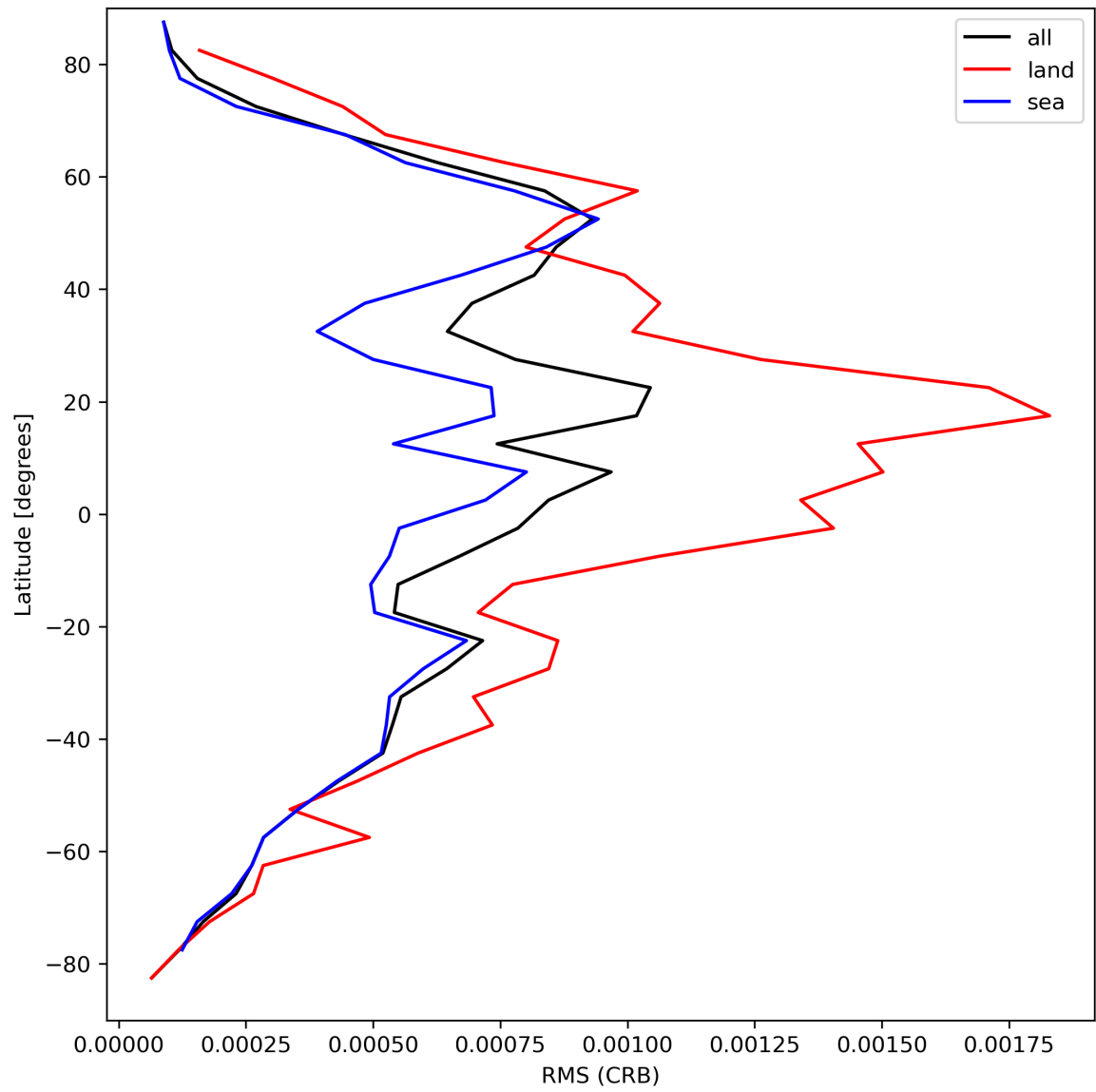
Figure 32: Zonal average of “RMS (CRB)” for 2023-09-07 to 2023-09-09.
