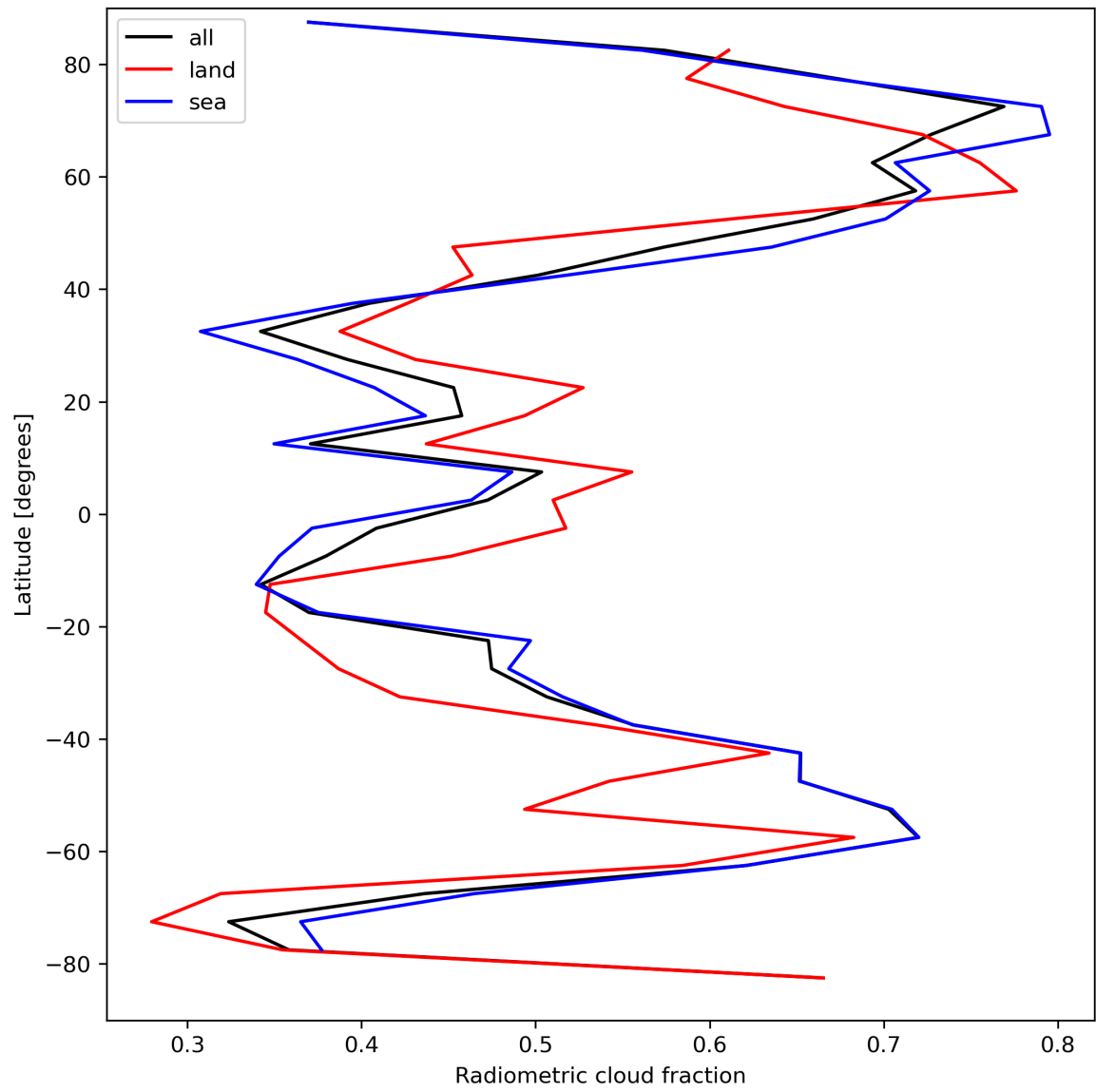
Figure 23: Zonal average of “Radiometric cloud fraction” for 2023-09-07 to 2023-09-09.
