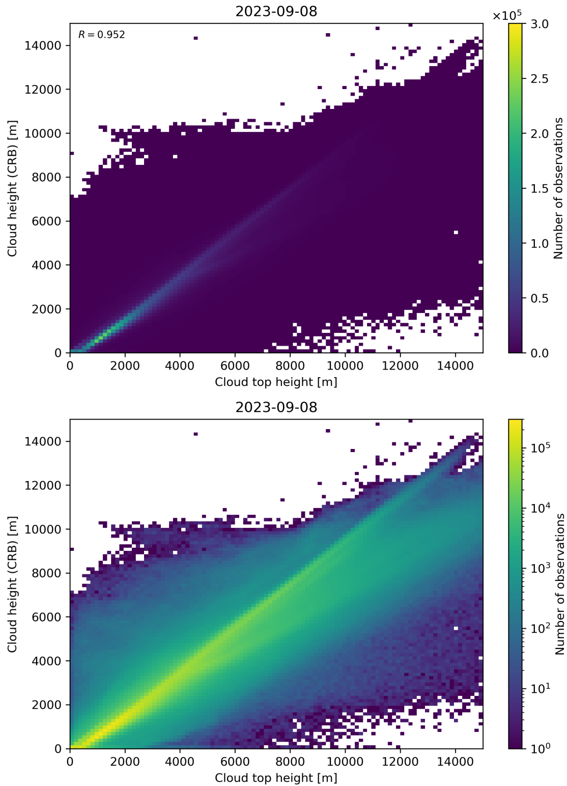
Figure 89: Scatter density plot of “Cloud top height” against “Cloud height (CRB)” for 2023-09-07 to 2023-09-09.
