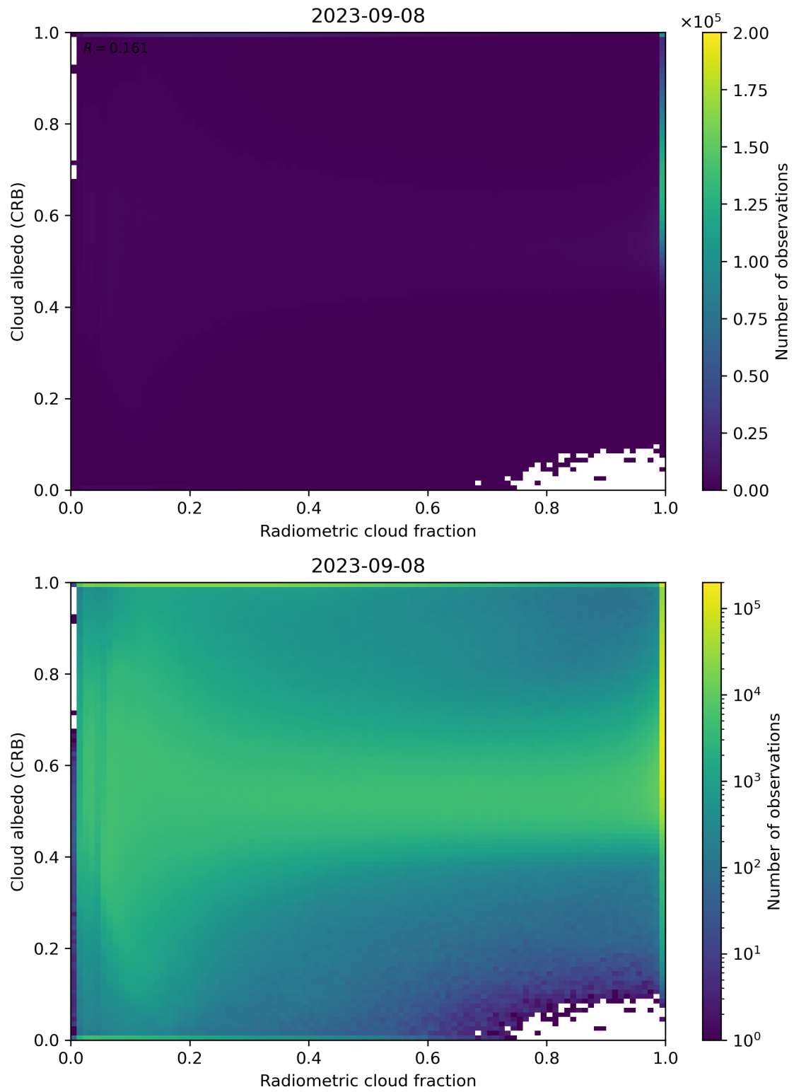
Figure 71: Scatter density plot of “Radiometric cloud fraction” against “Cloud albedo (CRB)” for 2023-09-07 to 2023-09-09.
