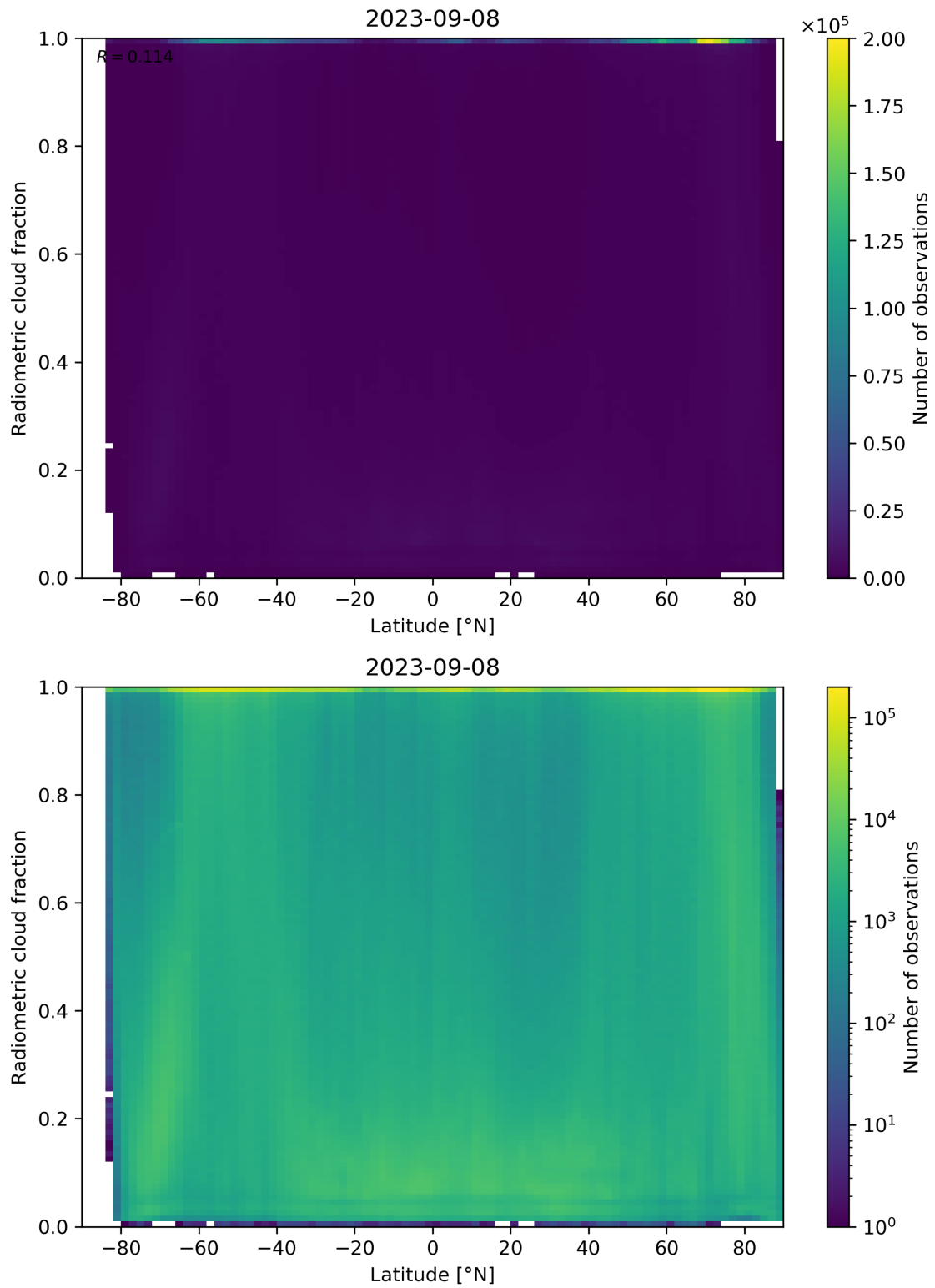
Figure 92: Scatter density plot of “Latitude” against “Radiometric cloud fraction” for 2023-09-07 to 2023-09-09.
