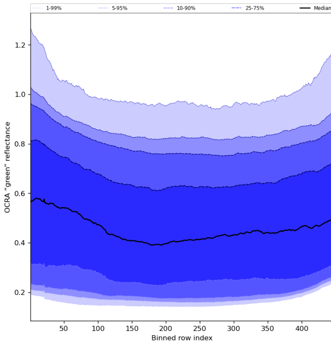
Figure 68: Along track statistics of “OCRA “green” reflectance” for 2023-09-07 to 2023-09-09
