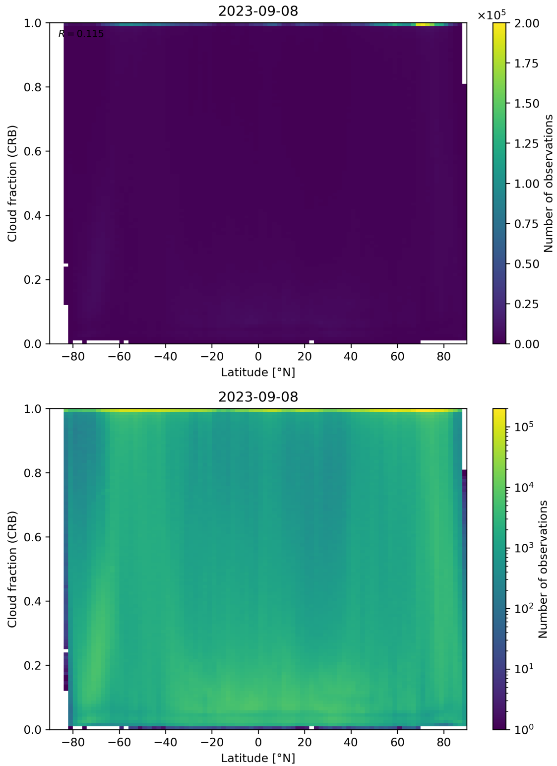
Figure 94: Scatter density plot of “Latitude” against “Cloud fraction (CRB)” for 2023-09-07 to 2023-09-09.
