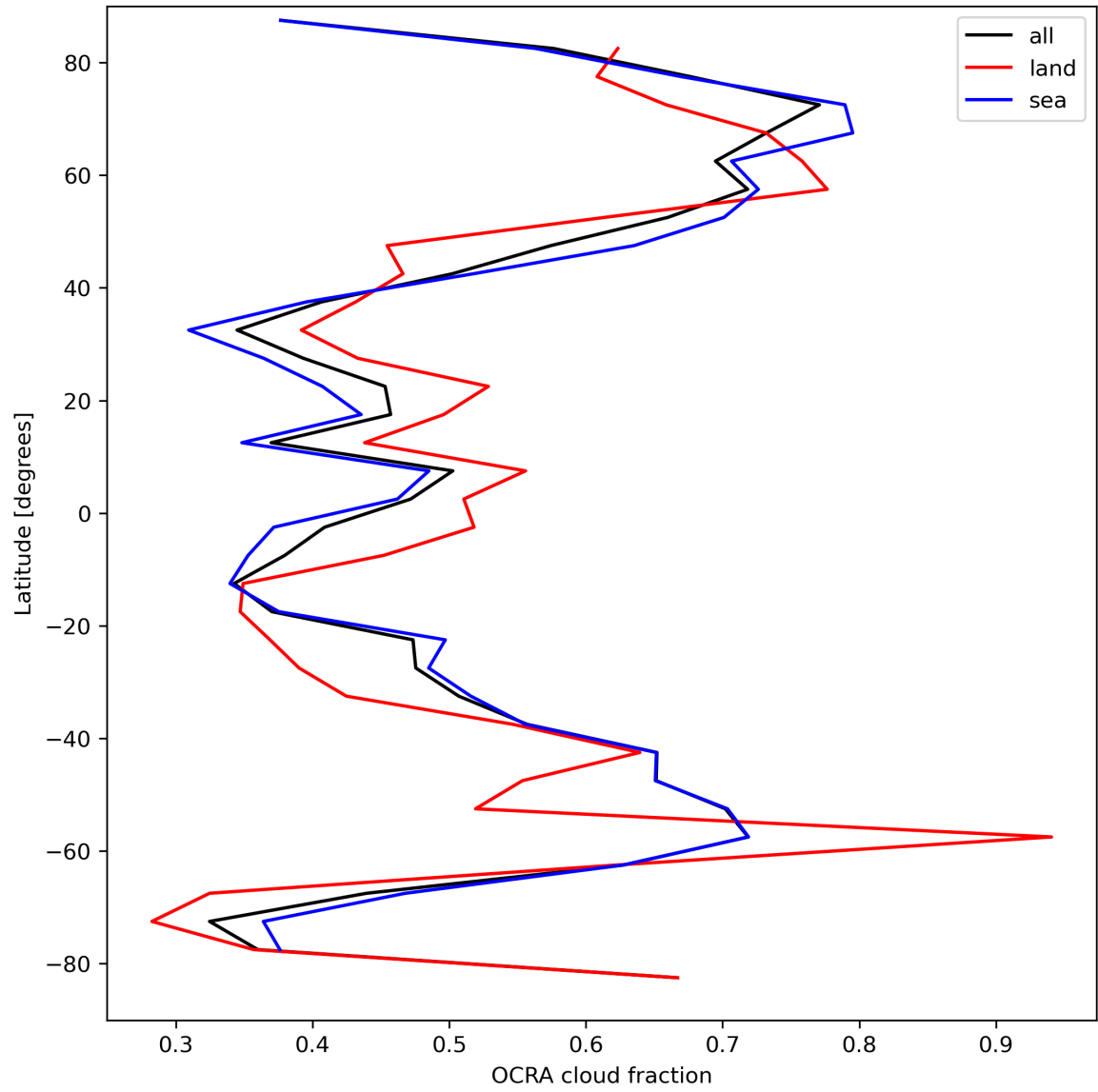
Figure 34: Zonal average of “OCRA cloud fraction” for 2023-09-07 to 2023-09-09.
