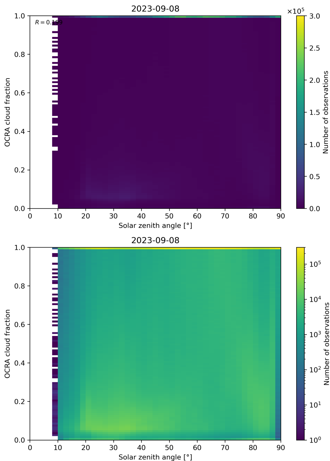
Figure 100: Scatter density plot of “Solar zenith angle” against “OCRA cloud fraction” for 2023-09-07 to 2023-09-09.
