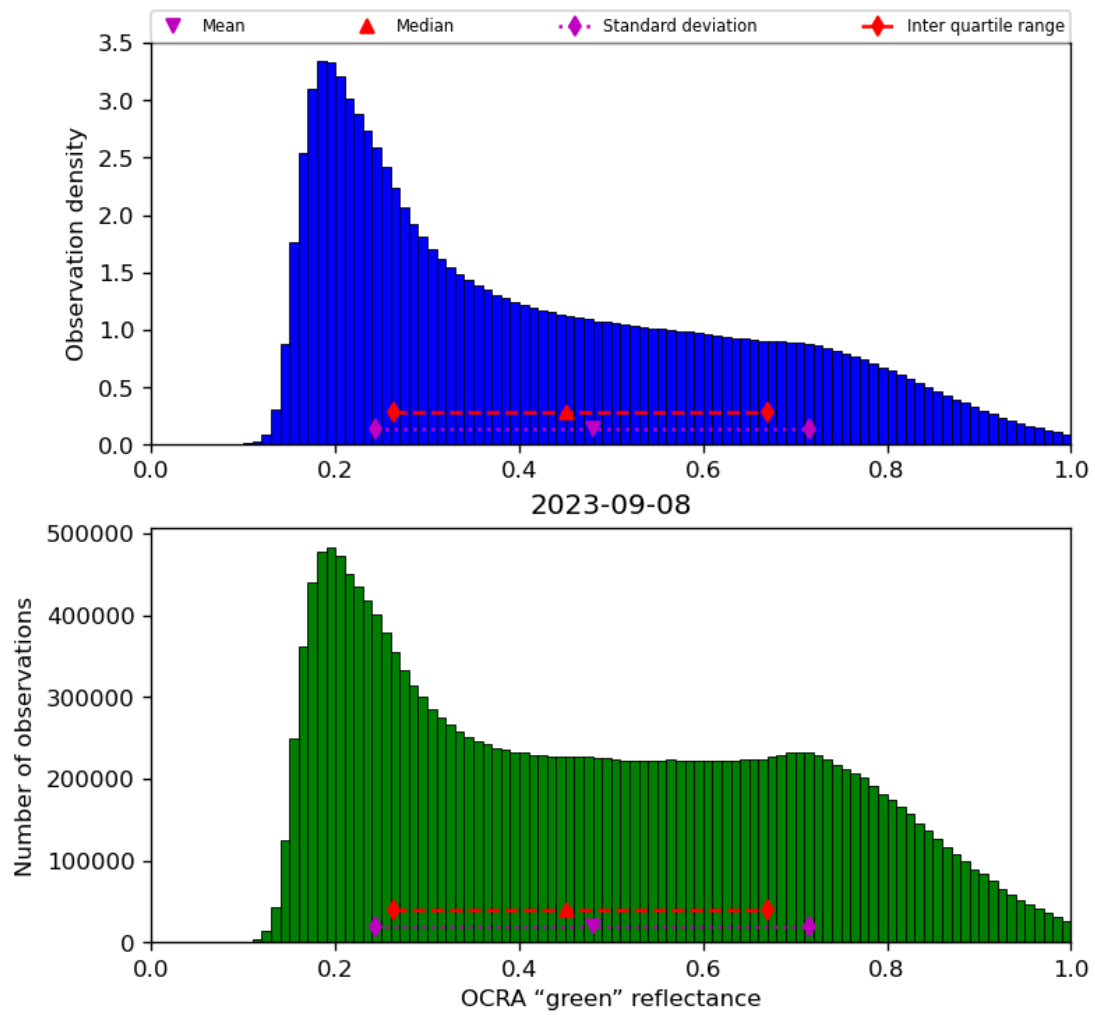
Figure 52: Histogram of “OCRA “green” reflectance” for 2023-09-07 to 2023-09-09
