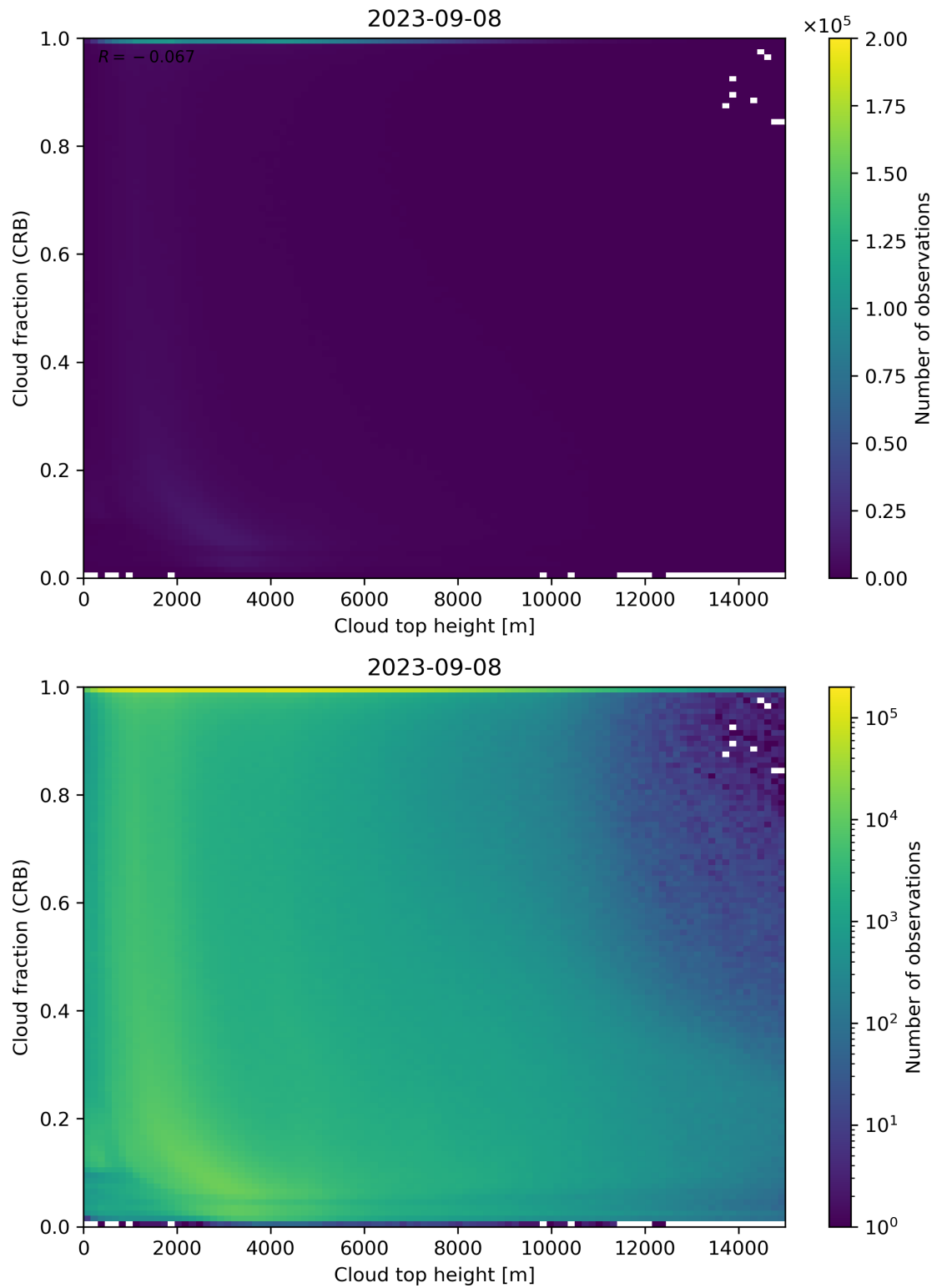
Figure 88: Scatter density plot of “Cloud top height” against “Cloud fraction (CRB)” for 2023-09-07 to 2023-09-09.
