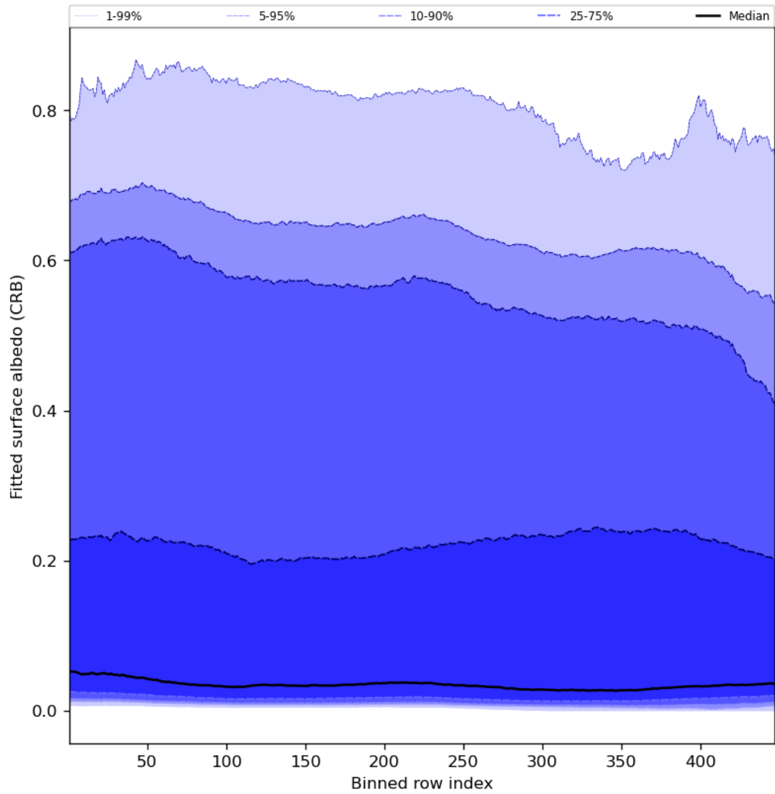
Figure 62: Along track statistics of “Fitted surface albedo (CRB)” for 2023-09-07 to 2023-09-09
