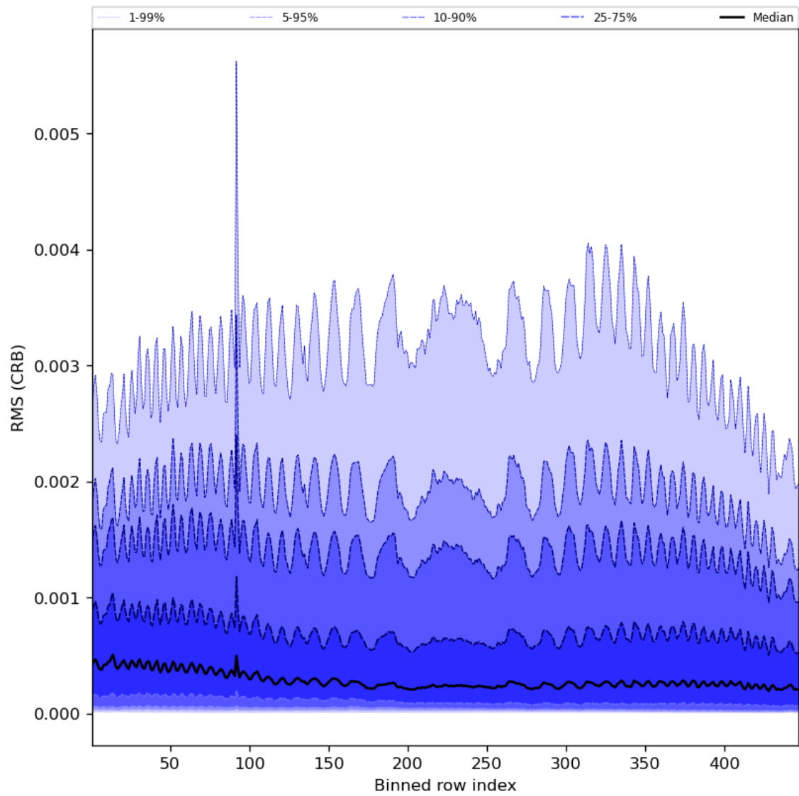
Figure 64: Along track statistics of “RMS (CRB)” for 2023-09-07 to 2023-09-09
