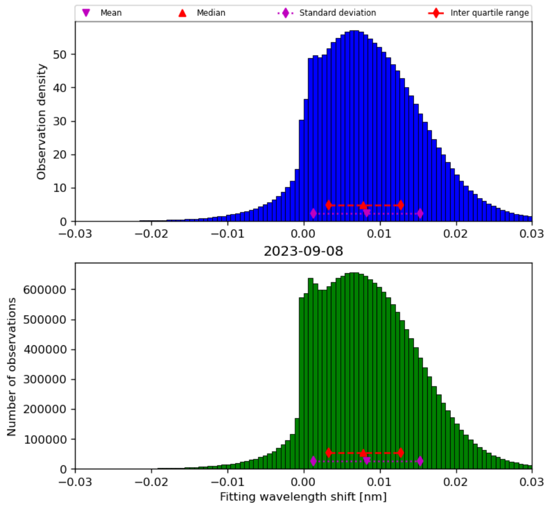
Figure 49: Histogram of “Fitting wavelength shift” for 2023-09-07 to 2023-09-09
