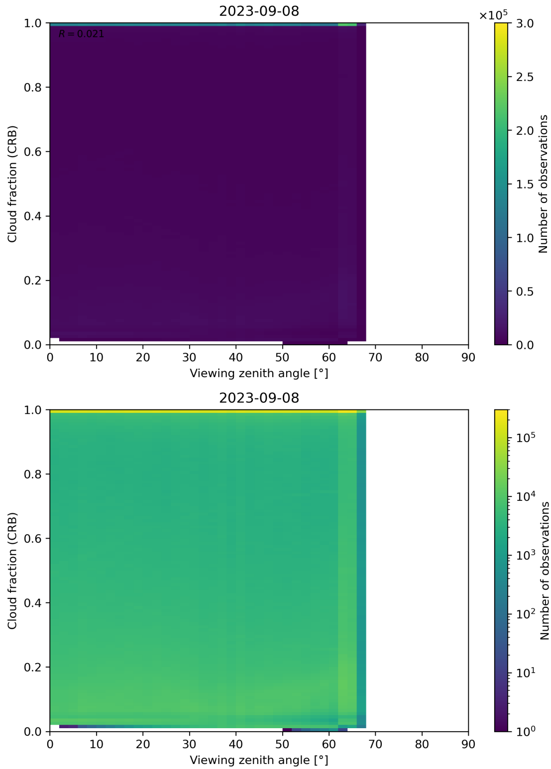
Figure 109: Scatter density plot of “Viewing zenith angle” against “Cloud fraction (CRB)” for 2023-09-07 to 2023-09-09.
