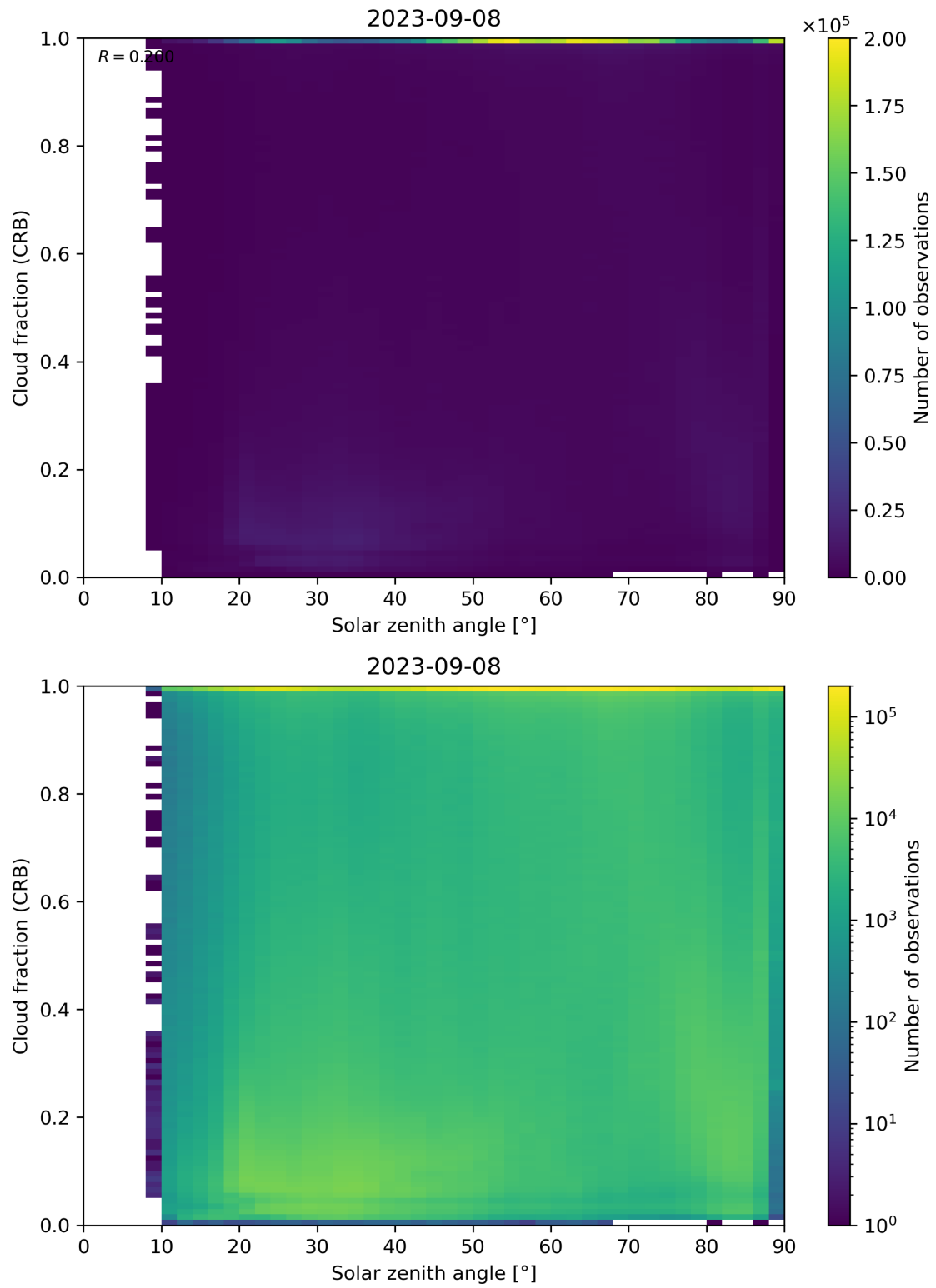
Figure 101: Scatter density plot of “Solar zenith angle” against “Cloud fraction (CRB)” for 2023-09-07 to 2023-09-09.
