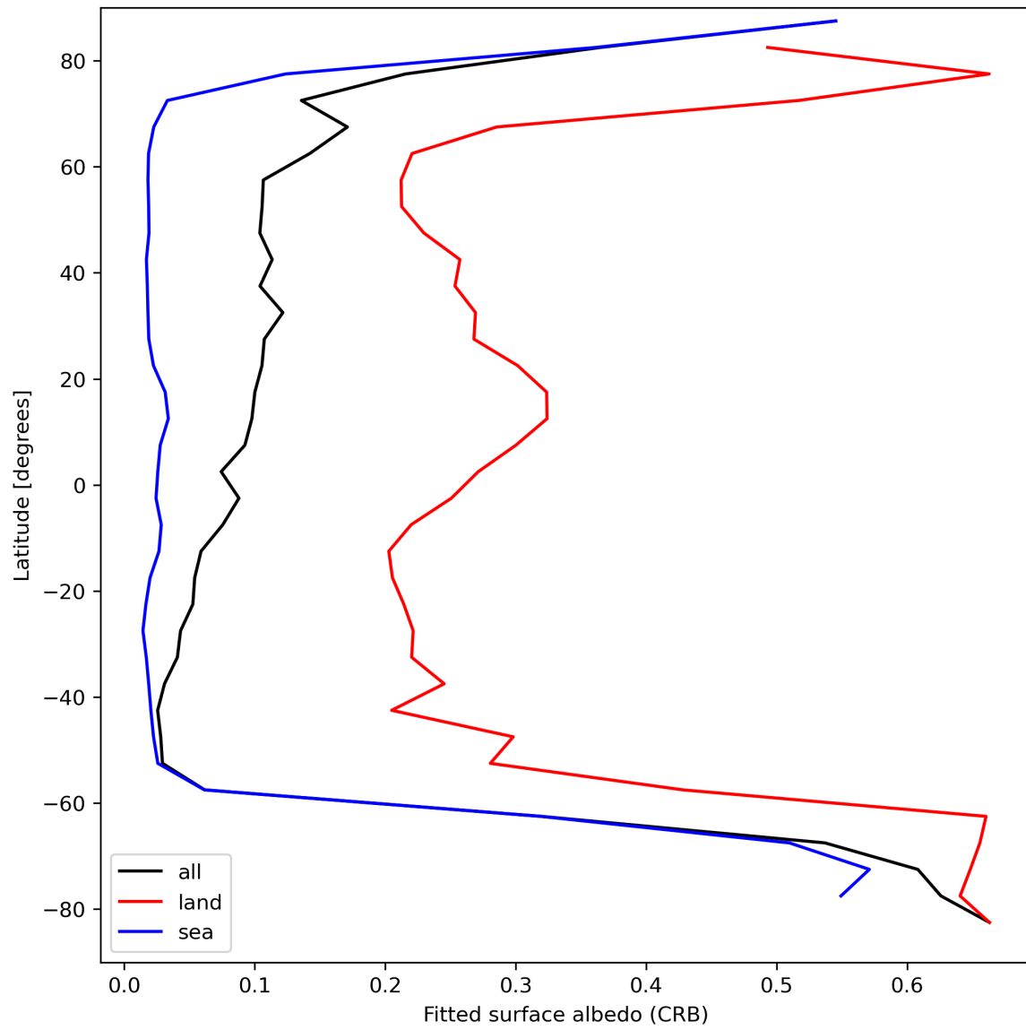
Figure 30: Zonal average of “Fitted surface albedo (CRB)” for 2023-09-07 to 2023-09-09.
