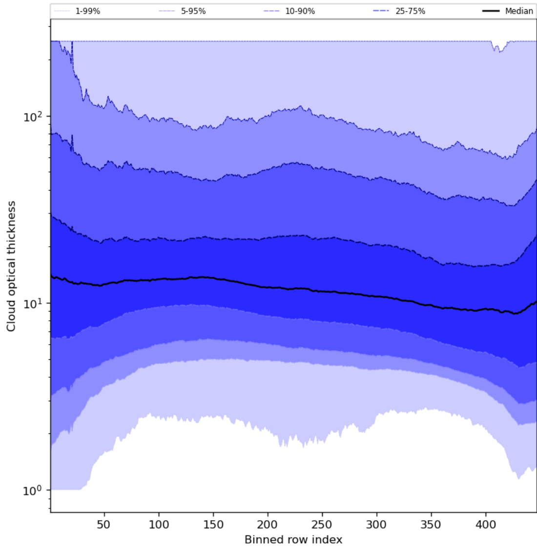
Figure 57: Along track statistics of “Cloud optical thickness” for 2023-09-07 to 2023-09-09
