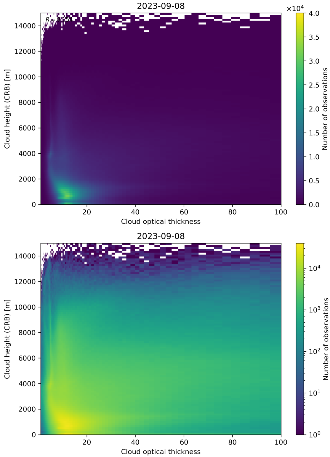
Figure 85: Scatter density plot of “Cloud optical thickness” against “Cloud height (CRB)” for 2023-09-07 to 2023-09-09.
