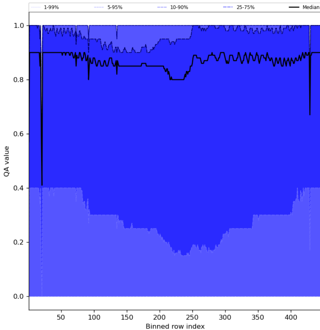
Figure 54: Along track statistics of “QA value” for 2023-09-07 to 2023-09-09
