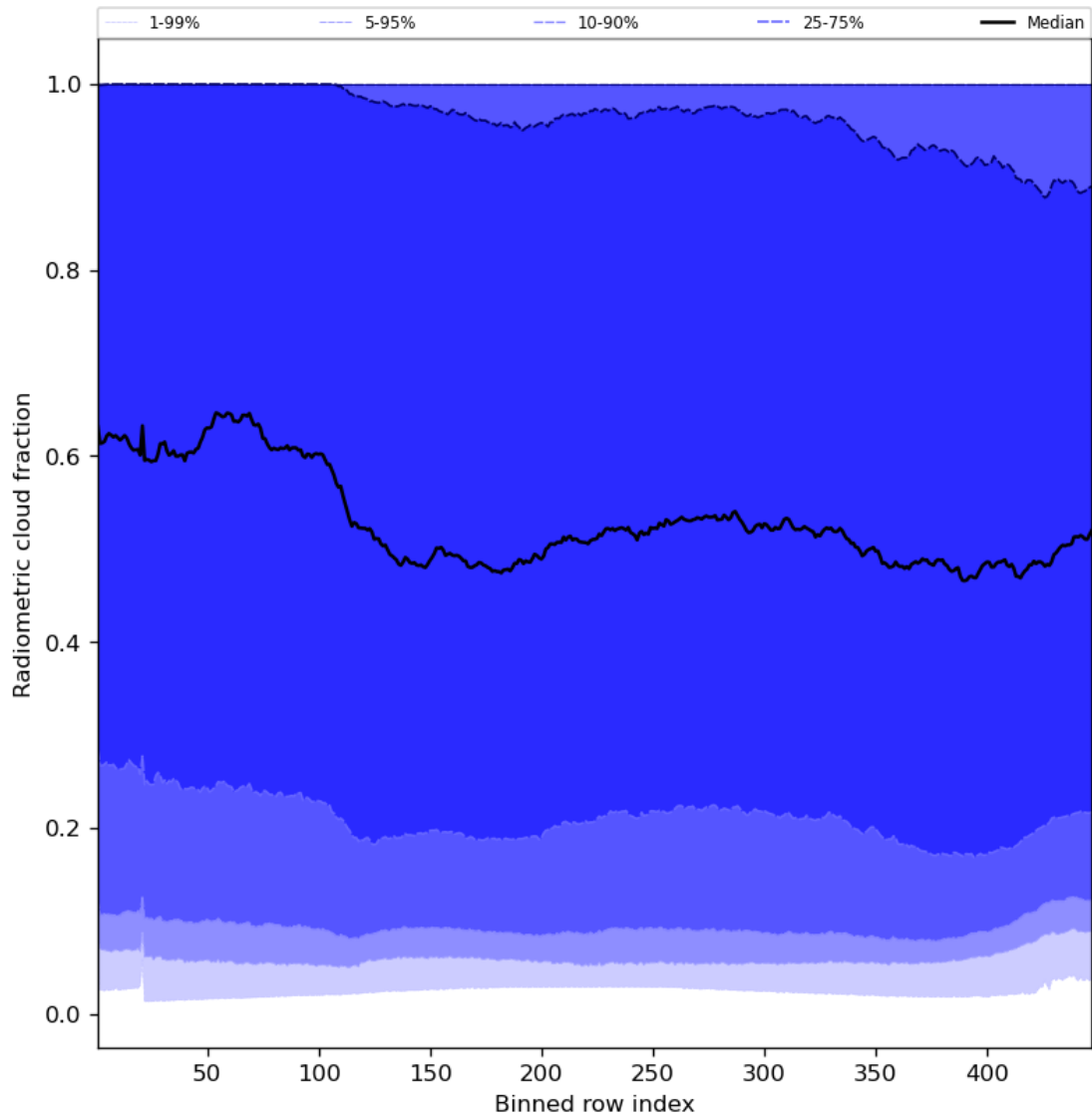
Figure 55: Along track statistics of “Radiometric cloud fraction” for 2023-09-07 to 2023-09-09
