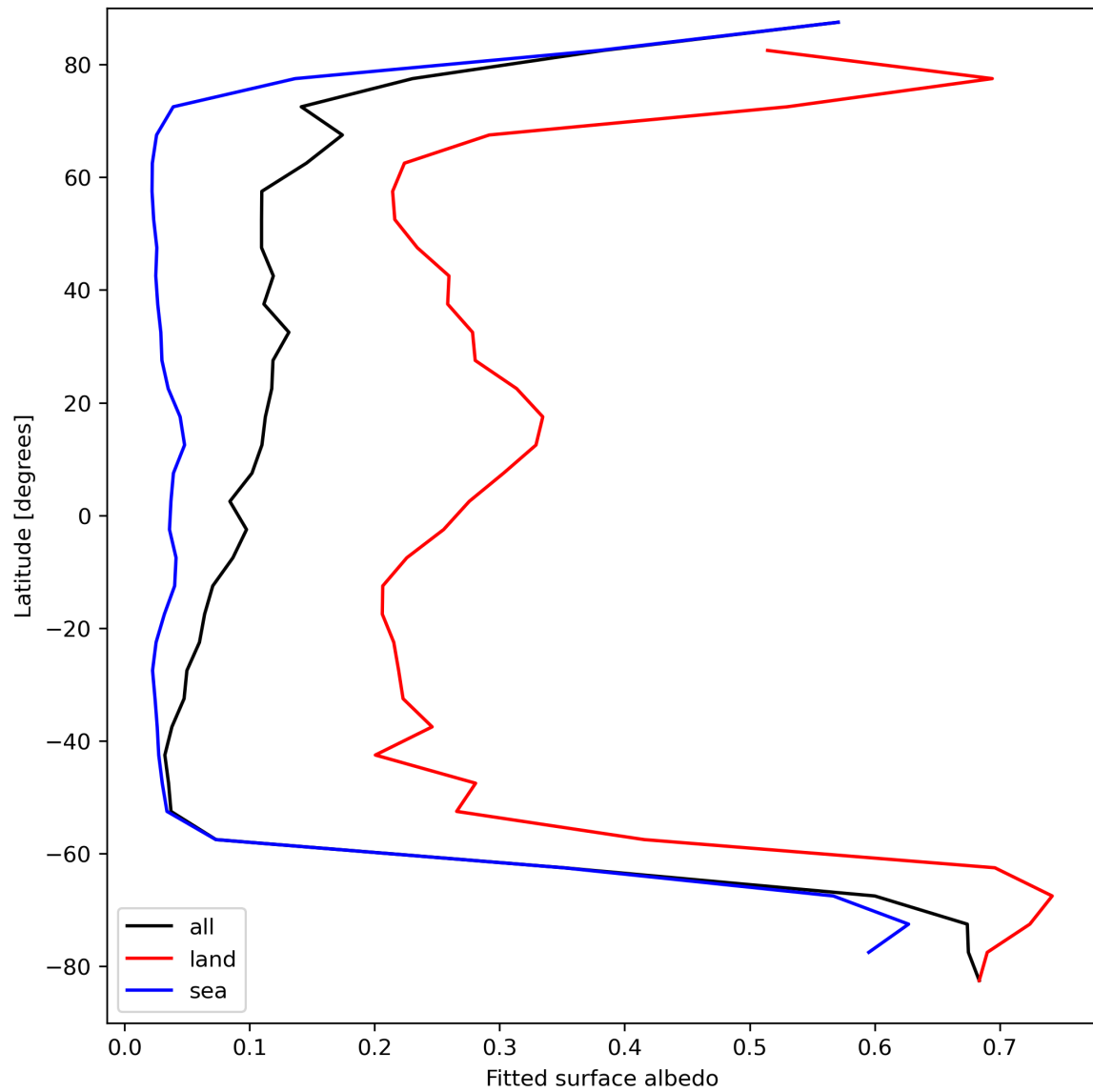
Figure 29: Zonal average of “Fitted surface albedo” for 2023-09-07 to 2023-09-09.
