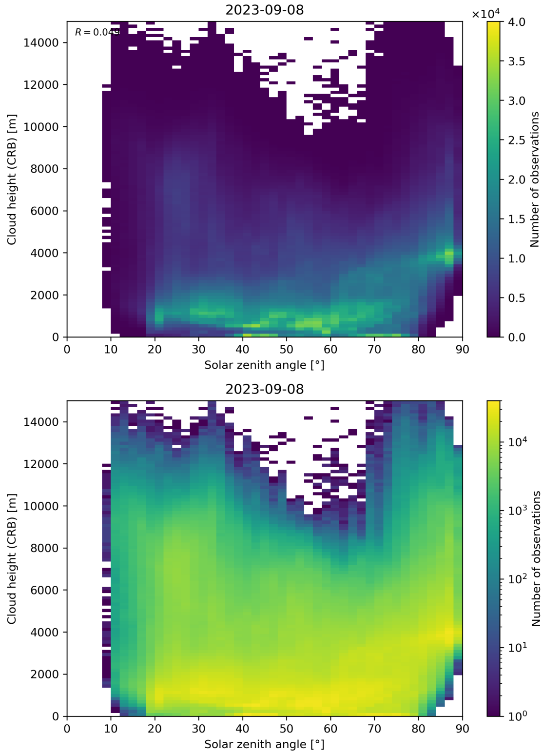
Figure 102: Scatter density plot of “Solar zenith angle” against “Cloud height (CRB)” for 2023-09-07 to 2023-09-09.
