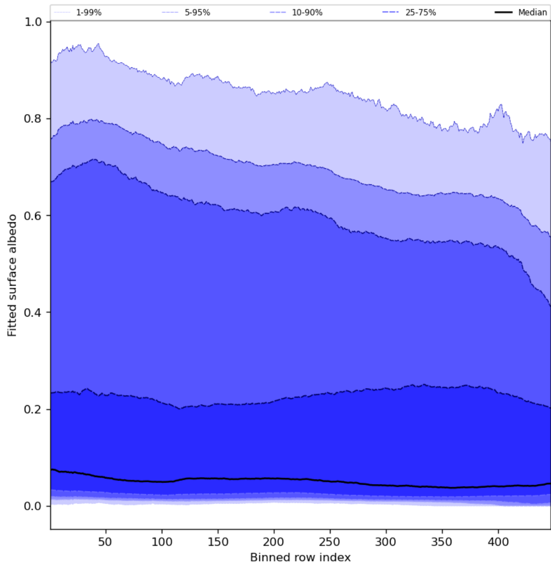
Figure 61: Along track statistics of “Fitted surface albedo” for 2023-09-07 to 2023-09-09
