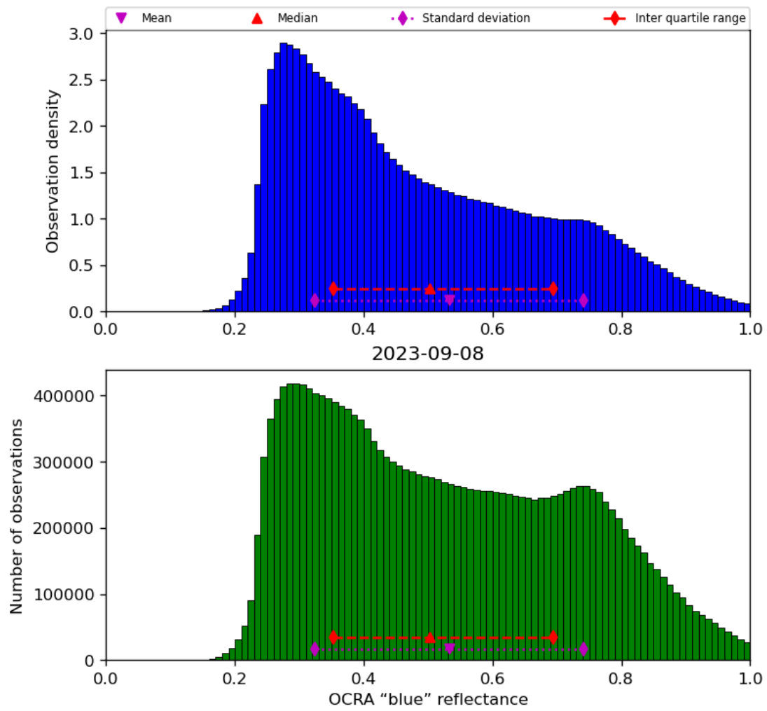
Figure 51: Histogram of “OCRA “blue” reflectance” for 2023-09-07 to 2023-09-09
