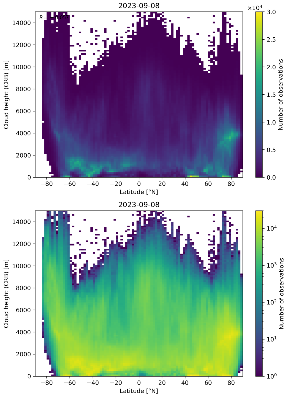
Figure 95: Scatter density plot of “Latitude” against “Cloud height (CRB)” for 2023-09-07 to 2023-09-09.
