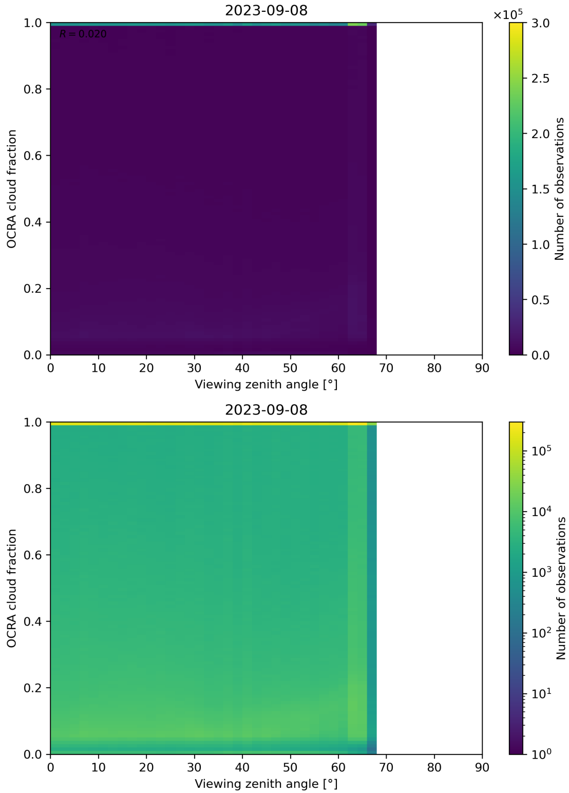
Figure 108: Scatter density plot of “Viewing zenith angle” against “OCRA cloud fraction” for 2023-09-07 to 2023-09-09.
