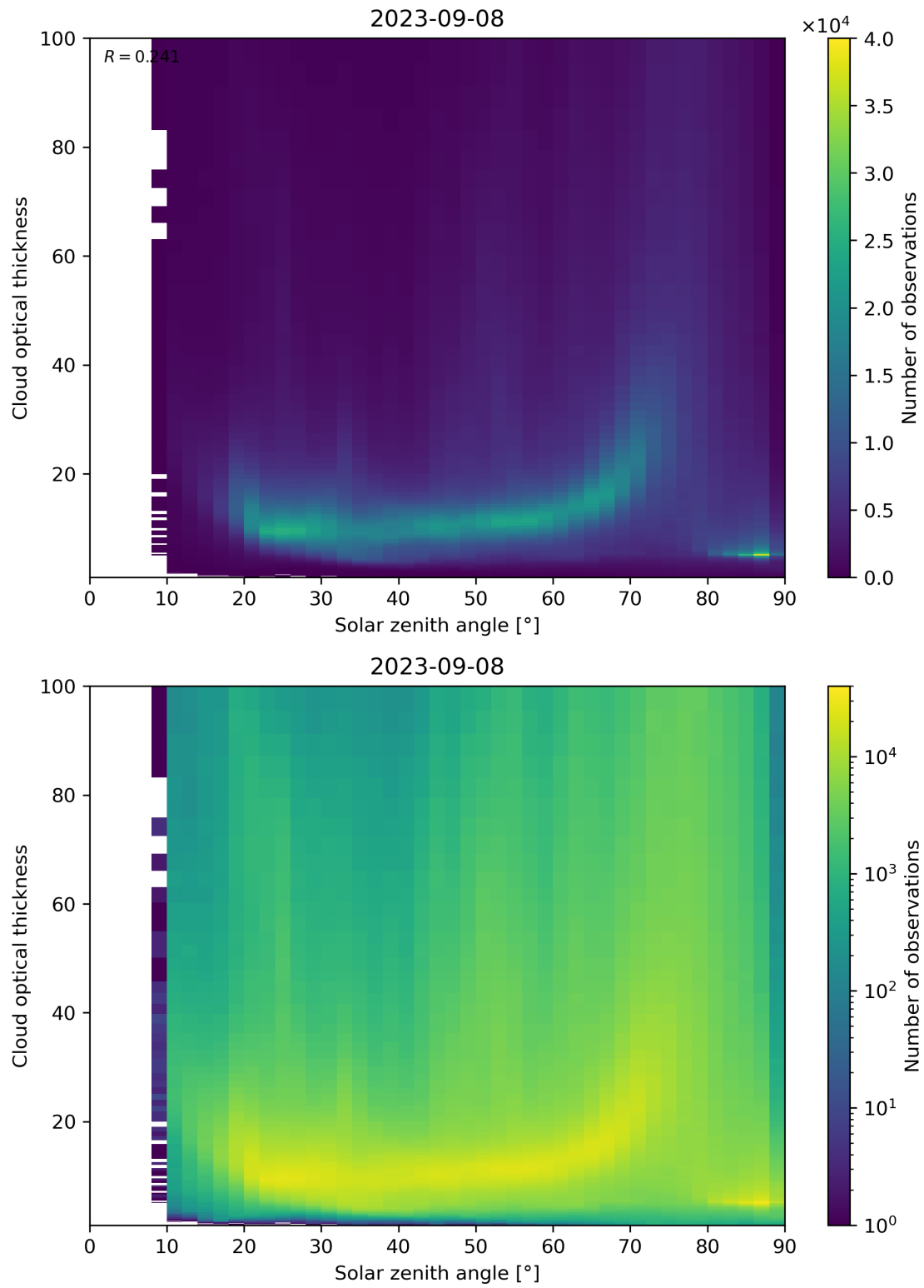
Figure 103: Scatter density plot of “Solar zenith angle” against “Cloud optical thickness” for 2023-09-07 to 2023-09-09.
