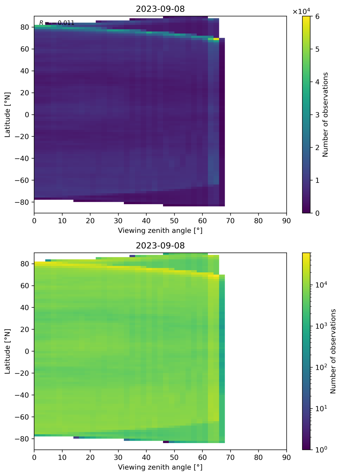
Figure 113: Scatter density plot of “Viewing zenith angle” against “Latitude” for 2023-09-07 to 2023-09-09.
