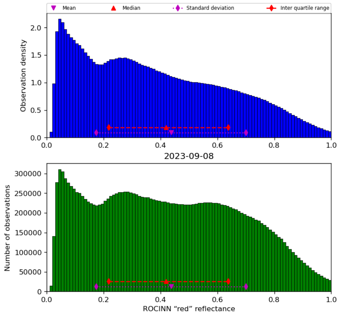
Figure 53: Histogram of “ROCINN “red” reflectance” for 2023-09-07 to 2023-09-09
