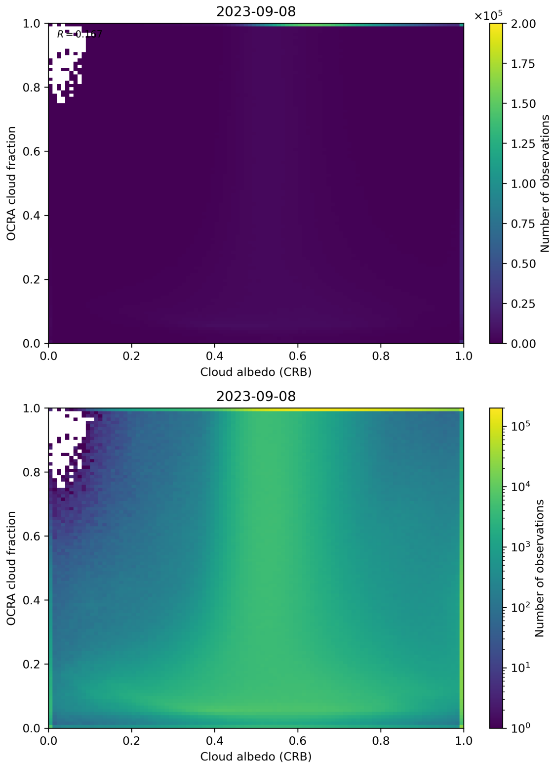
Figure 70: Scatter density plot of “Cloud albedo (CRB)” against “OCRA cloud fraction” for 2023-09-07 to 2023-09-09.
