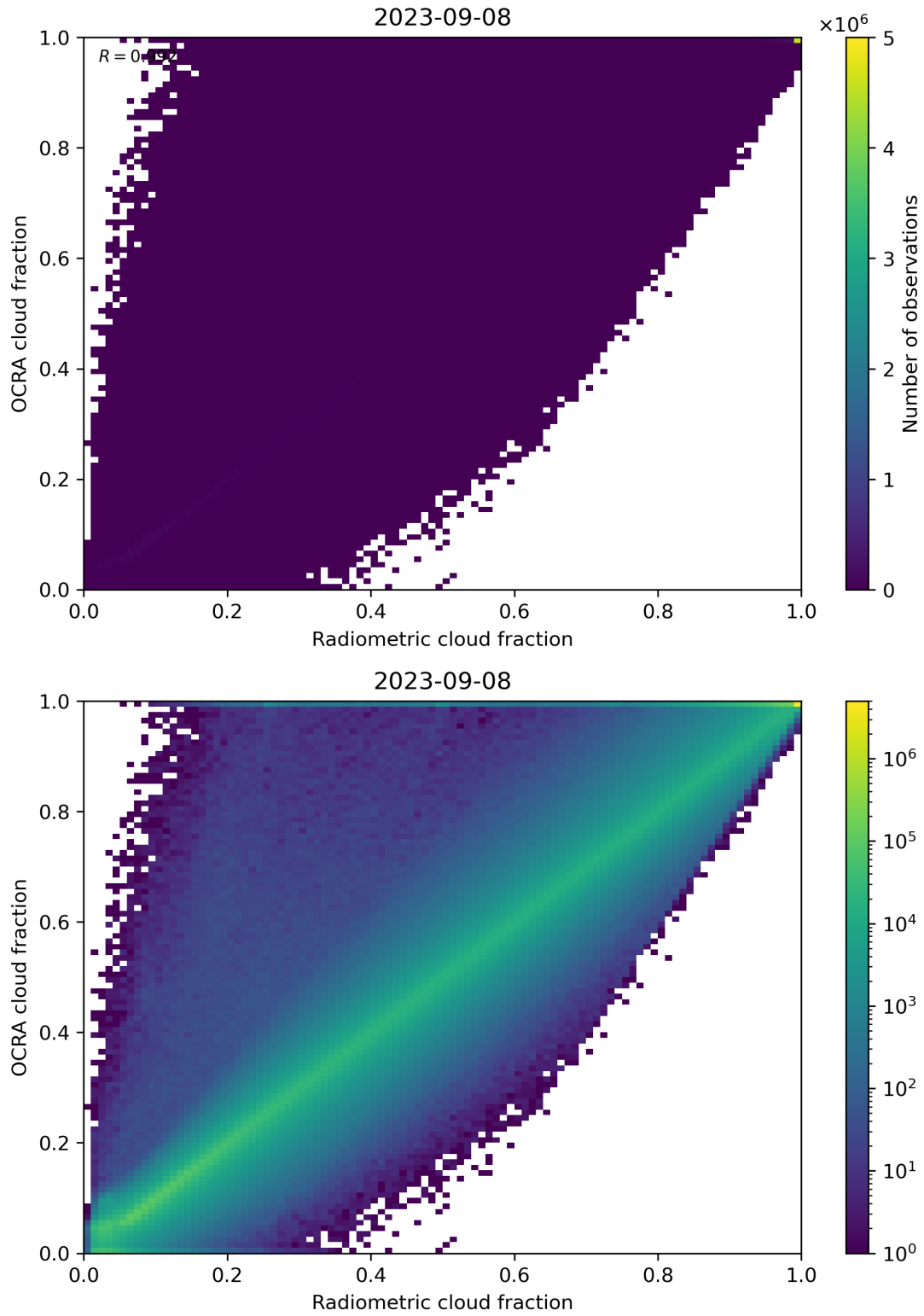
Figure 72: Scatter density plot of “Radiometric cloud fraction” against “OCRA cloud fraction” for 2023-09-07 to 2023-09-09.
