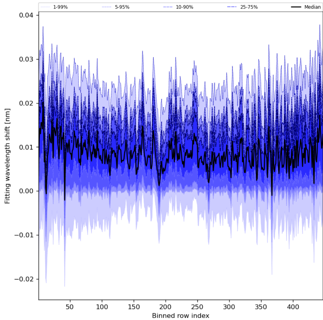
Figure 65: Along track statistics of “Fitting wavelength shift” for 2023-09-07 to 2023-09-09
