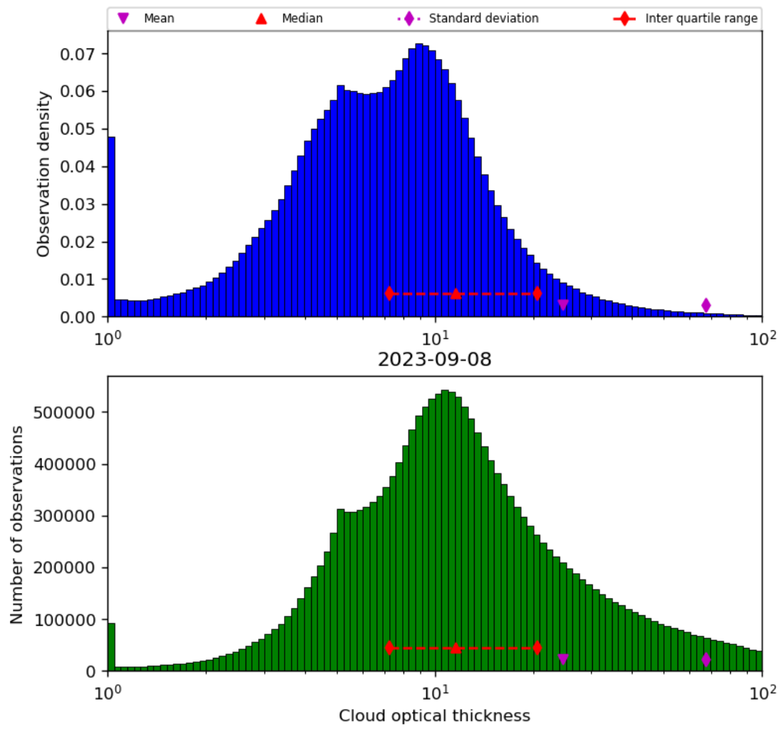
Figure 41: Histogram of “Cloud optical thickness” for 2023-09-07 to 2023-09-09
