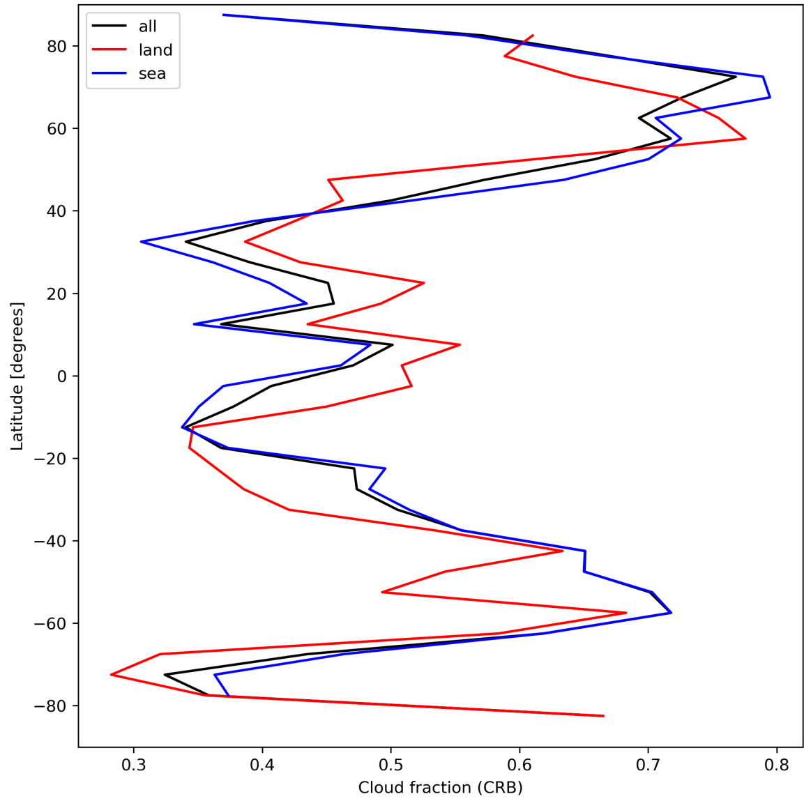
Figure 26: Zonal average of “Cloud fraction (CRB)” for 2023-09-07 to 2023-09-09.
