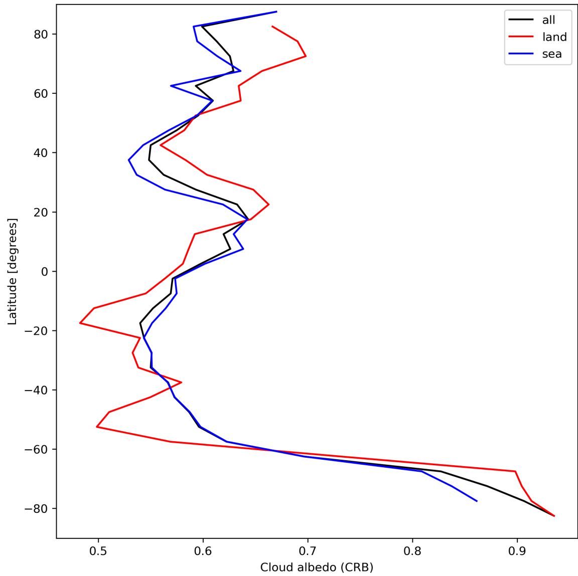
Figure 28: Zonal average of “Cloud albedo (CRB)” for 2023-09-07 to 2023-09-09.
