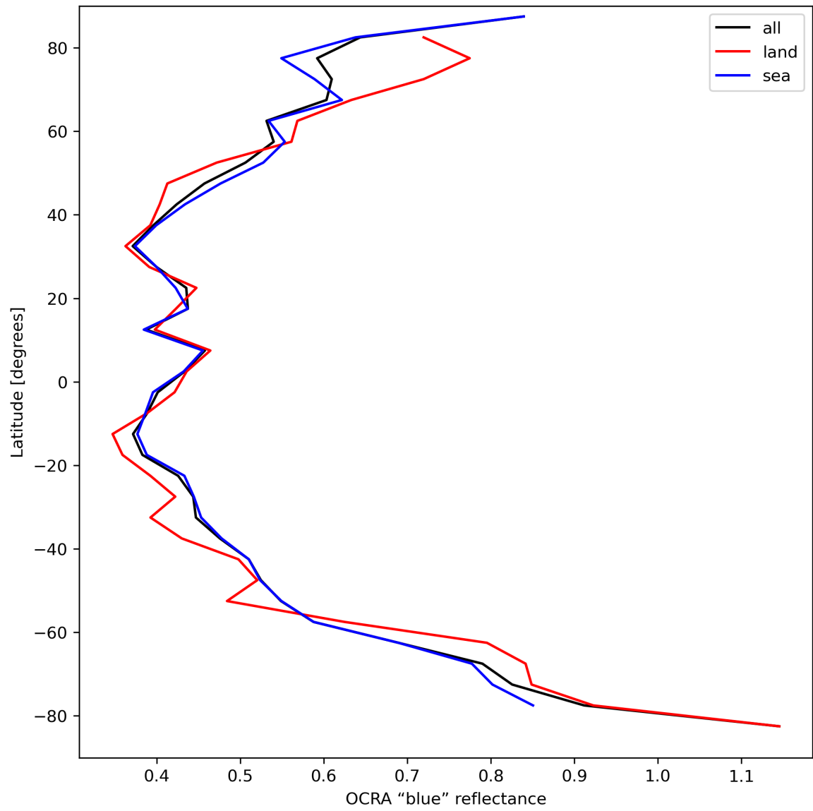
Figure 35: Zonal average of “OCRA “blue” reflectance” for 2023-09-07 to 2023-09-09.
