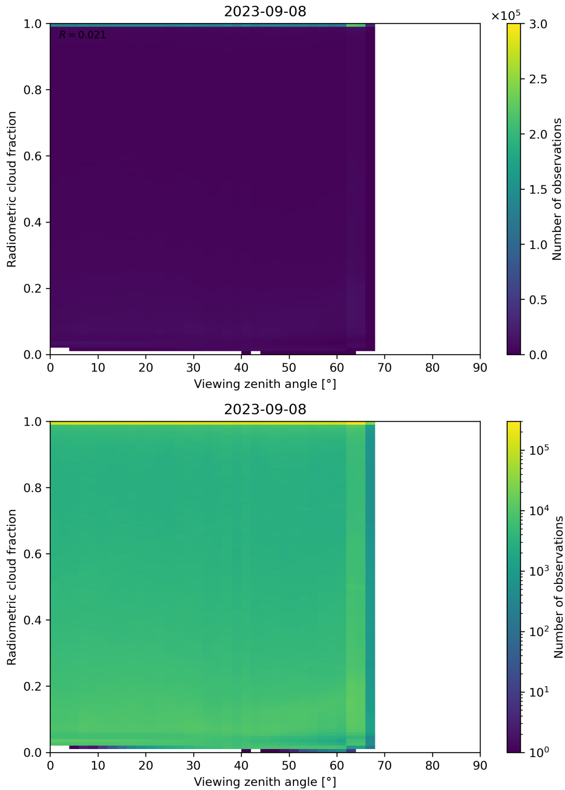
Figure 107: Scatter density plot of “Viewing zenith angle” against “Radiometric cloud fraction” for 2023-09-07 to 2023-09-09.
