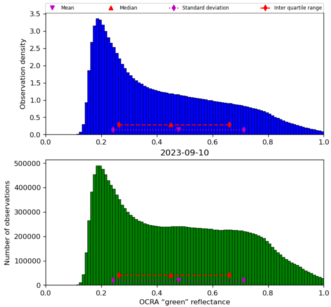
Figure 52: Histogram of “OCRA “green” reflectance” for 2023-09-10 to 2023-09-11
