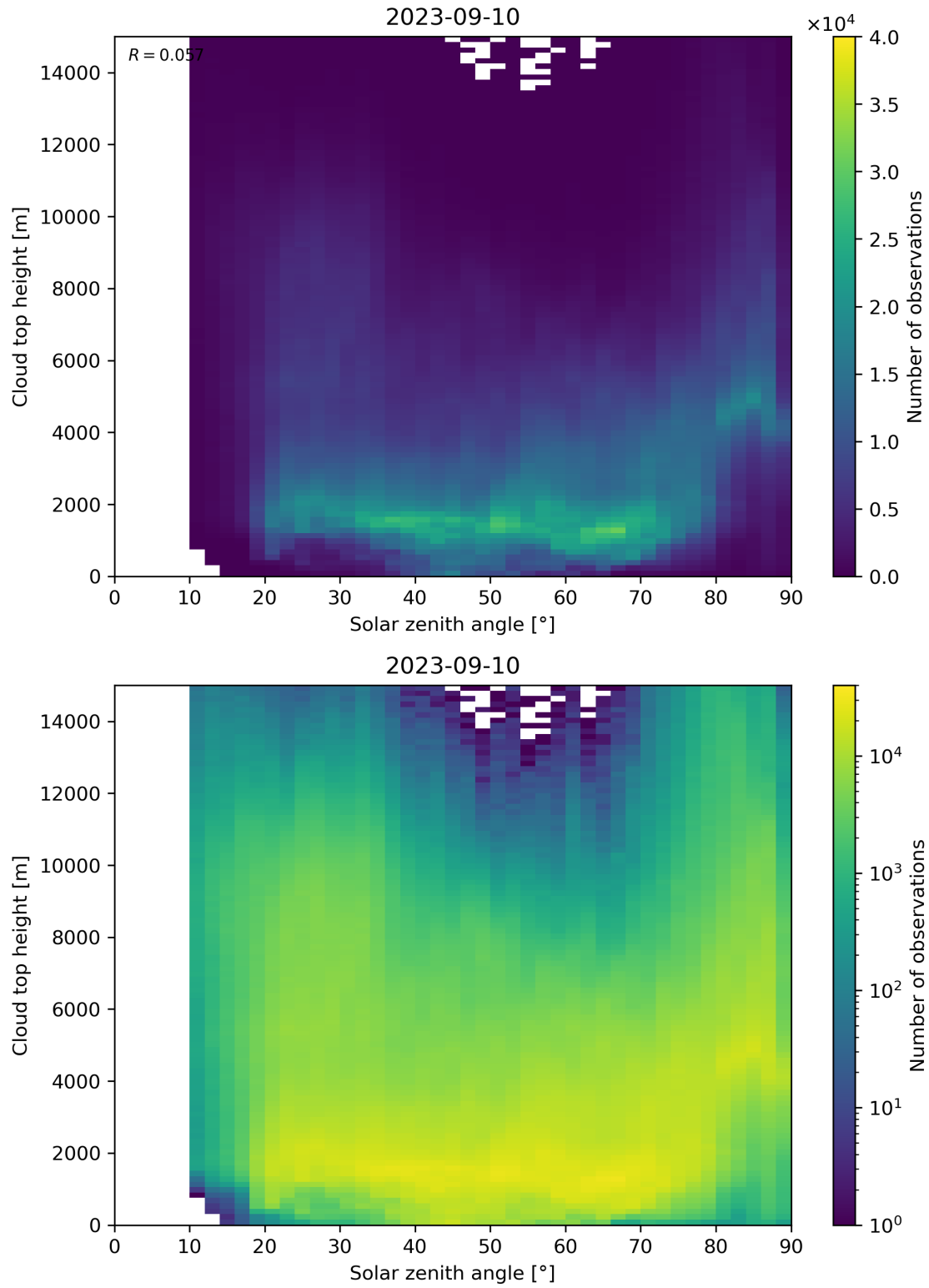
Figure 104: Scatter density plot of “Solar zenith angle” against “Cloud top height” for 2023-09-10 to 2023-09-11.
