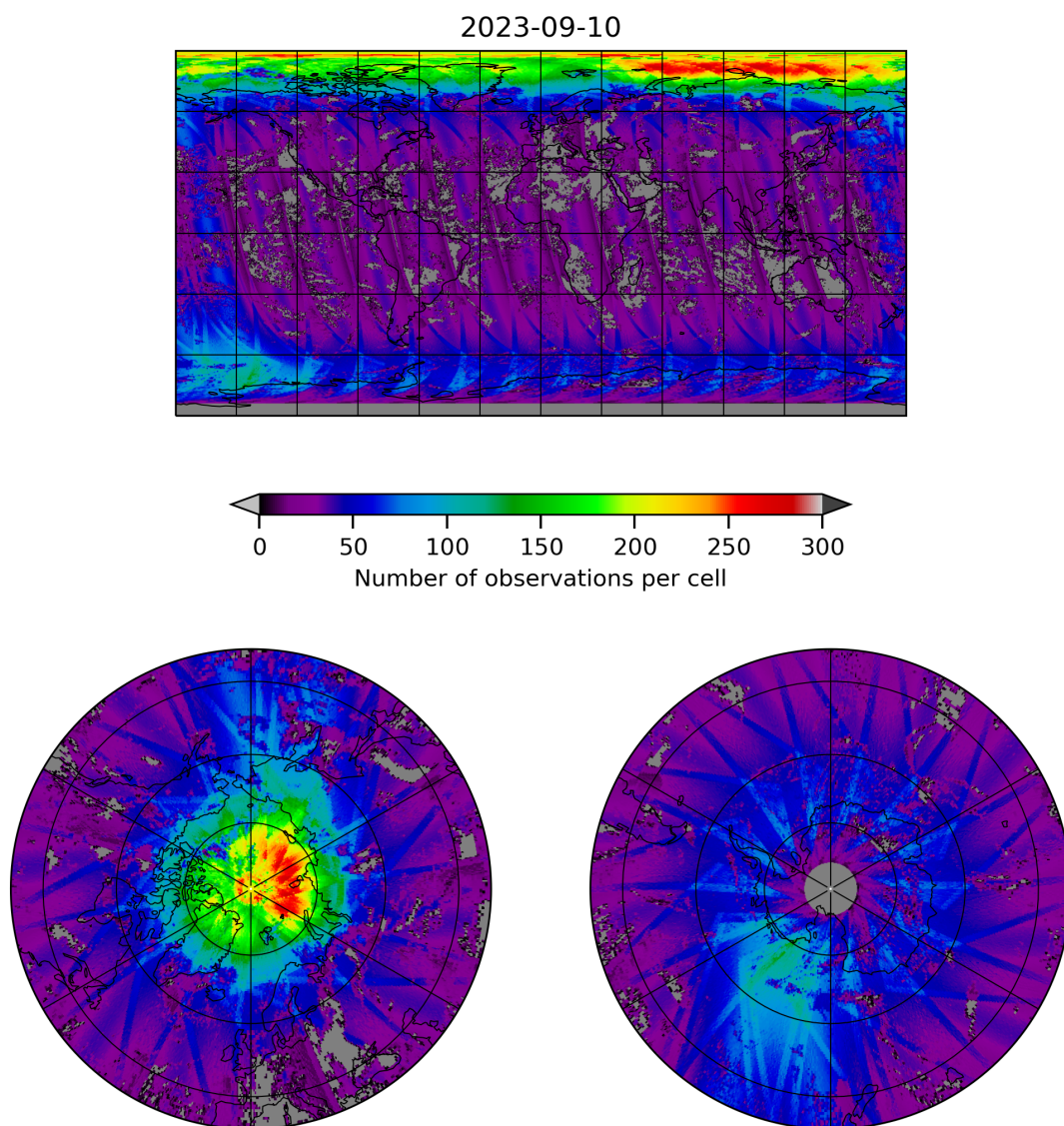
Figure 21: Map of the number of observations for 2023-09-10 to 2023-09-11
