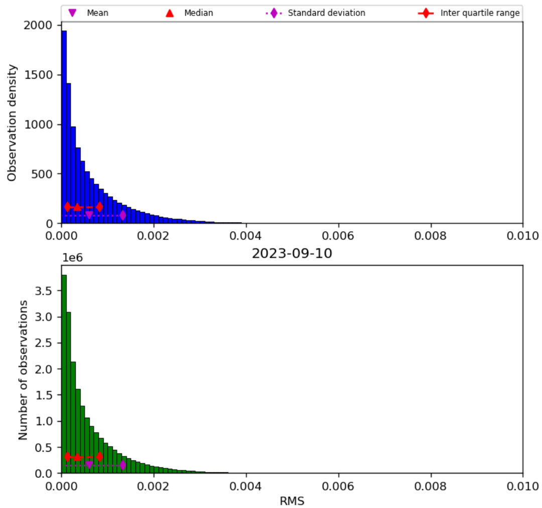
Figure 47: Histogram of “RMS” for 2023-09-10 to 2023-09-11
