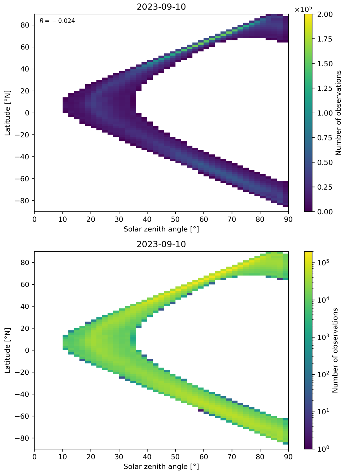
Figure 105: Scatter density plot of “Solar zenith angle” against “Latitude” for 2023-09-10 to 2023-09-11.
