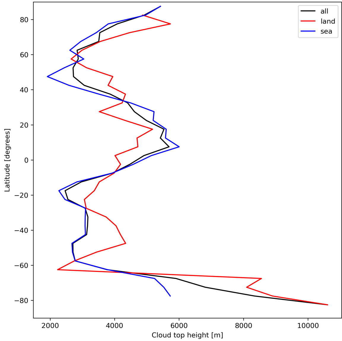
Figure 24: Zonal average of “Cloud top height” for 2023-09-10 to 2023-09-11.
