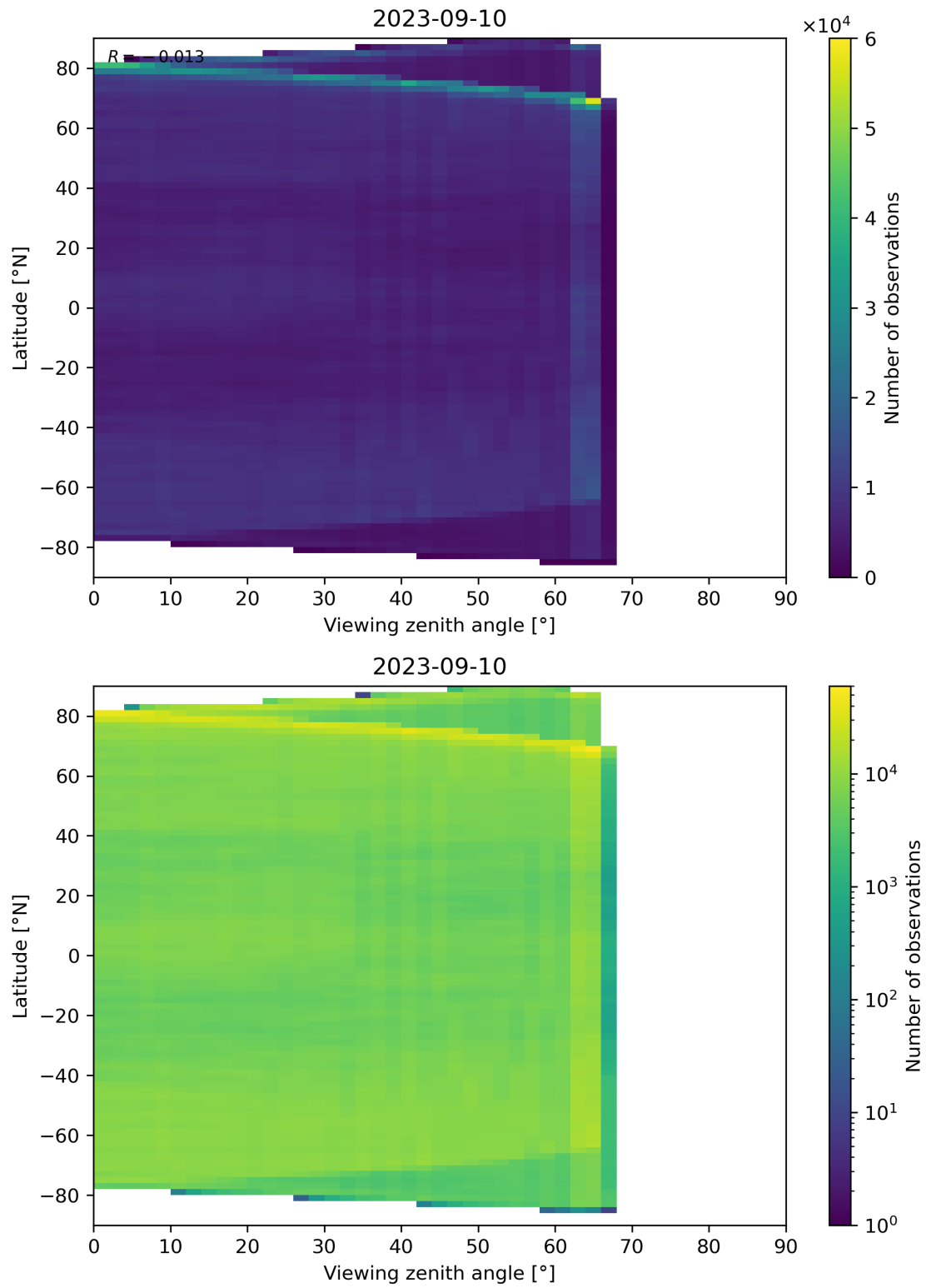
Figure 113: Scatter density plot of “Viewing zenith angle” against “Latitude” for 2023-09-10 to 2023-09-11.
