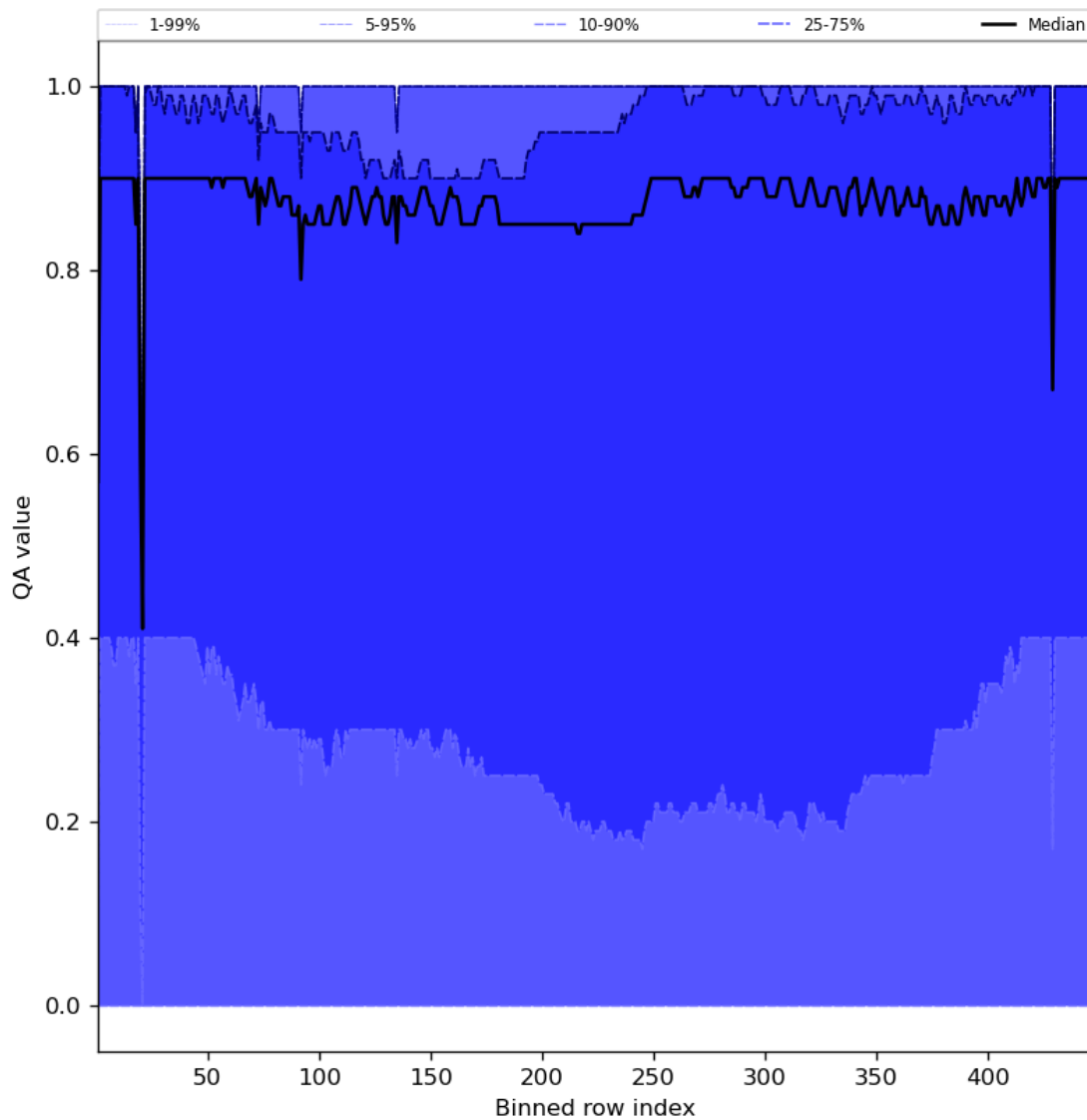
Figure 54: Along track statistics of “QA value” for 2023-09-10 to 2023-09-11
