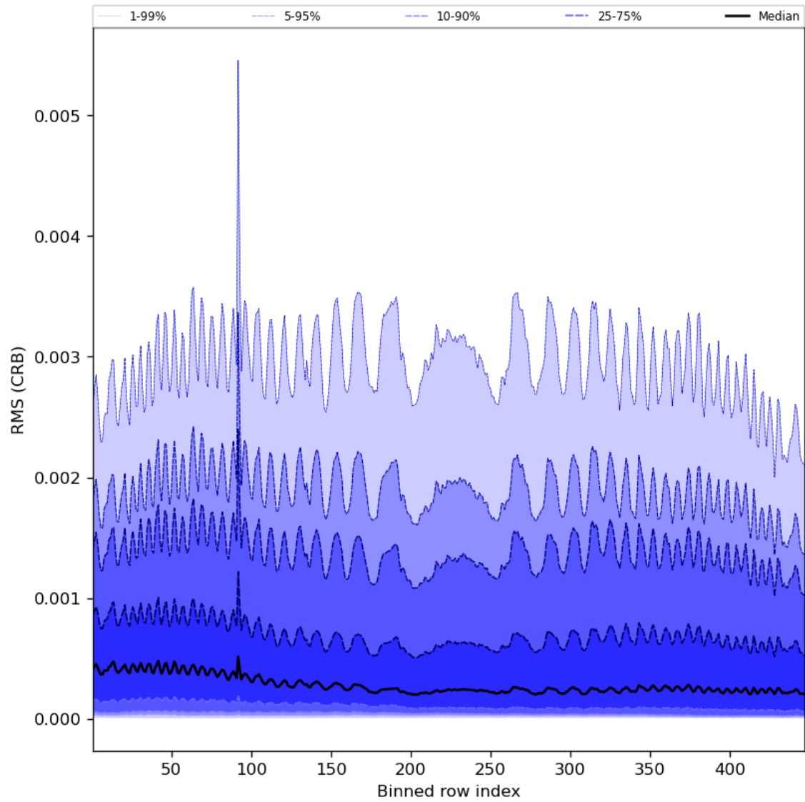
Figure 64: Along track statistics of “RMS (CRB)” for 2023-09-10 to 2023-09-11
