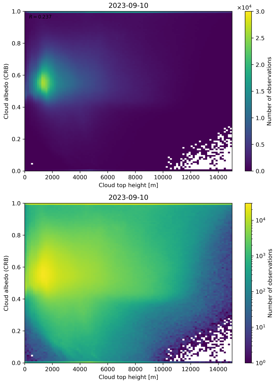
Figure 86: Scatter density plot of “Cloud top height” against “Cloud albedo (CRB)” for 2023-09-10 to 2023-09-11.
