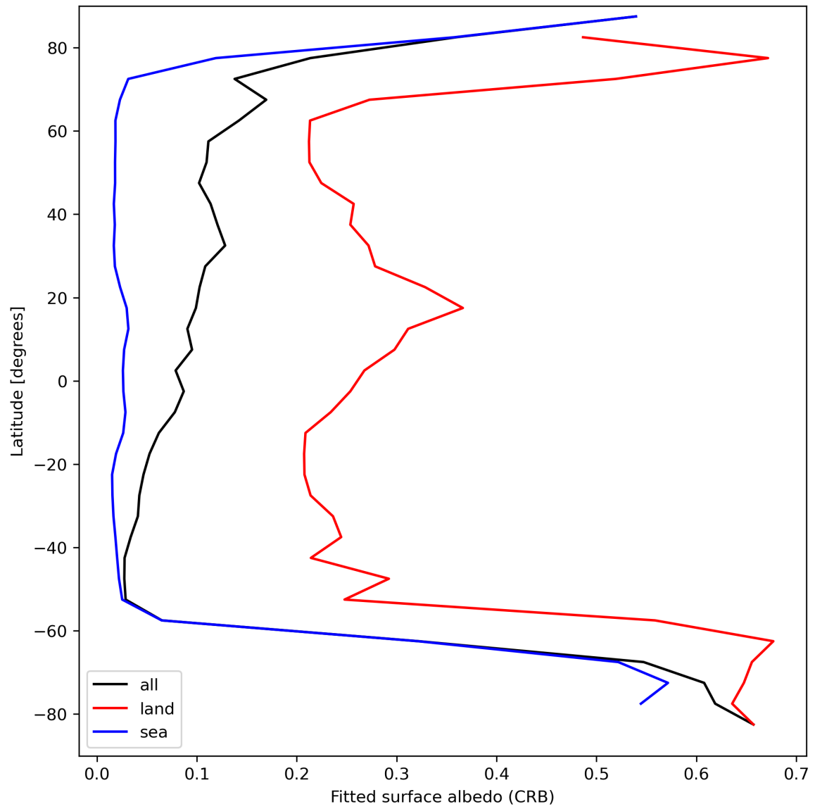
Figure 30: Zonal average of “Fitted surface albedo (CRB)” for 2023-09-10 to 2023-09-11.
