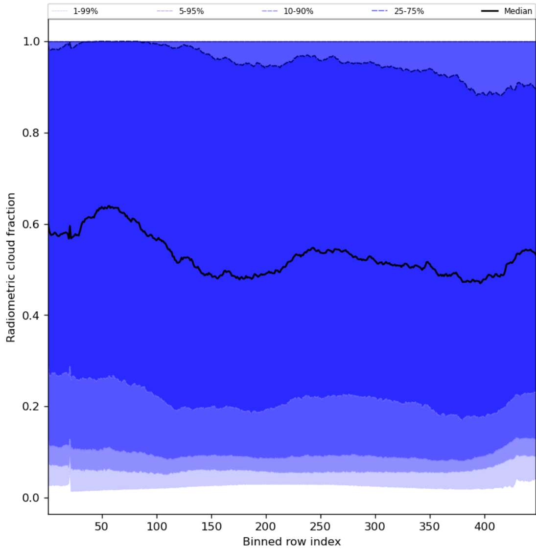
Figure 55: Along track statistics of “Radiometric cloud fraction” for 2023-09-10 to 2023-09-11
