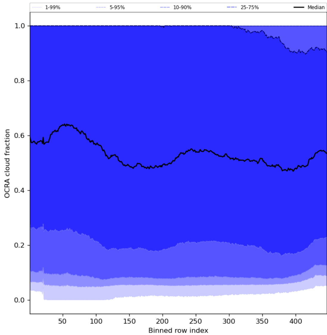
Figure 66: Along track statistics of “OCRA cloud fraction” for 2023-09-10 to 2023-09-11
