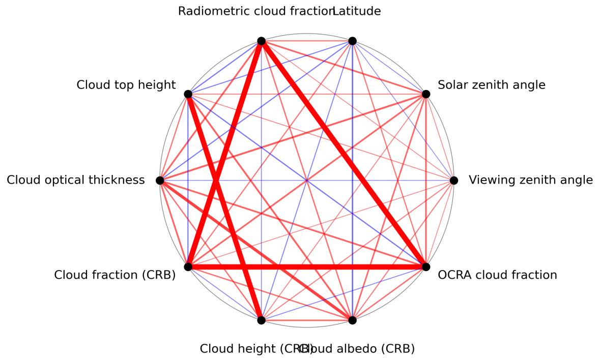
Figure 1: Map of correlation graph for 2023-09-10 to 2023-09-11.
