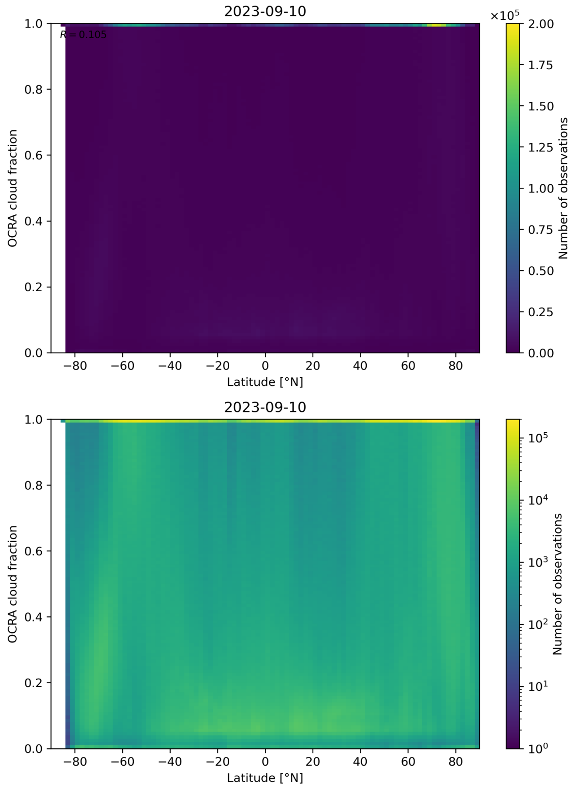
Figure 93: Scatter density plot of “Latitude” against “OCRA cloud fraction” for 2023-09-10 to 2023-09-11.
