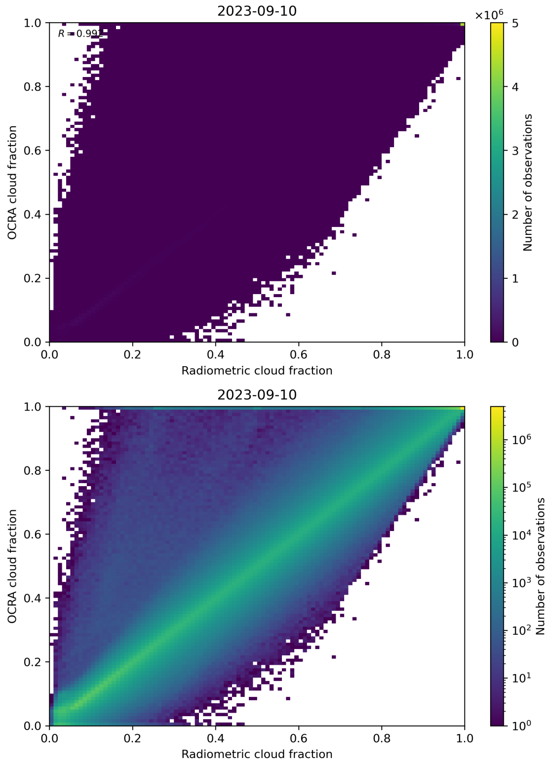
Figure 72: Scatter density plot of “Radiometric cloud fraction” against “OCRA cloud fraction” for 2023-09-10 to 2023-09-11.
