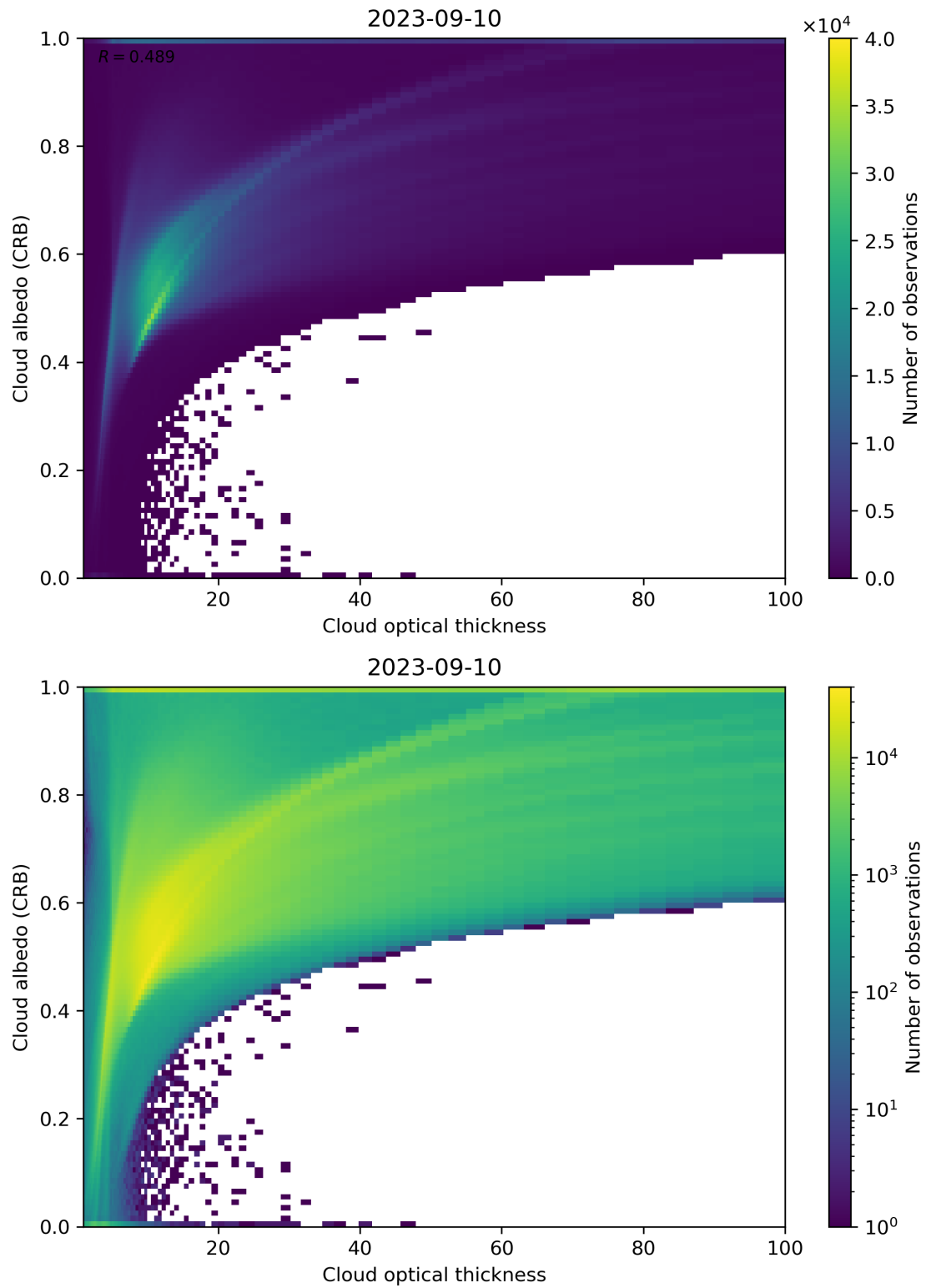
Figure 82: Scatter density plot of “Cloud optical thickness” against “Cloud albedo (CRB)” for 2023-09-10 to 2023-09-11.
