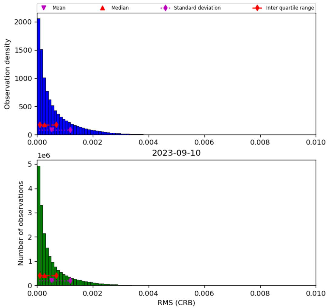
Figure 48: Histogram of “RMS (CRB)” for 2023-09-10 to 2023-09-11
