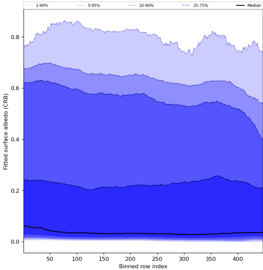
Figure 62: Along track statistics of “Fitted surface albedo (CRB)” for 2023-09-10 to 2023-09-11
