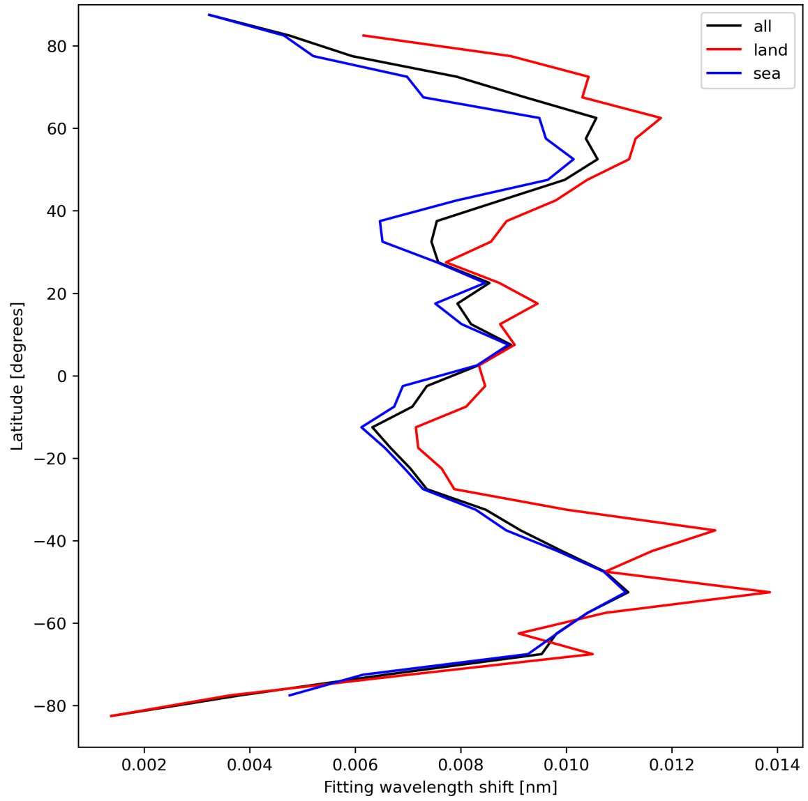
Figure 33: Zonal average of “Fitting wavelength shift” for 2023-09-10 to 2023-09-11.
