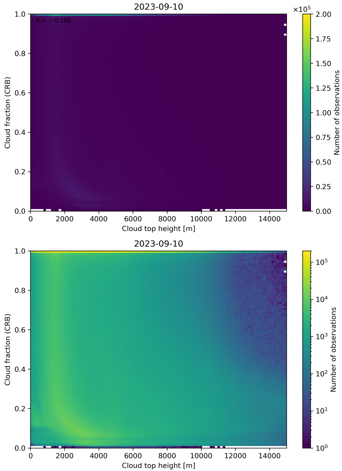
Figure 88: Scatter density plot of “Cloud top height” against “Cloud fraction (CRB)” for 2023-09-10 to 2023-09-11.
