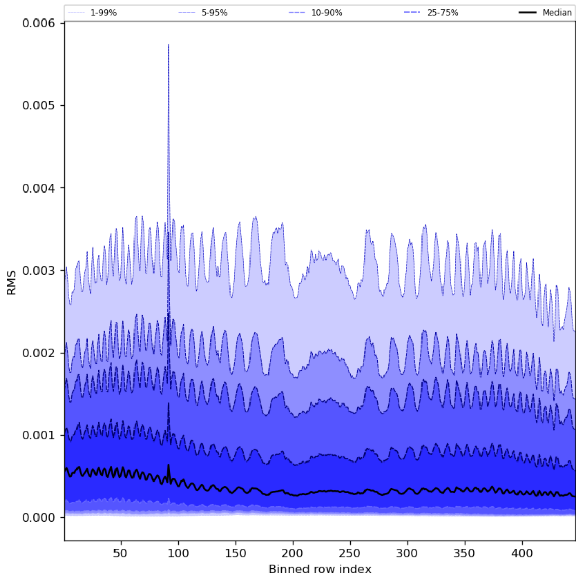
Figure 63: Along track statistics of “RMS” for 2023-09-10 to 2023-09-11
