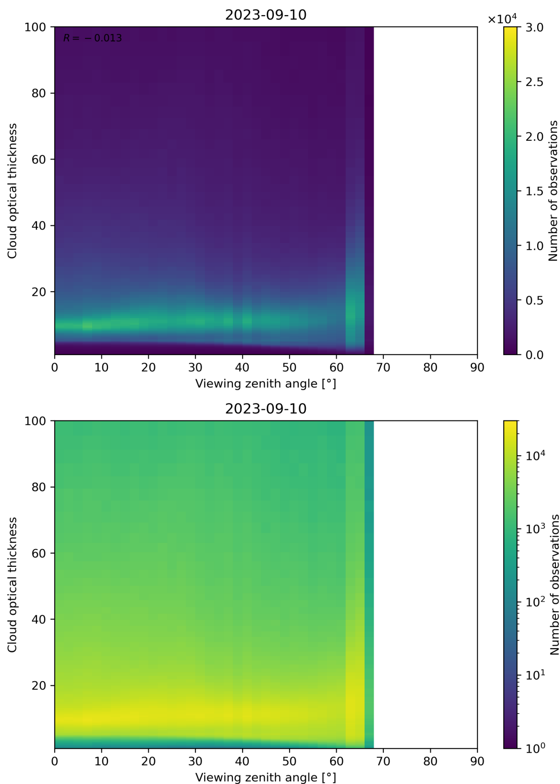
Figure 111: Scatter density plot of “Viewing zenith angle” against “Cloud optical thickness” for 2023-09-10 to 2023-09-11.
