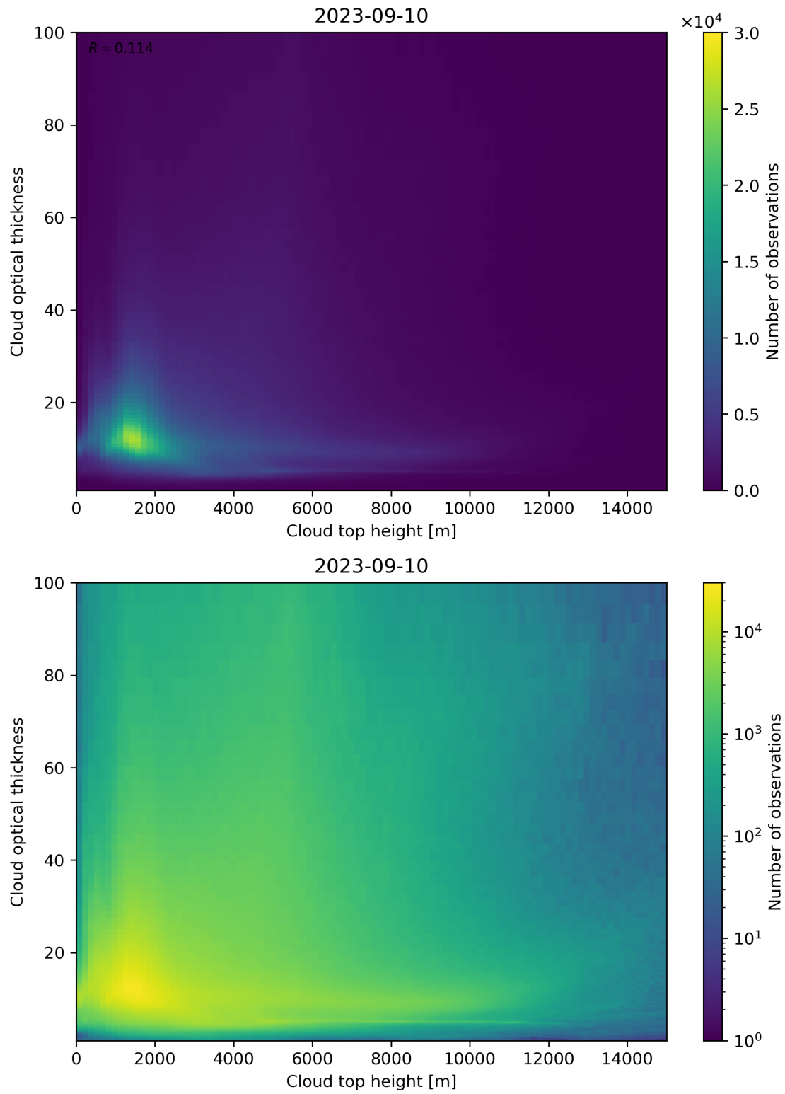
Figure 90: Scatter density plot of “Cloud top height” against “Cloud optical thickness” for 2023-09-10 to 2023-09-11.
