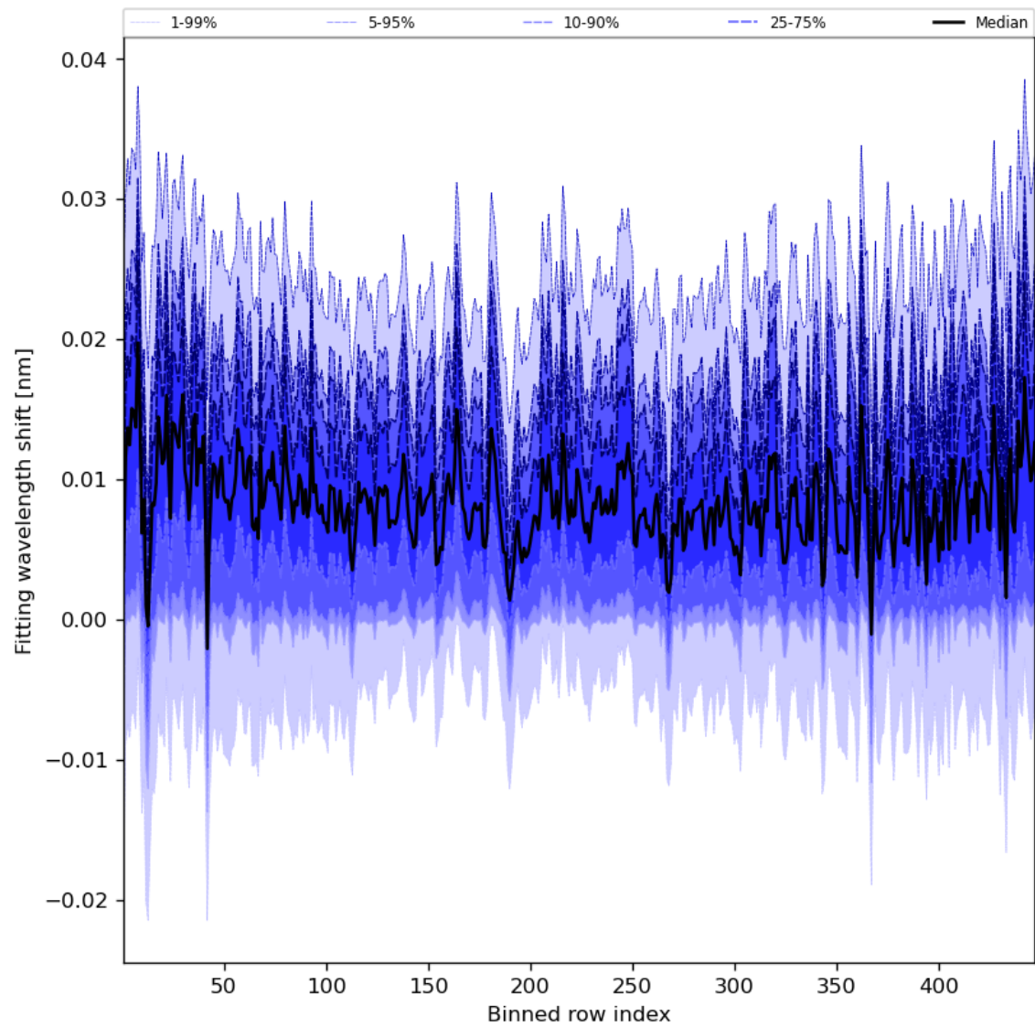
Figure 65: Along track statistics of “Fitting wavelength shift” for 2023-09-10 to 2023-09-11
