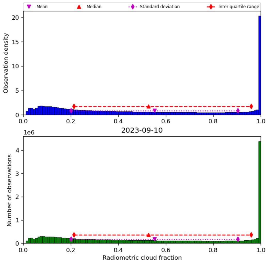
Figure 39: Histogram of “Radiometric cloud fraction” for 2023-09-10 to 2023-09-11
