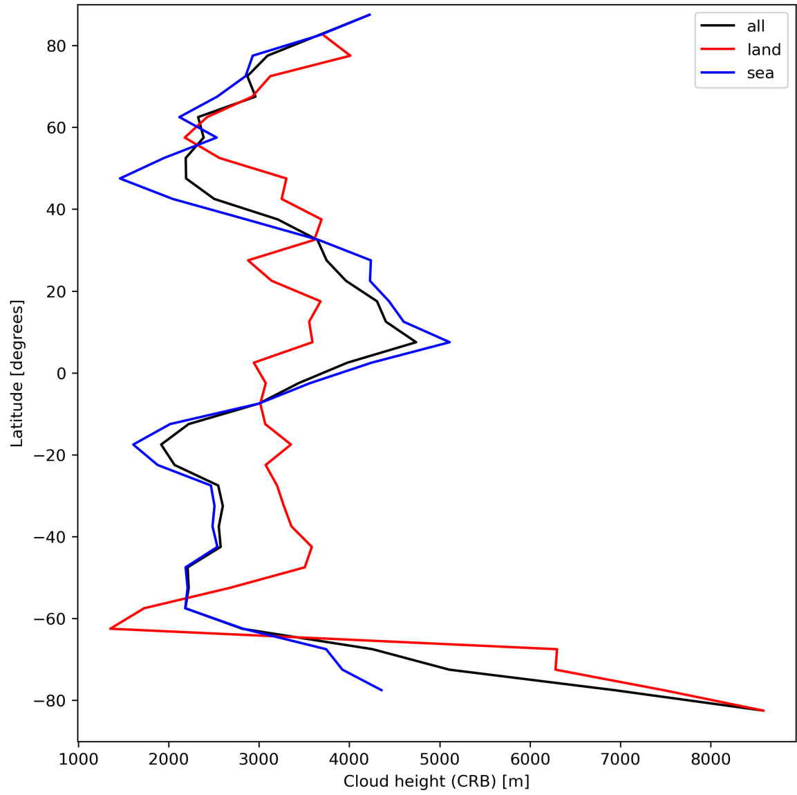
Figure 27: Zonal average of “Cloud height (CRB)” for 2023-09-10 to 2023-09-11.
