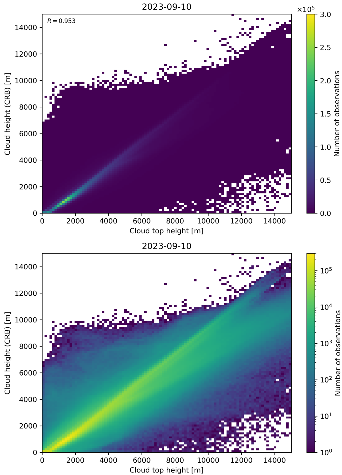
Figure 89: Scatter density plot of “Cloud top height” against “Cloud height (CRB)” for 2023-09-10 to 2023-09-11.
