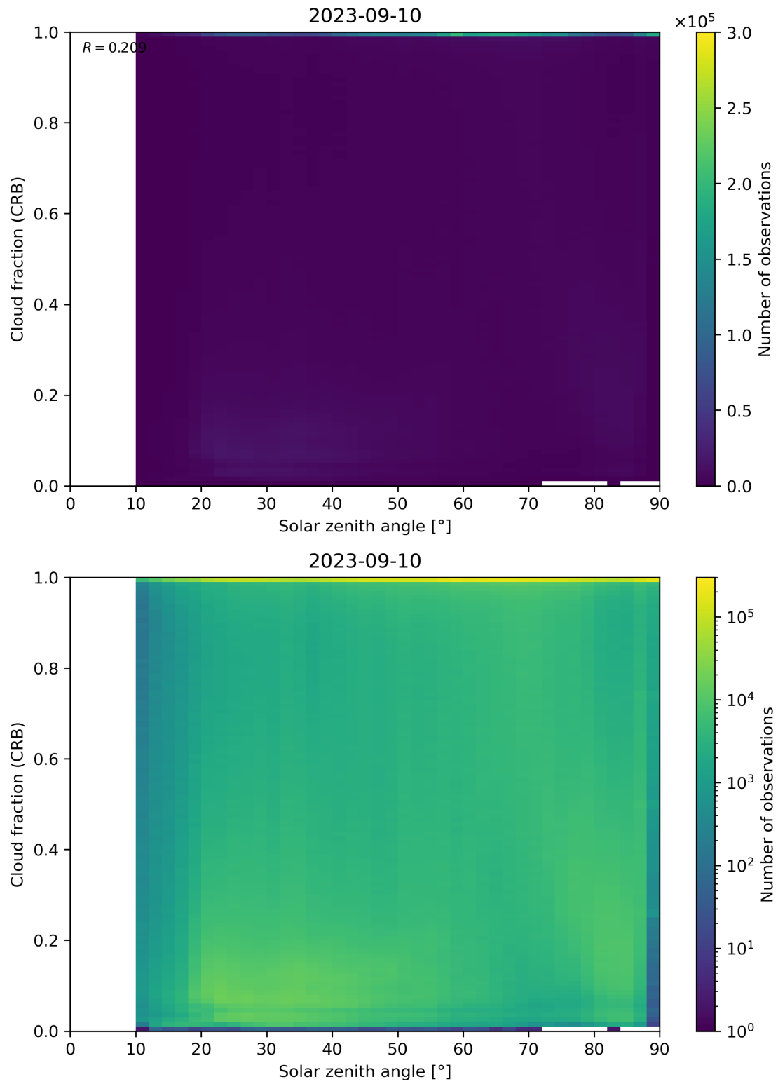
Figure 101: Scatter density plot of “Solar zenith angle” against “Cloud fraction (CRB)” for 2023-09-10 to 2023-09-11.
