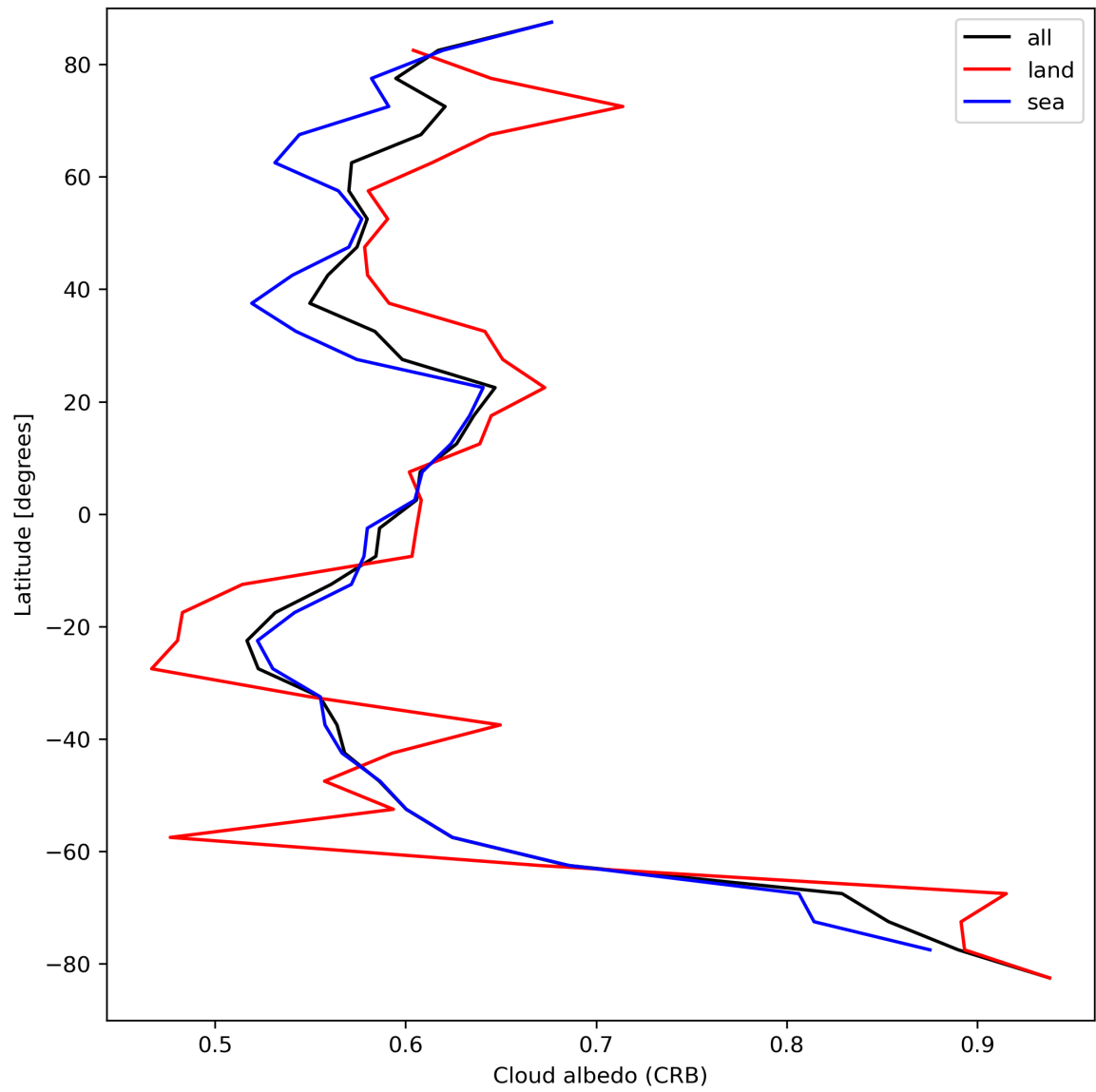
Figure 28: Zonal average of “Cloud albedo (CRB)” for 2023-09-10 to 2023-09-11.
