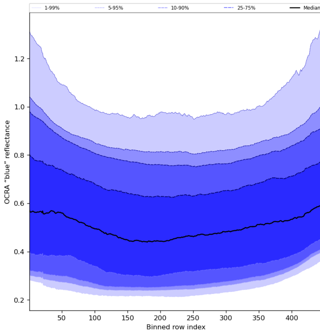
Figure 67: Along track statistics of “OCRA “blue” reflectance” for 2023-09-10 to 2023-09-11
