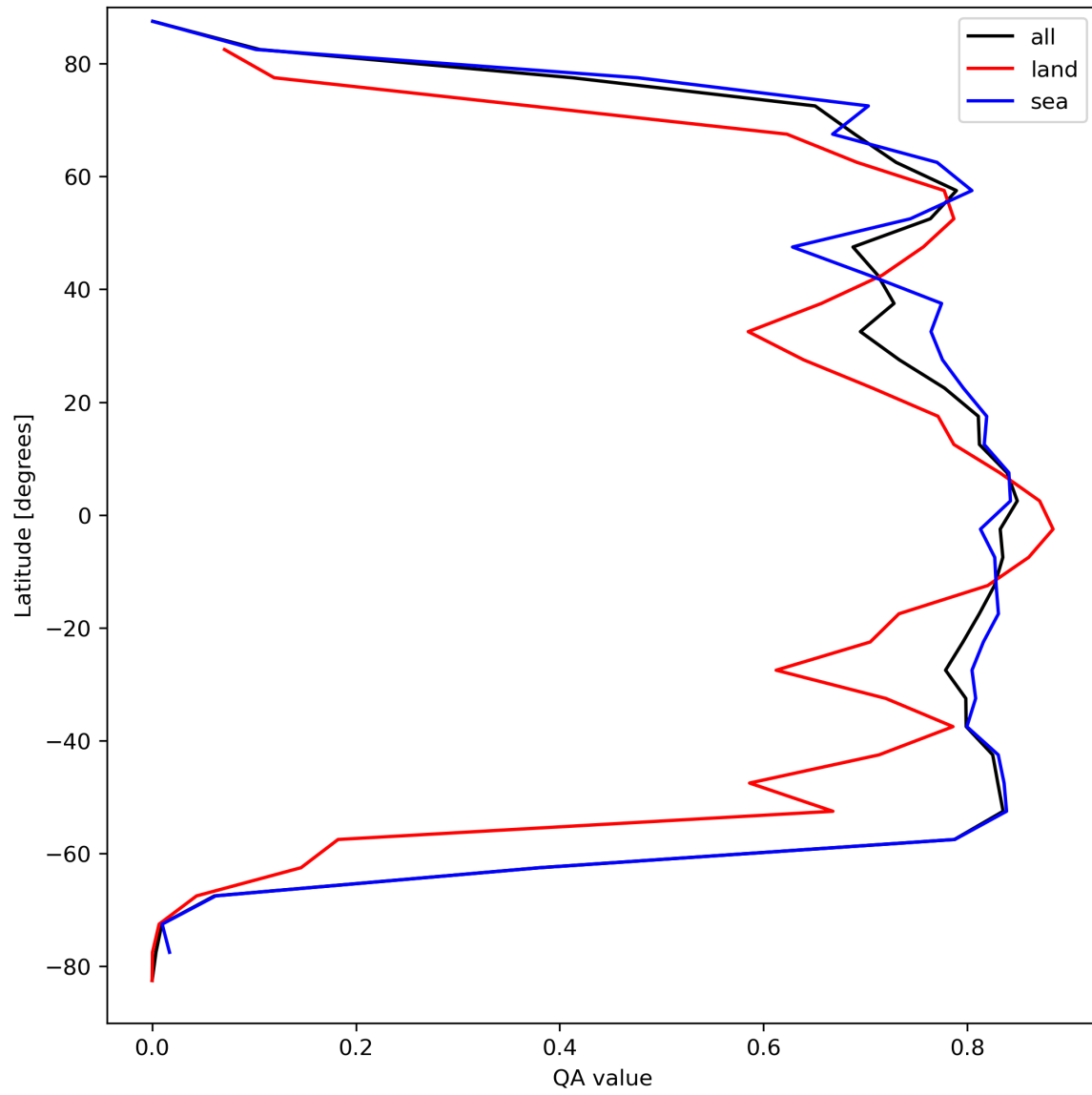
Figure 22: Zonal average of “QA value” for 2023-09-10 to 2023-09-11.
