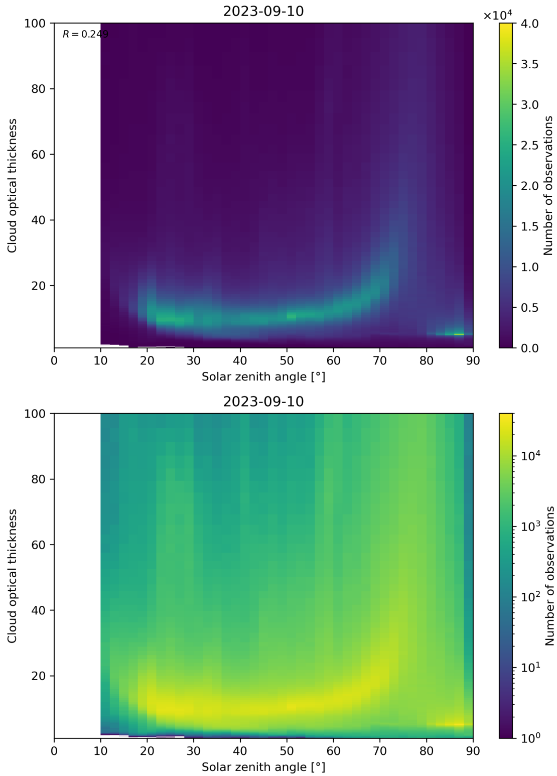
Figure 103: Scatter density plot of “Solar zenith angle” against “Cloud optical thickness” for 2023-09-10 to 2023-09-11.
