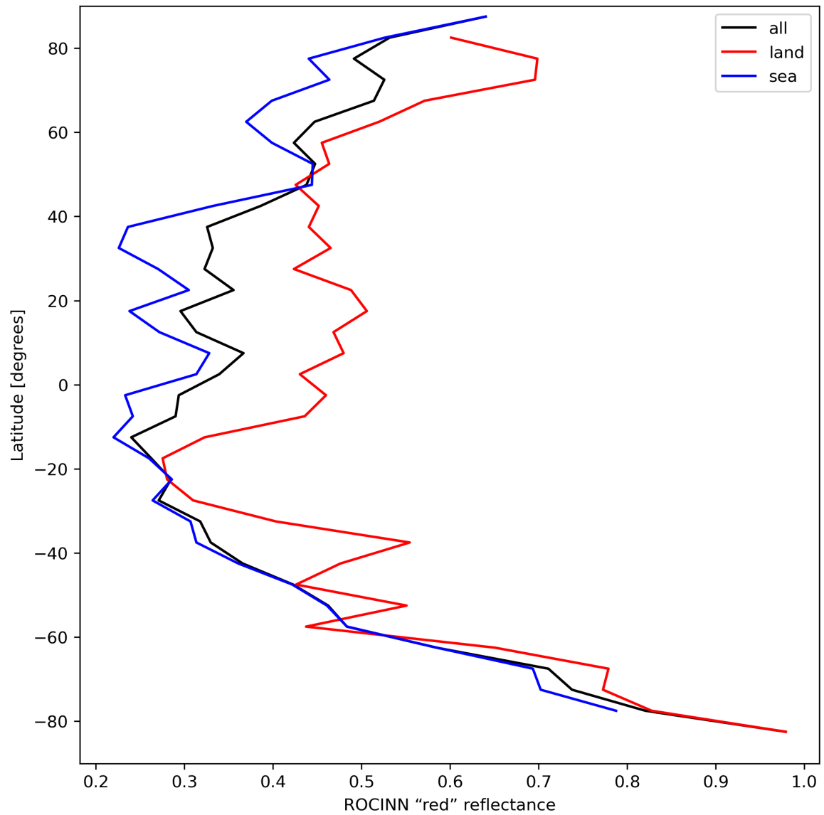
Figure 37: Zonal average of “ROCINN “red” reflectance” for 2023-09-10 to 2023-09-11.
