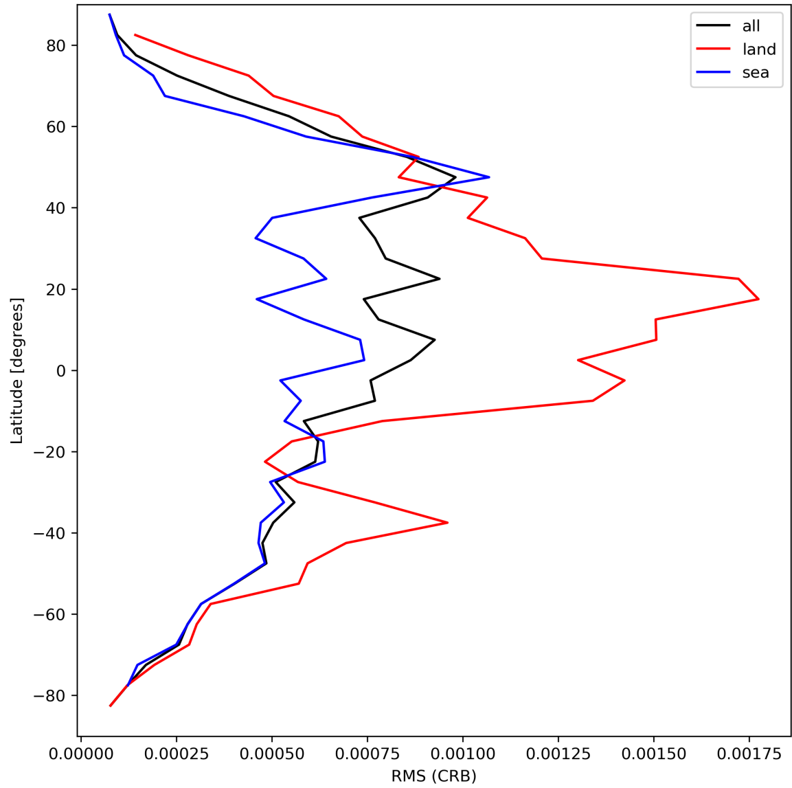
Figure 32: Zonal average of “RMS (CRB)” for 2023-09-10 to 2023-09-11.
