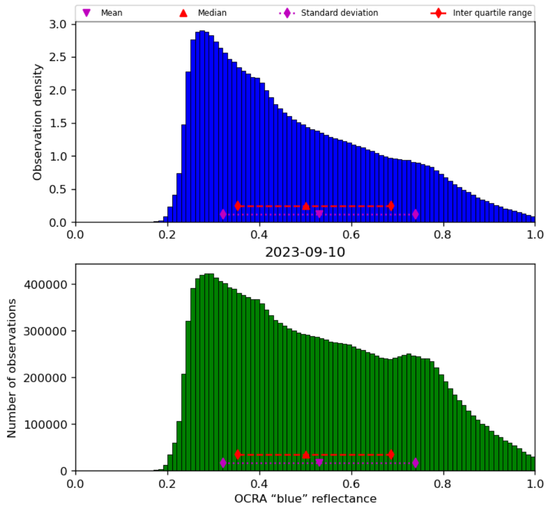
Figure 51: Histogram of “OCRA “blue” reflectance” for 2023-09-10 to 2023-09-11
