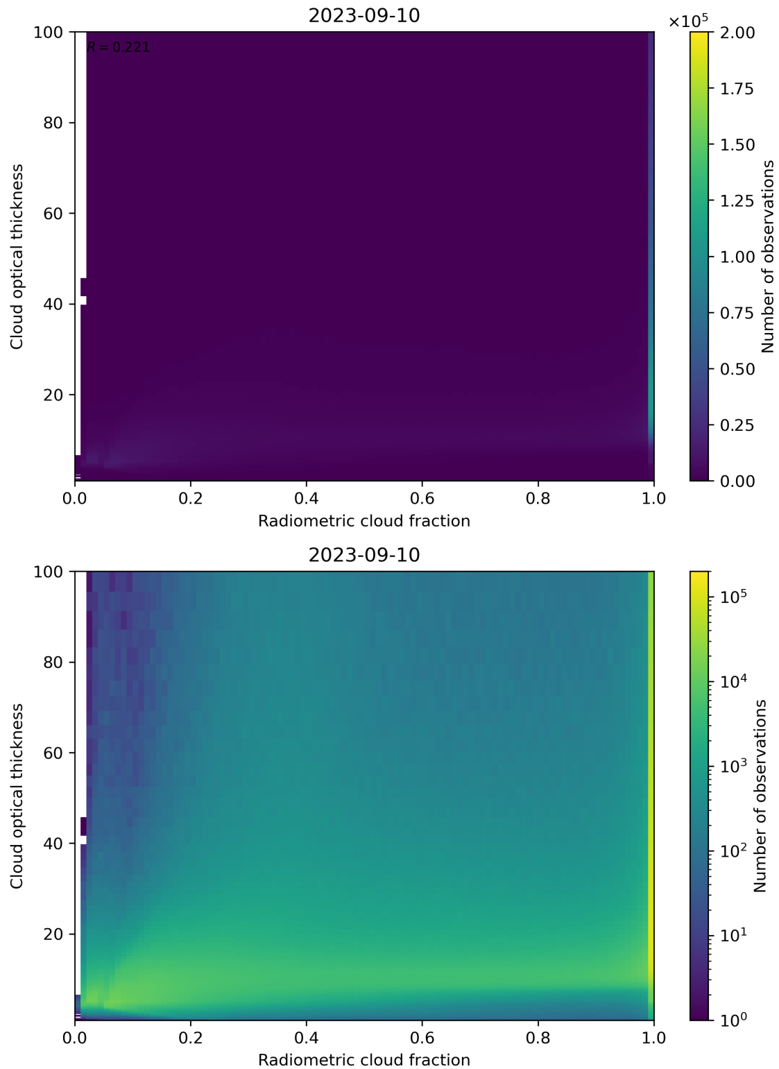
Figure 75: Scatter density plot of “Radiometric cloud fraction” against “Cloud optical thickness” for 2023-09-10 to 2023-09-11.
