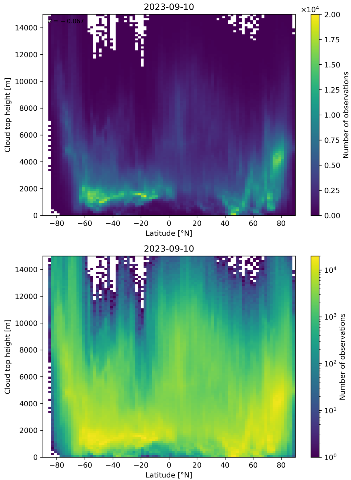
Figure 97: Scatter density plot of “Latitude” against “Cloud top height” for 2023-09-10 to 2023-09-11.
