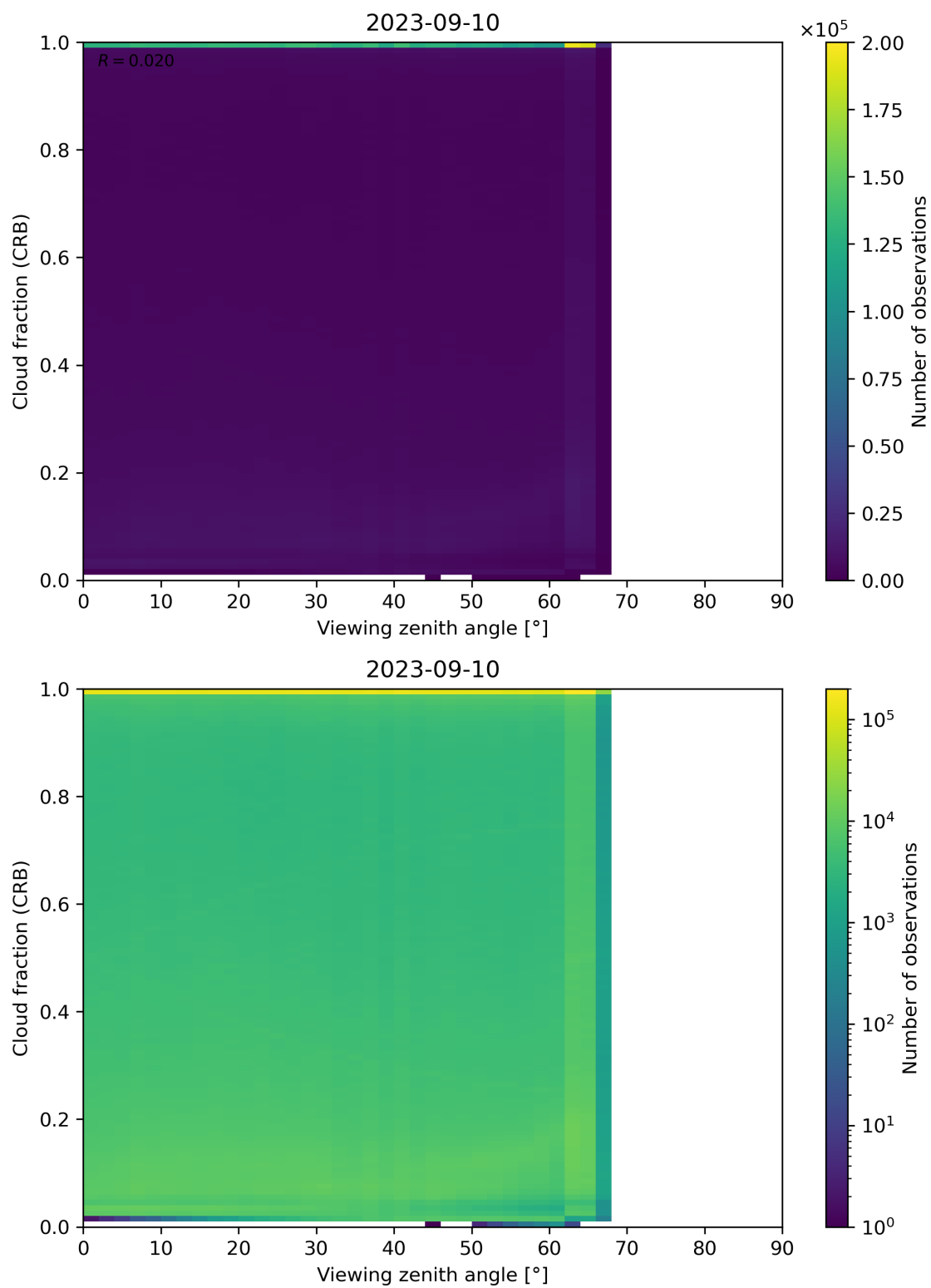
Figure 109: Scatter density plot of “Viewing zenith angle” against “Cloud fraction (CRB)” for 2023-09-10 to 2023-09-11.
