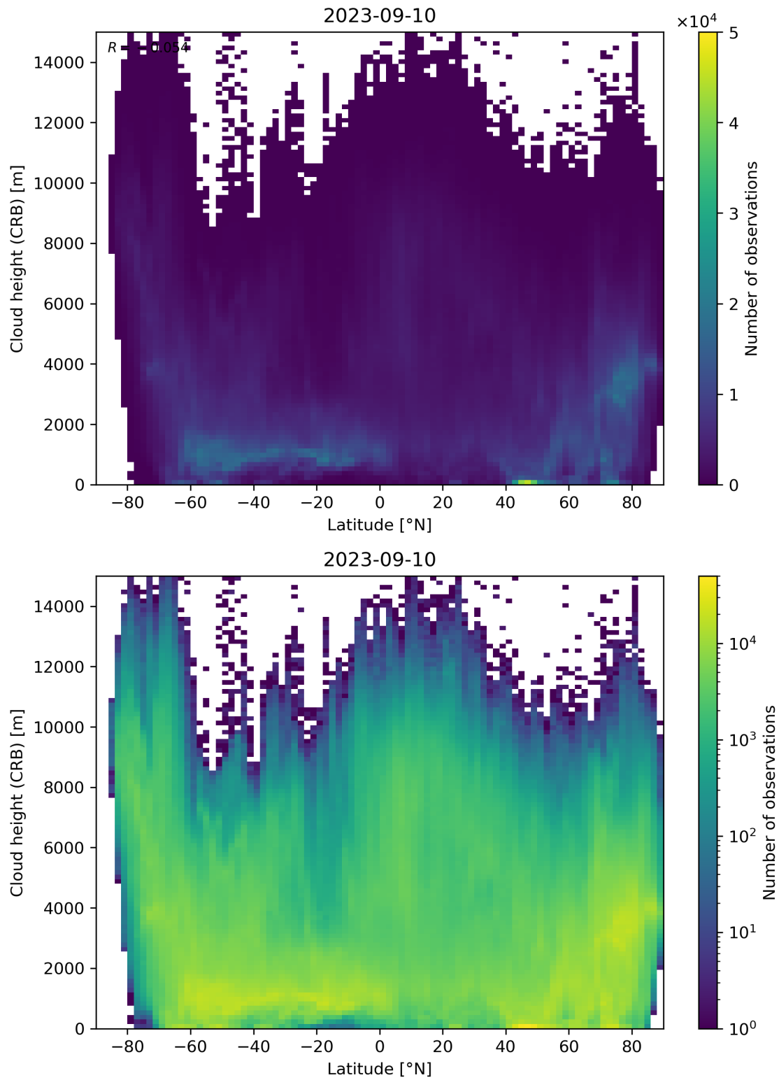
Figure 95: Scatter density plot of “Latitude” against “Cloud height (CRB)” for 2023-09-10 to 2023-09-11.
