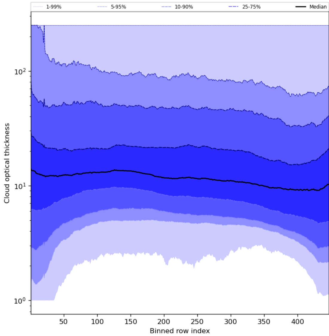
Figure 57: Along track statistics of “Cloud optical thickness” for 2023-09-10 to 2023-09-11
