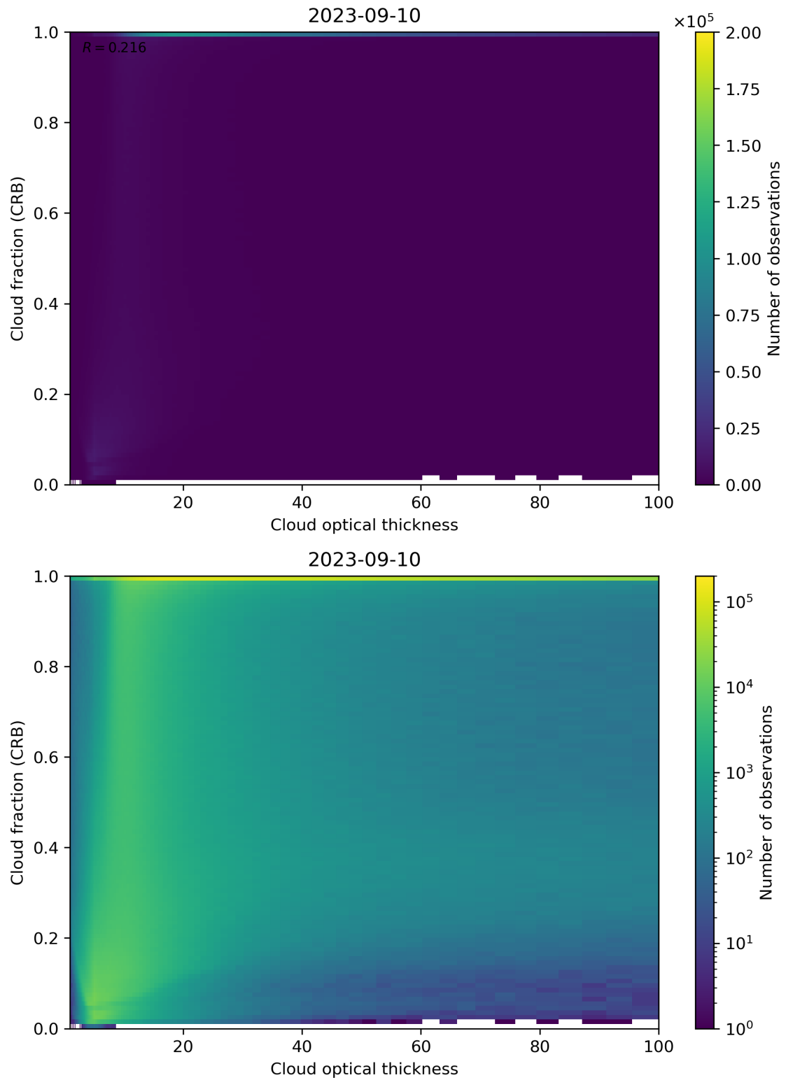
Figure 84: Scatter density plot of “Cloud optical thickness” against “Cloud fraction (CRB)” for 2023-09-10 to 2023-09-11.
