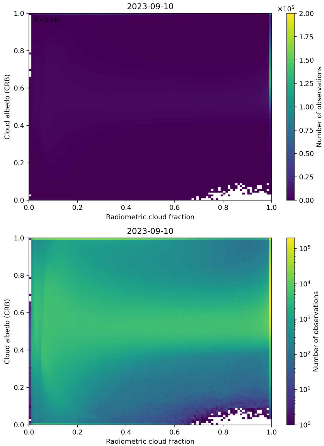
Figure 71: Scatter density plot of “Radiometric cloud fraction” against “Cloud albedo (CRB)” for 2023-09-10 to 2023-09-11.
