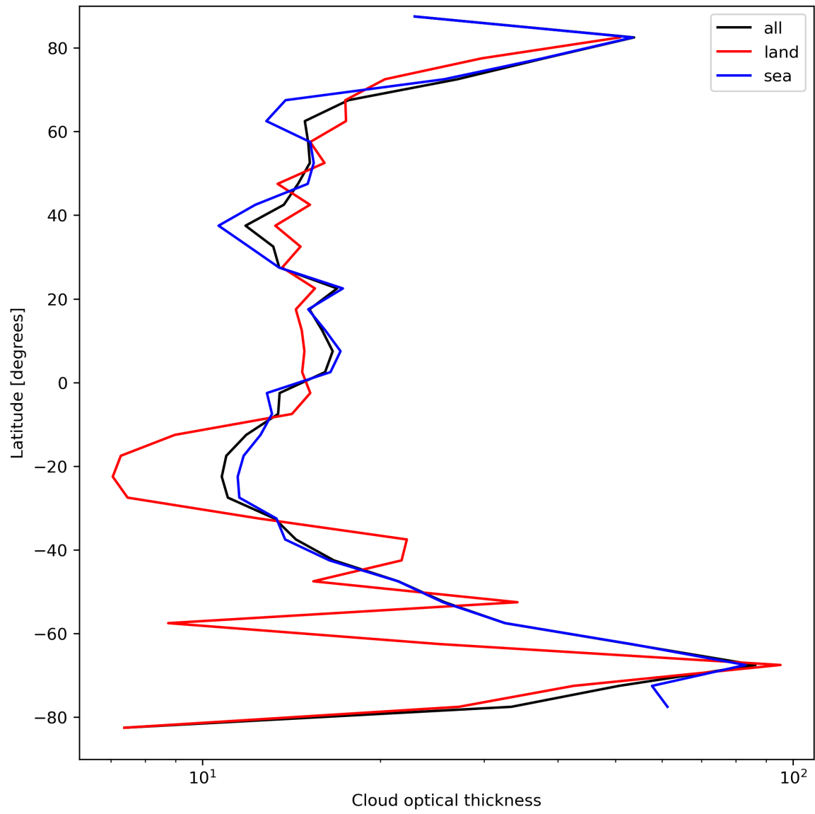
Figure 25: Zonal average of “Cloud optical thickness” for 2023-09-10 to 2023-09-11.
