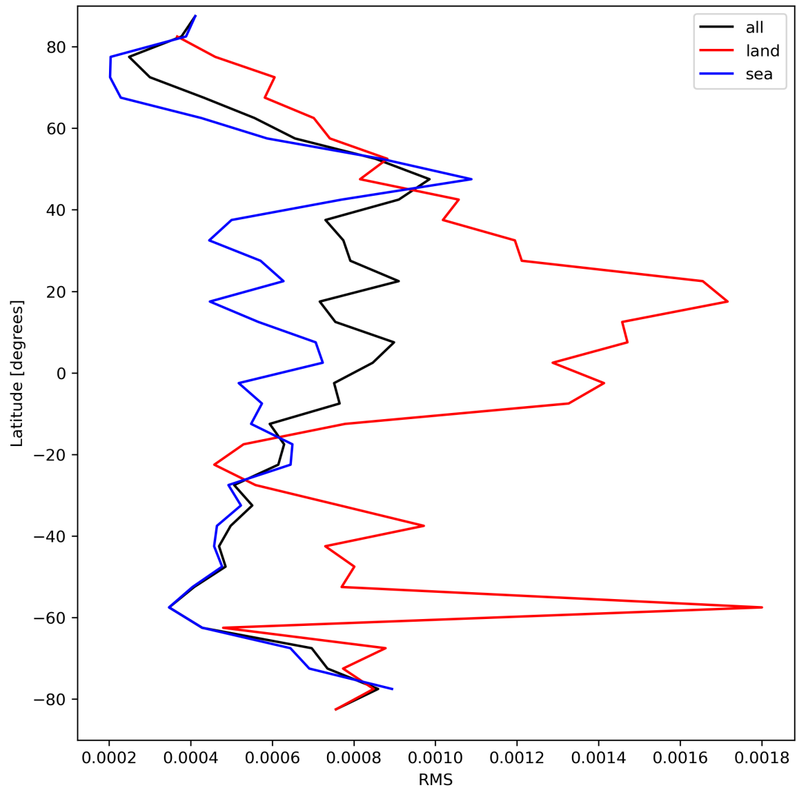
Figure 31: Zonal average of “RMS” for 2023-09-10 to 2023-09-11.
