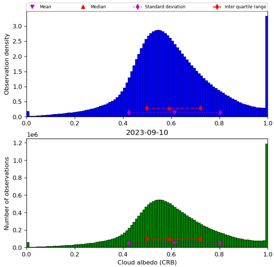
Figure 44: Histogram of “Cloud albedo (CRB)” for 2023-09-10 to 2023-09-11
