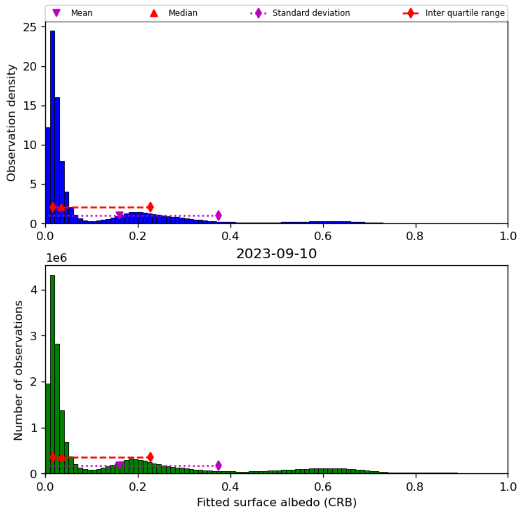
Figure 46: Histogram of “Fitted surface albedo (CRB)” for 2023-09-10 to 2023-09-11
