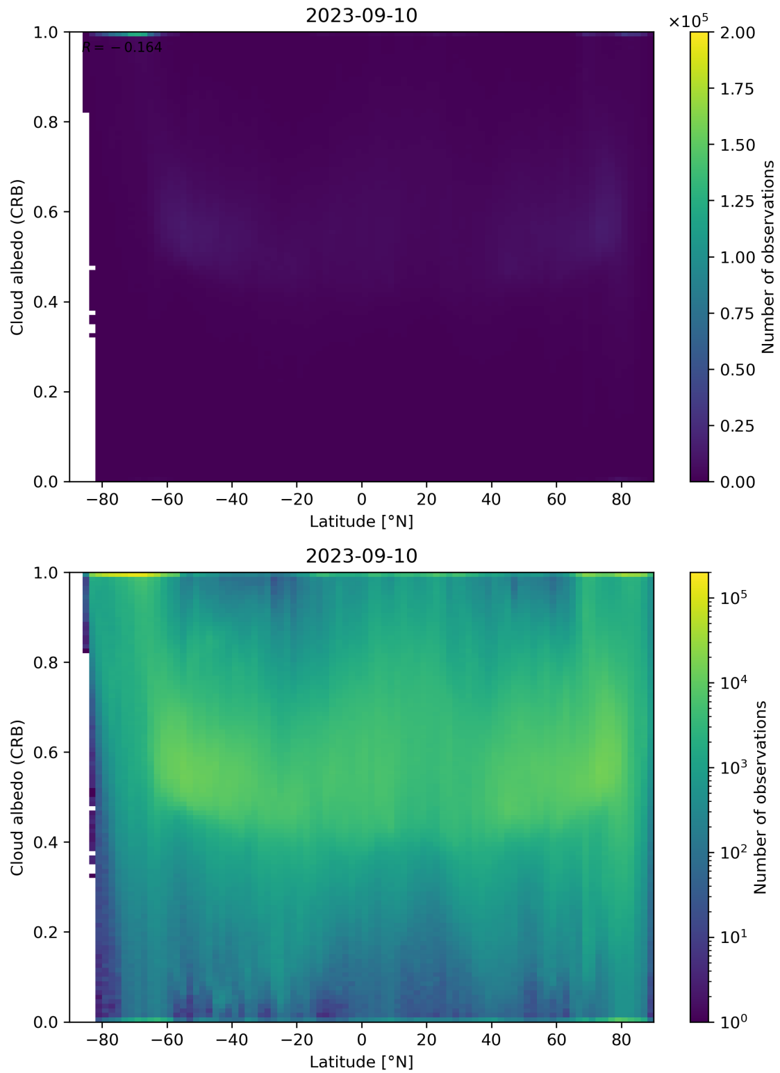
Figure 91: Scatter density plot of “Latitude” against “Cloud albedo (CRB)” for 2023-09-10 to 2023-09-11.
