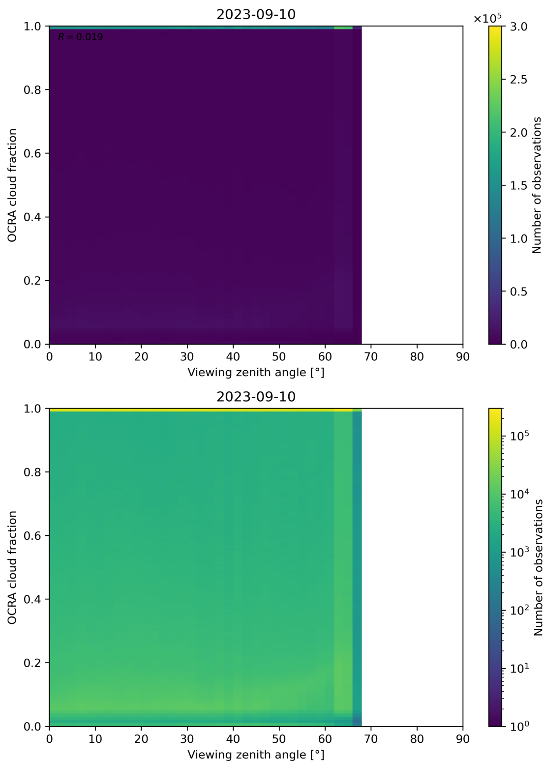
Figure 108: Scatter density plot of “Viewing zenith angle” against “OCRA cloud fraction” for 2023-09-10 to 2023-09-11.
