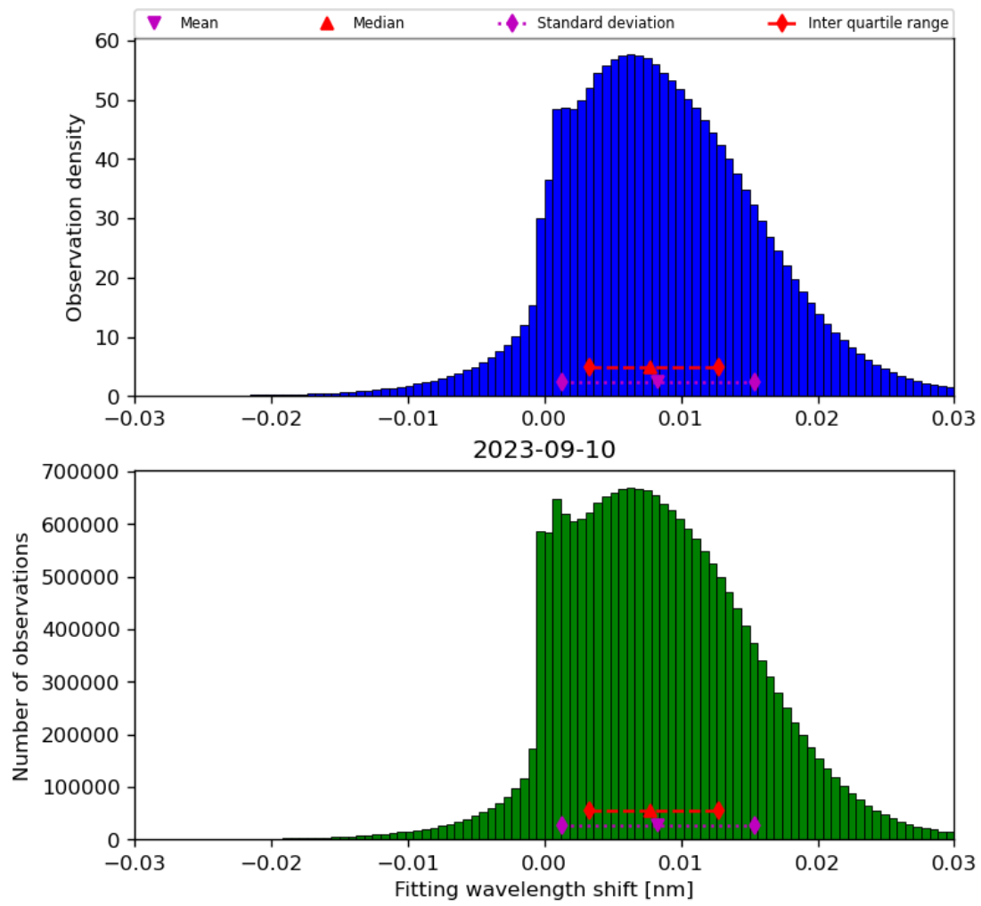
Figure 49: Histogram of “Fitting wavelength shift” for 2023-09-10 to 2023-09-11
