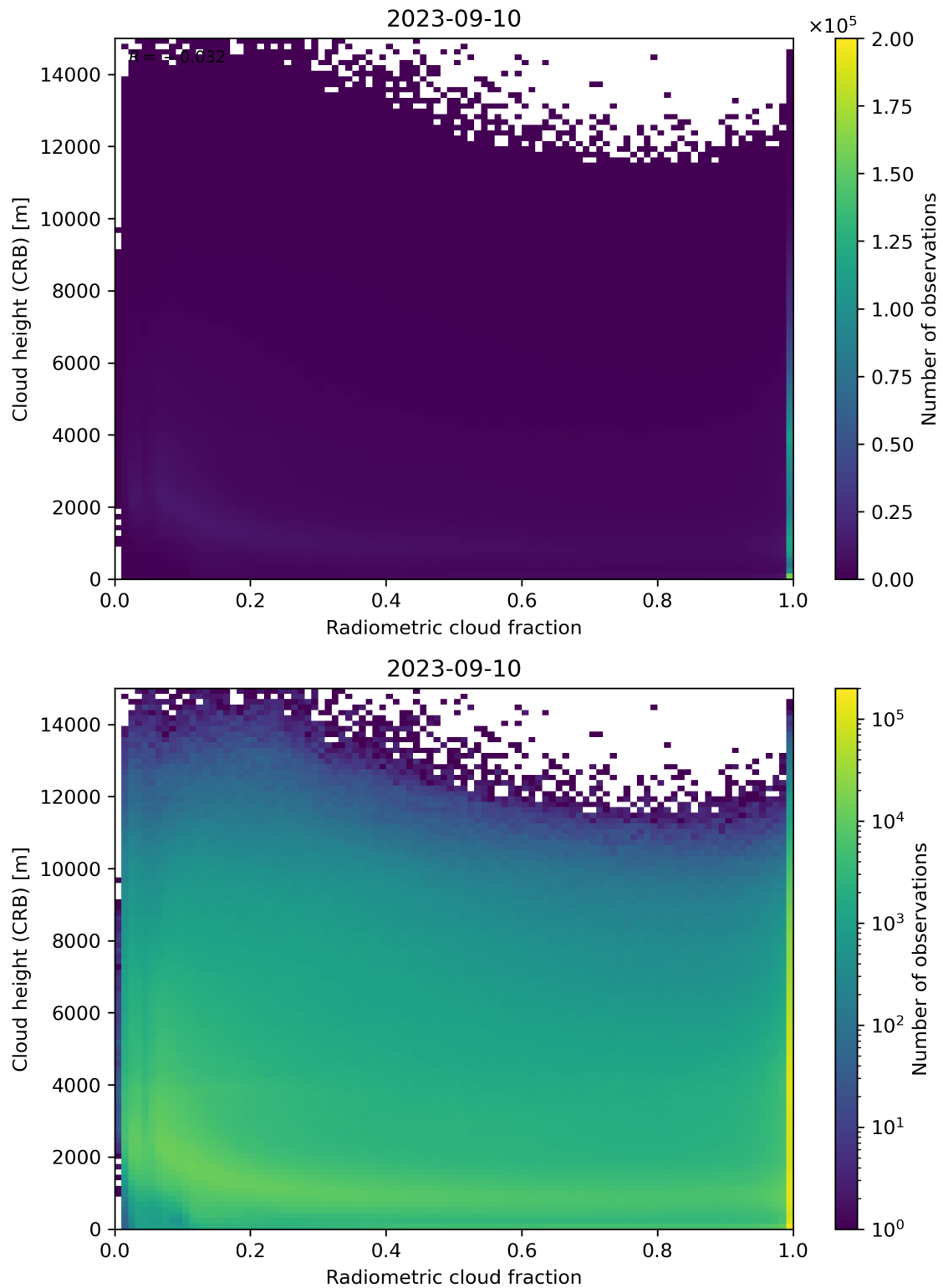
Figure 74: Scatter density plot of “Radiometric cloud fraction” against “Cloud height (CRB)” for 2023-09-10 to 2023-09-11.
