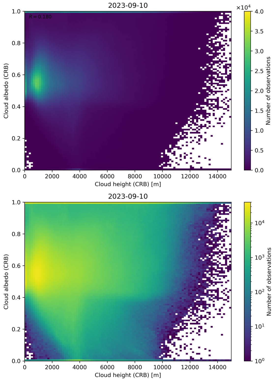
Figure 80: Scatter density plot of “Cloud height (CRB)” against “Cloud albedo (CRB)” for 2023-09-10 to 2023-09-11.
