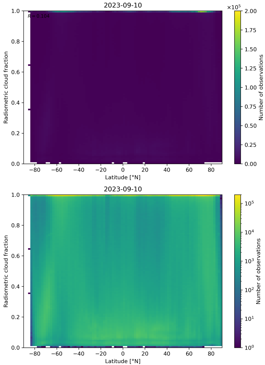
Figure 92: Scatter density plot of “Latitude” against “Radiometric cloud fraction” for 2023-09-10 to 2023-09-11.
