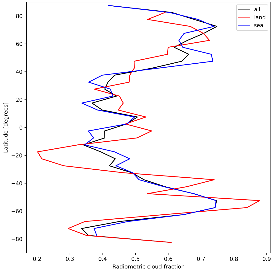
Figure 23: Zonal average of “Radiometric cloud fraction” for 2023-09-10 to 2023-09-11.
