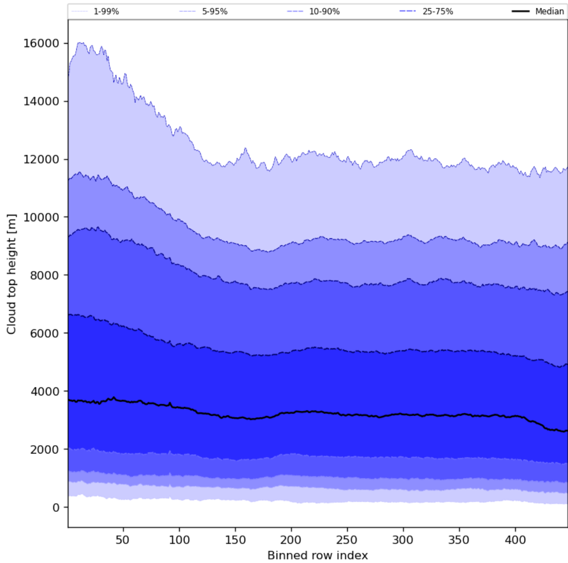
Figure 56: Along track statistics of “Cloud top height” for 2023-09-10 to 2023-09-11
