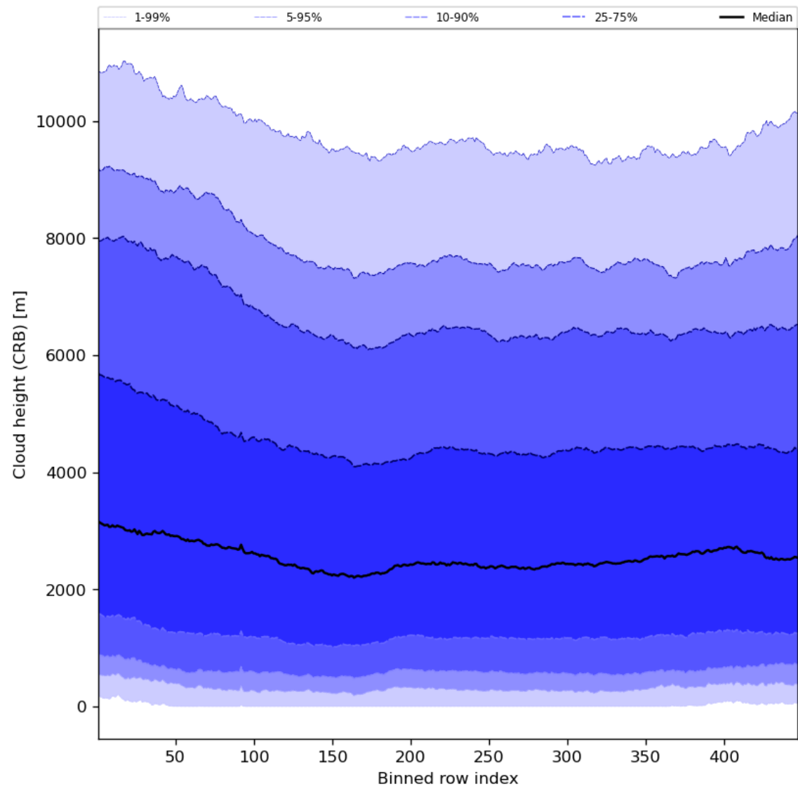
Figure 59: Along track statistics of “Cloud height (CRB)” for 2023-09-10 to 2023-09-11
