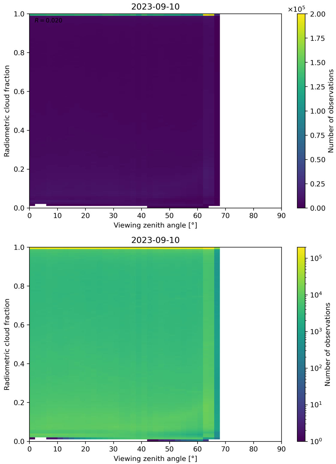
Figure 107: Scatter density plot of “Viewing zenith angle” against “Radiometric cloud fraction” for 2023-09-10 to 2023-09-11.
