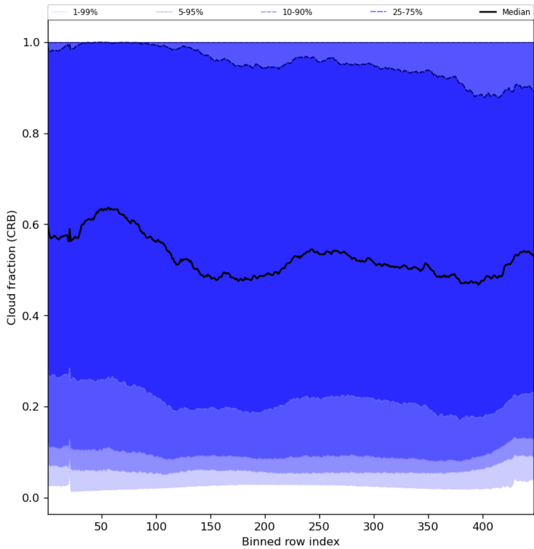
Figure 58: Along track statistics of “Cloud fraction (CRB)” for 2023-09-10 to 2023-09-11
