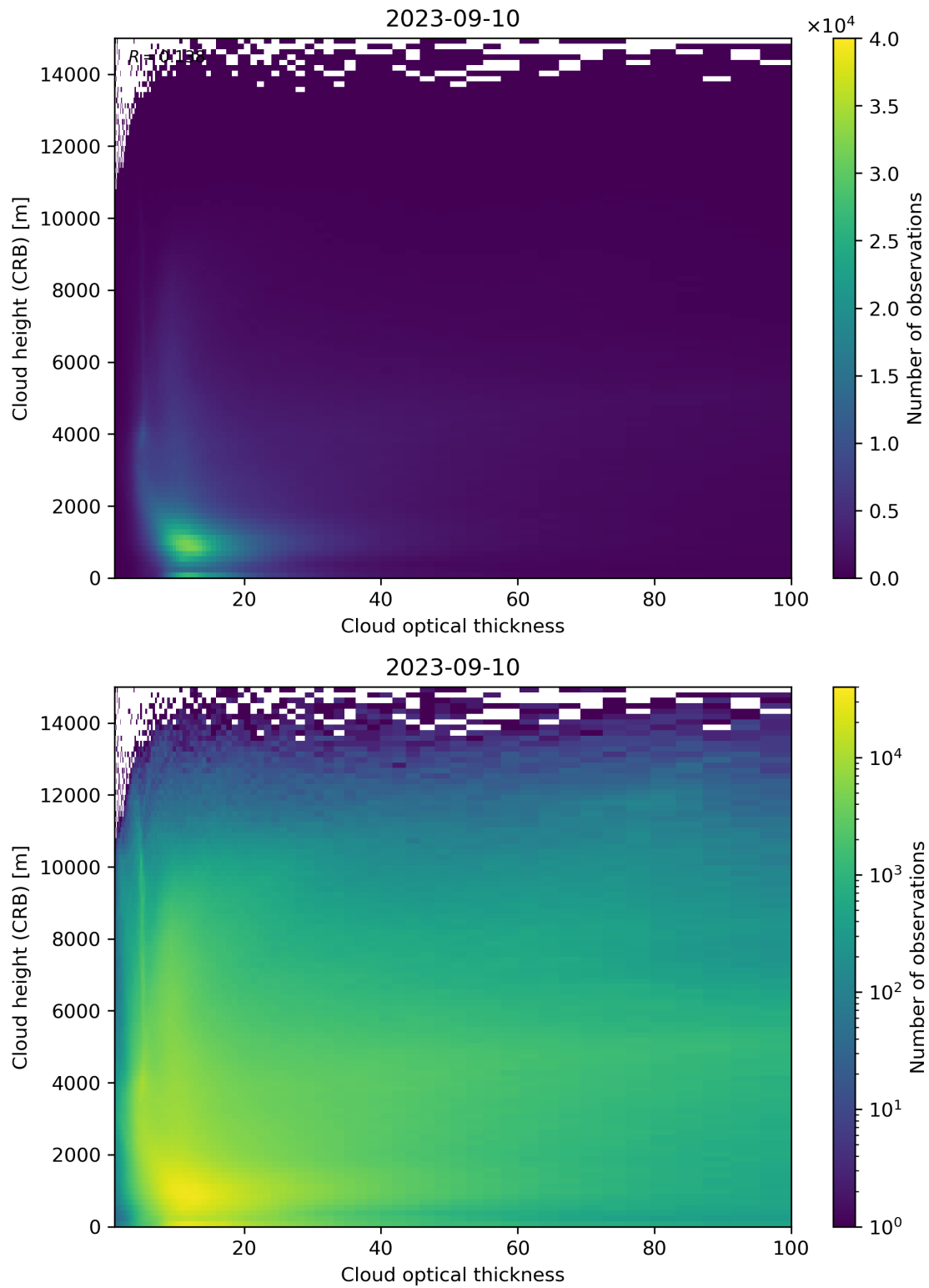
Figure 85: Scatter density plot of “Cloud optical thickness” against “Cloud height (CRB)” for 2023-09-10 to 2023-09-11.
