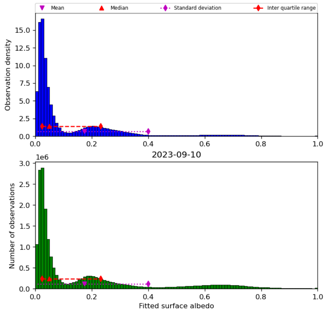
Figure 45: Histogram of “Fitted surface albedo” for 2023-09-10 to 2023-09-11
