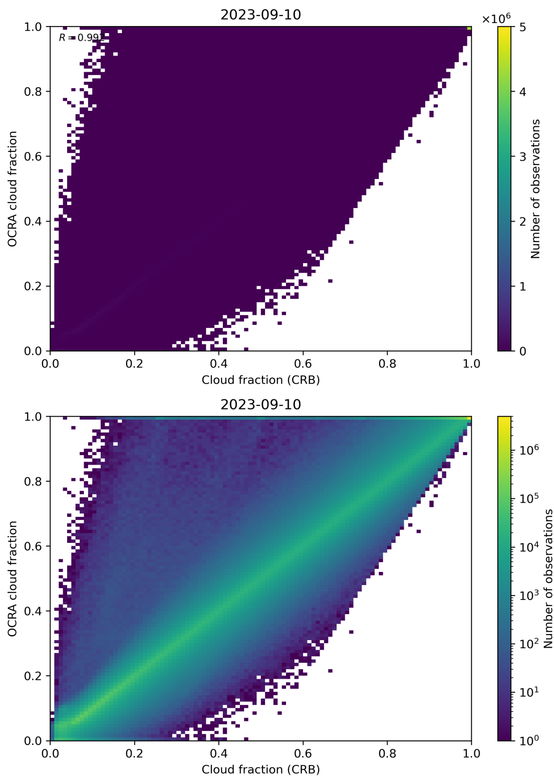
Figure 78: Scatter density plot of “Cloud fraction (CRB)” against “OCRA cloud fraction” for 2023-09-10 to 2023-09-11.
