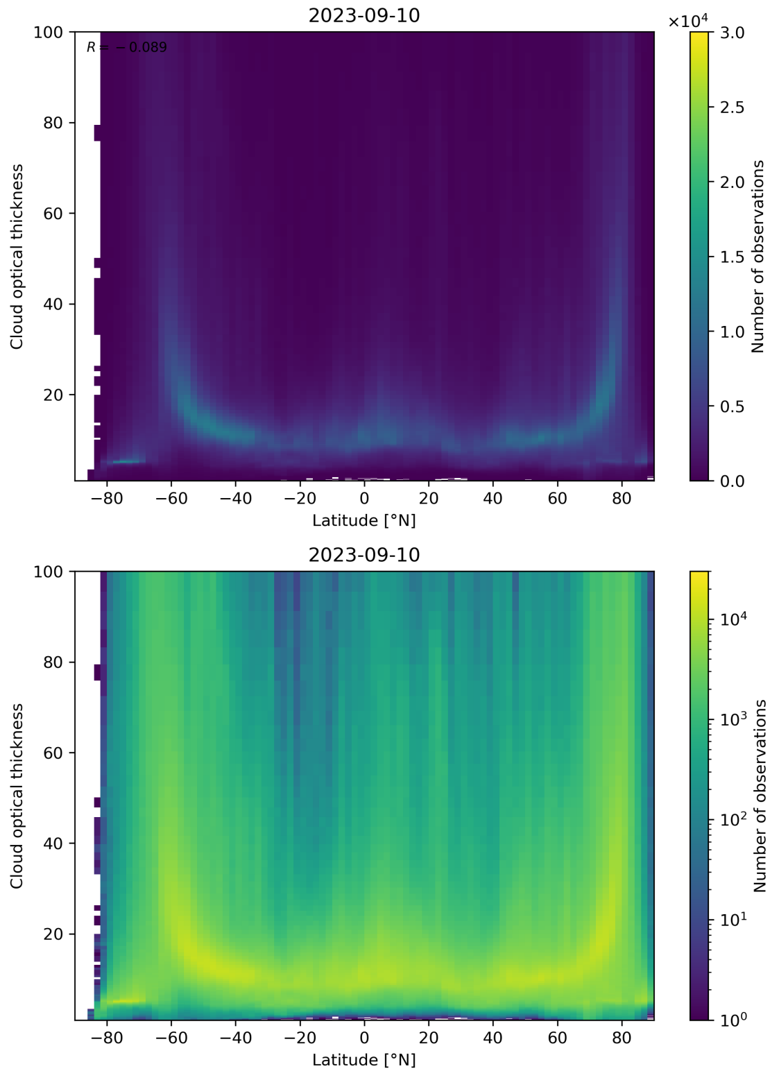
Figure 96: Scatter density plot of “Latitude” against “Cloud optical thickness” for 2023-09-10 to 2023-09-11.
