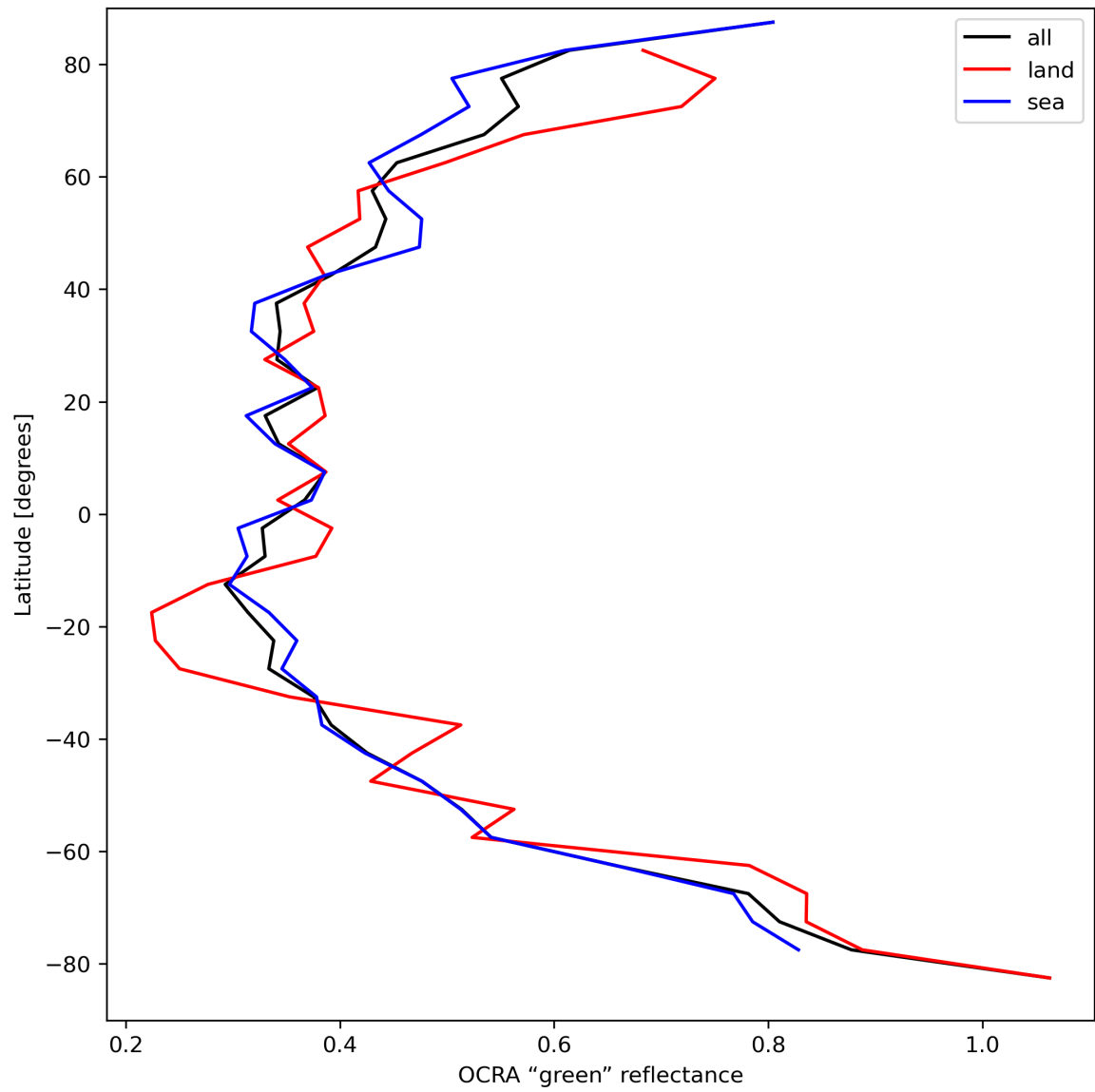
Figure 36: Zonal average of “OCRA “green” reflectance” for 2023-09-10 to 2023-09-11.
