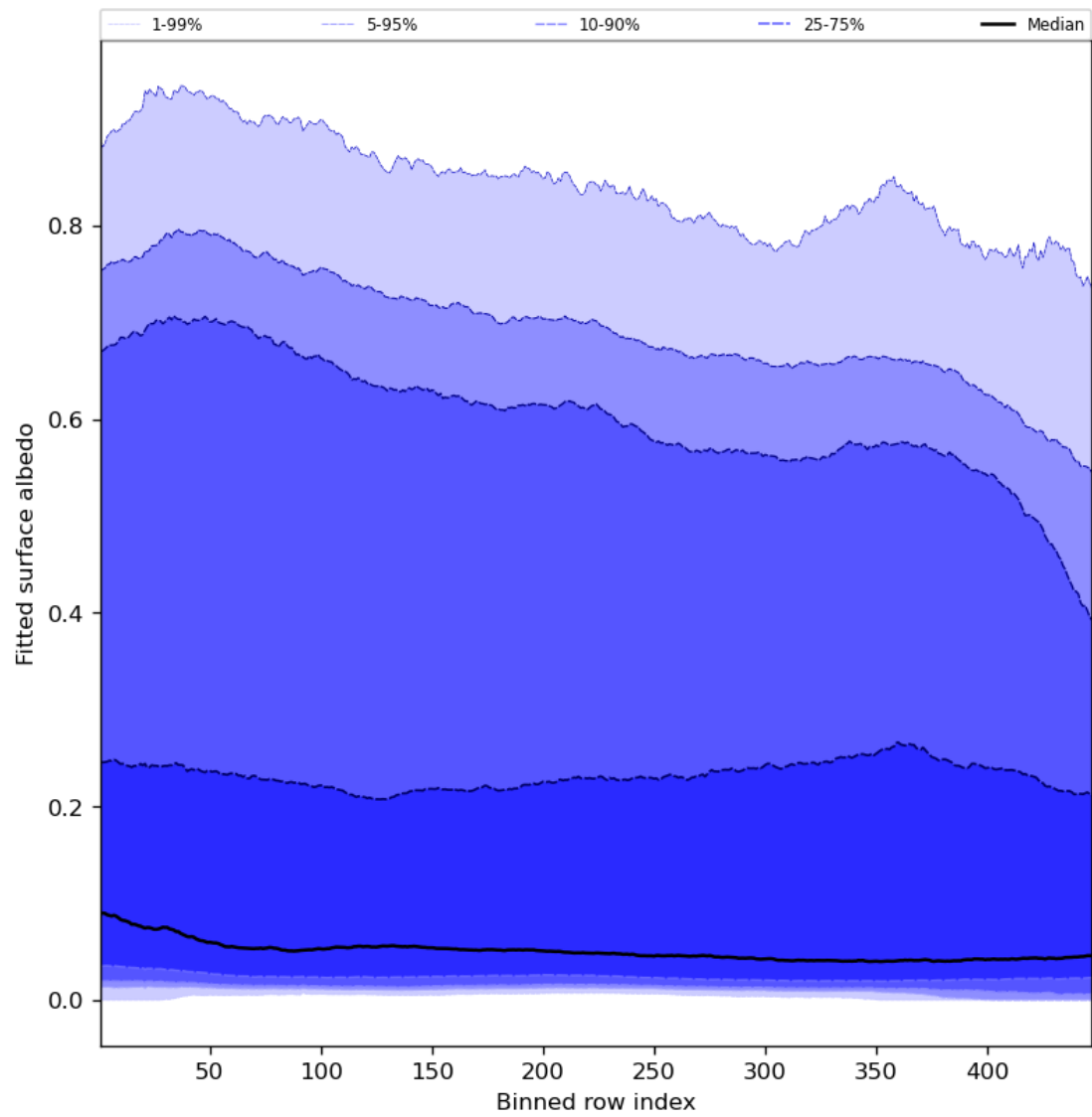
Figure 61: Along track statistics of “Fitted surface albedo” for 2023-09-10 to 2023-09-11
