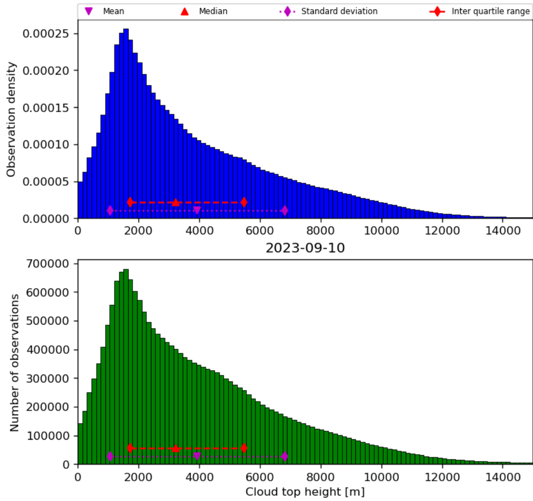
Figure 40: Histogram of “Cloud top height” for 2023-09-10 to 2023-09-11
