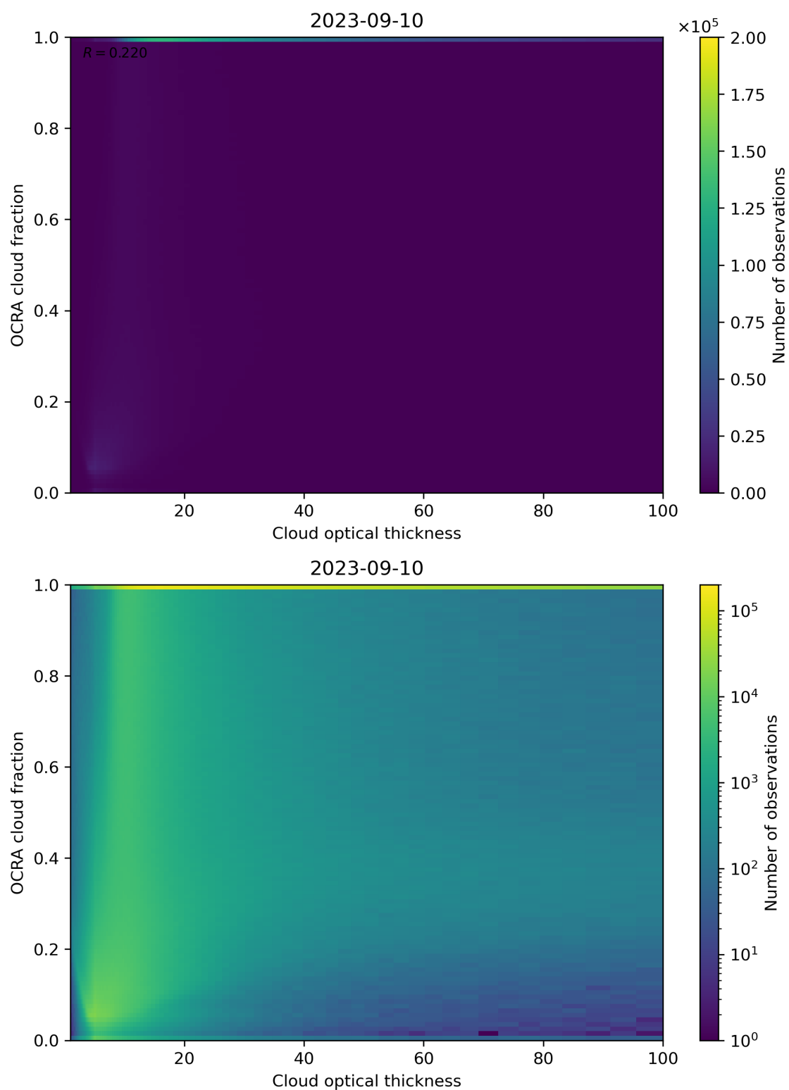
Figure 83: Scatter density plot of “Cloud optical thickness” against “OCRA cloud fraction” for 2023-09-10 to 2023-09-11.
