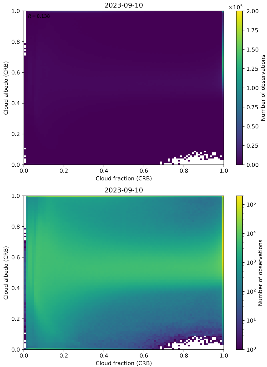
Figure 77: Scatter density plot of “Cloud fraction (CRB)” against “Cloud albedo (CRB)” for 2023-09-10 to 2023-09-11.
