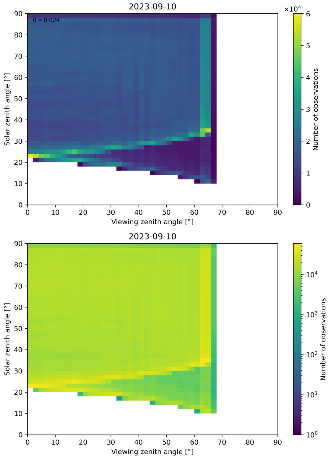
Figure 114: Scatter density plot of “Viewing zenith angle” against “Solar zenith angle” for 2023-09-10 to 2023-09-11.
