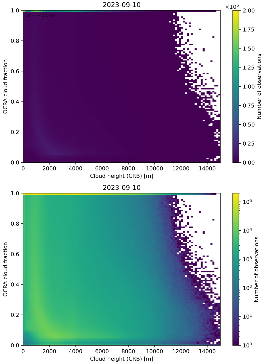
Figure 81: Scatter density plot of “Cloud height (CRB)” against “OCRA cloud fraction” for 2023-09-10 to 2023-09-11.
