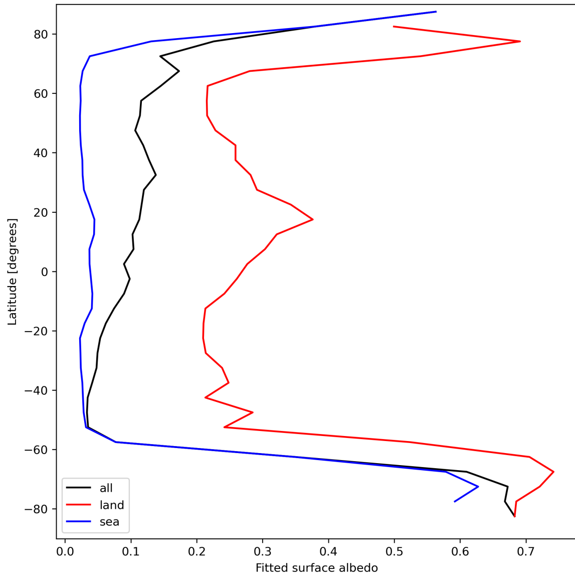
Figure 29: Zonal average of “Fitted surface albedo” for 2023-09-10 to 2023-09-11.
