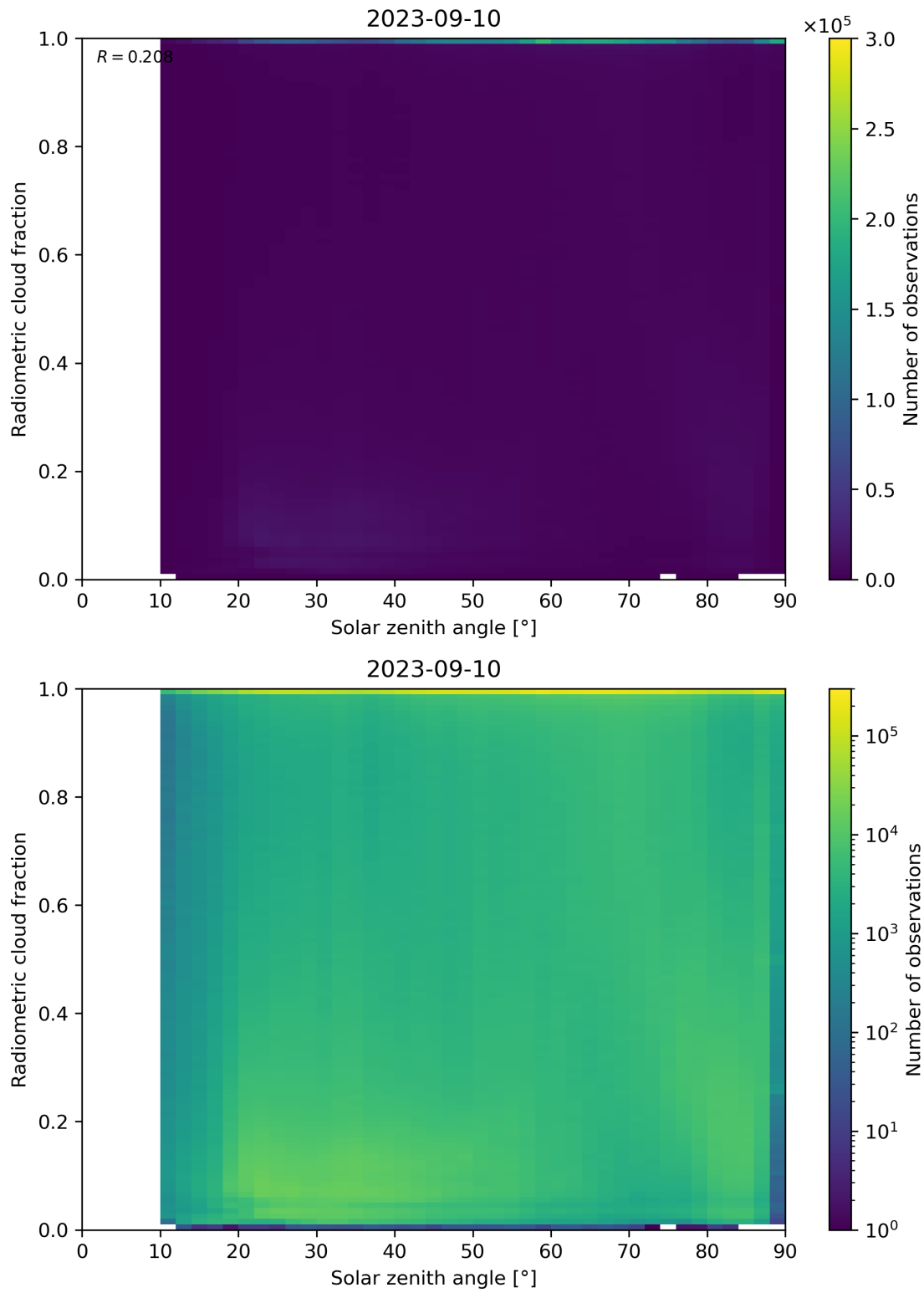
Figure 99: Scatter density plot of “Solar zenith angle” against “Radiometric cloud fraction” for 2023-09-10 to 2023-09-11.
