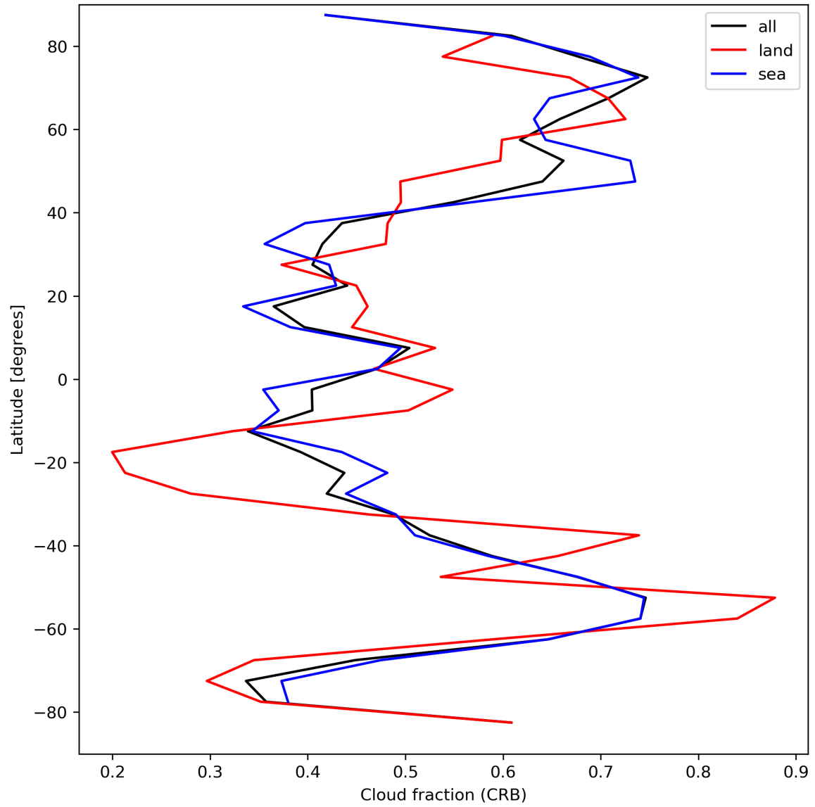
Figure 26: Zonal average of “Cloud fraction (CRB)” for 2023-09-10 to 2023-09-11.
