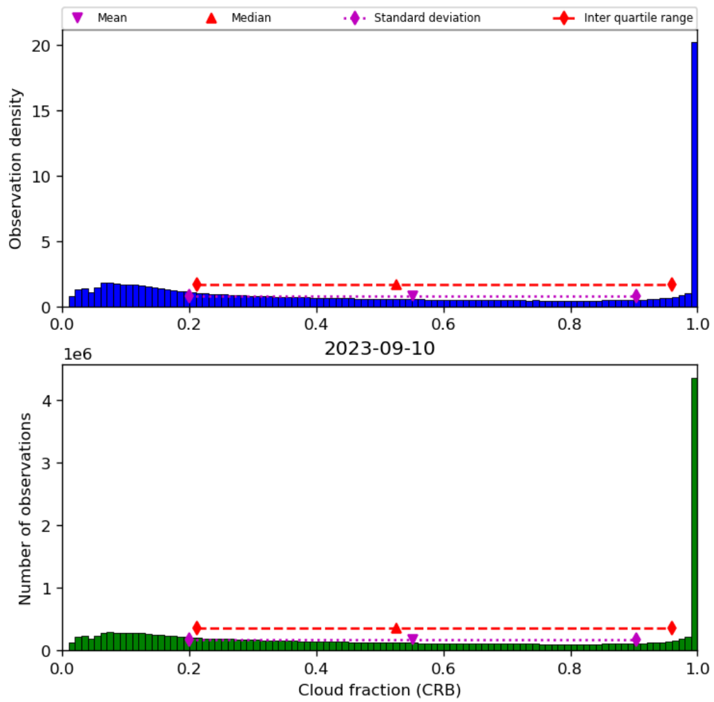
Figure 42: Histogram of “Cloud fraction (CRB)” for 2023-09-10 to 2023-09-11
