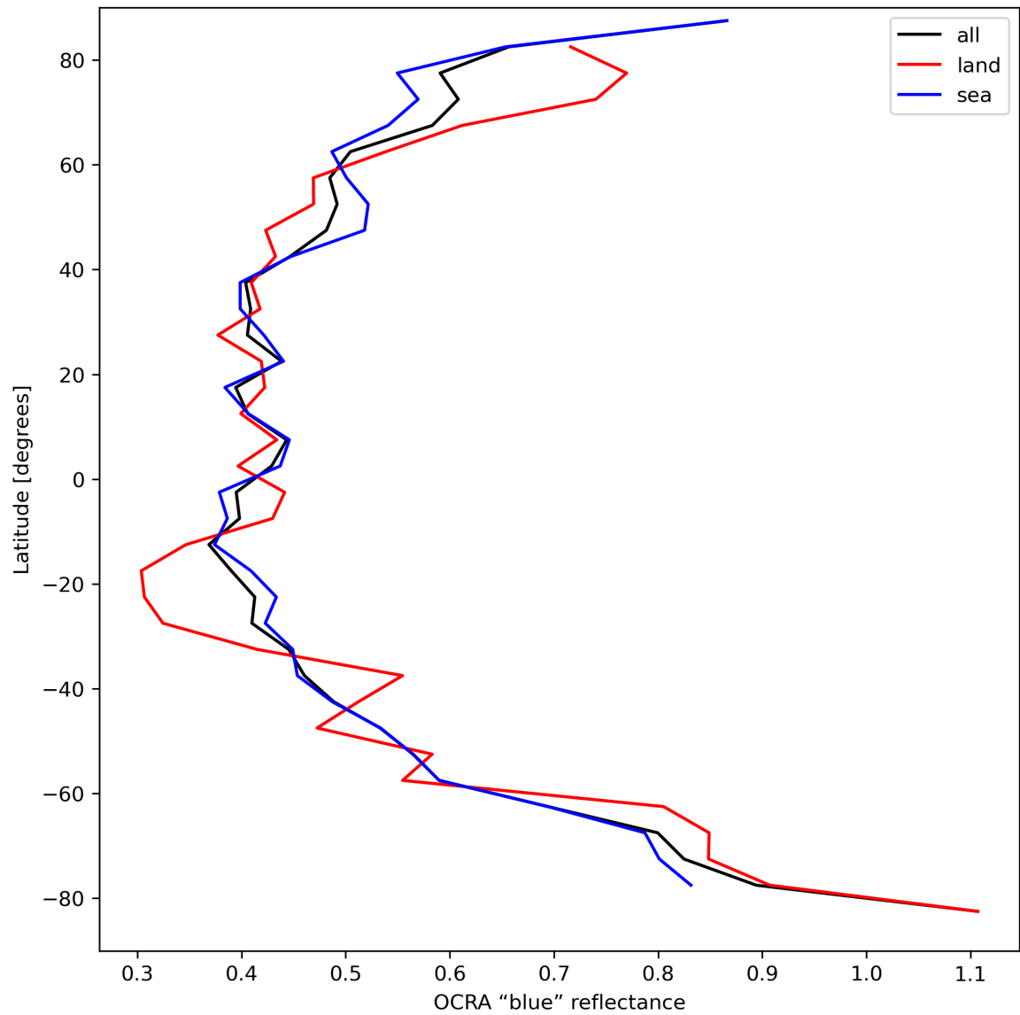
Figure 35: Zonal average of “OCRA “blue” reflectance” for 2023-09-10 to 2023-09-11.
