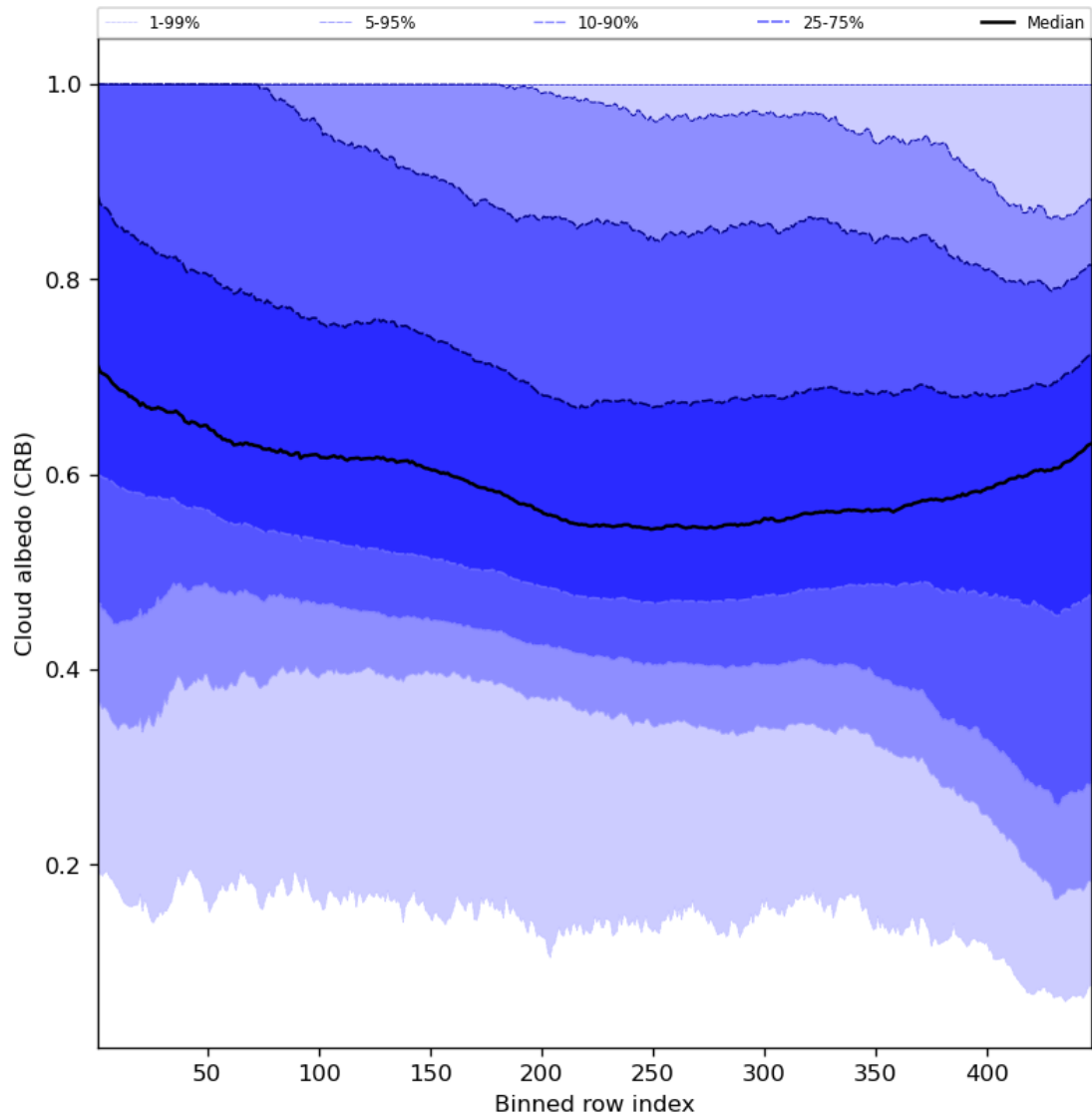
Figure 60: Along track statistics of “Cloud albedo (CRB)” for 2023-09-10 to 2023-09-11
