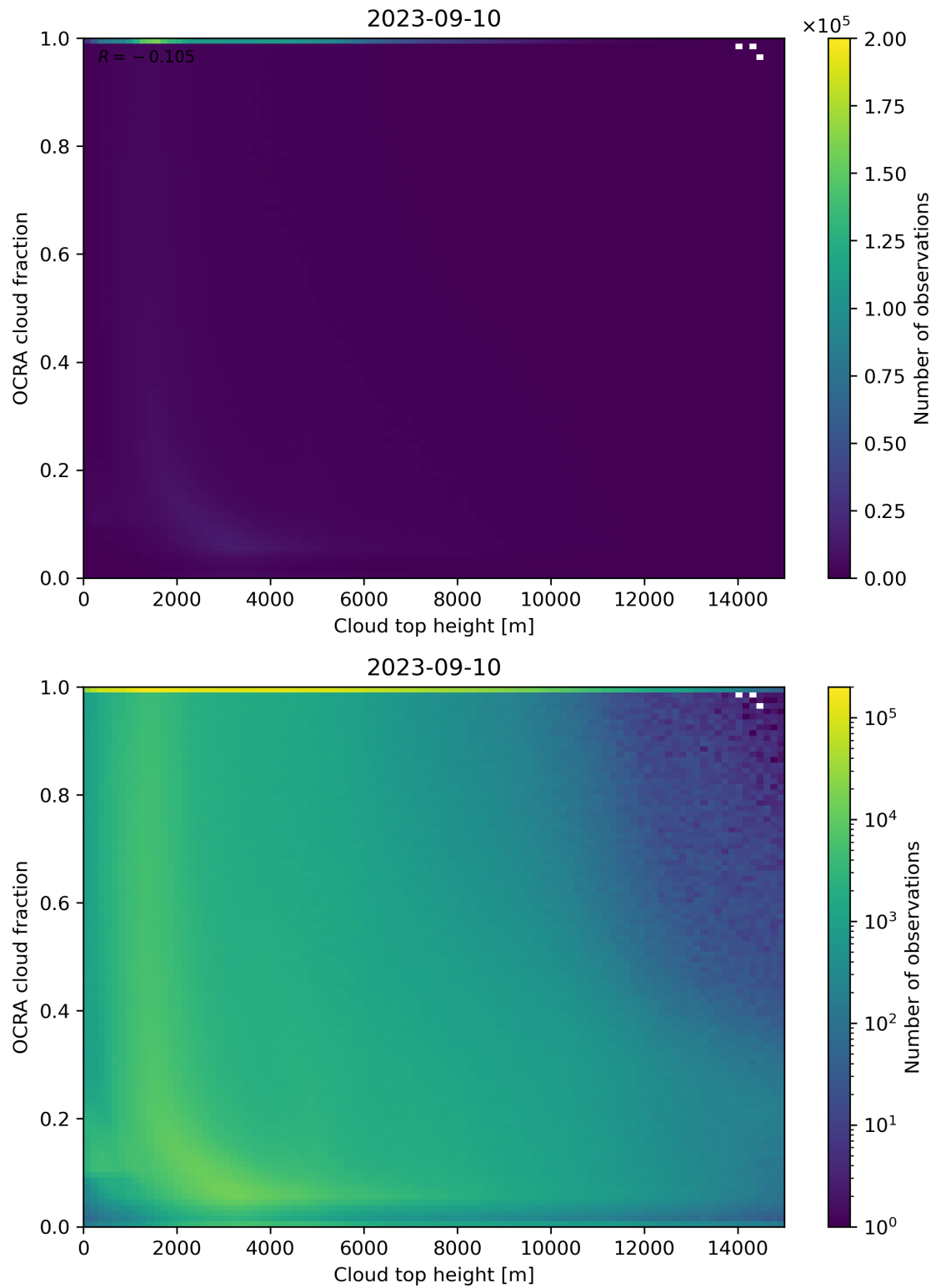
Figure 87: Scatter density plot of “Cloud top height” against “OCRA cloud fraction” for 2023-09-10 to 2023-09-11.
