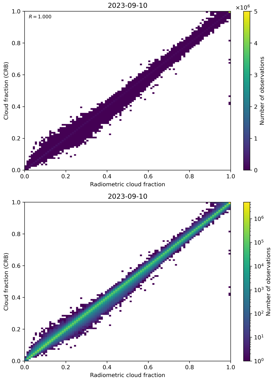
Figure 73: Scatter density plot of “Radiometric cloud fraction” against “Cloud fraction (CRB)” for 2023-09-10 to 2023-09-11.
