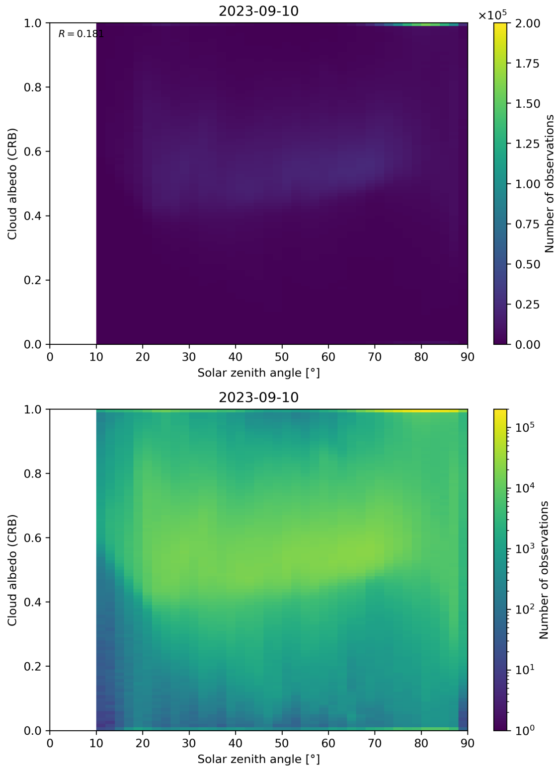
Figure 98: Scatter density plot of “Solar zenith angle” against “Cloud albedo (CRB)” for 2023-09-10 to 2023-09-11.
