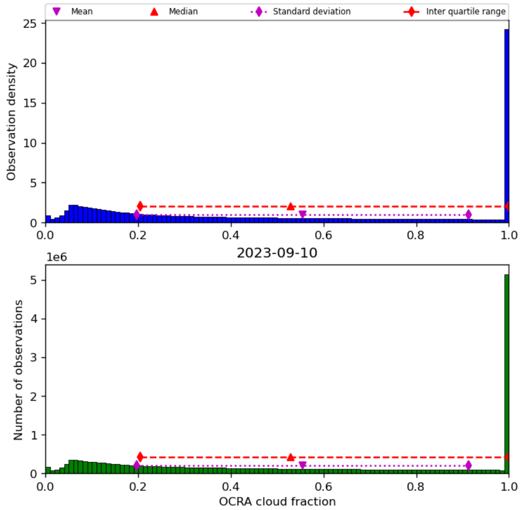
Figure 50: Histogram of “OCRA cloud fraction” for 2023-09-10 to 2023-09-11
