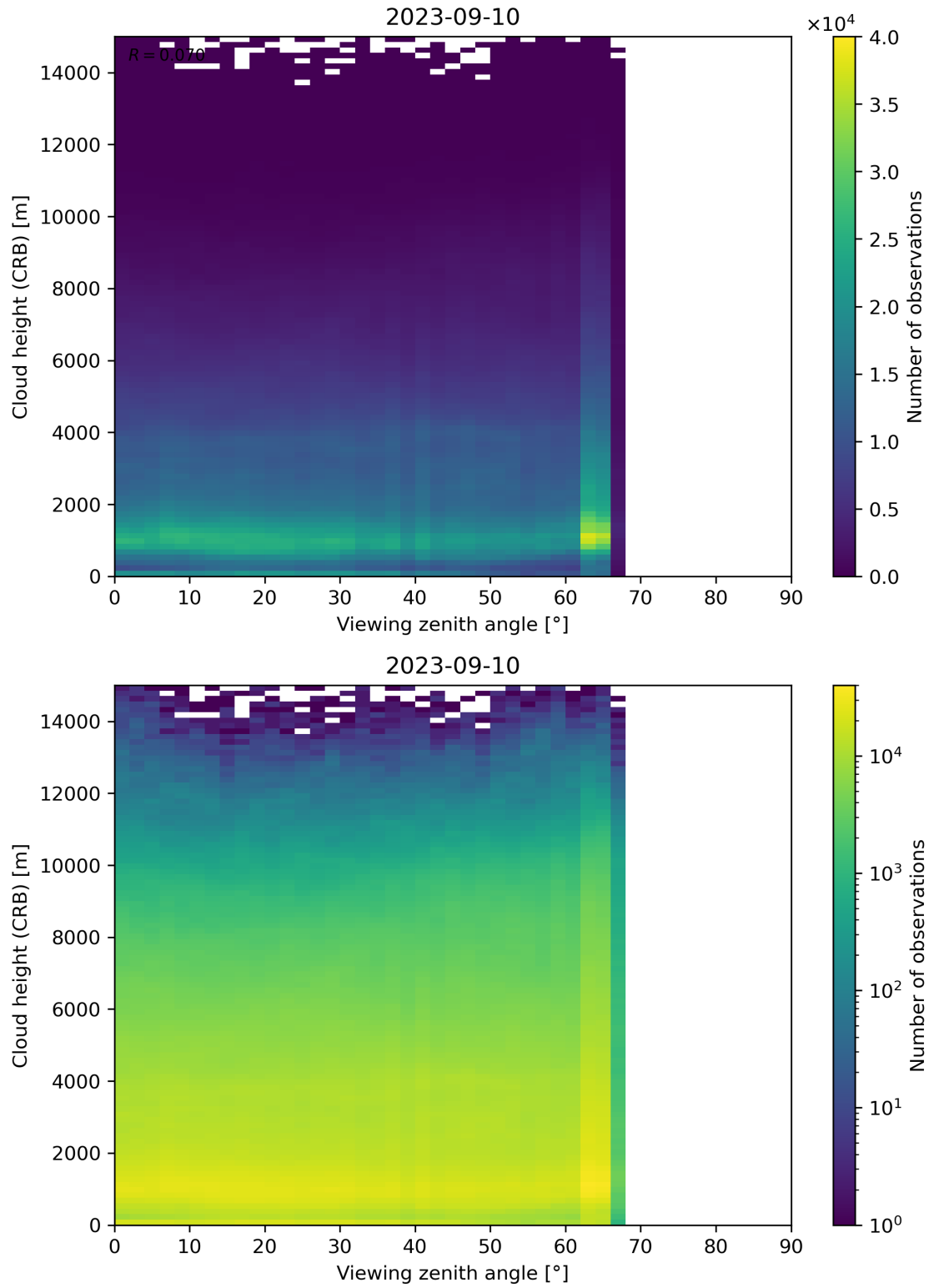
Figure 110: Scatter density plot of “Viewing zenith angle” against “Cloud height (CRB)” for 2023-09-10 to 2023-09-11.
