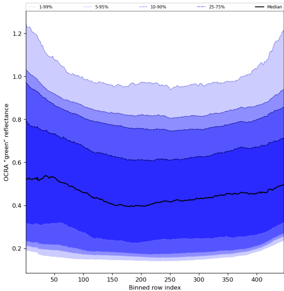
Figure 68: Along track statistics of “OCRA “green” reflectance” for 2023-09-10 to 2023-09-11
