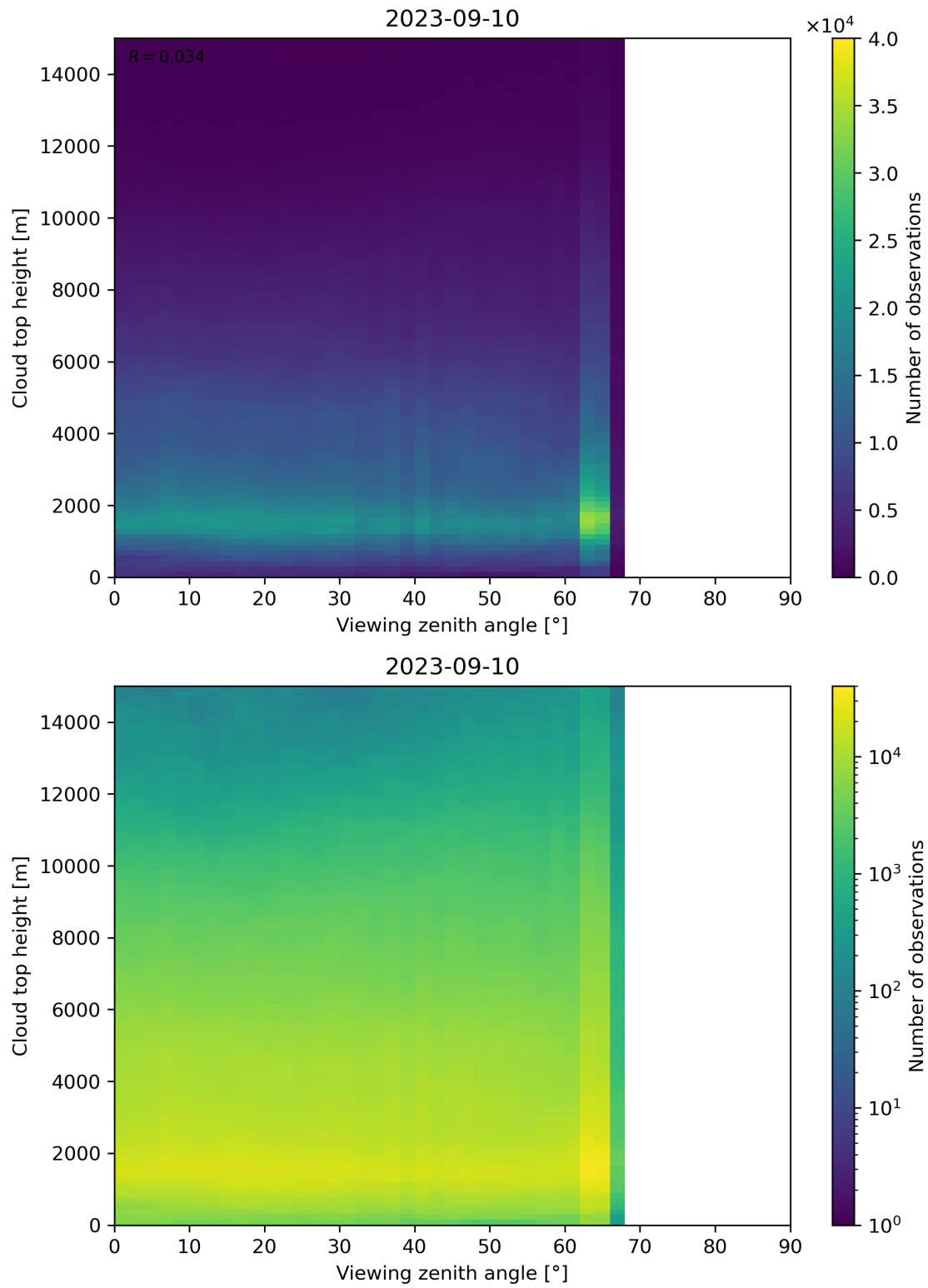
Figure 112: Scatter density plot of “Viewing zenith angle” against “Cloud top height” for 2023-09-10 to 2023-09-11.
