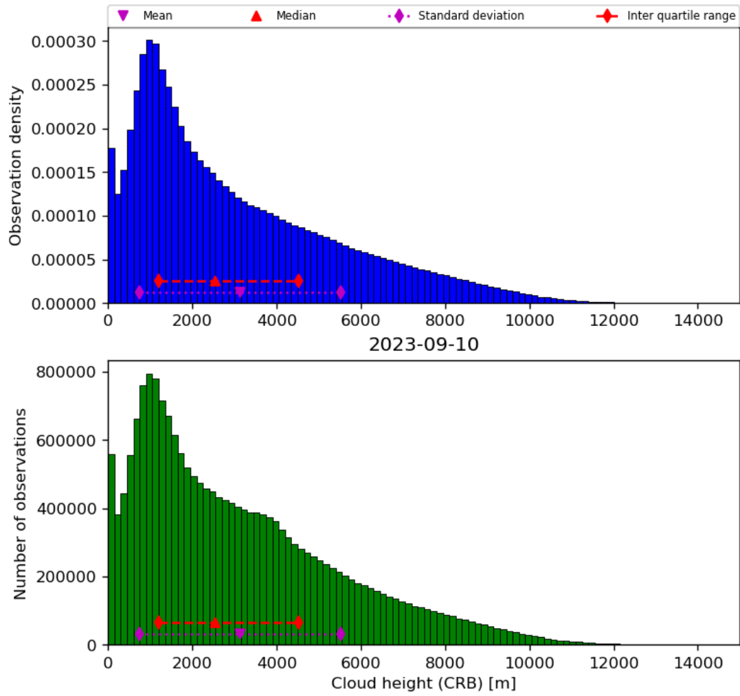
Figure 43: Histogram of “Cloud height (CRB)” for 2023-09-10 to 2023-09-11
