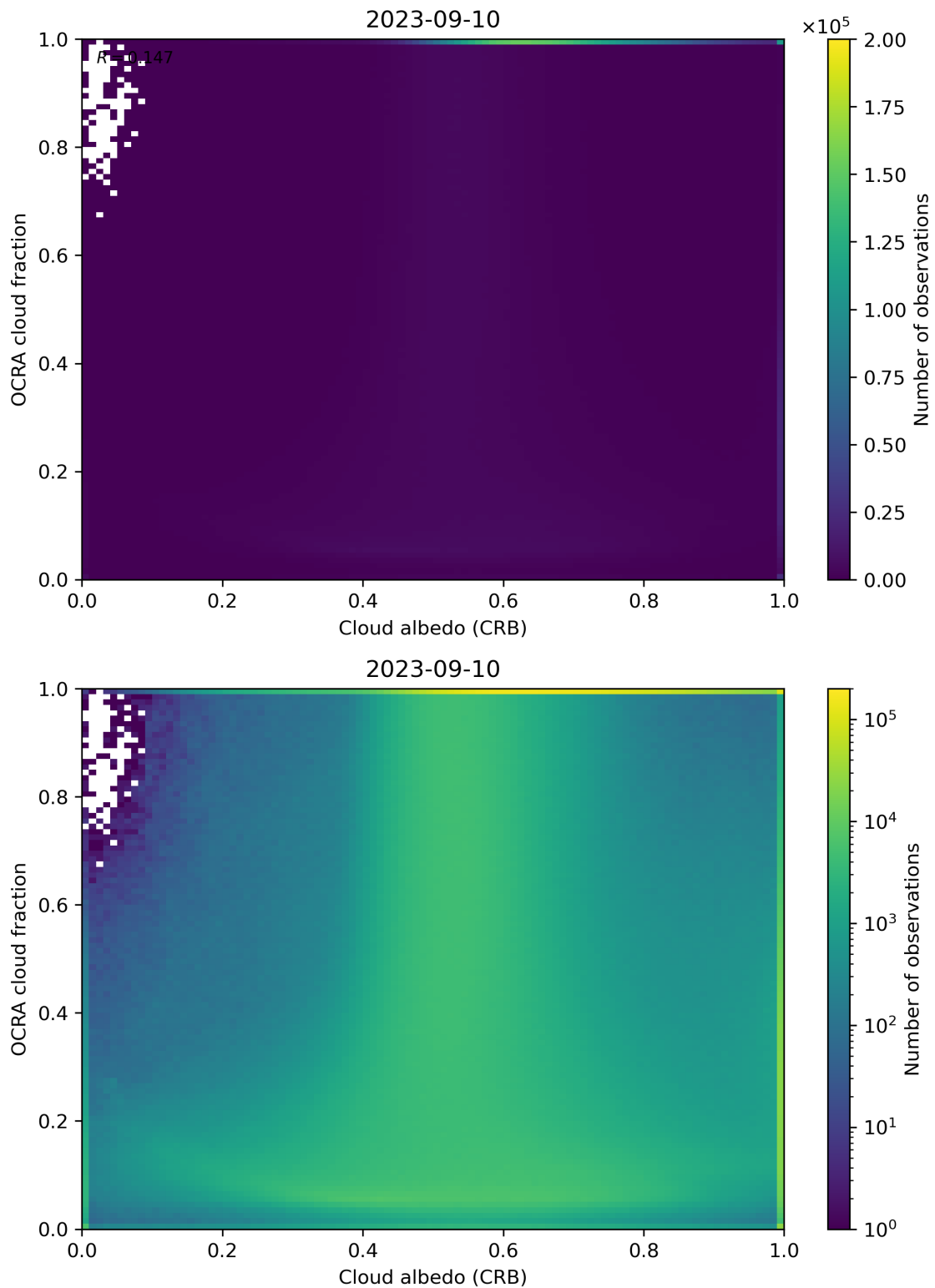
Figure 70: Scatter density plot of “Cloud albedo (CRB)” against “OCRA cloud fraction” for 2023-09-10 to 2023-09-11.
