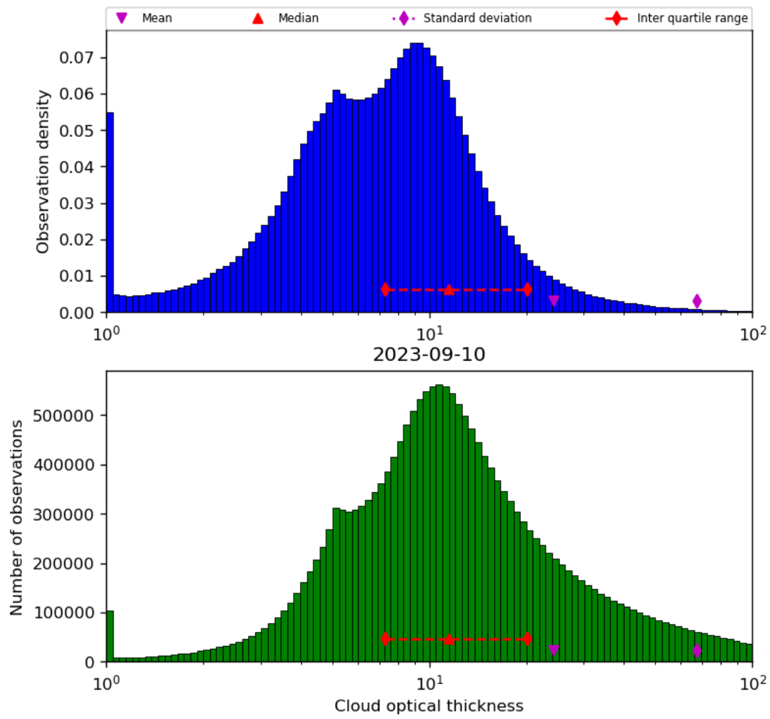
Figure 41: Histogram of “Cloud optical thickness” for 2023-09-10 to 2023-09-11
