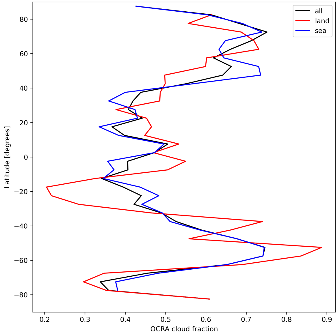
Figure 34: Zonal average of “OCRA cloud fraction” for 2023-09-10 to 2023-09-11.
