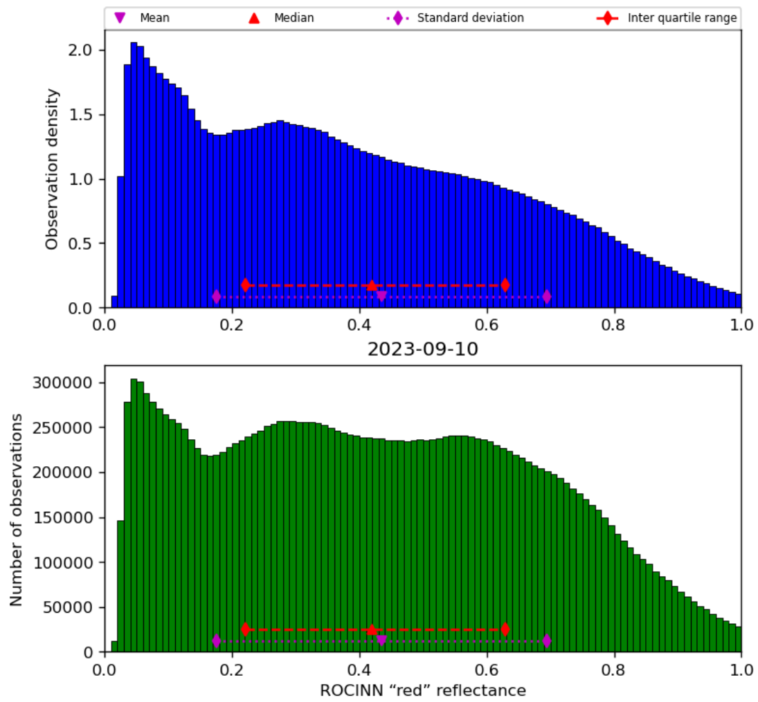
Figure 53: Histogram of “ROCINN “red” reflectance” for 2023-09-10 to 2023-09-11
