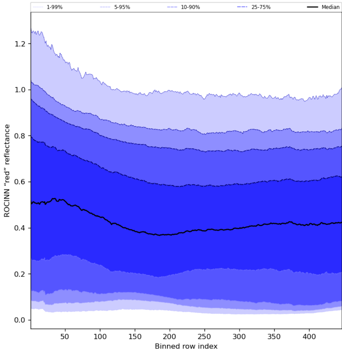
Figure 69: Along track statistics of “ROCINN “red” reflectance” for 2023-09-10 to 2023-09-11
