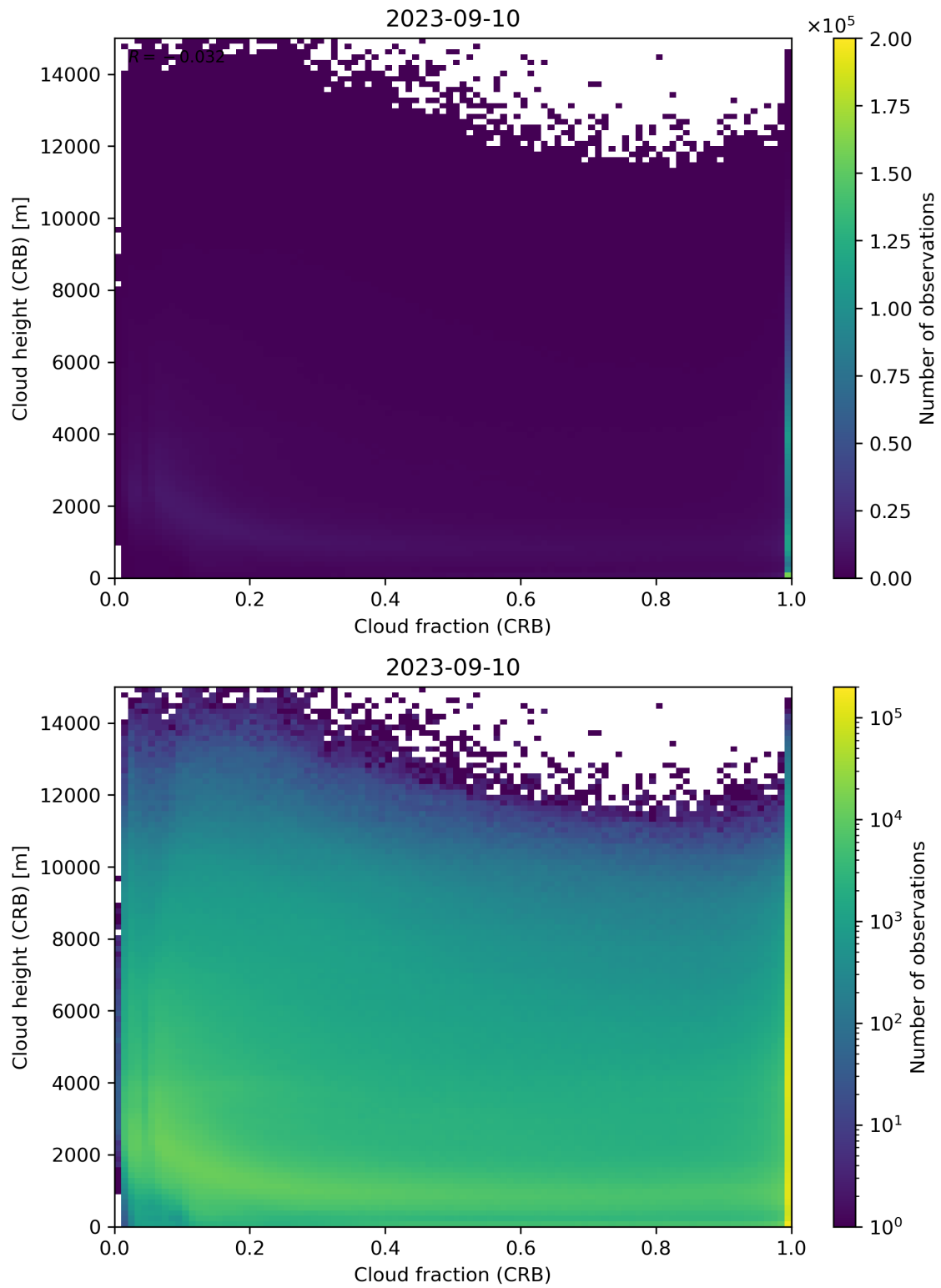
Figure 79: Scatter density plot of “Cloud fraction (CRB)” against “Cloud height (CRB)” for 2023-09-10 to 2023-09-11.
