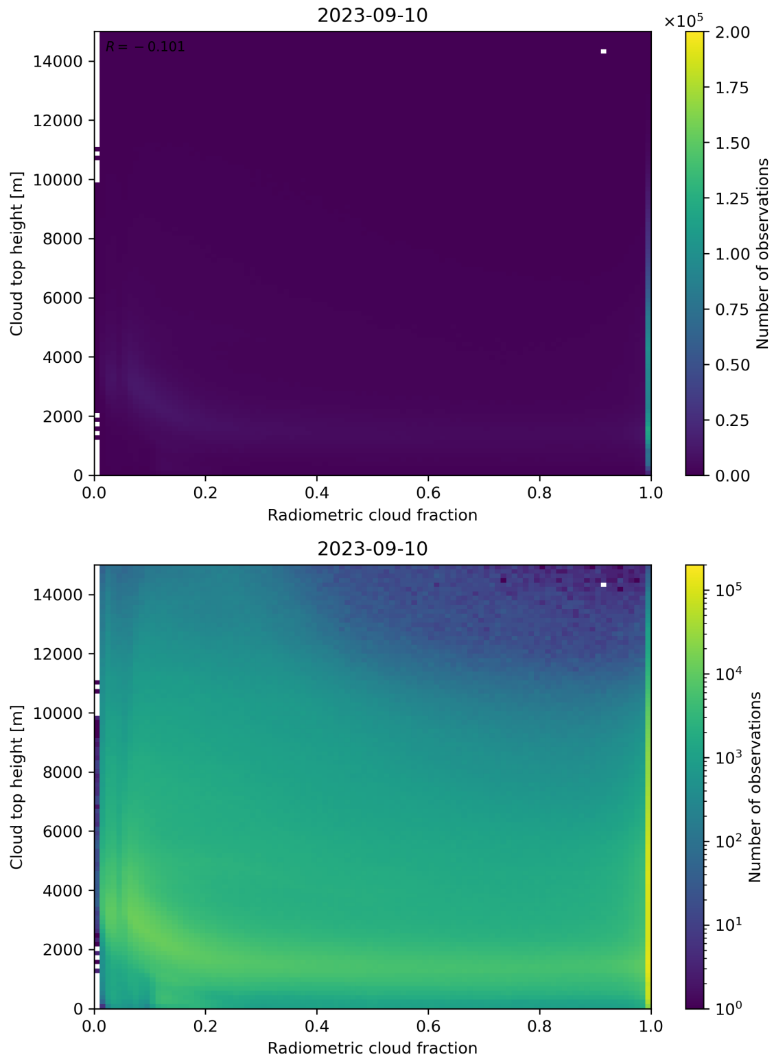
Figure 76: Scatter density plot of “Radiometric cloud fraction” against “Cloud top height” for 2023-09-10 to 2023-09-11.
