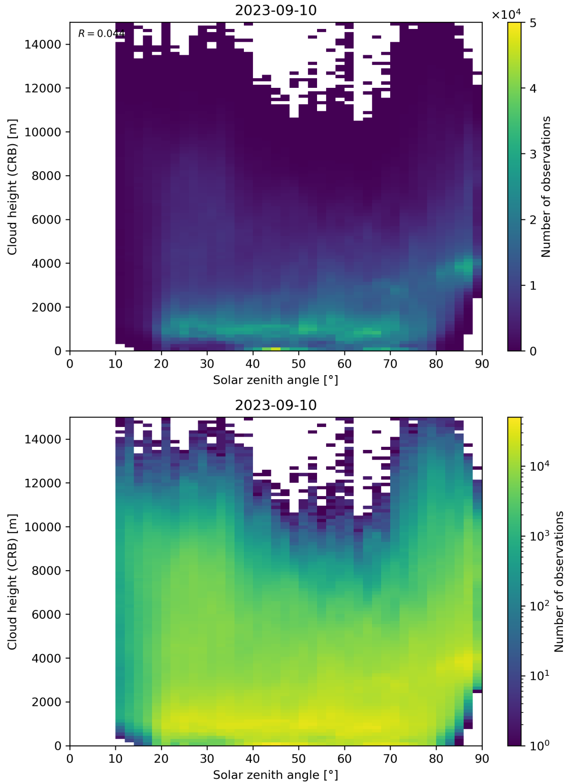
Figure 102: Scatter density plot of “Solar zenith angle” against “Cloud height (CRB)” for 2023-09-10 to 2023-09-11.
