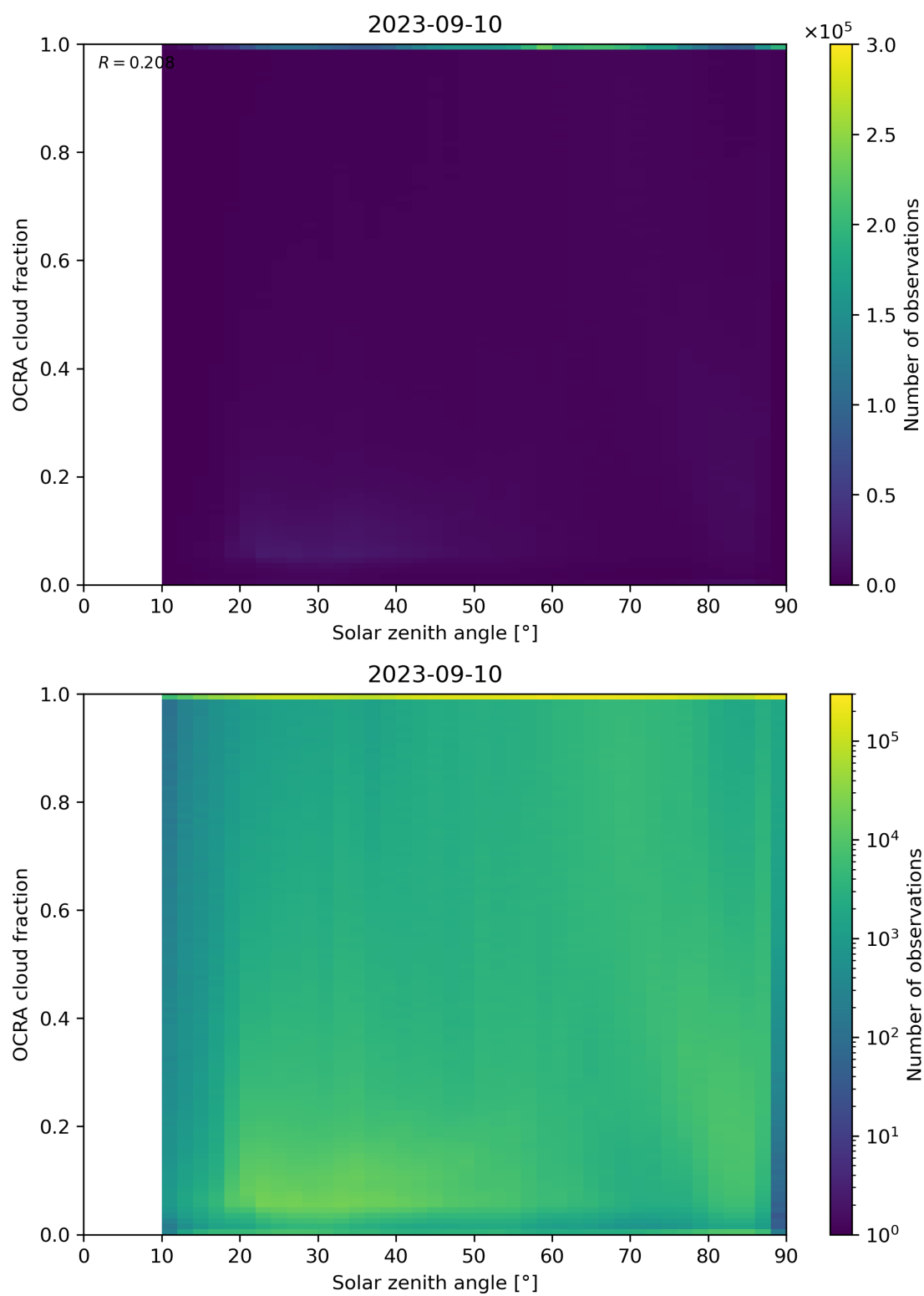
Figure 100: Scatter density plot of “Solar zenith angle” against “OCRA cloud fraction” for 2023-09-10 to 2023-09-11.
