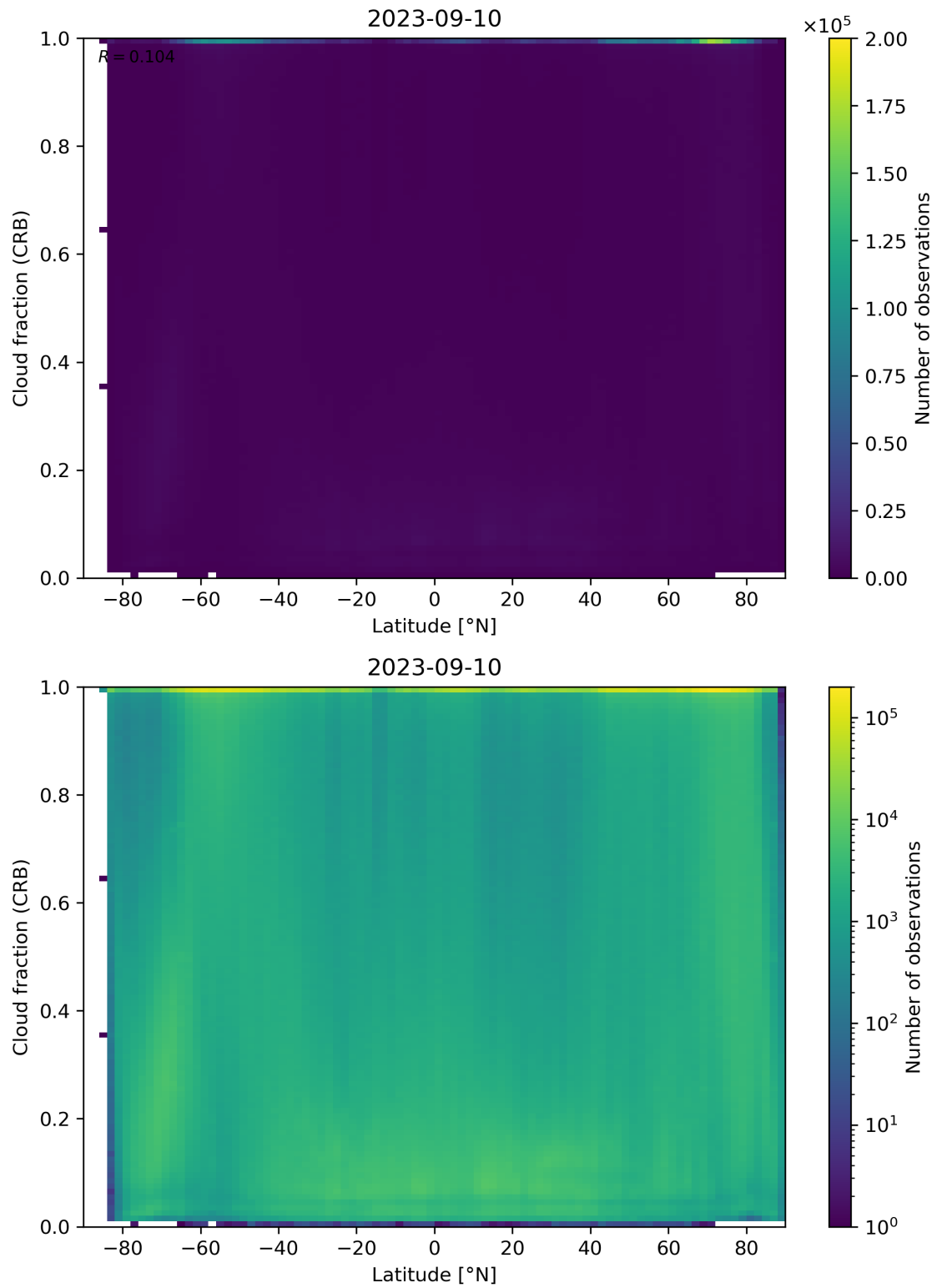
Figure 94: Scatter density plot of “Latitude” against “Cloud fraction (CRB)” for 2023-09-10 to 2023-09-11.
