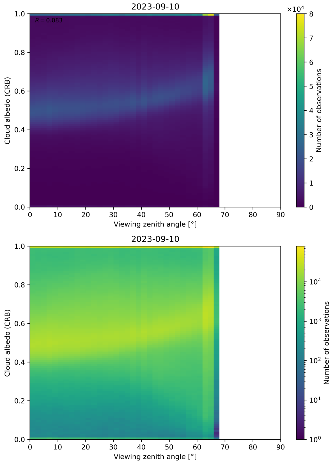
Figure 106: Scatter density plot of “Viewing zenith angle” against “Cloud albedo (CRB)” for 2023-09-10 to 2023-09-11.
