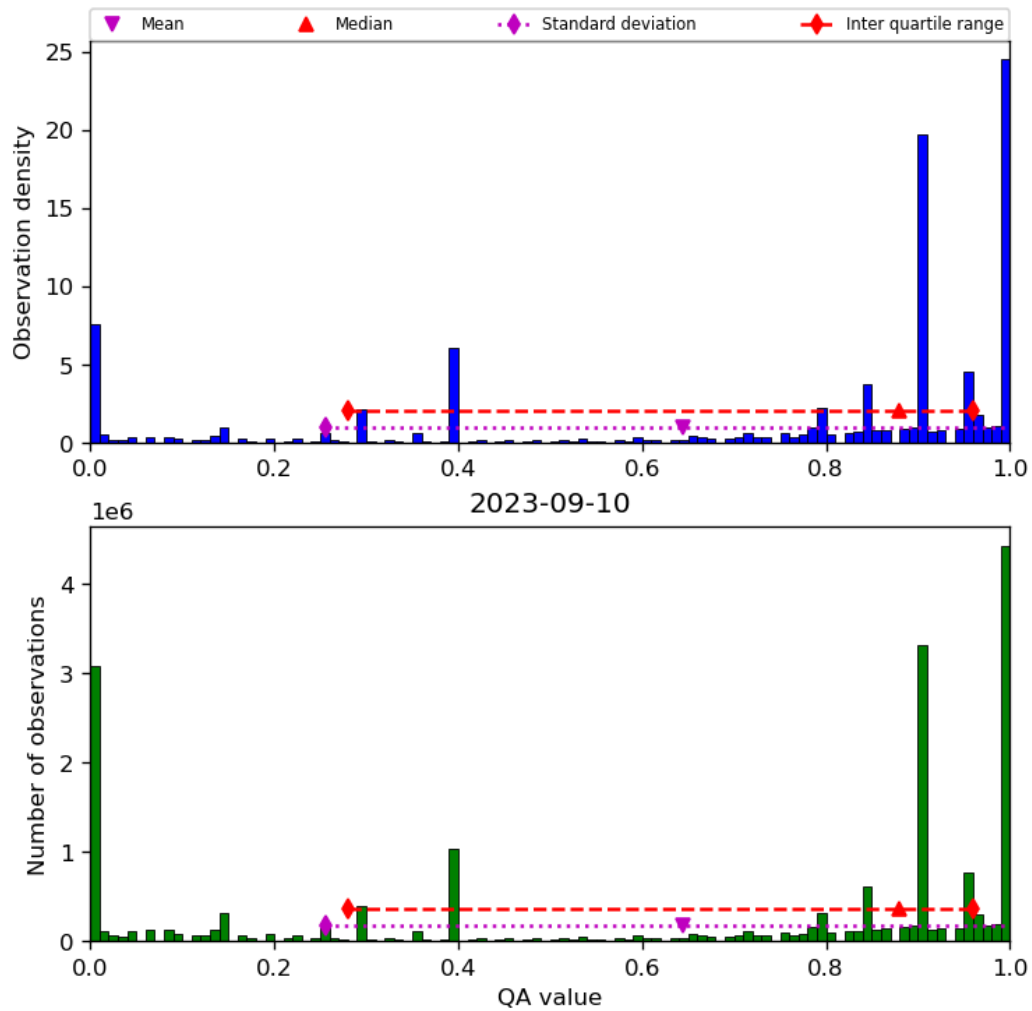
Figure 38: Histogram of “QA value” for 2023-09-10 to 2023-09-11
