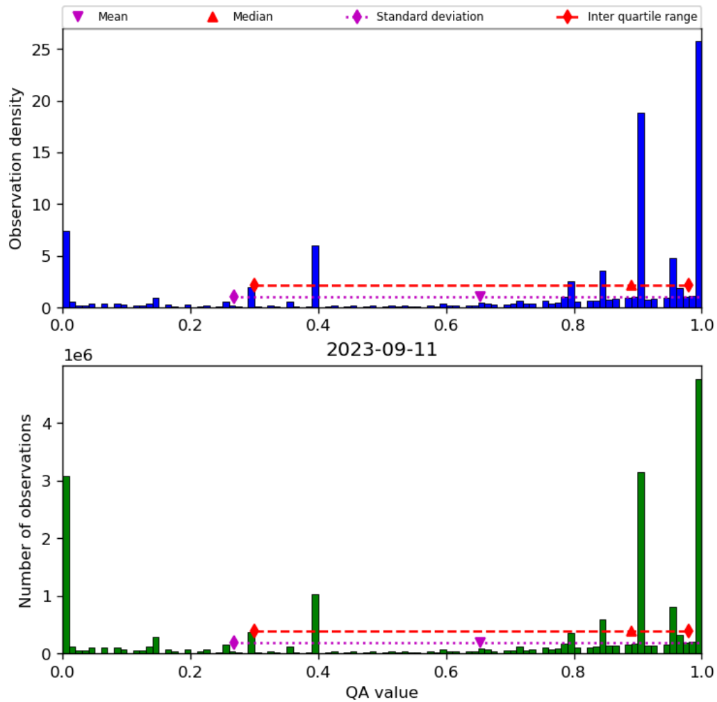
Figure 38: Histogram of “QA value” for 2023-09-10 to 2023-09-12
