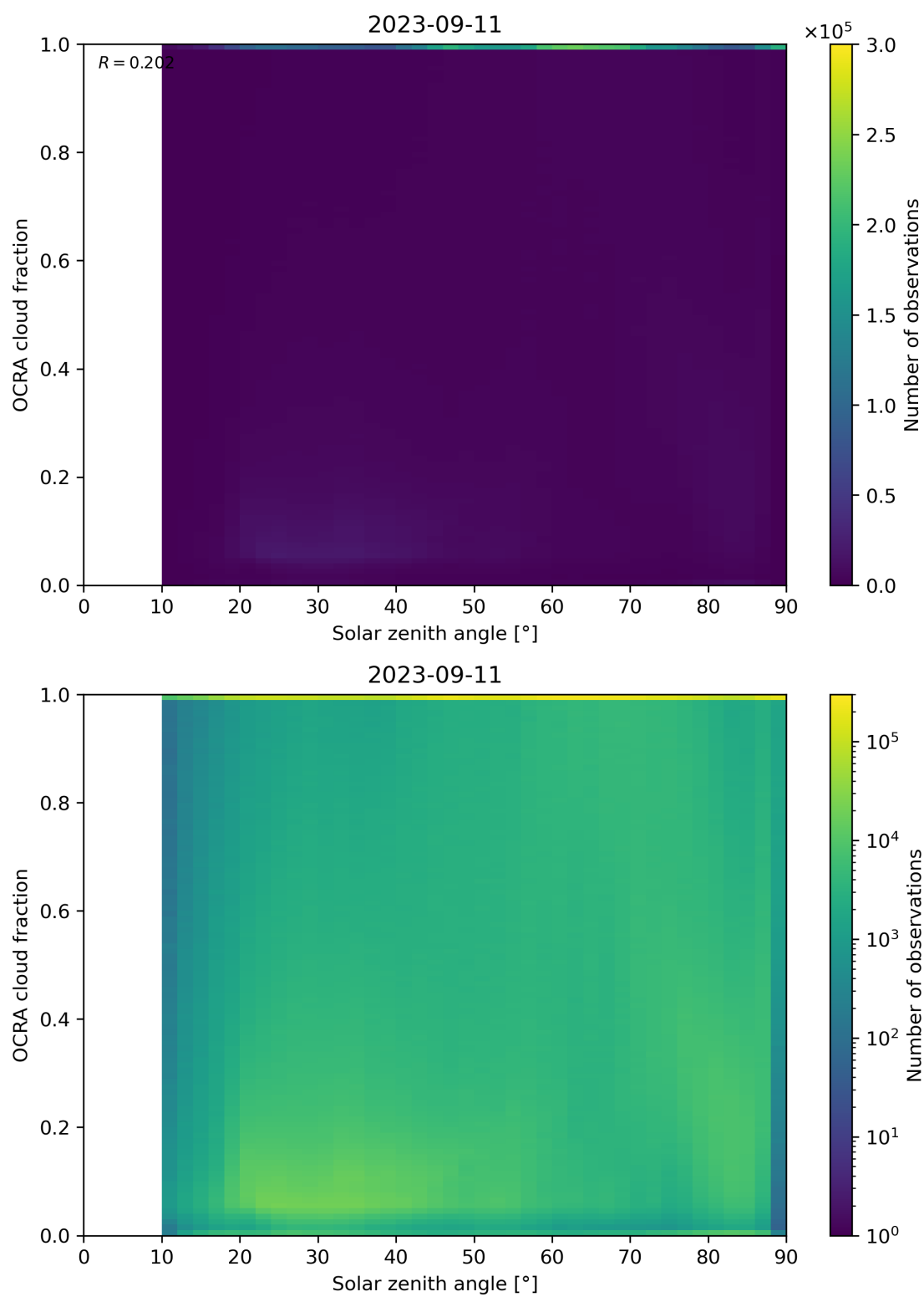
Figure 100: Scatter density plot of “Solar zenith angle” against “OCRA cloud fraction” for 2023-09-10 to 2023-09-12.
