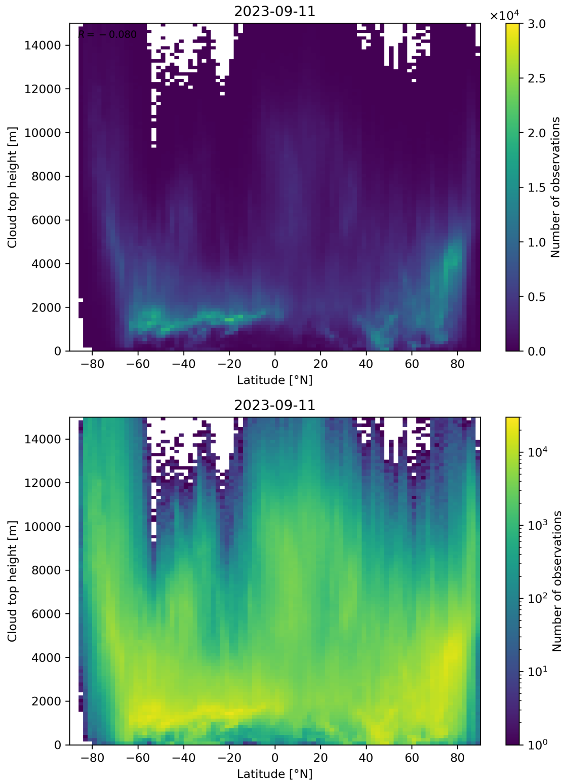
Figure 97: Scatter density plot of “Latitude” against “Cloud top height” for 2023-09-10 to 2023-09-12.
