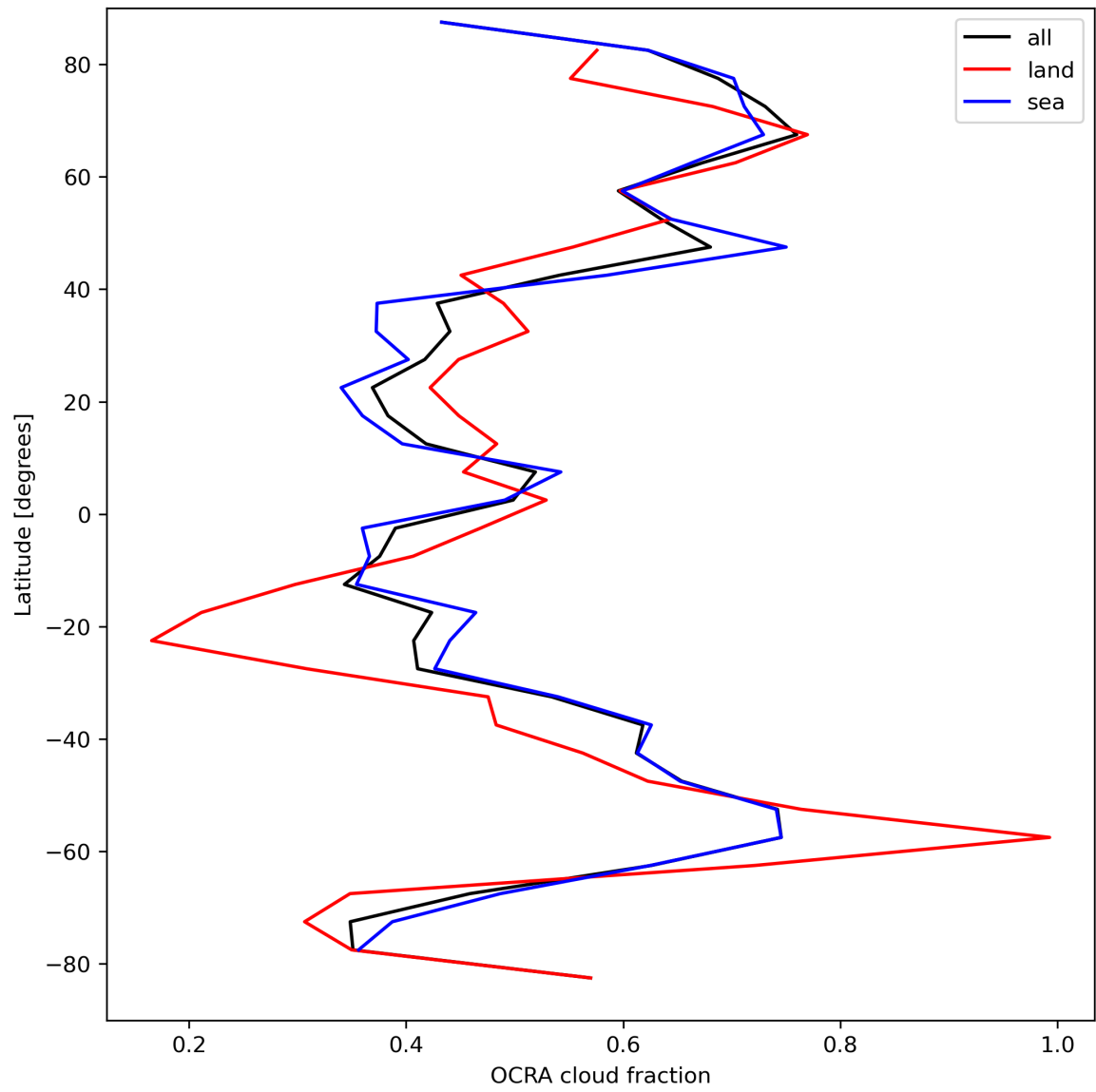
Figure 34: Zonal average of “OCRA cloud fraction” for 2023-09-10 to 2023-09-12.
