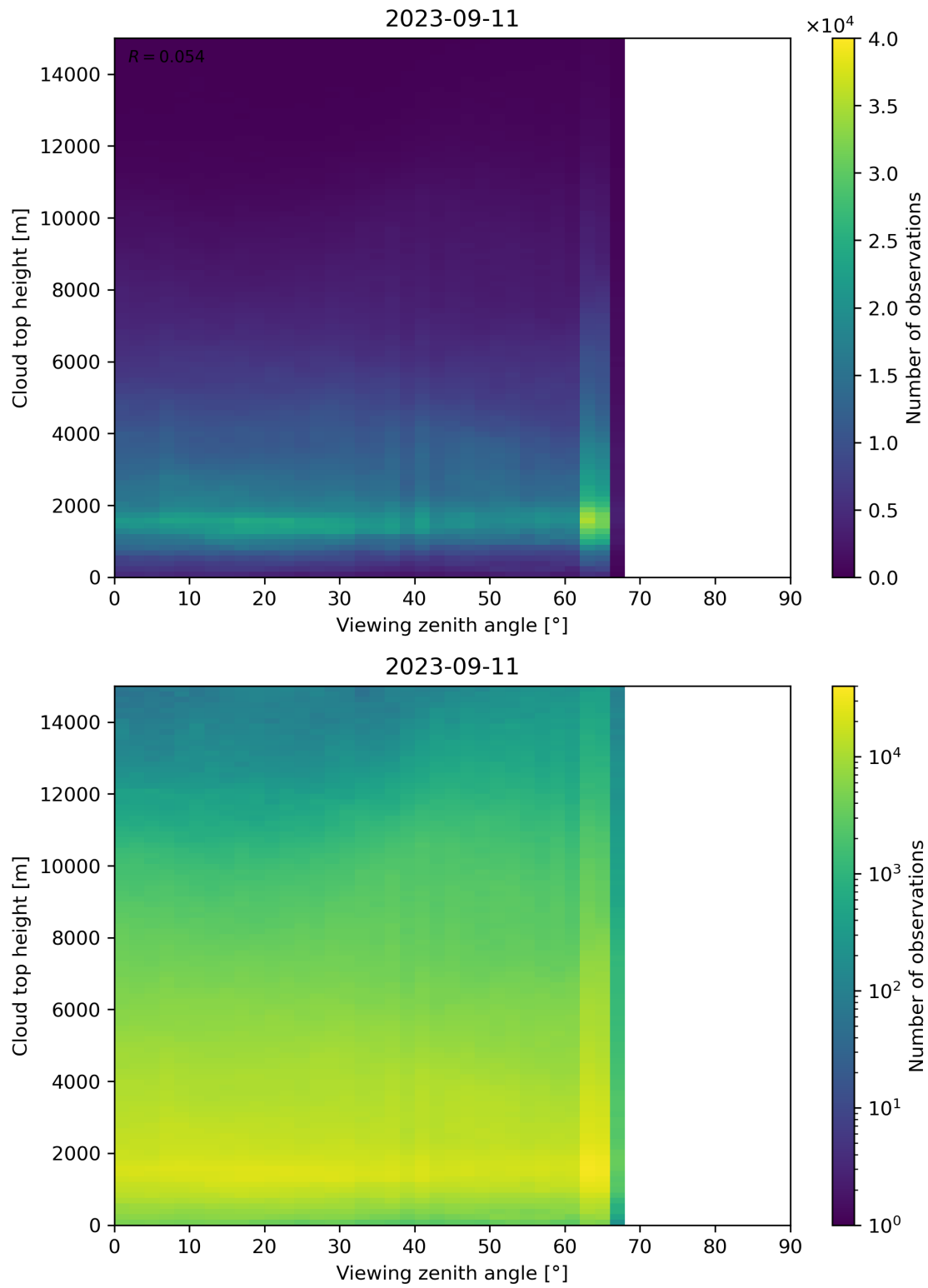
Figure 112: Scatter density plot of “Viewing zenith angle” against “Cloud top height” for 2023-09-10 to 2023-09-12.
