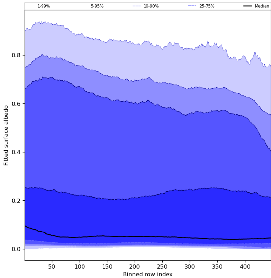
Figure 61: Along track statistics of “Fitted surface albedo” for 2023-09-10 to 2023-09-12
