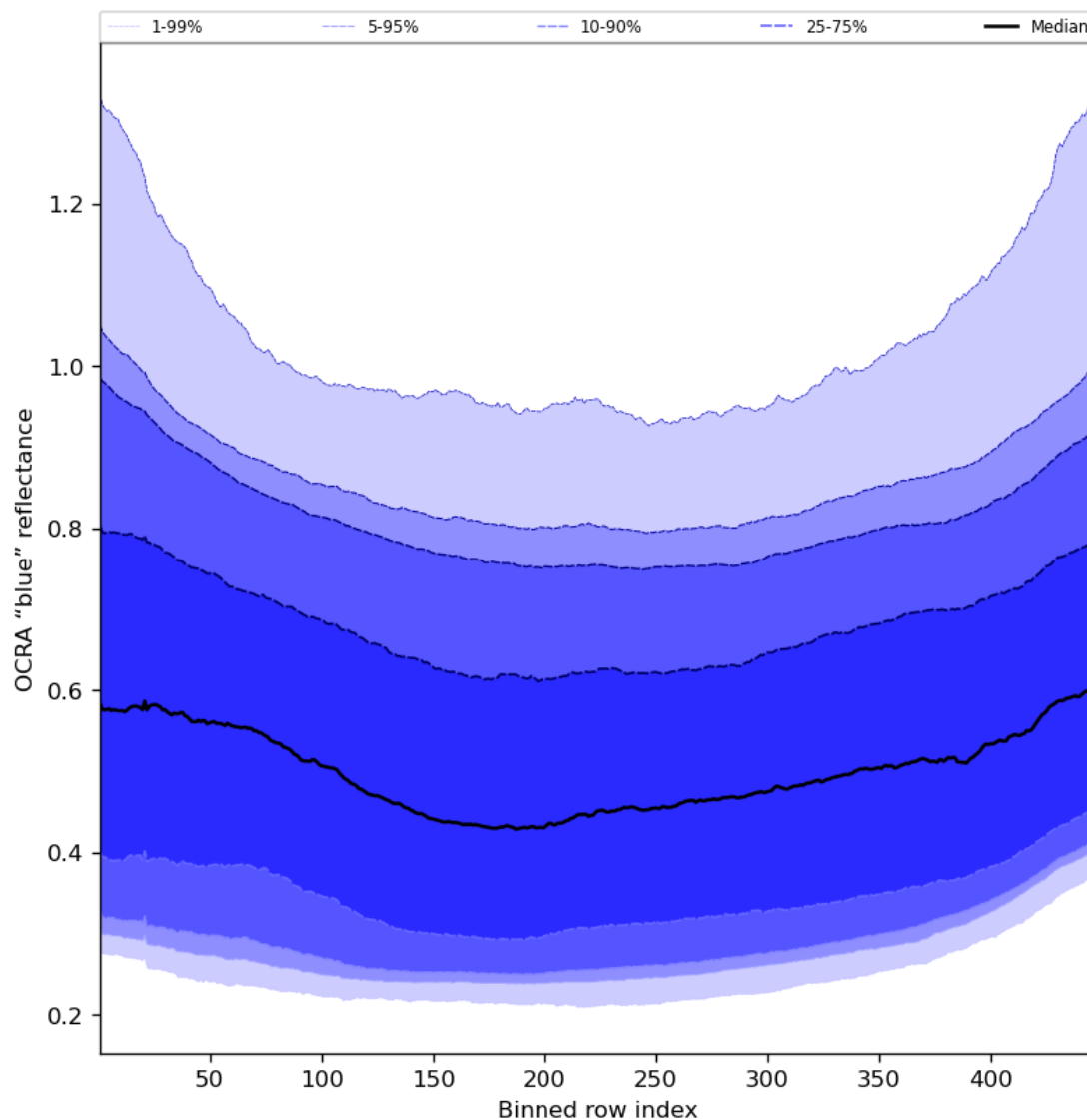
Figure 67: Along track statistics of “OCRA “blue” reflectance” for 2023-09-10 to 2023-09-12
