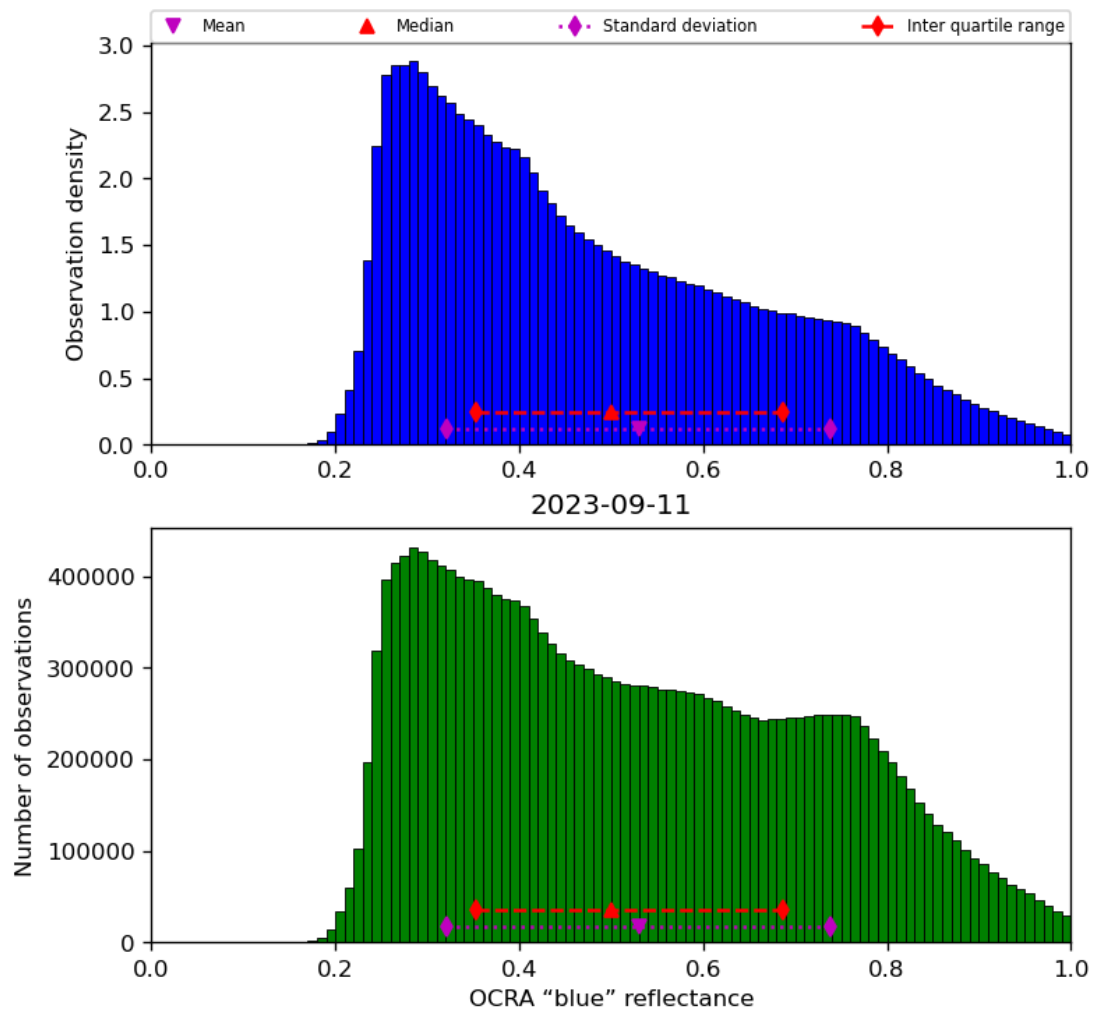
Figure 51: Histogram of “OCRA “blue” reflectance” for 2023-09-10 to 2023-09-12
