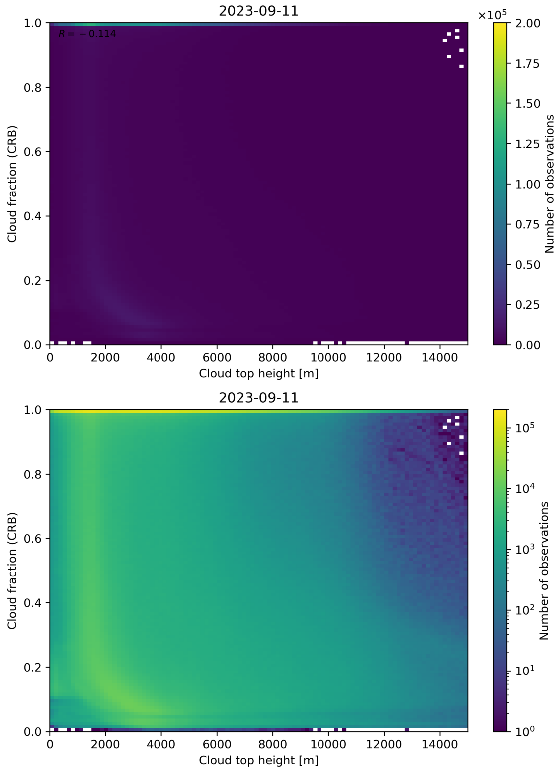
Figure 88: Scatter density plot of “Cloud top height” against “Cloud fraction (CRB)” for 2023-09-10 to 2023-09-12.
