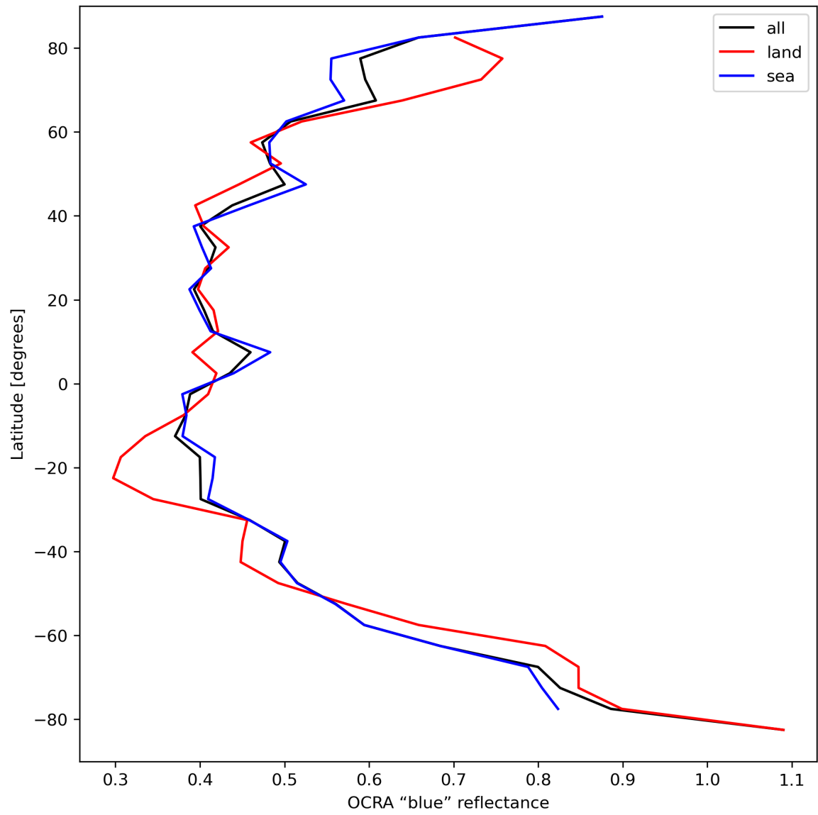
Figure 35: Zonal average of “OCRA “blue” reflectance” for 2023-09-10 to 2023-09-12.
