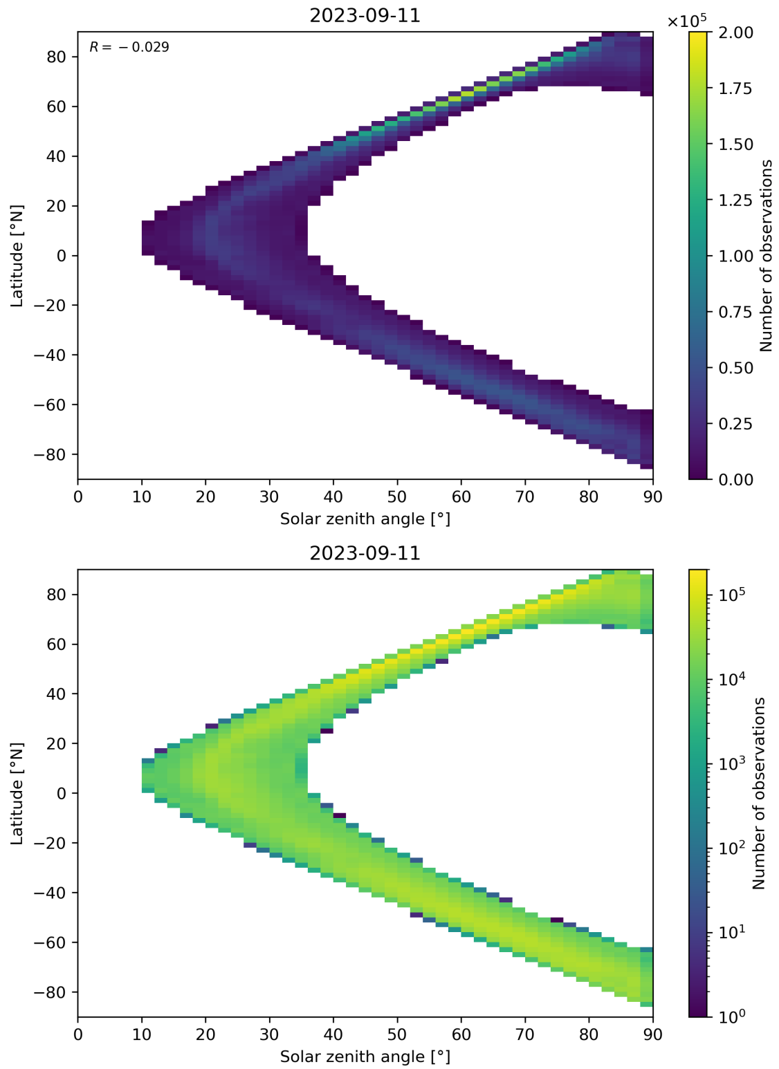
Figure 105: Scatter density plot of “Solar zenith angle” against “Latitude” for 2023-09-10 to 2023-09-12.
