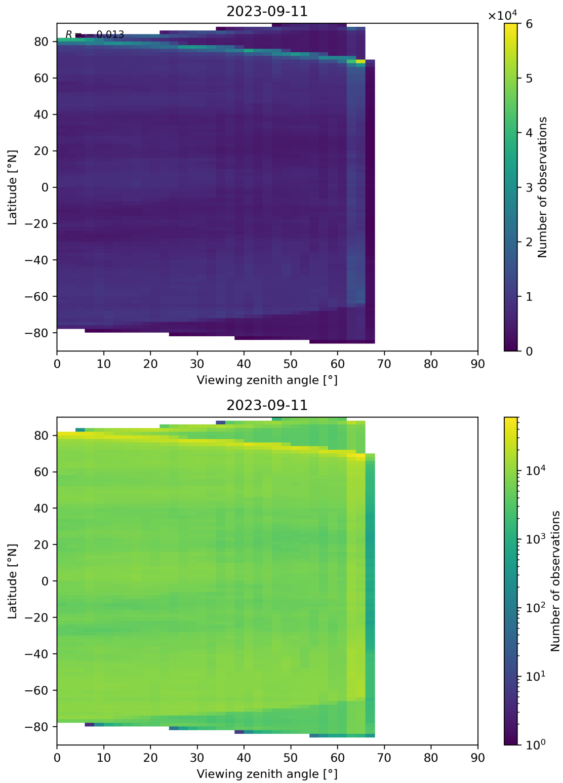
Figure 113: Scatter density plot of “Viewing zenith angle” against “Latitude” for 2023-09-10 to 2023-09-12.
