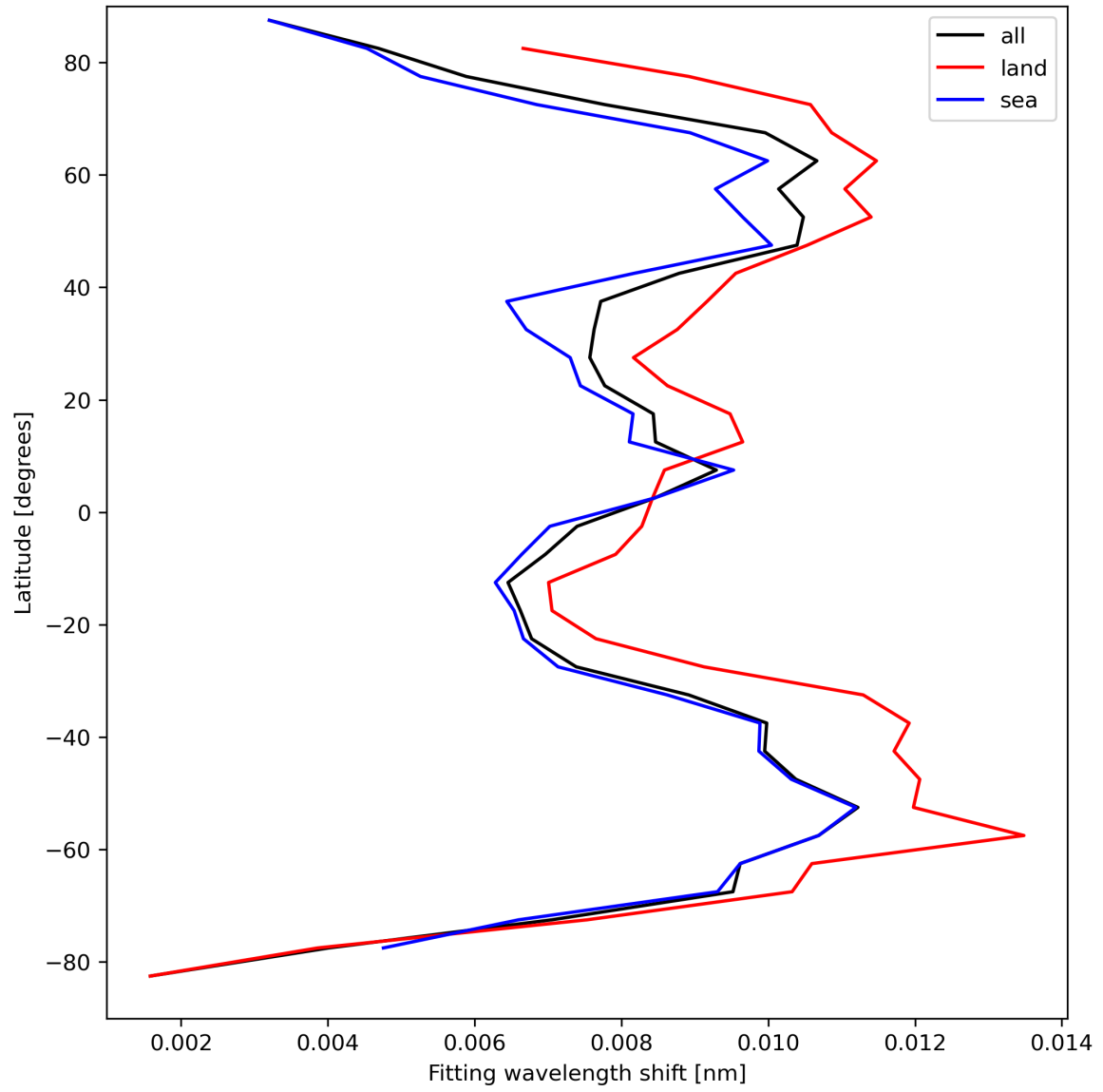
Figure 33: Zonal average of “Fitting wavelength shift” for 2023-09-10 to 2023-09-12.
