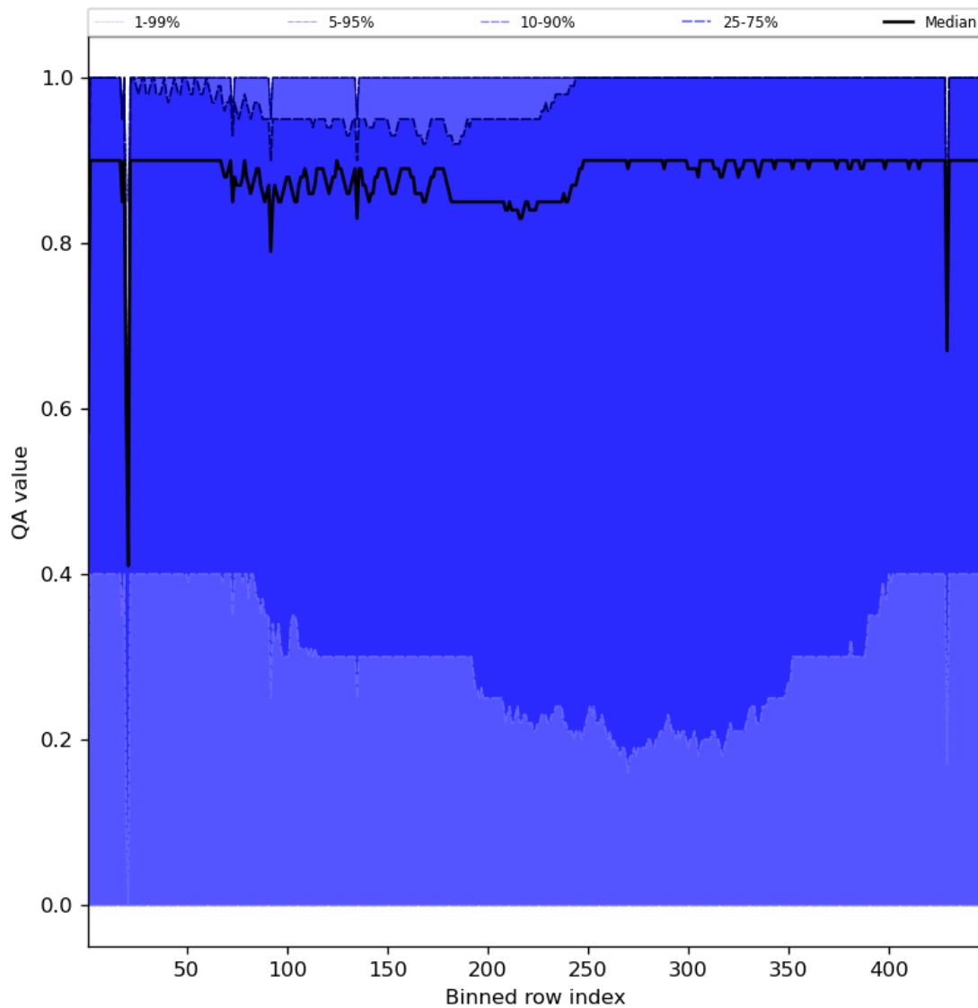
Figure 54: Along track statistics of “QA value” for 2023-09-10 to 2023-09-12
