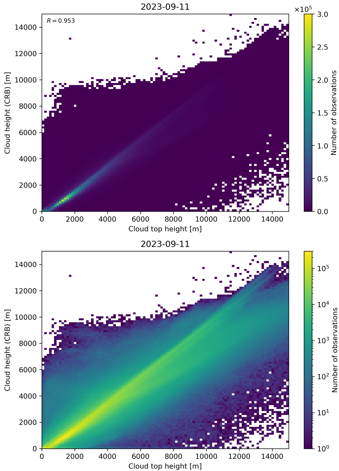
Figure 89: Scatter density plot of “Cloud top height” against “Cloud height (CRB)” for 2023-09-10 to 2023-09-12.
