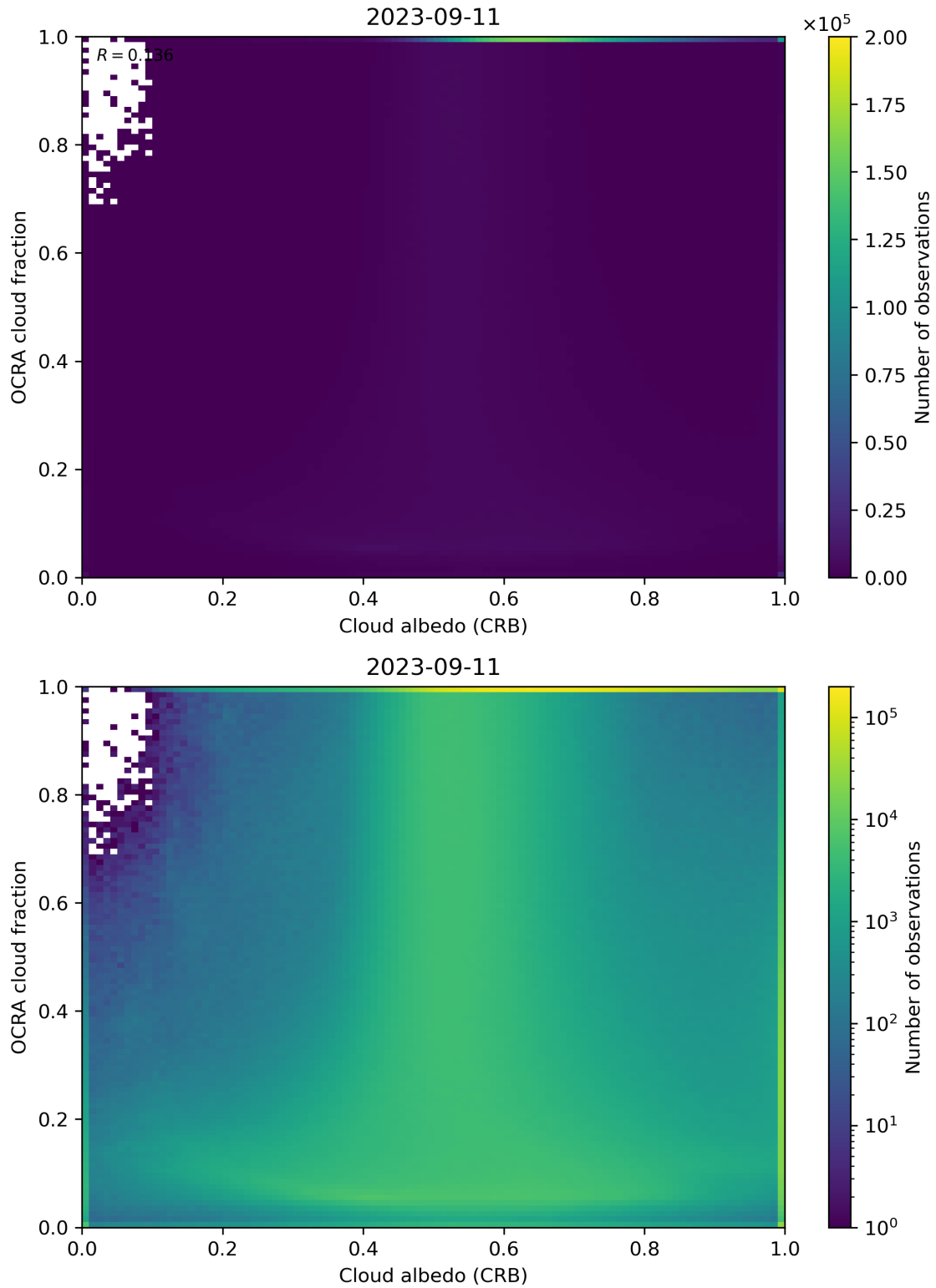
Figure 70: Scatter density plot of “Cloud albedo (CRB)” against “OCRA cloud fraction” for 2023-09-10 to 2023-09-12.
