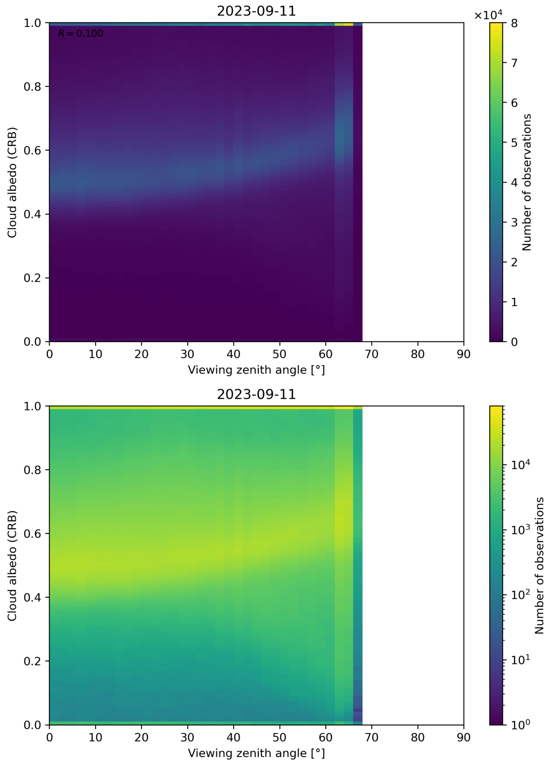
Figure 106: Scatter density plot of “Viewing zenith angle” against “Cloud albedo (CRB)” for 2023-09-10 to 2023-09-12.
