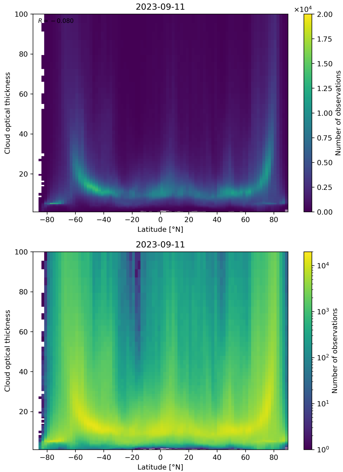
Figure 96: Scatter density plot of “Latitude” against “Cloud optical thickness” for 2023-09-10 to 2023-09-12.
