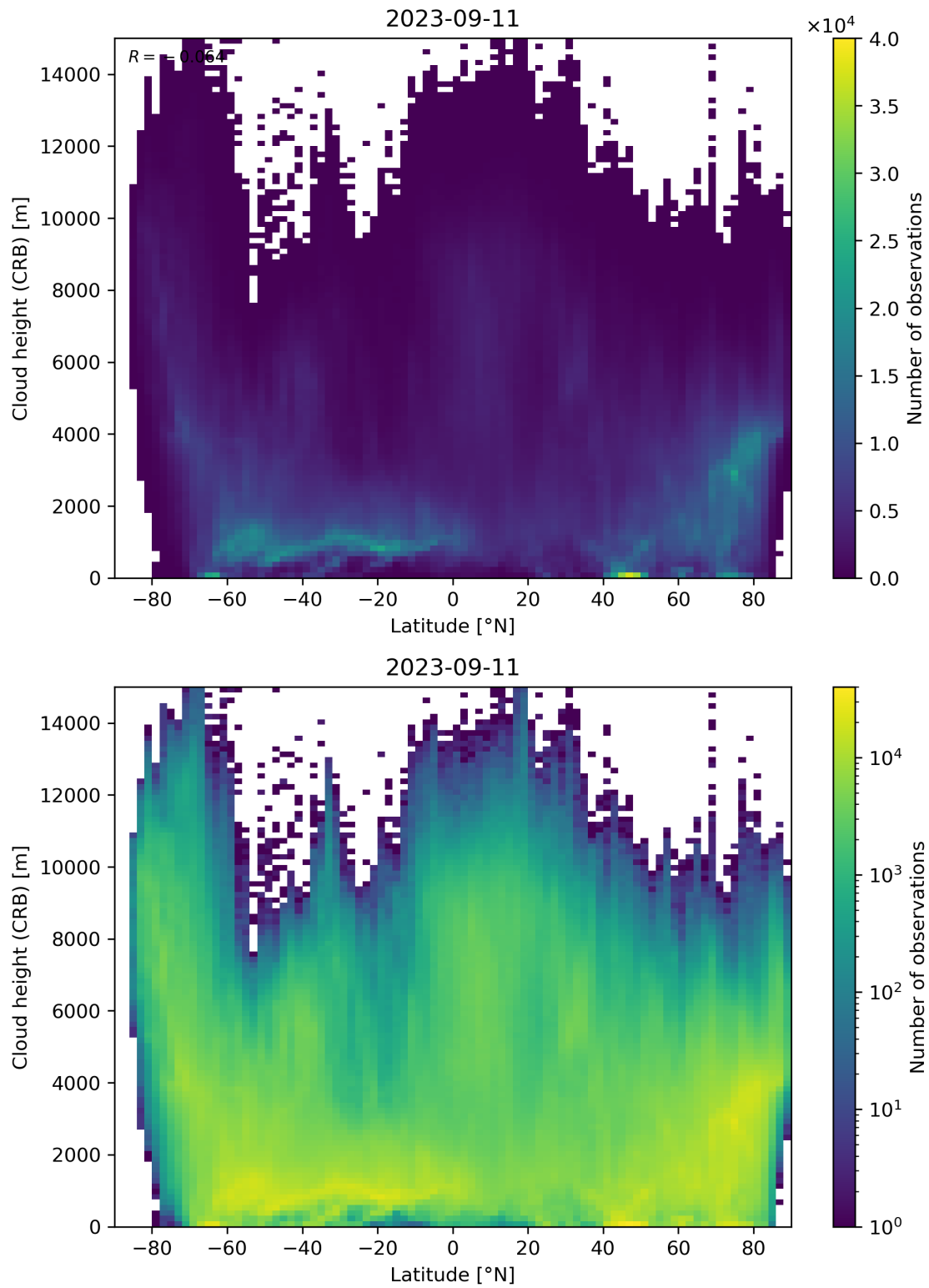
Figure 95: Scatter density plot of “Latitude” against “Cloud height (CRB)” for 2023-09-10 to 2023-09-12.
