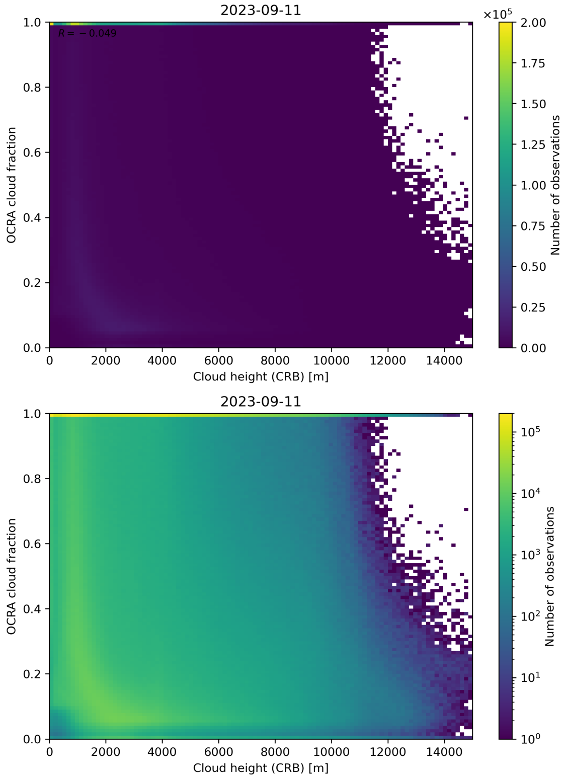
Figure 81: Scatter density plot of “Cloud height (CRB)” against “OCRA cloud fraction” for 2023-09-10 to 2023-09-12.
