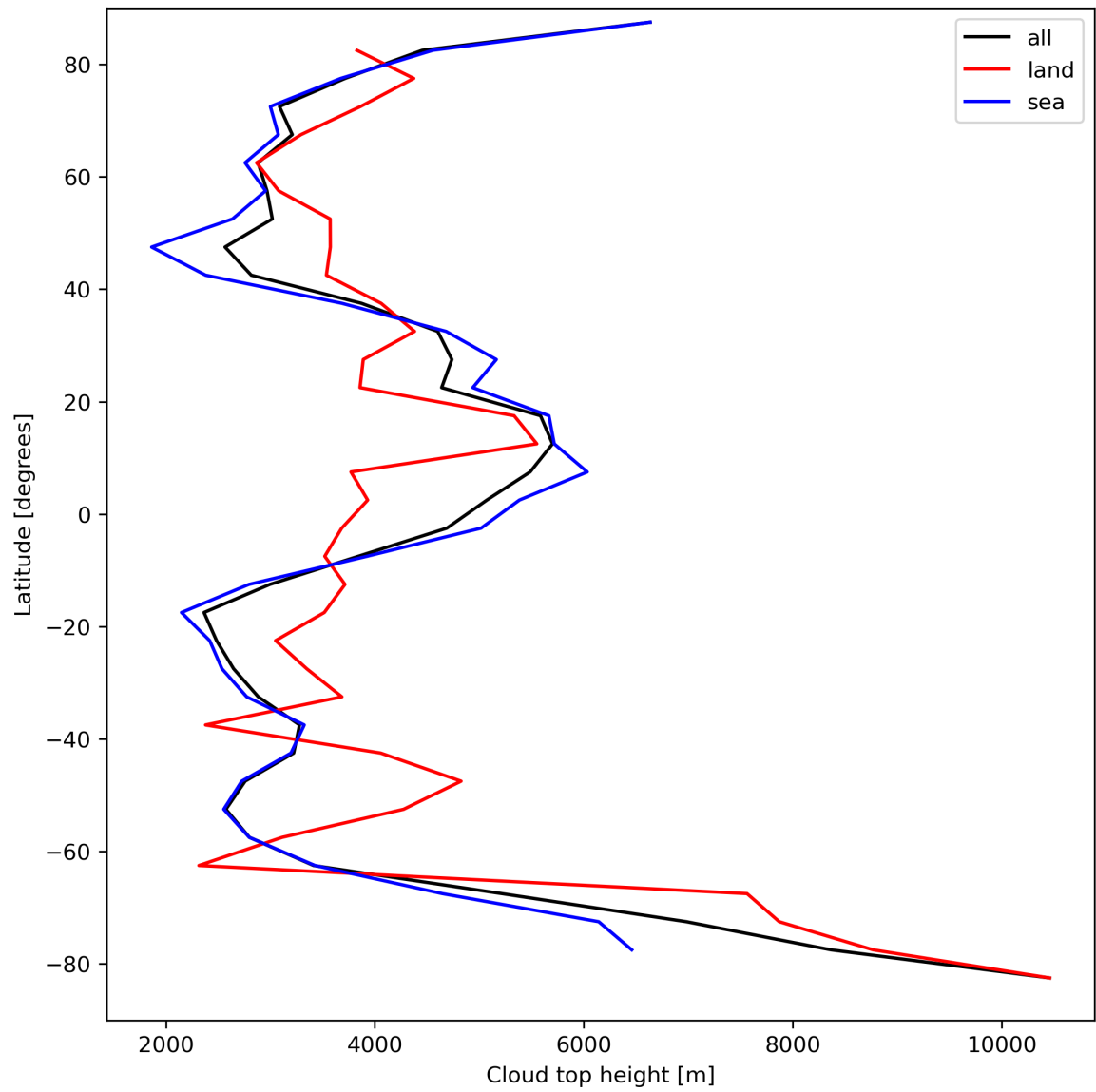
Figure 24: Zonal average of “Cloud top height” for 2023-09-10 to 2023-09-12.
