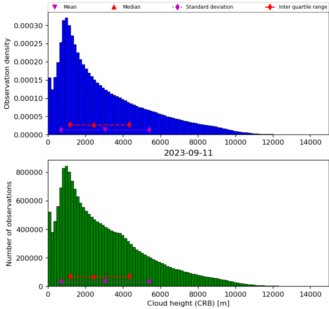
Figure 43: Histogram of “Cloud height (CRB)” for 2023-09-10 to 2023-09-12
