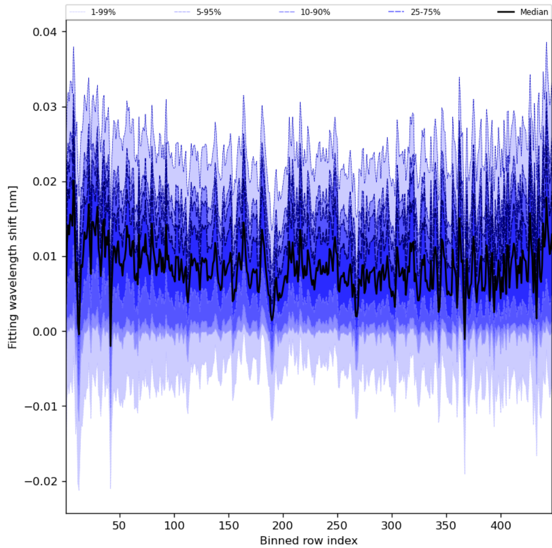
Figure 65: Along track statistics of “Fitting wavelength shift” for 2023-09-10 to 2023-09-12
