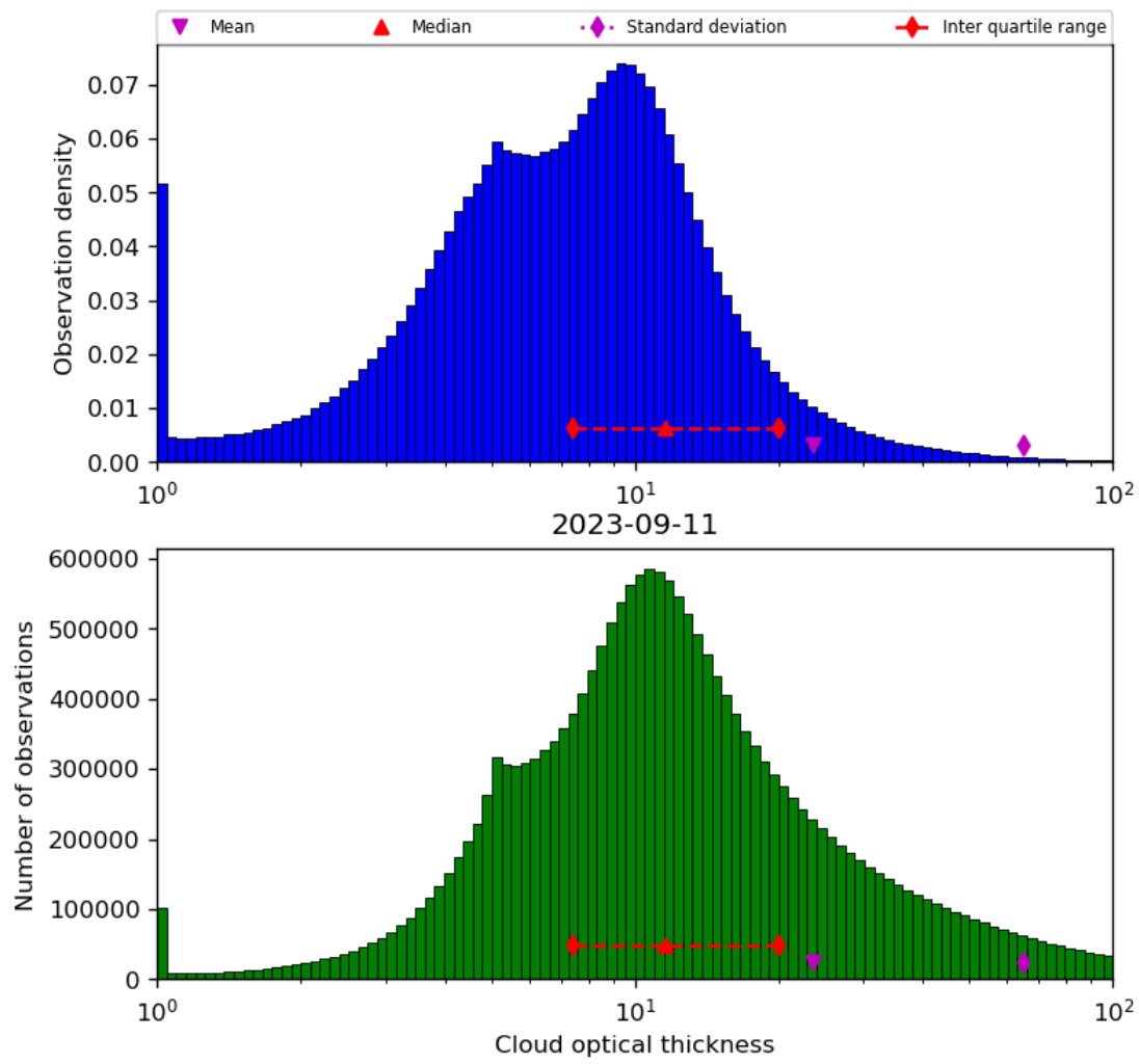
Figure 41: Histogram of “Cloud optical thickness” for 2023-09-10 to 2023-09-12
