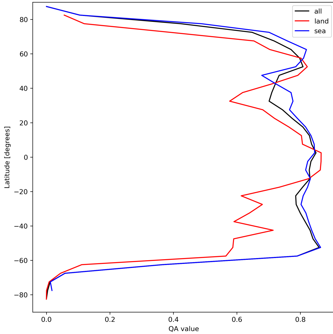
Figure 22: Zonal average of “QA value” for 2023-09-10 to 2023-09-12.
