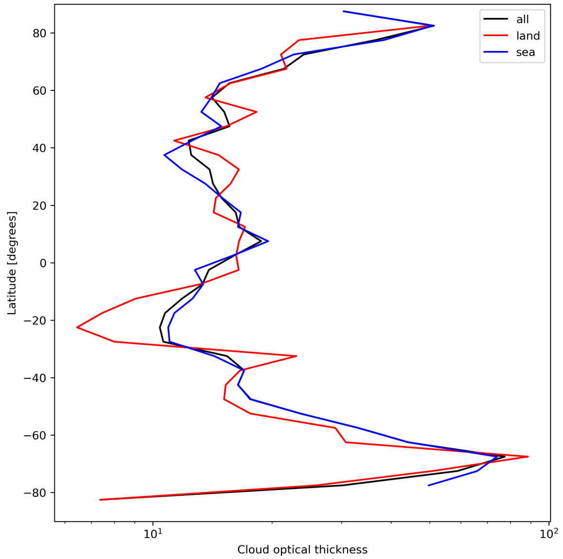
Figure 25: Zonal average of “Cloud optical thickness” for 2023-09-10 to 2023-09-12.
