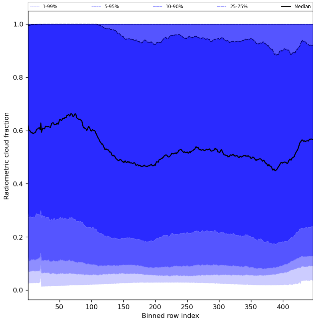
Figure 55: Along track statistics of “Radiometric cloud fraction” for 2023-09-10 to 2023-09-12
