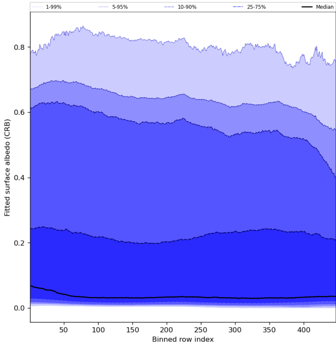
Figure 62: Along track statistics of “Fitted surface albedo (CRB)” for 2023-09-10 to 2023-09-12
