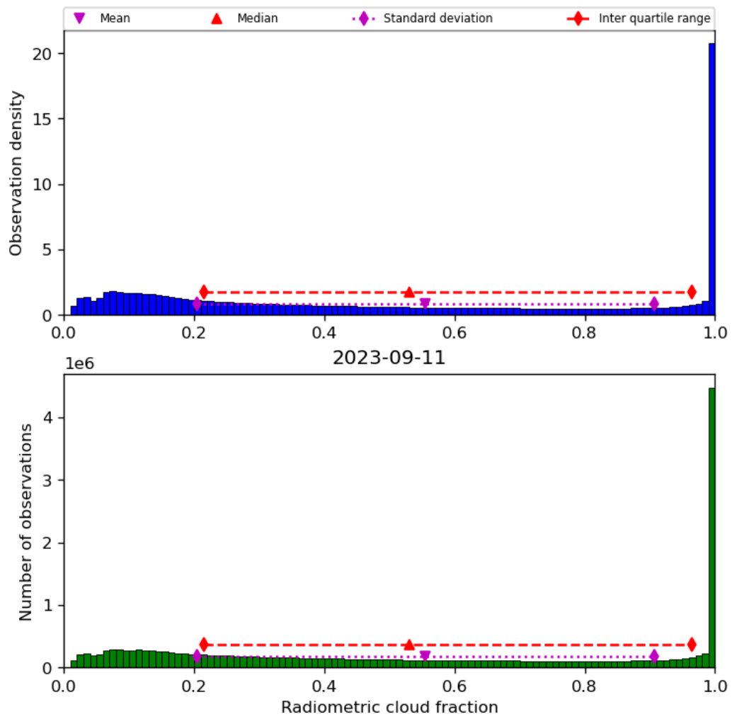
Figure 39: Histogram of “Radiometric cloud fraction” for 2023-09-10 to 2023-09-12
