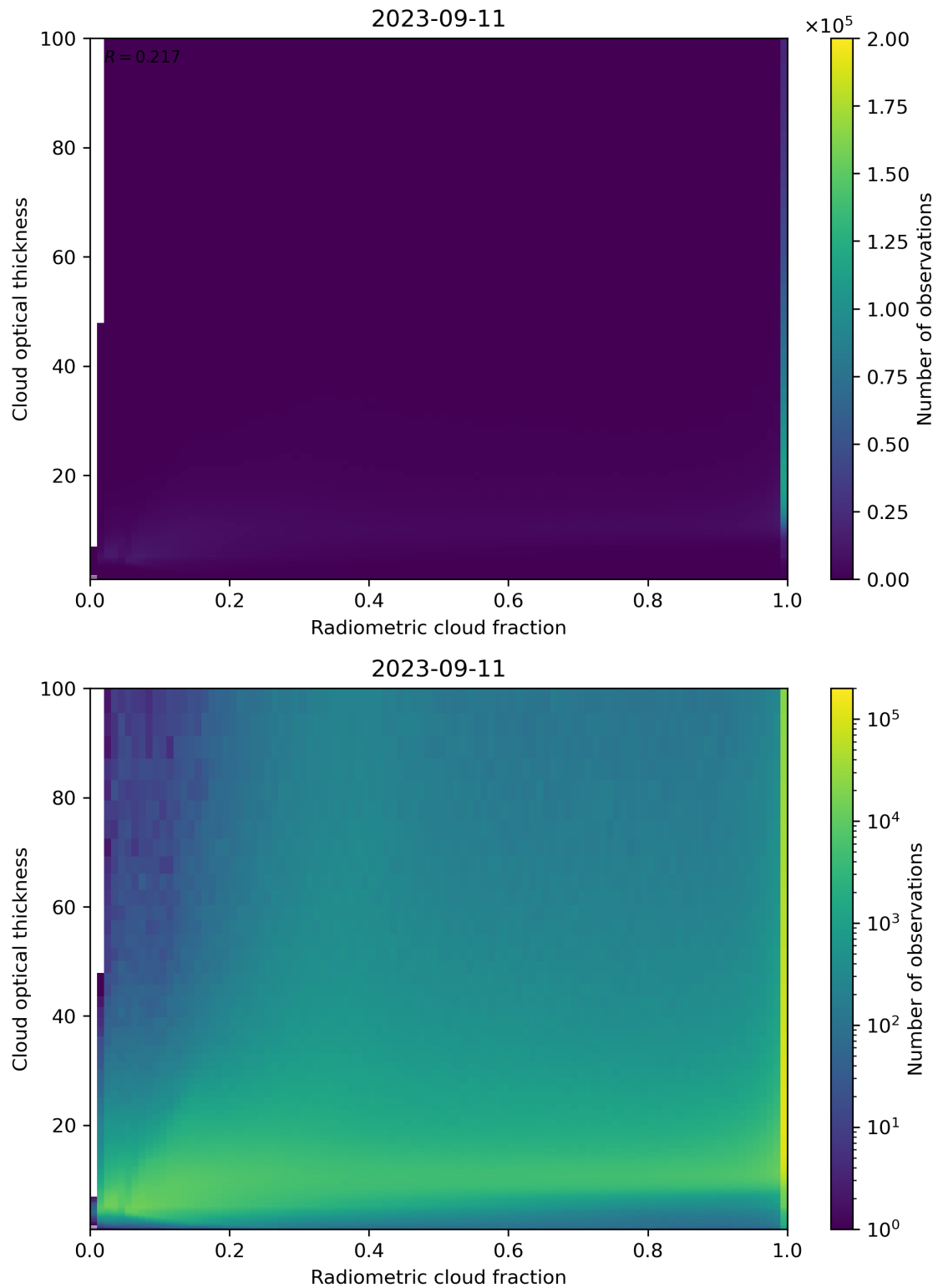
Figure 75: Scatter density plot of “Radiometric cloud fraction” against “Cloud optical thickness” for 2023-09-10 to 2023-09-12.
