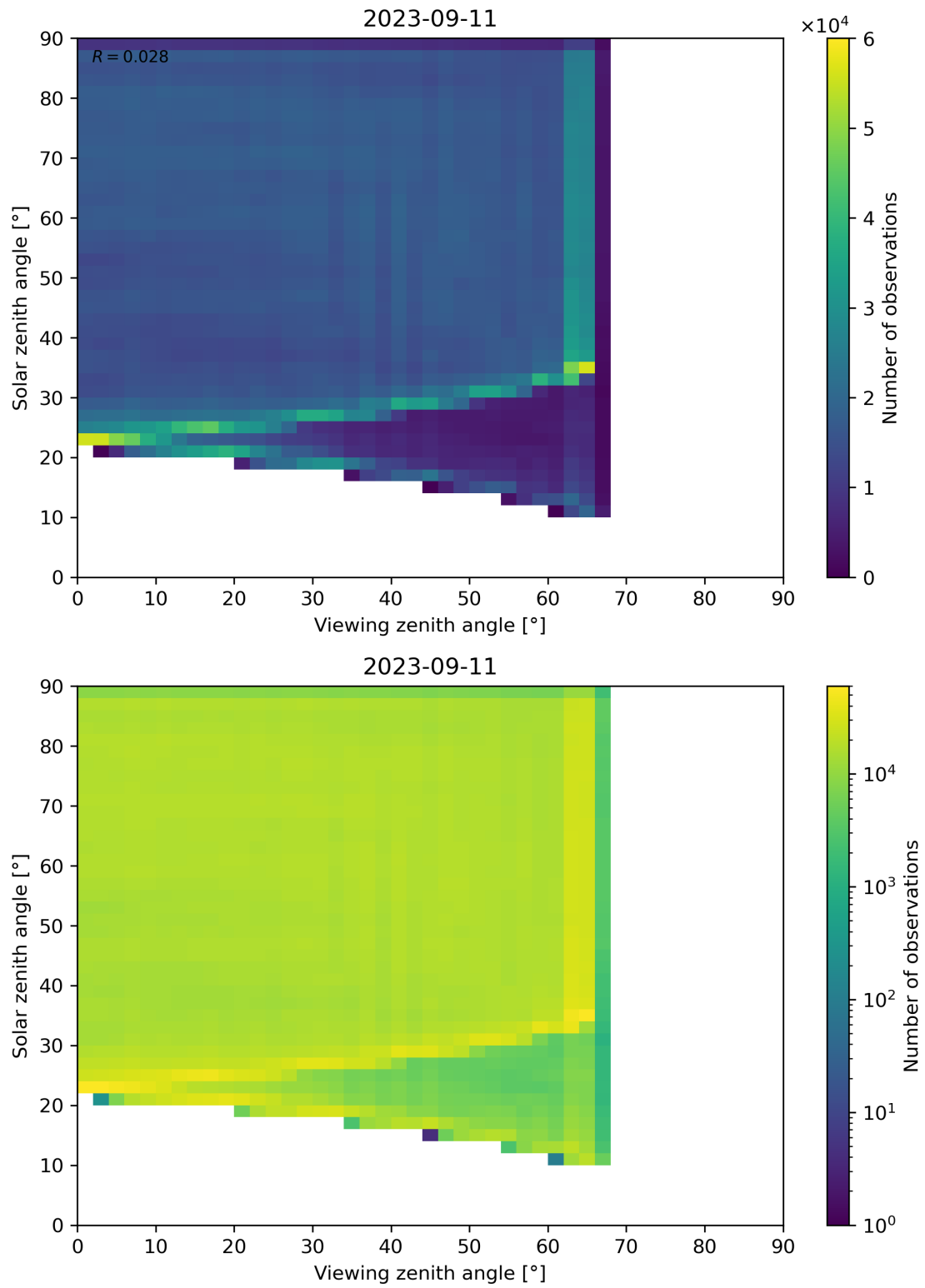
Figure 114: Scatter density plot of “Viewing zenith angle” against “Solar zenith angle” for 2023-09-10 to 2023-09-12.
