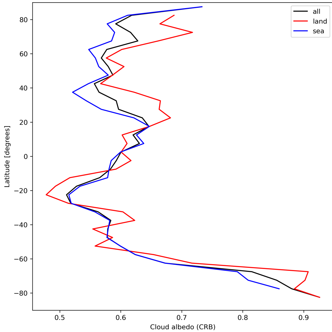
Figure 28: Zonal average of “Cloud albedo (CRB)” for 2023-09-10 to 2023-09-12.
