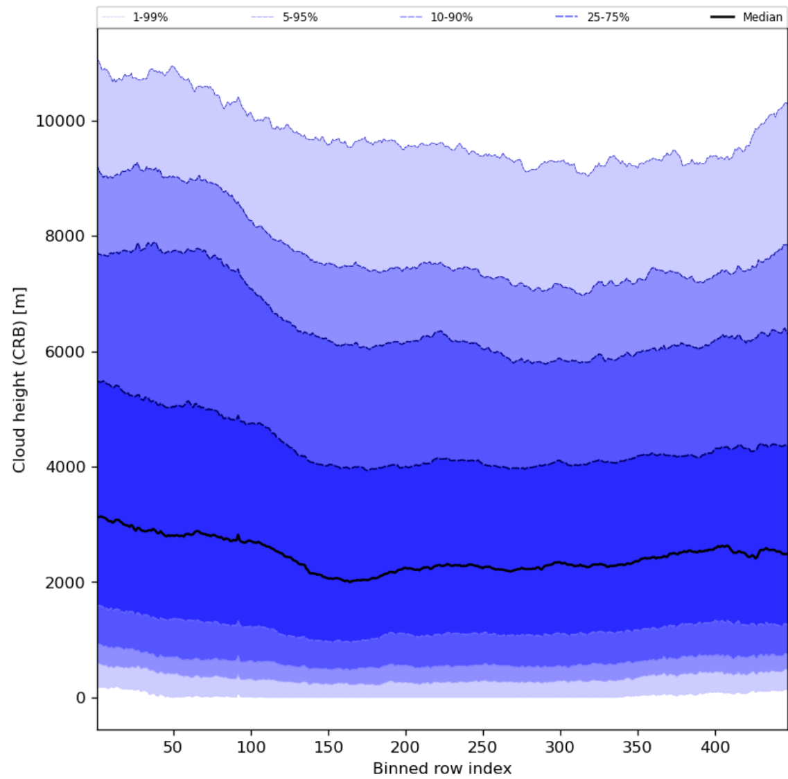
Figure 59: Along track statistics of “Cloud height (CRB)” for 2023-09-10 to 2023-09-12
