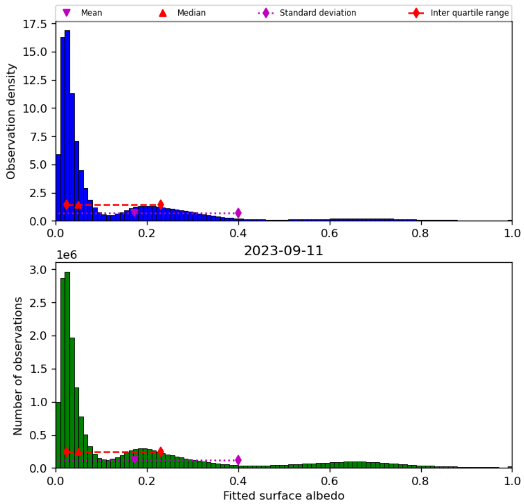
Figure 45: Histogram of “Fitted surface albedo” for 2023-09-10 to 2023-09-12
