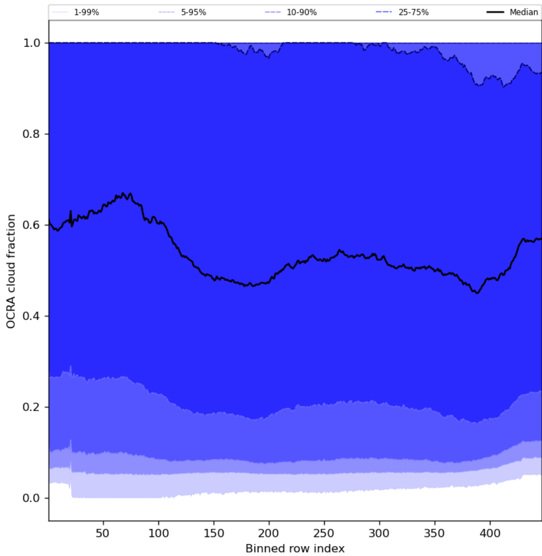
Figure 66: Along track statistics of “OCRA cloud fraction” for 2023-09-10 to 2023-09-12
