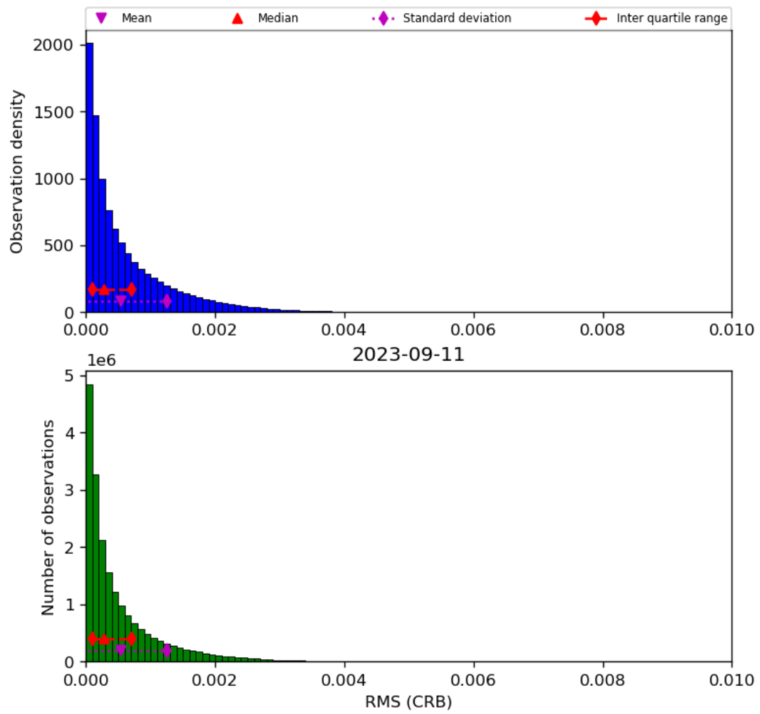
Figure 48: Histogram of “RMS (CRB)” for 2023-09-10 to 2023-09-12
