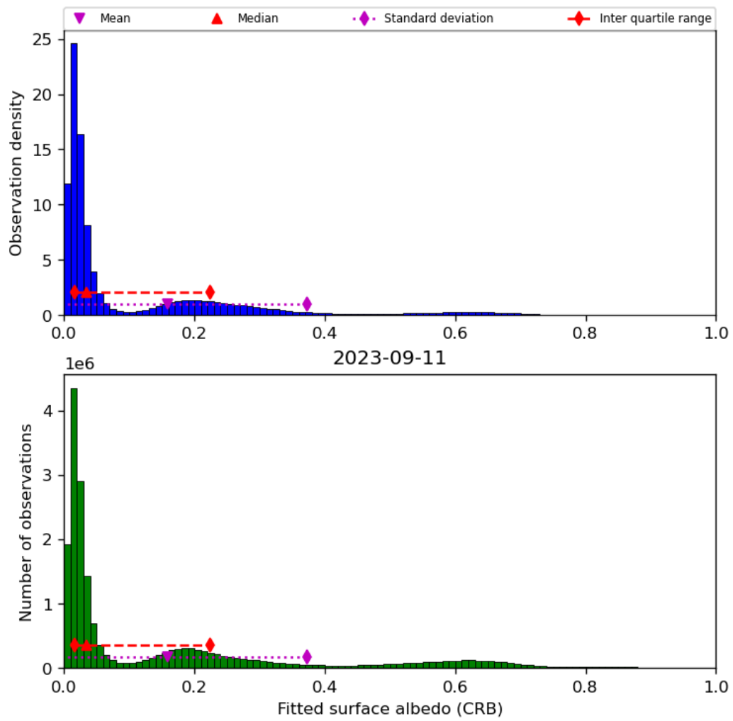
Figure 46: Histogram of “Fitted surface albedo (CRB)” for 2023-09-10 to 2023-09-12
