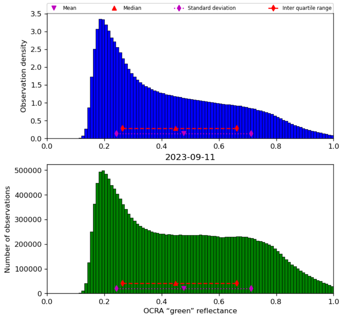
Figure 52: Histogram of “OCRA “green” reflectance” for 2023-09-10 to 2023-09-12
