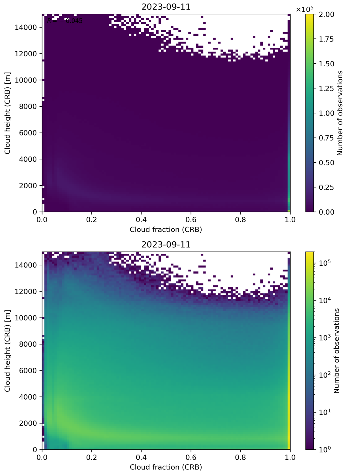
Figure 79: Scatter density plot of “Cloud fraction (CRB)” against “Cloud height (CRB)” for 2023-09-10 to 2023-09-12.
