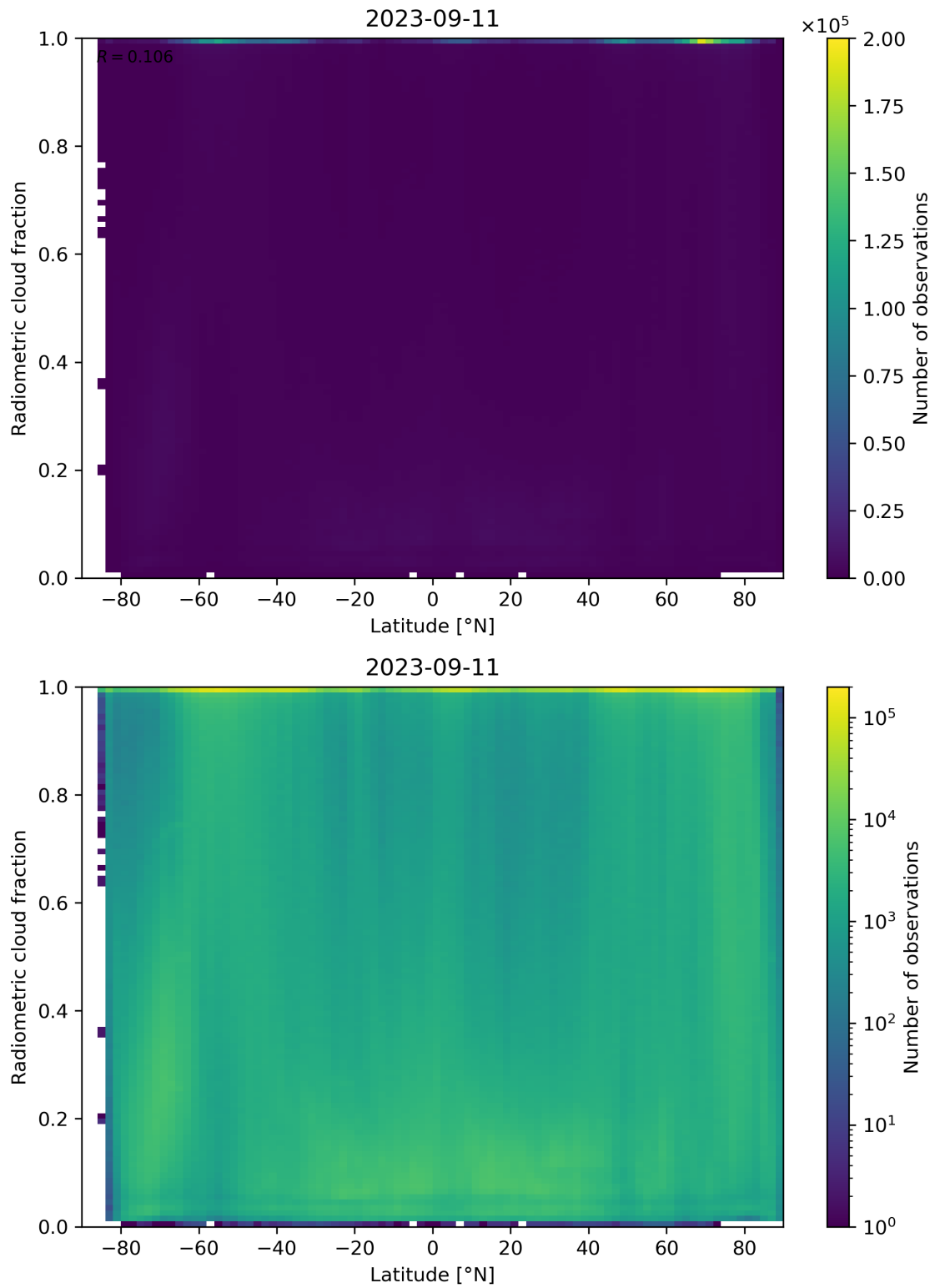
Figure 92: Scatter density plot of “Latitude” against “Radiometric cloud fraction” for 2023-09-10 to 2023-09-12.
