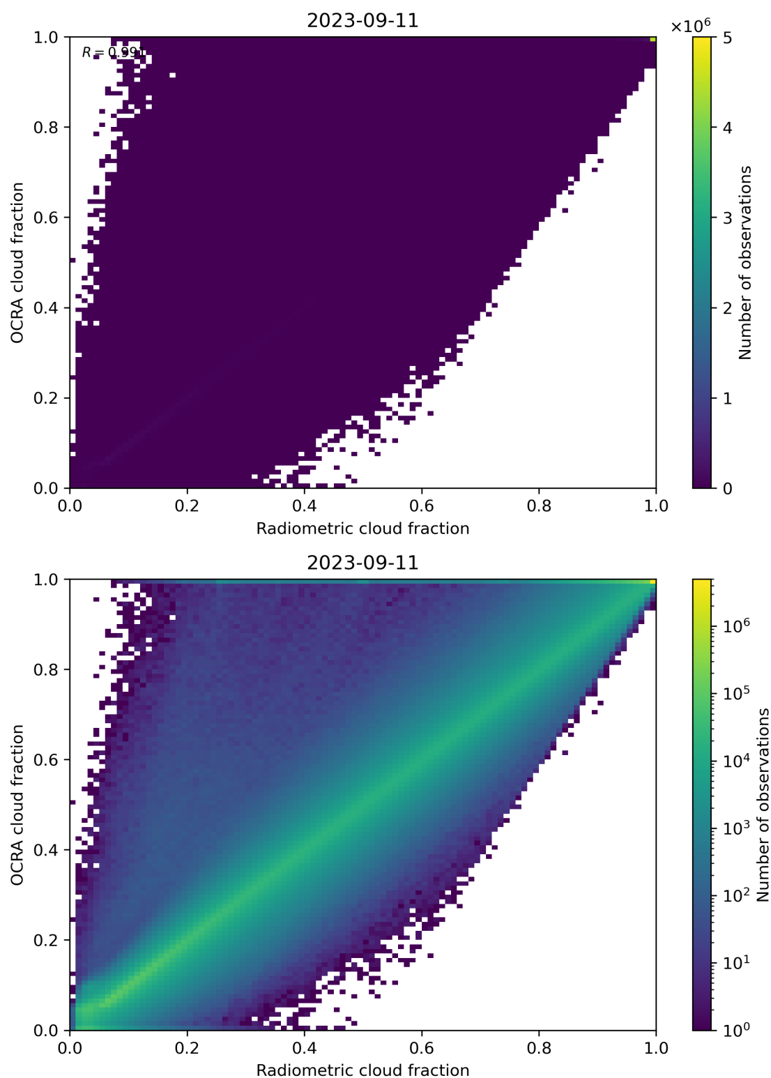
Figure 72: Scatter density plot of “Radiometric cloud fraction” against “OCRA cloud fraction” for 2023-09-10 to 2023-09-12.
