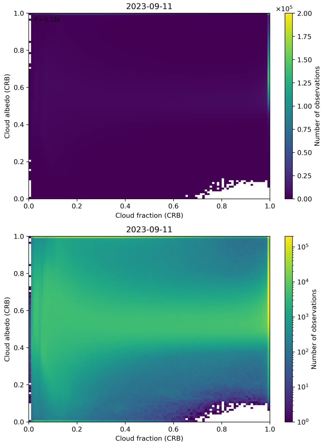
Figure 77: Scatter density plot of “Cloud fraction (CRB)” against “Cloud albedo (CRB)” for 2023-09-10 to 2023-09-12.
