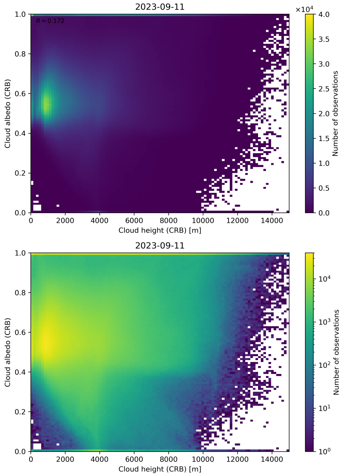
Figure 80: Scatter density plot of “Cloud height (CRB)” against “Cloud albedo (CRB)” for 2023-09-10 to 2023-09-12.
