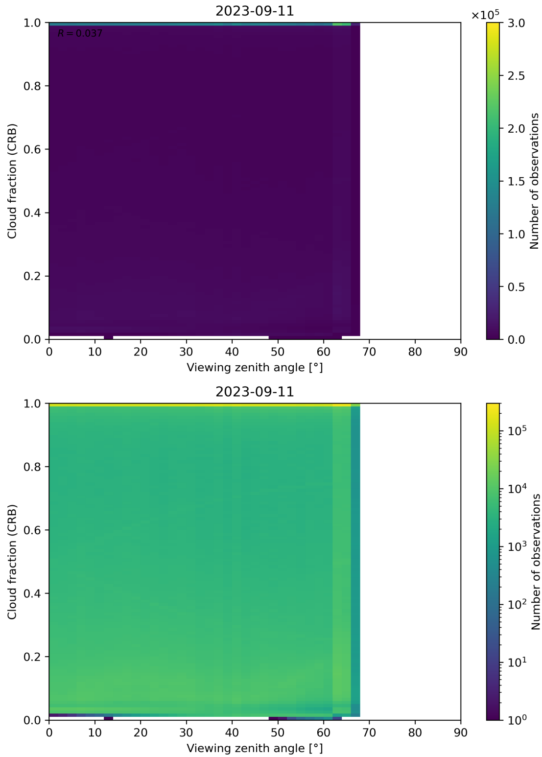
Figure 109: Scatter density plot of “Viewing zenith angle” against “Cloud fraction (CRB)” for 2023-09-10 to 2023-09-12.
