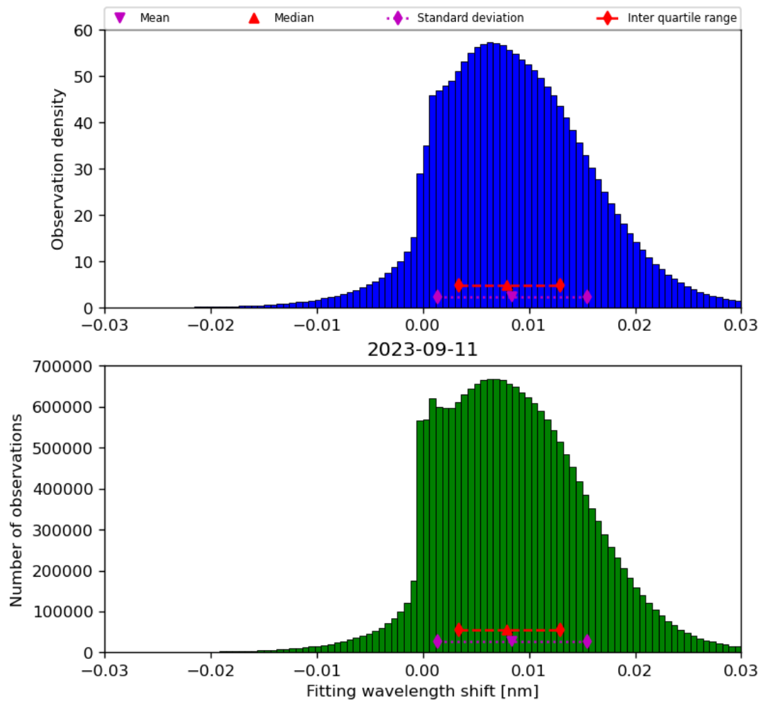
Figure 49: Histogram of “Fitting wavelength shift” for 2023-09-10 to 2023-09-12
