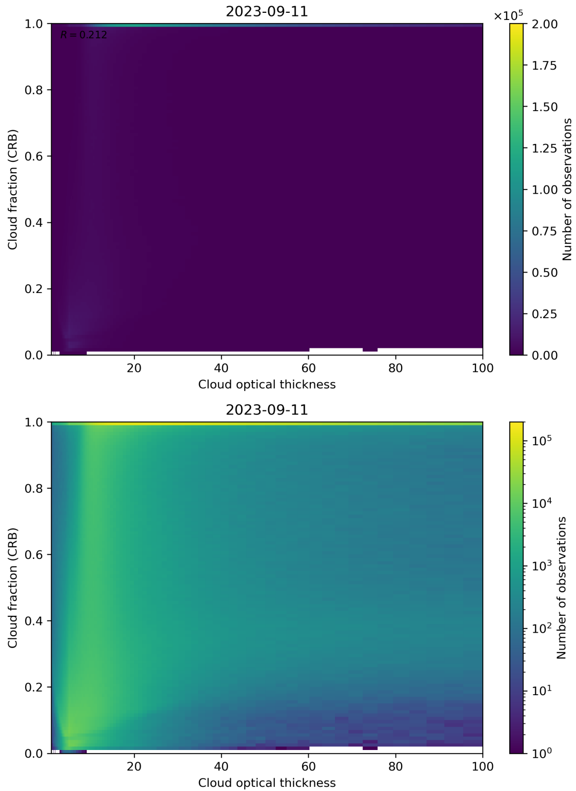
Figure 84: Scatter density plot of “Cloud optical thickness” against “Cloud fraction (CRB)” for 2023-09-10 to 2023-09-12.
