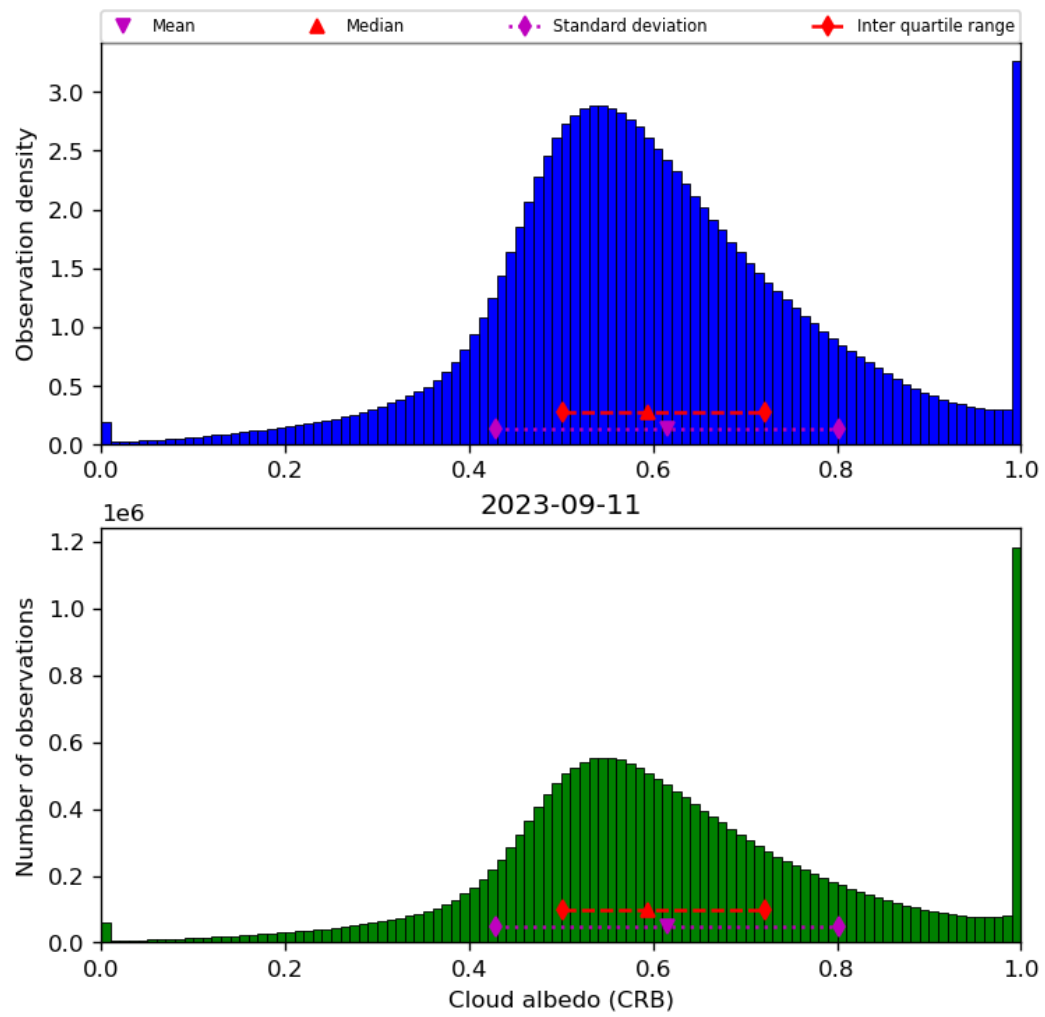
Figure 44: Histogram of “Cloud albedo (CRB)” for 2023-09-10 to 2023-09-12
