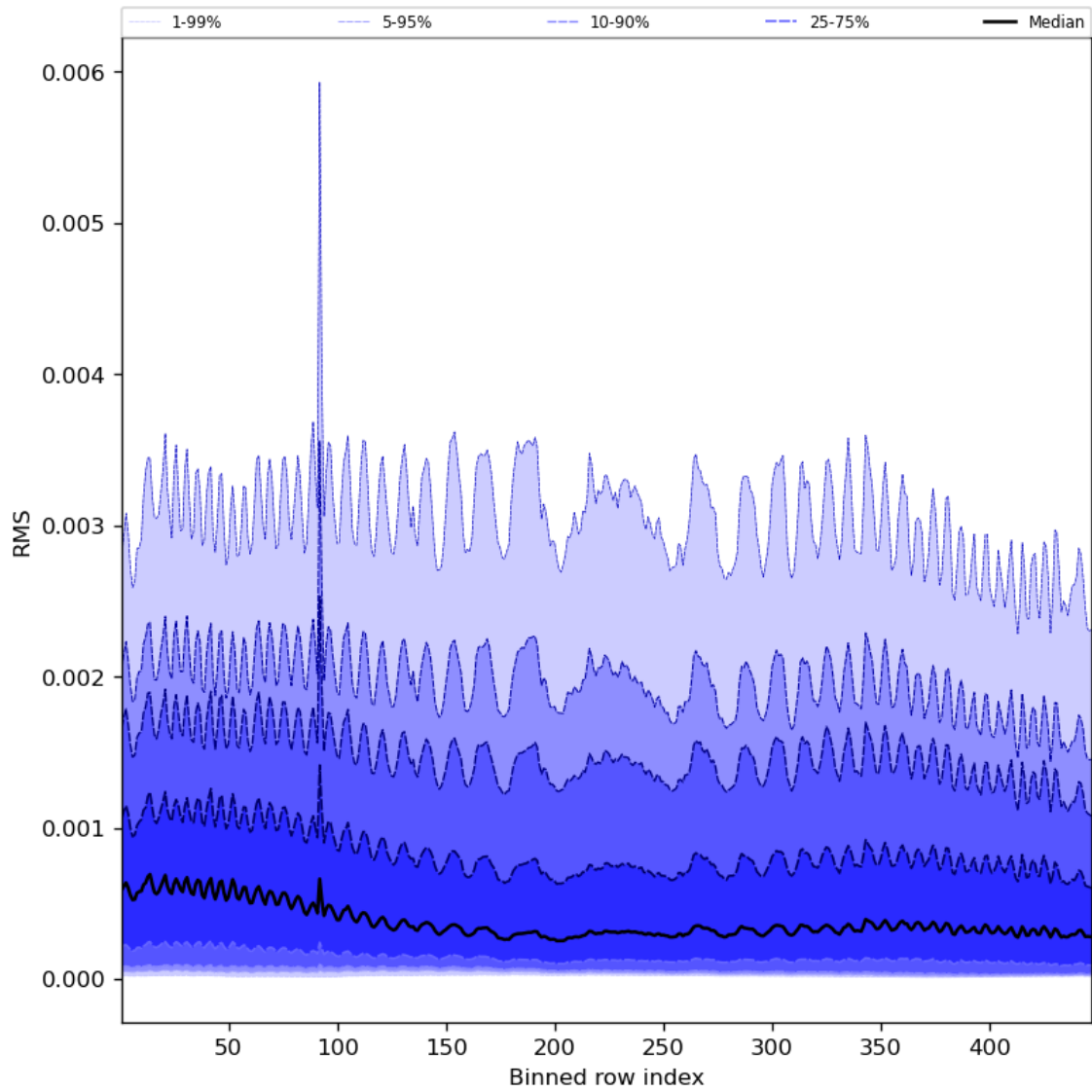
Figure 63: Along track statistics of “RMS” for 2023-09-10 to 2023-09-12
