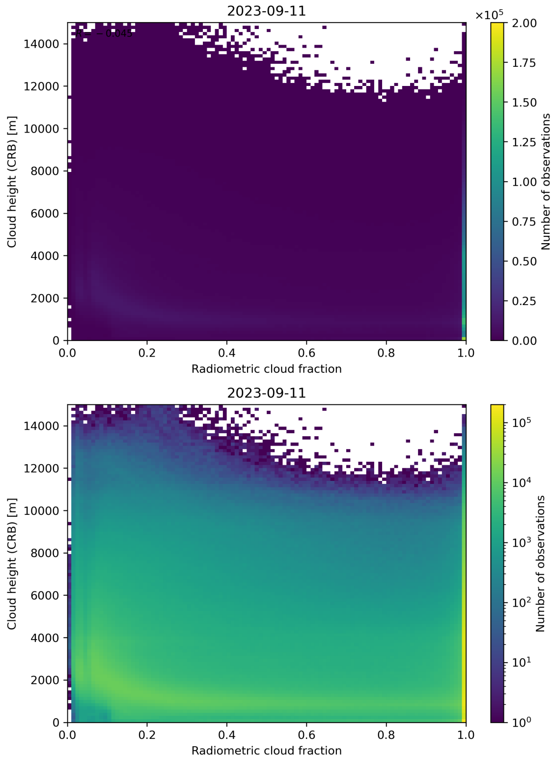
Figure 74: Scatter density plot of “Radiometric cloud fraction” against “Cloud height (CRB)” for 2023-09-10 to 2023-09-12.
