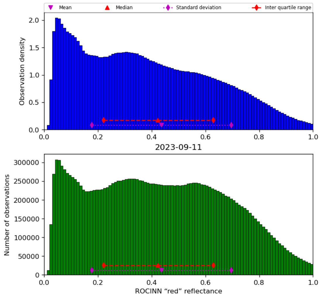
Figure 53: Histogram of “ROCINN “red” reflectance” for 2023-09-10 to 2023-09-12
