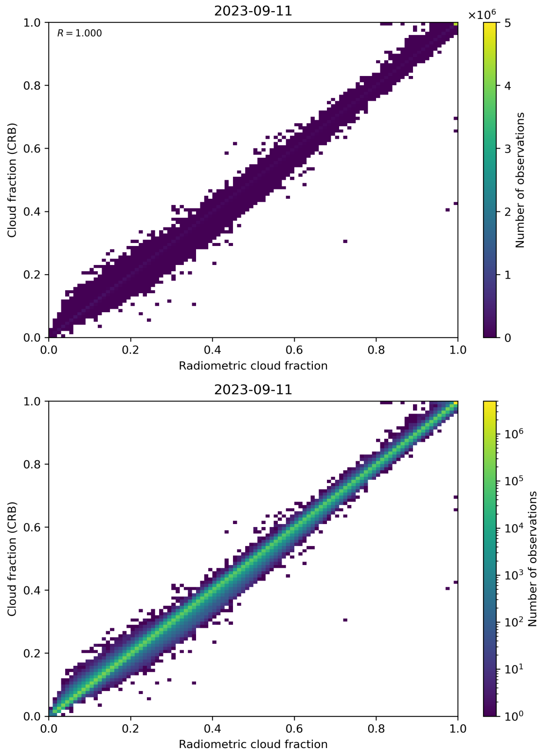
Figure 73: Scatter density plot of “Radiometric cloud fraction” against “Cloud fraction (CRB)” for 2023-09-10 to 2023-09-12.
