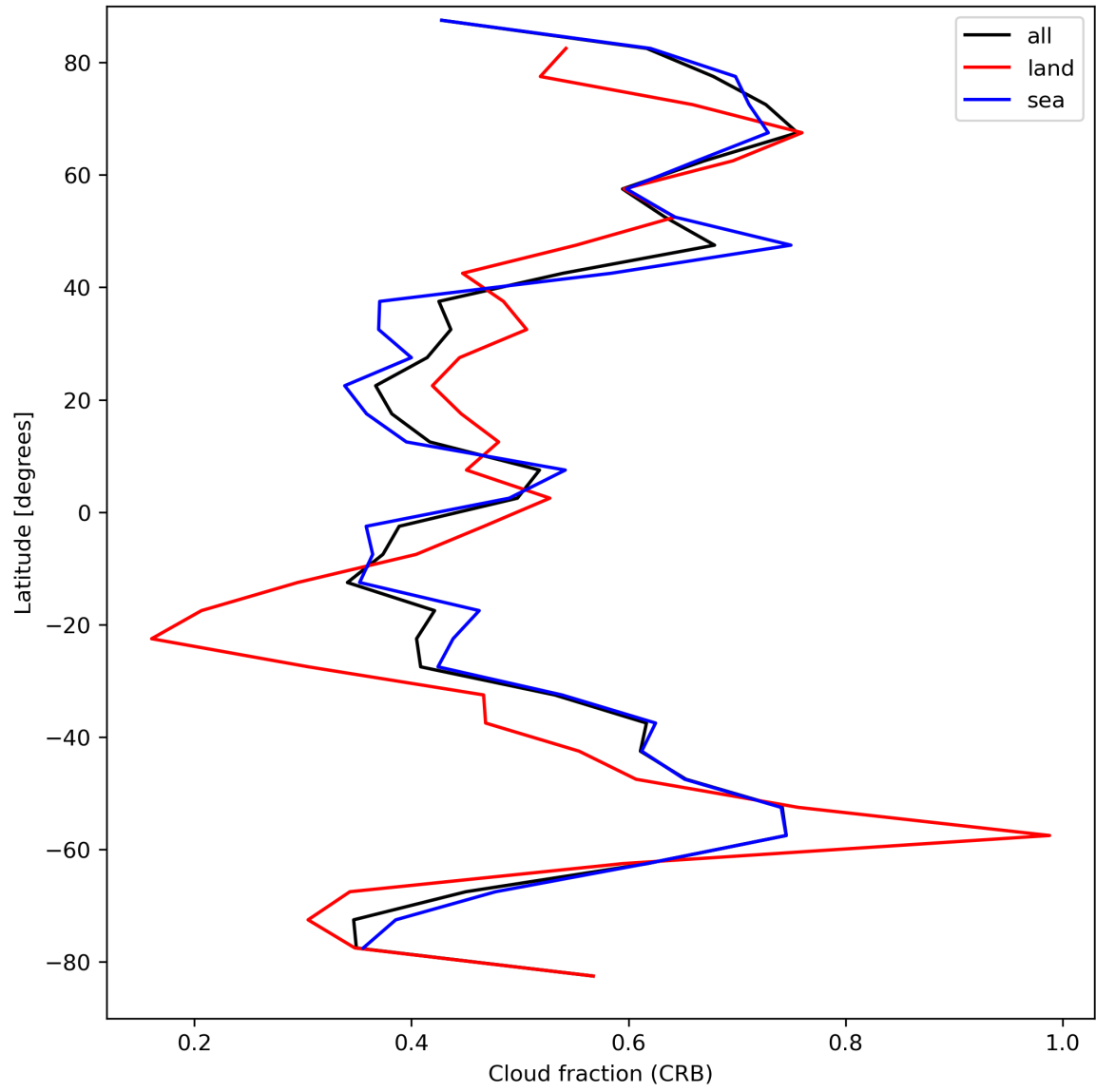
Figure 26: Zonal average of “Cloud fraction (CRB)” for 2023-09-10 to 2023-09-12.
