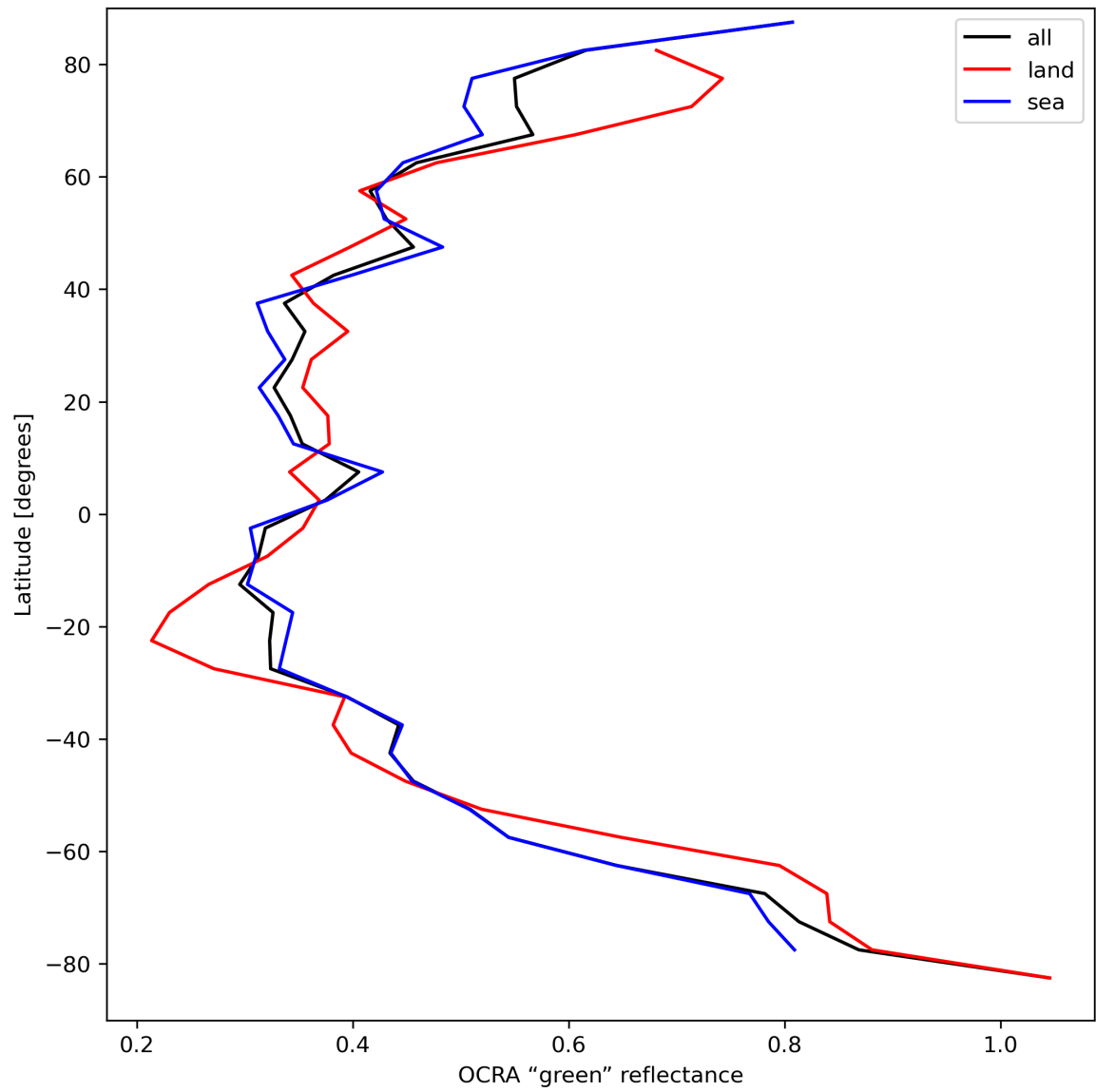
Figure 36: Zonal average of “OCRA “green” reflectance” for 2023-09-10 to 2023-09-12.
