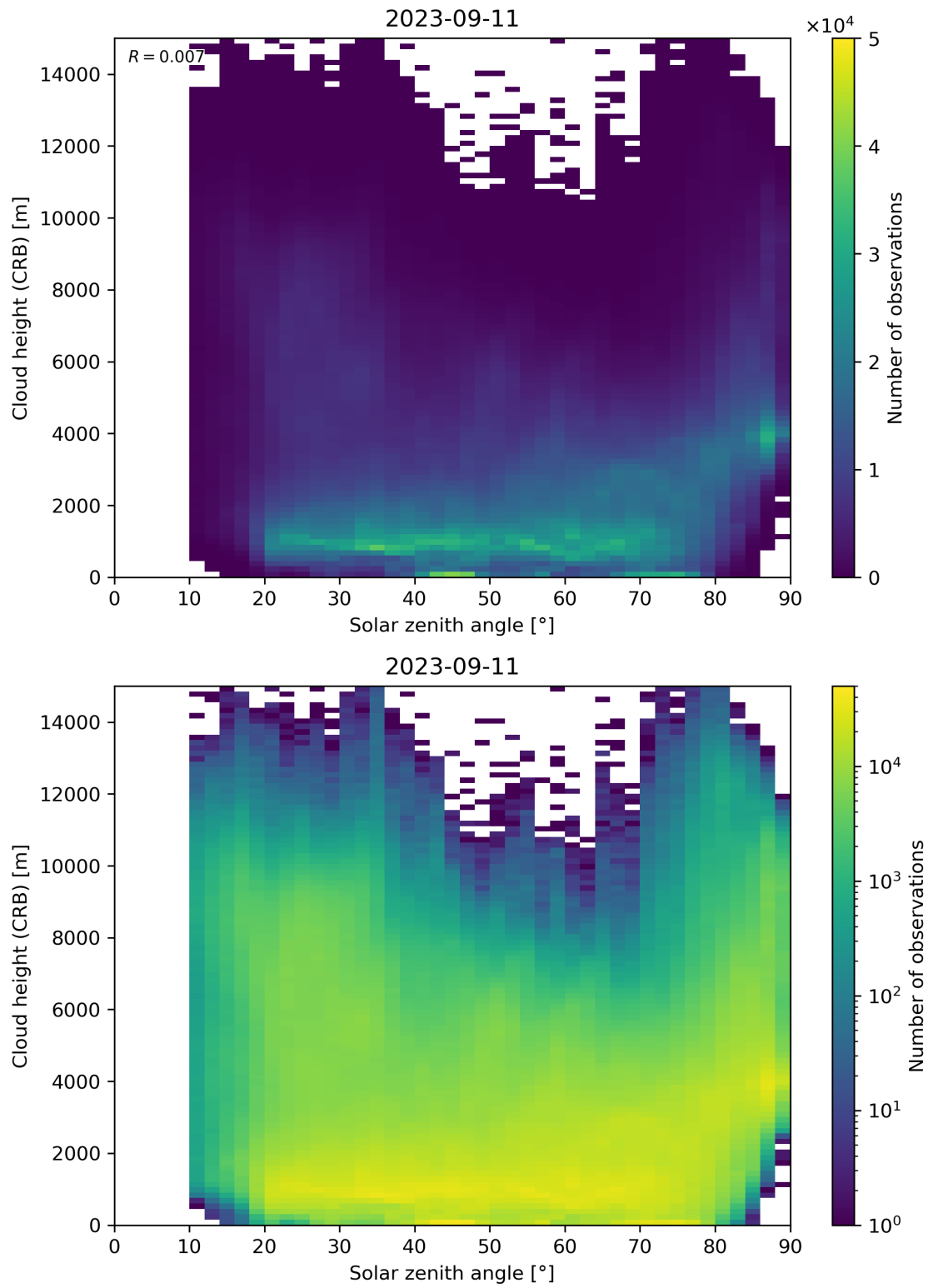
Figure 102: Scatter density plot of “Solar zenith angle” against “Cloud height (CRB)” for 2023-09-10 to 2023-09-12.
