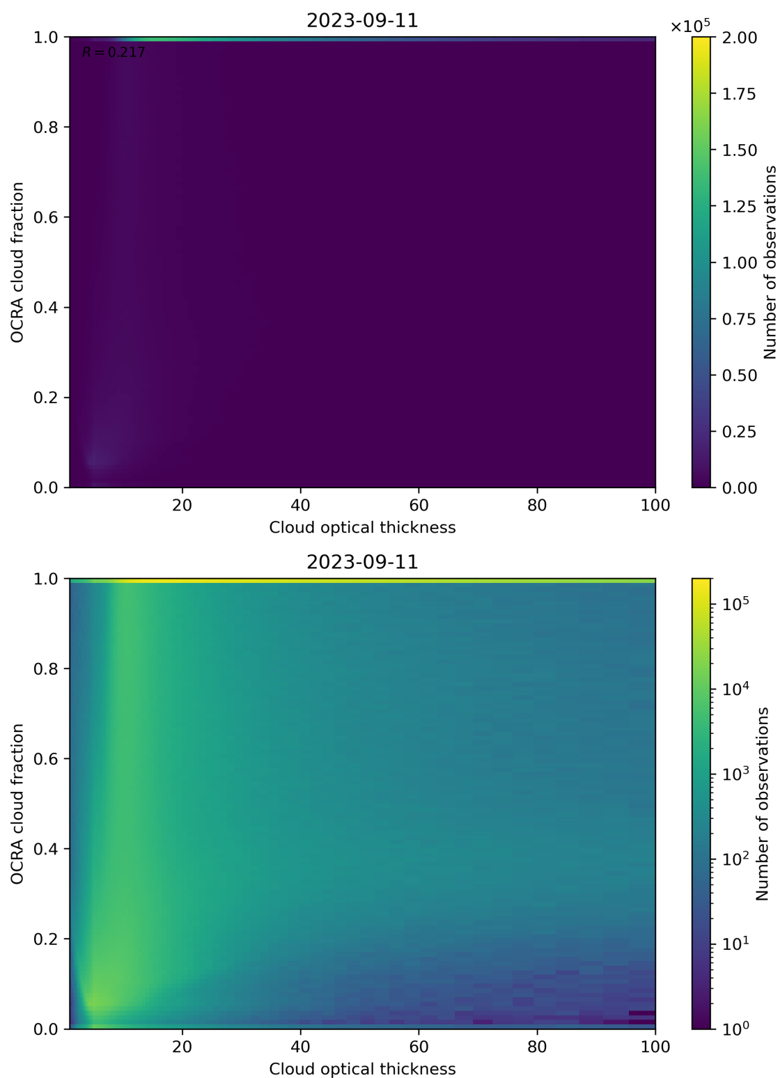
Figure 83: Scatter density plot of “Cloud optical thickness” against “OCRA cloud fraction” for 2023-09-10 to 2023-09-12.
