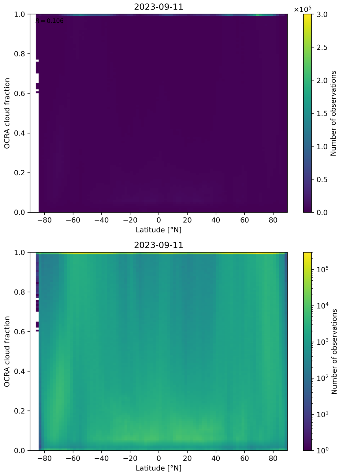
Figure 93: Scatter density plot of “Latitude” against “OCRA cloud fraction” for 2023-09-10 to 2023-09-12.
