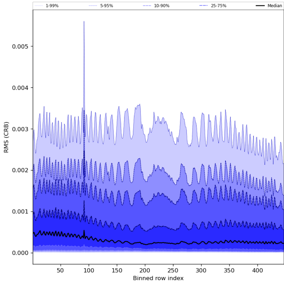
Figure 64: Along track statistics of “RMS (CRB)” for 2023-09-10 to 2023-09-12
