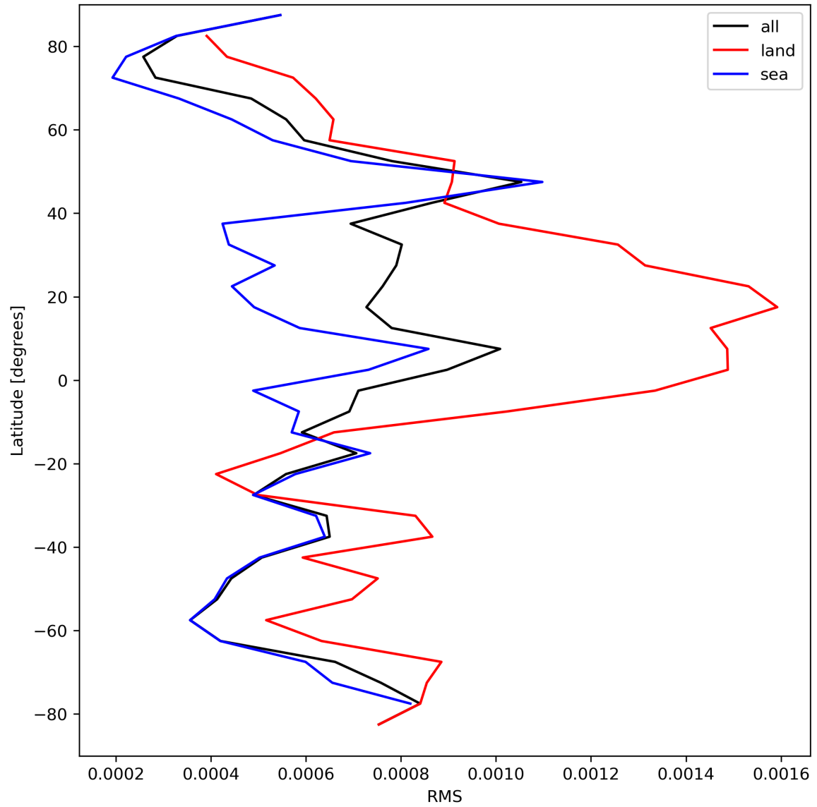
Figure 31: Zonal average of “RMS” for 2023-09-10 to 2023-09-12.
