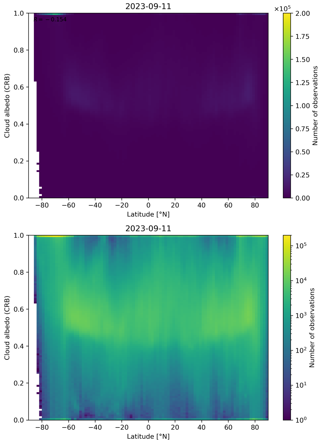
Figure 91: Scatter density plot of “Latitude” against “Cloud albedo (CRB)” for 2023-09-10 to 2023-09-12.
