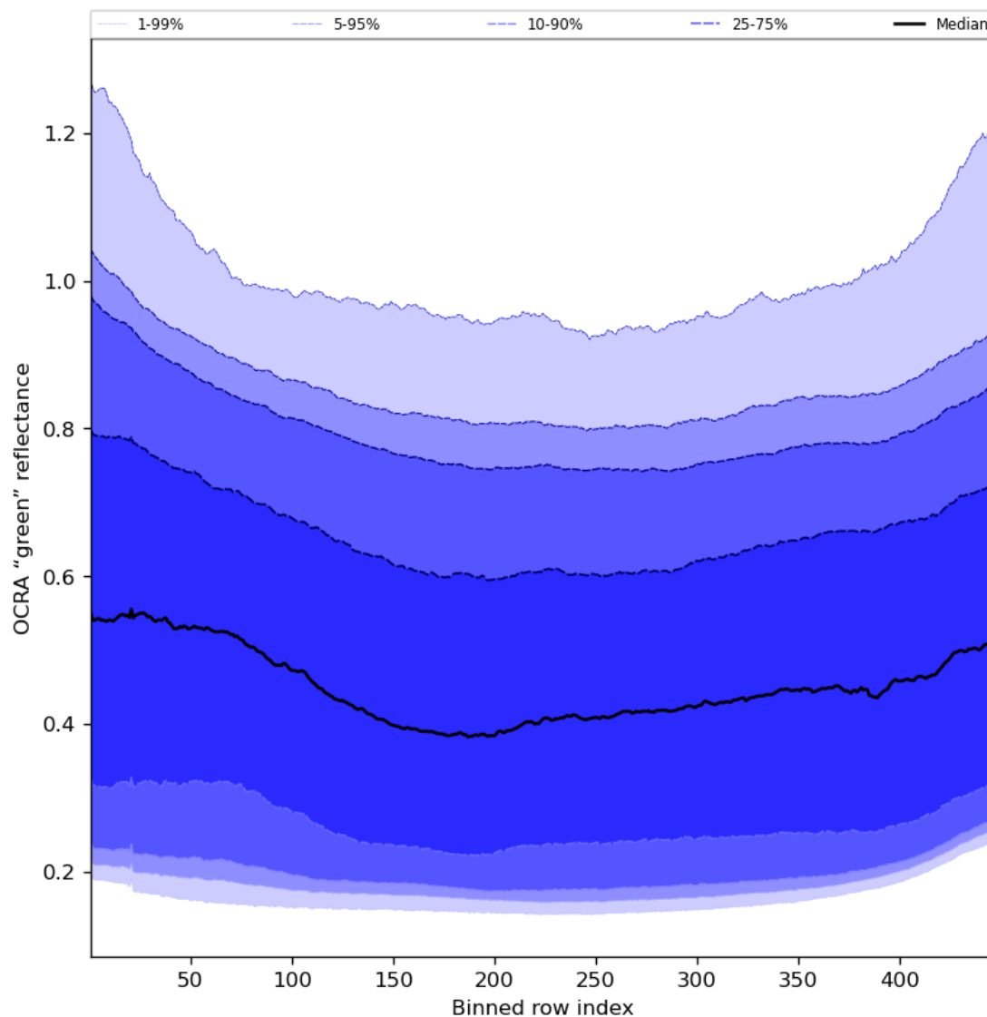
Figure 68: Along track statistics of “OCRA “green” reflectance” for 2023-09-10 to 2023-09-12
