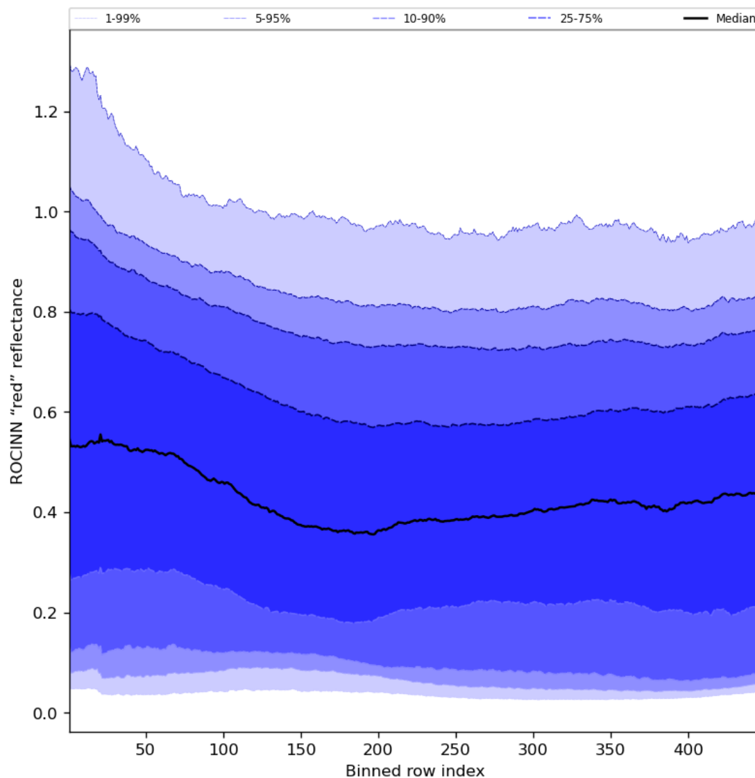
Figure 69: Along track statistics of “ROCINN “red” reflectance” for 2023-09-10 to 2023-09-12
