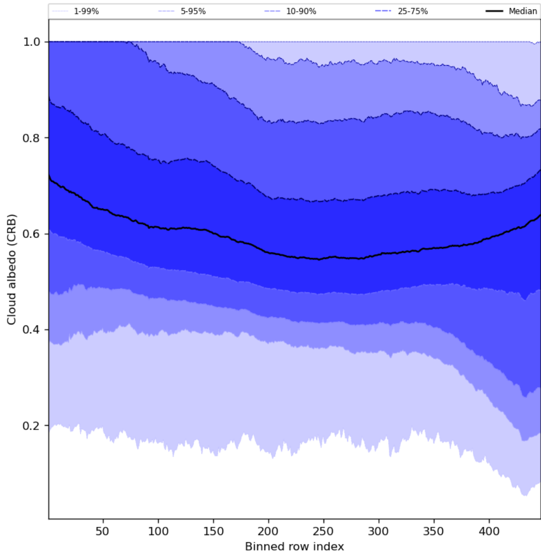
Figure 60: Along track statistics of “Cloud albedo (CRB)” for 2023-09-10 to 2023-09-12
