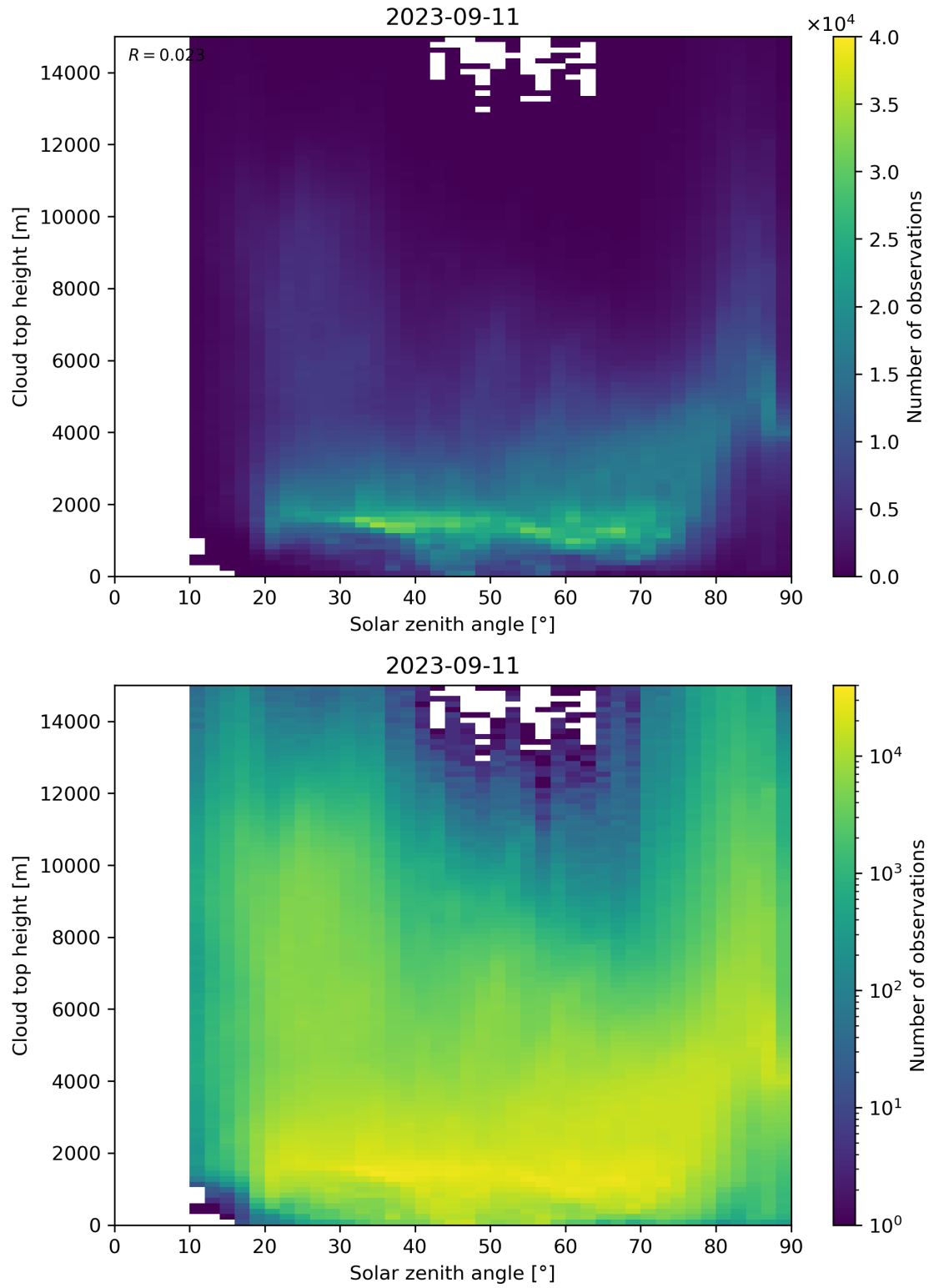
Figure 104: Scatter density plot of “Solar zenith angle” against “Cloud top height” for 2023-09-10 to 2023-09-12.
