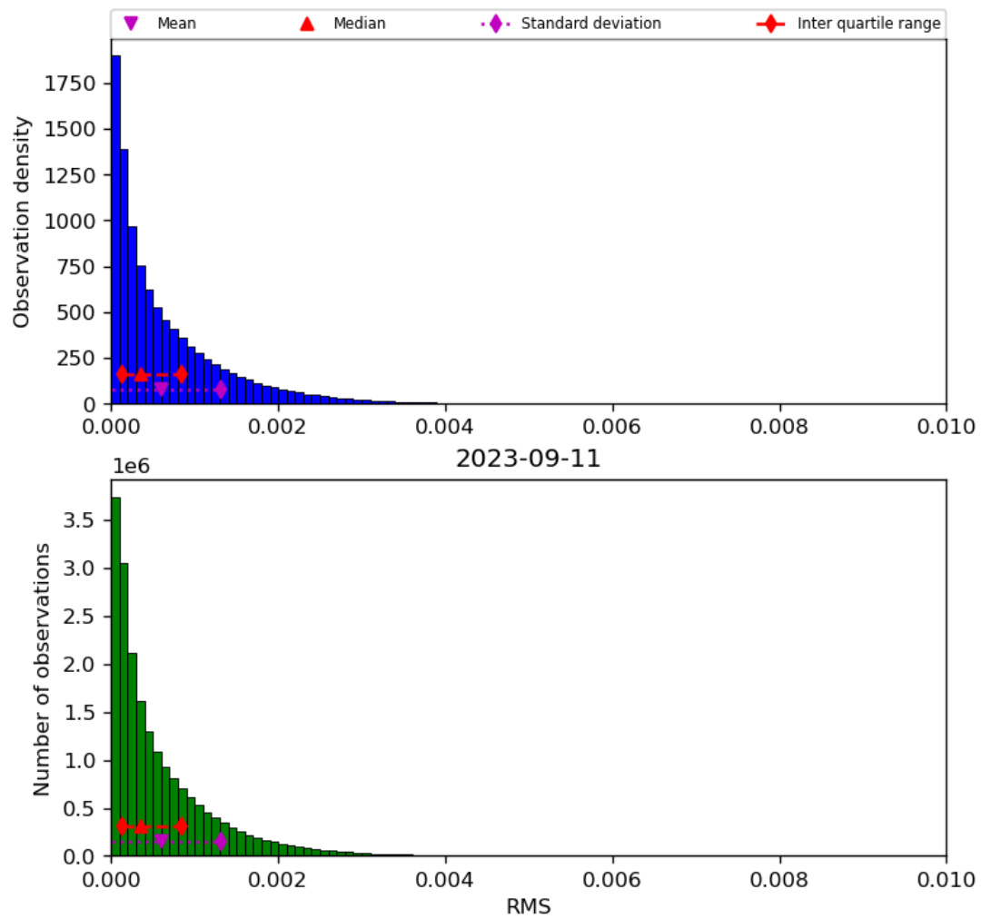
Figure 47: Histogram of “RMS” for 2023-09-10 to 2023-09-12
