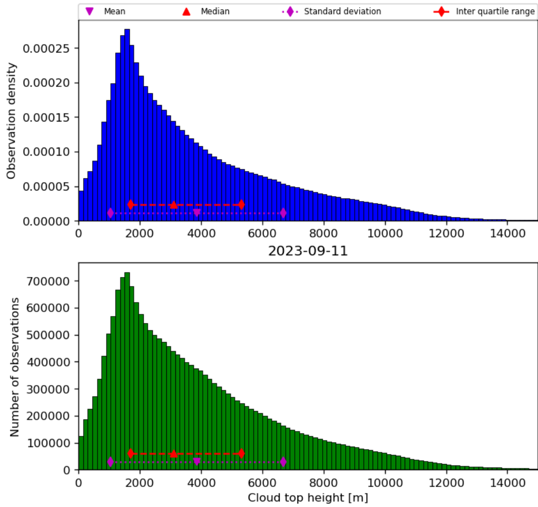
Figure 40: Histogram of “Cloud top height” for 2023-09-10 to 2023-09-12
