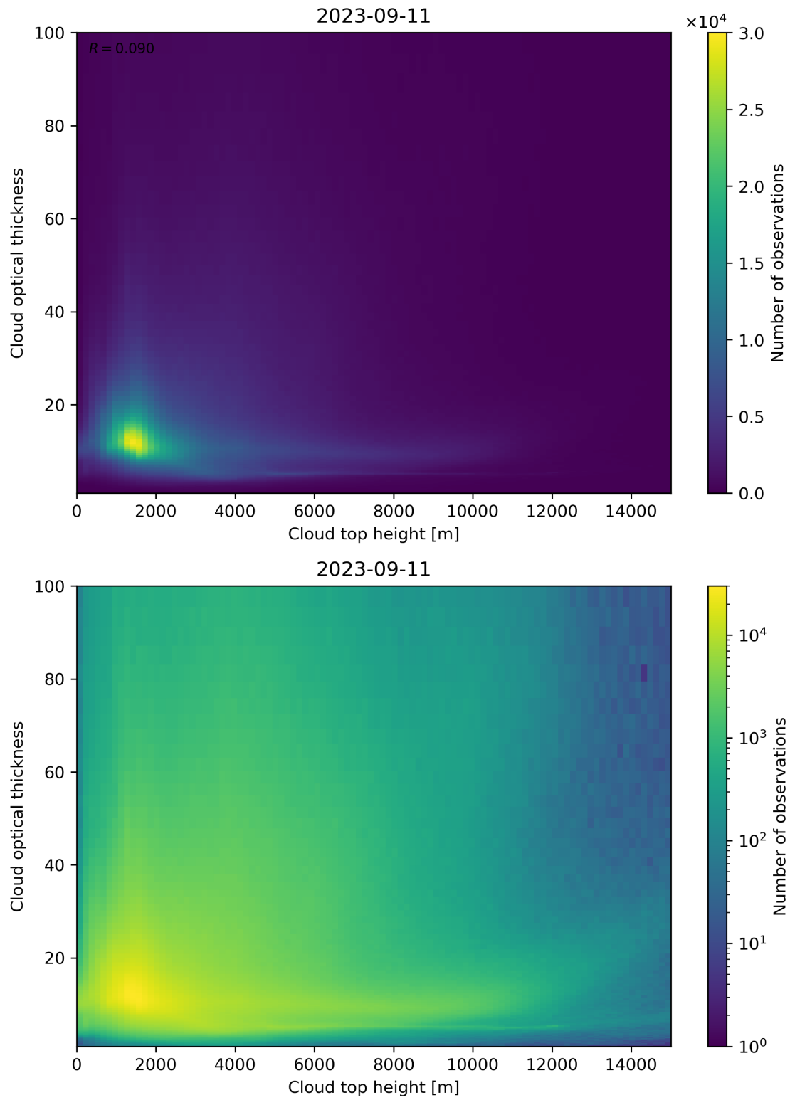
Figure 90: Scatter density plot of “Cloud top height” against “Cloud optical thickness” for 2023-09-10 to 2023-09-12.
