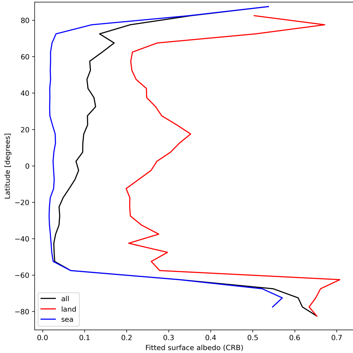
Figure 30: Zonal average of "Fitted surface albedo (CRB)" for 2023-09-10 to 2023-09-12.
