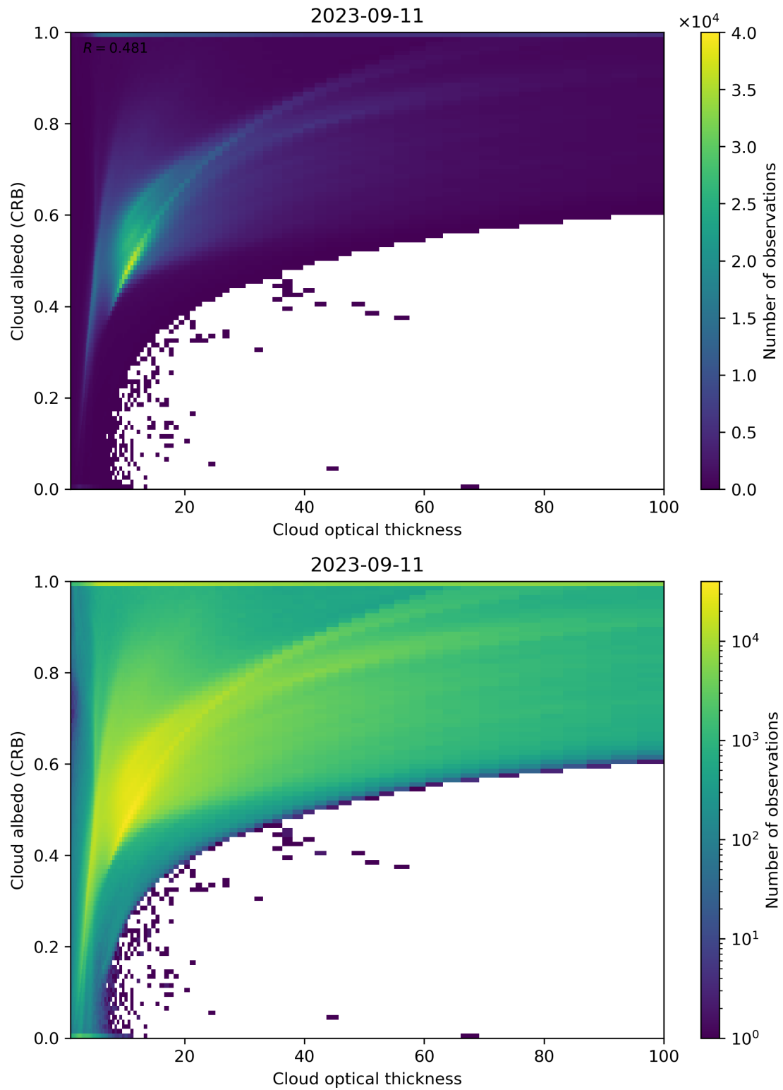
Figure 82: Scatter density plot of “Cloud optical thickness” against “Cloud albedo (CRB)” for 2023-09-10 to 2023-09-12.
