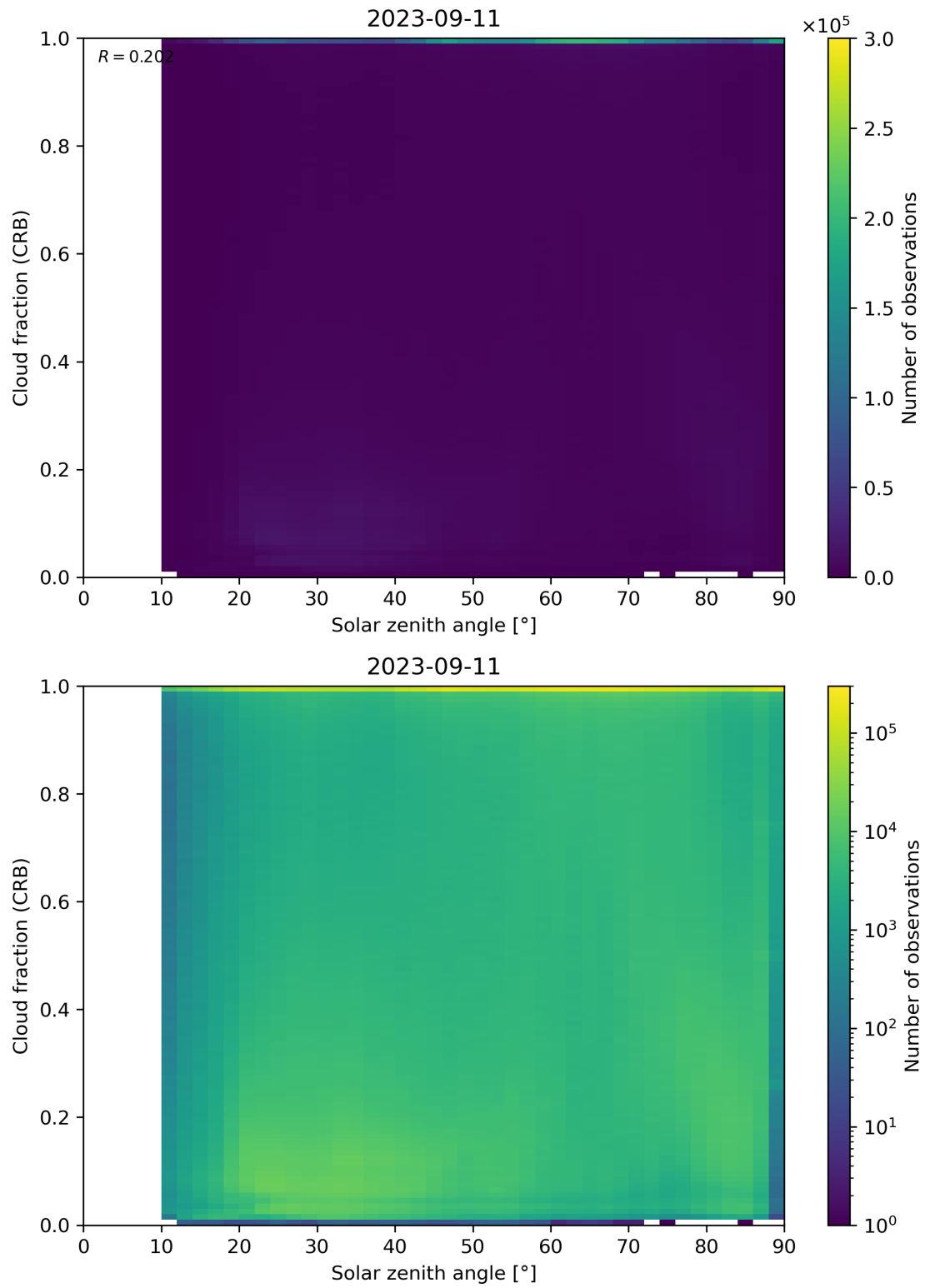
Figure 101: Scatter density plot of “Solar zenith angle” against “Cloud fraction (CRB)” for 2023-09-10 to 2023-09-12.
