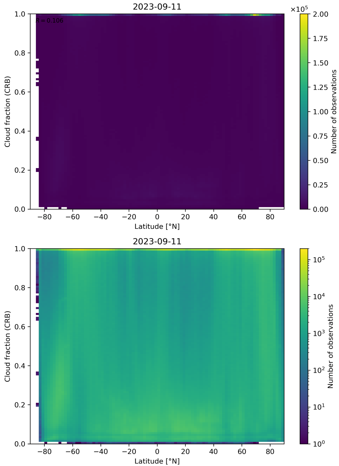
Figure 94: Scatter density plot of “Latitude” against “Cloud fraction (CRB)” for 2023-09-10 to 2023-09-12.
