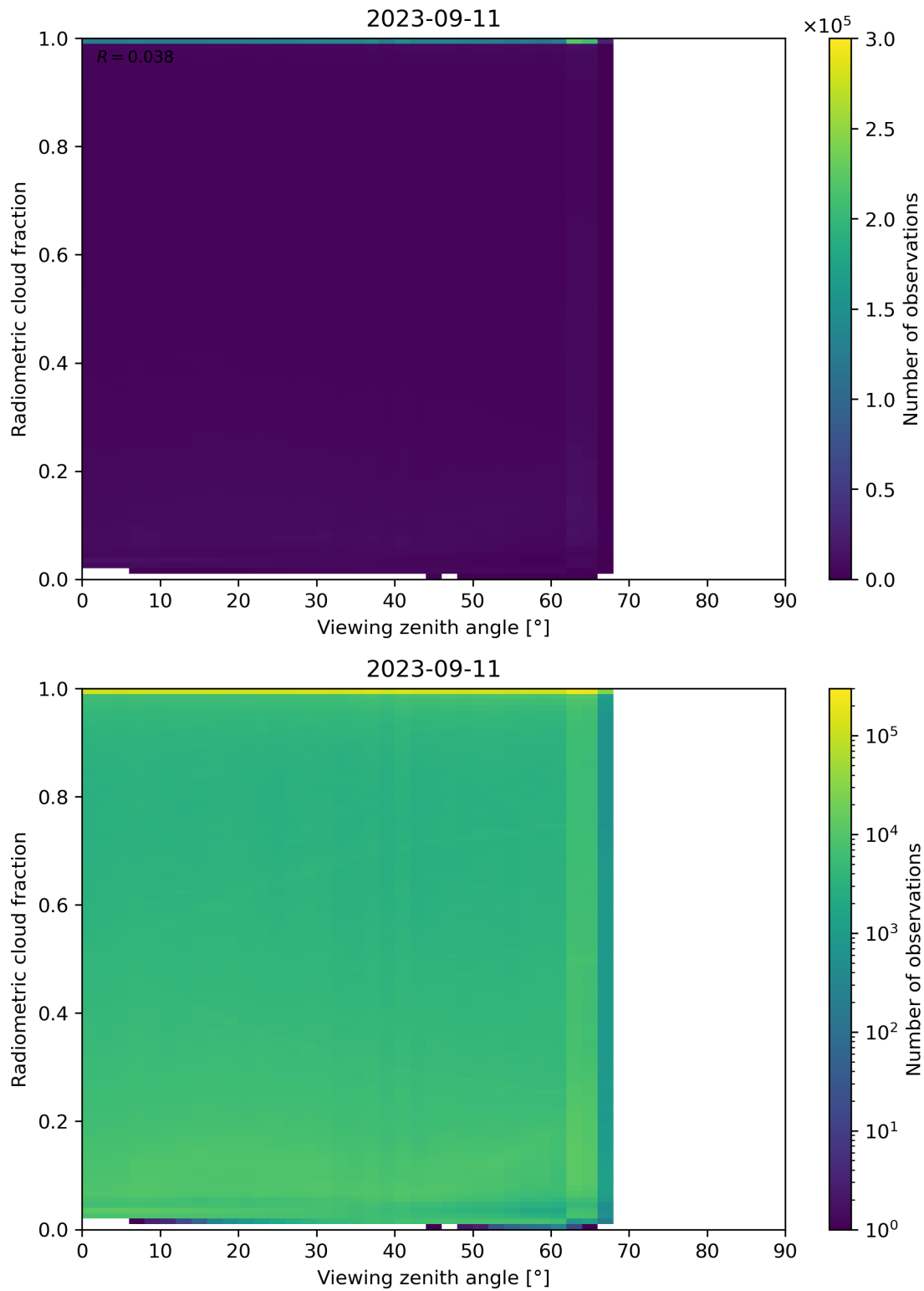
Figure 107: Scatter density plot of “Viewing zenith angle” against “Radiometric cloud fraction” for 2023-09-10 to 2023-09-12.
