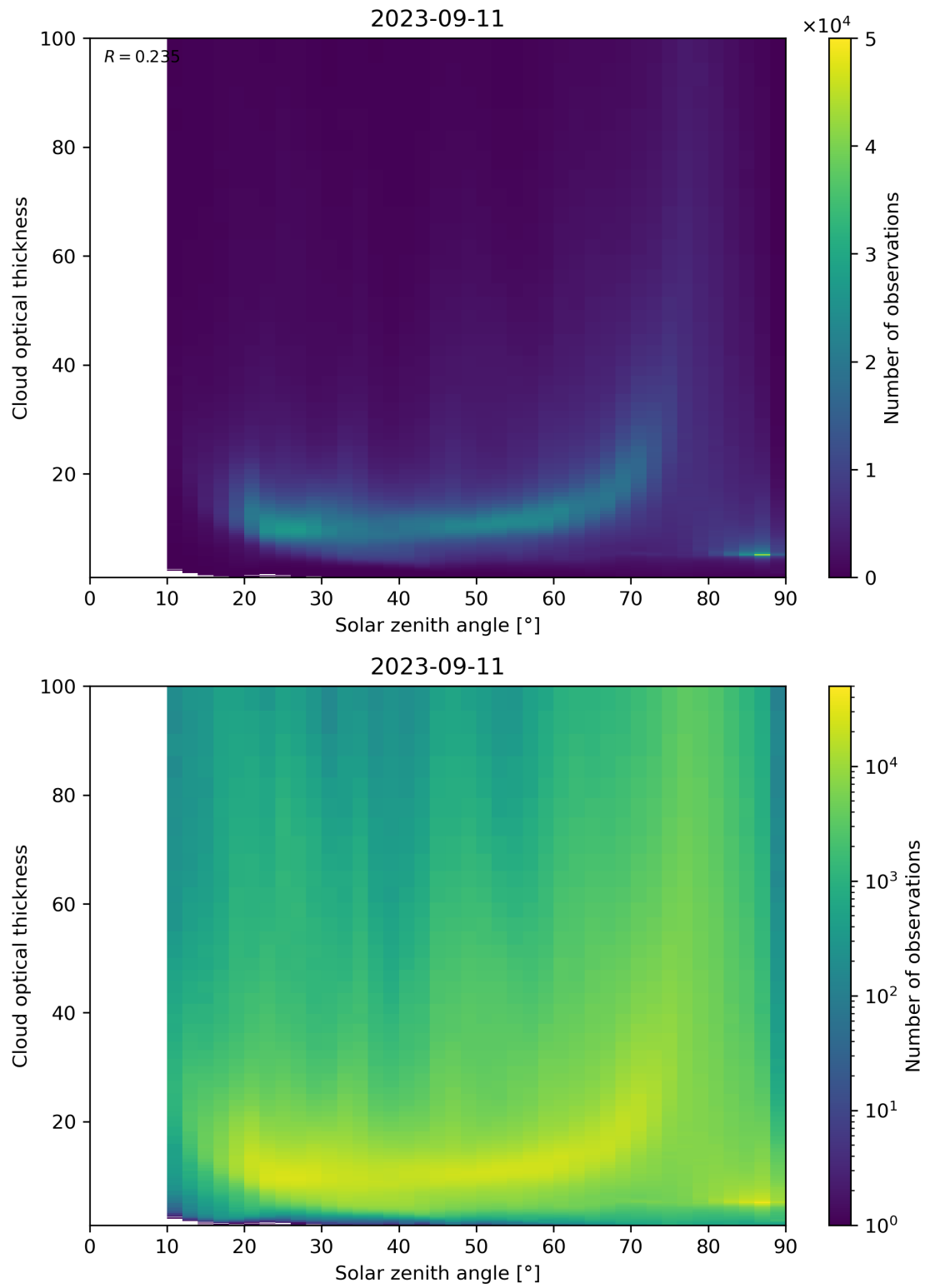
Figure 103: Scatter density plot of “Solar zenith angle” against “Cloud optical thickness” for 2023-09-10 to 2023-09-12.
