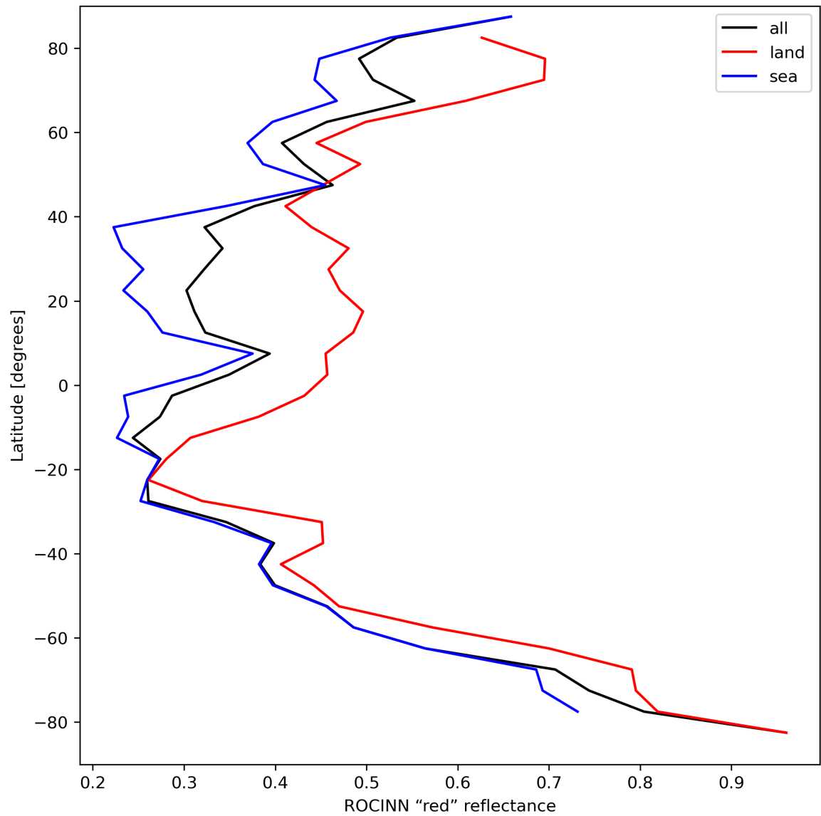
Figure 37: Zonal average of “ROCINN “red” reflectance” for 2023-09-10 to 2023-09-12.
