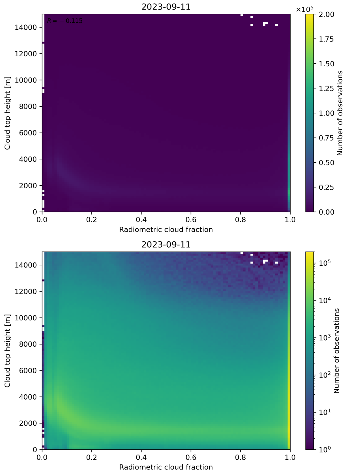
Figure 76: Scatter density plot of “Radiometric cloud fraction” against “Cloud top height” for 2023-09-10 to 2023-09-12.
