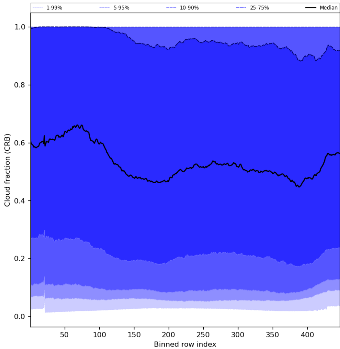
Figure 58: Along track statistics of “Cloud fraction (CRB)” for 2023-09-10 to 2023-09-12
