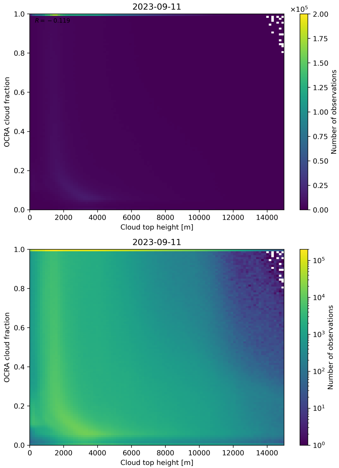
Figure 87: Scatter density plot of “Cloud top height” against “OCRA cloud fraction” for 2023-09-10 to 2023-09-12.
