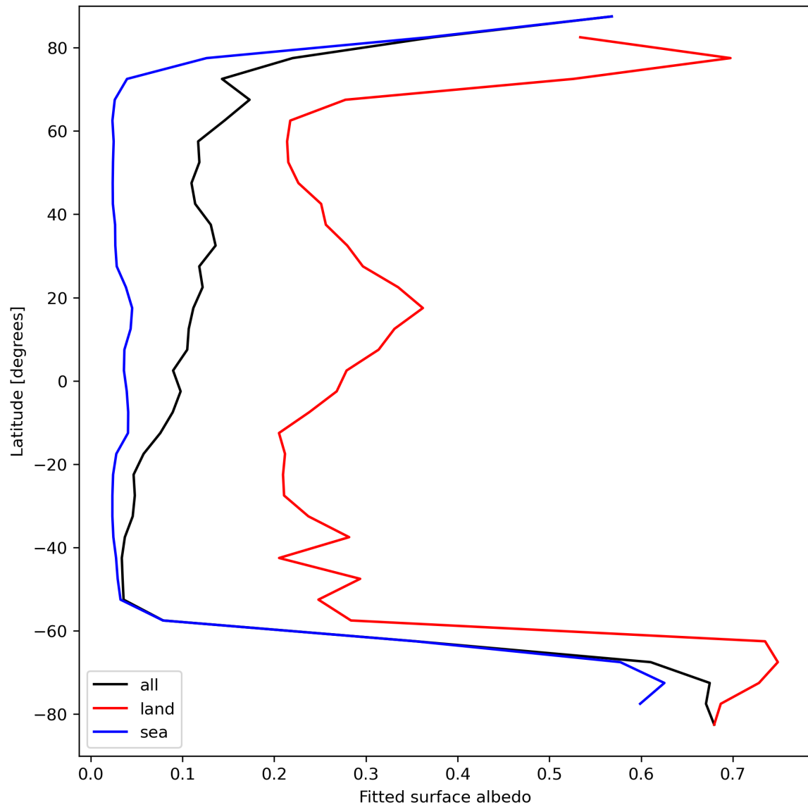
Figure 29: Zonal average of “Fitted surface albedo” for 2023-09-10 to 2023-09-12.
