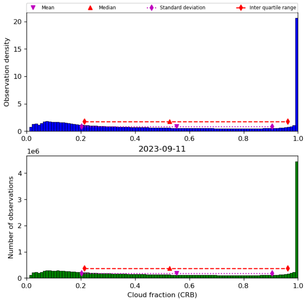
Figure 42: Histogram of “Cloud fraction (CRB)” for 2023-09-10 to 2023-09-12
