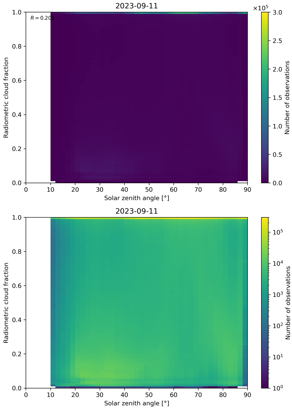
Figure 99: Scatter density plot of “Solar zenith angle” against “Radiometric cloud fraction” for 2023-09-10 to 2023-09-12.
