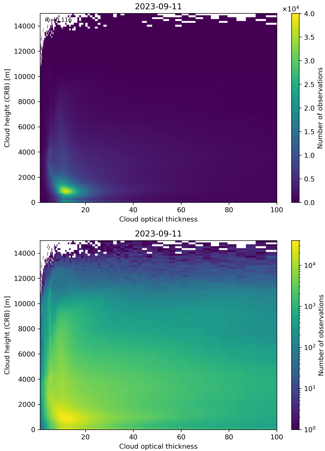
Figure 85: Scatter density plot of “Cloud optical thickness” against “Cloud height (CRB)” for 2023-09-10 to 2023-09-12.
