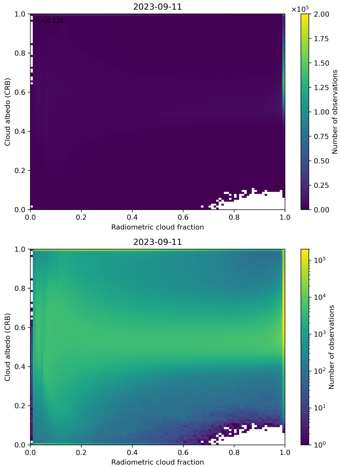
Figure 71: Scatter density plot of “Radiometric cloud fraction” against “Cloud albedo (CRB)” for 2023-09-10 to 2023-09-12.
