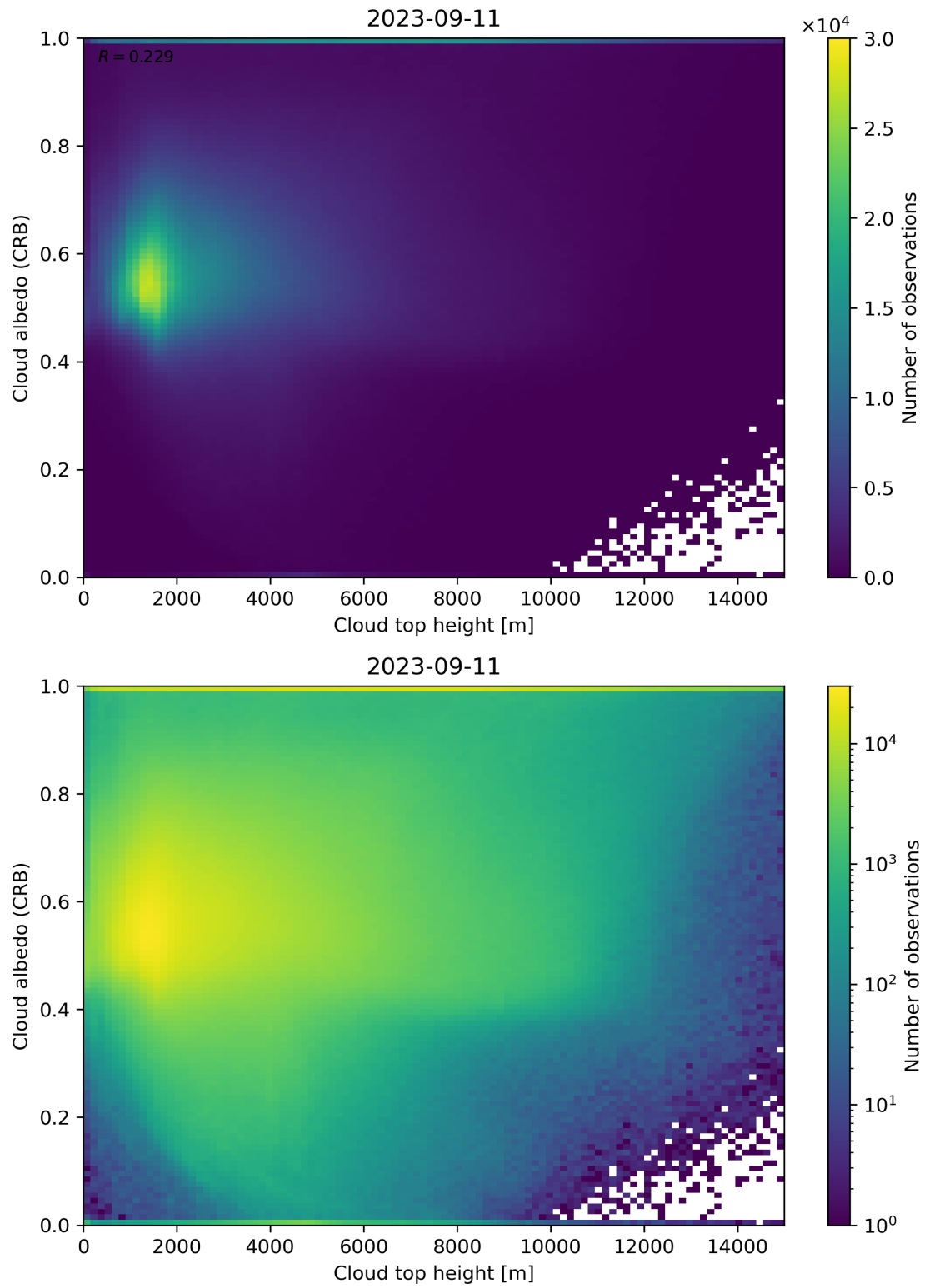
Figure 86: Scatter density plot of “Cloud top height” against “Cloud albedo (CRB)” for 2023-09-10 to 2023-09-12.
