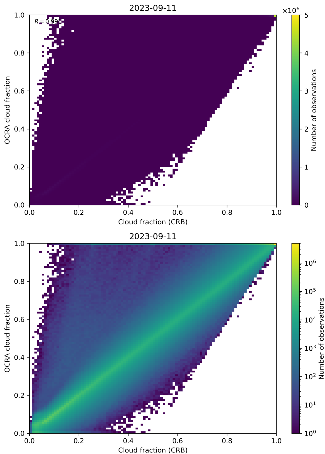
Figure 78: Scatter density plot of “Cloud fraction (CRB)” against “OCRA cloud fraction” for 2023-09-10 to 2023-09-12.
