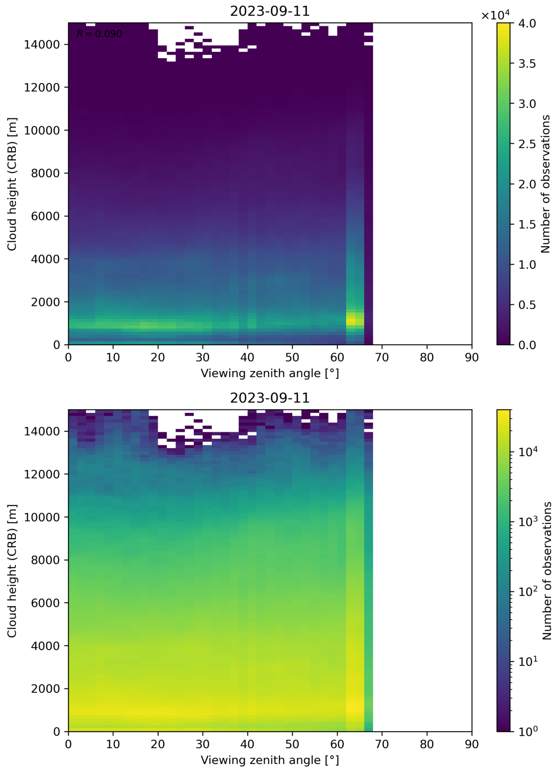
Figure 110: Scatter density plot of “Viewing zenith angle” against “Cloud height (CRB)” for 2023-09-10 to 2023-09-12.
