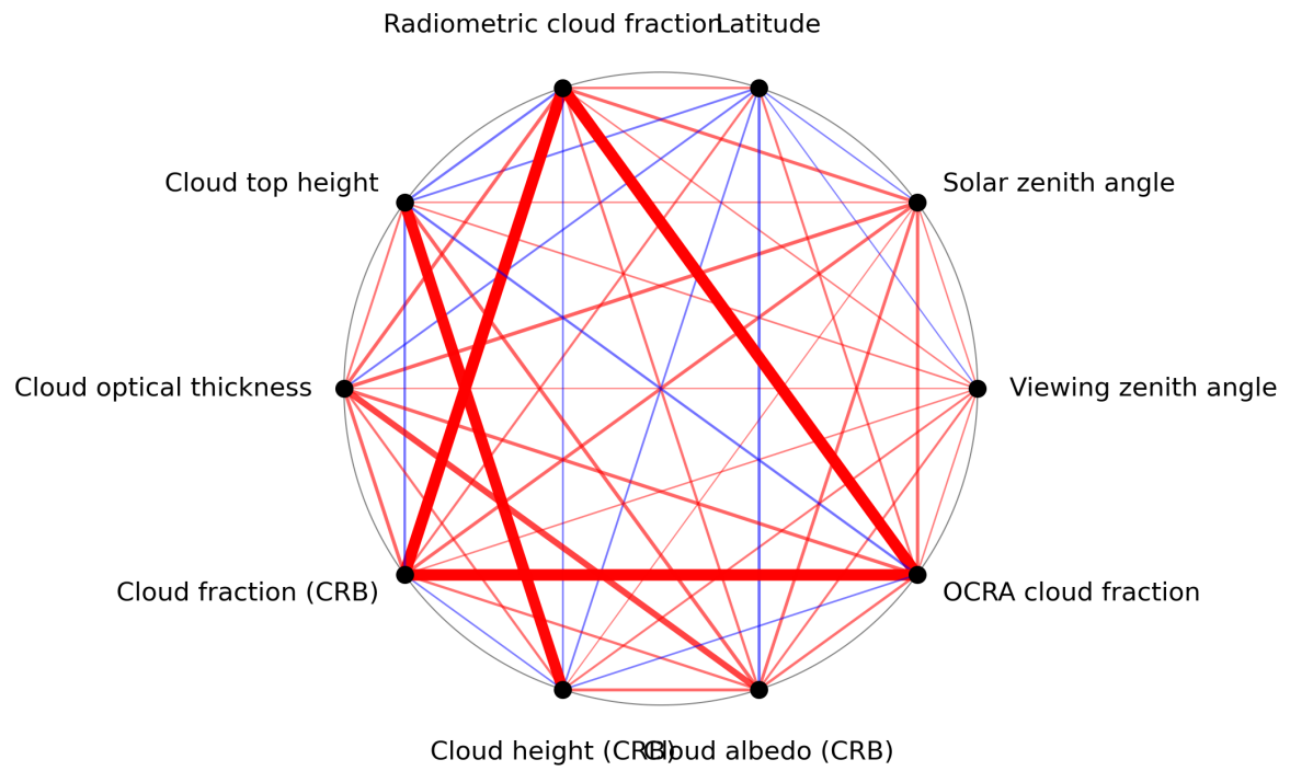
Figure 1: Map of correlation graph for 2023-09-10 to 2023-09-12.
