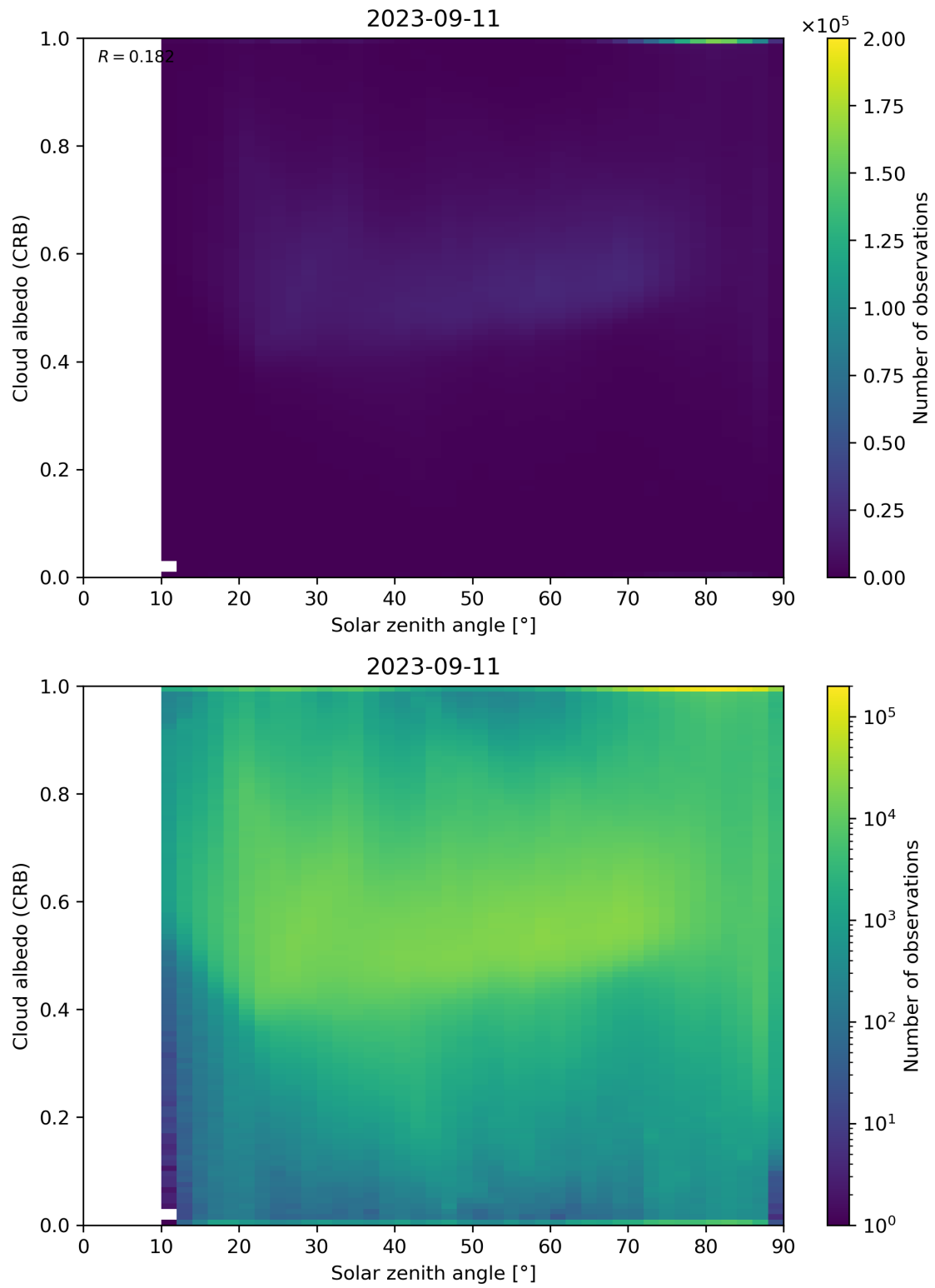
Figure 98: Scatter density plot of “Solar zenith angle” against “Cloud albedo (CRB)” for 2023-09-10 to 2023-09-12.
