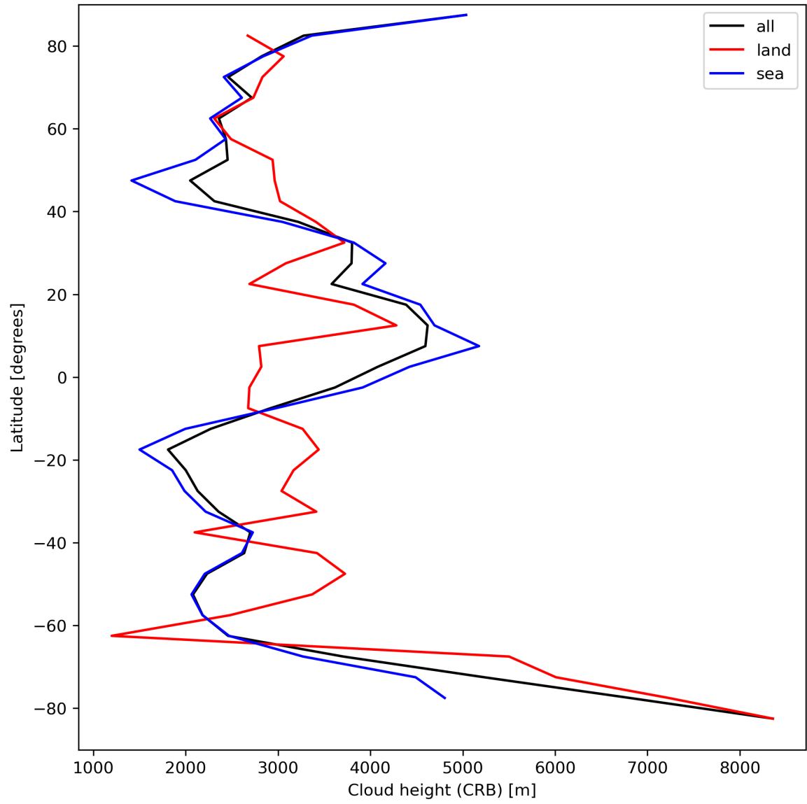
Figure 27: Zonal average of “Cloud height (CRB)” for 2023-09-10 to 2023-09-12.
