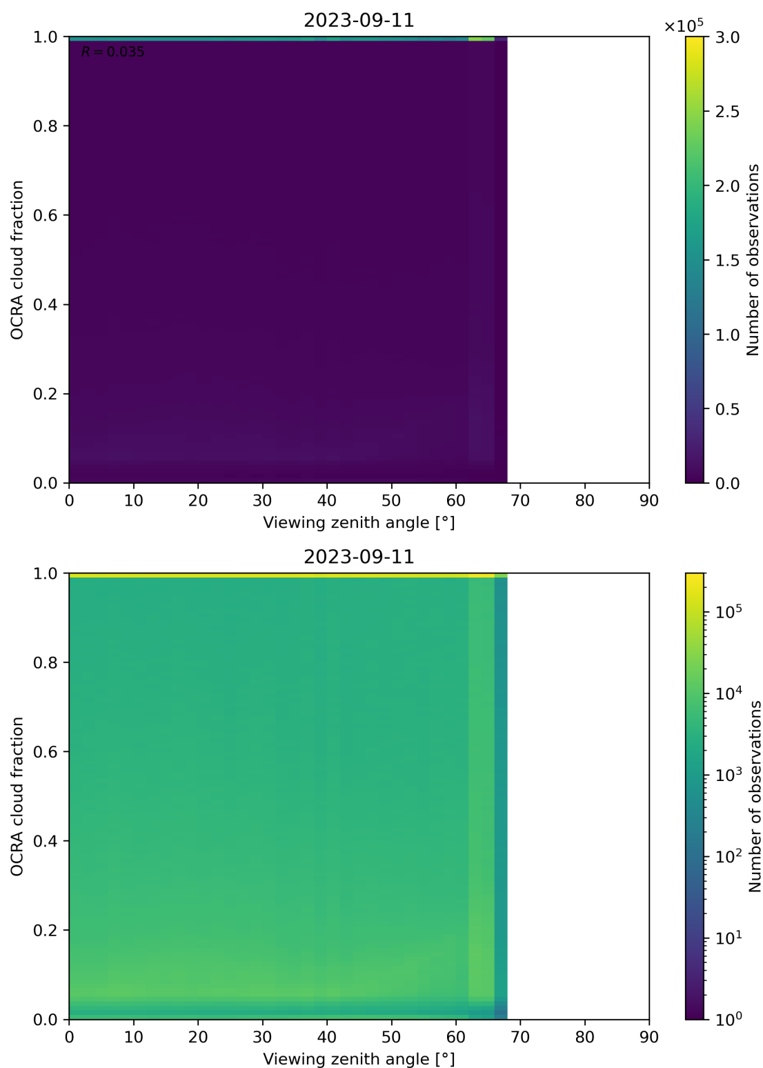
Figure 108: Scatter density plot of “Viewing zenith angle” against “OCRA cloud fraction” for 2023-09-10 to 2023-09-12.
