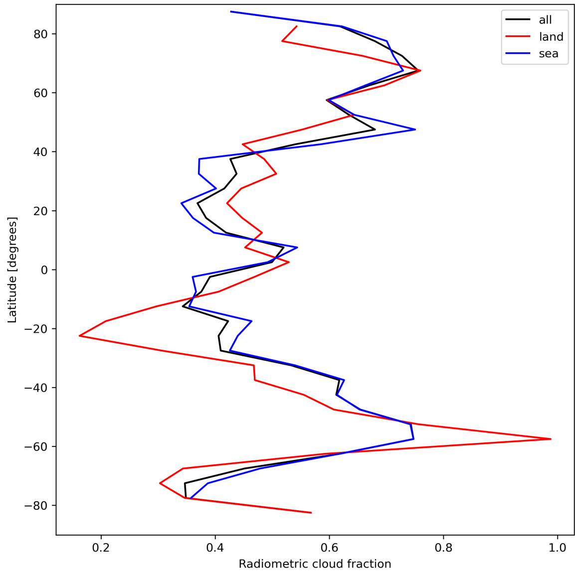
Figure 23: Zonal average of “Radiometric cloud fraction” for 2023-09-10 to 2023-09-12.
