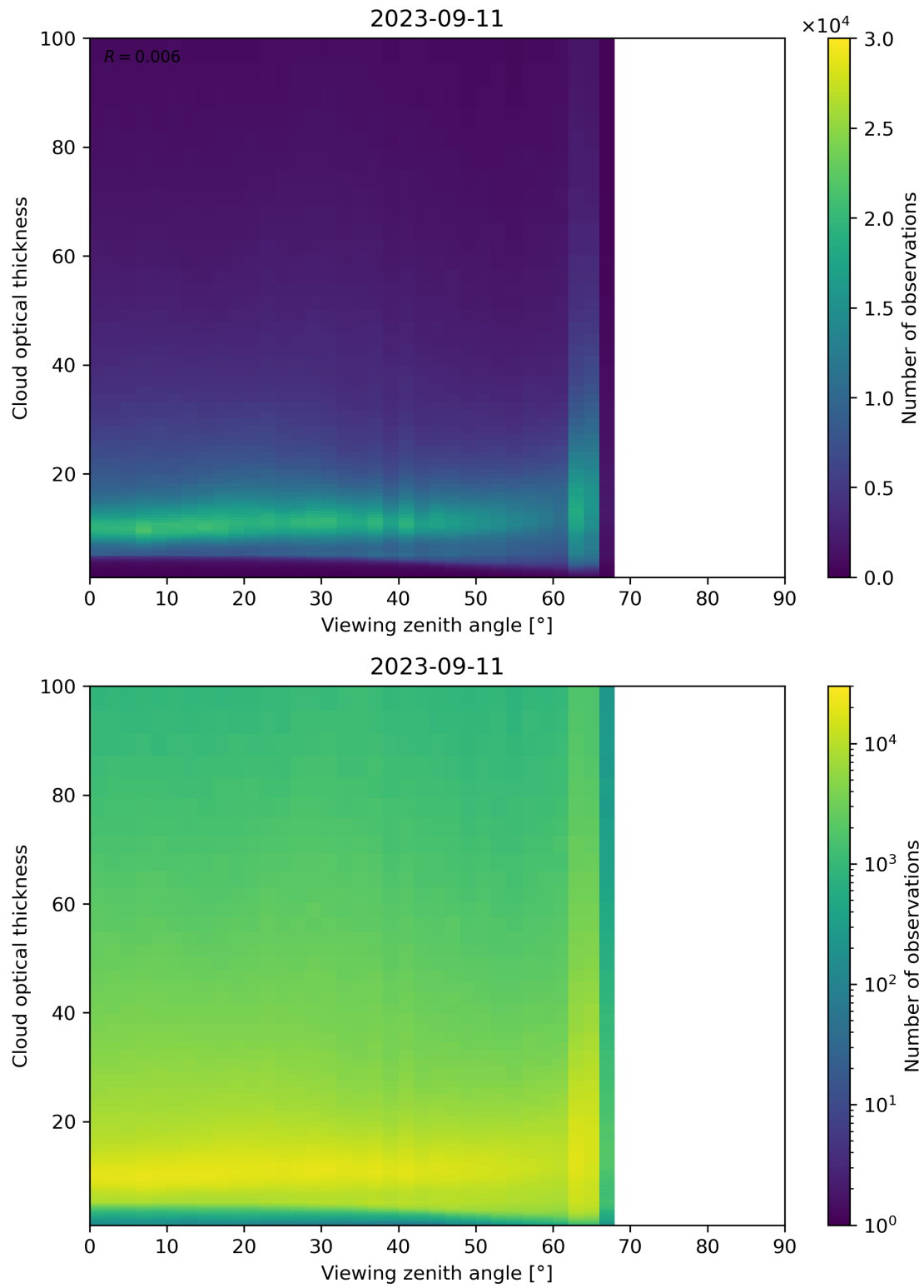
Figure 111: Scatter density plot of “Viewing zenith angle” against “Cloud optical thickness” for 2023-09-10 to 2023-09-12.
