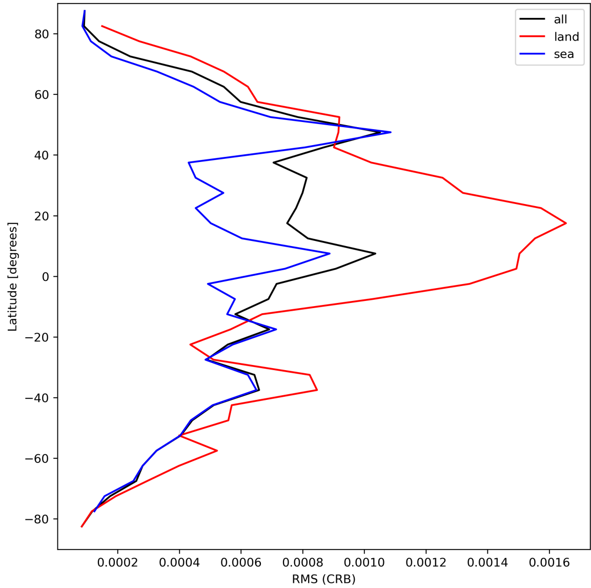
Figure 32: Zonal average of “RMS (CRB)” for 2023-09-10 to 2023-09-12.
