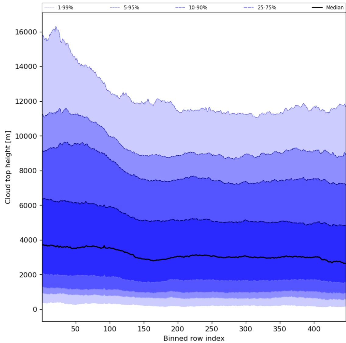
Figure 56: Along track statistics of “Cloud top height” for 2023-09-10 to 2023-09-12
