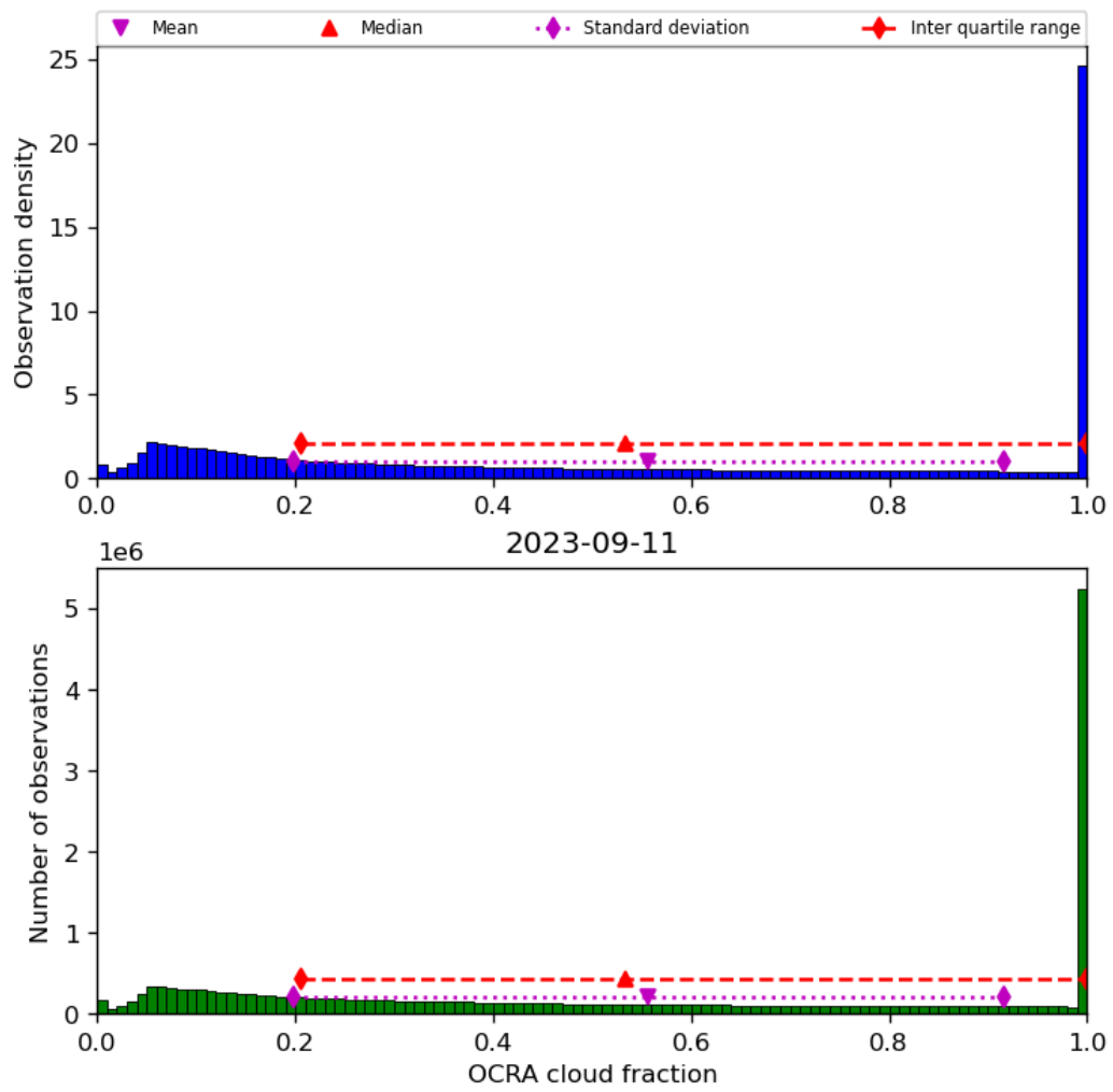
Figure 50: Histogram of “OCRA cloud fraction” for 2023-09-10 to 2023-09-12
