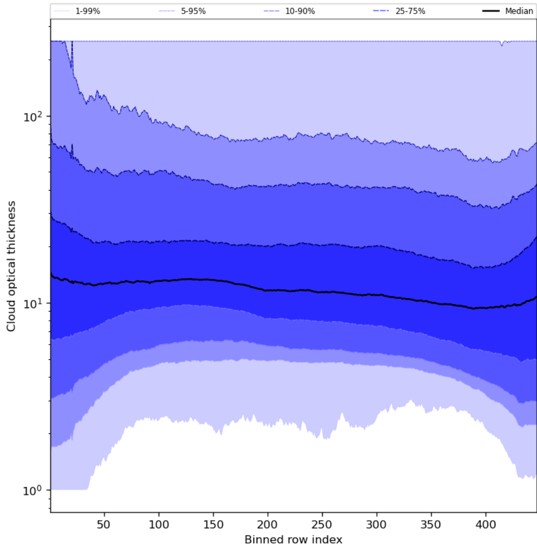
Figure 57: Along track statistics of “Cloud optical thickness” for 2023-09-10 to 2023-09-12
