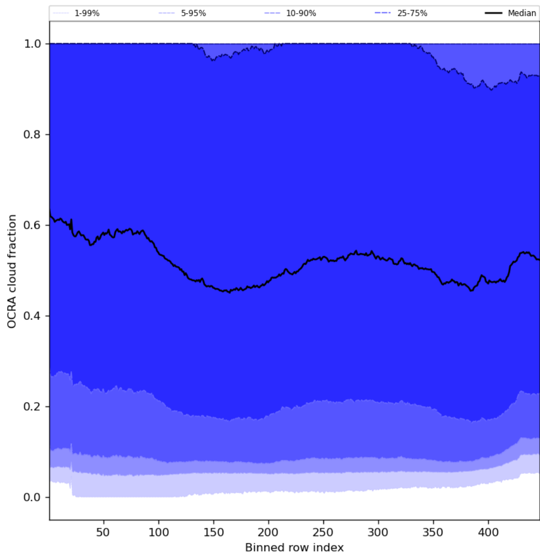
Figure 66: Along track statistics of “OCRA cloud fraction” for 2023-09-11 to 2023-09-13
