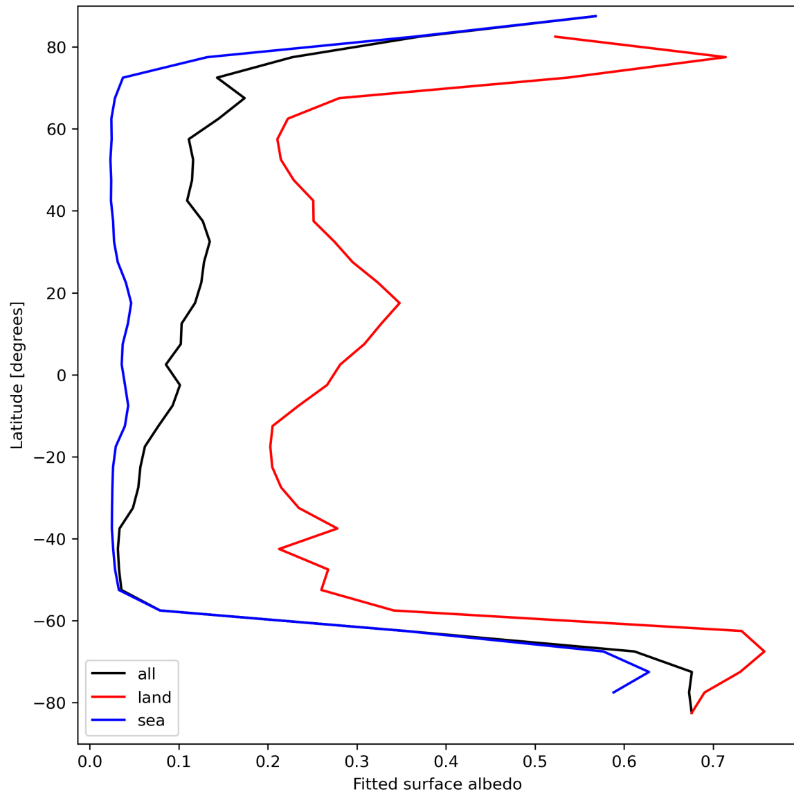
Figure 29: Zonal average of “Fitted surface albedo” for 2023-09-11 to 2023-09-13.
