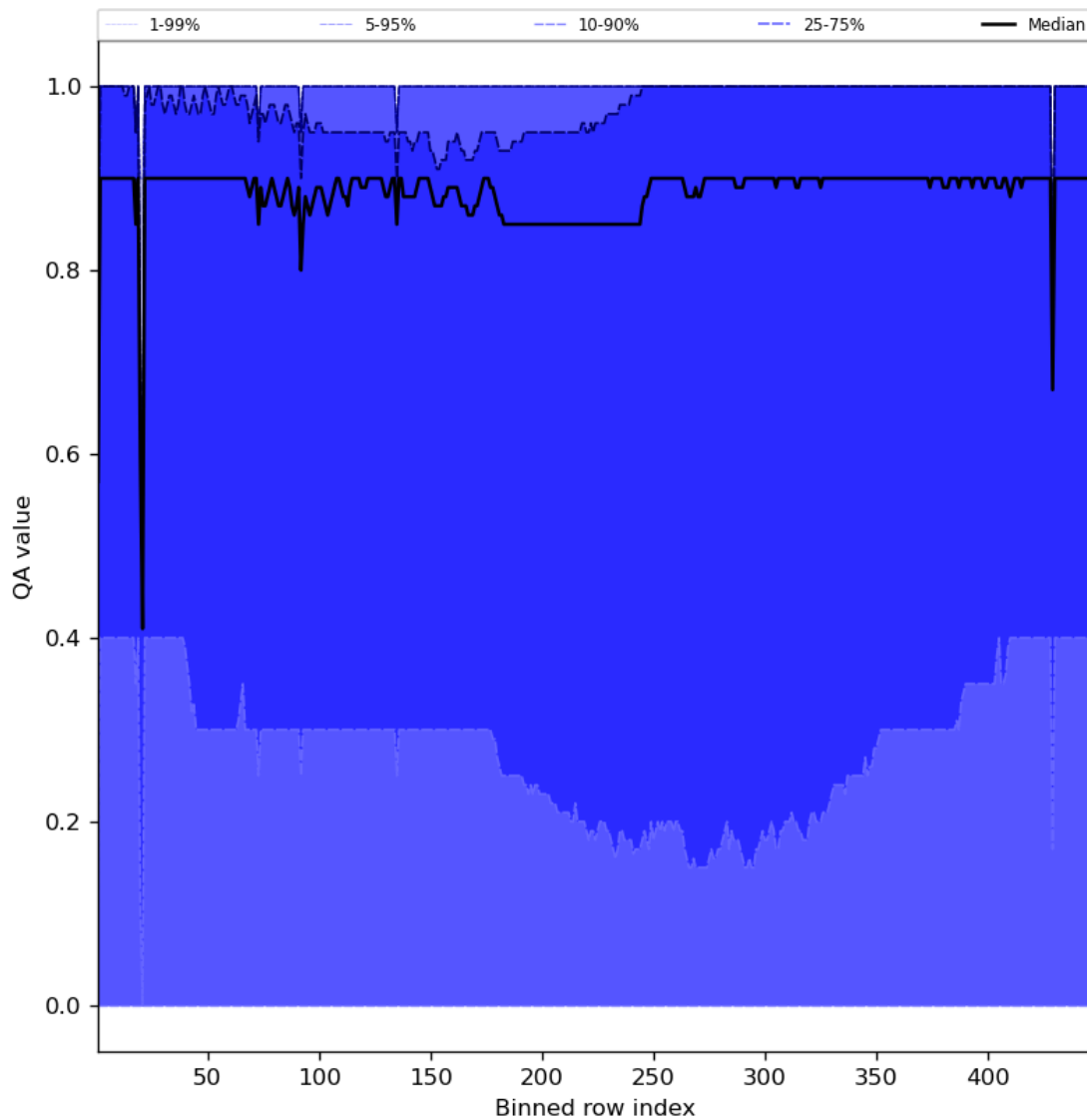
Figure 54: Along track statistics of “QA value” for 2023-09-11 to 2023-09-13
