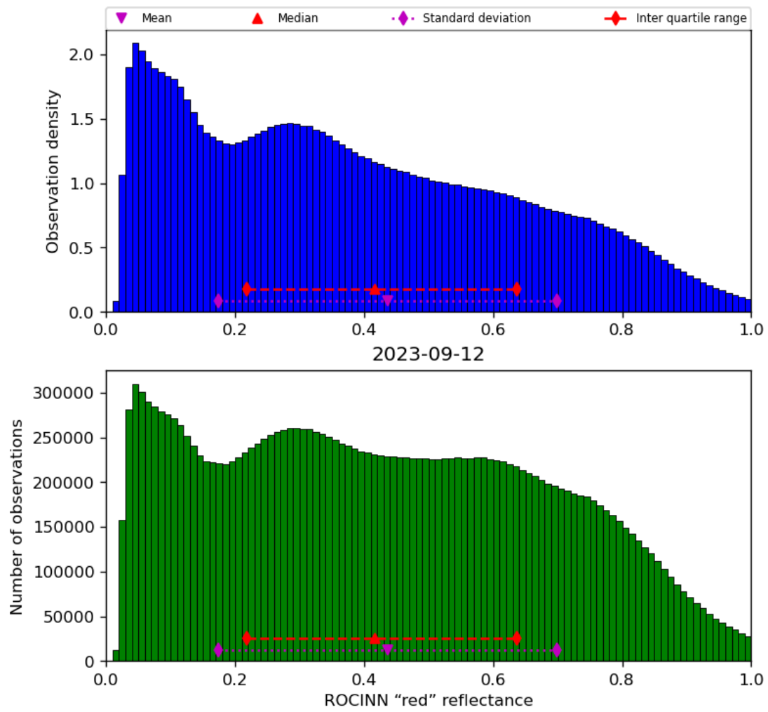
Figure 53: Histogram of “ROCINN “red” reflectance” for 2023-09-11 to 2023-09-13
