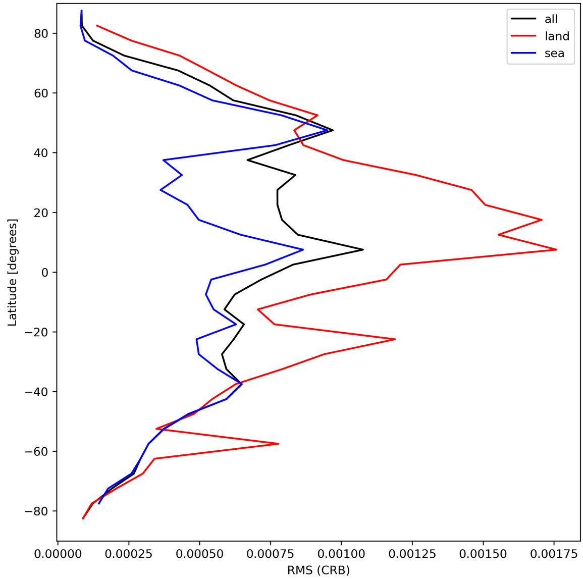
Figure 32: Zonal average of “RMS (CRB)” for 2023-09-11 to 2023-09-13.
