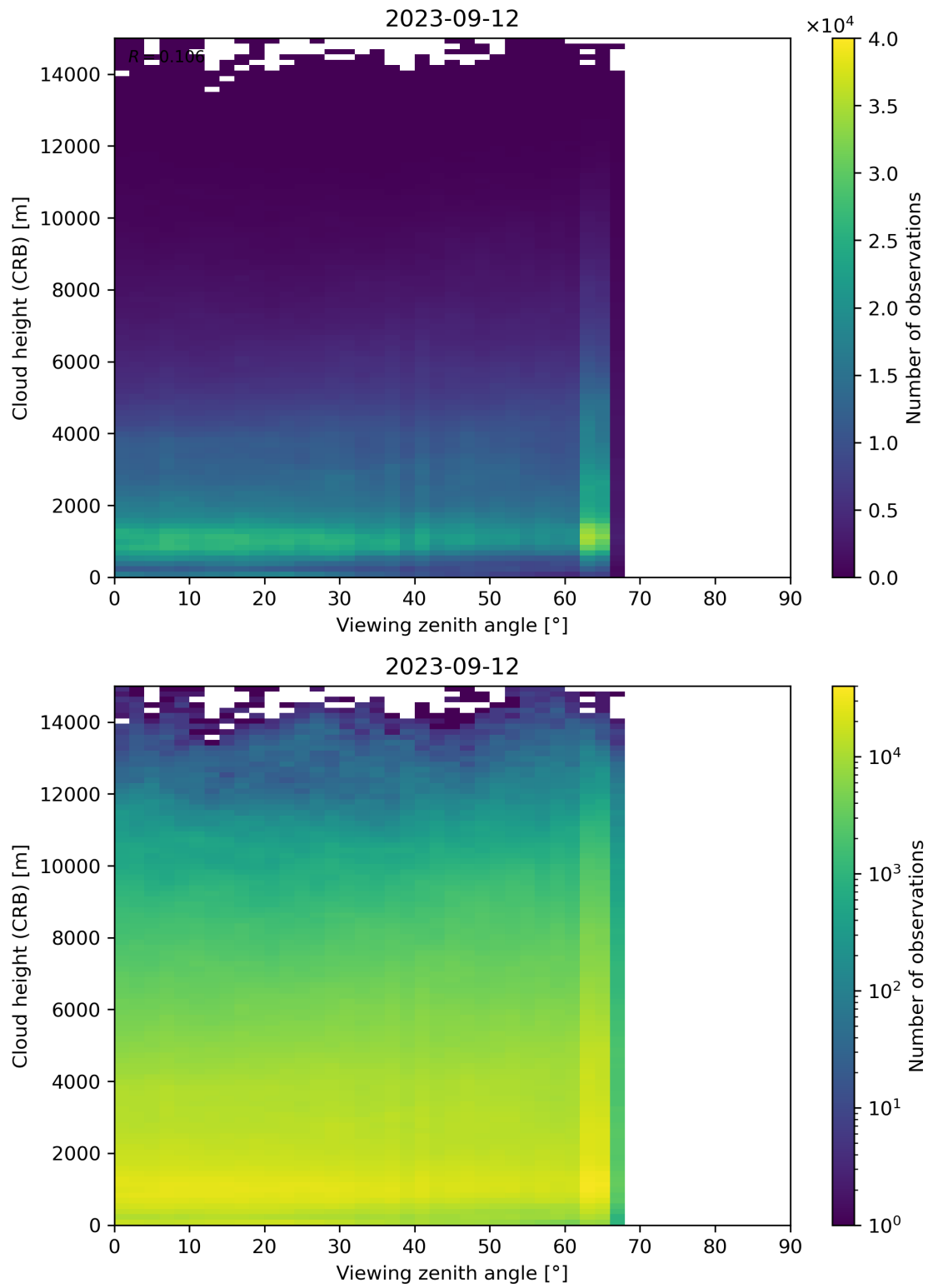
Figure 110: Scatter density plot of “Viewing zenith angle” against “Cloud height (CRB)” for 2023-09-11 to 2023-09-13.
