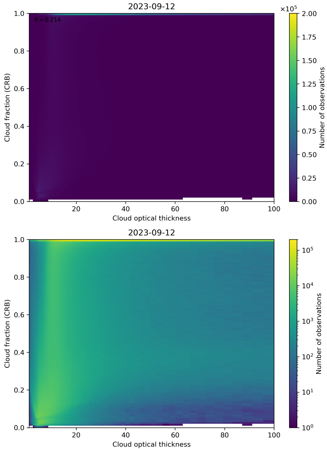
Figure 84: Scatter density plot of “Cloud optical thickness” against “Cloud fraction (CRB)” for 2023-09-11 to 2023-09-13.
