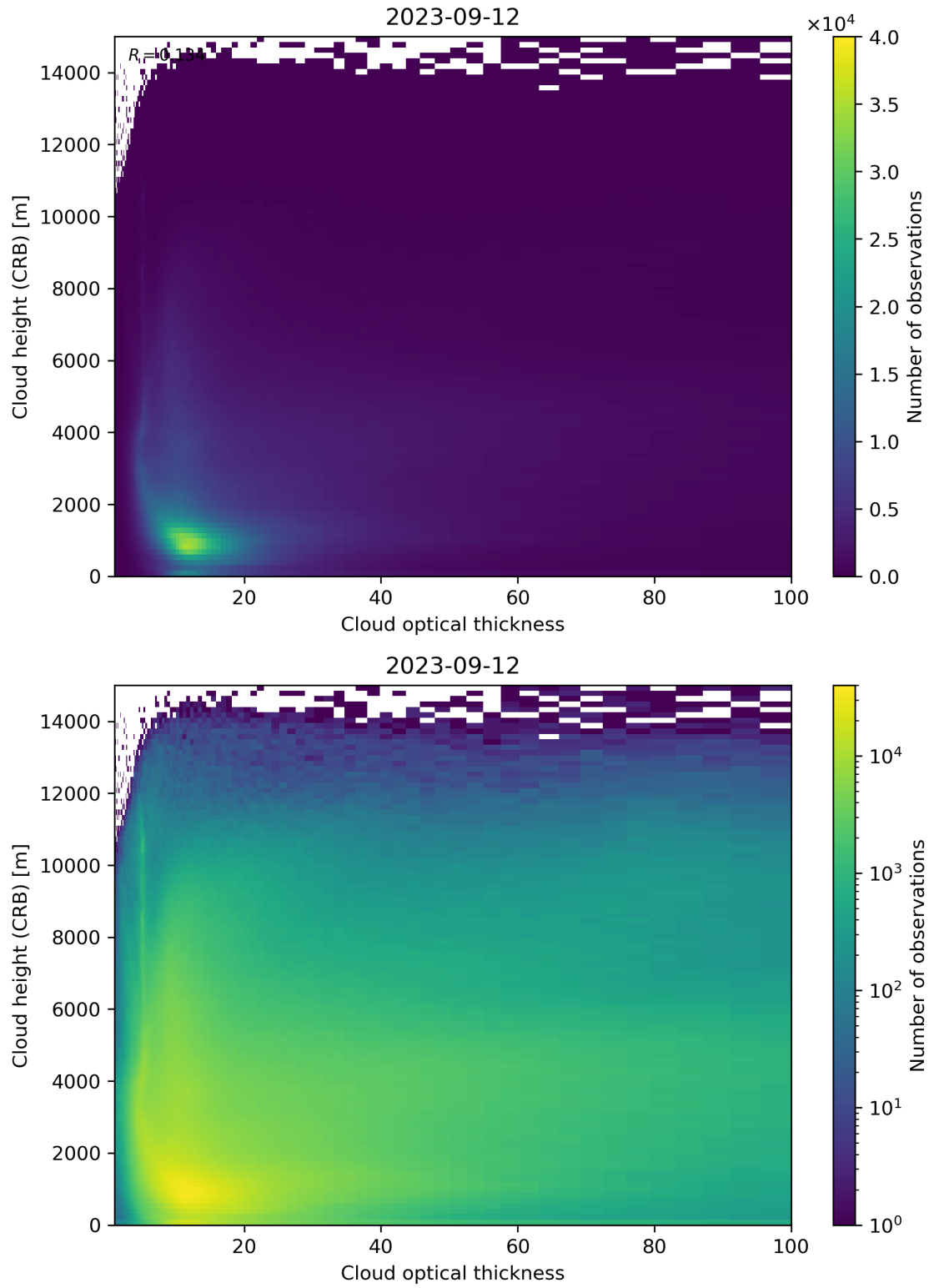
Figure 85: Scatter density plot of “Cloud optical thickness” against “Cloud height (CRB)” for 2023-09-11 to 2023-09-13.
