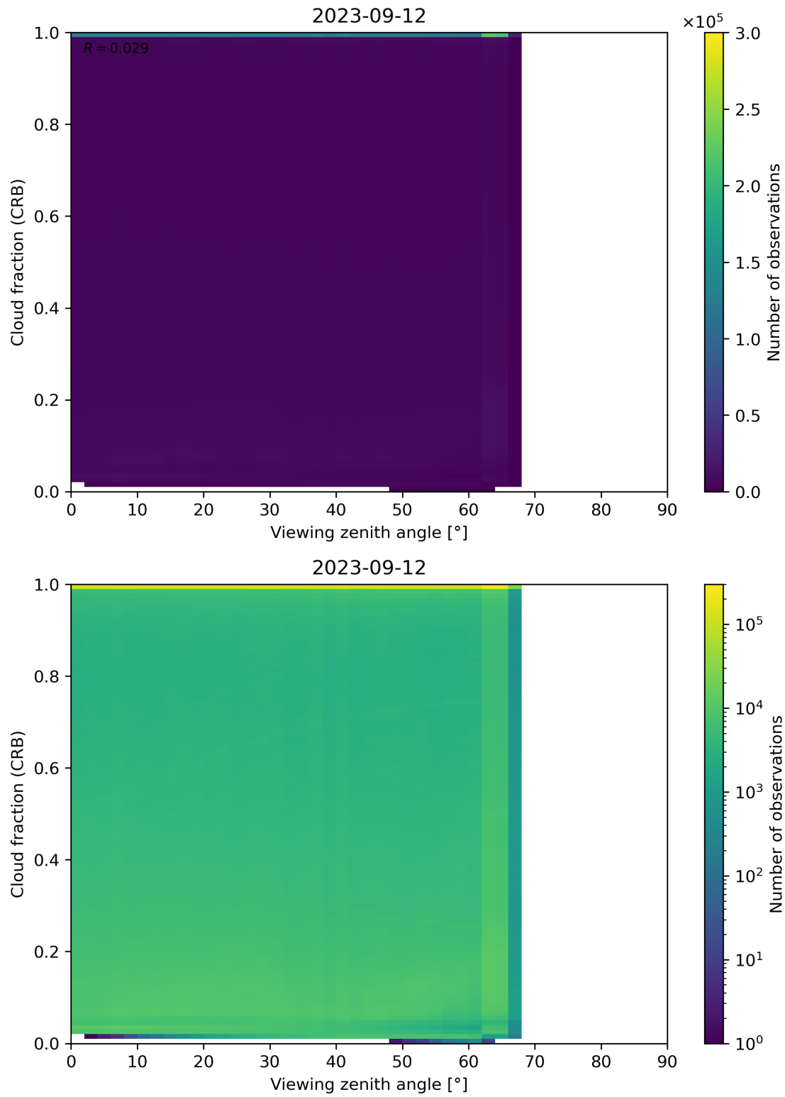
Figure 109: Scatter density plot of “Viewing zenith angle” against “Cloud fraction (CRB)” for 2023-09-11 to 2023-09-13.
