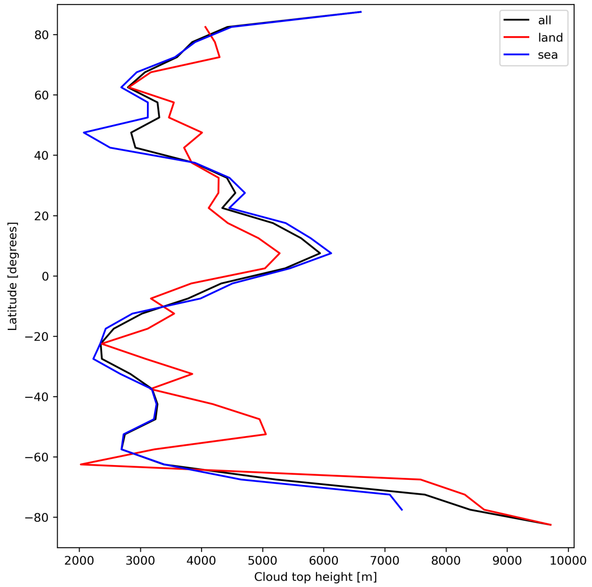
Figure 24: Zonal average of “Cloud top height” for 2023-09-11 to 2023-09-13.
