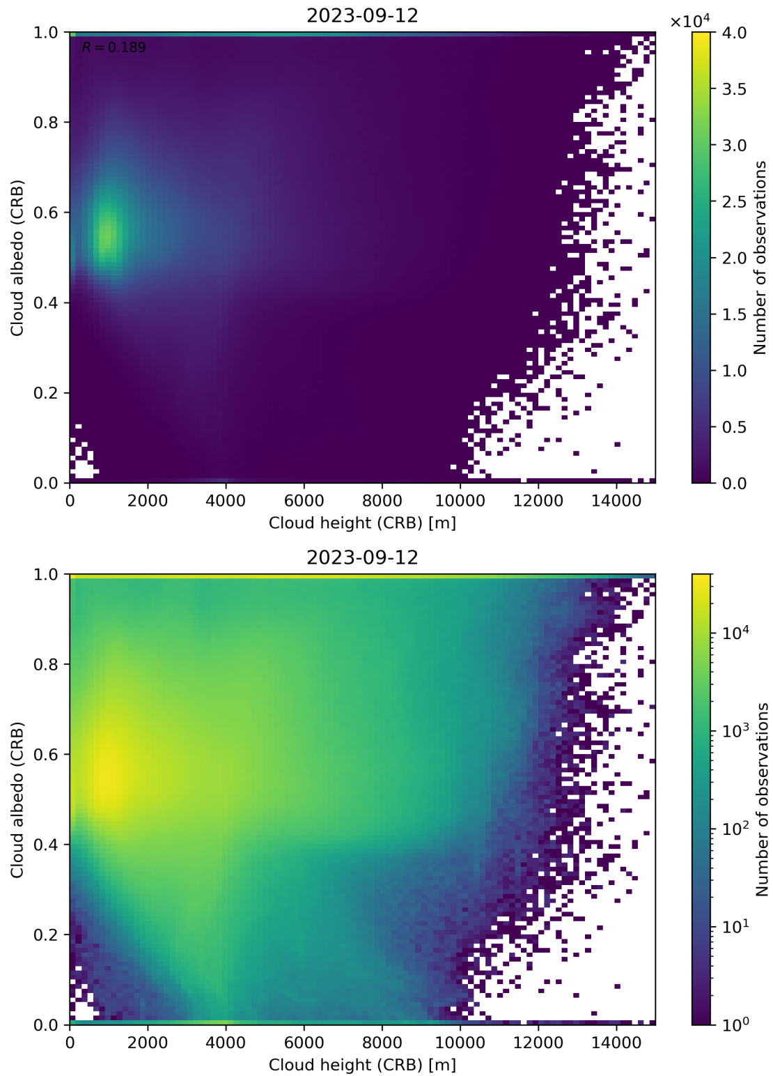
Figure 80: Scatter density plot of “Cloud height (CRB)” against “Cloud albedo (CRB)” for 2023-09-11 to 2023-09-13.
