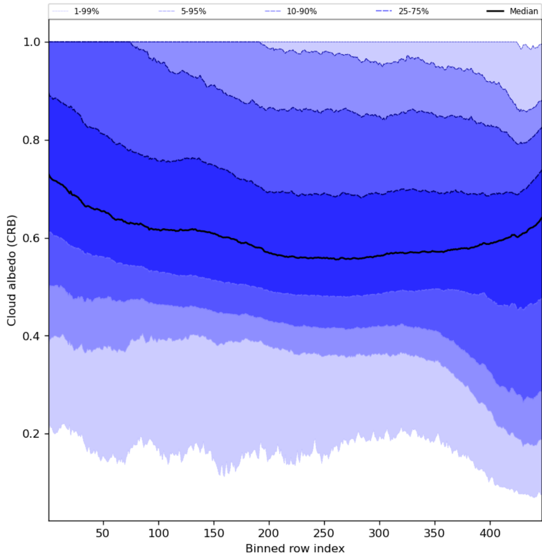
Figure 60: Along track statistics of “Cloud albedo (CRB)” for 2023-09-11 to 2023-09-13
