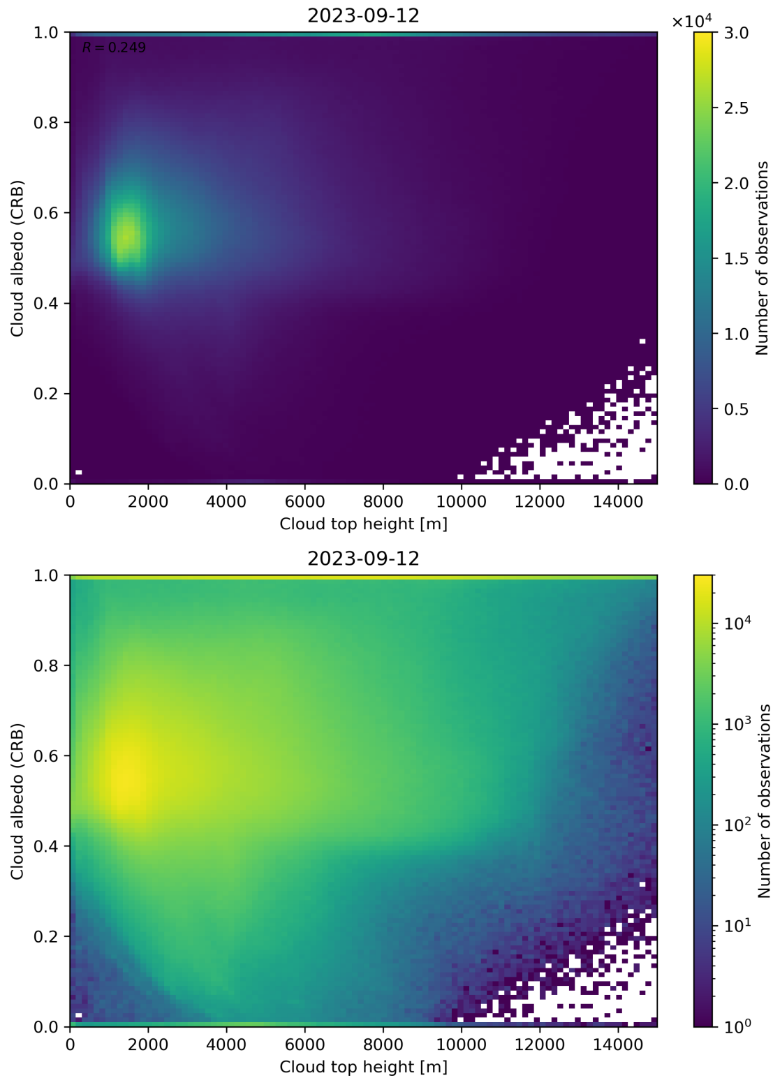
Figure 86: Scatter density plot of “Cloud top height” against “Cloud albedo (CRB)” for 2023-09-11 to 2023-09-13.
