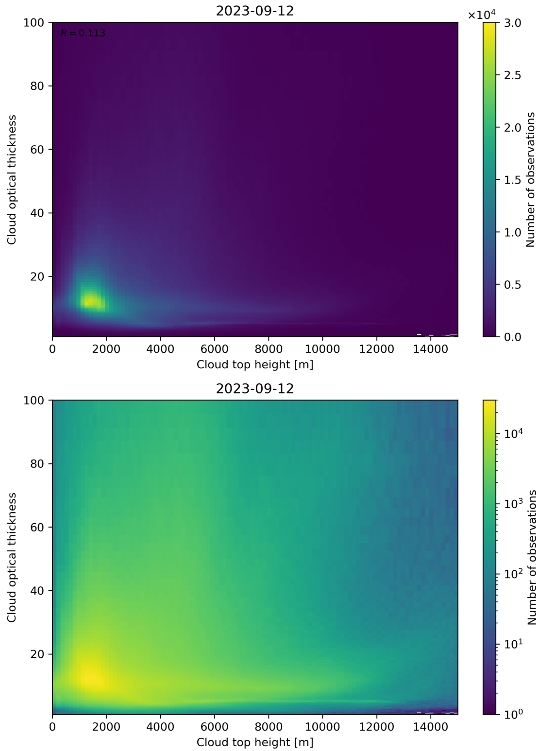
Figure 90: Scatter density plot of “Cloud top height” against “Cloud optical thickness” for 2023-09-11 to 2023-09-13.
