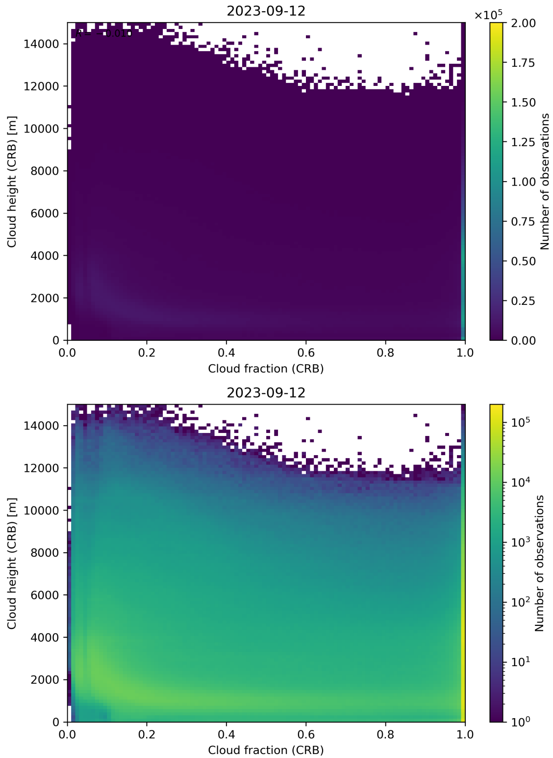
Figure 79: Scatter density plot of “Cloud fraction (CRB)” against “Cloud height (CRB)” for 2023-09-11 to 2023-09-13.
