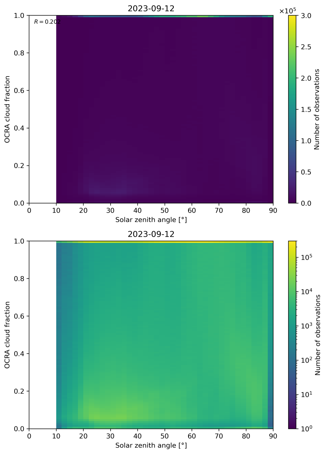
Figure 100: Scatter density plot of “Solar zenith angle” against “OCRA cloud fraction” for 2023-09-11 to 2023-09-13.
