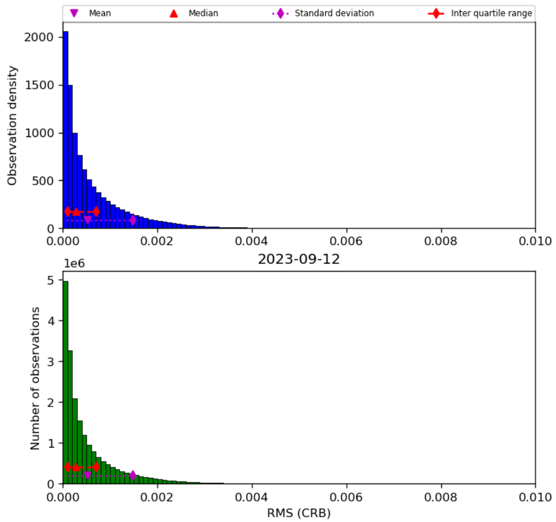
Figure 48: Histogram of “RMS (CRB)” for 2023-09-11 to 2023-09-13
