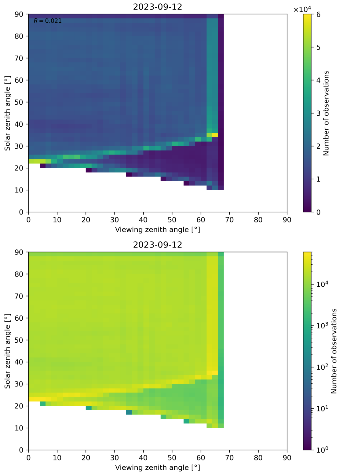
Figure 114: Scatter density plot of “Viewing zenith angle” against “Solar zenith angle” for 2023-09-11 to 2023-09-13.
