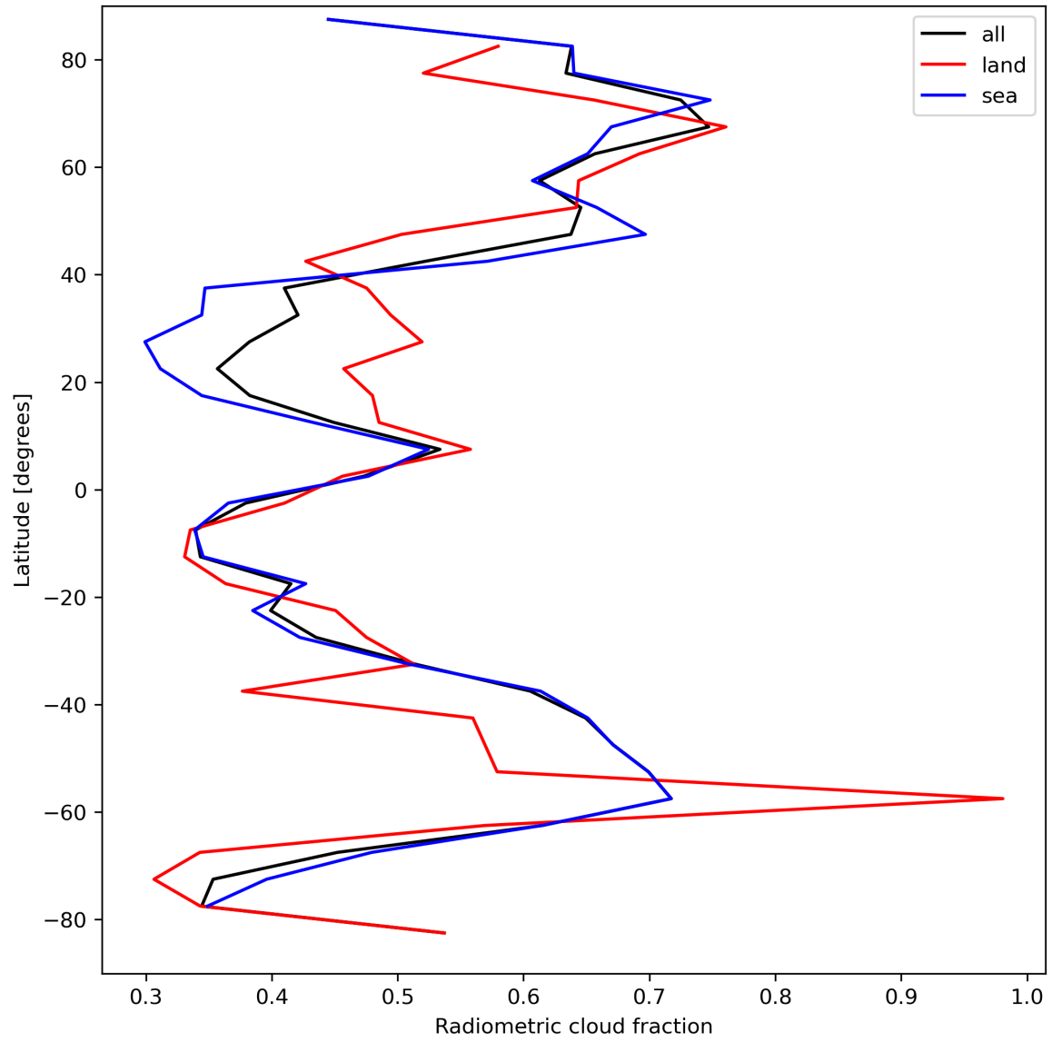
Figure 23: Zonal average of “Radiometric cloud fraction” for 2023-09-11 to 2023-09-13.
