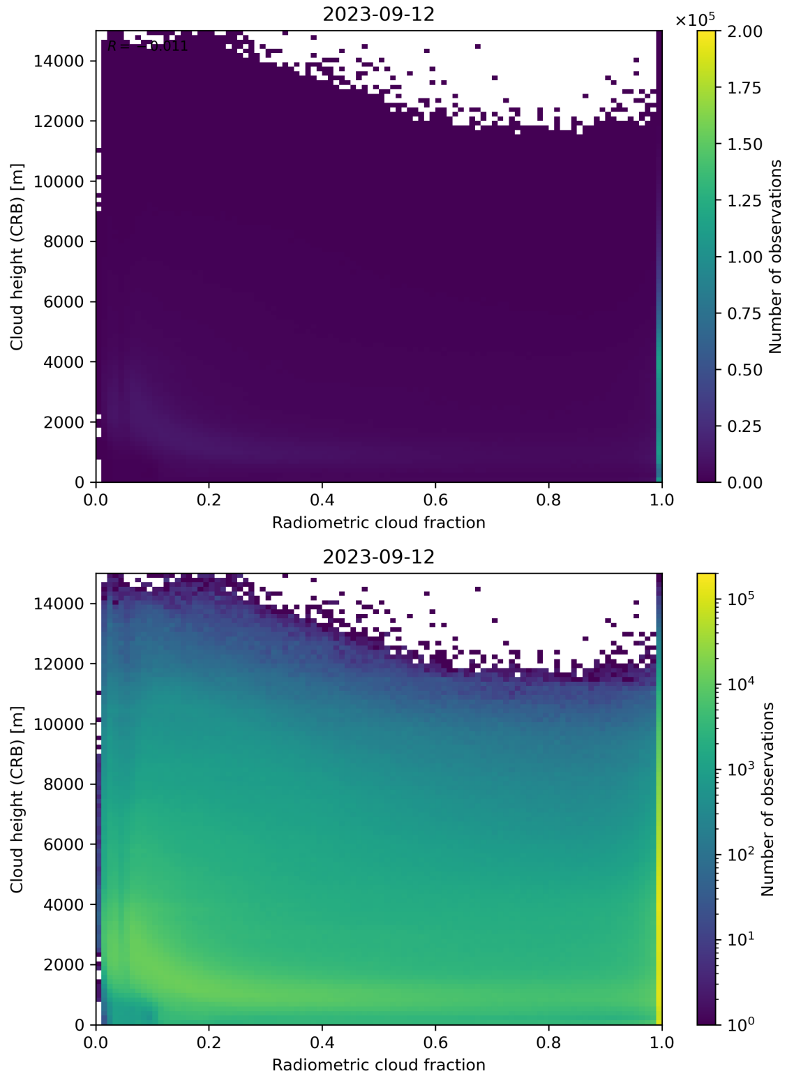
Figure 74: Scatter density plot of “Radiometric cloud fraction” against “Cloud height (CRB)” for 2023-09-11 to 2023-09-13.
