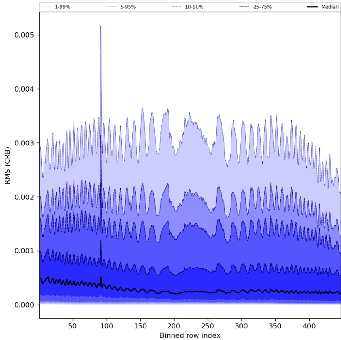
Figure 64: Along track statistics of “RMS (CRB)” for 2023-09-11 to 2023-09-13
