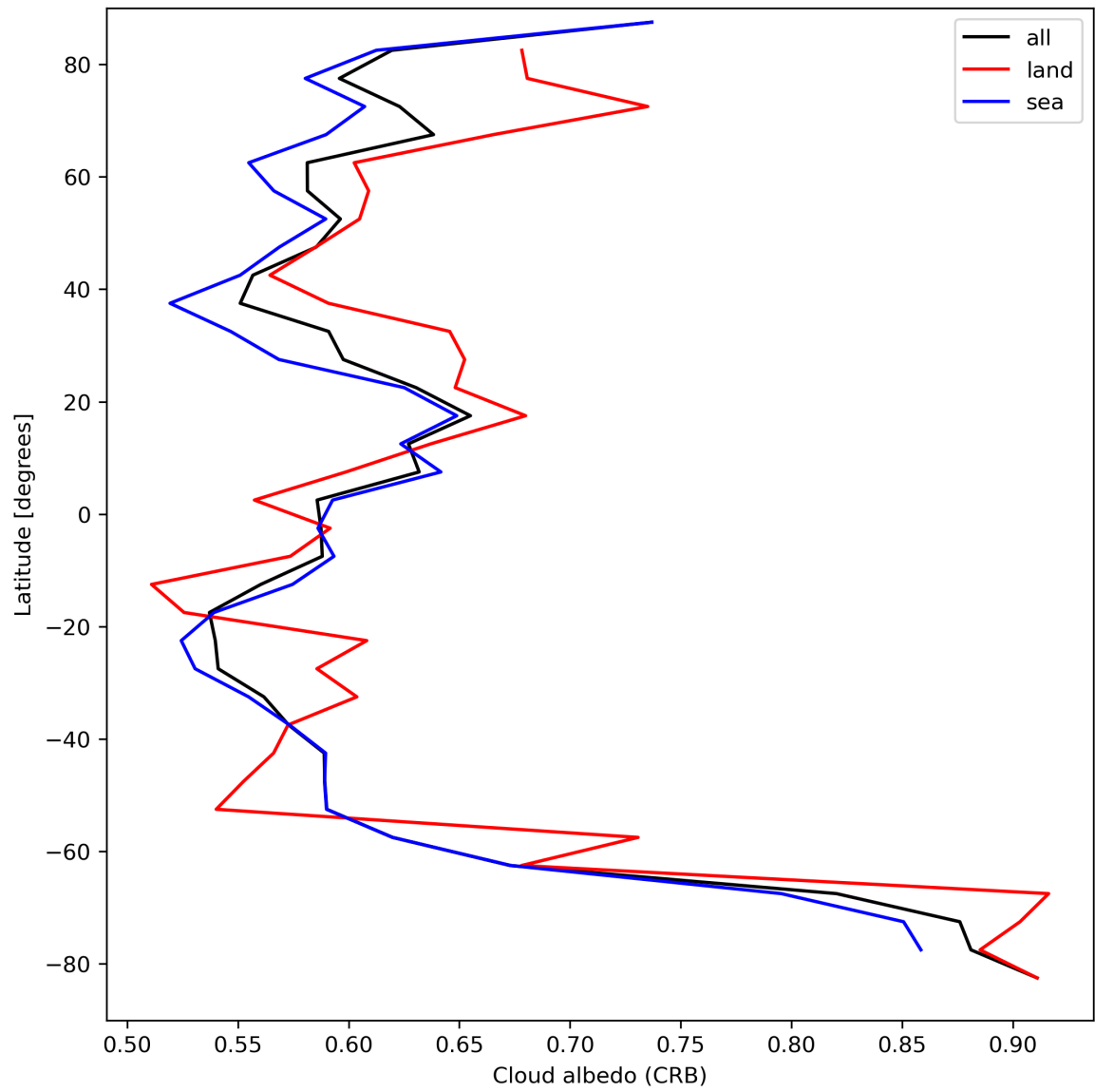
Figure 28: Zonal average of “Cloud albedo (CRB)” for 2023-09-11 to 2023-09-13.
