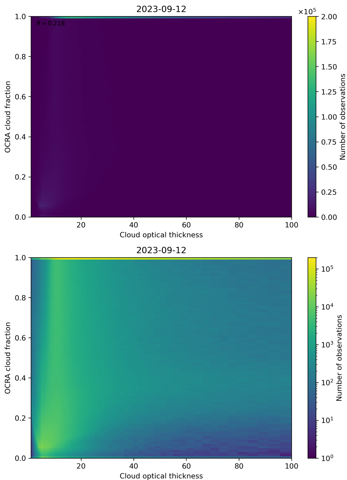
Figure 83: Scatter density plot of “Cloud optical thickness” against “OCRA cloud fraction” for 2023-09-11 to 2023-09-13.
