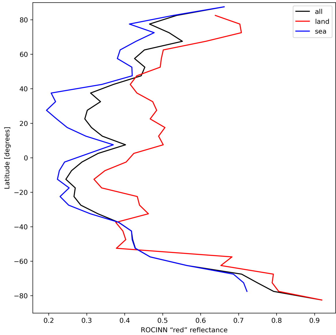
Figure 37: Zonal average of “ROCINN “red” reflectance” for 2023-09-11 to 2023-09-13.
