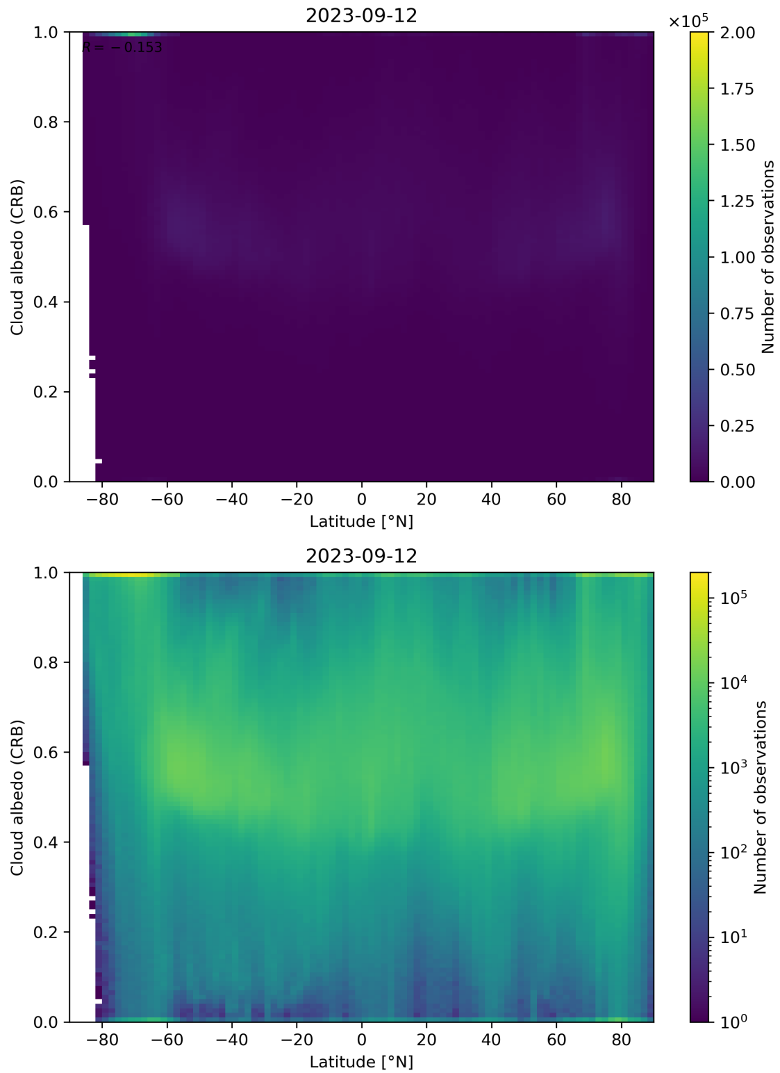
Figure 91: Scatter density plot of “Latitude” against “Cloud albedo (CRB)” for 2023-09-11 to 2023-09-13.
