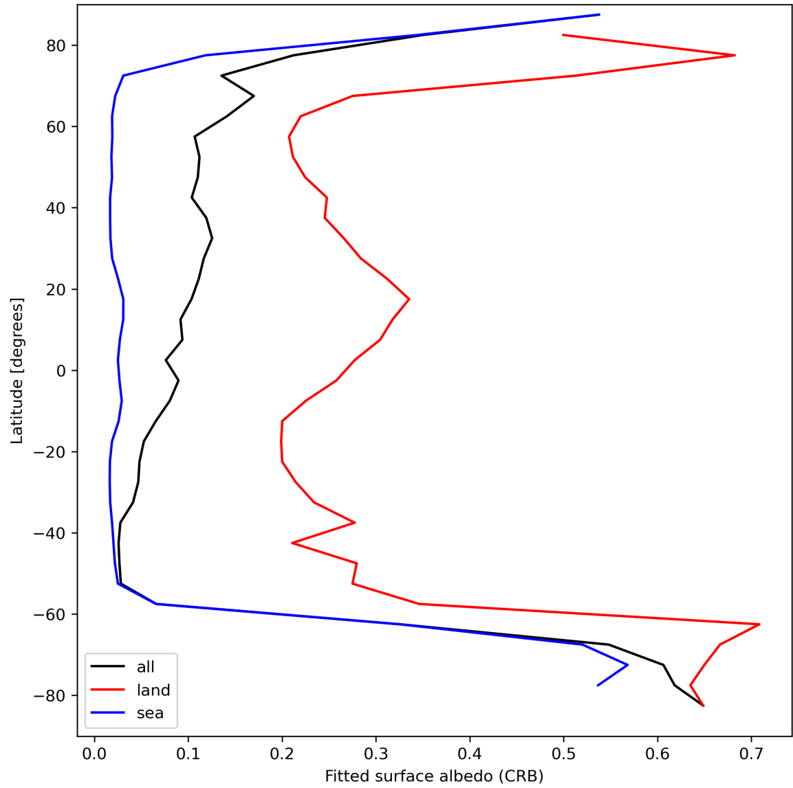
Figure 30: Zonal average of “Fitted surface albedo (CRB)” for 2023-09-11 to 2023-09-13.
