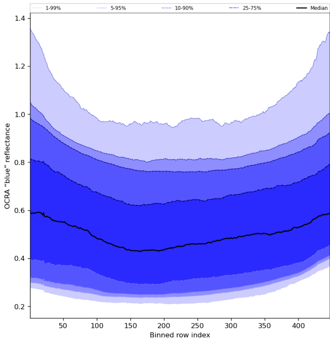
Figure 67: Along track statistics of “OCRA “blue” reflectance” for 2023-09-11 to 2023-09-13
