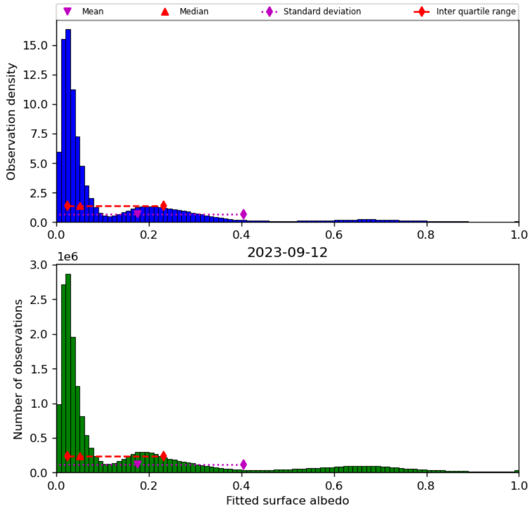
Figure 45: Histogram of “Fitted surface albedo” for 2023-09-11 to 2023-09-13
