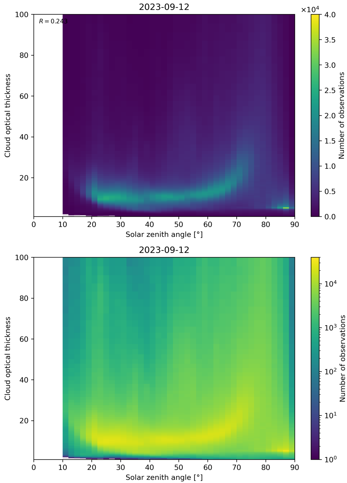
Figure 103: Scatter density plot of “Solar zenith angle” against “Cloud optical thickness” for 2023-09-11 to 2023-09-13.
