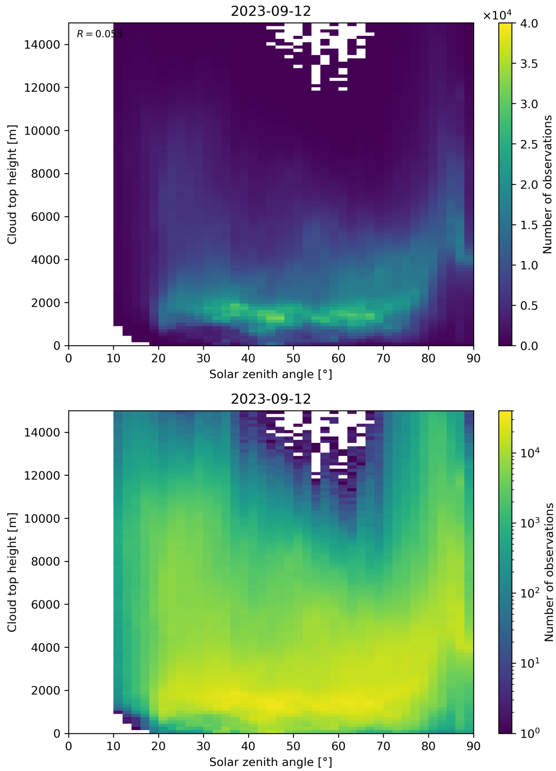
Figure 104: Scatter density plot of “Solar zenith angle” against “Cloud top height” for 2023-09-11 to 2023-09-13.
