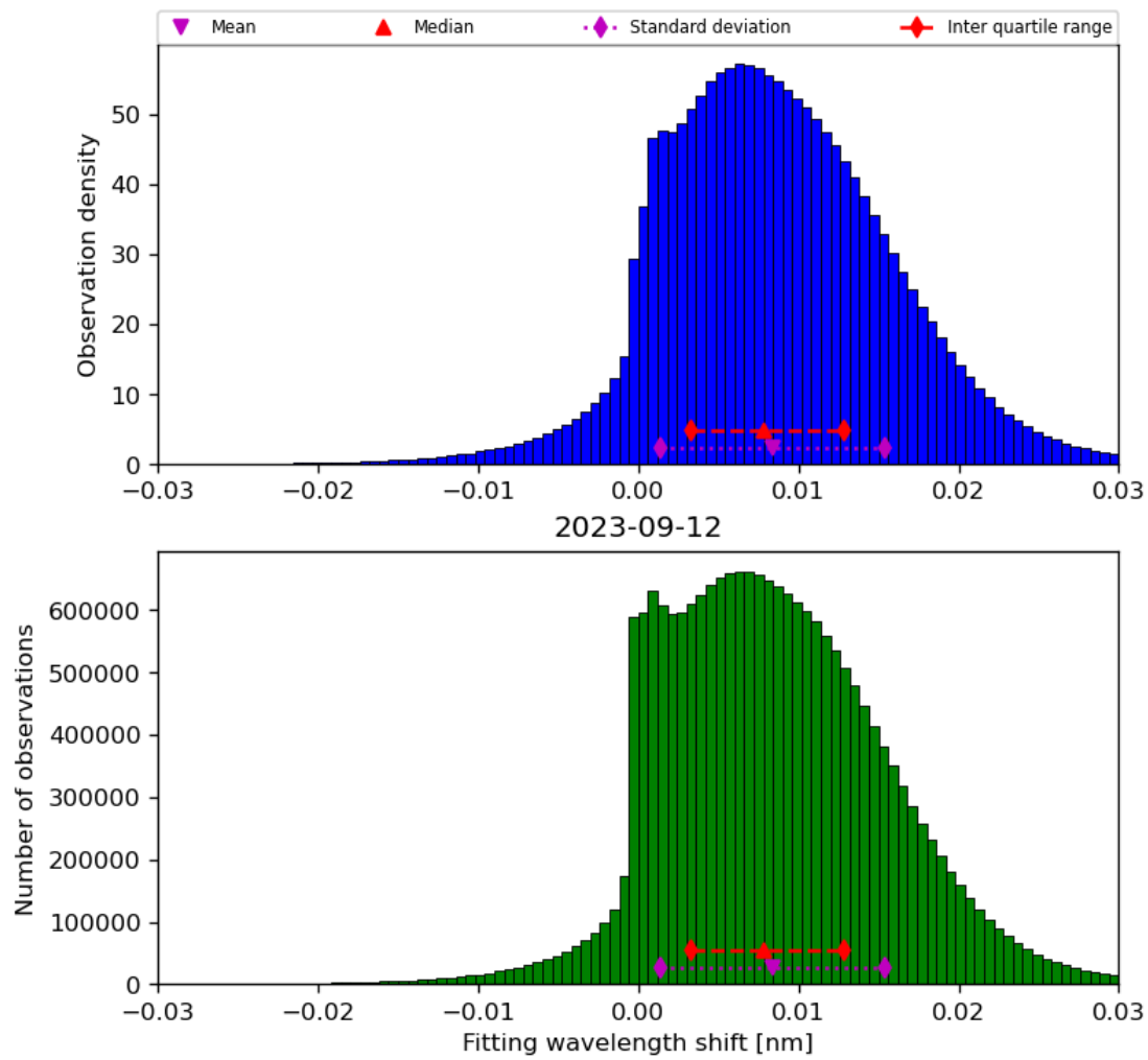
Figure 49: Histogram of “Fitting wavelength shift” for 2023-09-11 to 2023-09-13
