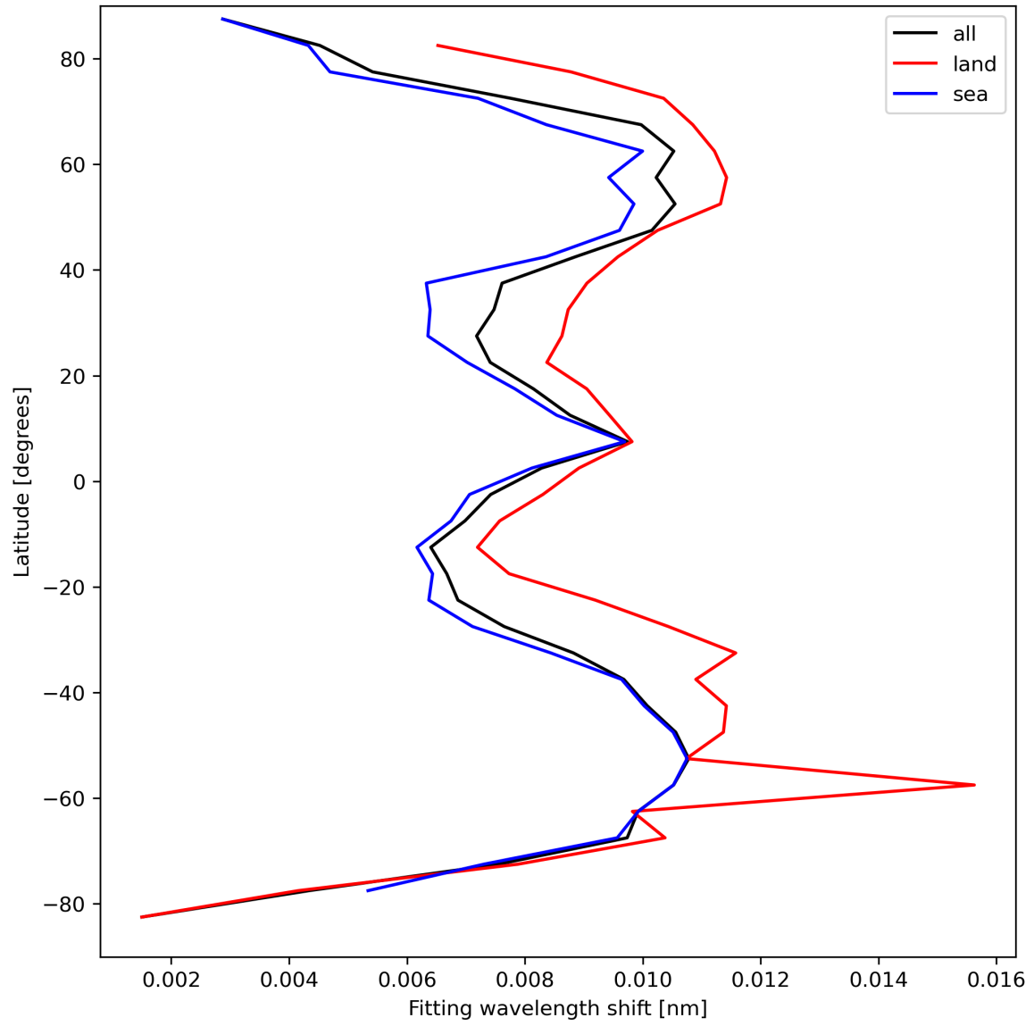
Figure 33: Zonal average of “Fitting wavelength shift” for 2023-09-11 to 2023-09-13.
