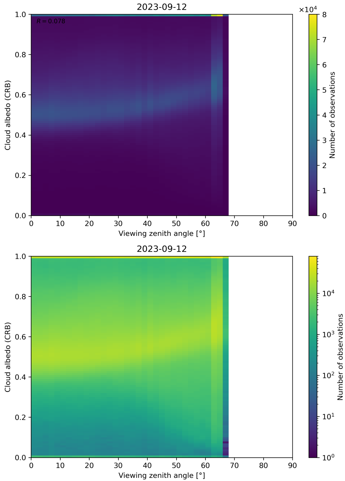
Figure 106: Scatter density plot of “Viewing zenith angle” against “Cloud albedo (CRB)” for 2023-09-11 to 2023-09-13.
