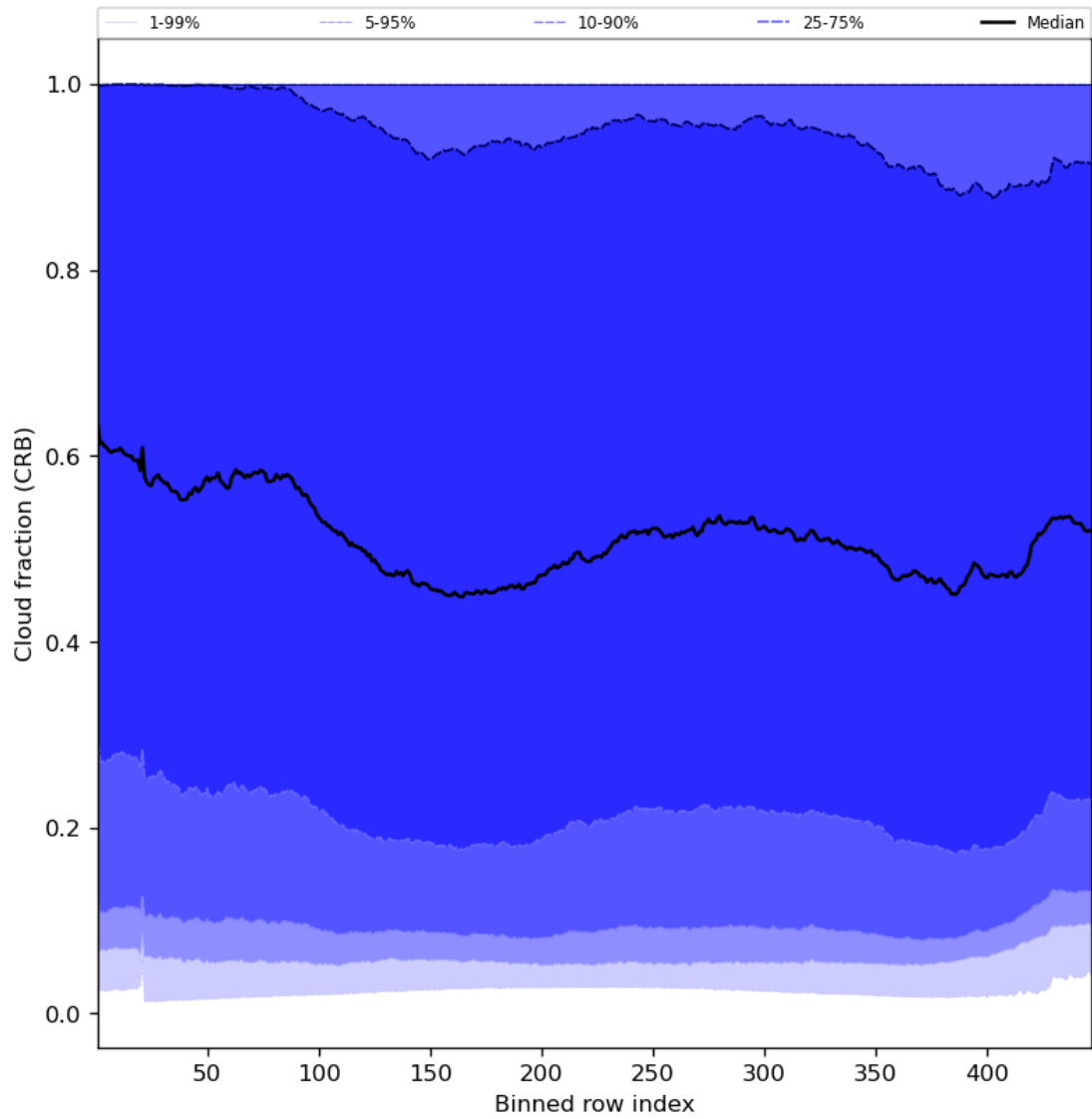
Figure 58: Along track statistics of “Cloud fraction (CRB)” for 2023-09-11 to 2023-09-13
