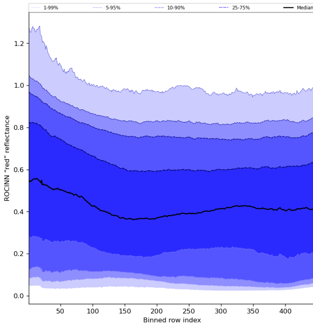
Figure 69: Along track statistics of “ROCINN “red” reflectance” for 2023-09-11 to 2023-09-13
