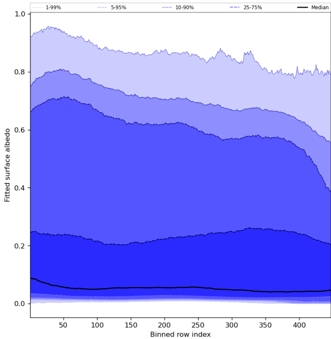
Figure 61: Along track statistics of "Fitted surface albedo" for 2023-09-11 to 2023-09-13
