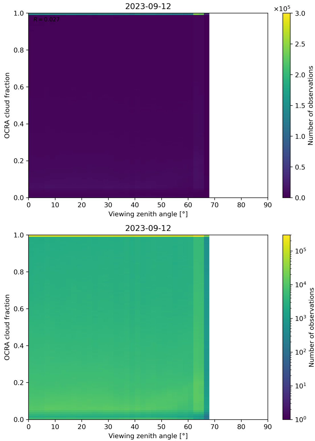
Figure 108: Scatter density plot of “Viewing zenith angle” against “OCRA cloud fraction” for 2023-09-11 to 2023-09-13.
