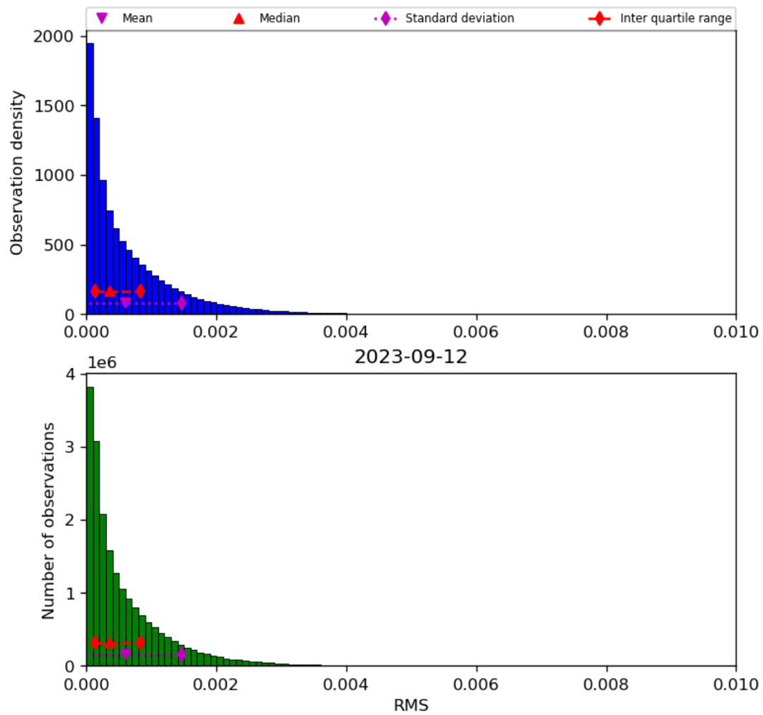
Figure 47: Histogram of “RMS” for 2023-09-11 to 2023-09-13
