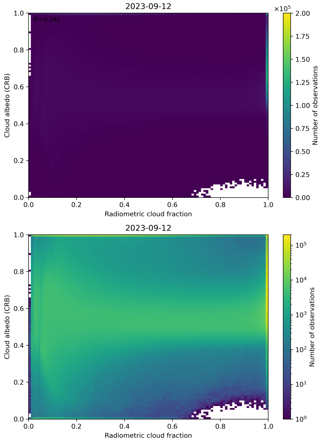
Figure 71: Scatter density plot of “Radiometric cloud fraction” against “Cloud albedo (CRB)” for 2023-09-11 to 2023-09-13.
