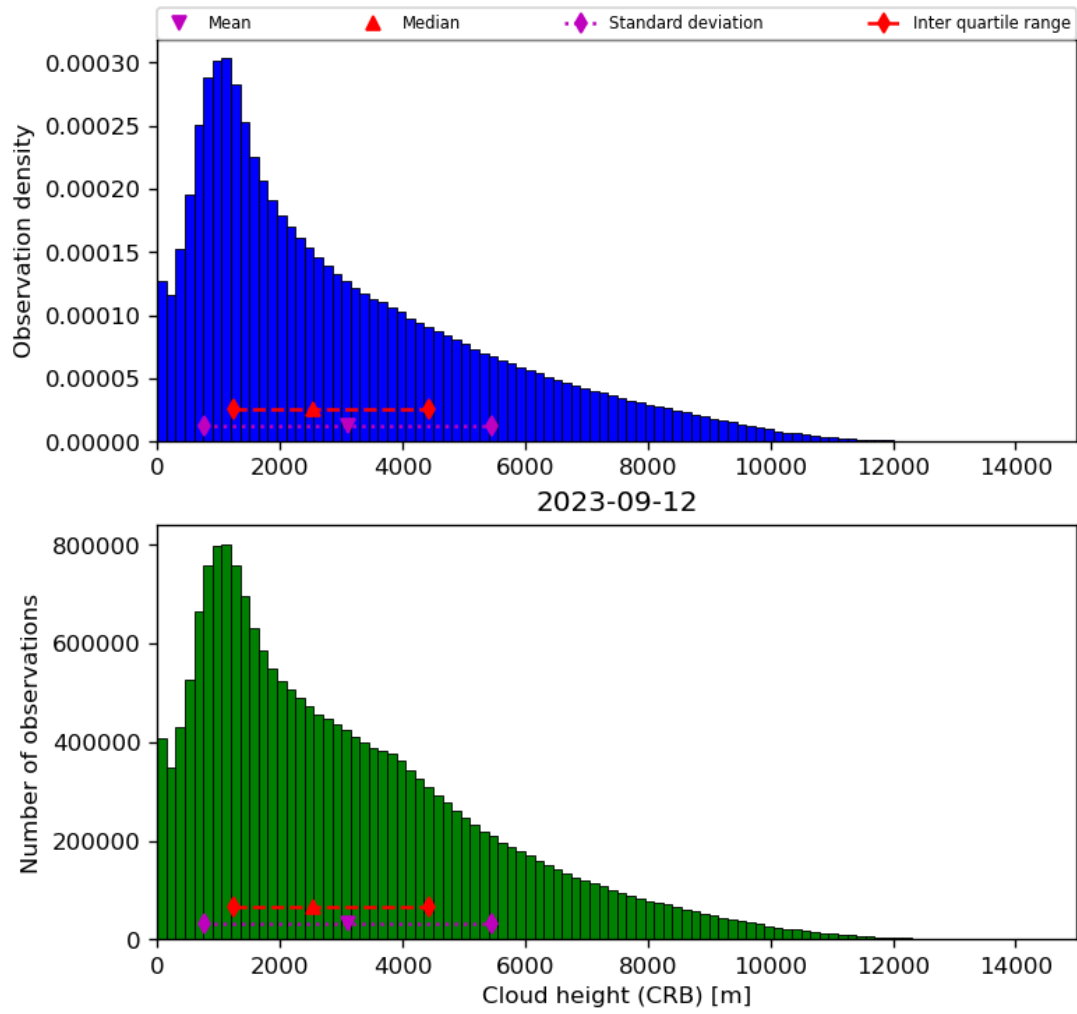
Figure 43: Histogram of “Cloud height (CRB)” for 2023-09-11 to 2023-09-13
