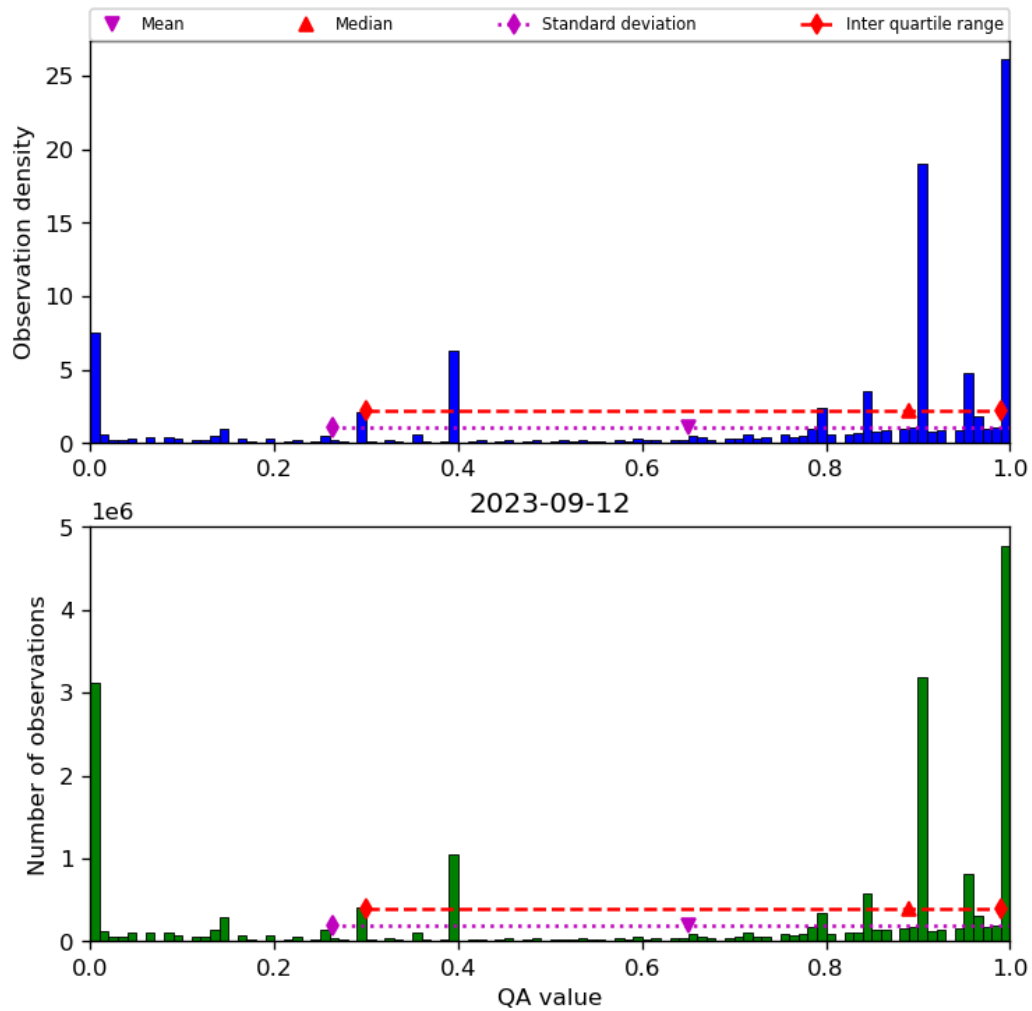
Figure 38: Histogram of “QA value” for 2023-09-11 to 2023-09-13
