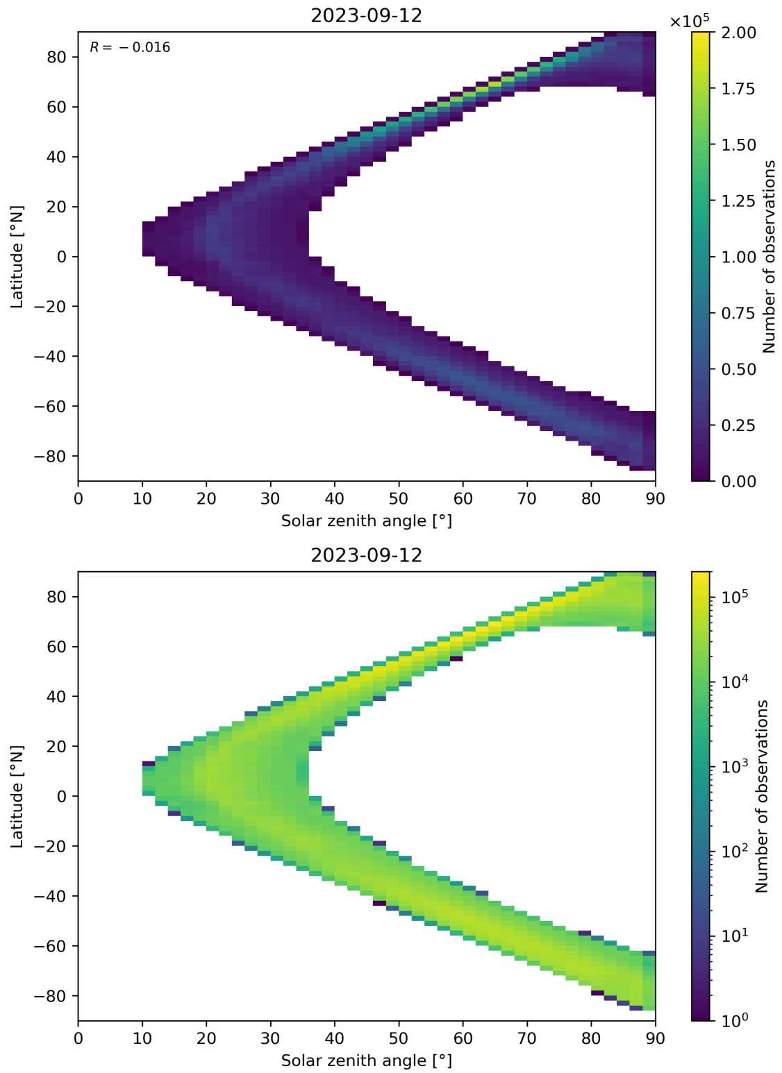
Figure 105: Scatter density plot of “Solar zenith angle” against “Latitude” for 2023-09-11 to 2023-09-13.
