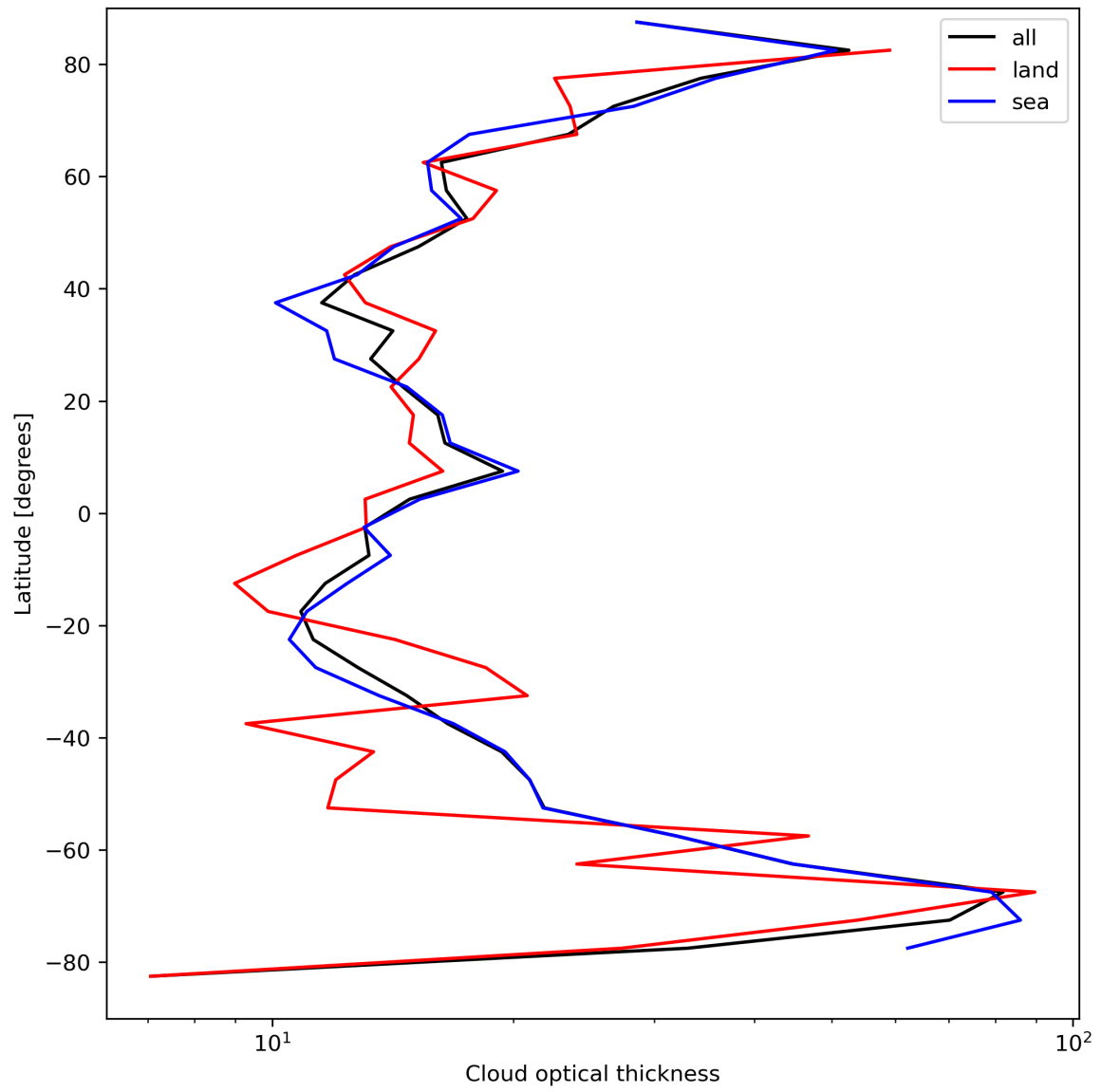
Figure 25: Zonal average of “Cloud optical thickness” for 2023-09-11 to 2023-09-13.
