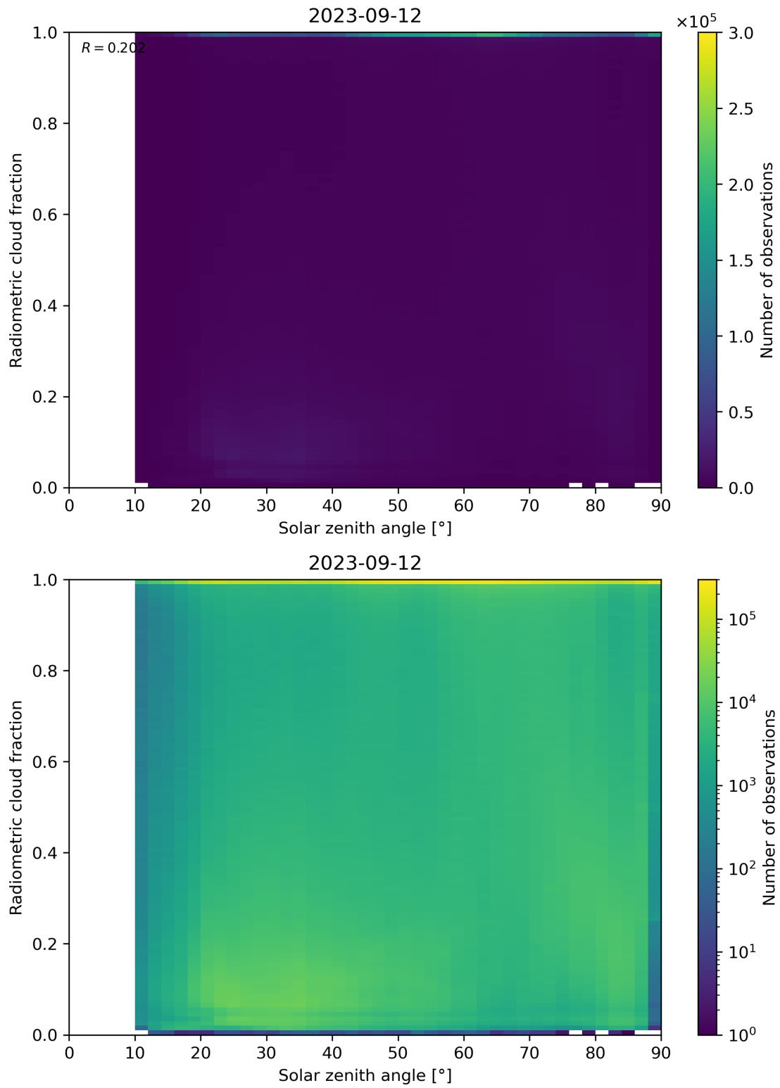
Figure 99: Scatter density plot of “Solar zenith angle” against “Radiometric cloud fraction” for 2023-09-11 to 2023-09-13.
