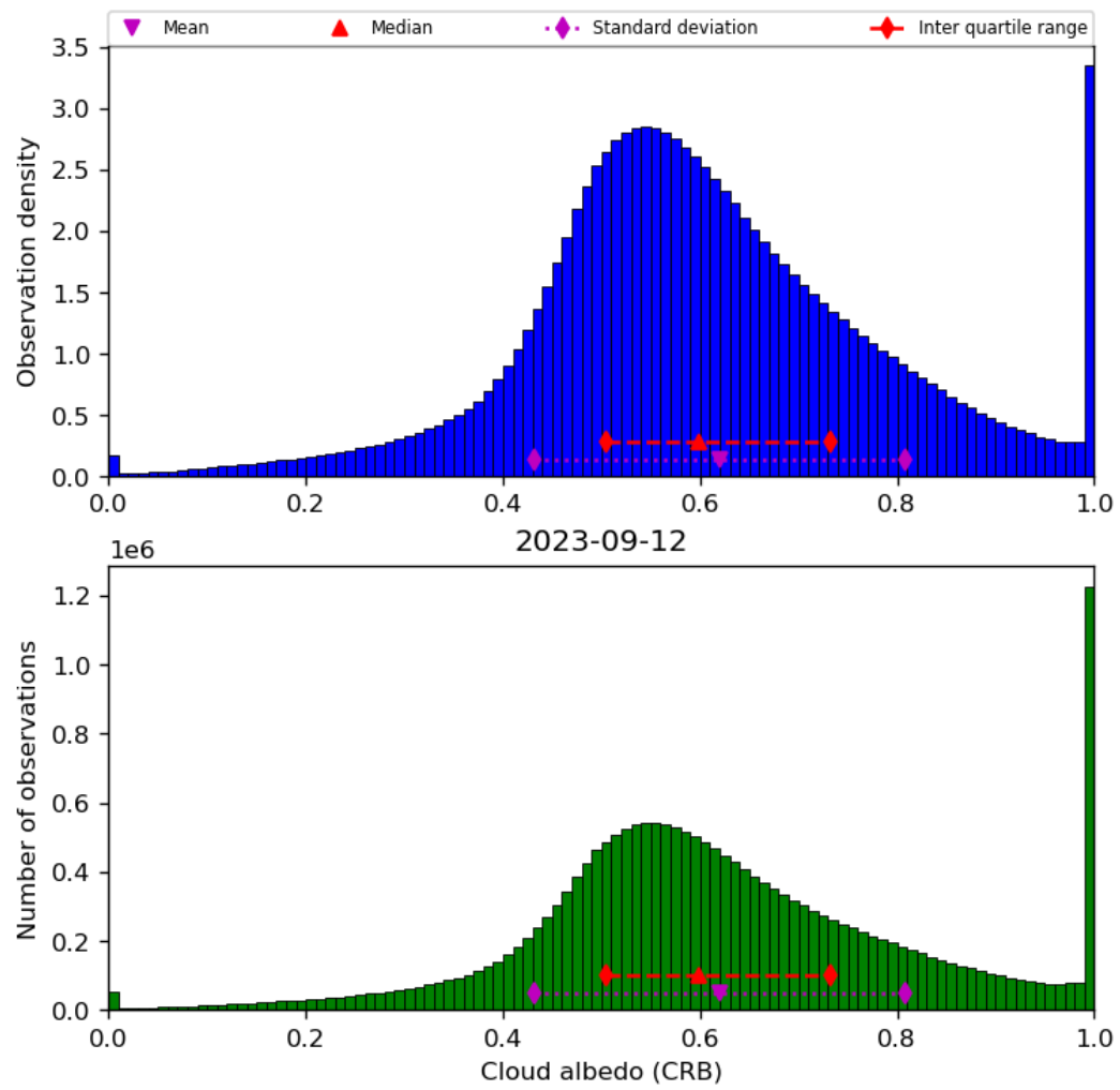
Figure 44: Histogram of “Cloud albedo (CRB)” for 2023-09-11 to 2023-09-13
