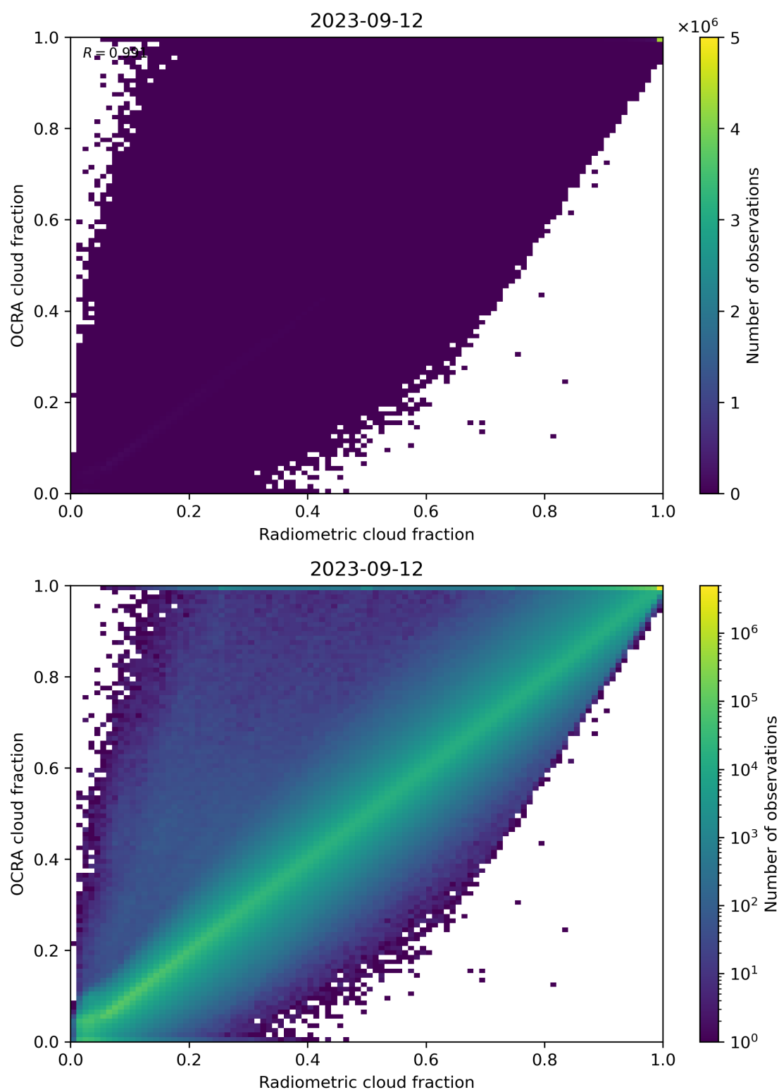
Figure 72: Scatter density plot of “Radiometric cloud fraction” against “OCRA cloud fraction” for 2023-09-11 to 2023-09-13.
