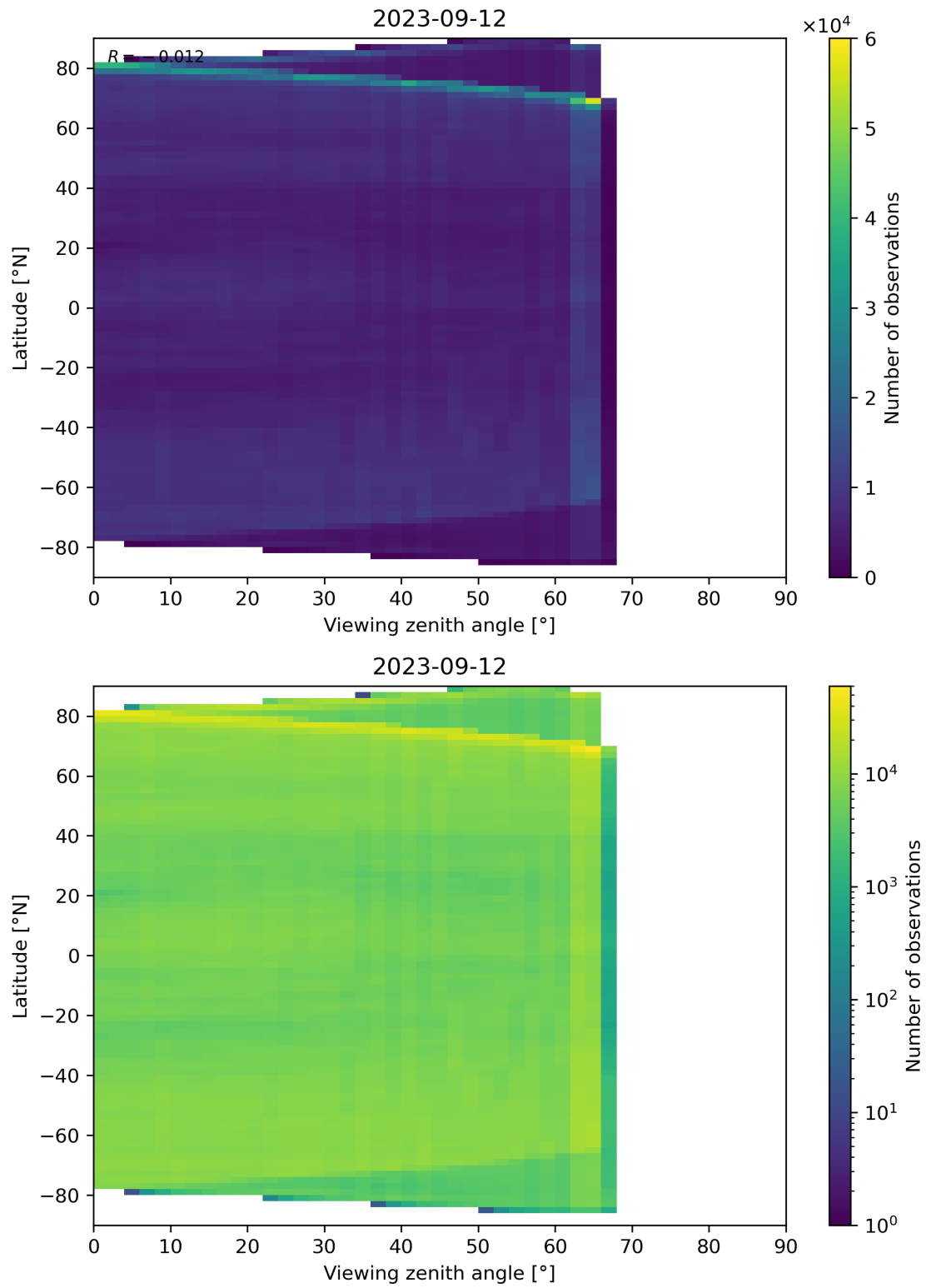
Figure 113: Scatter density plot of “Viewing zenith angle” against “Latitude” for 2023-09-11 to 2023-09-13.
