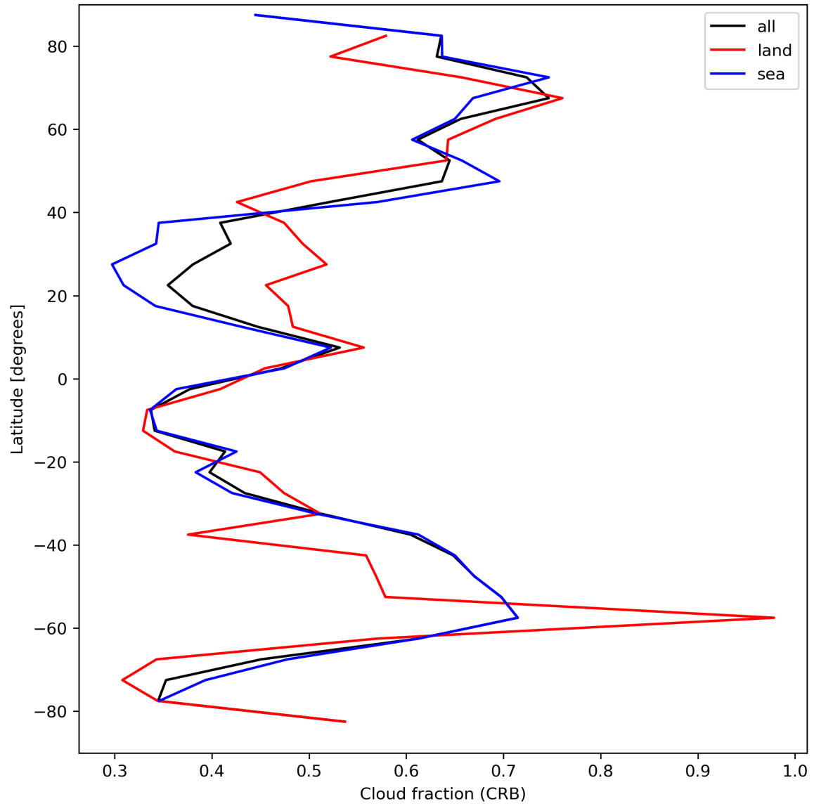
Figure 26: Zonal average of “Cloud fraction (CRB)” for 2023-09-11 to 2023-09-13.
