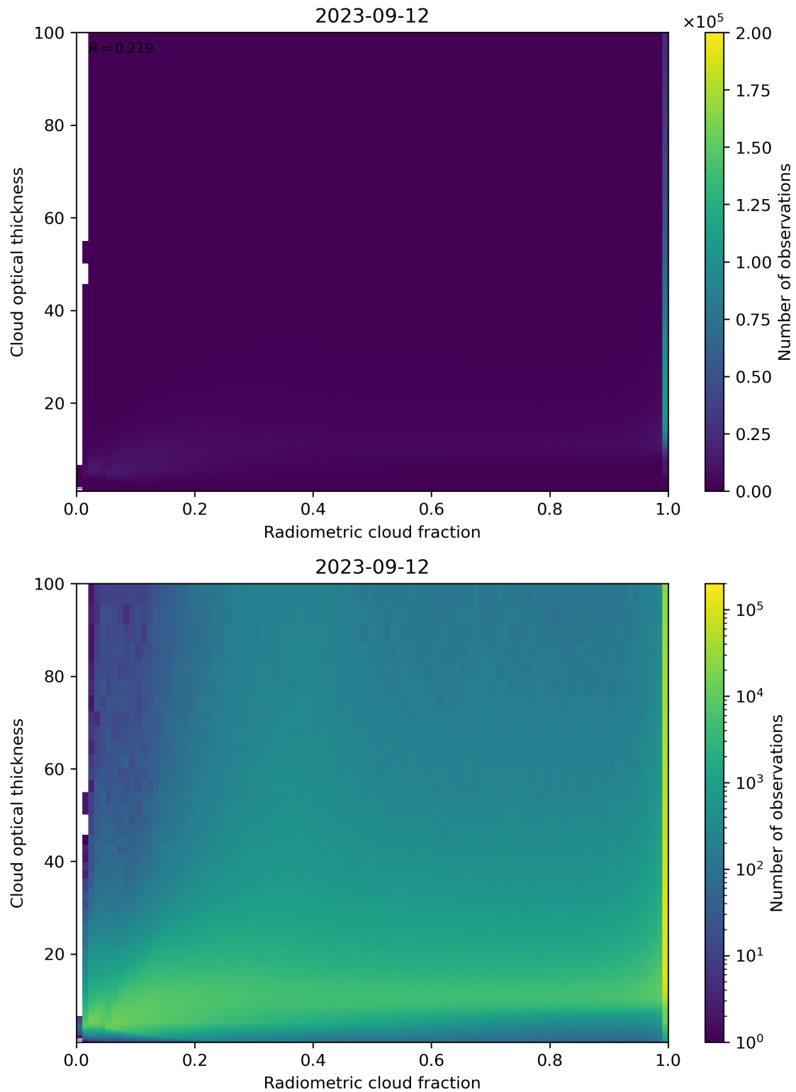
Figure 75: Scatter density plot of “Radiometric cloud fraction” against “Cloud optical thickness” for 2023-09-11 to 2023-09-13.
