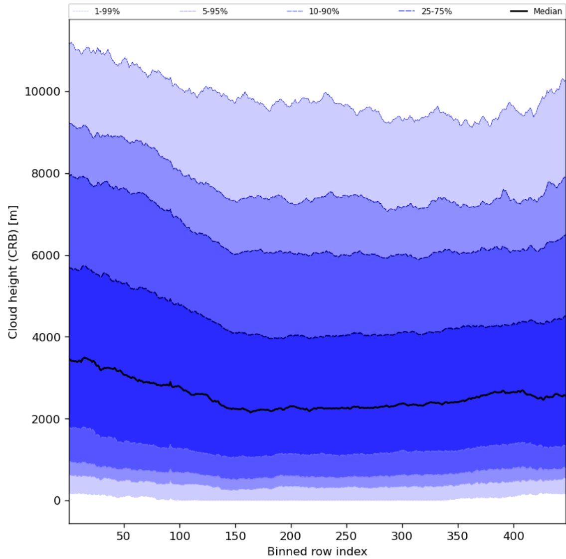
Figure 59: Along track statistics of “Cloud height (CRB)” for 2023-09-11 to 2023-09-13
