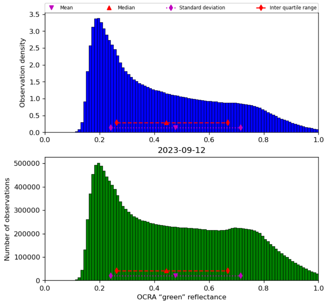
Figure 52: Histogram of “OCRA “green” reflectance” for 2023-09-11 to 2023-09-13
