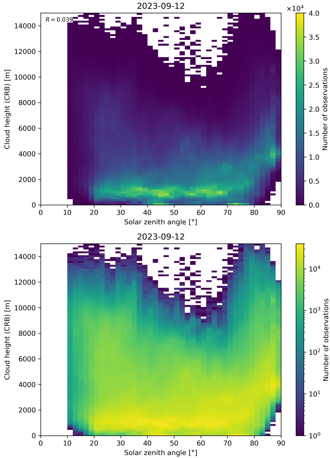
Figure 102: Scatter density plot of “Solar zenith angle” against “Cloud height (CRB)” for 2023-09-11 to 2023-09-13.
