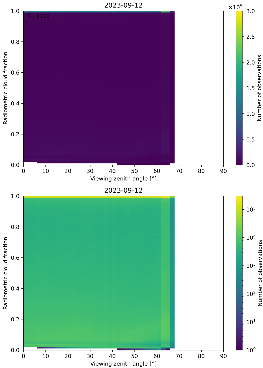
Figure 107: Scatter density plot of “Viewing zenith angle” against “Radiometric cloud fraction” for 2023-09-11 to 2023-09-13.
