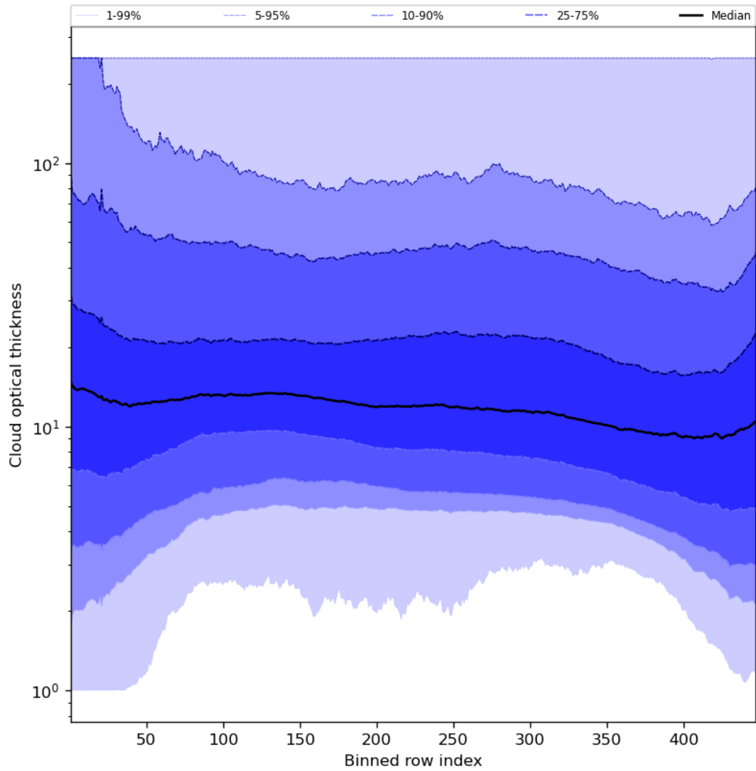
Figure 57: Along track statistics of “Cloud optical thickness” for 2023-09-11 to 2023-09-13
