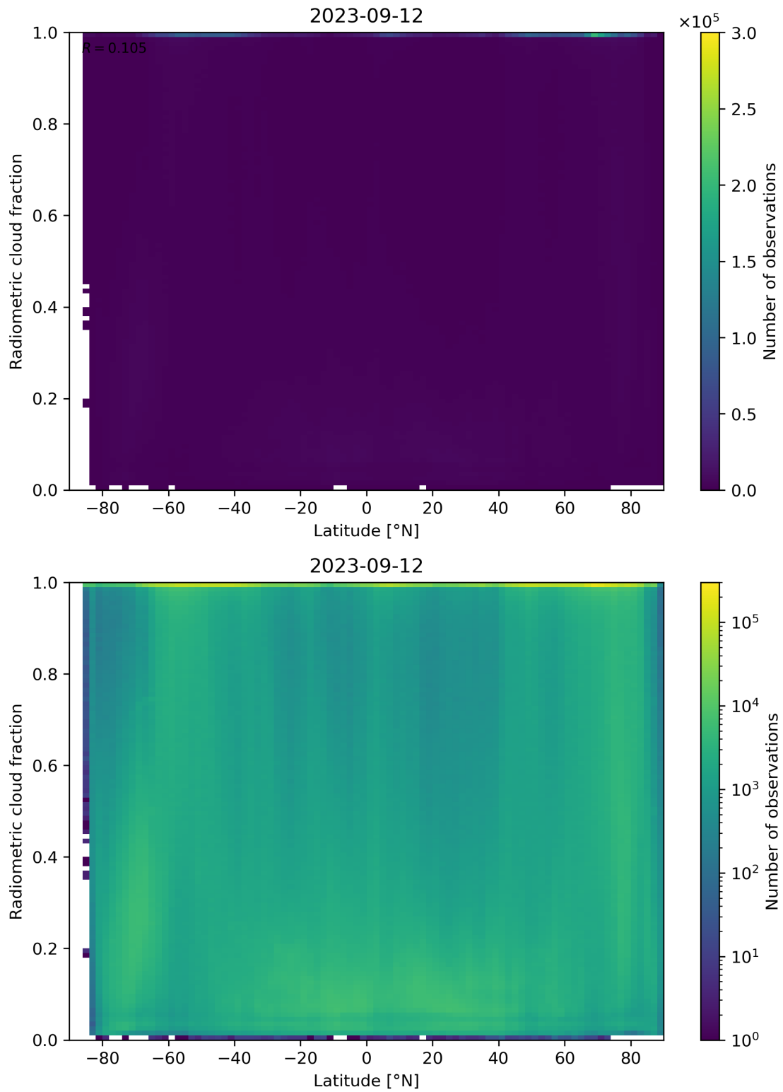
Figure 92: Scatter density plot of “Latitude” against “Radiometric cloud fraction” for 2023-09-11 to 2023-09-13.
