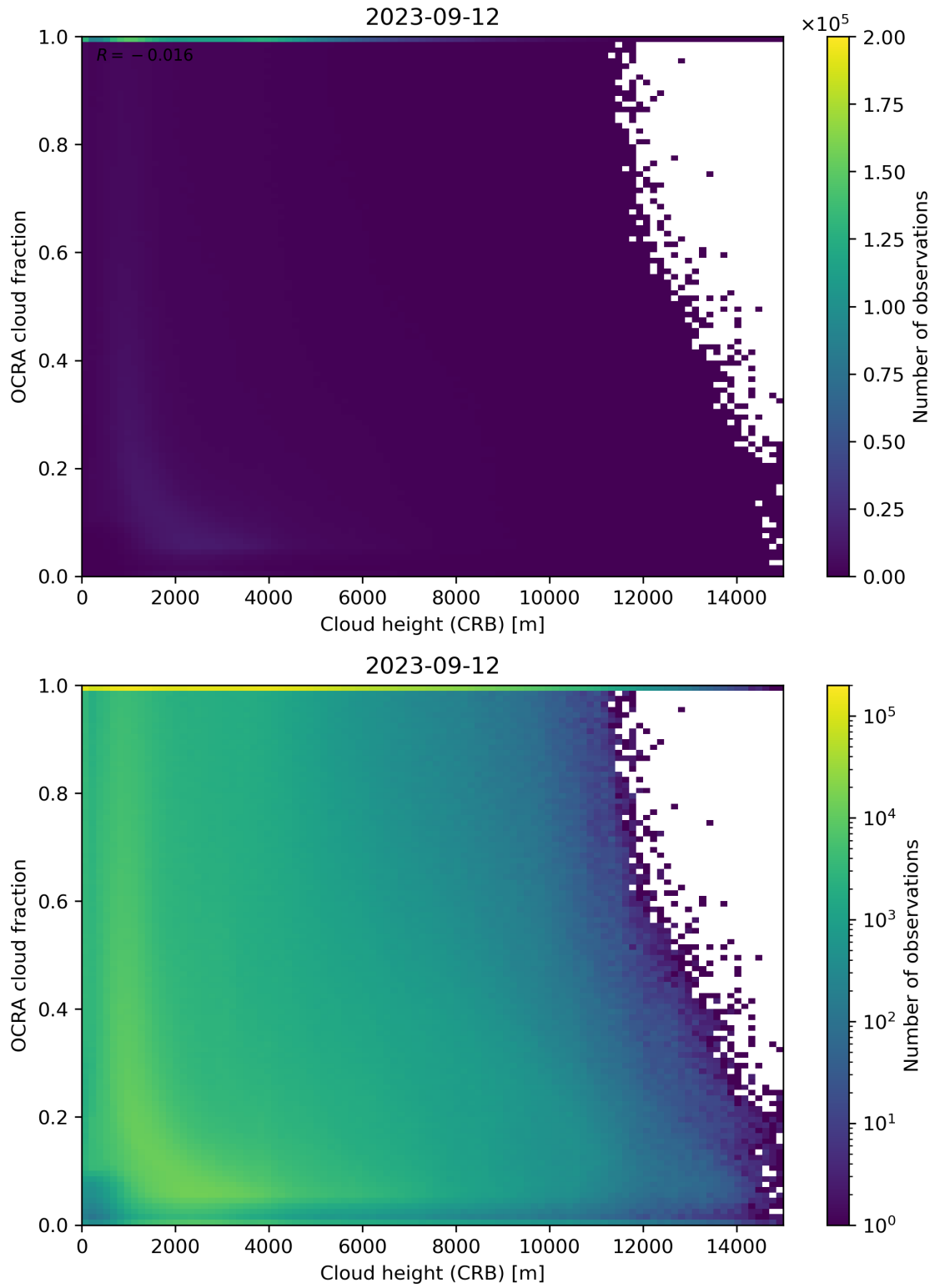
Figure 81: Scatter density plot of “Cloud height (CRB)” against “OCRA cloud fraction” for 2023-09-11 to 2023-09-13.
