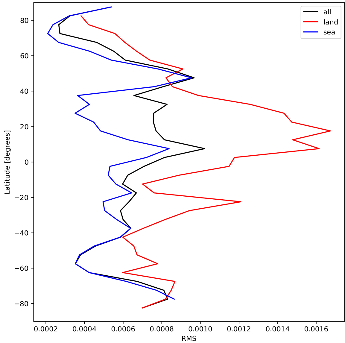
Figure 31: Zonal average of “RMS” for 2023-09-11 to 2023-09-13.
