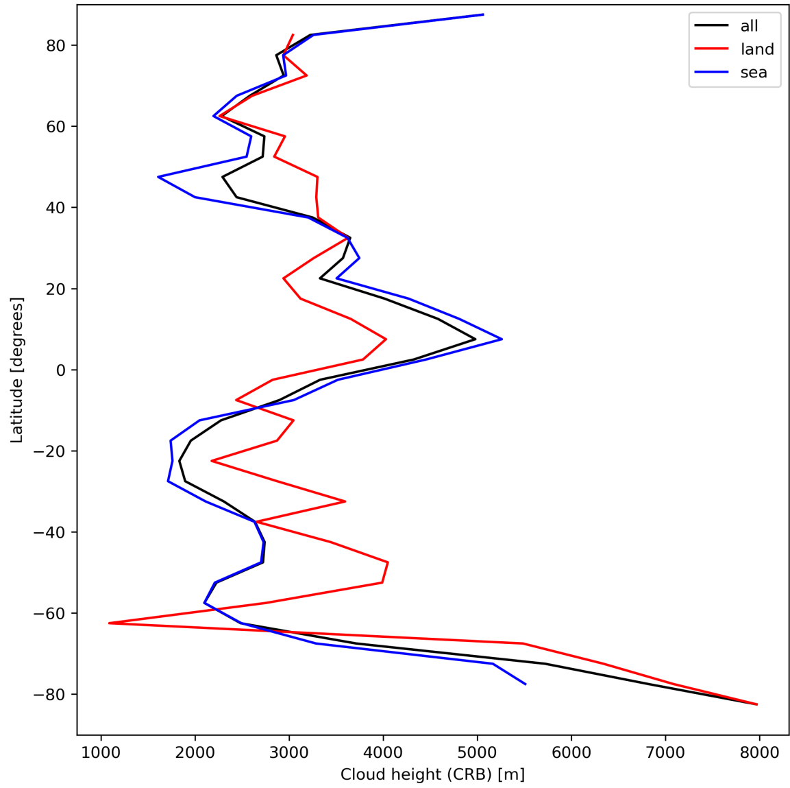
Figure 27: Zonal average of “Cloud height (CRB)” for 2023-09-11 to 2023-09-13.
