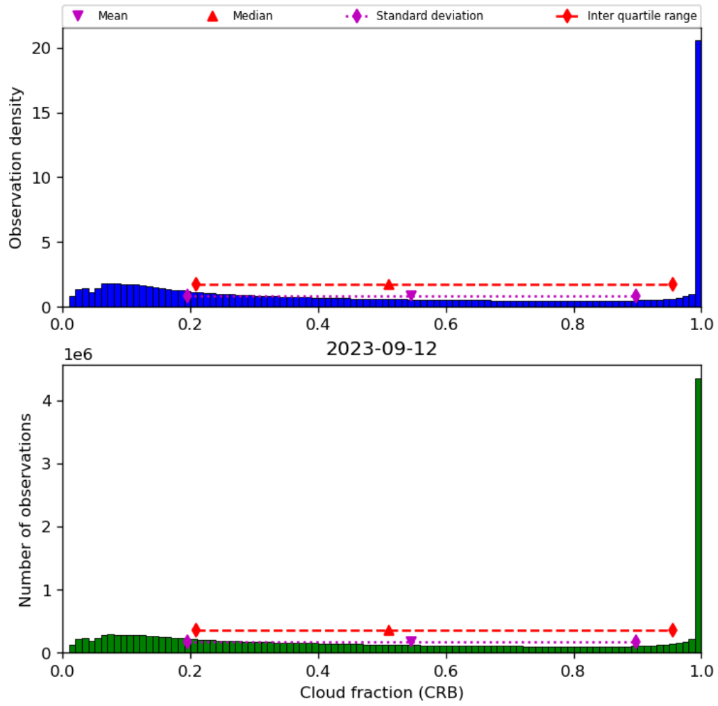
Figure 42: Histogram of “Cloud fraction (CRB)” for 2023-09-11 to 2023-09-13
