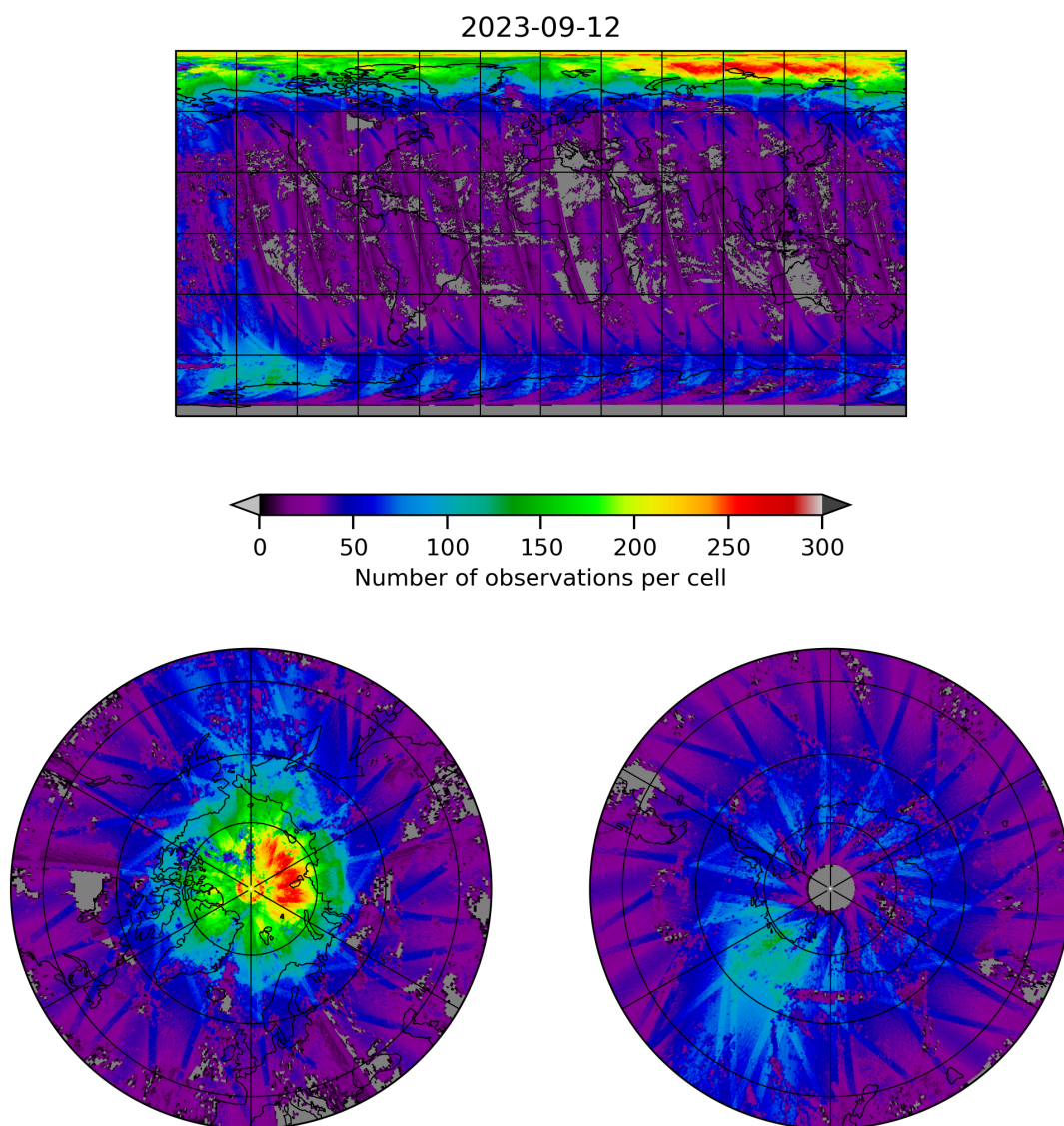
Figure 21: Map of the number of observations for 2023-09-11 to 2023-09-13
