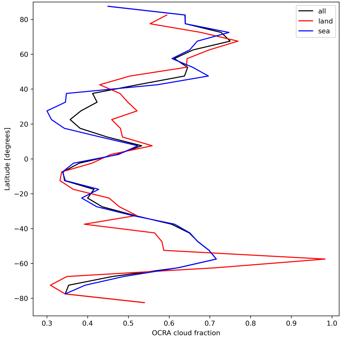
Figure 34: Zonal average of “OCRA cloud fraction” for 2023-09-11 to 2023-09-13.
