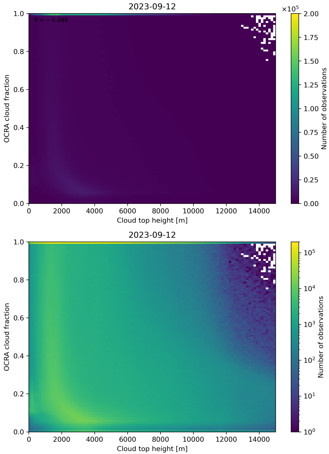
Figure 87: Scatter density plot of “Cloud top height” against “OCRA cloud fraction” for 2023-09-11 to 2023-09-13.
