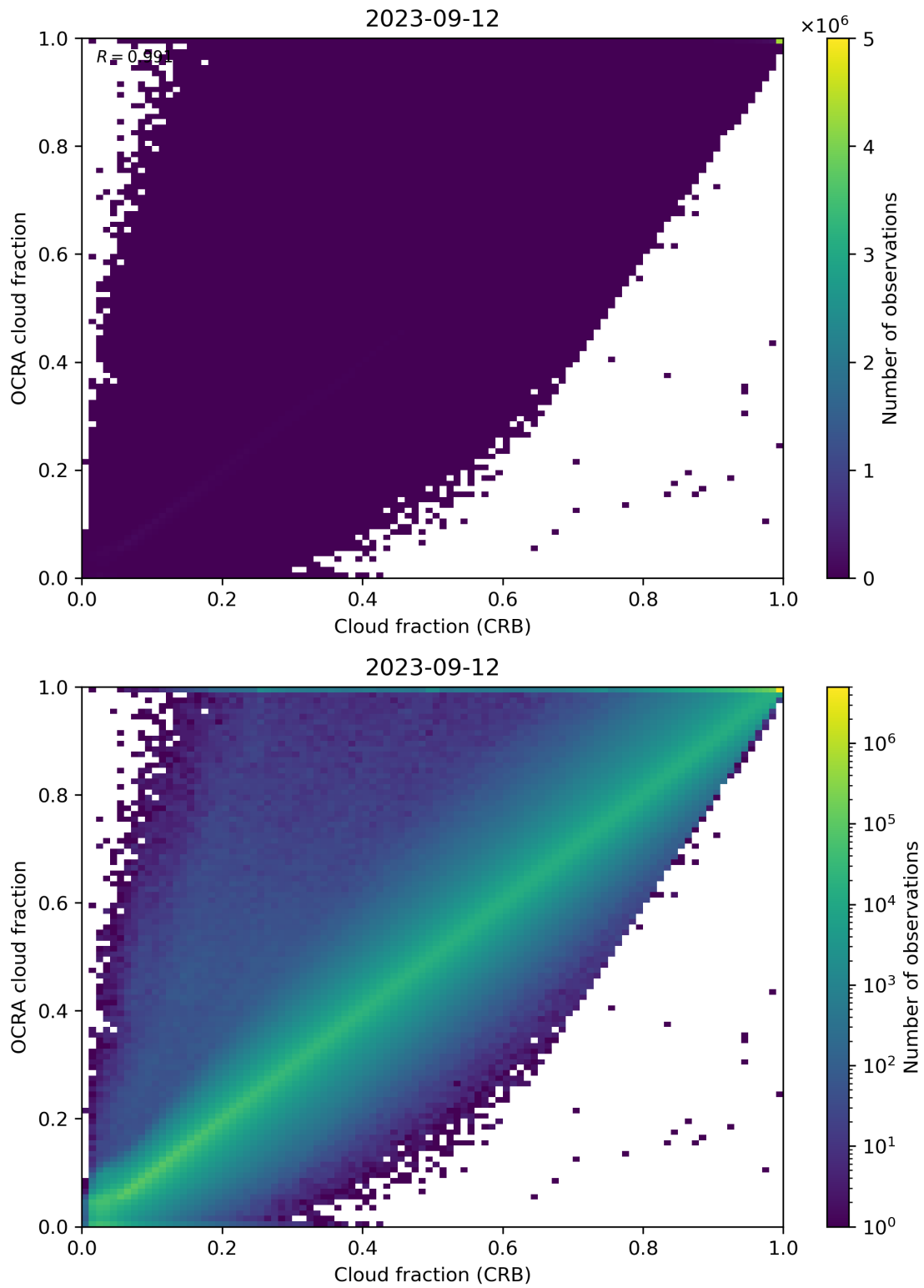
Figure 78: Scatter density plot of “Cloud fraction (CRB)” against “OCRA cloud fraction” for 2023-09-11 to 2023-09-13.
