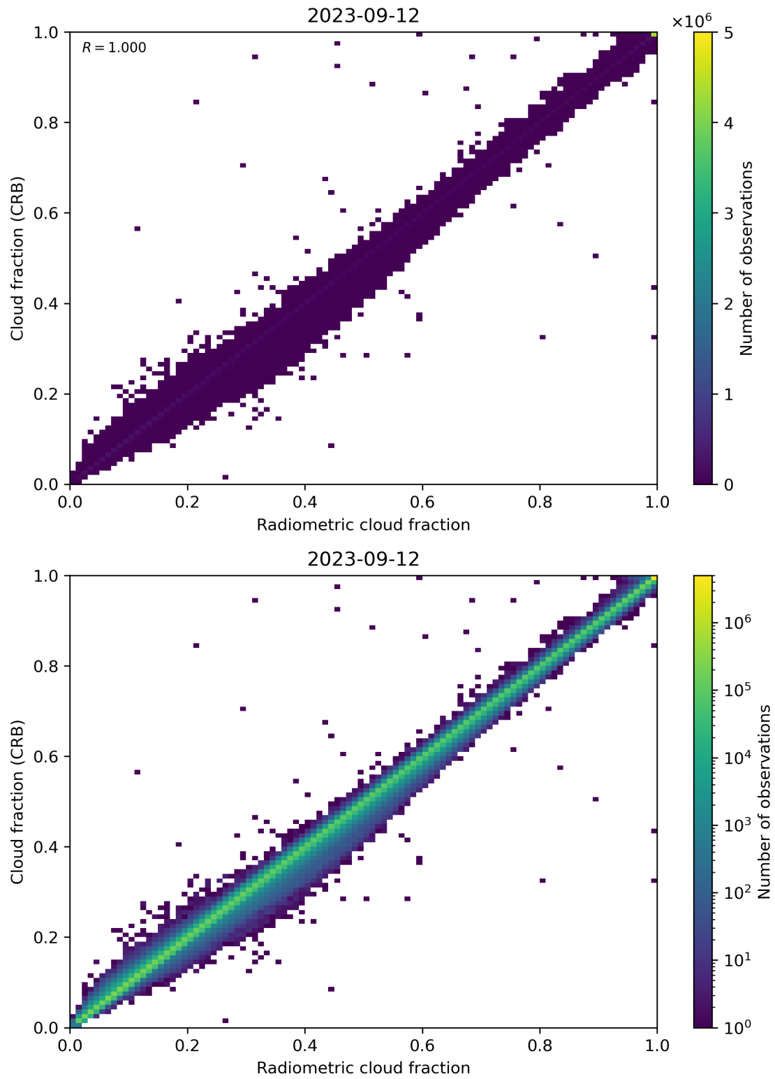
Figure 73: Scatter density plot of “Radiometric cloud fraction” against “Cloud fraction (CRB)” for 2023-09-11 to 2023-09-13.
