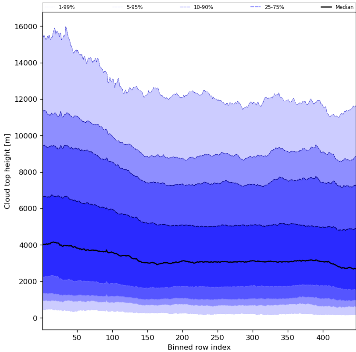
Figure 56: Along track statistics of “Cloud top height” for 2023-09-11 to 2023-09-13
