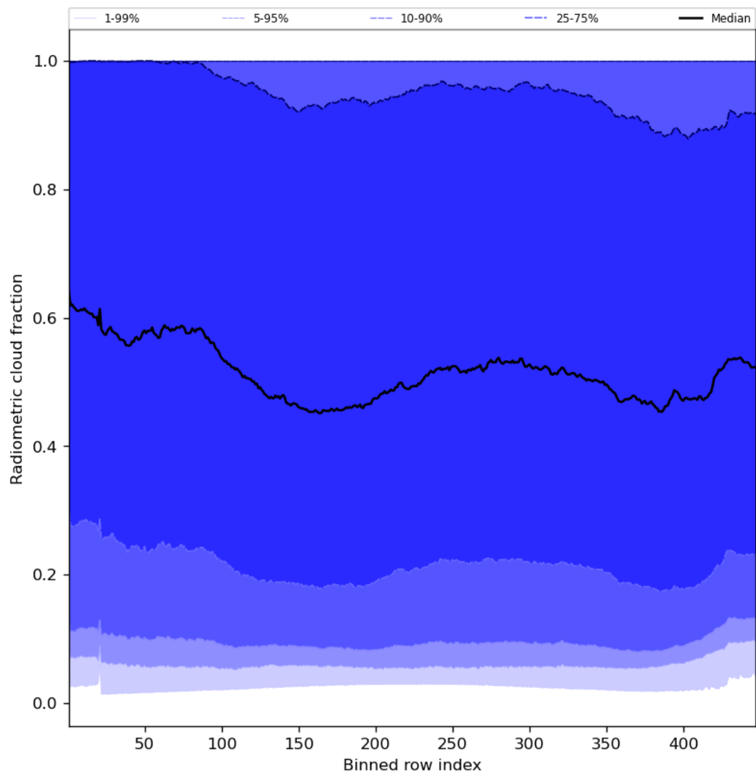
Figure 55: Along track statistics of “Radiometric cloud fraction” for 2023-09-11 to 2023-09-13
