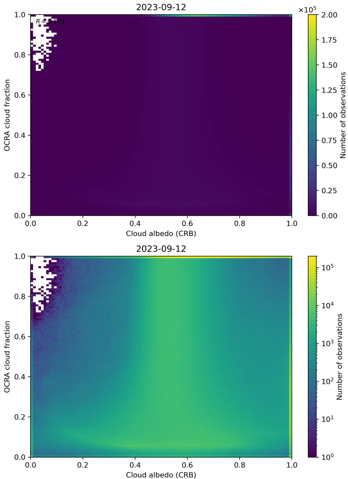
Figure 70: Scatter density plot of “Cloud albedo (CRB)” against “OCRA cloud fraction” for 2023-09-11 to 2023-09-13.
