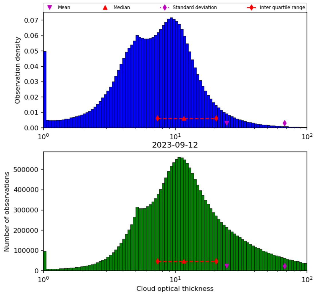
Figure 41: Histogram of “Cloud optical thickness” for 2023-09-11 to 2023-09-13
