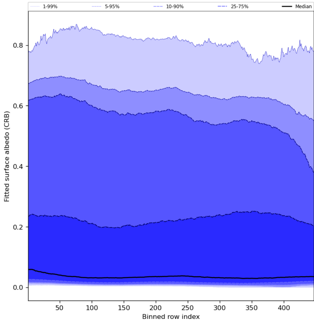
Figure 62: Along track statistics of “Fitted surface albedo (CRB)” for 2023-09-11 to 2023-09-13
