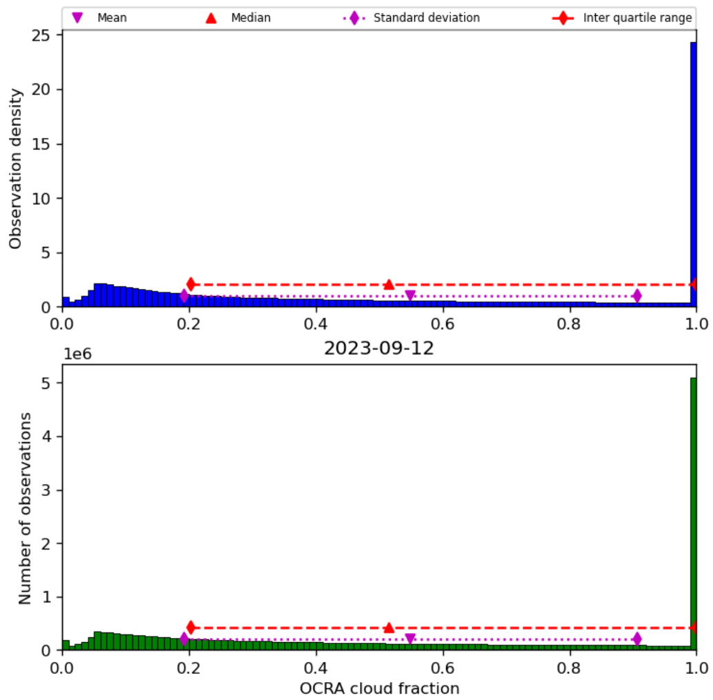
Figure 50: Histogram of “OCRA cloud fraction” for 2023-09-11 to 2023-09-13
