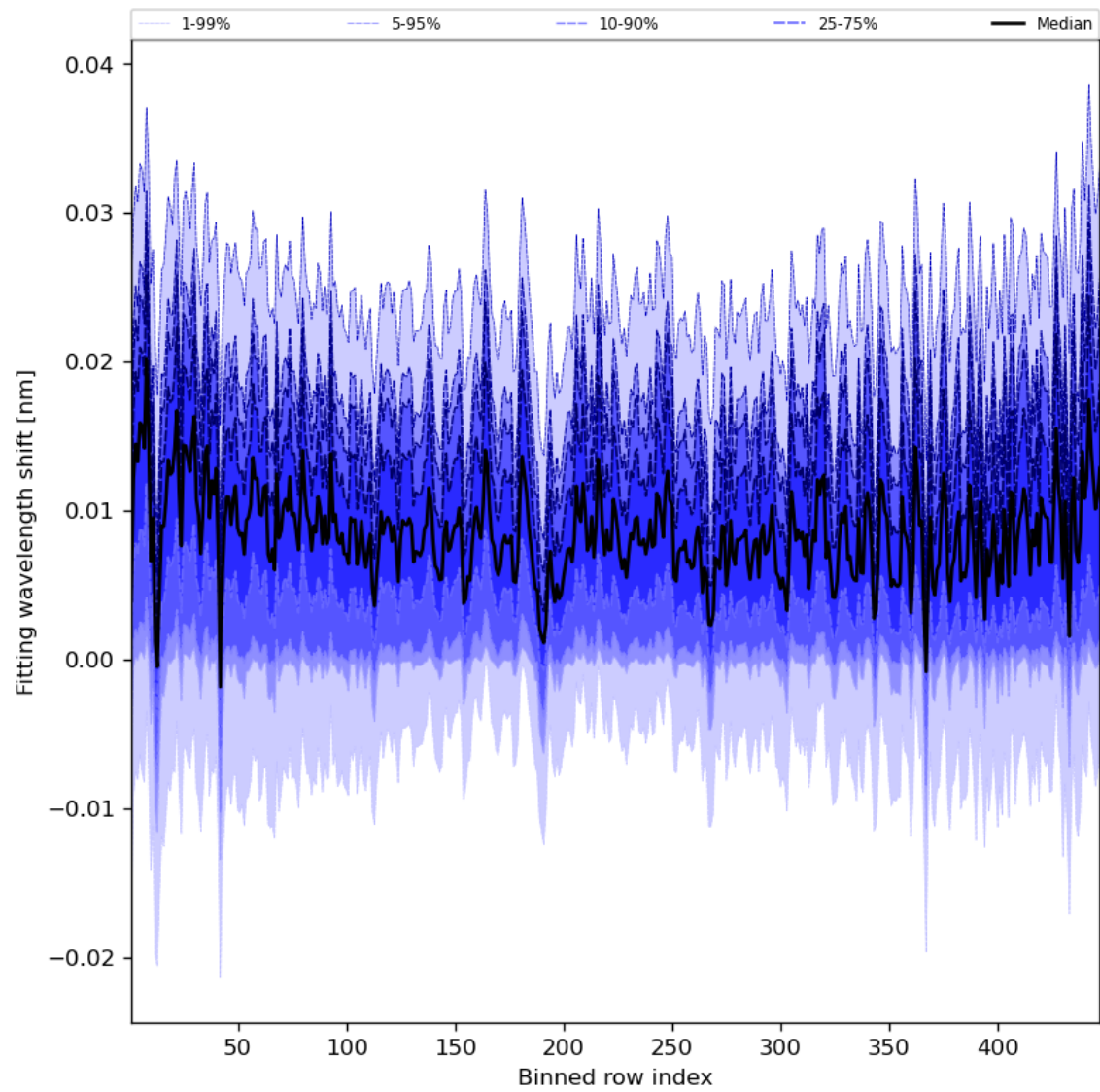
Figure 65: Along track statistics of “Fitting wavelength shift” for 2023-09-11 to 2023-09-13
