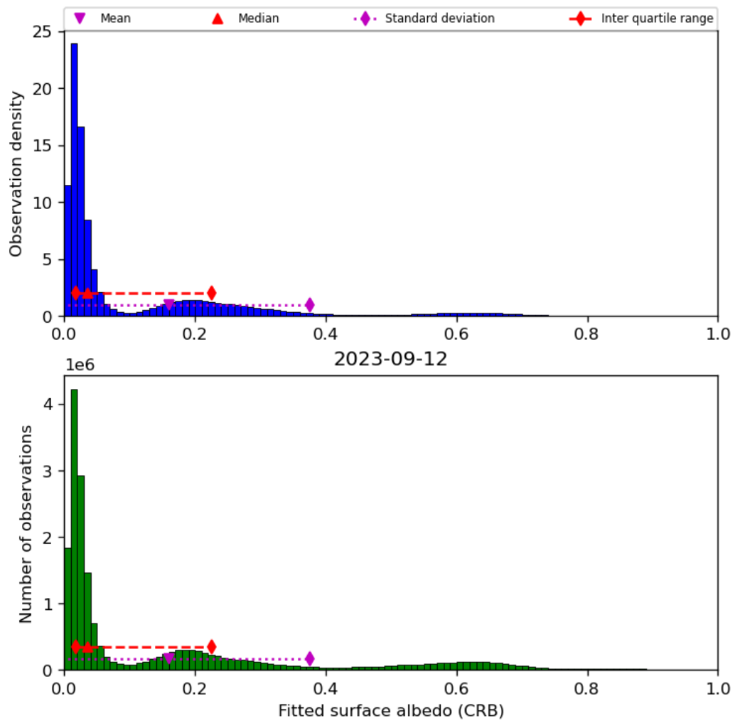
Figure 46: Histogram of “Fitted surface albedo (CRB)” for 2023-09-11 to 2023-09-13
