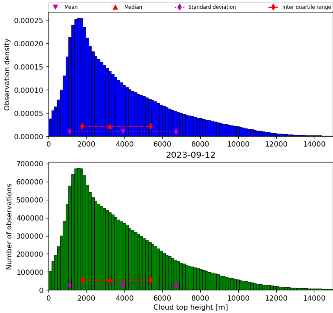
Figure 40: Histogram of “Cloud top height” for 2023-09-11 to 2023-09-13
