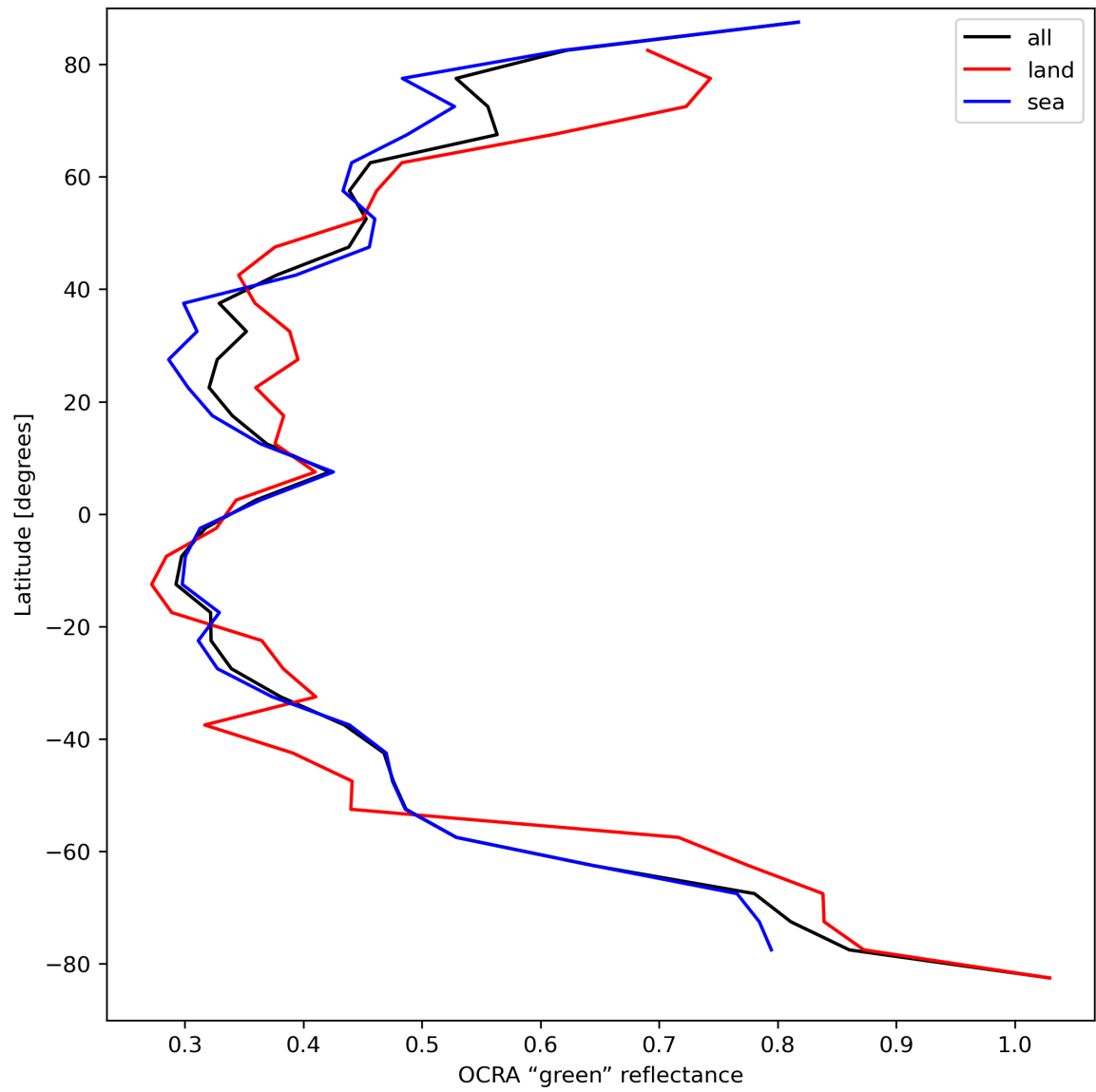
Figure 36: Zonal average of “OCRA “green” reflectance” for 2023-09-11 to 2023-09-13.
