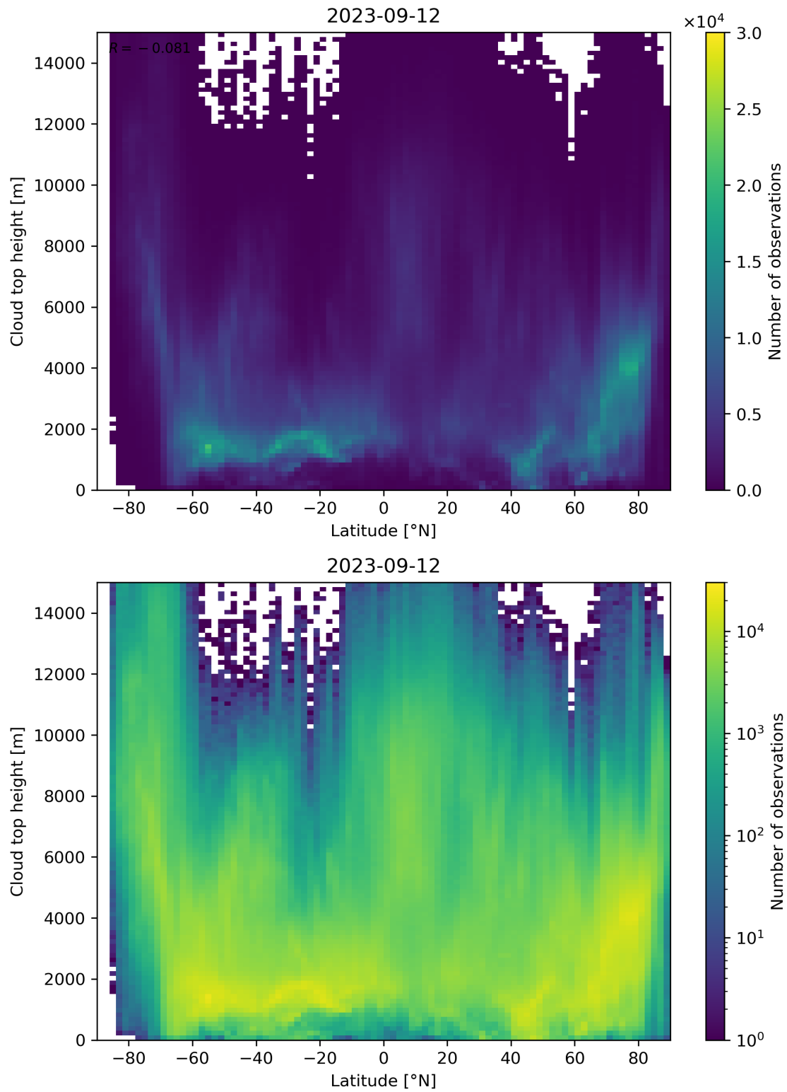
Figure 97: Scatter density plot of “Latitude” against “Cloud top height” for 2023-09-11 to 2023-09-13.
