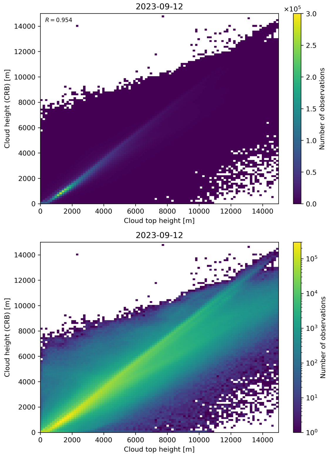
Figure 89: Scatter density plot of “Cloud top height” against “Cloud height (CRB)” for 2023-09-11 to 2023-09-13.
