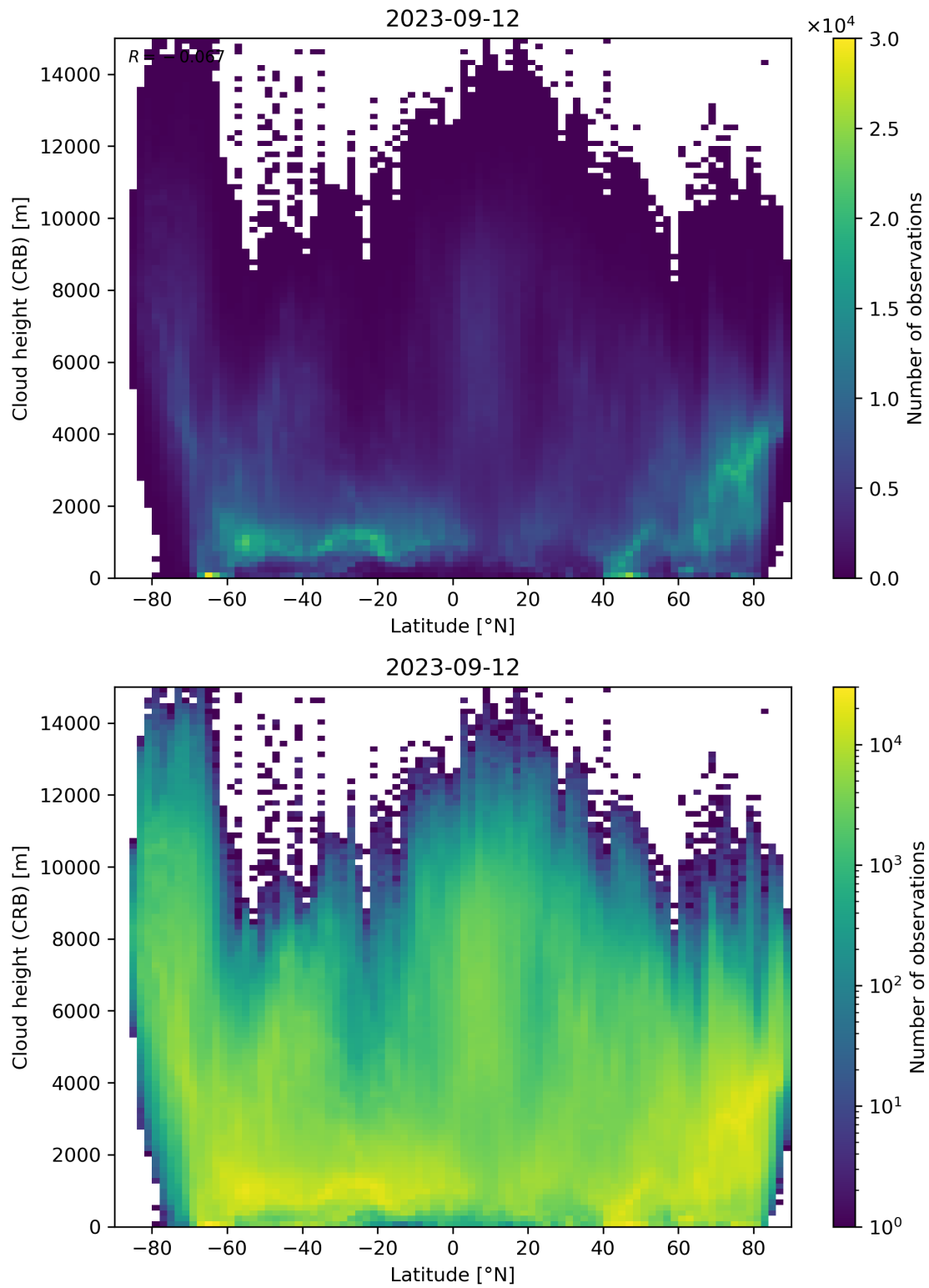
Figure 95: Scatter density plot of “Latitude” against “Cloud height (CRB)” for 2023-09-11 to 2023-09-13.
