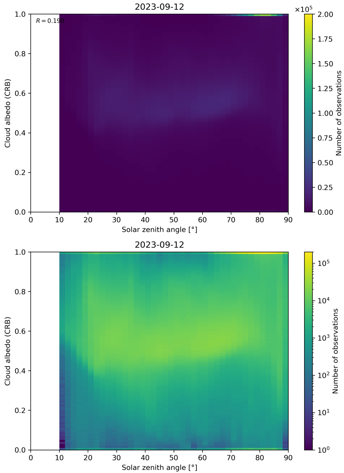
Figure 98: Scatter density plot of “Solar zenith angle” against “Cloud albedo (CRB)” for 2023-09-11 to 2023-09-13.
