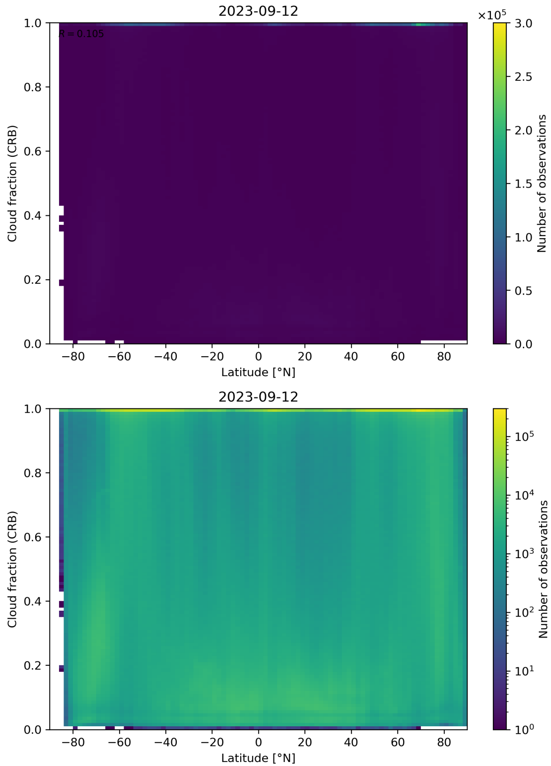
Figure 94: Scatter density plot of “Latitude” against “Cloud fraction (CRB)” for 2023-09-11 to 2023-09-13.
