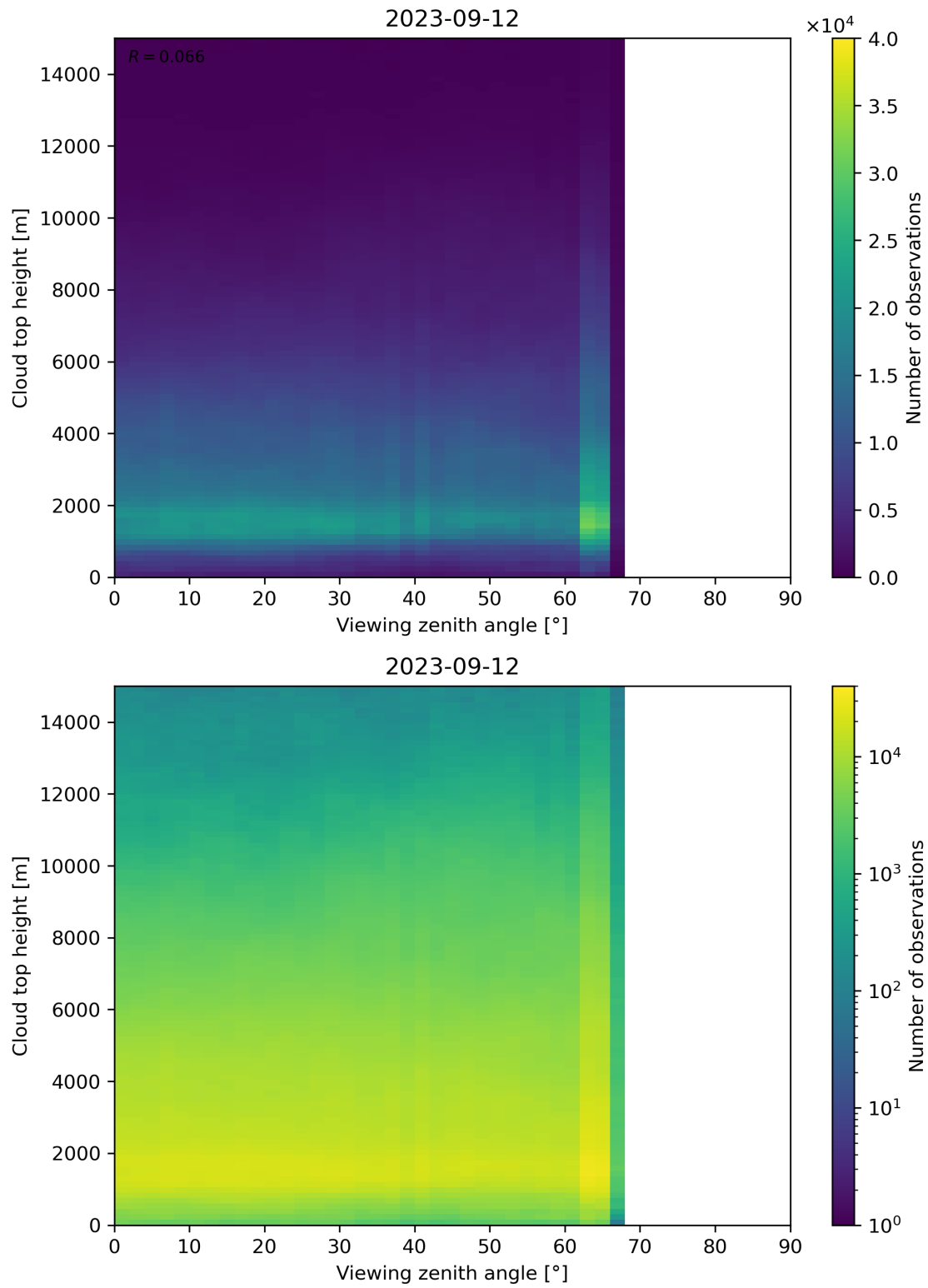
Figure 112: Scatter density plot of “Viewing zenith angle” against “Cloud top height” for 2023-09-11 to 2023-09-13.
