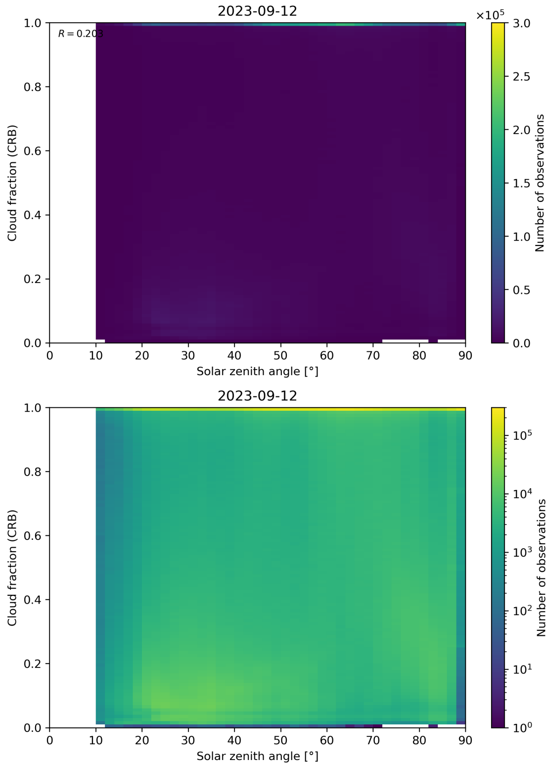
Figure 101: Scatter density plot of “Solar zenith angle” against “Cloud fraction (CRB)” for 2023-09-11 to 2023-09-13.
