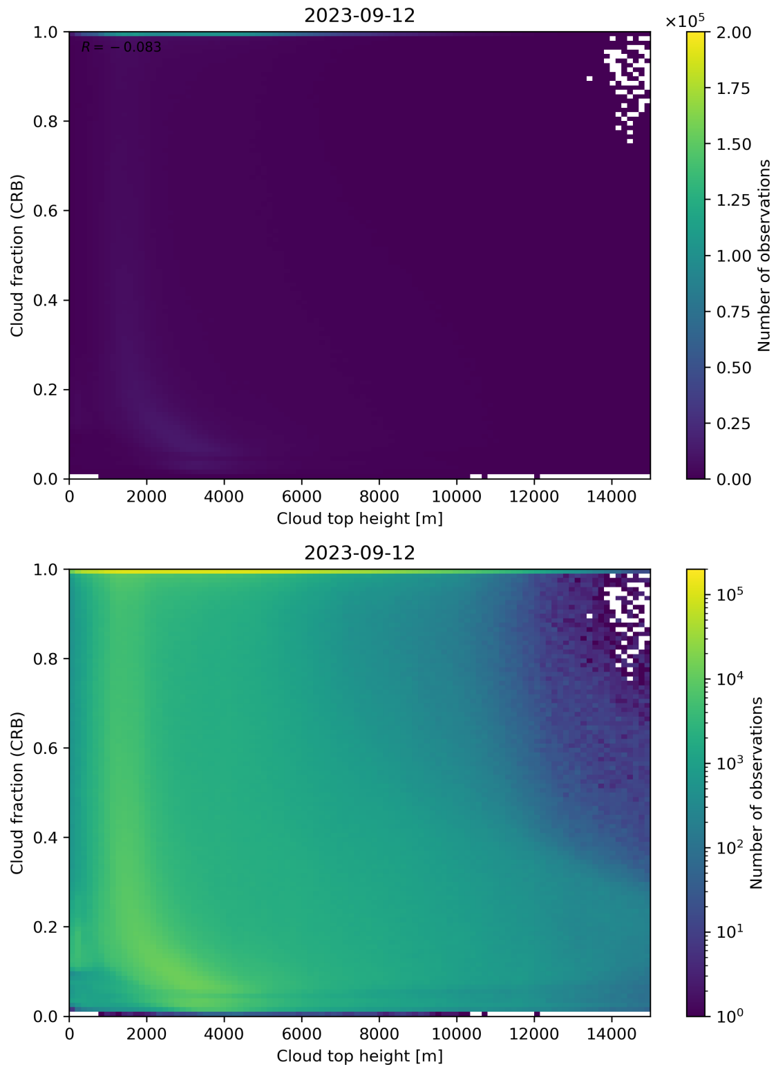
Figure 88: Scatter density plot of “Cloud top height” against “Cloud fraction (CRB)” for 2023-09-11 to 2023-09-13.
