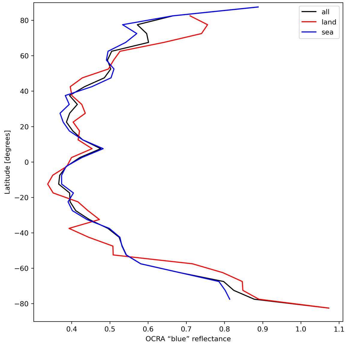
Figure 35: Zonal average of “OCRA “blue” reflectance” for 2023-09-11 to 2023-09-13.
