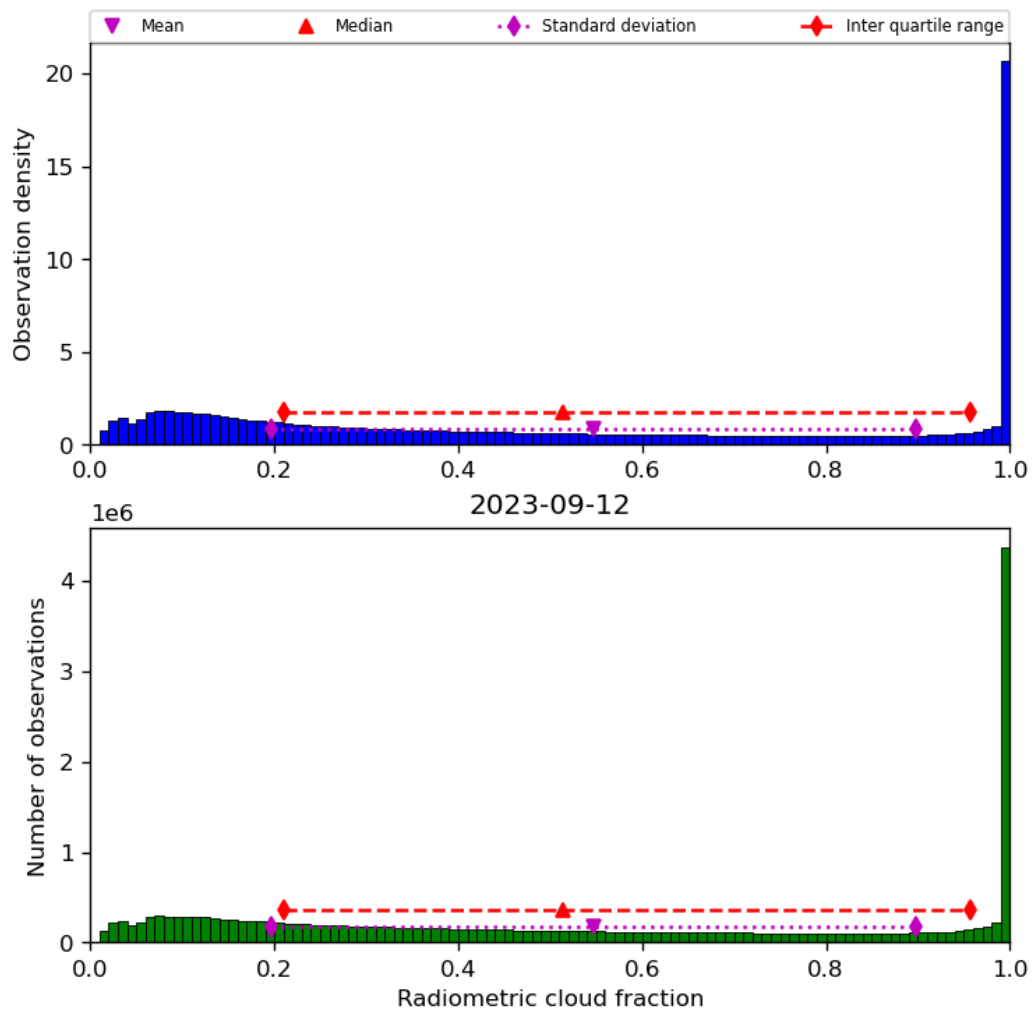
Figure 39: Histogram of “Radiometric cloud fraction” for 2023-09-11 to 2023-09-13
