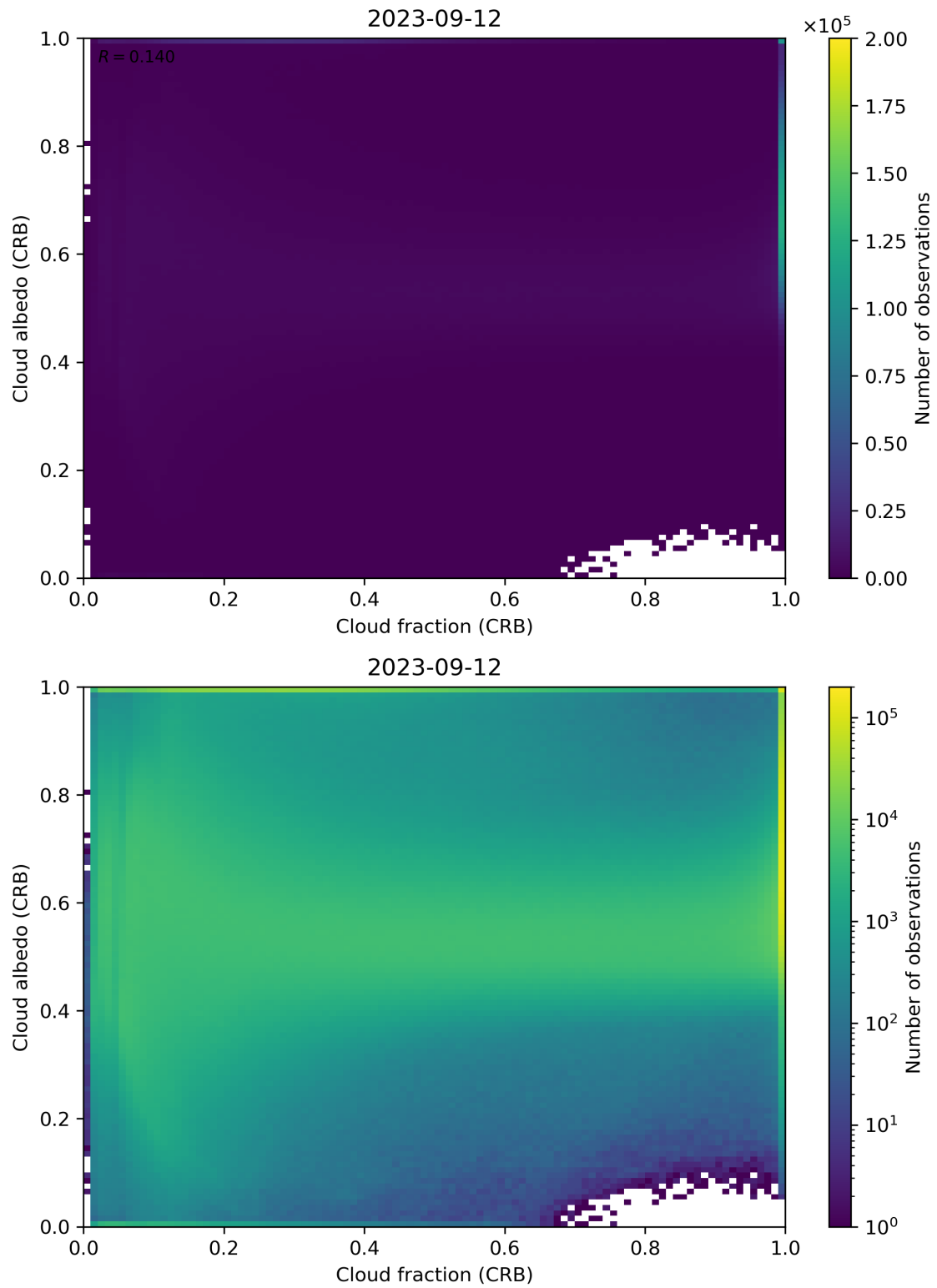
Figure 77: Scatter density plot of “Cloud fraction (CRB)” against “Cloud albedo (CRB)” for 2023-09-11 to 2023-09-13.
