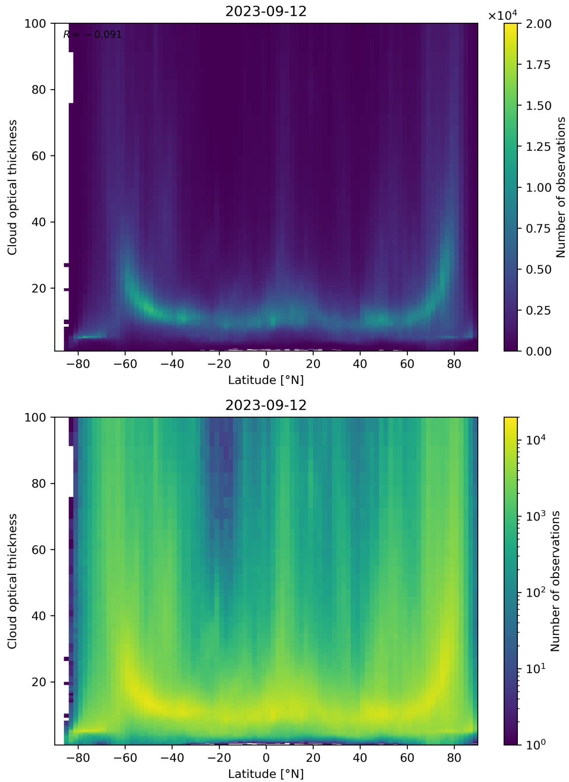
Figure 96: Scatter density plot of “Latitude” against “Cloud optical thickness” for 2023-09-11 to 2023-09-13.
