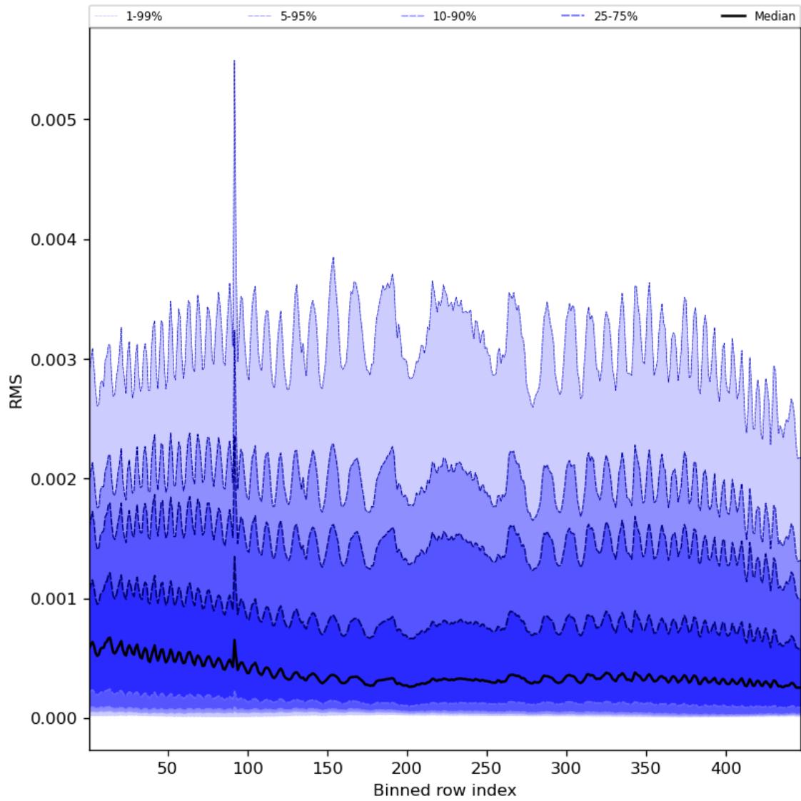
Figure 63: Along track statistics of “RMS” for 2023-09-11 to 2023-09-13
