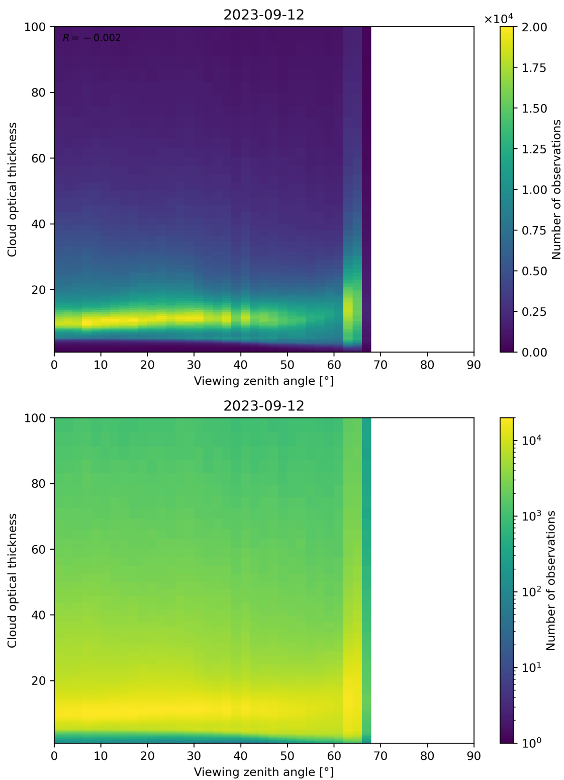
Figure 111: Scatter density plot of “Viewing zenith angle” against “Cloud optical thickness” for 2023-09-11 to 2023-09-13.
