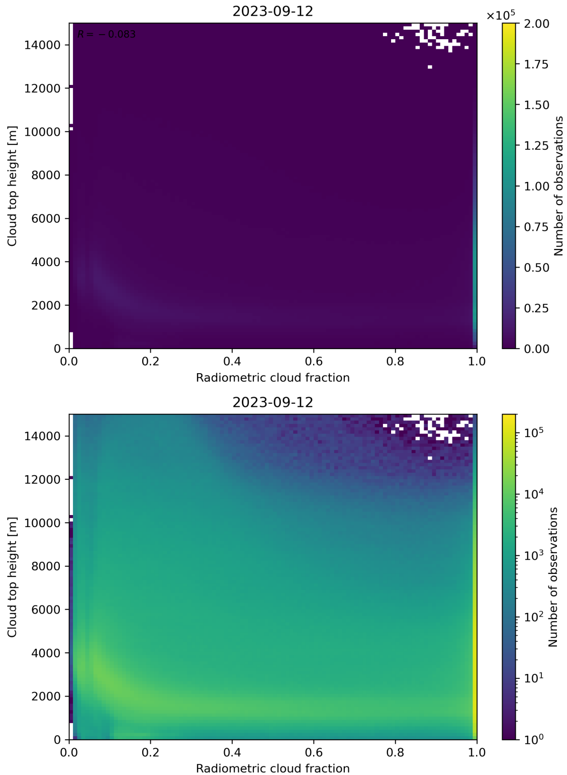
Figure 76: Scatter density plot of “Radiometric cloud fraction” against “Cloud top height” for 2023-09-11 to 2023-09-13.
