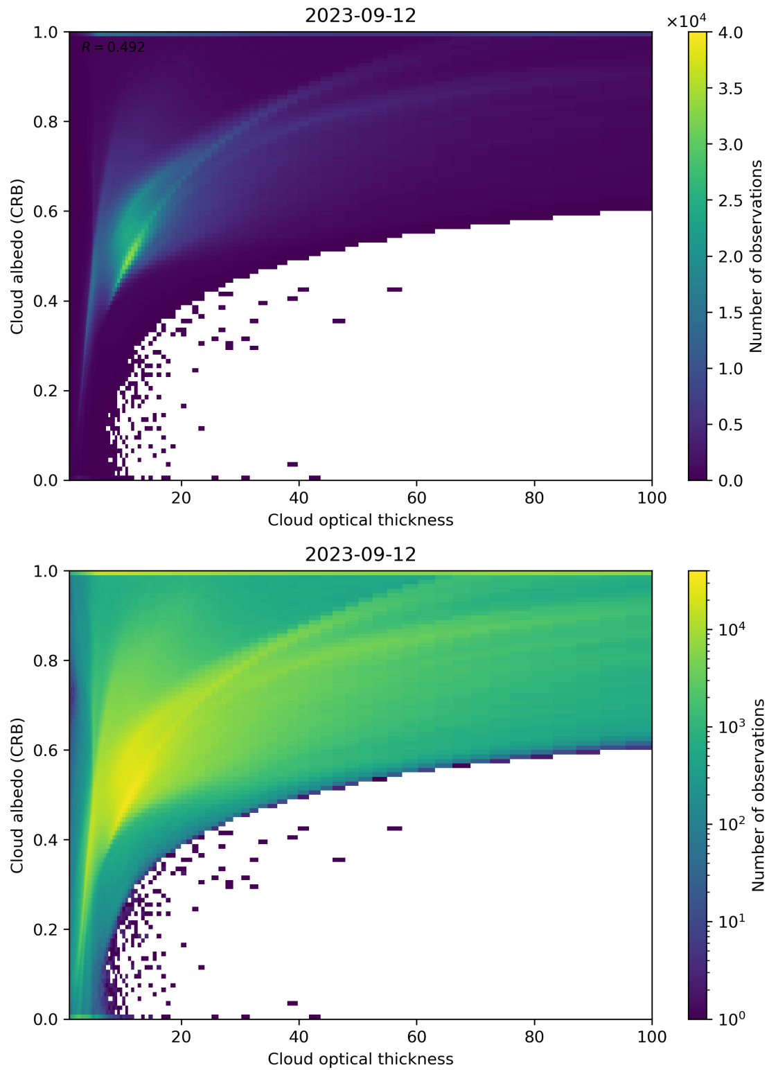
Figure 82: Scatter density plot of “Cloud optical thickness” against “Cloud albedo (CRB)” for 2023-09-11 to 2023-09-13.
