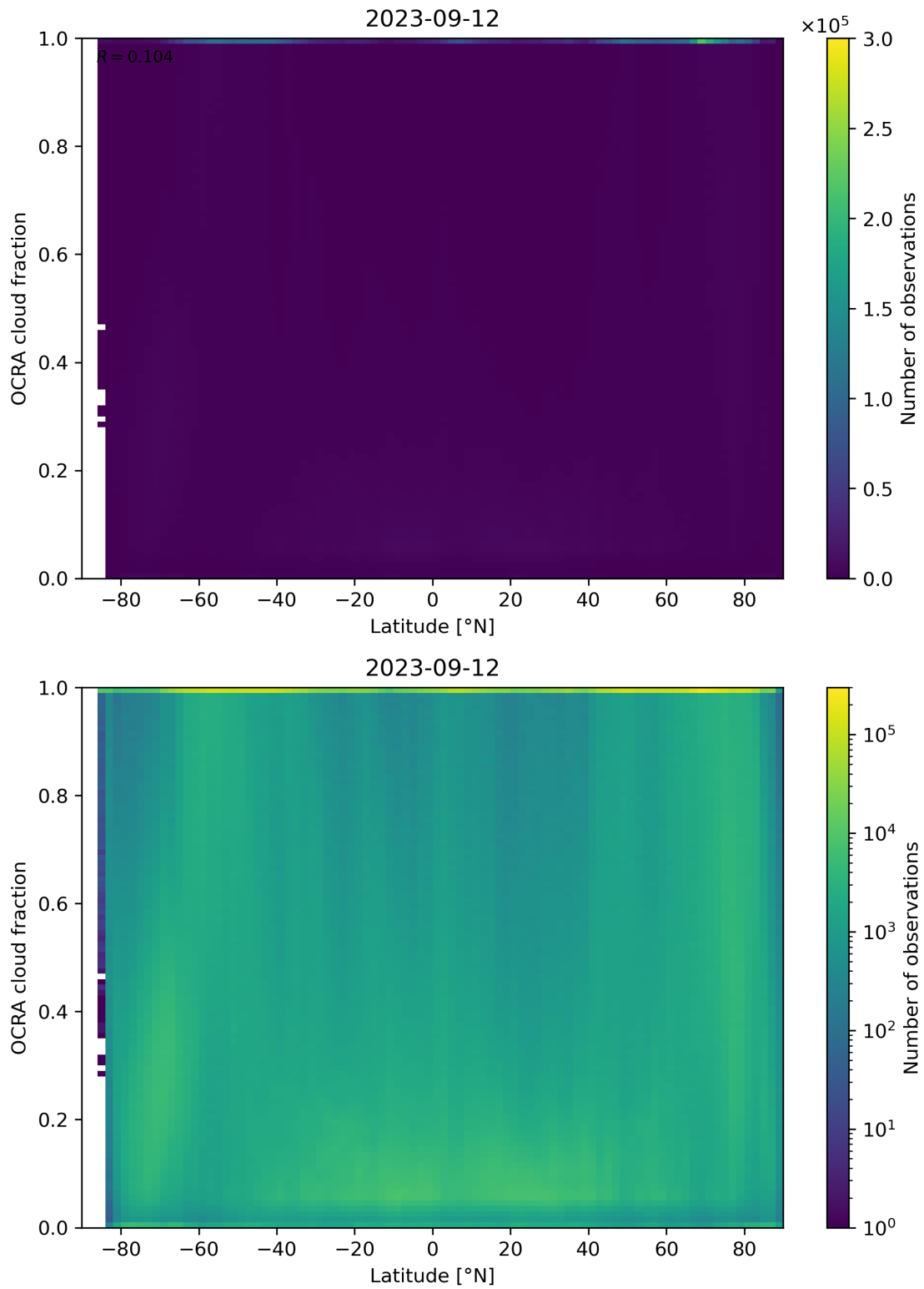
Figure 93: Scatter density plot of “Latitude” against “OCRA cloud fraction” for 2023-09-11 to 2023-09-13.
