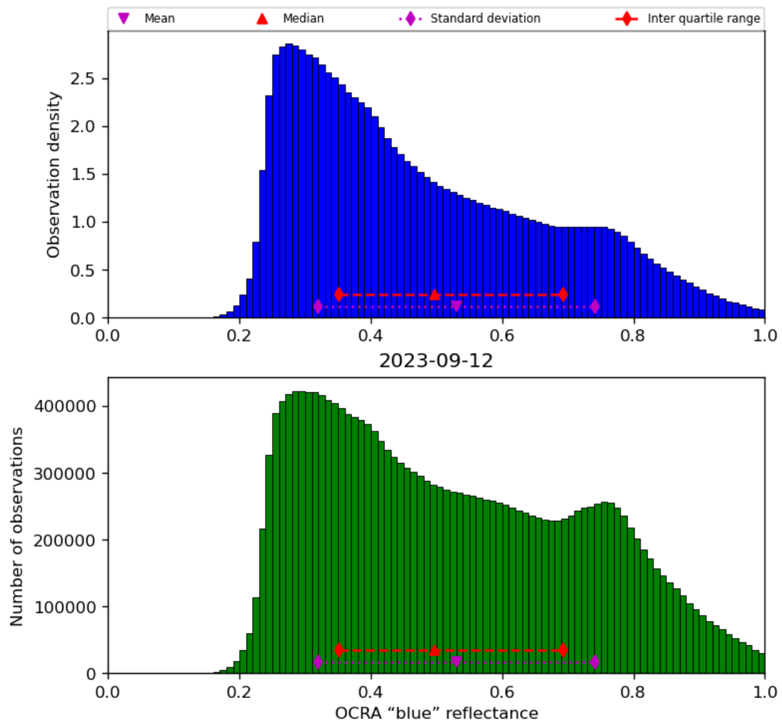
Figure 51: Histogram of “OCRA “blue” reflectance” for 2023-09-11 to 2023-09-13
