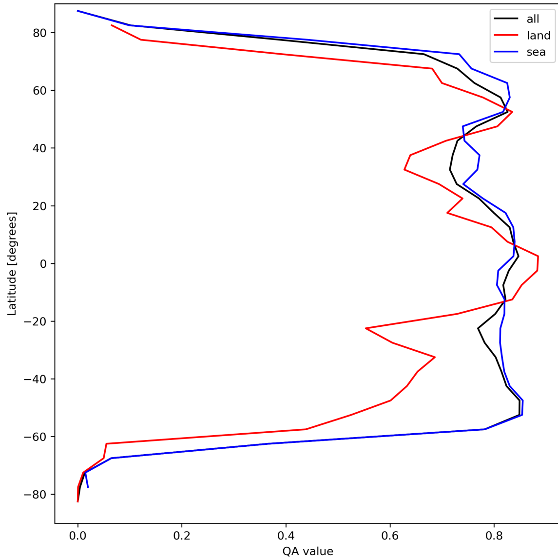
Figure 22: Zonal average of “QA value” for 2023-09-11 to 2023-09-13.
