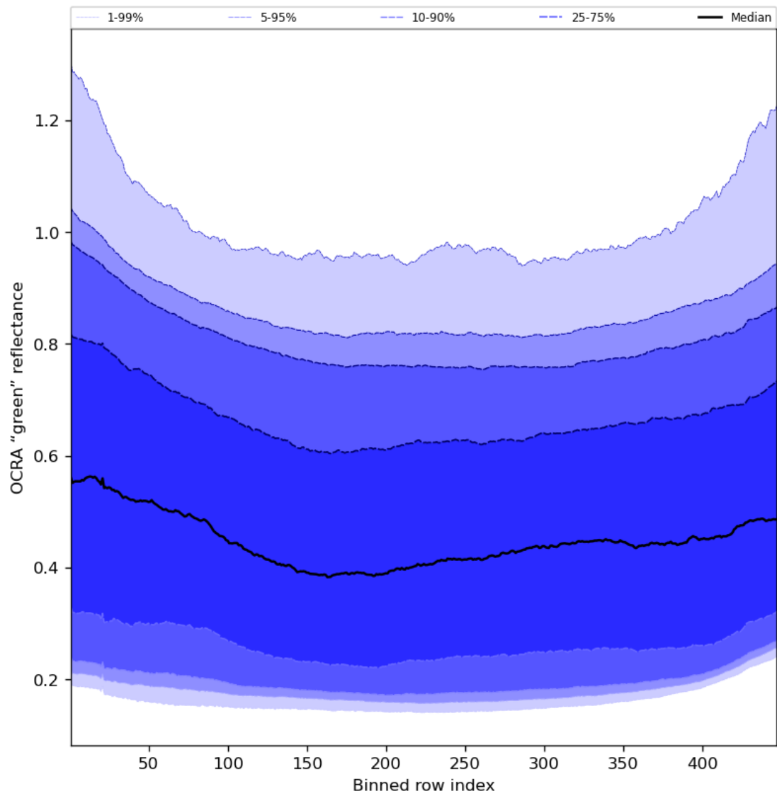
Figure 68: Along track statistics of “OCRA “green” reflectance” for 2023-09-11 to 2023-09-13
