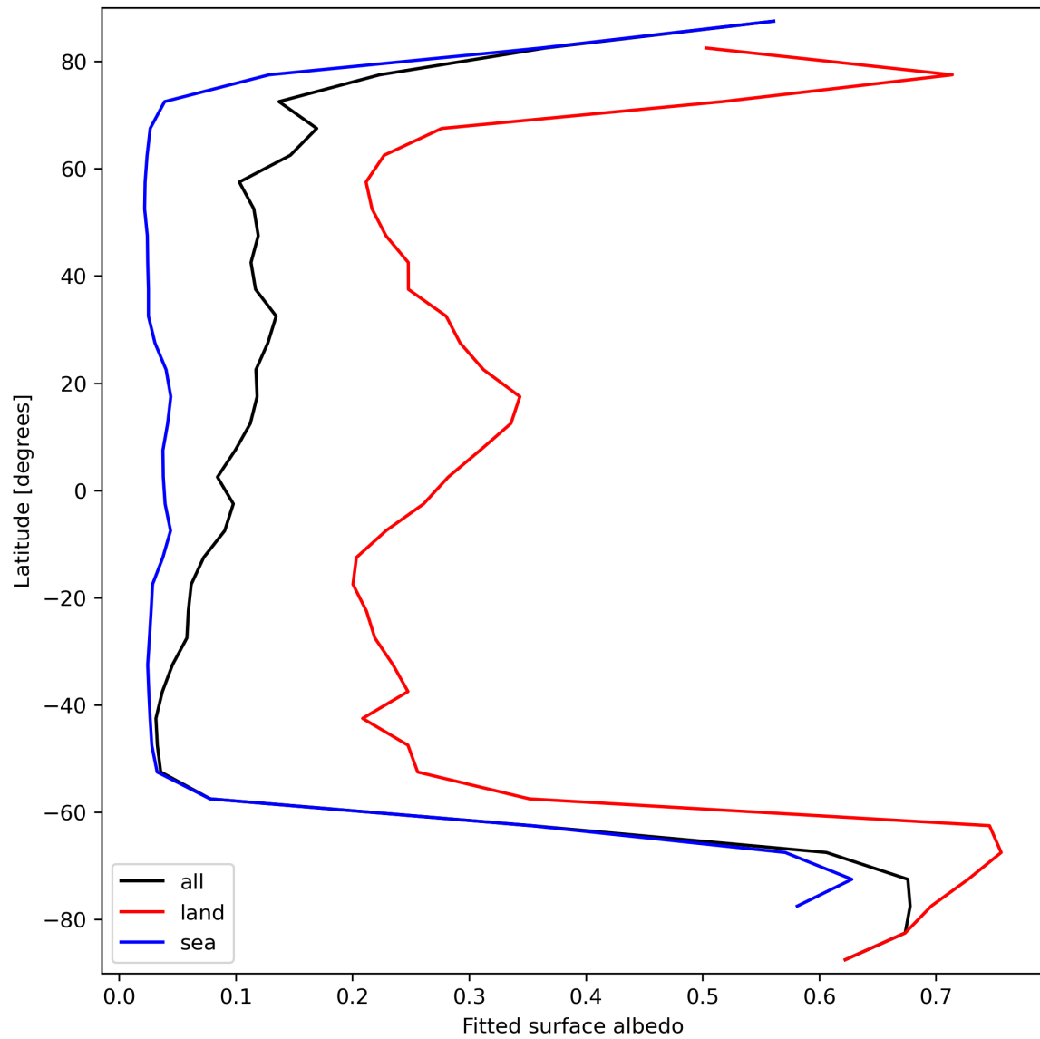
Figure 29: Zonal average of “Fitted surface albedo” for 2023-09-12 to 2023-09-14.
