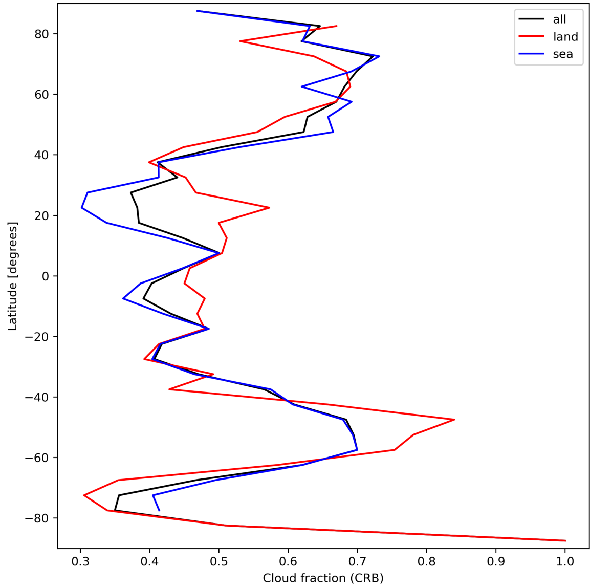
Figure 26: Zonal average of “Cloud fraction (CRB)” for 2023-09-12 to 2023-09-14.
