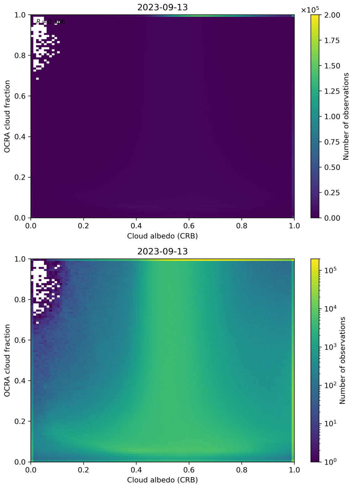
Figure 70: Scatter density plot of “Cloud albedo (CRB)” against “OCRA cloud fraction” for 2023-09-12 to 2023-09-14.
