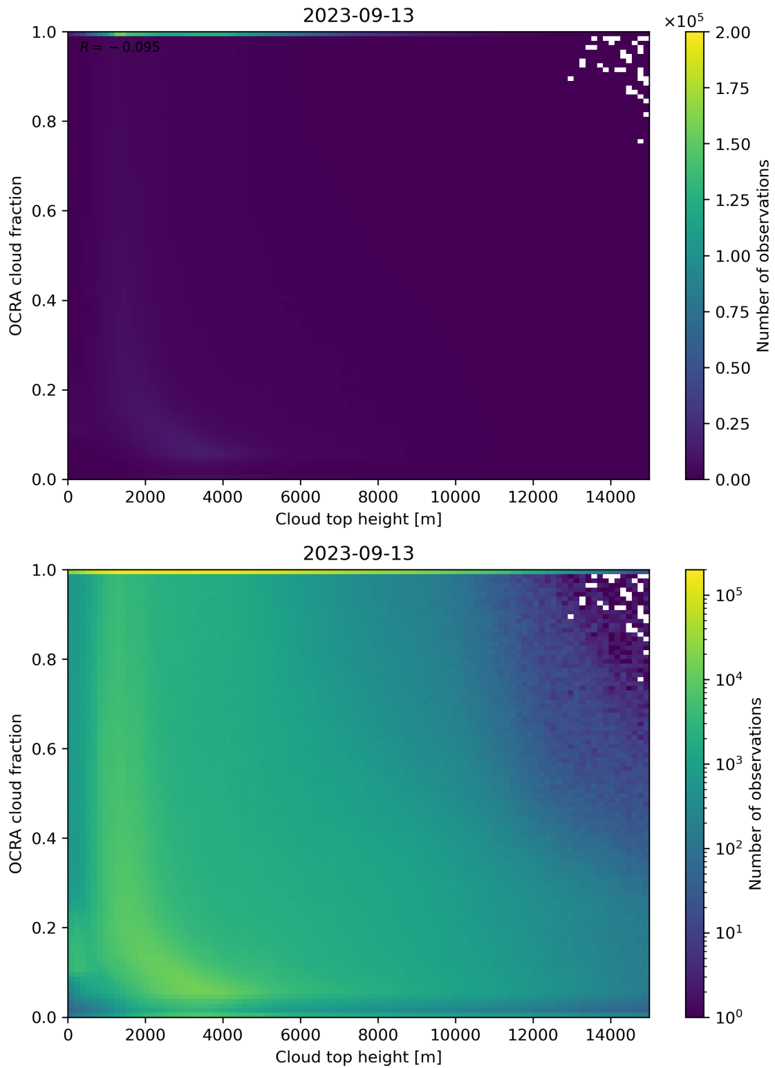
Figure 87: Scatter density plot of “Cloud top height” against “OCRA cloud fraction” for 2023-09-12 to 2023-09-14.
