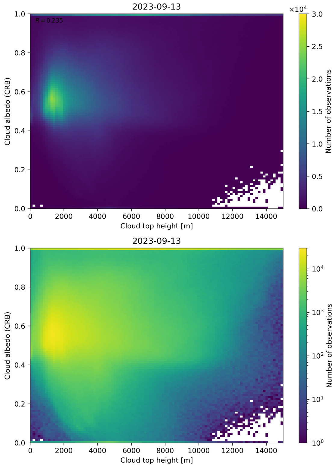
Figure 86: Scatter density plot of “Cloud top height” against “Cloud albedo (CRB)” for 2023-09-12 to 2023-09-14.
