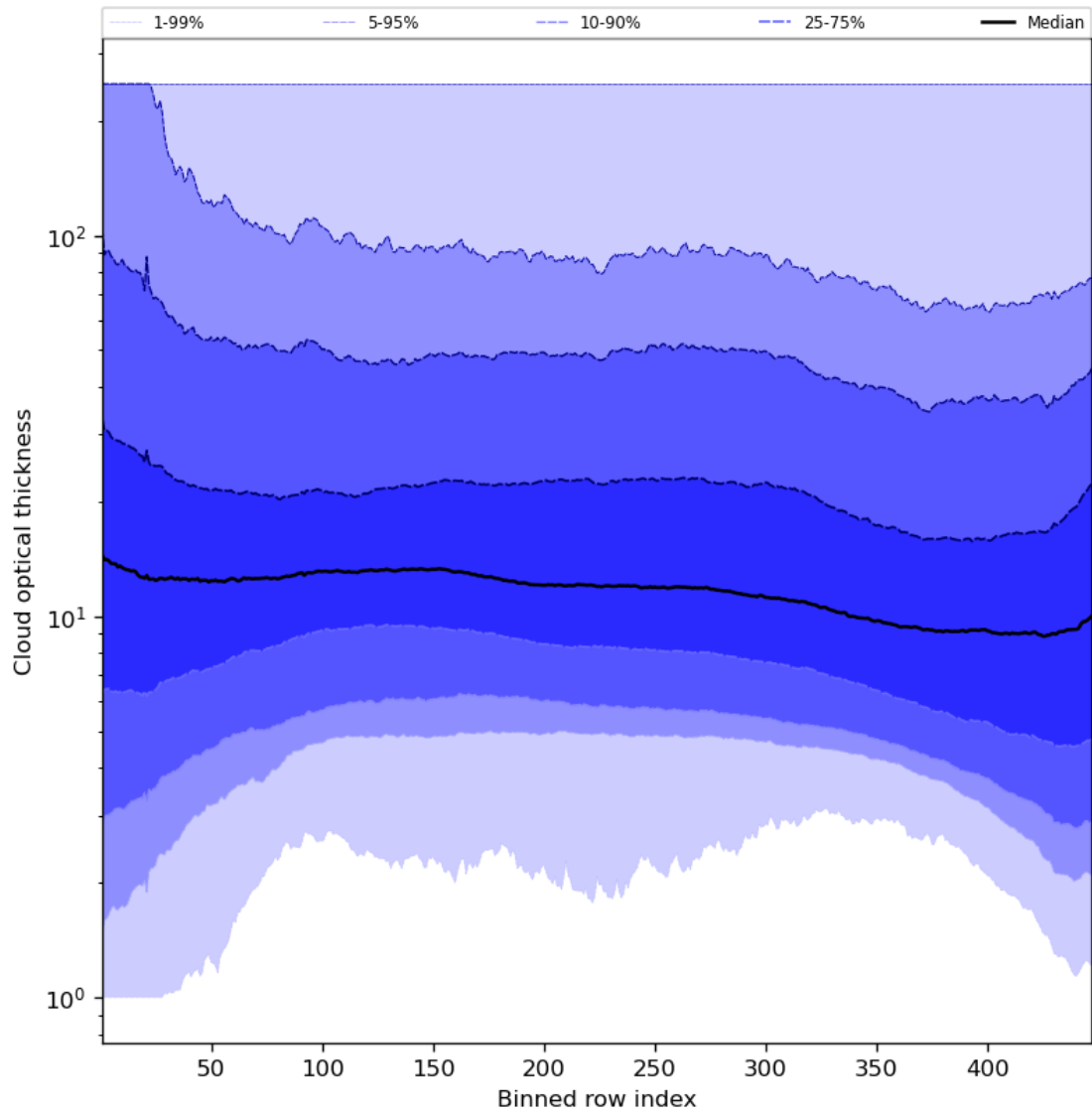
Figure 57: Along track statistics of “Cloud optical thickness” for 2023-09-12 to 2023-09-14
