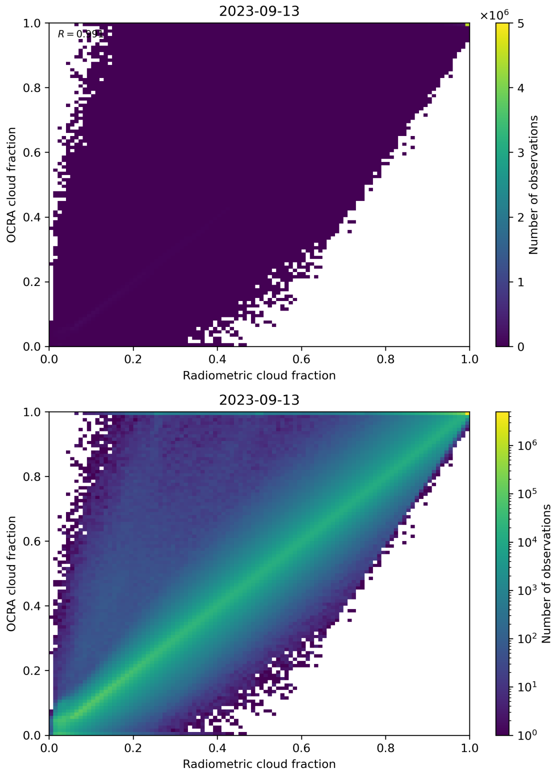
Figure 72: Scatter density plot of “Radiometric cloud fraction” against “OCRA cloud fraction” for 2023-09-12 to 2023-09-14.
