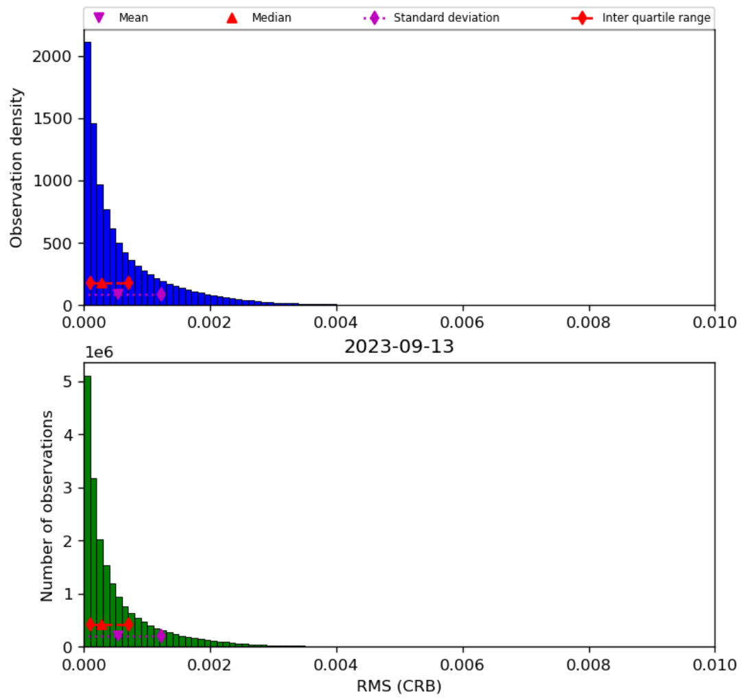
Figure 48: Histogram of “RMS (CRB)” for 2023-09-12 to 2023-09-14
