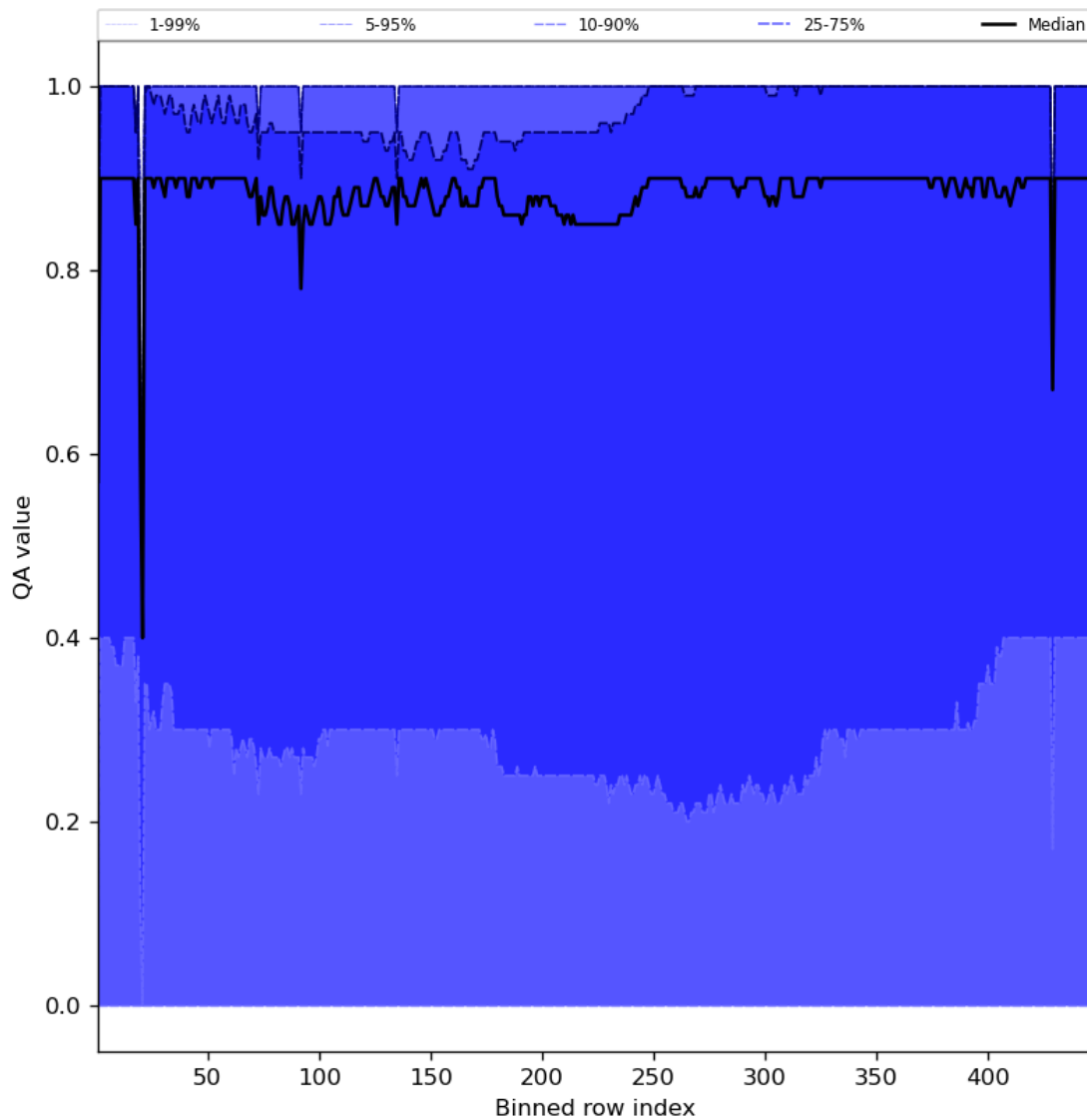
Figure 54: Along track statistics of “QA value” for 2023-09-12 to 2023-09-14
