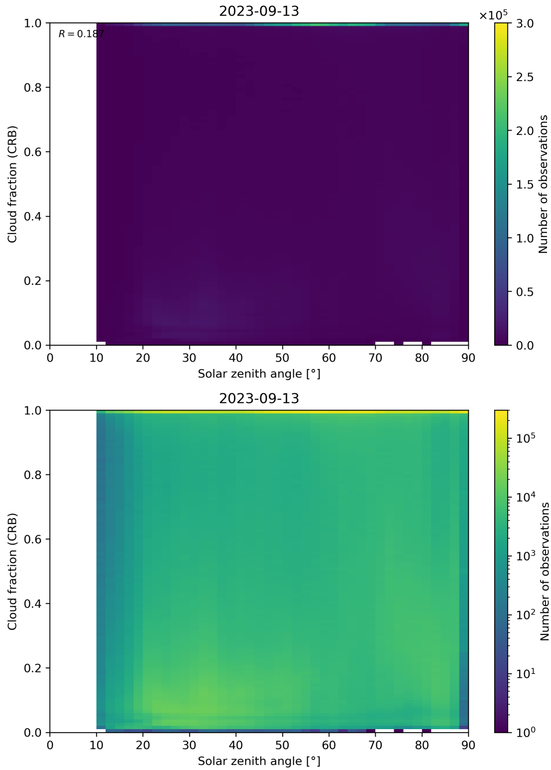
Figure 101: Scatter density plot of “Solar zenith angle” against “Cloud fraction (CRB)” for 2023-09-12 to 2023-09-14.
