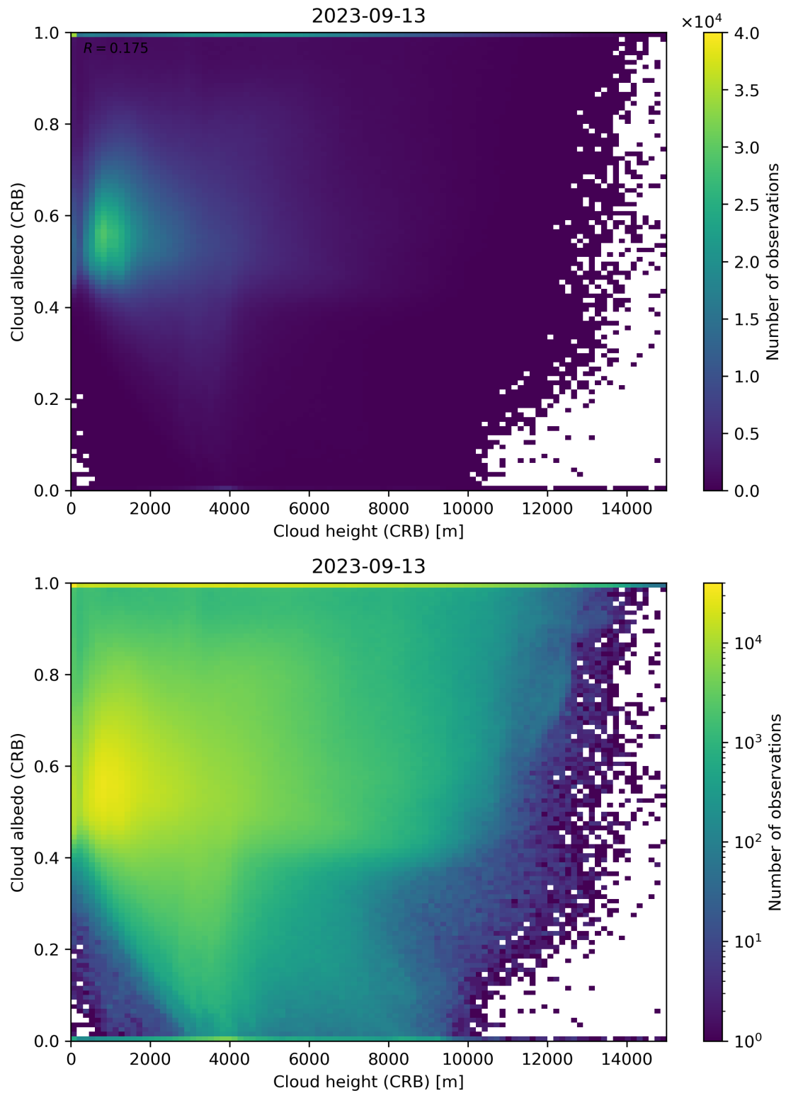
Figure 80: Scatter density plot of “Cloud height (CRB)” against “Cloud albedo (CRB)” for 2023-09-12 to 2023-09-14.
