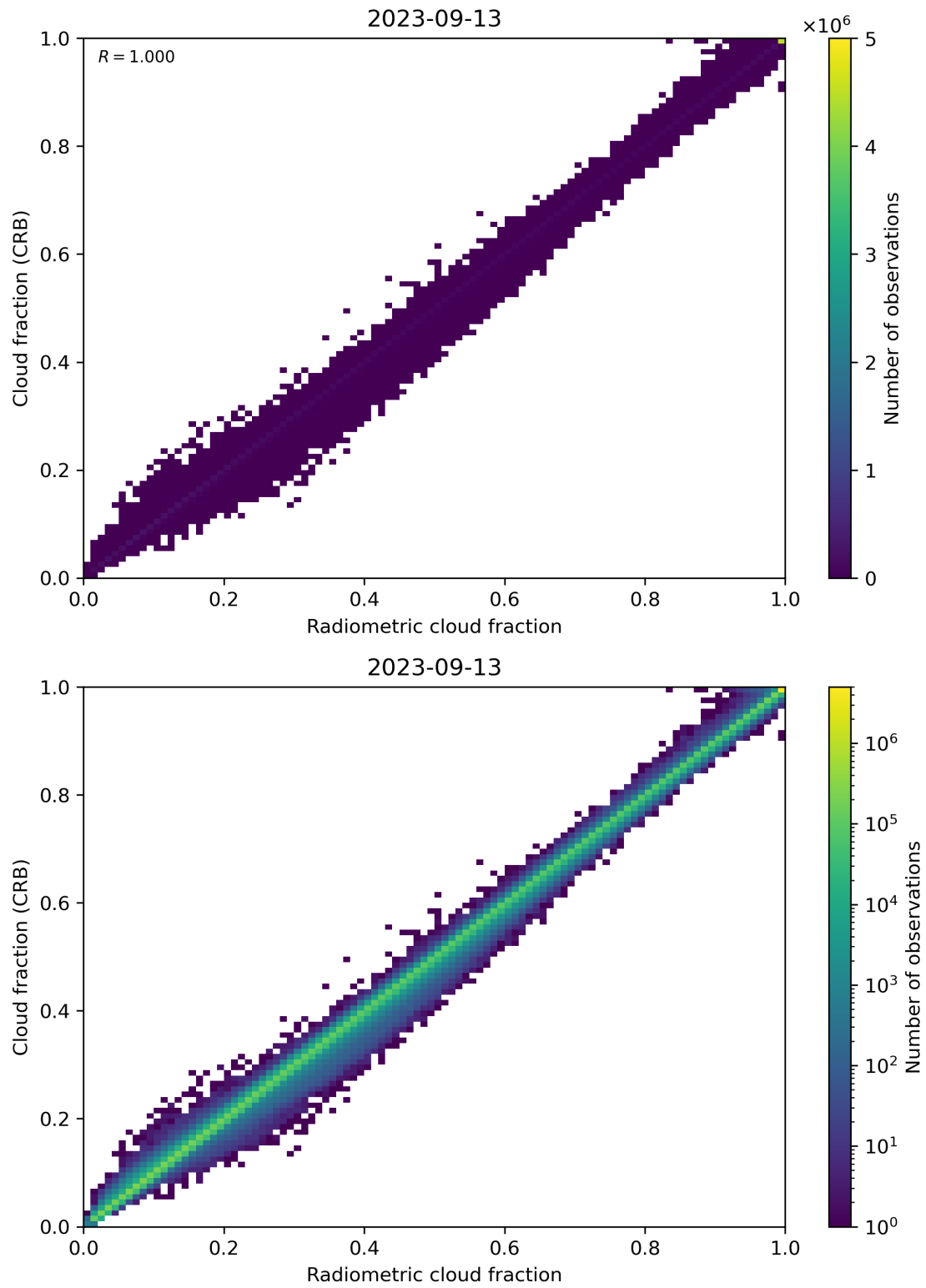
Figure 73: Scatter density plot of “Radiometric cloud fraction” against “Cloud fraction (CRB)” for 2023-09-12 to 2023-09-14.
