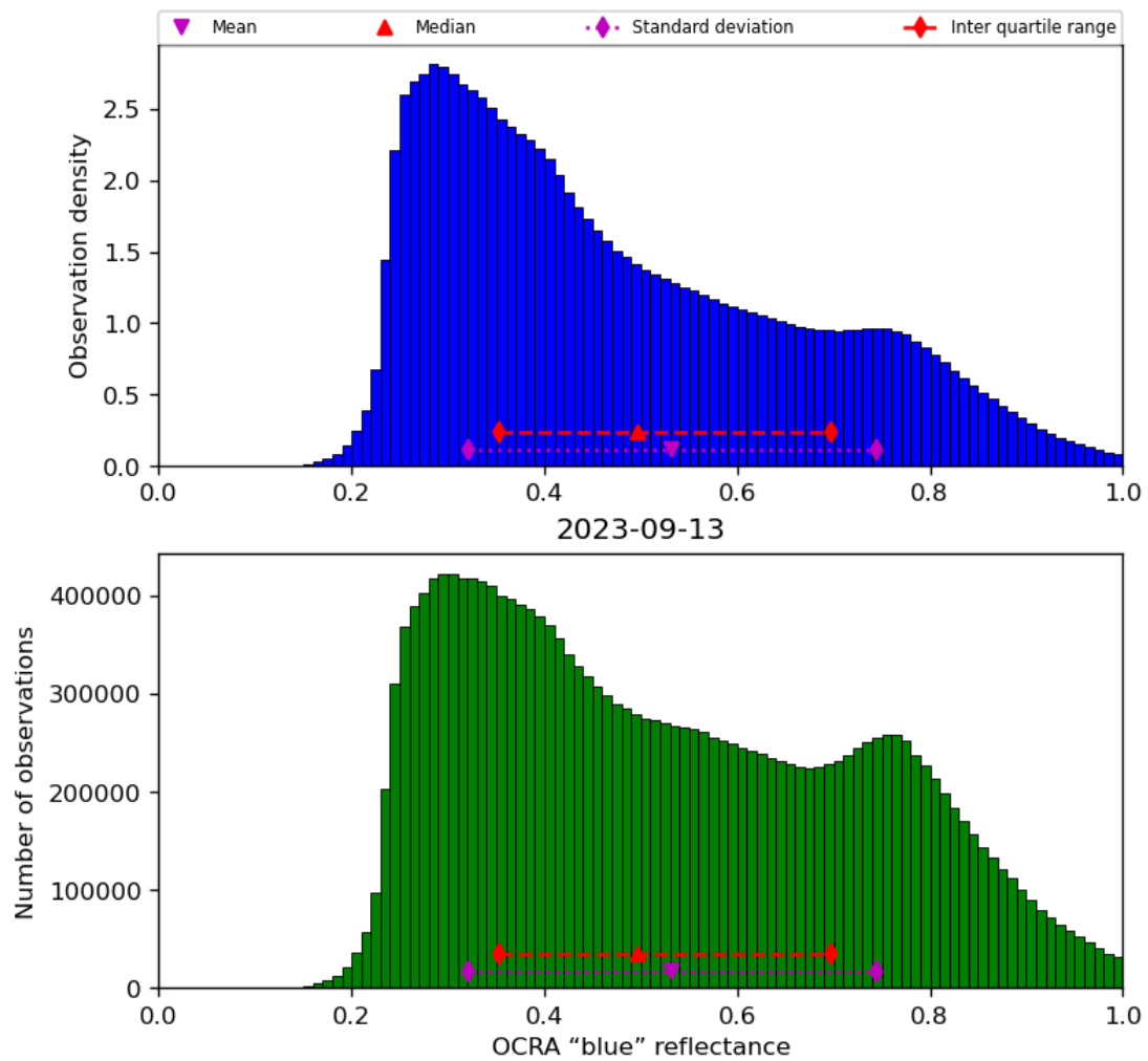
Figure 51: Histogram of “OCRA “blue” reflectance” for 2023-09-12 to 2023-09-14
