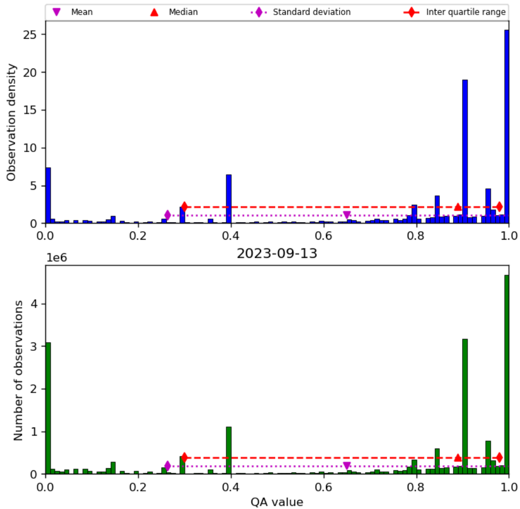
Figure 38: Histogram of “QA value” for 2023-09-12 to 2023-09-14
