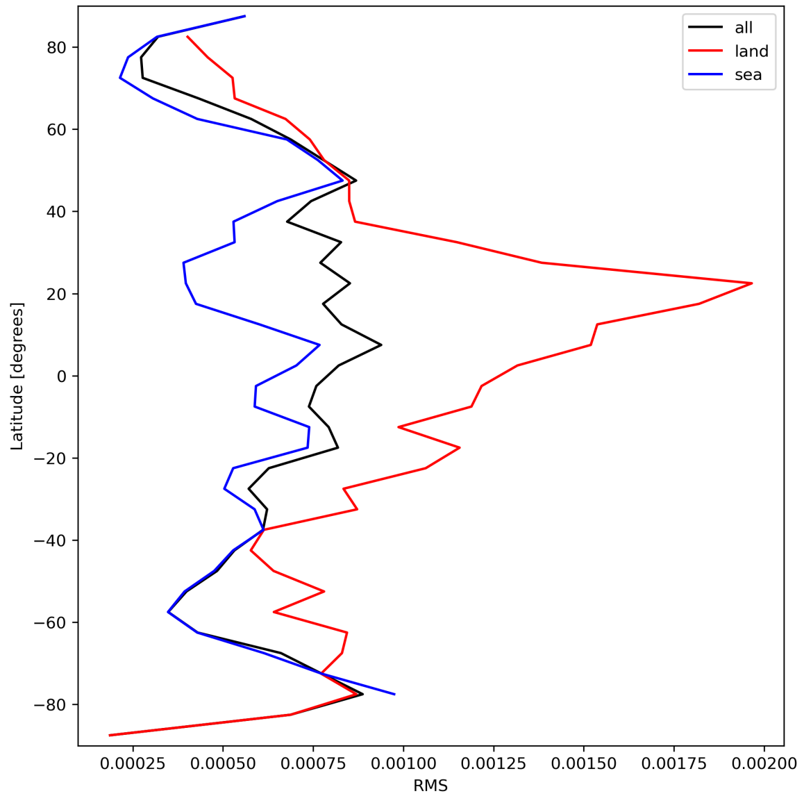
Figure 31: Zonal average of “RMS” for 2023-09-12 to 2023-09-14.
