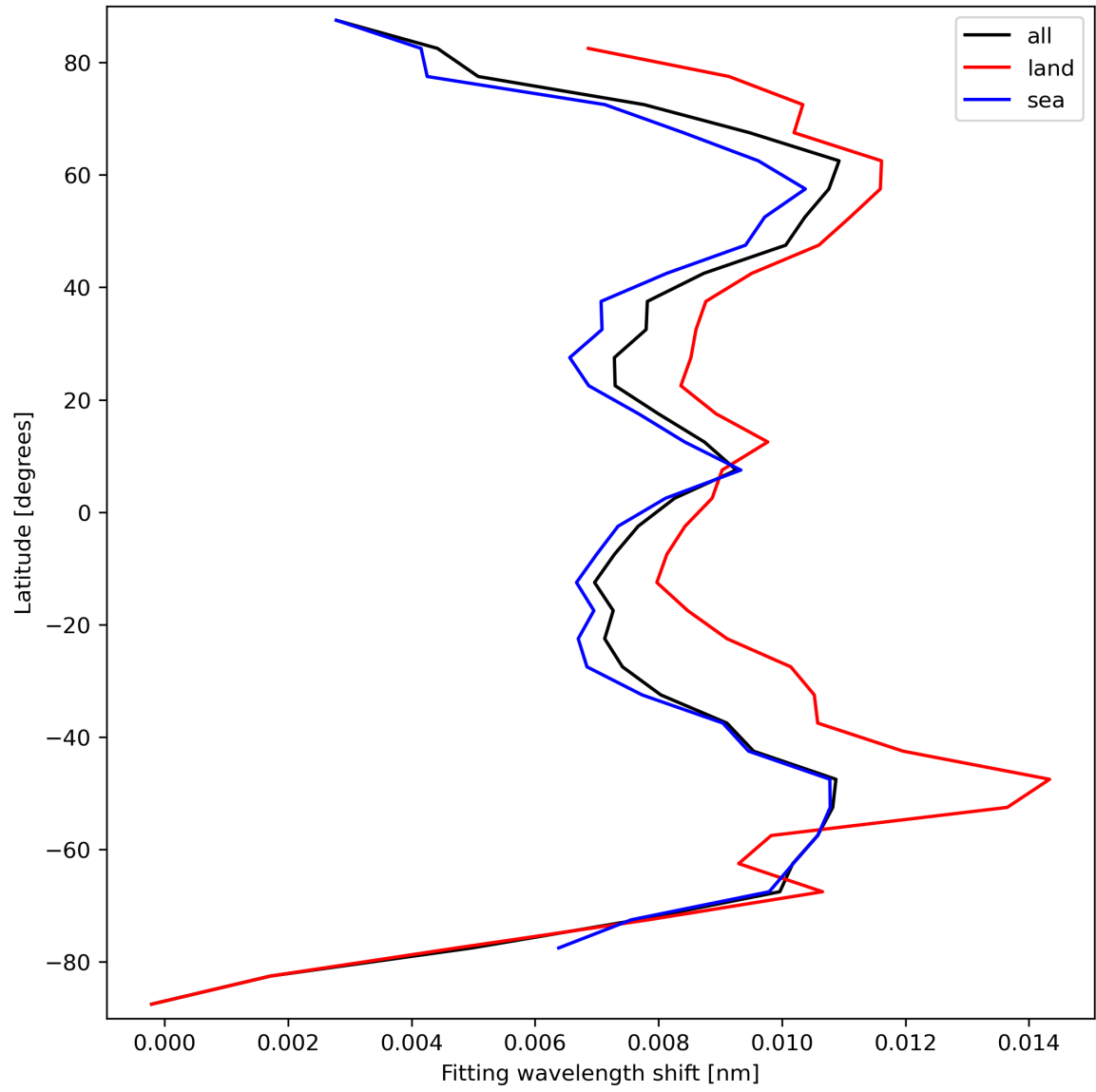
Figure 33: Zonal average of “Fitting wavelength shift” for 2023-09-12 to 2023-09-14.
