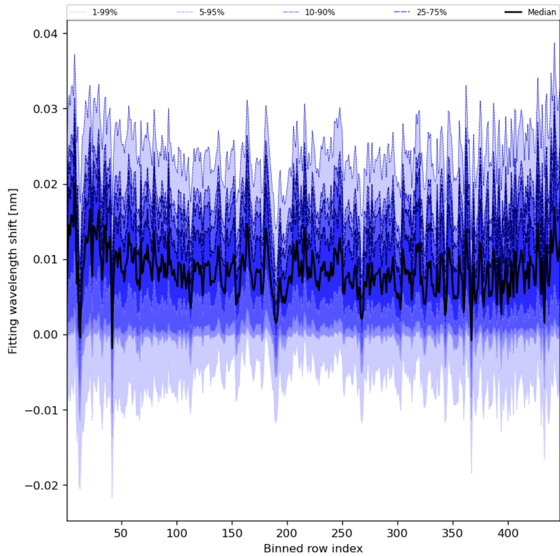
Figure 65: Along track statistics of “Fitting wavelength shift” for 2023-09-12 to 2023-09-14
