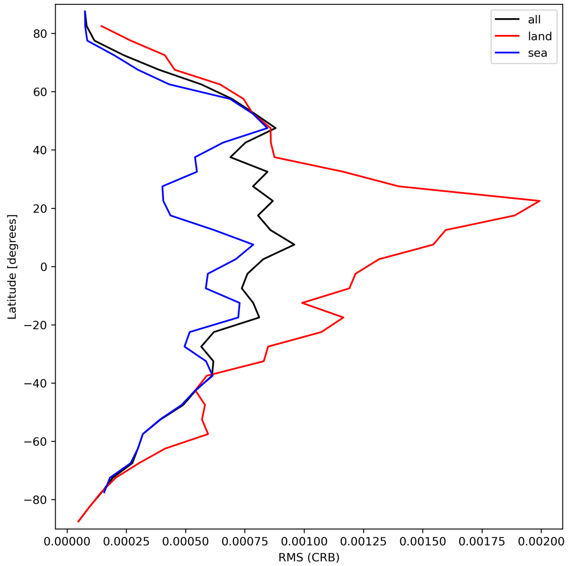
Figure 32: Zonal average of “RMS (CRB)” for 2023-09-12 to 2023-09-14.
