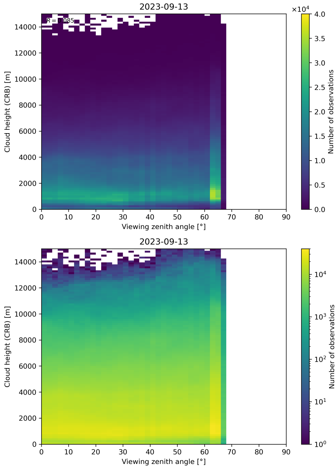
Figure 110: Scatter density plot of “Viewing zenith angle” against “Cloud height (CRB)” for 2023-09-12 to 2023-09-14.
