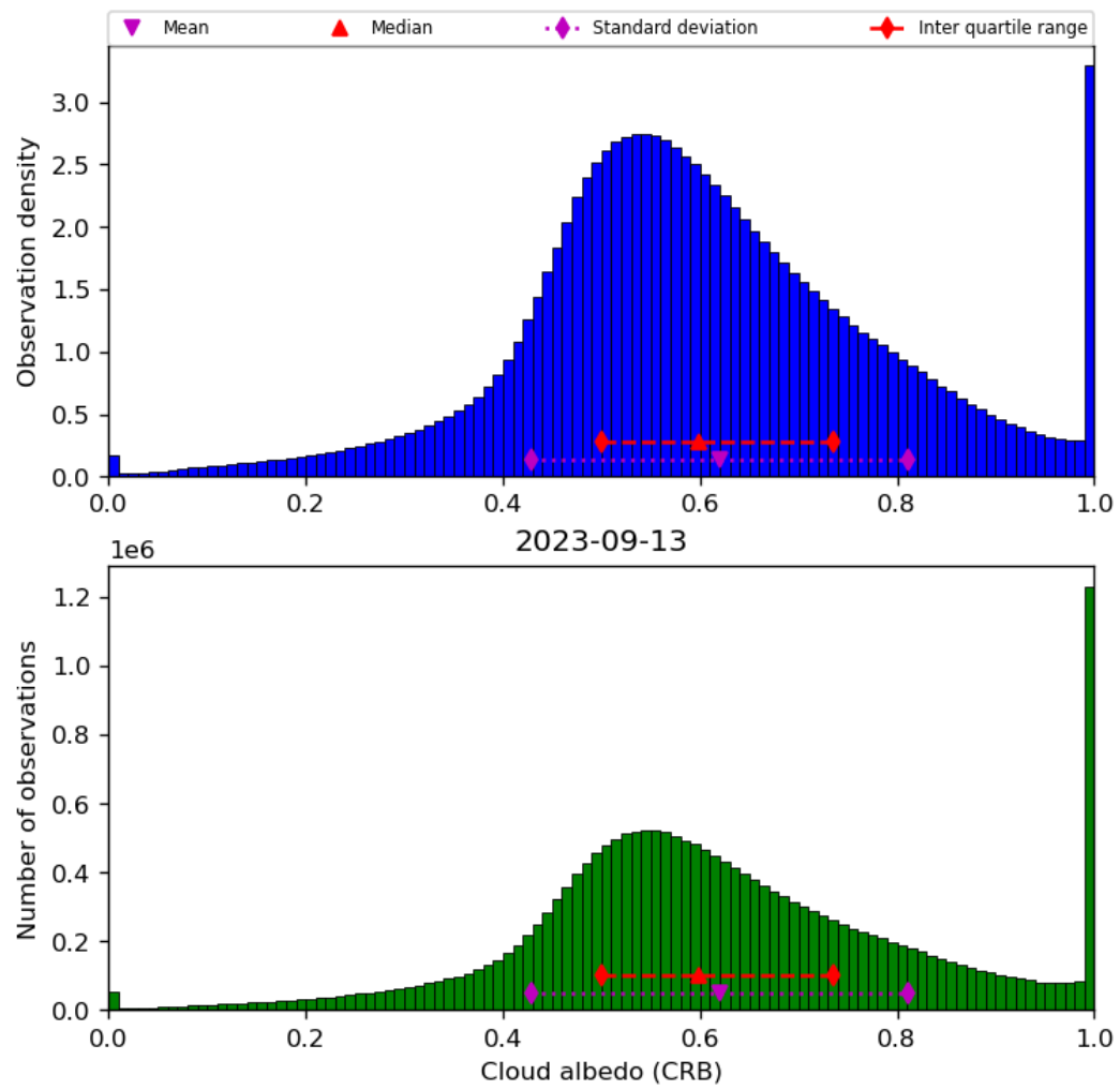
Figure 44: Histogram of “Cloud albedo (CRB)” for 2023-09-12 to 2023-09-14
