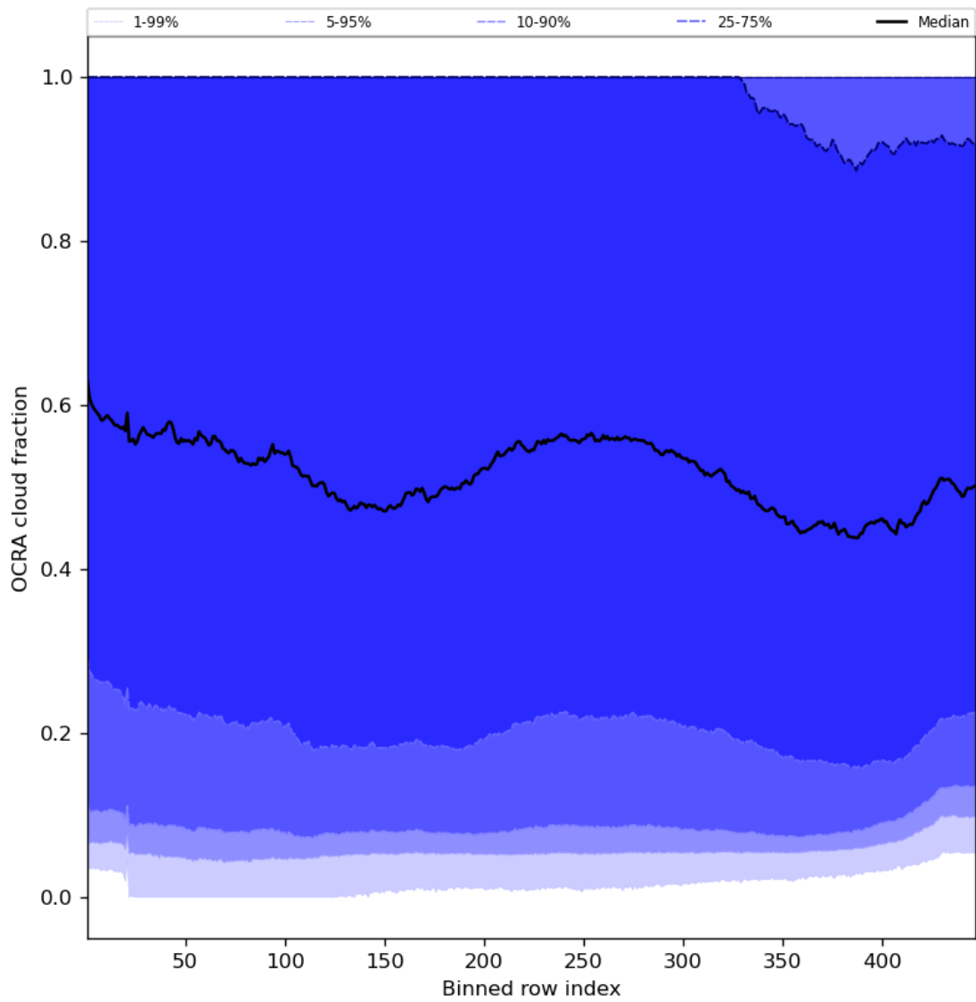
Figure 66: Along track statistics of “OCRA cloud fraction” for 2023-09-12 to 2023-09-14
