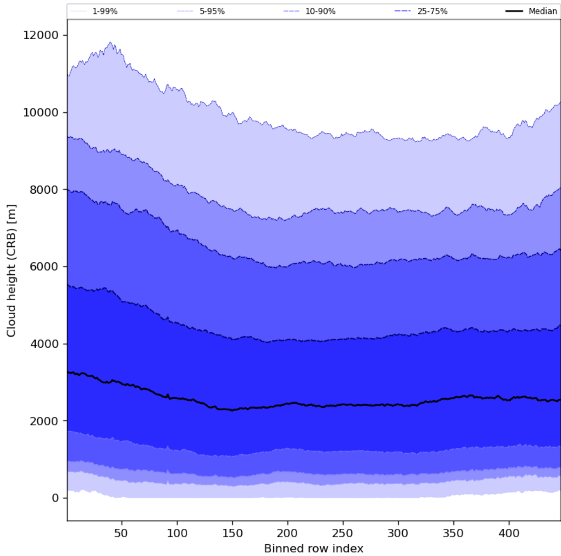
Figure 59: Along track statistics of “Cloud height (CRB)” for 2023-09-12 to 2023-09-14
