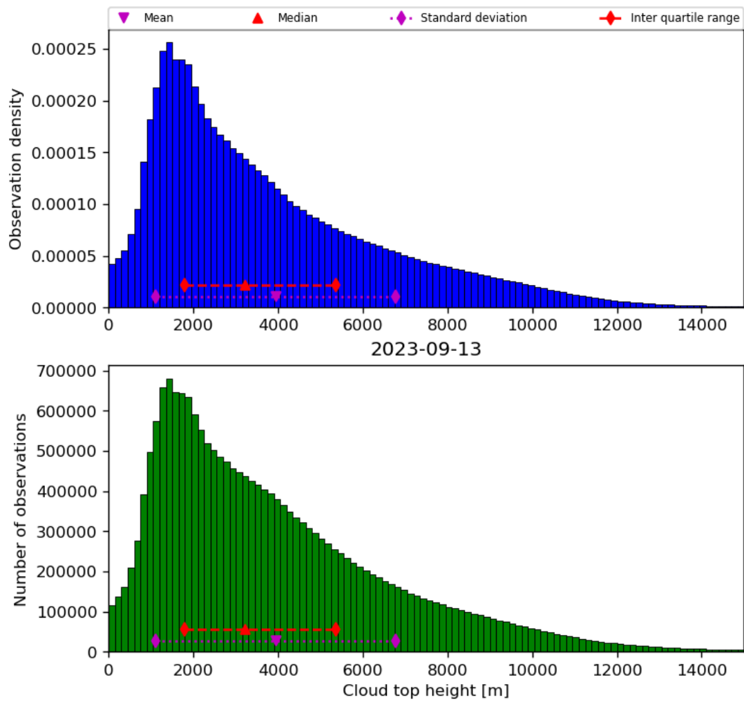
Figure 40: Histogram of “Cloud top height” for 2023-09-12 to 2023-09-14
