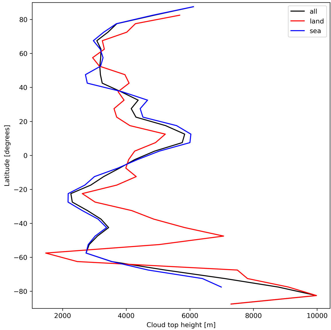
Figure 24: Zonal average of “Cloud top height” for 2023-09-12 to 2023-09-14.
