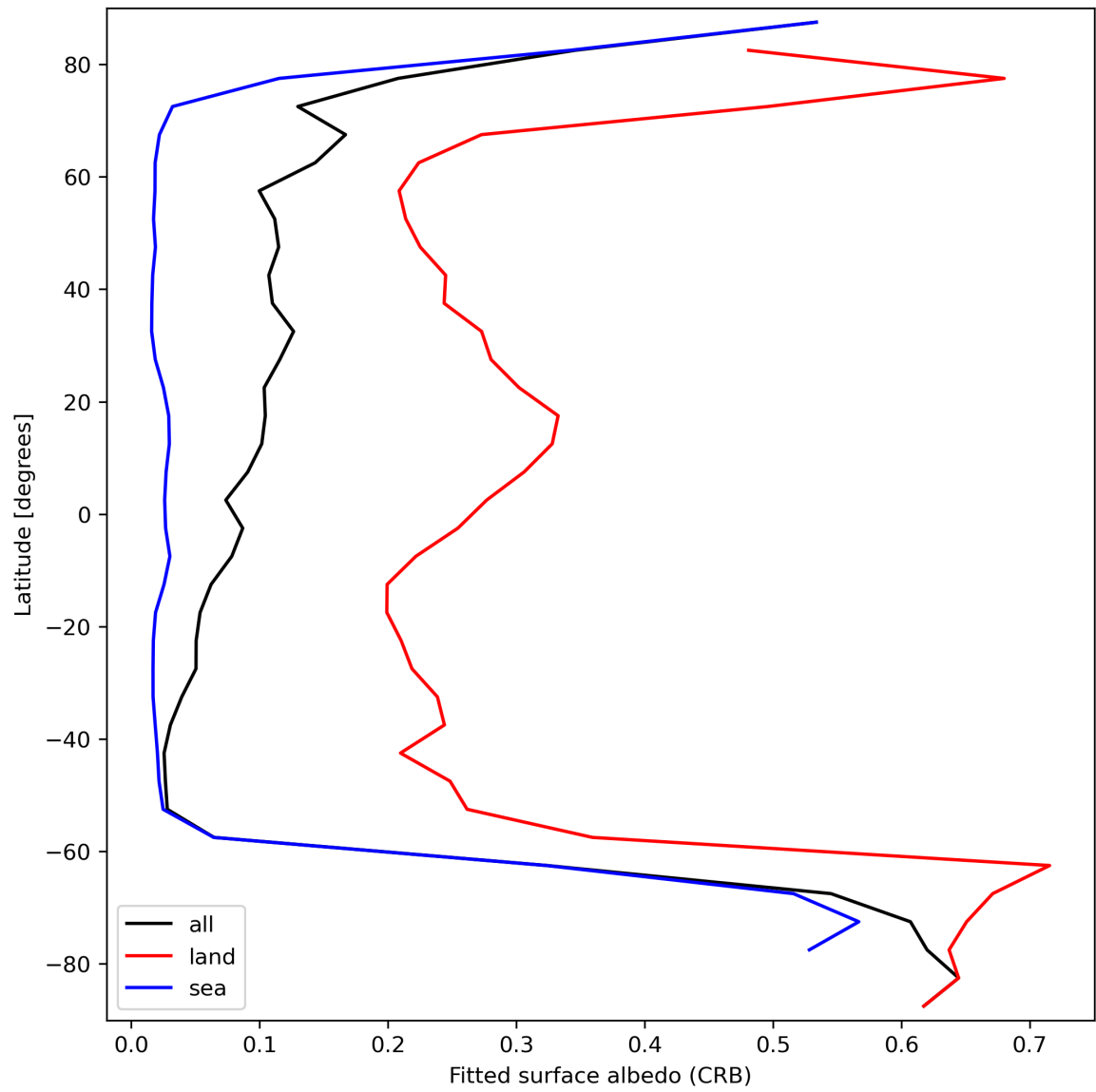
Figure 30: Zonal average of "Fitted surface albedo (CRB)" for 2023-09-12 to 2023-09-14.
