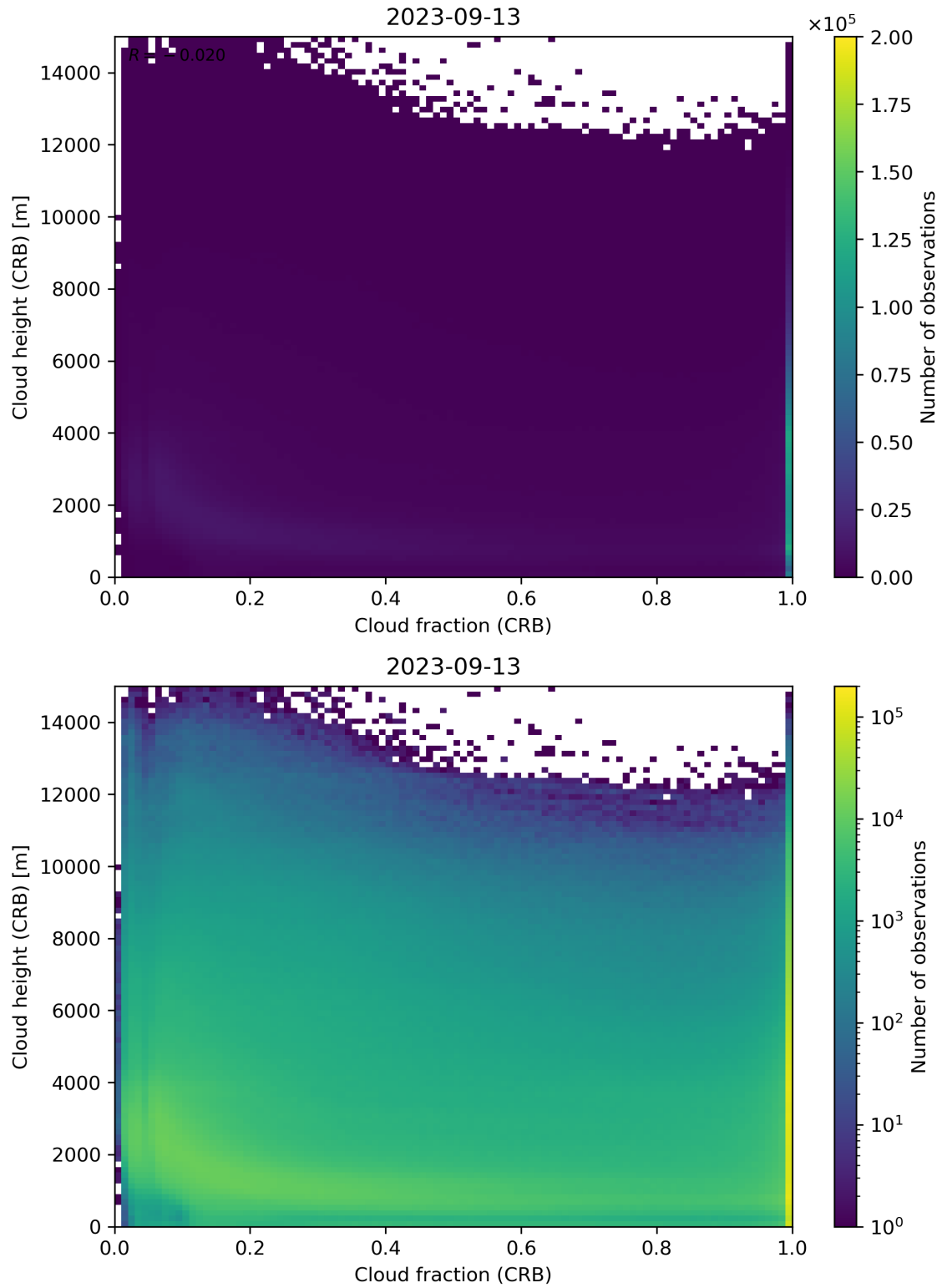
Figure 79: Scatter density plot of “Cloud fraction (CRB)” against “Cloud height (CRB)” for 2023-09-12 to 2023-09-14.
