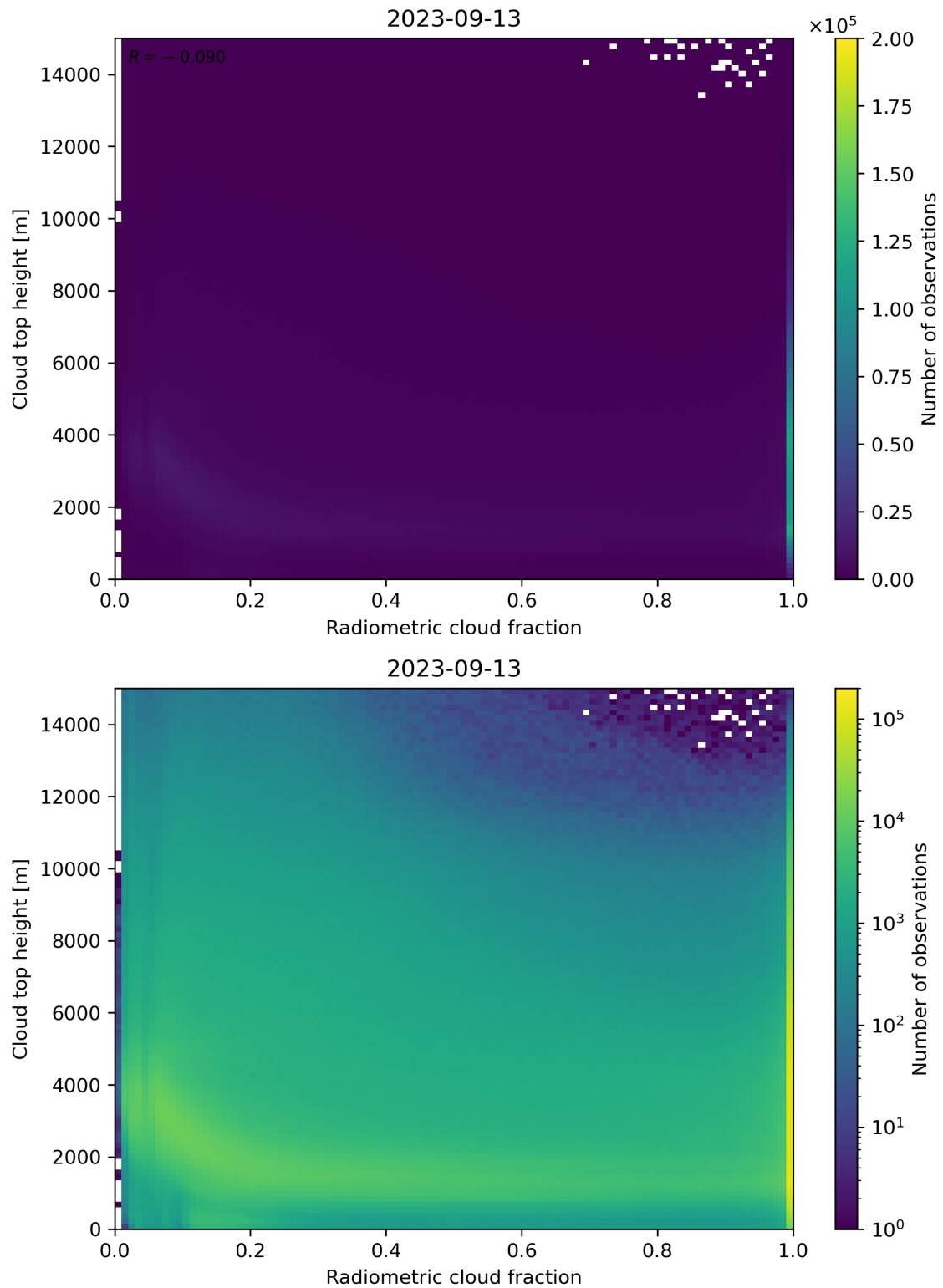
Figure 76: Scatter density plot of “Radiometric cloud fraction” against “Cloud top height” for 2023-09-12 to 2023-09-14.
