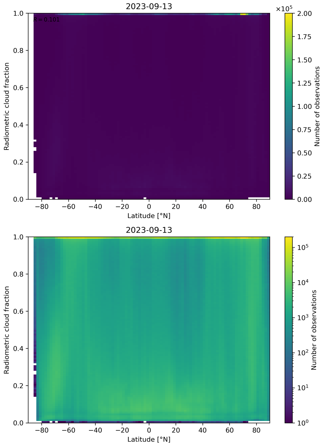
Figure 92: Scatter density plot of “Latitude” against “Radiometric cloud fraction” for 2023-09-12 to 2023-09-14.
