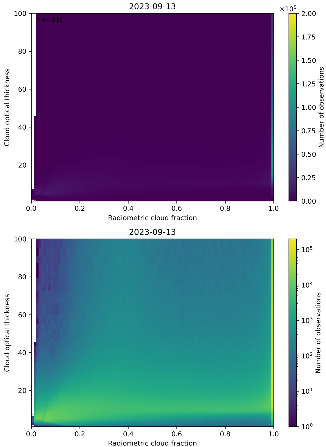
Figure 75: Scatter density plot of “Radiometric cloud fraction” against “Cloud optical thickness” for 2023-09-12 to 2023-09-14.
