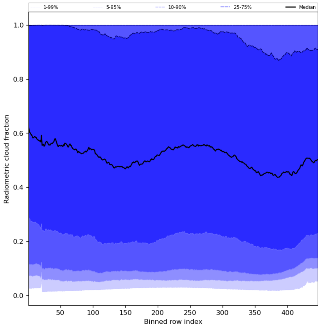
Figure 55: Along track statistics of “Radiometric cloud fraction” for 2023-09-12 to 2023-09-14
