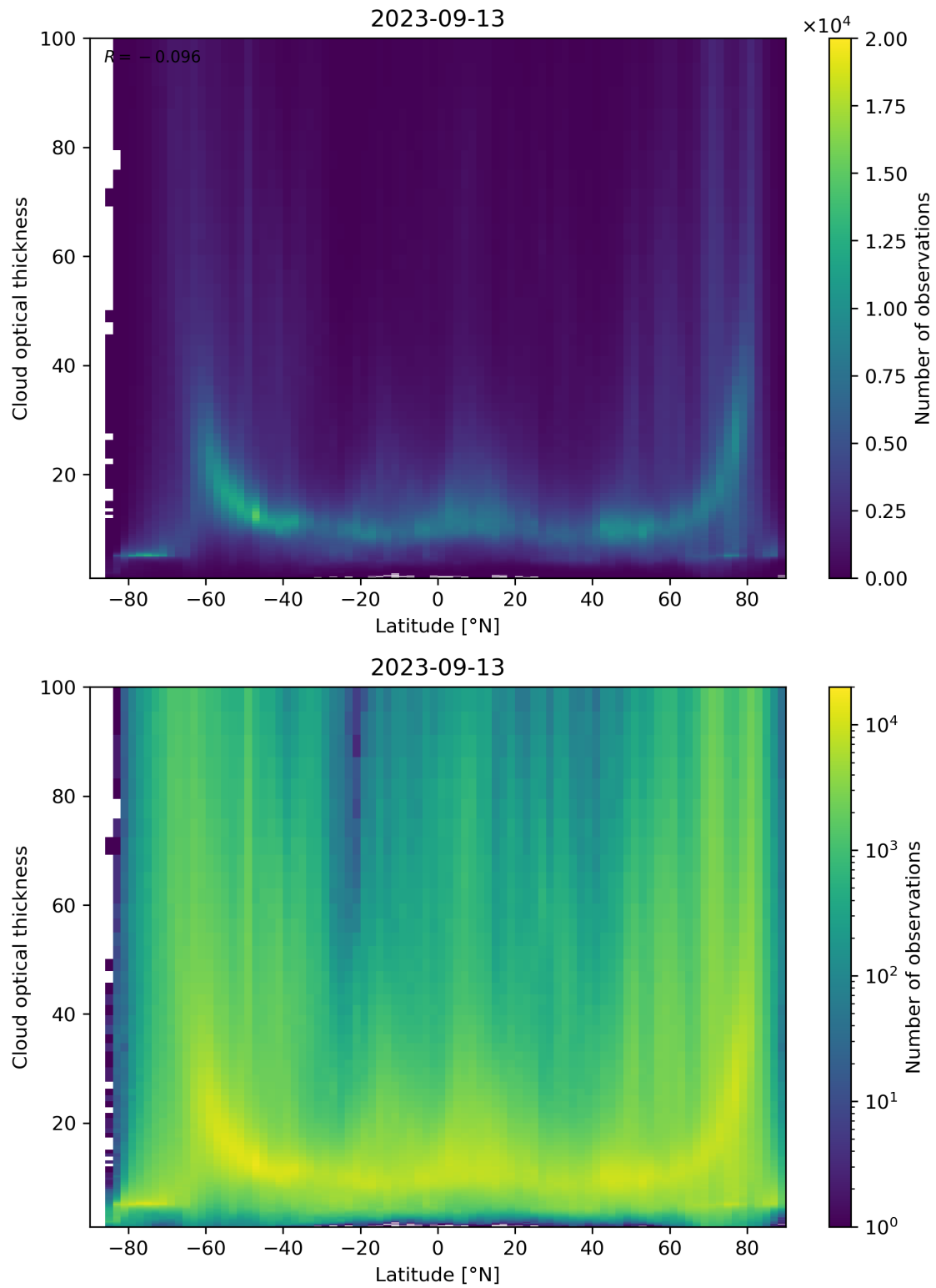
Figure 96: Scatter density plot of “Latitude” against “Cloud optical thickness” for 2023-09-12 to 2023-09-14.
