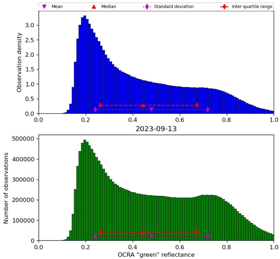
Figure 52: Histogram of “OCRA “green” reflectance” for 2023-09-12 to 2023-09-14
