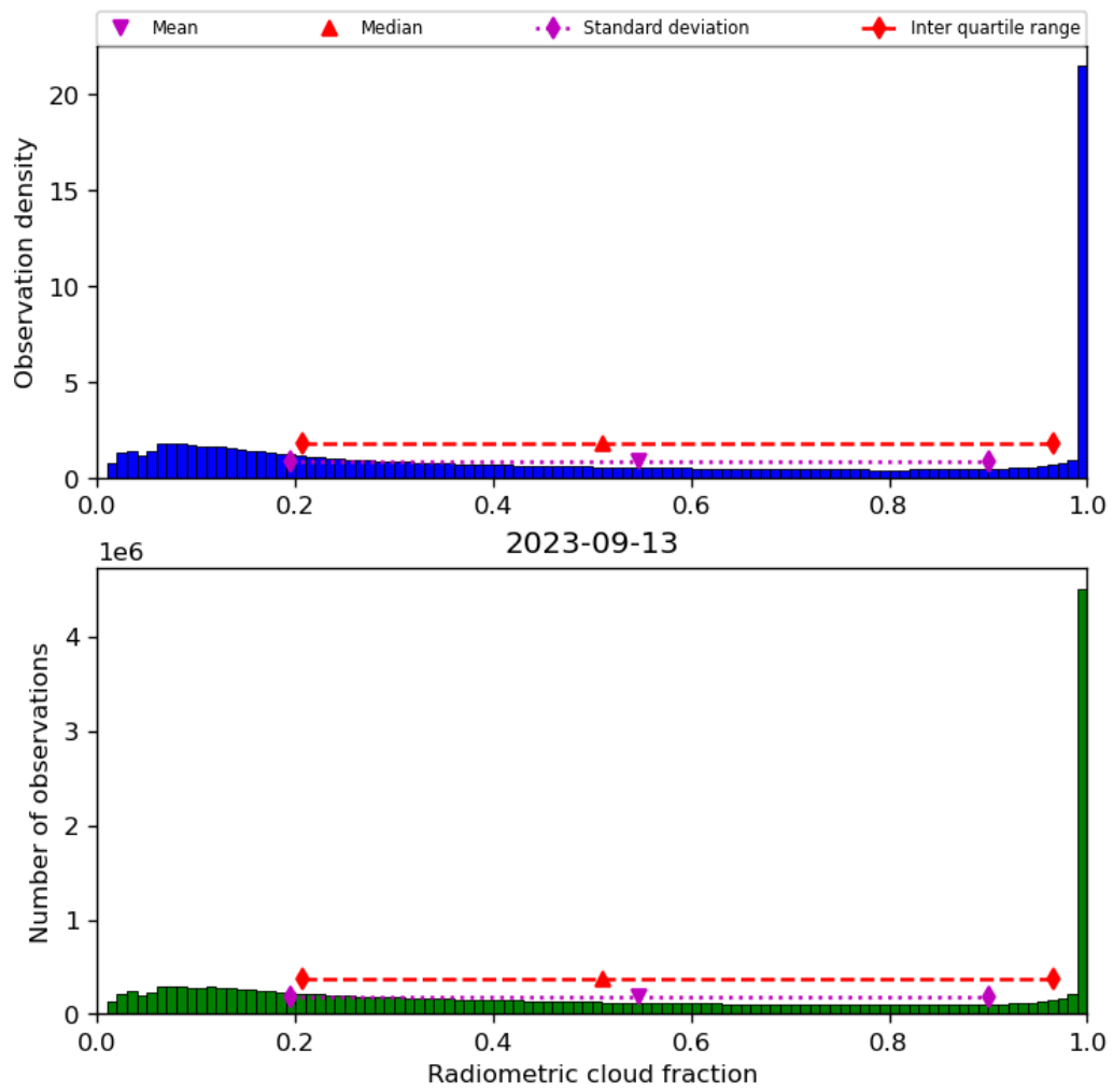
Figure 39: Histogram of “Radiometric cloud fraction” for 2023-09-12 to 2023-09-14
