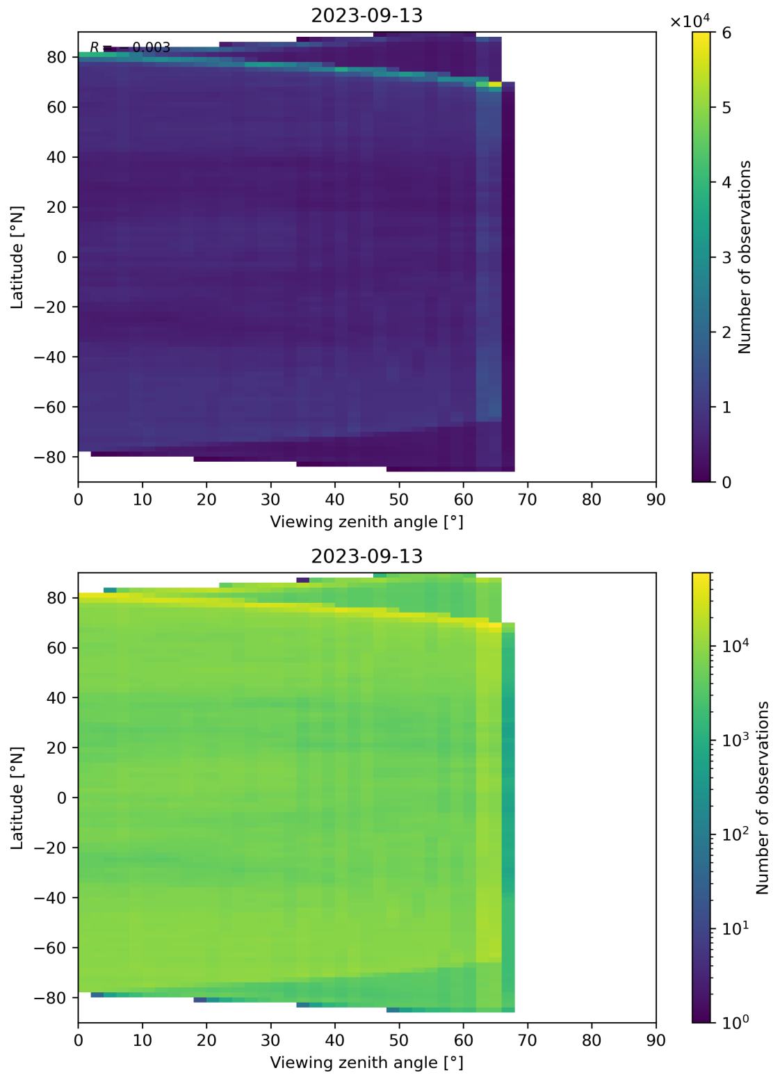
Figure 113: Scatter density plot of “Viewing zenith angle” against “Latitude” for 2023-09-12 to 2023-09-14.
