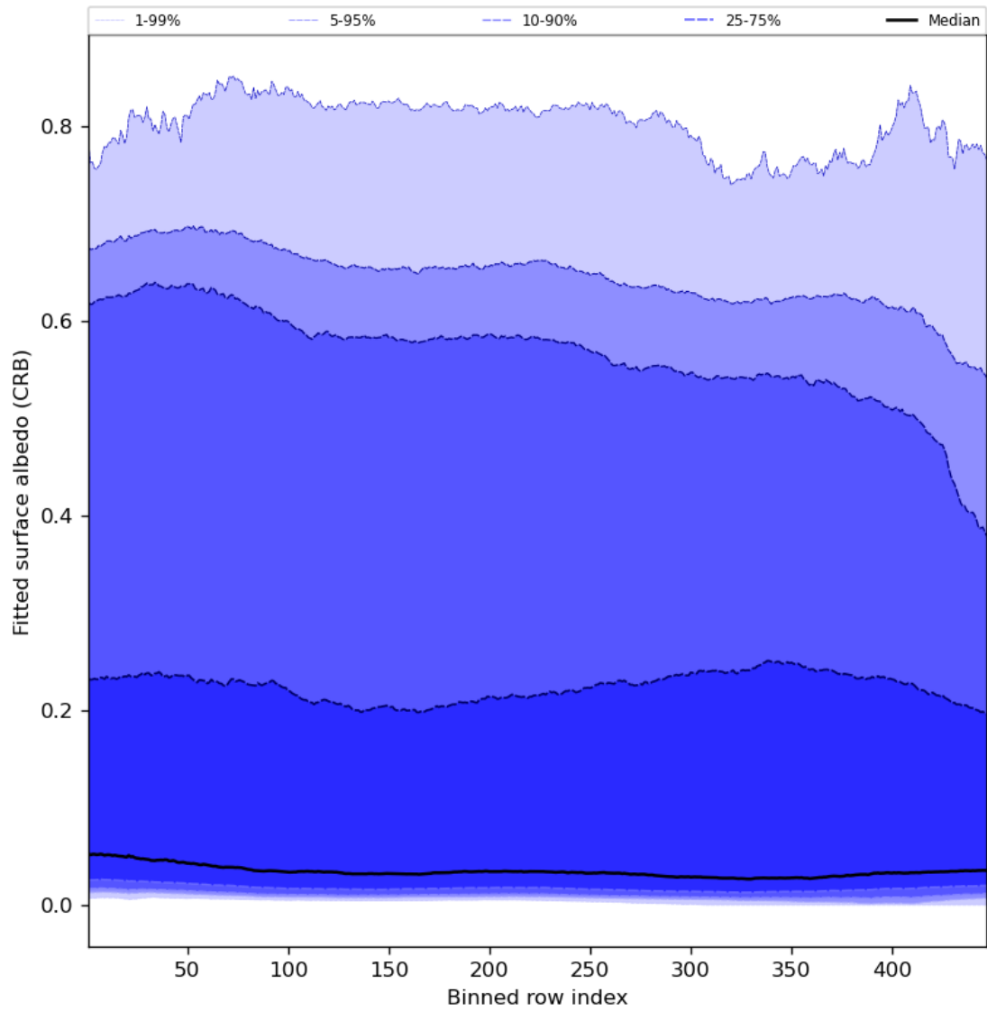
Figure 62: Along track statistics of “Fitted surface albedo (CRB)” for 2023-09-12 to 2023-09-14
