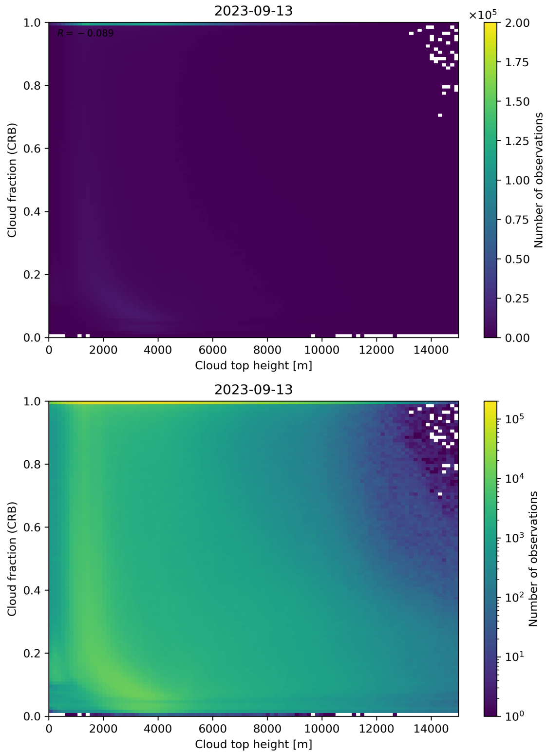
Figure 88: Scatter density plot of “Cloud top height” against “Cloud fraction (CRB)” for 2023-09-12 to 2023-09-14.
