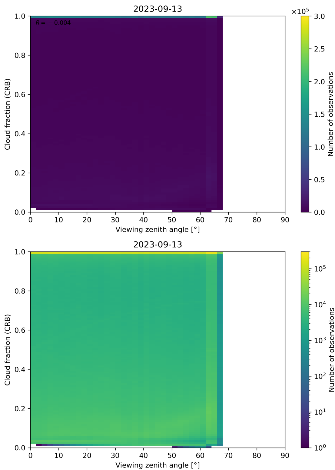
Figure 109: Scatter density plot of “Viewing zenith angle” against “Cloud fraction (CRB)” for 2023-09-12 to 2023-09-14.
