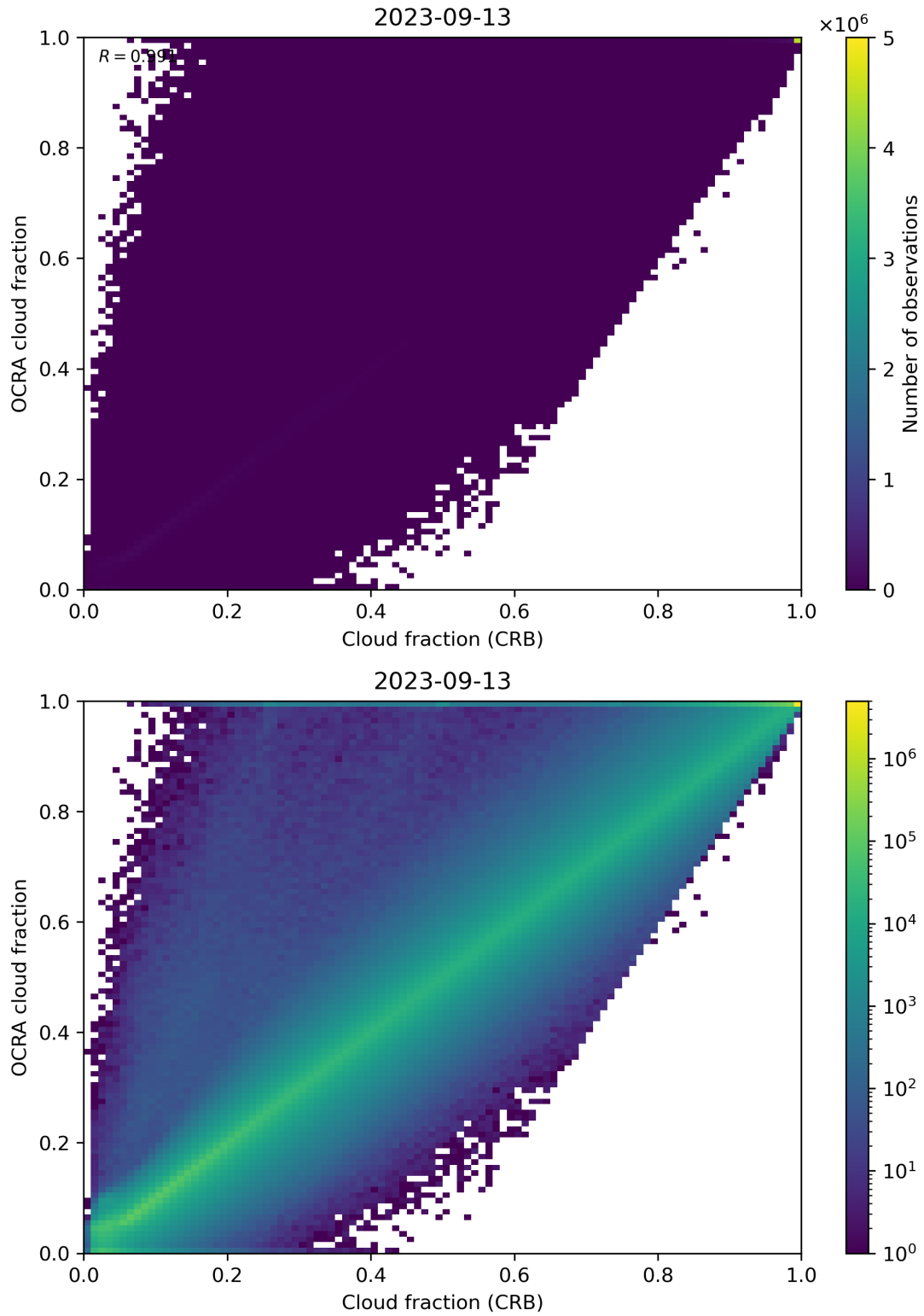
Figure 78: Scatter density plot of “Cloud fraction (CRB)” against “OCRA cloud fraction” for 2023-09-12 to 2023-09-14.
