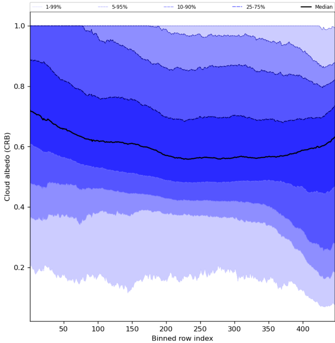
Figure 60: Along track statistics of “Cloud albedo (CRB)” for 2023-09-12 to 2023-09-14
