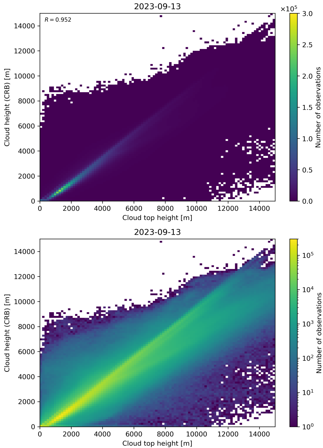
Figure 89: Scatter density plot of “Cloud top height” against “Cloud height (CRB)” for 2023-09-12 to 2023-09-14.
