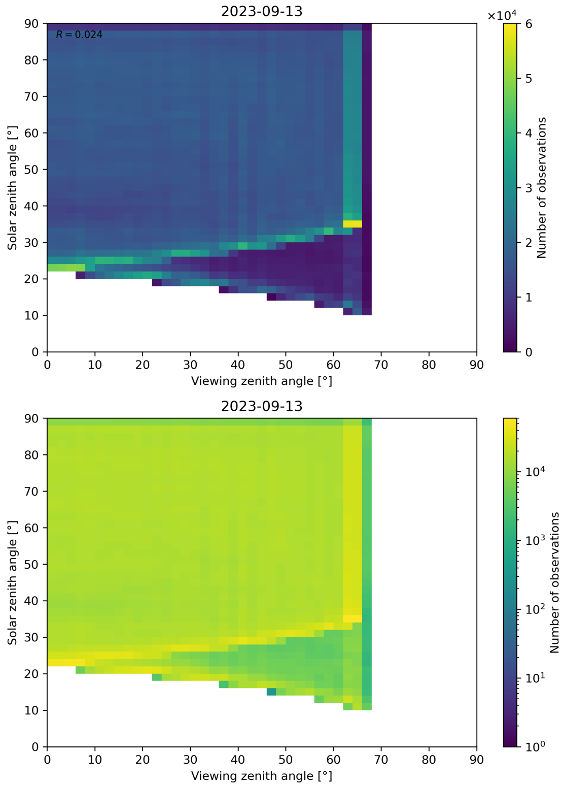
Figure 114: Scatter density plot of “Viewing zenith angle” against “Solar zenith angle” for 2023-09-12 to 2023-09-14.
