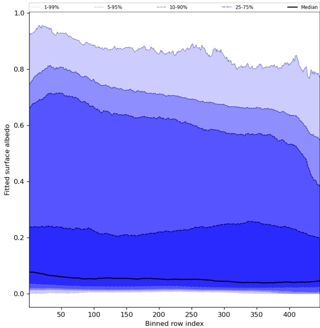
Figure 61: Along track statistics of “Fitted surface albedo” for 2023-09-12 to 2023-09-14
