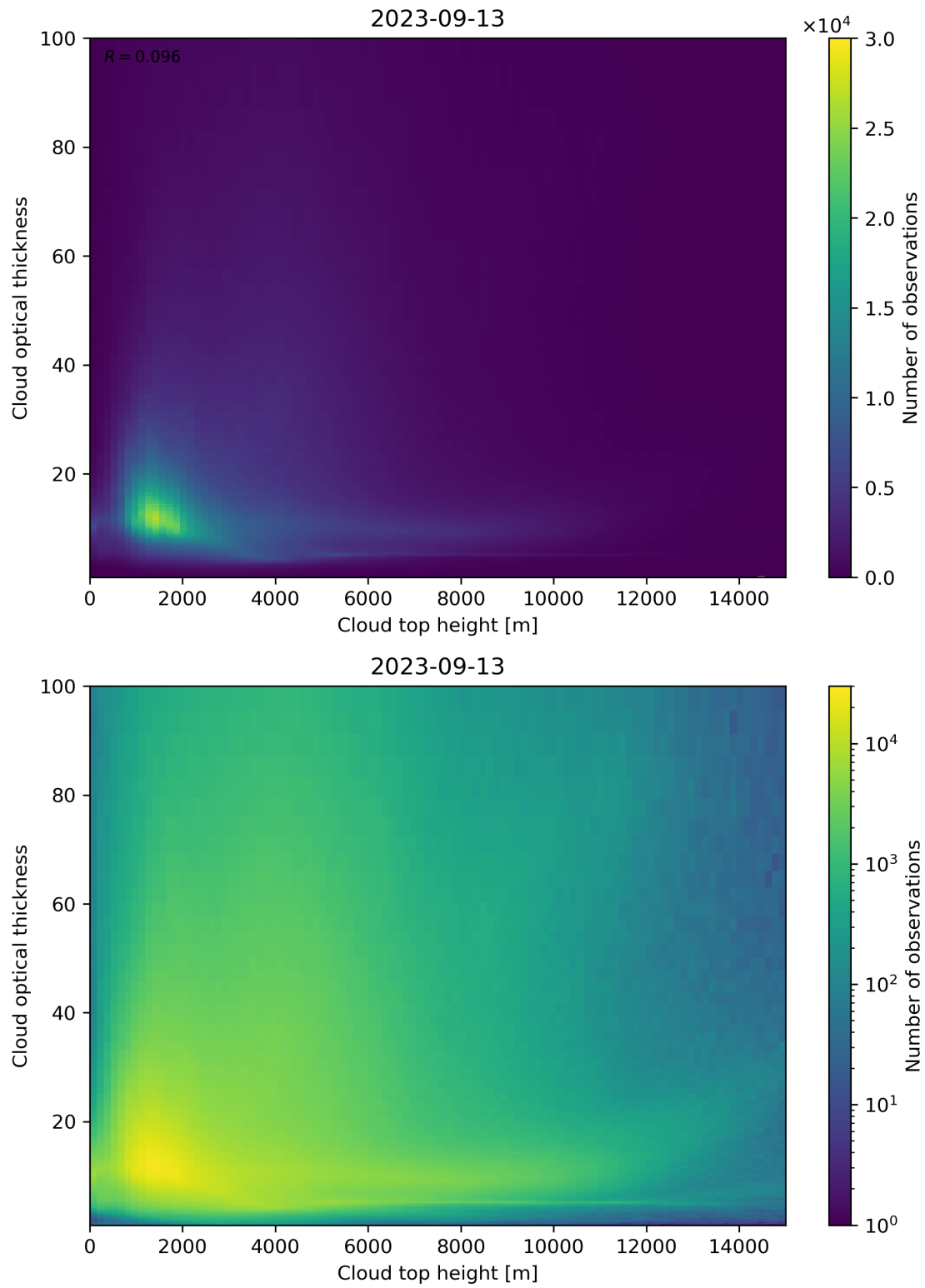
Figure 90: Scatter density plot of “Cloud top height” against “Cloud optical thickness” for 2023-09-12 to 2023-09-14.
