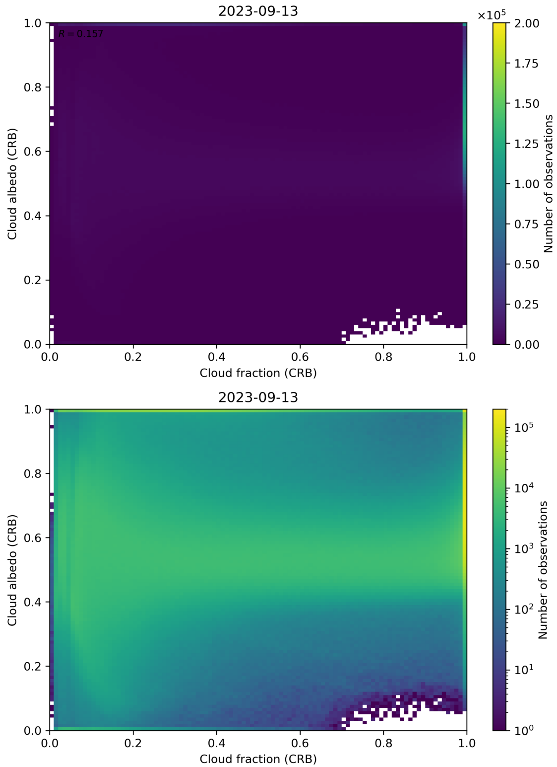
Figure 77: Scatter density plot of “Cloud fraction (CRB)” against “Cloud albedo (CRB)” for 2023-09-12 to 2023-09-14.
