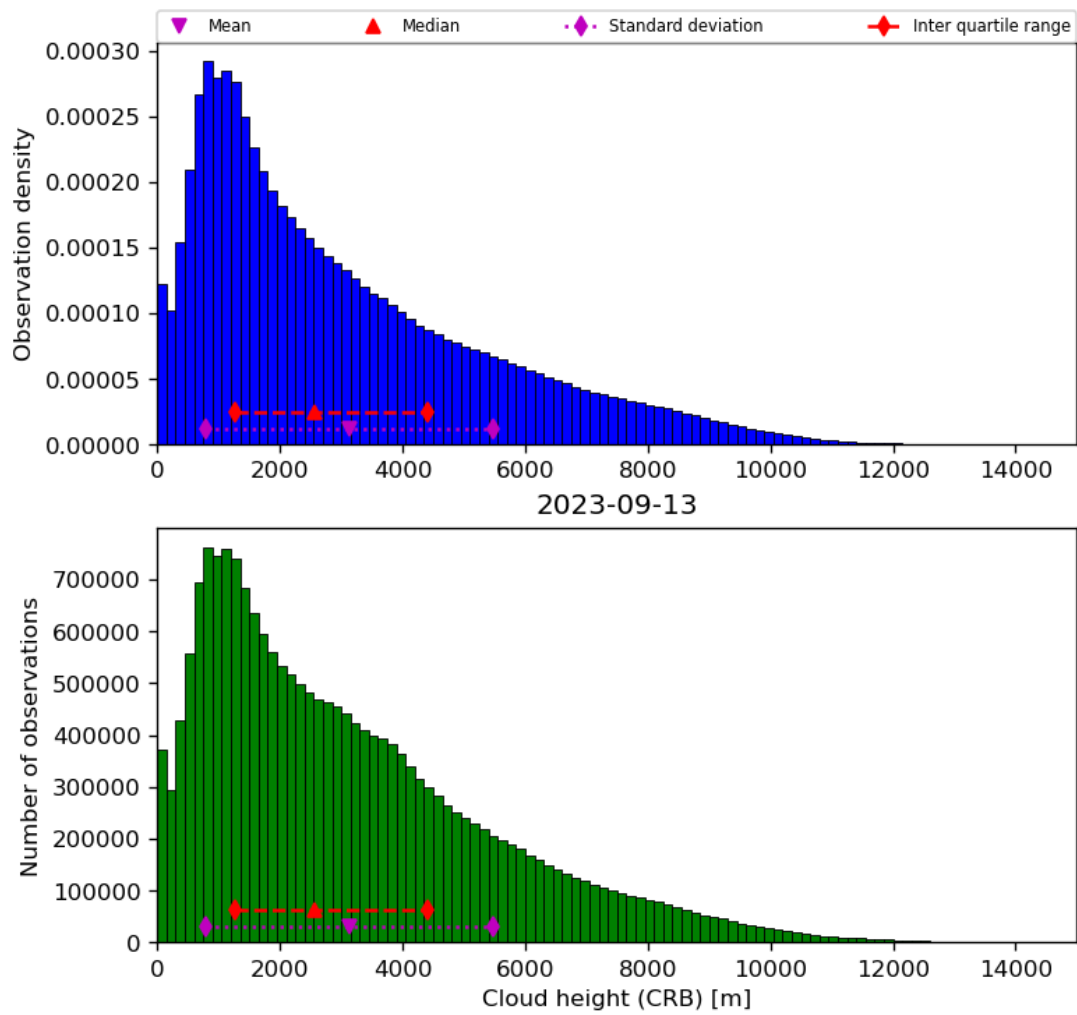
Figure 43: Histogram of “Cloud height (CRB)” for 2023-09-12 to 2023-09-14
