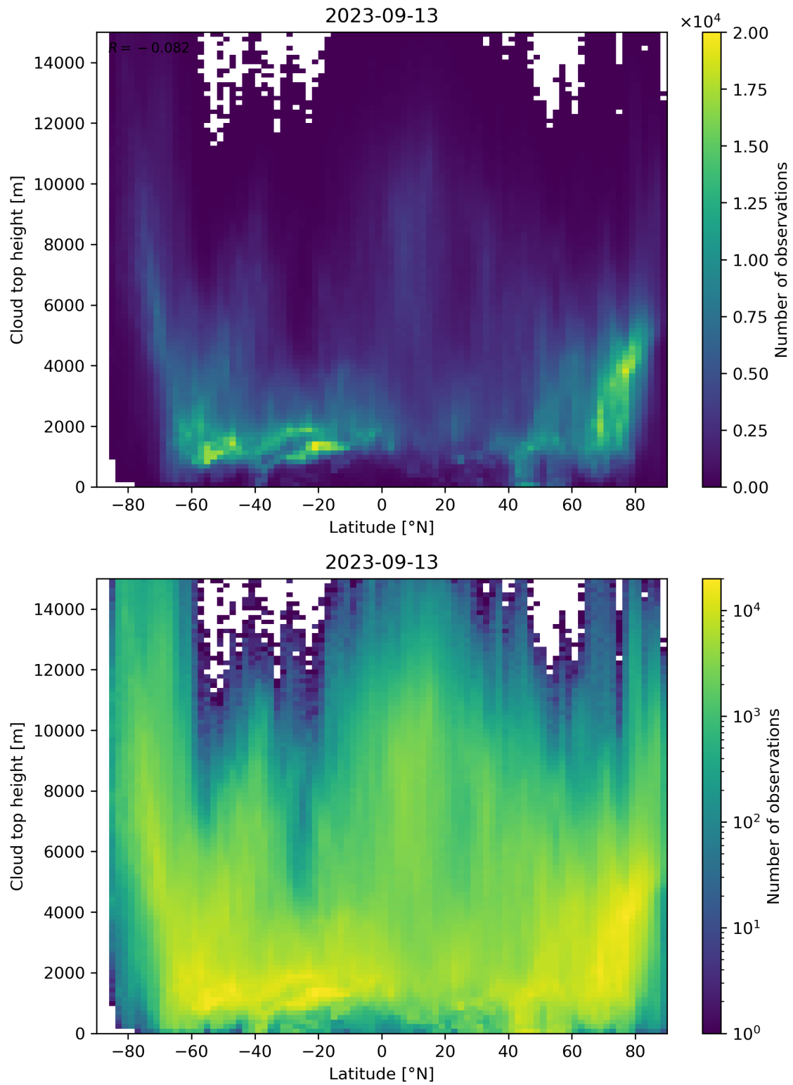
Figure 97: Scatter density plot of “Latitude” against “Cloud top height” for 2023-09-12 to 2023-09-14.
