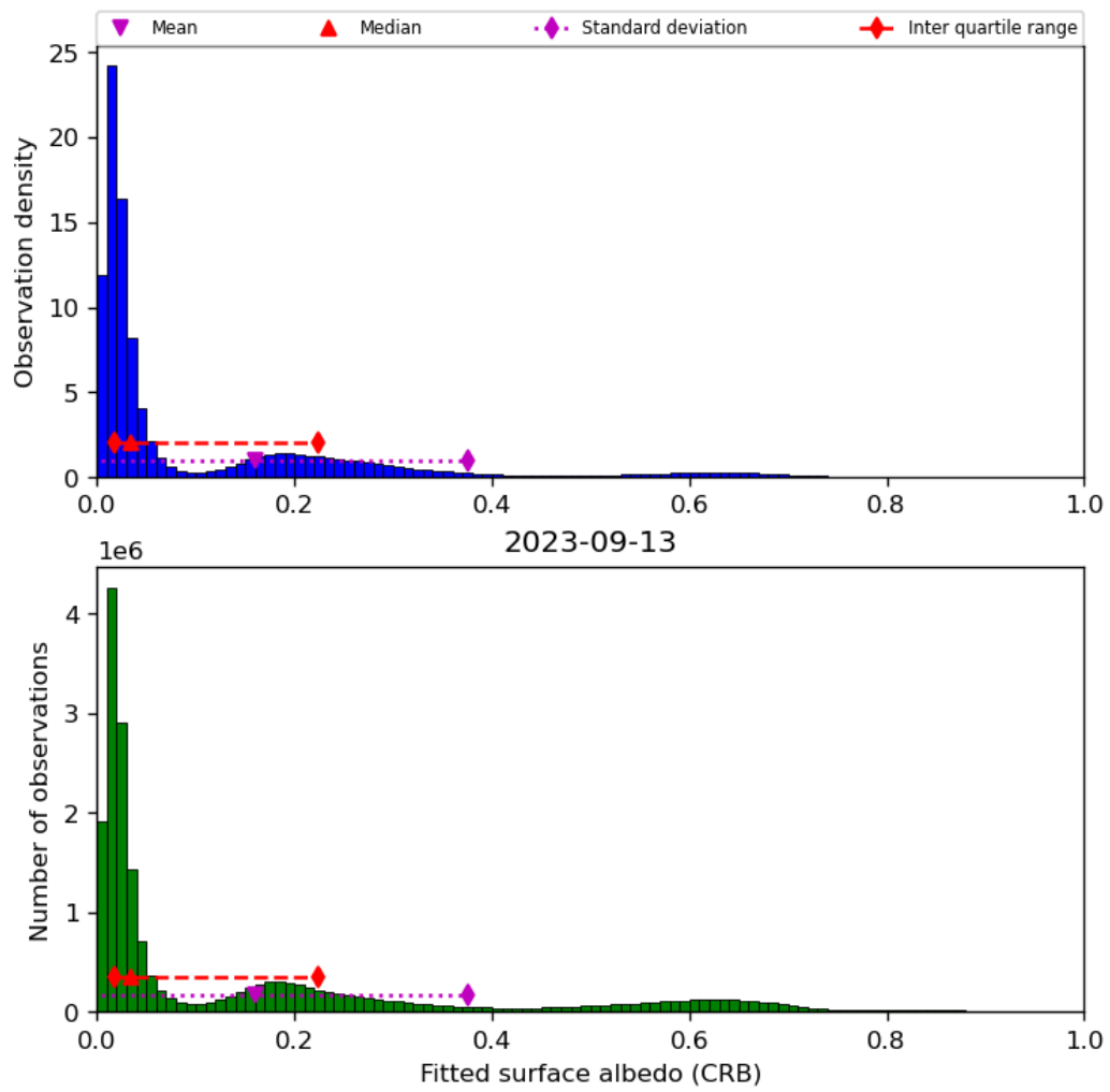
Figure 46: Histogram of “Fitted surface albedo (CRB)” for 2023-09-12 to 2023-09-14
