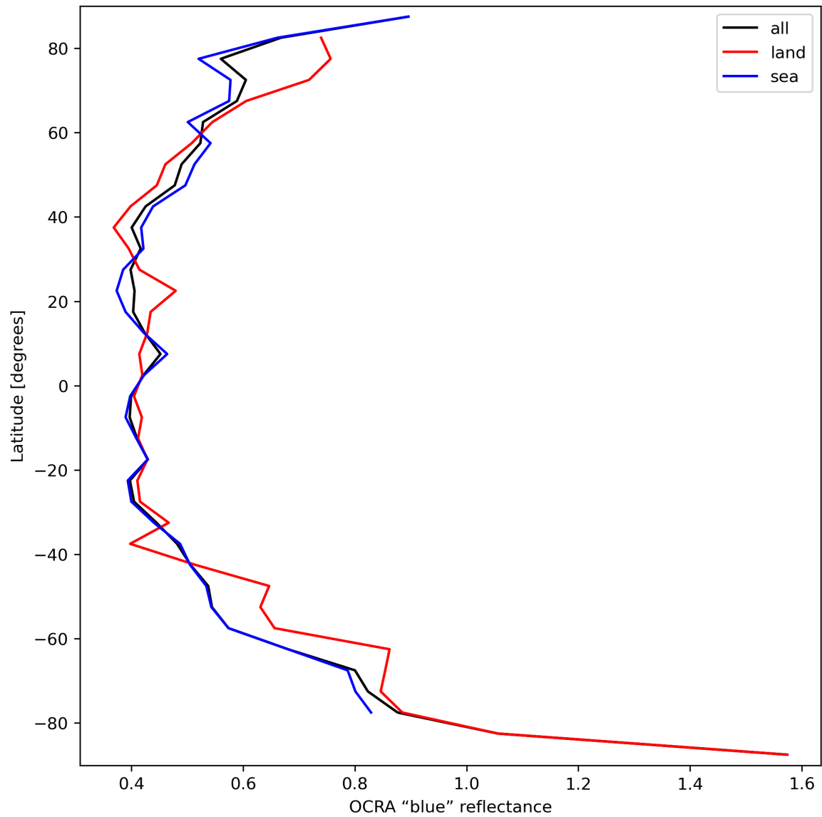
Figure 35: Zonal average of “OCRA “blue” reflectance” for 2023-09-12 to 2023-09-14.
