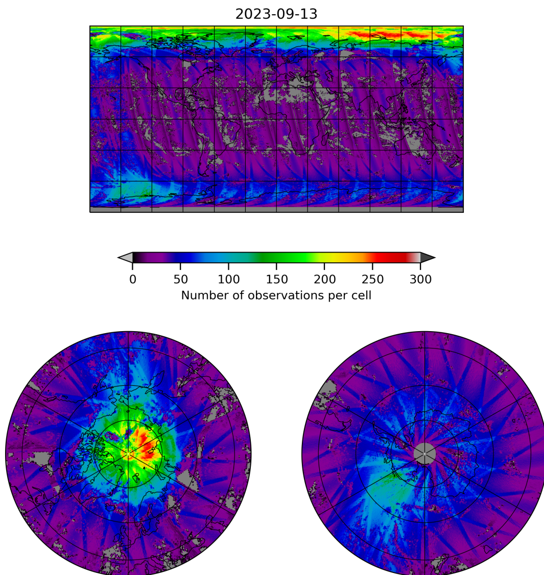
Figure 21: Map of the number of observations for 2023-09-12 to 2023-09-14
