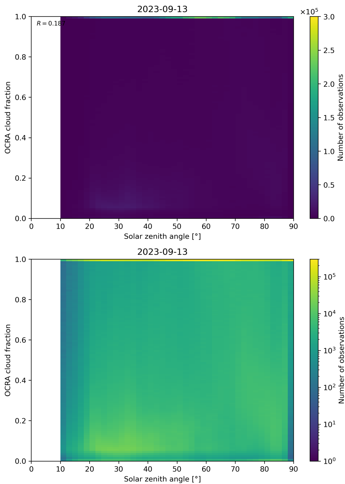
Figure 100: Scatter density plot of “Solar zenith angle” against “OCRA cloud fraction” for 2023-09-12 to 2023-09-14.
