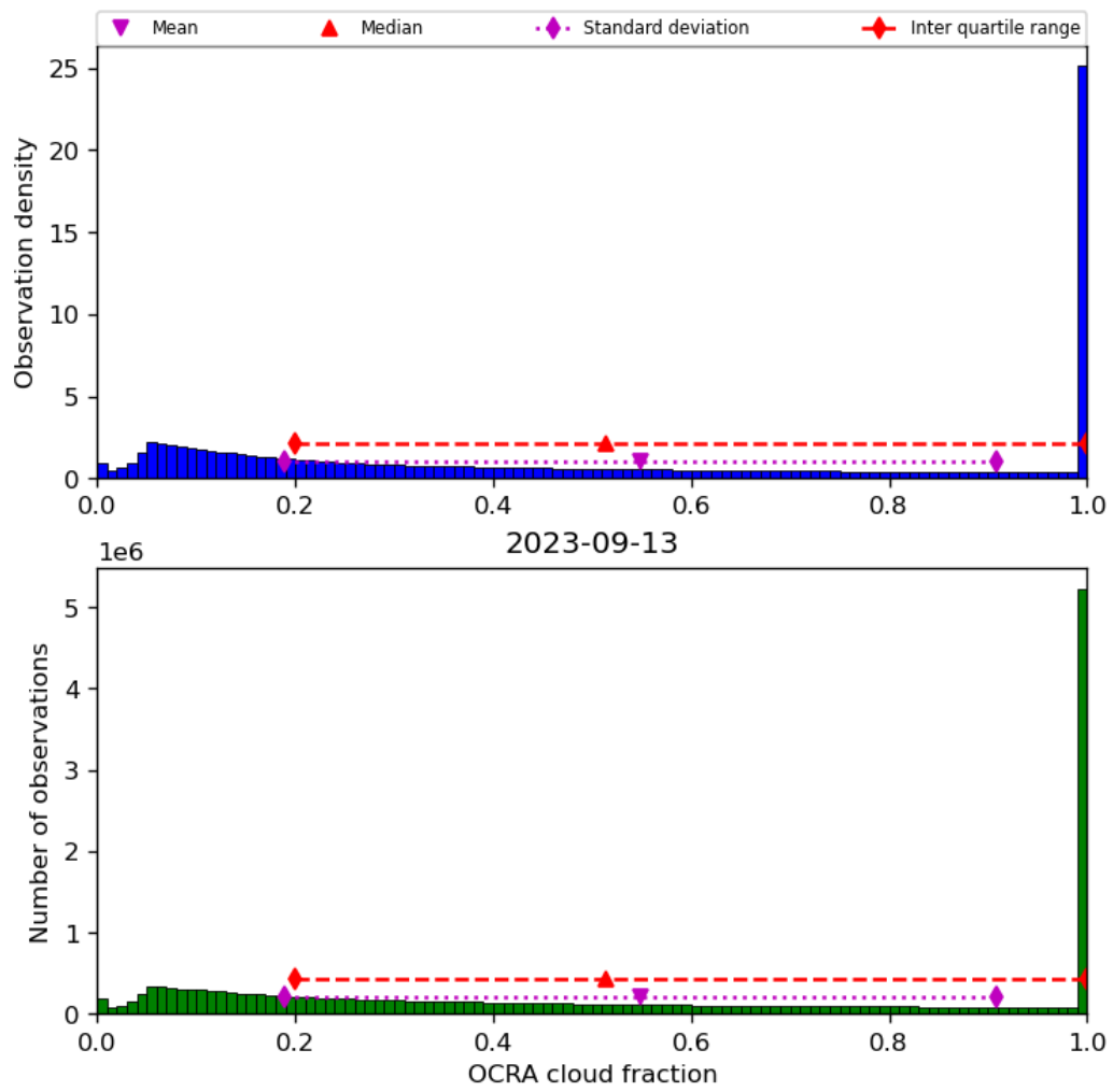
Figure 50: Histogram of “OCRA cloud fraction” for 2023-09-12 to 2023-09-14
