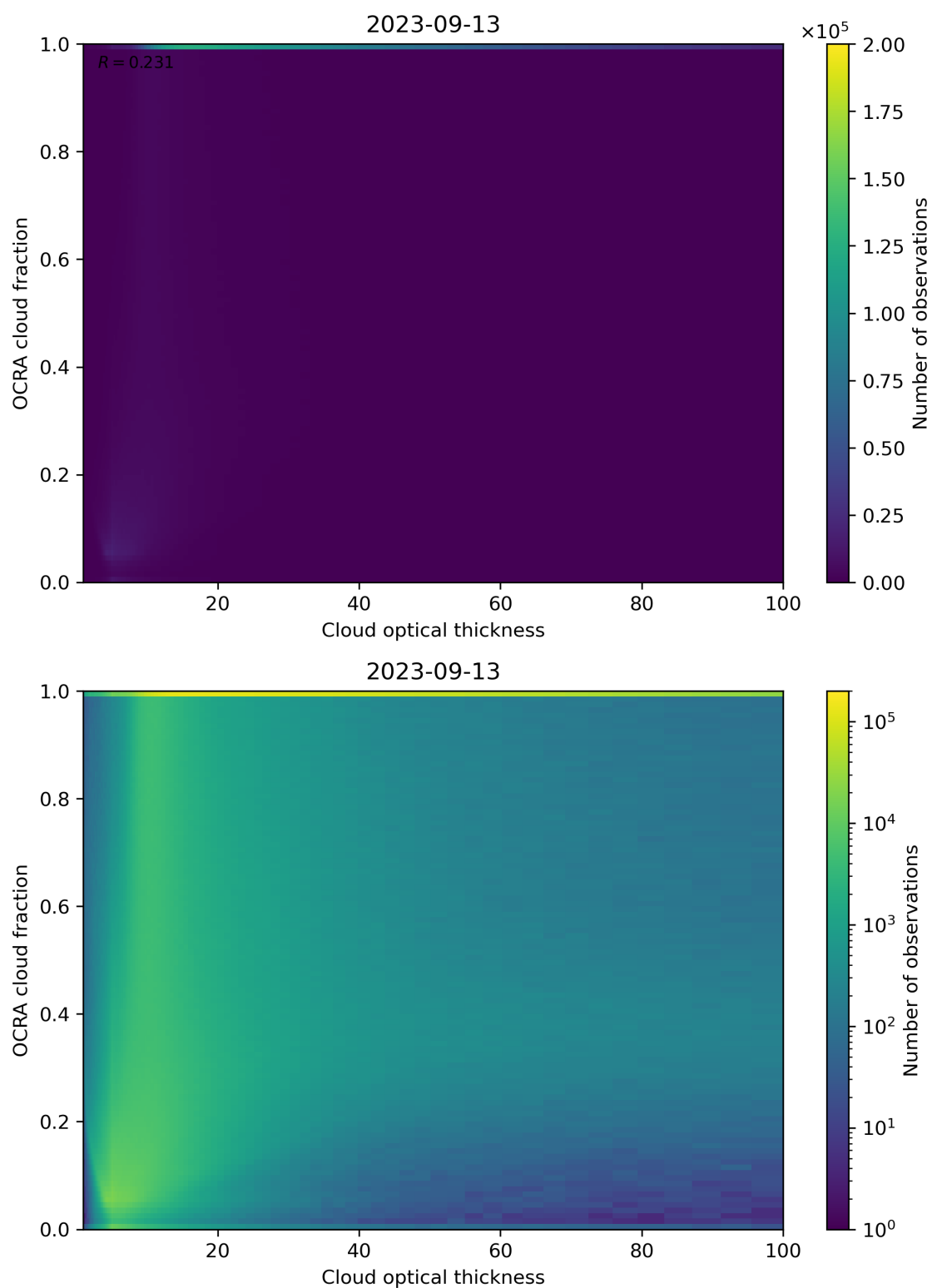
Figure 83: Scatter density plot of “Cloud optical thickness” against “OCRA cloud fraction” for 2023-09-12 to 2023-09-14.
