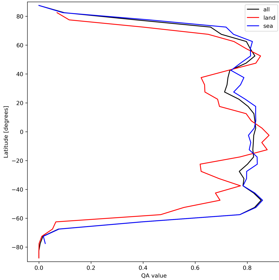
Figure 22: Zonal average of “QA value” for 2023-09-12 to 2023-09-14.
