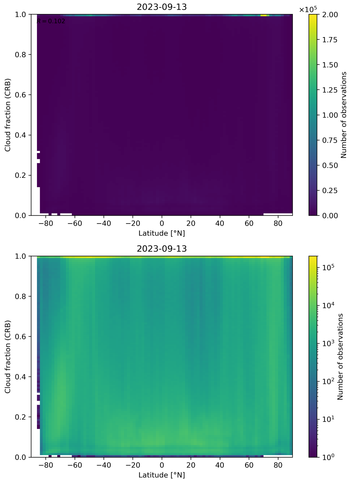
Figure 94: Scatter density plot of “Latitude” against “Cloud fraction (CRB)” for 2023-09-12 to 2023-09-14.
