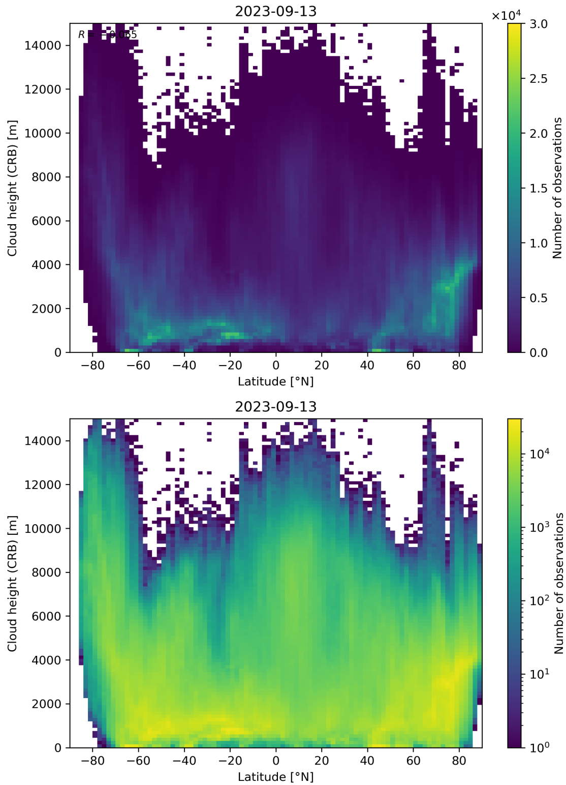
Figure 95: Scatter density plot of “Latitude” against “Cloud height (CRB)” for 2023-09-12 to 2023-09-14.
