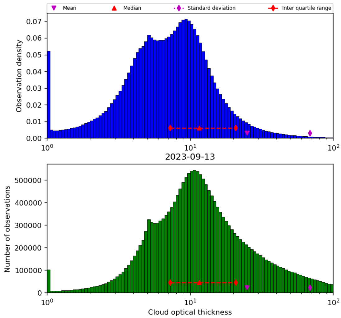
Figure 41: Histogram of “Cloud optical thickness” for 2023-09-12 to 2023-09-14
