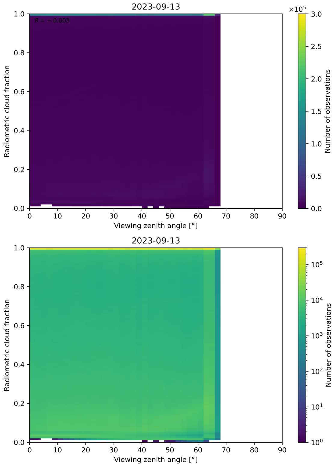
Figure 107: Scatter density plot of “Viewing zenith angle” against “Radiometric cloud fraction” for 2023-09-12 to 2023-09-14.
