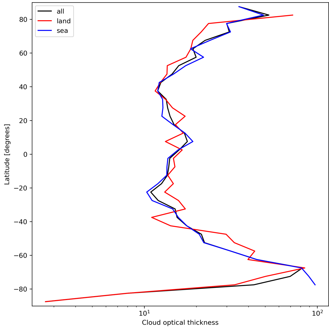
Figure 25: Zonal average of “Cloud optical thickness” for 2023-09-12 to 2023-09-14.
