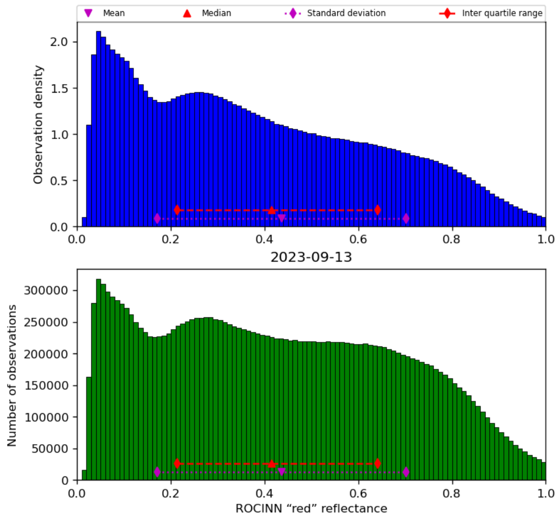
Figure 53: Histogram of “ROCINN “red” reflectance” for 2023-09-12 to 2023-09-14
