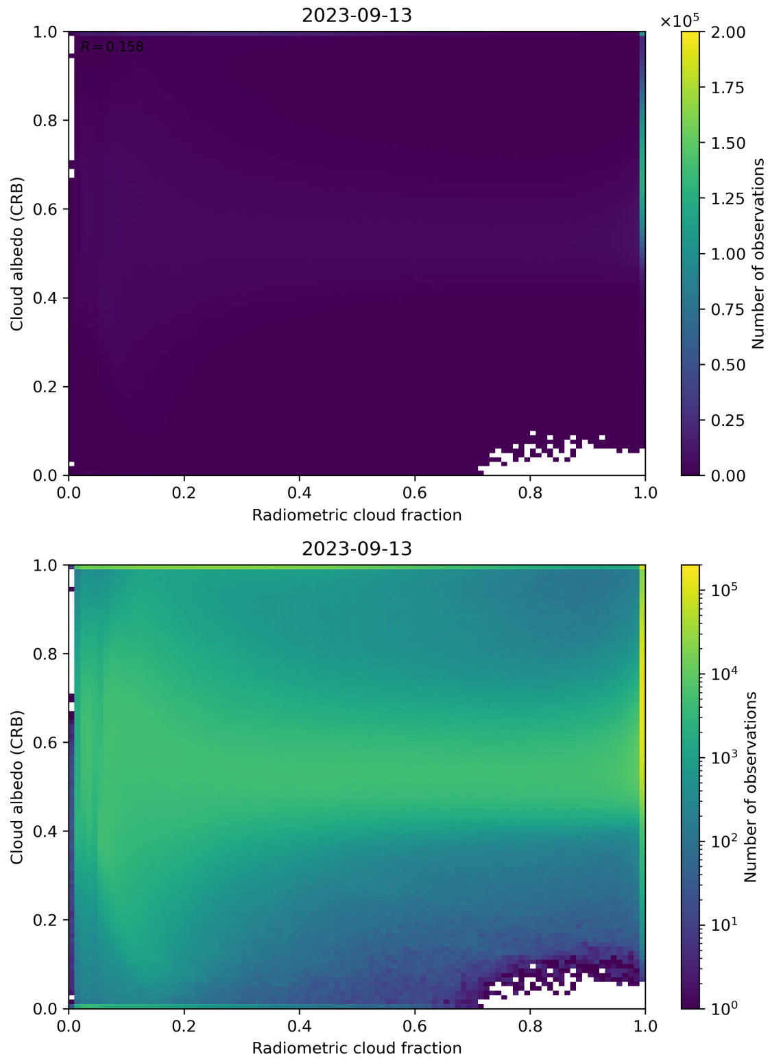
Figure 71: Scatter density plot of “Radiometric cloud fraction” against “Cloud albedo (CRB)” for 2023-09-12 to 2023-09-14.
