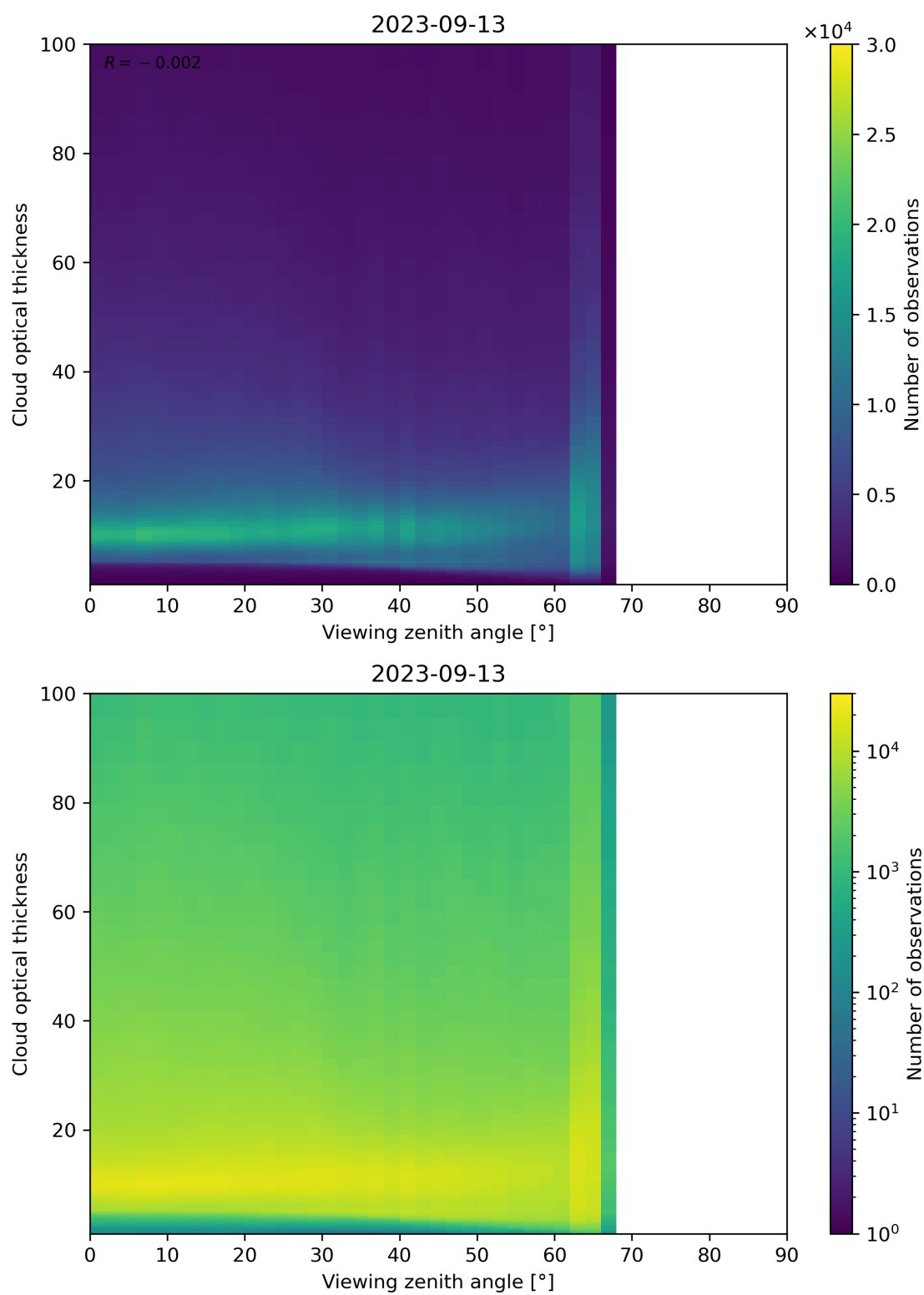
Figure 111: Scatter density plot of “Viewing zenith angle” against “Cloud optical thickness” for 2023-09-12 to 2023-09-14.
