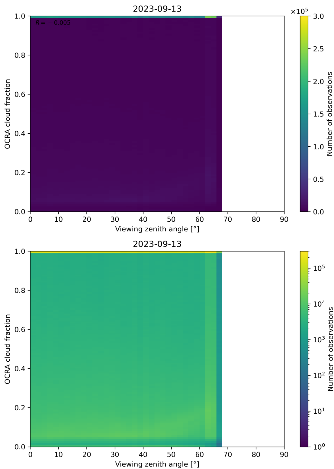
Figure 108: Scatter density plot of “Viewing zenith angle” against “OCRA cloud fraction” for 2023-09-12 to 2023-09-14.
