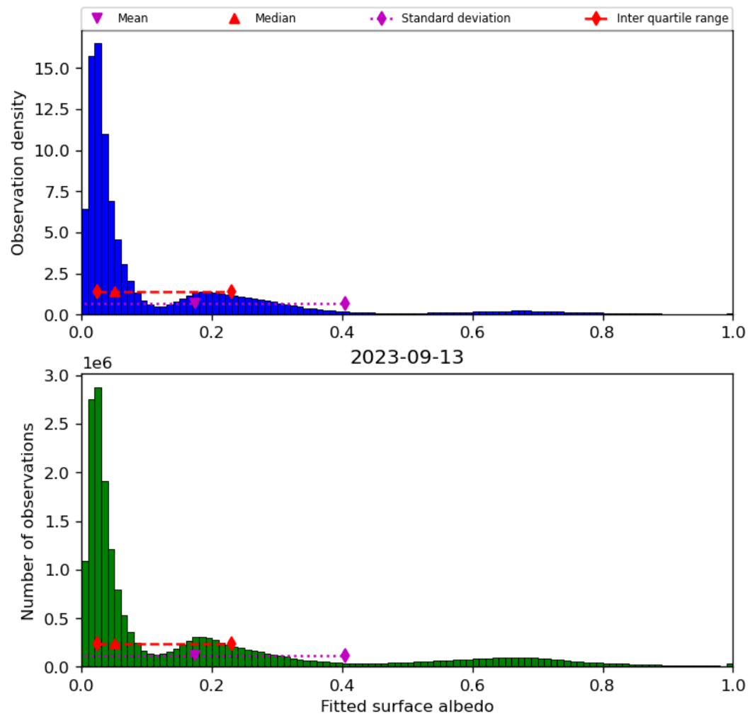
Figure 45: Histogram of “Fitted surface albedo” for 2023-09-12 to 2023-09-14
