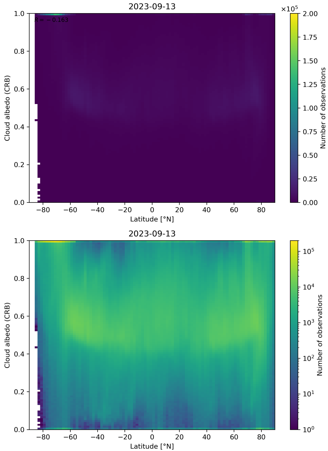
Figure 91: Scatter density plot of “Latitude” against “Cloud albedo (CRB)” for 2023-09-12 to 2023-09-14.
