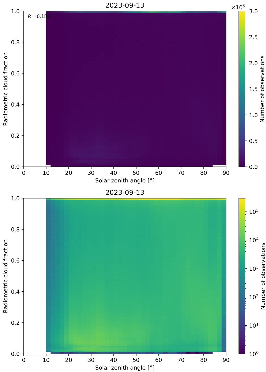
Figure 99: Scatter density plot of “Solar zenith angle” against “Radiometric cloud fraction” for 2023-09-12 to 2023-09-14.
