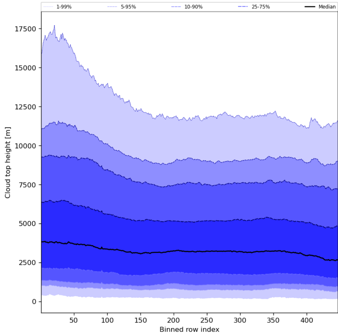
Figure 56: Along track statistics of “Cloud top height” for 2023-09-12 to 2023-09-14
