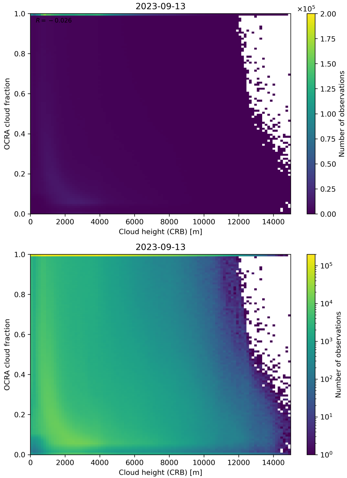
Figure 81: Scatter density plot of “Cloud height (CRB)” against “OCRA cloud fraction” for 2023-09-12 to 2023-09-14.
