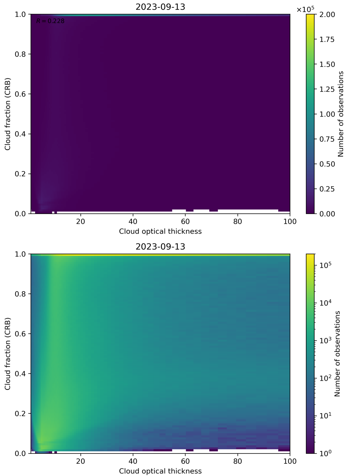
Figure 84: Scatter density plot of “Cloud optical thickness” against “Cloud fraction (CRB)” for 2023-09-12 to 2023-09-14.
