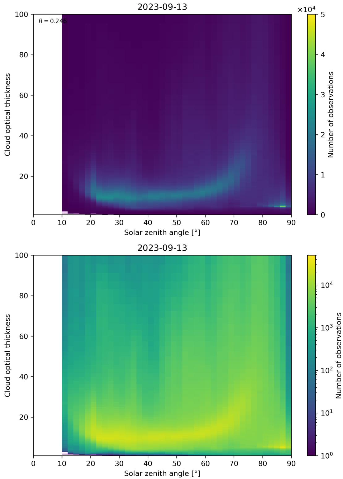
Figure 103: Scatter density plot of “Solar zenith angle” against “Cloud optical thickness” for 2023-09-12 to 2023-09-14.
