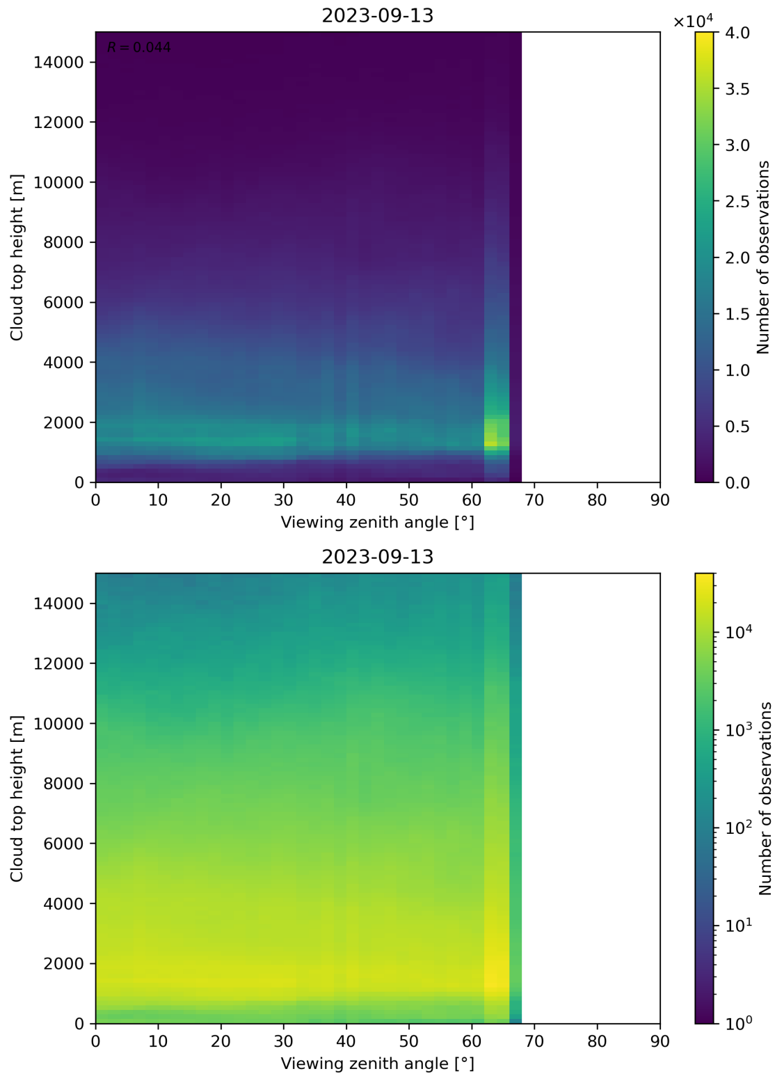
Figure 112: Scatter density plot of “Viewing zenith angle” against “Cloud top height” for 2023-09-12 to 2023-09-14.
