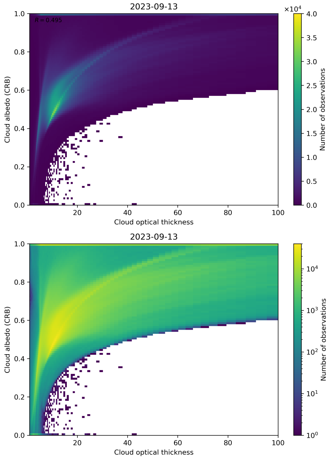
Figure 82: Scatter density plot of “Cloud optical thickness” against “Cloud albedo (CRB)” for 2023-09-12 to 2023-09-14.
