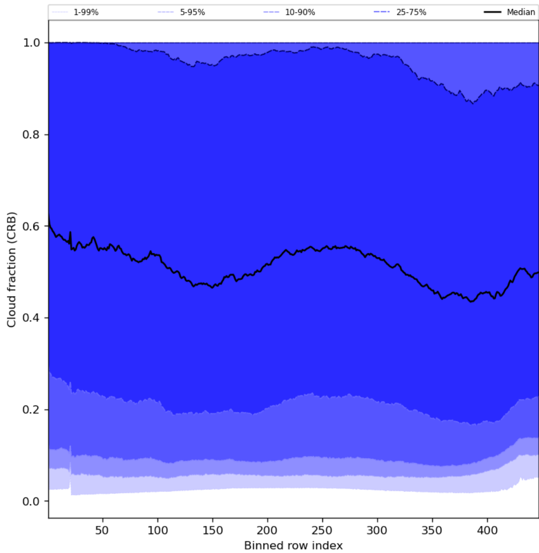
Figure 58: Along track statistics of “Cloud fraction (CRB)” for 2023-09-12 to 2023-09-14
