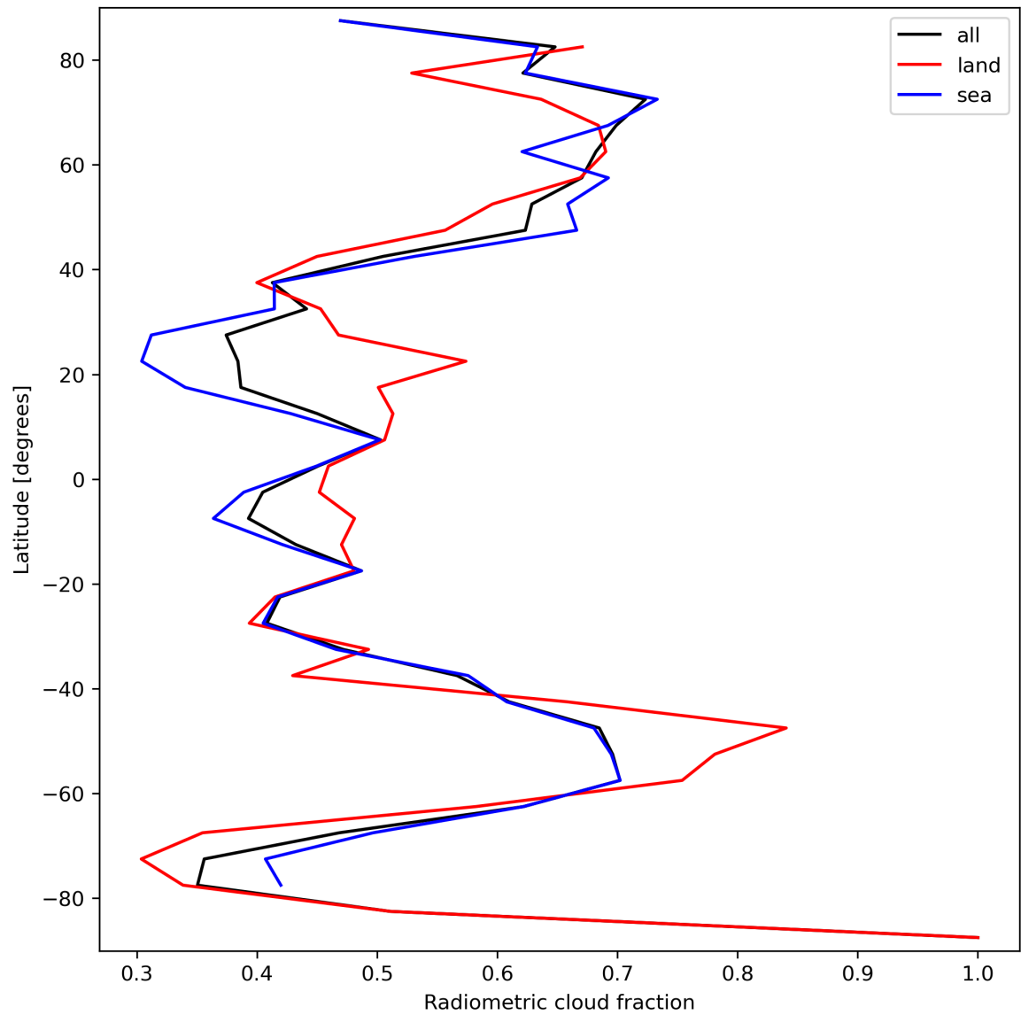
Figure 23: Zonal average of “Radiometric cloud fraction” for 2023-09-12 to 2023-09-14.
