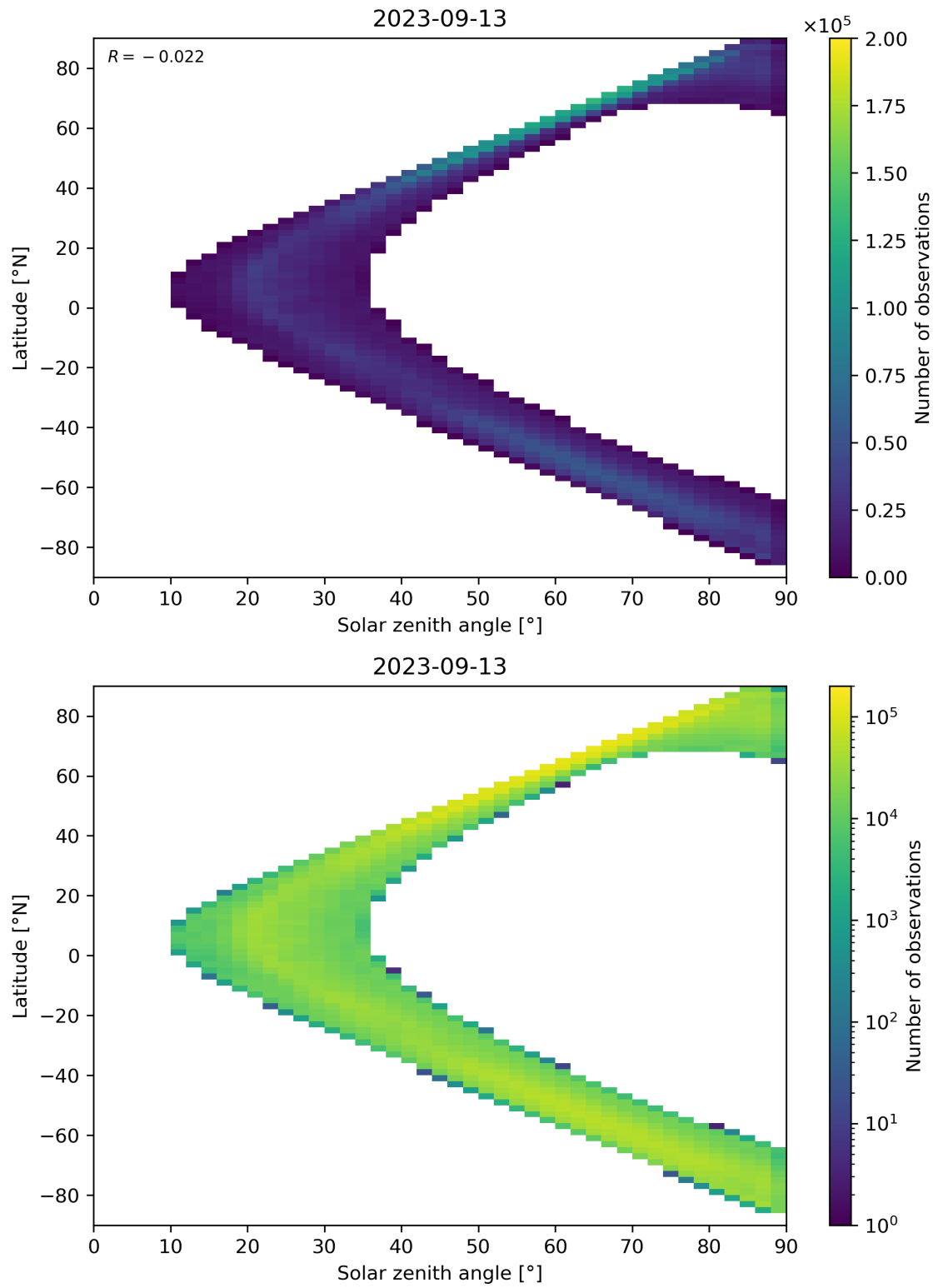
Figure 105: Scatter density plot of “Solar zenith angle” against “Latitude” for 2023-09-12 to 2023-09-14.
