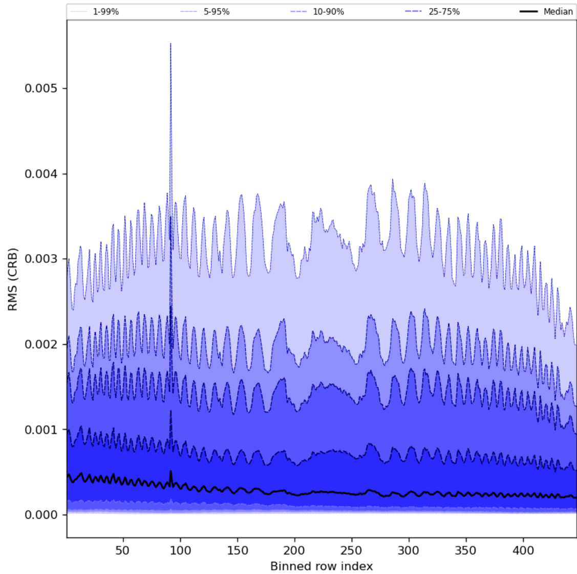
Figure 64: Along track statistics of “RMS (CRB)” for 2023-09-12 to 2023-09-14
