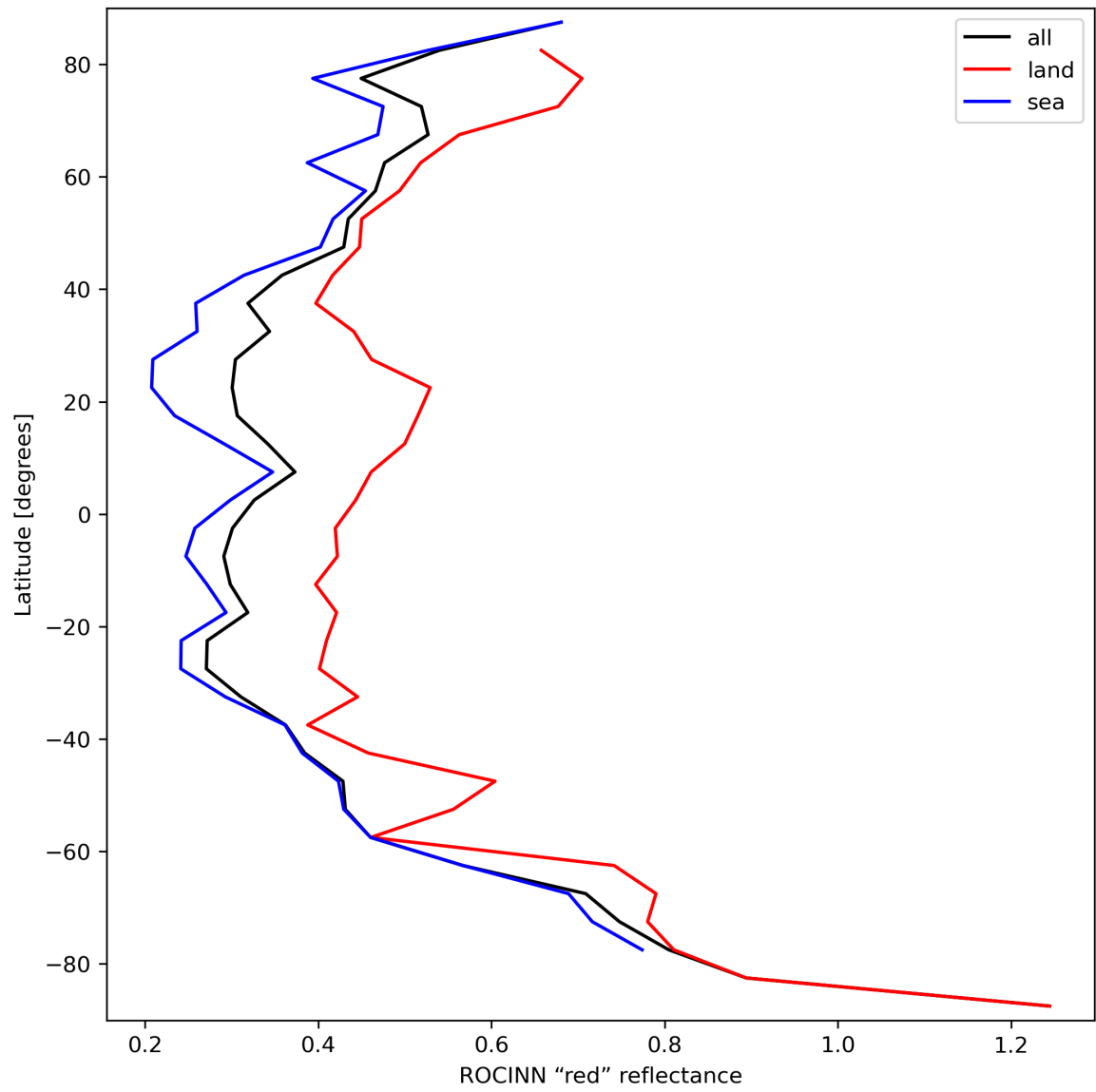
Figure 37: Zonal average of “ROCINN “red” reflectance” for 2023-09-12 to 2023-09-14.
