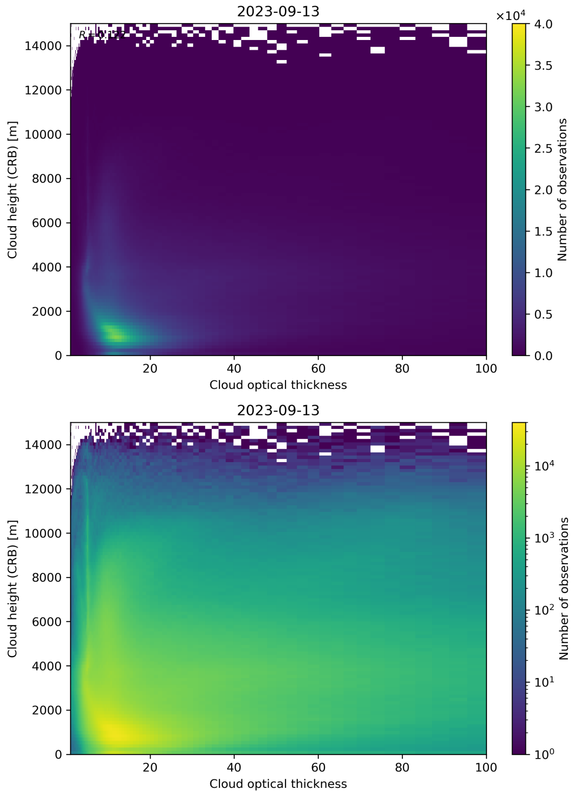
Figure 85: Scatter density plot of “Cloud optical thickness” against “Cloud height (CRB)” for 2023-09-12 to 2023-09-14.
