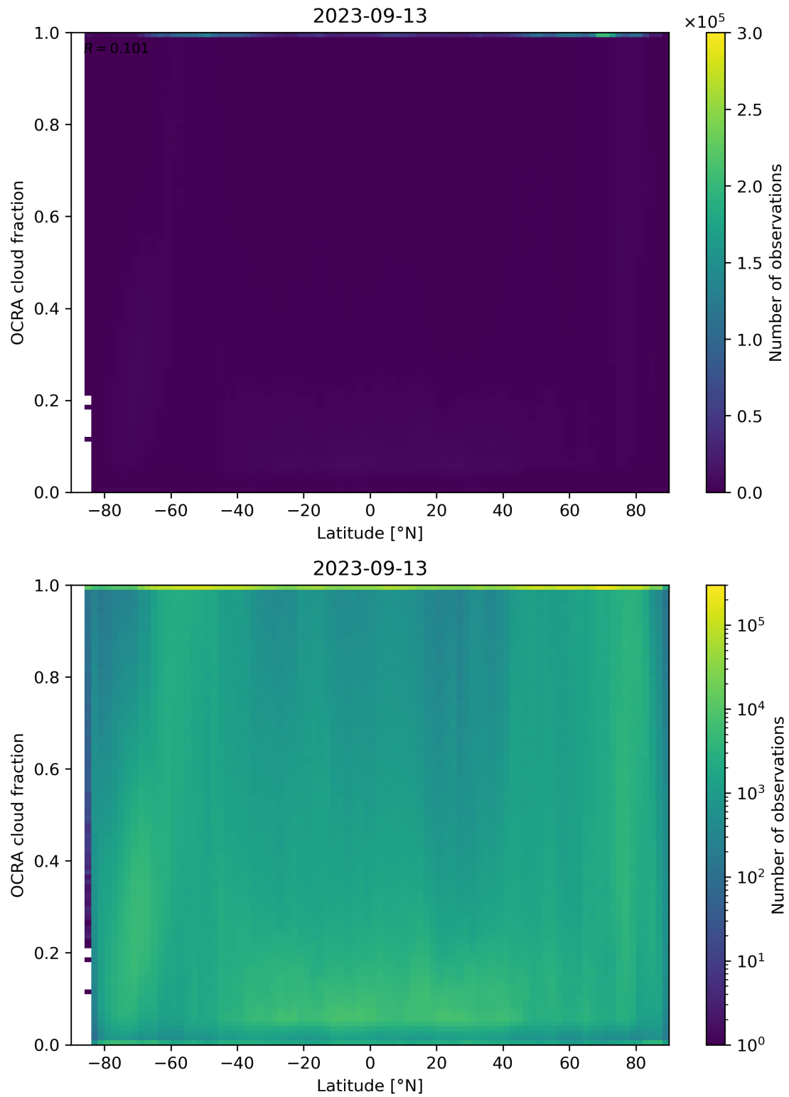
Figure 93: Scatter density plot of “Latitude” against “OCRA cloud fraction” for 2023-09-12 to 2023-09-14.
