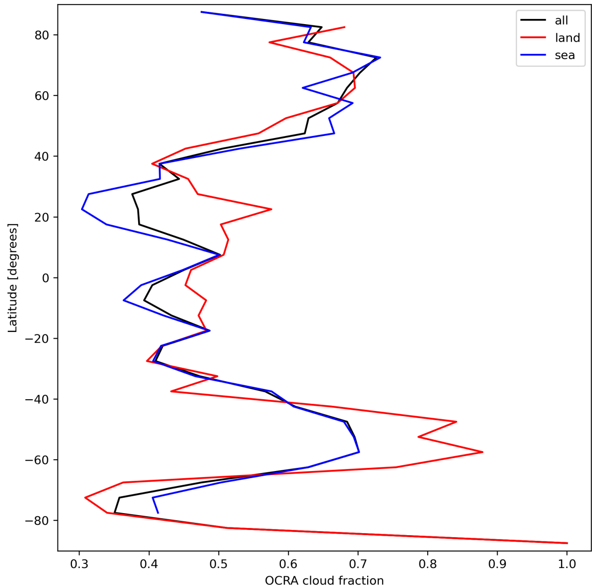
Figure 34: Zonal average of “OCRA cloud fraction” for 2023-09-12 to 2023-09-14.
