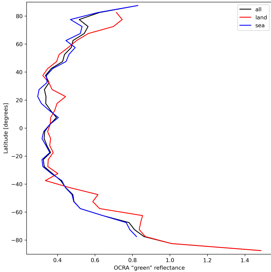
Figure 36: Zonal average of “OCRA “green” reflectance” for 2023-09-12 to 2023-09-14.
