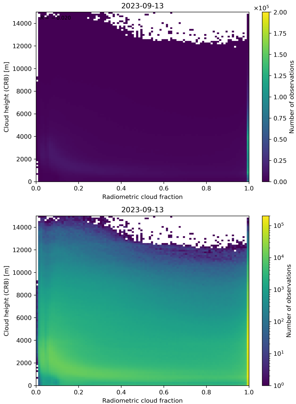
Figure 74: Scatter density plot of “Radiometric cloud fraction” against “Cloud height (CRB)” for 2023-09-12 to 2023-09-14.
