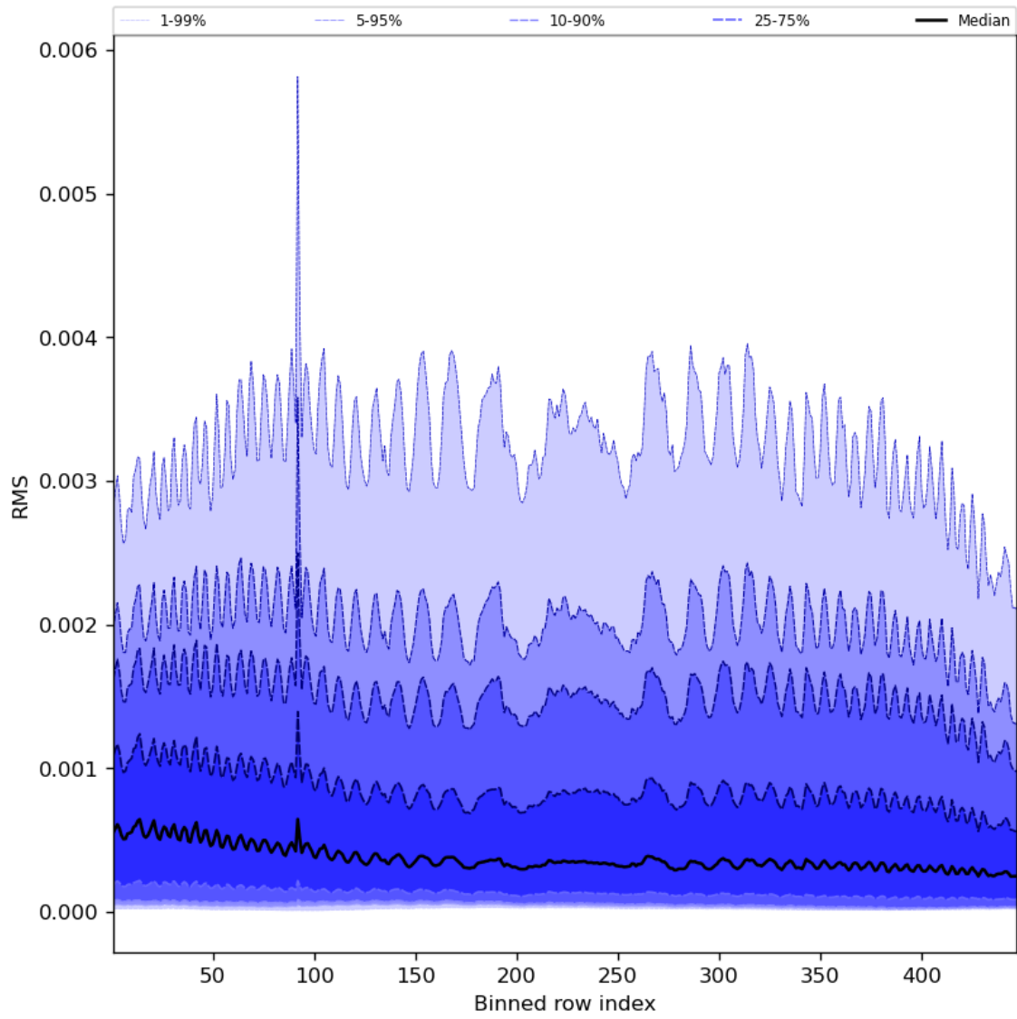
Figure 63: Along track statistics of “RMS” for 2023-09-12 to 2023-09-14
