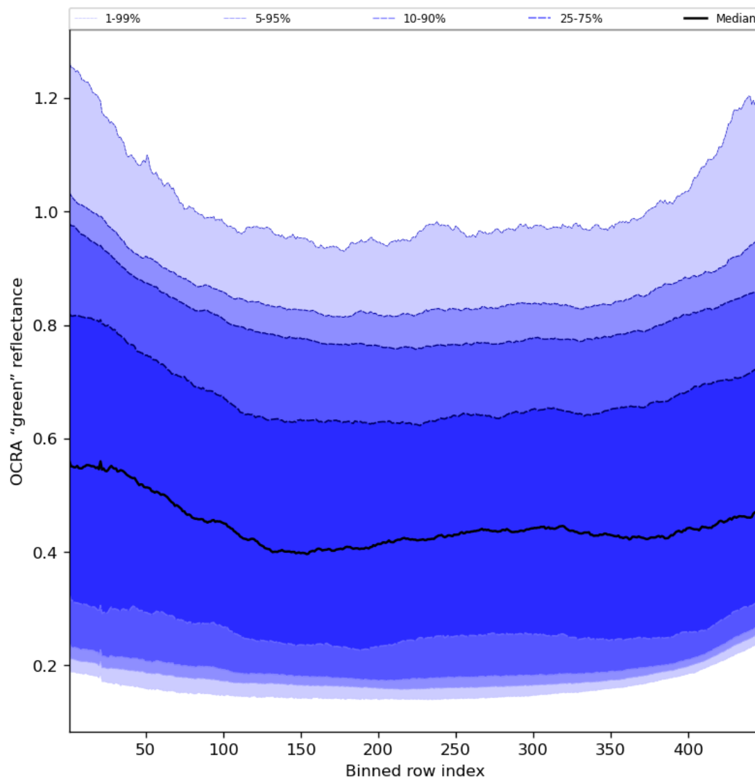
Figure 68: Along track statistics of “OCRA “green” reflectance” for 2023-09-12 to 2023-09-14
