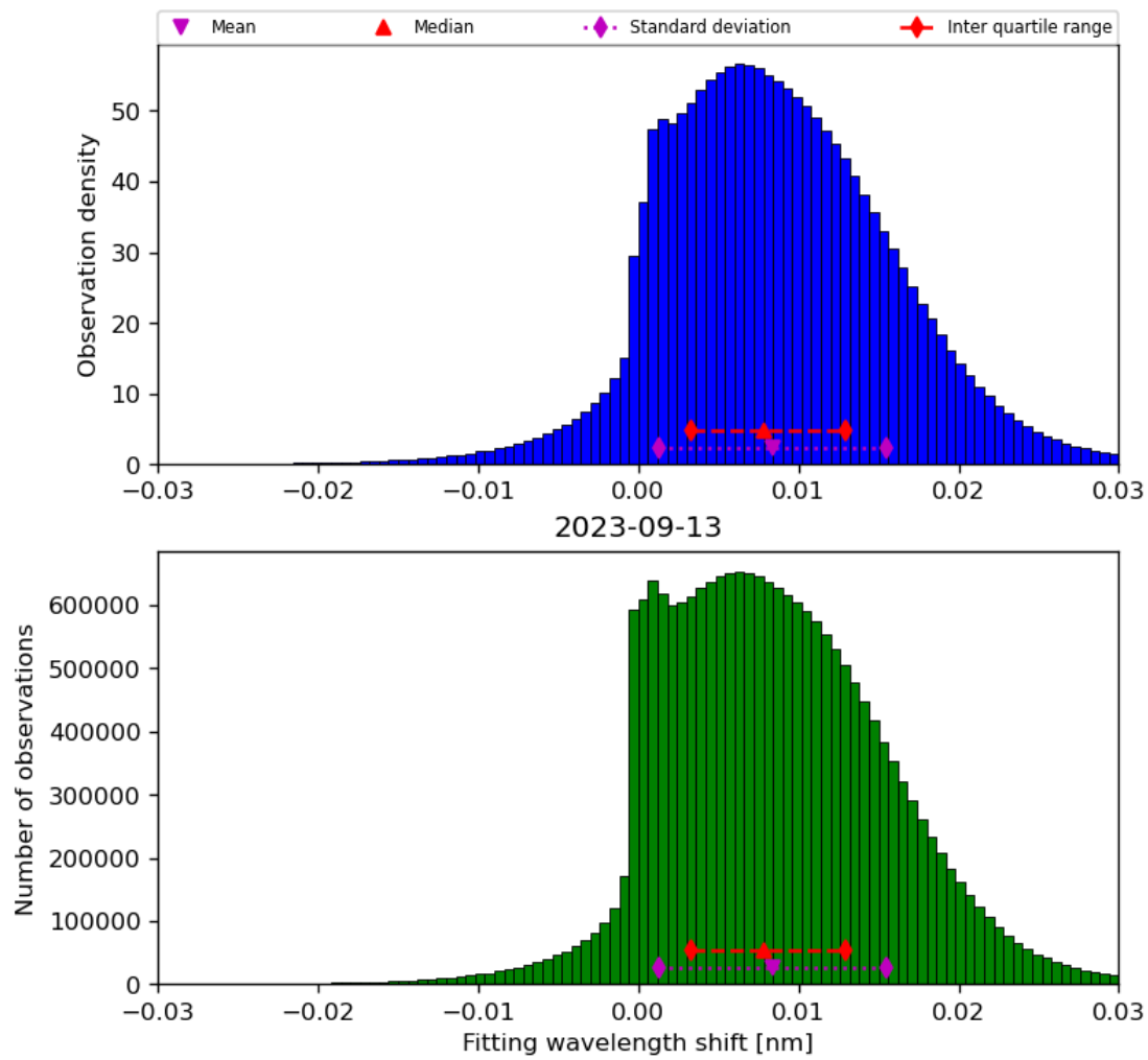
Figure 49: Histogram of “Fitting wavelength shift” for 2023-09-12 to 2023-09-14
