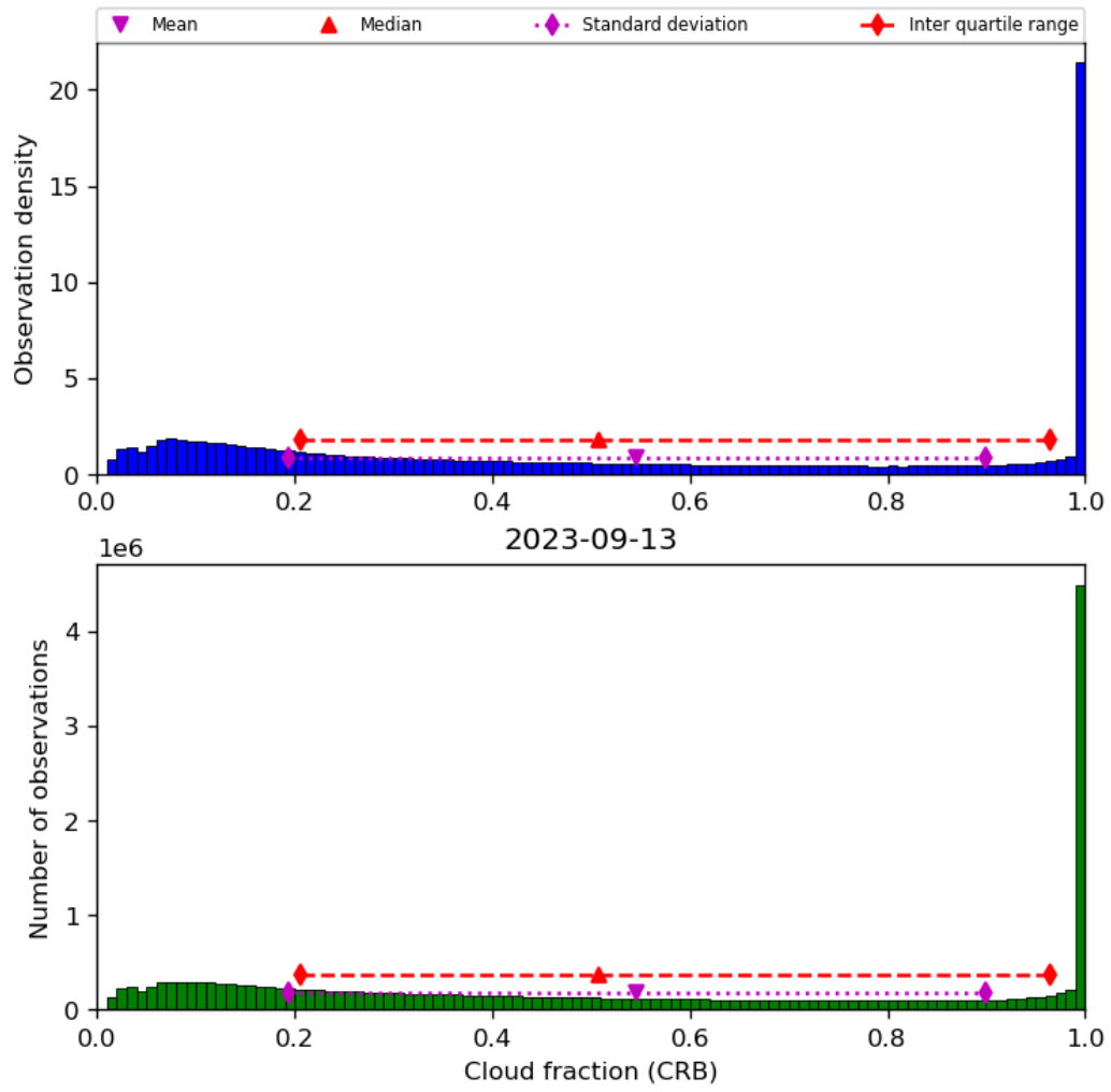
Figure 42: Histogram of “Cloud fraction (CRB)” for 2023-09-12 to 2023-09-14
