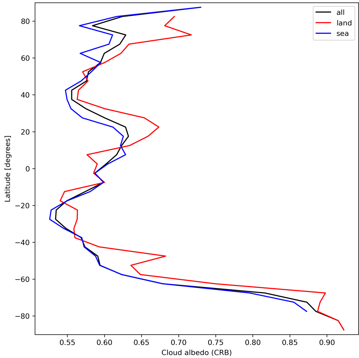
Figure 28: Zonal average of “Cloud albedo (CRB)” for 2023-09-12 to 2023-09-14.
