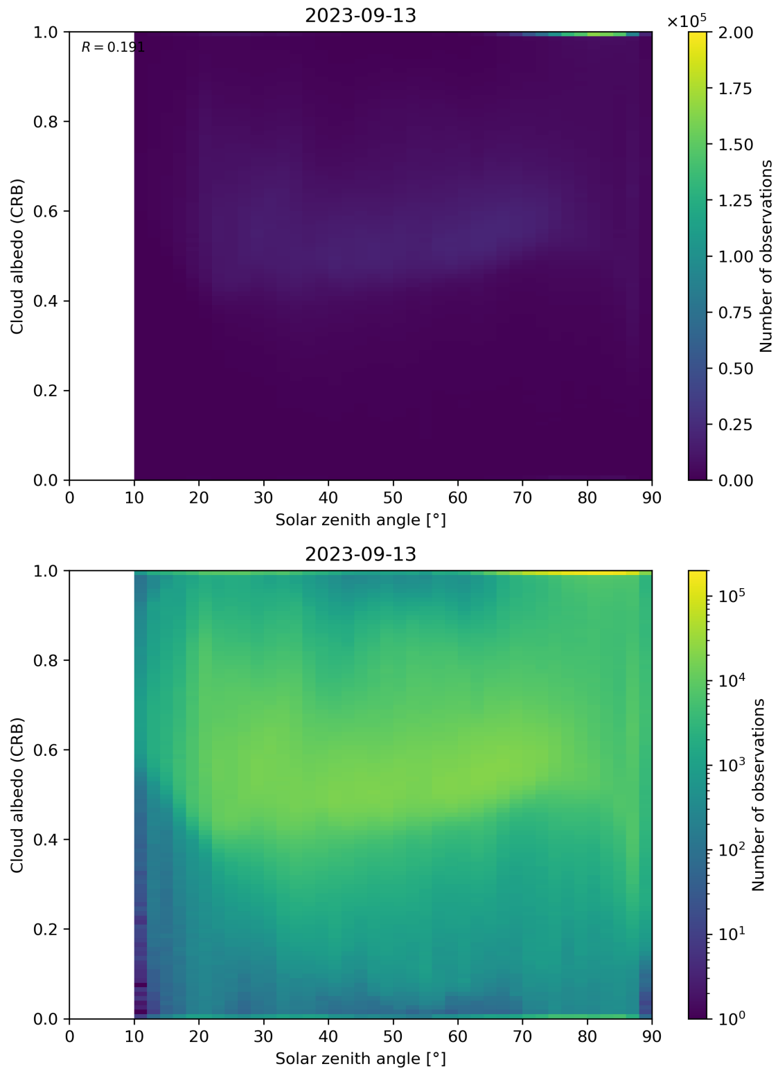
Figure 98: Scatter density plot of “Solar zenith angle” against “Cloud albedo (CRB)” for 2023-09-12 to 2023-09-14.
