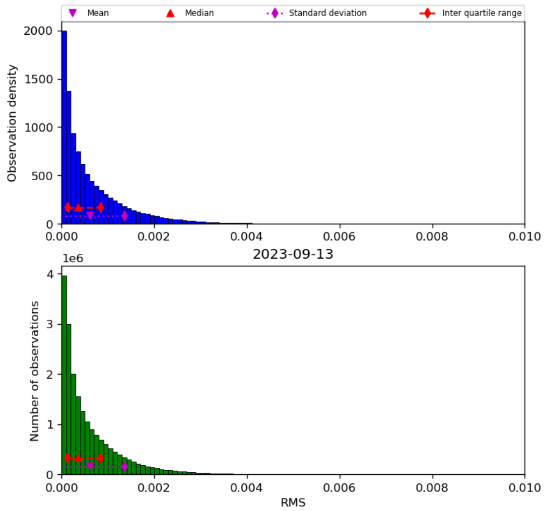
Figure 47: Histogram of “RMS” for 2023-09-12 to 2023-09-14
