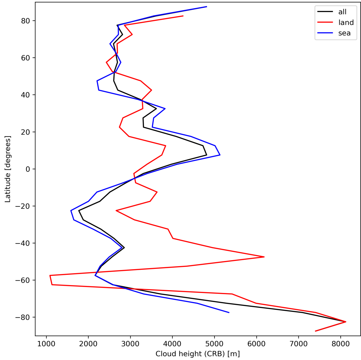
Figure 27: Zonal average of “Cloud height (CRB)” for 2023-09-12 to 2023-09-14.
