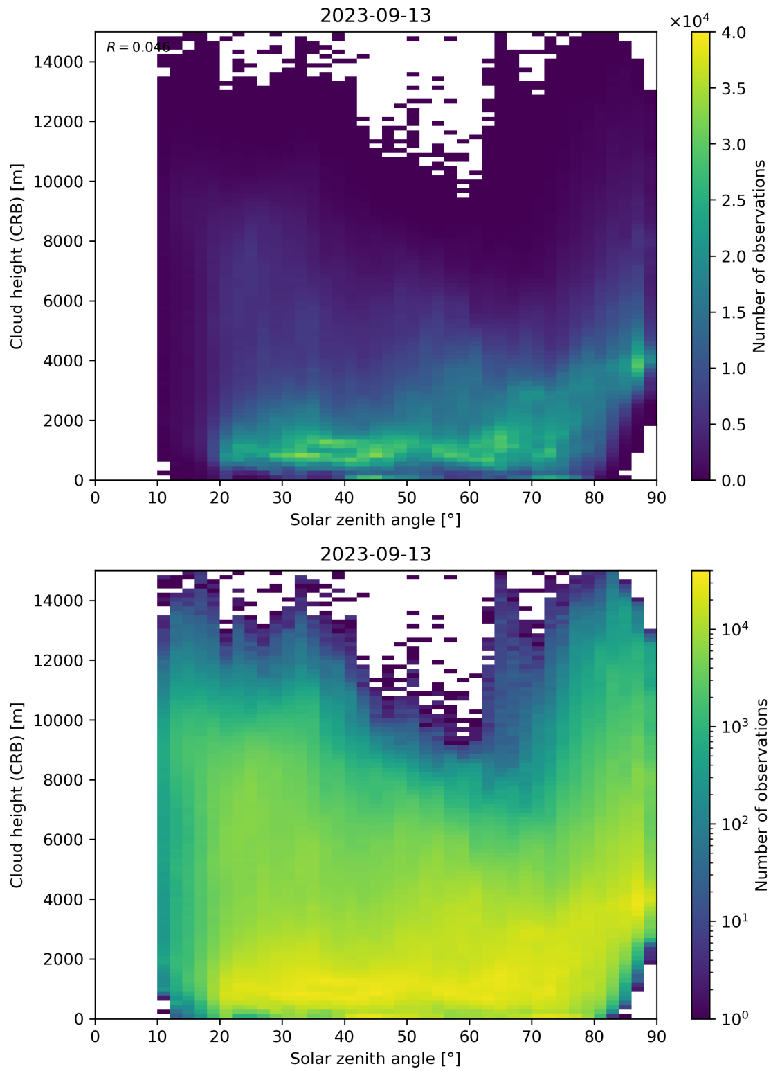
Figure 102: Scatter density plot of “Solar zenith angle” against “Cloud height (CRB)” for 2023-09-12 to 2023-09-14.
