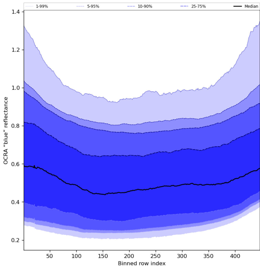
Figure 67: Along track statistics of “OCRA “blue” reflectance” for 2023-09-12 to 2023-09-14
