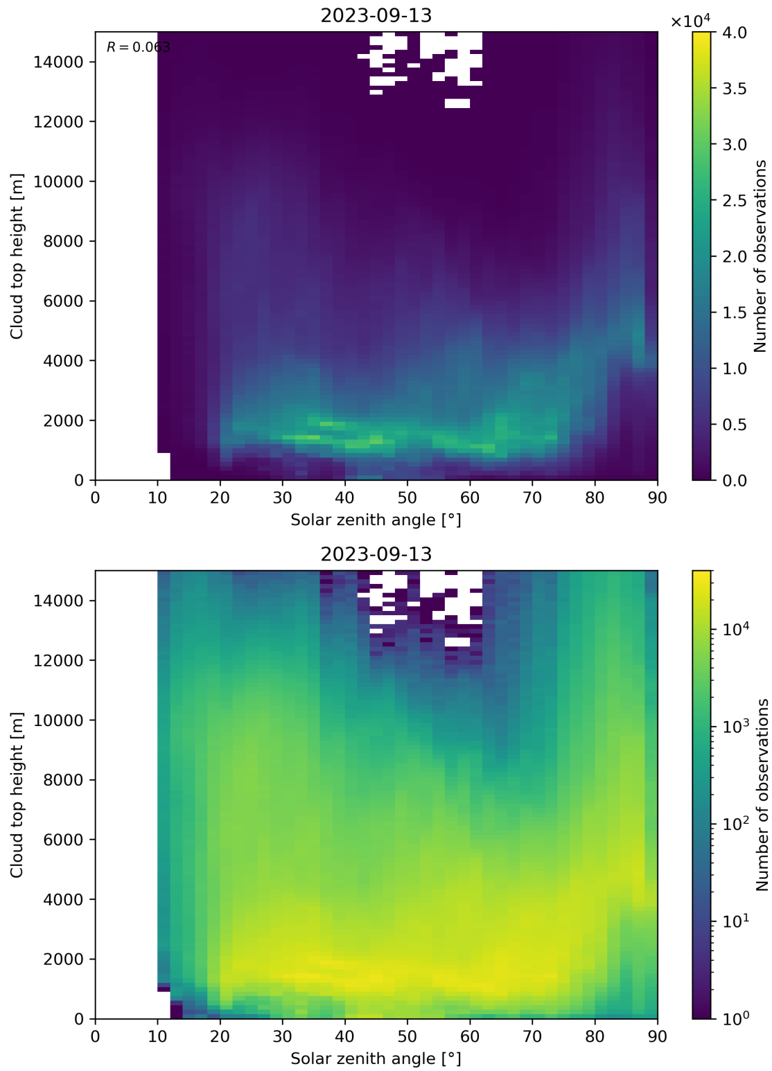
Figure 104: Scatter density plot of “Solar zenith angle” against “Cloud top height” for 2023-09-12 to 2023-09-14.
