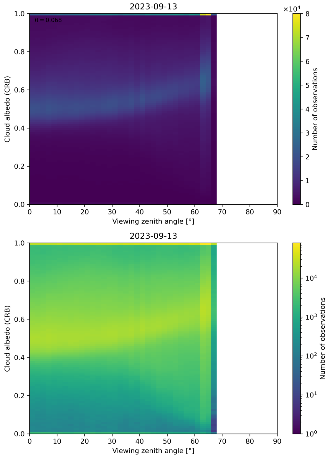
Figure 106: Scatter density plot of “Viewing zenith angle” against “Cloud albedo (CRB)” for 2023-09-12 to 2023-09-14.
