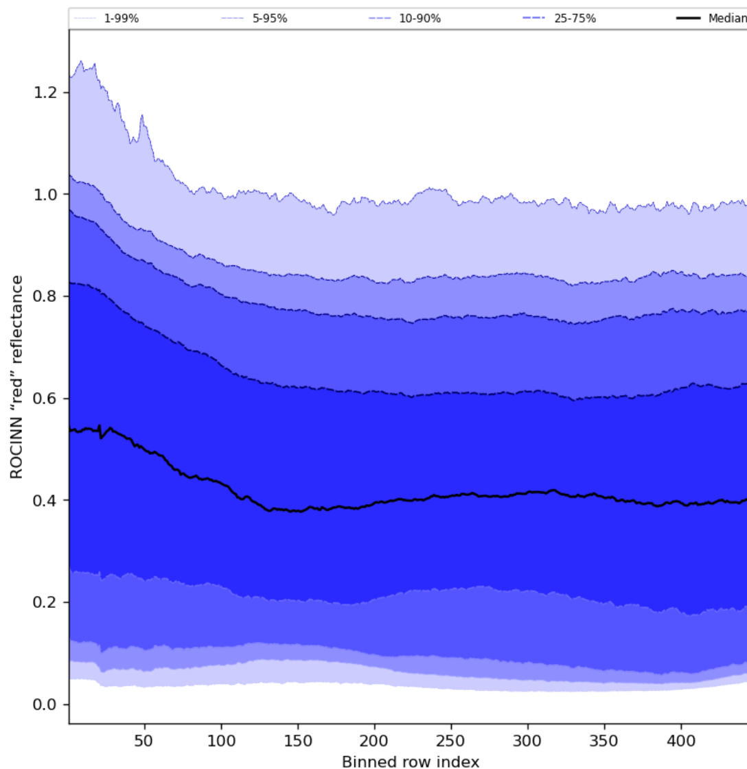
Figure 69: Along track statistics of “ROCINN “red” reflectance” for 2023-09-12 to 2023-09-14
