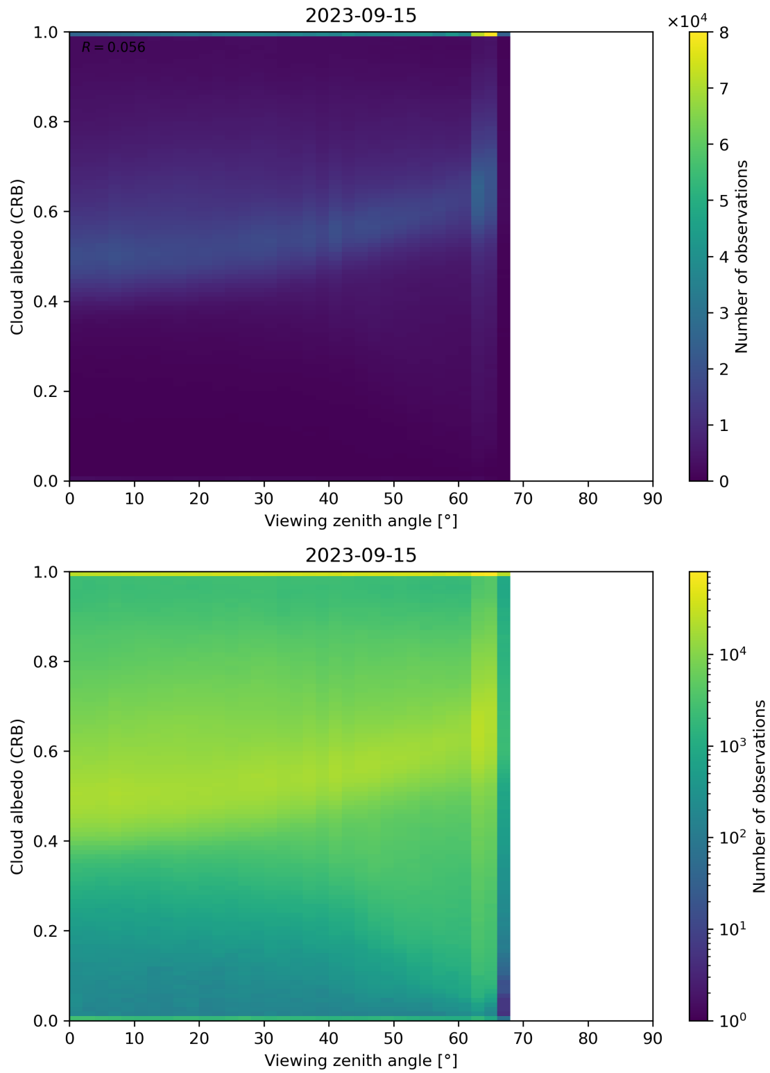
Figure 106: Scatter density plot of “Viewing zenith angle” against “Cloud albedo (CRB)” for 2023-09-15 to 2023-09-16.
