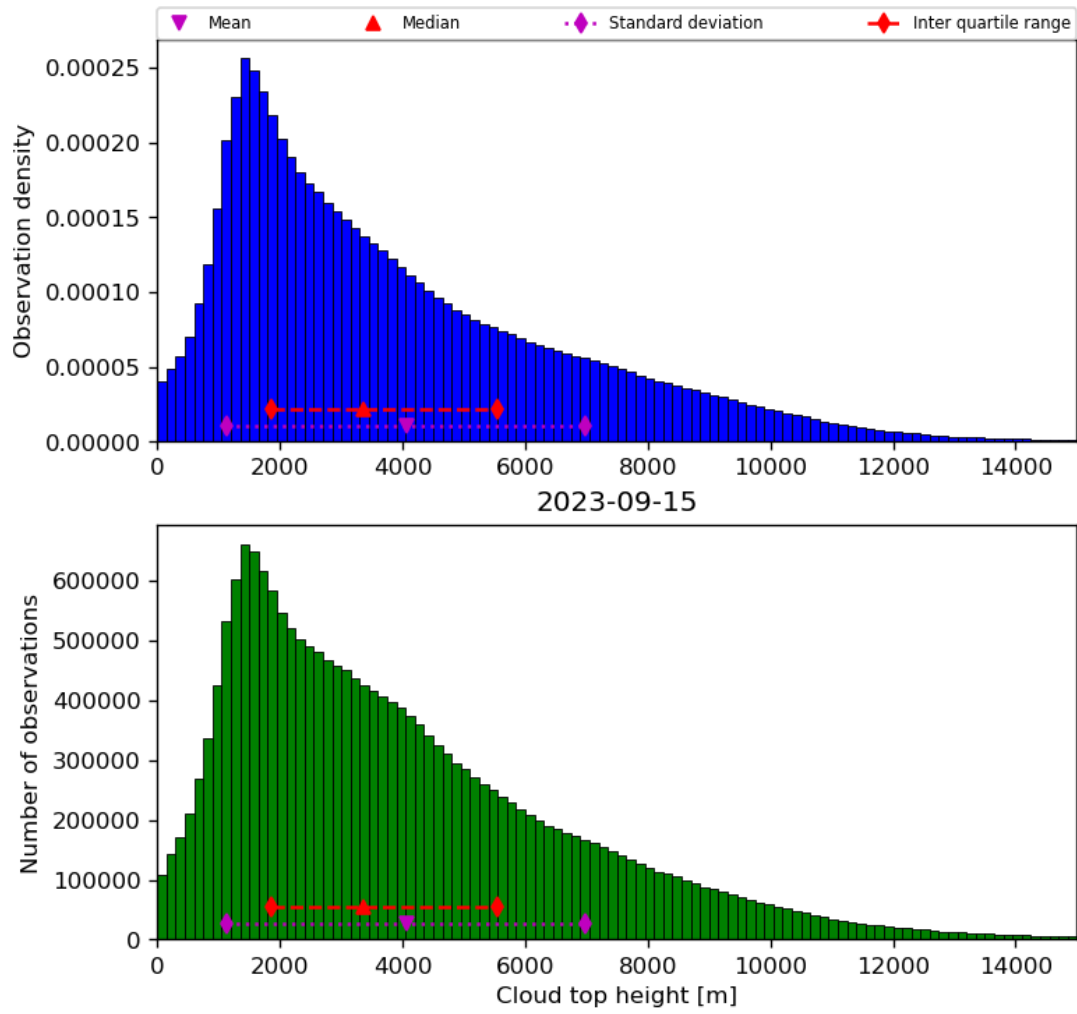
Figure 40: Histogram of “Cloud top height” for 2023-09-15 to 2023-09-16
