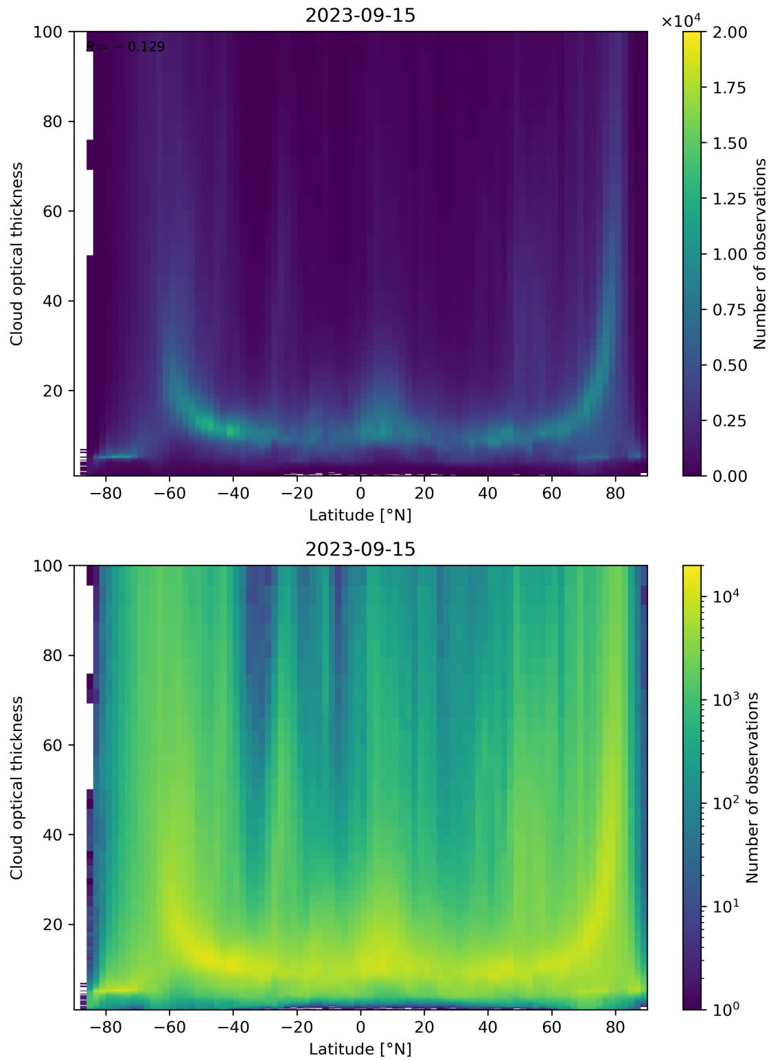
Figure 96: Scatter density plot of “Latitude” against “Cloud optical thickness” for 2023-09-15 to 2023-09-16.
