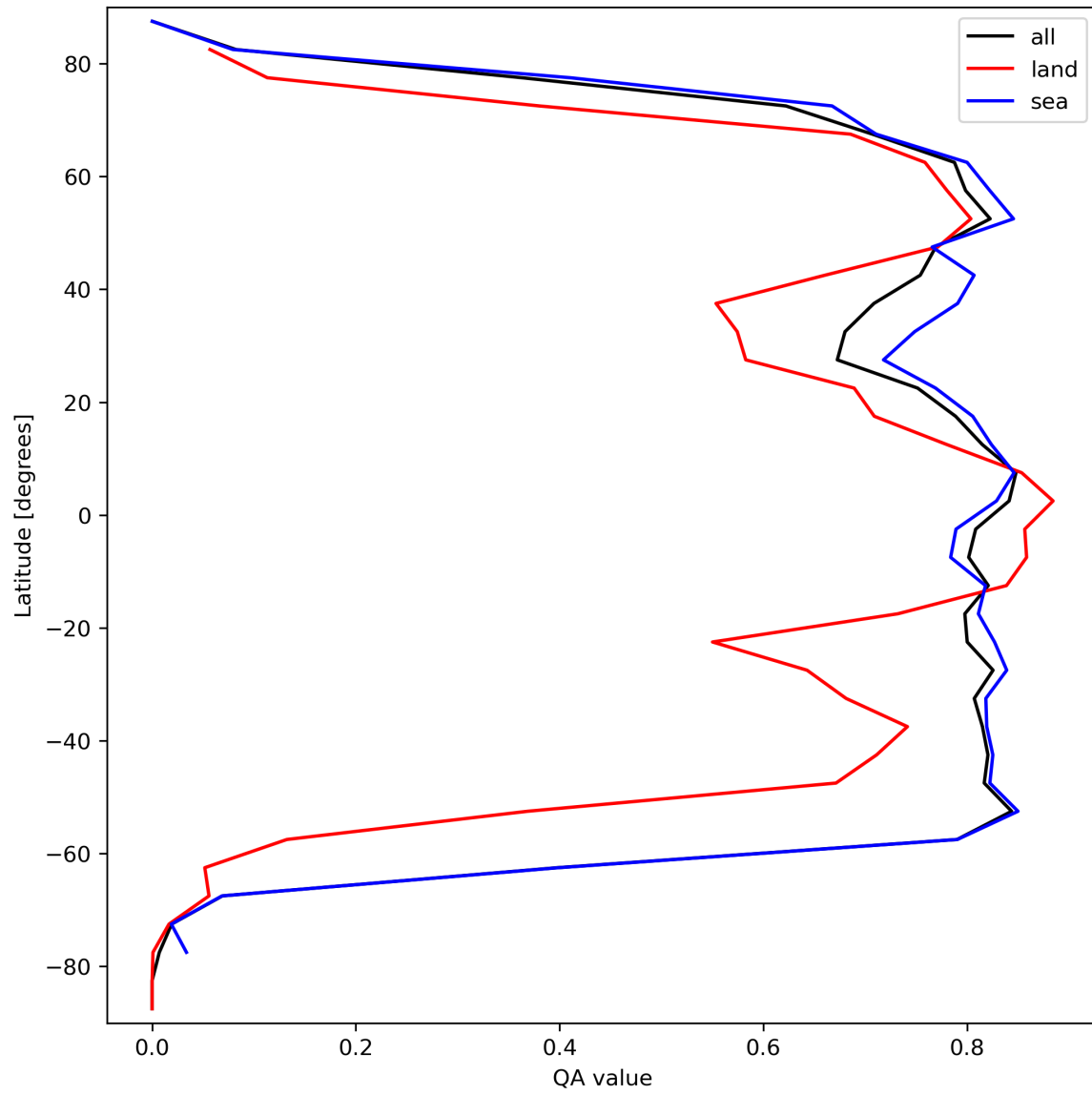
Figure 22: Zonal average of “QA value” for 2023-09-15 to 2023-09-16.
