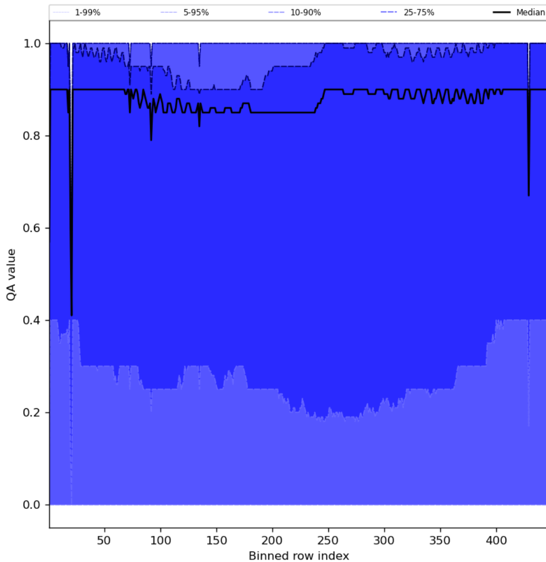
Figure 54: Along track statistics of “QA value” for 2023-09-15 to 2023-09-16
