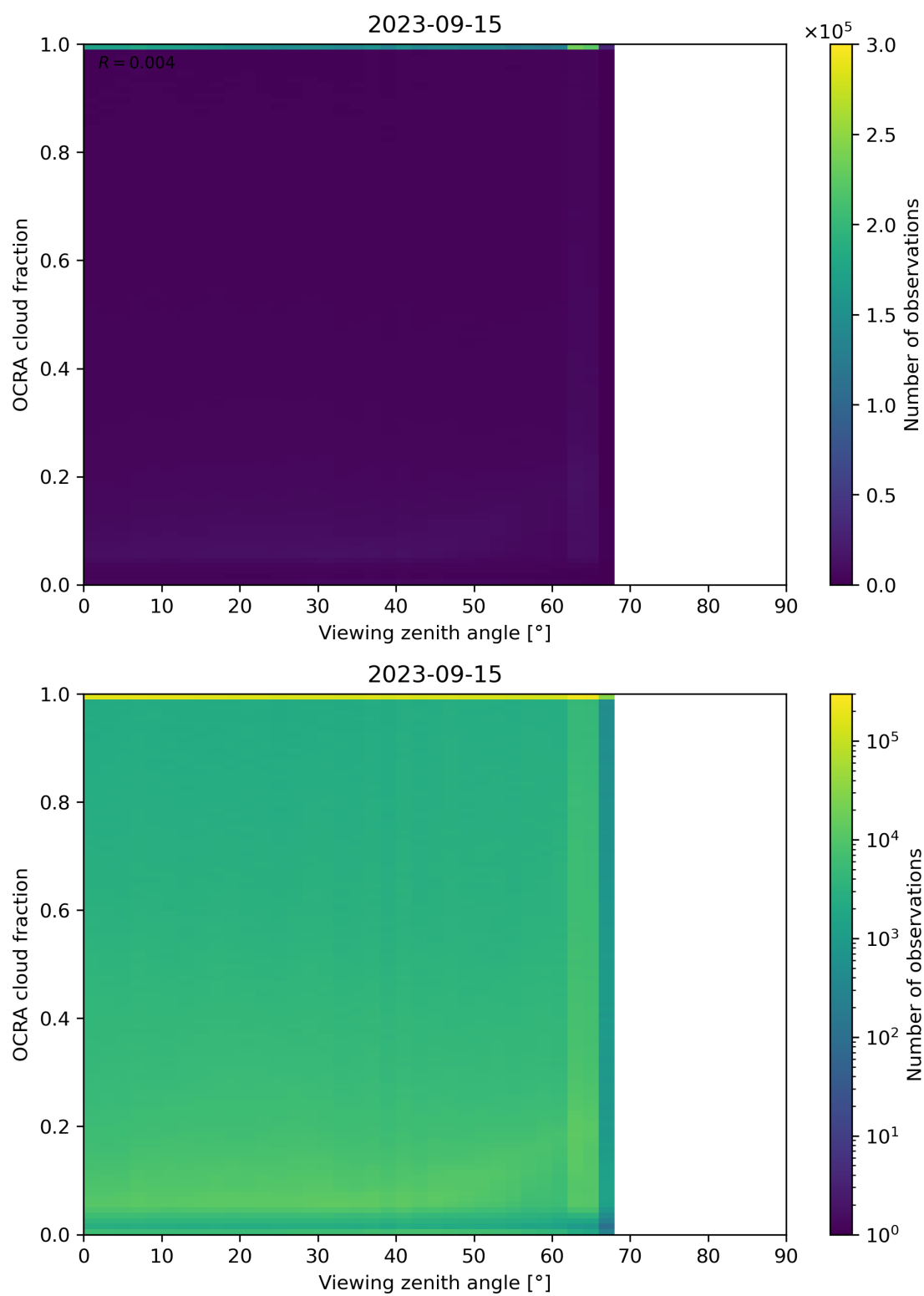
Figure 108: Scatter density plot of “Viewing zenith angle” against “OCRA cloud fraction” for 2023-09-15 to 2023-09-16.
