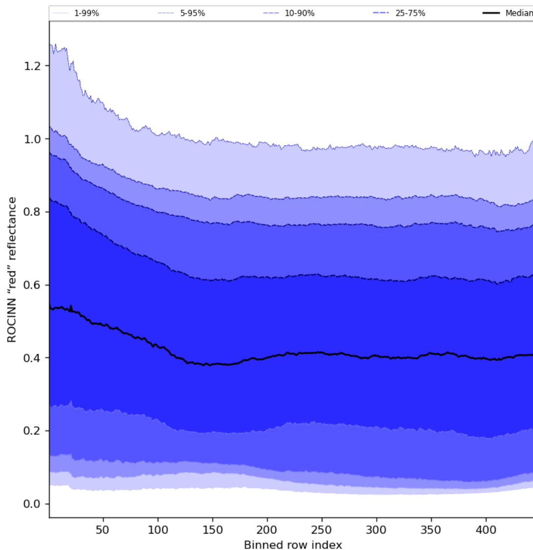
Figure 69: Along track statistics of “ROCINN “red” reflectance” for 2023-09-15 to 2023-09-16
