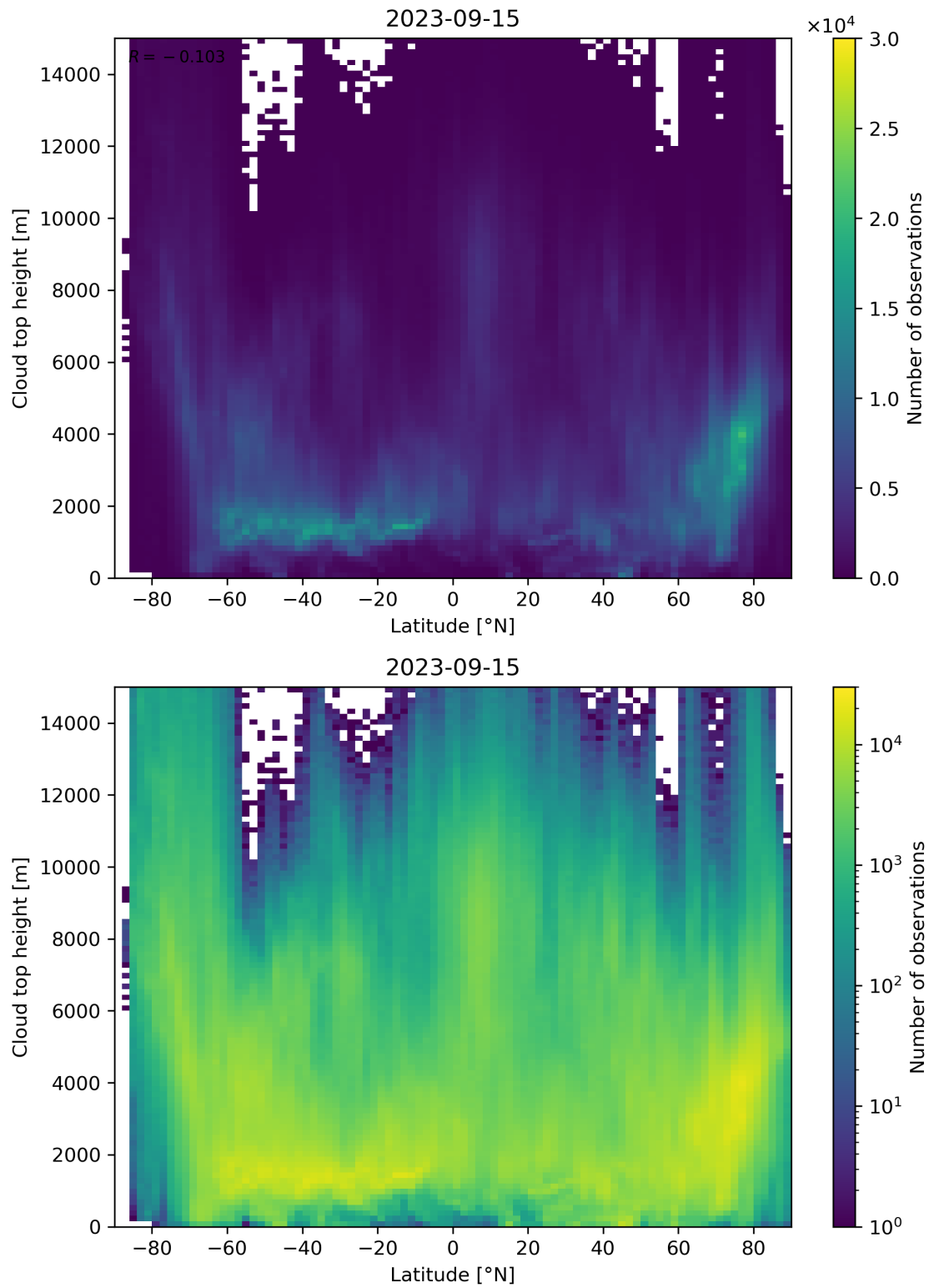
Figure 97: Scatter density plot of “Latitude” against “Cloud top height” for 2023-09-15 to 2023-09-16.
