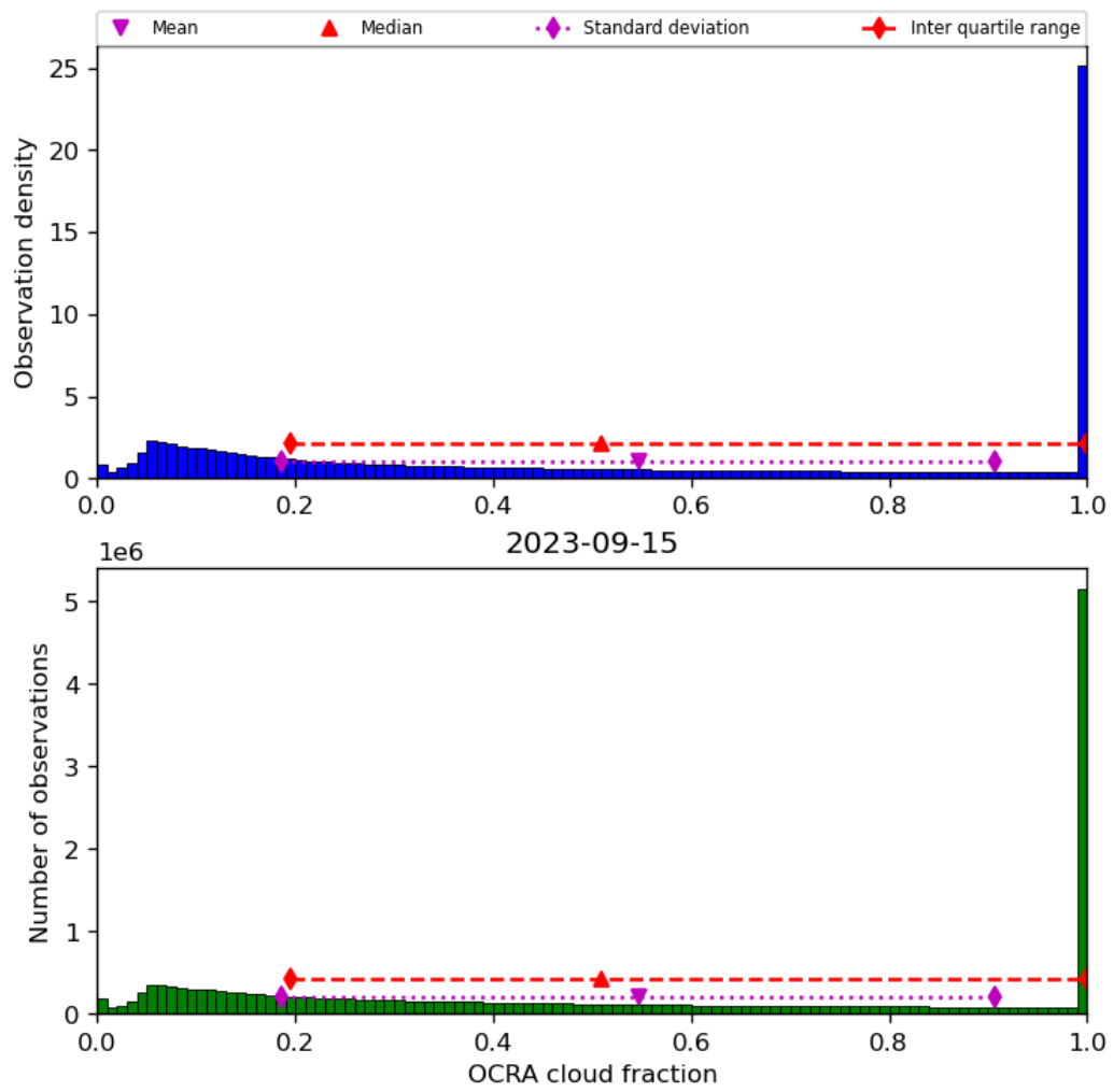
Figure 50: Histogram of “OCRA cloud fraction” for 2023-09-15 to 2023-09-16
