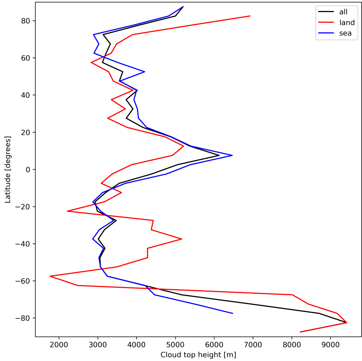
Figure 24: Zonal average of “Cloud top height” for 2023-09-15 to 2023-09-16.
