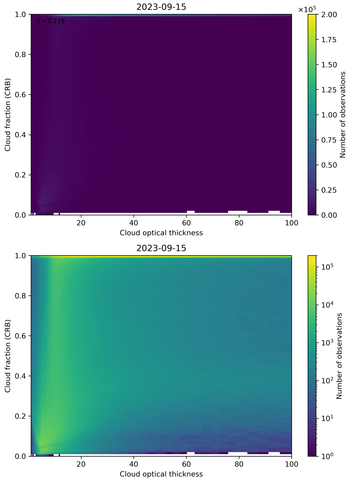
Figure 84: Scatter density plot of “Cloud optical thickness” against “Cloud fraction (CRB)” for 2023-09-15 to 2023-09-16.
