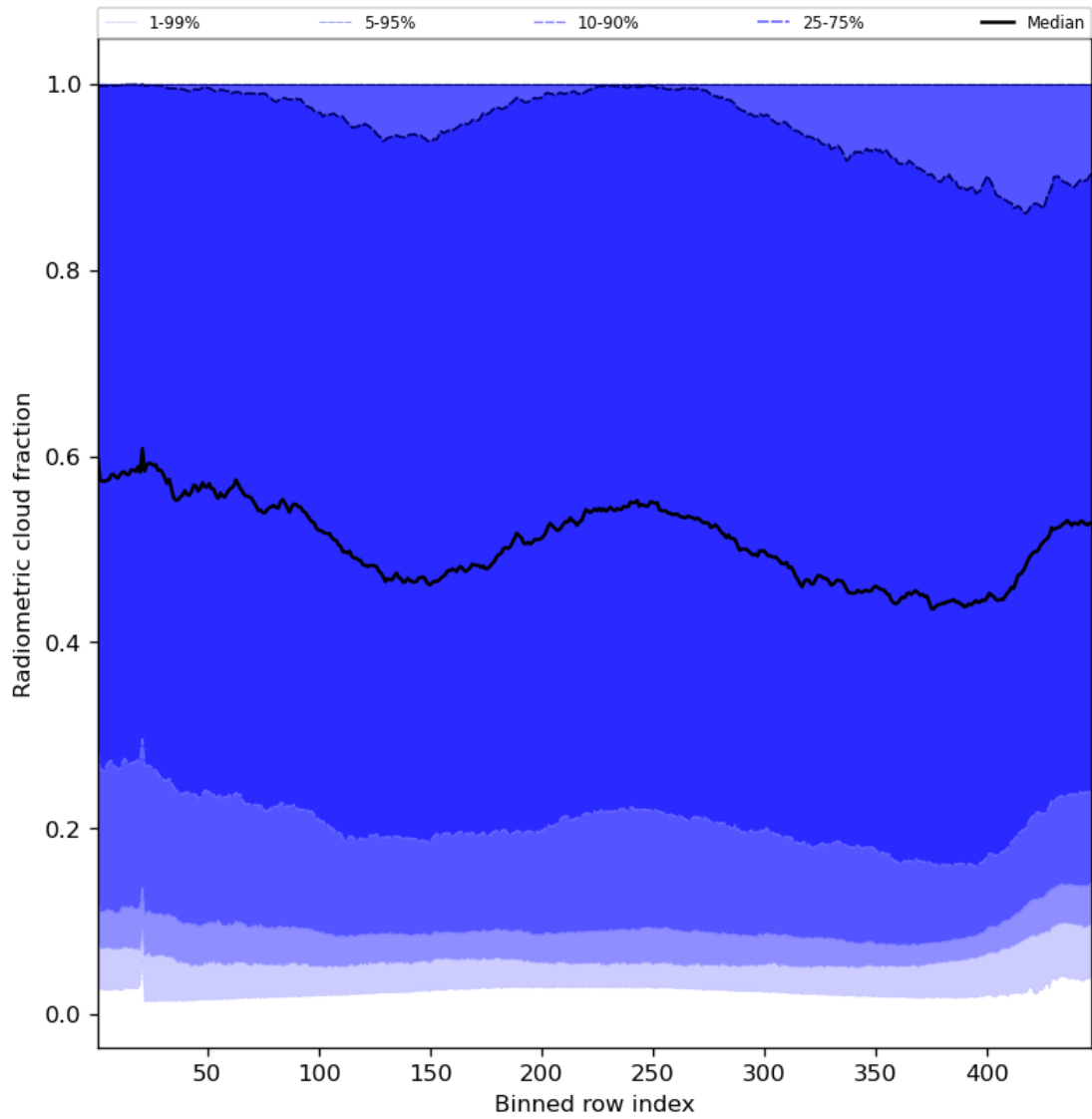
Figure 55: Along track statistics of “Radiometric cloud fraction” for 2023-09-15 to 2023-09-16
