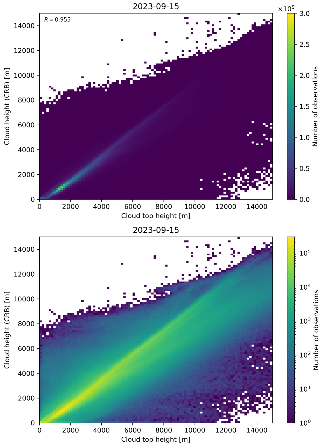
Figure 89: Scatter density plot of “Cloud top height” against “Cloud height (CRB)” for 2023-09-15 to 2023-09-16.
