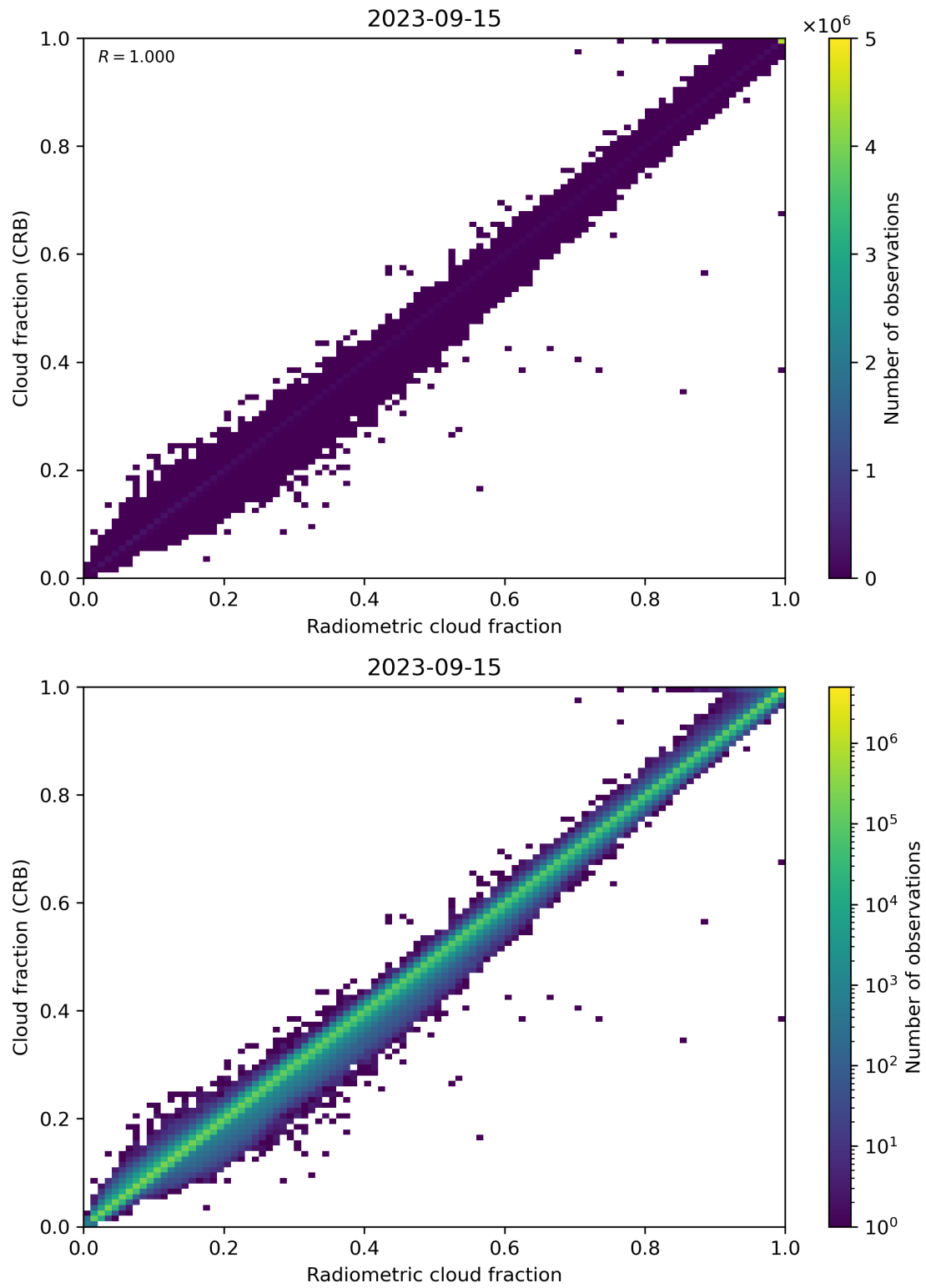
Figure 73: Scatter density plot of “Radiometric cloud fraction” against “Cloud fraction (CRB)” for 2023-09-15 to 2023-09-16.
