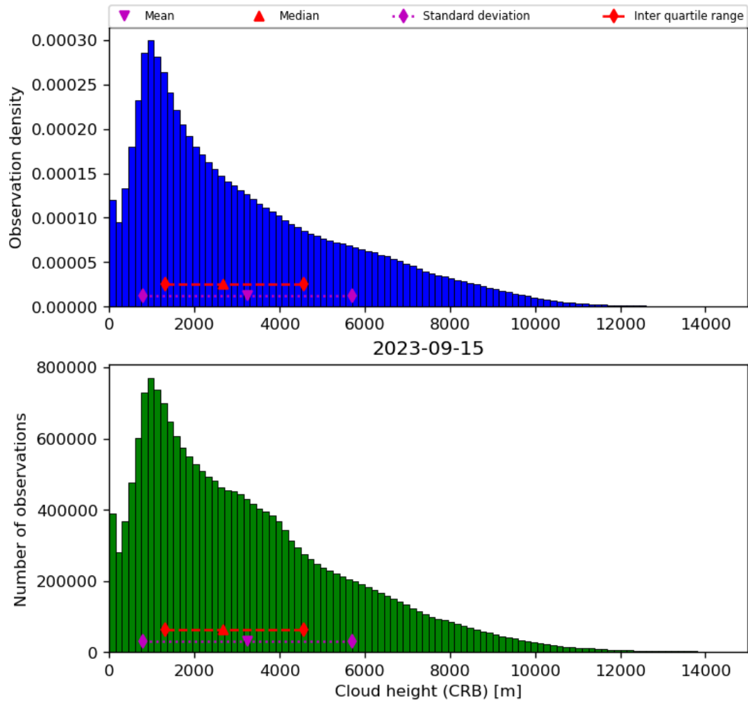
Figure 43: Histogram of “Cloud height (CRB)” for 2023-09-15 to 2023-09-16
