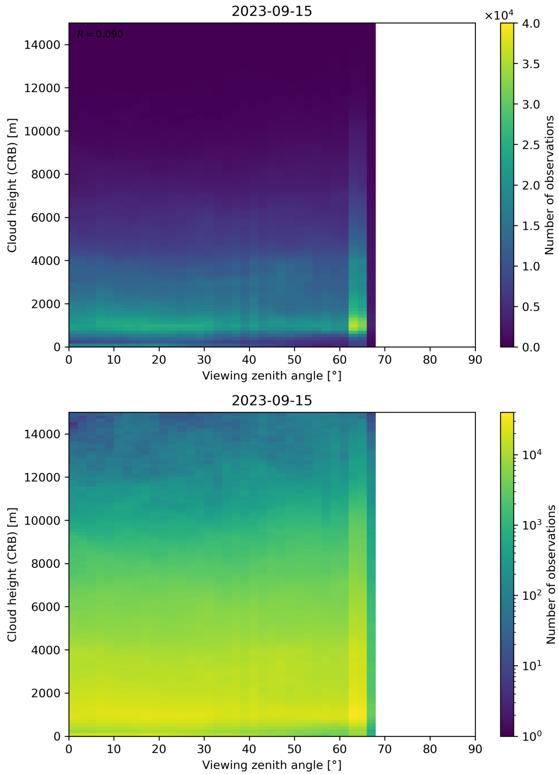
Figure 110: Scatter density plot of “Viewing zenith angle” against “Cloud height (CRB)” for 2023-09-15 to 2023-09-16.
