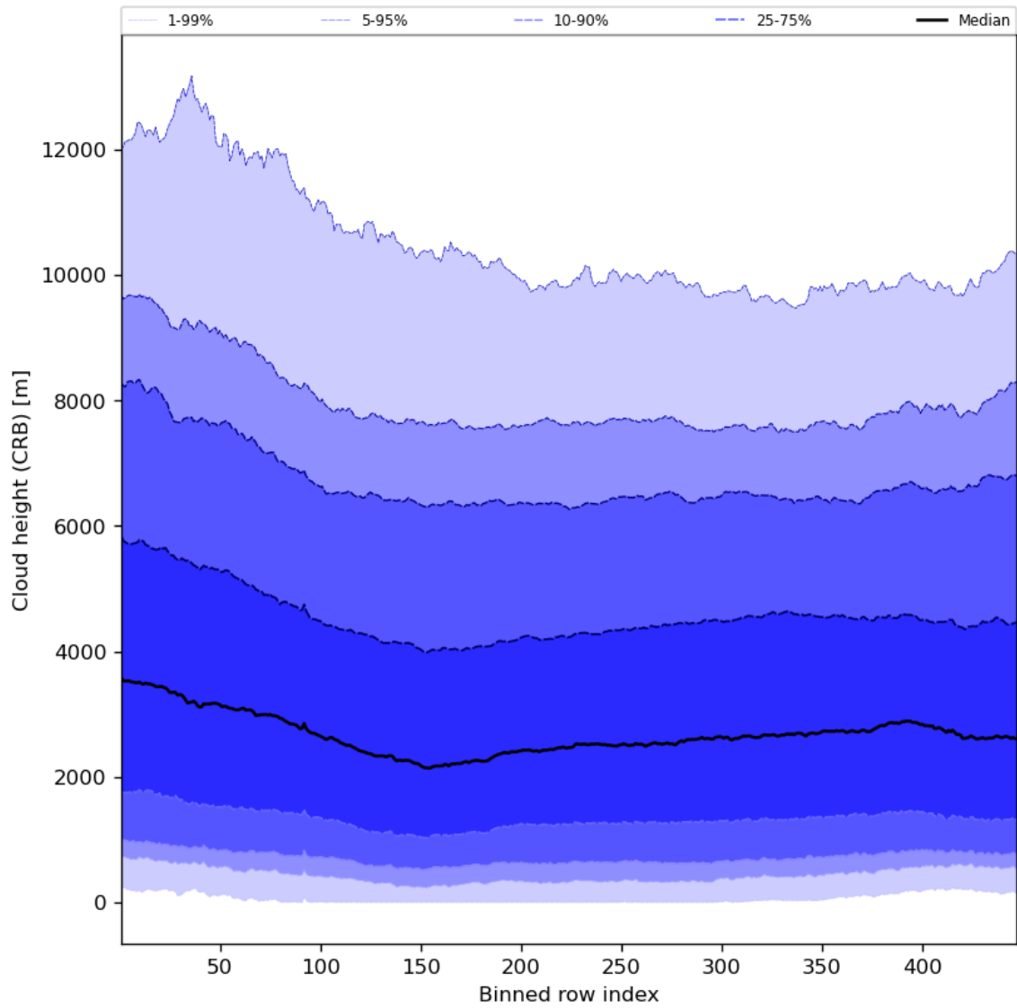
Figure 59: Along track statistics of “Cloud height (CRB)” for 2023-09-15 to 2023-09-16
