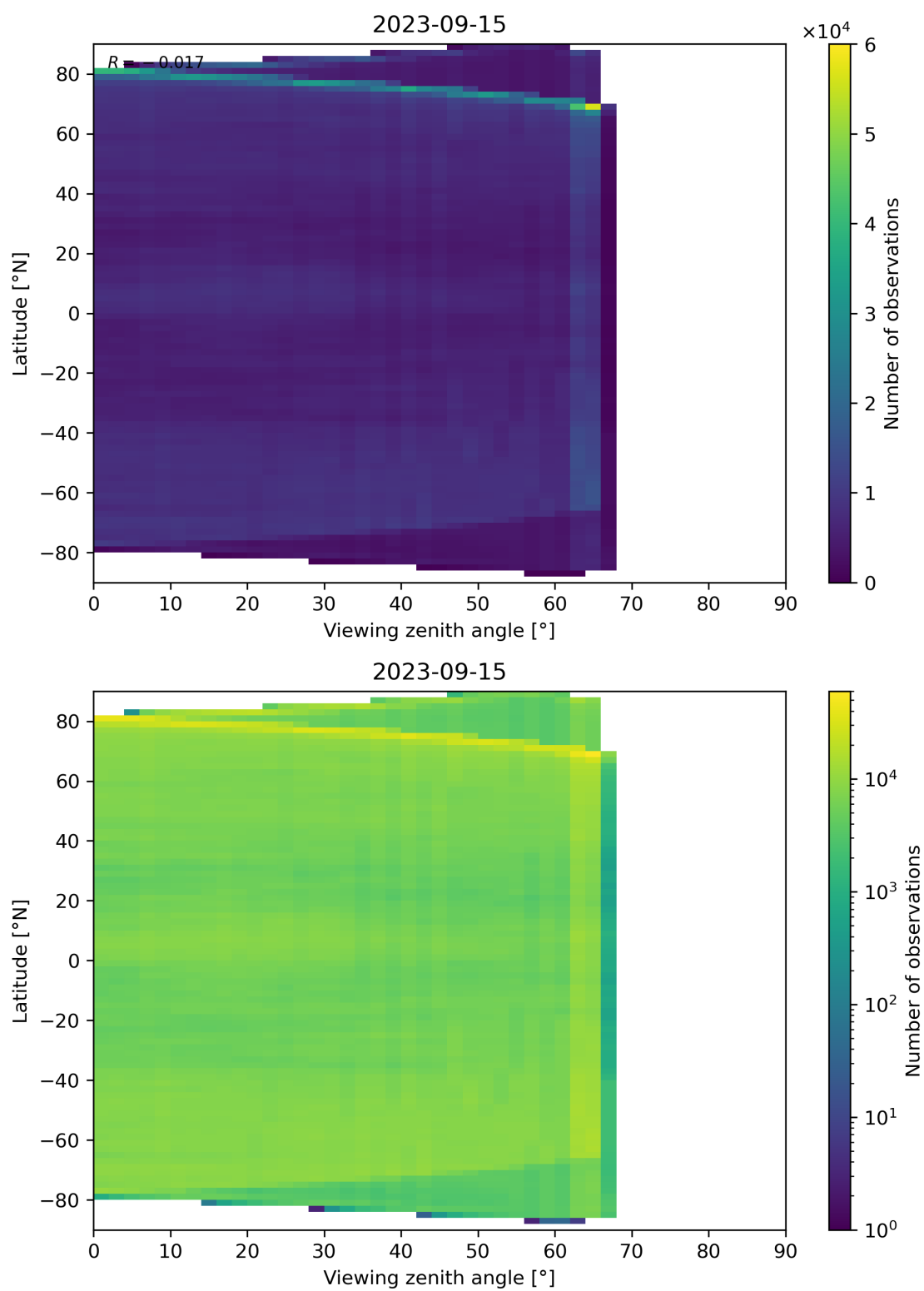
Figure 113: Scatter density plot of “Viewing zenith angle” against “Latitude” for 2023-09-15 to 2023-09-16.
