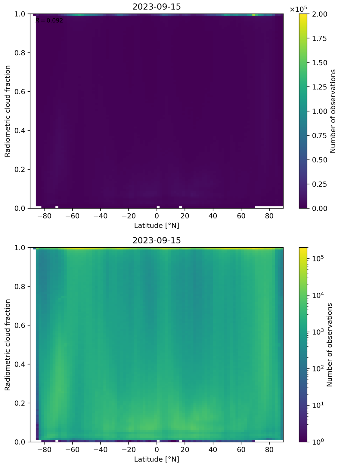
Figure 92: Scatter density plot of “Latitude” against “Radiometric cloud fraction” for 2023-09-15 to 2023-09-16.
