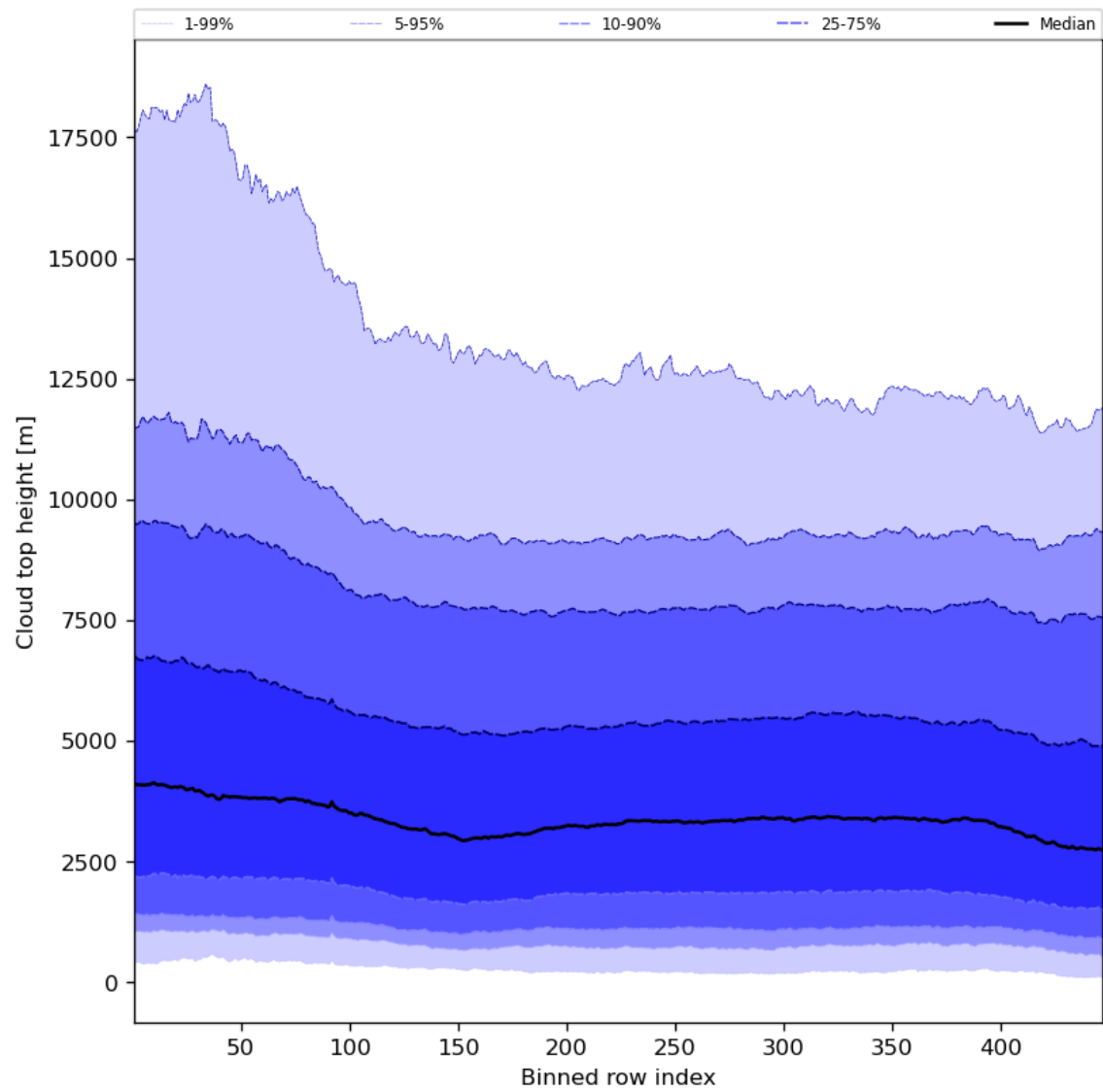
Figure 56: Along track statistics of “Cloud top height” for 2023-09-15 to 2023-09-16
