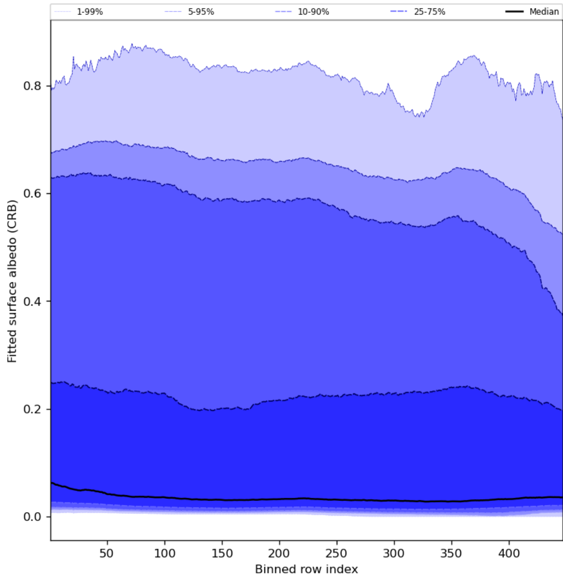
Figure 62: Along track statistics of “Fitted surface albedo (CRB)” for 2023-09-15 to 2023-09-16
