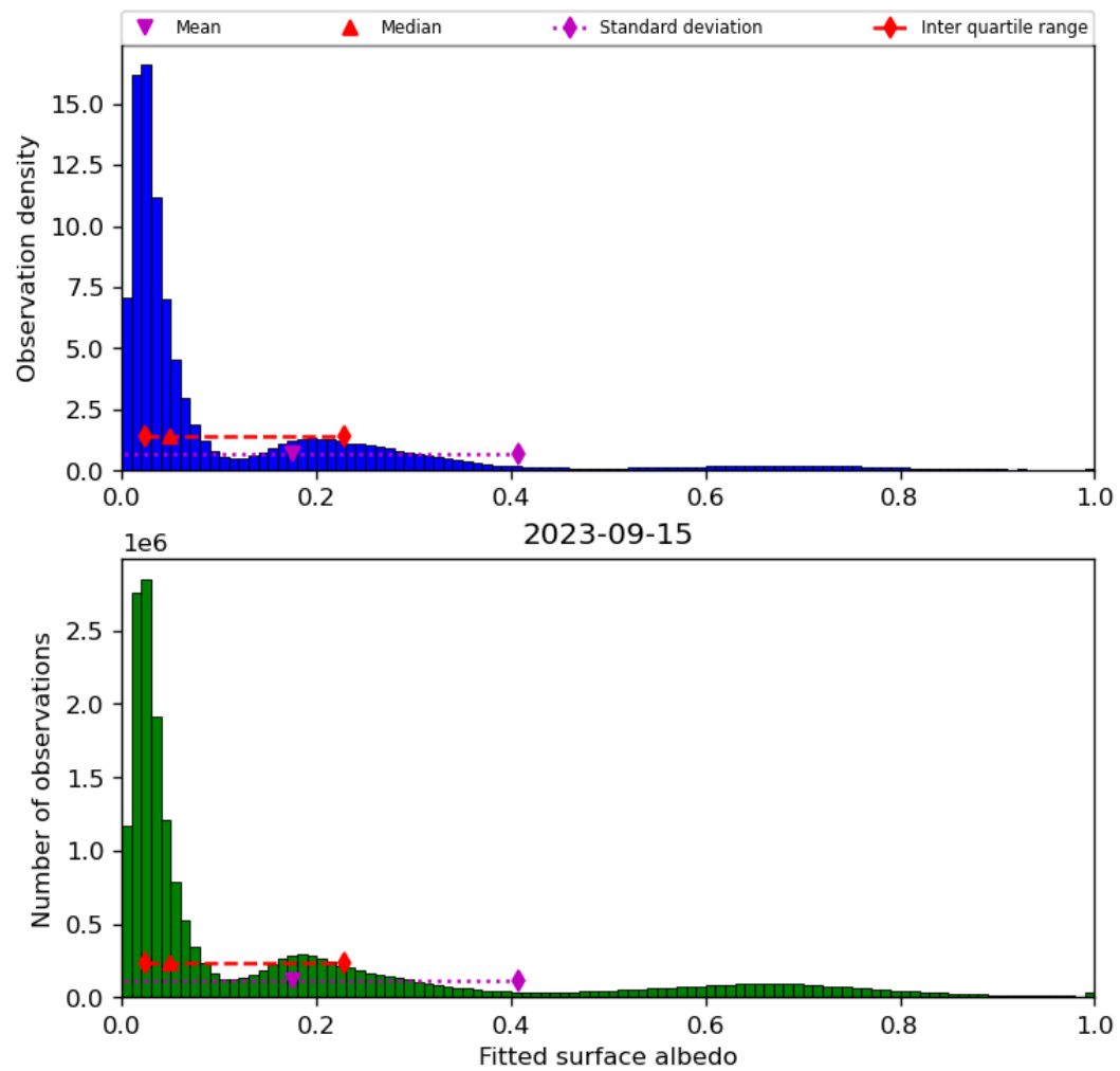
Figure 45: Histogram of “Fitted surface albedo” for 2023-09-15 to 2023-09-16
