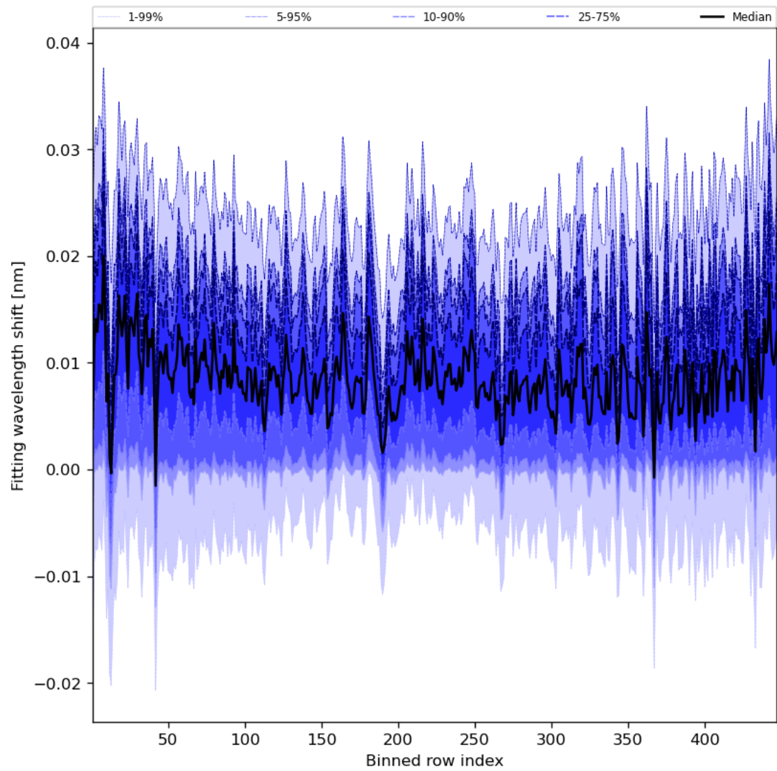
Figure 65: Along track statistics of “Fitting wavelength shift” for 2023-09-15 to 2023-09-16
