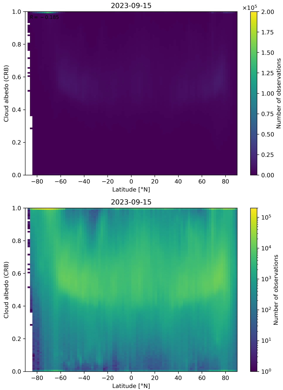
Figure 91: Scatter density plot of “Latitude” against “Cloud albedo (CRB)” for 2023-09-15 to 2023-09-16.
