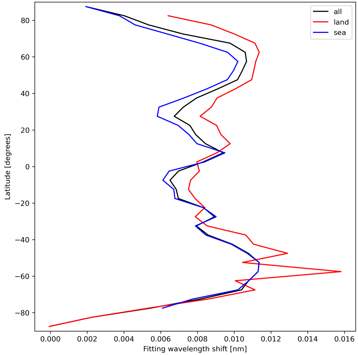
Figure 33: Zonal average of “Fitting wavelength shift” for 2023-09-15 to 2023-09-16.
