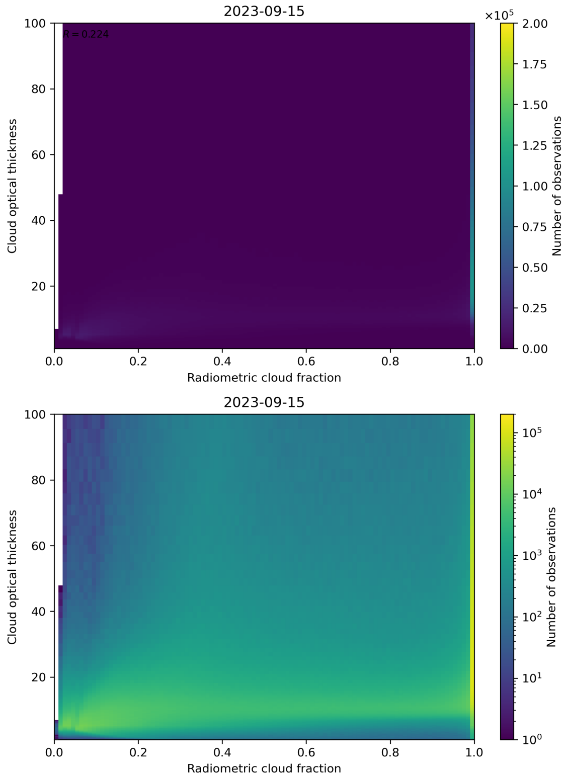
Figure 75: Scatter density plot of “Radiometric cloud fraction” against “Cloud optical thickness” for 2023-09-15 to 2023-09-16.
