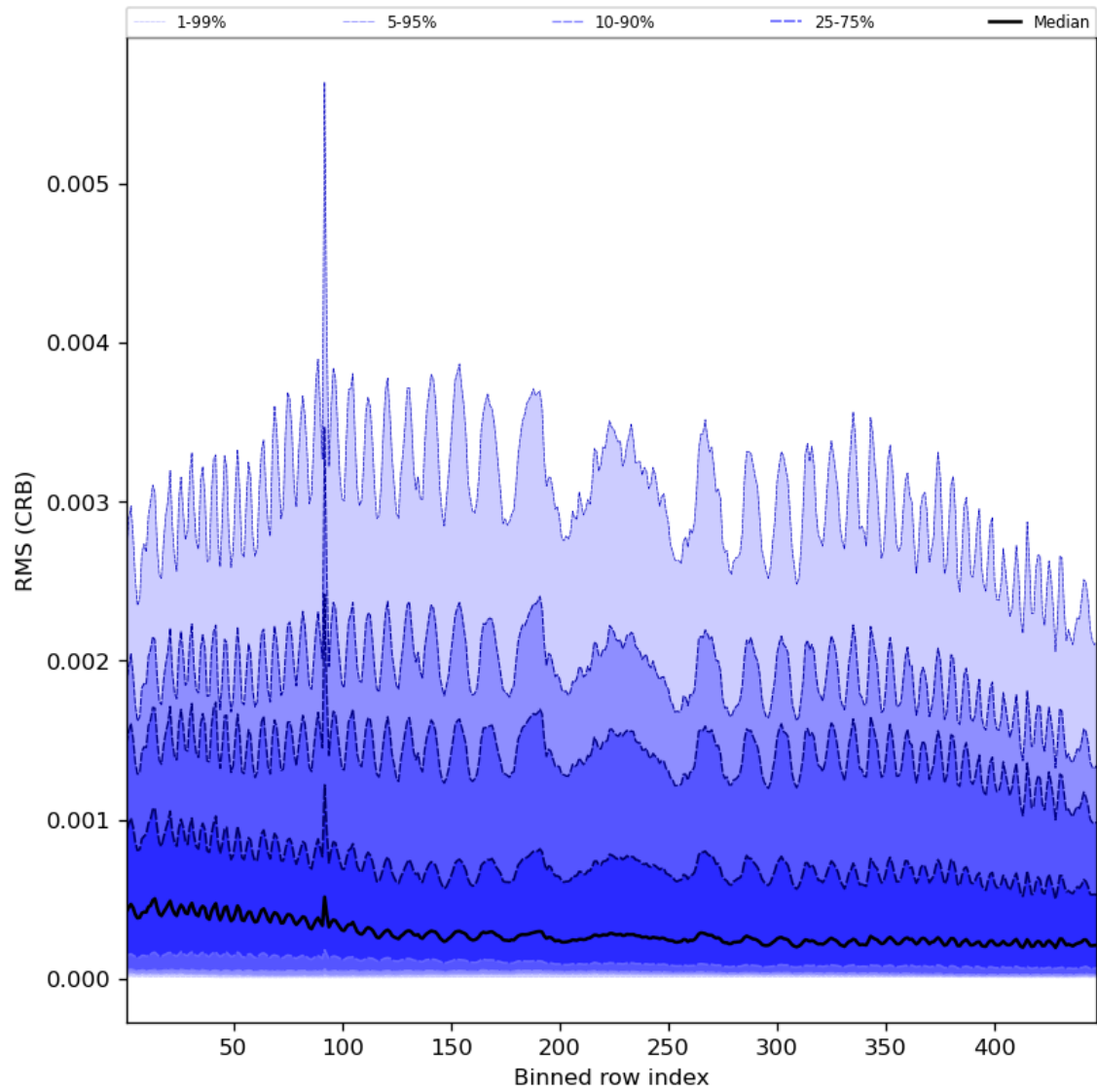
Figure 64: Along track statistics of “RMS (CRB)” for 2023-09-15 to 2023-09-16
