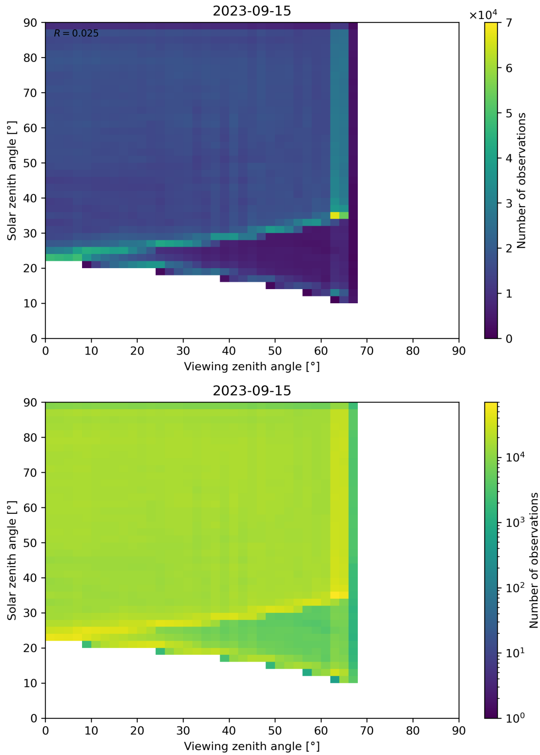
Figure 114: Scatter density plot of “Viewing zenith angle” against “Solar zenith angle” for 2023-09-15 to 2023-09-16.
