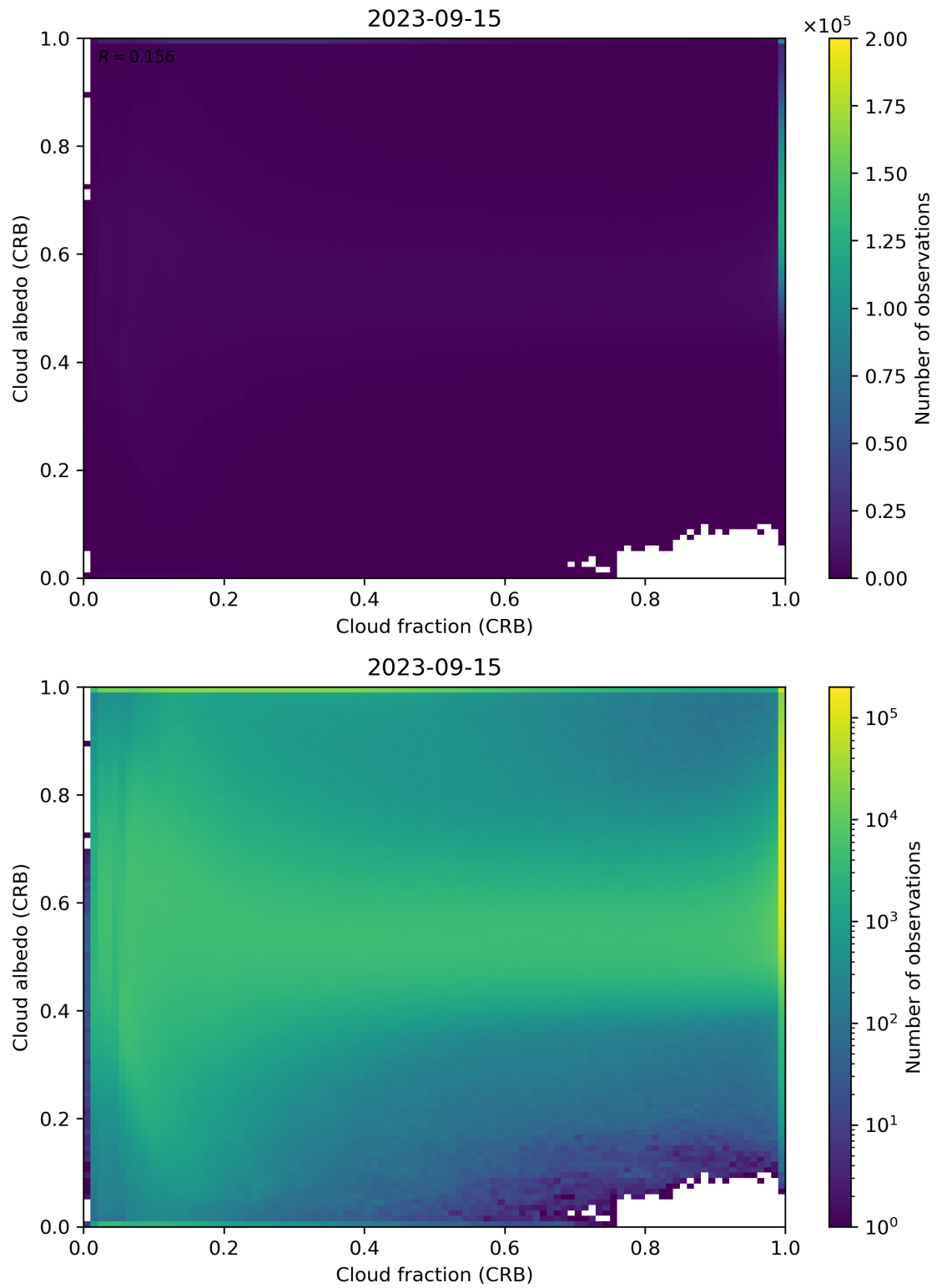
Figure 77: Scatter density plot of “Cloud fraction (CRB)” against “Cloud albedo (CRB)” for 2023-09-15 to 2023-09-16.
