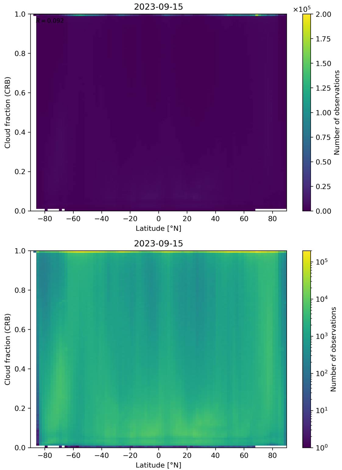
Figure 94: Scatter density plot of “Latitude” against “Cloud fraction (CRB)” for 2023-09-15 to 2023-09-16.
