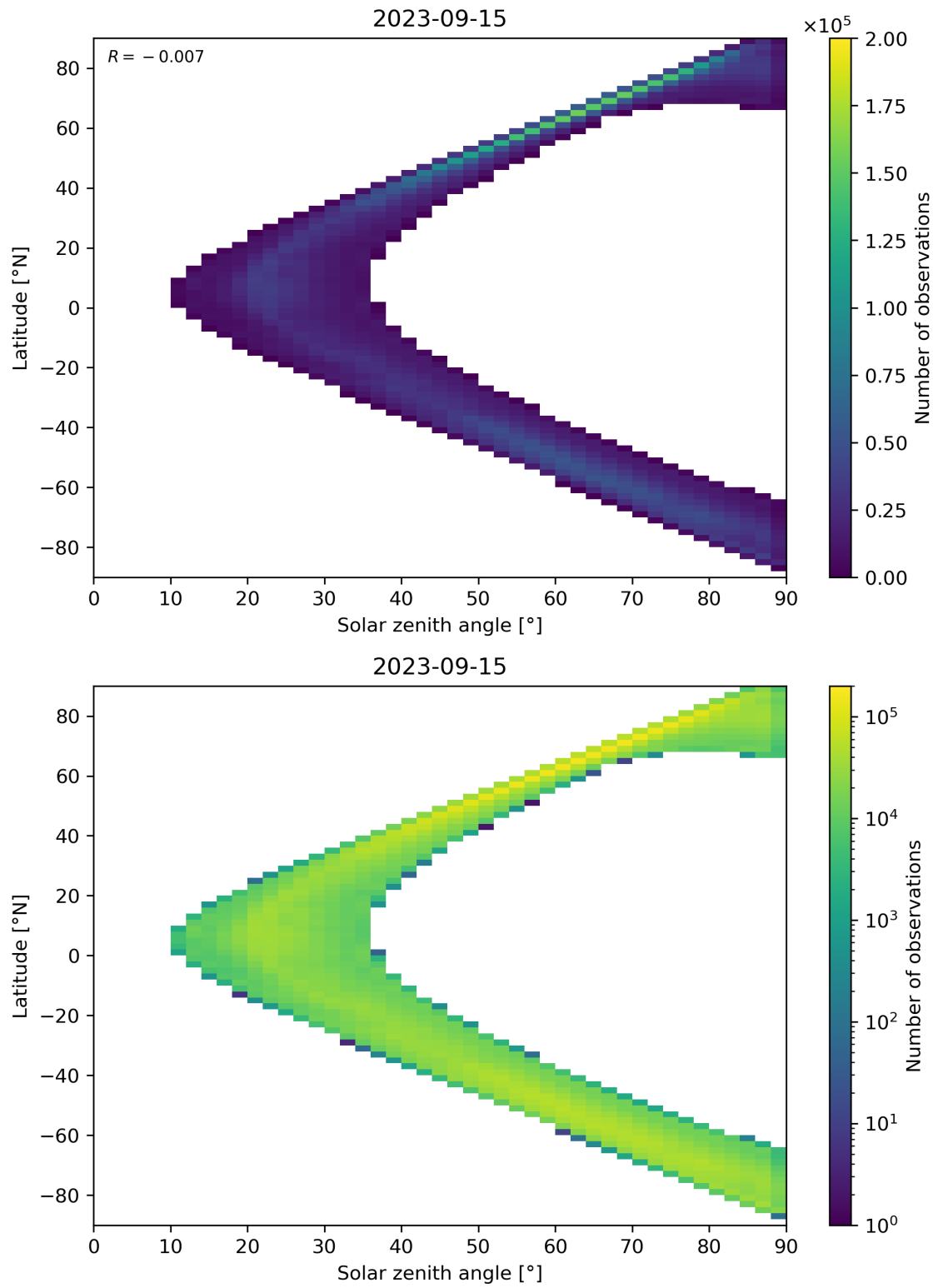
Figure 105: Scatter density plot of “Solar zenith angle” against “Latitude” for 2023-09-15 to 2023-09-16.
