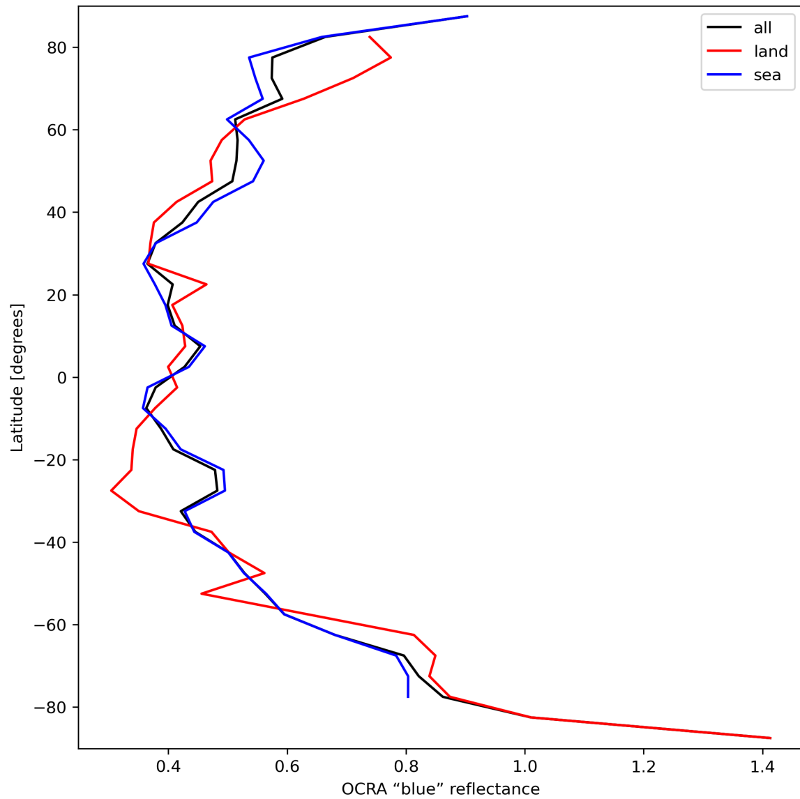
Figure 35: Zonal average of “OCRA “blue” reflectance” for 2023-09-15 to 2023-09-16.
