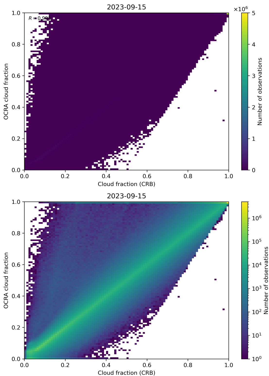
Figure 78: Scatter density plot of “Cloud fraction (CRB)” against “OCRA cloud fraction” for 2023-09-15 to 2023-09-16.
