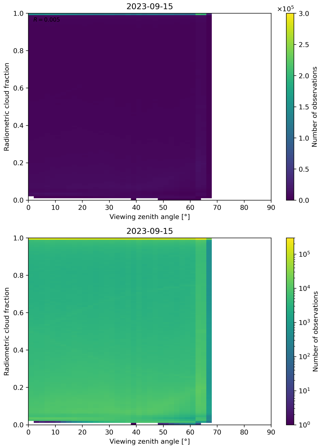
Figure 107: Scatter density plot of “Viewing zenith angle” against “Radiometric cloud fraction” for 2023-09-15 to 2023-09-16.
