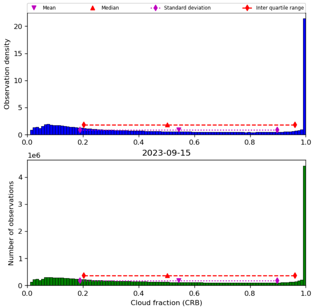
Figure 42: Histogram of “Cloud fraction (CRB)” for 2023-09-15 to 2023-09-16
