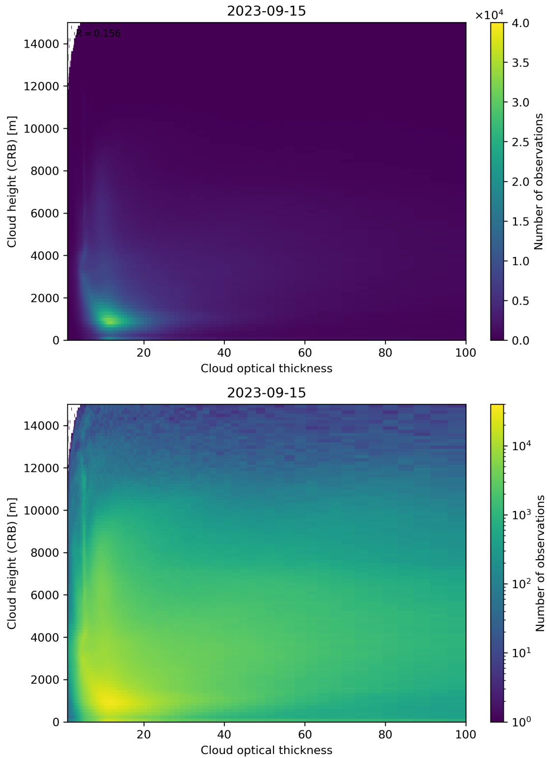
Figure 85: Scatter density plot of “Cloud optical thickness” against “Cloud height (CRB)” for 2023-09-15 to 2023-09-16.
