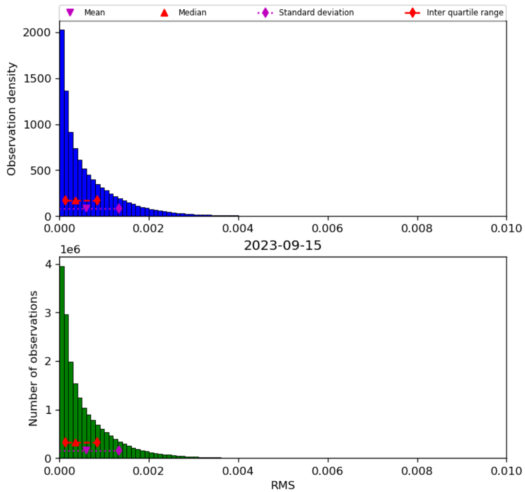
Figure 47: Histogram of “RMS” for 2023-09-15 to 2023-09-16
