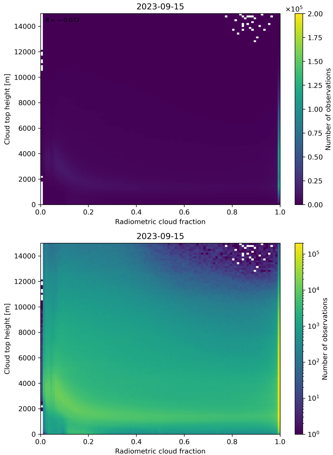
Figure 76: Scatter density plot of “Radiometric cloud fraction” against “Cloud top height” for 2023-09-15 to 2023-09-16.
