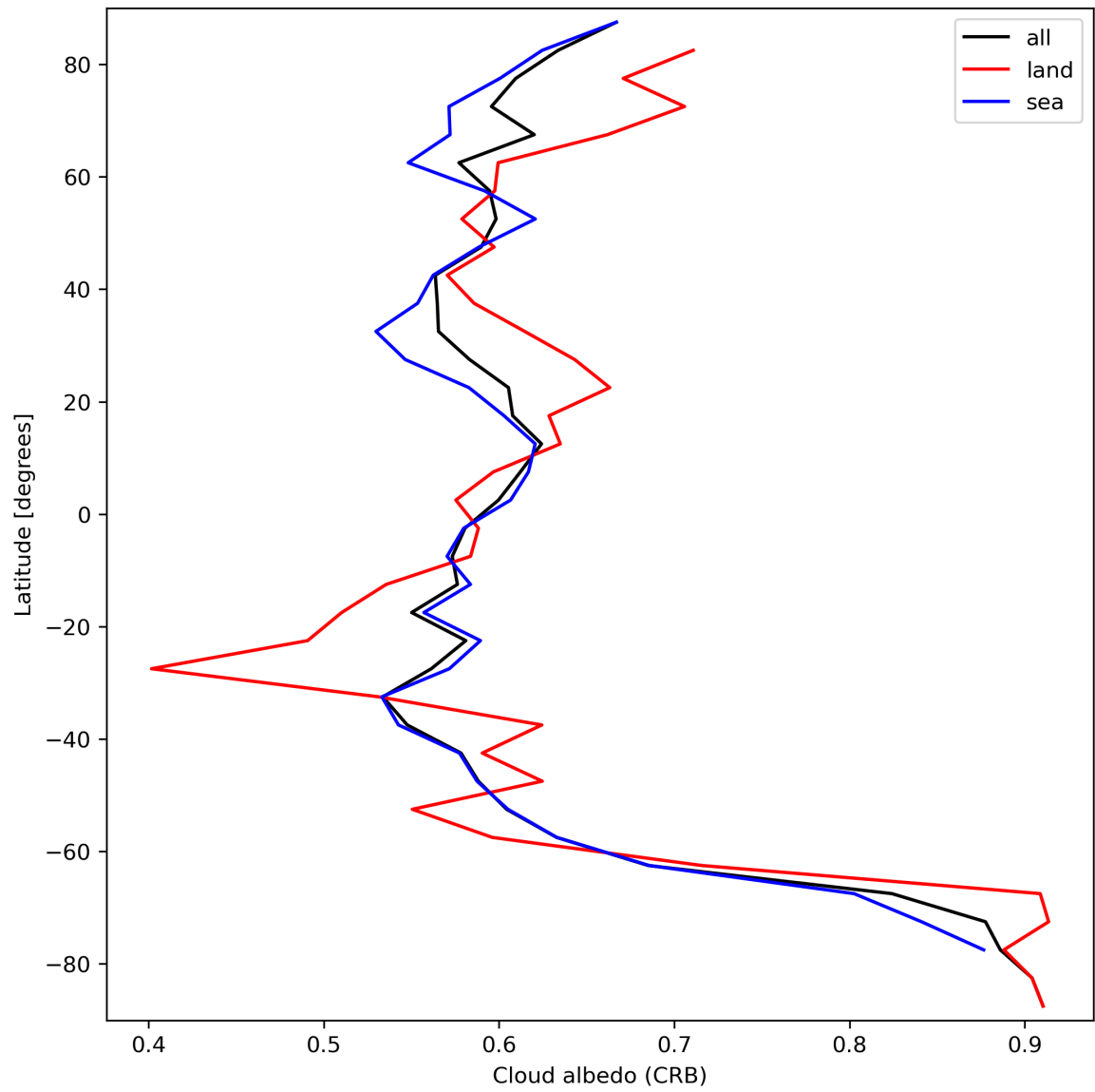
Figure 28: Zonal average of “Cloud albedo (CRB)” for 2023-09-15 to 2023-09-16.
