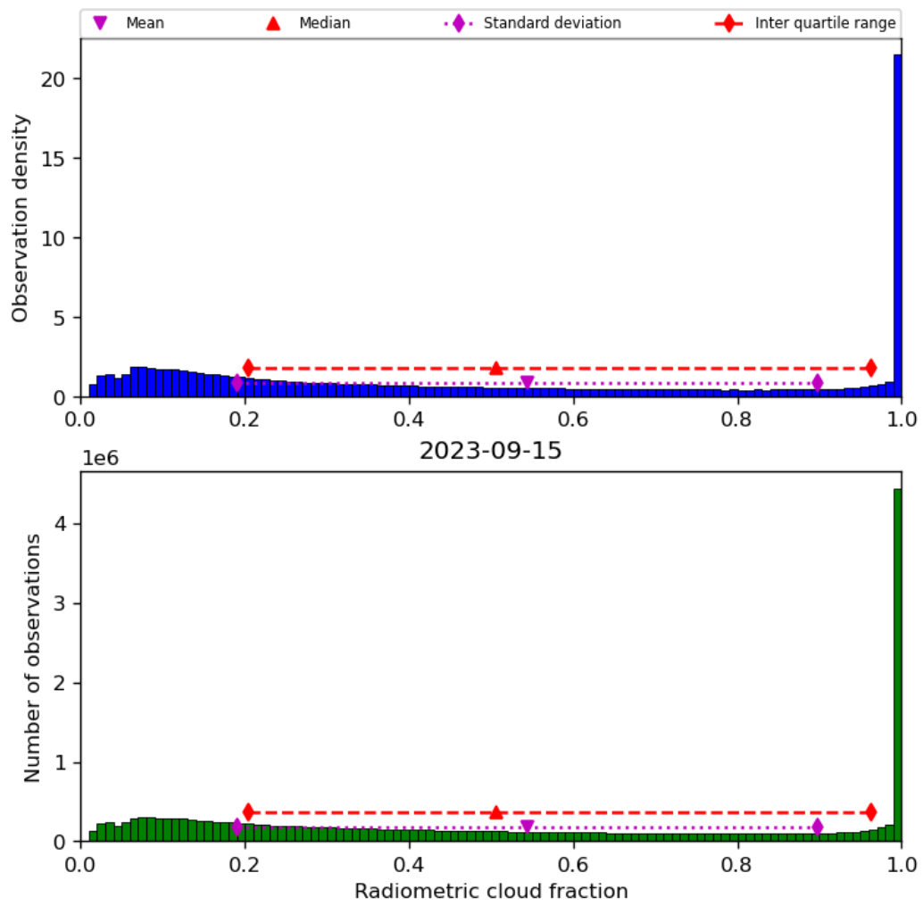
Figure 39: Histogram of “Radiometric cloud fraction” for 2023-09-15 to 2023-09-16
