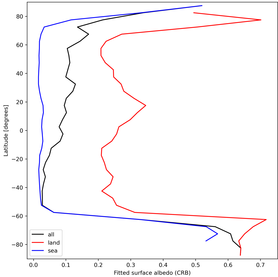
Figure 30: Zonal average of “Fitted surface albedo (CRB)” for 2023-09-15 to 2023-09-16.
