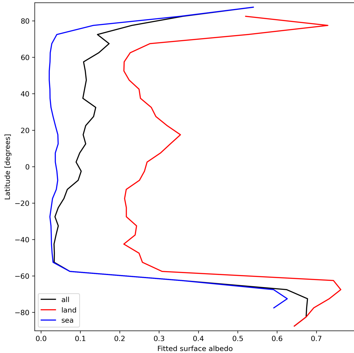
Figure 29: Zonal average of “Fitted surface albedo” for 2023-09-15 to 2023-09-16.
