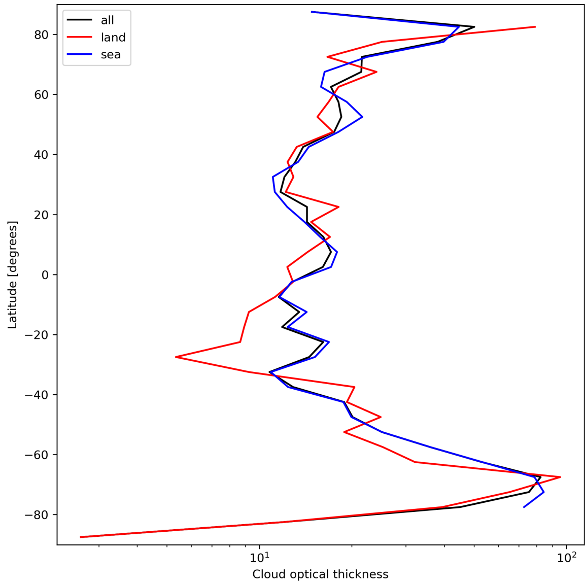
Figure 25: Zonal average of “Cloud optical thickness” for 2023-09-15 to 2023-09-16.
