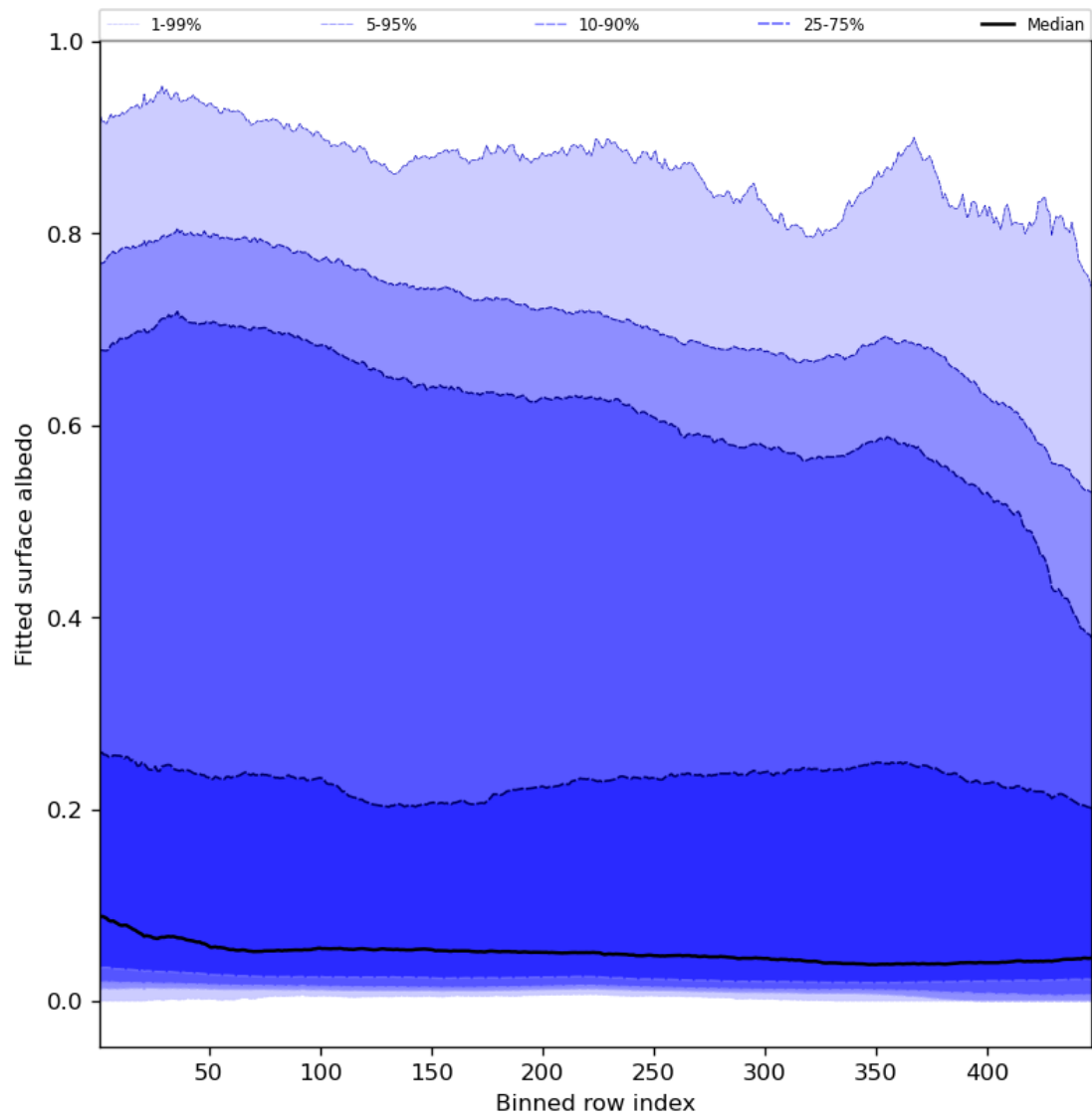
Figure 61: Along track statistics of “Fitted surface albedo” for 2023-09-15 to 2023-09-16
