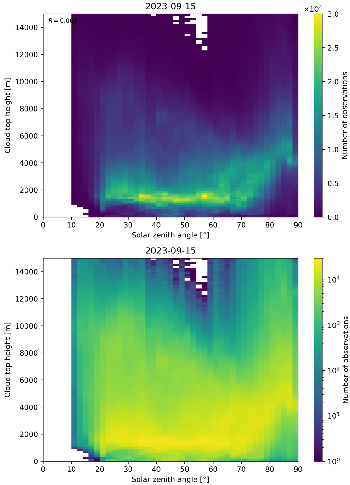
Figure 104: Scatter density plot of “Solar zenith angle” against “Cloud top height” for 2023-09-15 to 2023-09-16.
