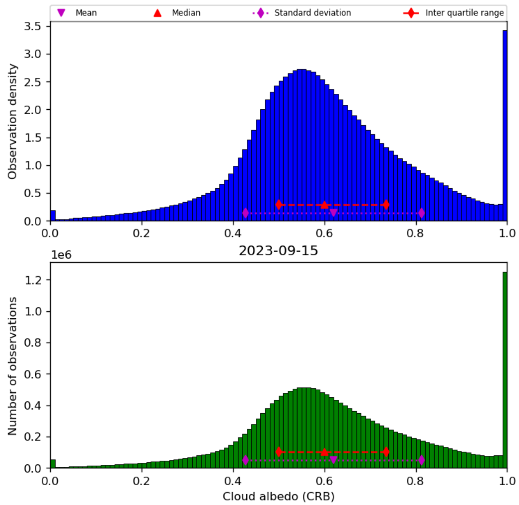
Figure 44: Histogram of “Cloud albedo (CRB)” for 2023-09-15 to 2023-09-16
