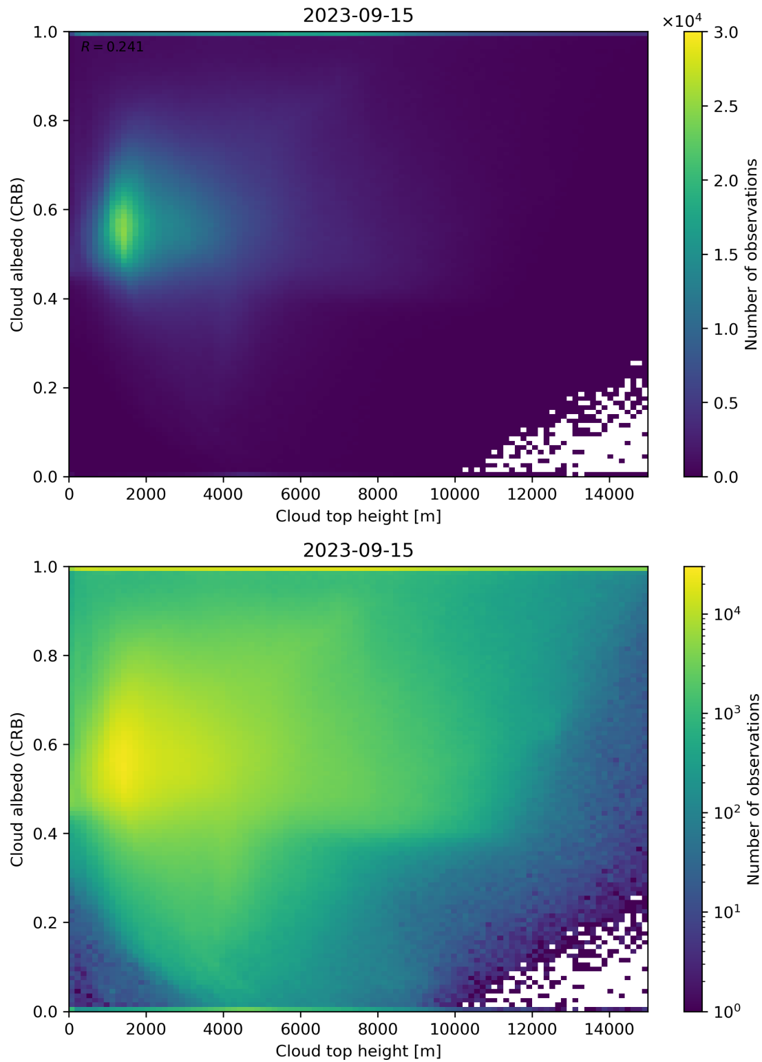
Figure 86: Scatter density plot of “Cloud top height” against “Cloud albedo (CRB)” for 2023-09-15 to 2023-09-16.
