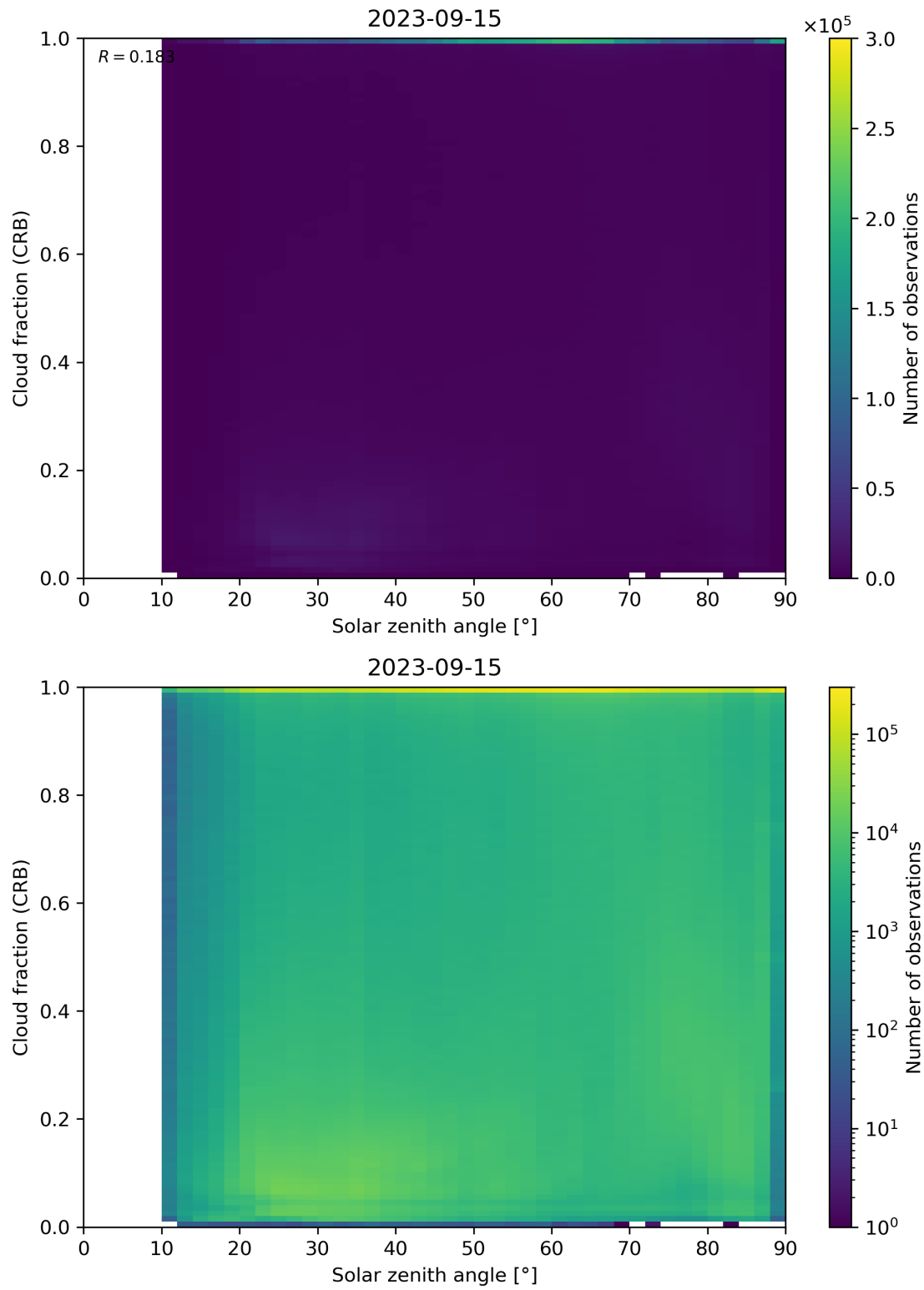
Figure 101: Scatter density plot of “Solar zenith angle” against “Cloud fraction (CRB)” for 2023-09-15 to 2023-09-16.
