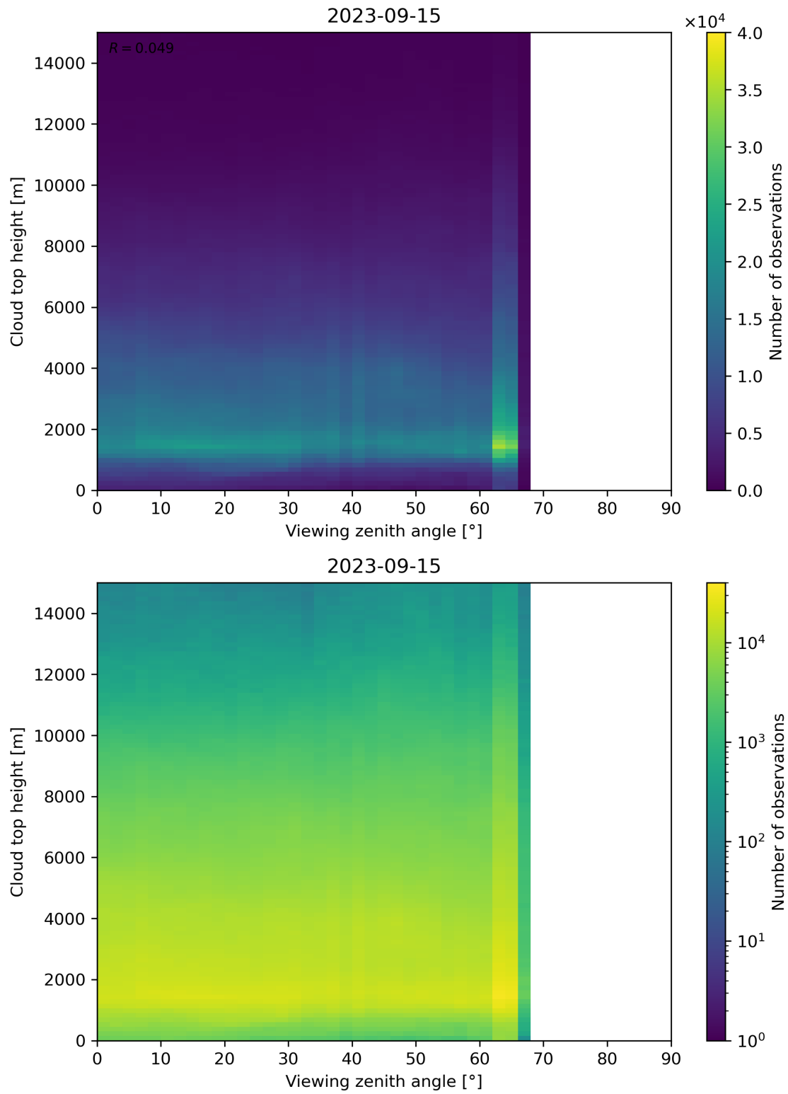
Figure 112: Scatter density plot of “Viewing zenith angle” against “Cloud top height” for 2023-09-15 to 2023-09-16.
