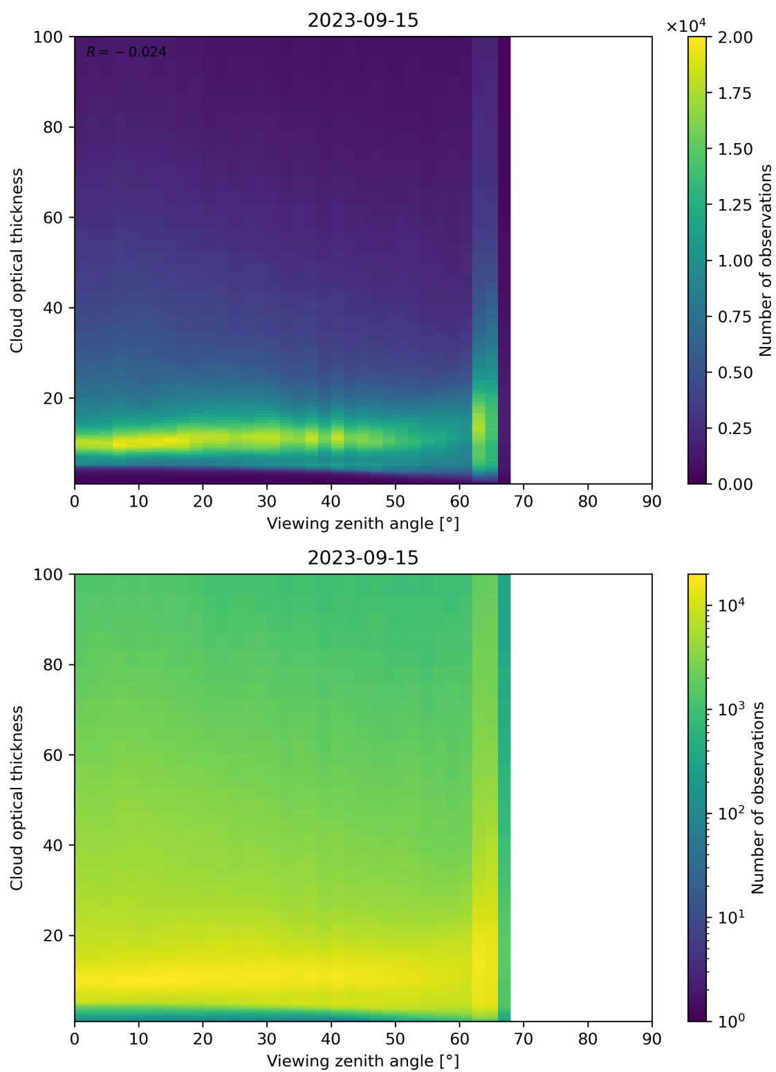
Figure 111: Scatter density plot of “Viewing zenith angle” against “Cloud optical thickness” for 2023-09-15 to 2023-09-16.
