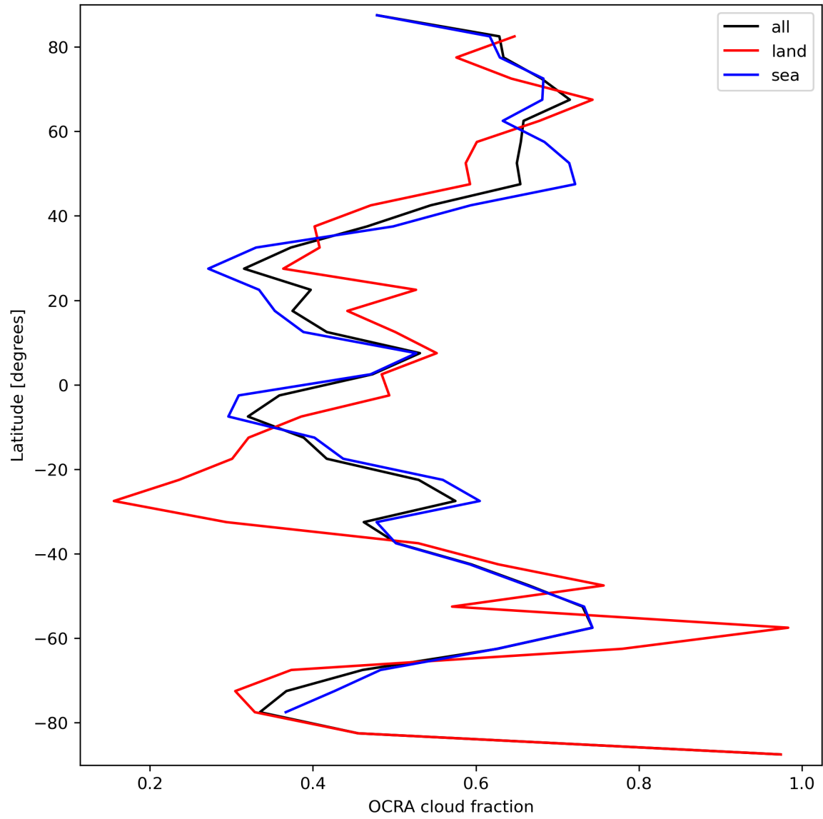
Figure 34: Zonal average of “OCRA cloud fraction” for 2023-09-15 to 2023-09-16.
