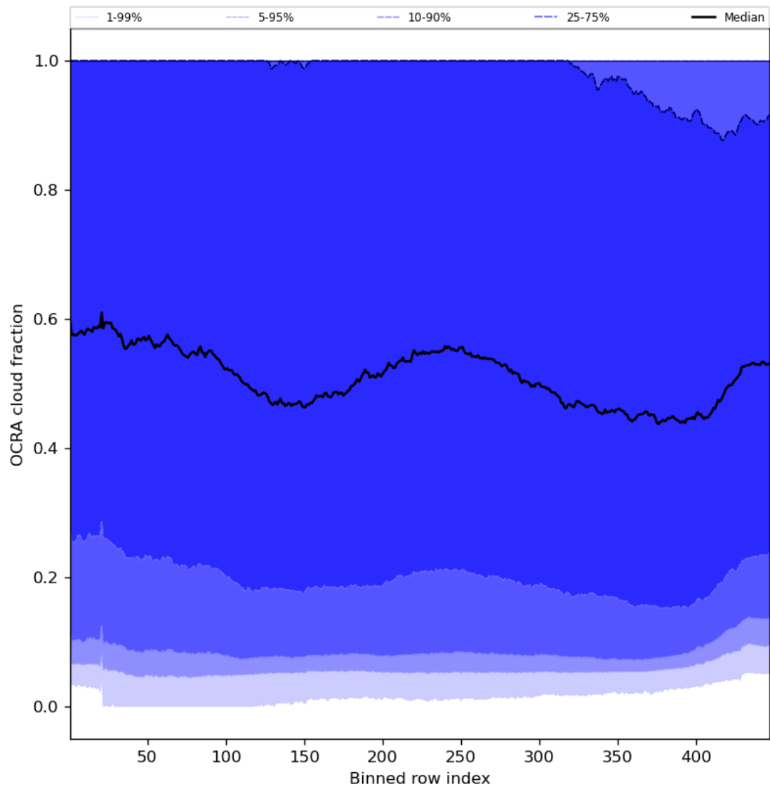
Figure 66: Along track statistics of “OCRA cloud fraction” for 2023-09-15 to 2023-09-16
