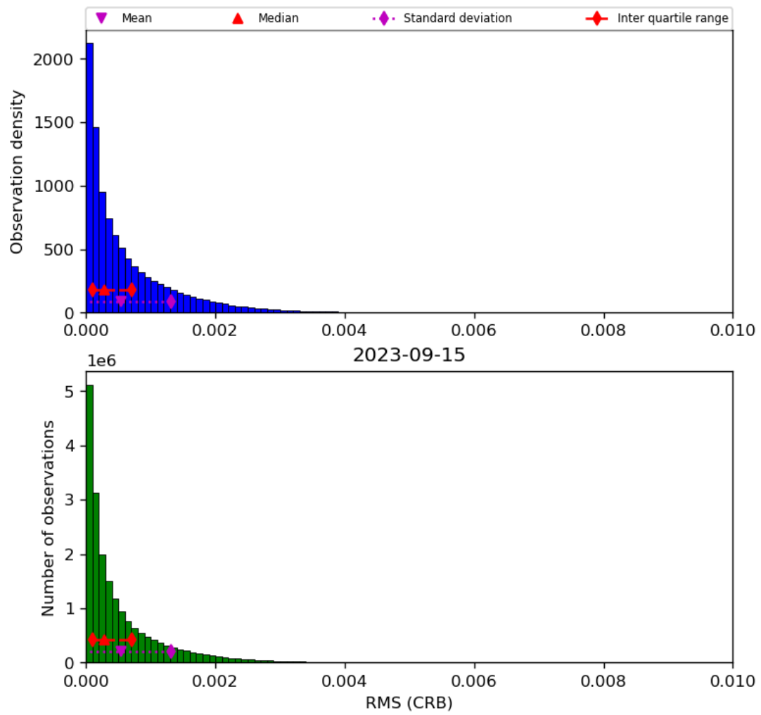
Figure 48: Histogram of “RMS (CRB)” for 2023-09-15 to 2023-09-16
