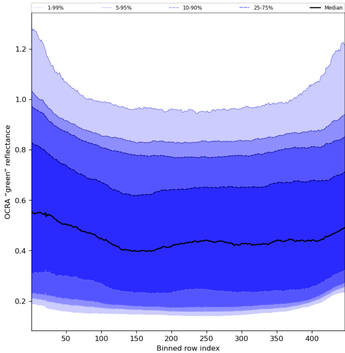
Figure 68: Along track statistics of “OCRA “green” reflectance” for 2023-09-15 to 2023-09-16
