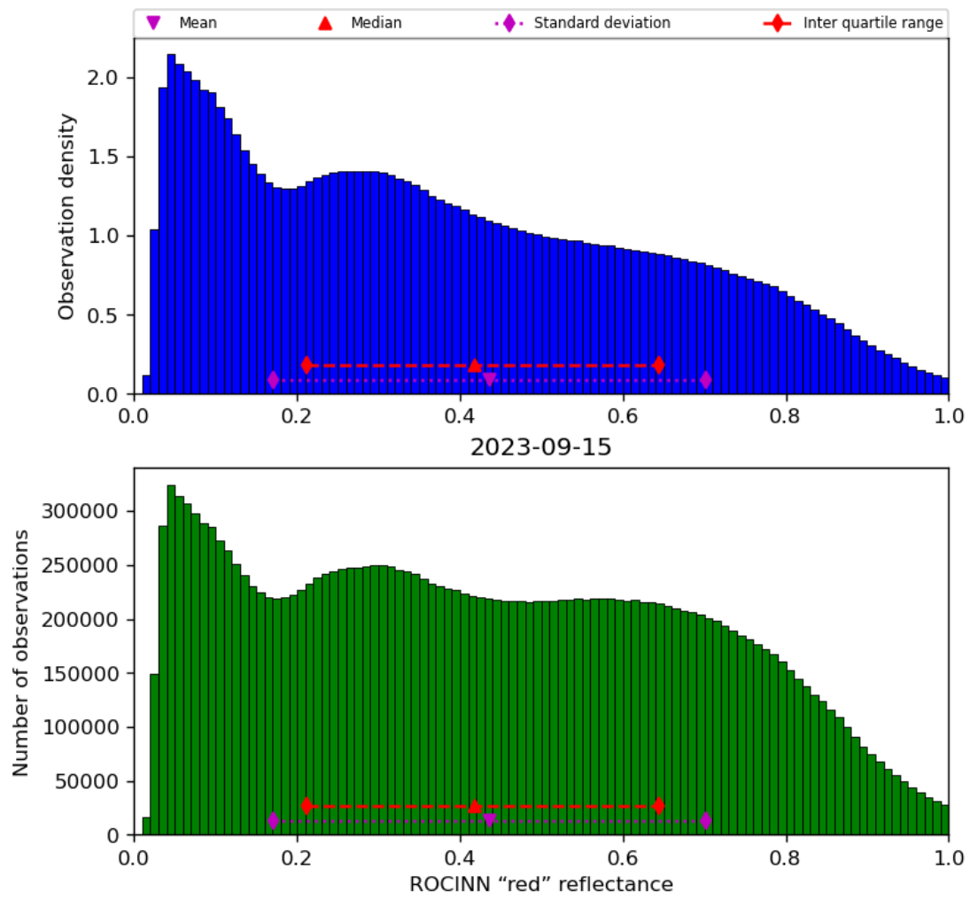
Figure 53: Histogram of “ROCINN “red” reflectance” for 2023-09-15 to 2023-09-16
