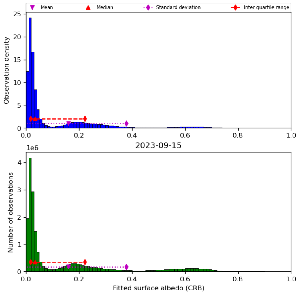
Figure 46: Histogram of “Fitted surface albedo (CRB)” for 2023-09-15 to 2023-09-16
