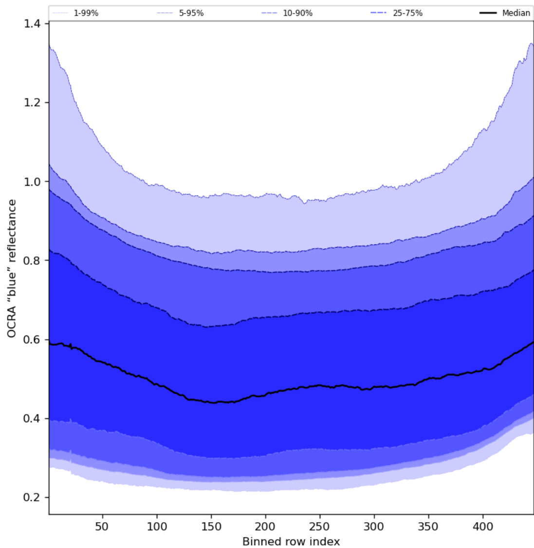
Figure 67: Along track statistics of “OCRA “blue” reflectance” for 2023-09-15 to 2023-09-16
