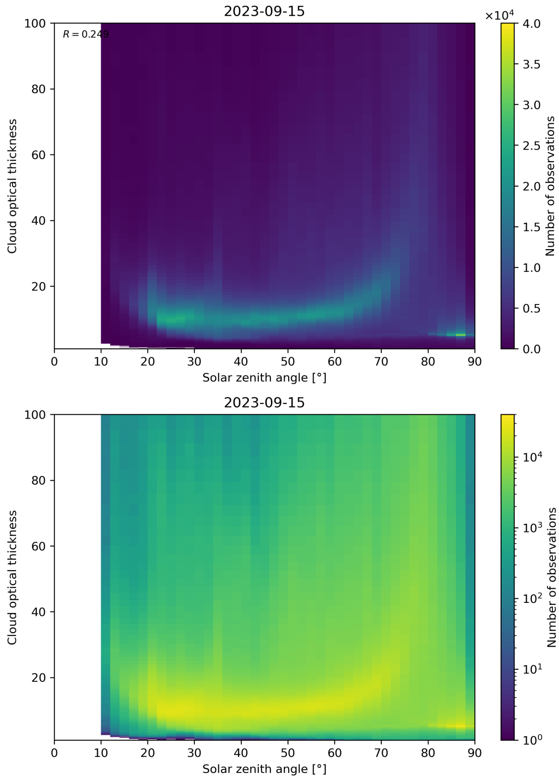
Figure 103: Scatter density plot of “Solar zenith angle” against “Cloud optical thickness” for 2023-09-15 to 2023-09-16.
