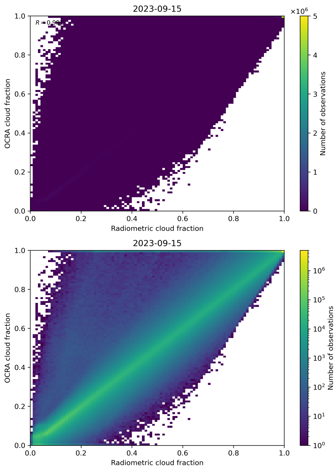
Figure 72: Scatter density plot of “Radiometric cloud fraction” against “OCRA cloud fraction” for 2023-09-15 to 2023-09-16.
