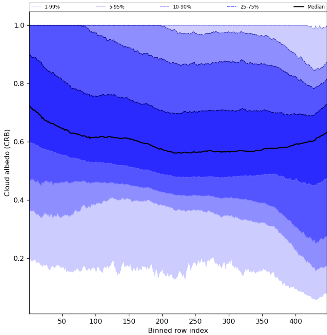
Figure 60: Along track statistics of “Cloud albedo (CRB)” for 2023-09-15 to 2023-09-16
