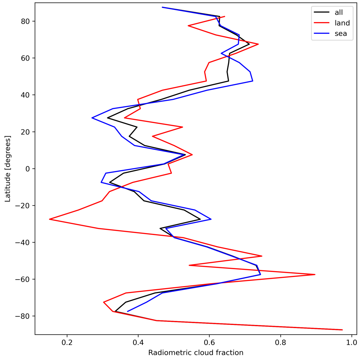
Figure 23: Zonal average of “Radiometric cloud fraction” for 2023-09-15 to 2023-09-16.
