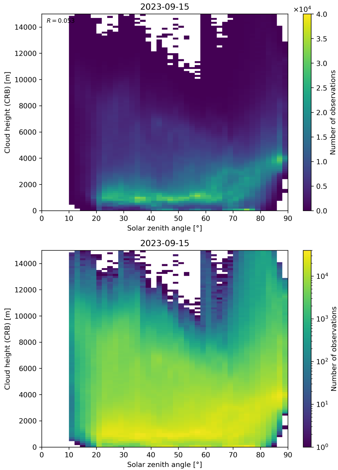
Figure 102: Scatter density plot of “Solar zenith angle” against “Cloud height (CRB)” for 2023-09-15 to 2023-09-16.
