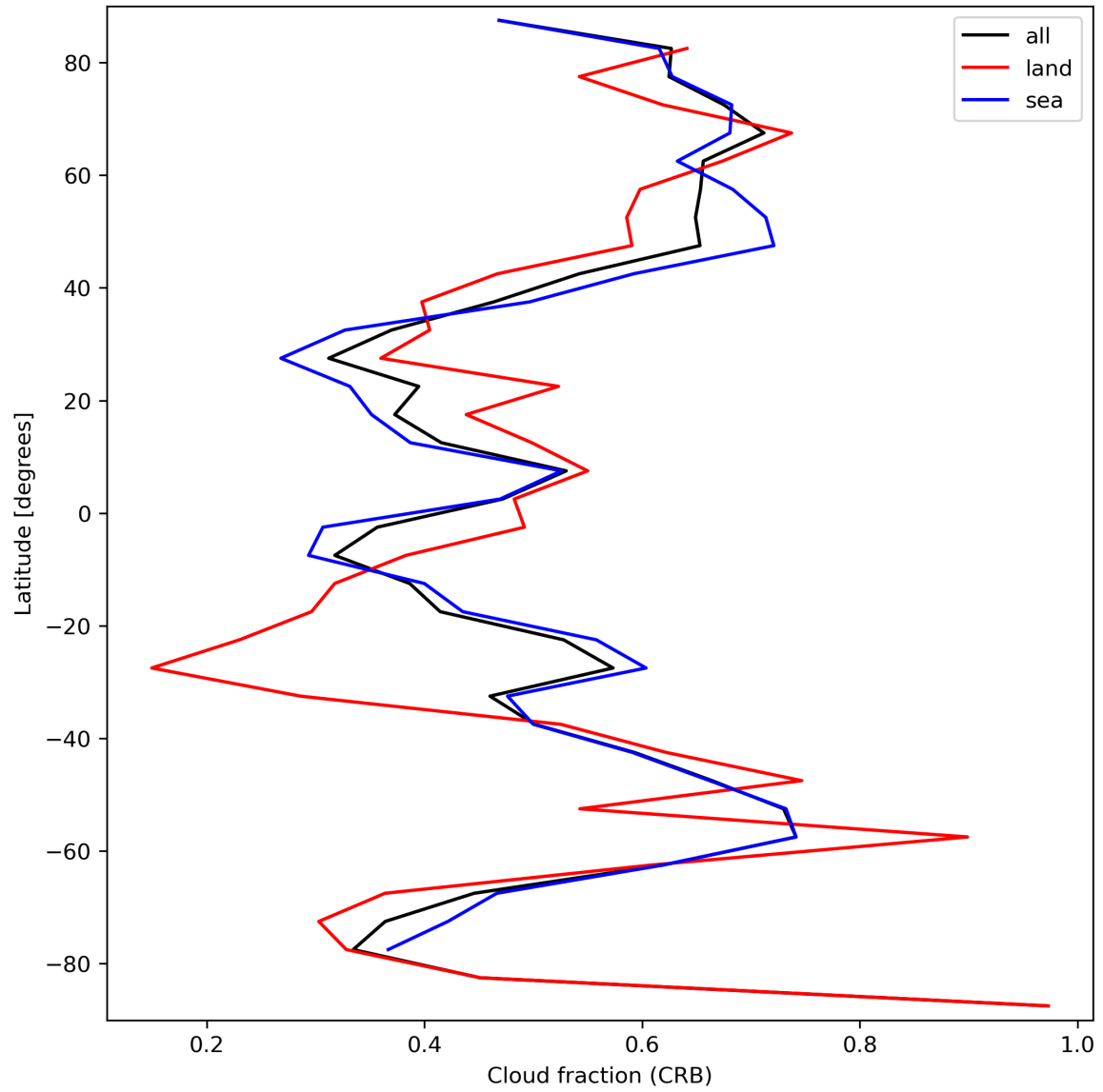
Figure 26: Zonal average of “Cloud fraction (CRB)” for 2023-09-15 to 2023-09-16.
