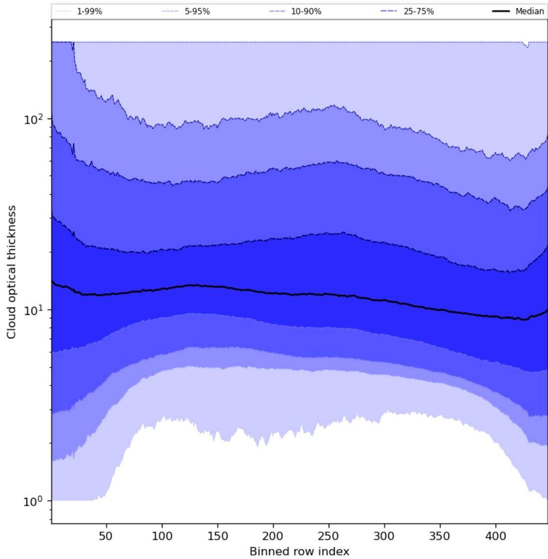
Figure 57: Along track statistics of “Cloud optical thickness” for 2023-09-15 to 2023-09-16
