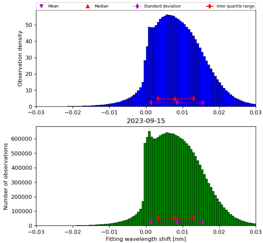
Figure 49: Histogram of “Fitting wavelength shift” for 2023-09-15 to 2023-09-16
