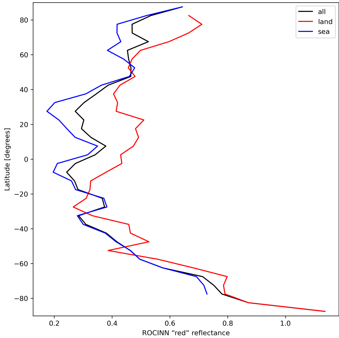
Figure 37: Zonal average of "ROCINN "red" reflectance" for 2023-09-15 to 2023-09-16.
