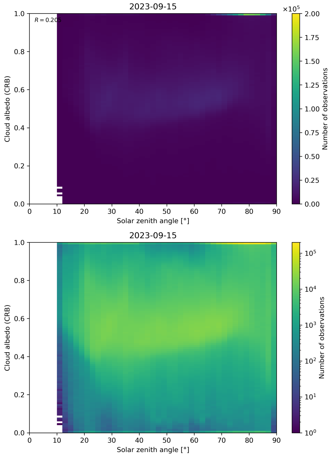
Figure 98: Scatter density plot of “Solar zenith angle” against “Cloud albedo (CRB)” for 2023-09-15 to 2023-09-16.
