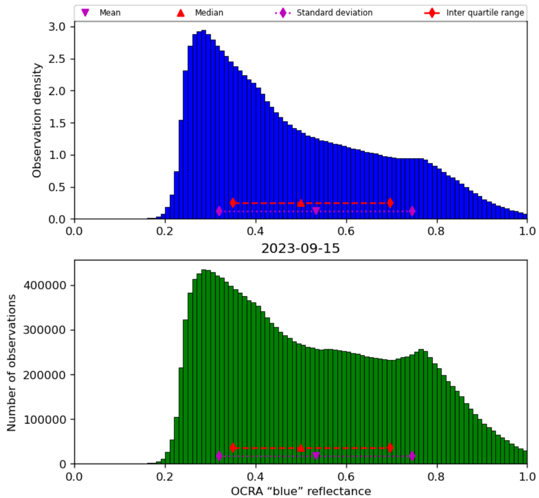
Figure 51: Histogram of “OCRA “blue” reflectance” for 2023-09-15 to 2023-09-16
