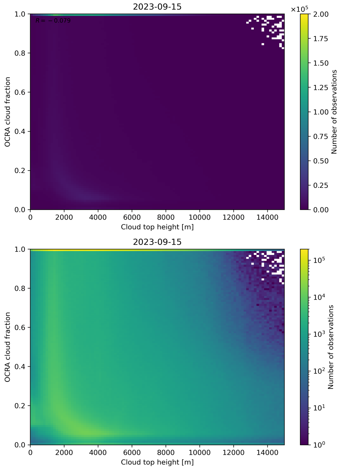
Figure 87: Scatter density plot of “Cloud top height” against “OCRA cloud fraction” for 2023-09-15 to 2023-09-16.
