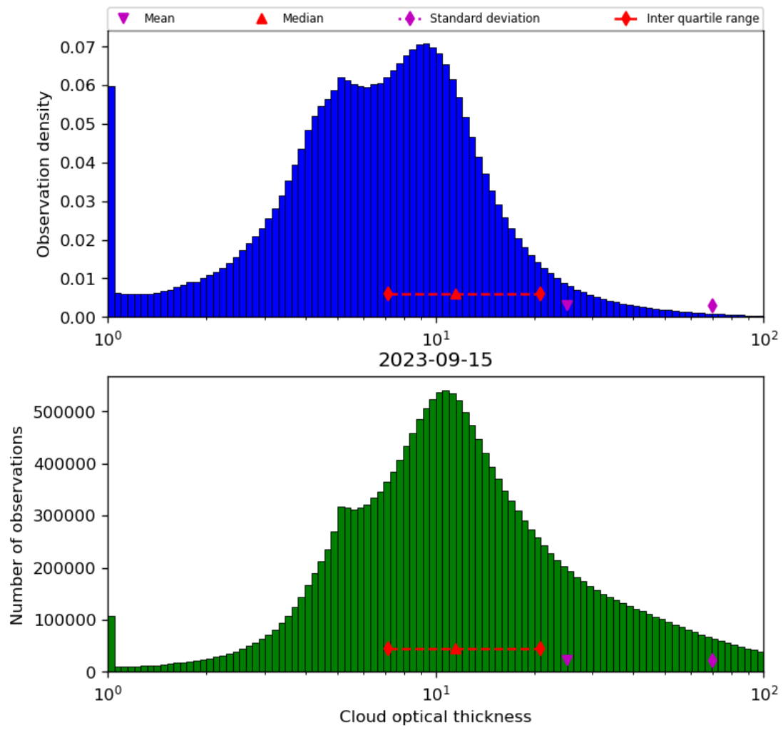
Figure 41: Histogram of “Cloud optical thickness” for 2023-09-15 to 2023-09-16
