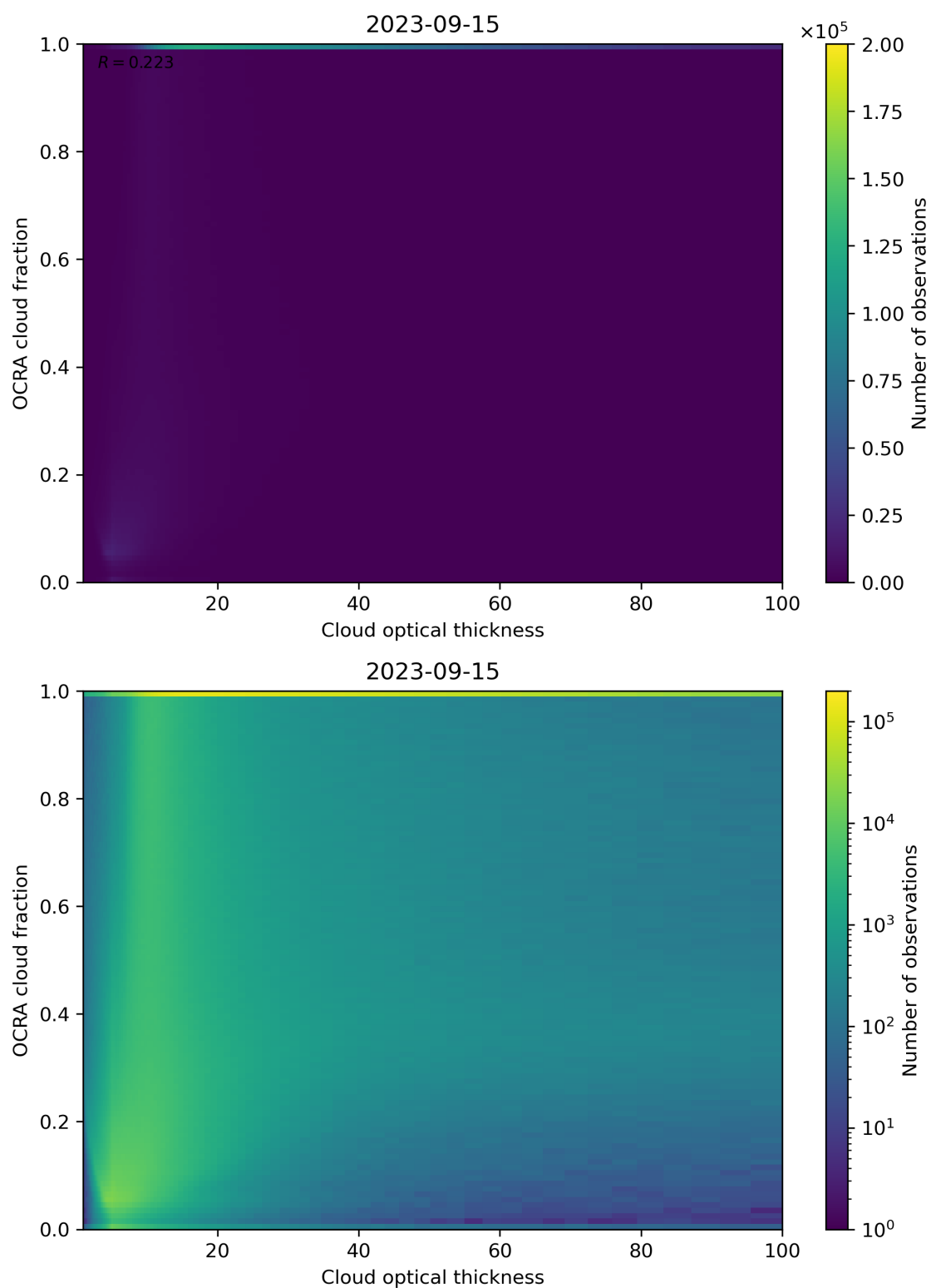
Figure 83: Scatter density plot of “Cloud optical thickness” against “OCRA cloud fraction” for 2023-09-15 to 2023-09-16.
