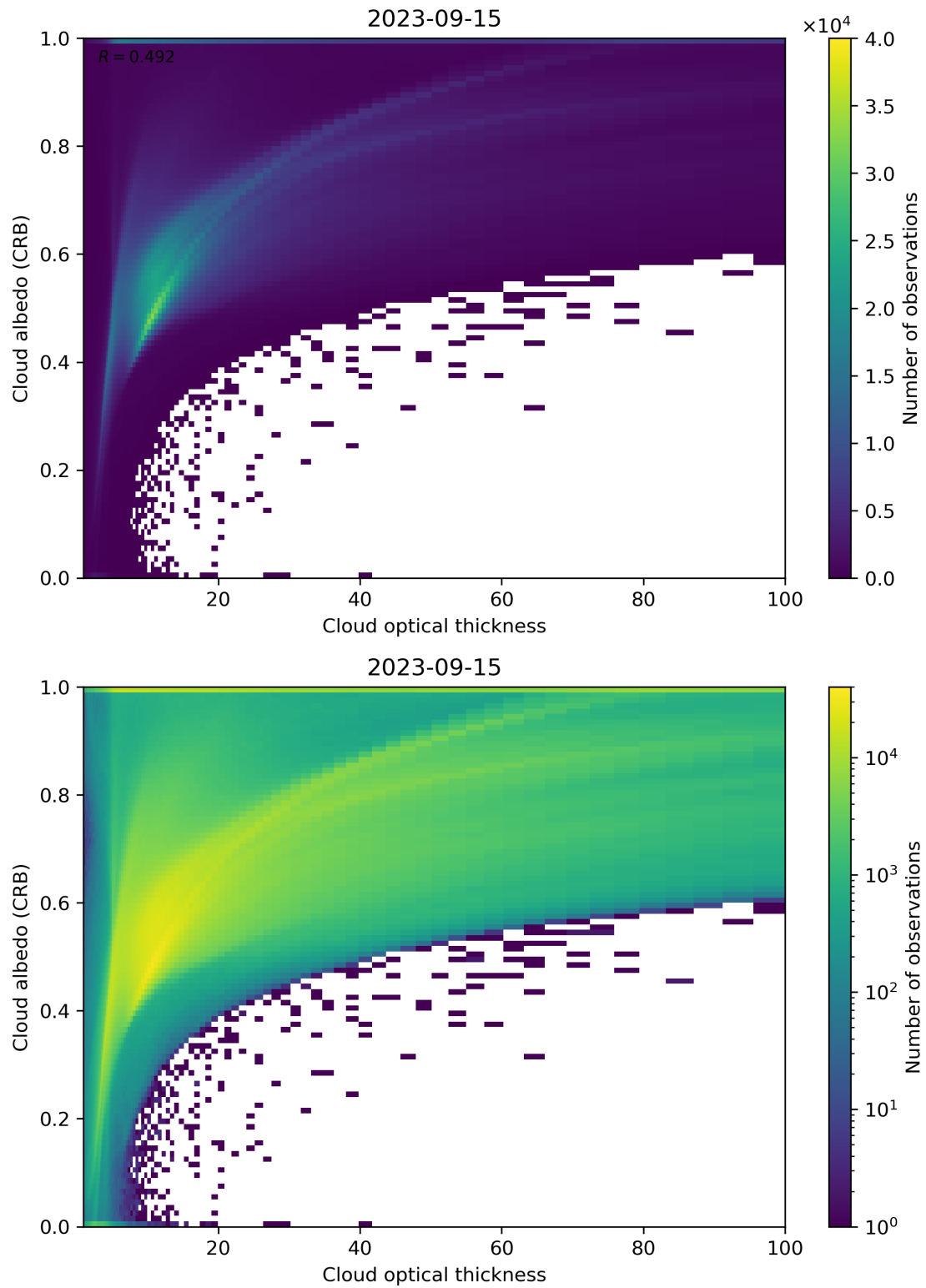
Figure 82: Scatter density plot of “Cloud optical thickness” against “Cloud albedo (CRB)” for 2023-09-15 to 2023-09-16.
