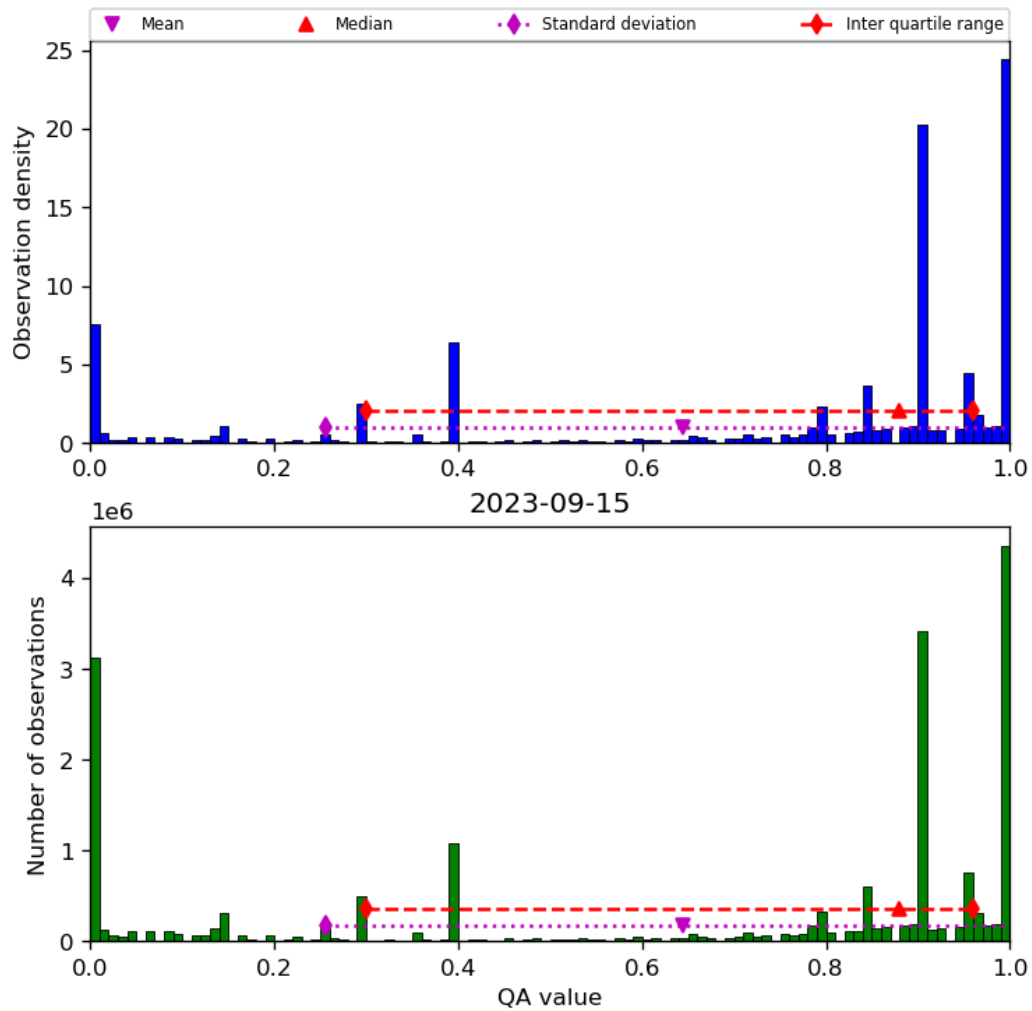
Figure 38: Histogram of “QA value” for 2023-09-15 to 2023-09-16
