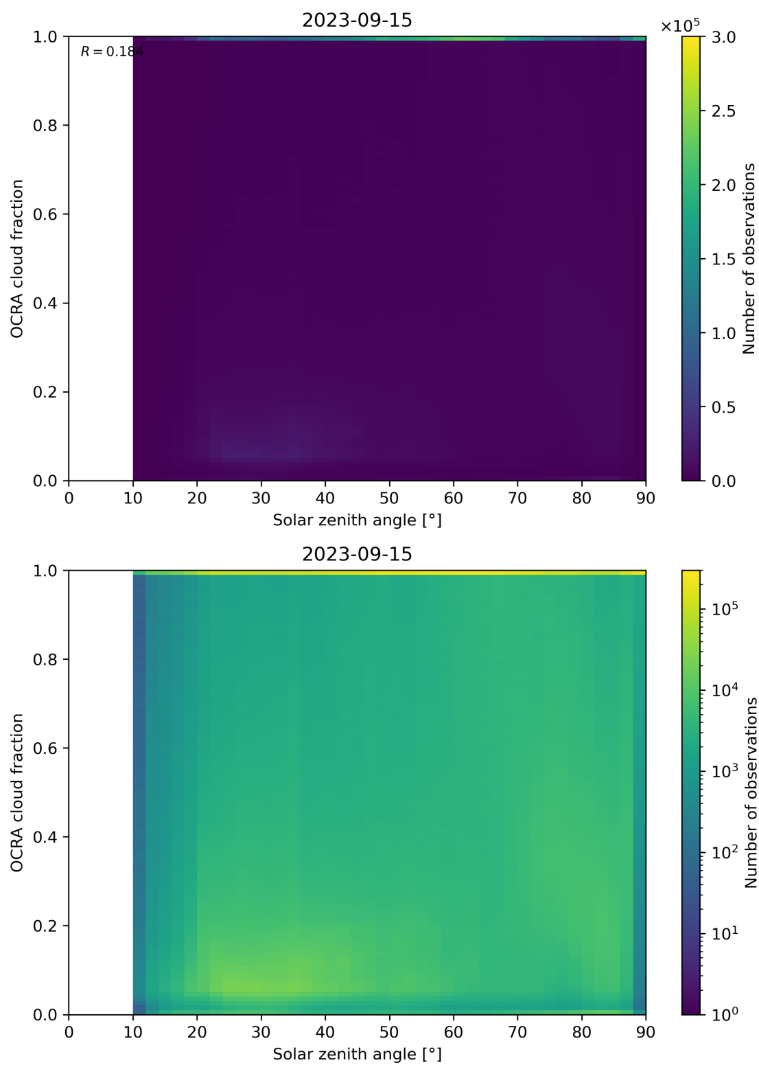
Figure 100: Scatter density plot of “Solar zenith angle” against “OCRA cloud fraction” for 2023-09-15 to 2023-09-16.
