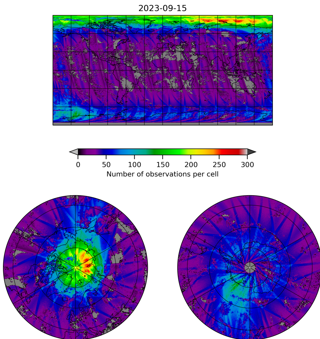
Figure 21: Map of the number of observations for 2023-09-15 to 2023-09-16
