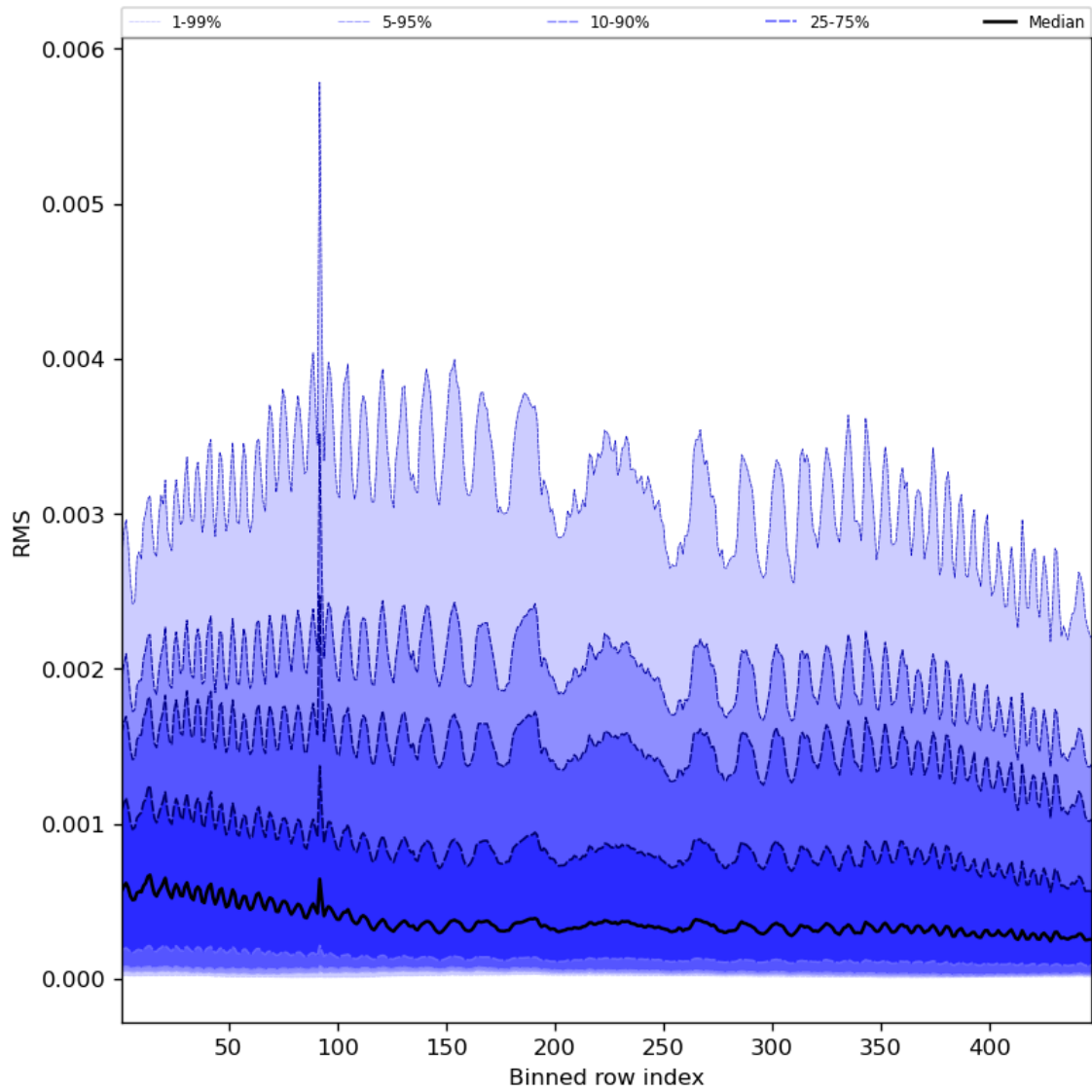
Figure 63: Along track statistics of “RMS” for 2023-09-15 to 2023-09-16
