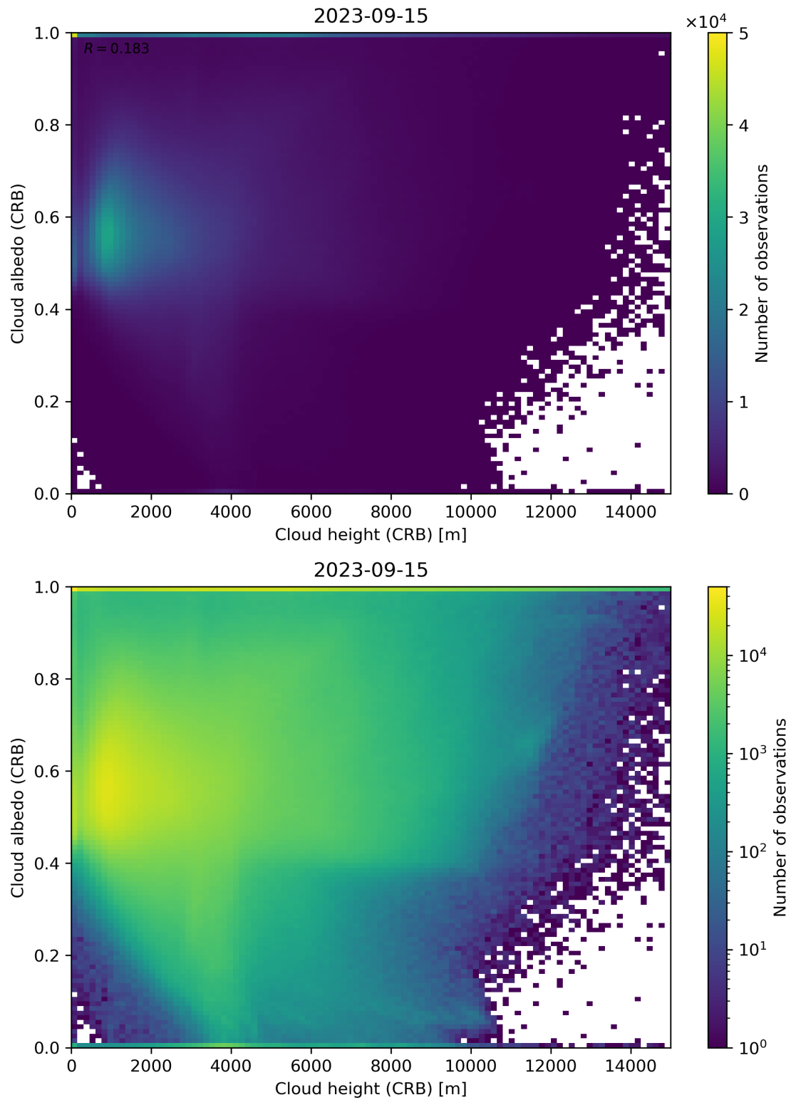
Figure 80: Scatter density plot of “Cloud height (CRB)” against “Cloud albedo (CRB)” for 2023-09-15 to 2023-09-16.
