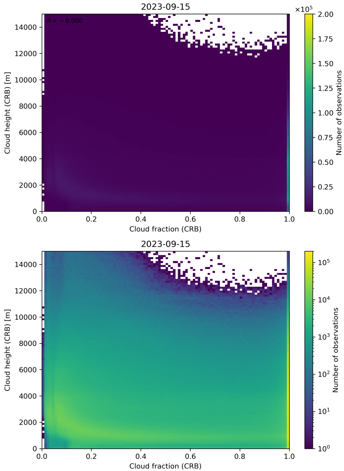
Figure 79: Scatter density plot of “Cloud fraction (CRB)” against “Cloud height (CRB)” for 2023-09-15 to 2023-09-16.
