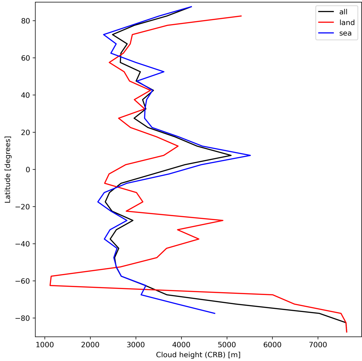
Figure 27: Zonal average of “Cloud height (CRB)” for 2023-09-15 to 2023-09-16.
