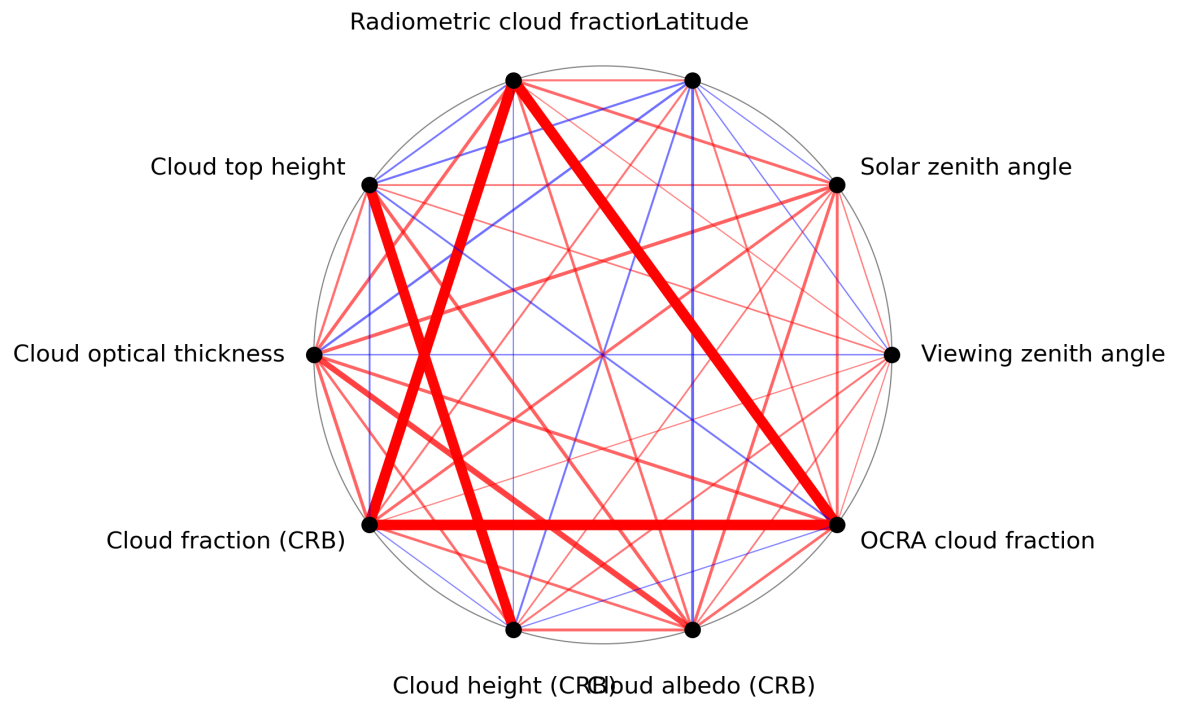
Figure 1: Map of correlation graph for 2023-09-15 to 2023-09-16.
