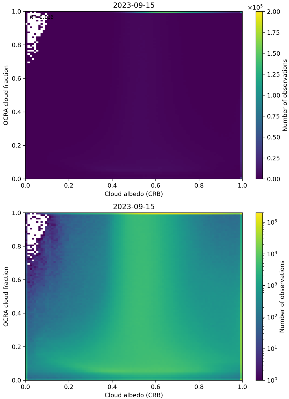
Figure 70: Scatter density plot of “Cloud albedo (CRB)” against “OCRA cloud fraction” for 2023-09-15 to 2023-09-16.
