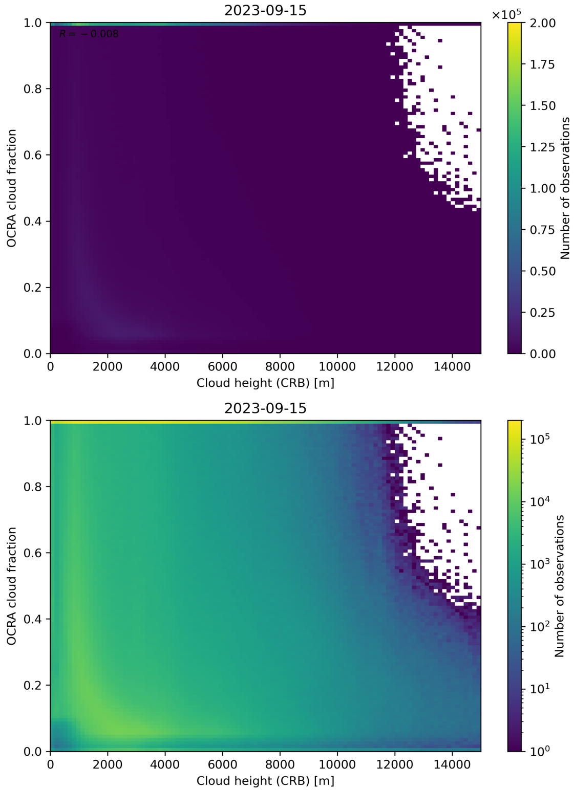
Figure 81: Scatter density plot of “Cloud height (CRB)” against “OCRA cloud fraction” for 2023-09-15 to 2023-09-16.
