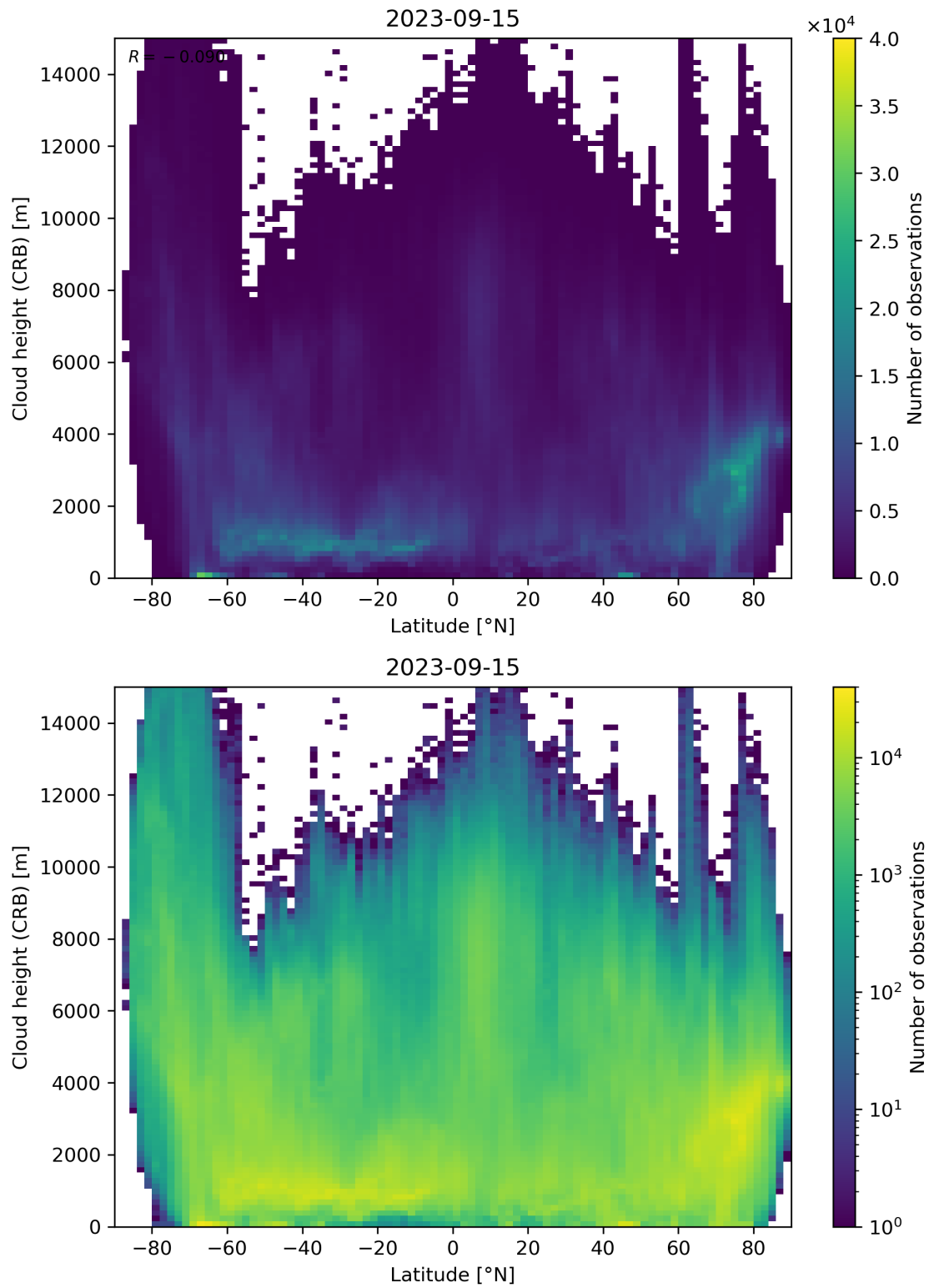
Figure 95: Scatter density plot of “Latitude” against “Cloud height (CRB)” for 2023-09-15 to 2023-09-16.
