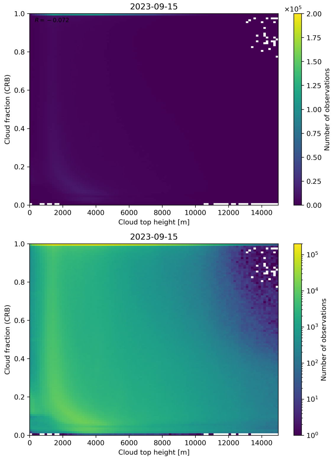
Figure 88: Scatter density plot of “Cloud top height” against “Cloud fraction (CRB)” for 2023-09-15 to 2023-09-16.
