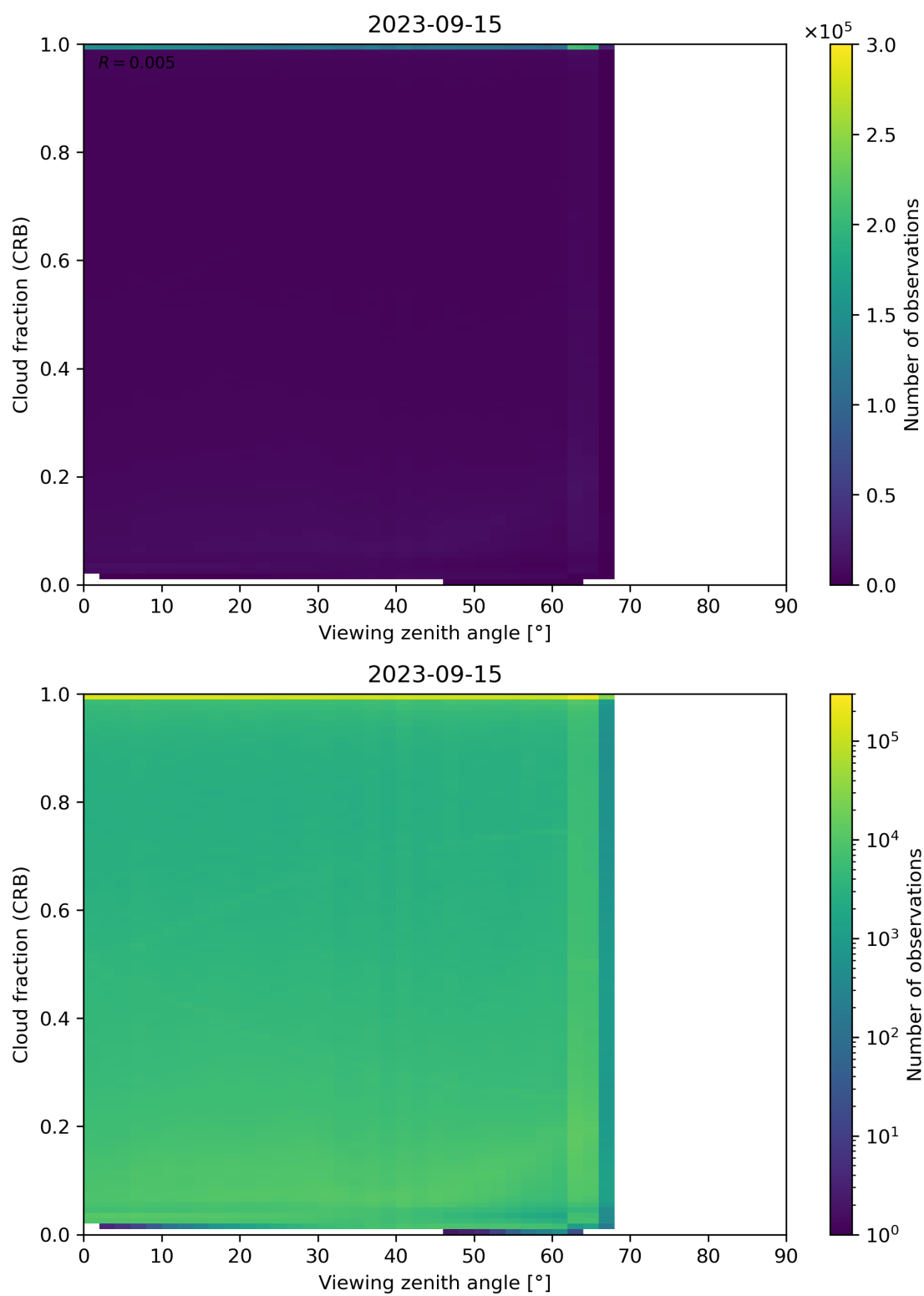
Figure 109: Scatter density plot of “Viewing zenith angle” against “Cloud fraction (CRB)” for 2023-09-15 to 2023-09-16.
