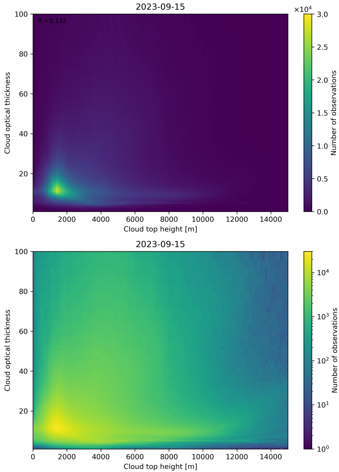
Figure 90: Scatter density plot of “Cloud top height” against “Cloud optical thickness” for 2023-09-15 to 2023-09-16.
