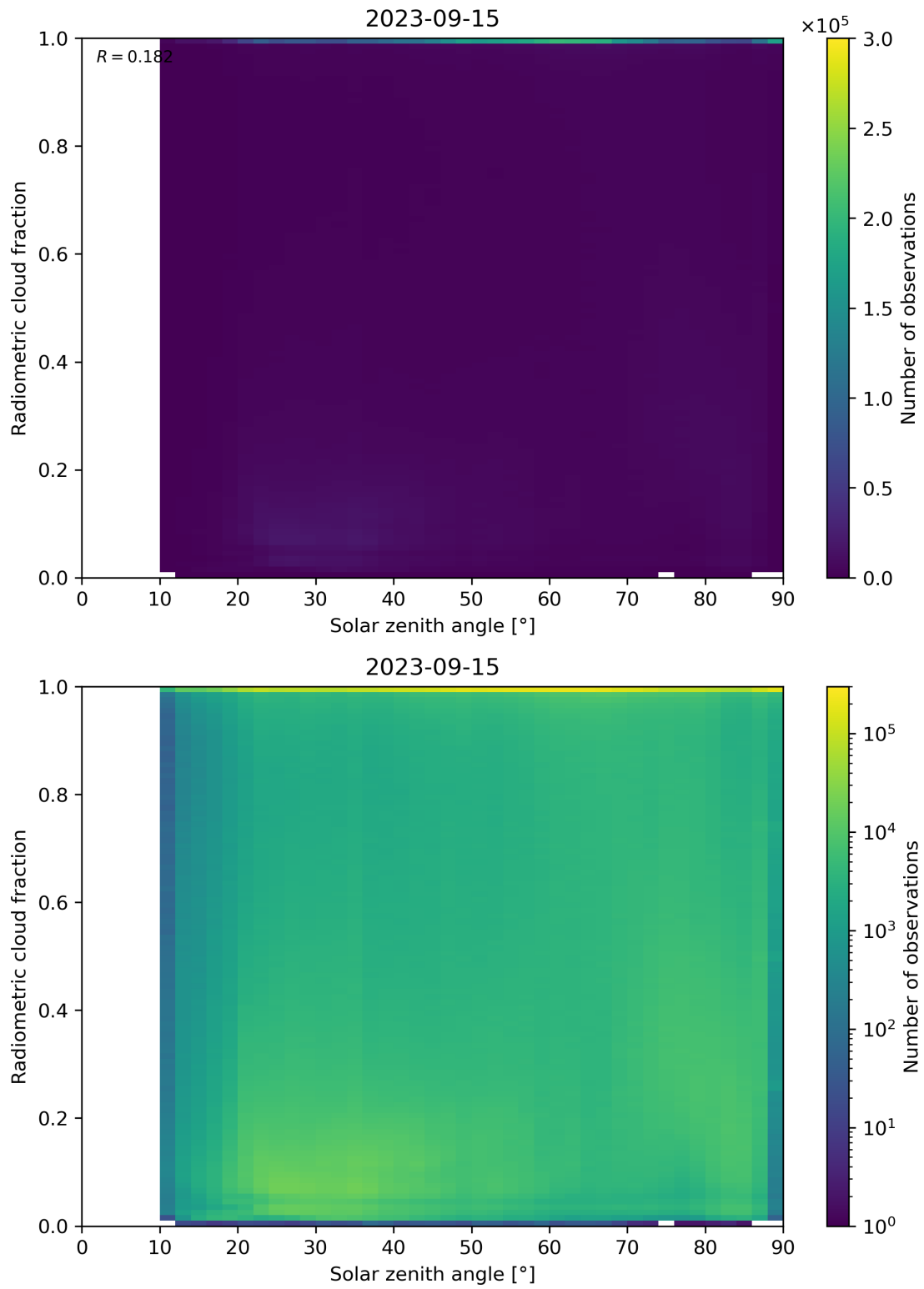
Figure 99: Scatter density plot of “Solar zenith angle” against “Radiometric cloud fraction” for 2023-09-15 to 2023-09-16.
