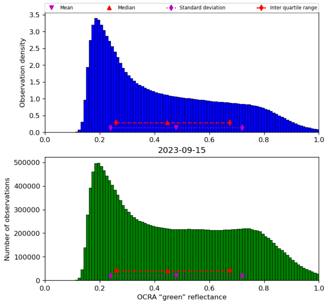
Figure 52: Histogram of “OCRA “green” reflectance” for 2023-09-15 to 2023-09-16
