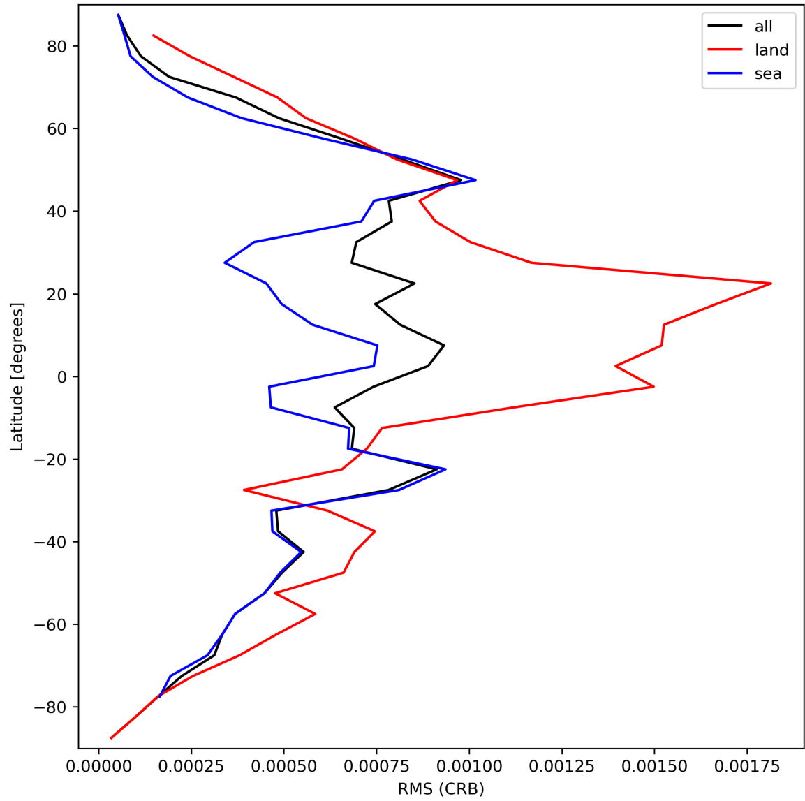
Figure 32: Zonal average of “RMS (CRB)” for 2023-09-15 to 2023-09-16.
