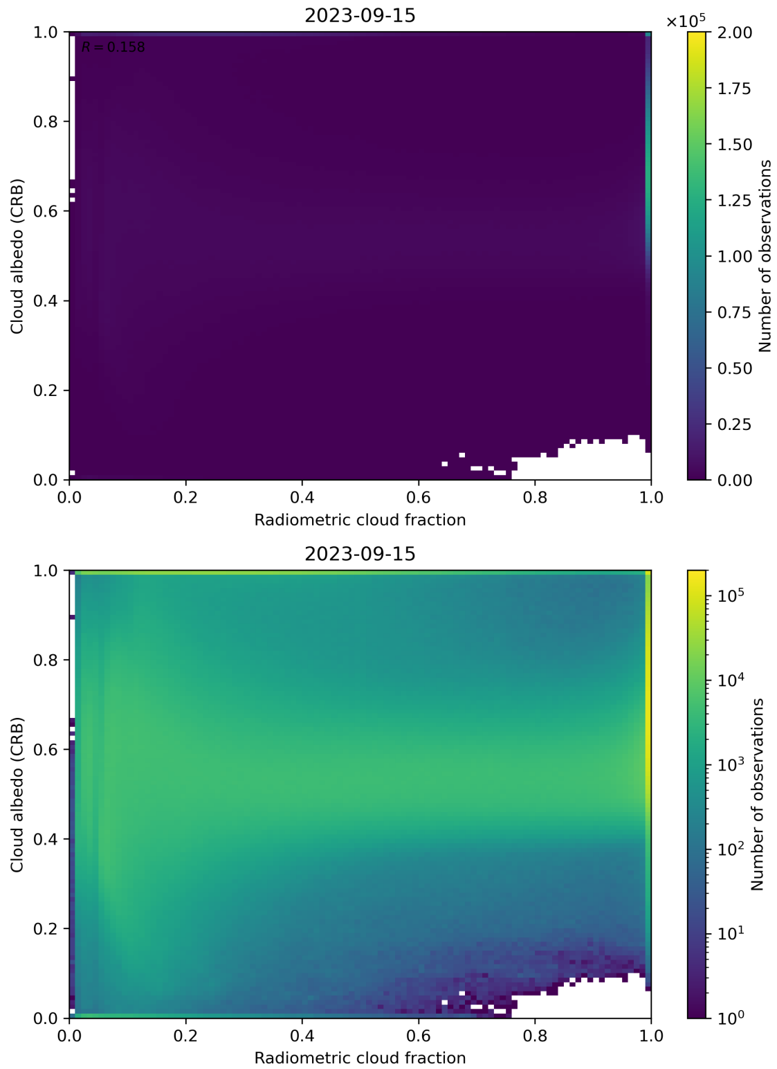
Figure 71: Scatter density plot of “Radiometric cloud fraction” against “Cloud albedo (CRB)” for 2023-09-15 to 2023-09-16.
