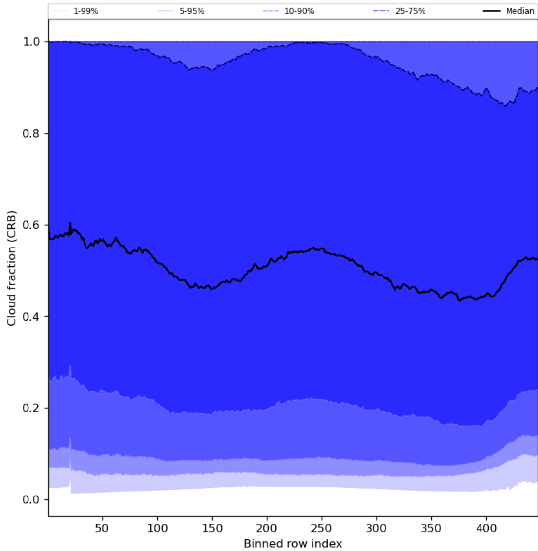
Figure 58: Along track statistics of “Cloud fraction (CRB)” for 2023-09-15 to 2023-09-16
