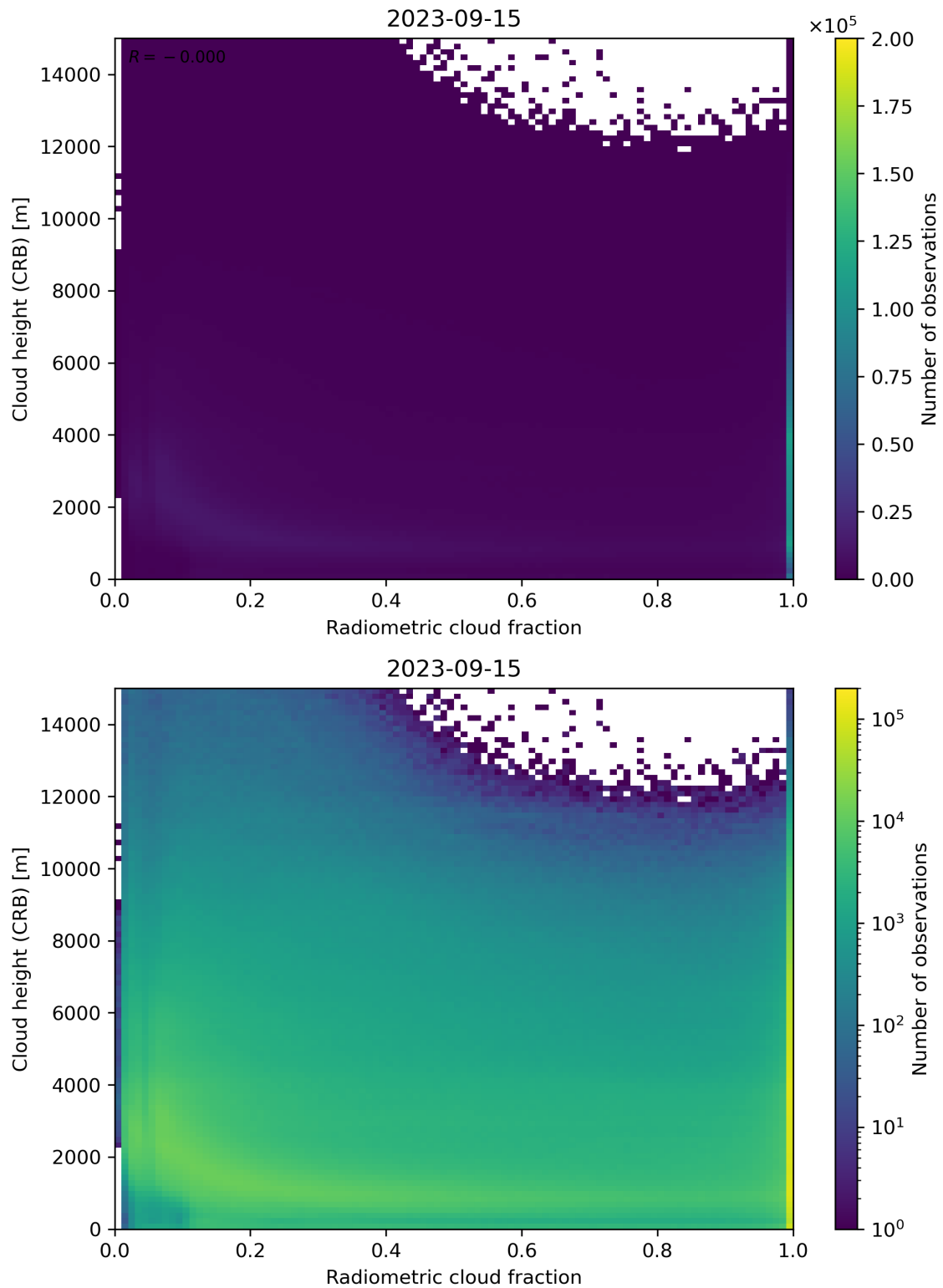
Figure 74: Scatter density plot of “Radiometric cloud fraction” against “Cloud height (CRB)” for 2023-09-15 to 2023-09-16.
