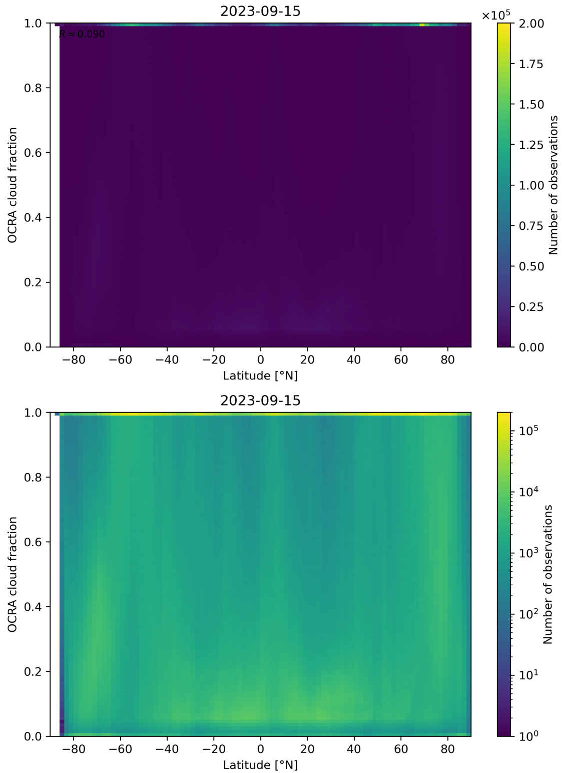
Figure 93: Scatter density plot of “Latitude” against “OCRA cloud fraction” for 2023-09-15 to 2023-09-16.
