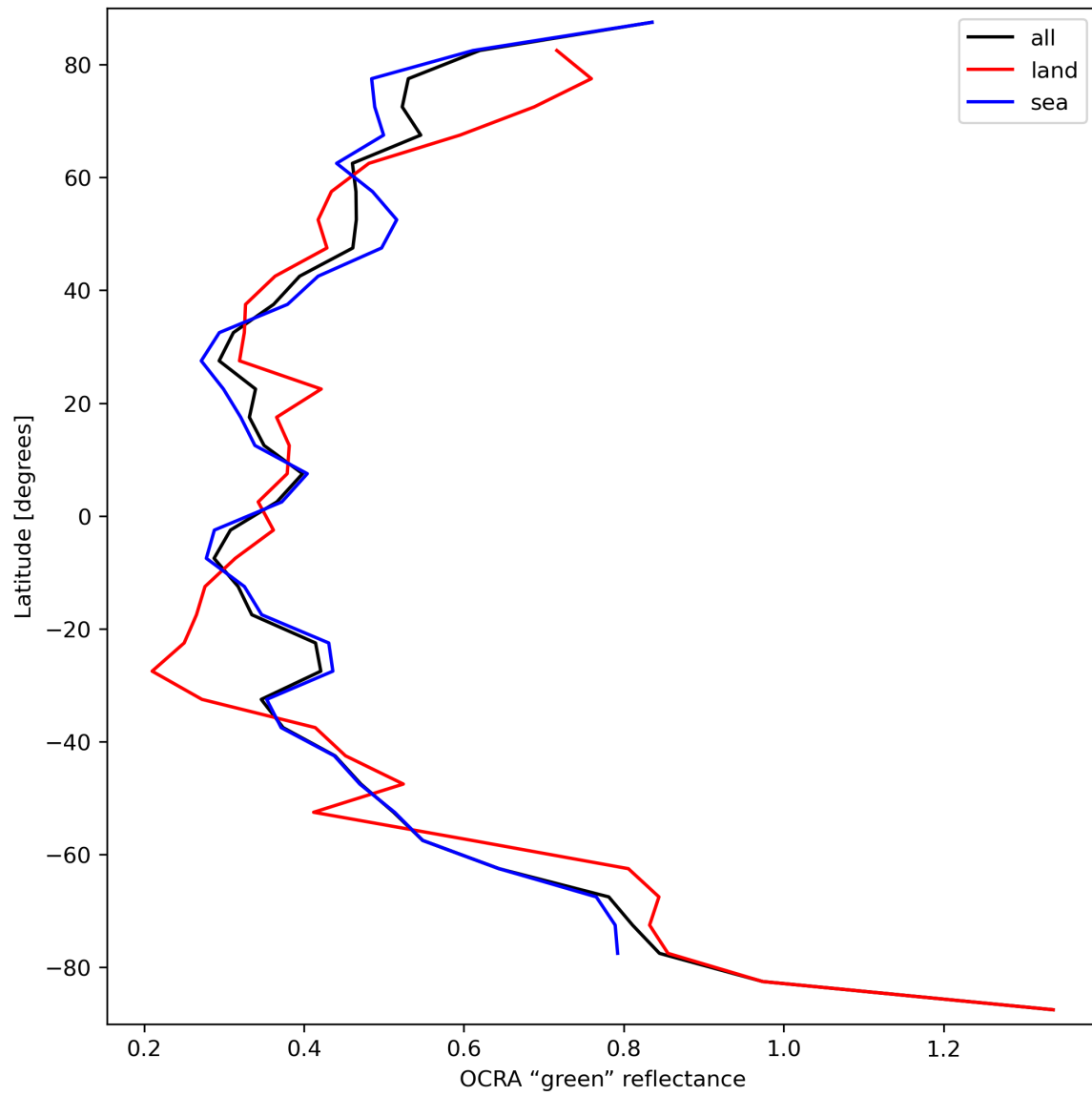
Figure 36: Zonal average of “OCRA “green” reflectance” for 2023-09-15 to 2023-09-16.
