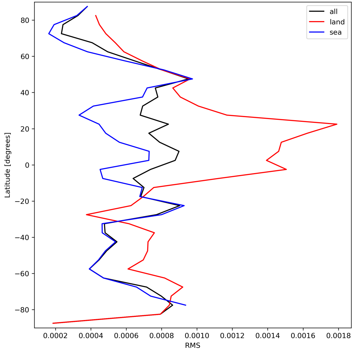
Figure 31: Zonal average of “RMS” for 2023-09-15 to 2023-09-16.
