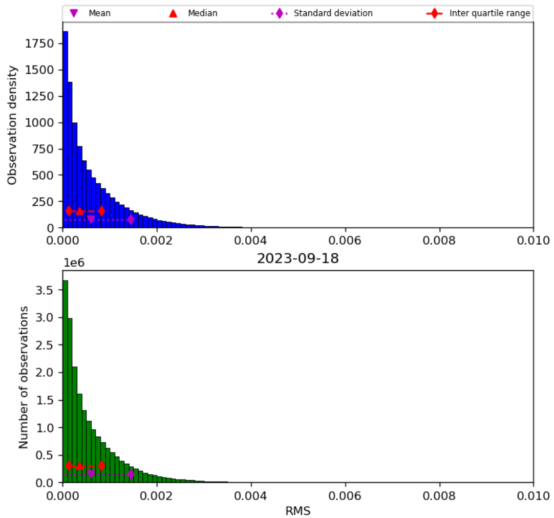
Figure 47: Histogram of “RMS” for 2023-09-17 to 2023-09-19
