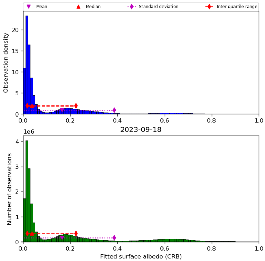
Figure 46: Histogram of “Fitted surface albedo (CRB)” for 2023-09-17 to 2023-09-19
