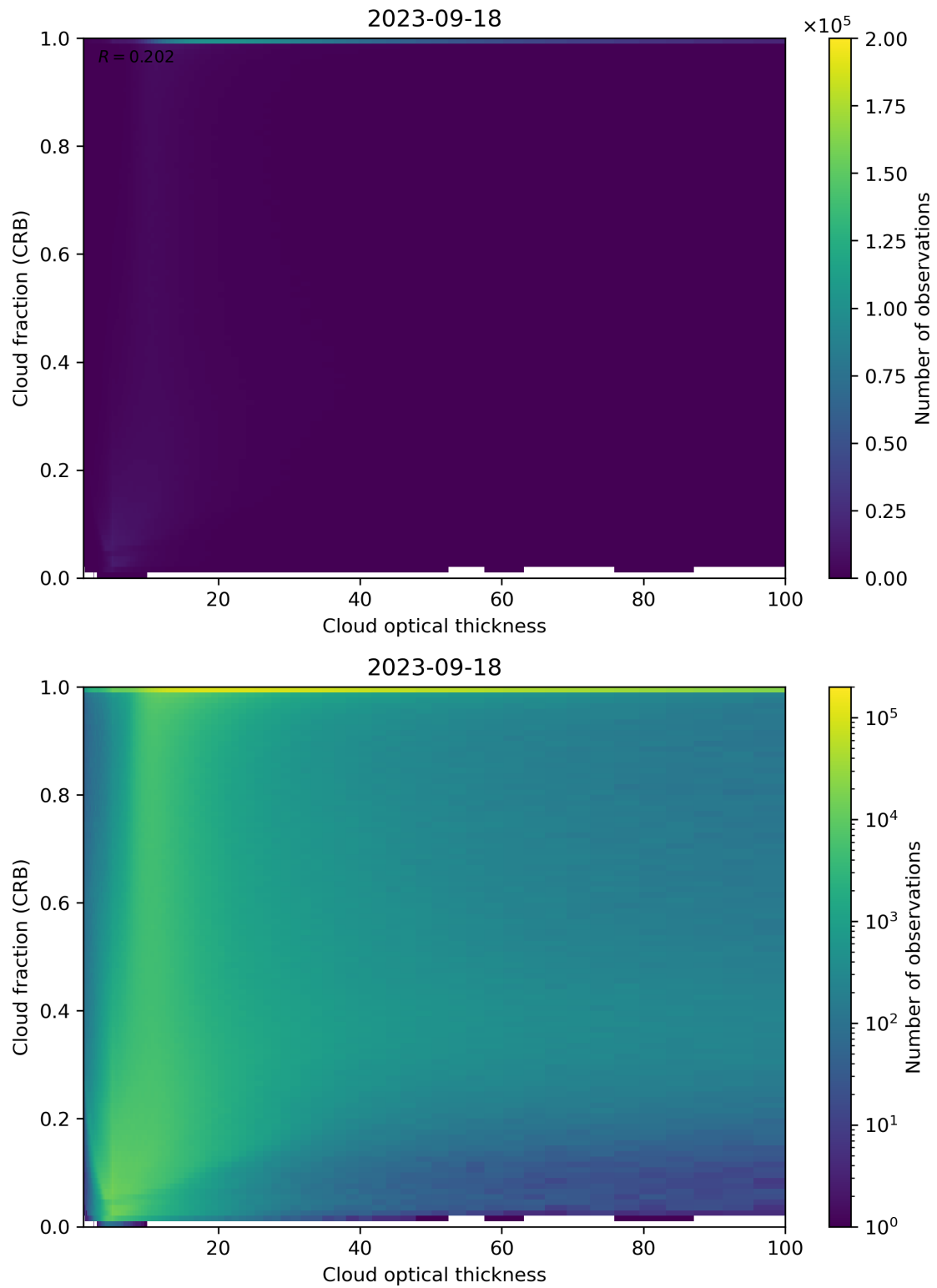
Figure 84: Scatter density plot of “Cloud optical thickness” against “Cloud fraction (CRB)” for 2023-09-17 to 2023-09-19.
