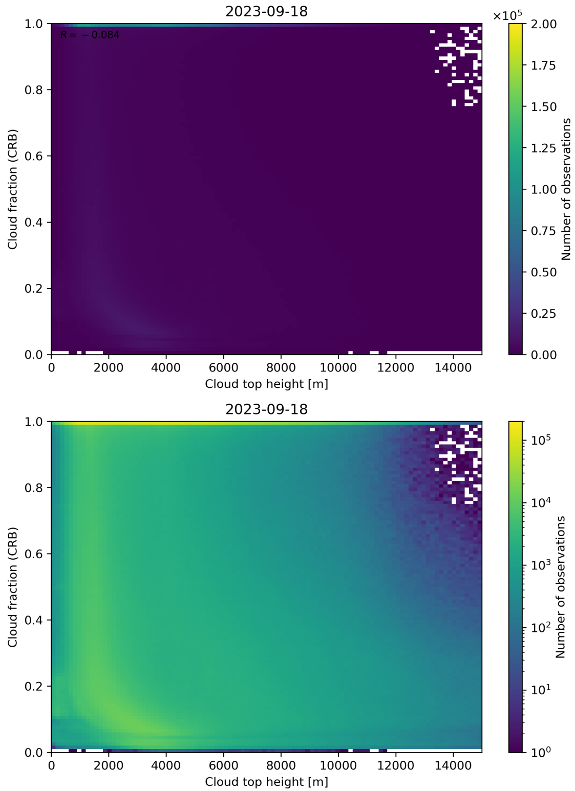
Figure 88: Scatter density plot of “Cloud top height” against “Cloud fraction (CRB)” for 2023-09-17 to 2023-09-19.
