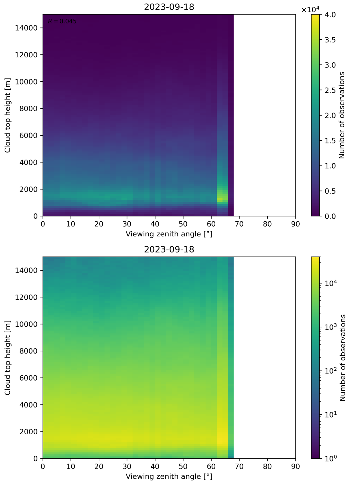
Figure 112: Scatter density plot of “Viewing zenith angle” against “Cloud top height” for 2023-09-17 to 2023-09-19.
