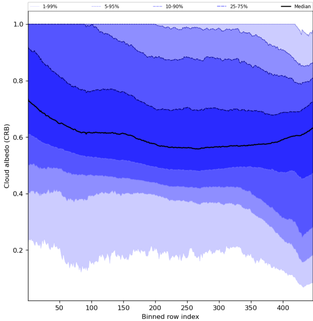
Figure 60: Along track statistics of “Cloud albedo (CRB)” for 2023-09-17 to 2023-09-19
