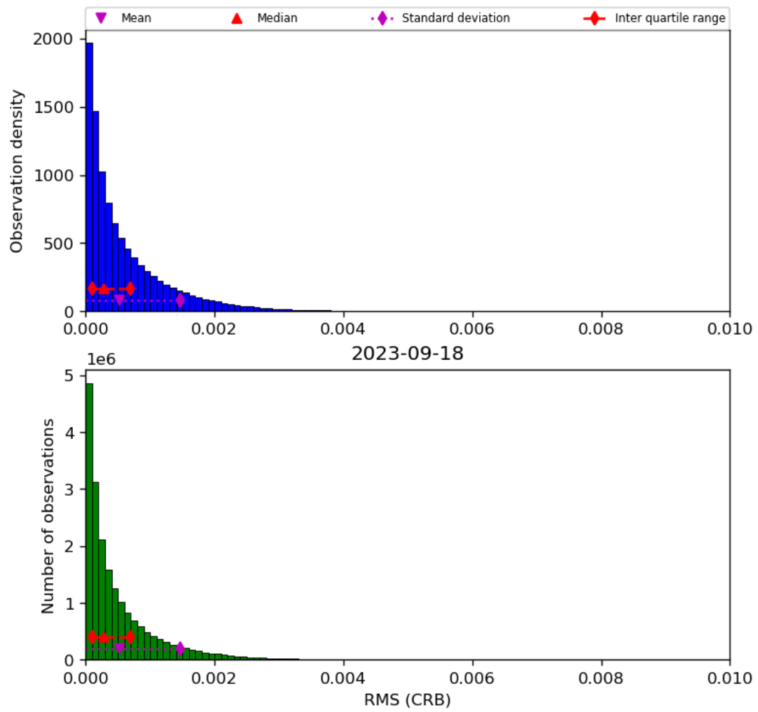
Figure 48: Histogram of “RMS (CRB)” for 2023-09-17 to 2023-09-19
