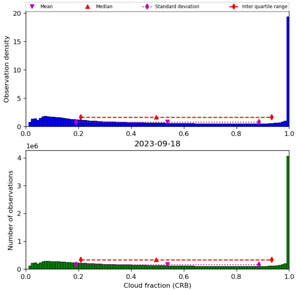
Figure 42: Histogram of “Cloud fraction (CRB)” for 2023-09-17 to 2023-09-19
