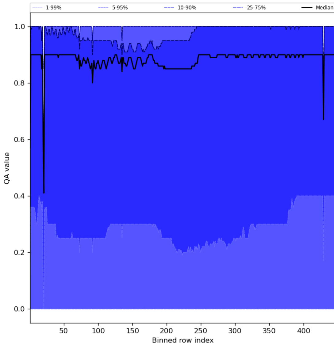
Figure 54: Along track statistics of “QA value” for 2023-09-17 to 2023-09-19
