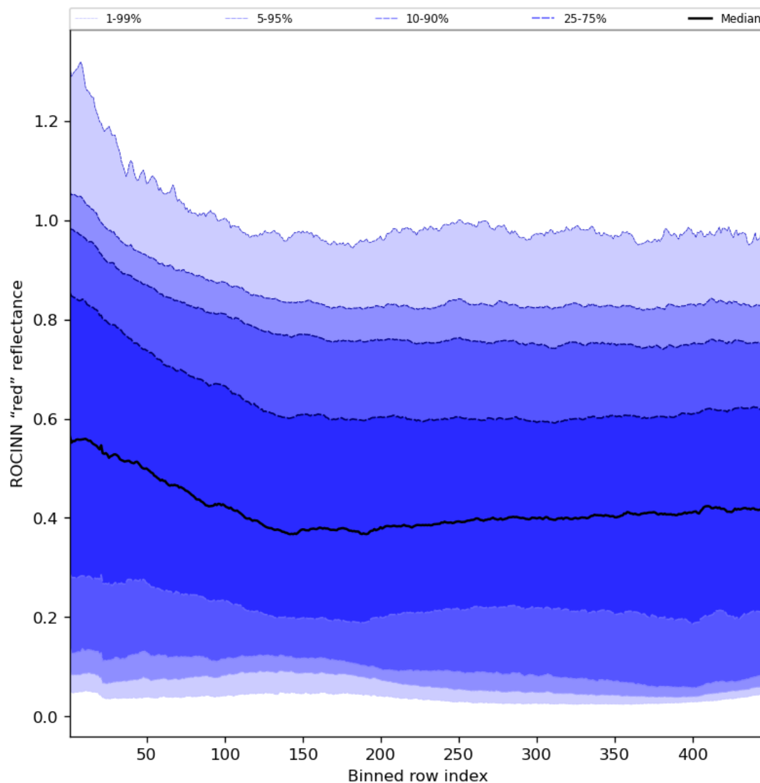
Figure 69: Along track statistics of “ROCINN “red” reflectance” for 2023-09-17 to 2023-09-19
