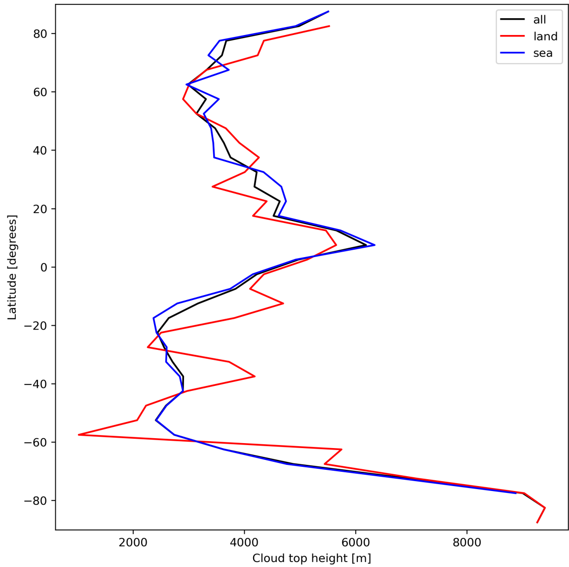
Figure 24: Zonal average of “Cloud top height” for 2023-09-17 to 2023-09-19.
