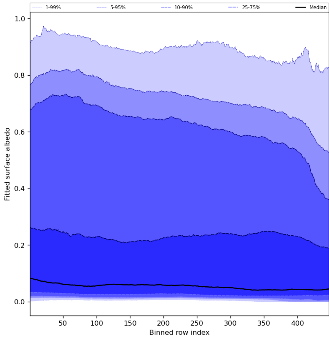
Figure 61: Along track statistics of “Fitted surface albedo” for 2023-09-17 to 2023-09-19
