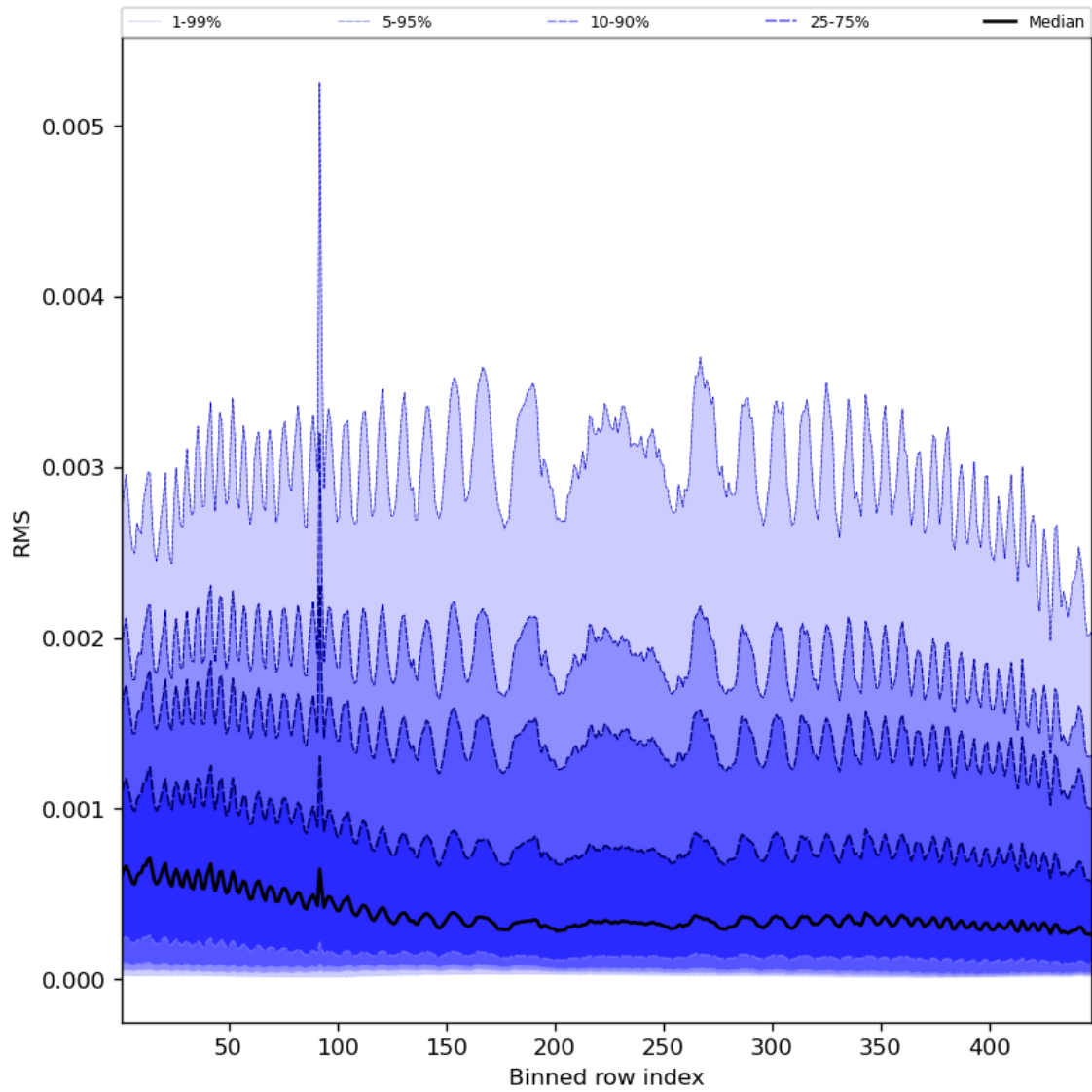
Figure 63: Along track statistics of “RMS” for 2023-09-17 to 2023-09-19
