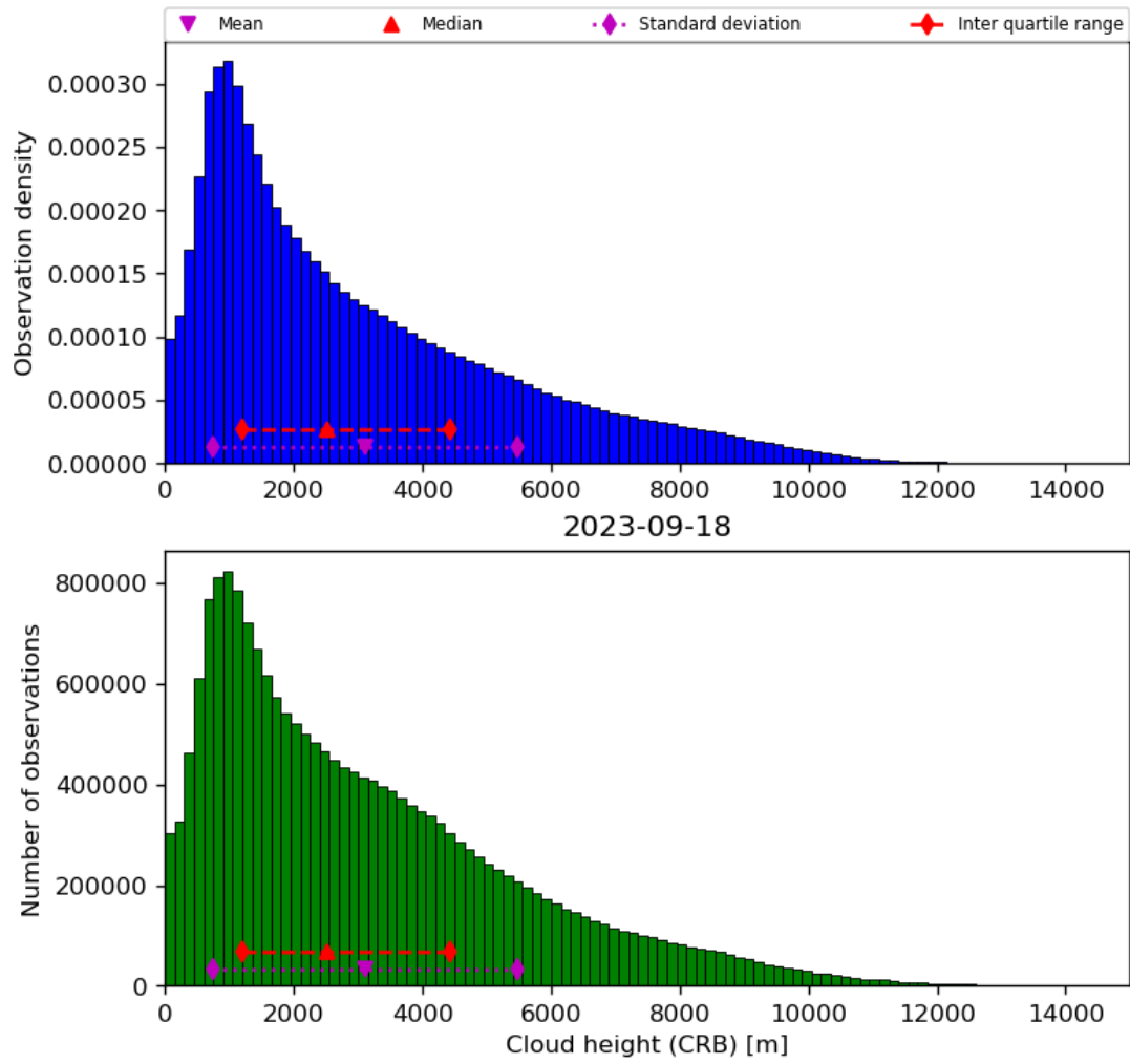
Figure 43: Histogram of “Cloud height (CRB)” for 2023-09-17 to 2023-09-19
