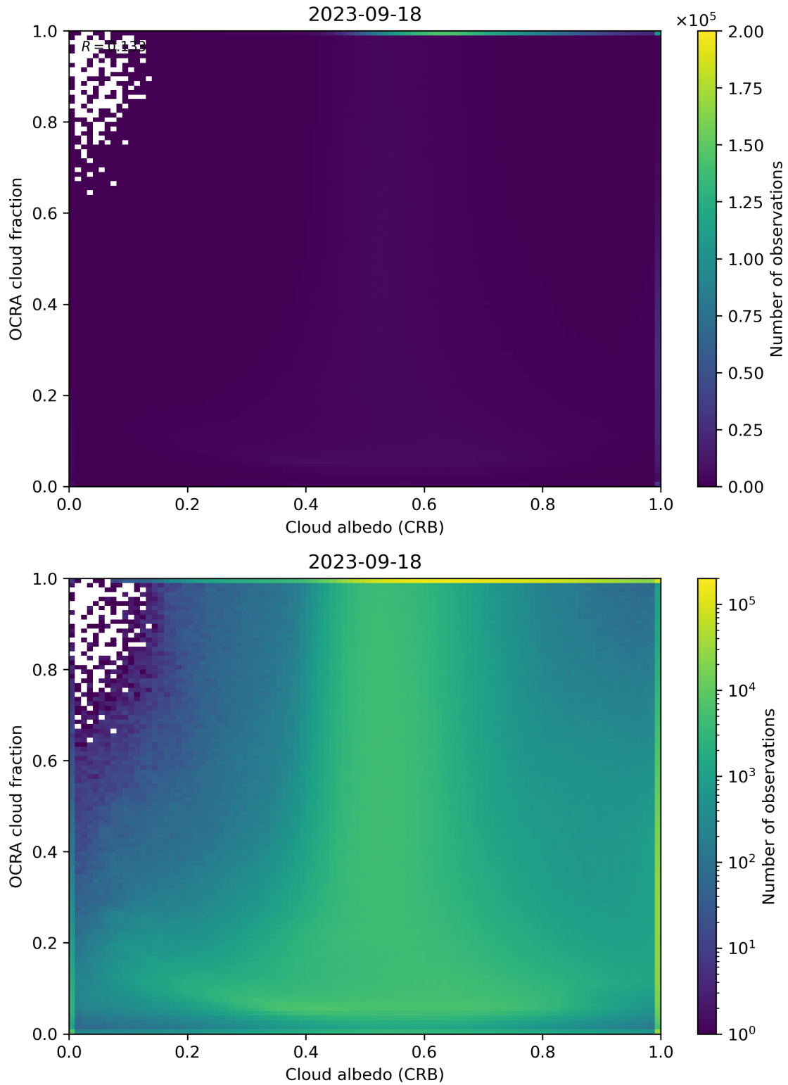
Figure 70: Scatter density plot of “Cloud albedo (CRB)” against “OCRA cloud fraction” for 2023-09-17 to 2023-09-19.
