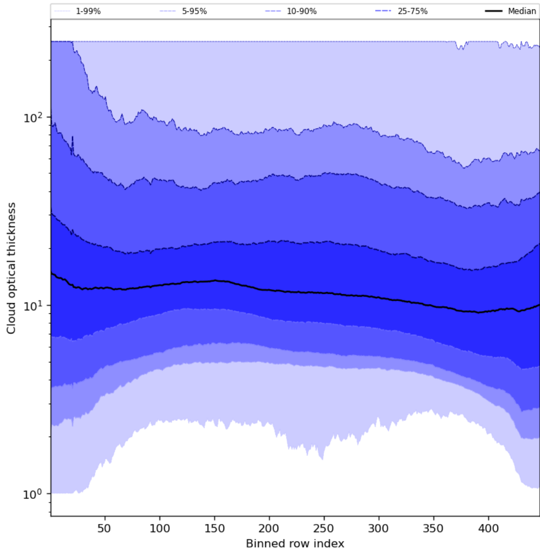
Figure 57: Along track statistics of “Cloud optical thickness” for 2023-09-17 to 2023-09-19
