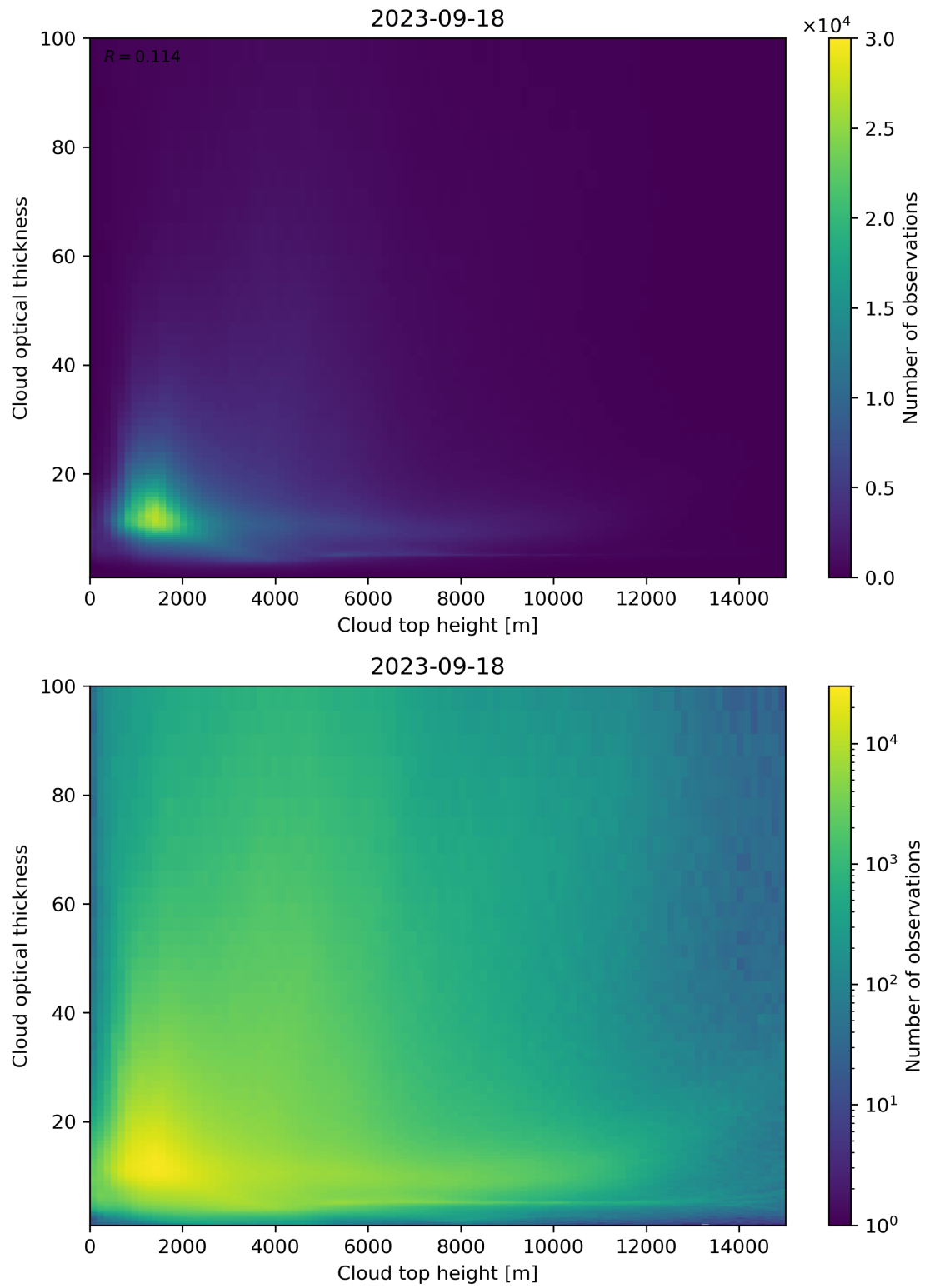
Figure 90: Scatter density plot of “Cloud top height” against “Cloud optical thickness” for 2023-09-17 to 2023-09-19.
