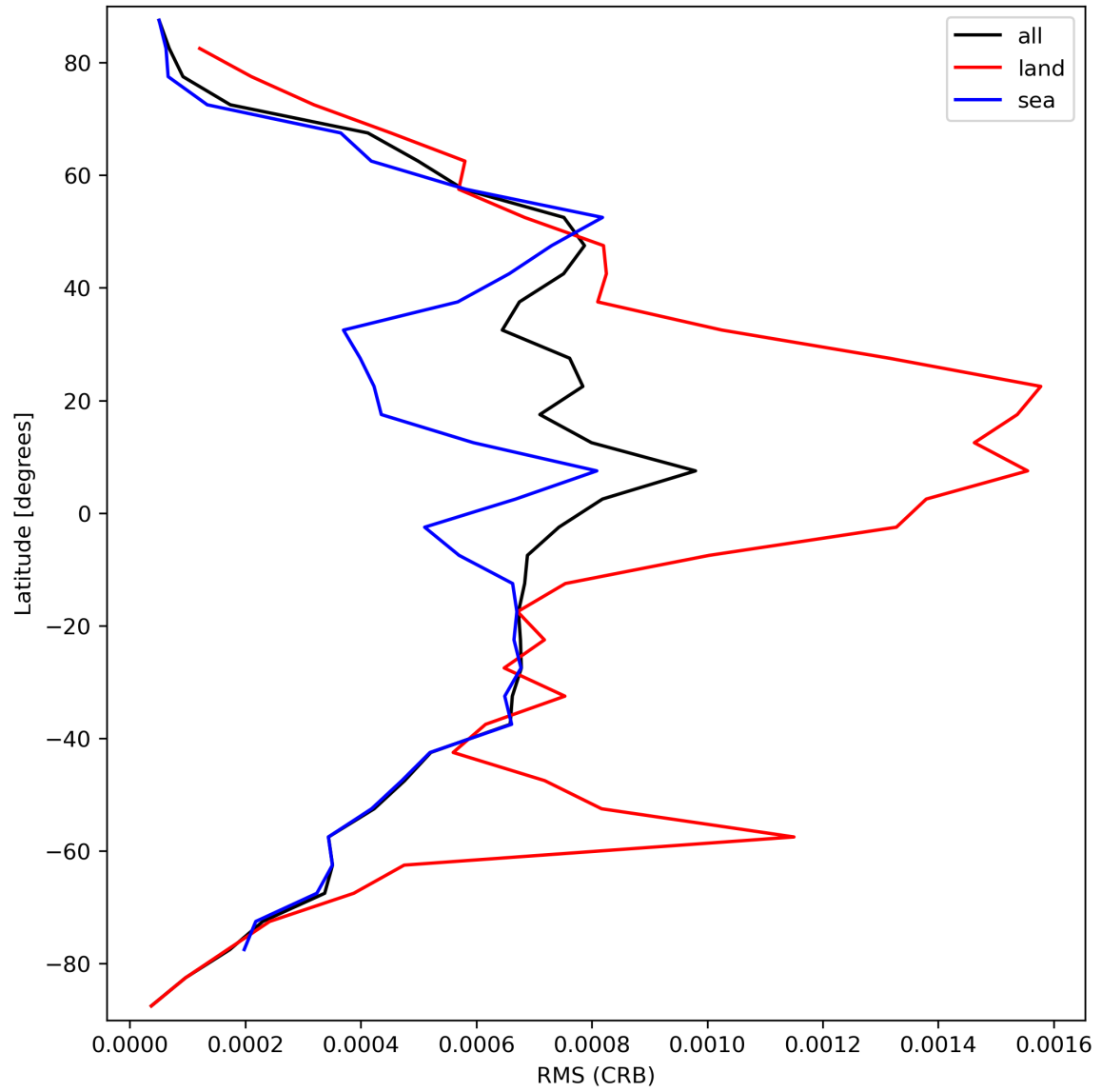
Figure 32: Zonal average of “RMS (CRB)” for 2023-09-17 to 2023-09-19.
