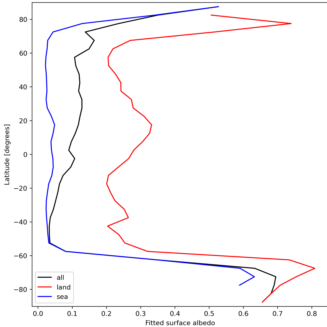
Figure 29: Zonal average of “Fitted surface albedo” for 2023-09-17 to 2023-09-19.
