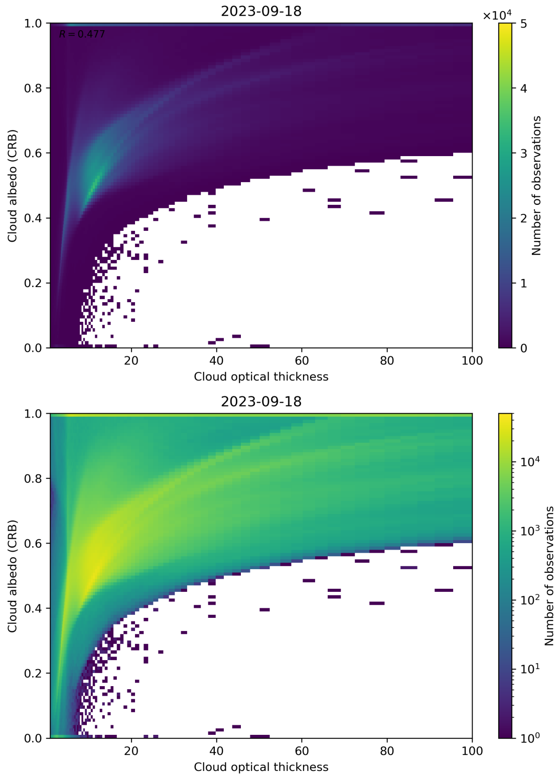
Figure 82: Scatter density plot of “Cloud optical thickness” against “Cloud albedo (CRB)” for 2023-09-17 to 2023-09-19.
