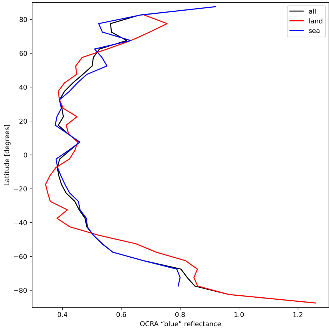
Figure 35: Zonal average of “OCRA “blue” reflectance” for 2023-09-17 to 2023-09-19.
