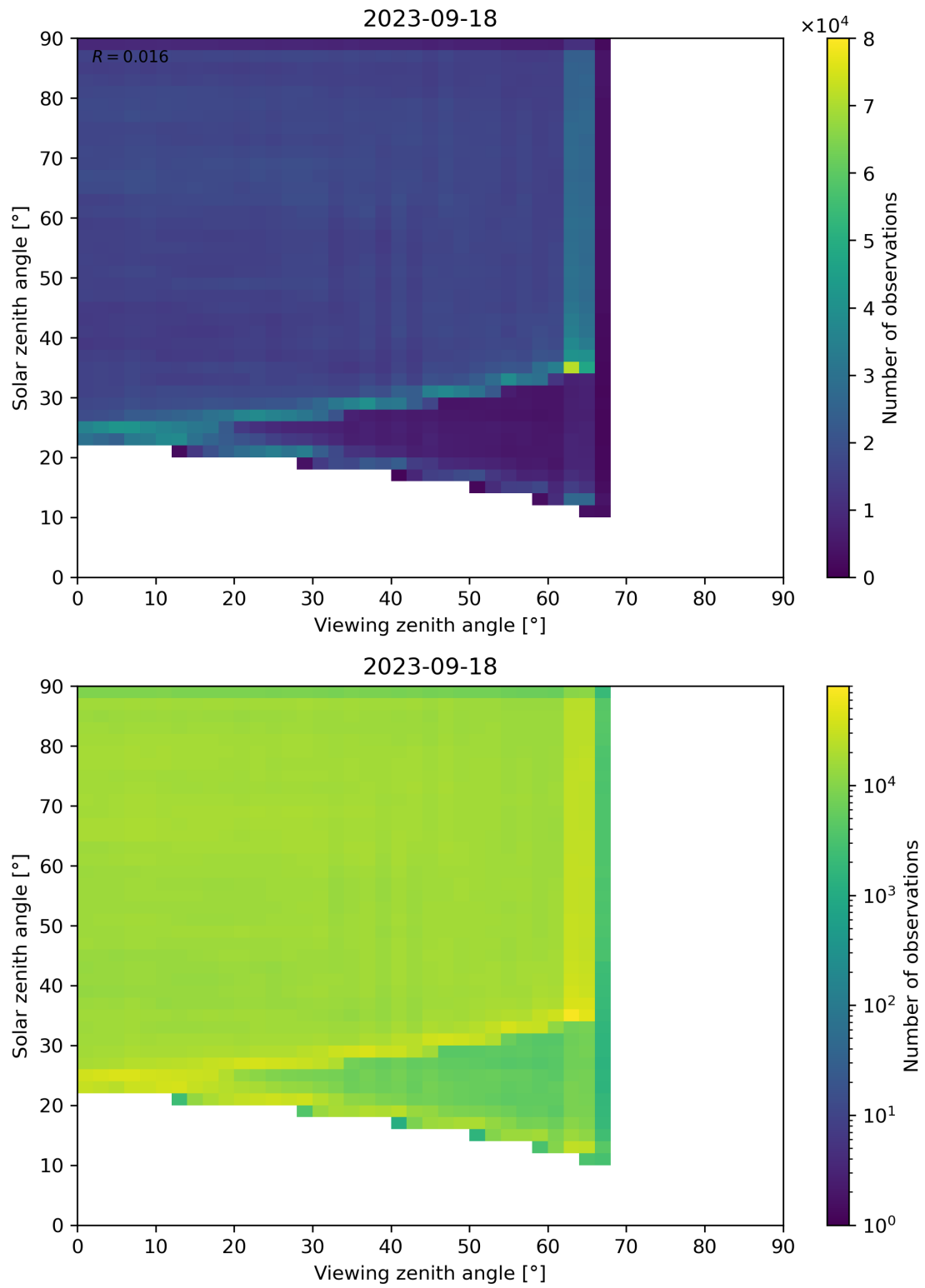
Figure 114: Scatter density plot of “Viewing zenith angle” against “Solar zenith angle” for 2023-09-17 to 2023-09-19.
