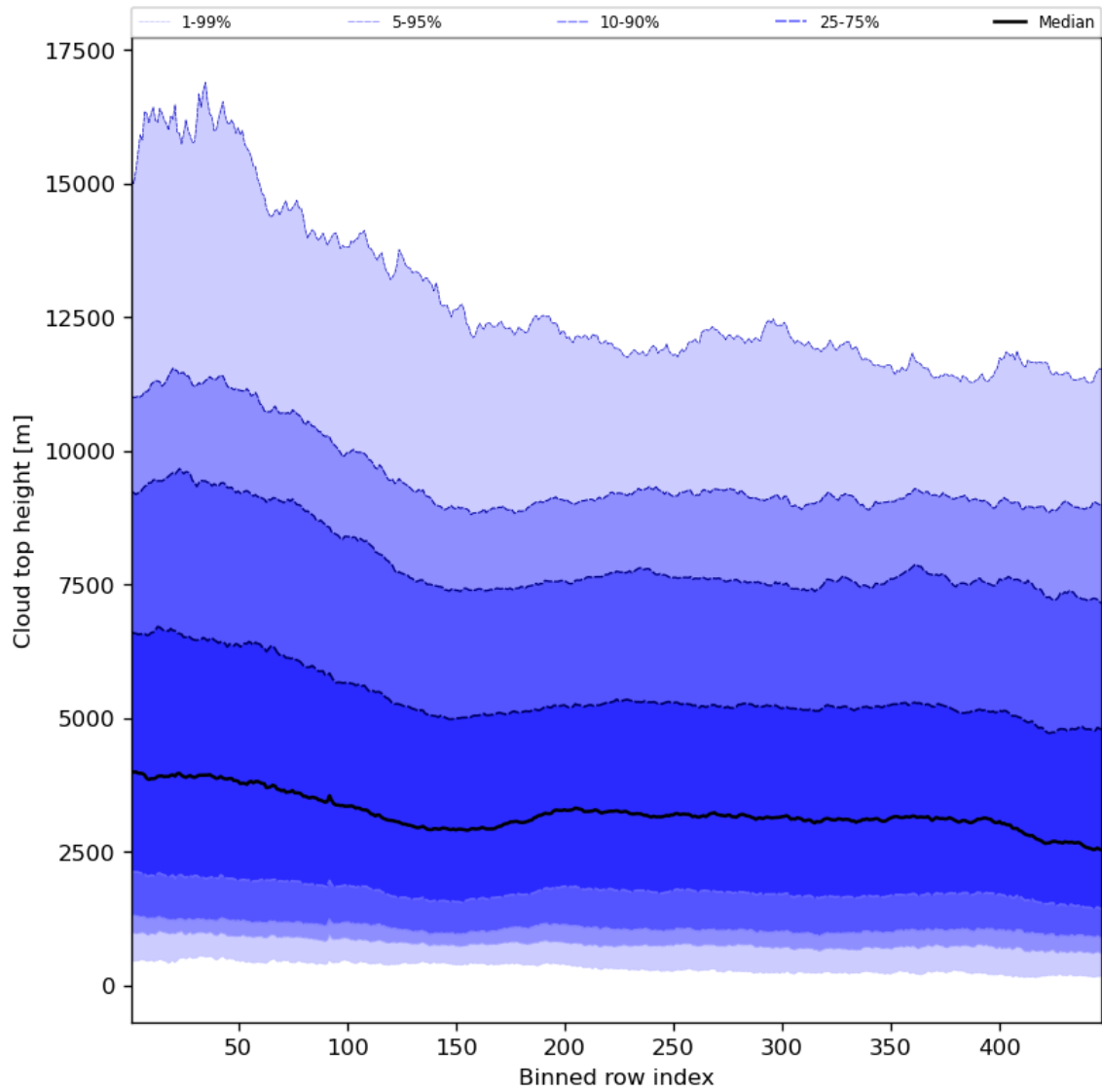
Figure 56: Along track statistics of “Cloud top height” for 2023-09-17 to 2023-09-19
