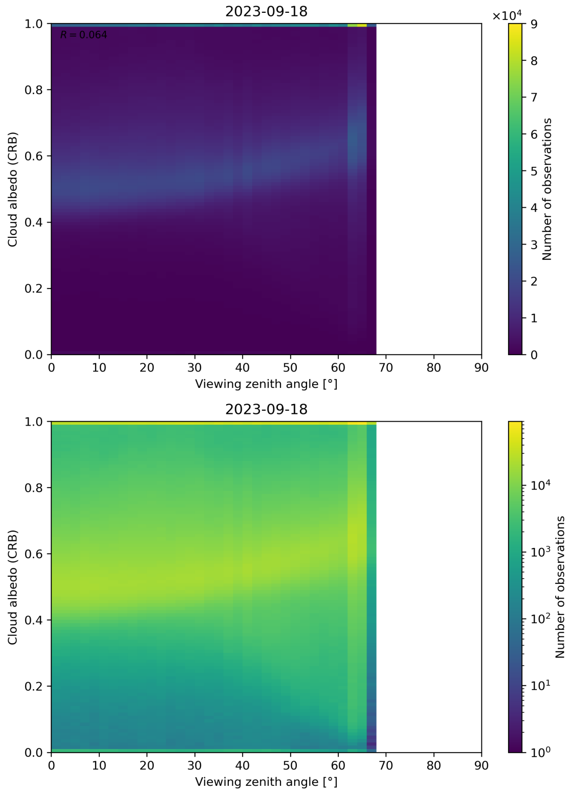
Figure 106: Scatter density plot of “Viewing zenith angle” against “Cloud albedo (CRB)” for 2023-09-17 to 2023-09-19.
