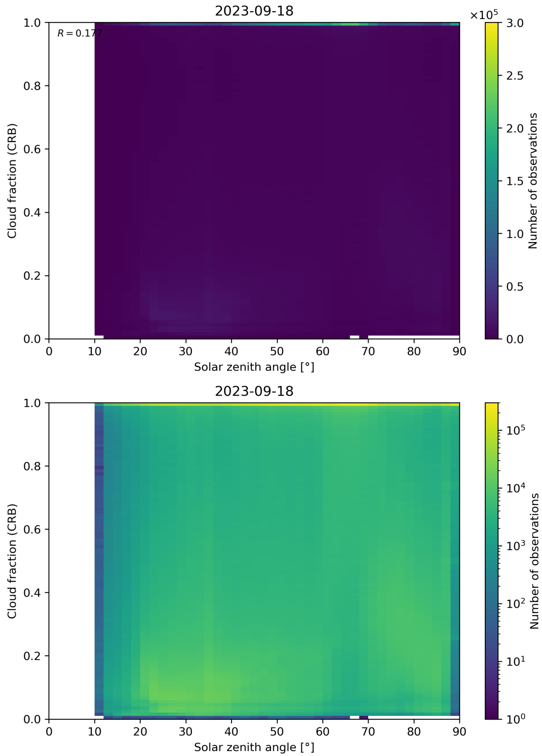
Figure 101: Scatter density plot of “Solar zenith angle” against “Cloud fraction (CRB)” for 2023-09-17 to 2023-09-19.
