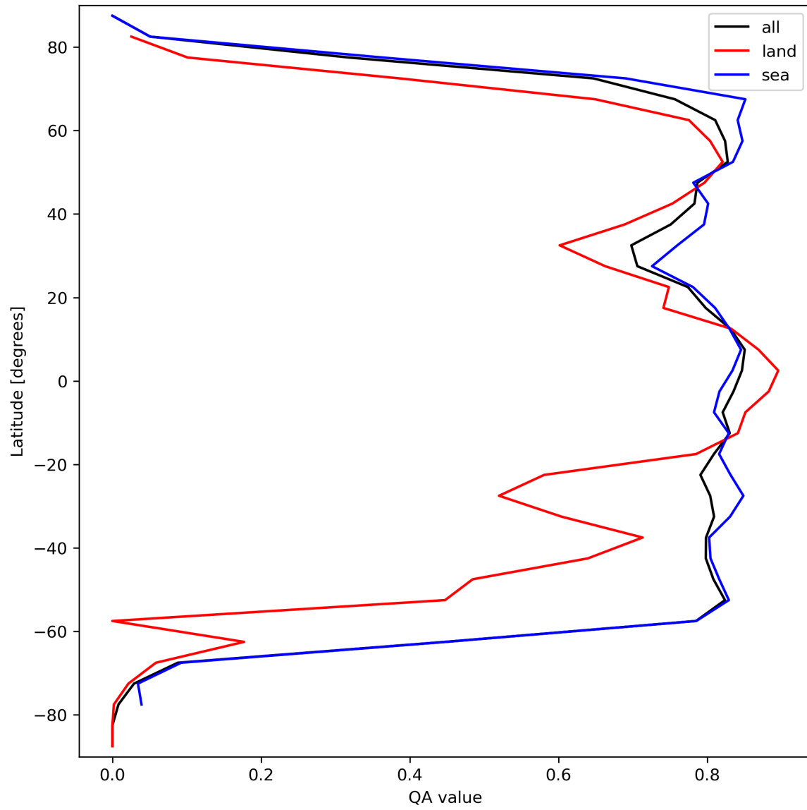
Figure 22: Zonal average of “QA value” for 2023-09-17 to 2023-09-19.
