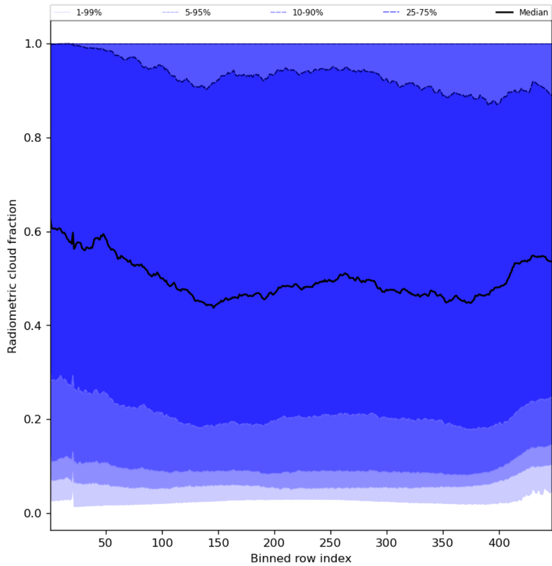
Figure 55: Along track statistics of “Radiometric cloud fraction” for 2023-09-17 to 2023-09-19
