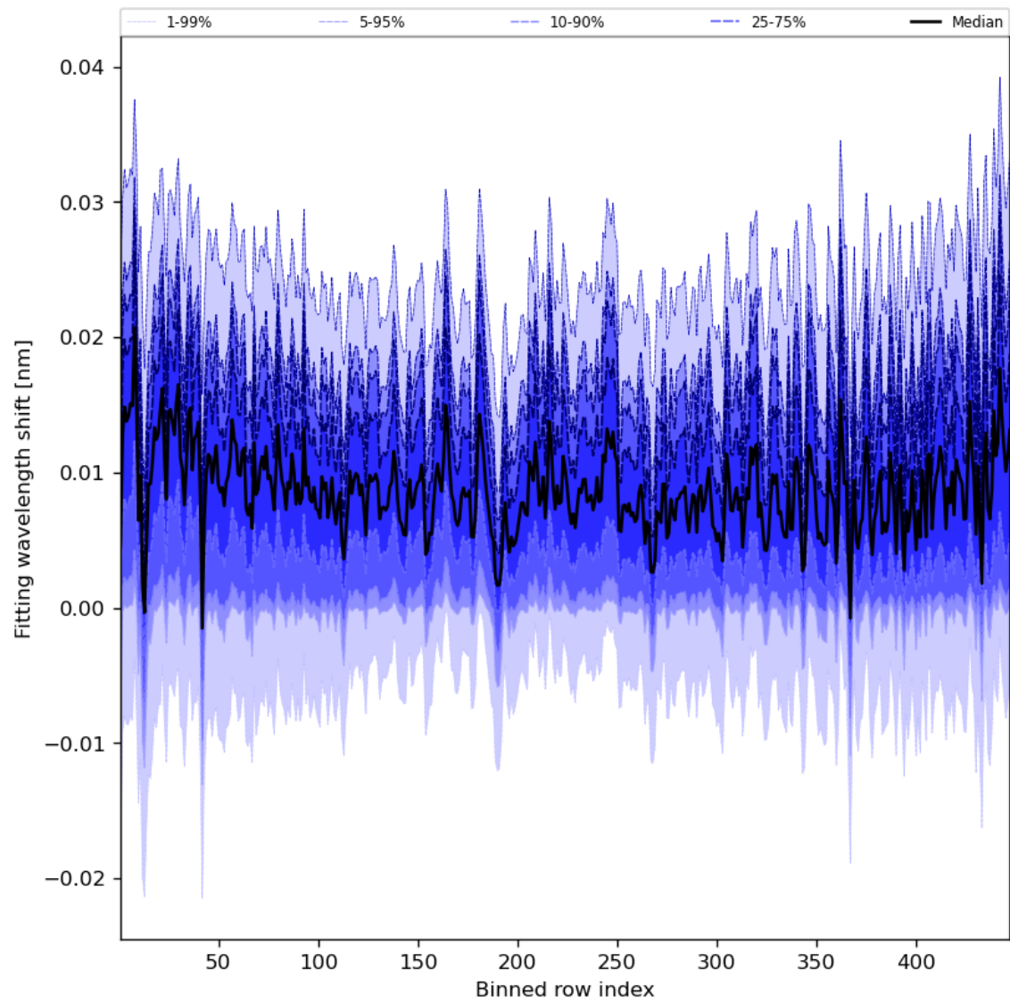
Figure 65: Along track statistics of “Fitting wavelength shift” for 2023-09-17 to 2023-09-19
