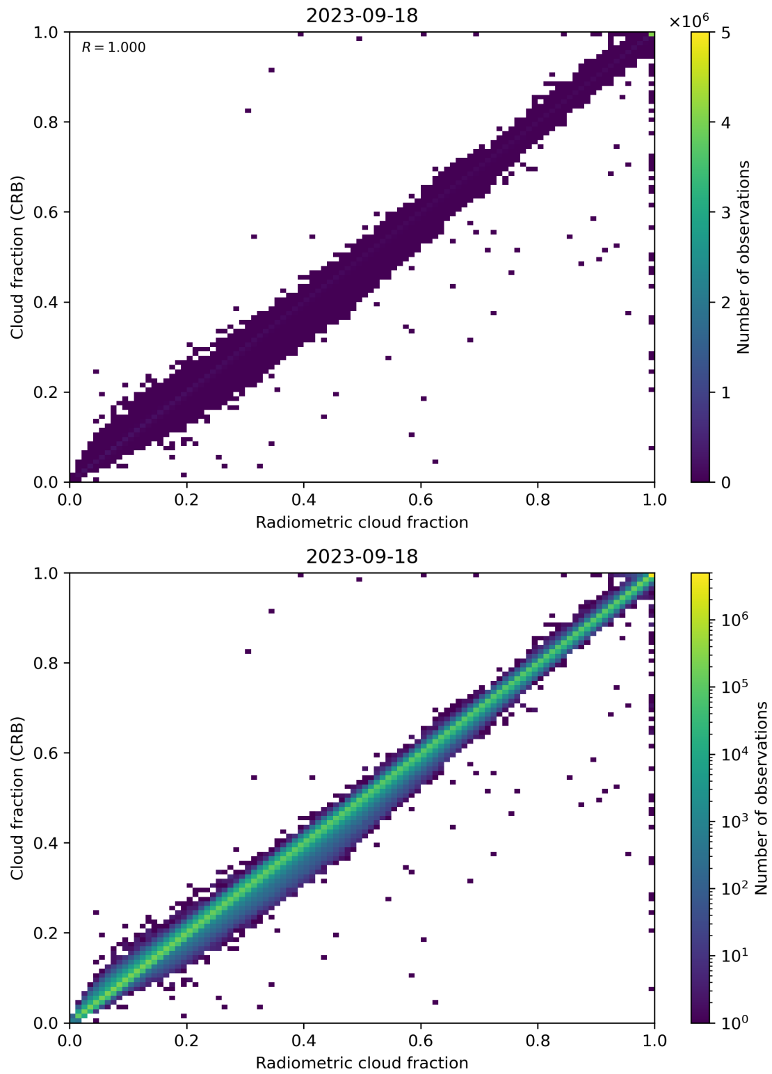
Figure 73: Scatter density plot of “Radiometric cloud fraction” against “Cloud fraction (CRB)” for 2023-09-17 to 2023-09-19.
