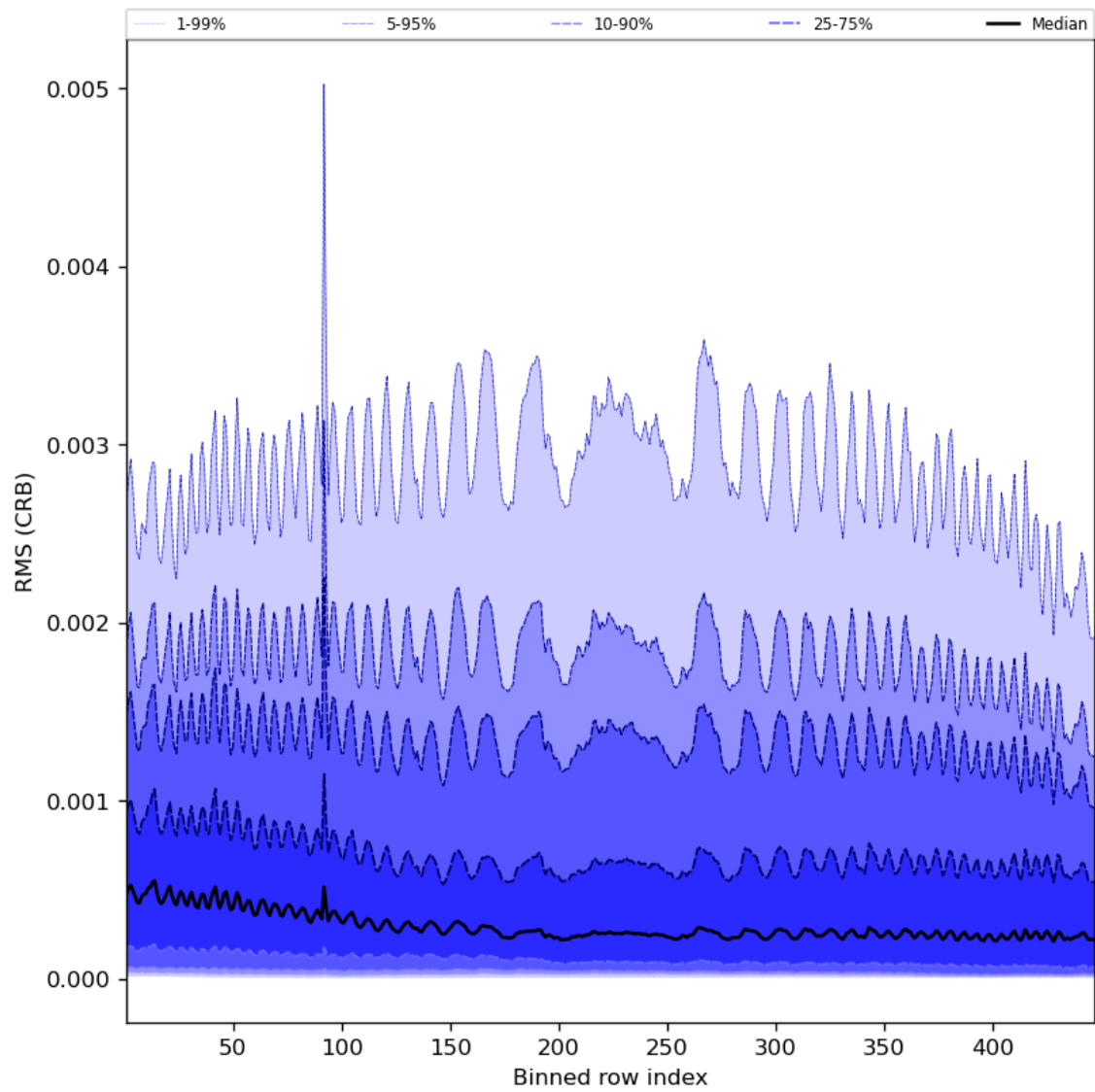
Figure 64: Along track statistics of “RMS (CRB)” for 2023-09-17 to 2023-09-19
