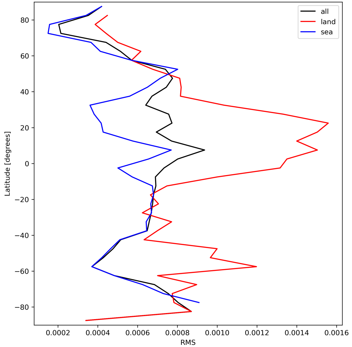
Figure 31: Zonal average of “RMS” for 2023-09-17 to 2023-09-19.
