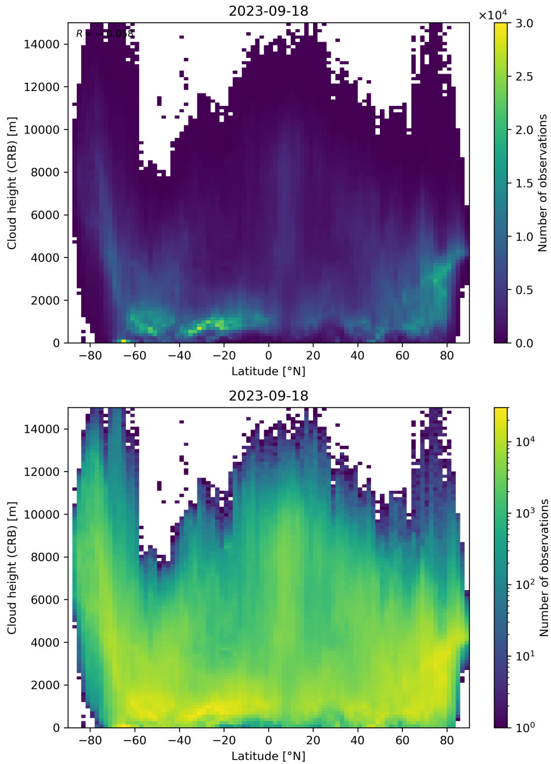
Figure 95: Scatter density plot of “Latitude” against “Cloud height (CRB)” for 2023-09-17 to 2023-09-19.
