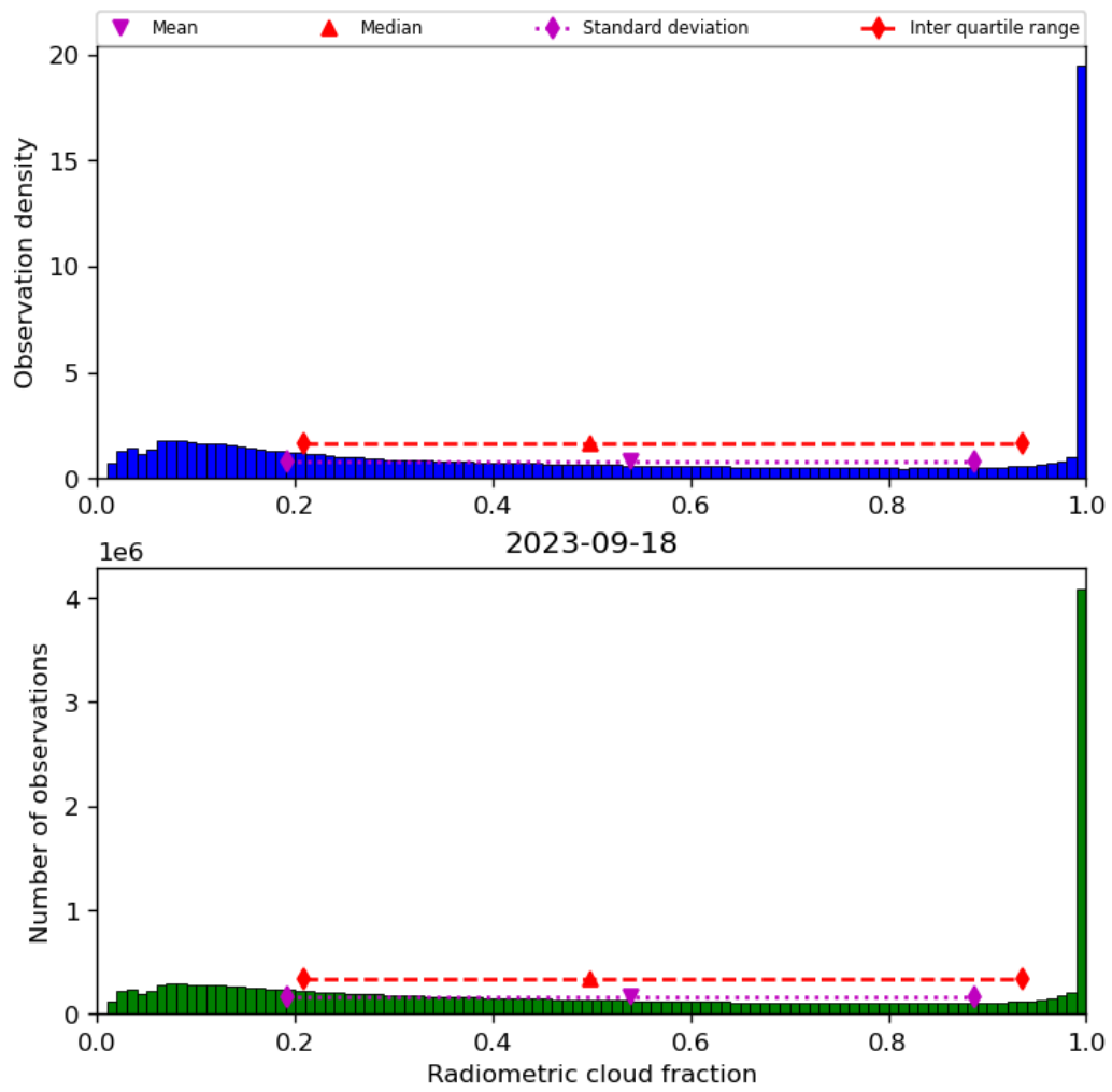
Figure 39: Histogram of “Radiometric cloud fraction” for 2023-09-17 to 2023-09-19
