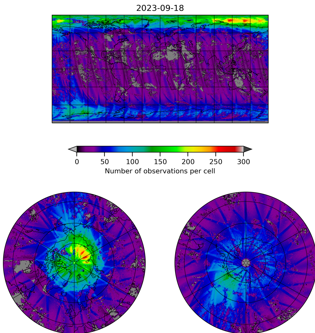
Figure 21: Map of the number of observations for 2023-09-17 to 2023-09-19
