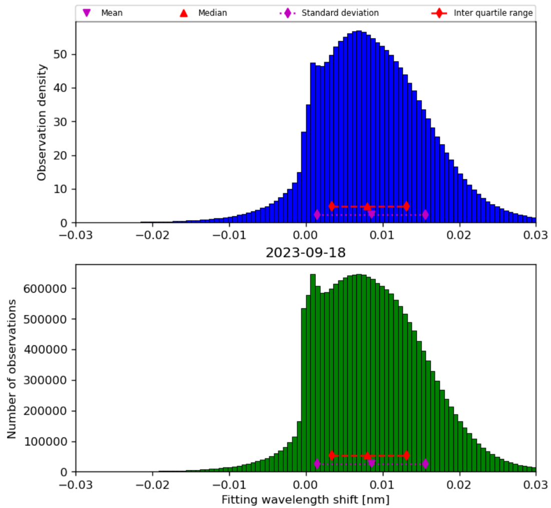
Figure 49: Histogram of “Fitting wavelength shift” for 2023-09-17 to 2023-09-19
