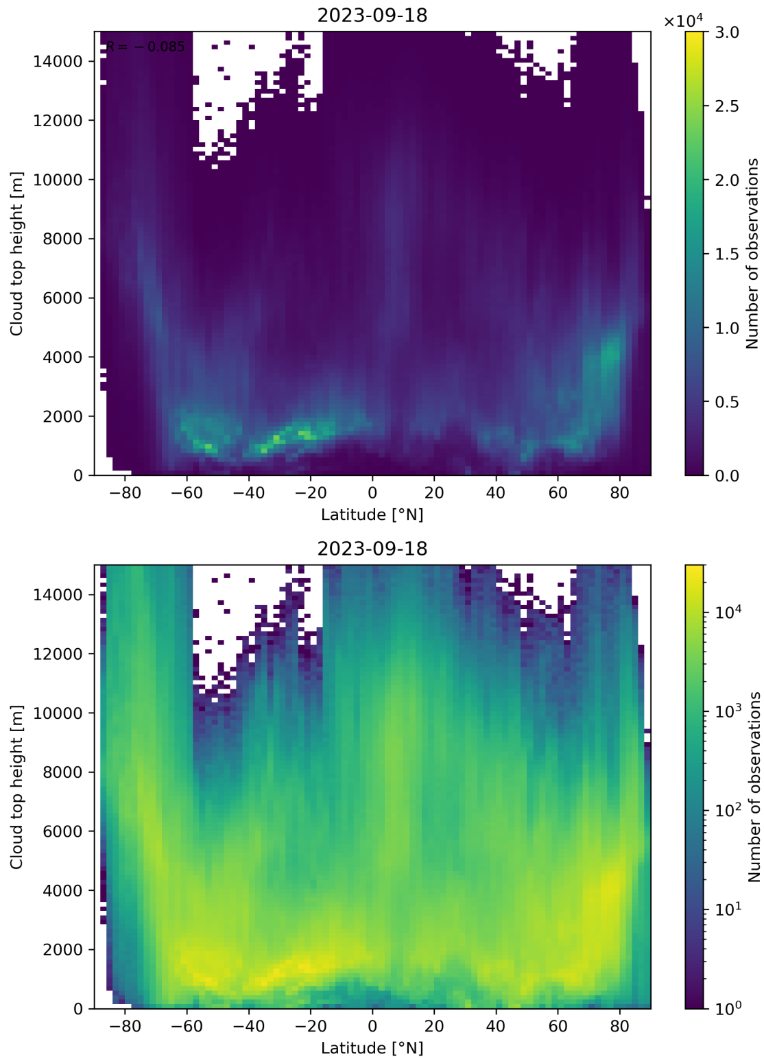
Figure 97: Scatter density plot of “Latitude” against “Cloud top height” for 2023-09-17 to 2023-09-19.
