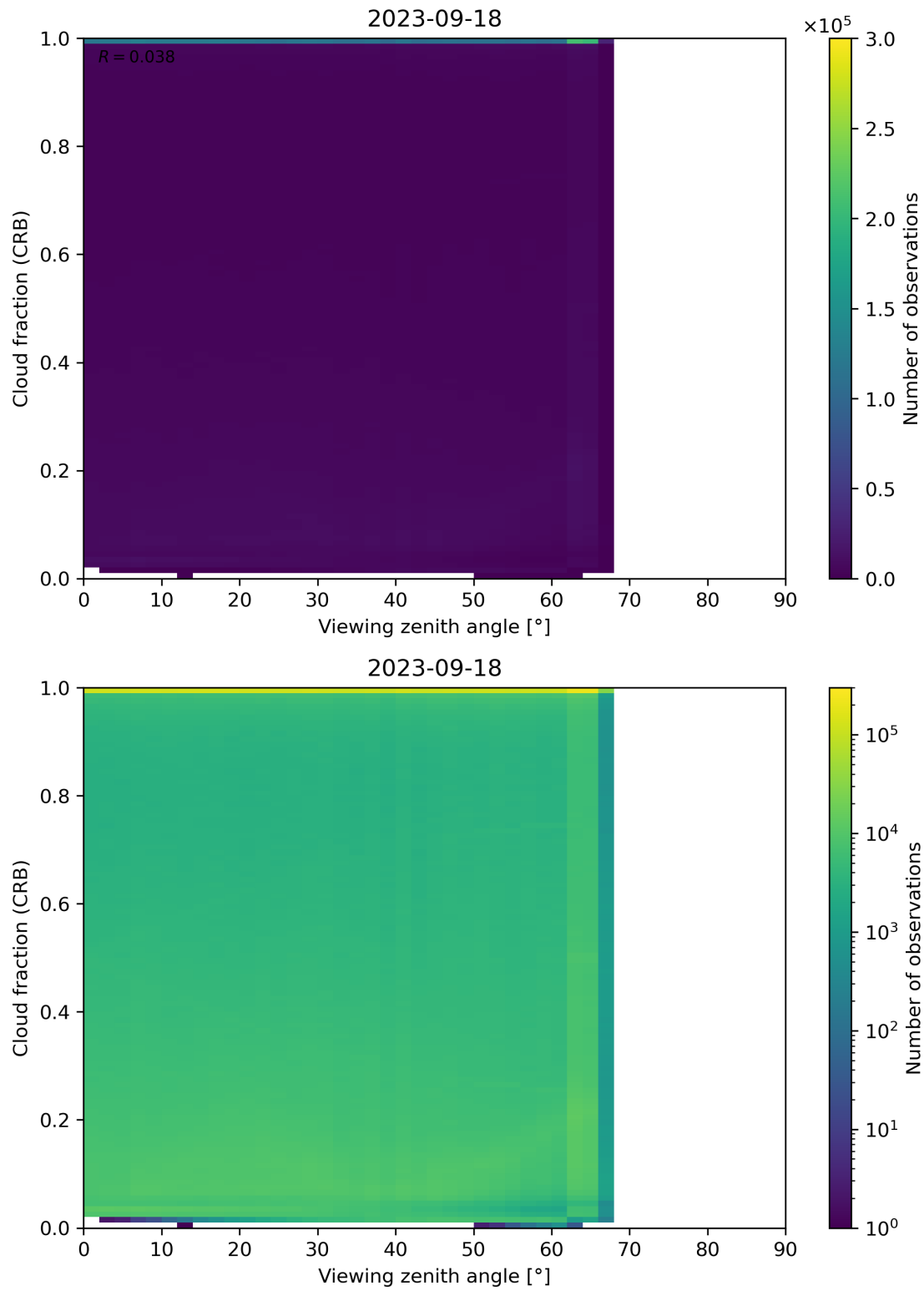
Figure 109: Scatter density plot of “Viewing zenith angle” against “Cloud fraction (CRB)” for 2023-09-17 to 2023-09-19.
