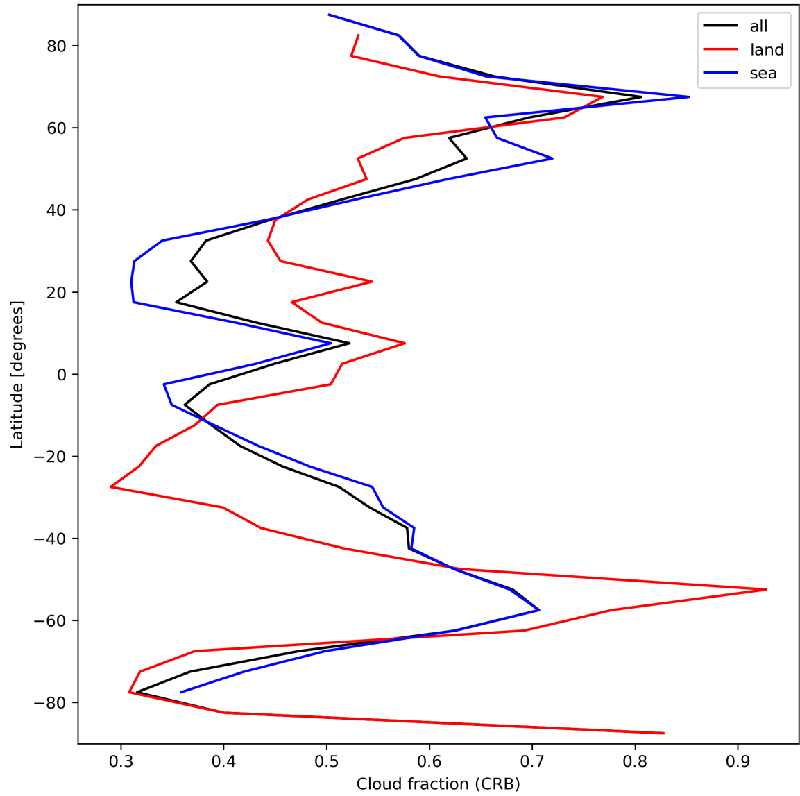
Figure 26: Zonal average of “Cloud fraction (CRB)” for 2023-09-17 to 2023-09-19.
