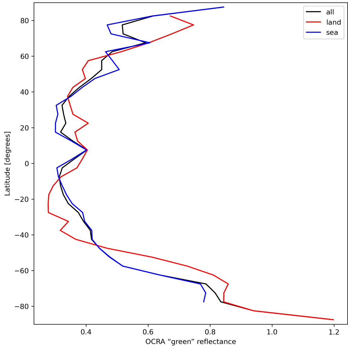
Figure 36: Zonal average of “OCRA “green” reflectance” for 2023-09-17 to 2023-09-19.
