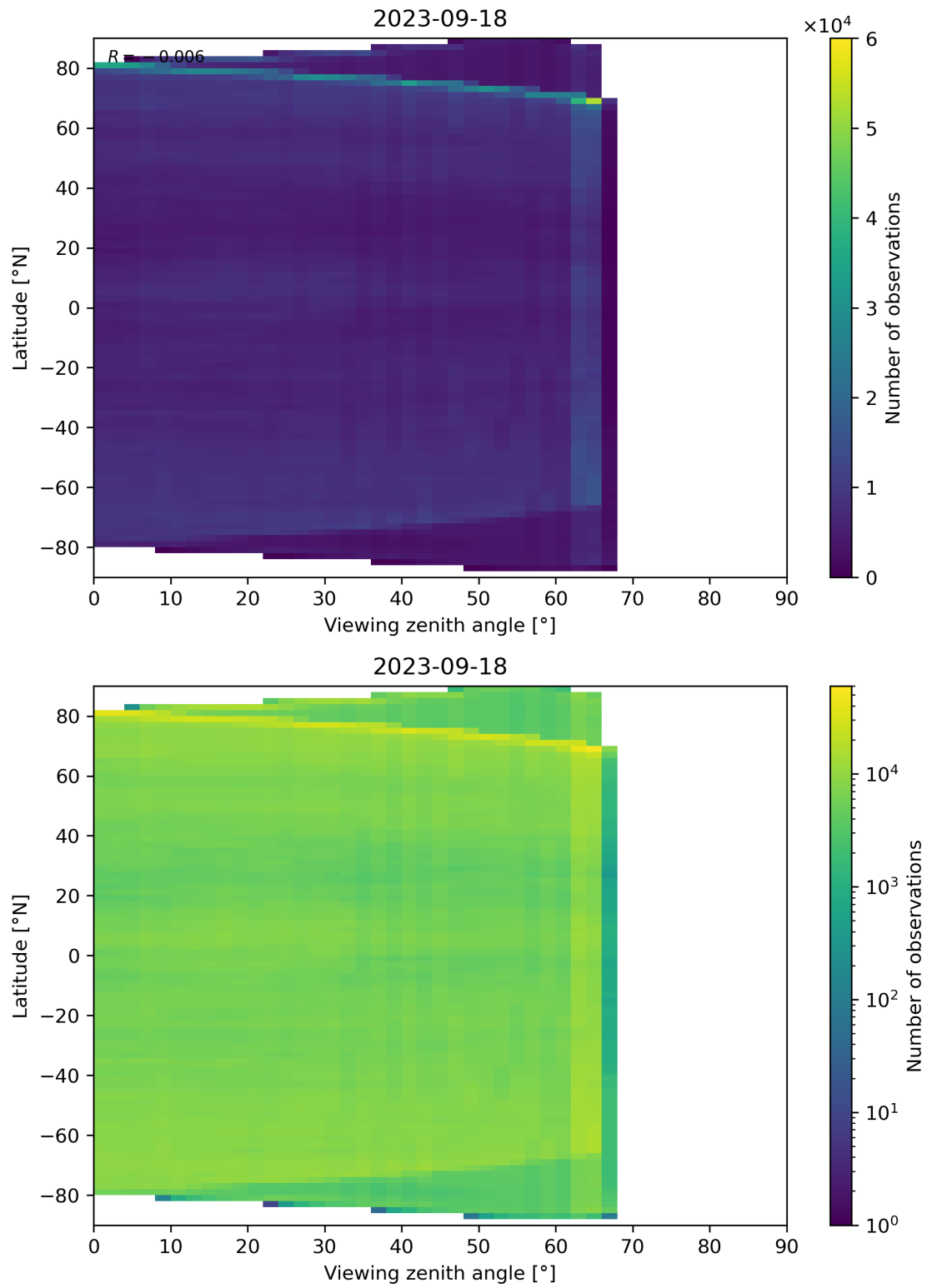
Figure 113: Scatter density plot of “Viewing zenith angle” against “Latitude” for 2023-09-17 to 2023-09-19.
