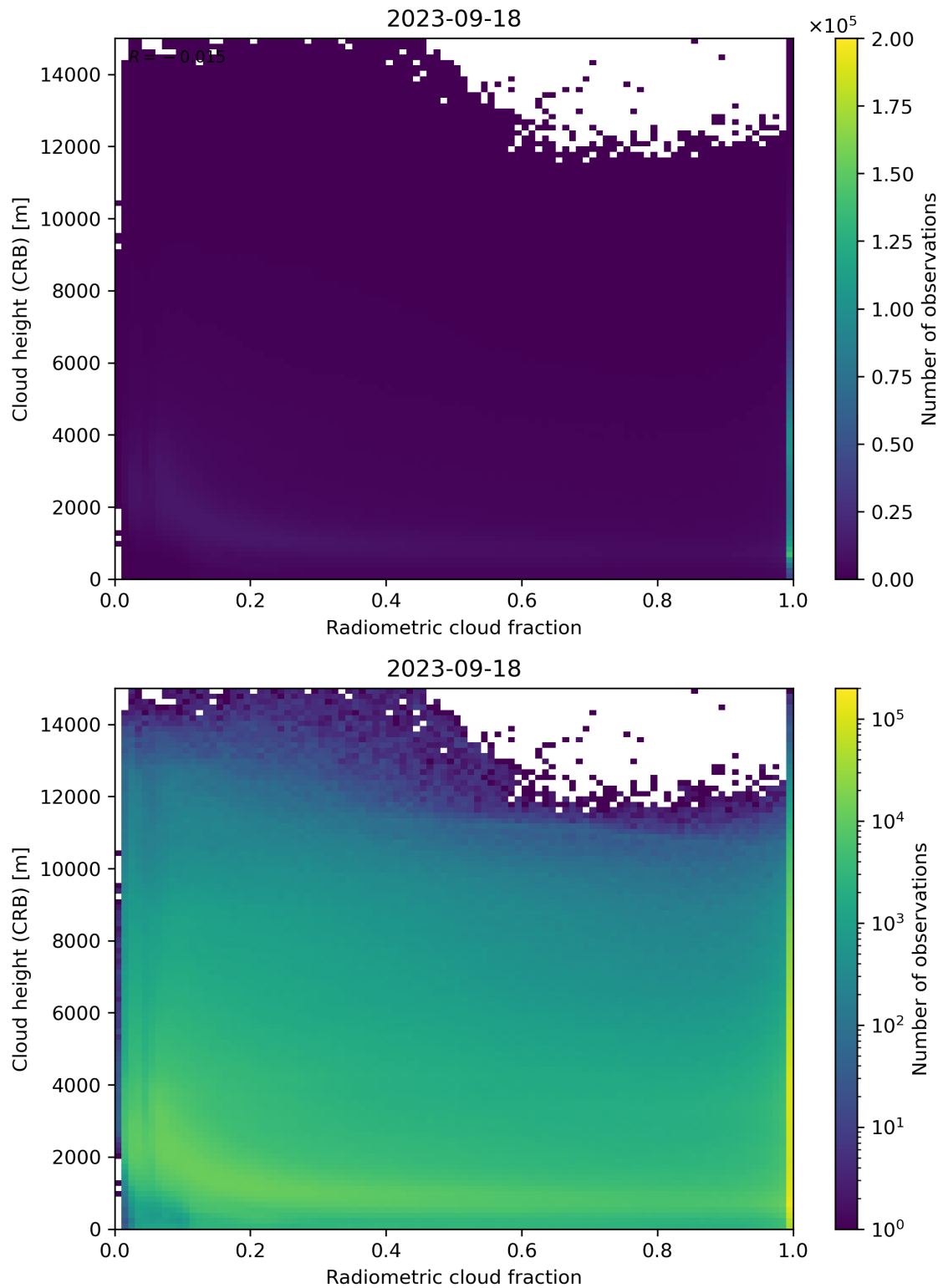
Figure 74: Scatter density plot of “Radiometric cloud fraction” against “Cloud height (CRB)” for 2023-09-17 to 2023-09-19.
