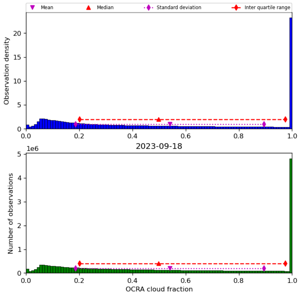
Figure 50: Histogram of “OCRA cloud fraction” for 2023-09-17 to 2023-09-19
