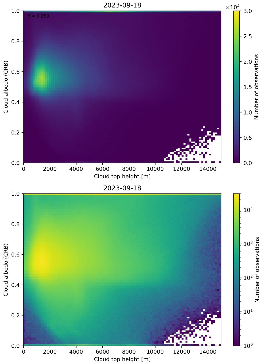
Figure 86: Scatter density plot of “Cloud top height” against “Cloud albedo (CRB)” for 2023-09-17 to 2023-09-19.
