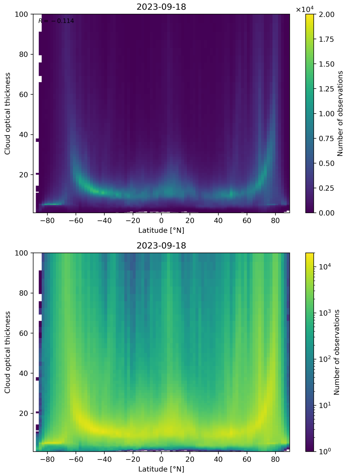
Figure 96: Scatter density plot of “Latitude” against “Cloud optical thickness” for 2023-09-17 to 2023-09-19.
