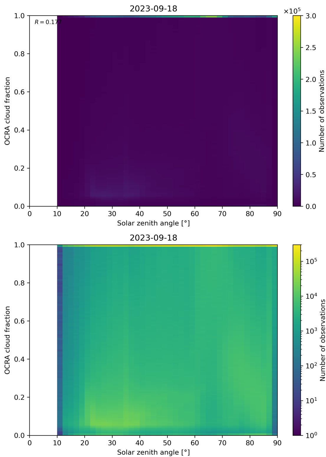
Figure 100: Scatter density plot of “Solar zenith angle” against “OCRA cloud fraction” for 2023-09-17 to 2023-09-19.
