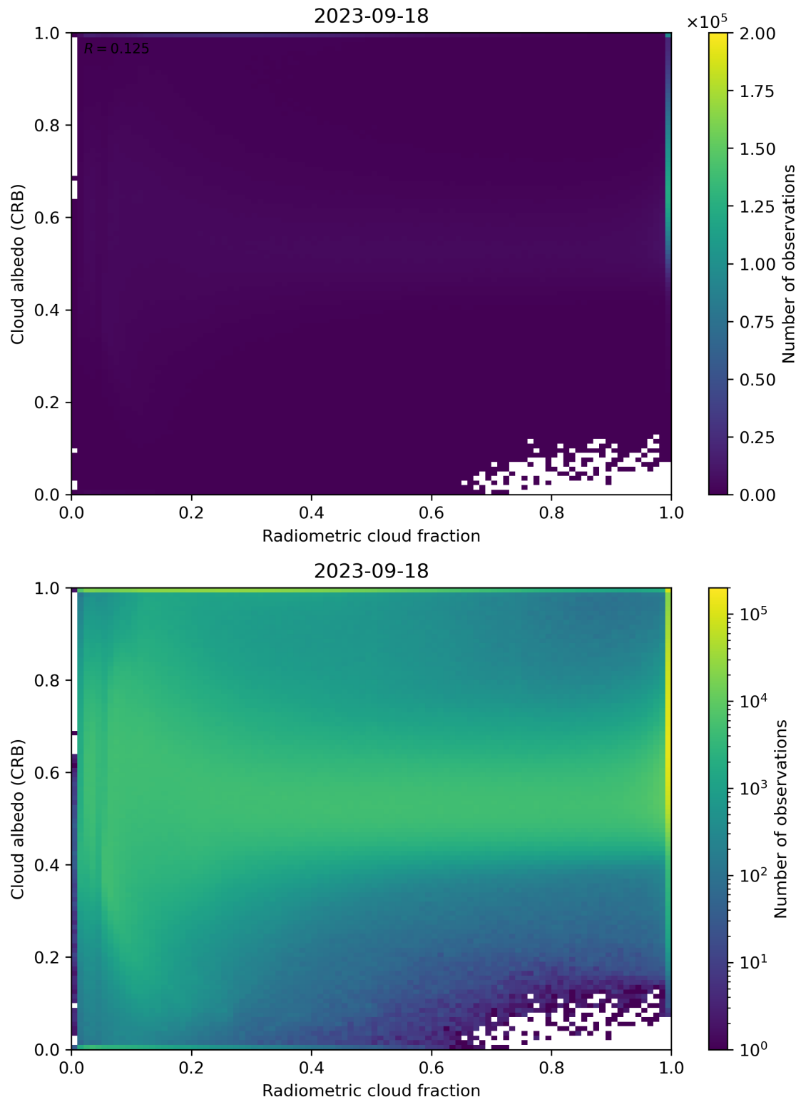
Figure 71: Scatter density plot of “Radiometric cloud fraction” against “Cloud albedo (CRB)” for 2023-09-17 to 2023-09-19.
