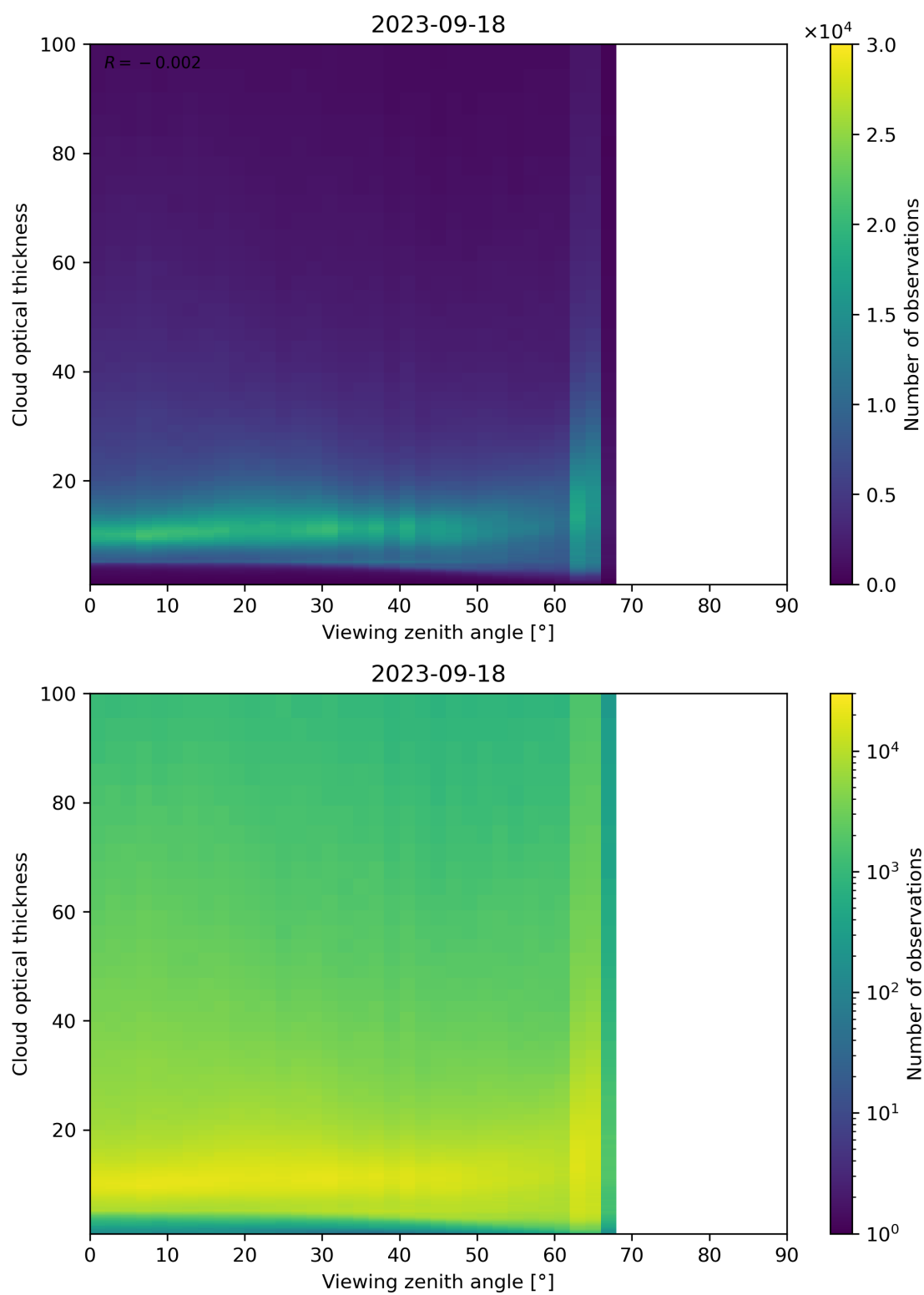
Figure 111: Scatter density plot of “Viewing zenith angle” against “Cloud optical thickness” for 2023-09-17 to 2023-09-19.
