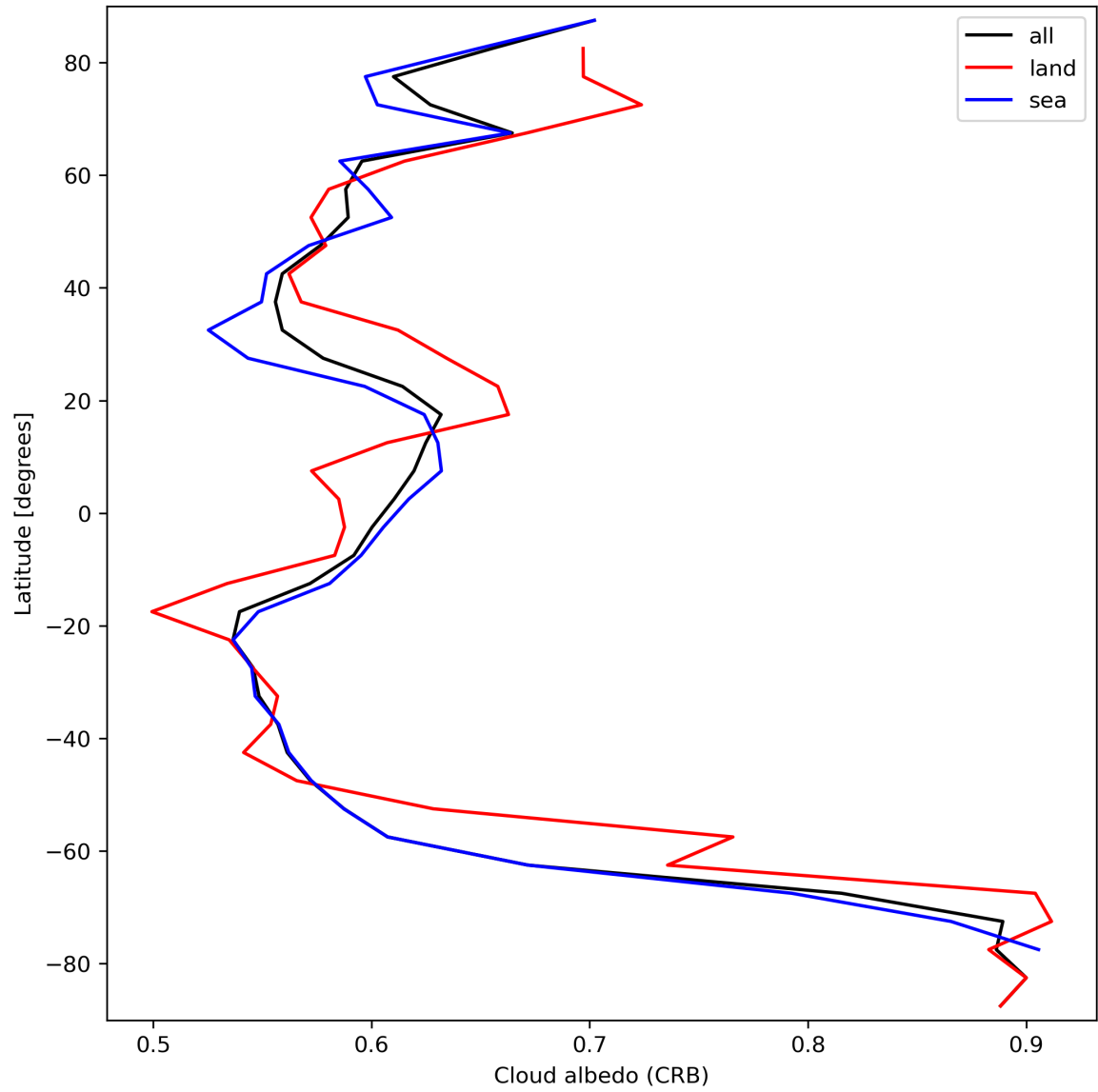
Figure 28: Zonal average of “Cloud albedo (CRB)” for 2023-09-17 to 2023-09-19.
