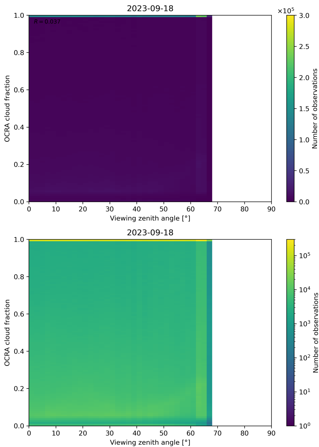
Figure 108: Scatter density plot of “Viewing zenith angle” against “OCRA cloud fraction” for 2023-09-17 to 2023-09-19.
