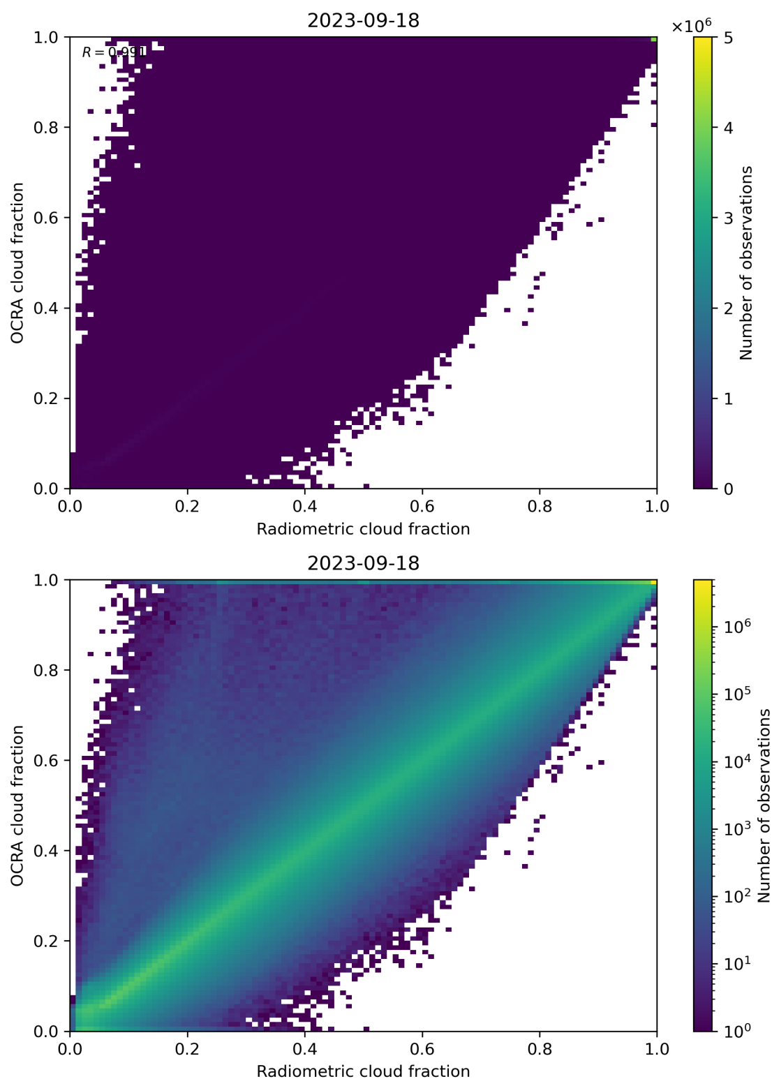
Figure 72: Scatter density plot of “Radiometric cloud fraction” against “OCRA cloud fraction” for 2023-09-17 to 2023-09-19.
