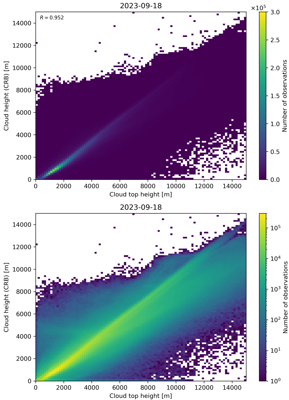
Figure 89: Scatter density plot of “Cloud top height” against “Cloud height (CRB)” for 2023-09-17 to 2023-09-19.
