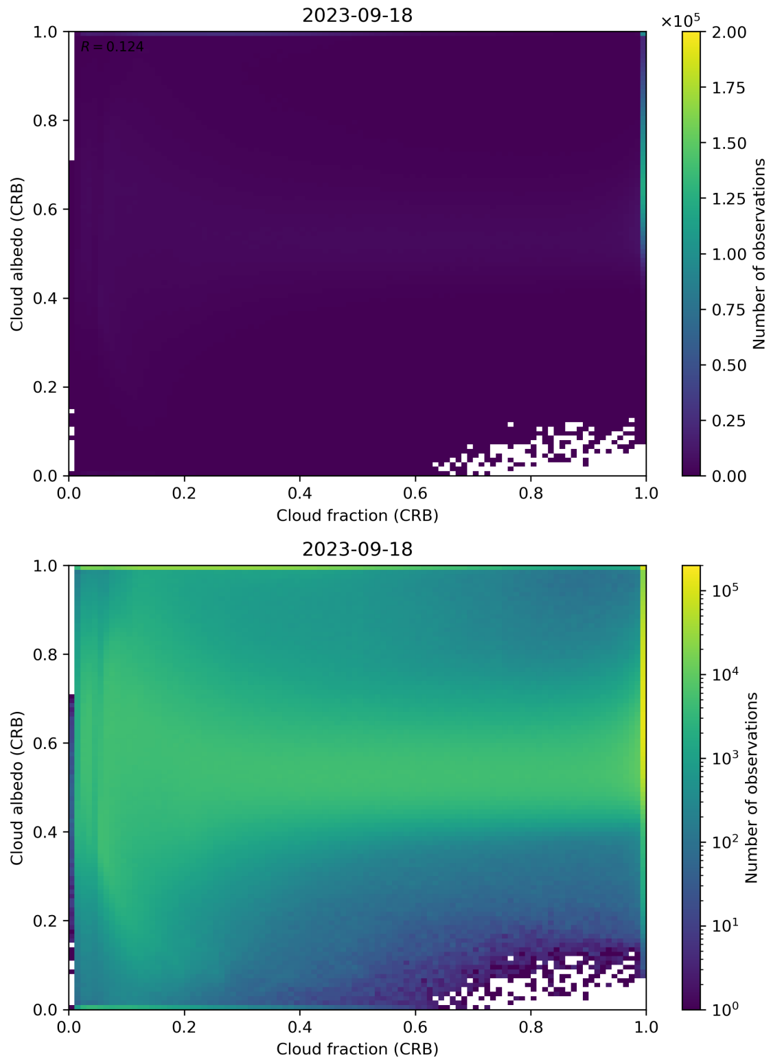
Figure 77: Scatter density plot of “Cloud fraction (CRB)” against “Cloud albedo (CRB)” for 2023-09-17 to 2023-09-19.
