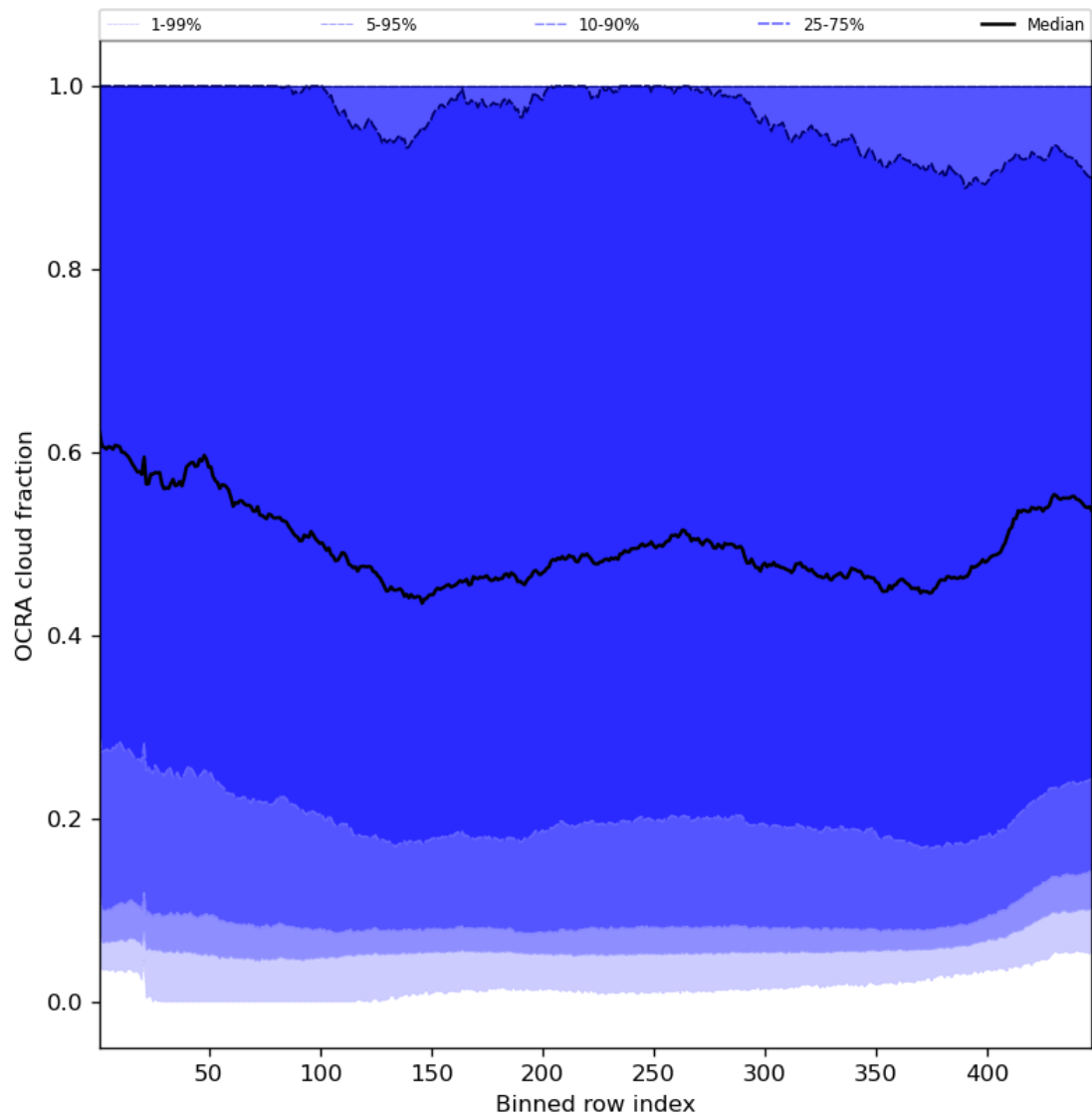
Figure 66: Along track statistics of “OCRA cloud fraction” for 2023-09-17 to 2023-09-19
