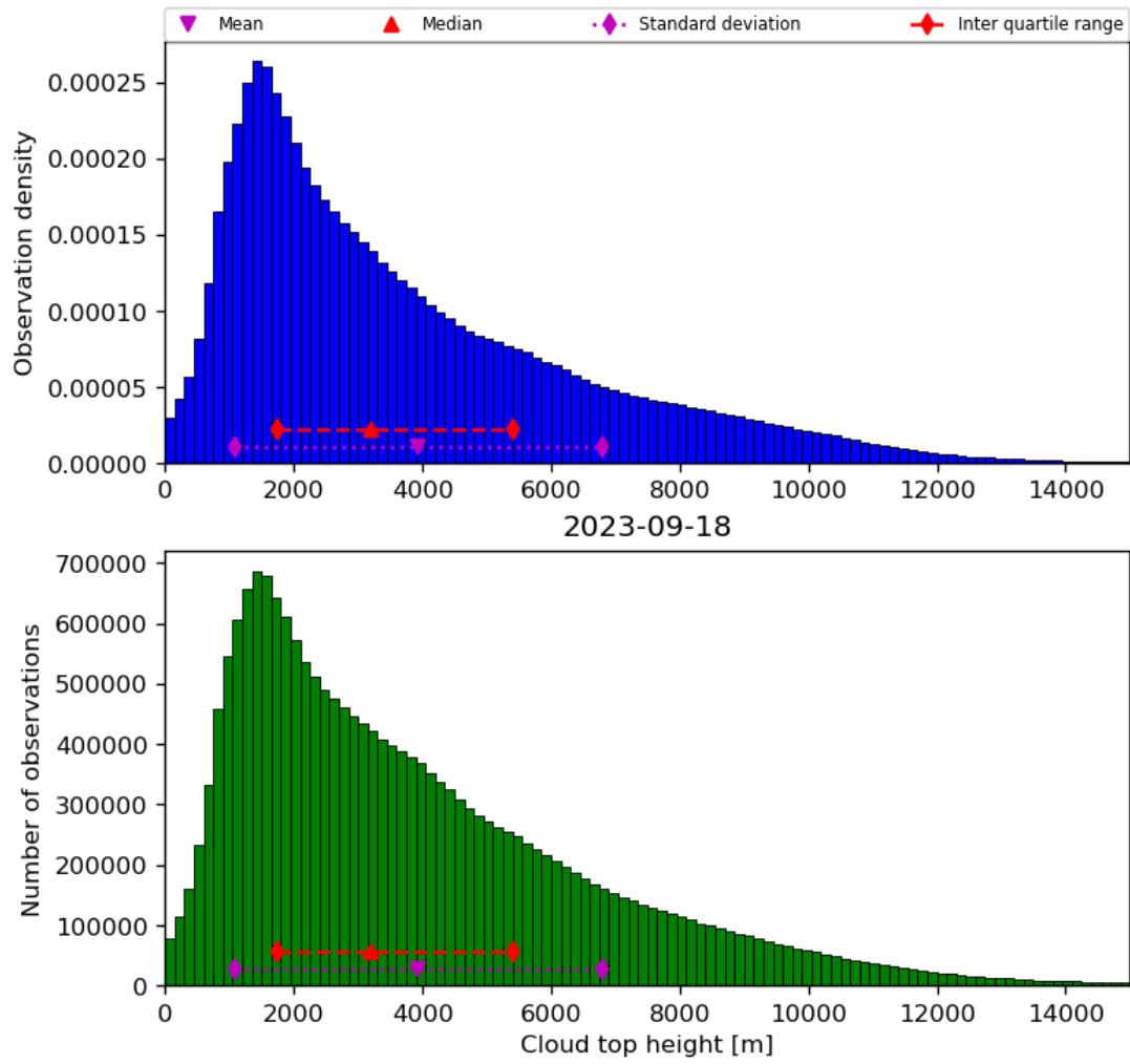
Figure 40: Histogram of “Cloud top height” for 2023-09-17 to 2023-09-19
