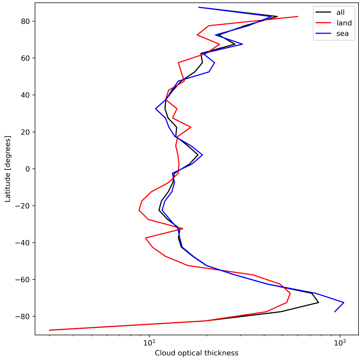
Figure 25: Zonal average of “Cloud optical thickness” for 2023-09-17 to 2023-09-19.
