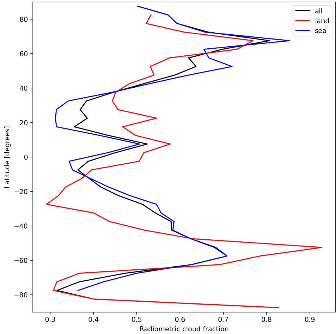
Figure 23: Zonal average of “Radiometric cloud fraction” for 2023-09-17 to 2023-09-19.
