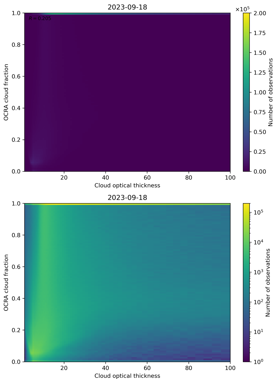
Figure 83: Scatter density plot of “Cloud optical thickness” against “OCRA cloud fraction” for 2023-09-17 to 2023-09-19.
