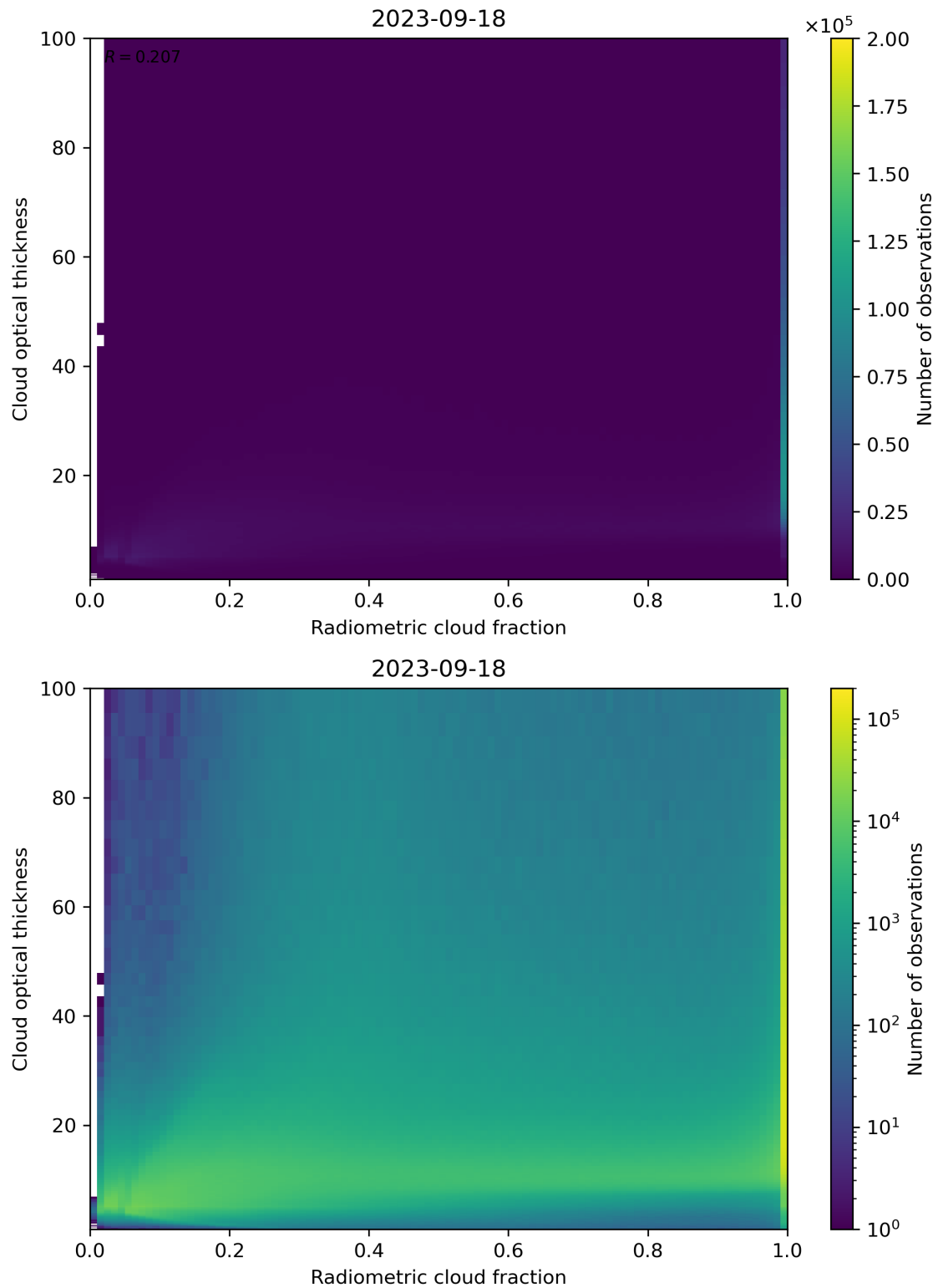
Figure 75: Scatter density plot of “Radiometric cloud fraction” against “Cloud optical thickness” for 2023-09-17 to 2023-09-19.
