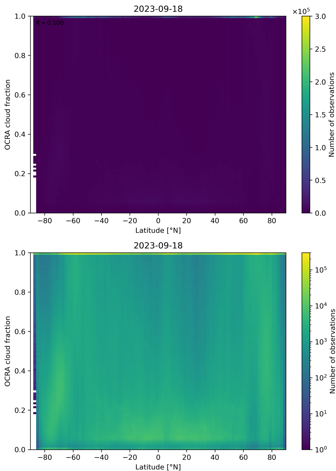
Figure 93: Scatter density plot of “Latitude” against “OCRA cloud fraction” for 2023-09-17 to 2023-09-19.
