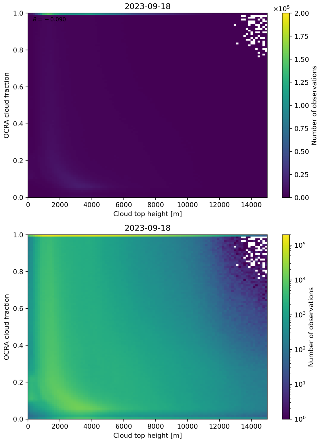
Figure 87: Scatter density plot of “Cloud top height” against “OCRA cloud fraction” for 2023-09-17 to 2023-09-19.
