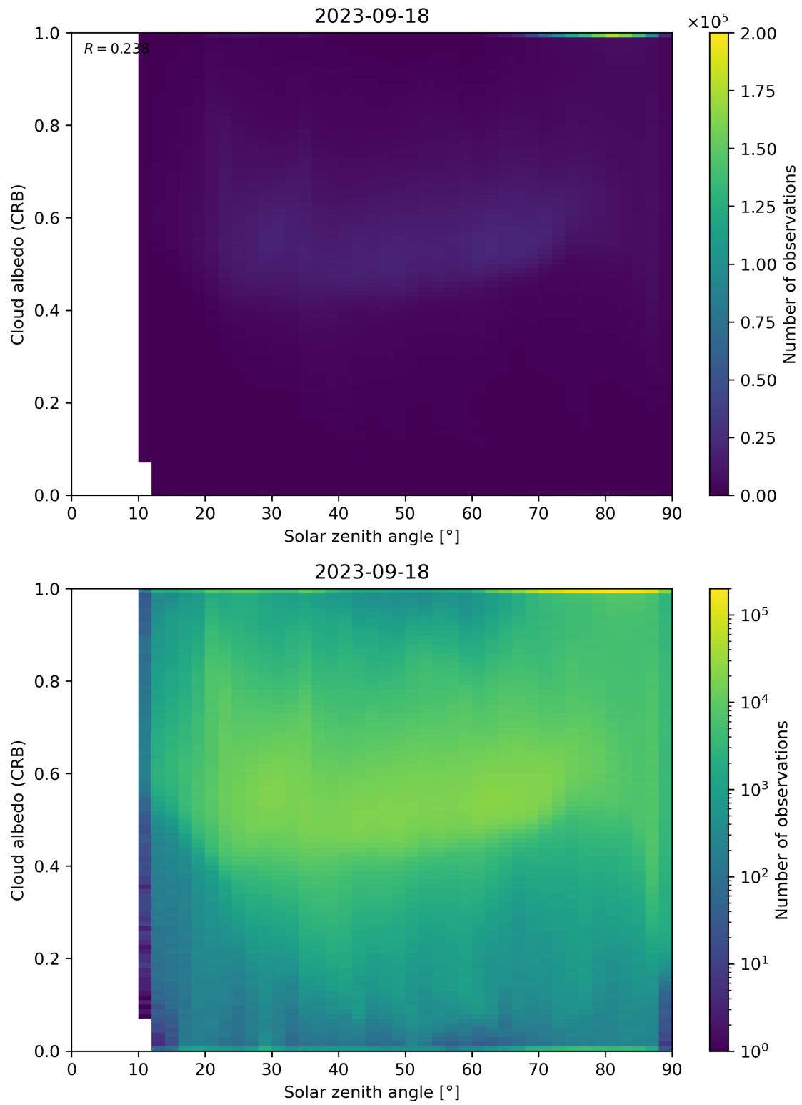
Figure 98: Scatter density plot of “Solar zenith angle” against “Cloud albedo (CRB)” for 2023-09-17 to 2023-09-19.
