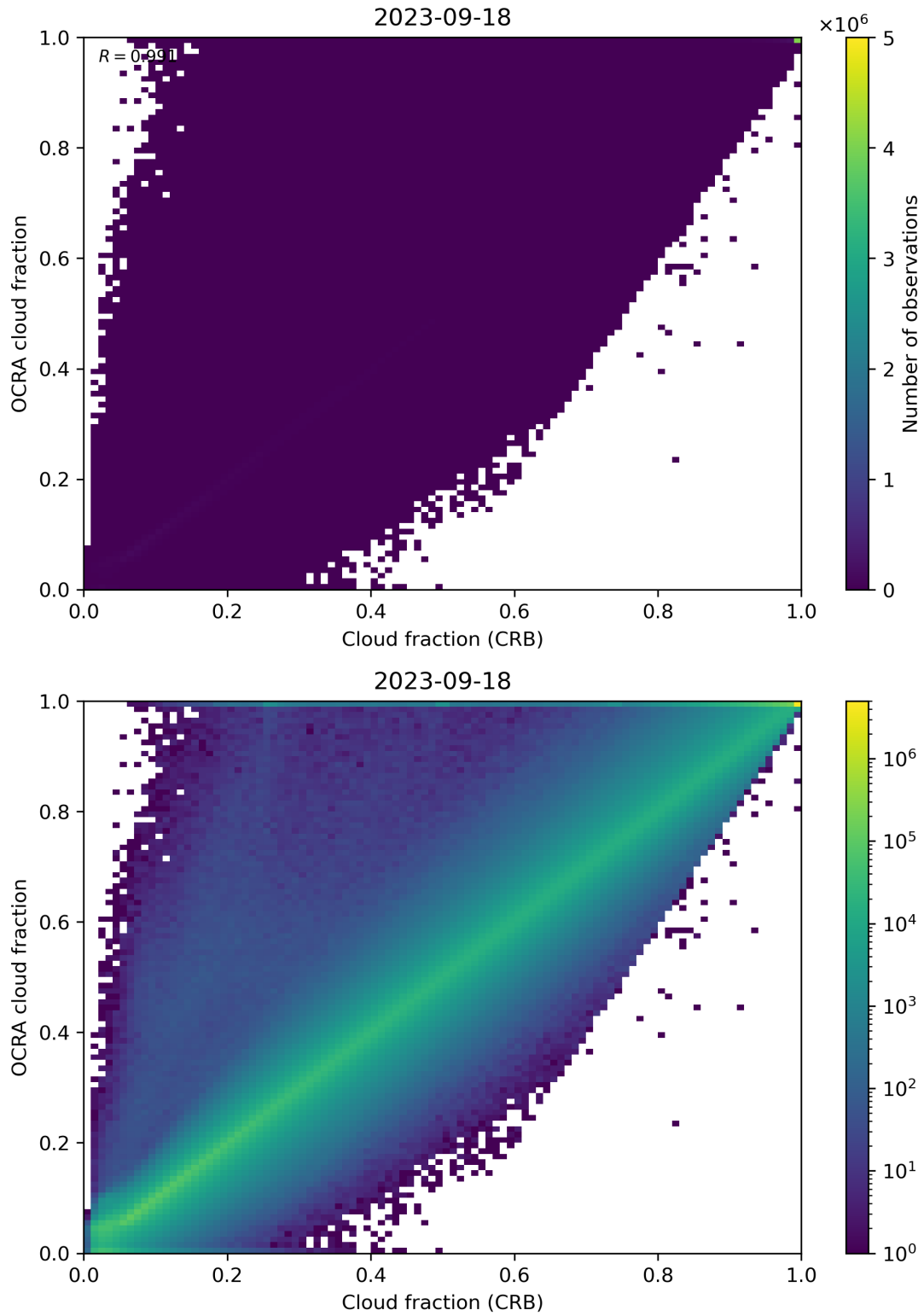
Figure 78: Scatter density plot of “Cloud fraction (CRB)” against “OCRA cloud fraction” for 2023-09-17 to 2023-09-19.
