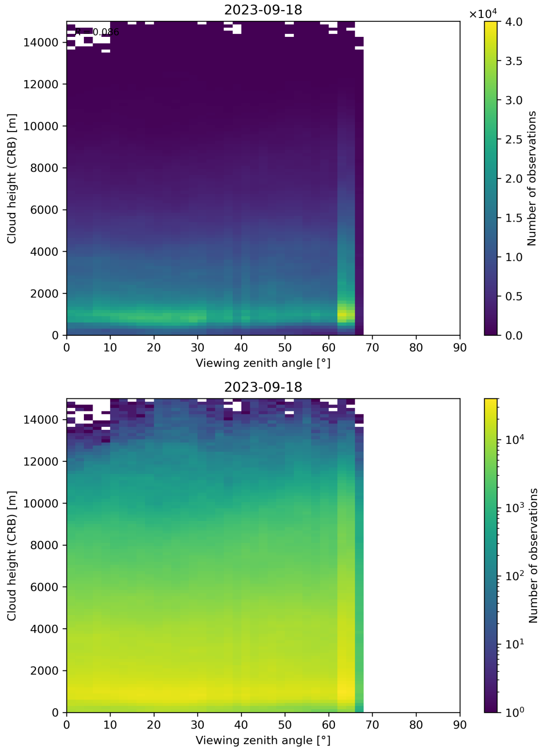
Figure 110: Scatter density plot of “Viewing zenith angle” against “Cloud height (CRB)” for 2023-09-17 to 2023-09-19.
