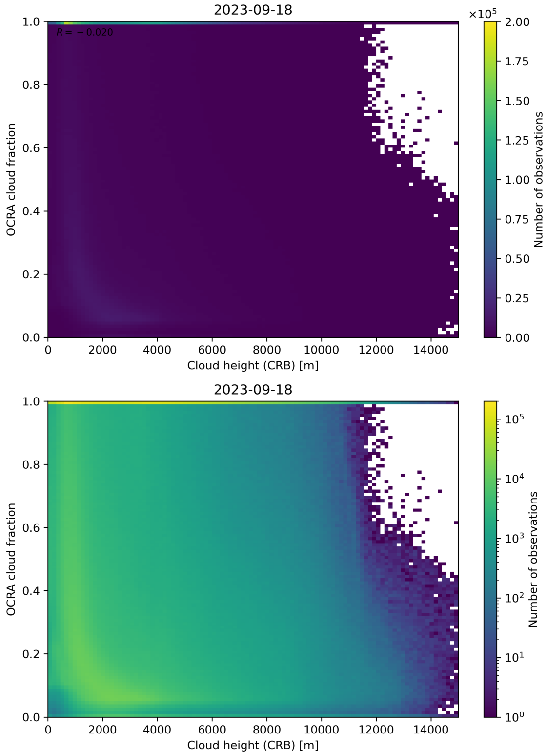
Figure 81: Scatter density plot of “Cloud height (CRB)” against “OCRA cloud fraction” for 2023-09-17 to 2023-09-19.
