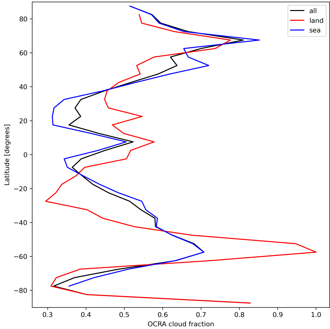
Figure 34: Zonal average of “OCRA cloud fraction” for 2023-09-17 to 2023-09-19.
