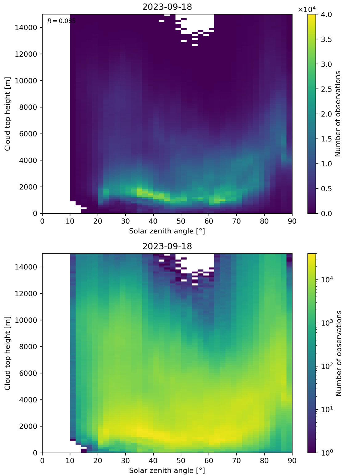
Figure 104: Scatter density plot of “Solar zenith angle” against “Cloud top height” for 2023-09-17 to 2023-09-19.
