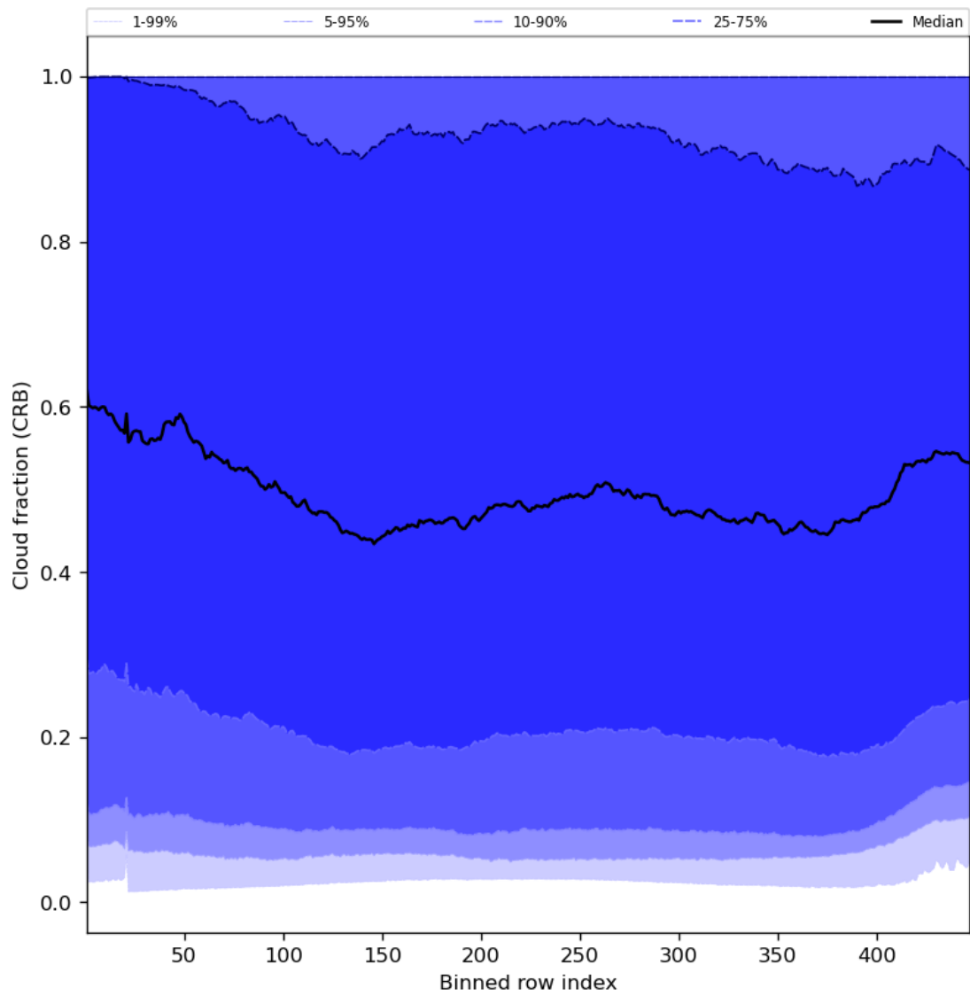
Figure 58: Along track statistics of “Cloud fraction (CRB)” for 2023-09-17 to 2023-09-19
