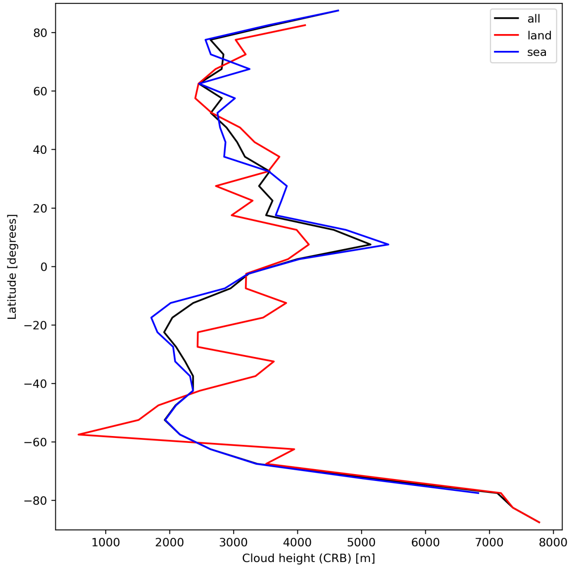
Figure 27: Zonal average of “Cloud height (CRB)” for 2023-09-17 to 2023-09-19.
