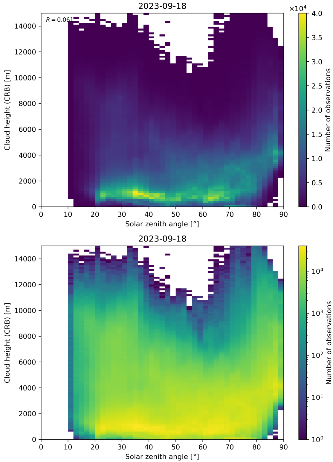
Figure 102: Scatter density plot of “Solar zenith angle” against “Cloud height (CRB)” for 2023-09-17 to 2023-09-19.
