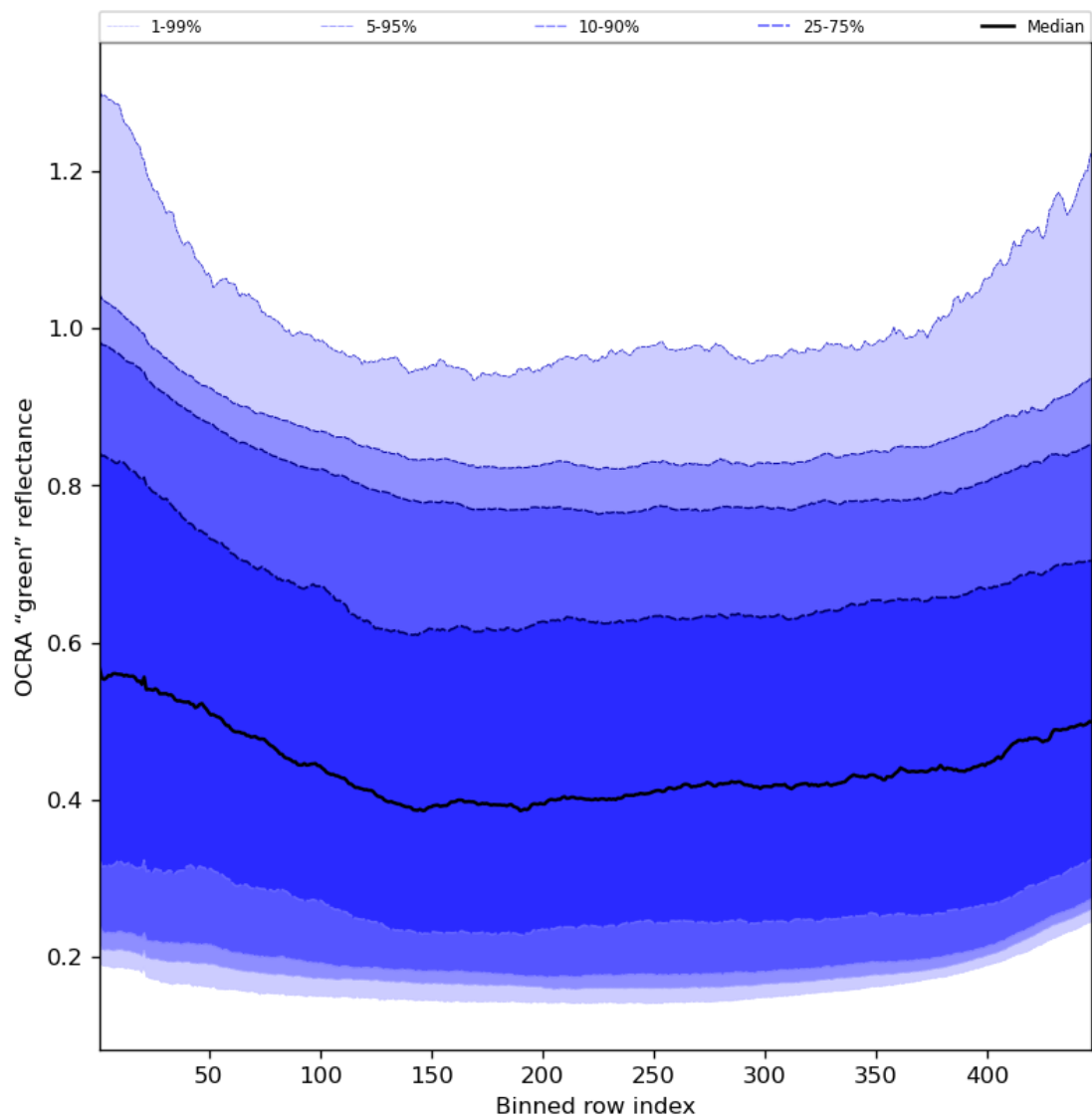
Figure 68: Along track statistics of “OCRA “green” reflectance” for 2023-09-17 to 2023-09-19
