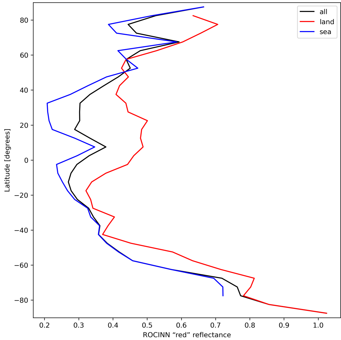
Figure 37: Zonal average of “ROCINN “red” reflectance” for 2023-09-17 to 2023-09-19.
