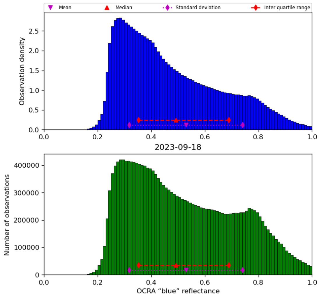
Figure 51: Histogram of “OCRA “blue” reflectance” for 2023-09-17 to 2023-09-19
