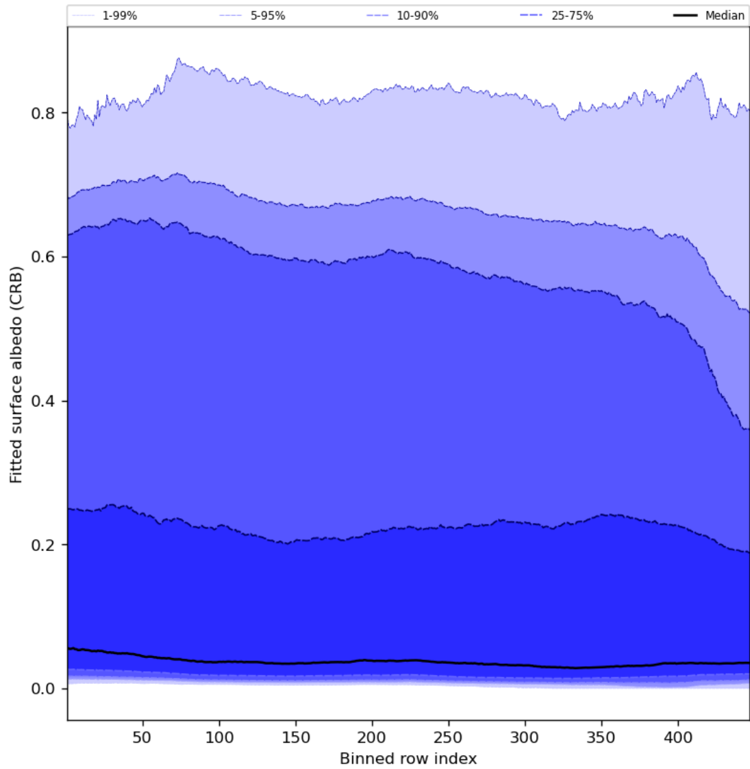
Figure 62: Along track statistics of “Fitted surface albedo (CRB)” for 2023-09-17 to 2023-09-19
