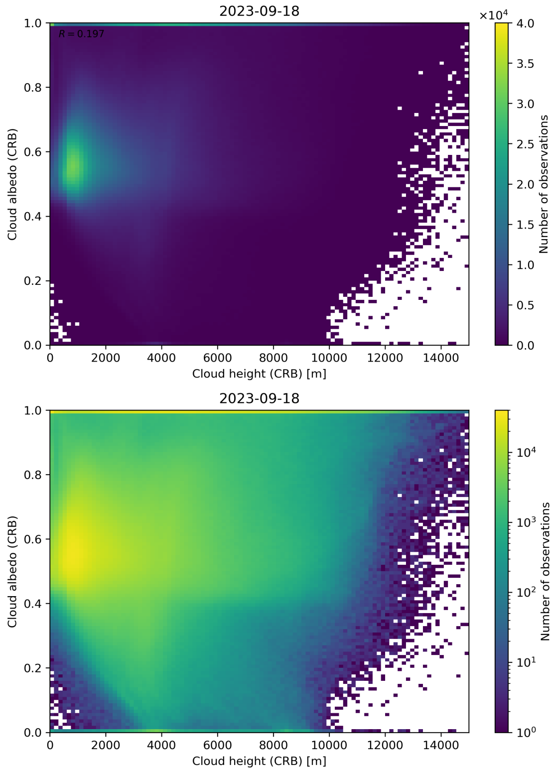
Figure 80: Scatter density plot of “Cloud height (CRB)” against “Cloud albedo (CRB)” for 2023-09-17 to 2023-09-19.
