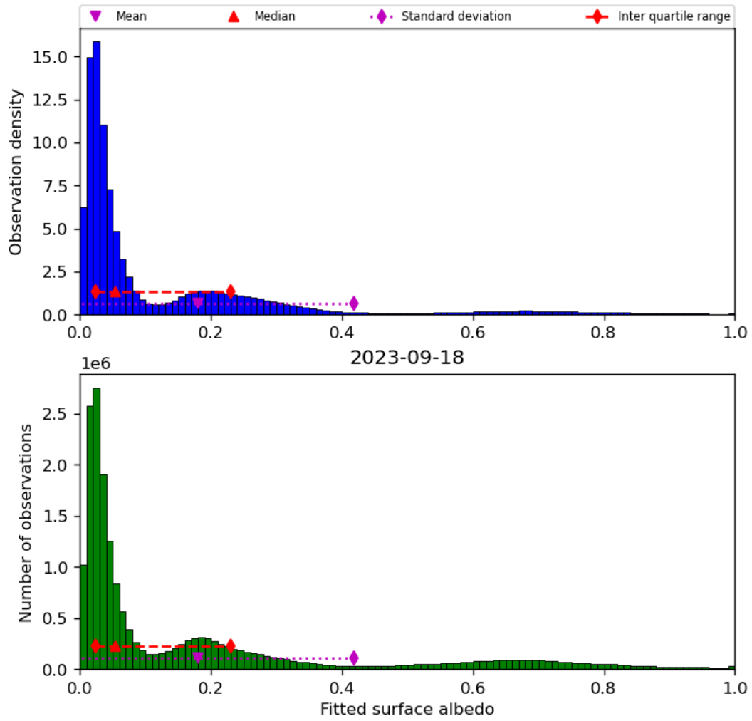
Figure 45: Histogram of “Fitted surface albedo” for 2023-09-17 to 2023-09-19
