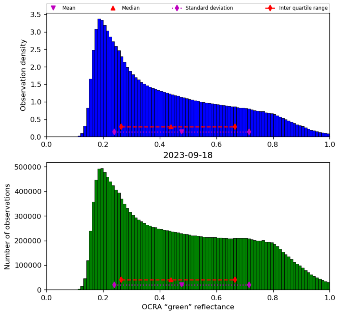
Figure 52: Histogram of “OCRA “green” reflectance” for 2023-09-17 to 2023-09-19
