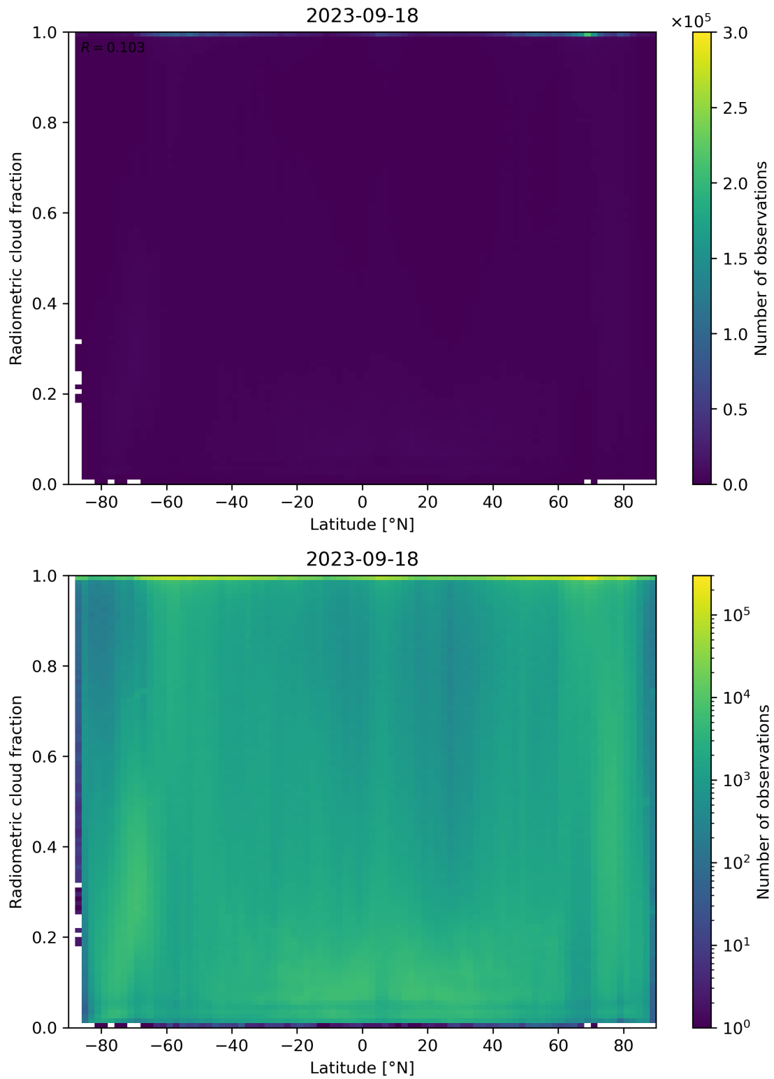
Figure 92: Scatter density plot of “Latitude” against “Radiometric cloud fraction” for 2023-09-17 to 2023-09-19.
