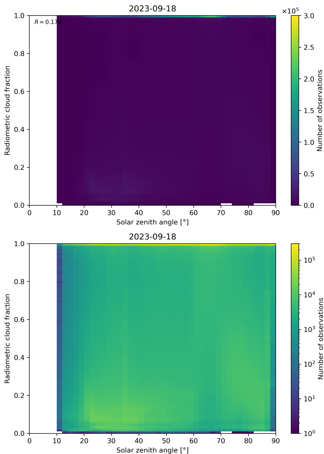
Figure 99: Scatter density plot of “Solar zenith angle” against “Radiometric cloud fraction” for 2023-09-17 to 2023-09-19.
