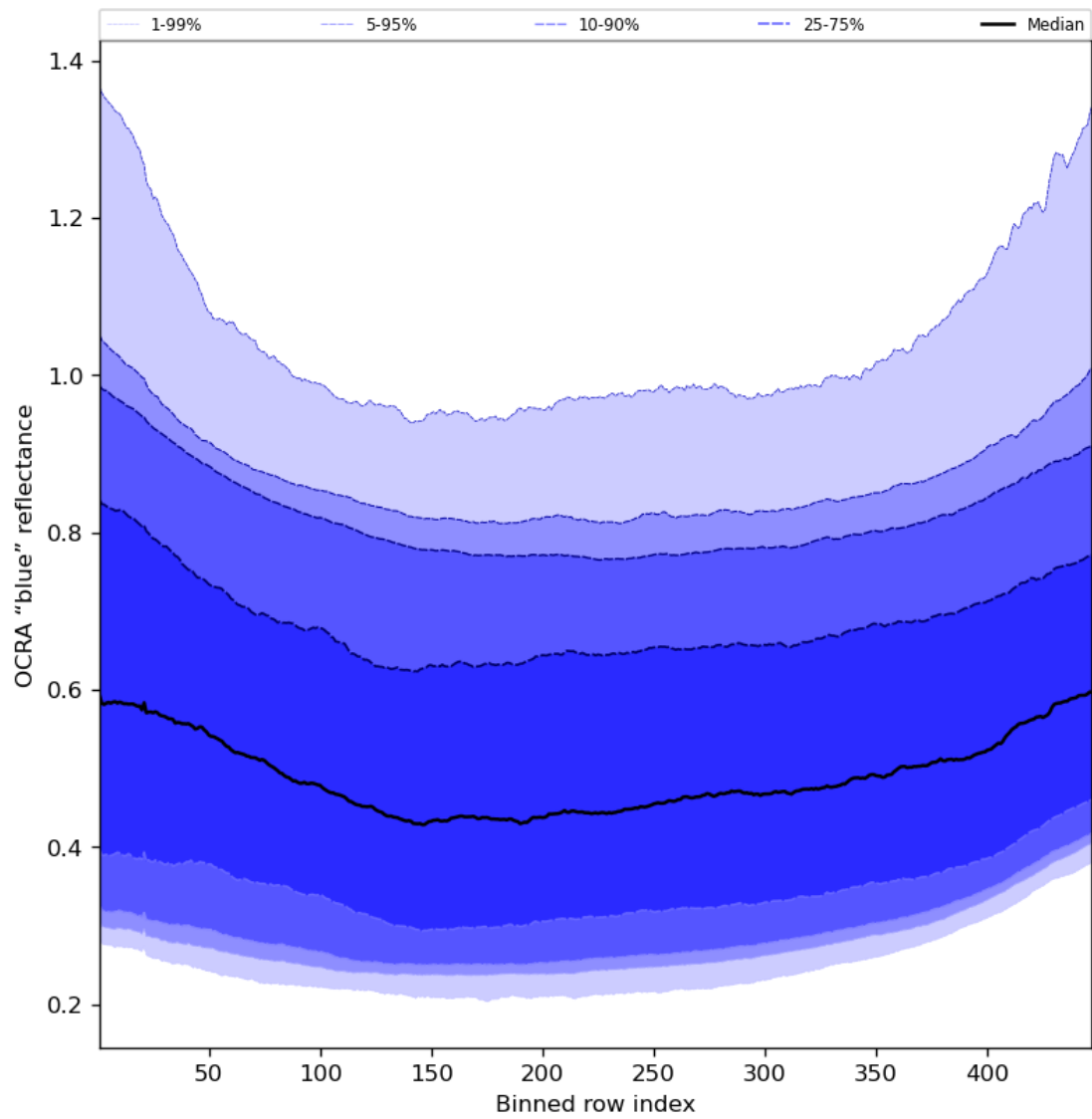
Figure 67: Along track statistics of “OCRA “blue” reflectance” for 2023-09-17 to 2023-09-19
