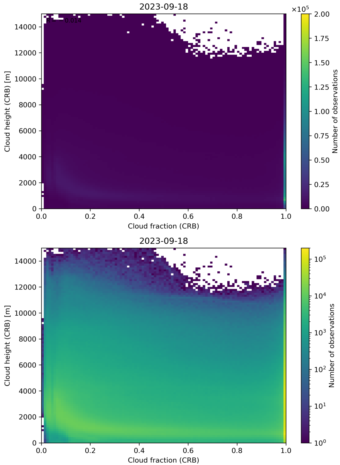
Figure 79: Scatter density plot of “Cloud fraction (CRB)” against “Cloud height (CRB)” for 2023-09-17 to 2023-09-19.
