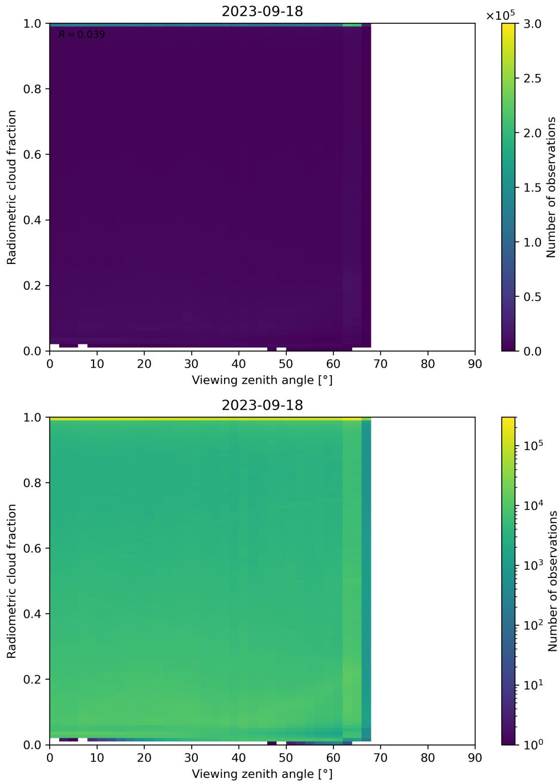
Figure 107: Scatter density plot of “Viewing zenith angle” against “Radiometric cloud fraction” for 2023-09-17 to 2023-09-19.
