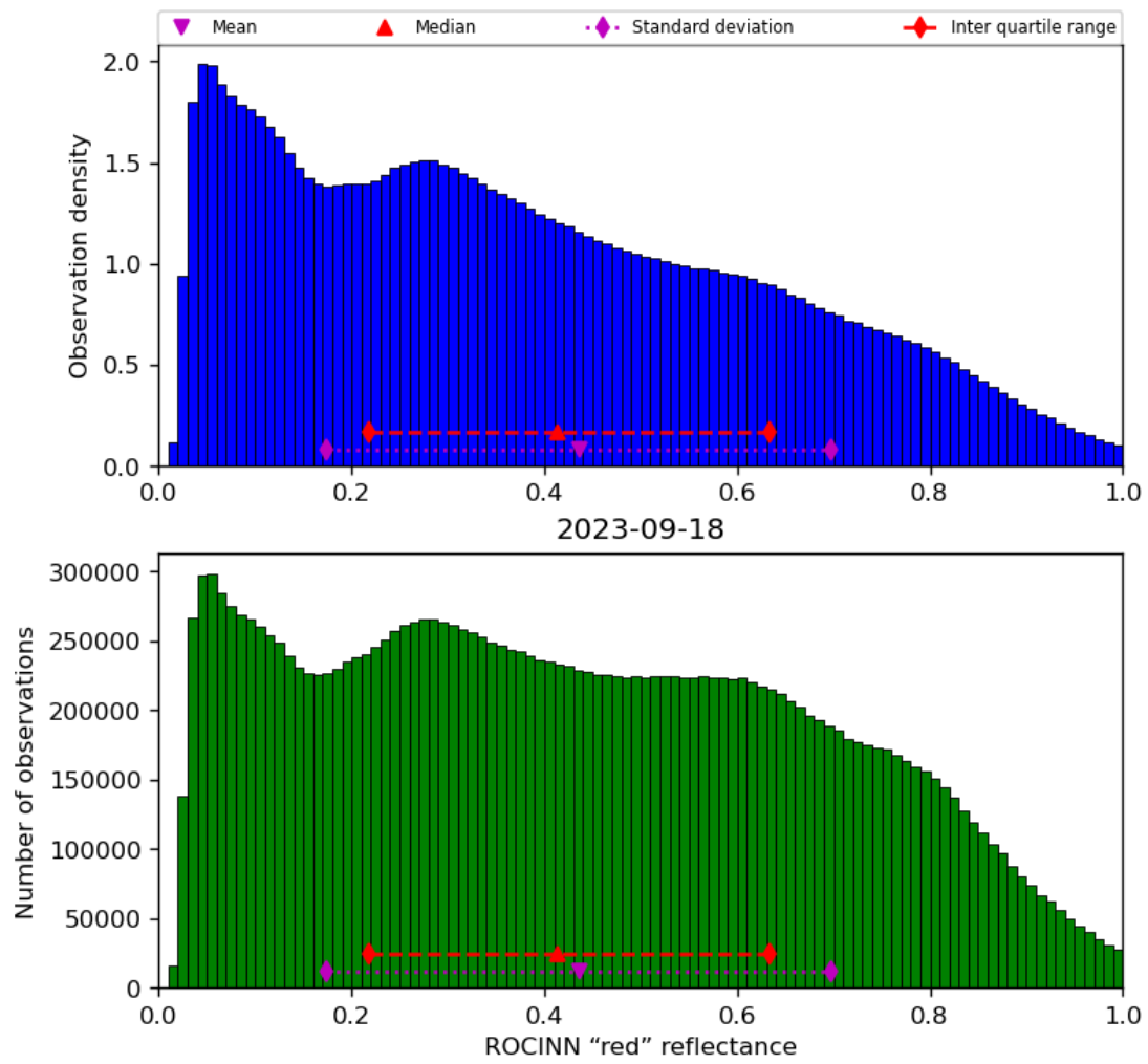
Figure 53: Histogram of “ROCINN “red” reflectance” for 2023-09-17 to 2023-09-19
