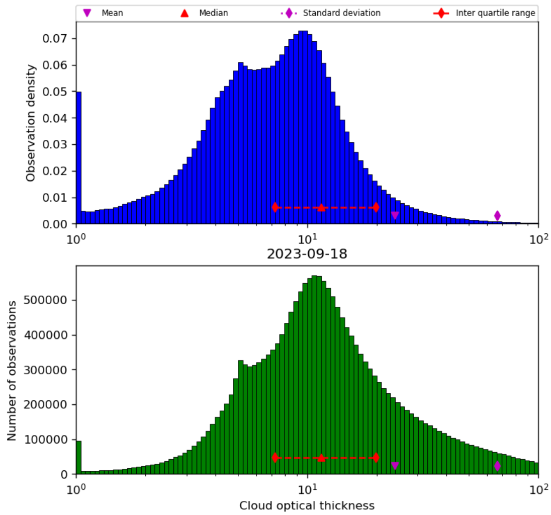
Figure 41: Histogram of “Cloud optical thickness” for 2023-09-17 to 2023-09-19
