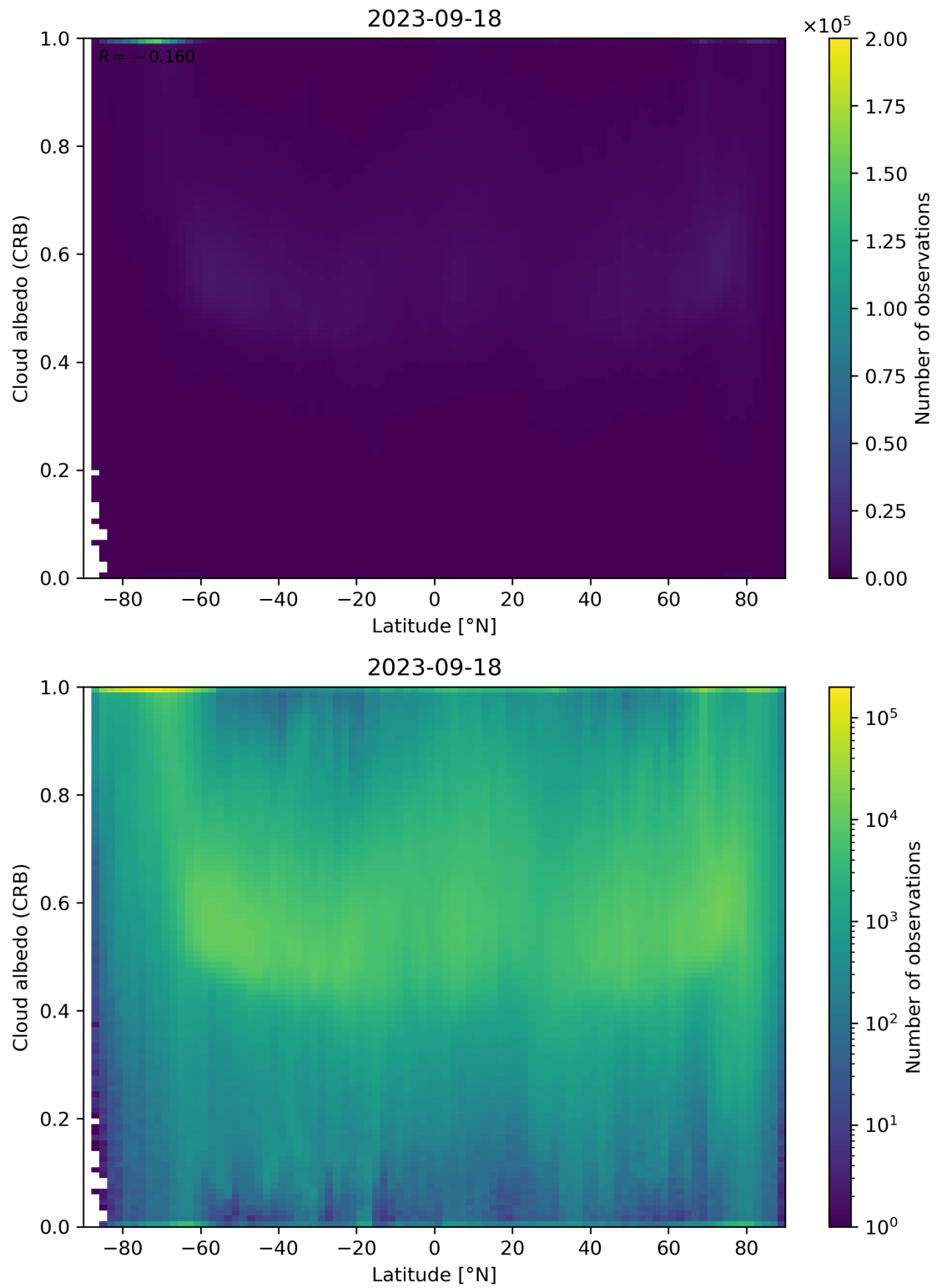
Figure 91: Scatter density plot of “Latitude” against “Cloud albedo (CRB)” for 2023-09-17 to 2023-09-19.
