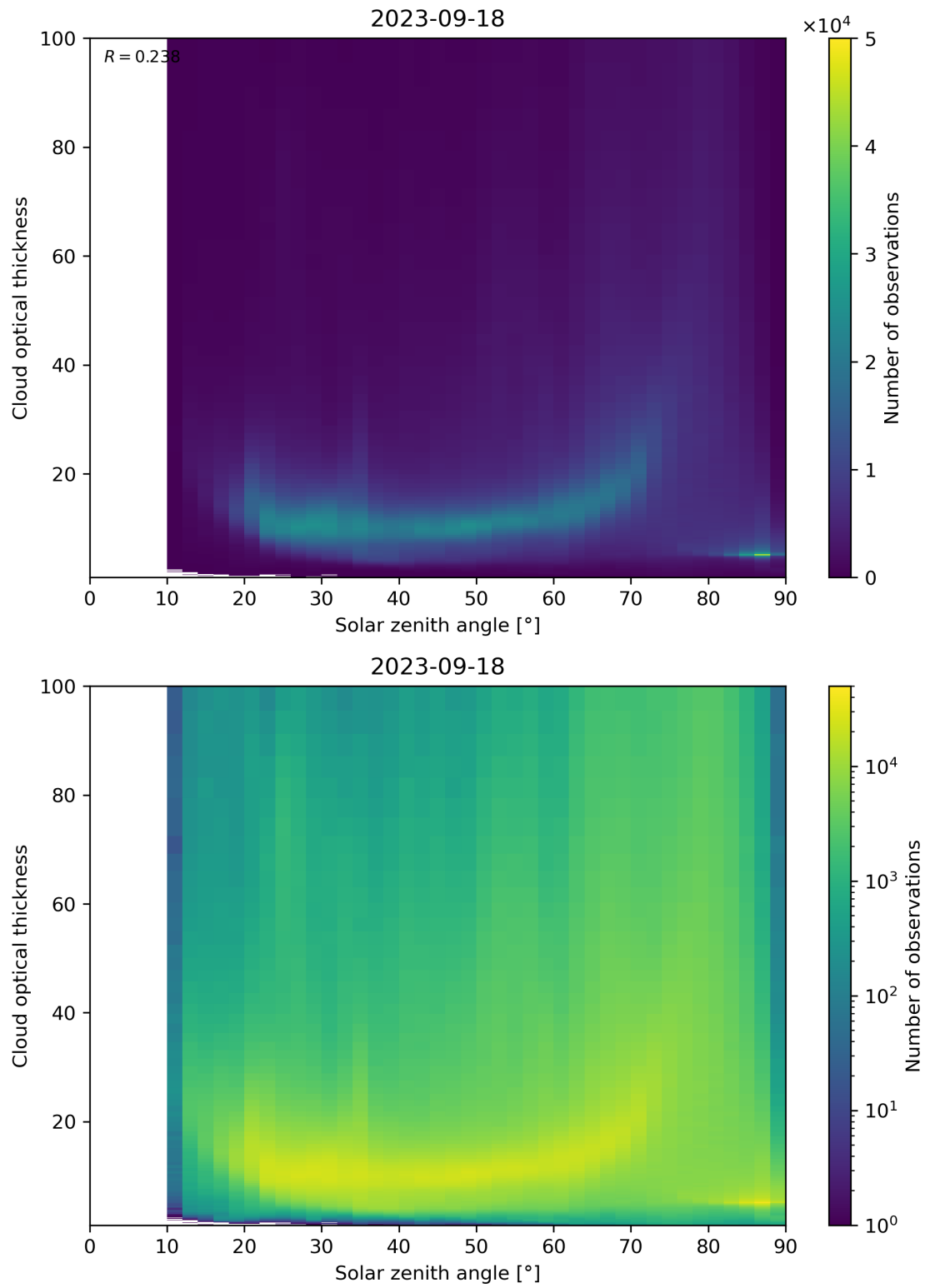
Figure 103: Scatter density plot of “Solar zenith angle” against “Cloud optical thickness” for 2023-09-17 to 2023-09-19.
