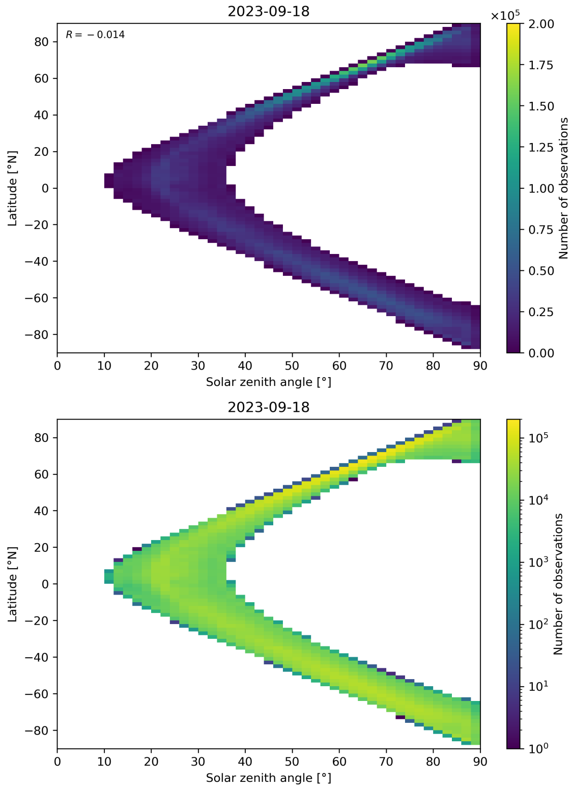
Figure 105: Scatter density plot of “Solar zenith angle” against “Latitude” for 2023-09-17 to 2023-09-19.
