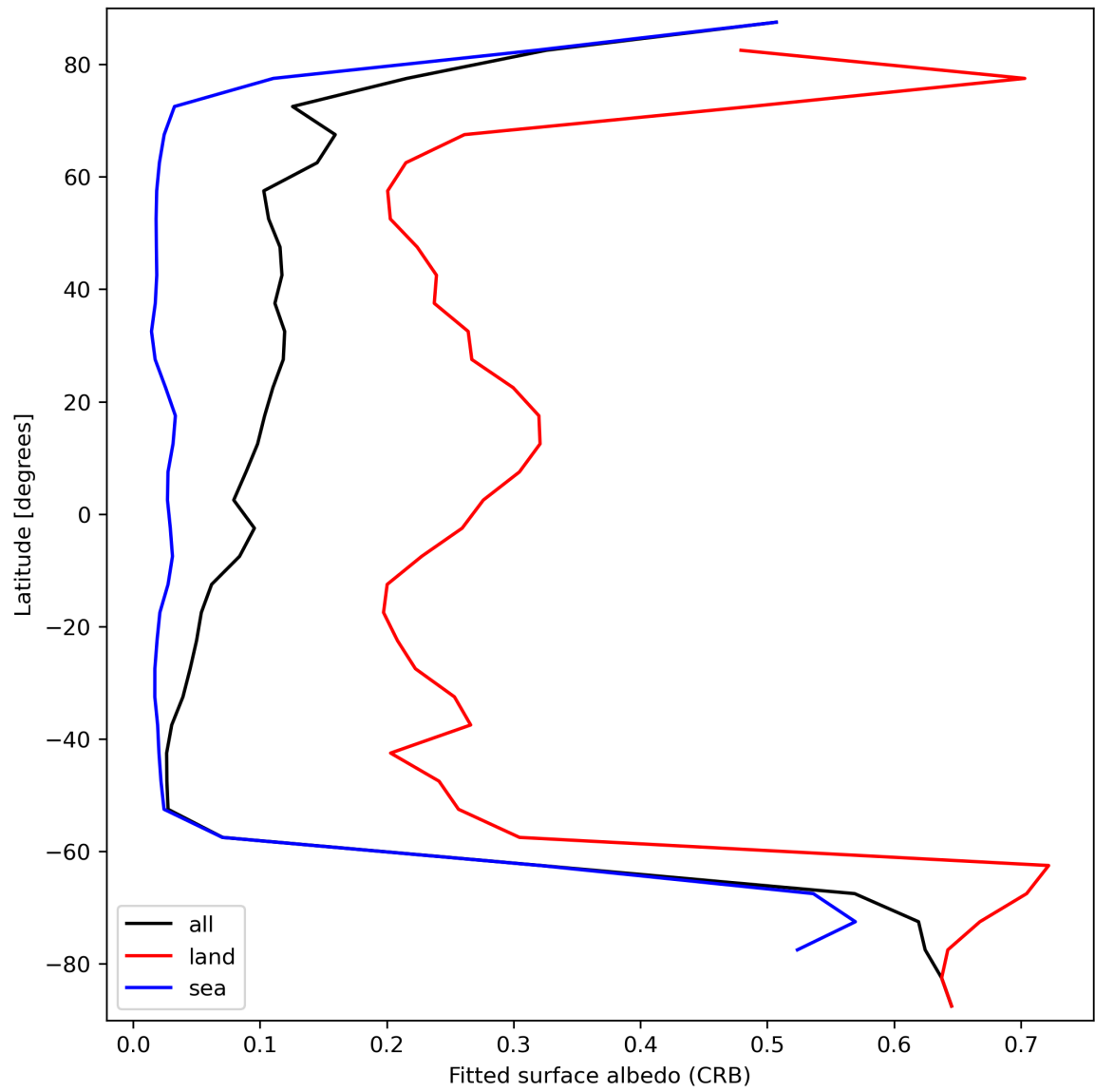
Figure 30: Zonal average of “Fitted surface albedo (CRB)” for 2023-09-17 to 2023-09-19.
