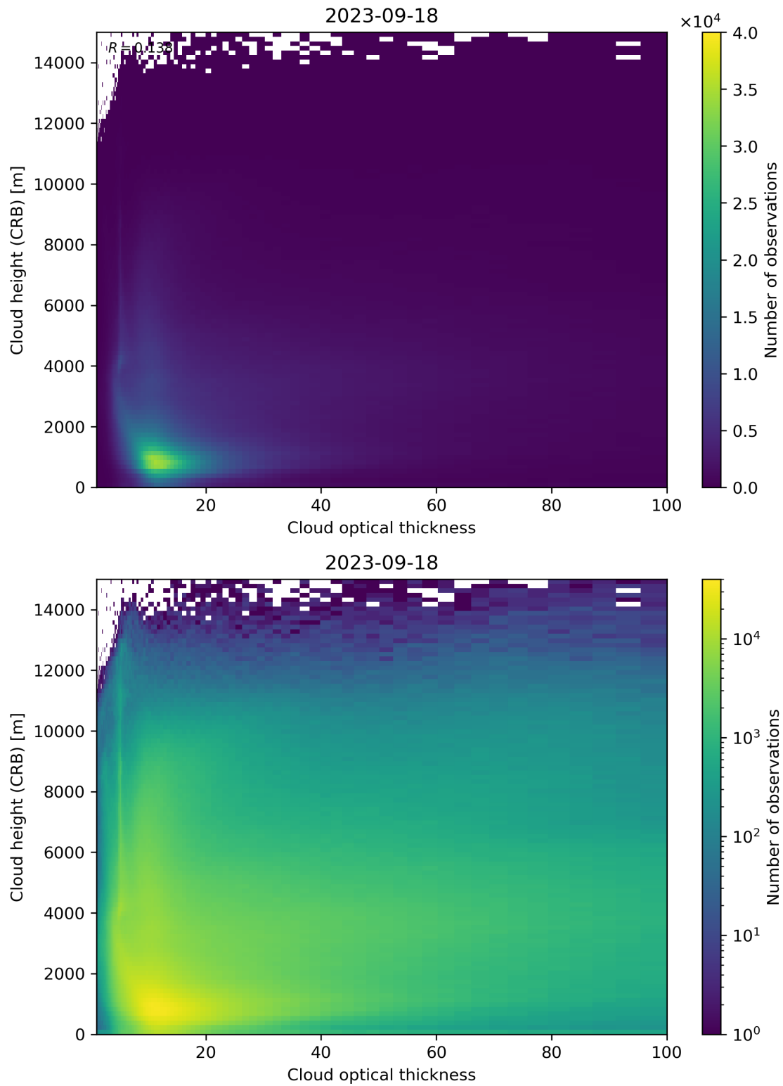
Figure 85: Scatter density plot of “Cloud optical thickness” against “Cloud height (CRB)” for 2023-09-17 to 2023-09-19.
