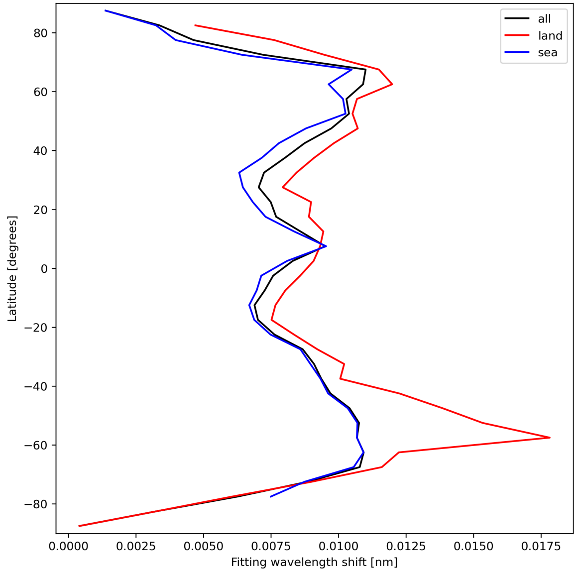
Figure 33: Zonal average of “Fitting wavelength shift” for 2023-09-17 to 2023-09-19.
