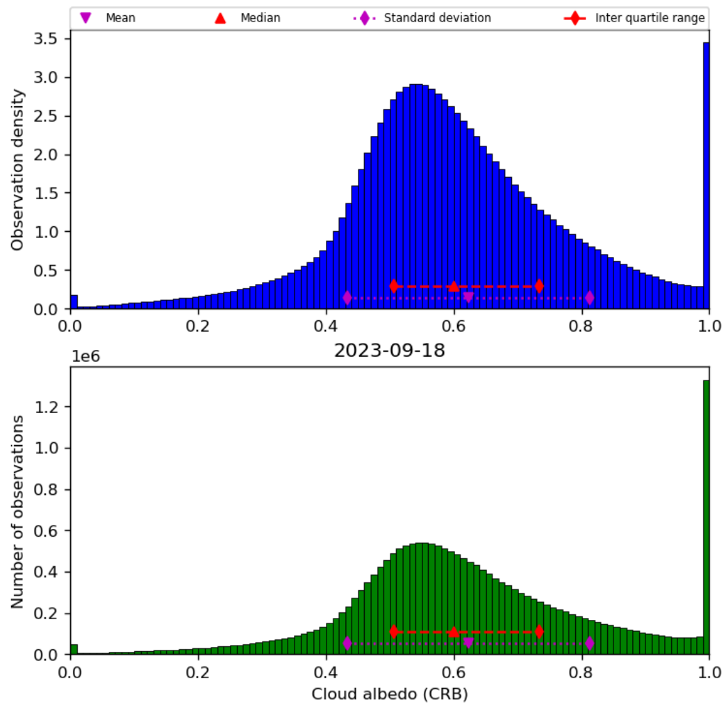
Figure 44: Histogram of “Cloud albedo (CRB)” for 2023-09-17 to 2023-09-19
