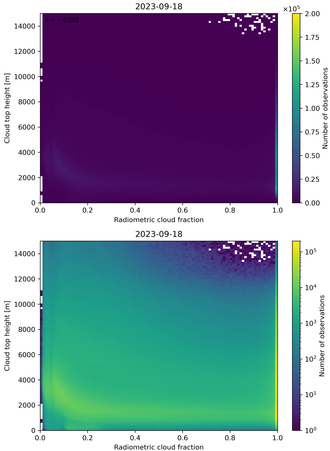
Figure 76: Scatter density plot of “Radiometric cloud fraction” against “Cloud top height” for 2023-09-17 to 2023-09-19.
