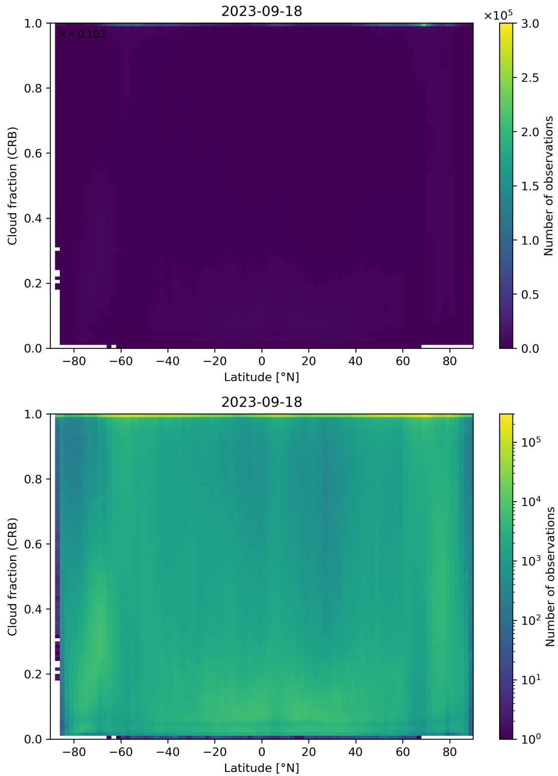
Figure 94: Scatter density plot of “Latitude” against “Cloud fraction (CRB)” for 2023-09-17 to 2023-09-19.
