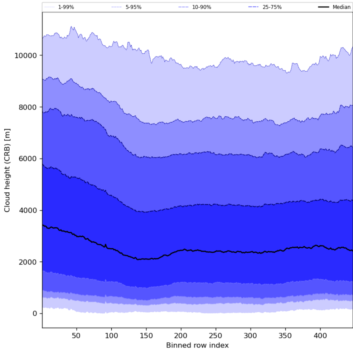
Figure 59: Along track statistics of “Cloud height (CRB)” for 2023-09-17 to 2023-09-19
