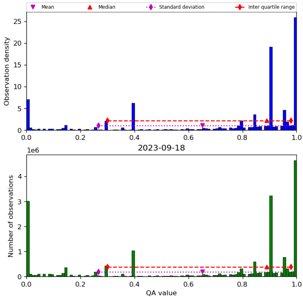
Figure 38: Histogram of “QA value” for 2023-09-17 to 2023-09-19
