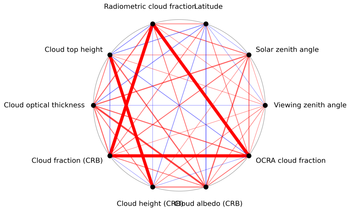
Figure 1: Map of correlation graph for 2023-09-18 to 2023-09-20.
