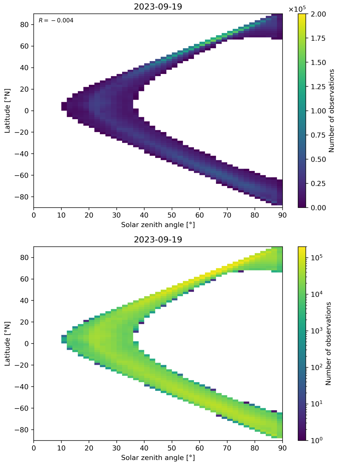
Figure 105: Scatter density plot of “Solar zenith angle” against “Latitude” for 2023-09-18 to 2023-09-20.
