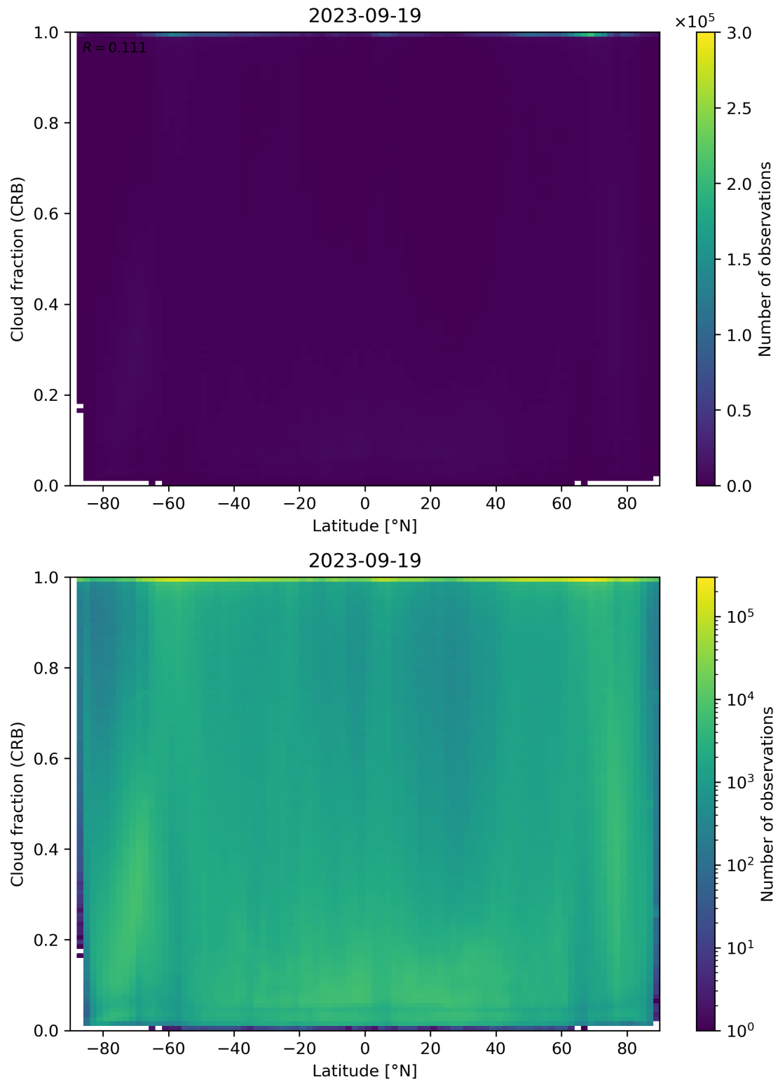
Figure 94: Scatter density plot of “Latitude” against “Cloud fraction (CRB)” for 2023-09-18 to 2023-09-20.
