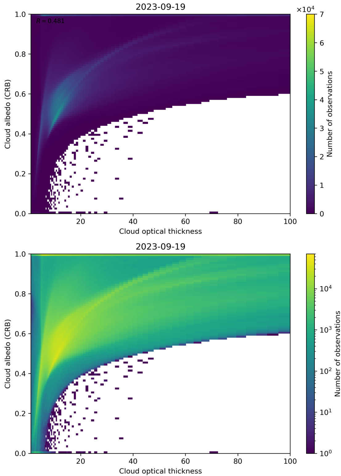
Figure 82: Scatter density plot of “Cloud optical thickness” against “Cloud albedo (CRB)” for 2023-09-18 to 2023-09-20.
