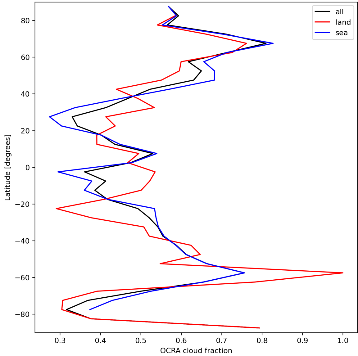
Figure 34: Zonal average of “OCRA cloud fraction” for 2023-09-18 to 2023-09-20.
