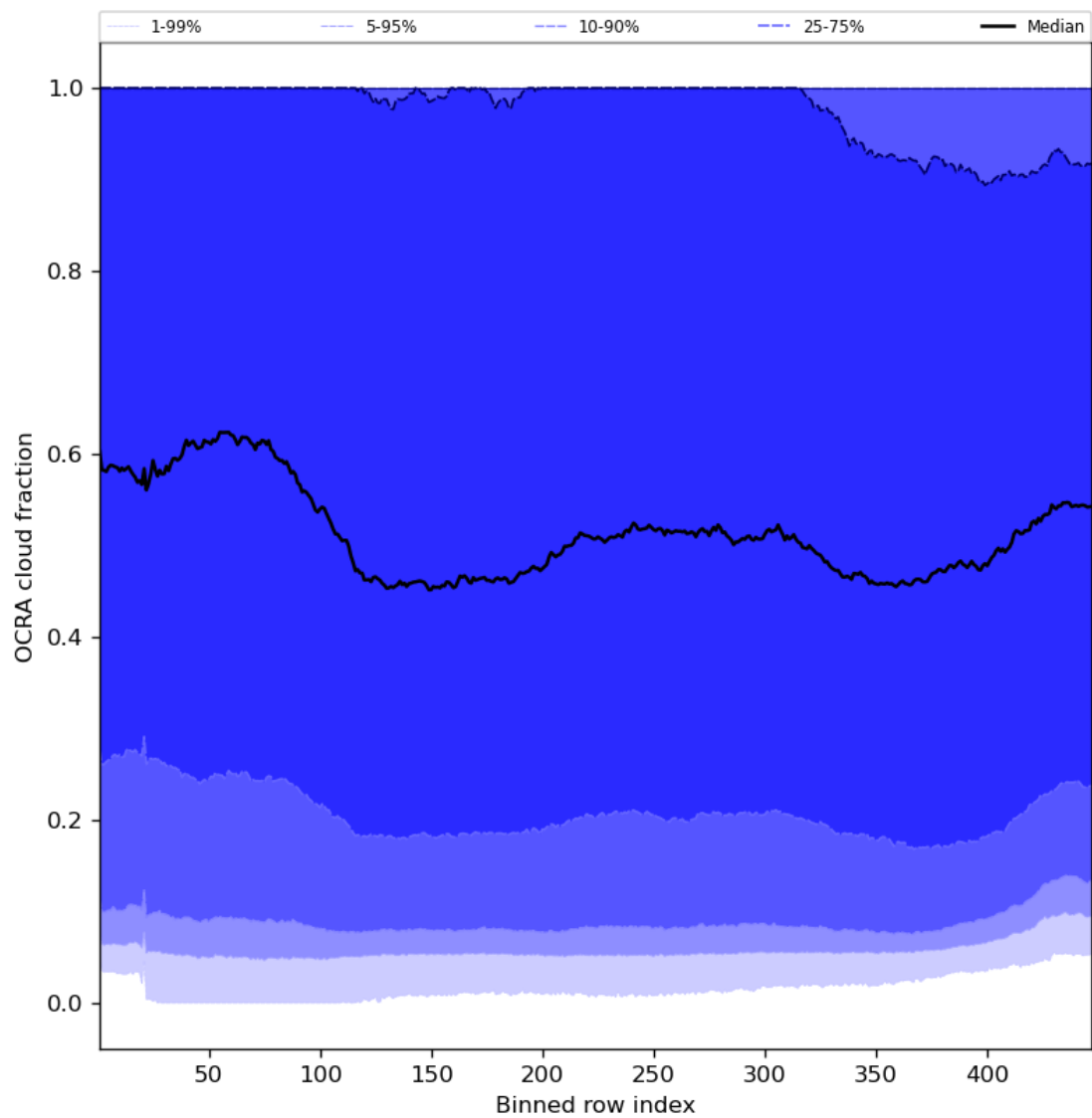
Figure 66: Along track statistics of “OCRA cloud fraction” for 2023-09-18 to 2023-09-20
