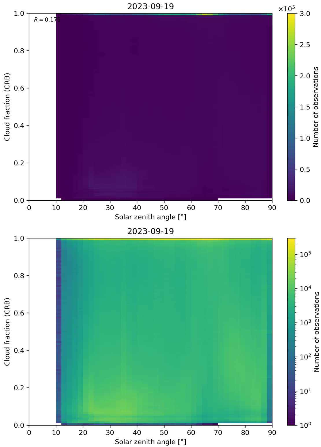
Figure 101: Scatter density plot of “Solar zenith angle” against “Cloud fraction (CRB)” for 2023-09-18 to 2023-09-20.
