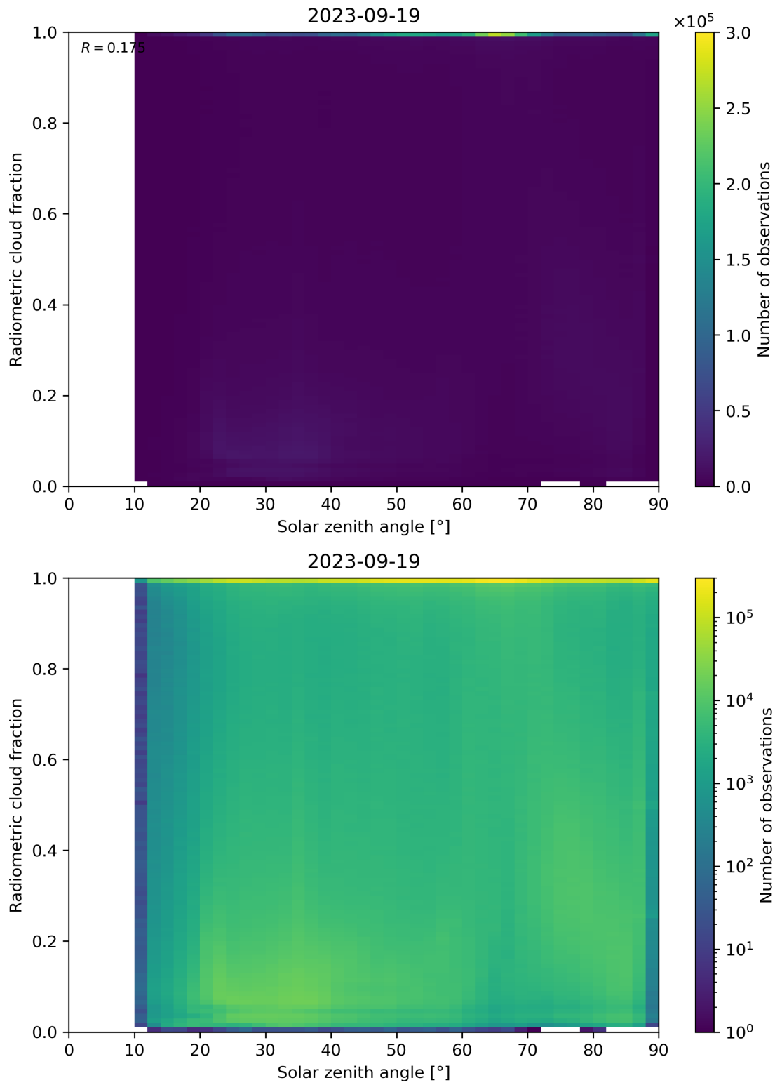
Figure 99: Scatter density plot of “Solar zenith angle” against “Radiometric cloud fraction” for 2023-09-18 to 2023-09-20.
