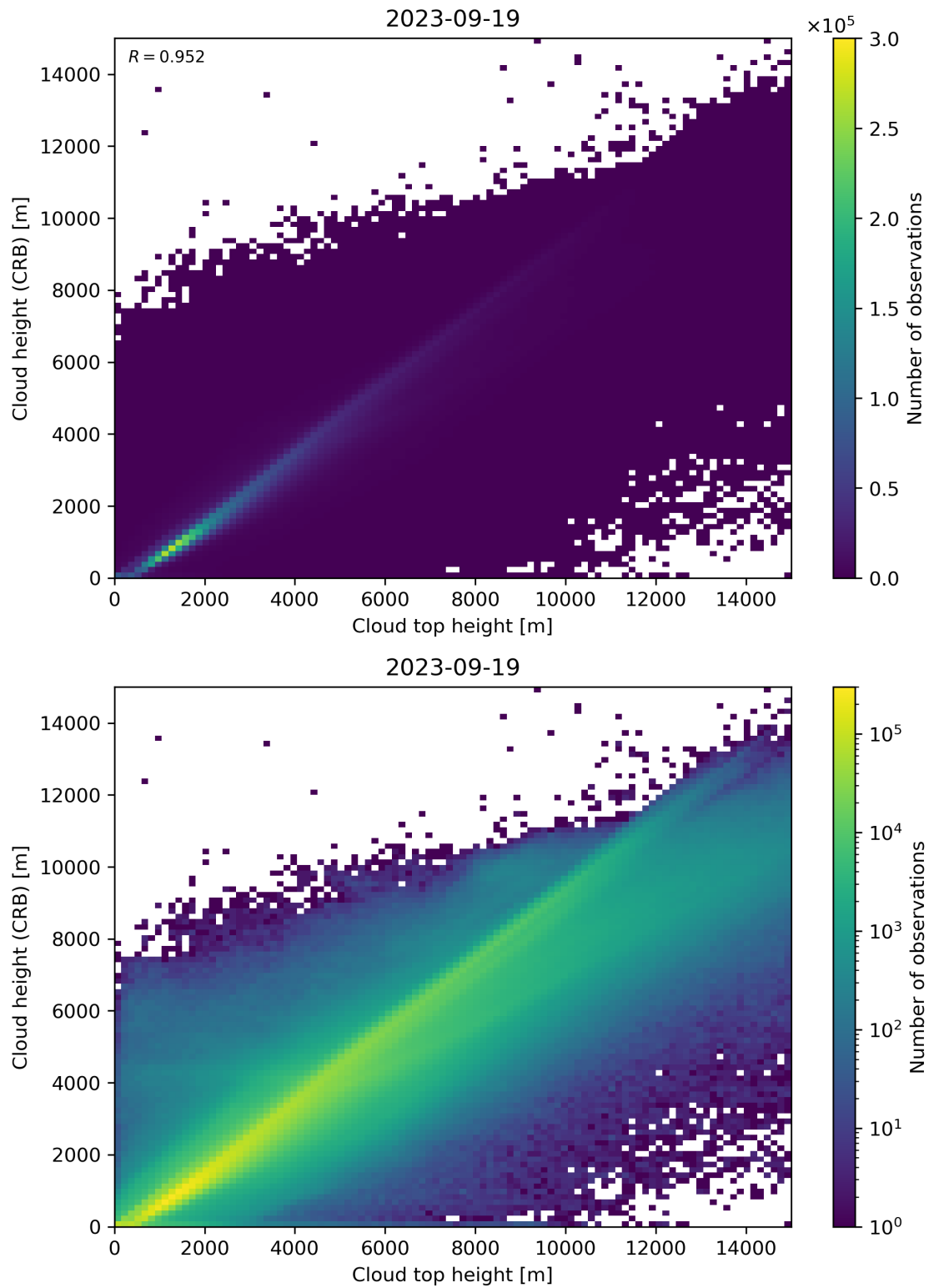
Figure 89: Scatter density plot of “Cloud top height” against “Cloud height (CRB)” for 2023-09-18 to 2023-09-20.
