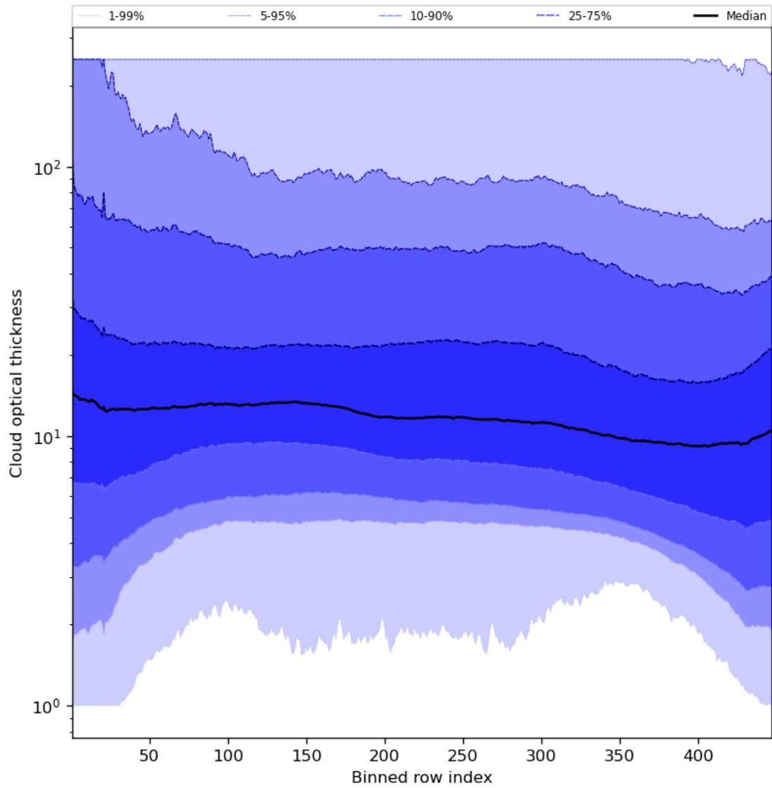
Figure 57: Along track statistics of “Cloud optical thickness” for 2023-09-18 to 2023-09-20
