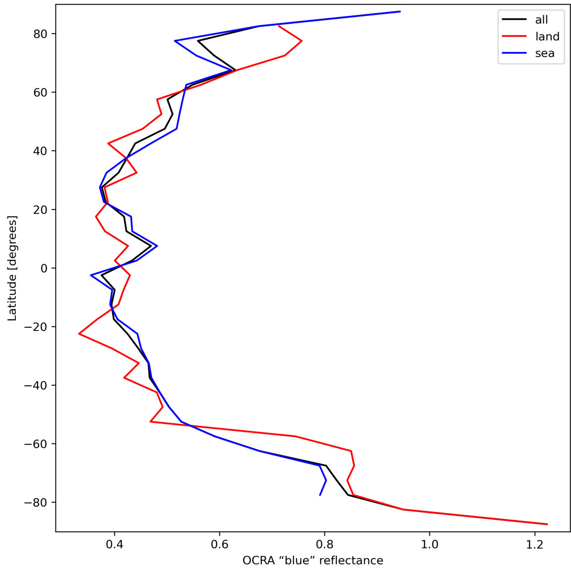
Figure 35: Zonal average of “OCRA “blue” reflectance” for 2023-09-18 to 2023-09-20.
