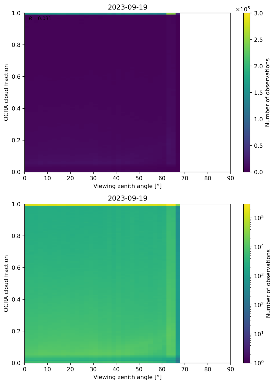
Figure 108: Scatter density plot of “Viewing zenith angle” against “OCRA cloud fraction” for 2023-09-18 to 2023-09-20.
