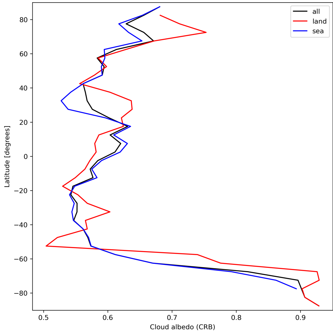
Figure 28: Zonal average of “Cloud albedo (CRB)” for 2023-09-18 to 2023-09-20.
