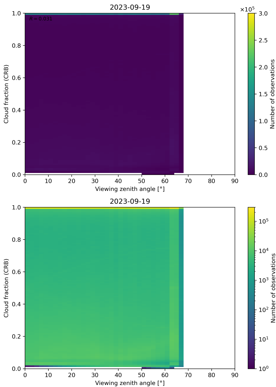
Figure 109: Scatter density plot of “Viewing zenith angle” against “Cloud fraction (CRB)” for 2023-09-18 to 2023-09-20.
