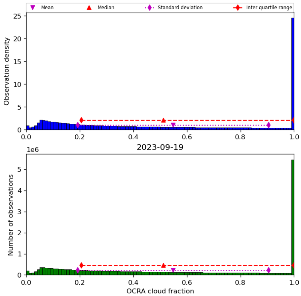
Figure 50: Histogram of “OCRA cloud fraction” for 2023-09-18 to 2023-09-20
