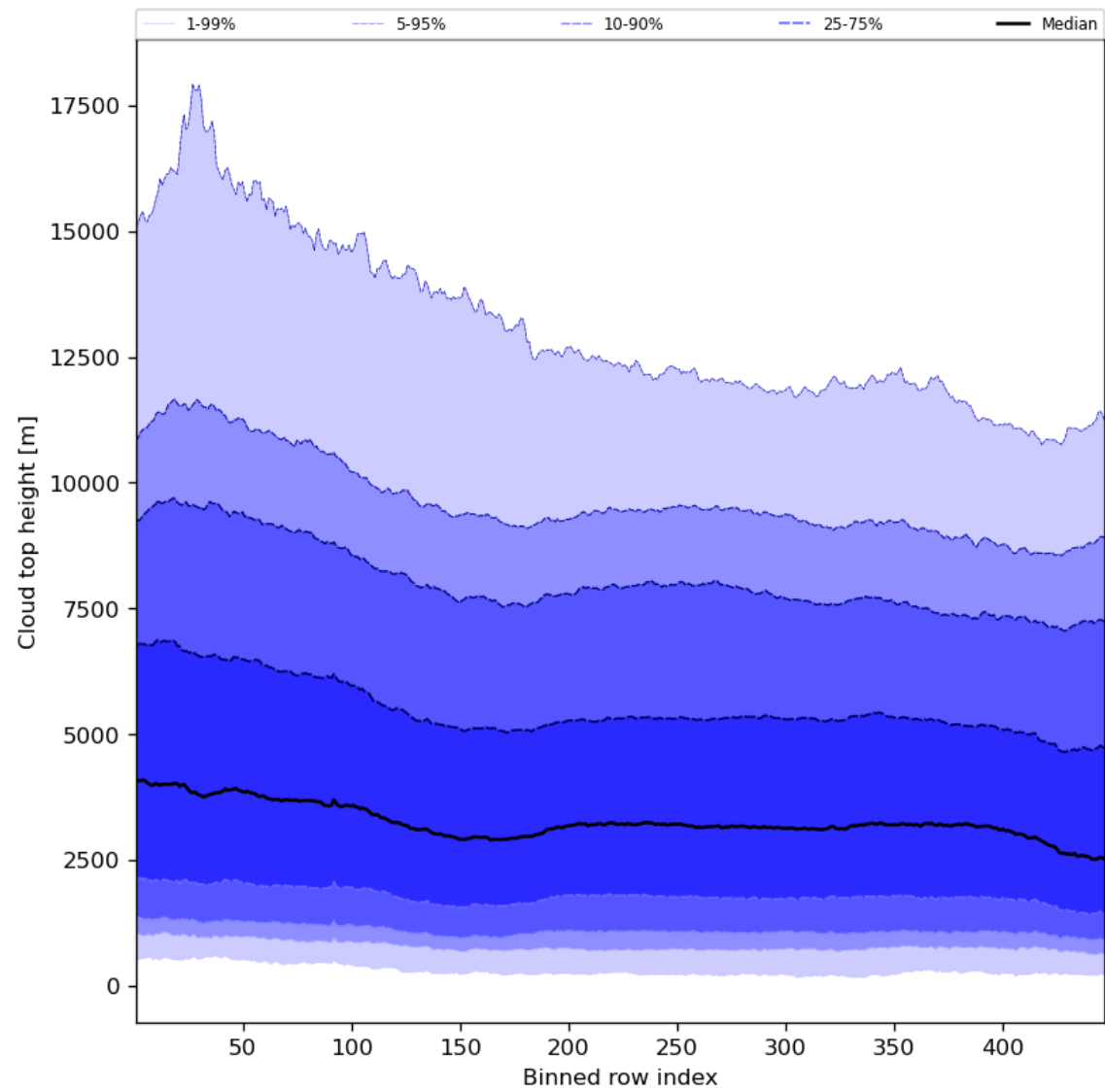
Figure 56: Along track statistics of “Cloud top height” for 2023-09-18 to 2023-09-20
