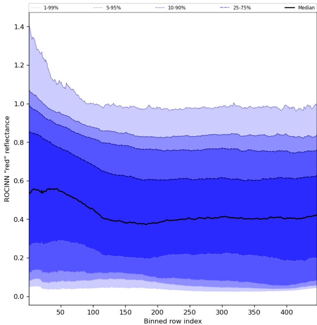
Figure 69: Along track statistics of “ROCINN “red” reflectance” for 2023-09-18 to 2023-09-20
