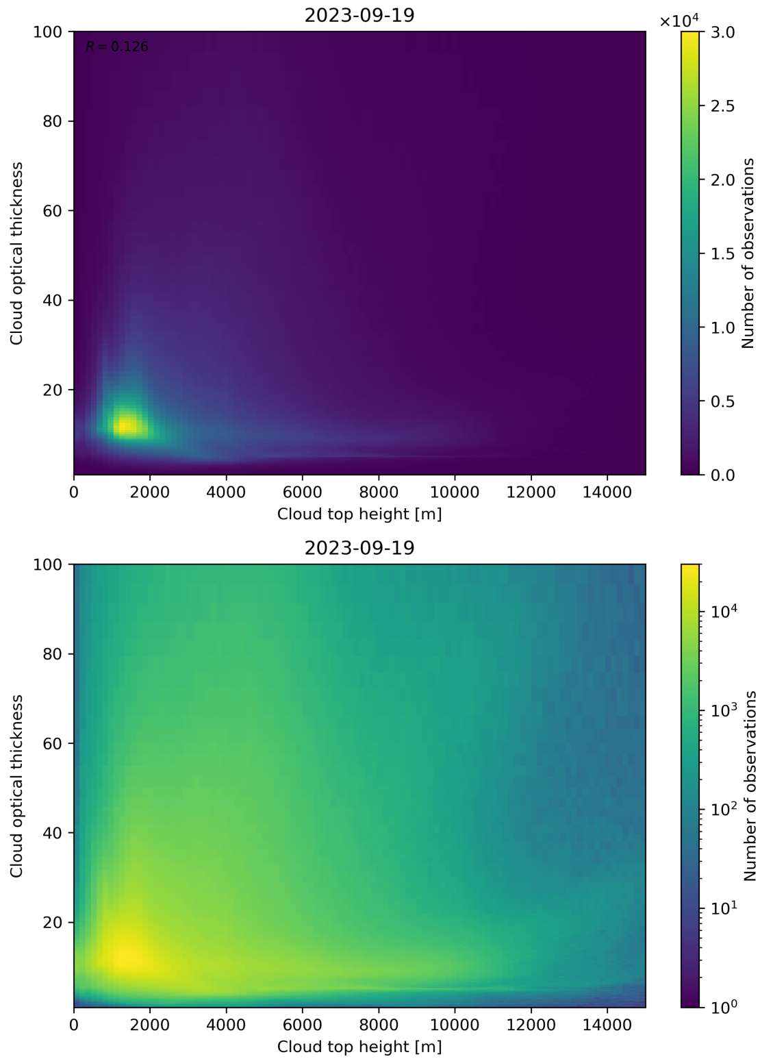
Figure 90: Scatter density plot of “Cloud top height” against “Cloud optical thickness” for 2023-09-18 to 2023-09-20.
