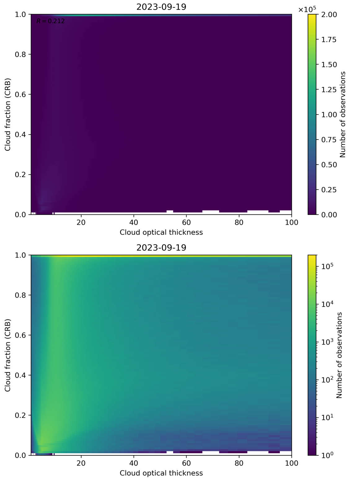
Figure 84: Scatter density plot of “Cloud optical thickness” against “Cloud fraction (CRB)” for 2023-09-18 to 2023-09-20.
