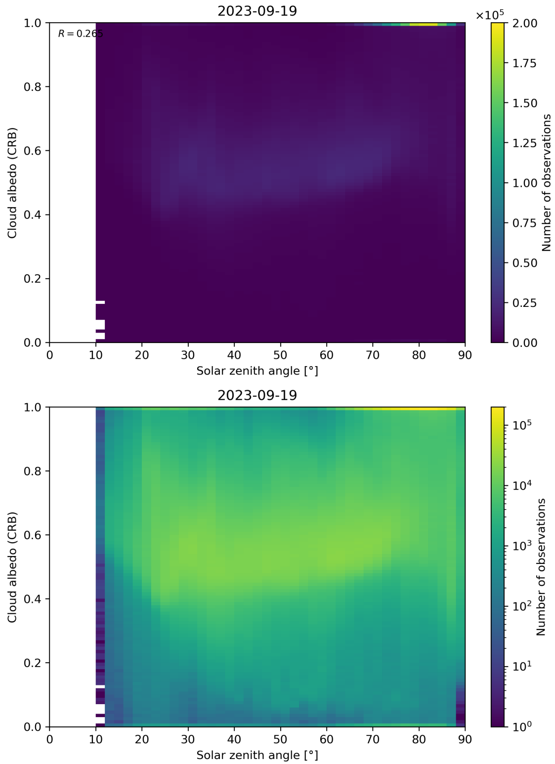
Figure 98: Scatter density plot of “Solar zenith angle” against “Cloud albedo (CRB)” for 2023-09-18 to 2023-09-20.
