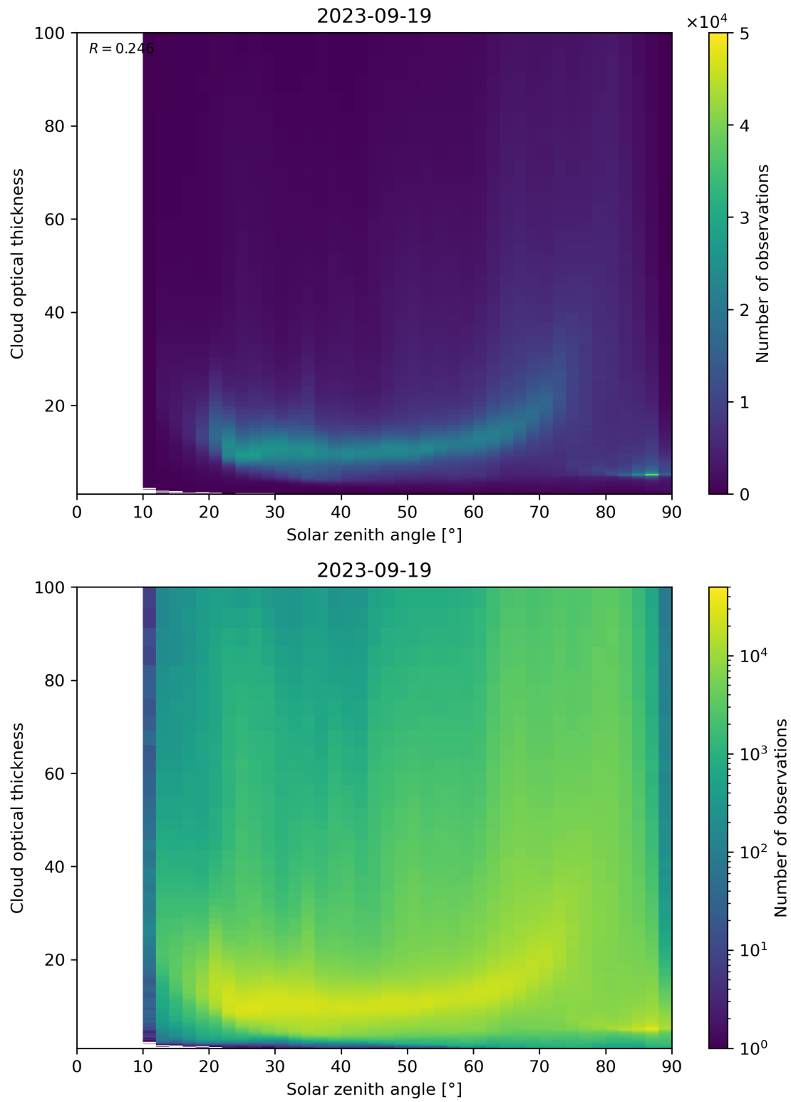
Figure 103: Scatter density plot of “Solar zenith angle” against “Cloud optical thickness” for 2023-09-18 to 2023-09-20.
