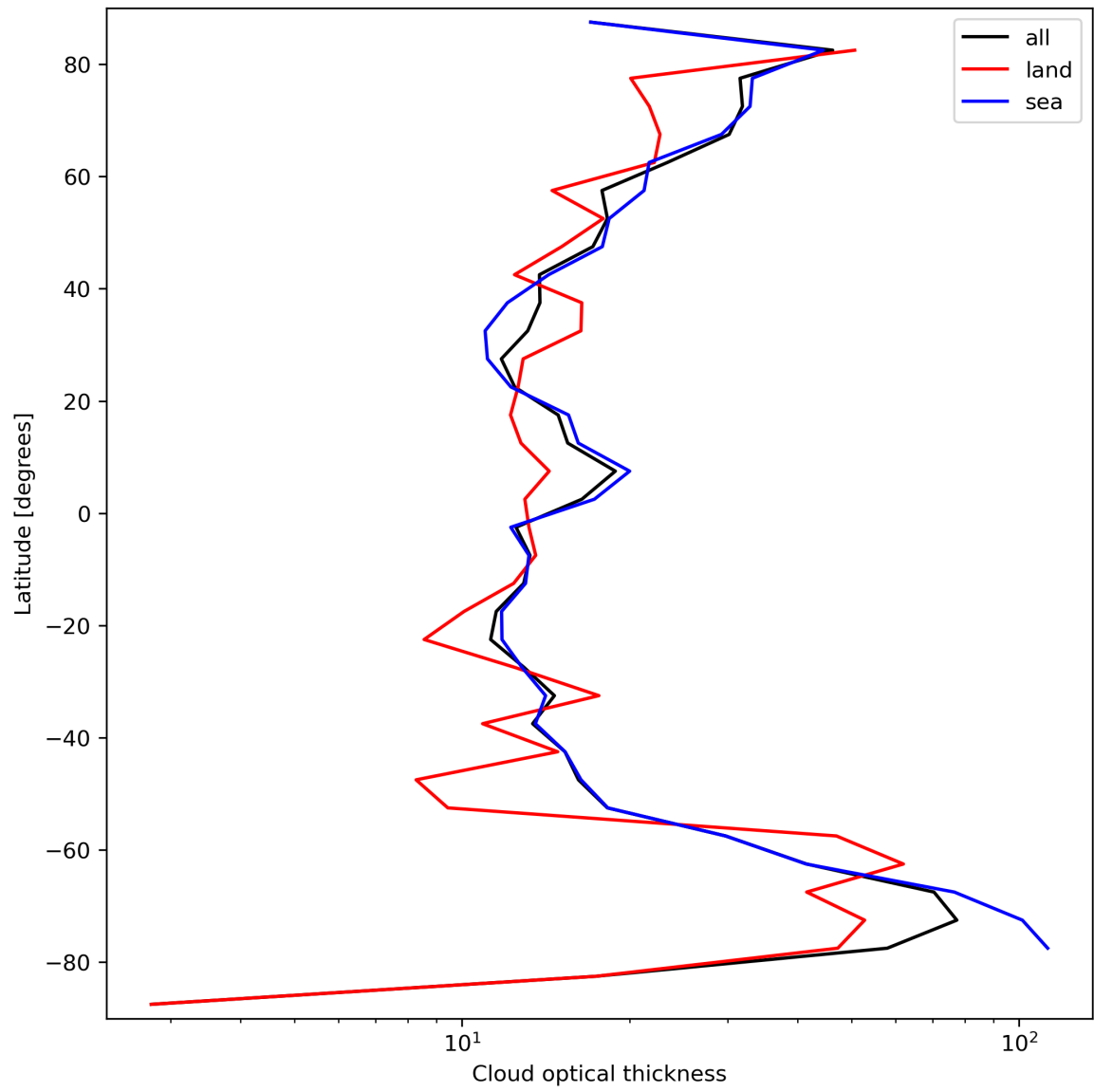
Figure 25: Zonal average of “Cloud optical thickness” for 2023-09-18 to 2023-09-20.
