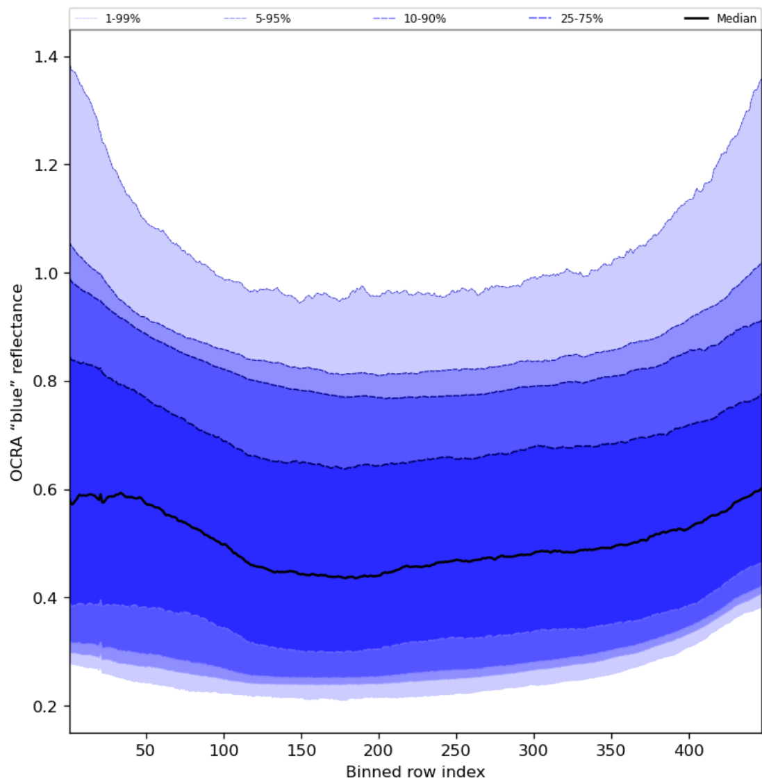
Figure 67: Along track statistics of “OCRA “blue” reflectance” for 2023-09-18 to 2023-09-20
