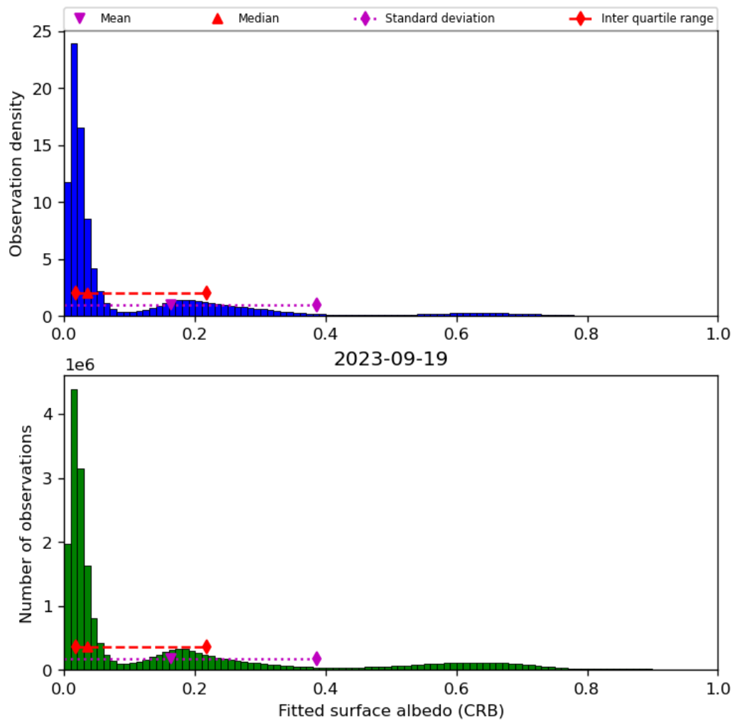
Figure 46: Histogram of “Fitted surface albedo (CRB)” for 2023-09-18 to 2023-09-20
