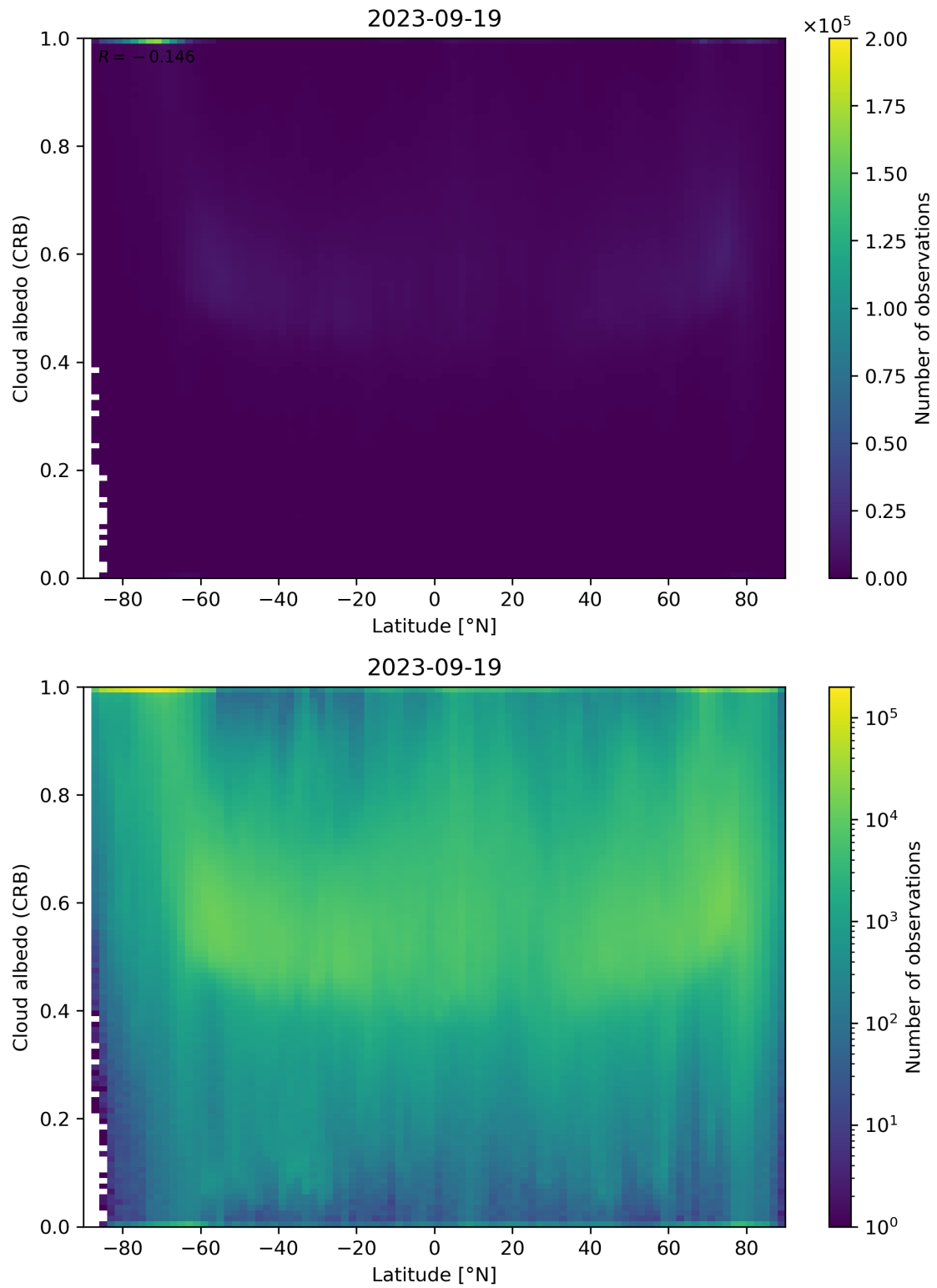
Figure 91: Scatter density plot of “Latitude” against “Cloud albedo (CRB)” for 2023-09-18 to 2023-09-20.
