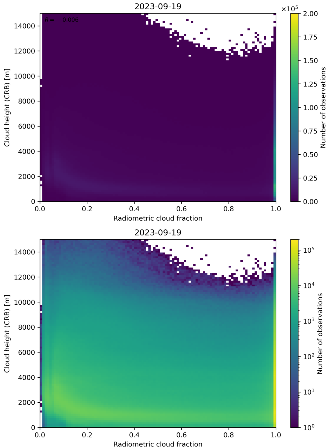
Figure 74: Scatter density plot of “Radiometric cloud fraction” against “Cloud height (CRB)” for 2023-09-18 to 2023-09-20.
