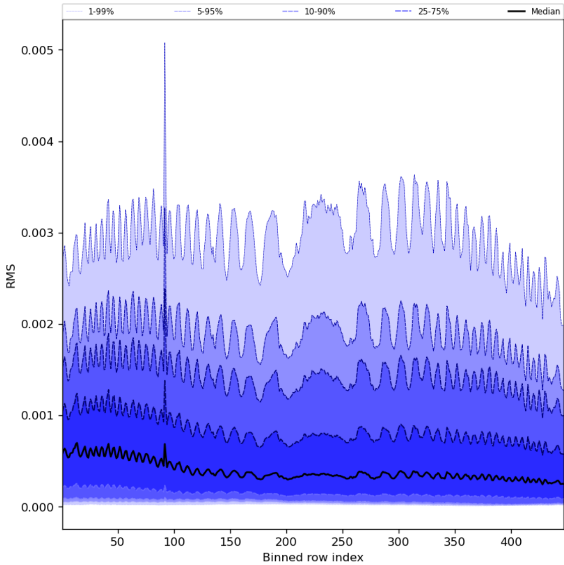
Figure 63: Along track statistics of “RMS” for 2023-09-18 to 2023-09-20
