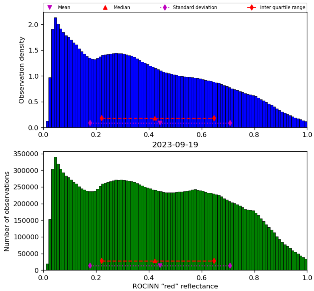
Figure 53: Histogram of “ROCINN “red” reflectance” for 2023-09-18 to 2023-09-20
