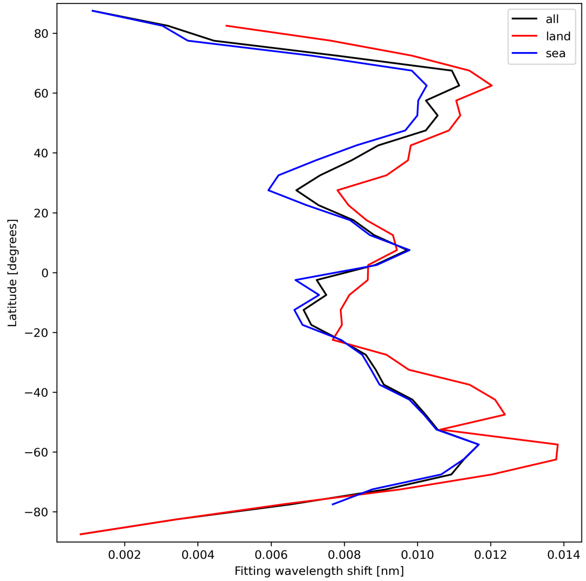
Figure 33: Zonal average of “Fitting wavelength shift” for 2023-09-18 to 2023-09-20.
