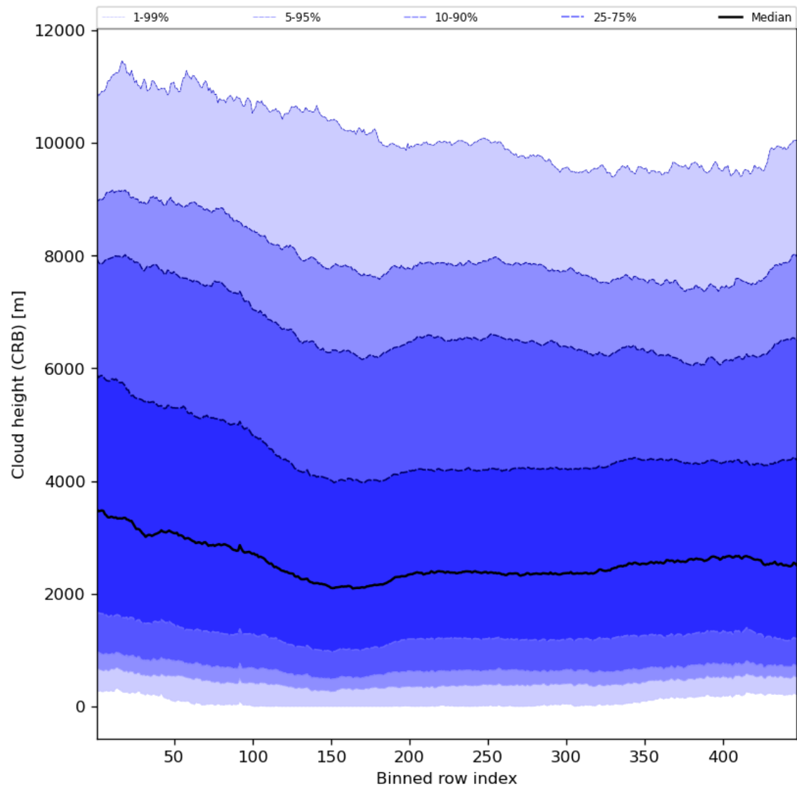
Figure 59: Along track statistics of “Cloud height (CRB)” for 2023-09-18 to 2023-09-20
