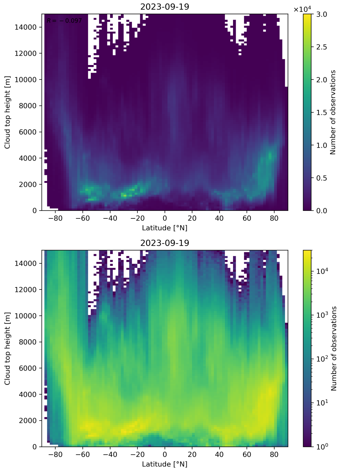
Figure 97: Scatter density plot of “Latitude” against “Cloud top height” for 2023-09-18 to 2023-09-20.
