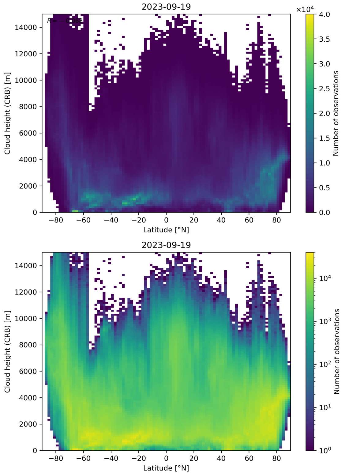
Figure 95: Scatter density plot of “Latitude” against “Cloud height (CRB)” for 2023-09-18 to 2023-09-20.
