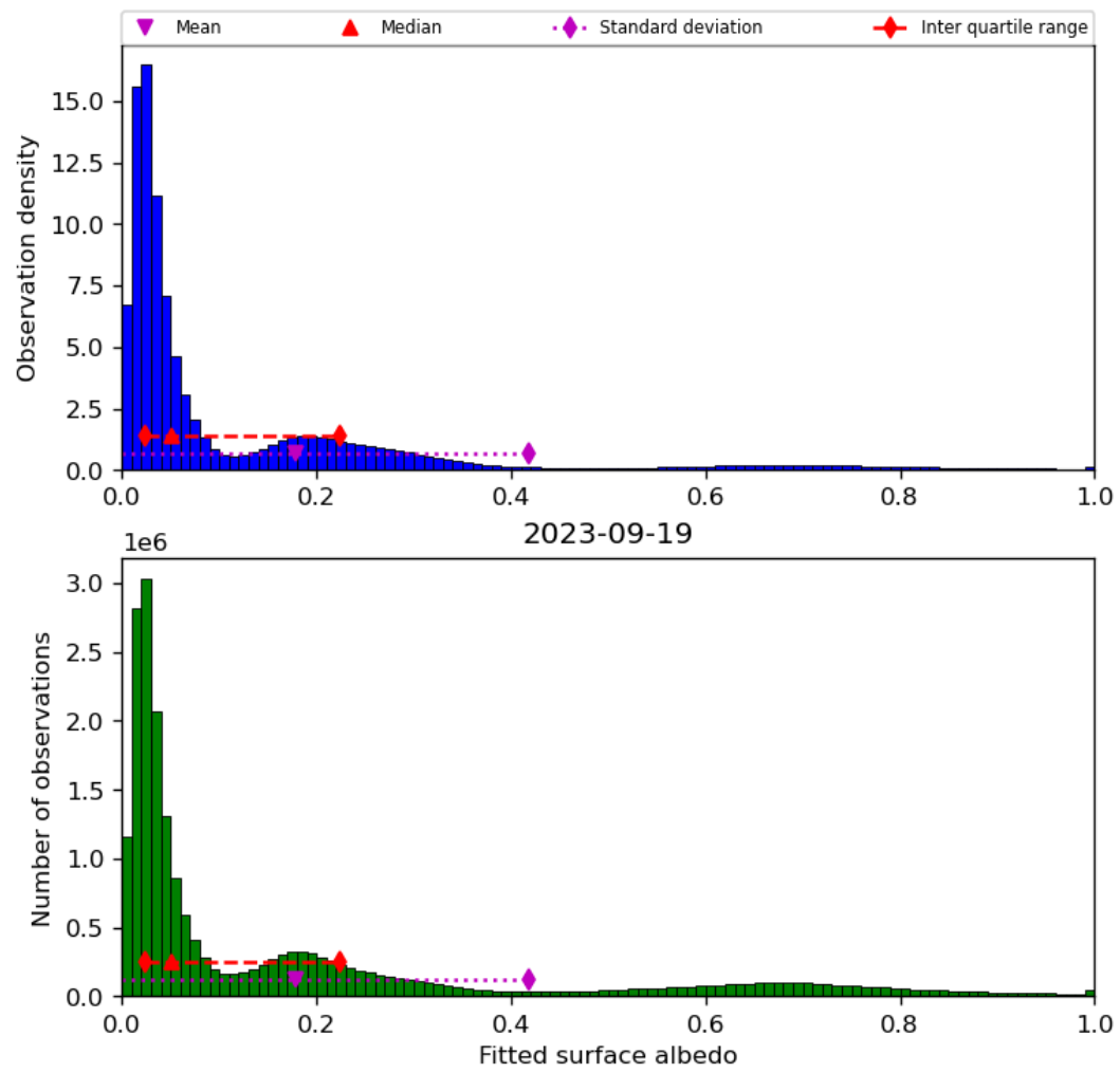
Figure 45: Histogram of “Fitted surface albedo” for 2023-09-18 to 2023-09-20
