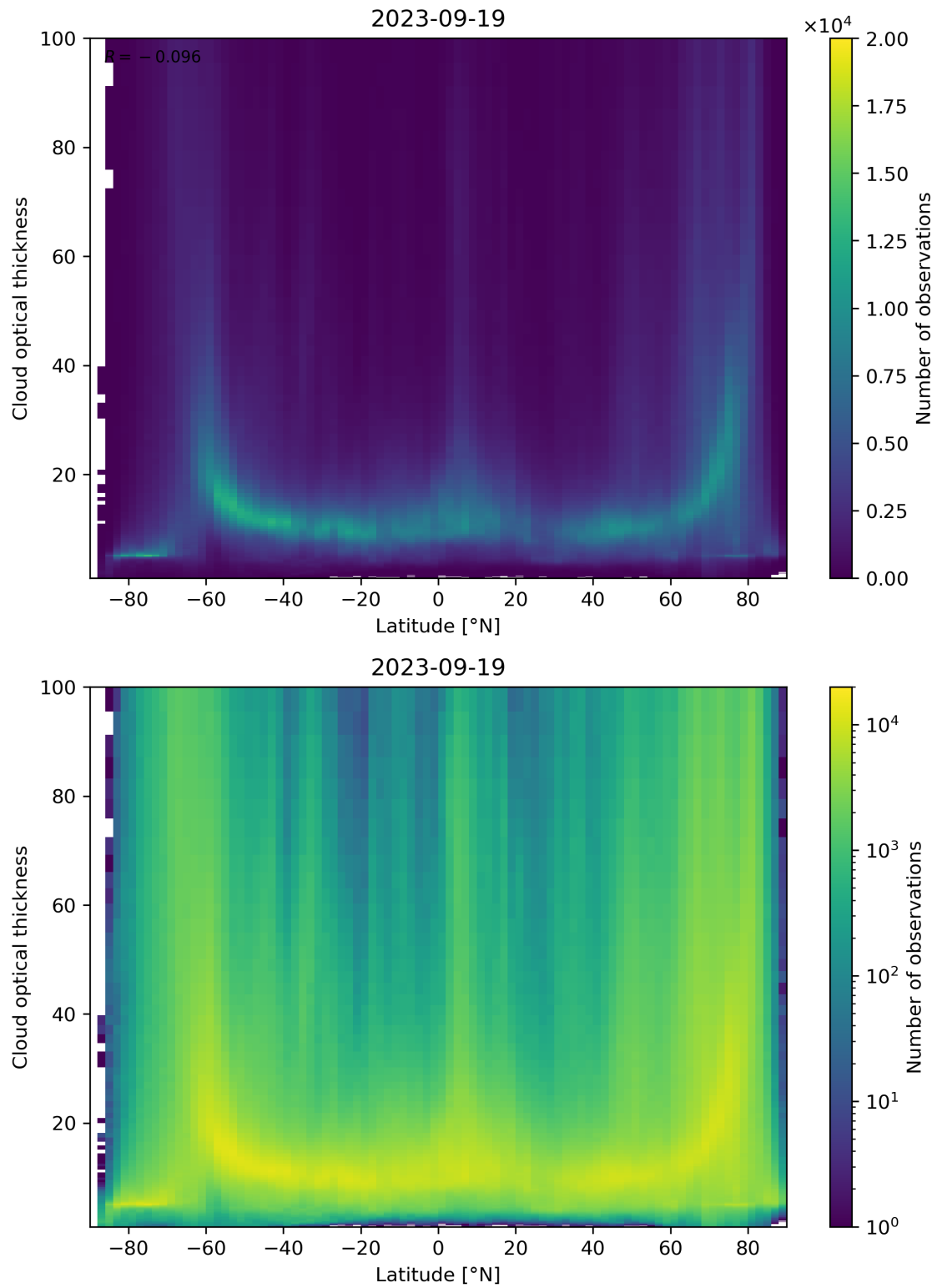
Figure 96: Scatter density plot of “Latitude” against “Cloud optical thickness” for 2023-09-18 to 2023-09-20.
