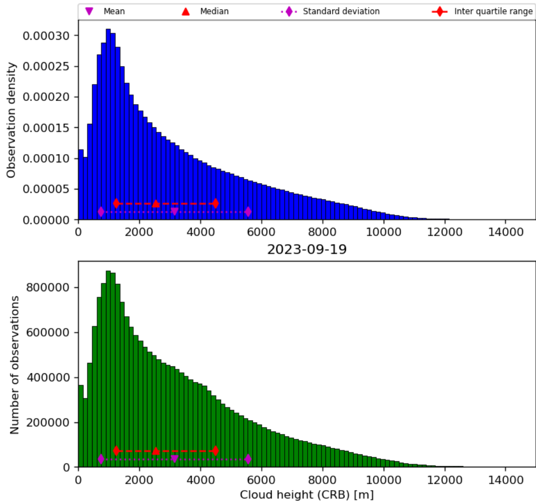
Figure 43: Histogram of “Cloud height (CRB)” for 2023-09-18 to 2023-09-20
