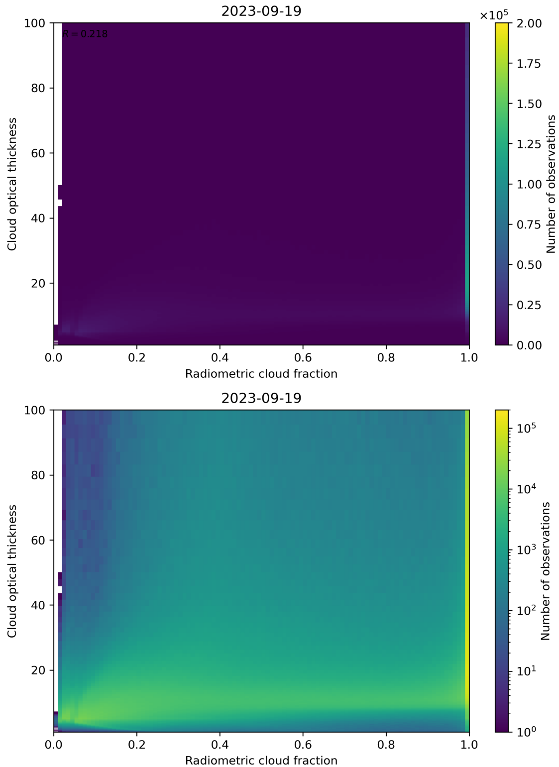
Figure 75: Scatter density plot of “Radiometric cloud fraction” against “Cloud optical thickness” for 2023-09-18 to 2023-09-20.
