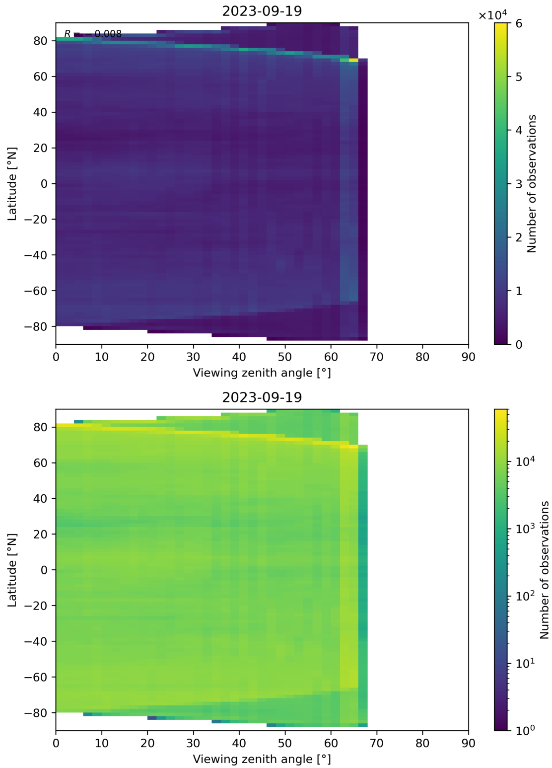
Figure 113: Scatter density plot of “Viewing zenith angle” against “Latitude” for 2023-09-18 to 2023-09-20.
