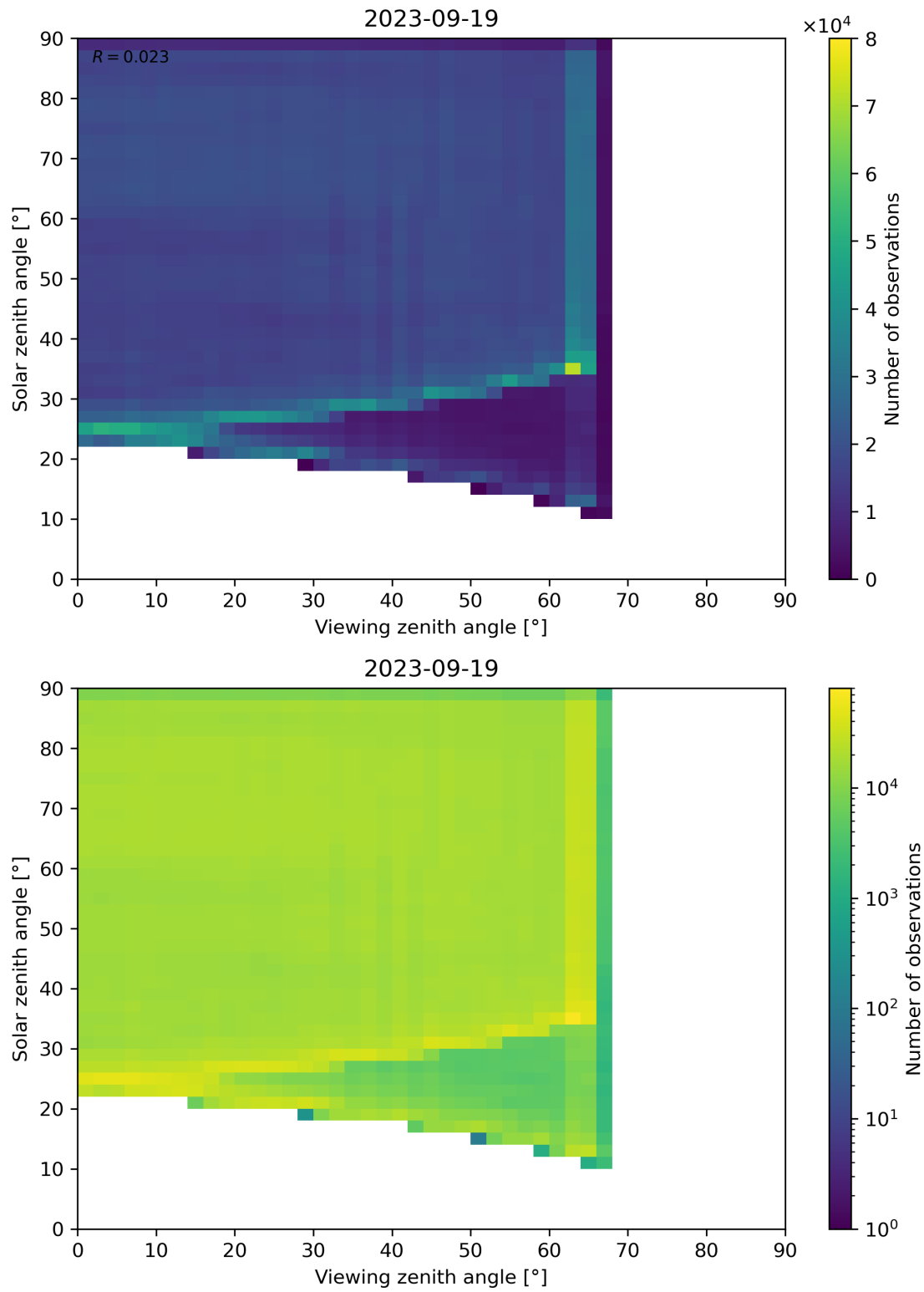
Figure 114: Scatter density plot of “Viewing zenith angle” against “Solar zenith angle” for 2023-09-18 to 2023-09-20.
