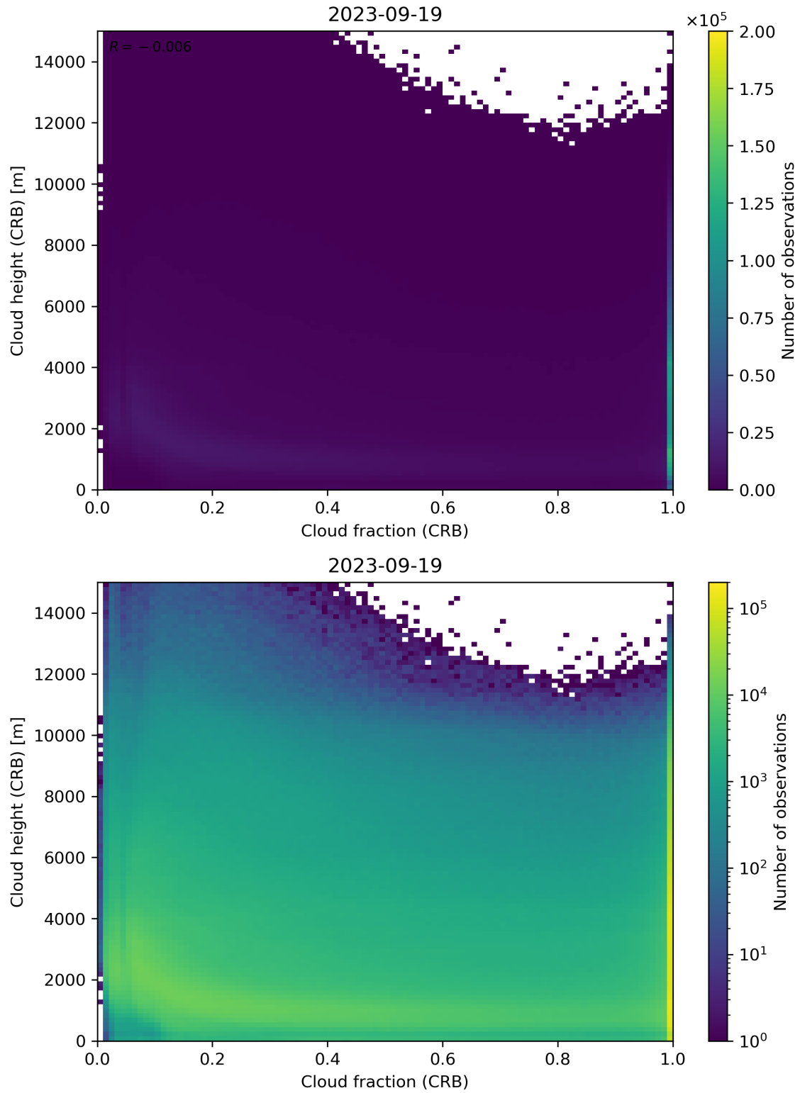
Figure 79: Scatter density plot of “Cloud fraction (CRB)” against “Cloud height (CRB)” for 2023-09-18 to 2023-09-20.
