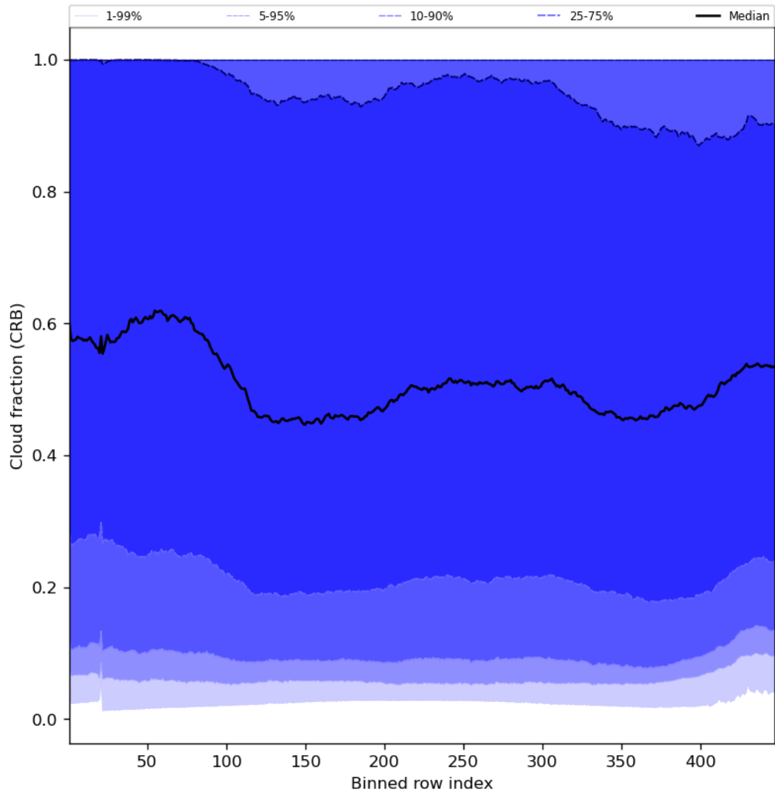
Figure 58: Along track statistics of “Cloud fraction (CRB)” for 2023-09-18 to 2023-09-20
