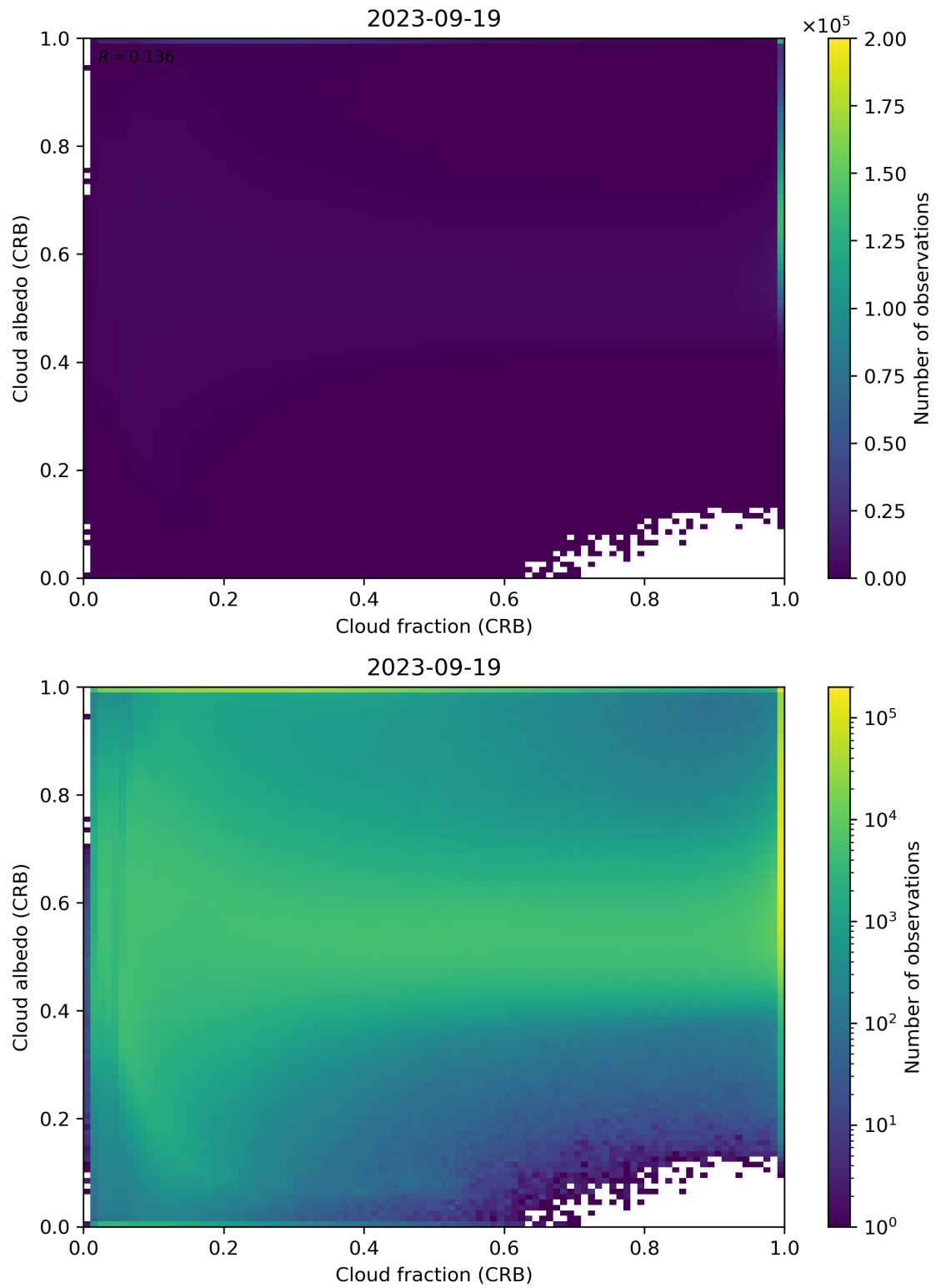
Figure 77: Scatter density plot of “Cloud fraction (CRB)” against “Cloud albedo (CRB)” for 2023-09-18 to 2023-09-20.
