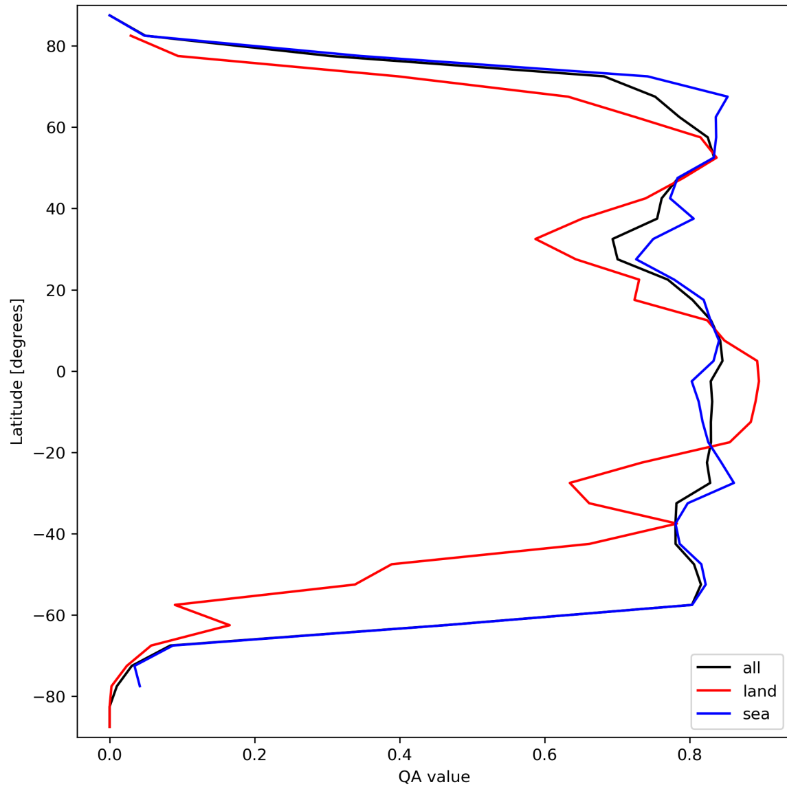
Figure 22: Zonal average of “QA value” for 2023-09-18 to 2023-09-20.
