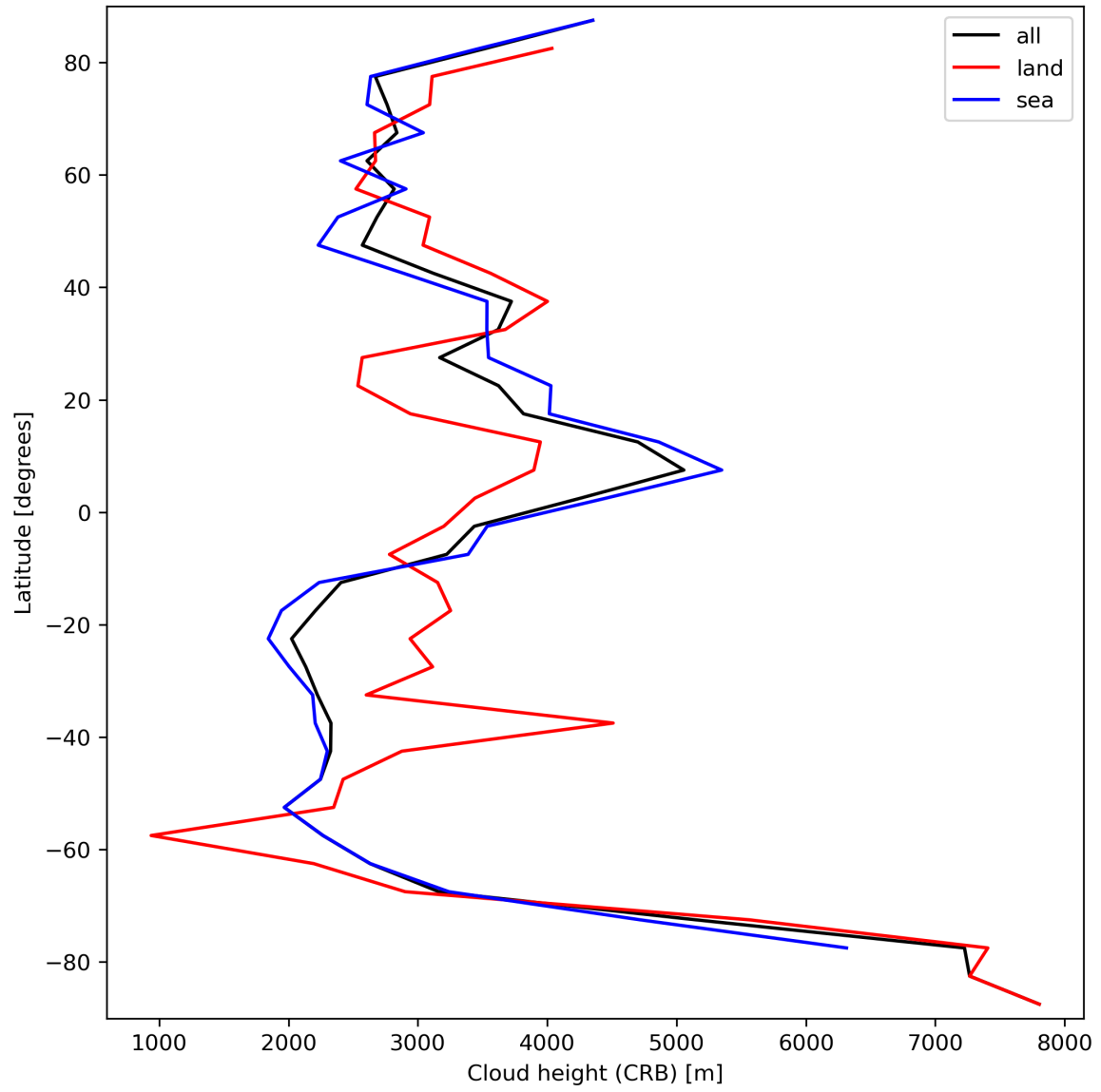
Figure 27: Zonal average of “Cloud height (CRB)” for 2023-09-18 to 2023-09-20.
