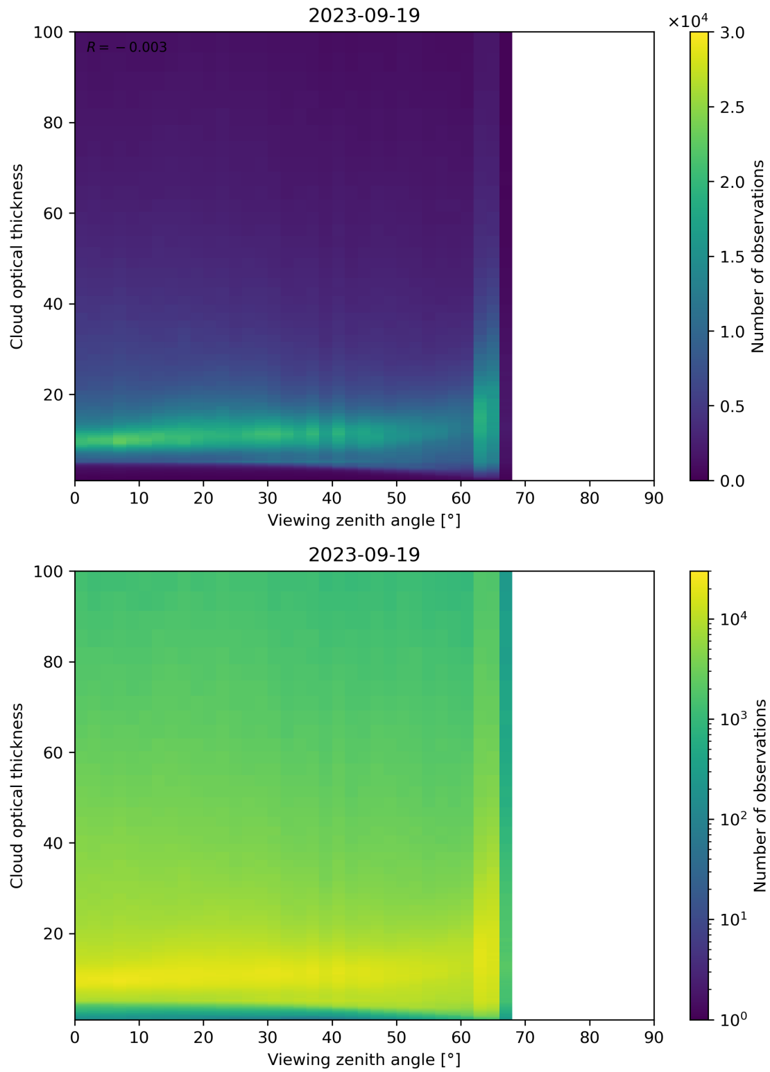
Figure 111: Scatter density plot of “Viewing zenith angle” against “Cloud optical thickness” for 2023-09-18 to 2023-09-20.
