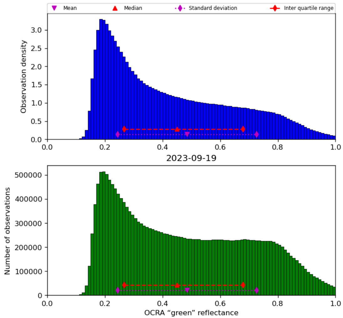
Figure 52: Histogram of “OCRA “green” reflectance” for 2023-09-18 to 2023-09-20
