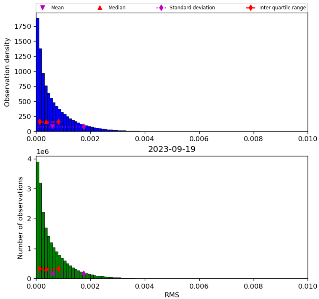
Figure 47: Histogram of “RMS” for 2023-09-18 to 2023-09-20
