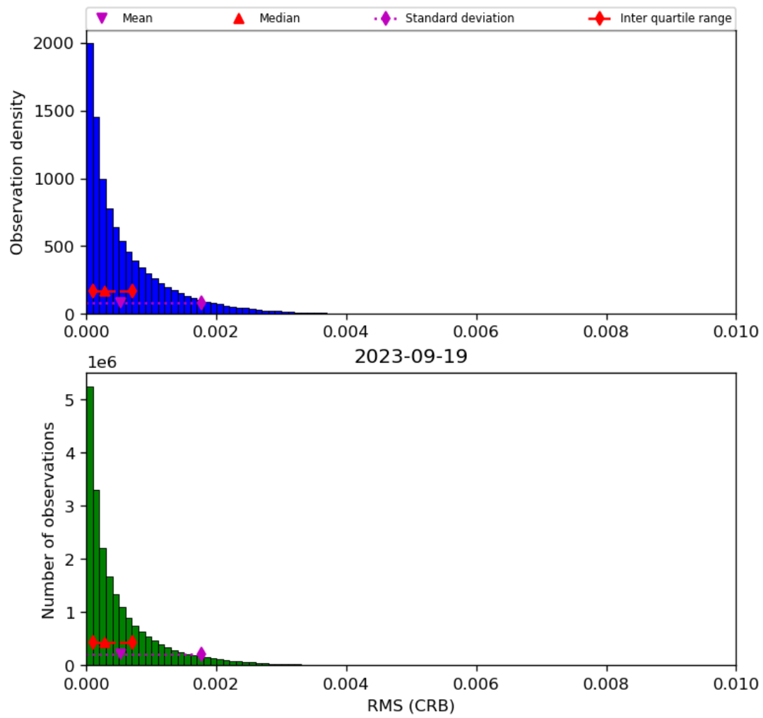
Figure 48: Histogram of “RMS (CRB)” for 2023-09-18 to 2023-09-20
