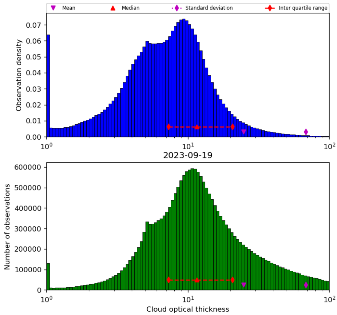
Figure 41: Histogram of “Cloud optical thickness” for 2023-09-18 to 2023-09-20
