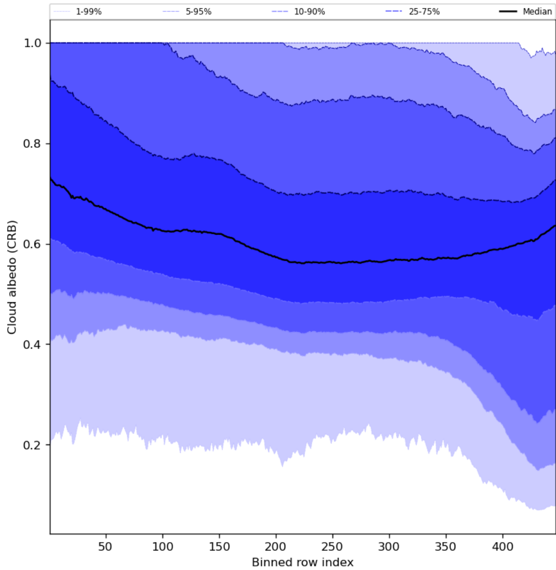
Figure 60: Along track statistics of “Cloud albedo (CRB)” for 2023-09-18 to 2023-09-20
