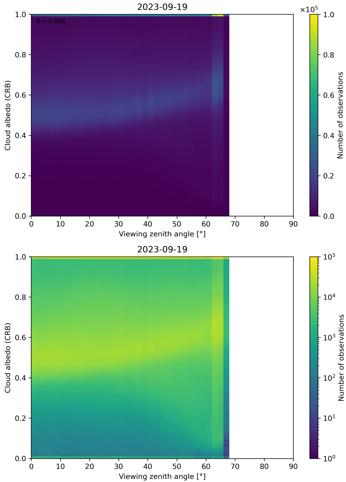
Figure 106: Scatter density plot of “Viewing zenith angle” against “Cloud albedo (CRB)” for 2023-09-18 to 2023-09-20.
