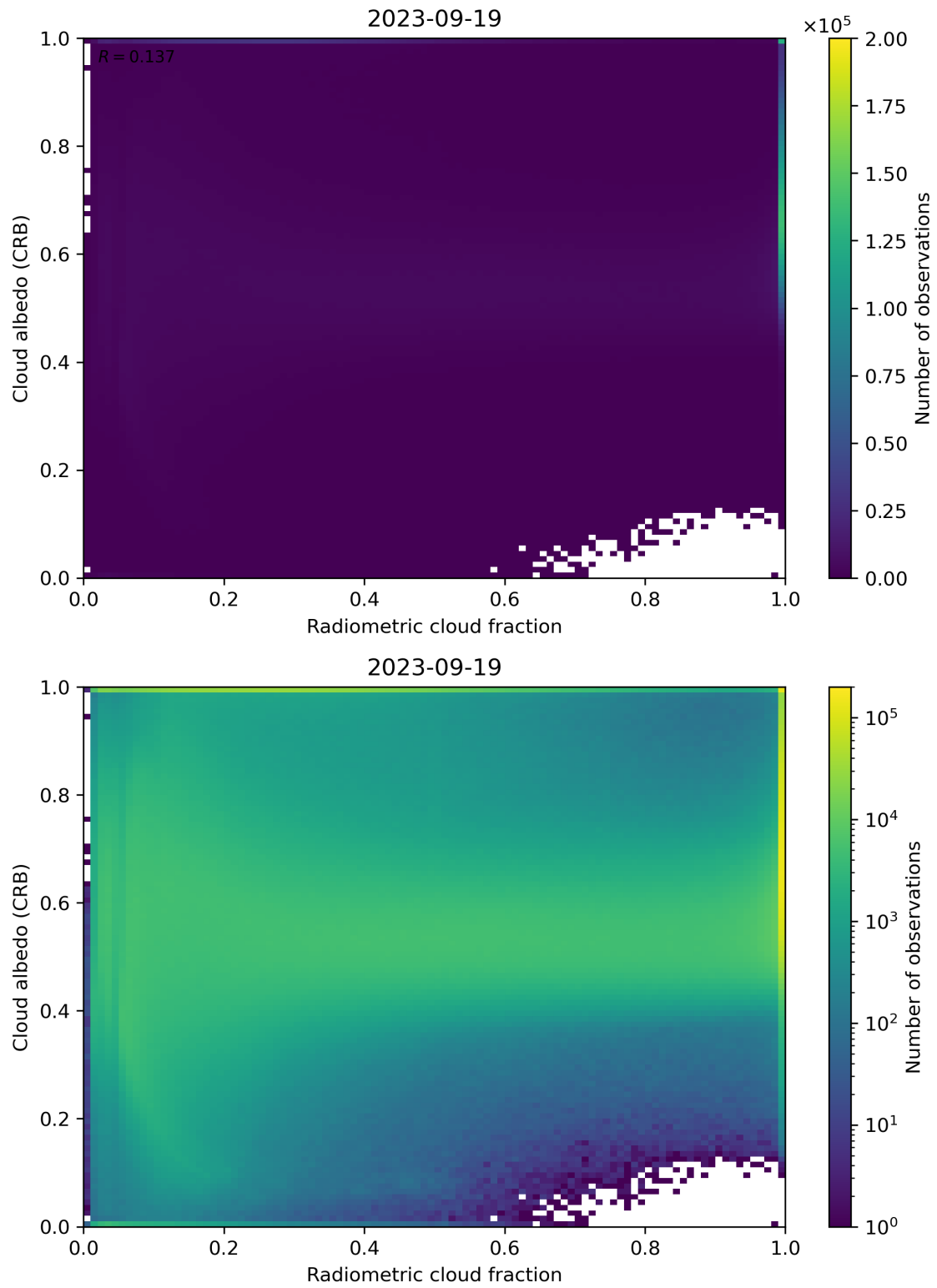
Figure 71: Scatter density plot of “Radiometric cloud fraction” against “Cloud albedo (CRB)” for 2023-09-18 to 2023-09-20.
