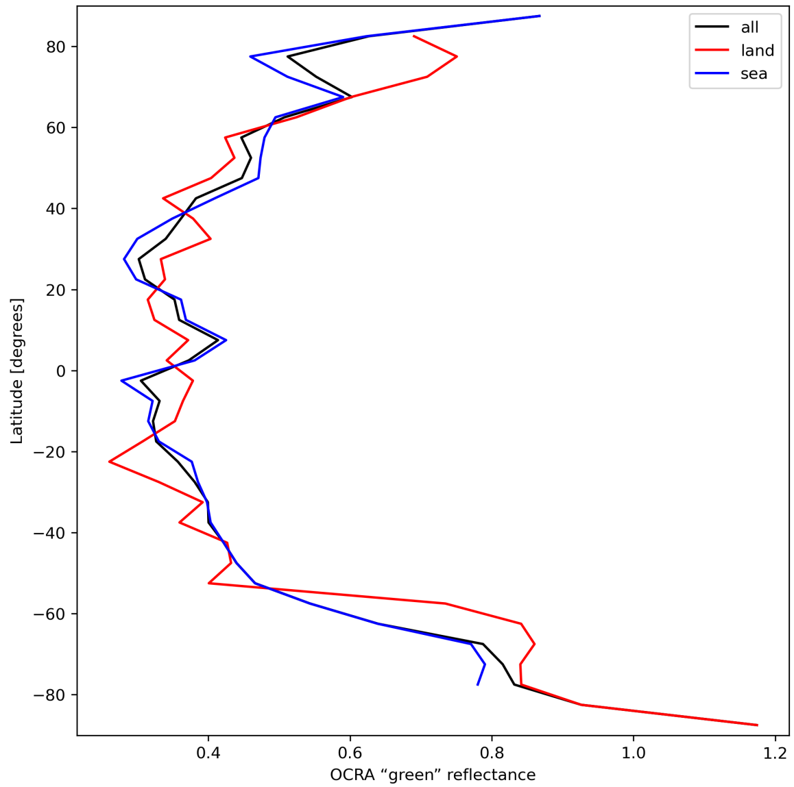
Figure 36: Zonal average of “OCRA “green” reflectance” for 2023-09-18 to 2023-09-20.
