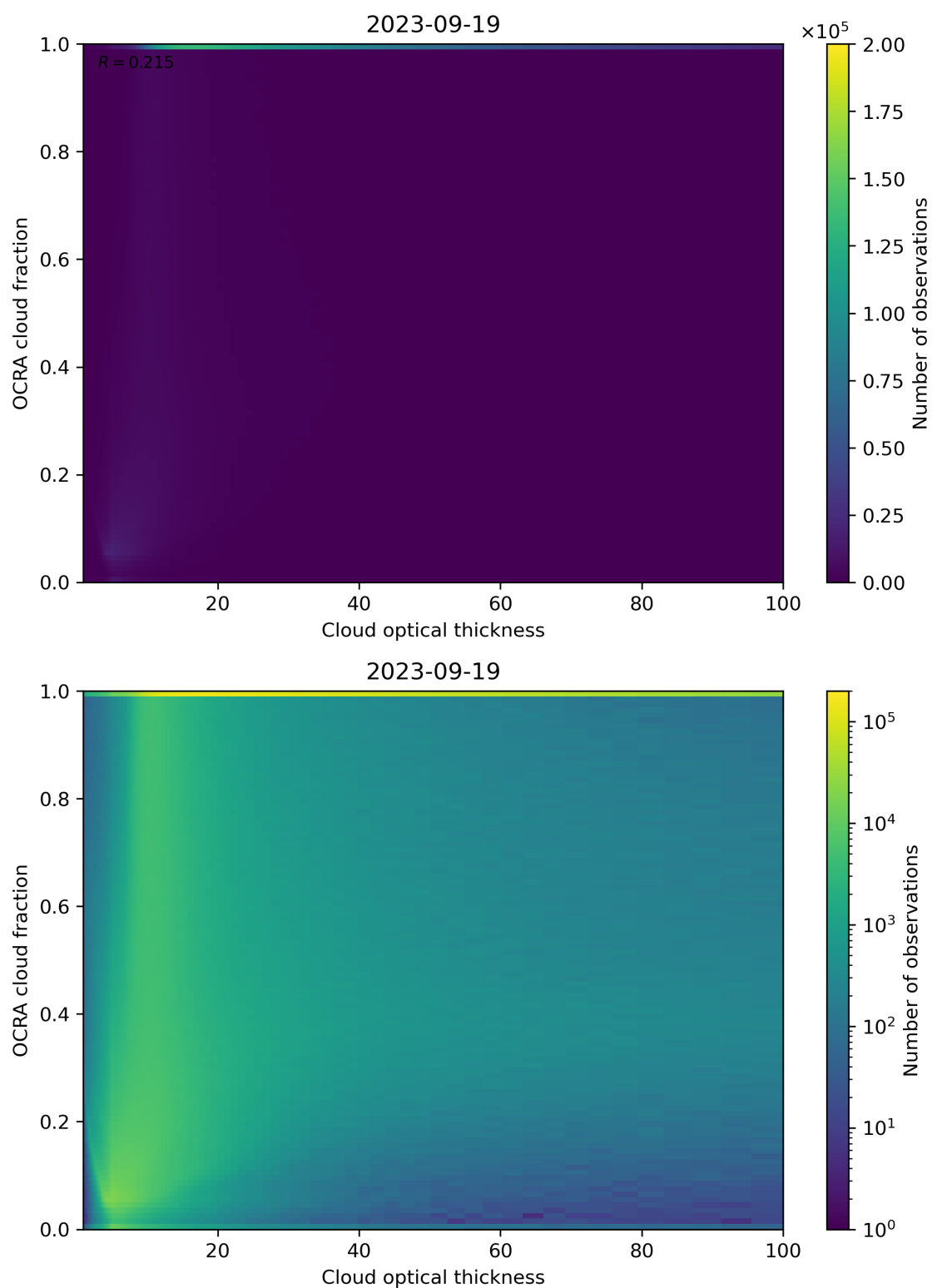
Figure 83: Scatter density plot of “Cloud optical thickness” against “OCRA cloud fraction” for 2023-09-18 to 2023-09-20.
