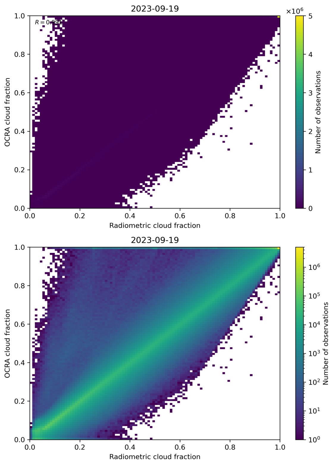
Figure 72: Scatter density plot of “Radiometric cloud fraction” against “OCRA cloud fraction” for 2023-09-18 to 2023-09-20.
