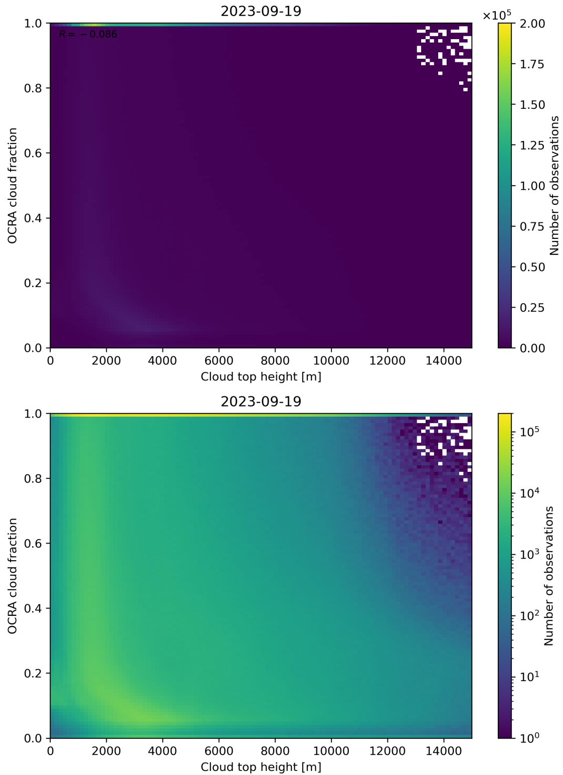
Figure 87: Scatter density plot of “Cloud top height” against “OCRA cloud fraction” for 2023-09-18 to 2023-09-20.
