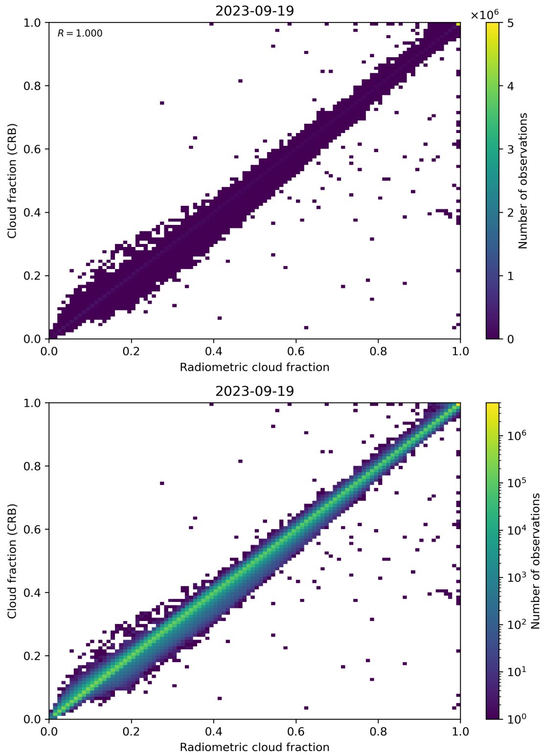
Figure 73: Scatter density plot of “Radiometric cloud fraction” against “Cloud fraction (CRB)” for 2023-09-18 to 2023-09-20.
