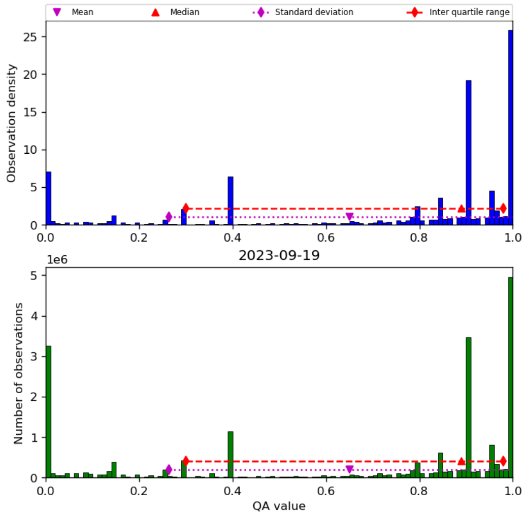
Figure 38: Histogram of “QA value” for 2023-09-18 to 2023-09-20
