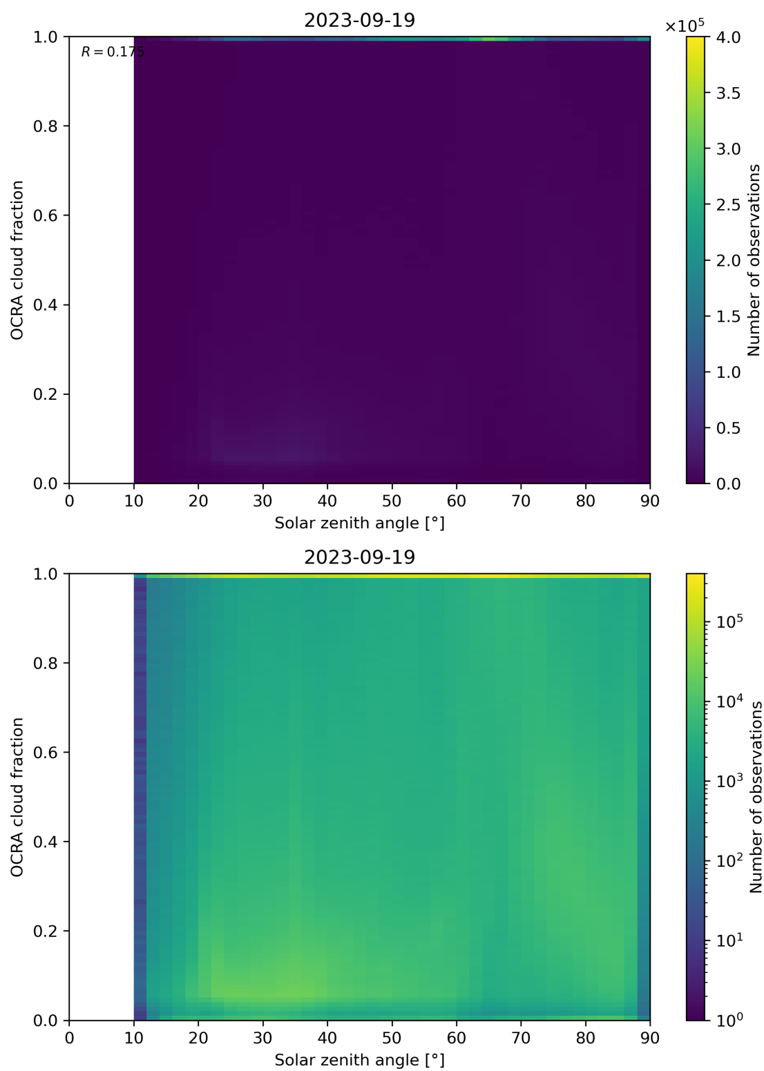
Figure 100: Scatter density plot of “Solar zenith angle” against “OCRA cloud fraction” for 2023-09-18 to 2023-09-20.
