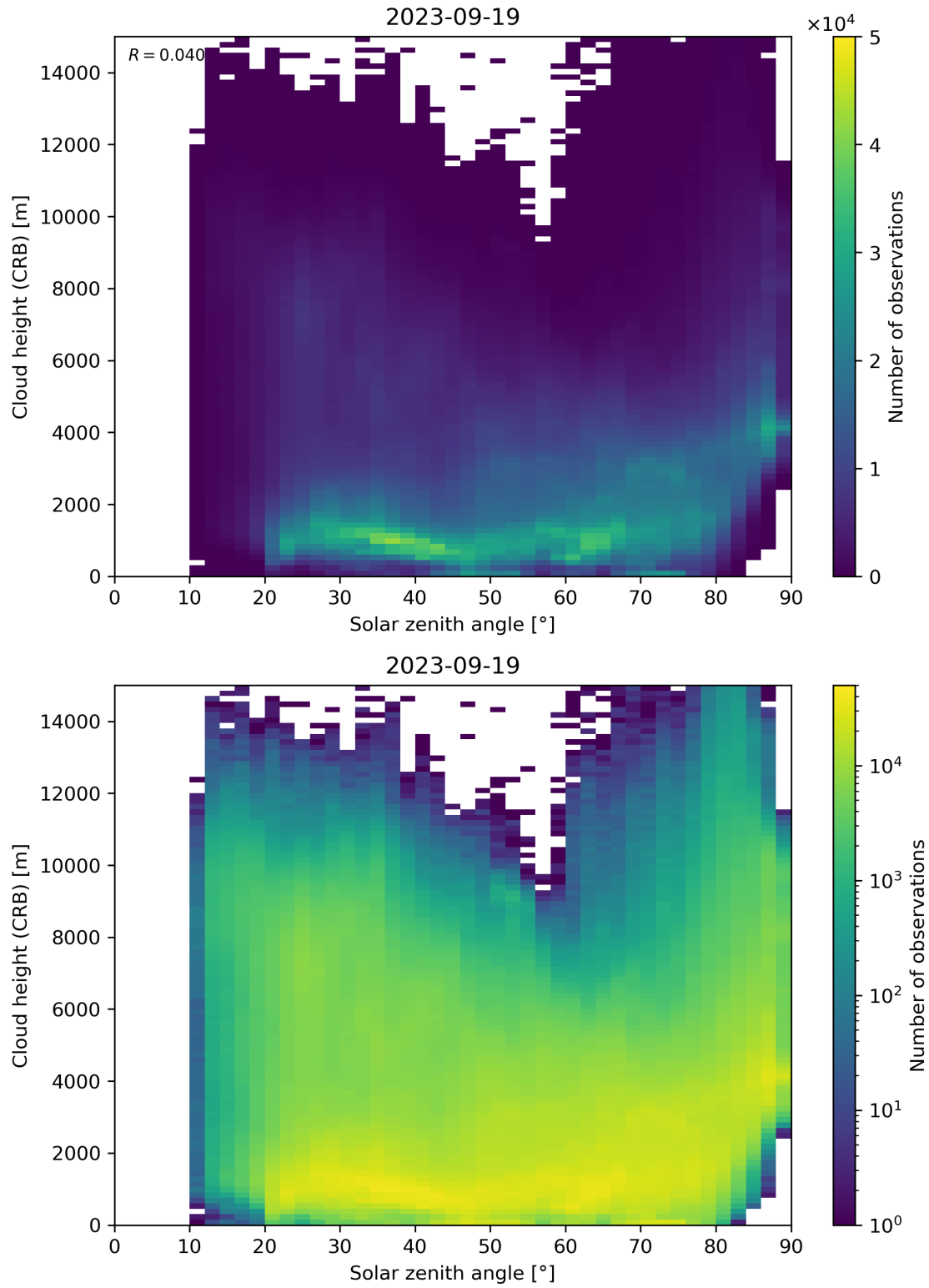
Figure 102: Scatter density plot of “Solar zenith angle” against “Cloud height (CRB)” for 2023-09-18 to 2023-09-20.
