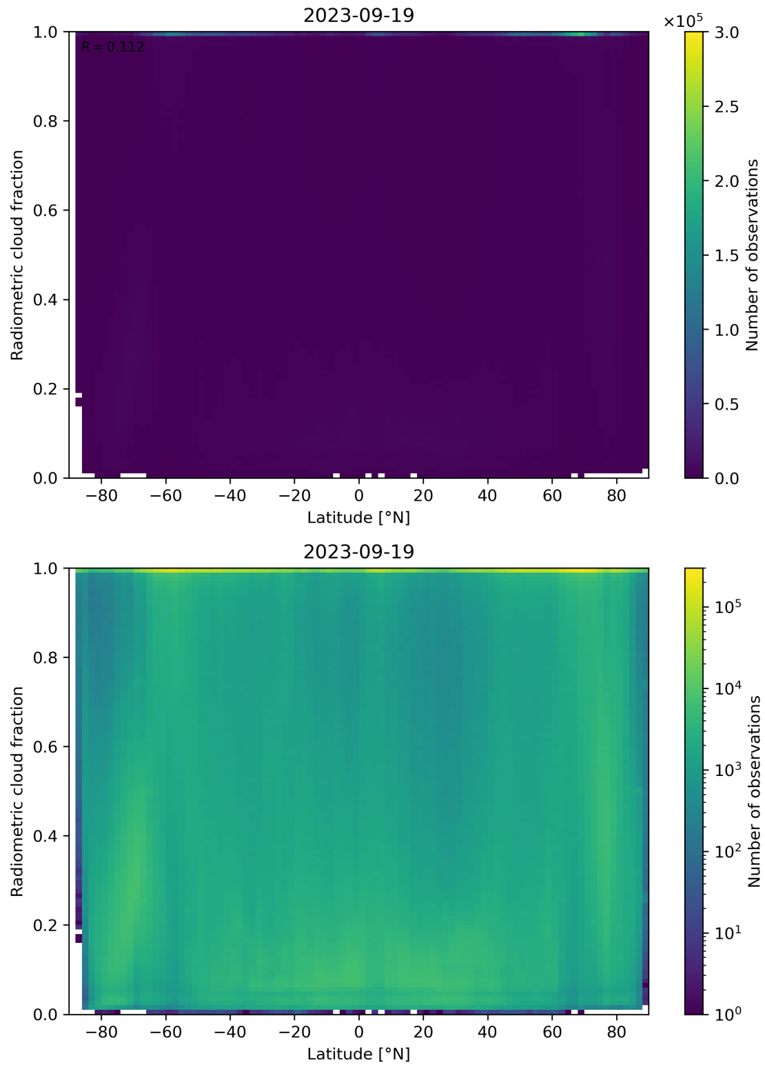
Figure 92: Scatter density plot of “Latitude” against “Radiometric cloud fraction” for 2023-09-18 to 2023-09-20.
