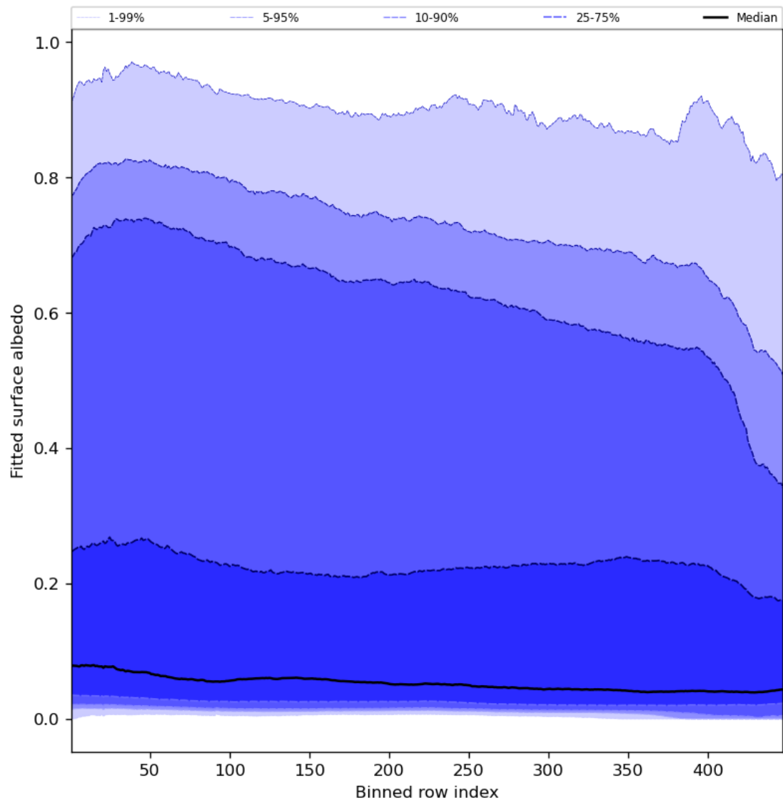
Figure 61: Along track statistics of “Fitted surface albedo” for 2023-09-18 to 2023-09-20
