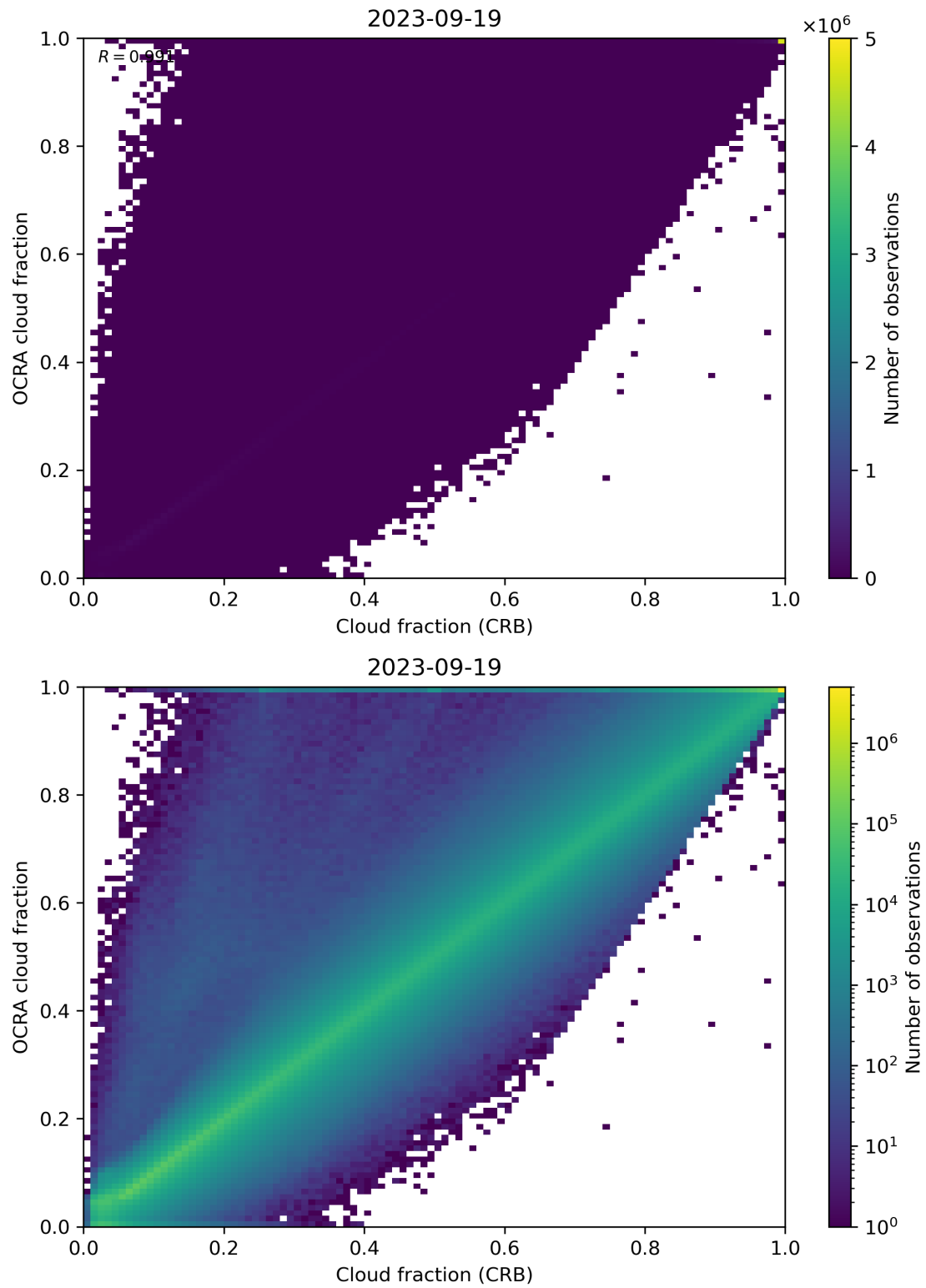
Figure 78: Scatter density plot of “Cloud fraction (CRB)” against “OCRA cloud fraction” for 2023-09-18 to 2023-09-20.
