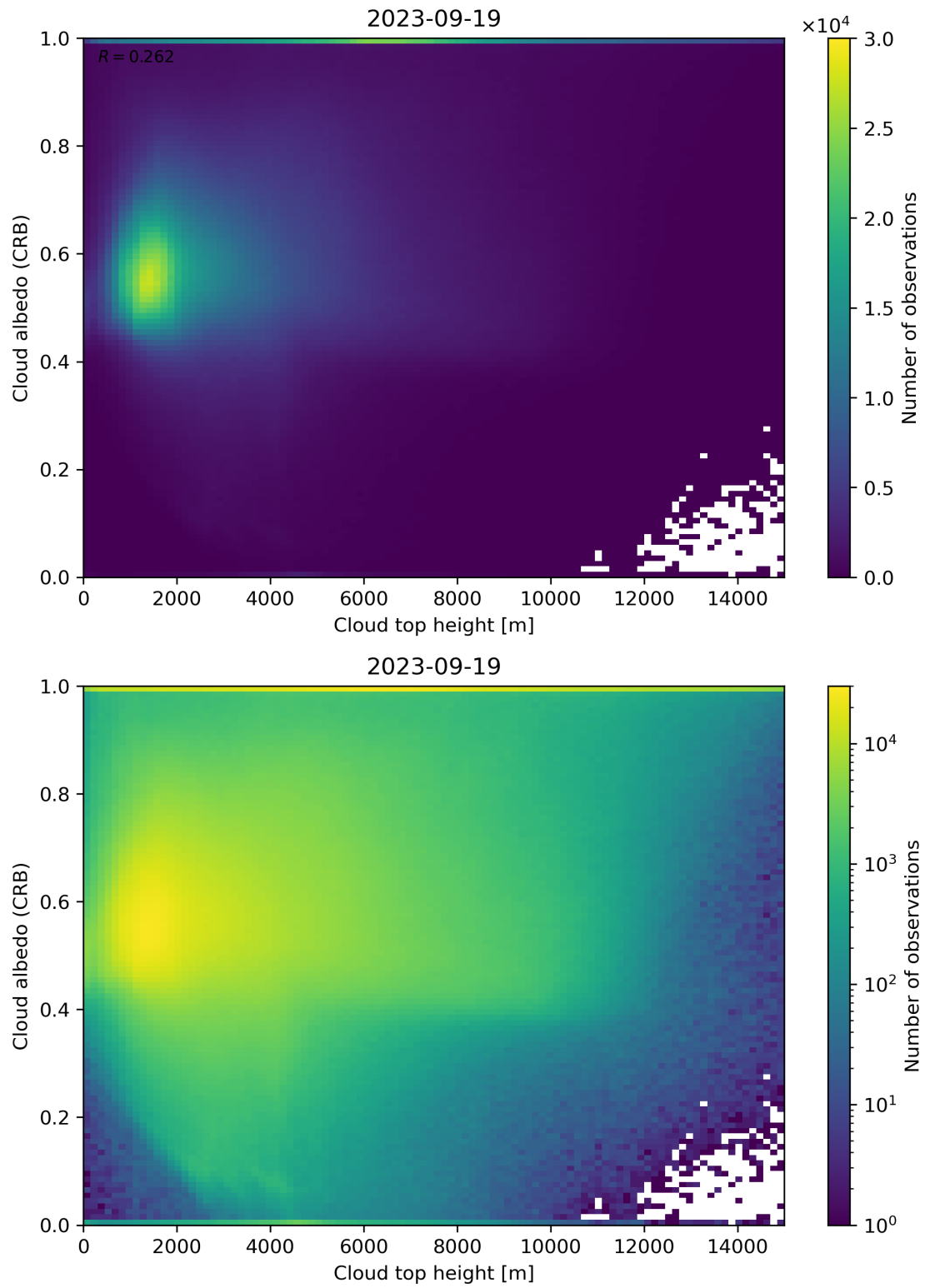
Figure 86: Scatter density plot of “Cloud top height” against “Cloud albedo (CRB)” for 2023-09-18 to 2023-09-20.
