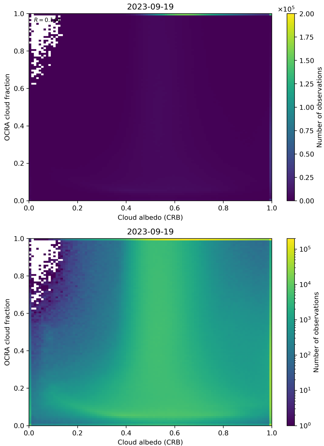
Figure 70: Scatter density plot of “Cloud albedo (CRB)” against “OCRA cloud fraction” for 2023-09-18 to 2023-09-20.
