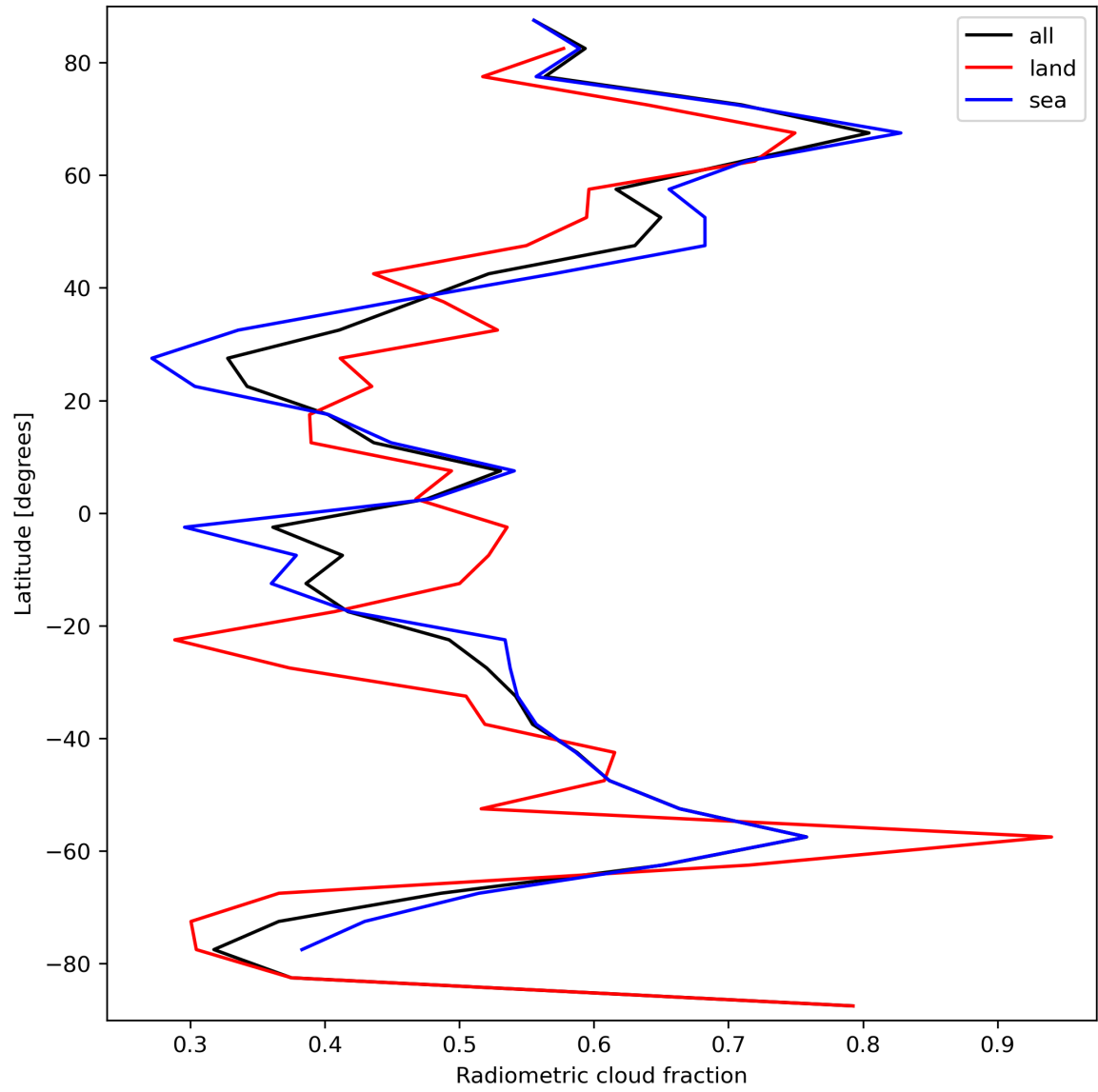
Figure 23: Zonal average of “Radiometric cloud fraction” for 2023-09-18 to 2023-09-20.
