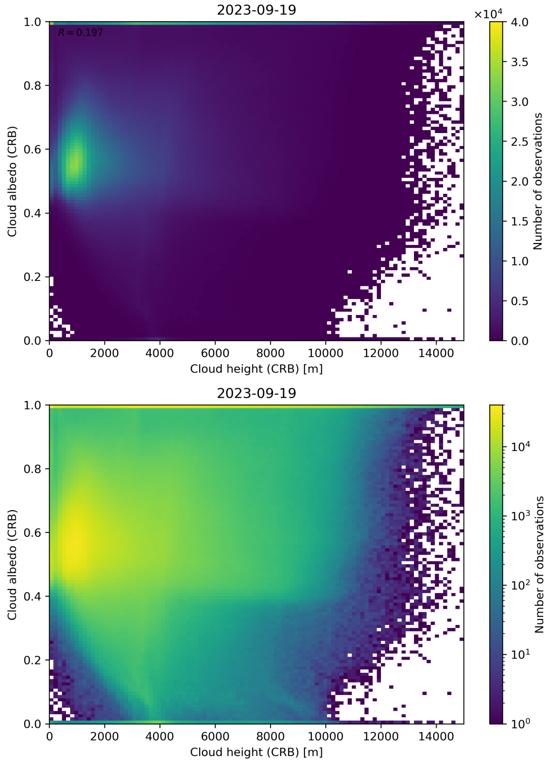
Figure 80: Scatter density plot of “Cloud height (CRB)” against “Cloud albedo (CRB)” for 2023-09-18 to 2023-09-20.
