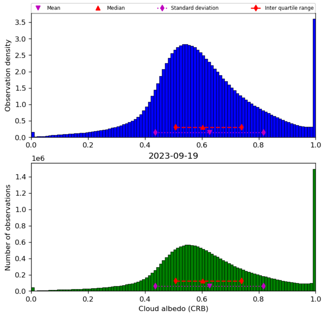
Figure 44: Histogram of “Cloud albedo (CRB)” for 2023-09-18 to 2023-09-20
