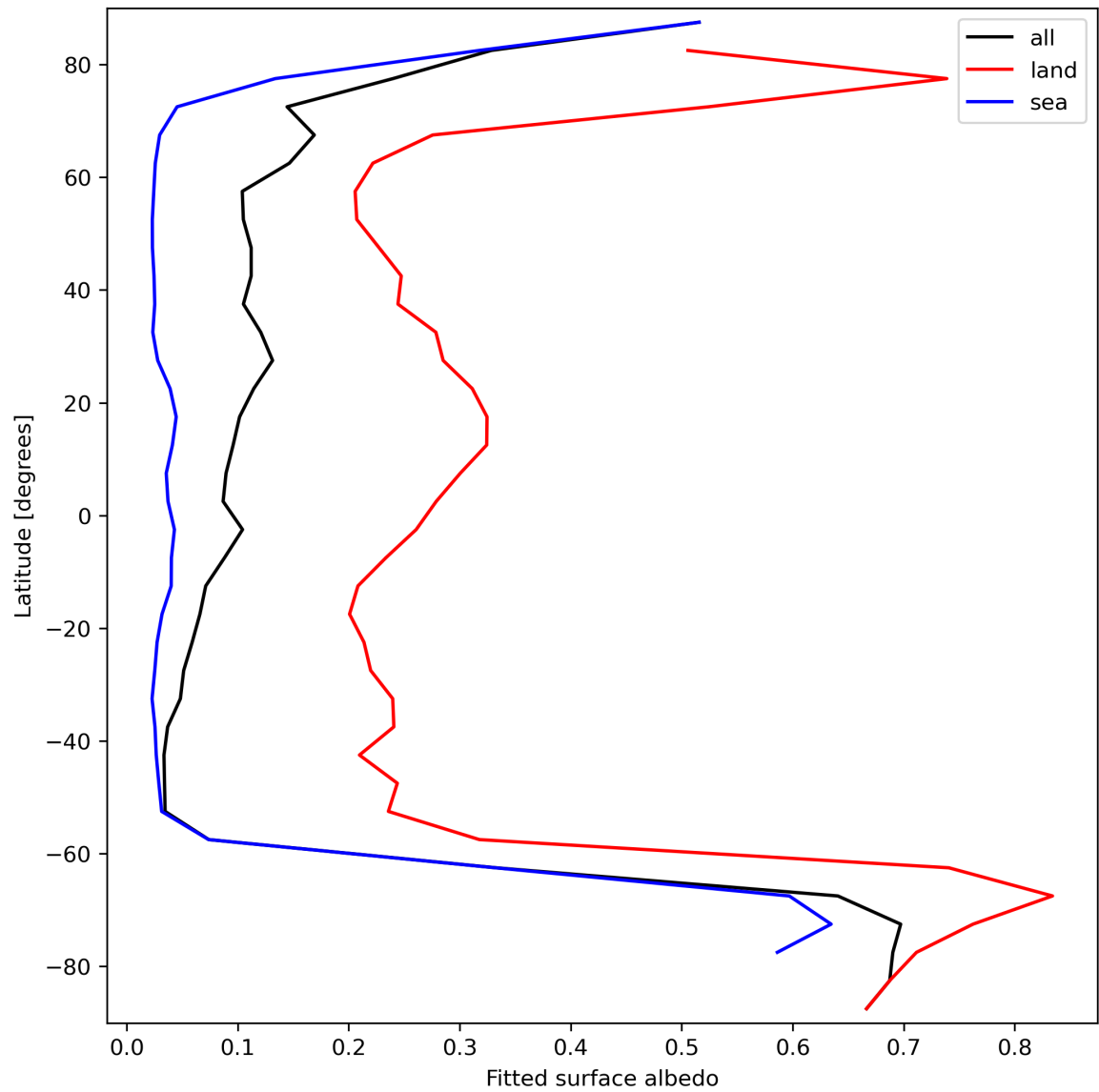
Figure 29: Zonal average of “Fitted surface albedo” for 2023-09-18 to 2023-09-20.
