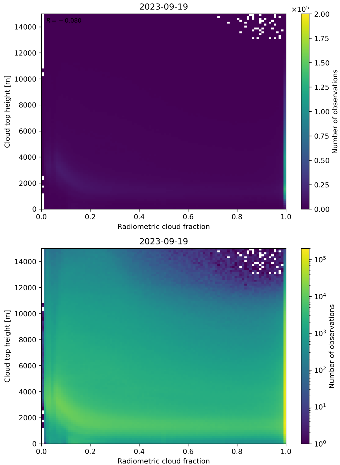
Figure 76: Scatter density plot of “Radiometric cloud fraction” against “Cloud top height” for 2023-09-18 to 2023-09-20.
