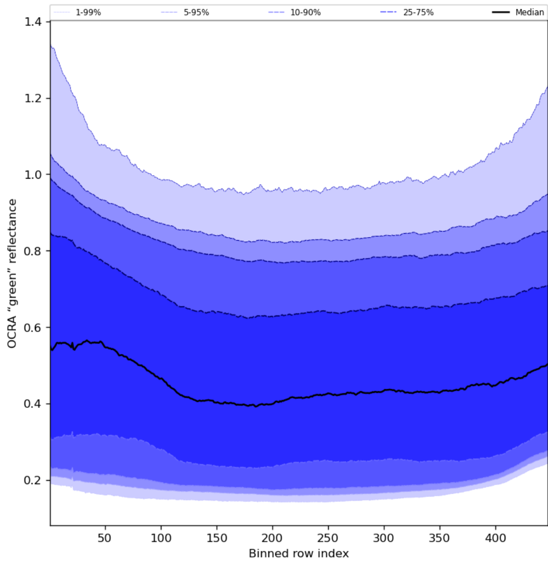
Figure 68: Along track statistics of “OCRA “green” reflectance” for 2023-09-18 to 2023-09-20
