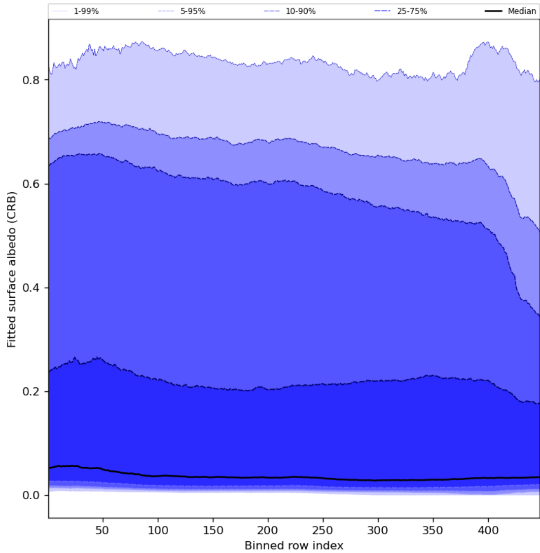
Figure 62: Along track statistics of “Fitted surface albedo (CRB)” for 2023-09-18 to 2023-09-20
