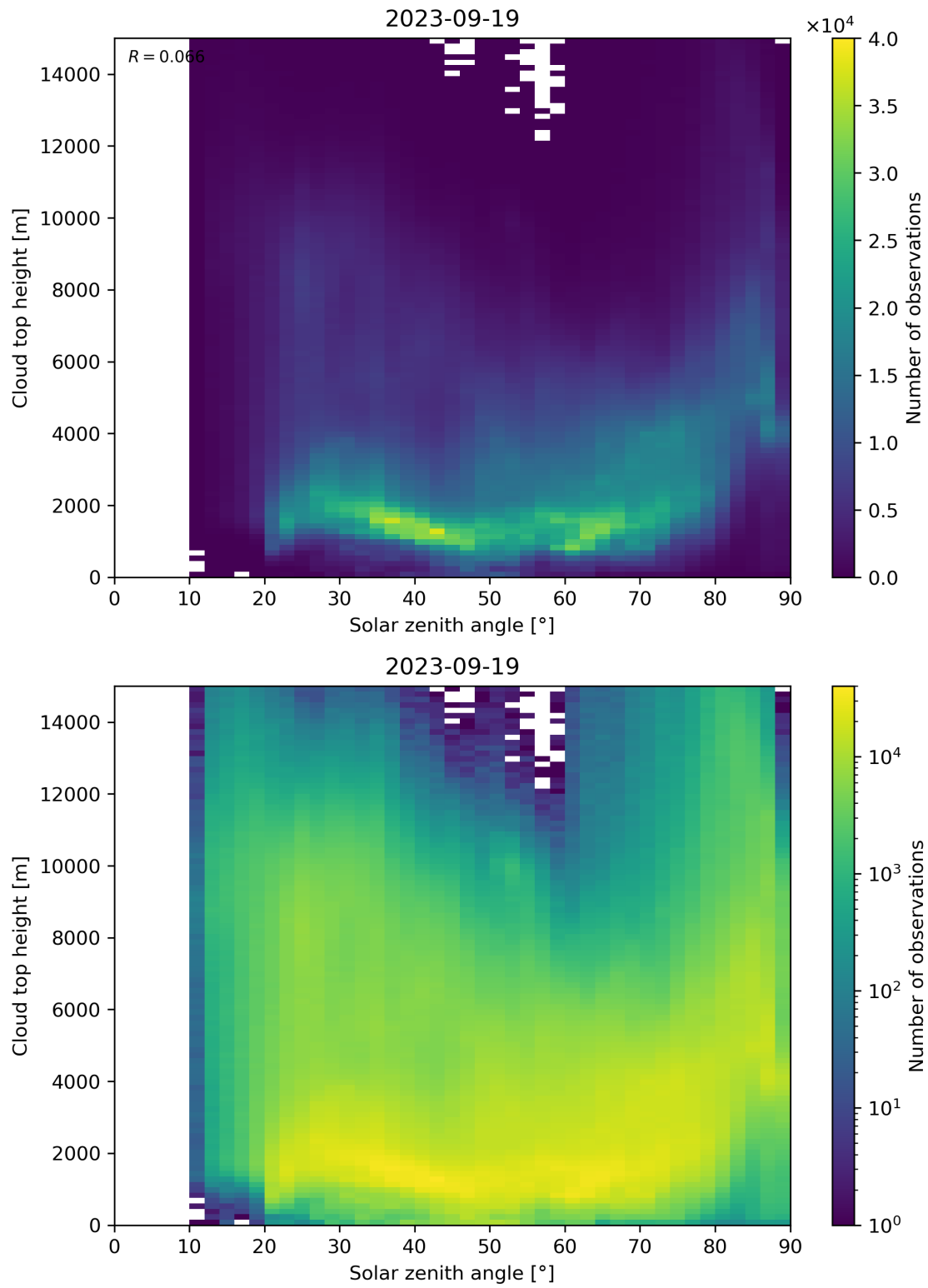
Figure 104: Scatter density plot of “Solar zenith angle” against “Cloud top height” for 2023-09-18 to 2023-09-20.
