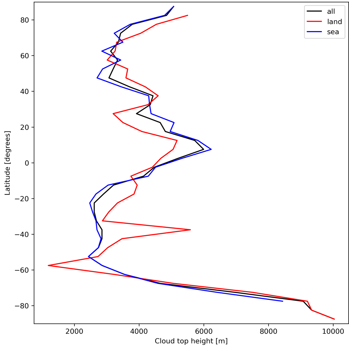
Figure 24: Zonal average of “Cloud top height” for 2023-09-18 to 2023-09-20.
