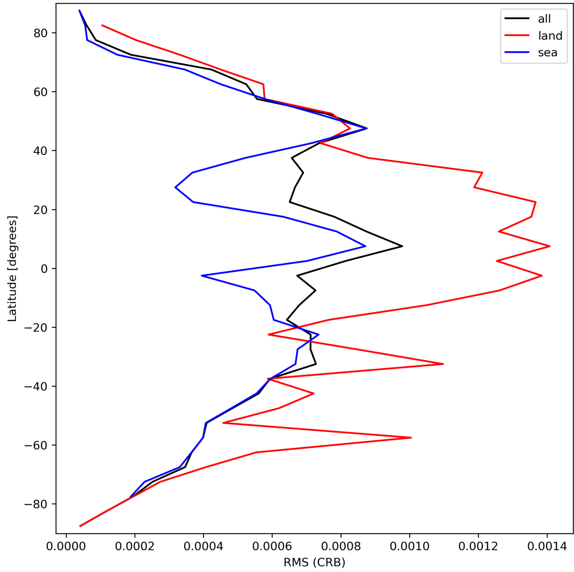
Figure 32: Zonal average of “RMS (CRB)” for 2023-09-18 to 2023-09-20.
