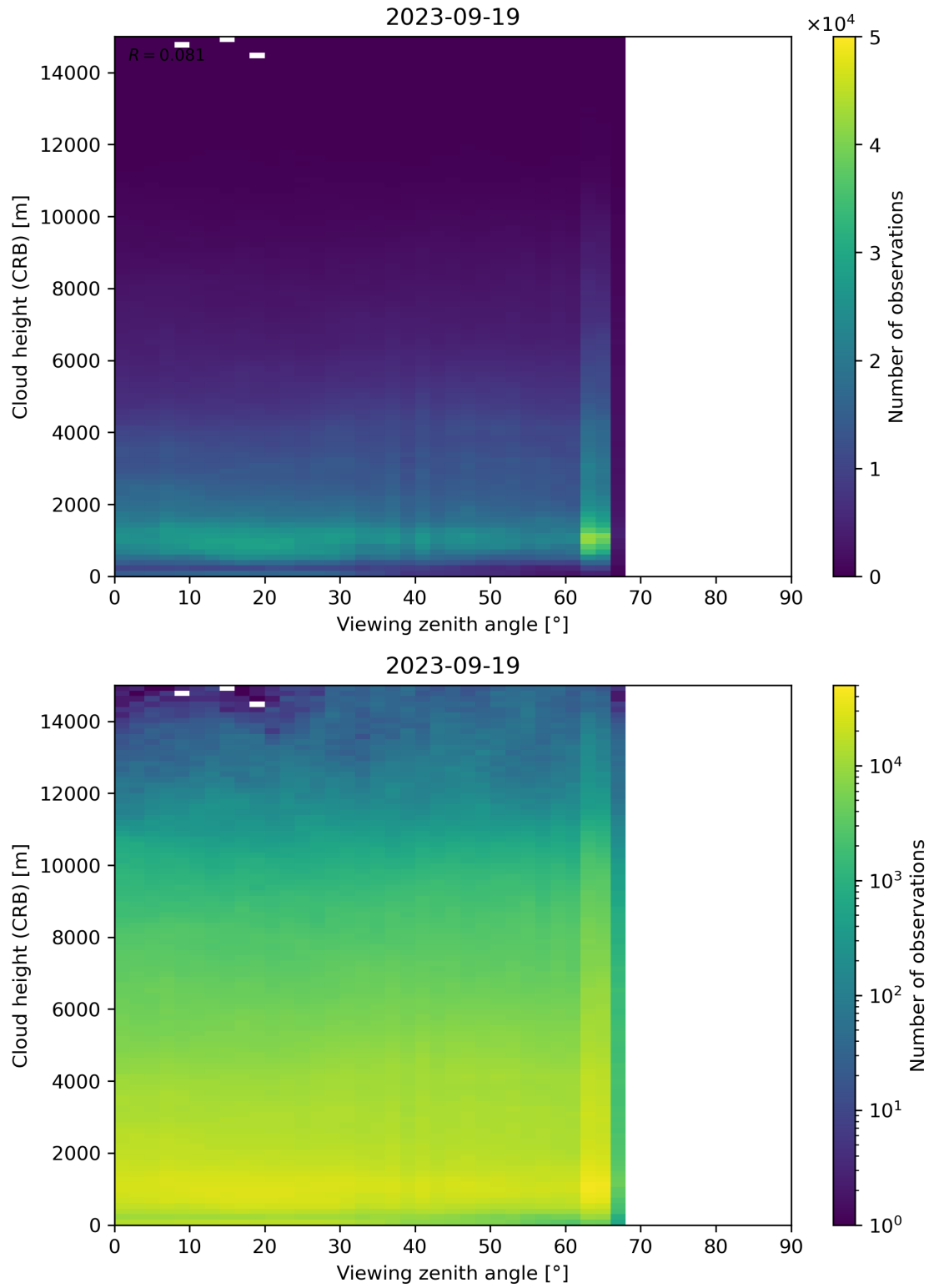
Figure 110: Scatter density plot of “Viewing zenith angle” against “Cloud height (CRB)” for 2023-09-18 to 2023-09-20.
