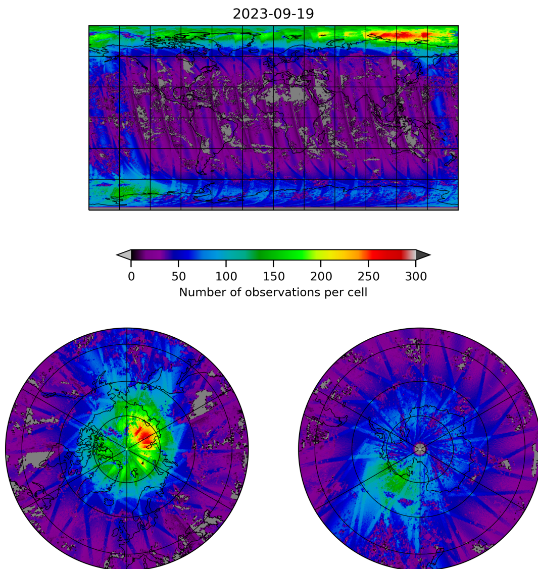
Figure 21: Map of the number of observations for 2023-09-18 to 2023-09-20
