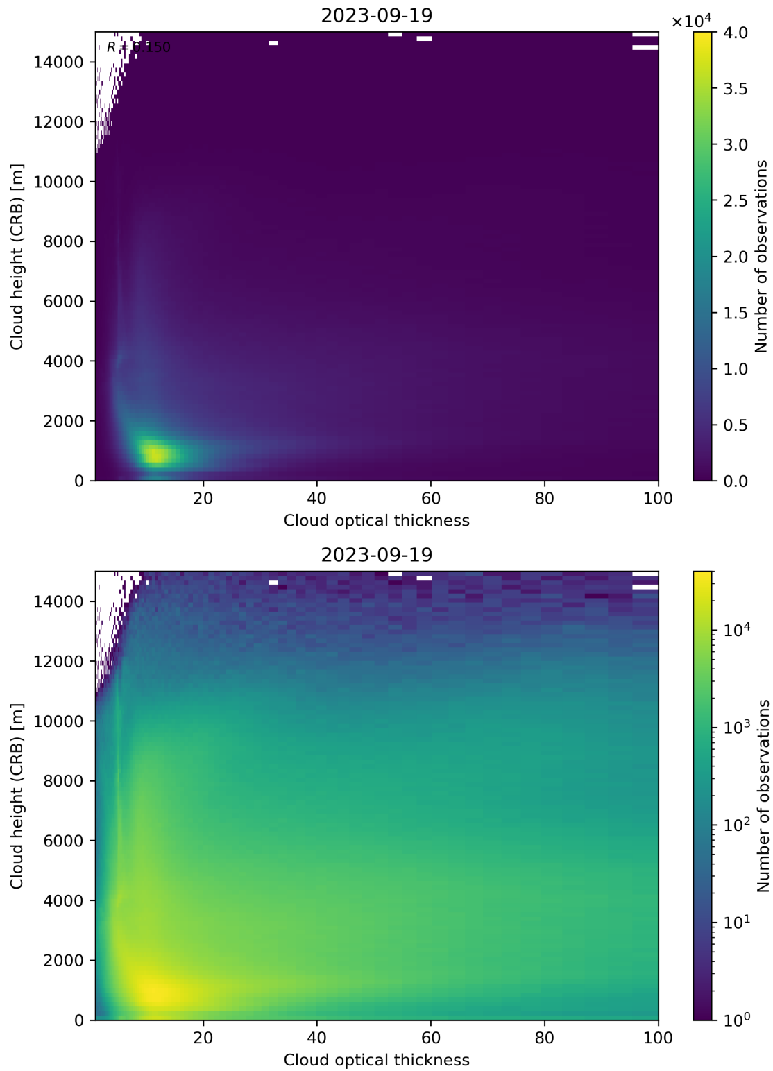
Figure 85: Scatter density plot of “Cloud optical thickness” against “Cloud height (CRB)” for 2023-09-18 to 2023-09-20.
