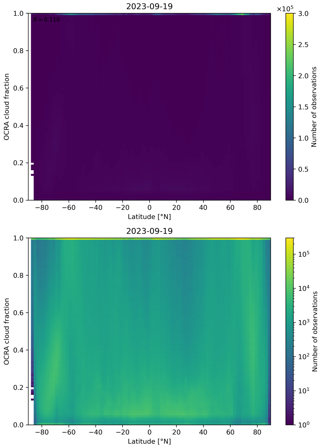
Figure 93: Scatter density plot of “Latitude” against “OCRA cloud fraction” for 2023-09-18 to 2023-09-20.
