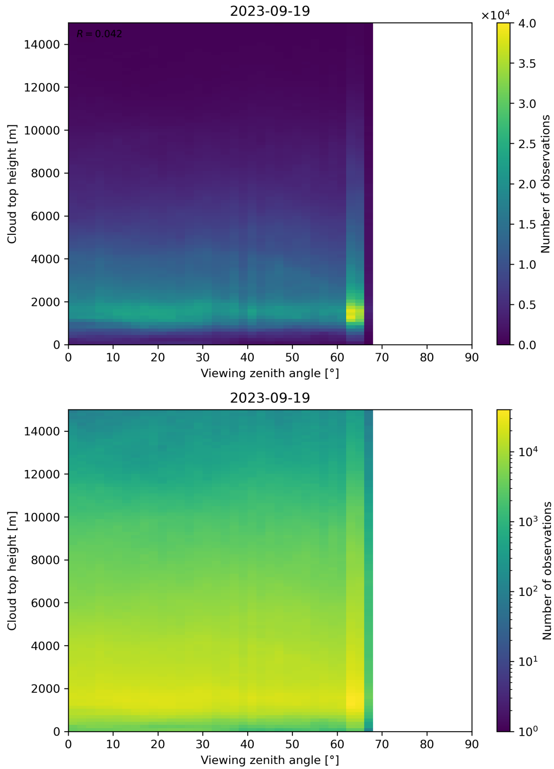
Figure 112: Scatter density plot of “Viewing zenith angle” against “Cloud top height” for 2023-09-18 to 2023-09-20.
