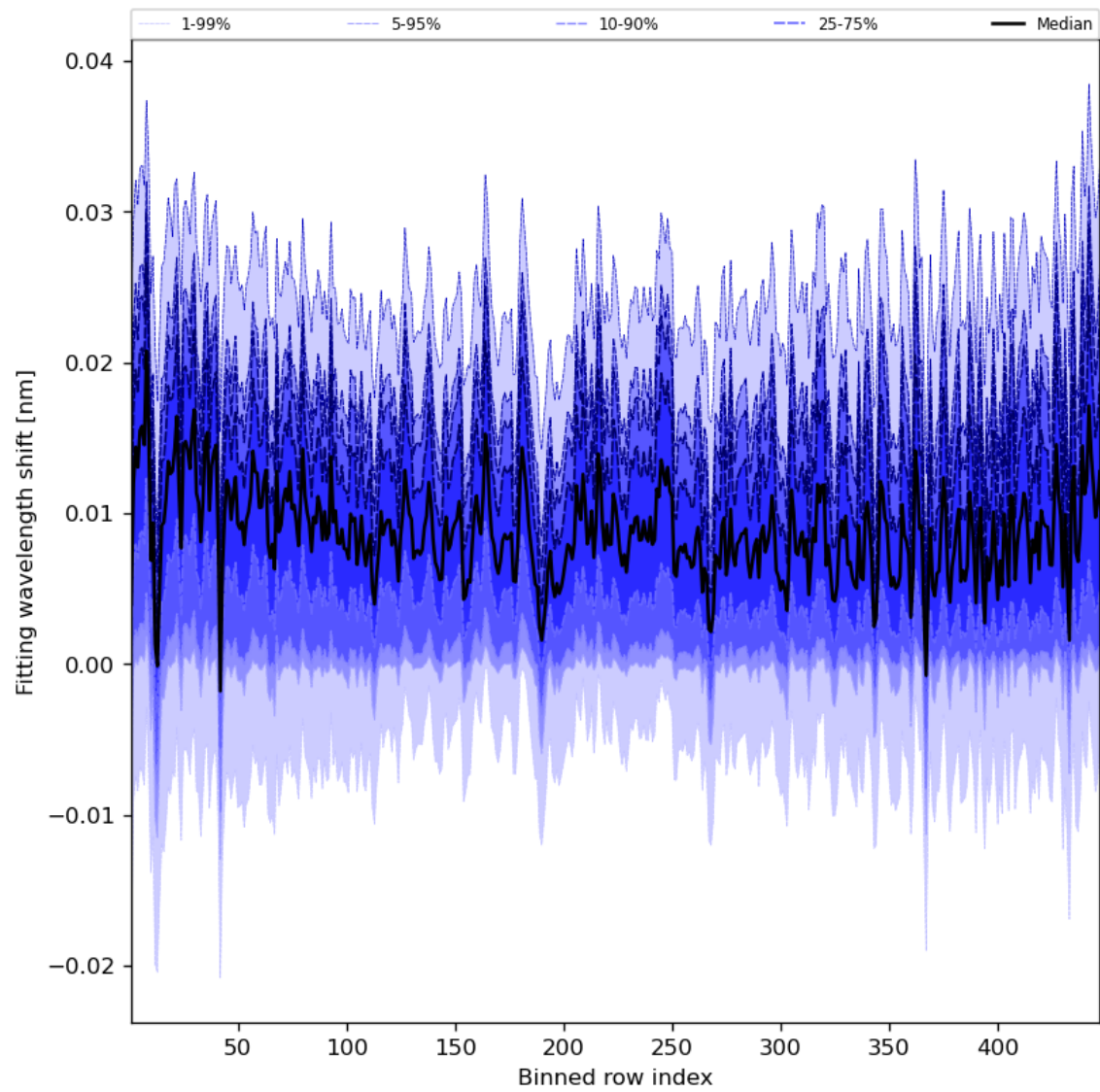
Figure 65: Along track statistics of “Fitting wavelength shift” for 2023-09-18 to 2023-09-20
