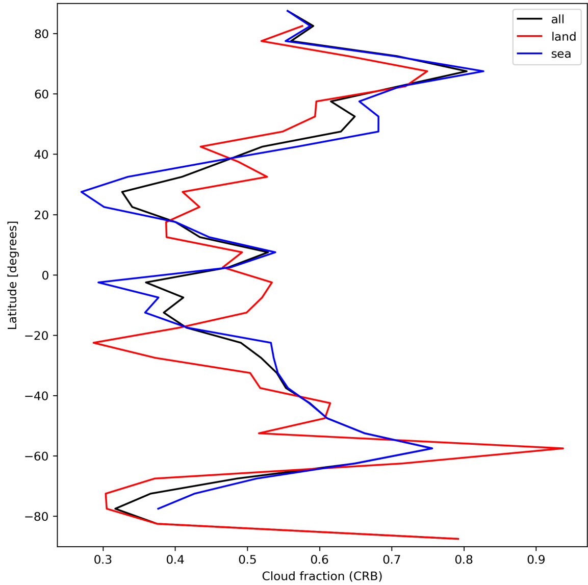
Figure 26: Zonal average of “Cloud fraction (CRB)” for 2023-09-18 to 2023-09-20.
