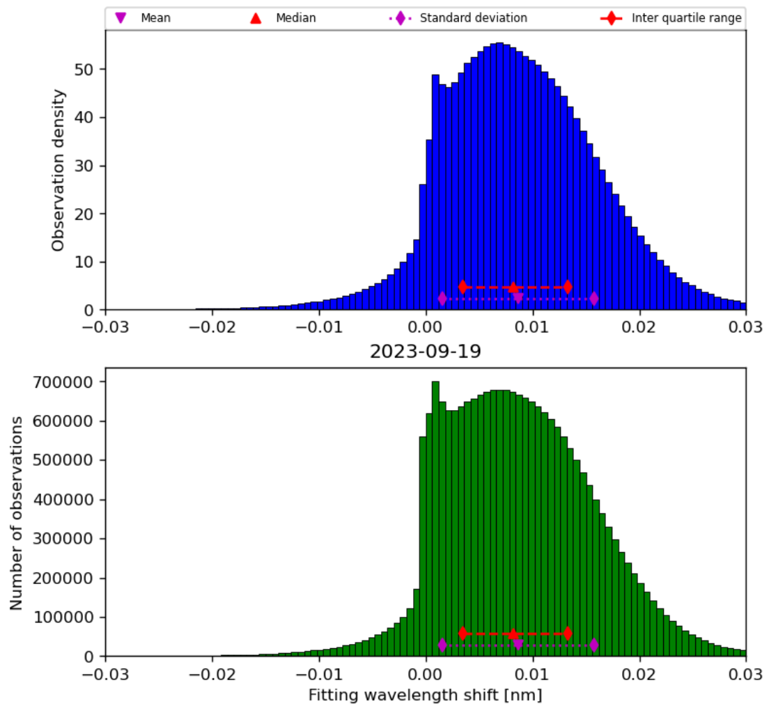
Figure 49: Histogram of “Fitting wavelength shift” for 2023-09-18 to 2023-09-20
