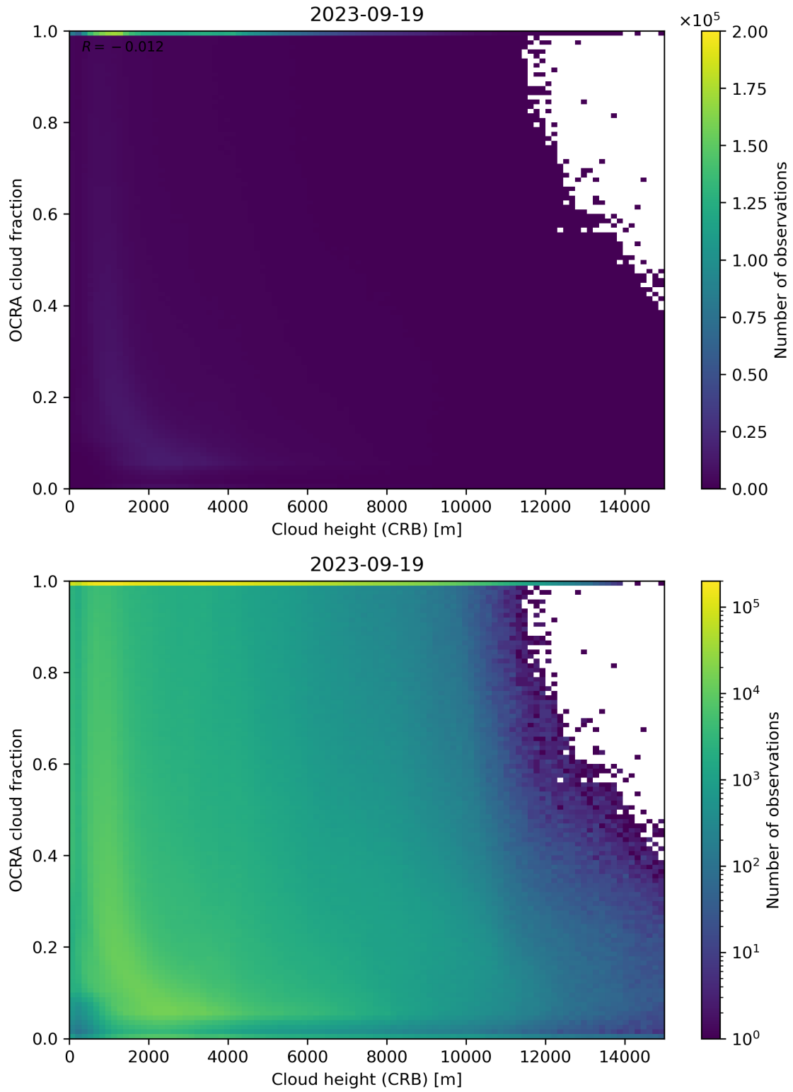
Figure 81: Scatter density plot of “Cloud height (CRB)” against “OCRA cloud fraction” for 2023-09-18 to 2023-09-20.
