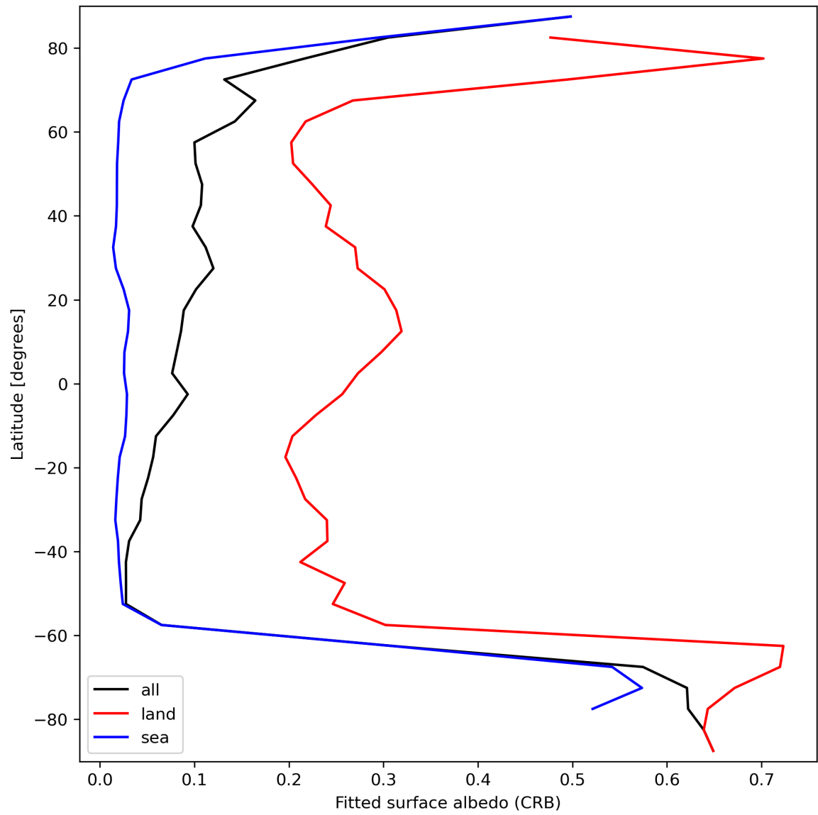
Figure 30: Zonal average of “Fitted surface albedo (CRB)” for 2023-09-18 to 2023-09-20.
