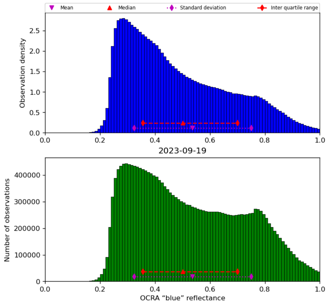
Figure 51: Histogram of “OCRA “blue” reflectance” for 2023-09-18 to 2023-09-20
