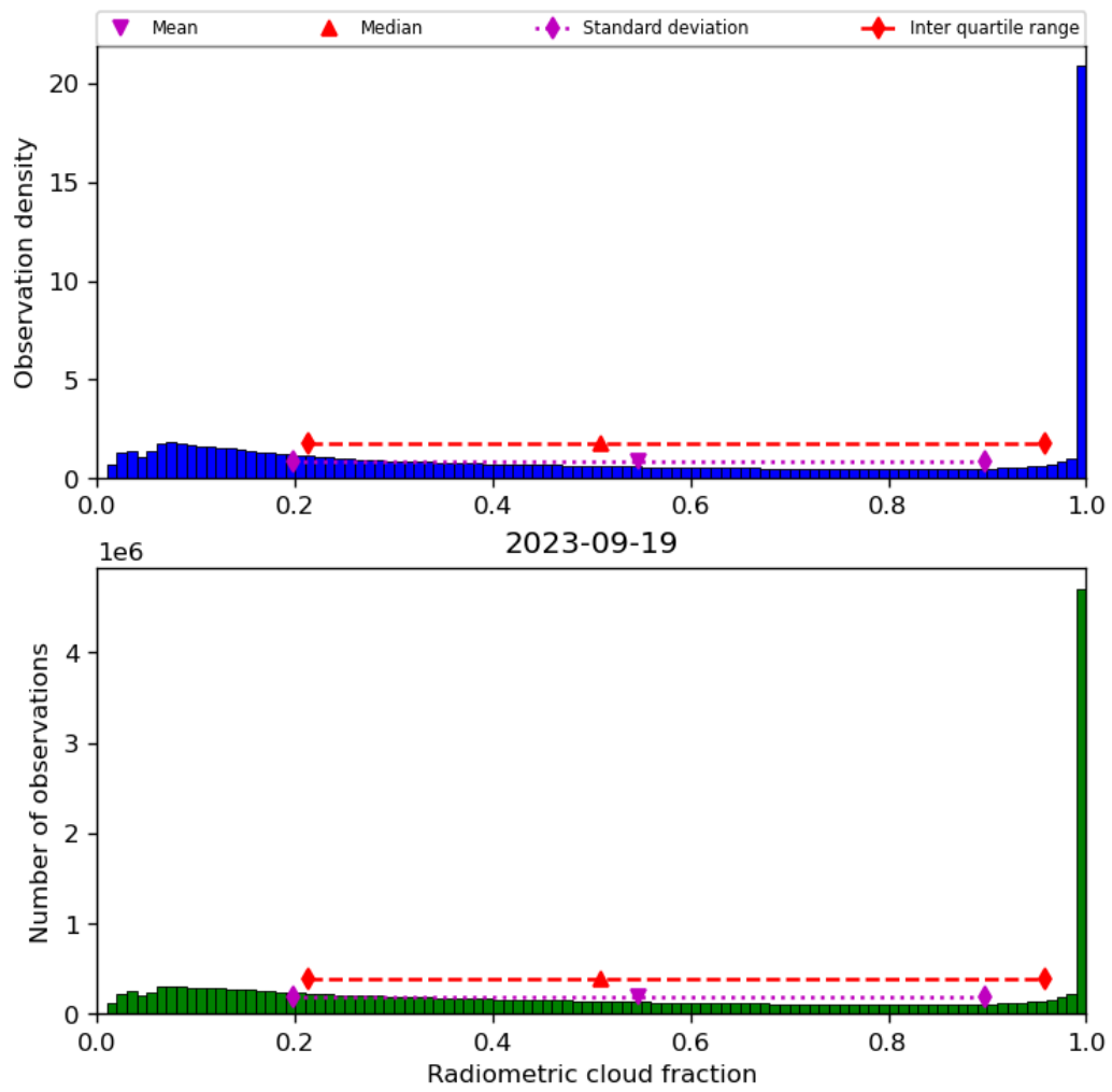
Figure 39: Histogram of “Radiometric cloud fraction” for 2023-09-18 to 2023-09-20
