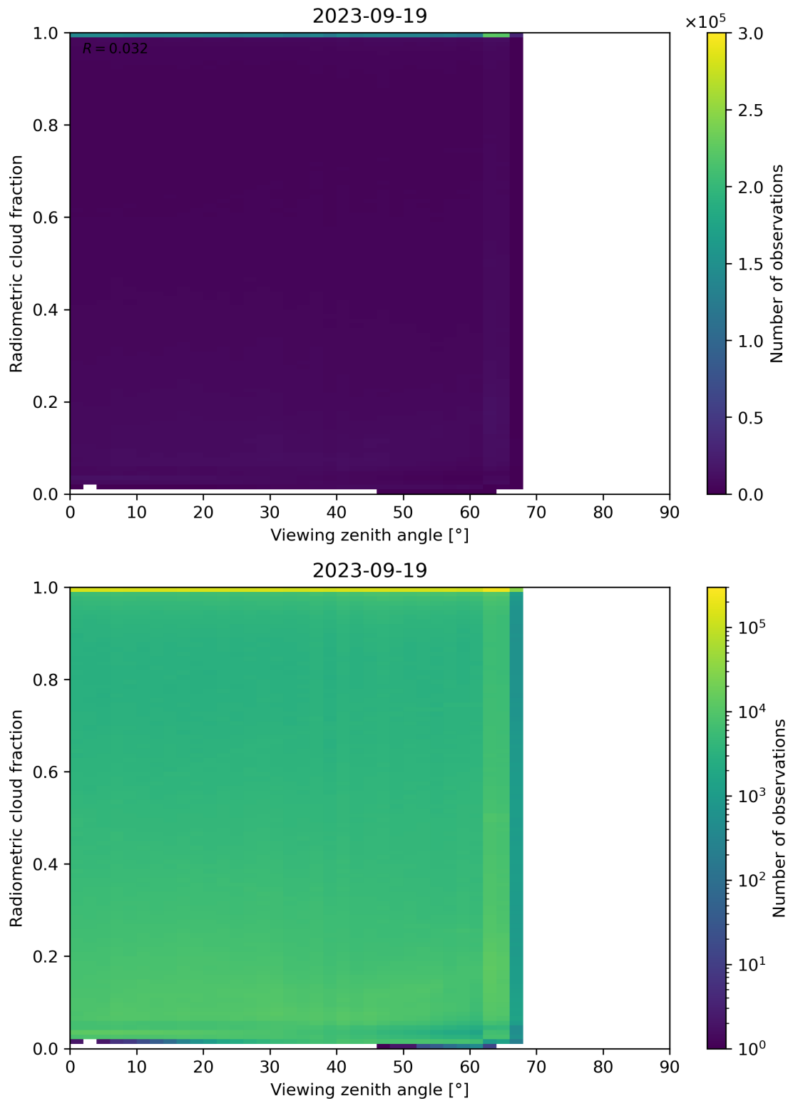
Figure 107: Scatter density plot of “Viewing zenith angle” against “Radiometric cloud fraction” for 2023-09-18 to 2023-09-20.
