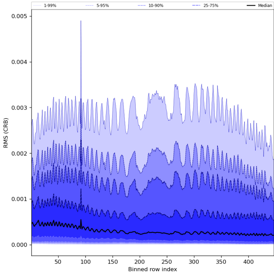
Figure 64: Along track statistics of “RMS (CRB)” for 2023-09-18 to 2023-09-20
