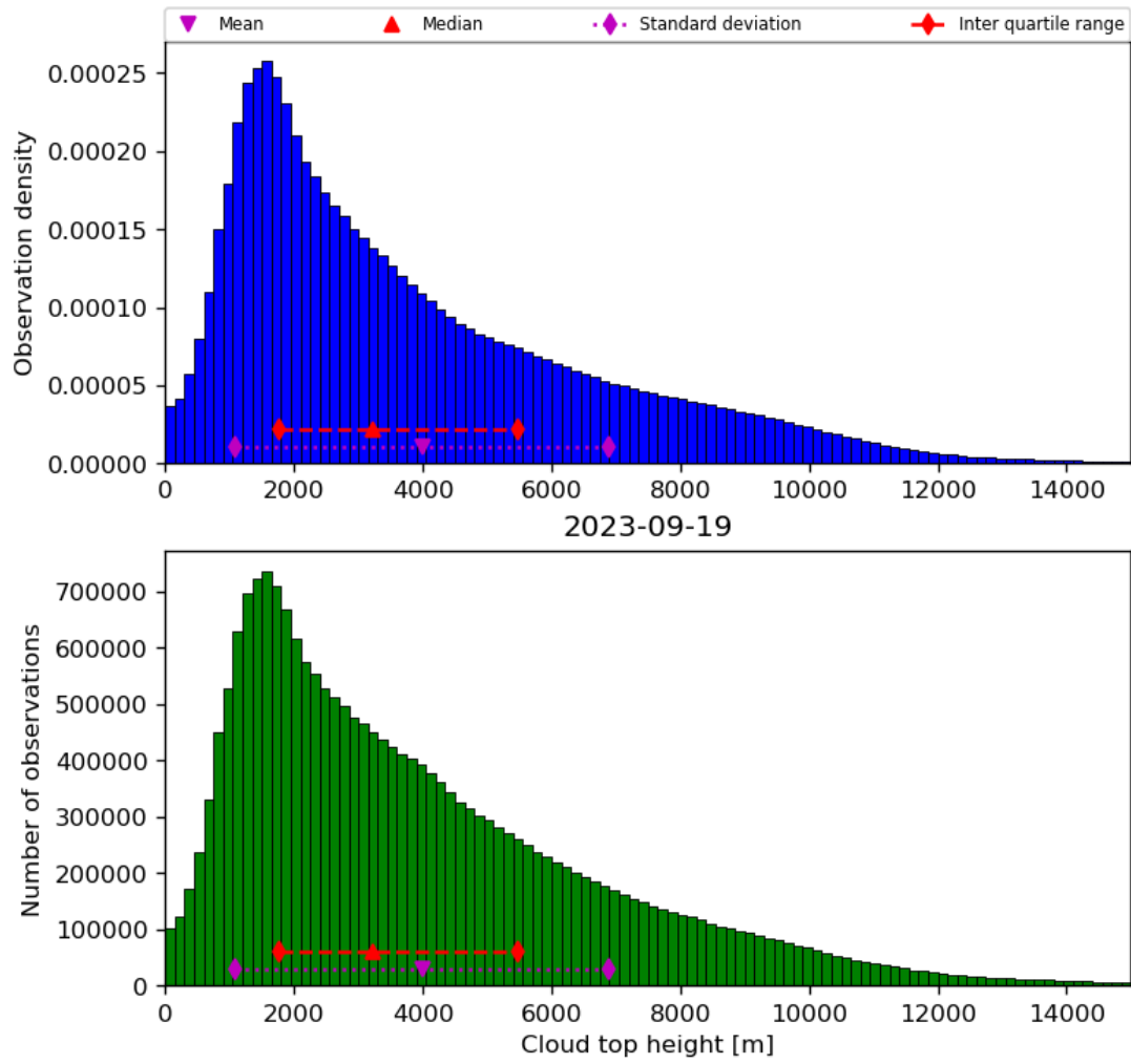
Figure 40: Histogram of “Cloud top height” for 2023-09-18 to 2023-09-20
