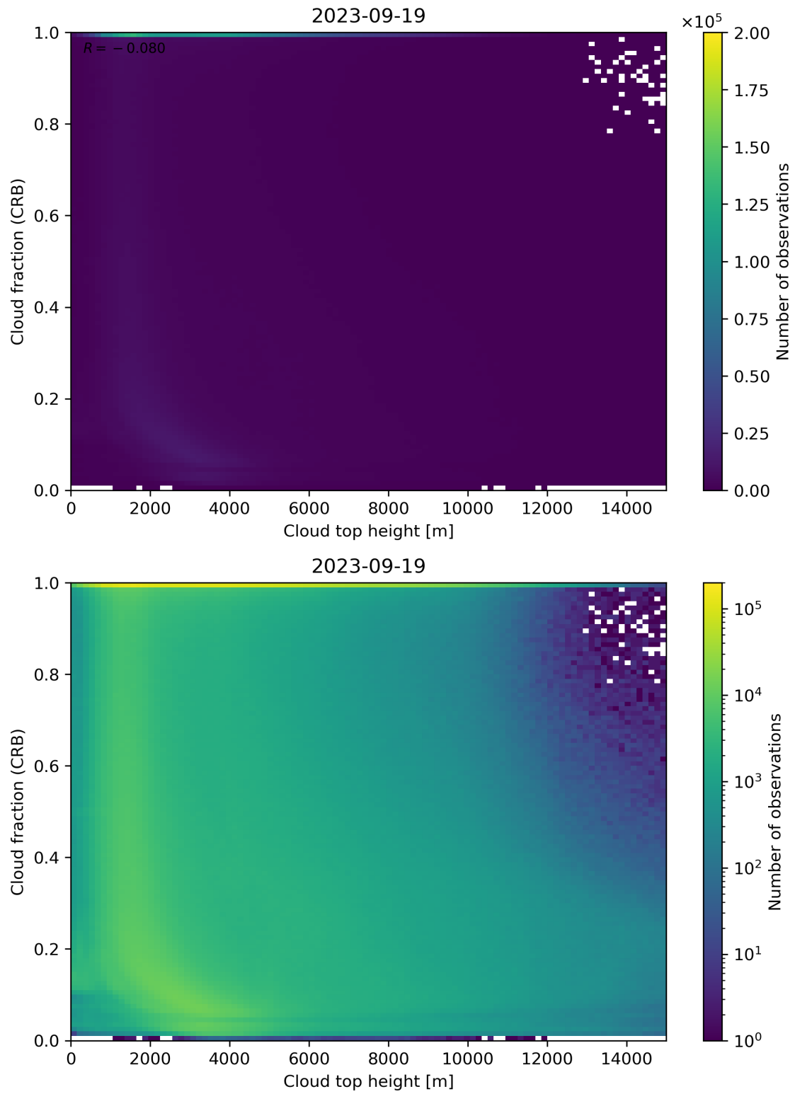
Figure 88: Scatter density plot of “Cloud top height” against “Cloud fraction (CRB)” for 2023-09-18 to 2023-09-20.
