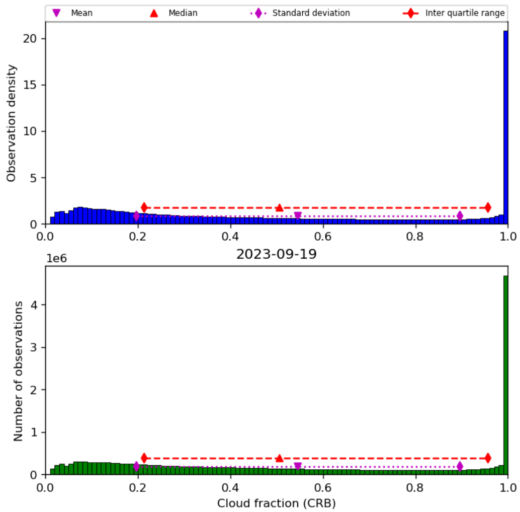
Figure 42: Histogram of “Cloud fraction (CRB)” for 2023-09-18 to 2023-09-20
