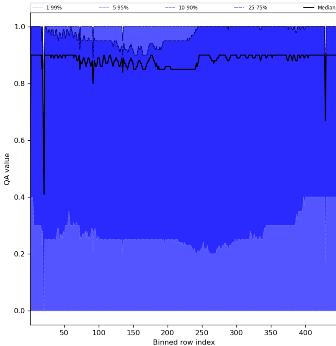
Figure 54: Along track statistics of “QA value” for 2023-09-18 to 2023-09-20
