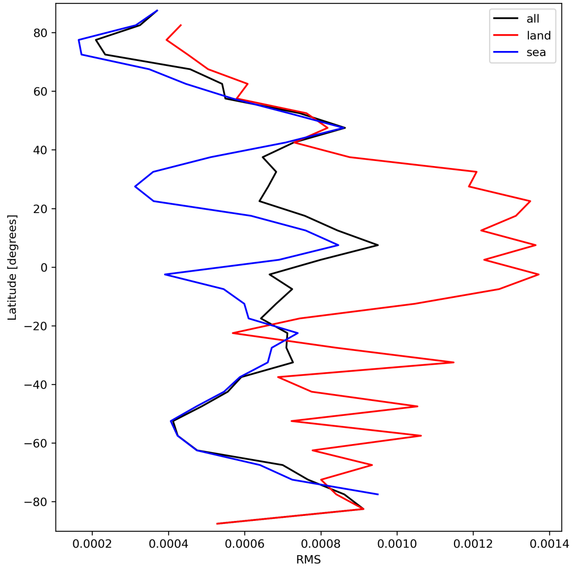
Figure 31: Zonal average of “RMS” for 2023-09-18 to 2023-09-20.
