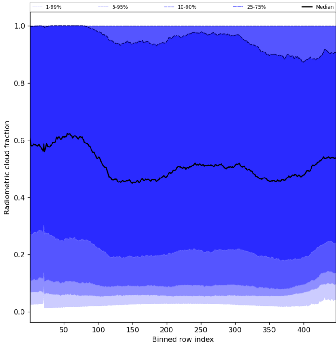
Figure 55: Along track statistics of “Radiometric cloud fraction” for 2023-09-18 to 2023-09-20
