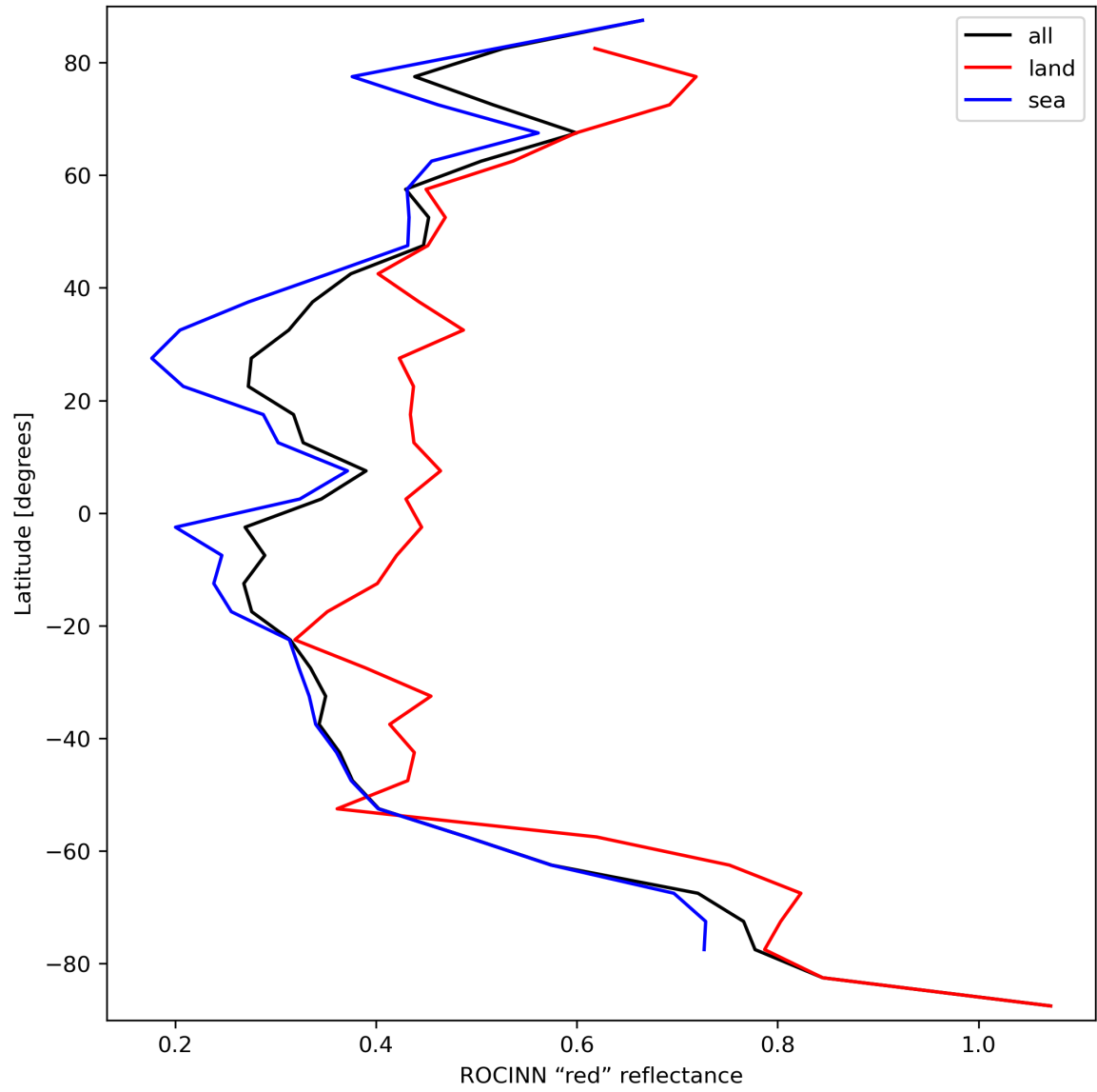
Figure 37: Zonal average of “ROCINN “red” reflectance” for 2023-09-18 to 2023-09-20.
