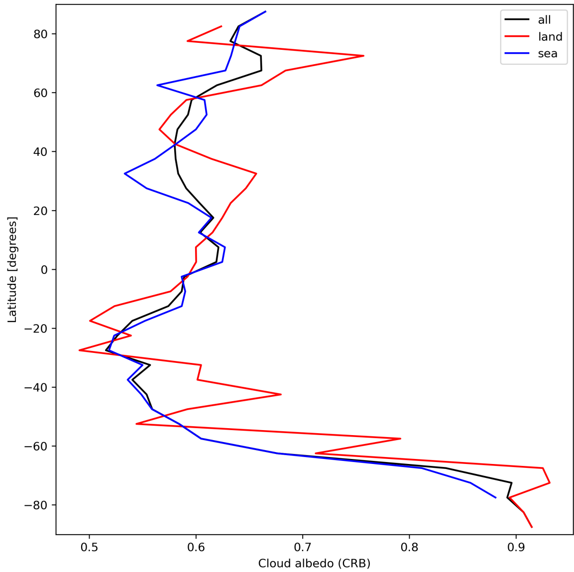
Figure 28: Zonal average of “Cloud albedo (CRB)” for 2023-09-20 to 2023-09-21.
