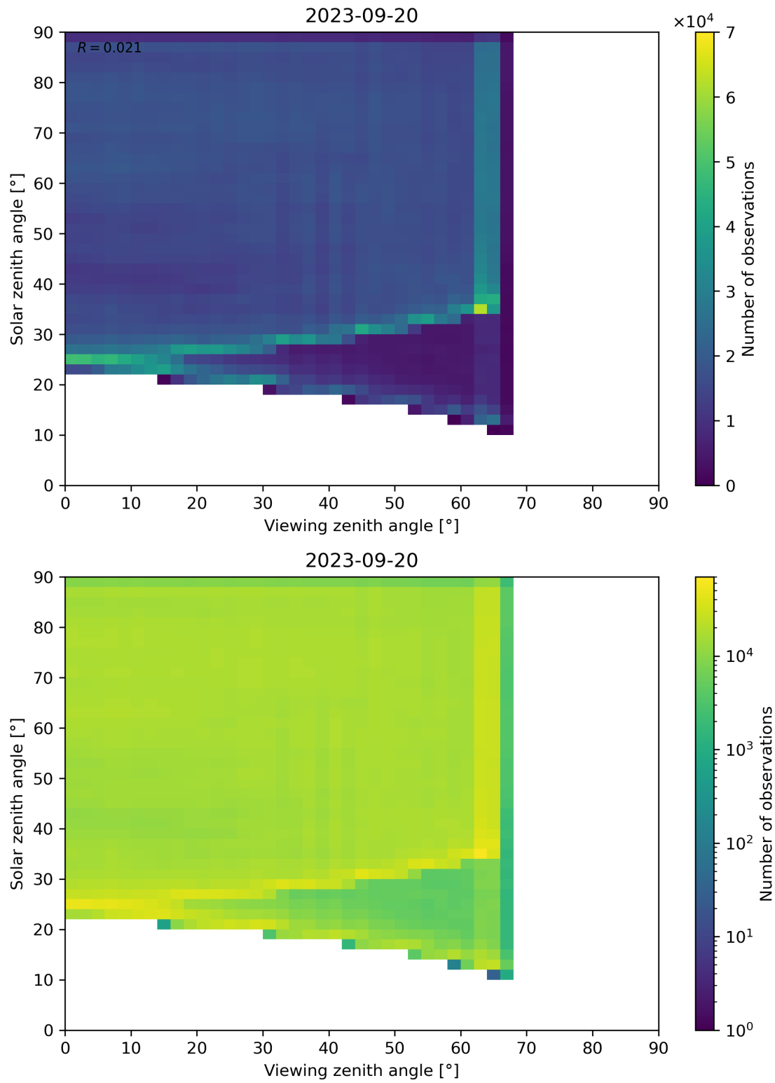
Figure 114: Scatter density plot of “Viewing zenith angle” against “Solar zenith angle” for 2023-09-20 to 2023-09-21.
