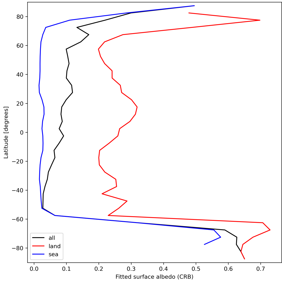
Figure 30: Zonal average of “Fitted surface albedo (CRB)” for 2023-09-20 to 2023-09-21.
