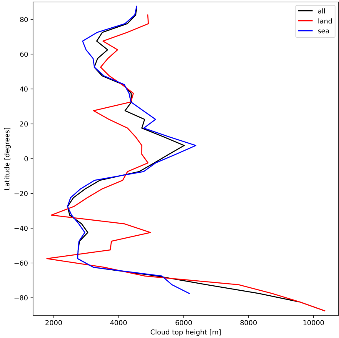
Figure 24: Zonal average of “Cloud top height” for 2023-09-20 to 2023-09-21.
