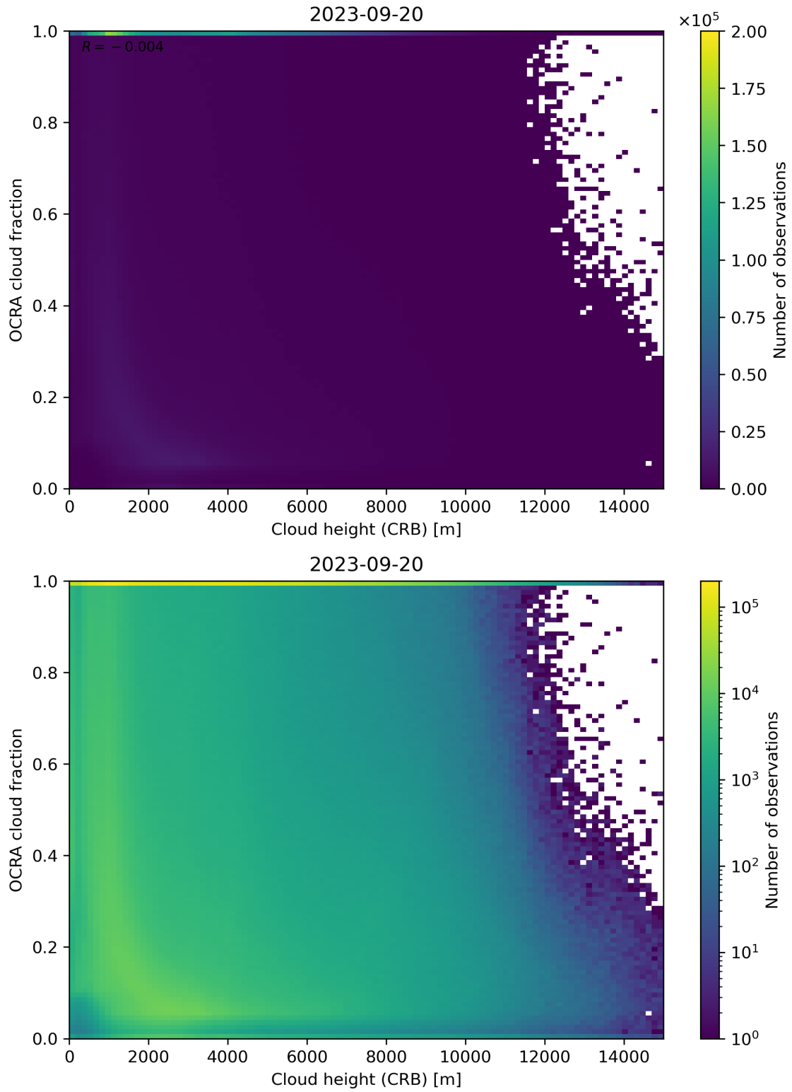
Figure 81: Scatter density plot of “Cloud height (CRB)” against “OCRA cloud fraction” for 2023-09-20 to 2023-09-21.
