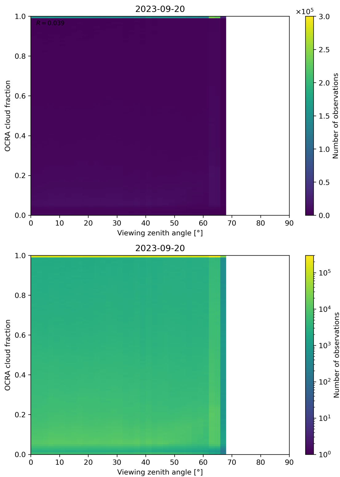
Figure 108: Scatter density plot of “Viewing zenith angle” against “OCRA cloud fraction” for 2023-09-20 to 2023-09-21.
