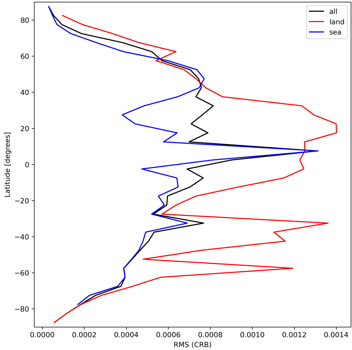
Figure 32: Zonal average of “RMS (CRB)” for 2023-09-20 to 2023-09-21.
