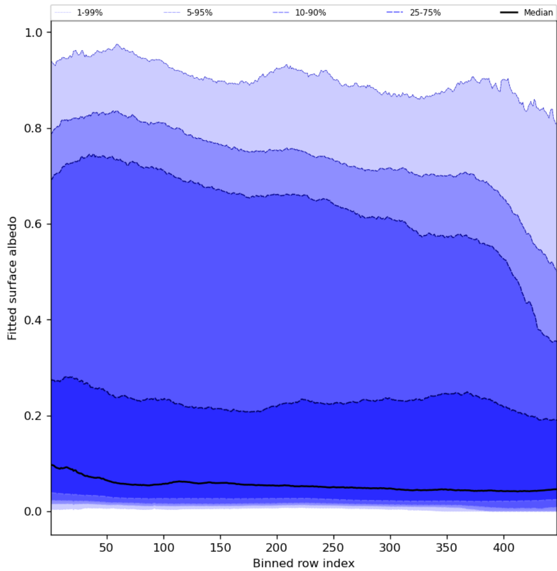
Figure 61: Along track statistics of “Fitted surface albedo” for 2023-09-20 to 2023-09-21
