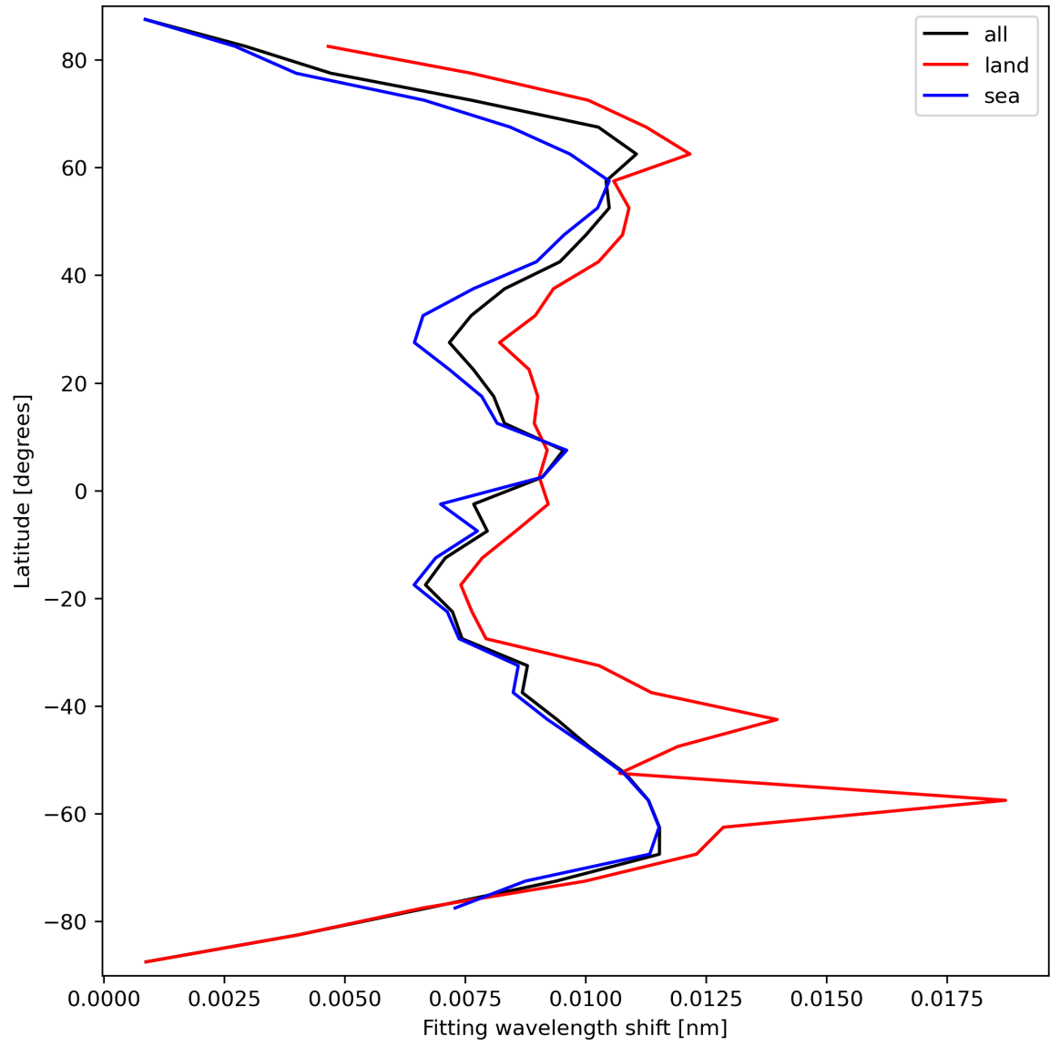
Figure 33: Zonal average of “Fitting wavelength shift” for 2023-09-20 to 2023-09-21.
