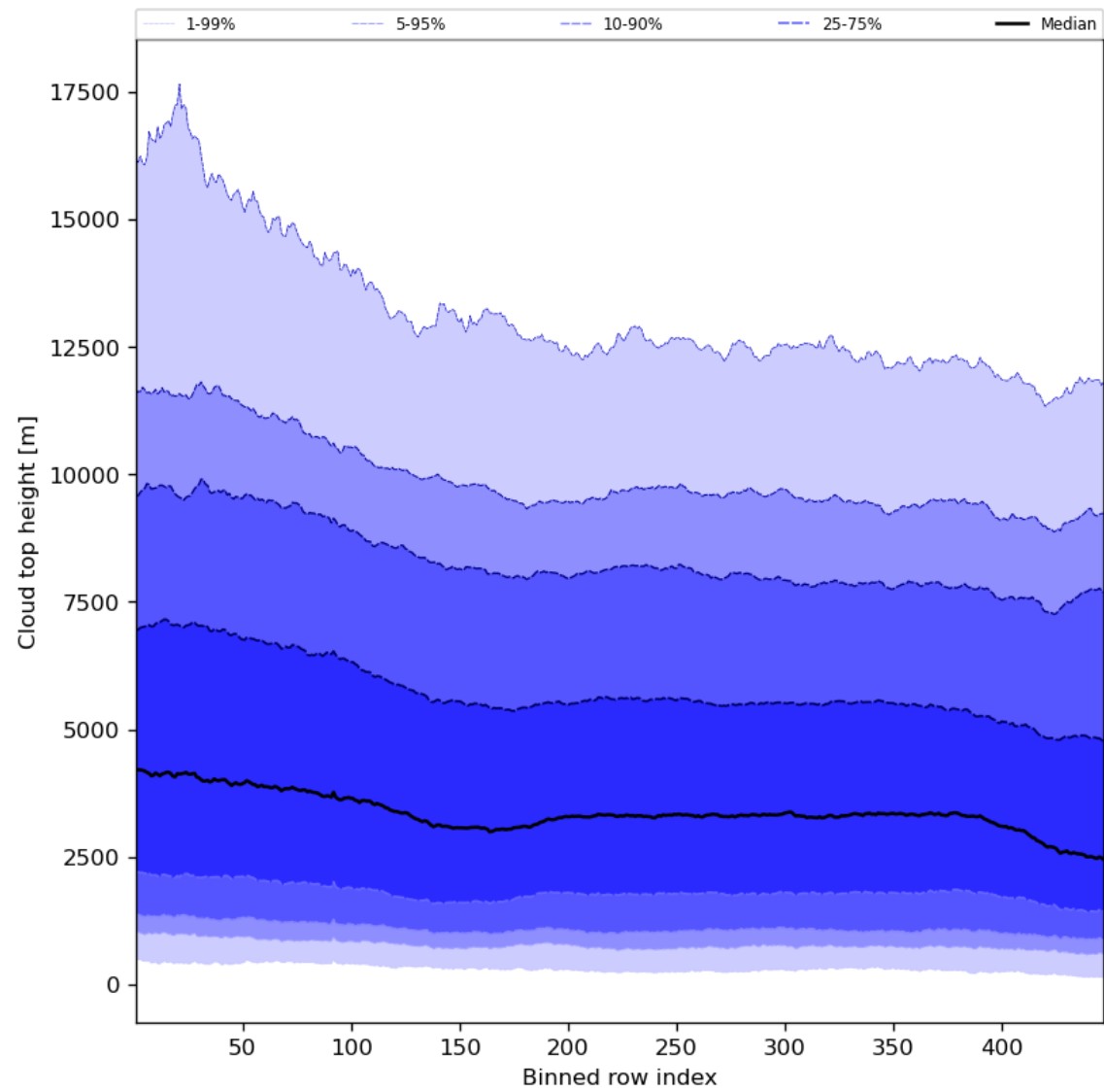
Figure 56: Along track statistics of “Cloud top height” for 2023-09-20 to 2023-09-21
