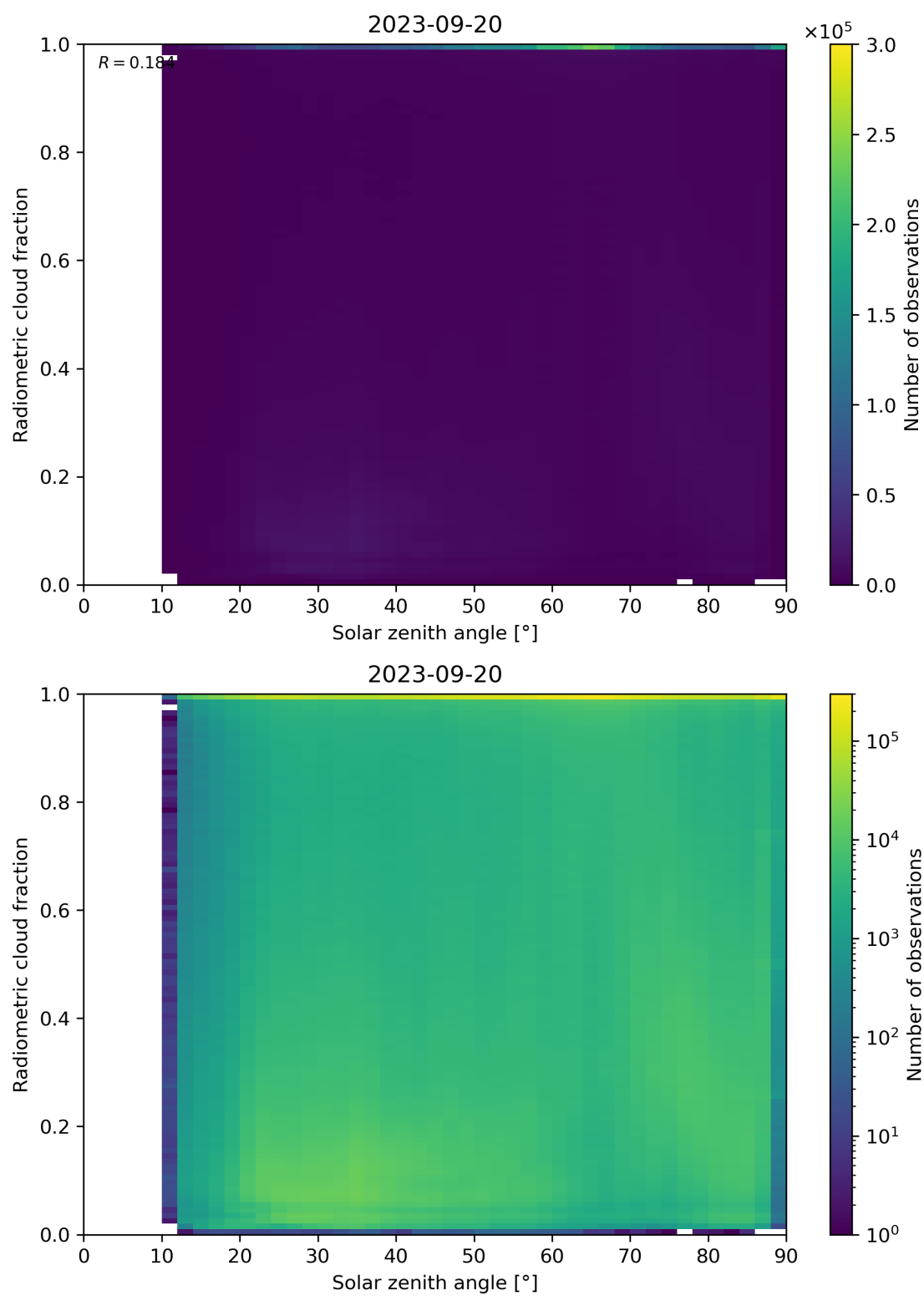
Figure 99: Scatter density plot of “Solar zenith angle” against “Radiometric cloud fraction” for 2023-09-20 to 2023-09-21.
