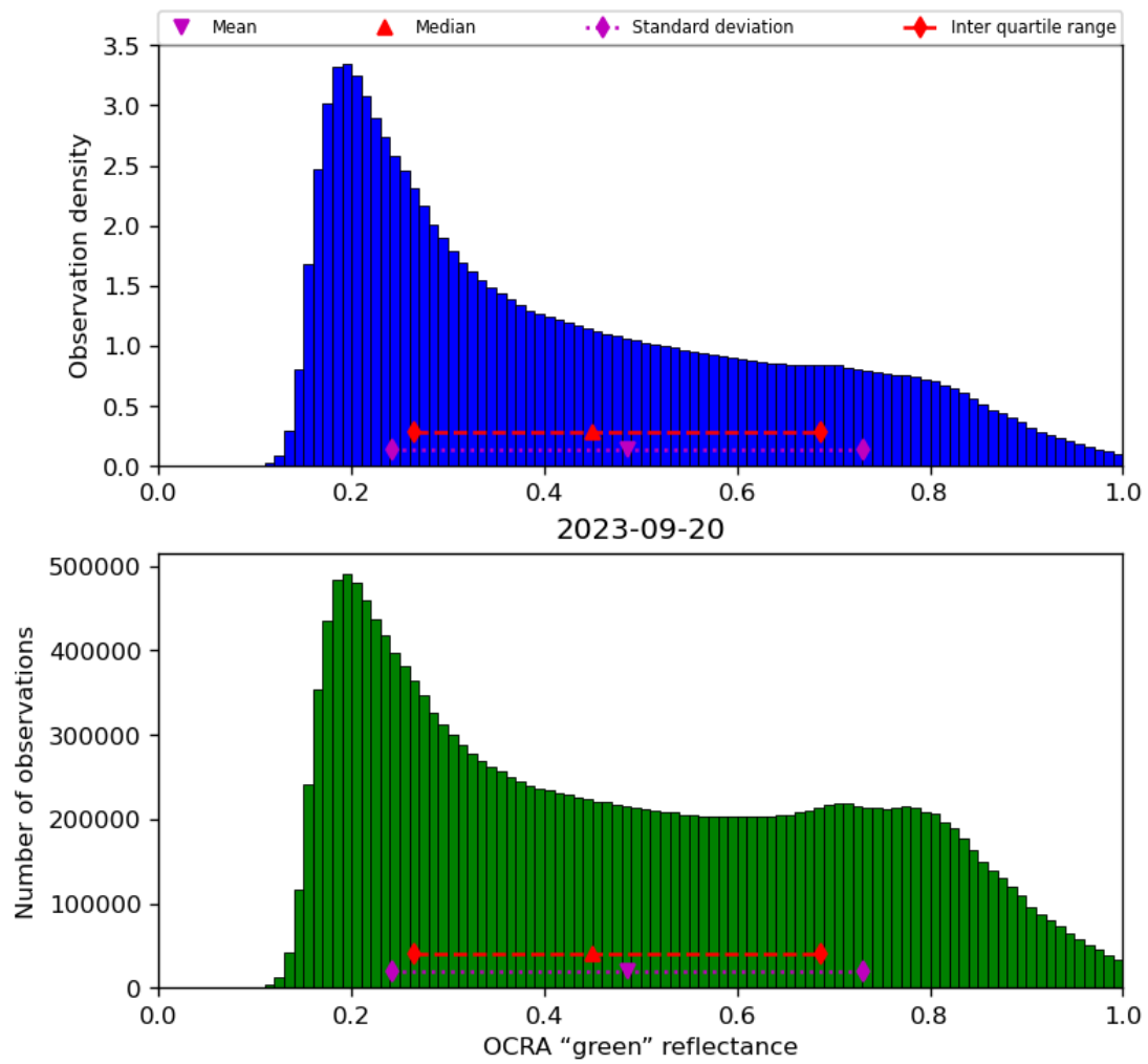
Figure 52: Histogram of “OCRA “green” reflectance” for 2023-09-20 to 2023-09-21
