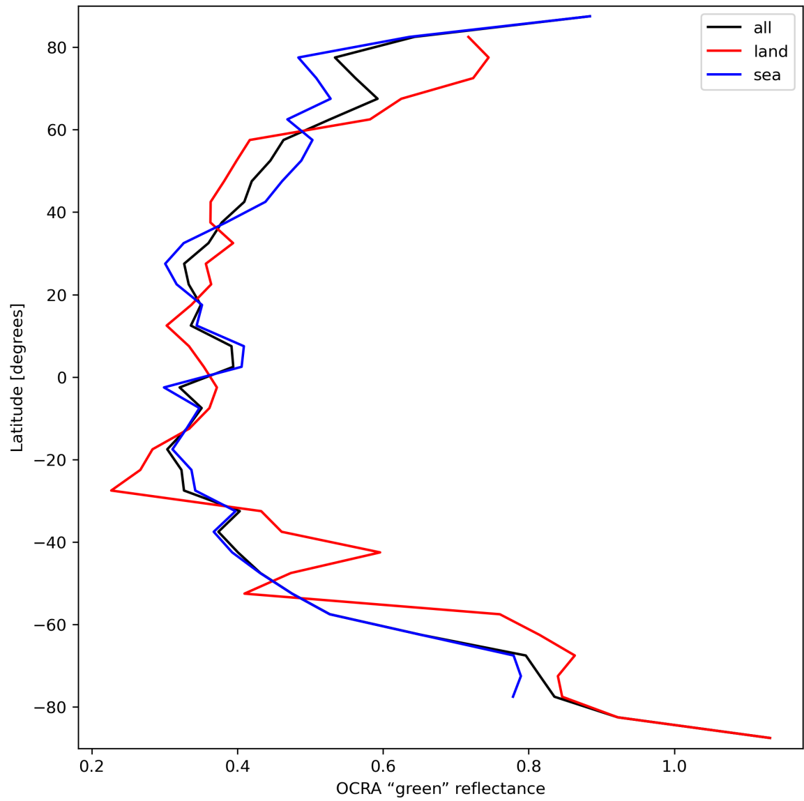
Figure 36: Zonal average of “OCRA “green” reflectance” for 2023-09-20 to 2023-09-21.
