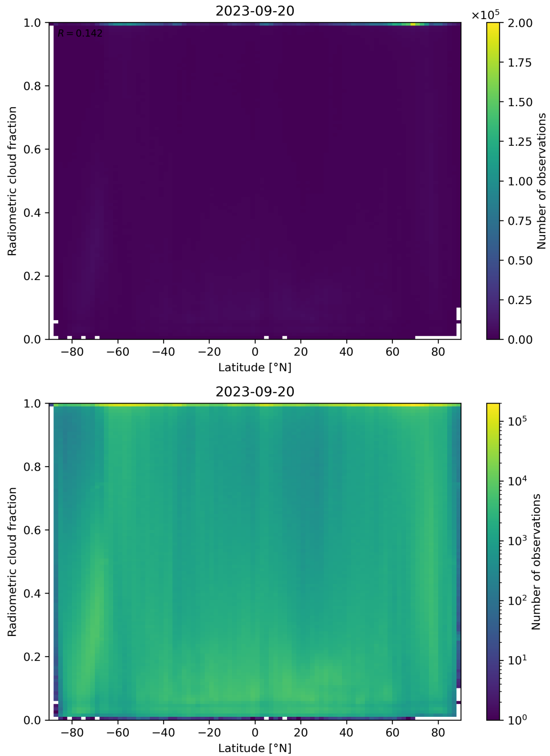
Figure 92: Scatter density plot of “Latitude” against “Radiometric cloud fraction” for 2023-09-20 to 2023-09-21.
