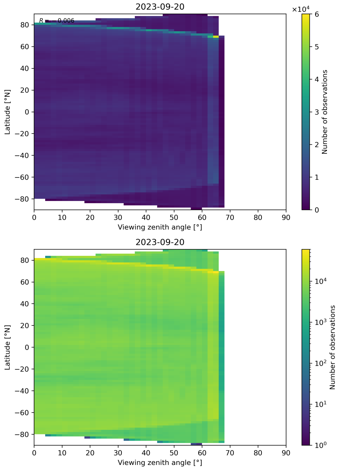
Figure 113: Scatter density plot of “Viewing zenith angle” against “Latitude” for 2023-09-20 to 2023-09-21.
