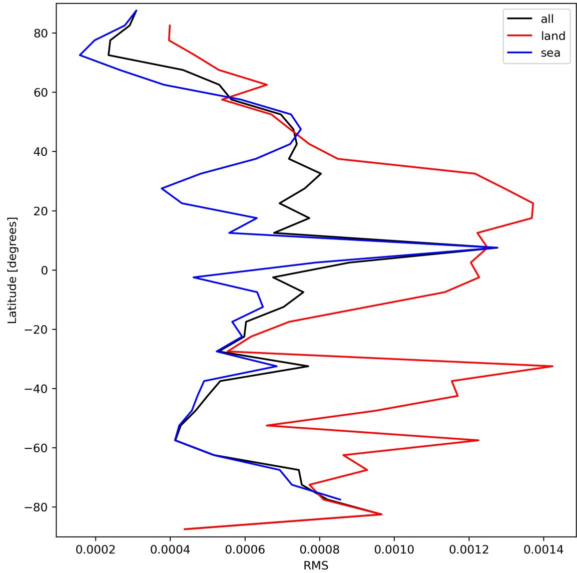
Figure 31: Zonal average of “RMS” for 2023-09-20 to 2023-09-21.
