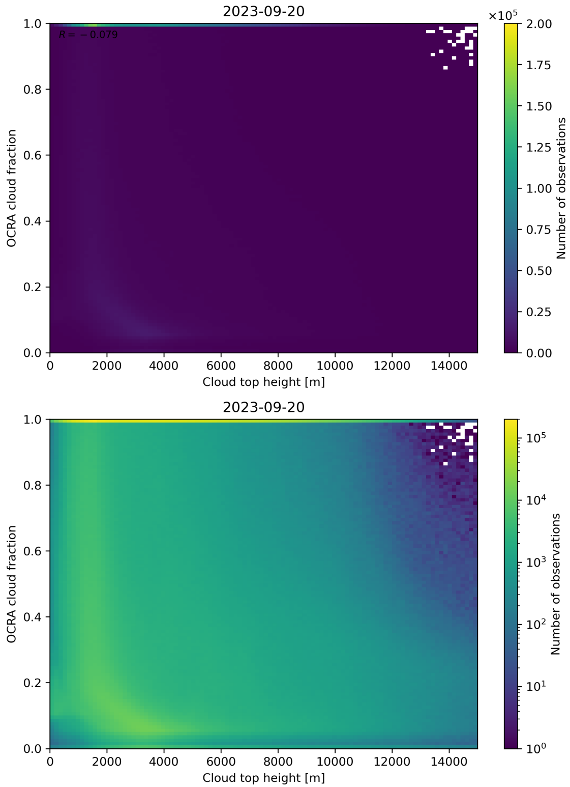
Figure 87: Scatter density plot of “Cloud top height” against “OCRA cloud fraction” for 2023-09-20 to 2023-09-21.
