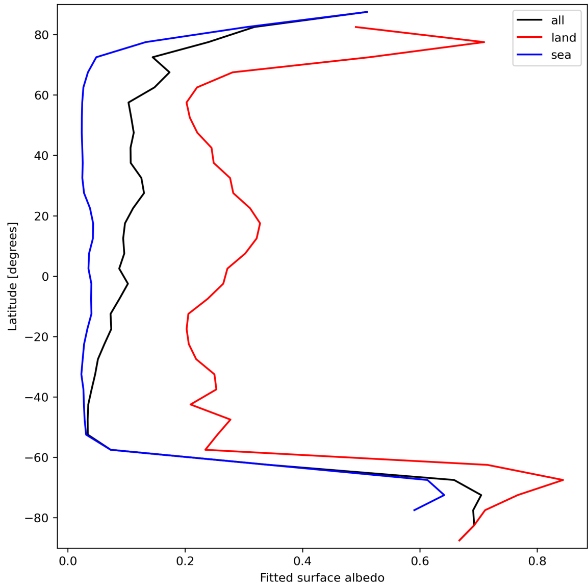
Figure 29: Zonal average of “Fitted surface albedo” for 2023-09-20 to 2023-09-21.
