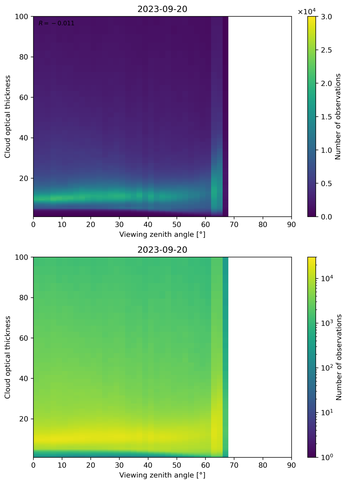
Figure 111: Scatter density plot of “Viewing zenith angle” against “Cloud optical thickness” for 2023-09-20 to 2023-09-21.
