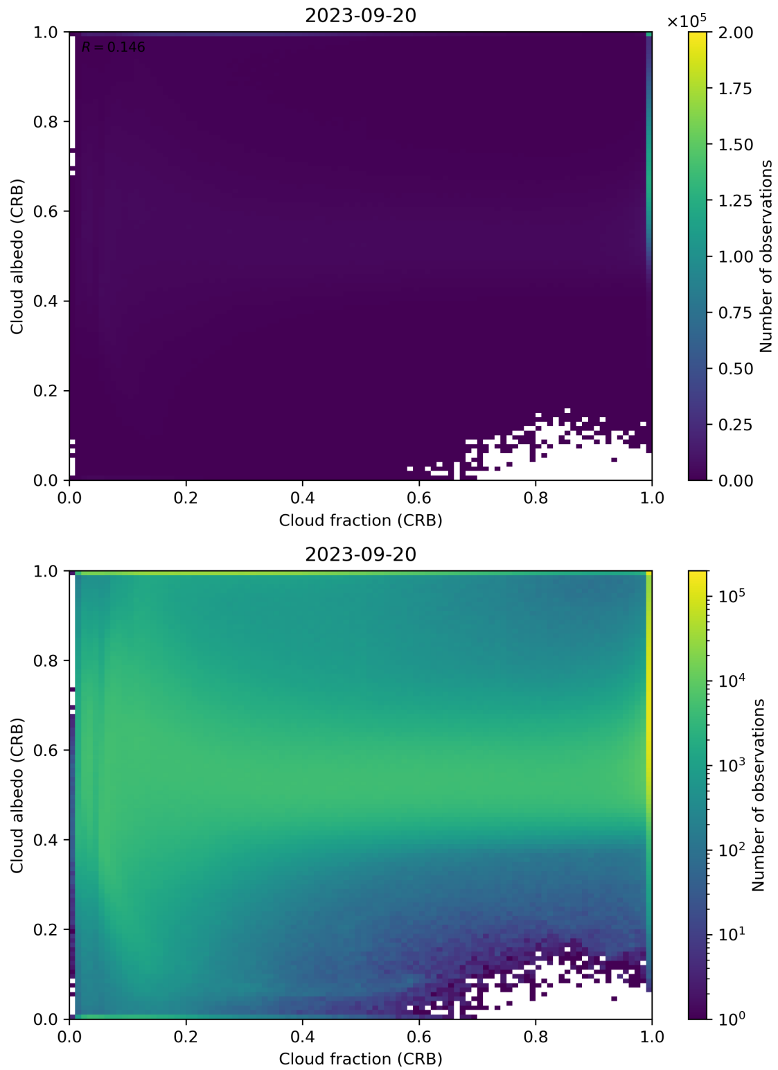
Figure 77: Scatter density plot of “Cloud fraction (CRB)” against “Cloud albedo (CRB)” for 2023-09-20 to 2023-09-21.
