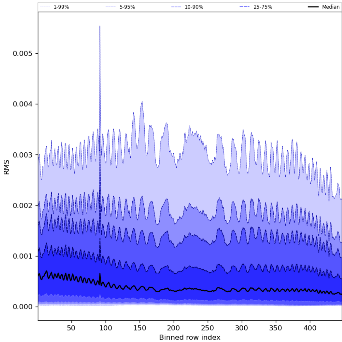
Figure 63: Along track statistics of “RMS” for 2023-09-20 to 2023-09-21
