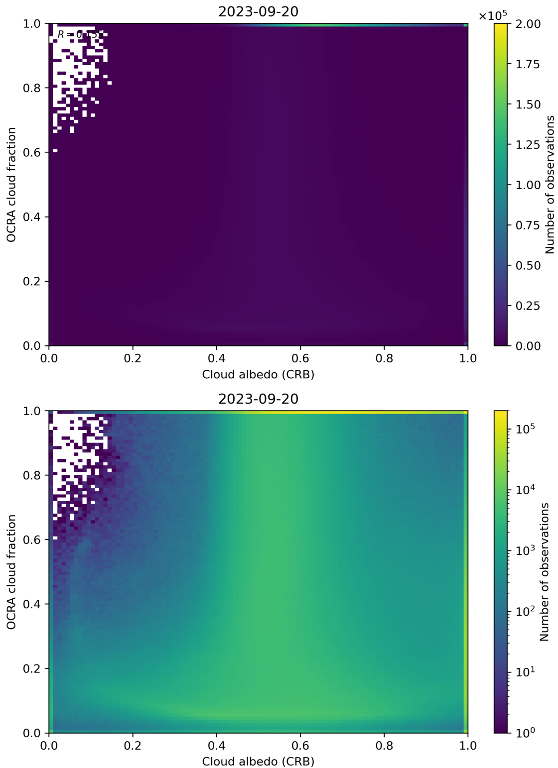
Figure 70: Scatter density plot of “Cloud albedo (CRB)” against “OCRA cloud fraction” for 2023-09-20 to 2023-09-21.
