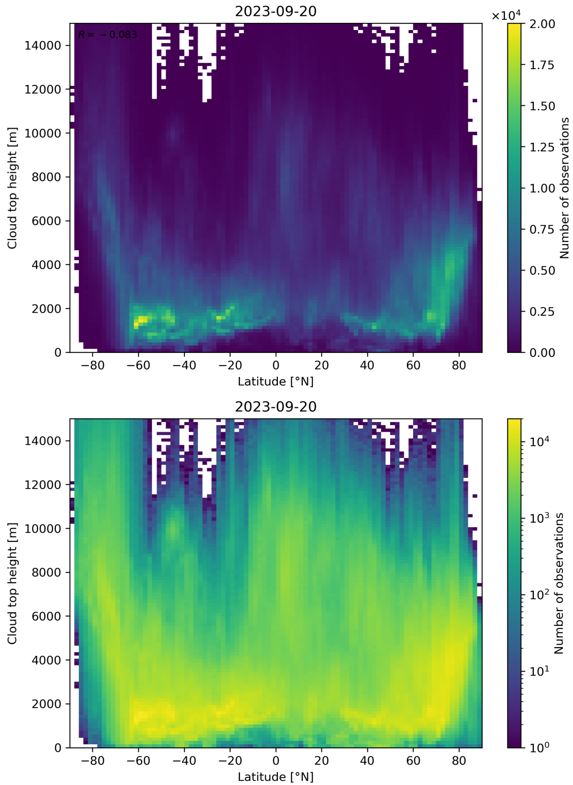
Figure 97: Scatter density plot of “Latitude” against “Cloud top height” for 2023-09-20 to 2023-09-21.
