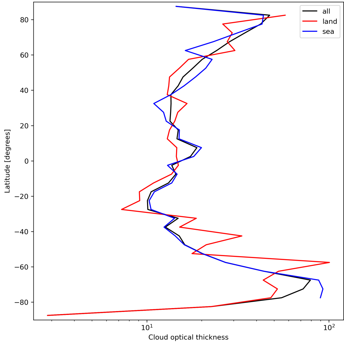
Figure 25: Zonal average of “Cloud optical thickness” for 2023-09-20 to 2023-09-21.
