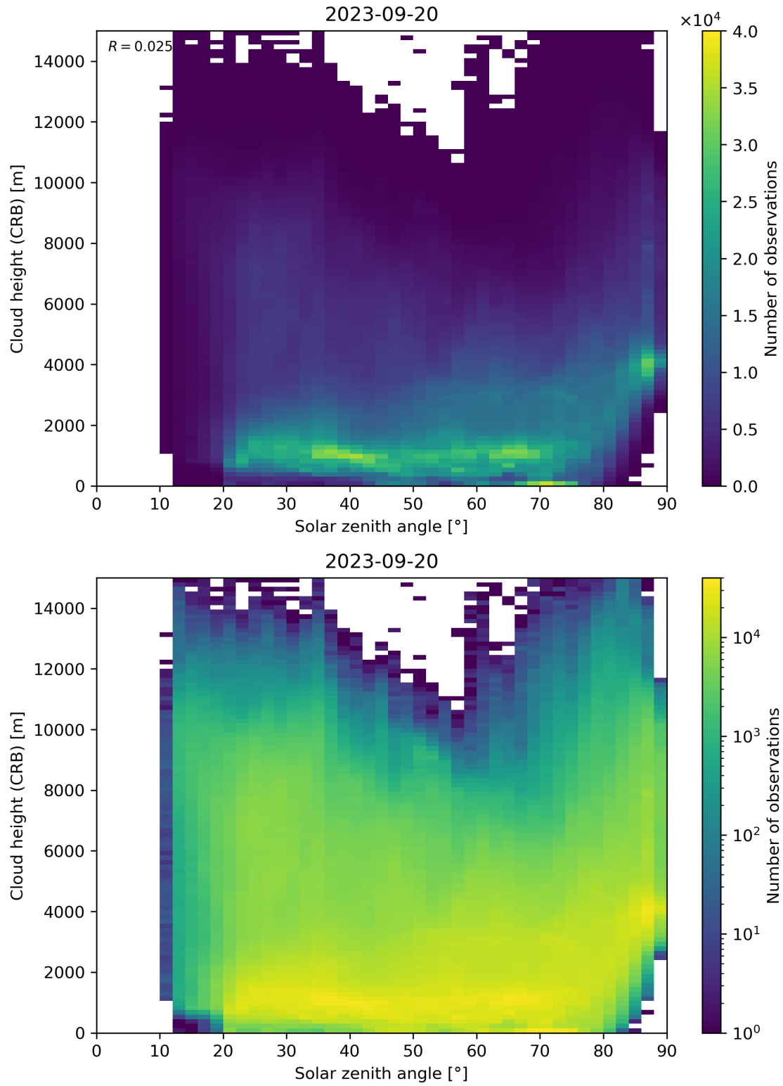
Figure 102: Scatter density plot of “Solar zenith angle” against “Cloud height (CRB)” for 2023-09-20 to 2023-09-21.
