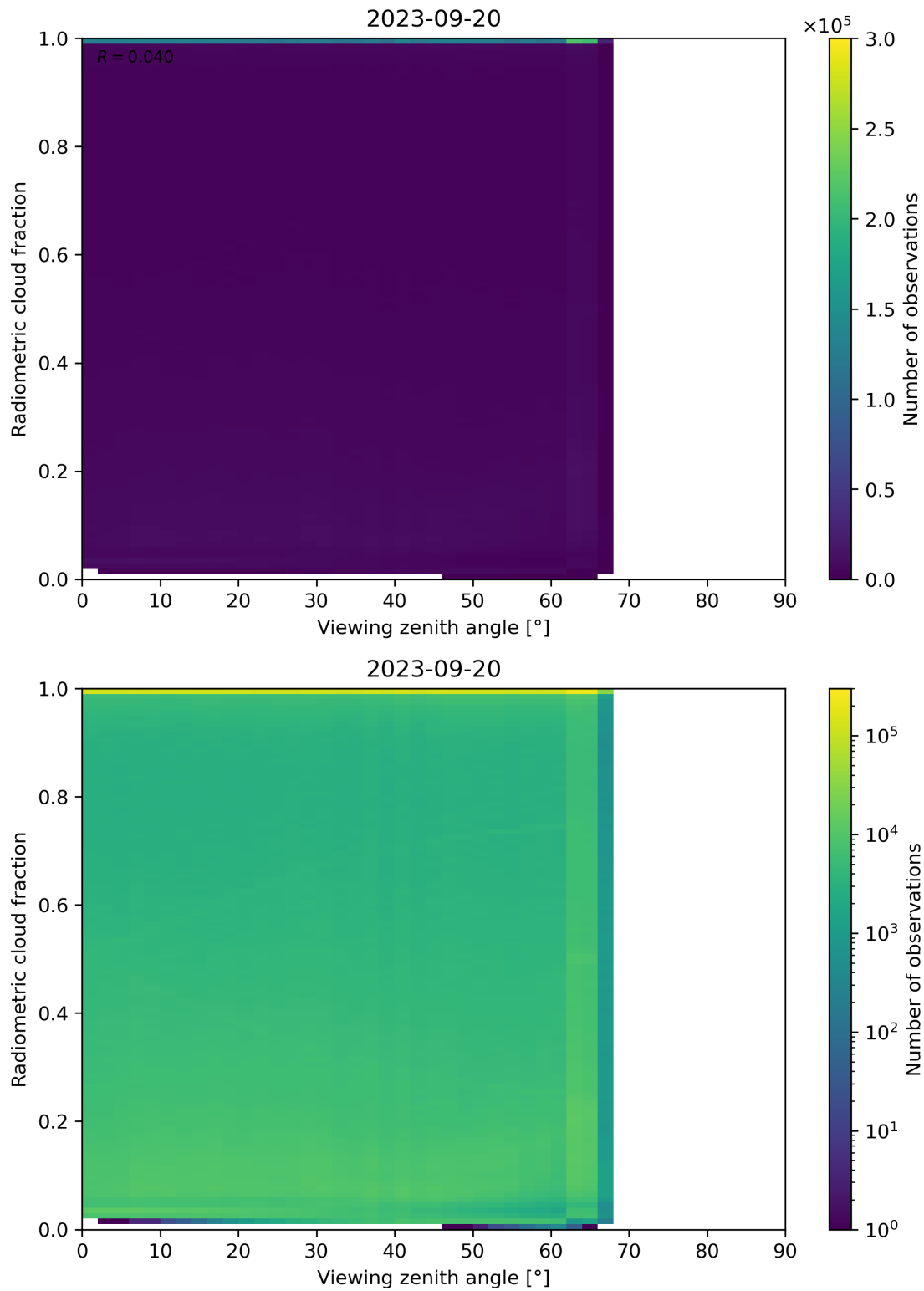
Figure 107: Scatter density plot of “Viewing zenith angle” against “Radiometric cloud fraction” for 2023-09-20 to 2023-09-21.
