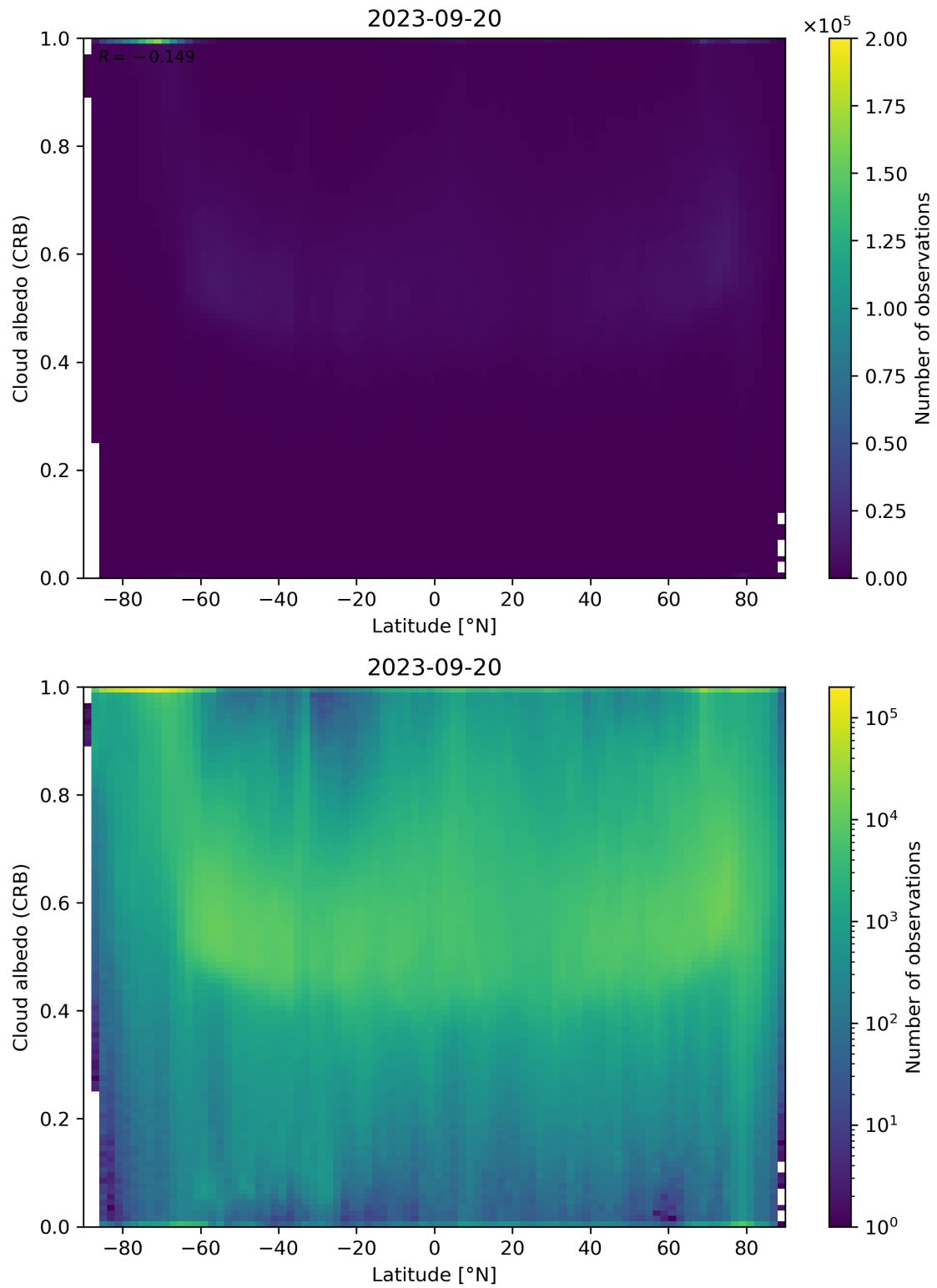
Figure 91: Scatter density plot of “Latitude” against “Cloud albedo (CRB)” for 2023-09-20 to 2023-09-21.
