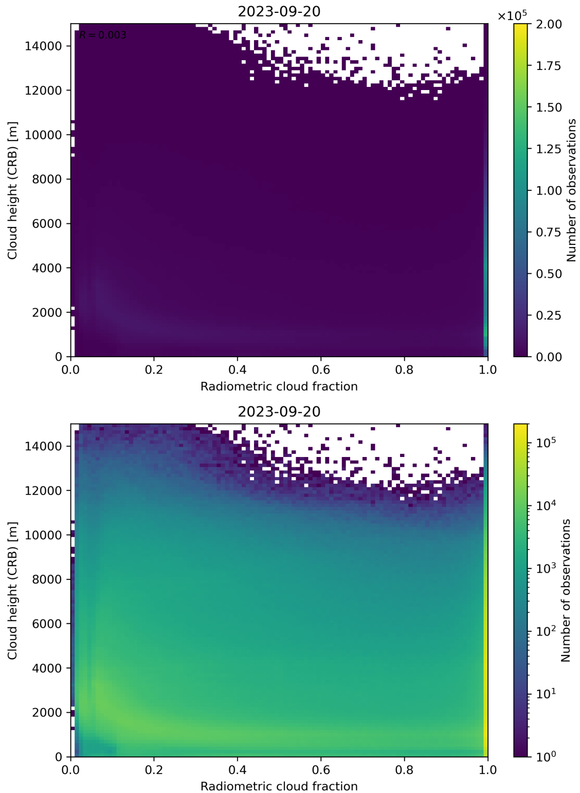
Figure 74: Scatter density plot of “Radiometric cloud fraction” against “Cloud height (CRB)” for 2023-09-20 to 2023-09-21.
