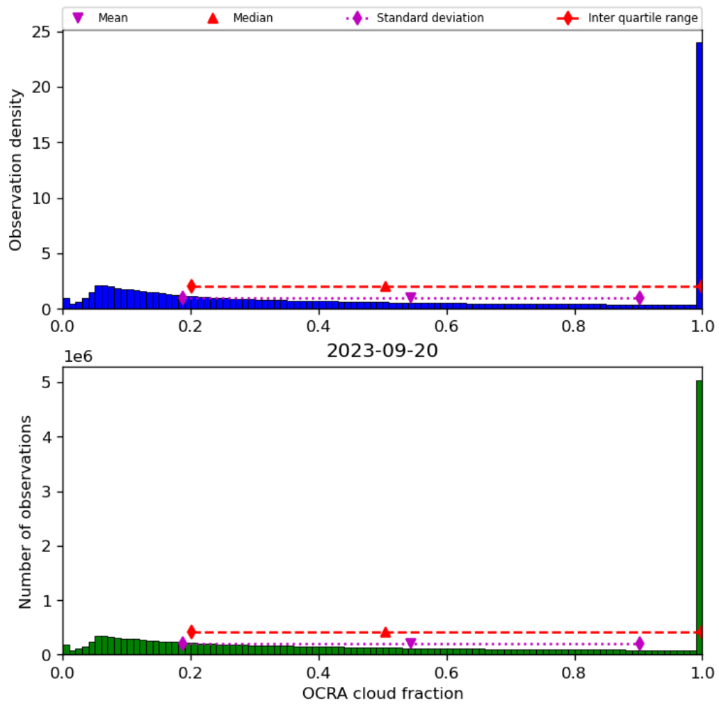
Figure 50: Histogram of “OCRA cloud fraction” for 2023-09-20 to 2023-09-21
