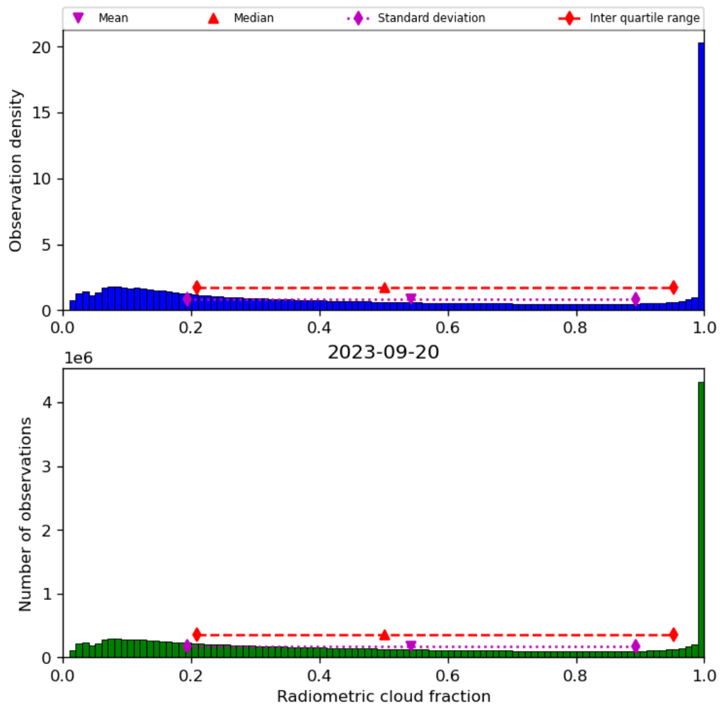
Figure 39: Histogram of “Radiometric cloud fraction” for 2023-09-20 to 2023-09-21
