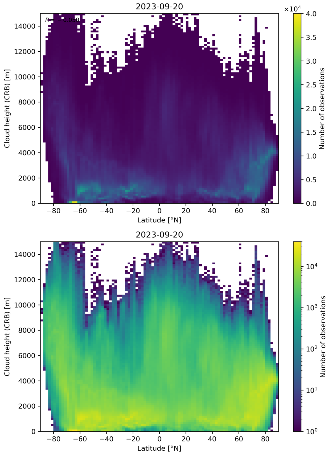
Figure 95: Scatter density plot of “Latitude” against “Cloud height (CRB)” for 2023-09-20 to 2023-09-21.
