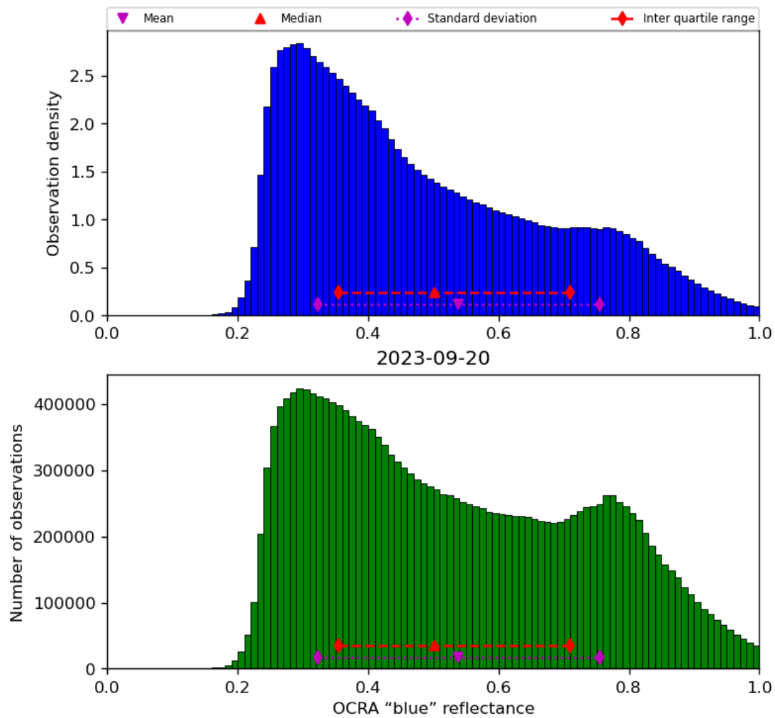
Figure 51: Histogram of “OCRA “blue” reflectance” for 2023-09-20 to 2023-09-21
