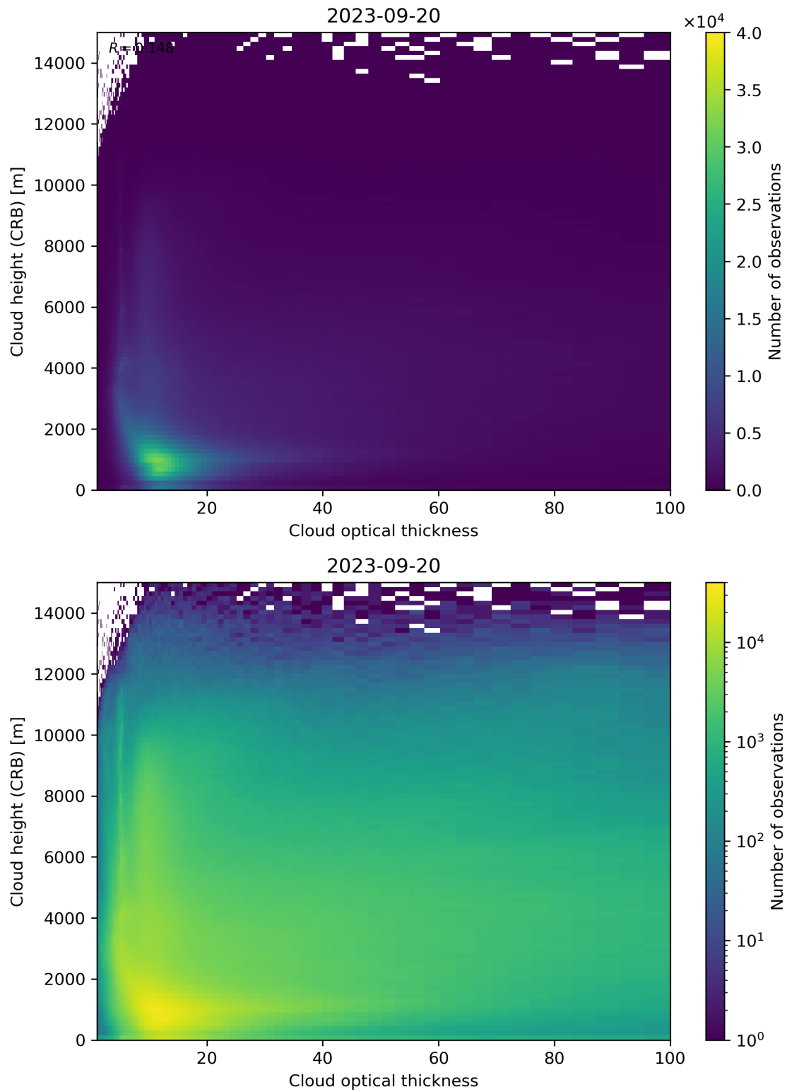
Figure 85: Scatter density plot of “Cloud optical thickness” against “Cloud height (CRB)” for 2023-09-20 to 2023-09-21.
