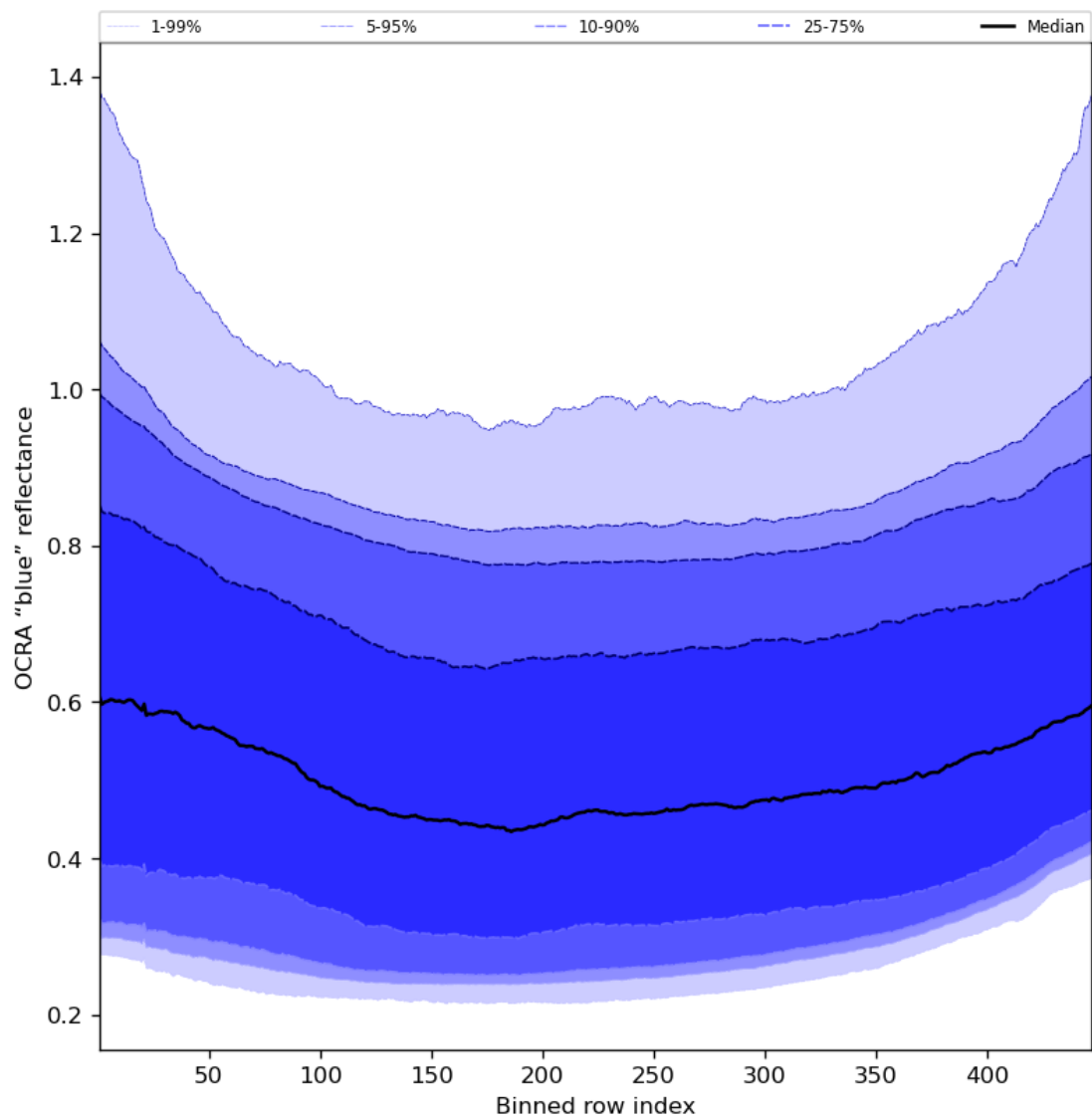
Figure 67: Along track statistics of “OCRA “blue” reflectance” for 2023-09-20 to 2023-09-21
