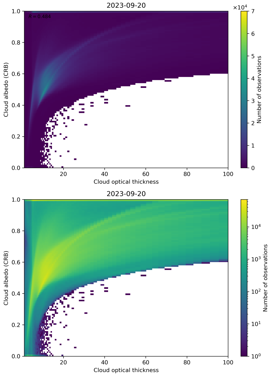
Figure 82: Scatter density plot of “Cloud optical thickness” against “Cloud albedo (CRB)” for 2023-09-20 to 2023-09-21.
