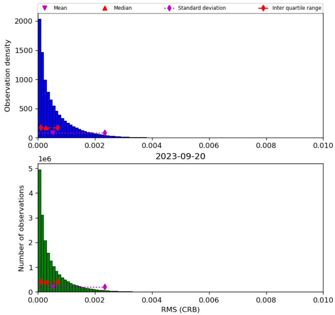
Figure 48: Histogram of "RMS (CRB)" for 2023-09-20 to 2023-09-21
