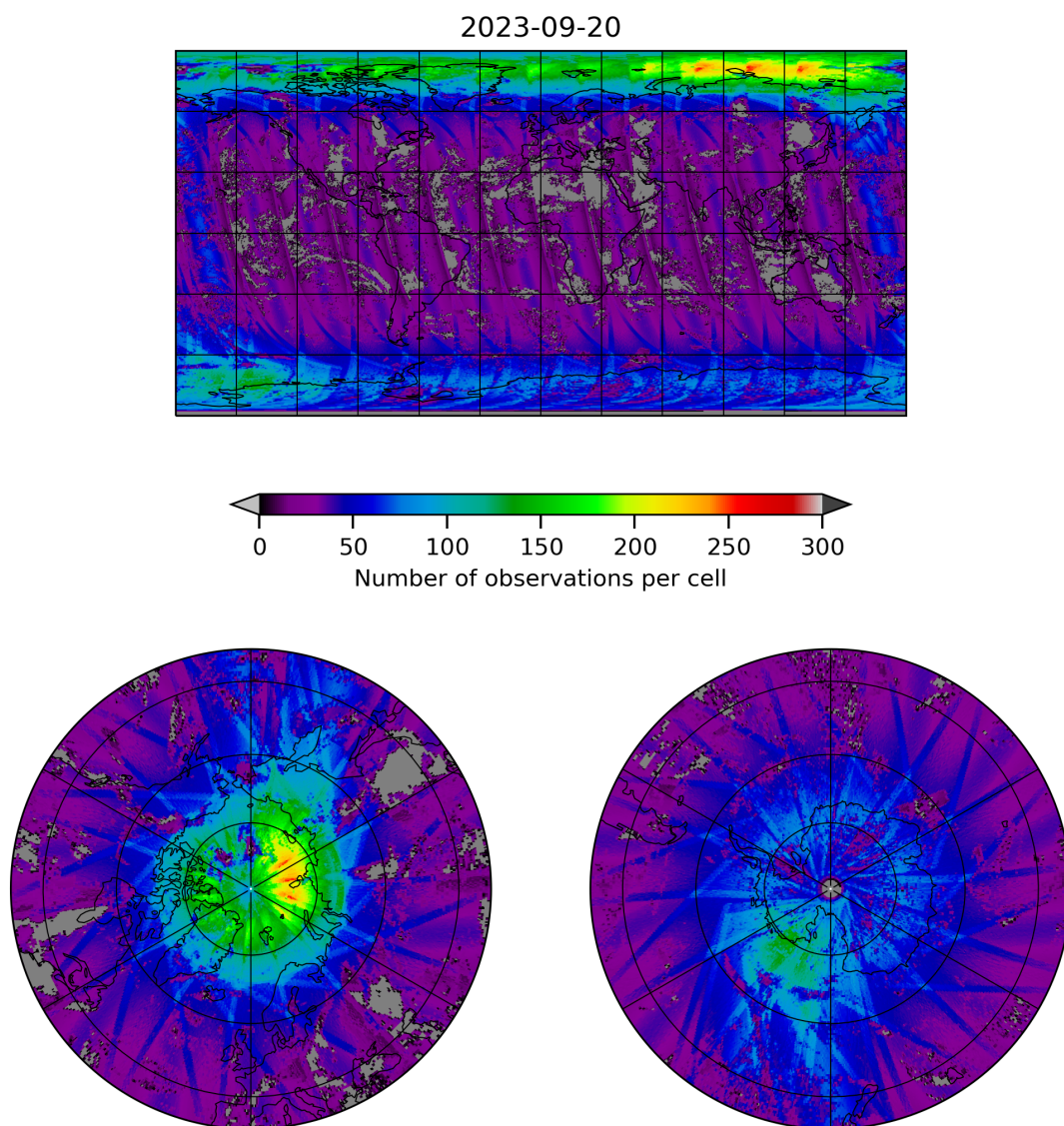
Figure 21: Map of the number of observations for 2023-09-20 to 2023-09-21
