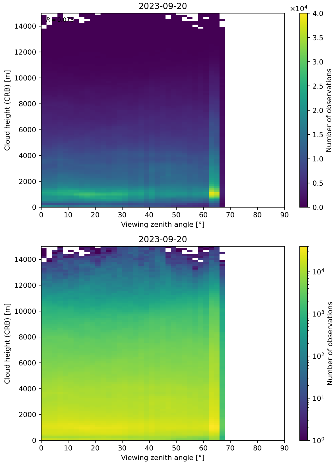
Figure 110: Scatter density plot of “Viewing zenith angle” against “Cloud height (CRB)” for 2023-09-20 to 2023-09-21.
