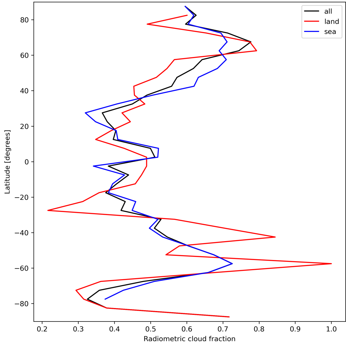
Figure 23: Zonal average of “Radiometric cloud fraction” for 2023-09-20 to 2023-09-21.
