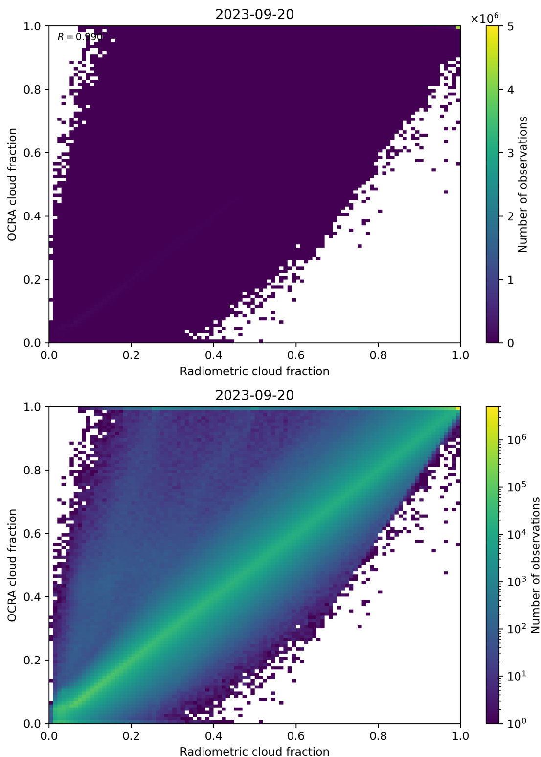
Figure 72: Scatter density plot of “Radiometric cloud fraction” against “OCRA cloud fraction” for 2023-09-20 to 2023-09-21.
