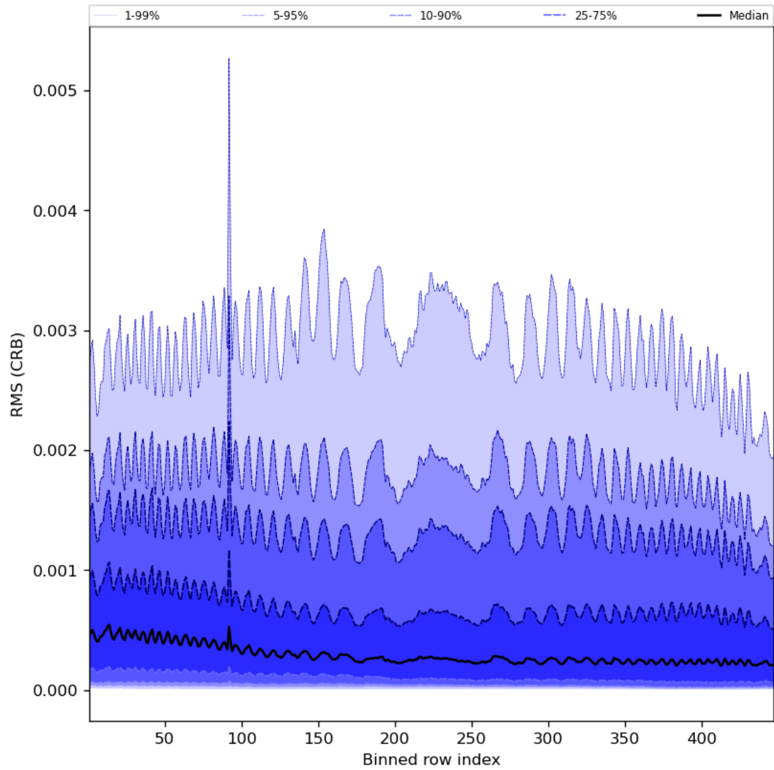
Figure 64: Along track statistics of "RMS (CRB)" for 2023-09-20 to 2023-09-21
