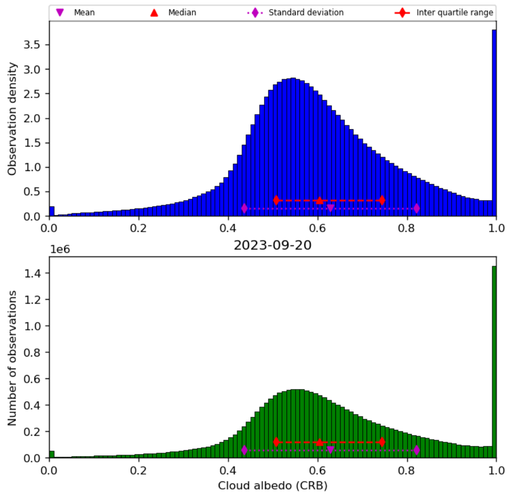
Figure 44: Histogram of “Cloud albedo (CRB)” for 2023-09-20 to 2023-09-21
