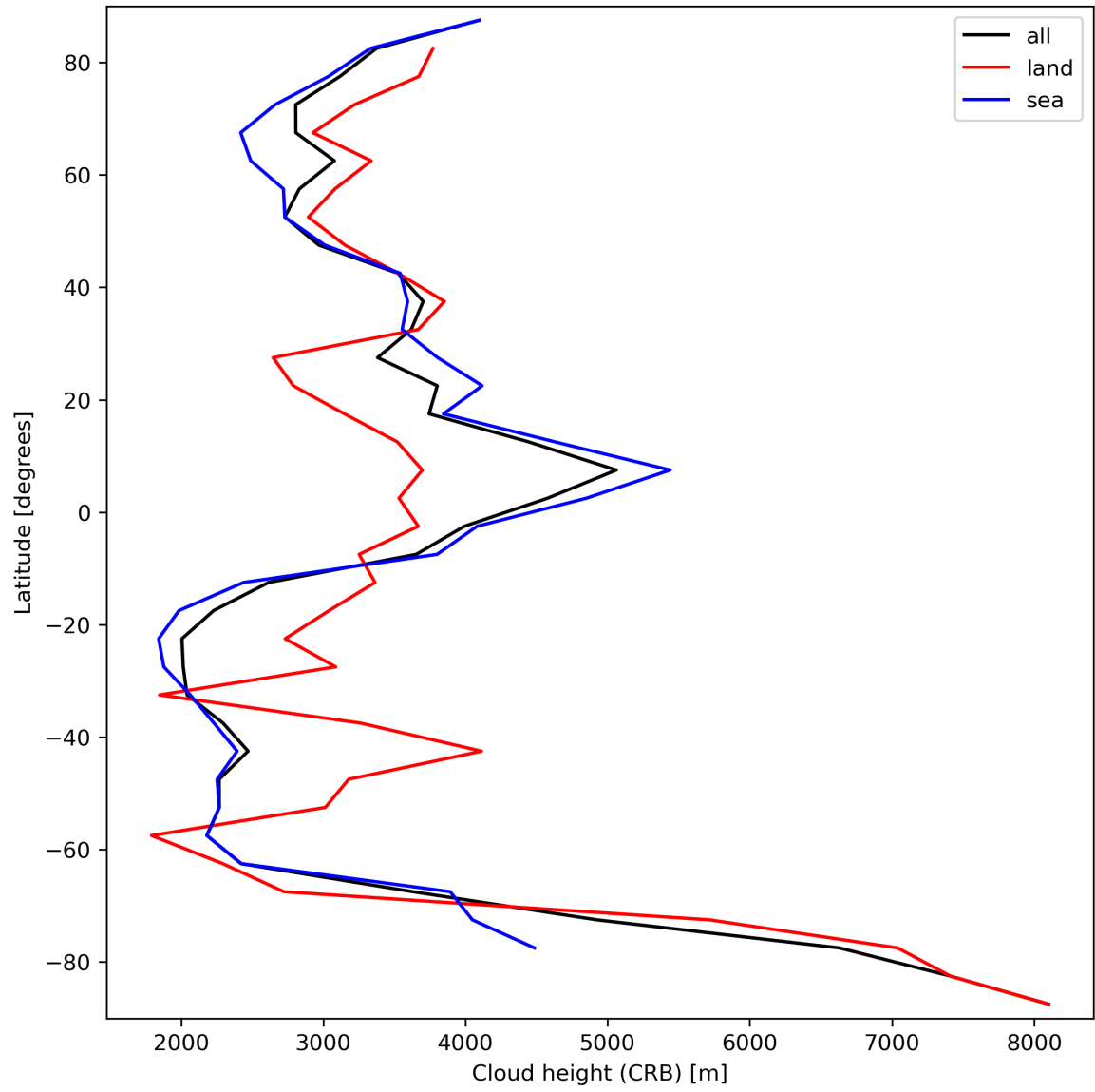
Figure 27: Zonal average of “Cloud height (CRB)” for 2023-09-20 to 2023-09-21.
