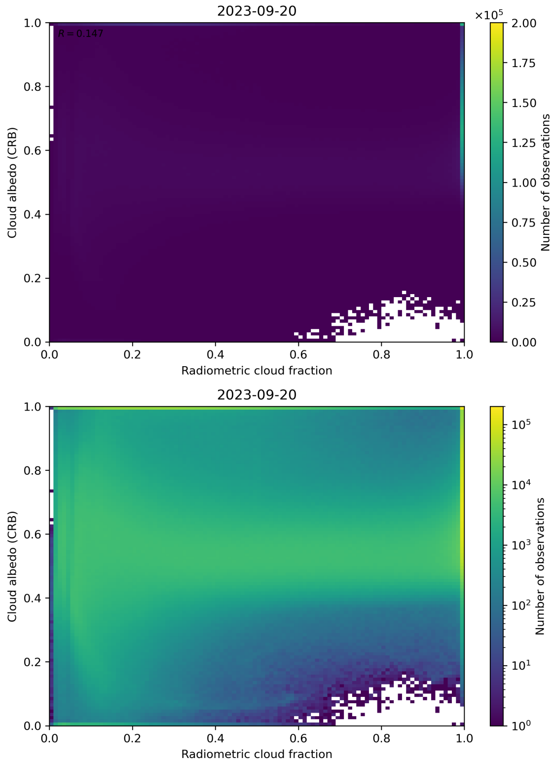
Figure 71: Scatter density plot of “Radiometric cloud fraction” against “Cloud albedo (CRB)” for 2023-09-20 to 2023-09-21.
