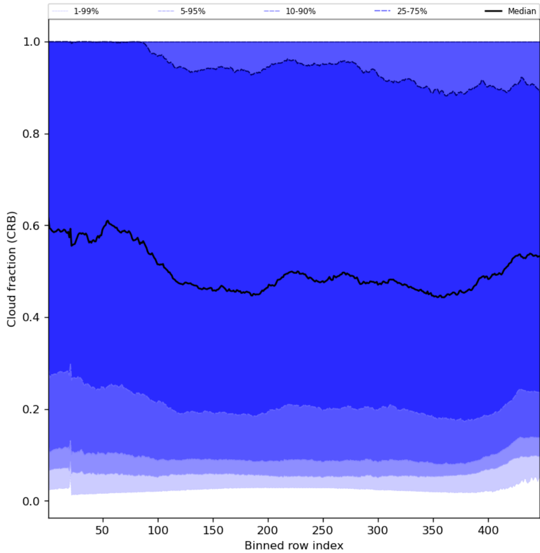
Figure 58: Along track statistics of “Cloud fraction (CRB)” for 2023-09-20 to 2023-09-21
