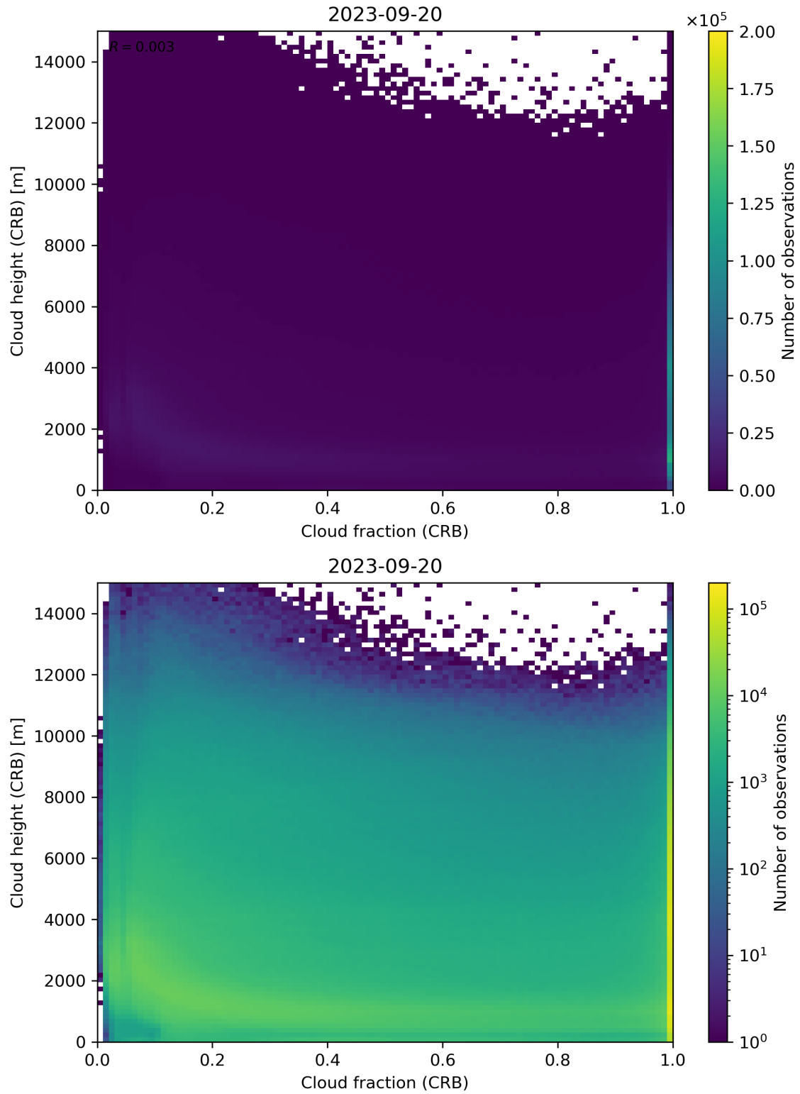
Figure 79: Scatter density plot of “Cloud fraction (CRB)” against “Cloud height (CRB)” for 2023-09-20 to 2023-09-21.
