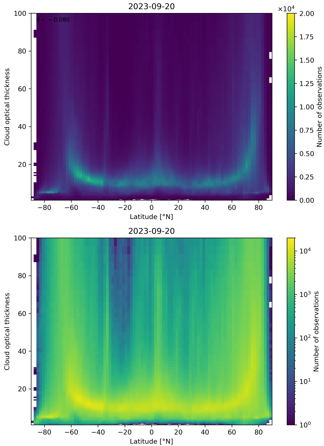
Figure 96: Scatter density plot of “Latitude” against “Cloud optical thickness” for 2023-09-20 to 2023-09-21.
