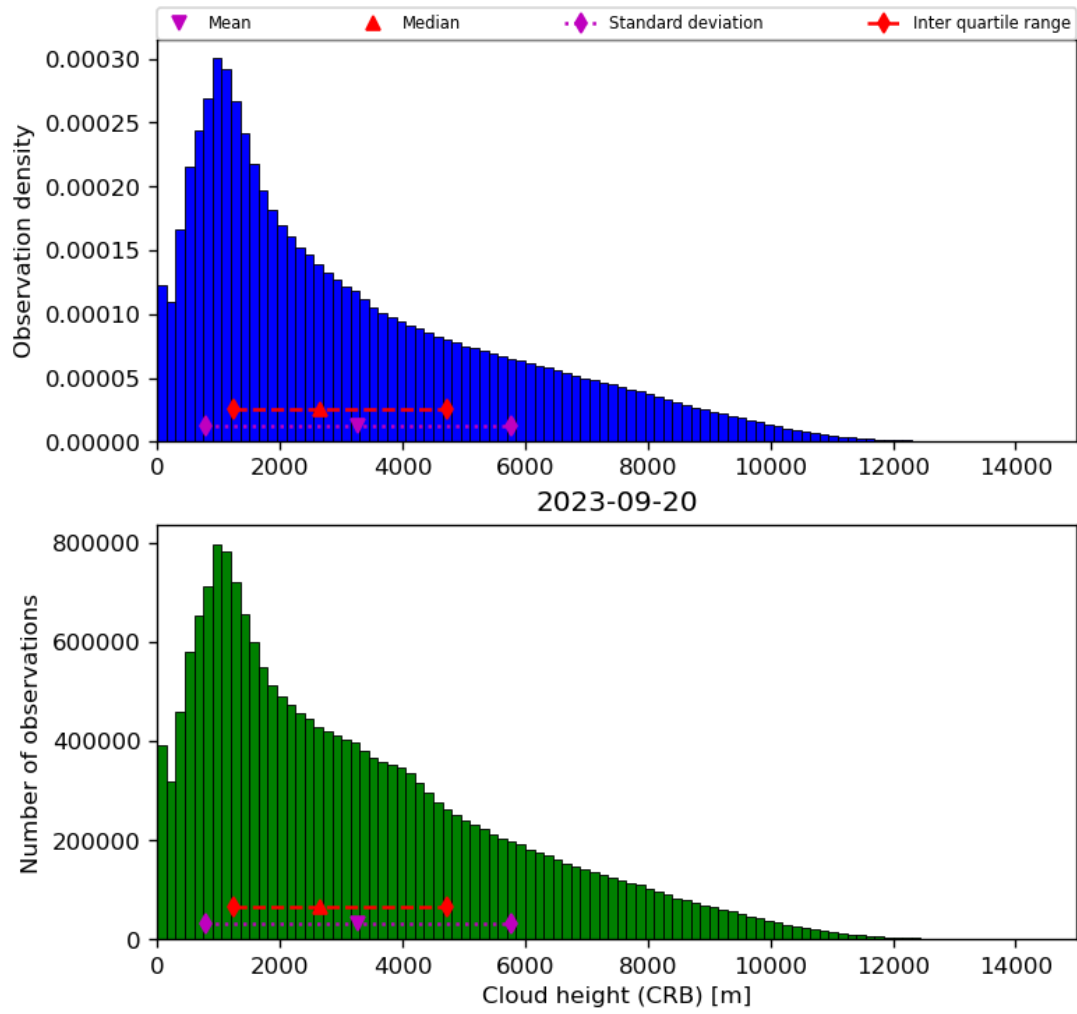
Figure 43: Histogram of “Cloud height (CRB)” for 2023-09-20 to 2023-09-21
