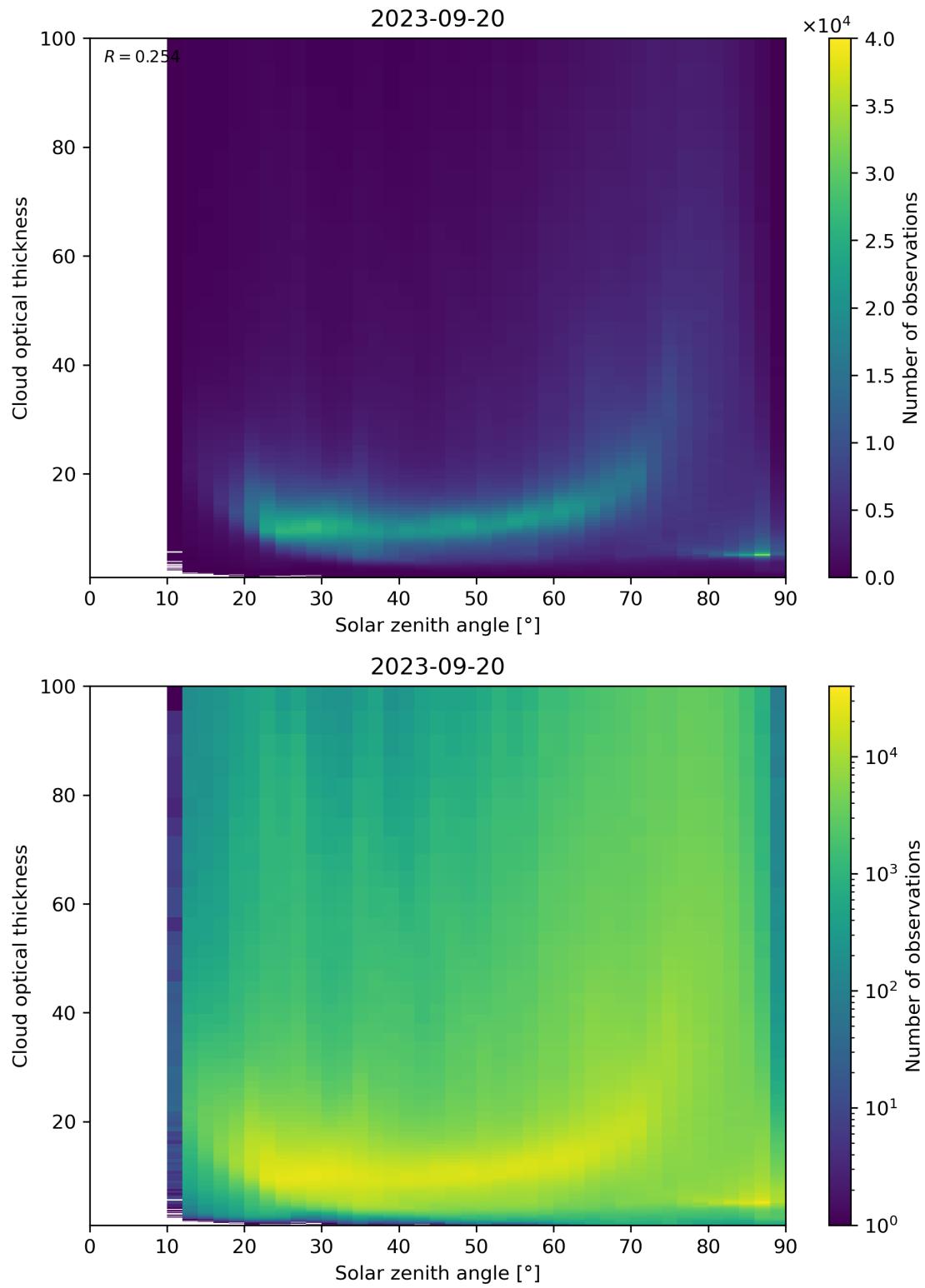
Figure 103: Scatter density plot of “Solar zenith angle” against “Cloud optical thickness” for 2023-09-20 to 2023-09-21.
