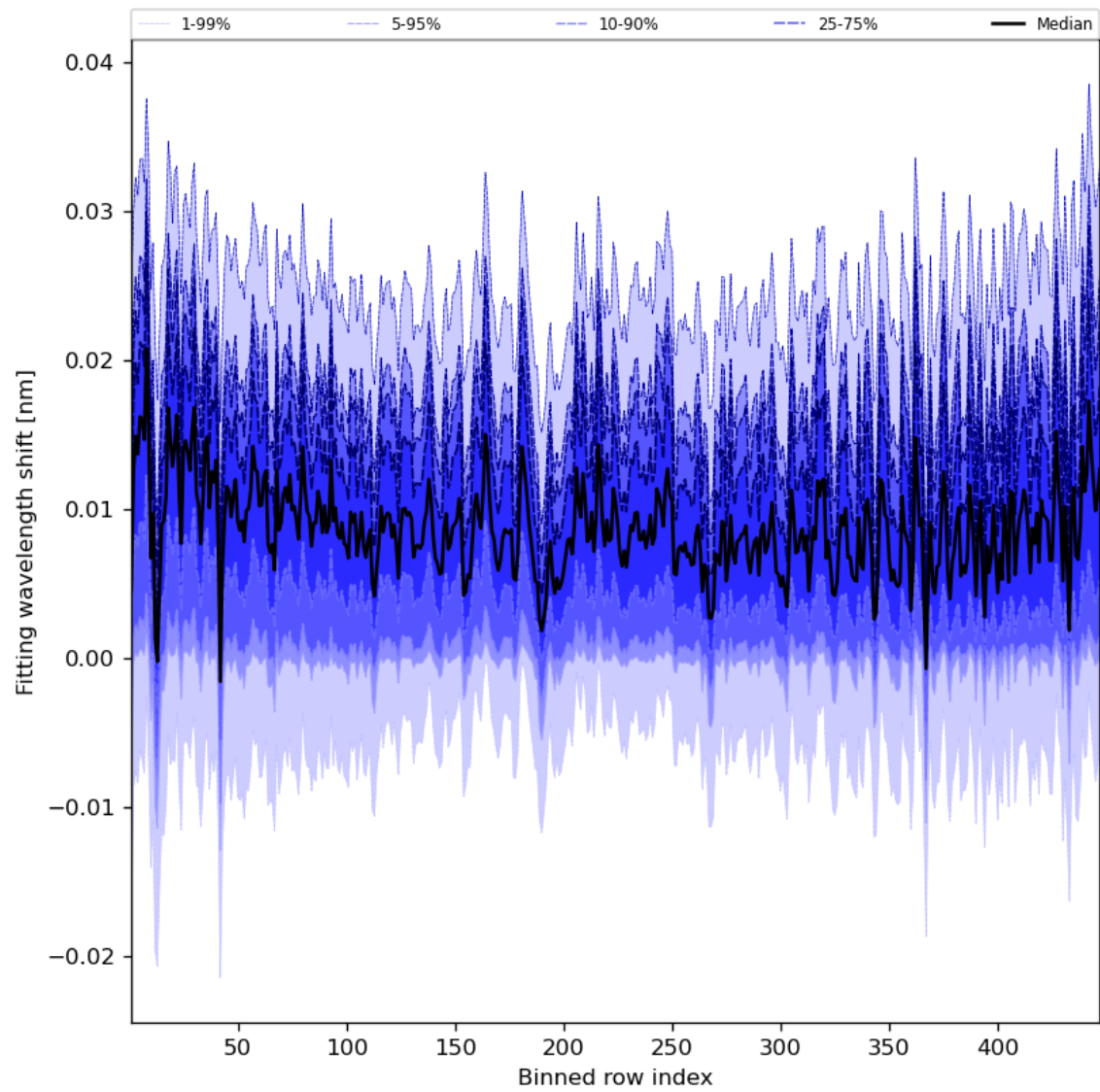
Figure 65: Along track statistics of “Fitting wavelength shift” for 2023-09-20 to 2023-09-21
