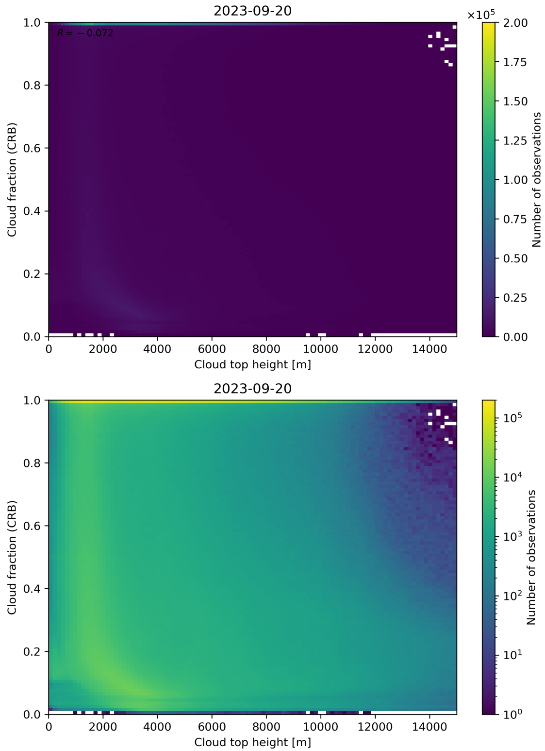
Figure 88: Scatter density plot of “Cloud top height” against “Cloud fraction (CRB)” for 2023-09-20 to 2023-09-21.
