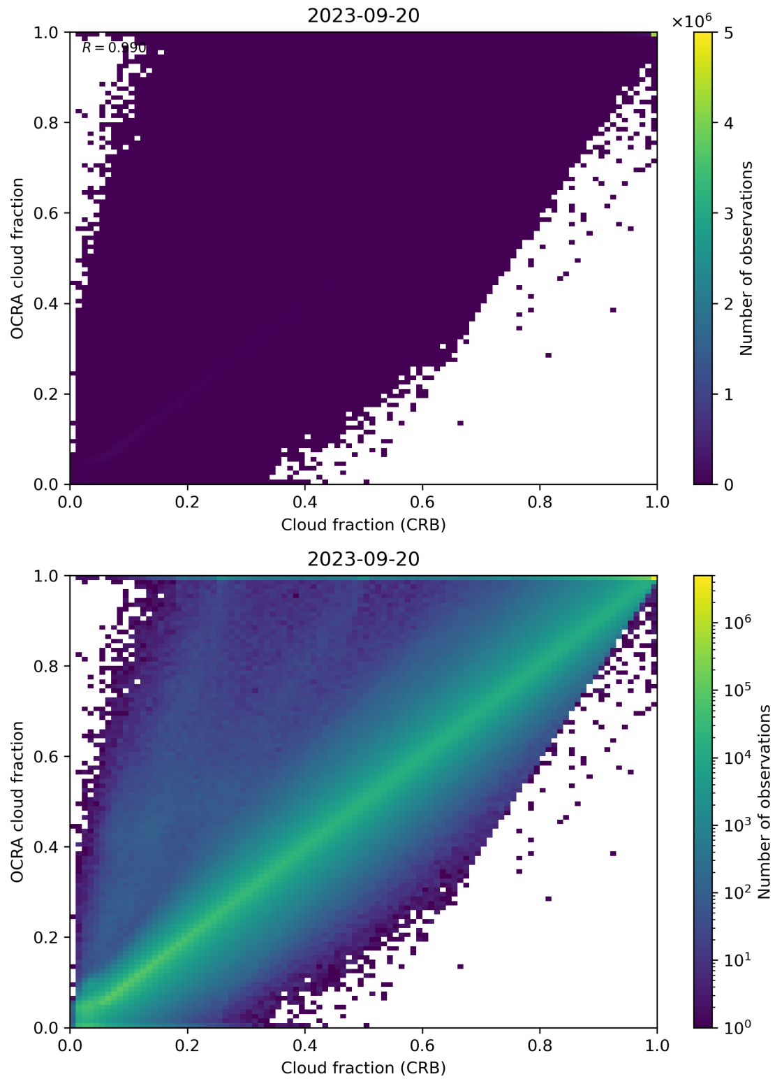
Figure 78: Scatter density plot of “Cloud fraction (CRB)” against “OCRA cloud fraction” for 2023-09-20 to 2023-09-21.
