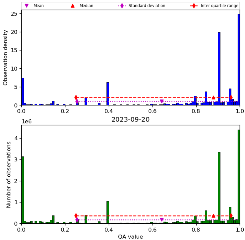
Figure 38: Histogram of “QA value” for 2023-09-20 to 2023-09-21
