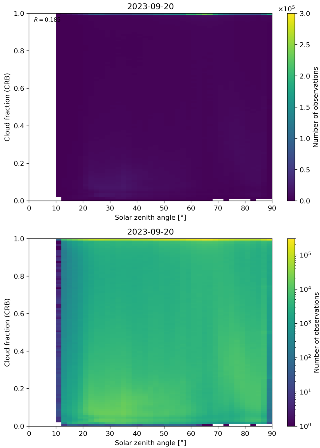
Figure 101: Scatter density plot of “Solar zenith angle” against “Cloud fraction (CRB)” for 2023-09-20 to 2023-09-21.
