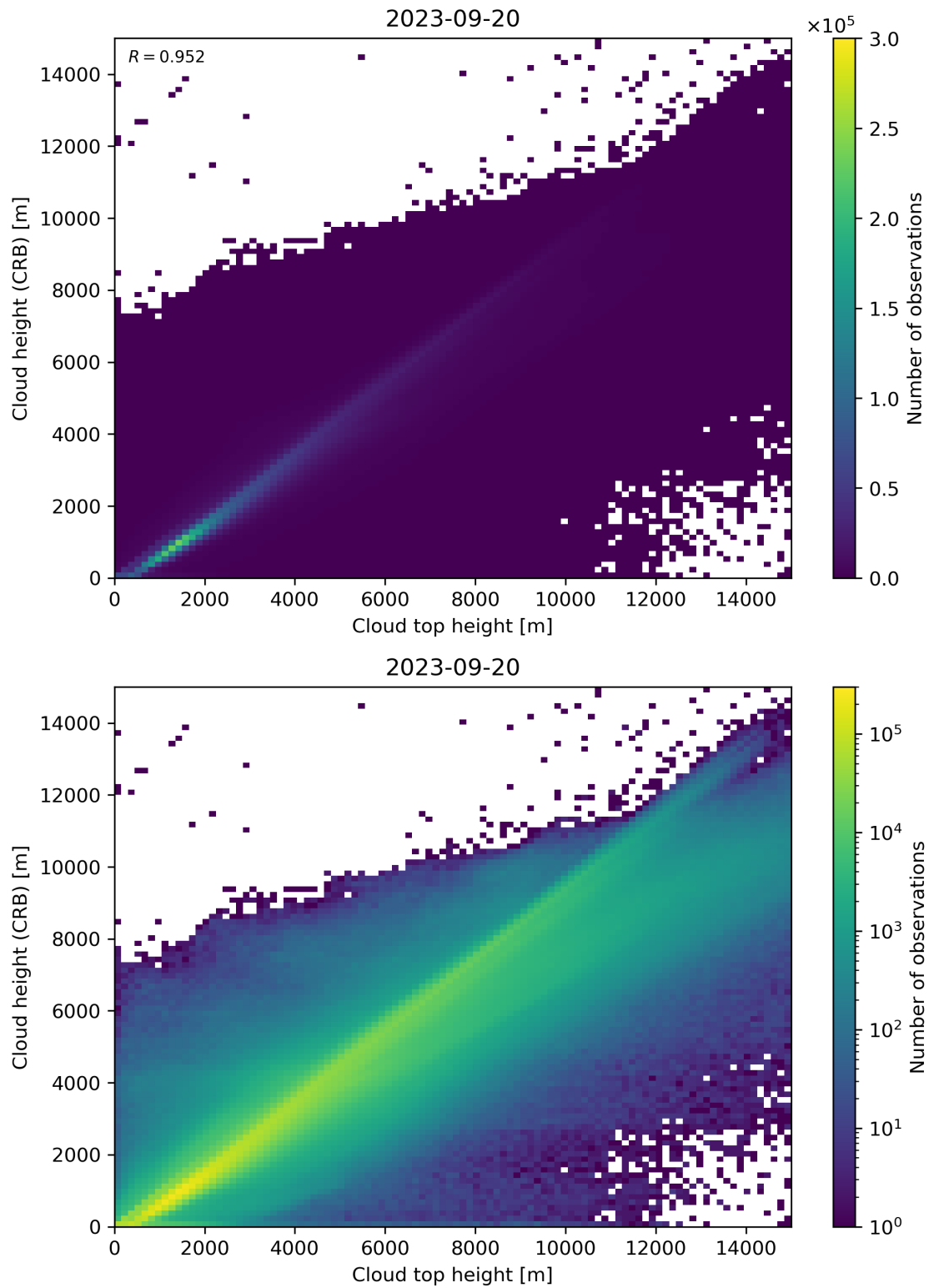
Figure 89: Scatter density plot of “Cloud top height” against “Cloud height (CRB)” for 2023-09-20 to 2023-09-21.
