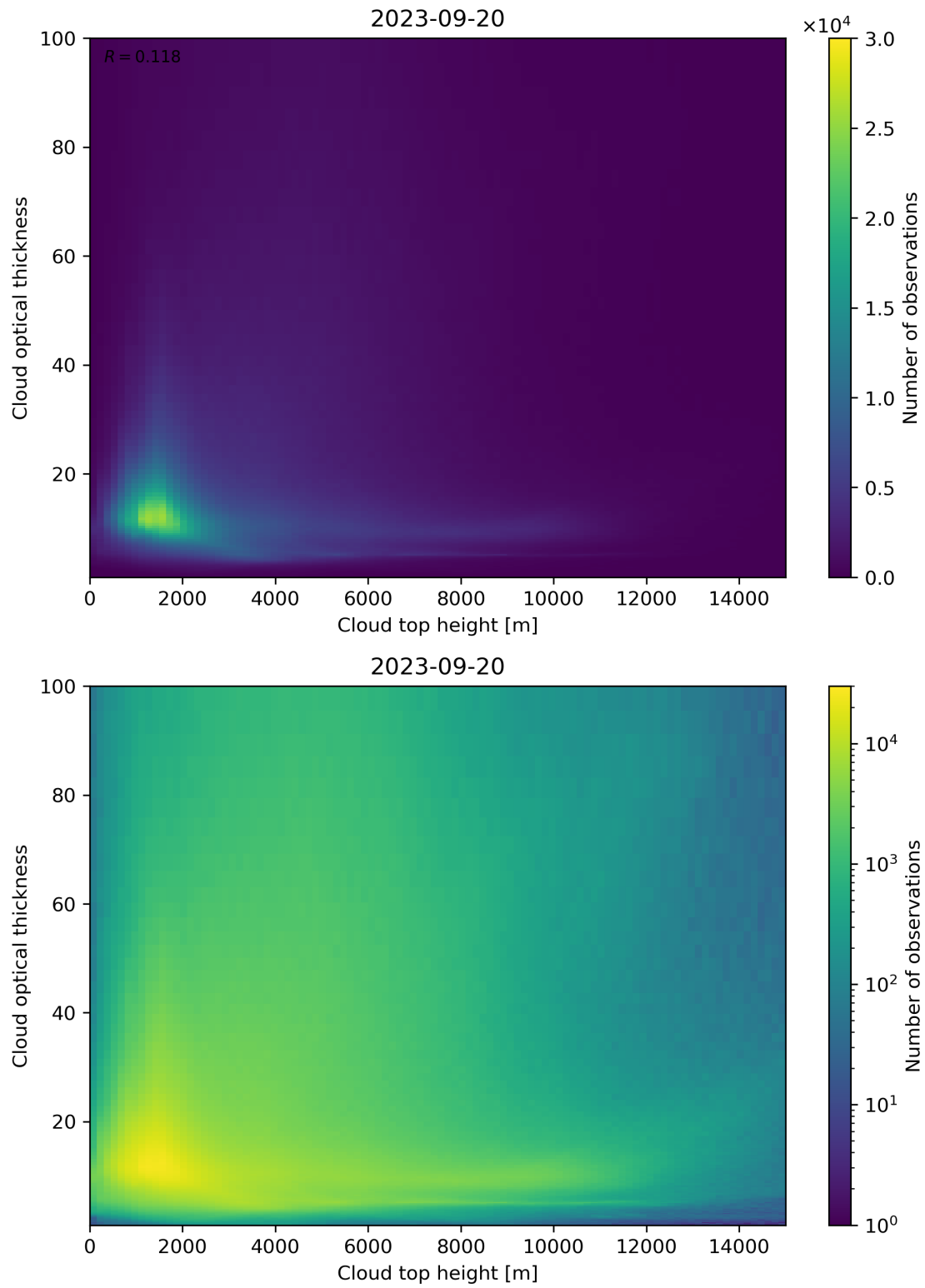
Figure 90: Scatter density plot of “Cloud top height” against “Cloud optical thickness” for 2023-09-20 to 2023-09-21.
