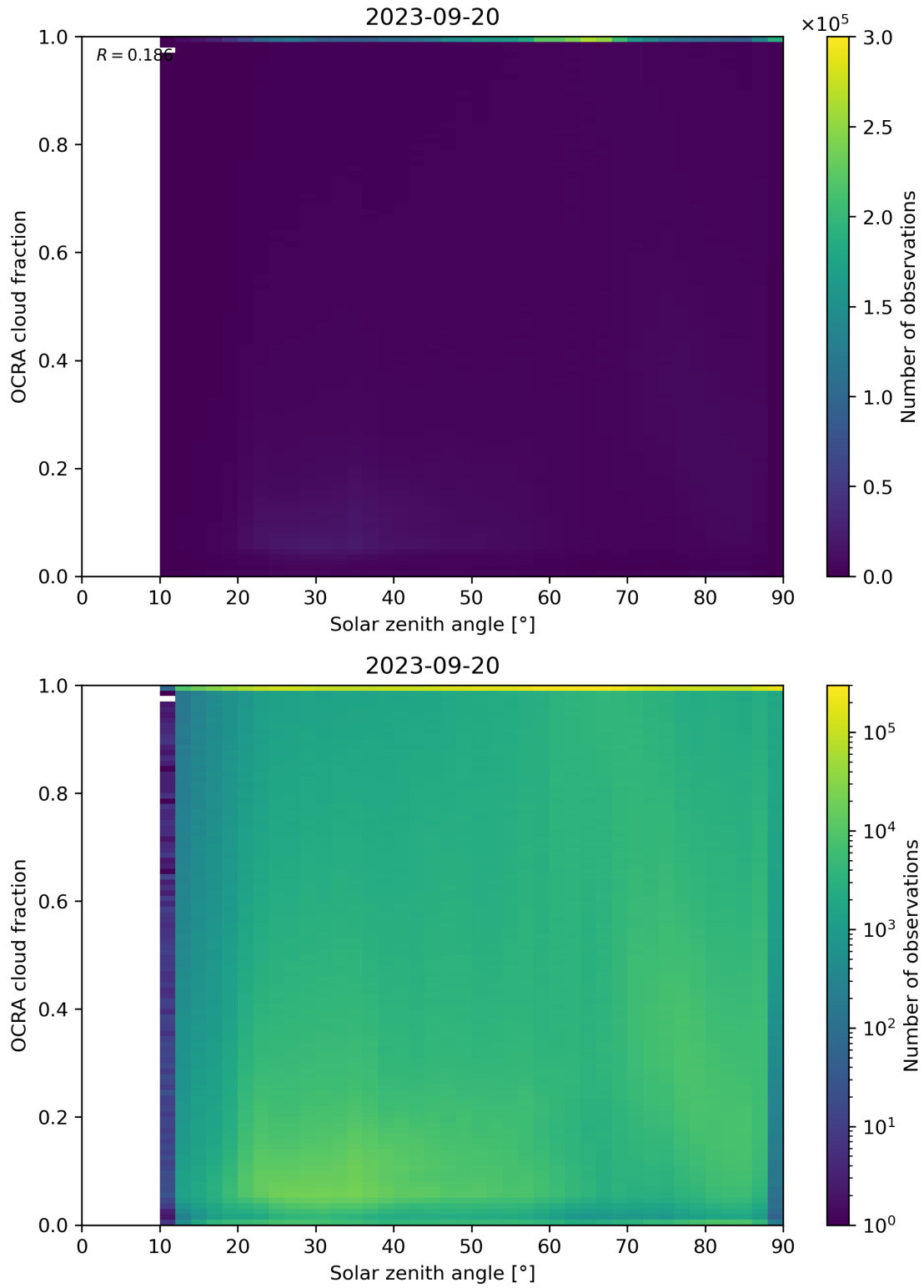
Figure 100: Scatter density plot of “Solar zenith angle” against “OCRA cloud fraction” for 2023-09-20 to 2023-09-21.
