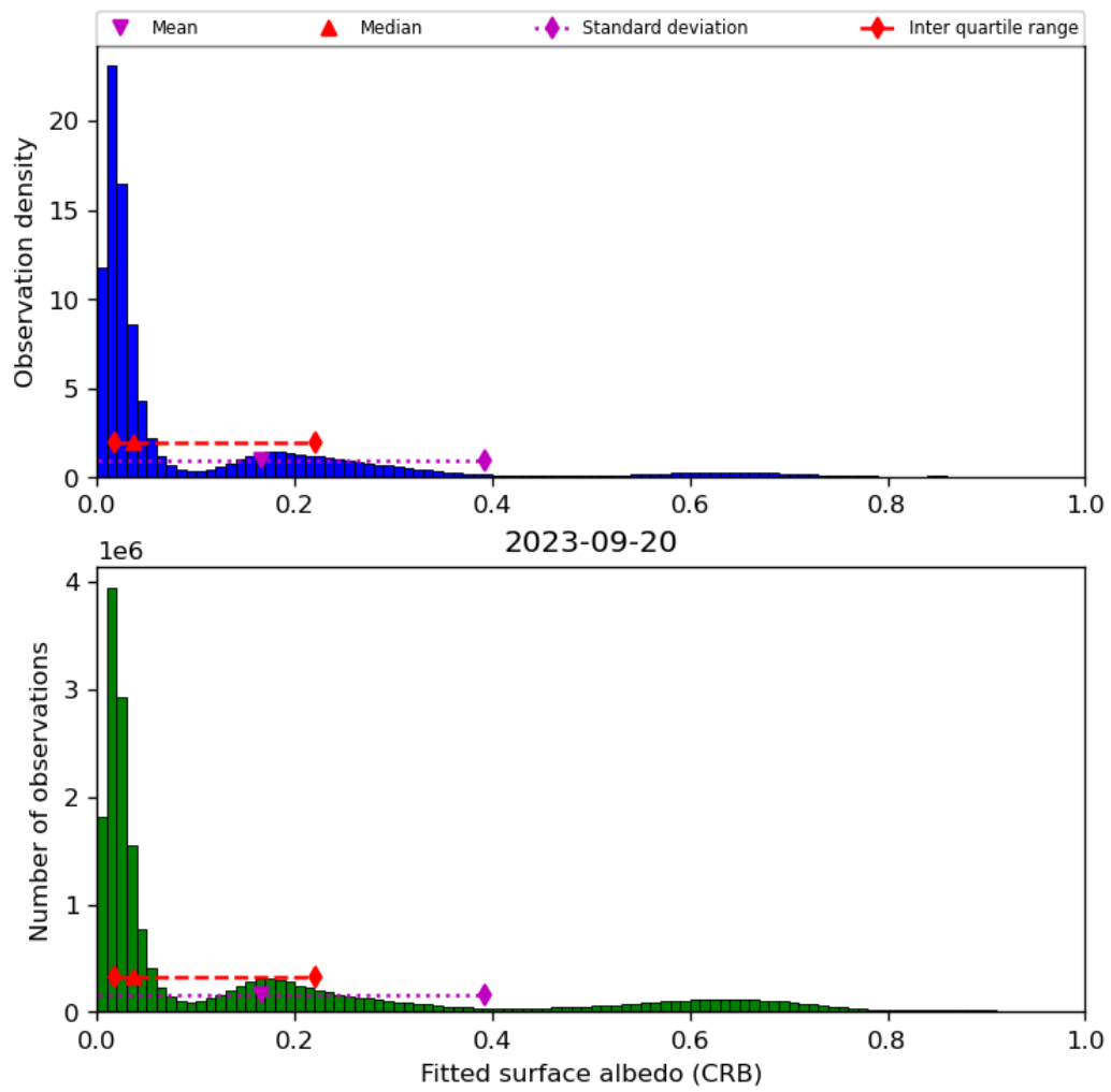
Figure 46: Histogram of “Fitted surface albedo (CRB)” for 2023-09-20 to 2023-09-21
