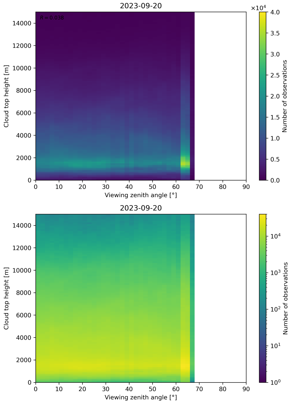
Figure 112: Scatter density plot of “Viewing zenith angle” against “Cloud top height” for 2023-09-20 to 2023-09-21.
