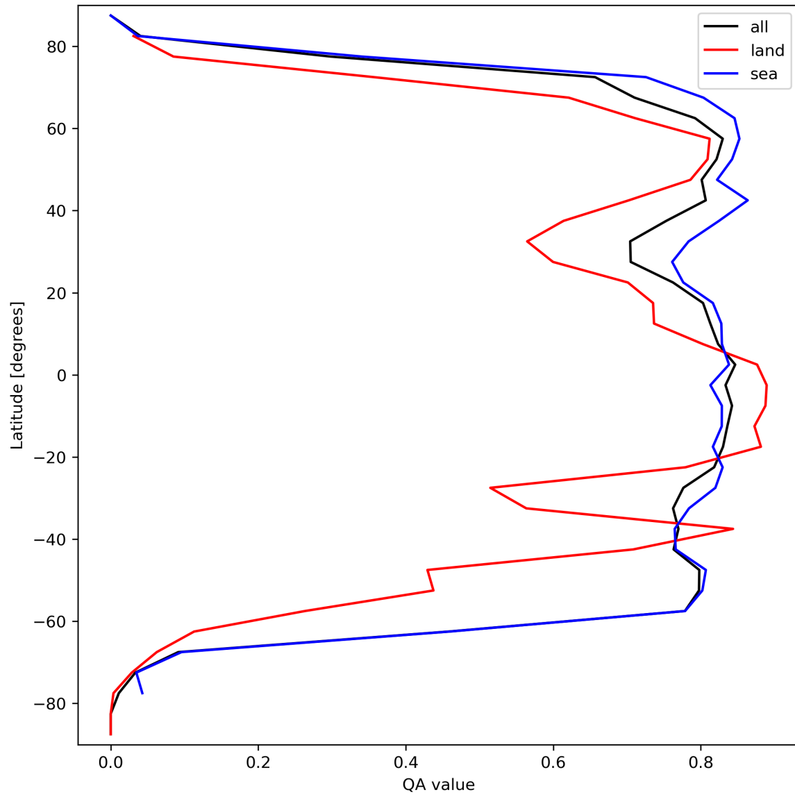
Figure 22: Zonal average of “QA value” for 2023-09-20 to 2023-09-21.
