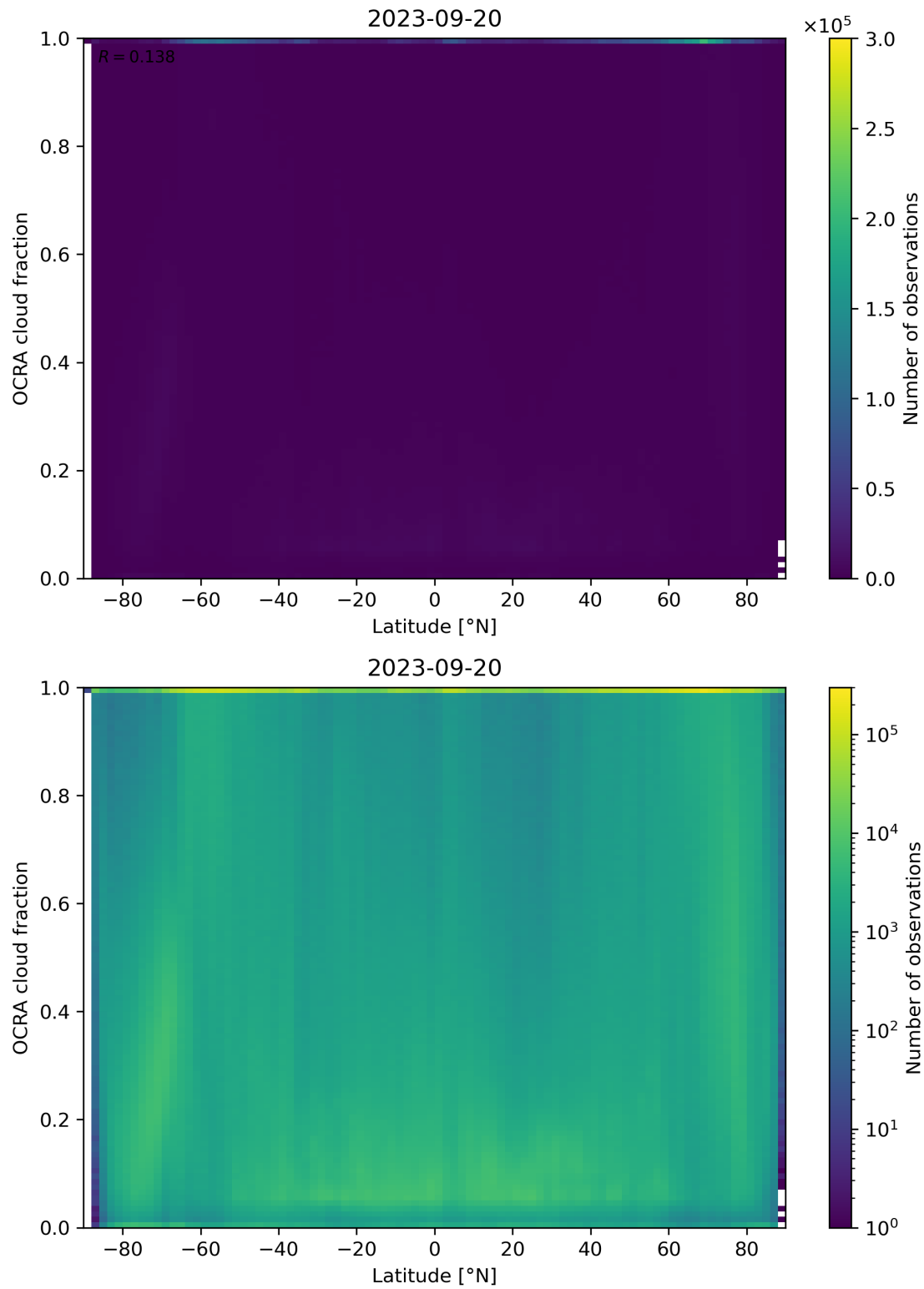
Figure 93: Scatter density plot of “Latitude” against “OCRA cloud fraction” for 2023-09-20 to 2023-09-21.
