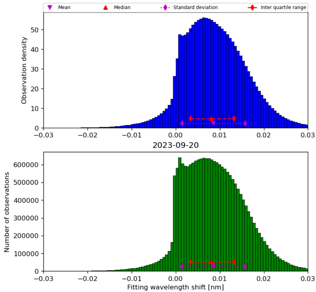
Figure 49: Histogram of “Fitting wavelength shift” for 2023-09-20 to 2023-09-21
