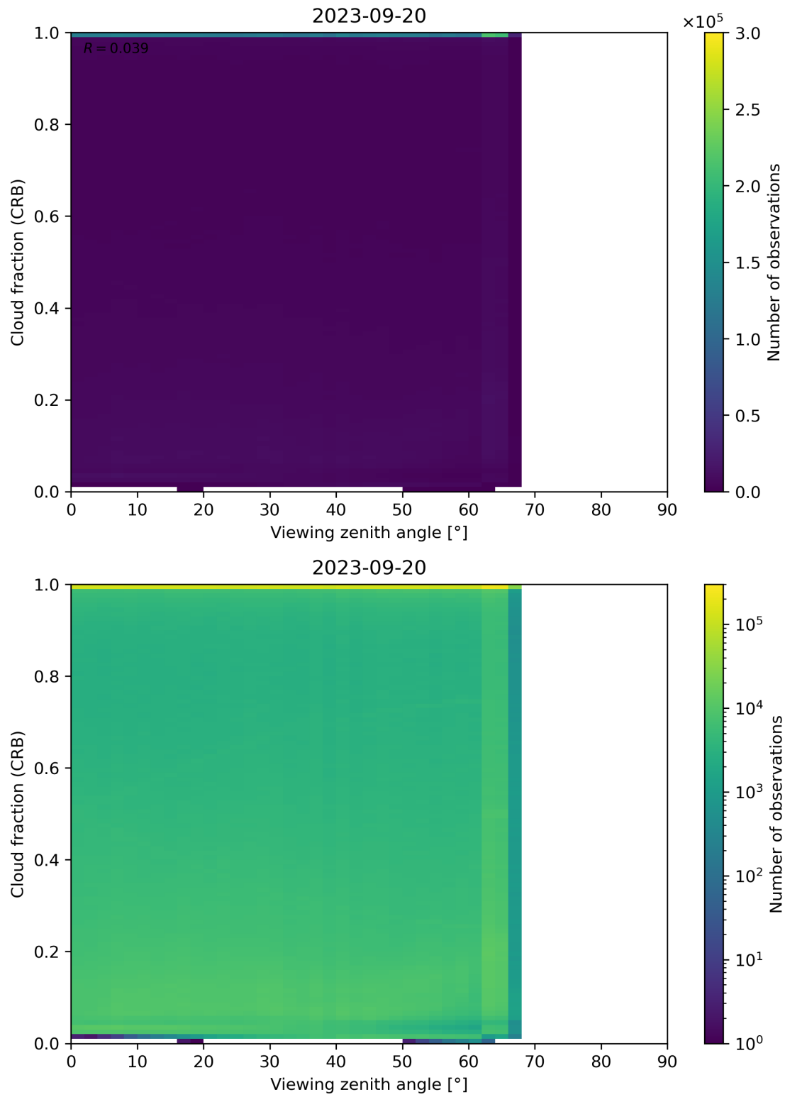
Figure 109: Scatter density plot of “Viewing zenith angle” against “Cloud fraction (CRB)” for 2023-09-20 to 2023-09-21.
