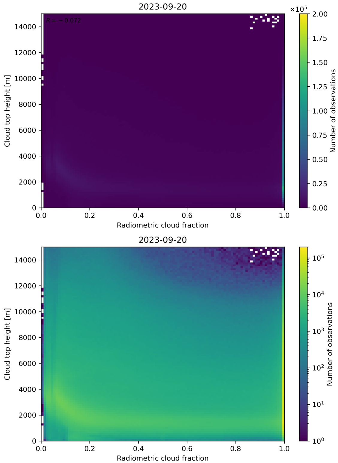
Figure 76: Scatter density plot of “Radiometric cloud fraction” against “Cloud top height” for 2023-09-20 to 2023-09-21.
