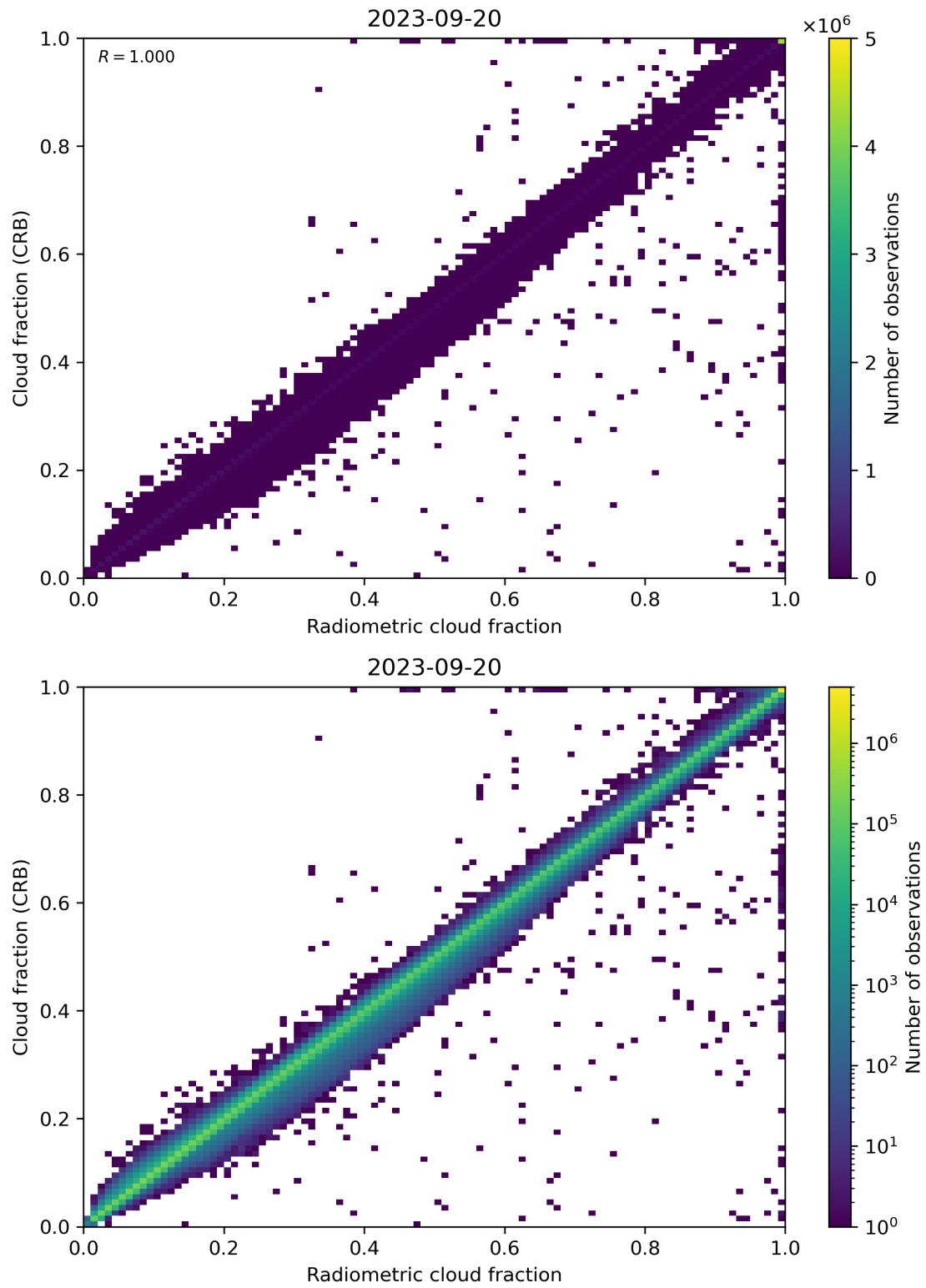
Figure 73: Scatter density plot of “Radiometric cloud fraction” against “Cloud fraction (CRB)” for 2023-09-20 to 2023-09-21.
