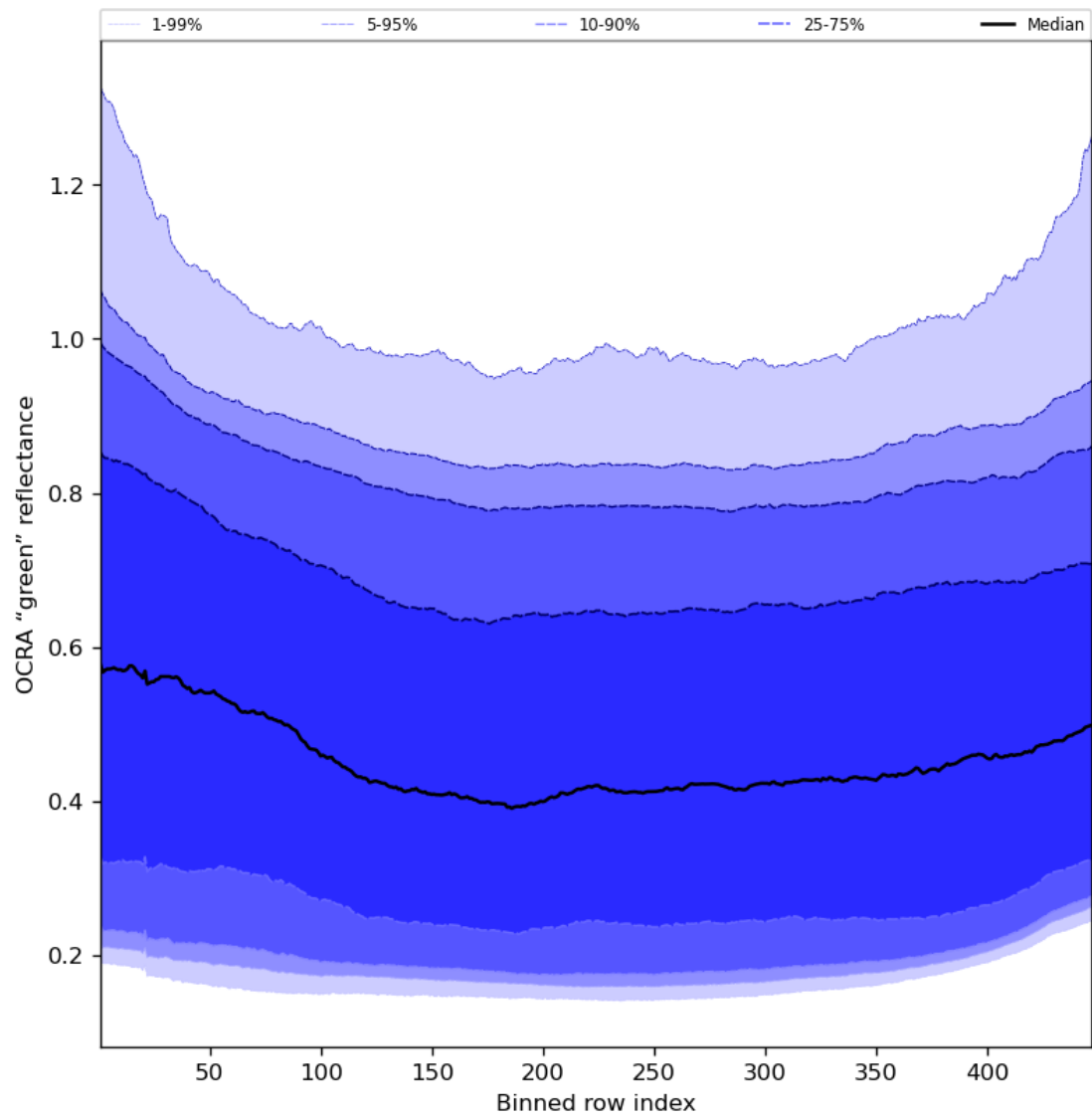
Figure 68: Along track statistics of "OCRA "green" reflectance" for 2023-09-20 to 2023-09-21
