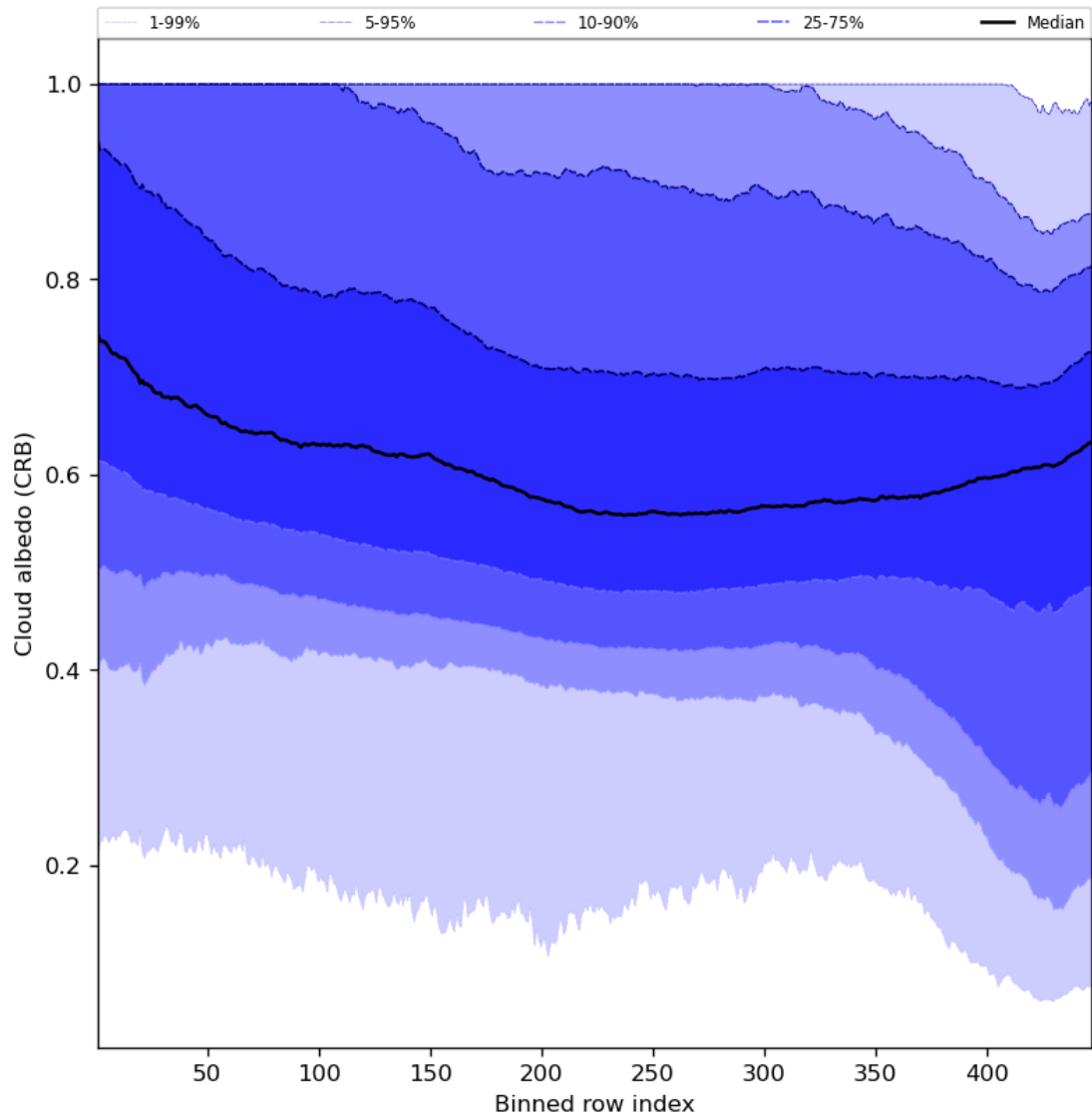
Figure 60: Along track statistics of “Cloud albedo (CRB)” for 2023-09-20 to 2023-09-21
