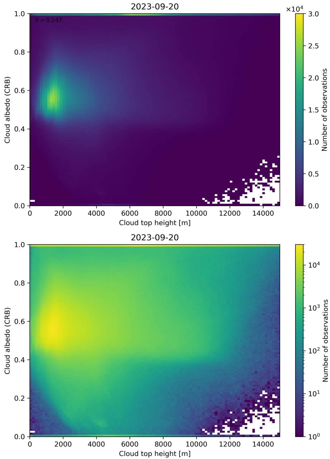
Figure 86: Scatter density plot of “Cloud top height” against “Cloud albedo (CRB)” for 2023-09-20 to 2023-09-21.
