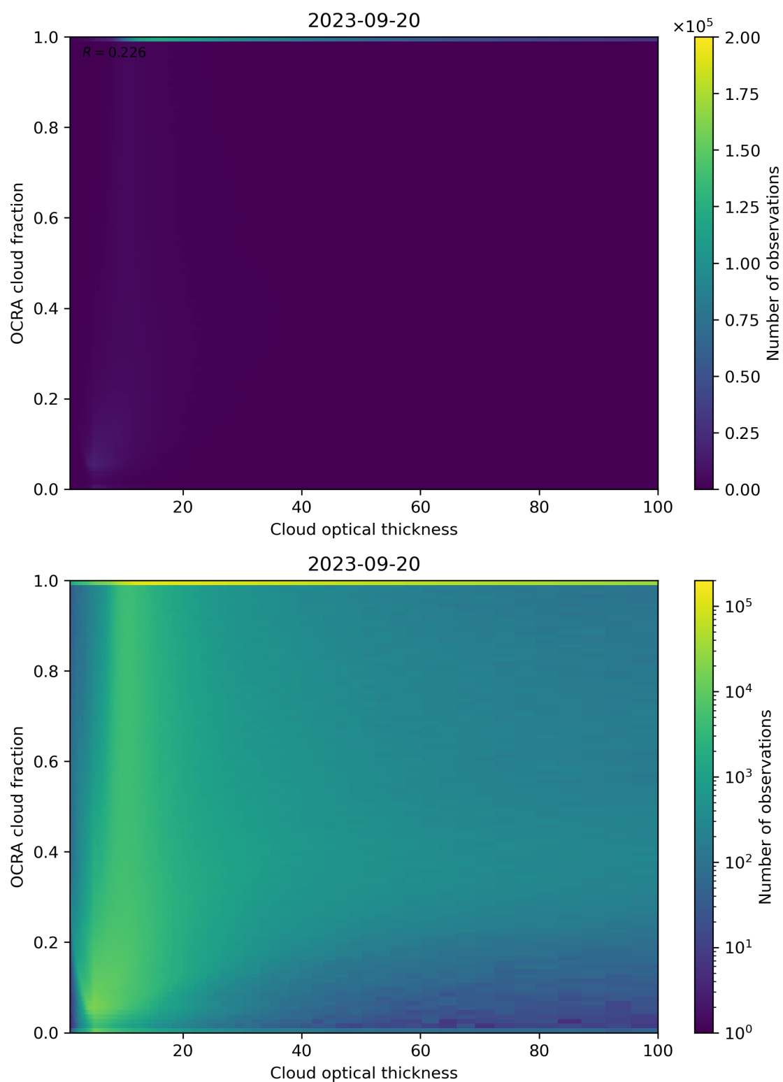
Figure 83: Scatter density plot of “Cloud optical thickness” against “OCRA cloud fraction” for 2023-09-20 to 2023-09-21.
