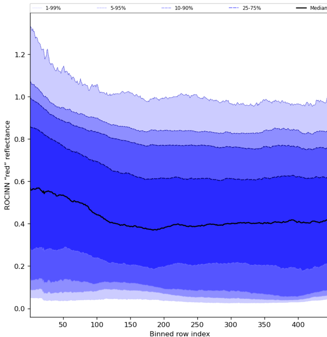
Figure 69: Along track statistics of “ROCINN “red” reflectance” for 2023-09-20 to 2023-09-21
