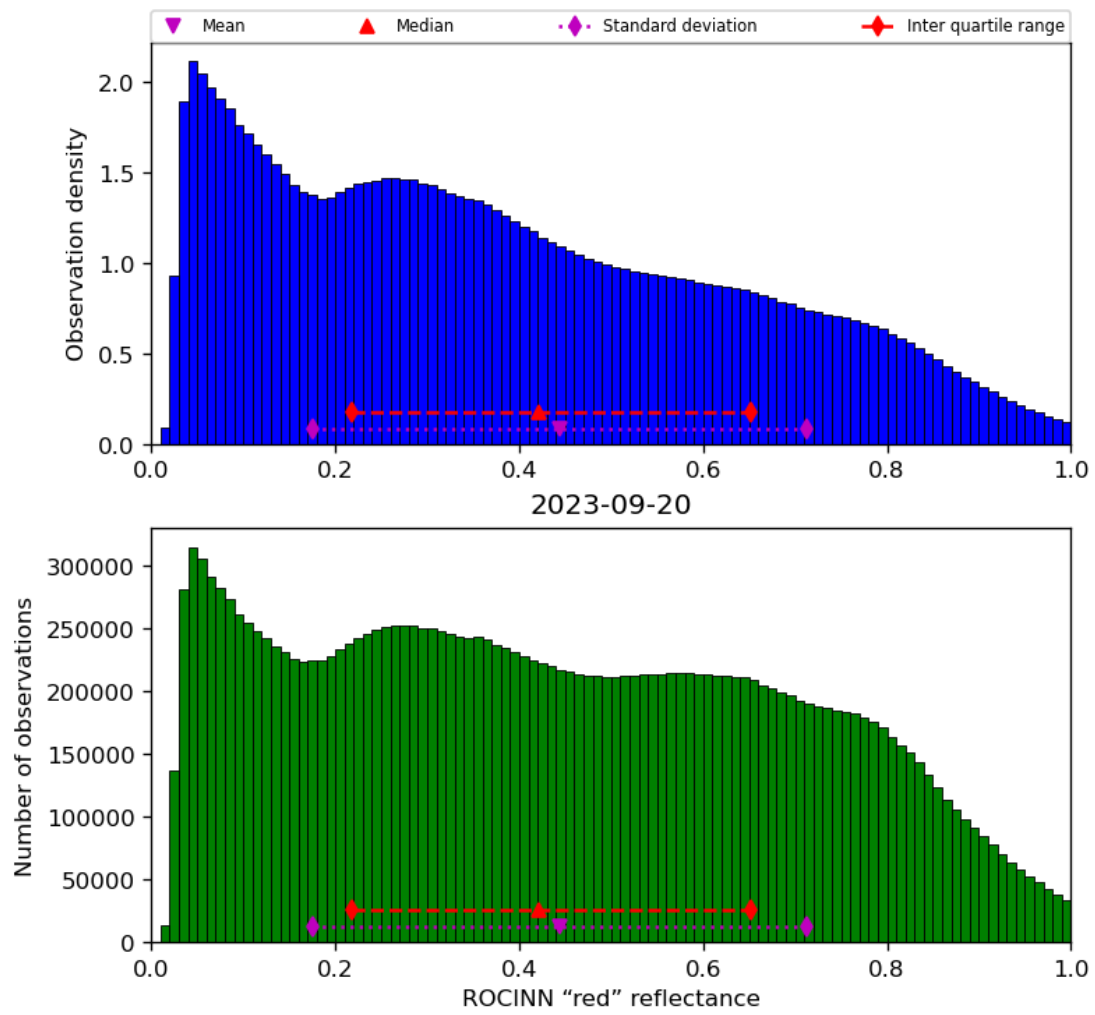
Figure 53: Histogram of “ROCINN “red” reflectance” for 2023-09-20 to 2023-09-21
