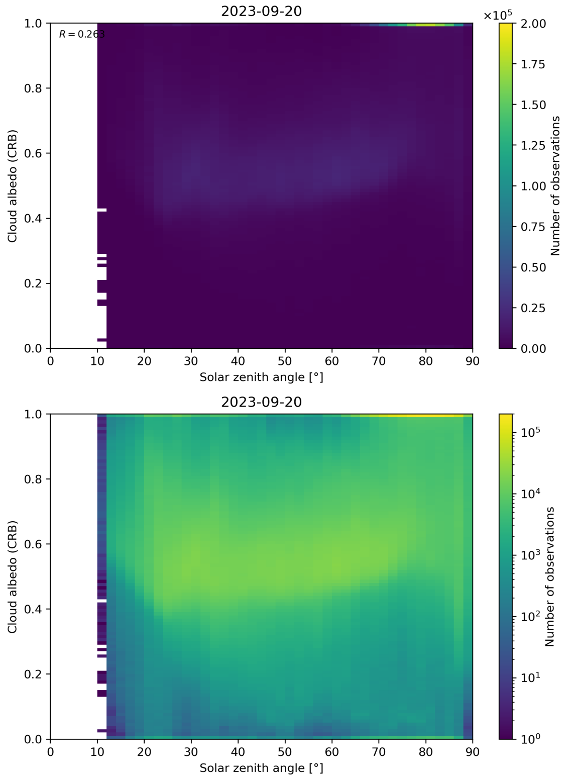
Figure 98: Scatter density plot of “Solar zenith angle” against “Cloud albedo (CRB)” for 2023-09-20 to 2023-09-21.
