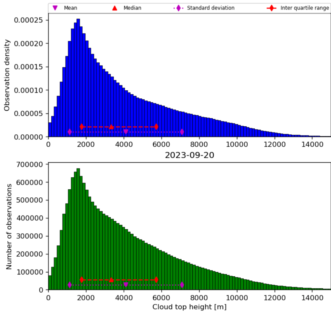
Figure 40: Histogram of “Cloud top height” for 2023-09-20 to 2023-09-21
