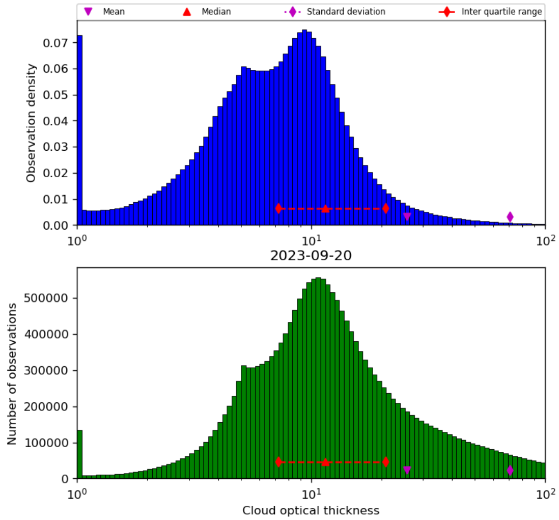
Figure 41: Histogram of “Cloud optical thickness” for 2023-09-20 to 2023-09-21
