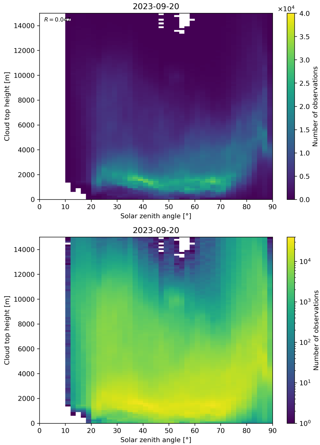
Figure 104: Scatter density plot of “Solar zenith angle” against “Cloud top height” for 2023-09-20 to 2023-09-21.
