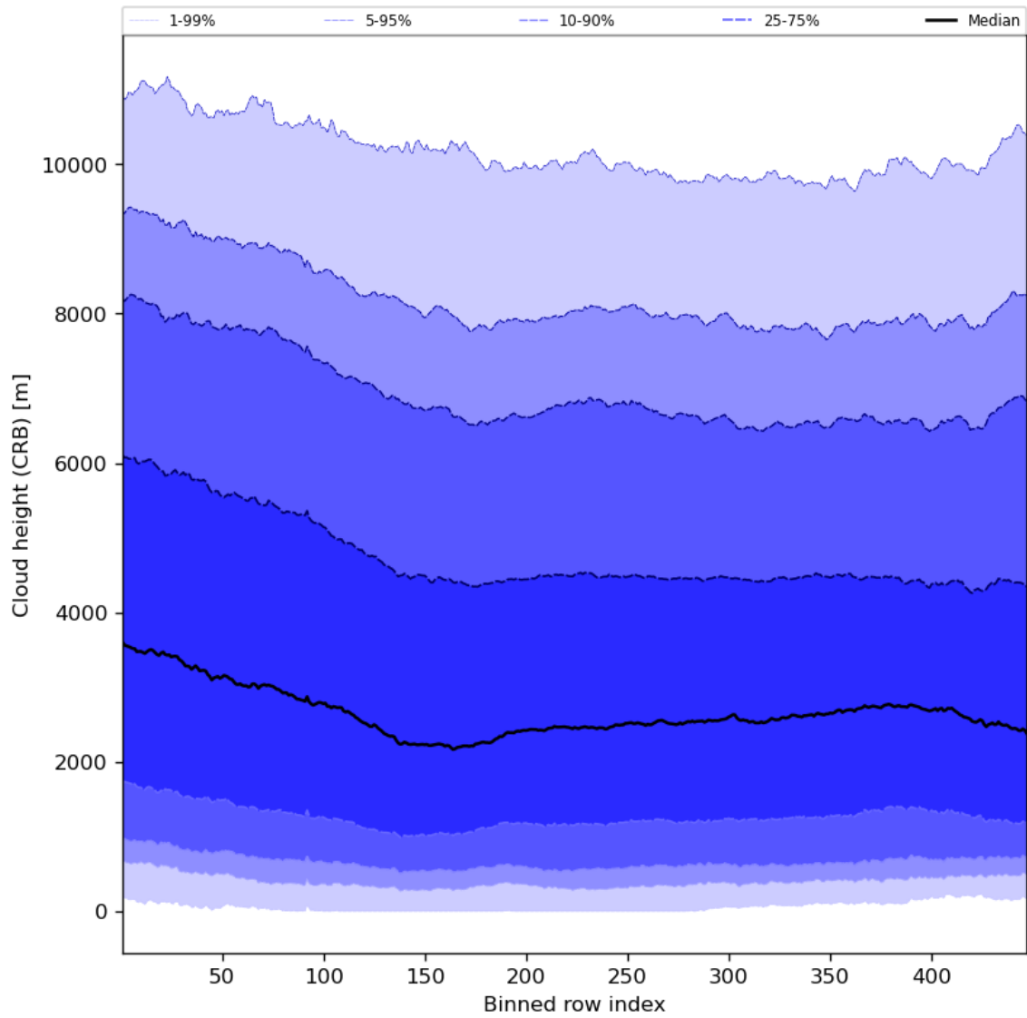
Figure 59: Along track statistics of “Cloud height (CRB)” for 2023-09-20 to 2023-09-21
