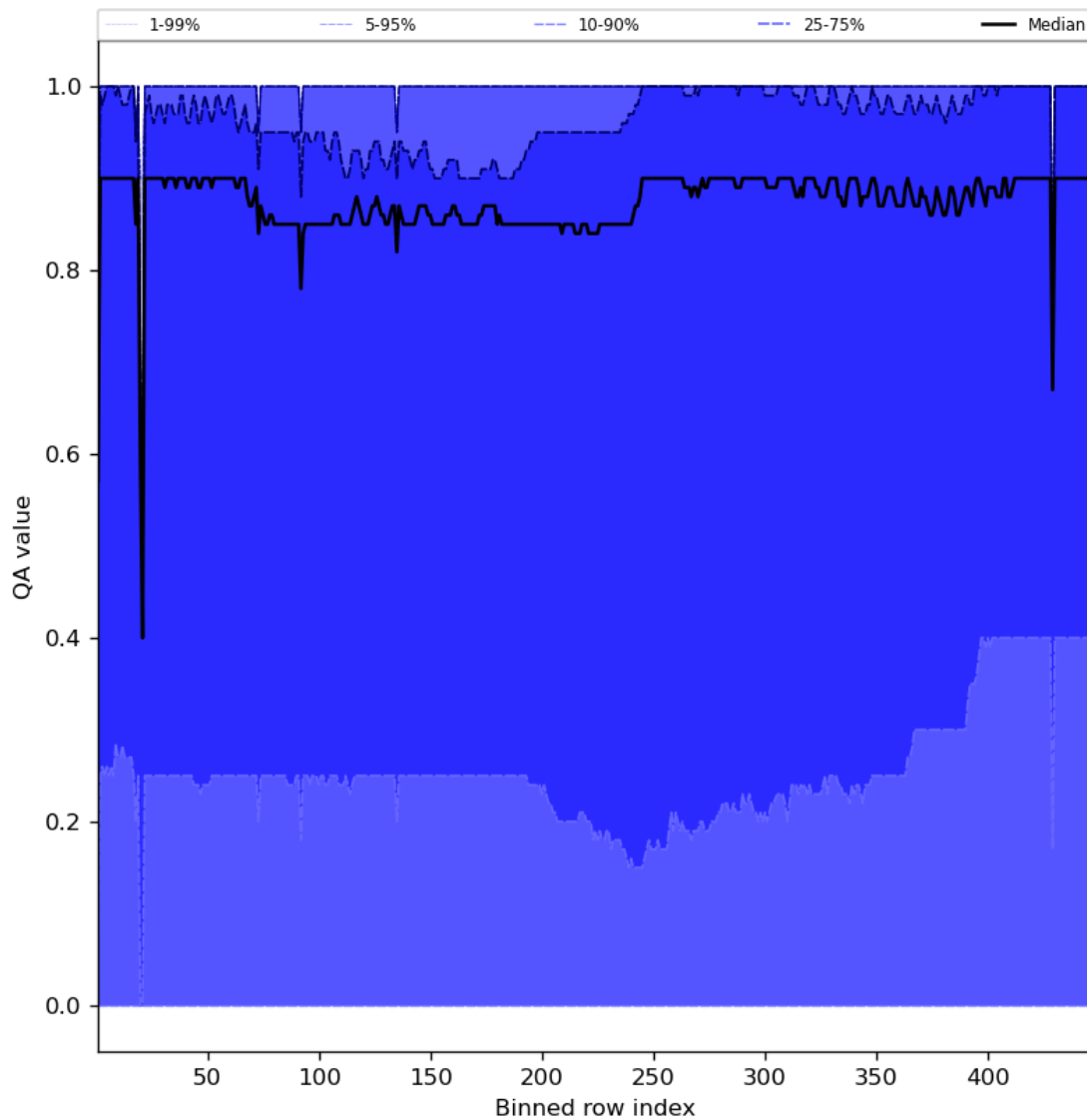
Figure 54: Along track statistics of “QA value” for 2023-09-20 to 2023-09-21
