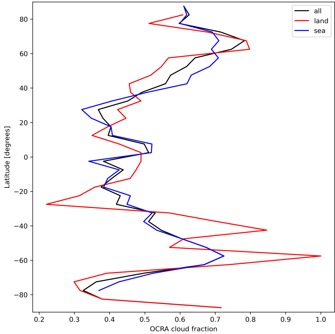
Figure 34: Zonal average of “OCRA cloud fraction” for 2023-09-20 to 2023-09-21.
