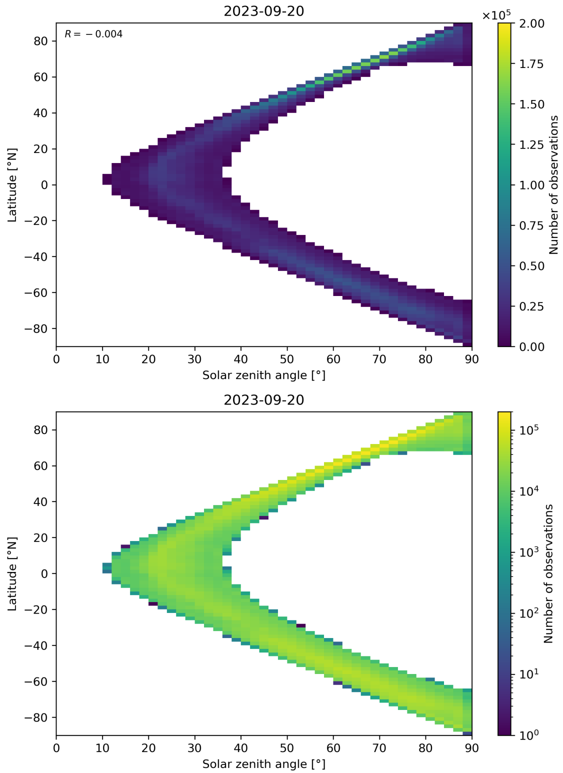
Figure 105: Scatter density plot of “Solar zenith angle” against “Latitude” for 2023-09-20 to 2023-09-21.
