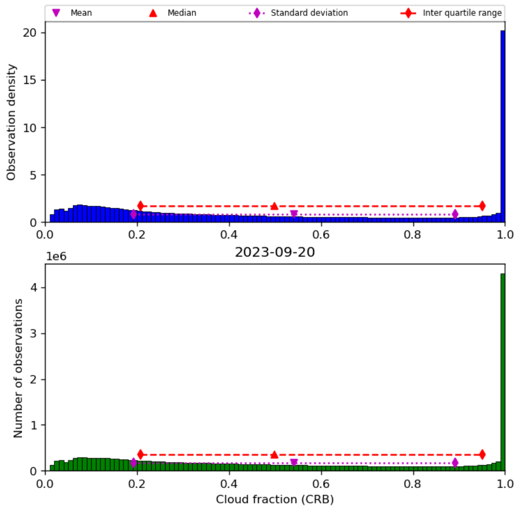
Figure 42: Histogram of “Cloud fraction (CRB)” for 2023-09-20 to 2023-09-21
