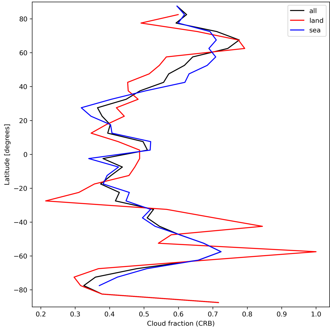
Figure 26: Zonal average of “Cloud fraction (CRB)” for 2023-09-20 to 2023-09-21.
