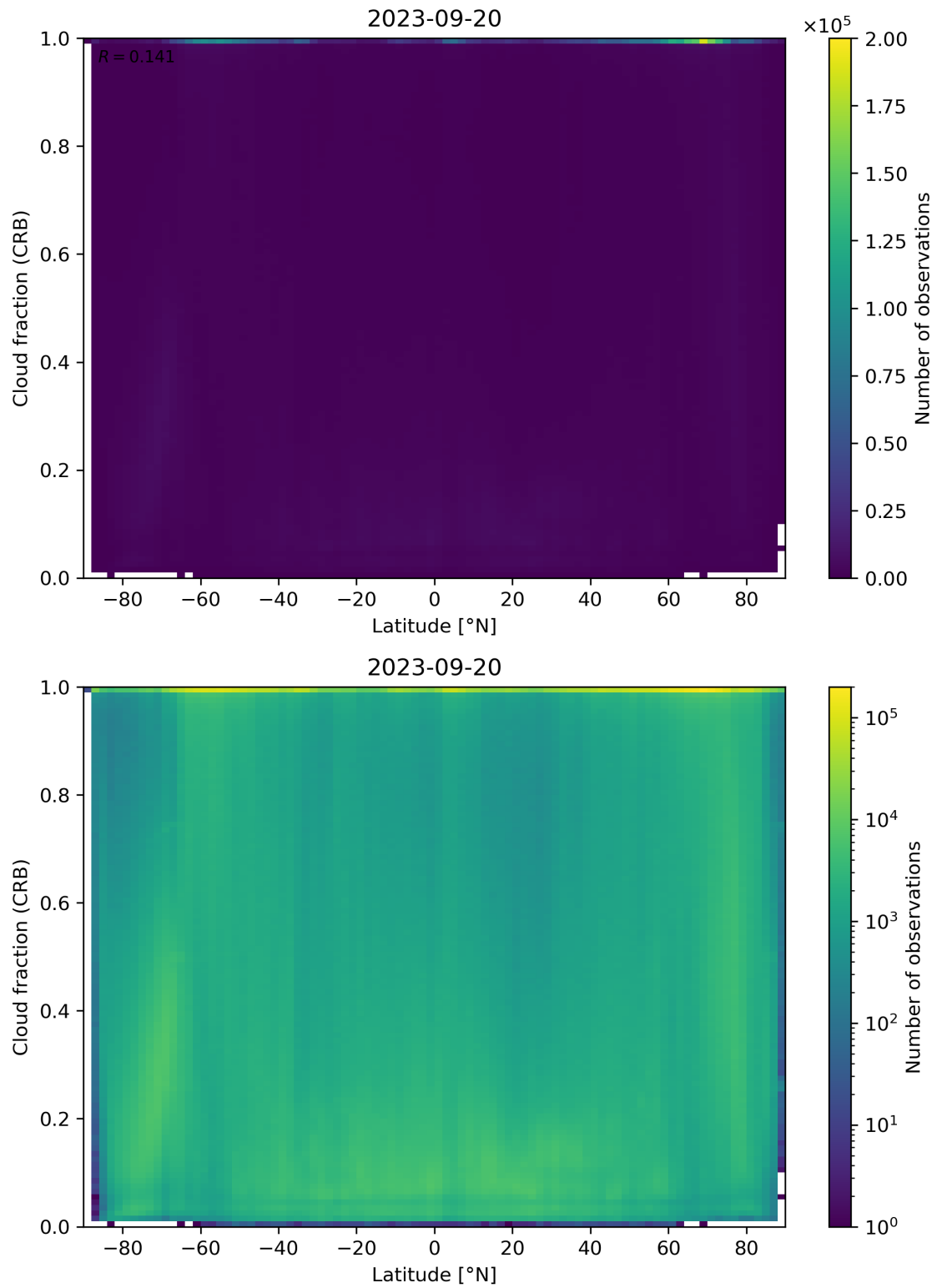
Figure 94: Scatter density plot of “Latitude” against “Cloud fraction (CRB)” for 2023-09-20 to 2023-09-21.
