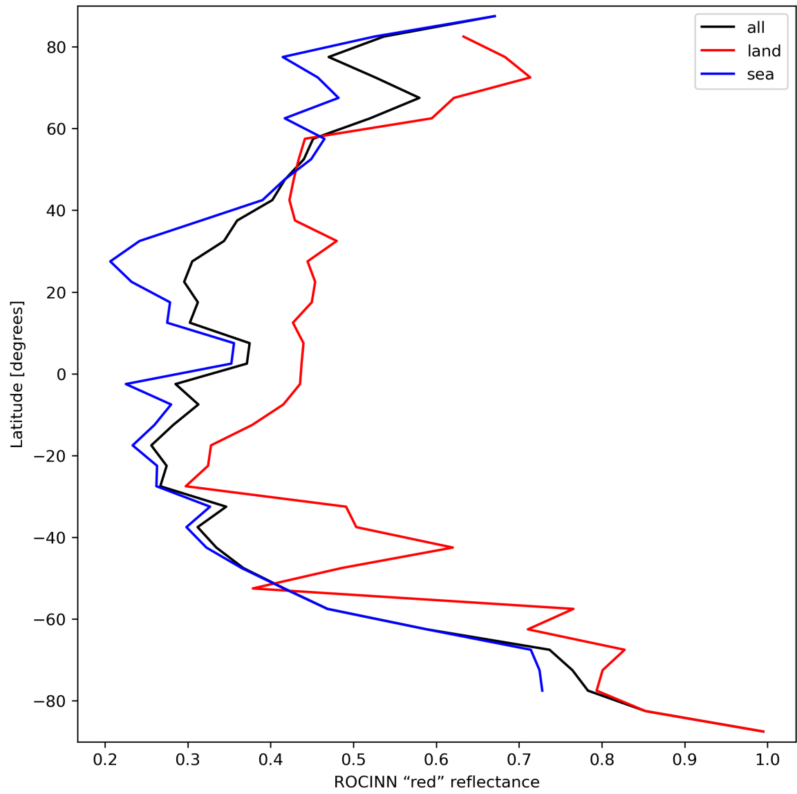
Figure 37: Zonal average of “ROCINN “red” reflectance” for 2023-09-20 to 2023-09-21.
