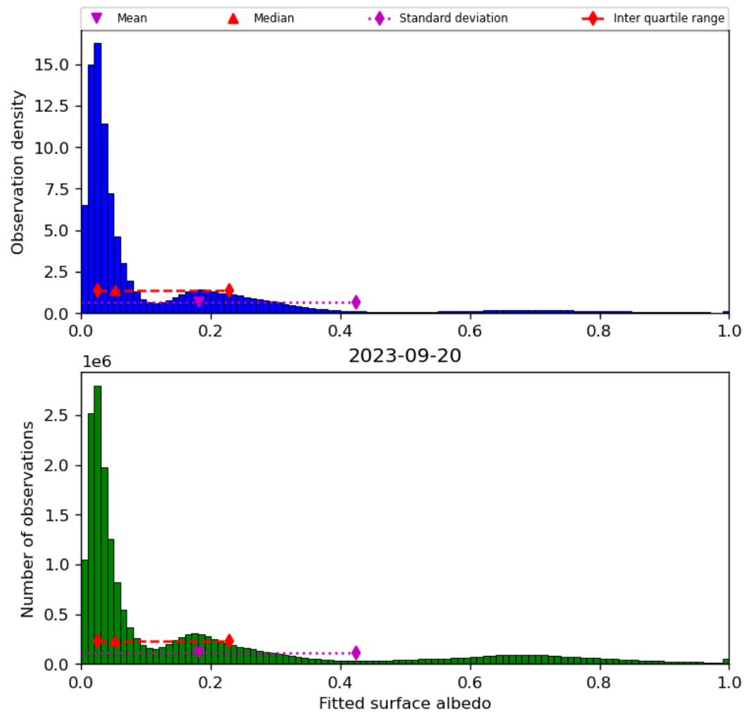
Figure 45: Histogram of “Fitted surface albedo” for 2023-09-20 to 2023-09-21
