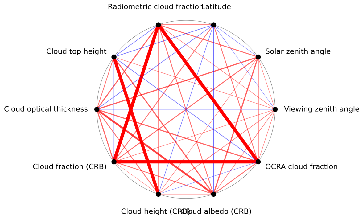
Figure 1: Map of correlation graph for 2023-09-20 to 2023-09-21.
