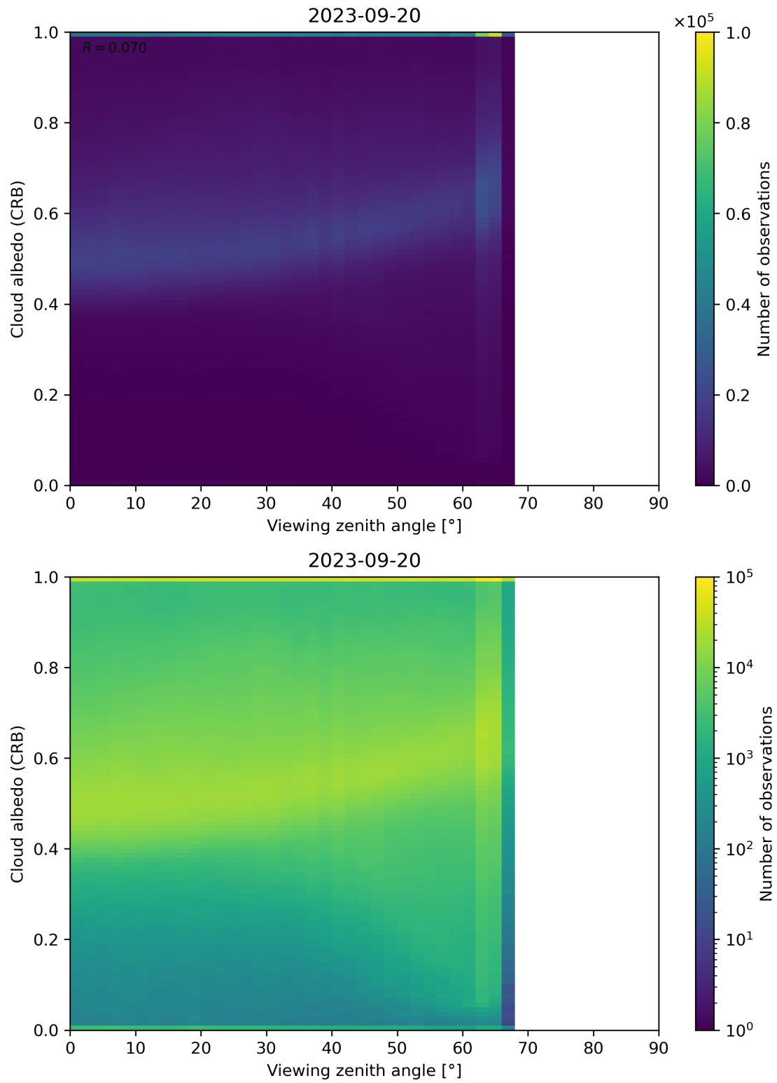
Figure 106: Scatter density plot of “Viewing zenith angle” against “Cloud albedo (CRB)” for 2023-09-20 to 2023-09-21.
