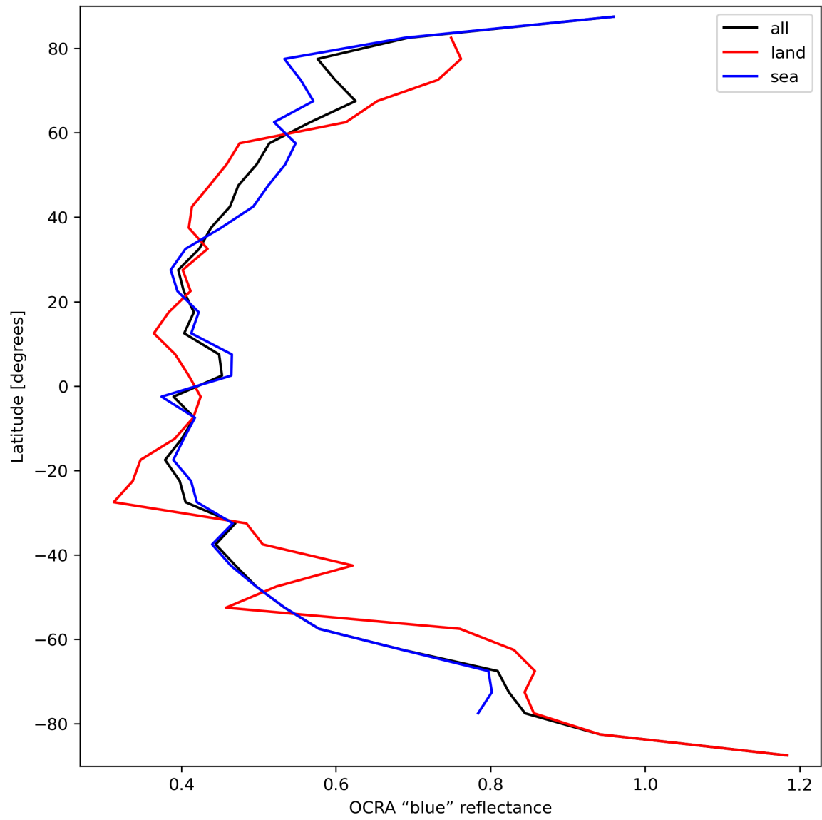
Figure 35: Zonal average of “OCRA “blue” reflectance” for 2023-09-20 to 2023-09-21.
