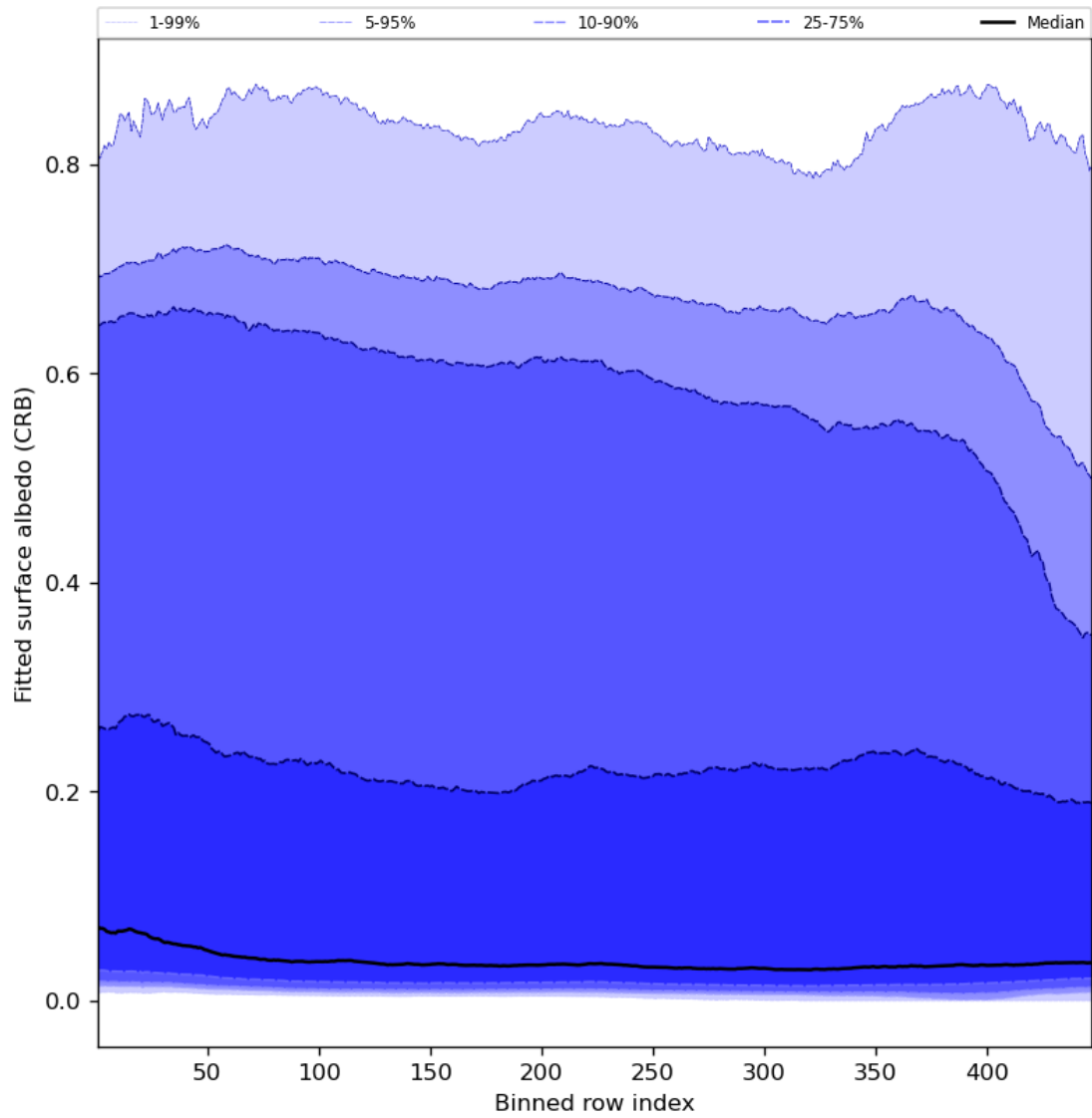
Figure 62: Along track statistics of “Fitted surface albedo (CRB)” for 2023-09-20 to 2023-09-21
