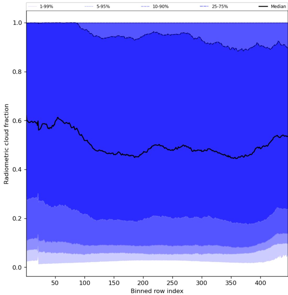
Figure 55: Along track statistics of “Radiometric cloud fraction” for 2023-09-20 to 2023-09-21
