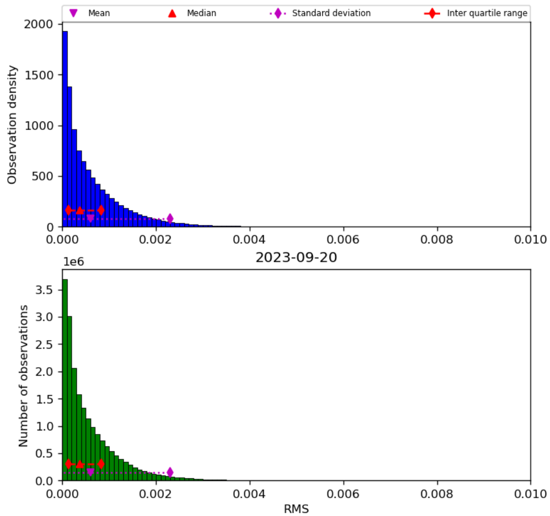
Figure 47: Histogram of “RMS” for 2023-09-20 to 2023-09-21
