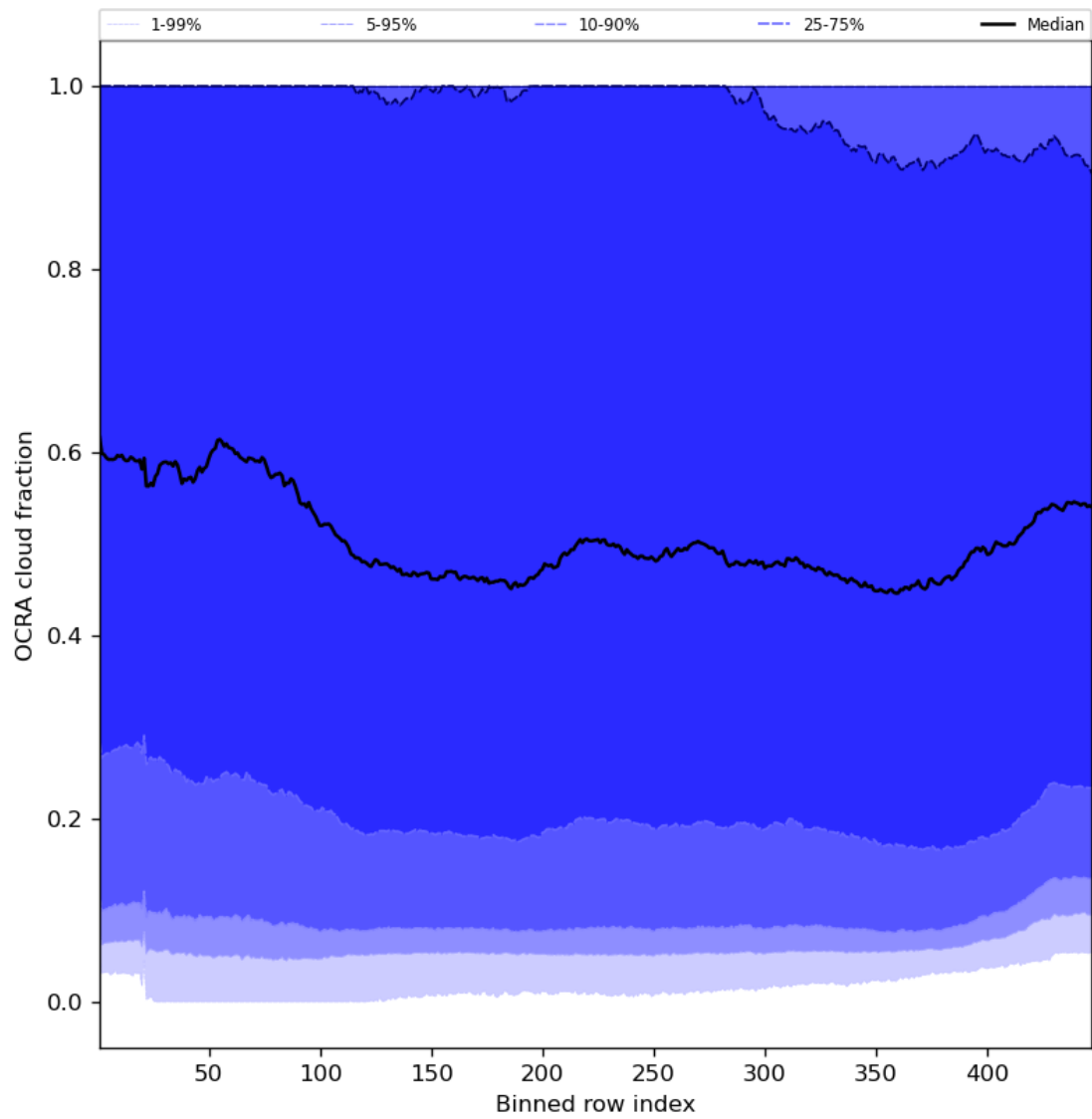
Figure 66: Along track statistics of “OCRA cloud fraction” for 2023-09-20 to 2023-09-21
