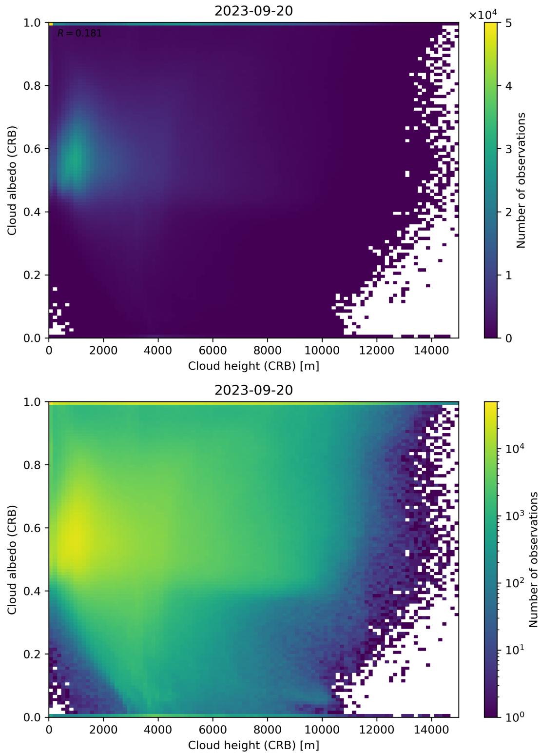
Figure 80: Scatter density plot of “Cloud height (CRB)” against “Cloud albedo (CRB)” for 2023-09-20 to 2023-09-21.
