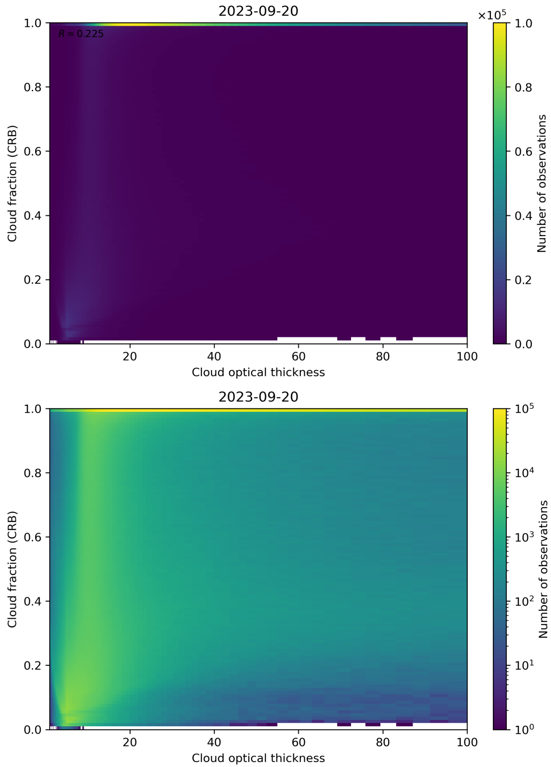
Figure 84: Scatter density plot of “Cloud optical thickness” against “Cloud fraction (CRB)” for 2023-09-20 to 2023-09-21.
