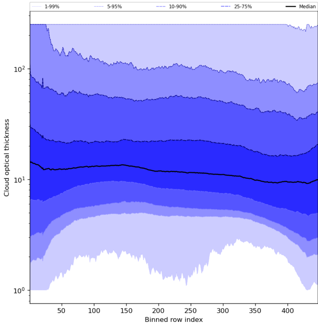
Figure 57: Along track statistics of “Cloud optical thickness” for 2023-09-20 to 2023-09-21
