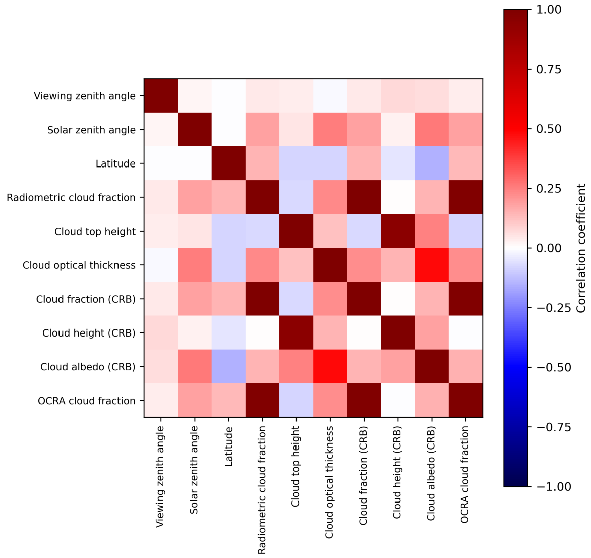
Figure 2: Map of correlation matrix for 2023-09-20 to 2023-09-21.
