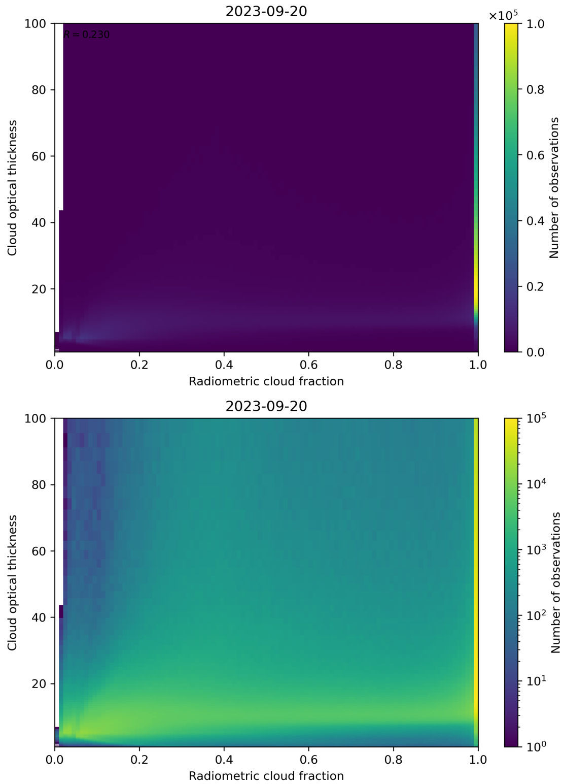
Figure 75: Scatter density plot of “Radiometric cloud fraction” against “Cloud optical thickness” for 2023-09-20 to 2023-09-21.
