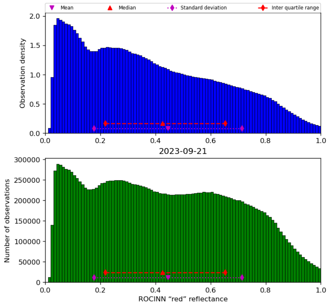
Figure 53: Histogram of “ROCINN “red” reflectance” for 2023-09-20 to 2023-09-22
