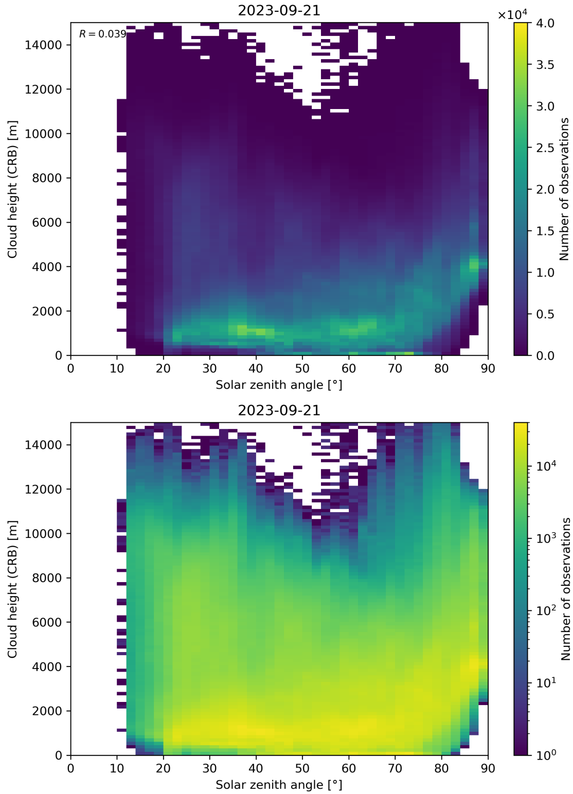
Figure 102: Scatter density plot of “Solar zenith angle” against “Cloud height (CRB)” for 2023-09-20 to 2023-09-22.
