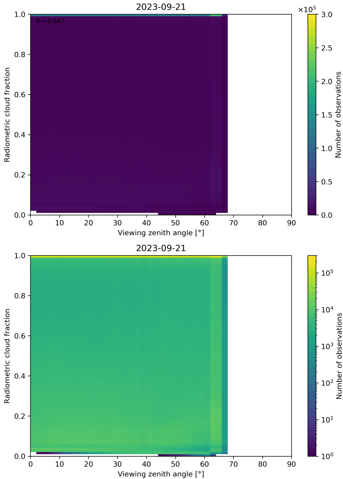
Figure 107: Scatter density plot of “Viewing zenith angle” against “Radiometric cloud fraction” for 2023-09-20 to 2023-09-22.
