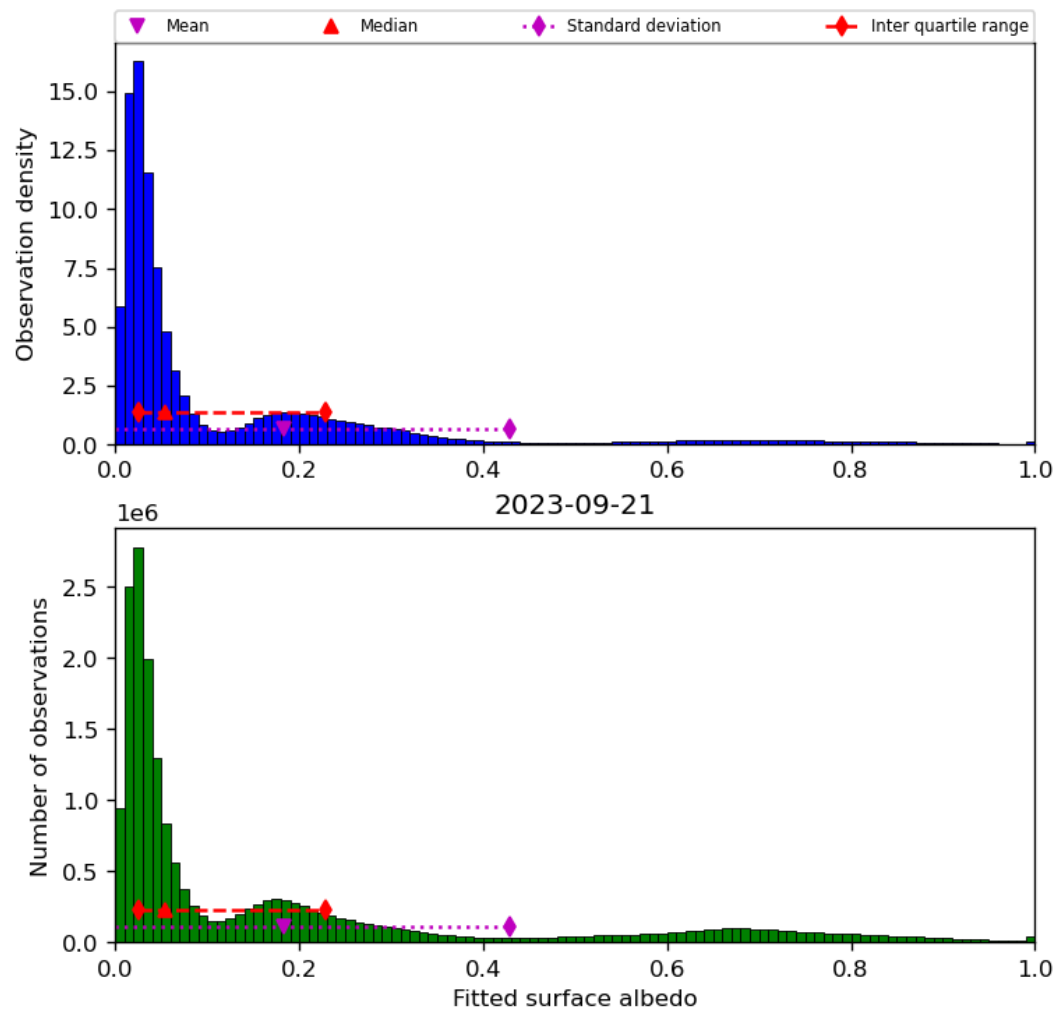
Figure 45: Histogram of “Fitted surface albedo” for 2023-09-20 to 2023-09-22
