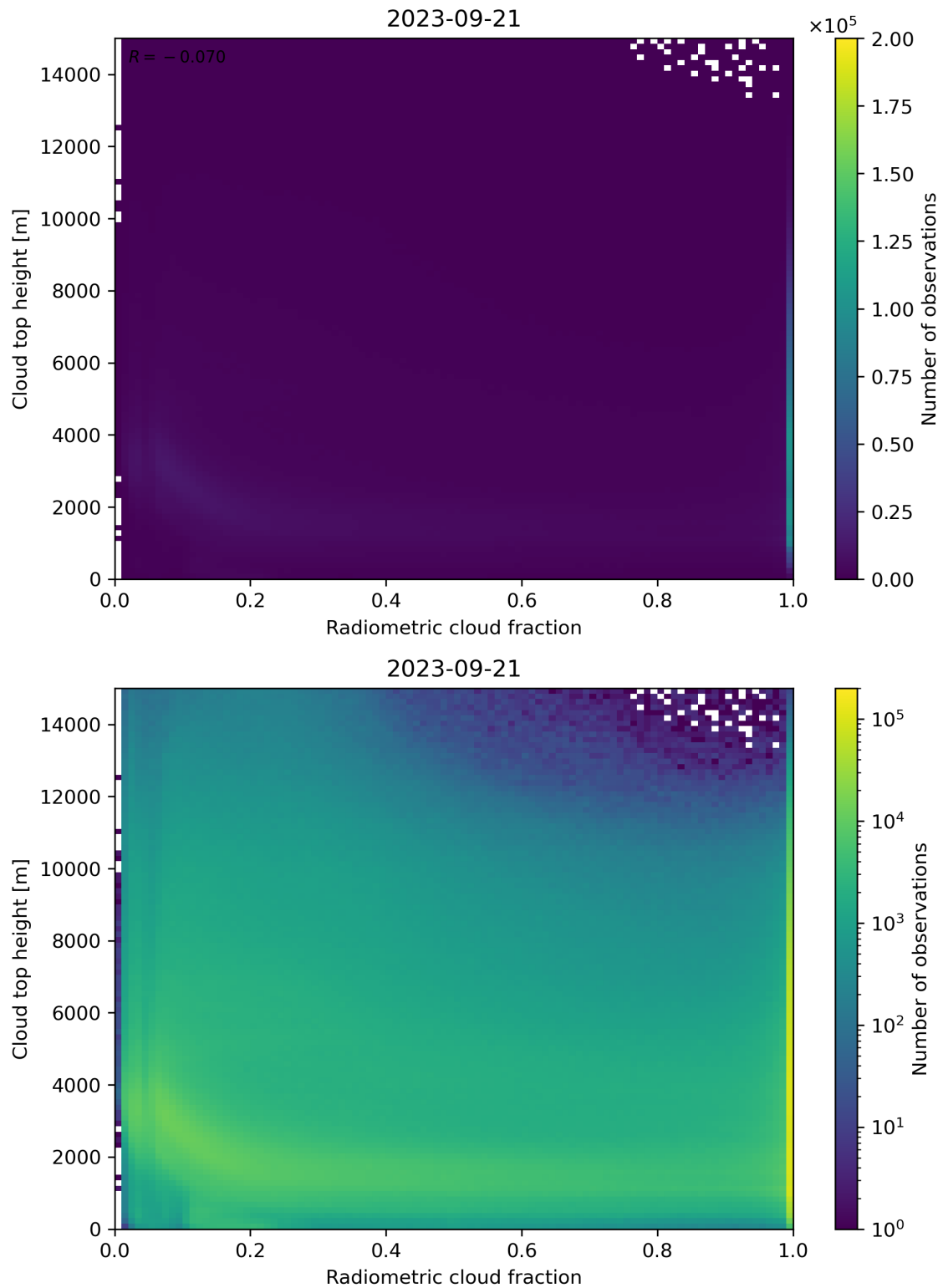
Figure 76: Scatter density plot of “Radiometric cloud fraction” against “Cloud top height” for 2023-09-20 to 2023-09-22.
