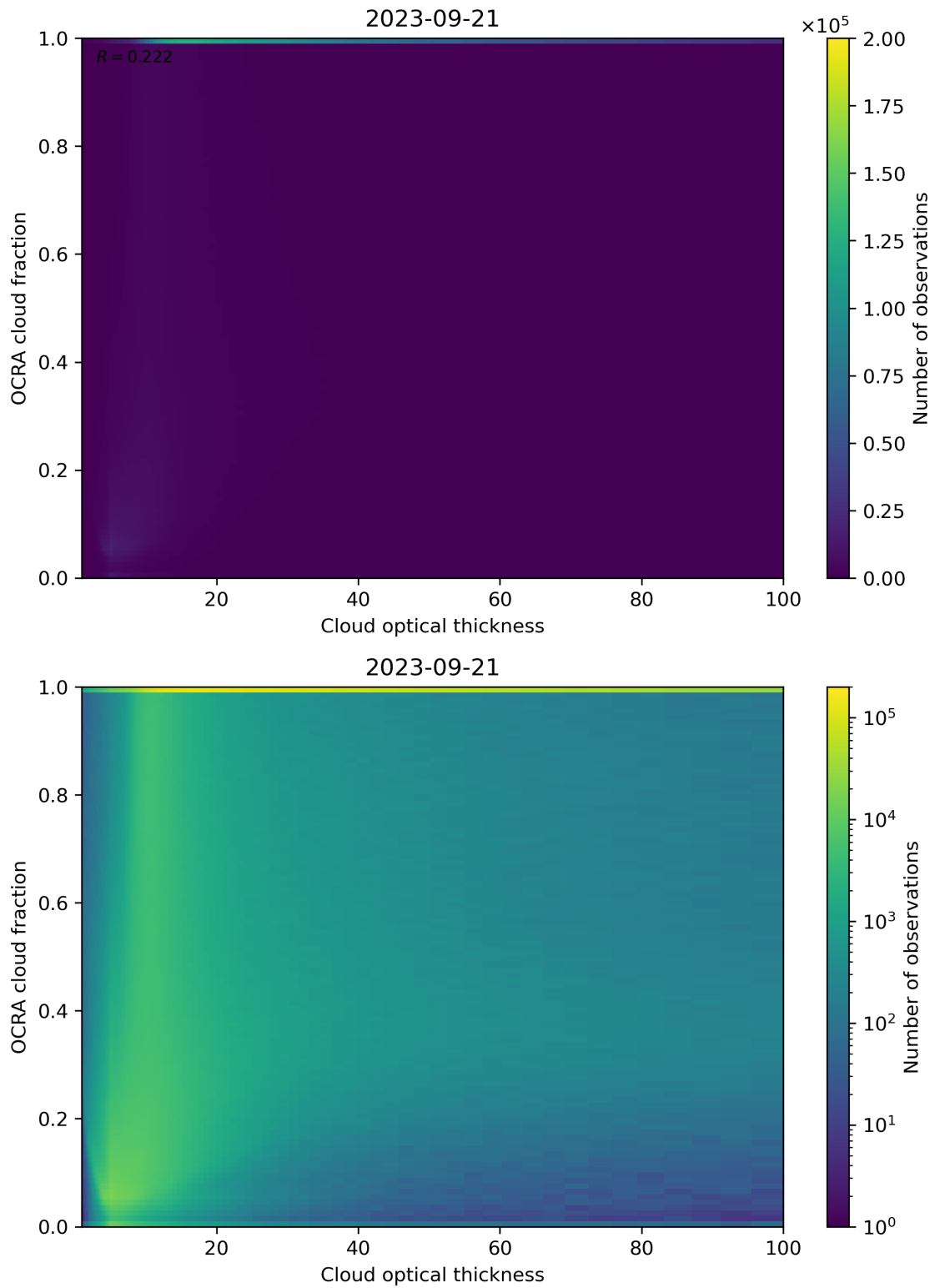
Figure 83: Scatter density plot of “Cloud optical thickness” against “OCRA cloud fraction” for 2023-09-20 to 2023-09-22.
