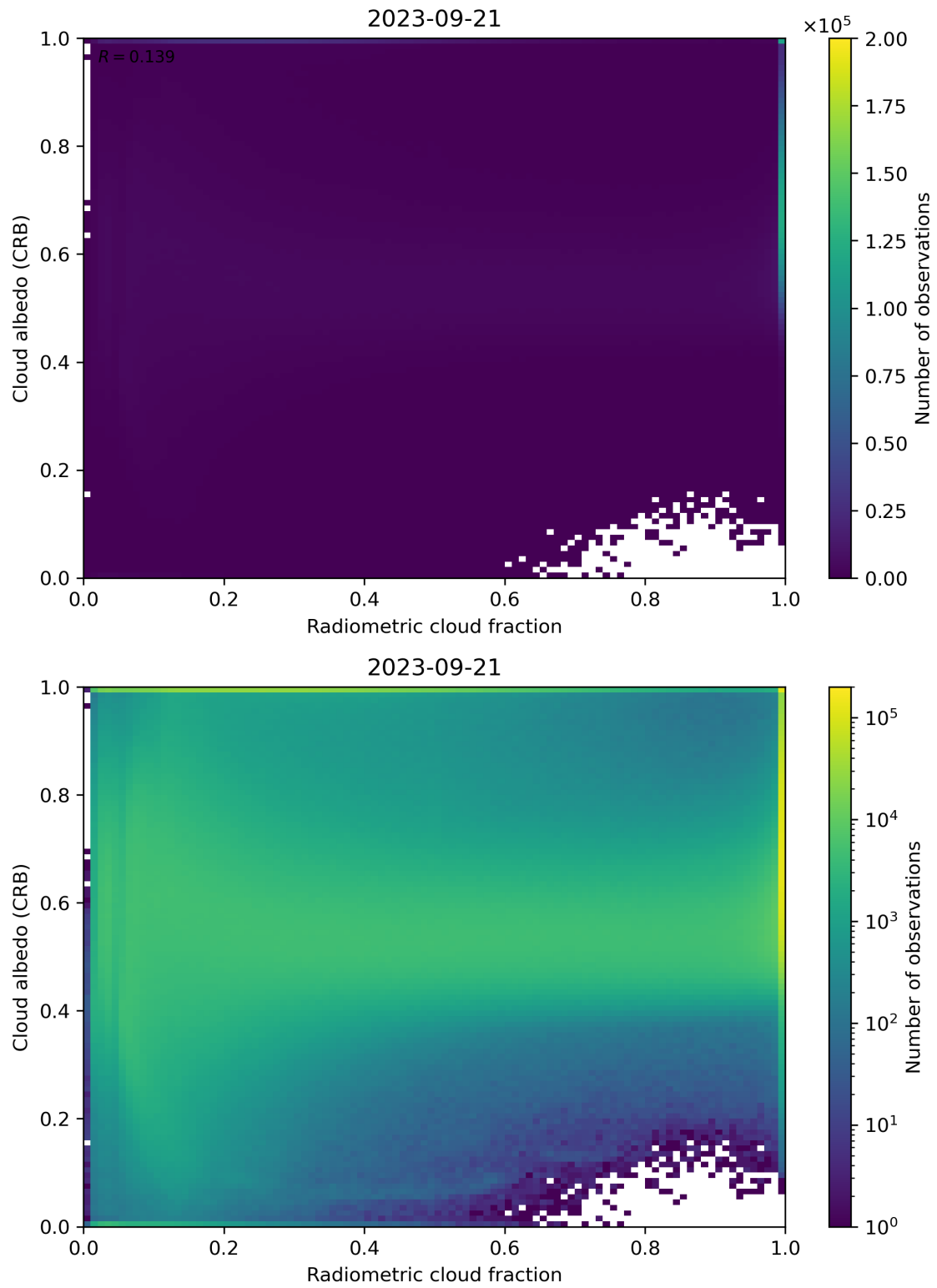
Figure 71: Scatter density plot of “Radiometric cloud fraction” against “Cloud albedo (CRB)” for 2023-09-20 to 2023-09-22.
