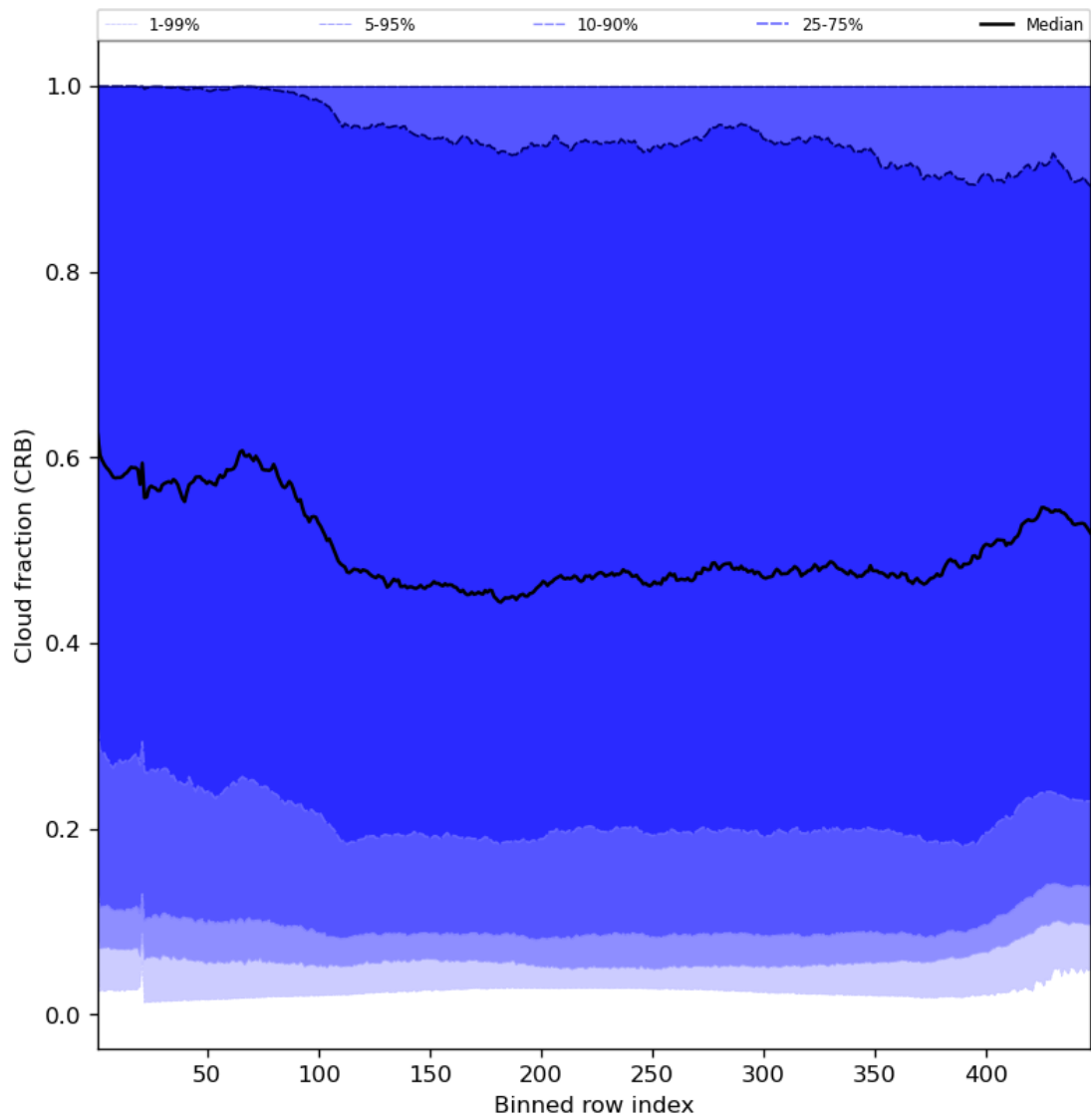
Figure 58: Along track statistics of “Cloud fraction (CRB)” for 2023-09-20 to 2023-09-22
