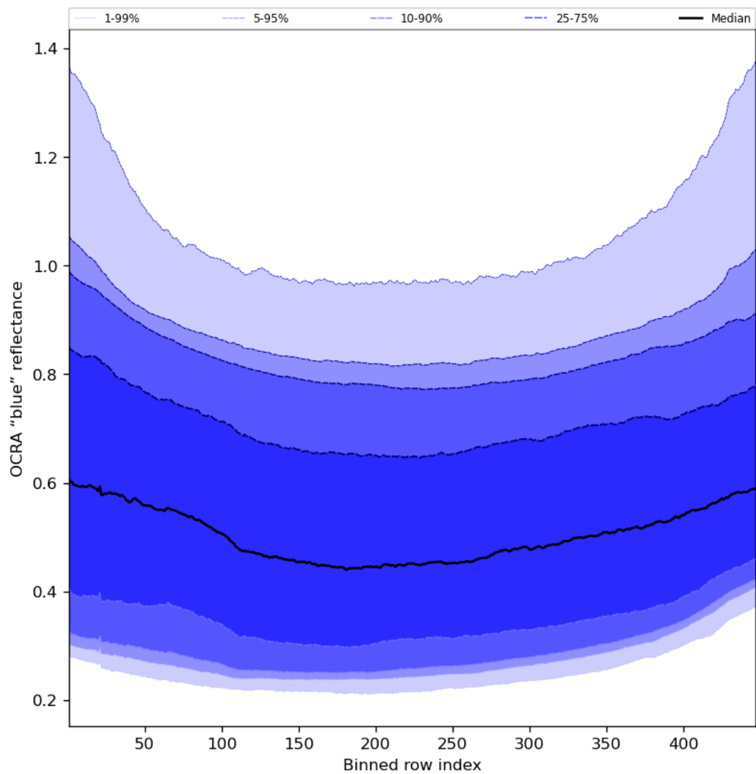
Figure 67: Along track statistics of “OCRA “blue” reflectance” for 2023-09-20 to 2023-09-22
