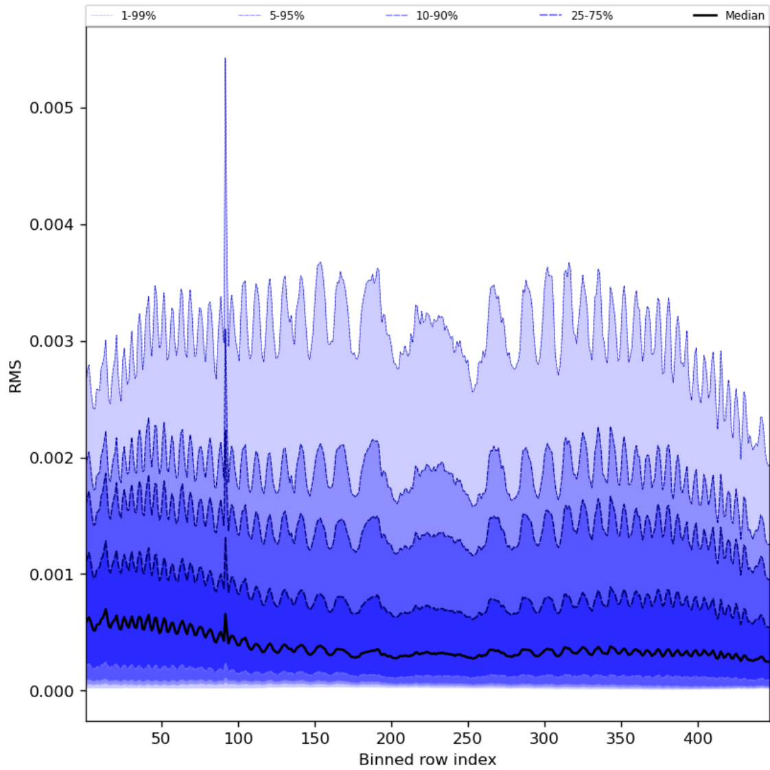
Figure 63: Along track statistics of “RMS” for 2023-09-20 to 2023-09-22
