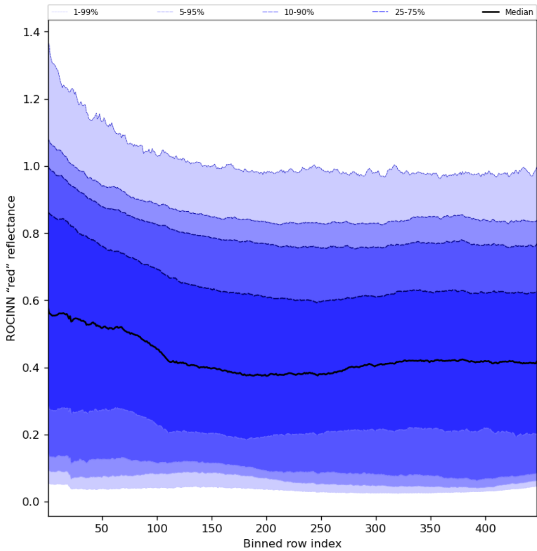
Figure 69: Along track statistics of “ROCINN “red” reflectance” for 2023-09-20 to 2023-09-22
