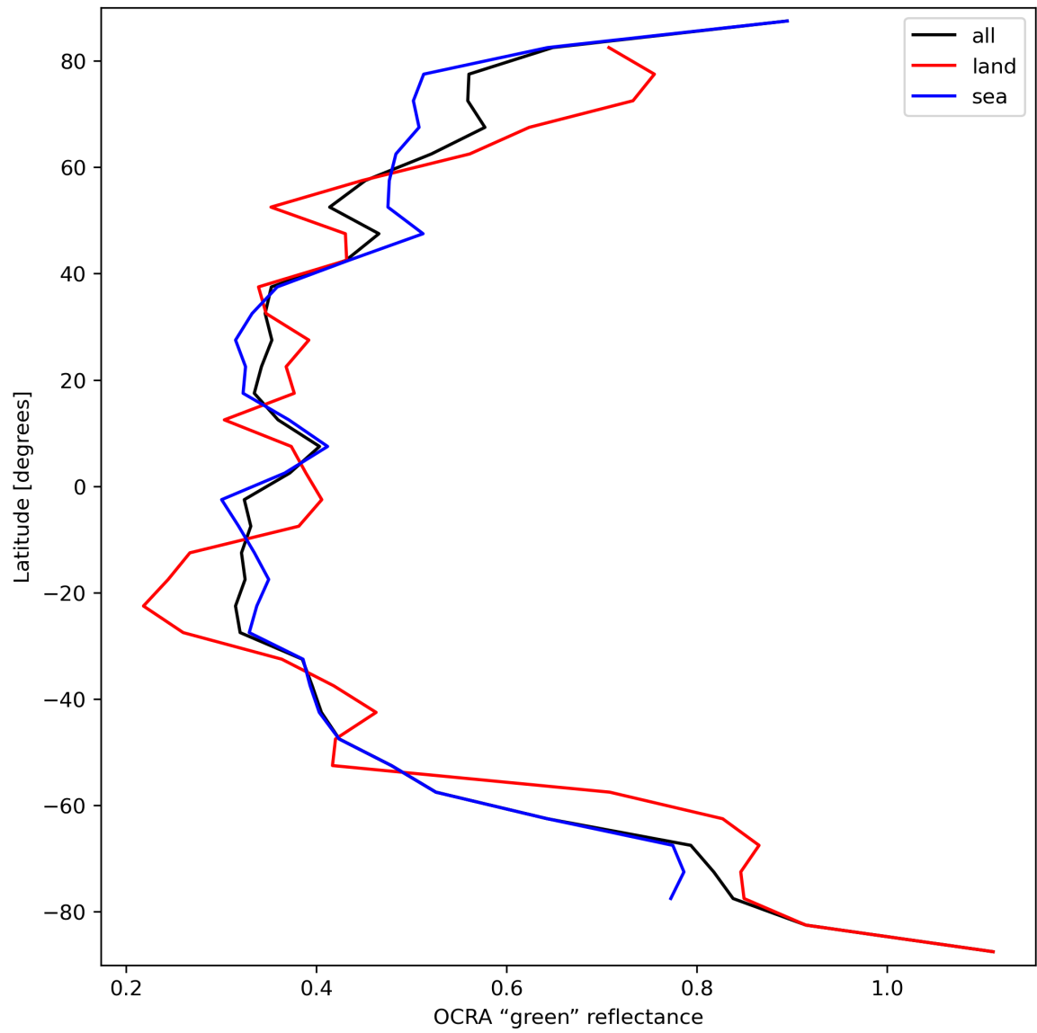
Figure 36: Zonal average of “OCRA “green” reflectance” for 2023-09-20 to 2023-09-22.
