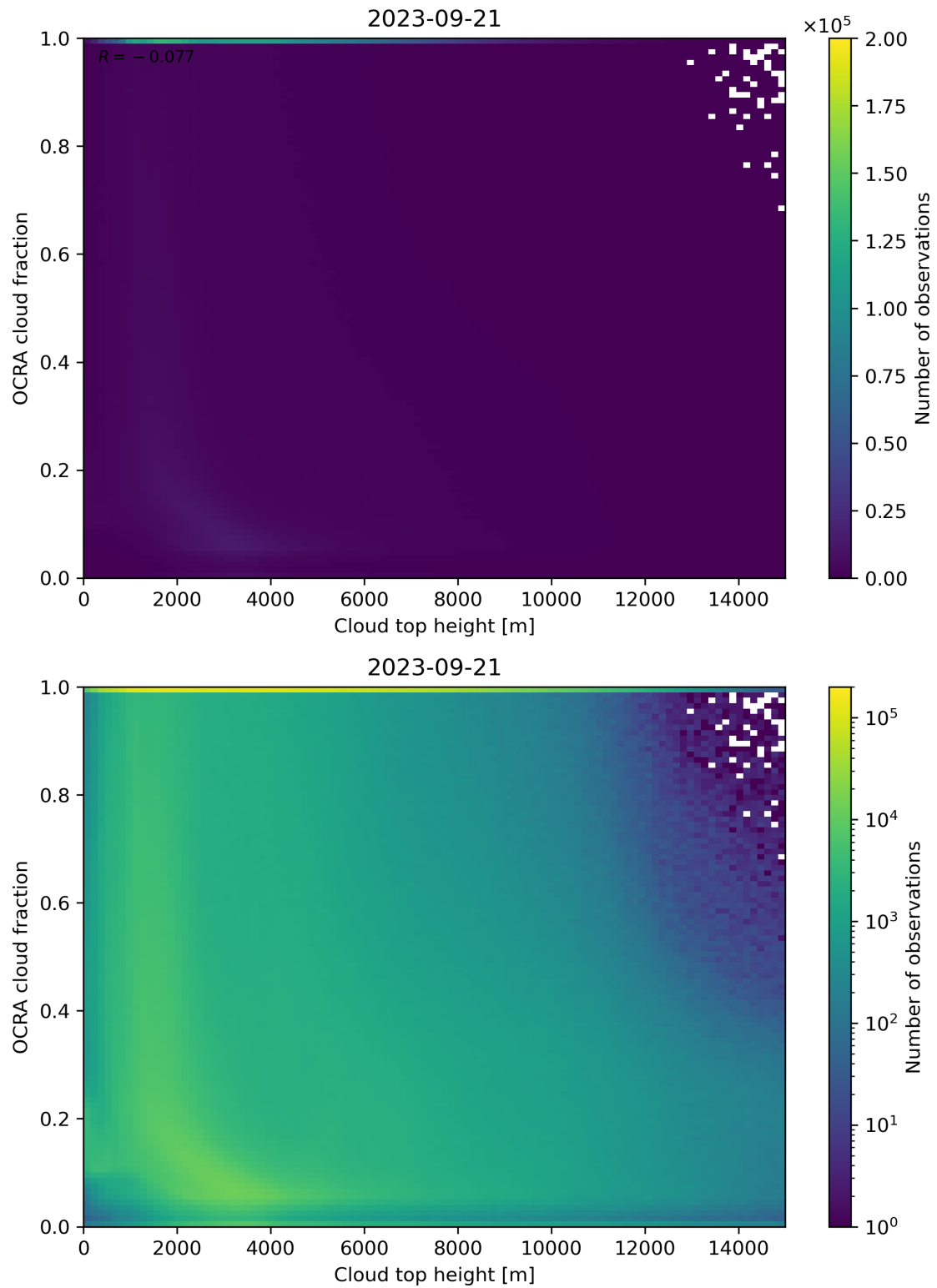
Figure 87: Scatter density plot of “Cloud top height” against “OCRA cloud fraction” for 2023-09-20 to 2023-09-22.
