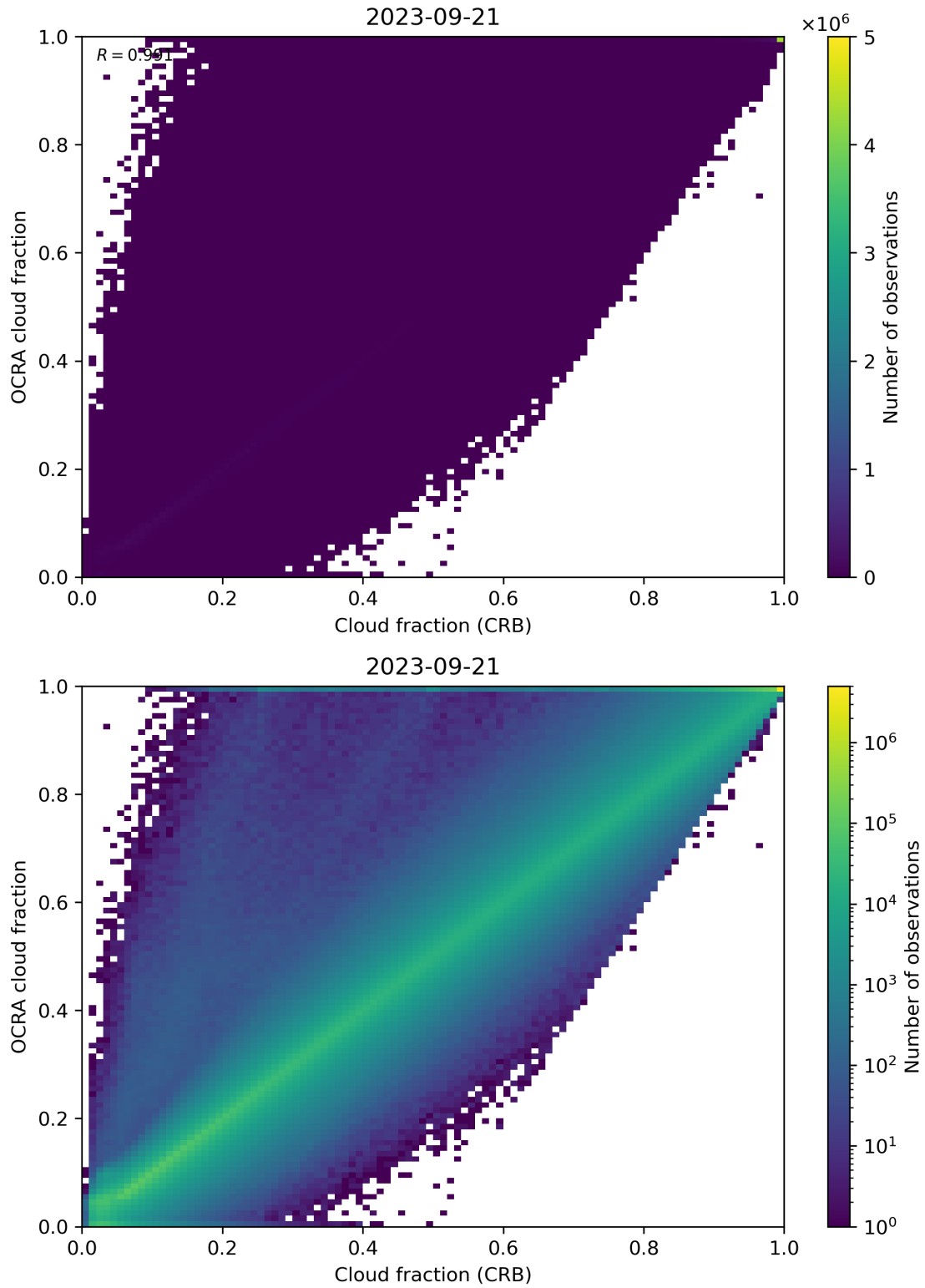
Figure 78: Scatter density plot of “Cloud fraction (CRB)” against “OCRA cloud fraction” for 2023-09-20 to 2023-09-22.
