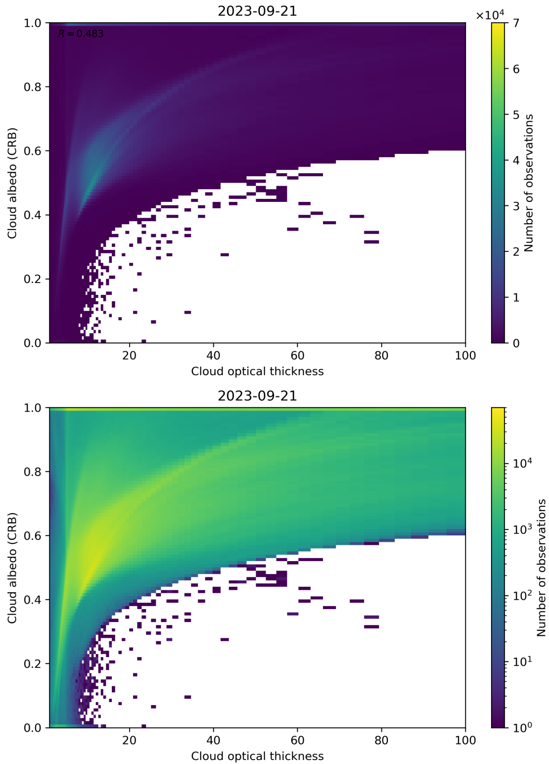
Figure 82: Scatter density plot of “Cloud optical thickness” against “Cloud albedo (CRB)” for 2023-09-20 to 2023-09-22.
