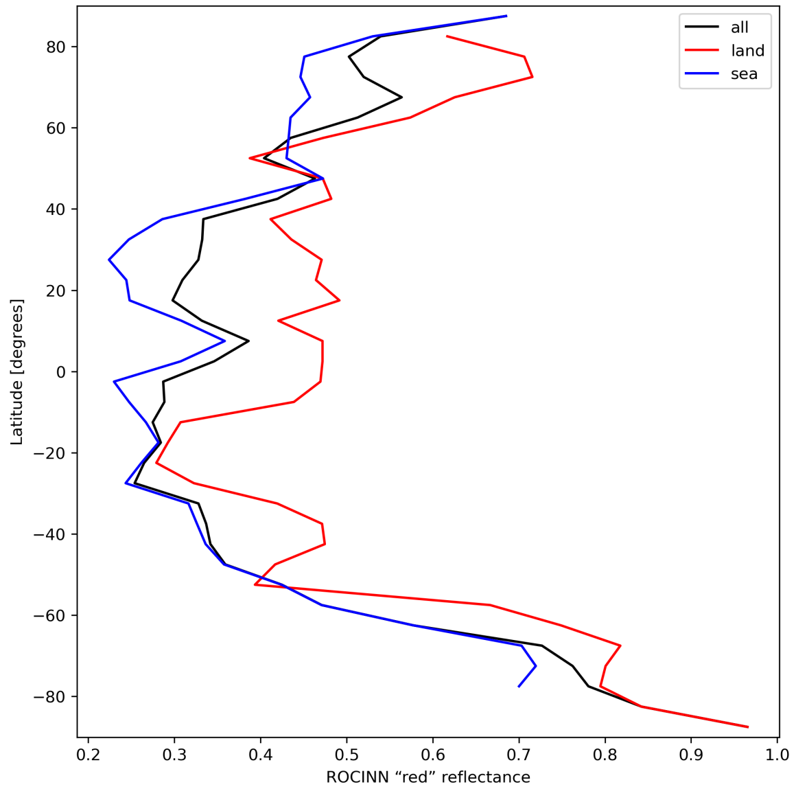
Figure 37: Zonal average of “ROCINN “red” reflectance” for 2023-09-20 to 2023-09-22.
