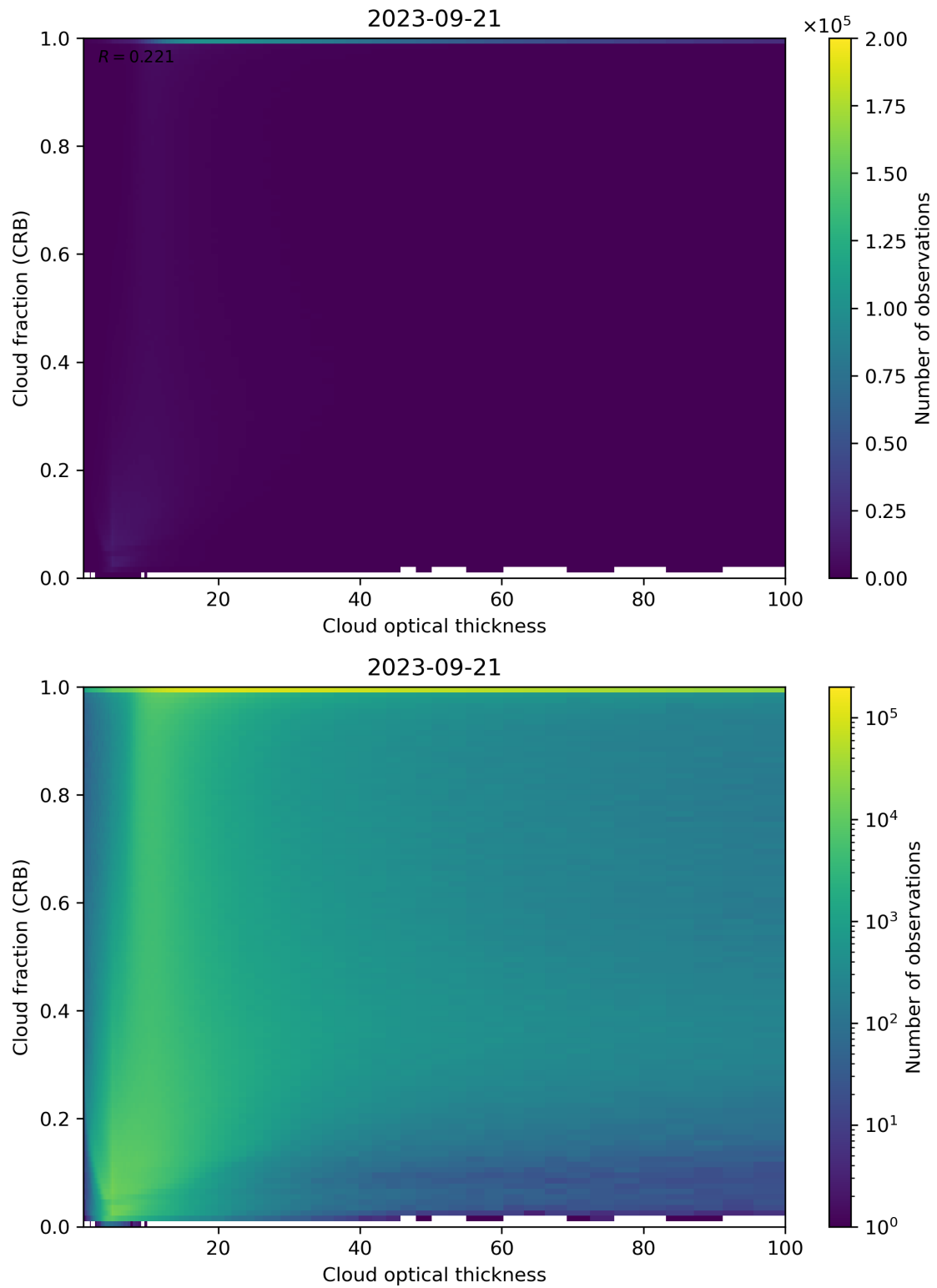
Figure 84: Scatter density plot of “Cloud optical thickness” against “Cloud fraction (CRB)” for 2023-09-20 to 2023-09-22.
