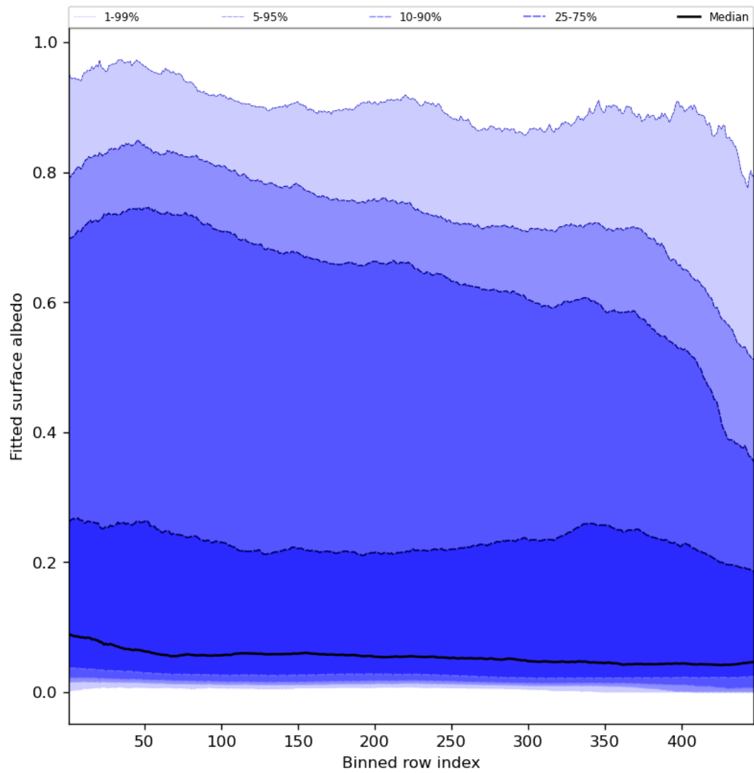
Figure 61: Along track statistics of “Fitted surface albedo” for 2023-09-20 to 2023-09-22
