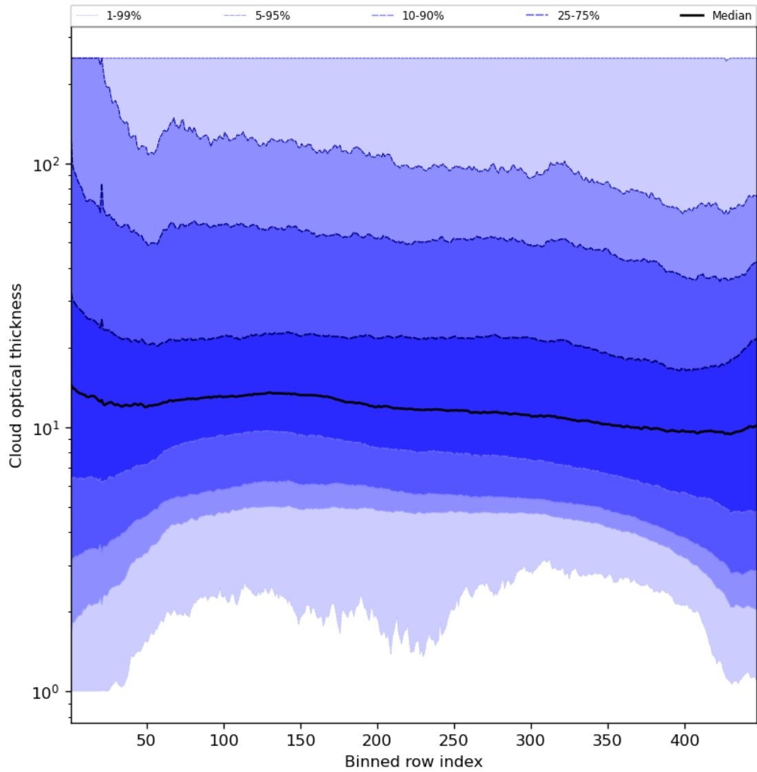
Figure 57: Along track statistics of “Cloud optical thickness” for 2023-09-20 to 2023-09-22
