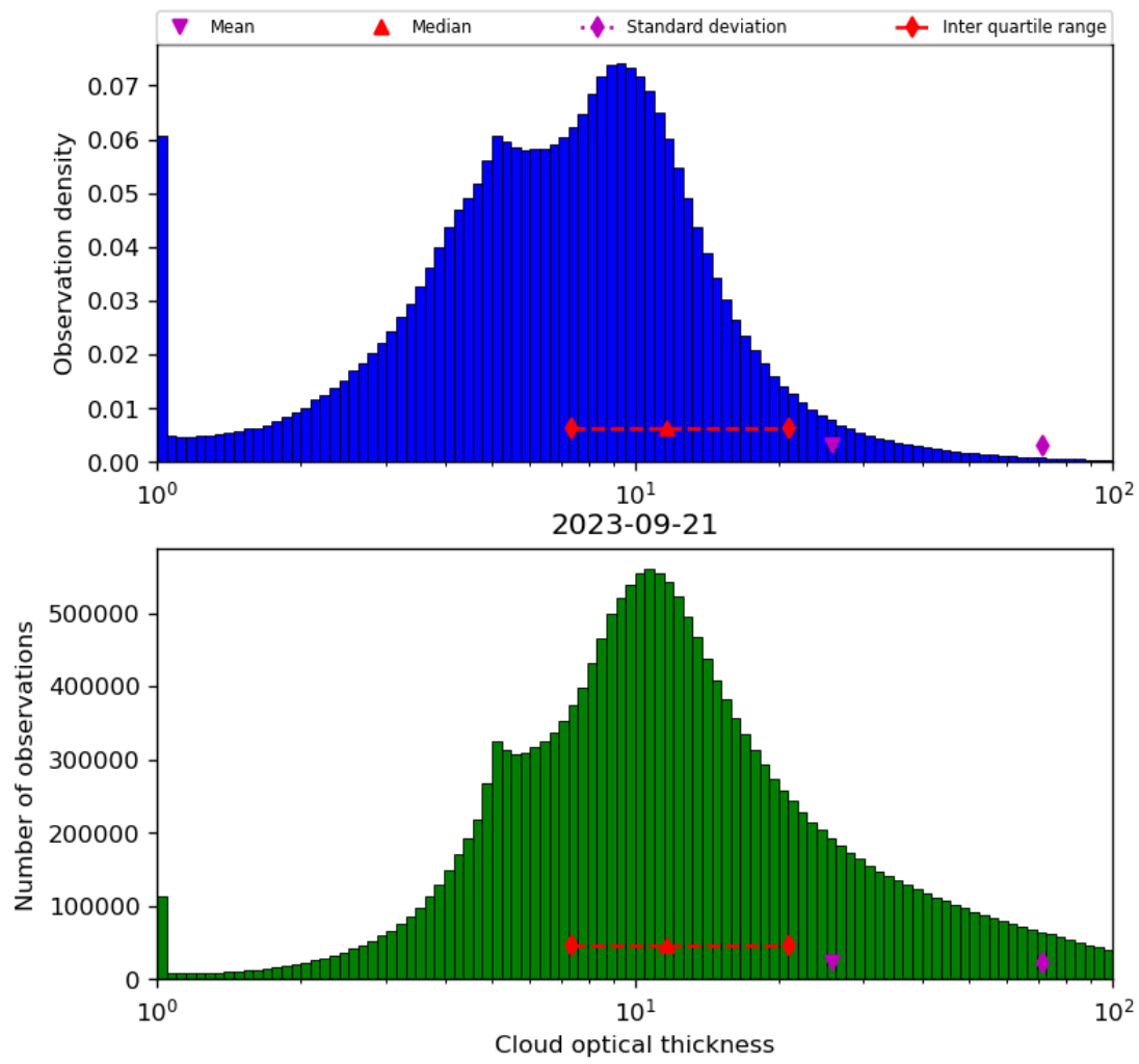
Figure 41: Histogram of “Cloud optical thickness” for 2023-09-20 to 2023-09-22
