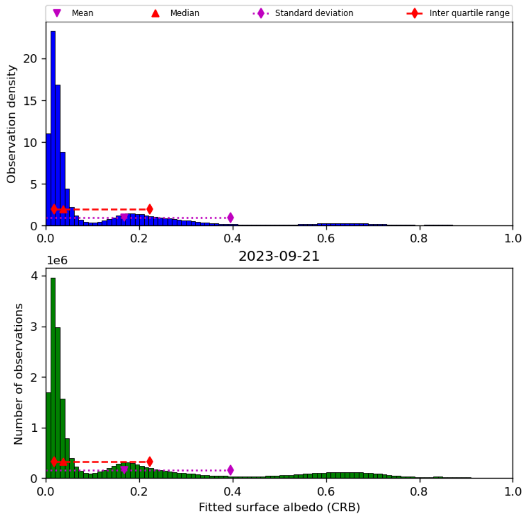
Figure 46: Histogram of “Fitted surface albedo (CRB)” for 2023-09-20 to 2023-09-22
