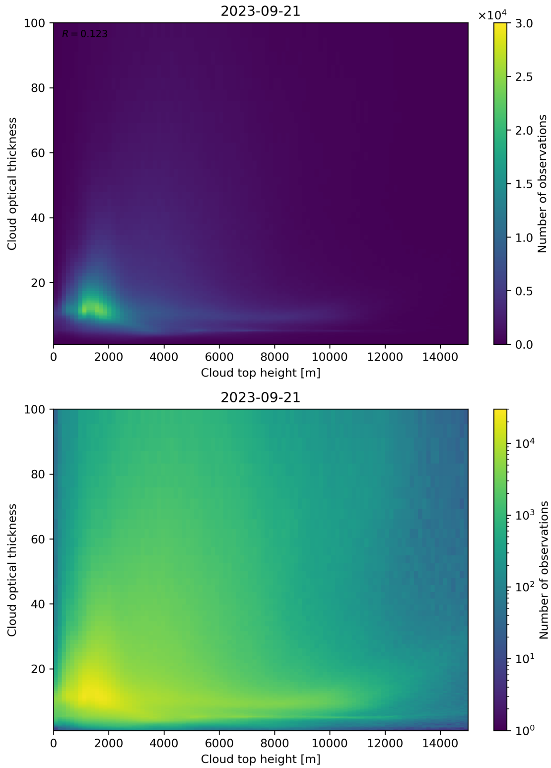
Figure 90: Scatter density plot of “Cloud top height” against “Cloud optical thickness” for 2023-09-20 to 2023-09-22.
