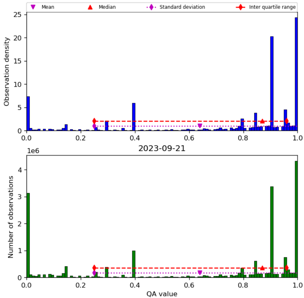
Figure 38: Histogram of “QA value” for 2023-09-20 to 2023-09-22
