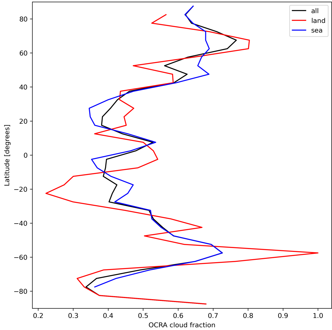
Figure 34: Zonal average of “OCRA cloud fraction” for 2023-09-20 to 2023-09-22.
