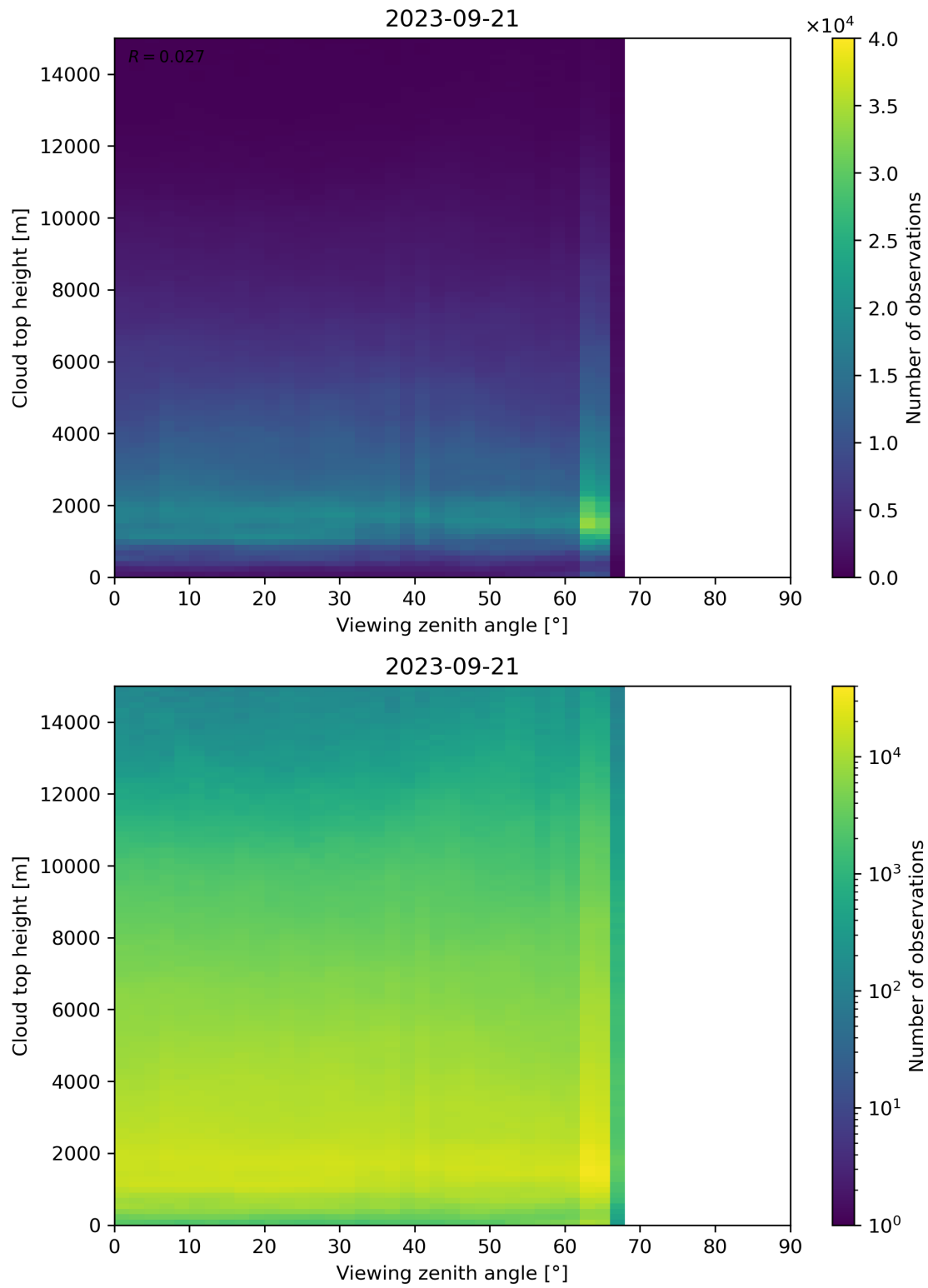
Figure 112: Scatter density plot of “Viewing zenith angle” against “Cloud top height” for 2023-09-20 to 2023-09-22.
