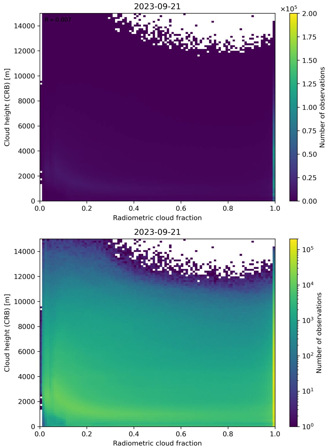
Figure 74: Scatter density plot of “Radiometric cloud fraction” against “Cloud height (CRB)” for 2023-09-20 to 2023-09-22.
