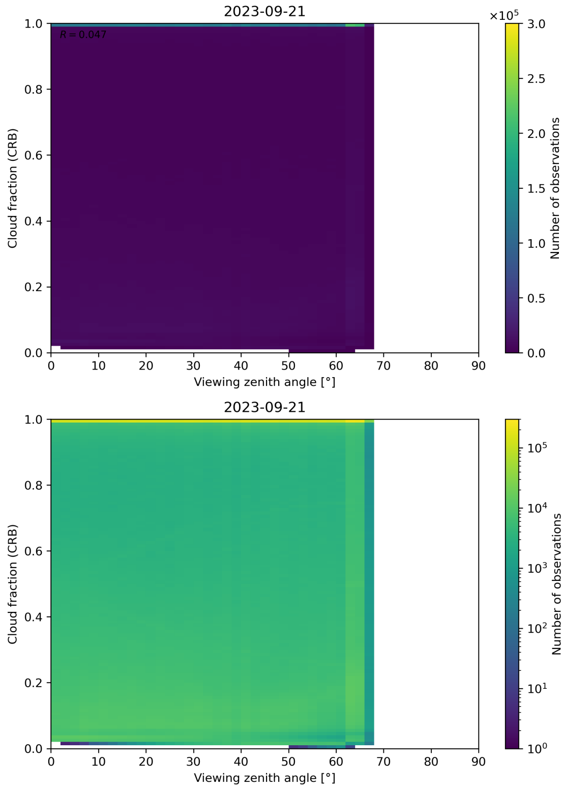
Figure 109: Scatter density plot of “Viewing zenith angle” against “Cloud fraction (CRB)” for 2023-09-20 to 2023-09-22.
