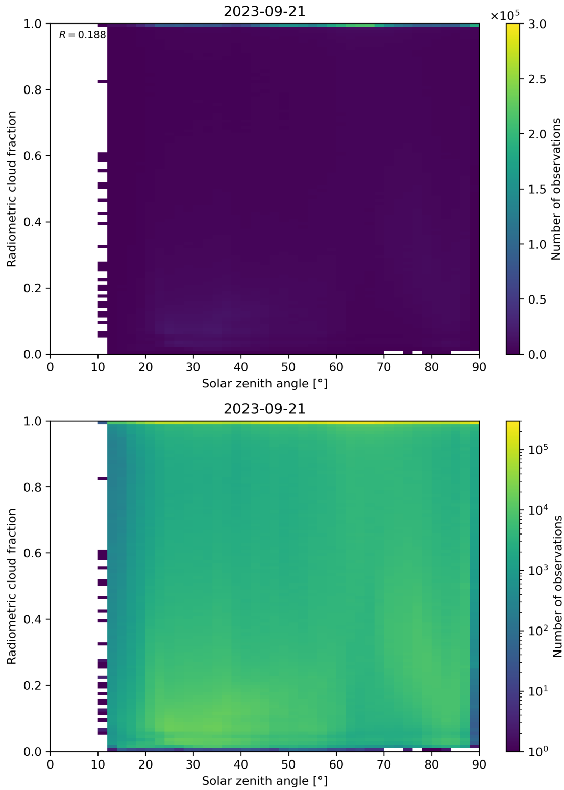
Figure 99: Scatter density plot of “Solar zenith angle” against “Radiometric cloud fraction” for 2023-09-20 to 2023-09-22.
