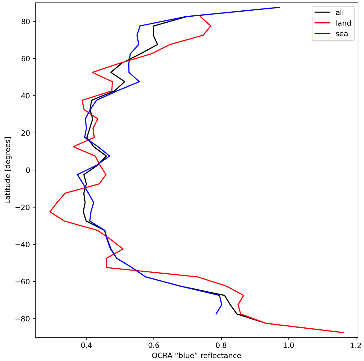
Figure 35: Zonal average of “OCRA “blue” reflectance” for 2023-09-20 to 2023-09-22.
