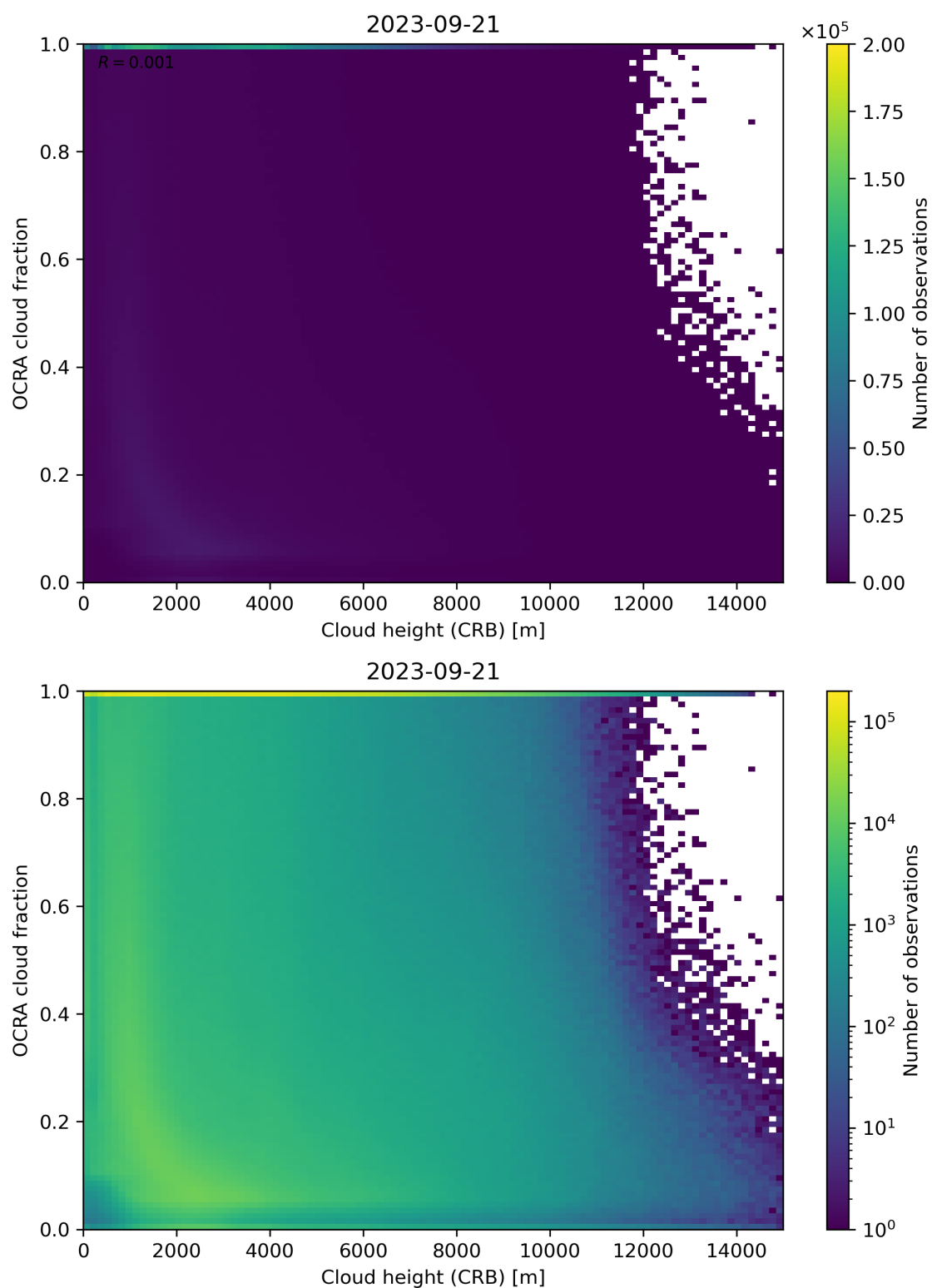
Figure 81: Scatter density plot of “Cloud height (CRB)” against “OCRA cloud fraction” for 2023-09-20 to 2023-09-22.
