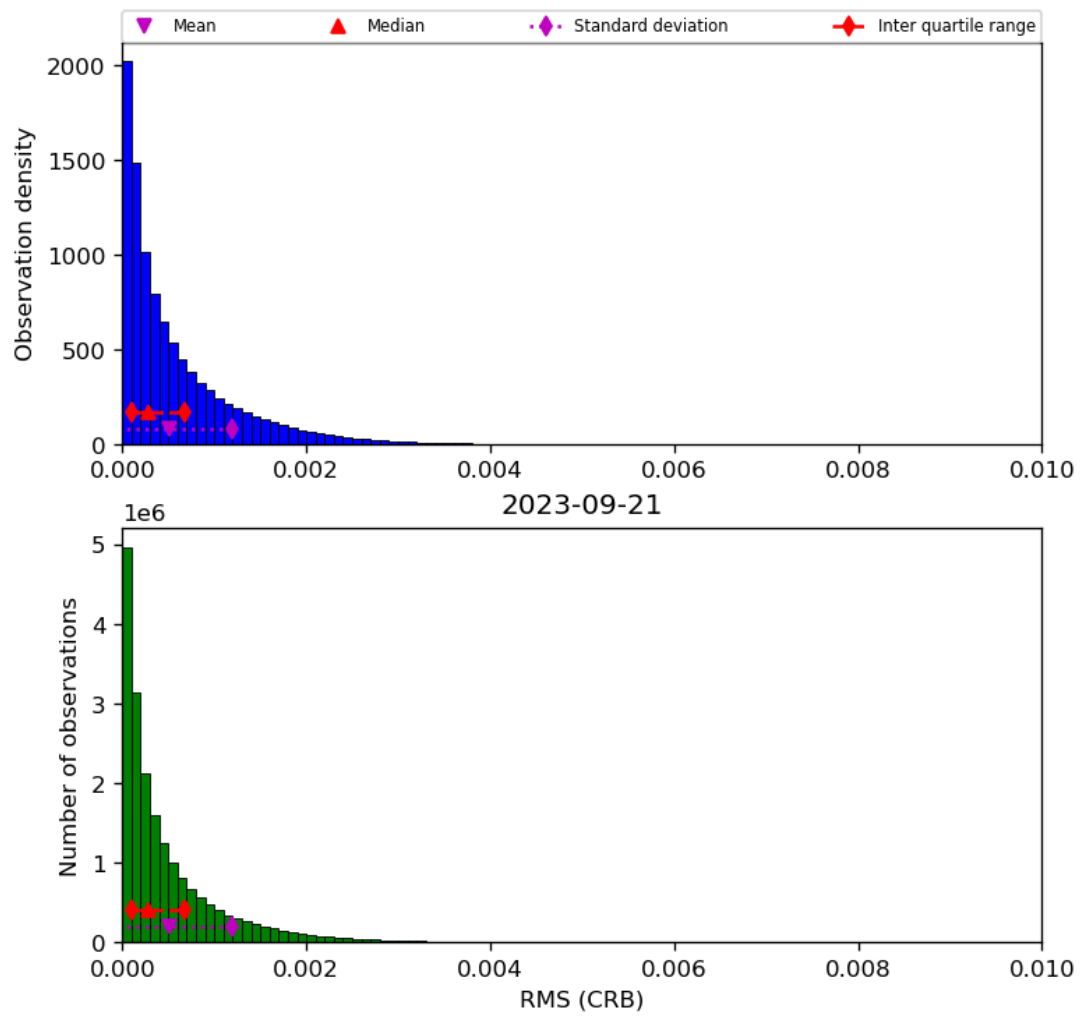
Figure 48: Histogram of “RMS (CRB)” for 2023-09-20 to 2023-09-22
