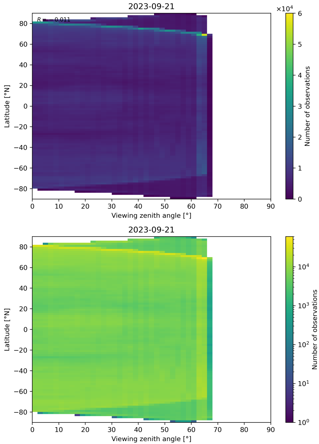
Figure 113: Scatter density plot of “Viewing zenith angle” against “Latitude” for 2023-09-20 to 2023-09-22.
