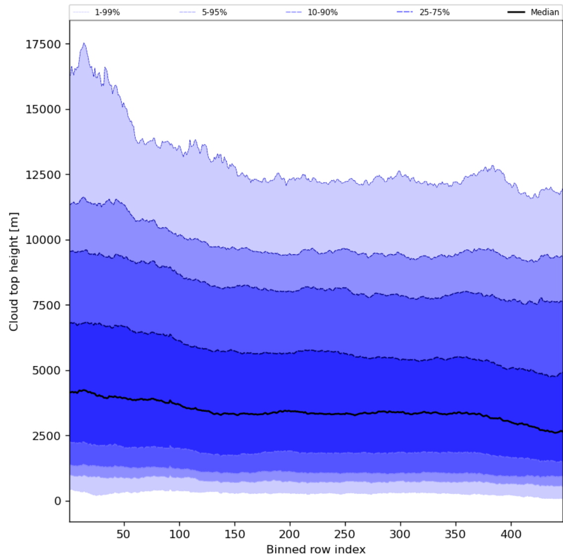
Figure 56: Along track statistics of “Cloud top height” for 2023-09-20 to 2023-09-22
