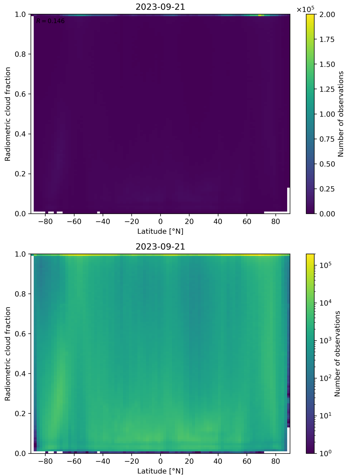
Figure 92: Scatter density plot of “Latitude” against “Radiometric cloud fraction” for 2023-09-20 to 2023-09-22.
