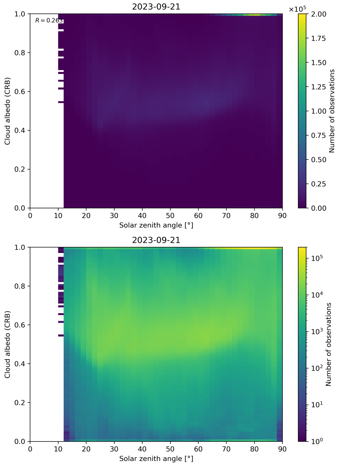
Figure 98: Scatter density plot of “Solar zenith angle” against “Cloud albedo (CRB)” for 2023-09-20 to 2023-09-22.
