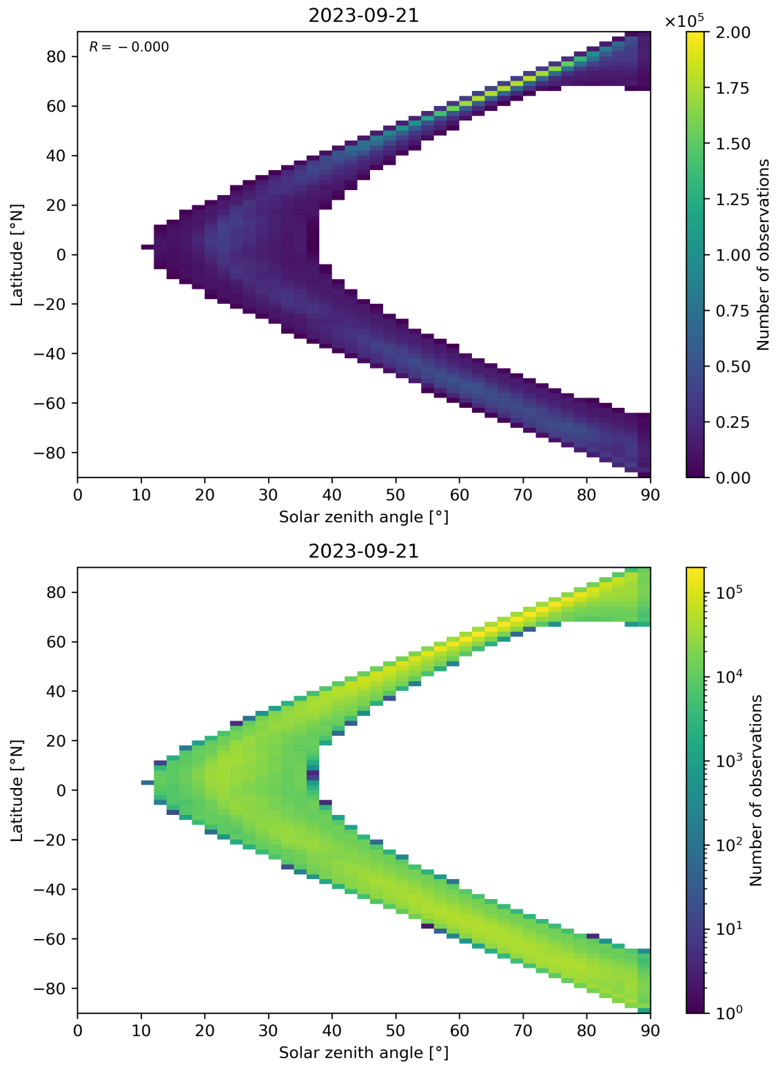
Figure 105: Scatter density plot of “Solar zenith angle” against “Latitude” for 2023-09-20 to 2023-09-22.
