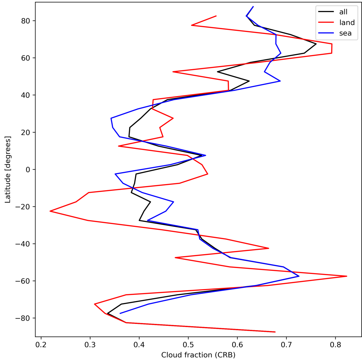
Figure 26: Zonal average of “Cloud fraction (CRB)” for 2023-09-20 to 2023-09-22.
