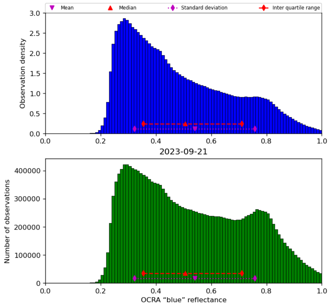
Figure 51: Histogram of “OCRA “blue” reflectance” for 2023-09-20 to 2023-09-22
