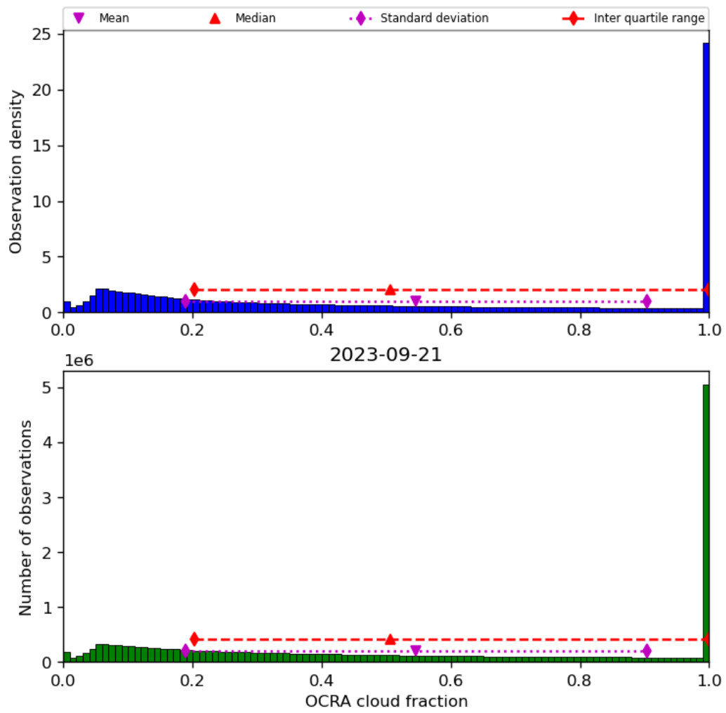
Figure 50: Histogram of “OCRA cloud fraction” for 2023-09-20 to 2023-09-22
