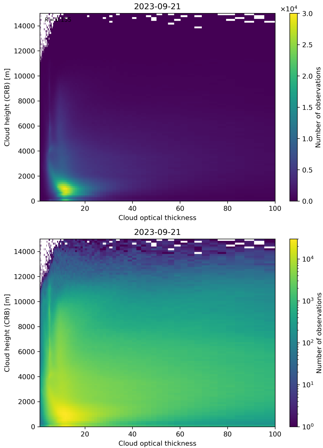
Figure 85: Scatter density plot of “Cloud optical thickness” against “Cloud height (CRB)” for 2023-09-20 to 2023-09-22.
