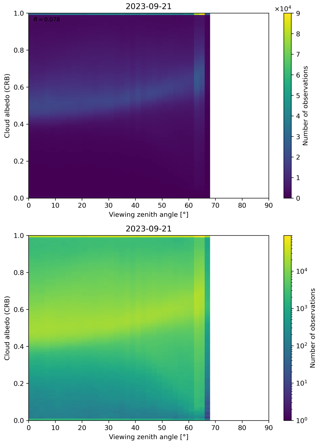
Figure 106: Scatter density plot of “Viewing zenith angle” against “Cloud albedo (CRB)” for 2023-09-20 to 2023-09-22.
