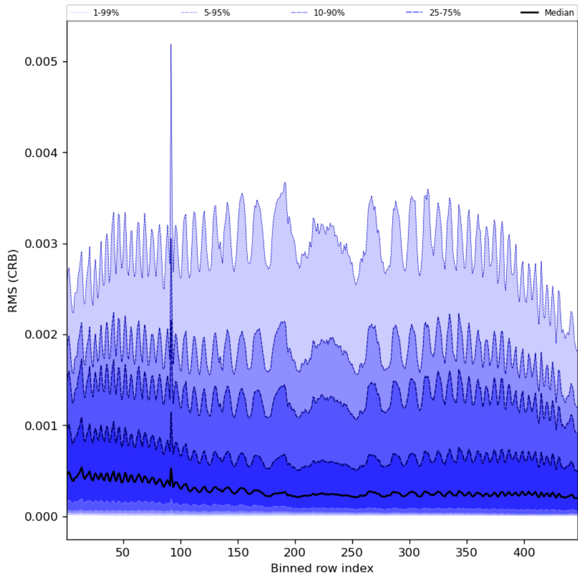
Figure 64: Along track statistics of “RMS (CRB)” for 2023-09-20 to 2023-09-22
