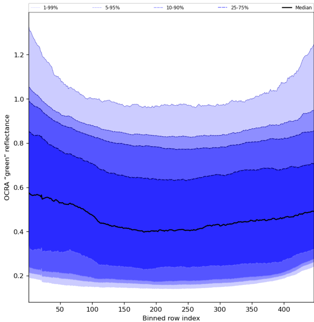
Figure 68: Along track statistics of “OCRA “green” reflectance” for 2023-09-20 to 2023-09-22
