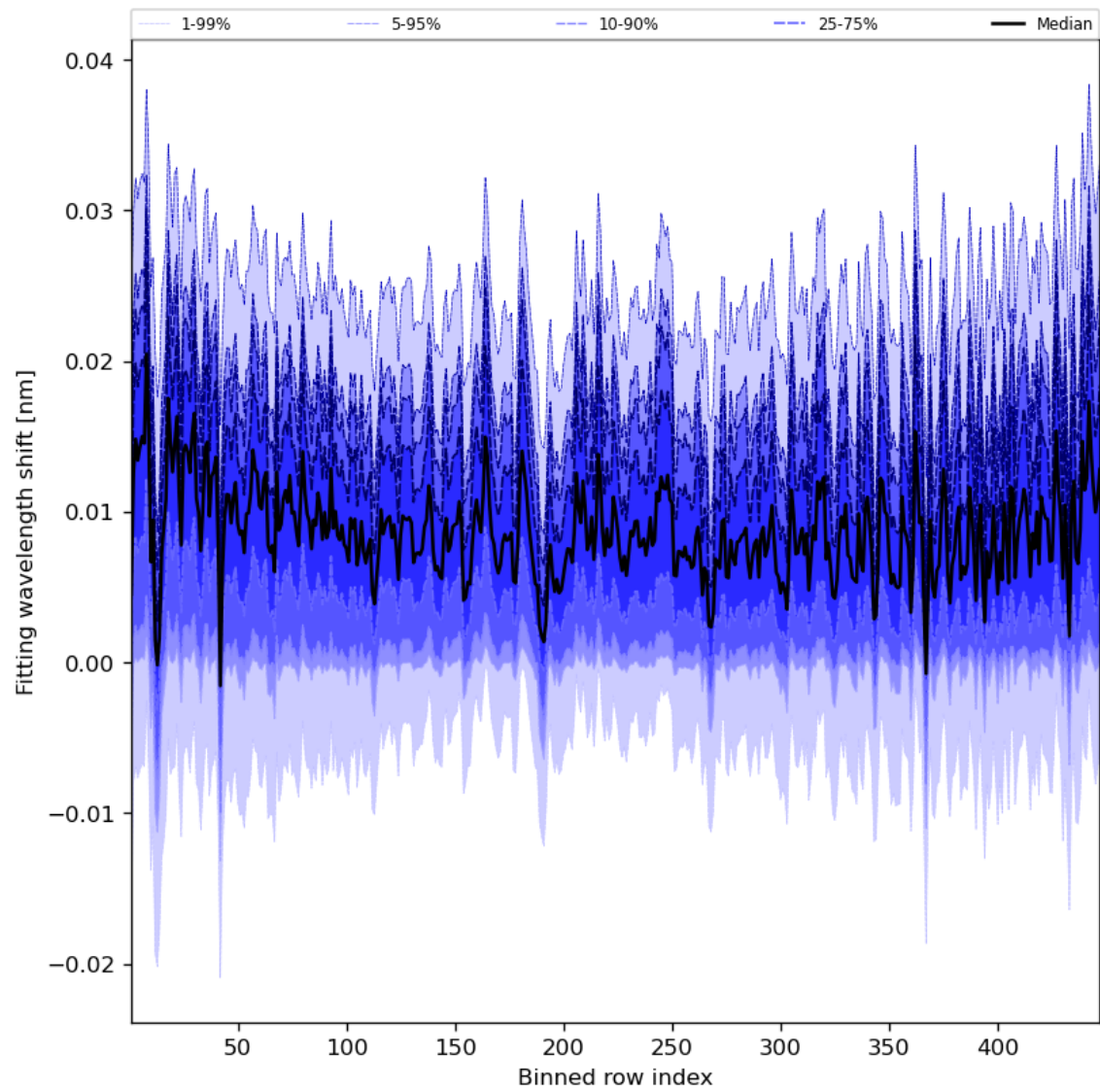
Figure 65: Along track statistics of “Fitting wavelength shift” for 2023-09-20 to 2023-09-22
