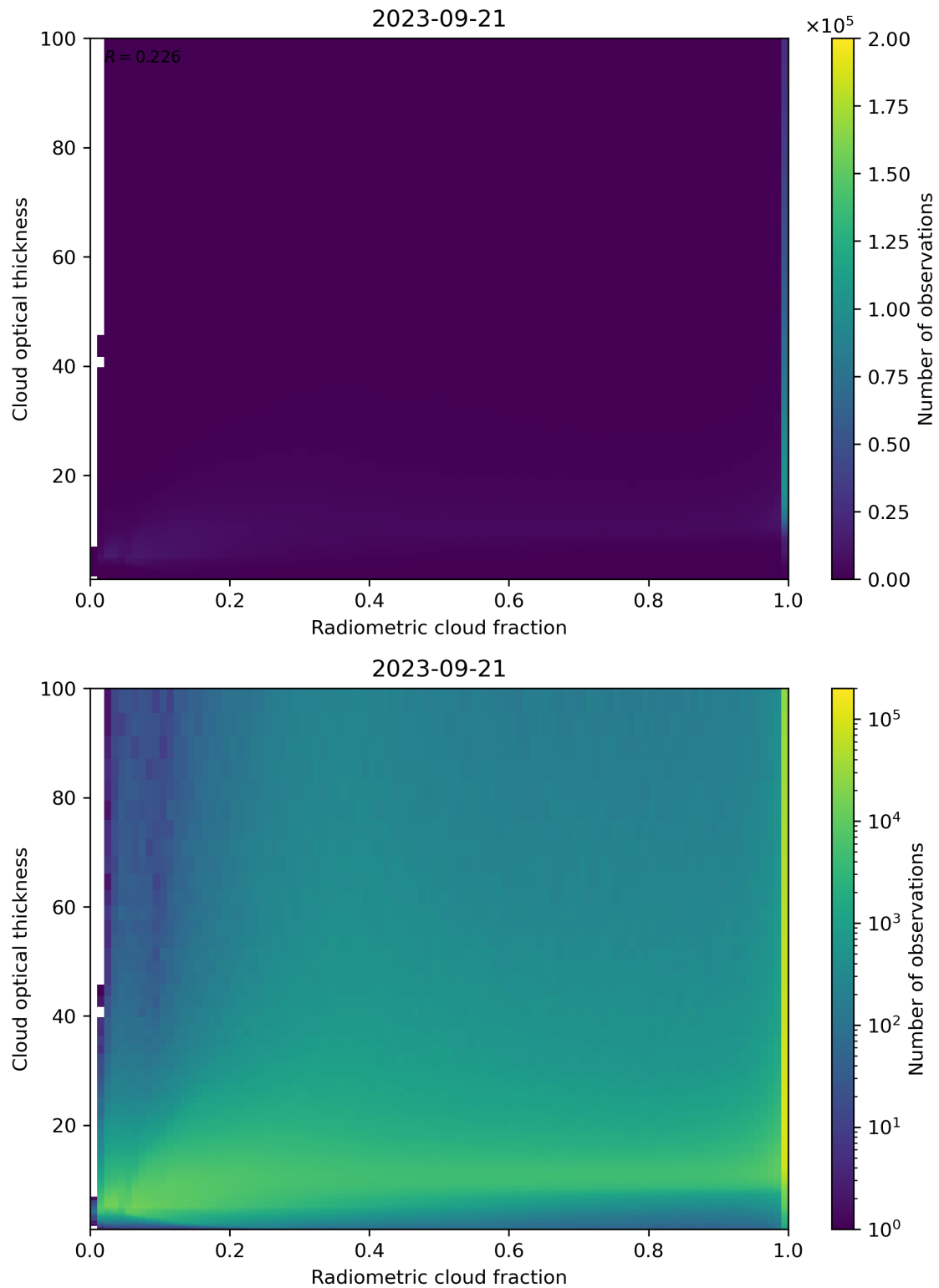
Figure 75: Scatter density plot of “Radiometric cloud fraction” against “Cloud optical thickness” for 2023-09-20 to 2023-09-22.
