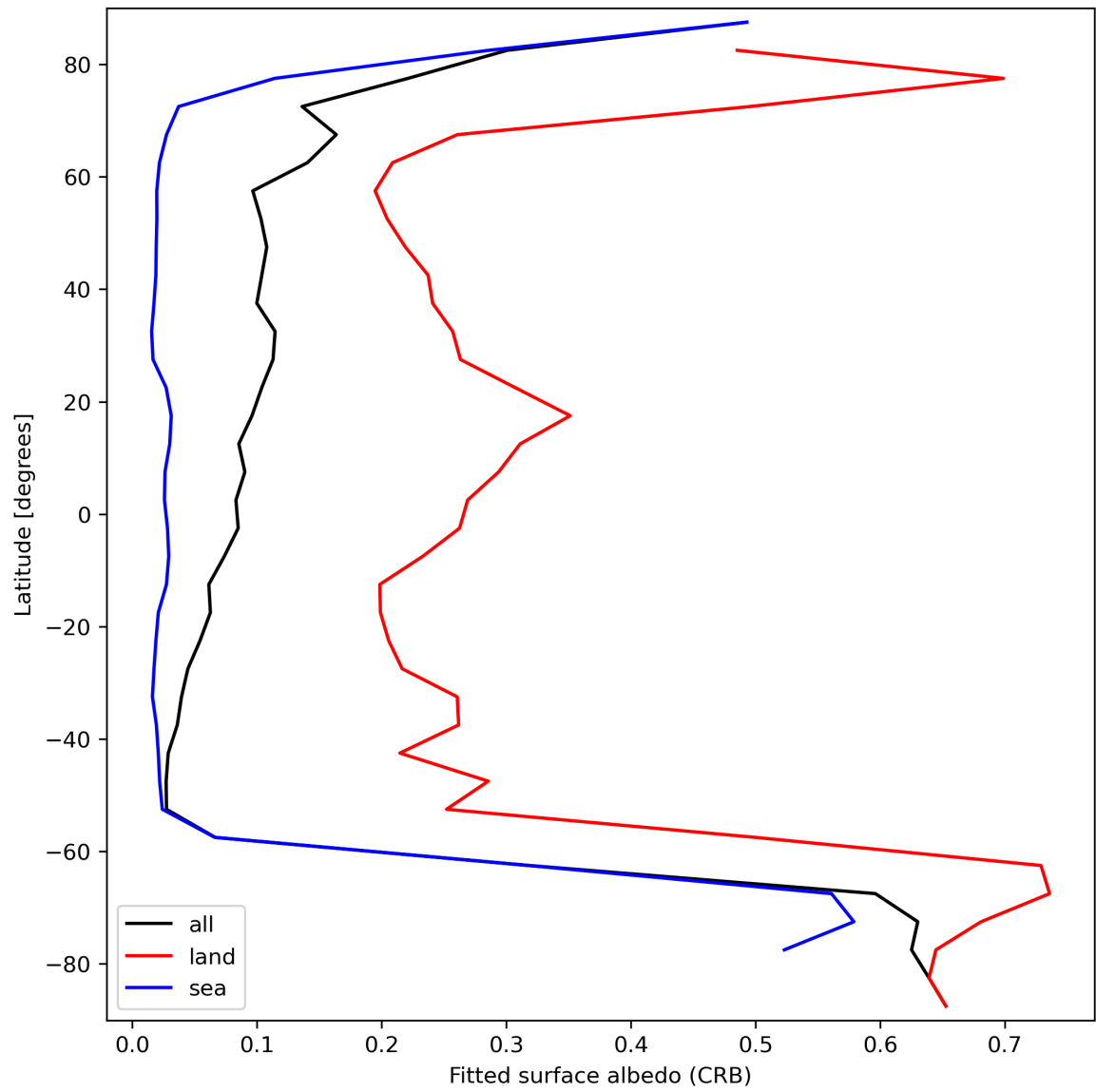
Figure 30: Zonal average of “Fitted surface albedo (CRB)” for 2023-09-20 to 2023-09-22.
