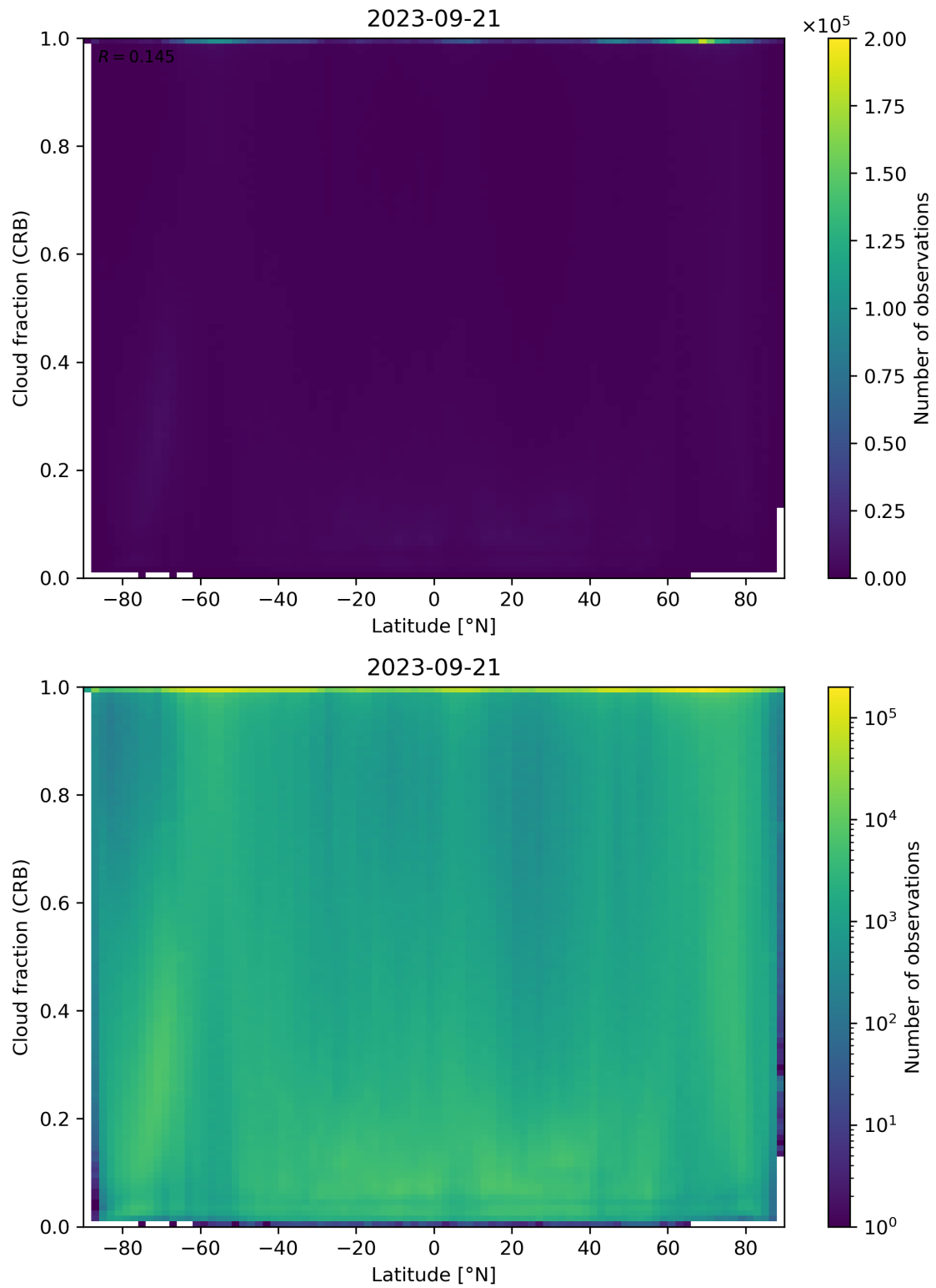
Figure 94: Scatter density plot of “Latitude” against “Cloud fraction (CRB)” for 2023-09-20 to 2023-09-22.
