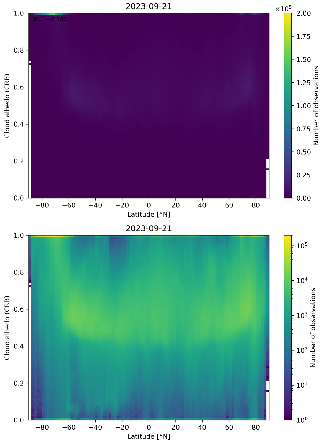
Figure 91: Scatter density plot of “Latitude” against “Cloud albedo (CRB)” for 2023-09-20 to 2023-09-22.
