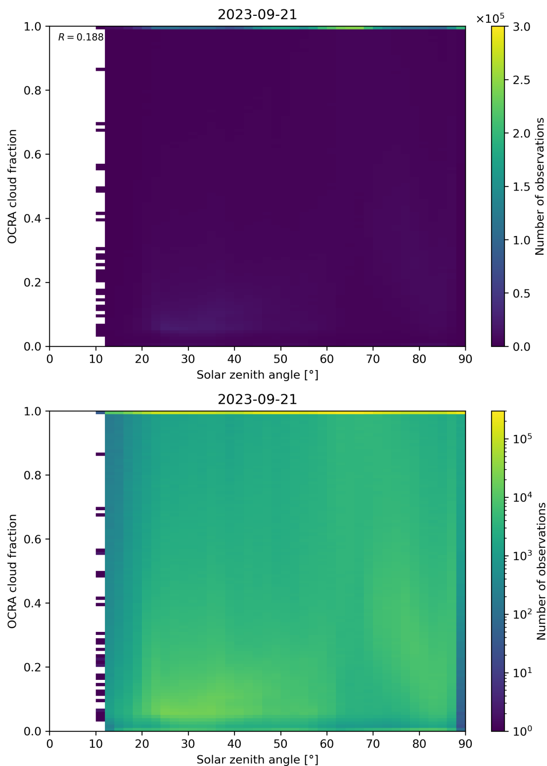
Figure 100: Scatter density plot of “Solar zenith angle” against “OCRA cloud fraction” for 2023-09-20 to 2023-09-22.
