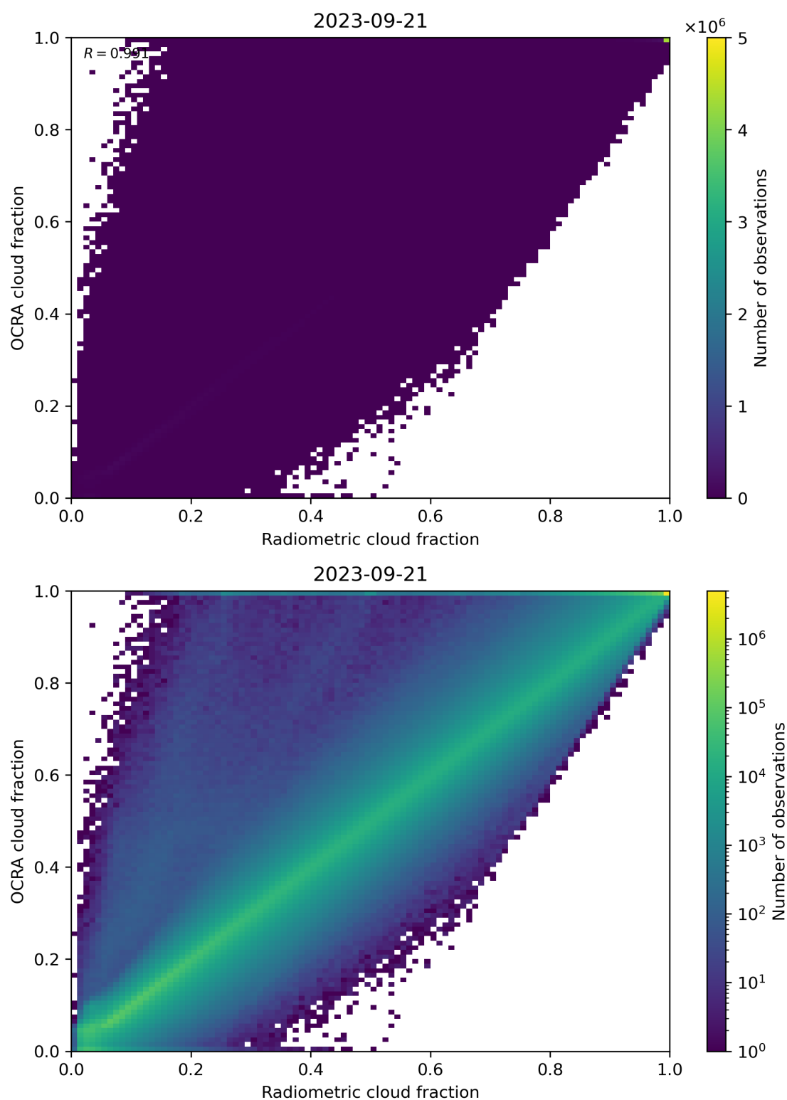
Figure 72: Scatter density plot of “Radiometric cloud fraction” against “OCRA cloud fraction” for 2023-09-20 to 2023-09-22.
