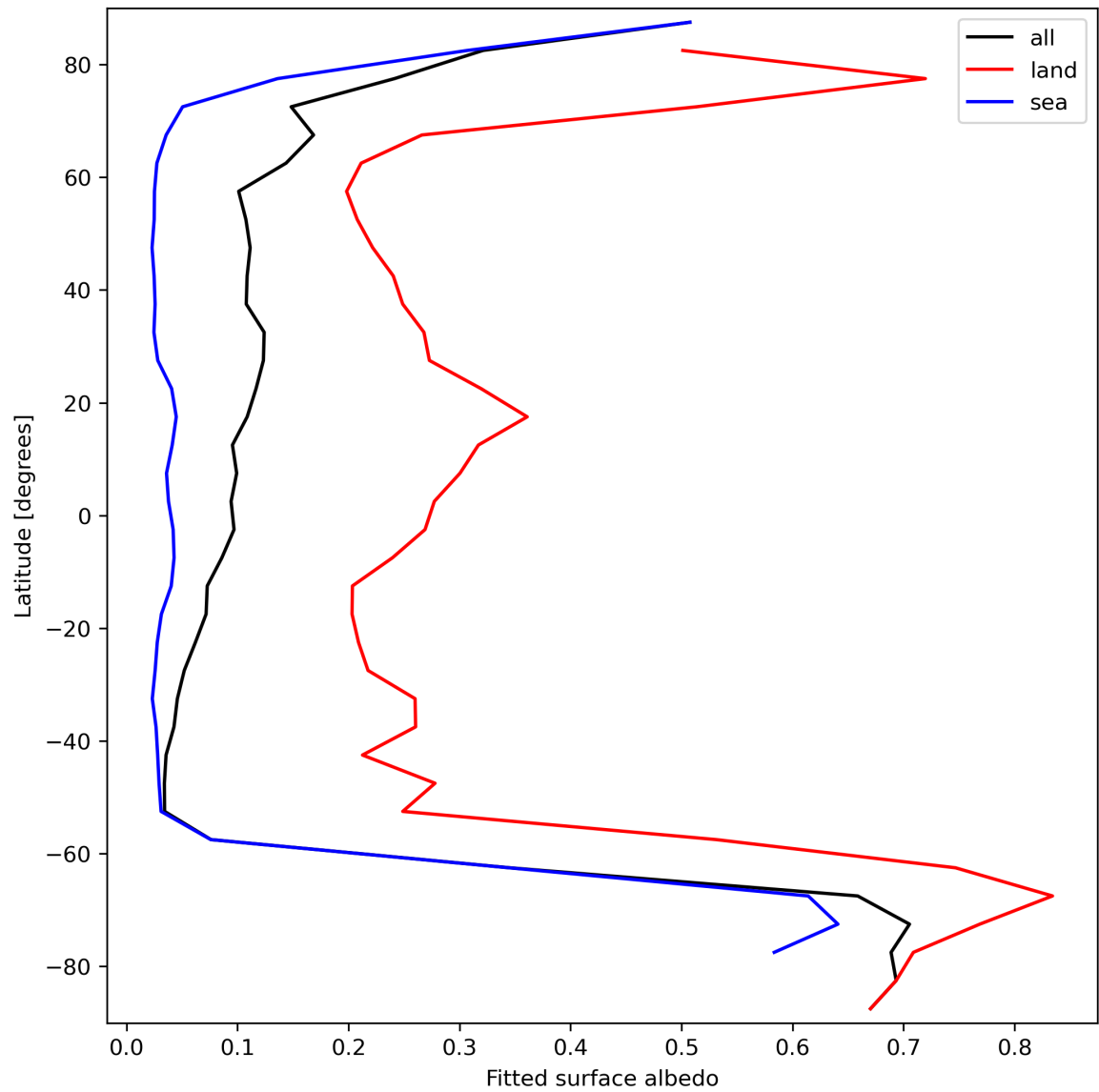
Figure 29: Zonal average of “Fitted surface albedo” for 2023-09-20 to 2023-09-22.
