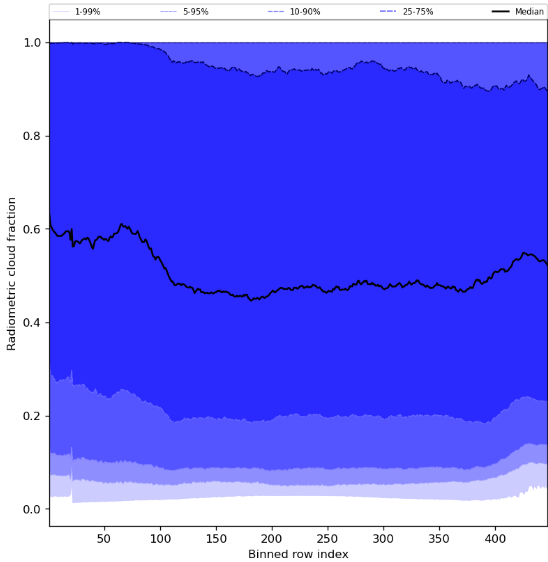
Figure 55: Along track statistics of “Radiometric cloud fraction” for 2023-09-20 to 2023-09-22
