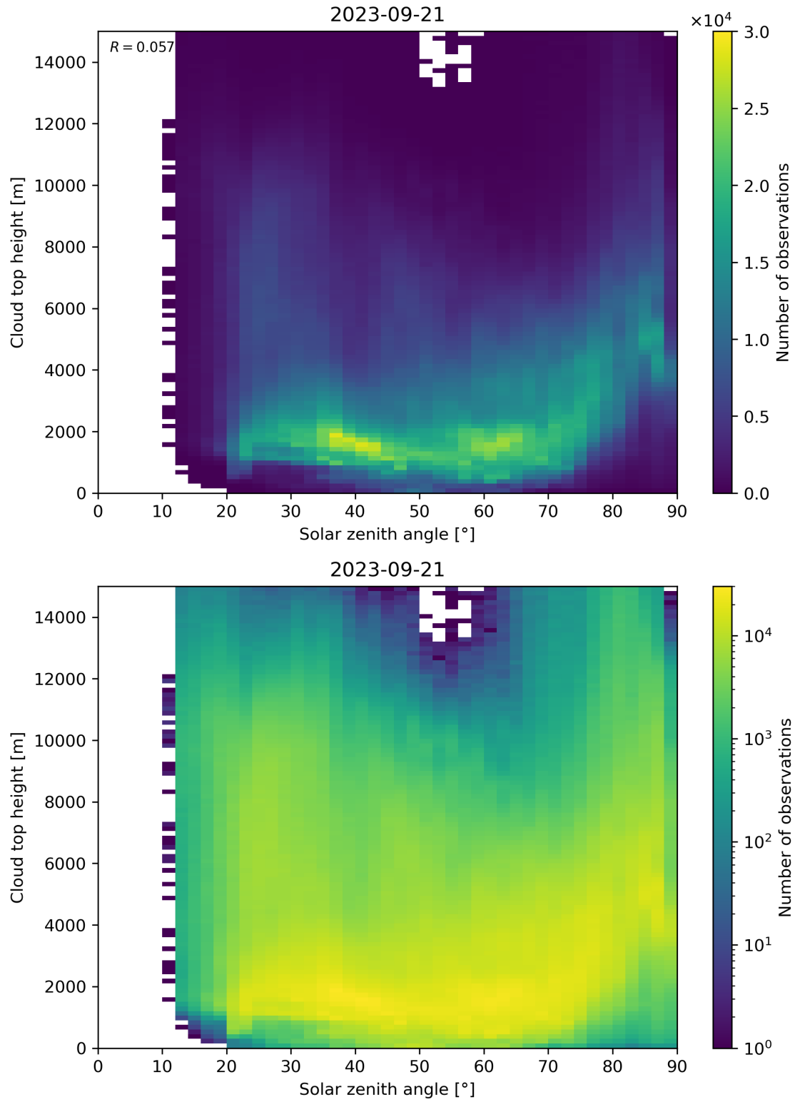
Figure 104: Scatter density plot of “Solar zenith angle” against “Cloud top height” for 2023-09-20 to 2023-09-22.
