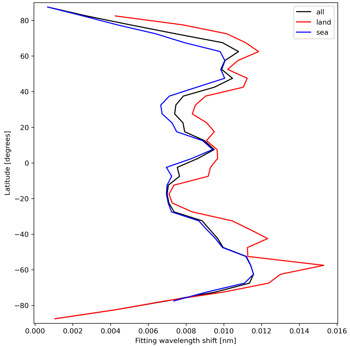
Figure 33: Zonal average of “Fitting wavelength shift” for 2023-09-20 to 2023-09-22.
