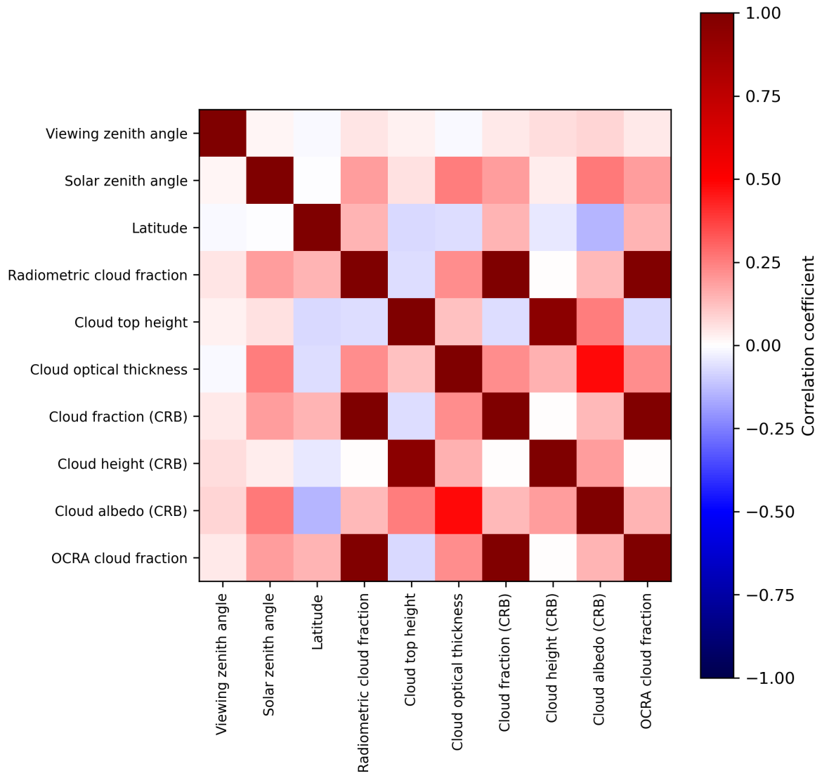
Figure 2: Map of correlation matrix for 2023-09-20 to 2023-09-22.
