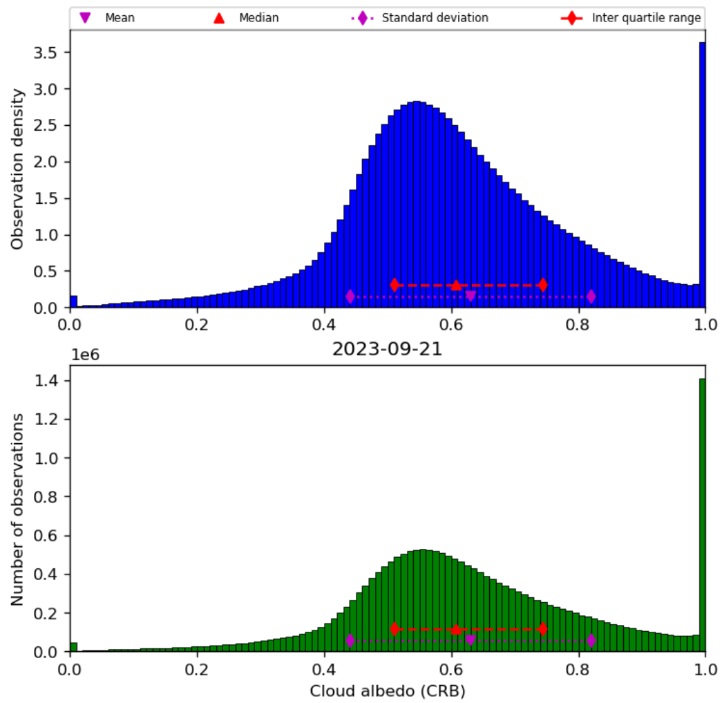
Figure 44: Histogram of “Cloud albedo (CRB)” for 2023-09-20 to 2023-09-22
