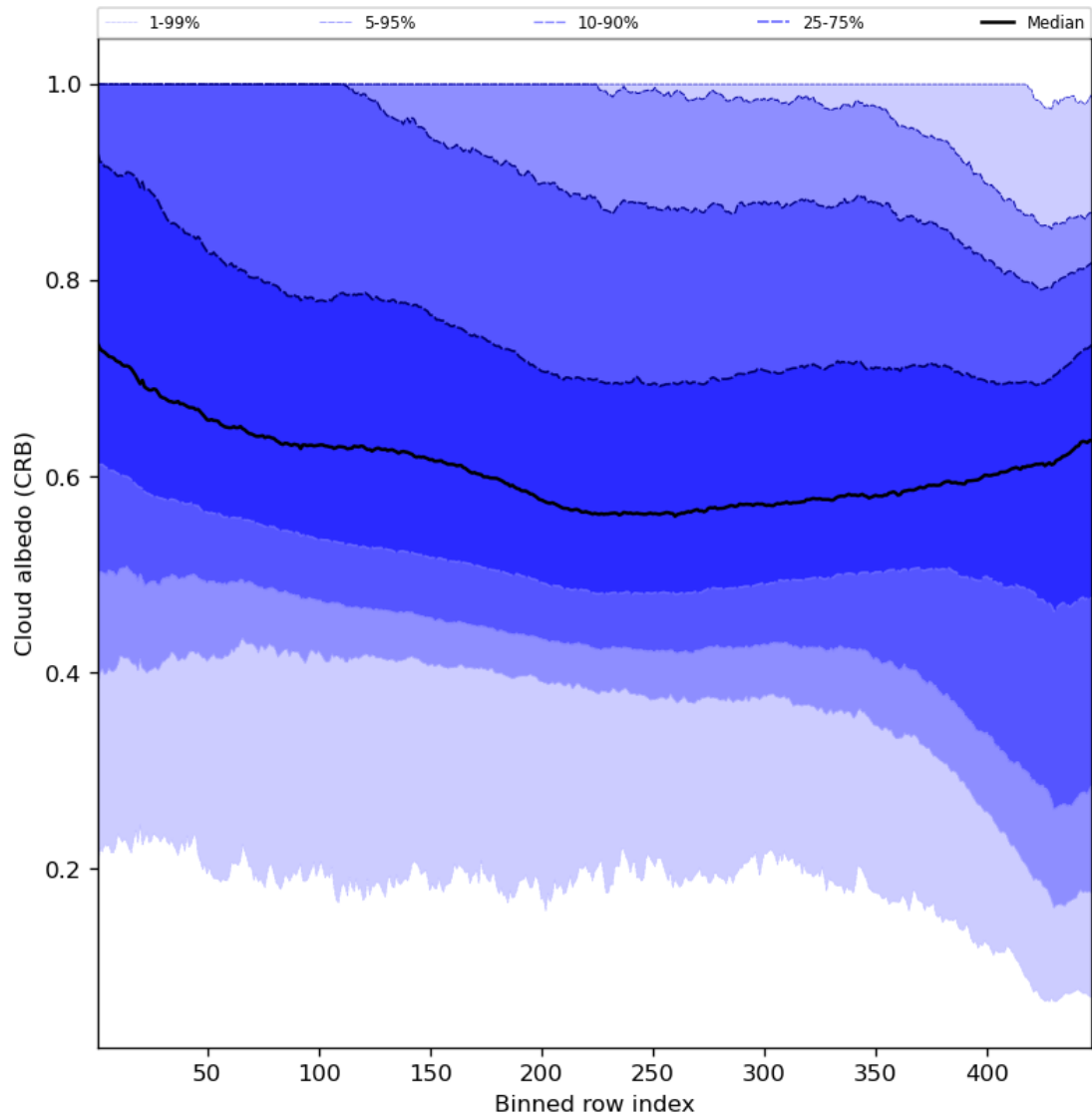
Figure 60: Along track statistics of “Cloud albedo (CRB)” for 2023-09-20 to 2023-09-22
