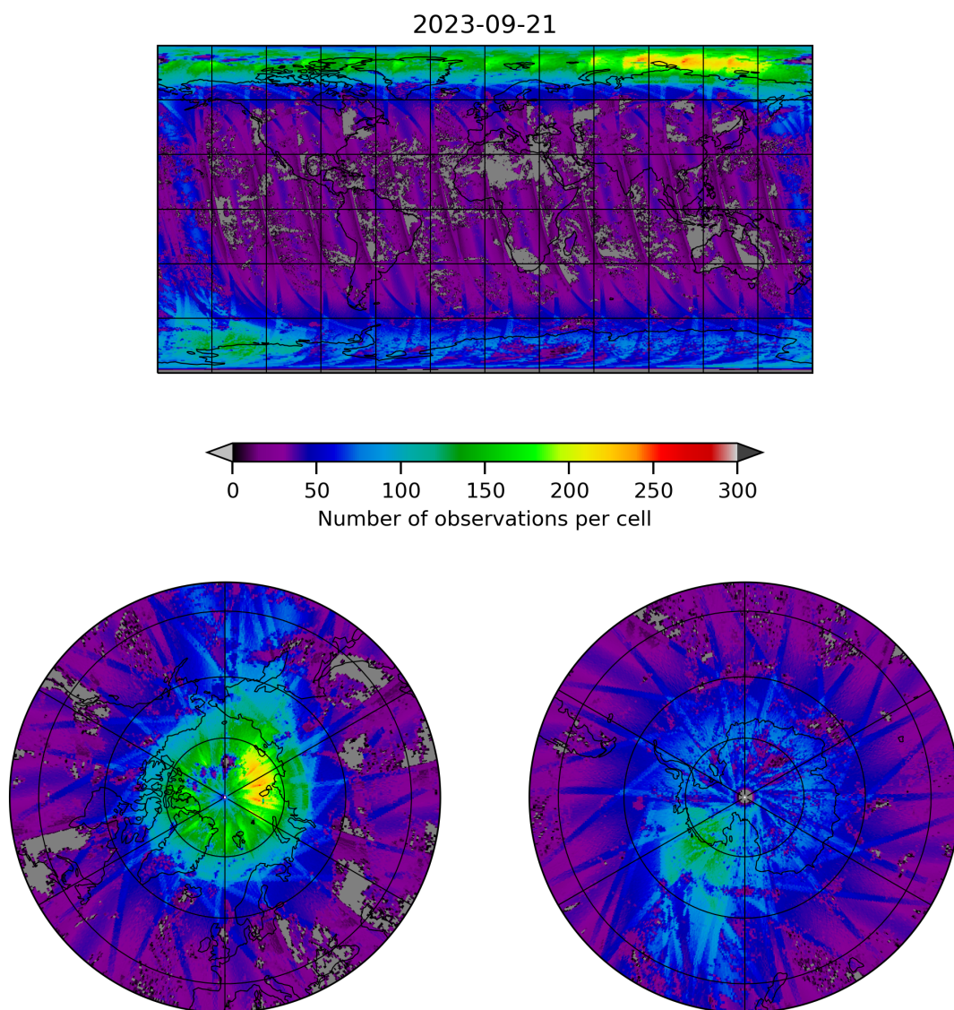
Figure 21: Map of the number of observations for 2023-09-20 to 2023-09-22
