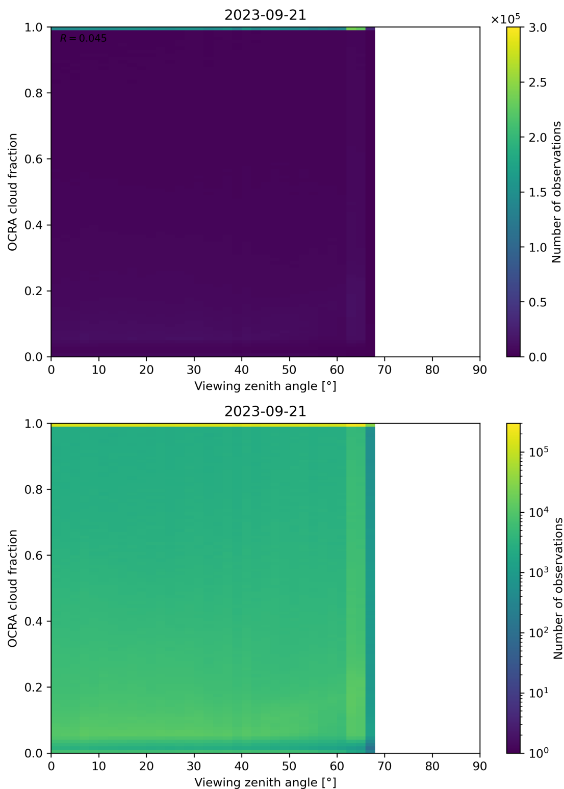
Figure 108: Scatter density plot of “Viewing zenith angle” against “OCRA cloud fraction” for 2023-09-20 to 2023-09-22.
