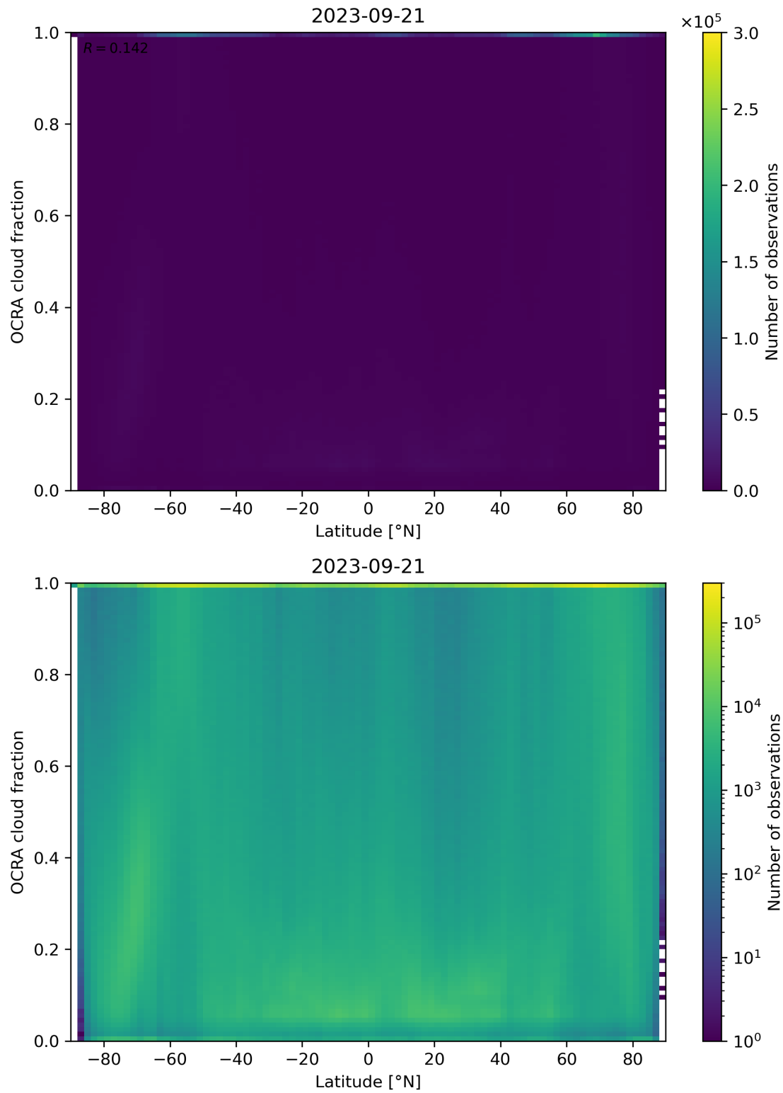
Figure 93: Scatter density plot of “Latitude” against “OCRA cloud fraction” for 2023-09-20 to 2023-09-22.
