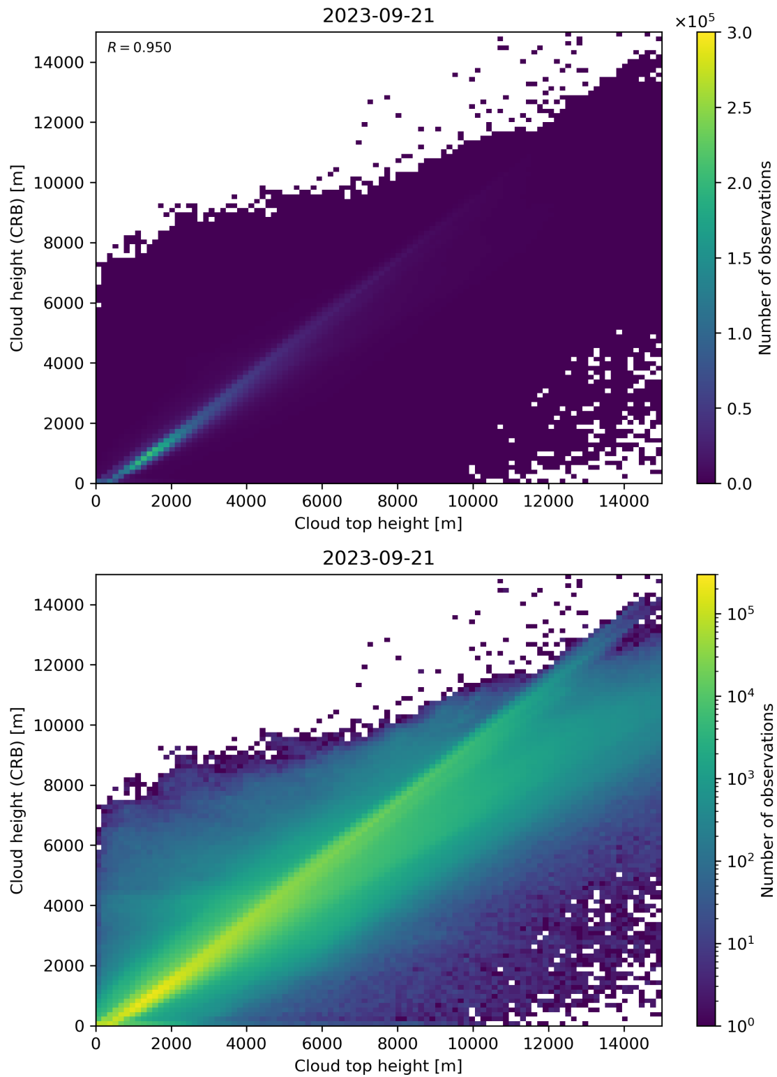
Figure 89: Scatter density plot of “Cloud top height” against “Cloud height (CRB)” for 2023-09-20 to 2023-09-22.
