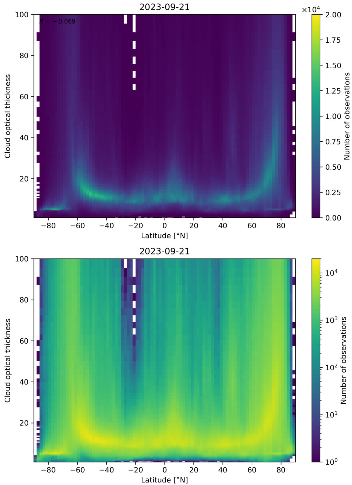
Figure 96: Scatter density plot of “Latitude” against “Cloud optical thickness” for 2023-09-20 to 2023-09-22.
