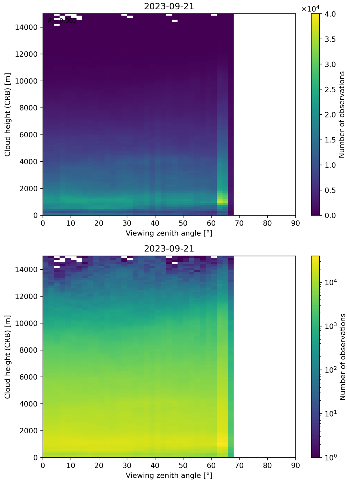
Figure 110: Scatter density plot of “Viewing zenith angle” against “Cloud height (CRB)” for 2023-09-20 to 2023-09-22.
