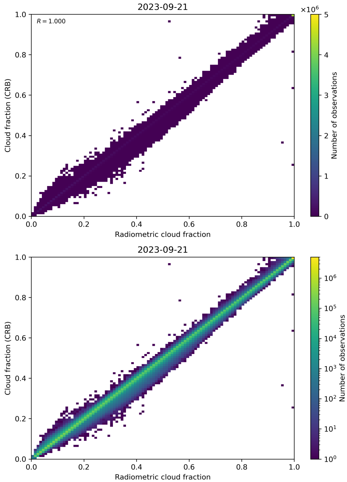
Figure 73: Scatter density plot of “Radiometric cloud fraction” against “Cloud fraction (CRB)” for 2023-09-20 to 2023-09-22.
