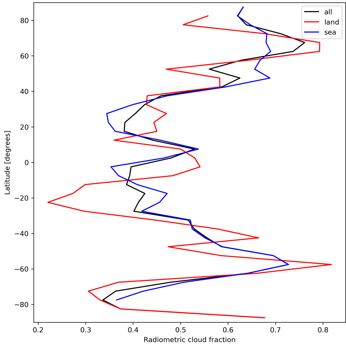
Figure 23: Zonal average of “Radiometric cloud fraction” for 2023-09-20 to 2023-09-22.
