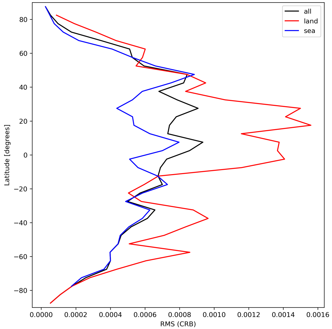
Figure 32: Zonal average of “RMS (CRB)” for 2023-09-20 to 2023-09-22.
