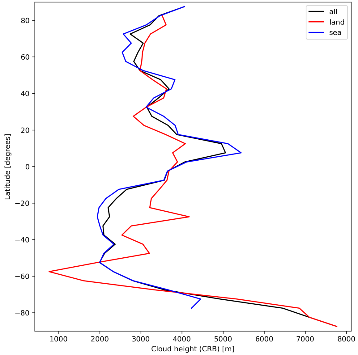
Figure 27: Zonal average of “Cloud height (CRB)” for 2023-09-20 to 2023-09-22.
