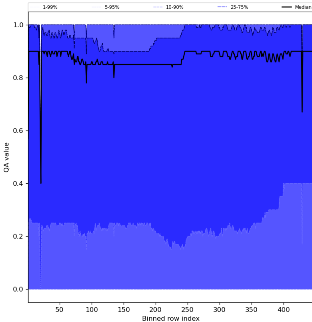
Figure 54: Along track statistics of “QA value” for 2023-09-20 to 2023-09-22
