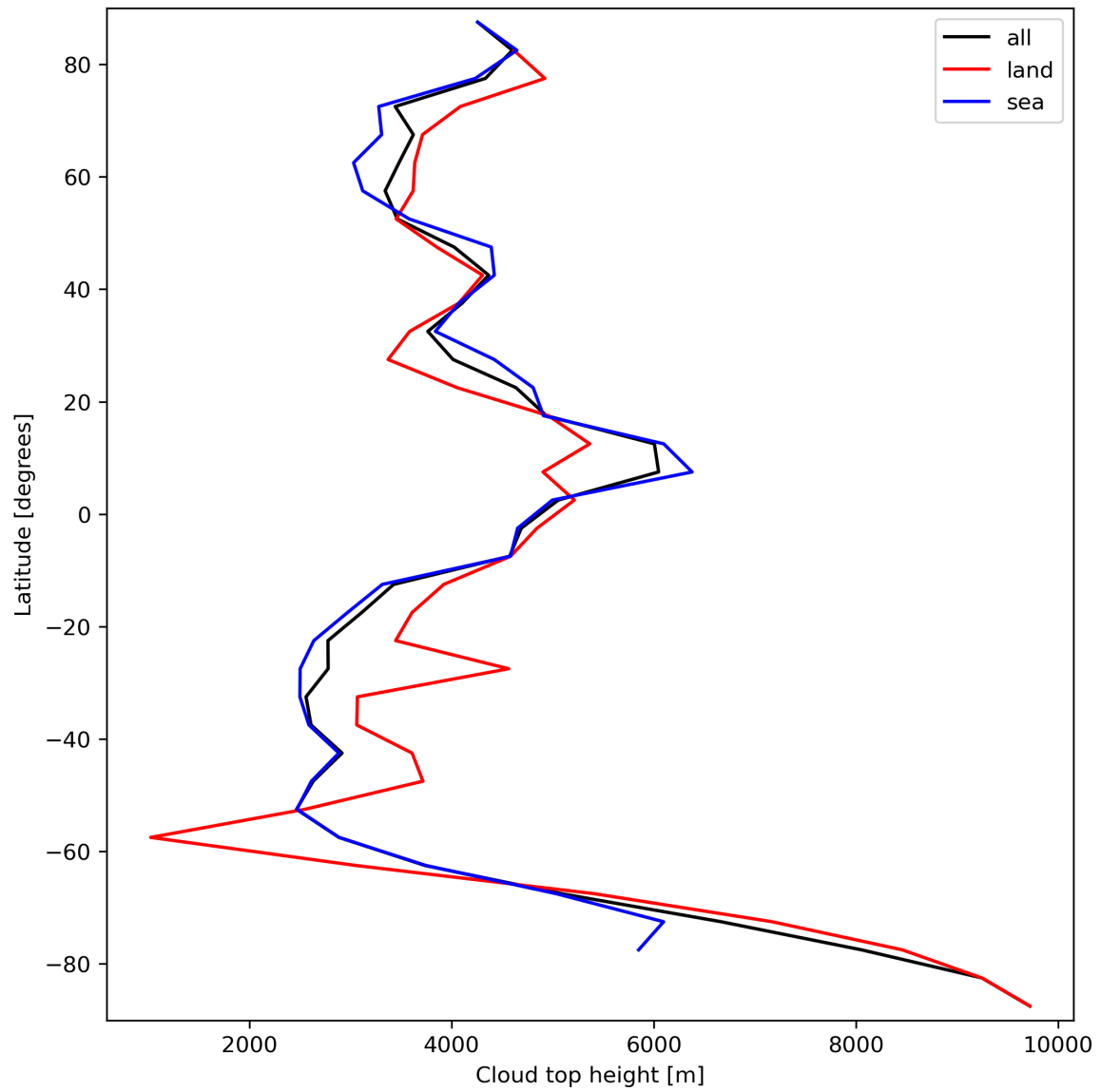
Figure 24: Zonal average of “Cloud top height” for 2023-09-20 to 2023-09-22.
