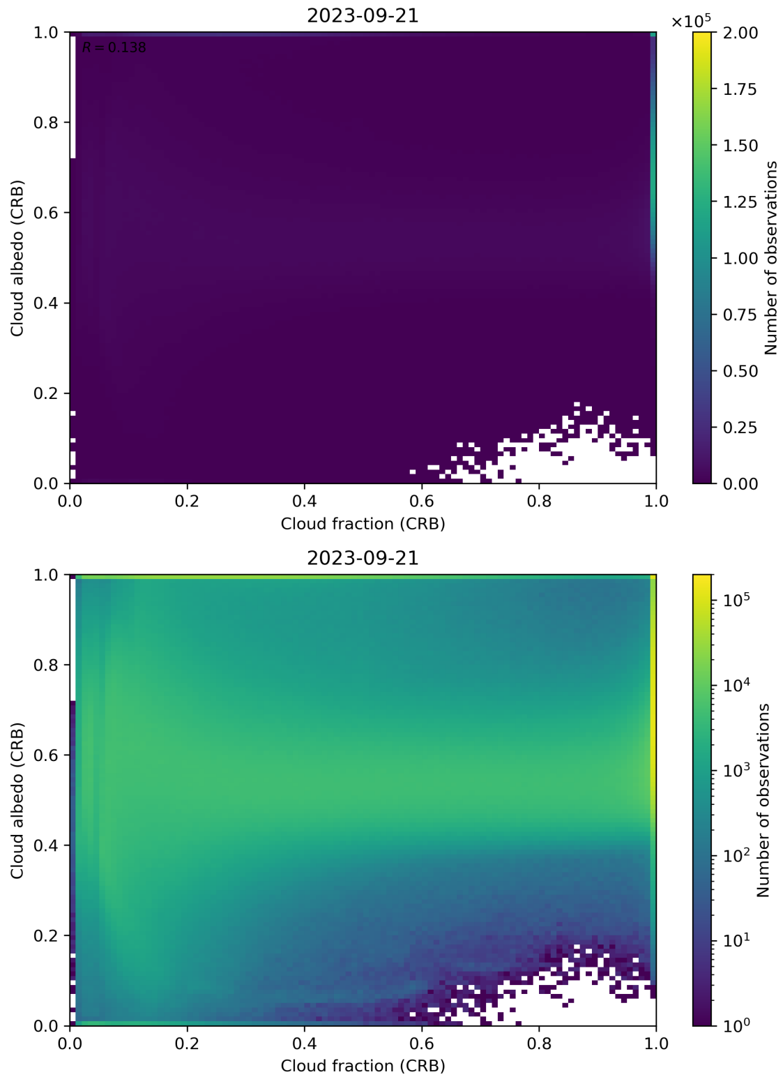
Figure 77: Scatter density plot of “Cloud fraction (CRB)” against “Cloud albedo (CRB)” for 2023-09-20 to 2023-09-22.
