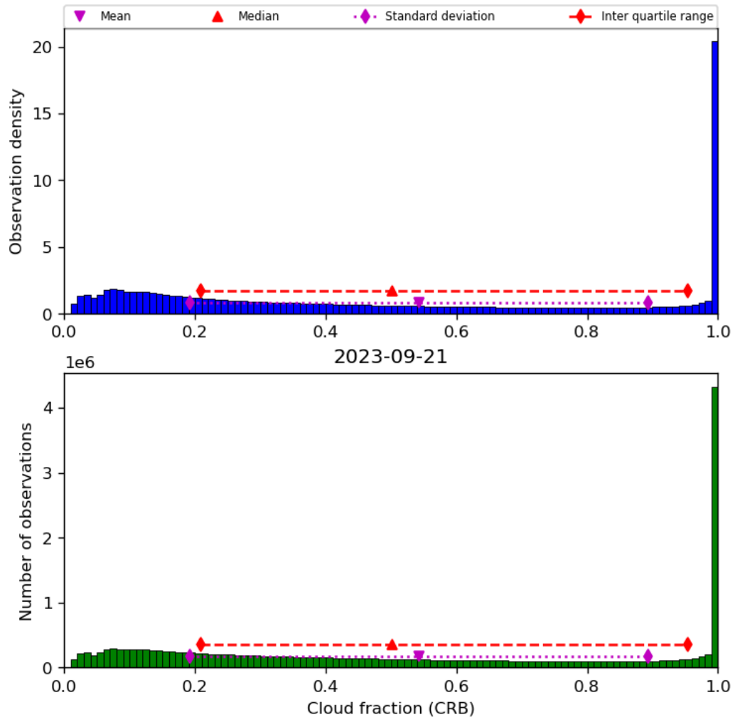
Figure 42: Histogram of “Cloud fraction (CRB)” for 2023-09-20 to 2023-09-22
