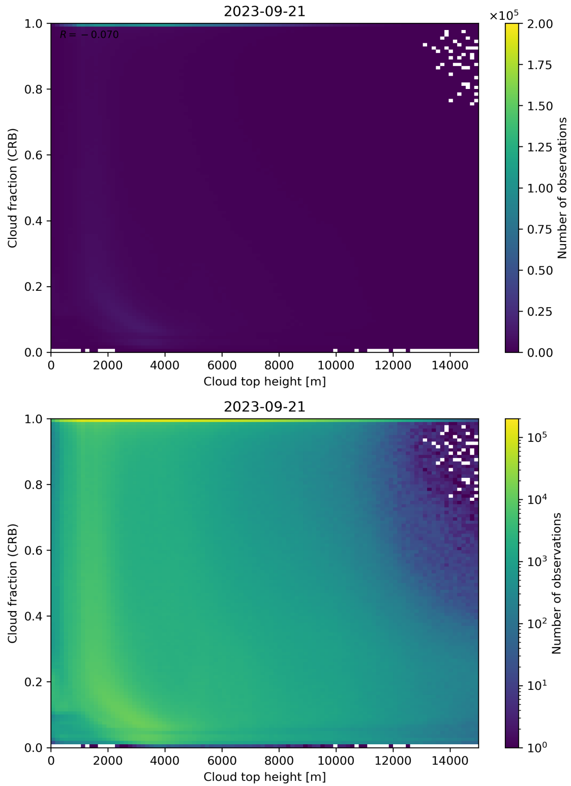
Figure 88: Scatter density plot of “Cloud top height” against “Cloud fraction (CRB)” for 2023-09-20 to 2023-09-22.
