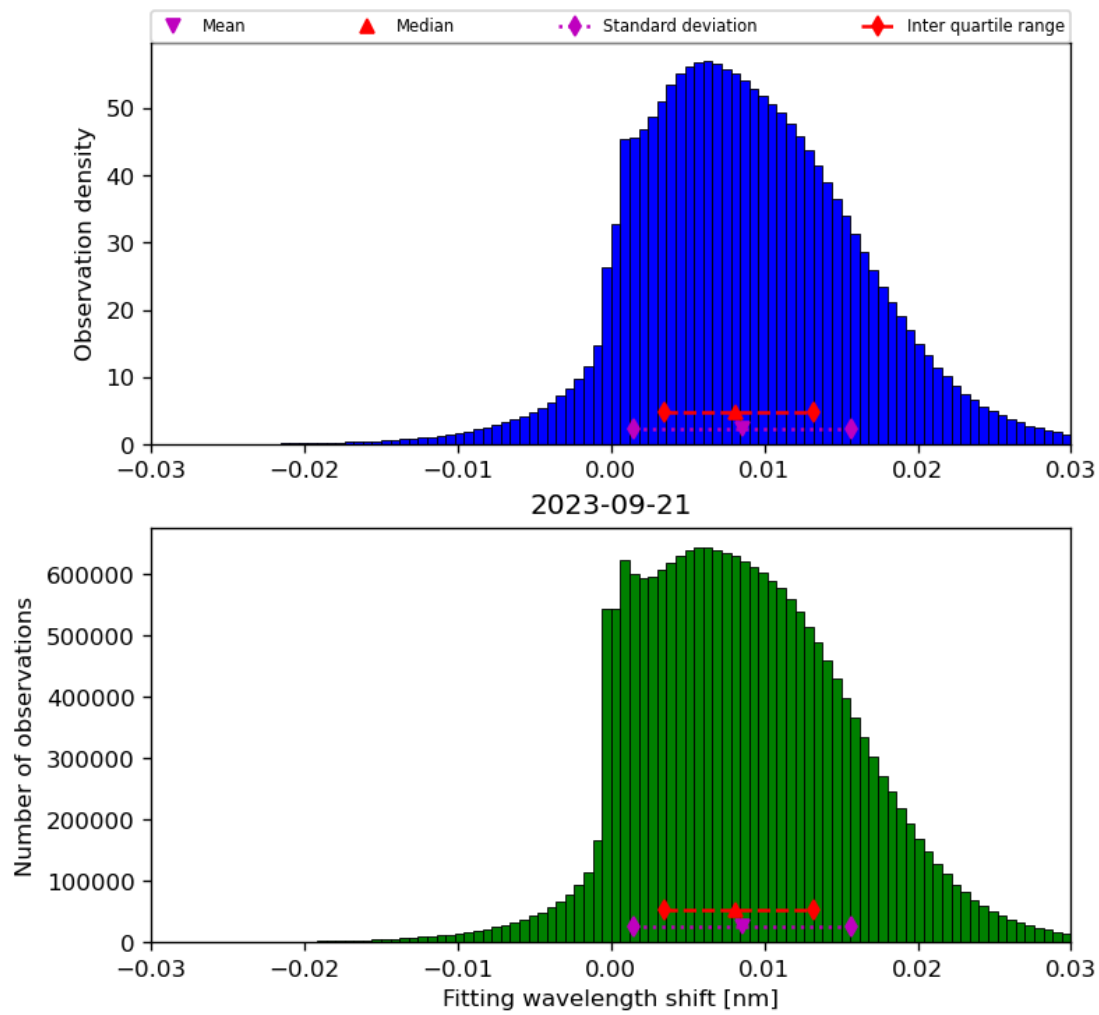
Figure 49: Histogram of “Fitting wavelength shift” for 2023-09-20 to 2023-09-22
