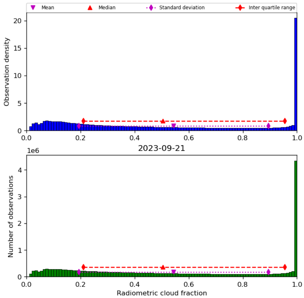
Figure 39: Histogram of “Radiometric cloud fraction” for 2023-09-20 to 2023-09-22
