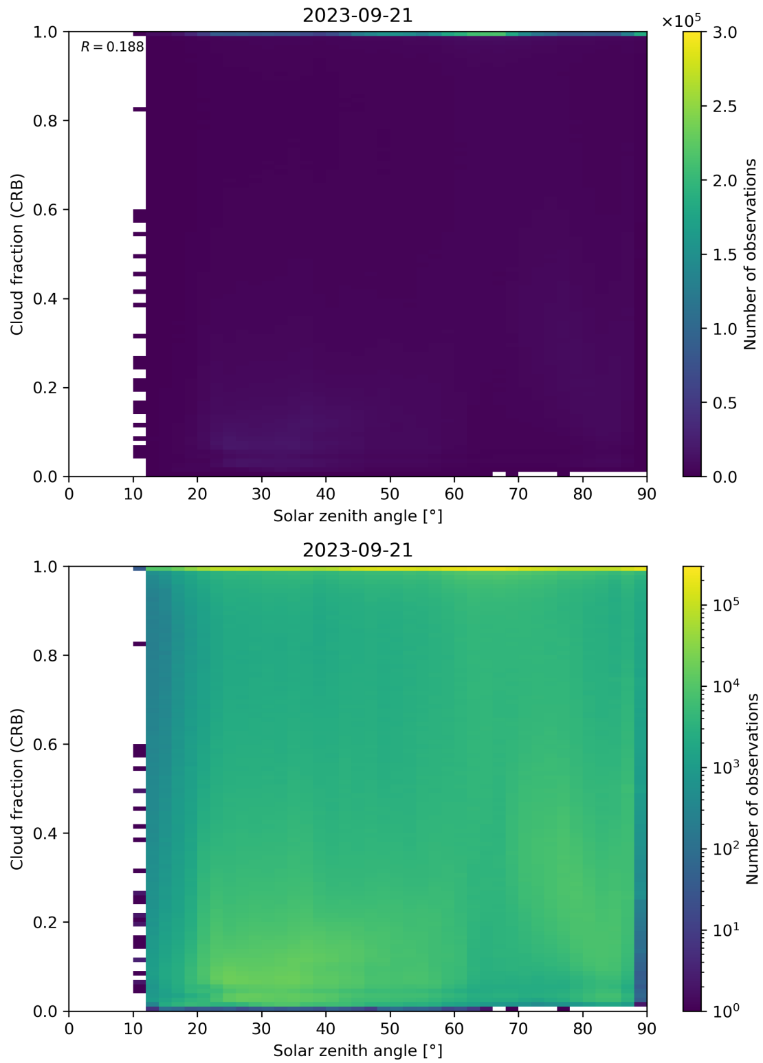
Figure 101: Scatter density plot of “Solar zenith angle” against “Cloud fraction (CRB)” for 2023-09-20 to 2023-09-22.
