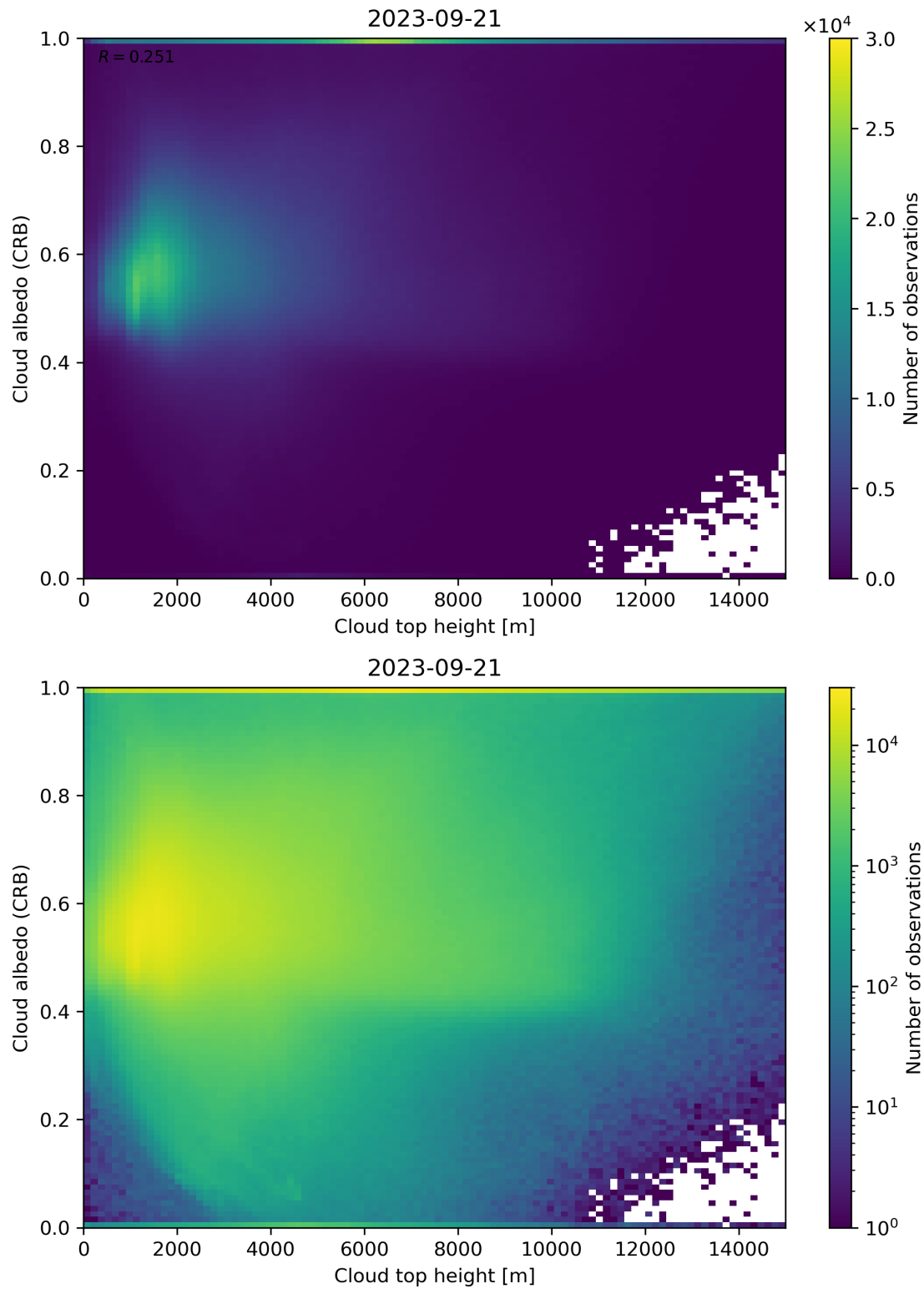
Figure 86: Scatter density plot of “Cloud top height” against “Cloud albedo (CRB)” for 2023-09-20 to 2023-09-22.
