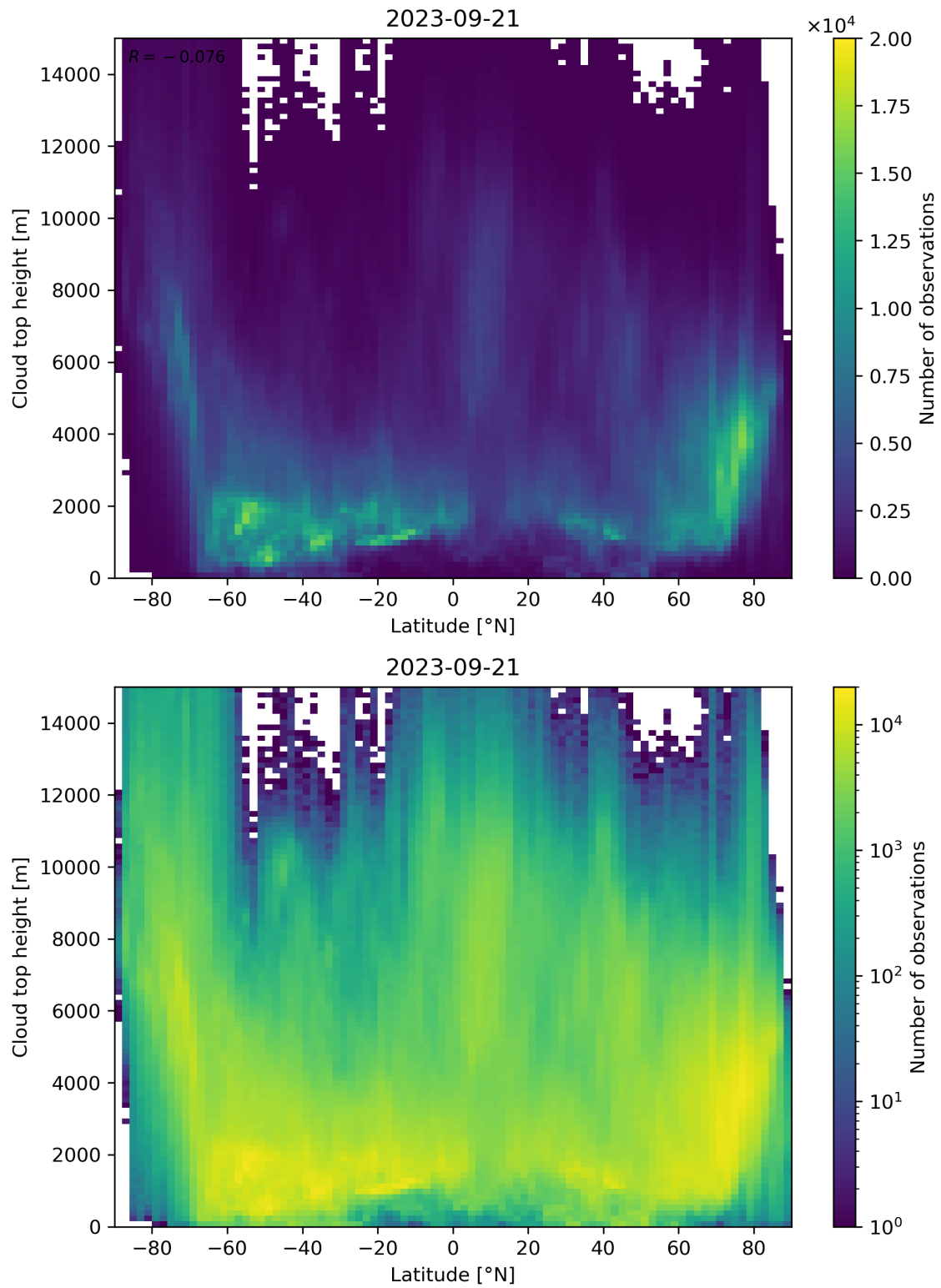
Figure 97: Scatter density plot of “Latitude” against “Cloud top height” for 2023-09-20 to 2023-09-22.
