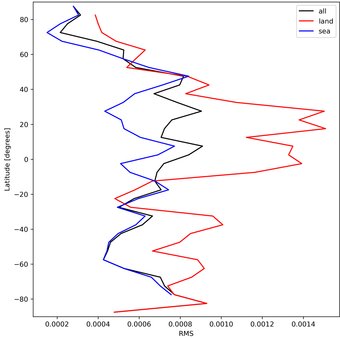
Figure 31: Zonal average of “RMS” for 2023-09-20 to 2023-09-22.
