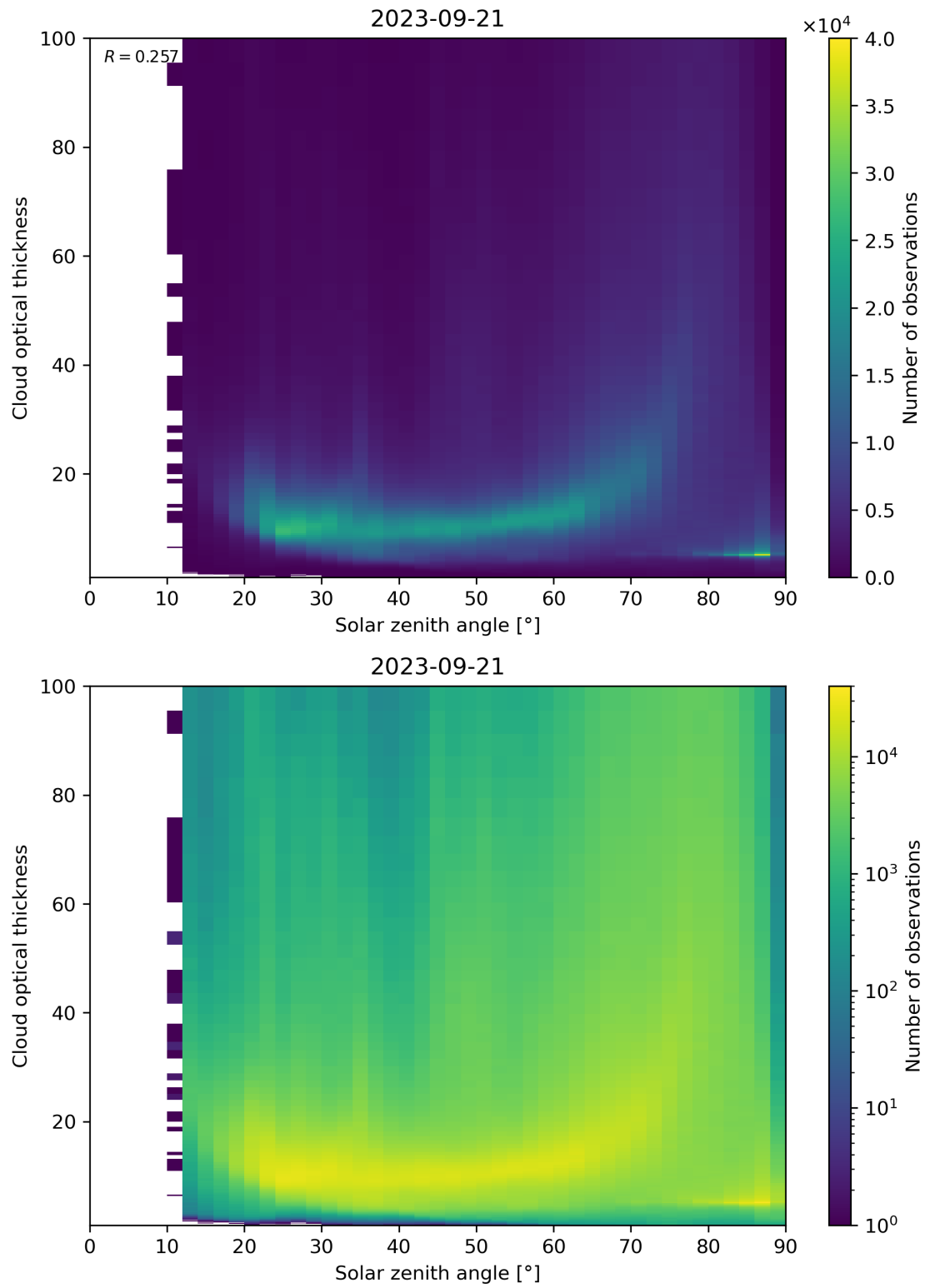
Figure 103: Scatter density plot of “Solar zenith angle” against “Cloud optical thickness” for 2023-09-20 to 2023-09-22.
