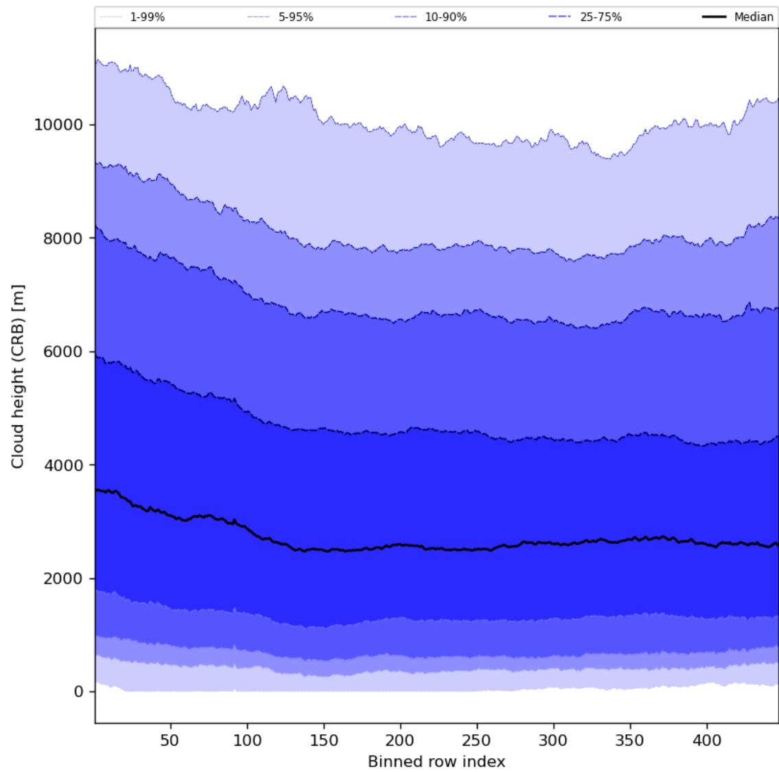
Figure 59: Along track statistics of “Cloud height (CRB)” for 2023-09-20 to 2023-09-22
