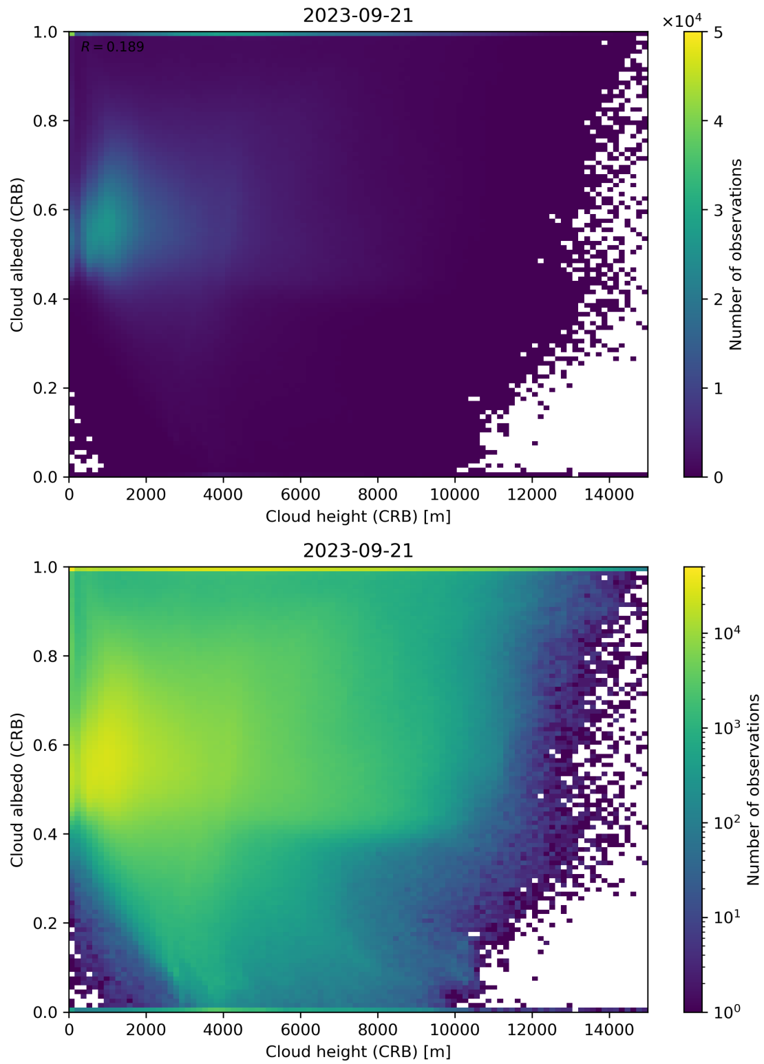
Figure 80: Scatter density plot of “Cloud height (CRB)” against “Cloud albedo (CRB)” for 2023-09-20 to 2023-09-22.
