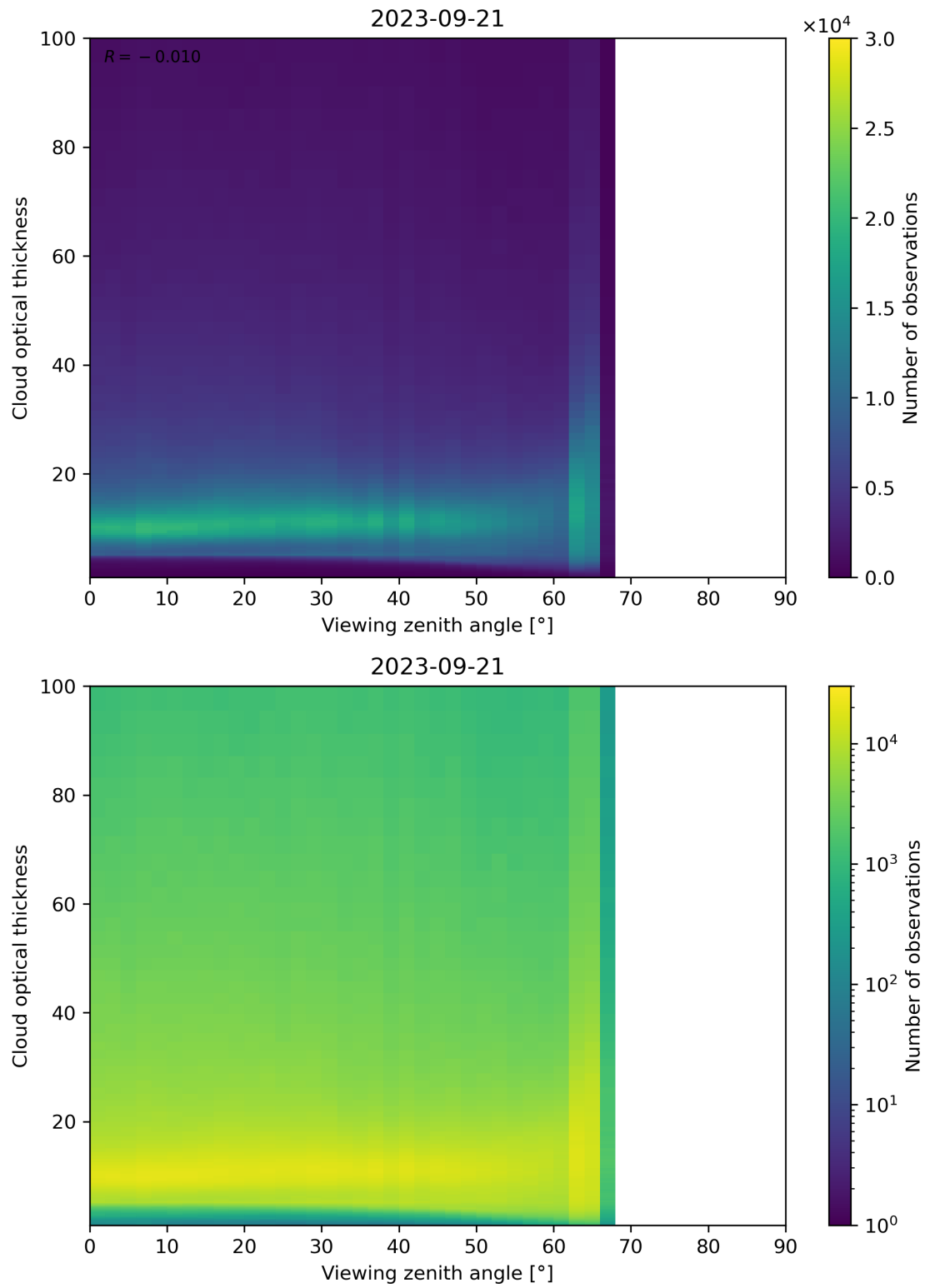
Figure 111: Scatter density plot of “Viewing zenith angle” against “Cloud optical thickness” for 2023-09-20 to 2023-09-22.
