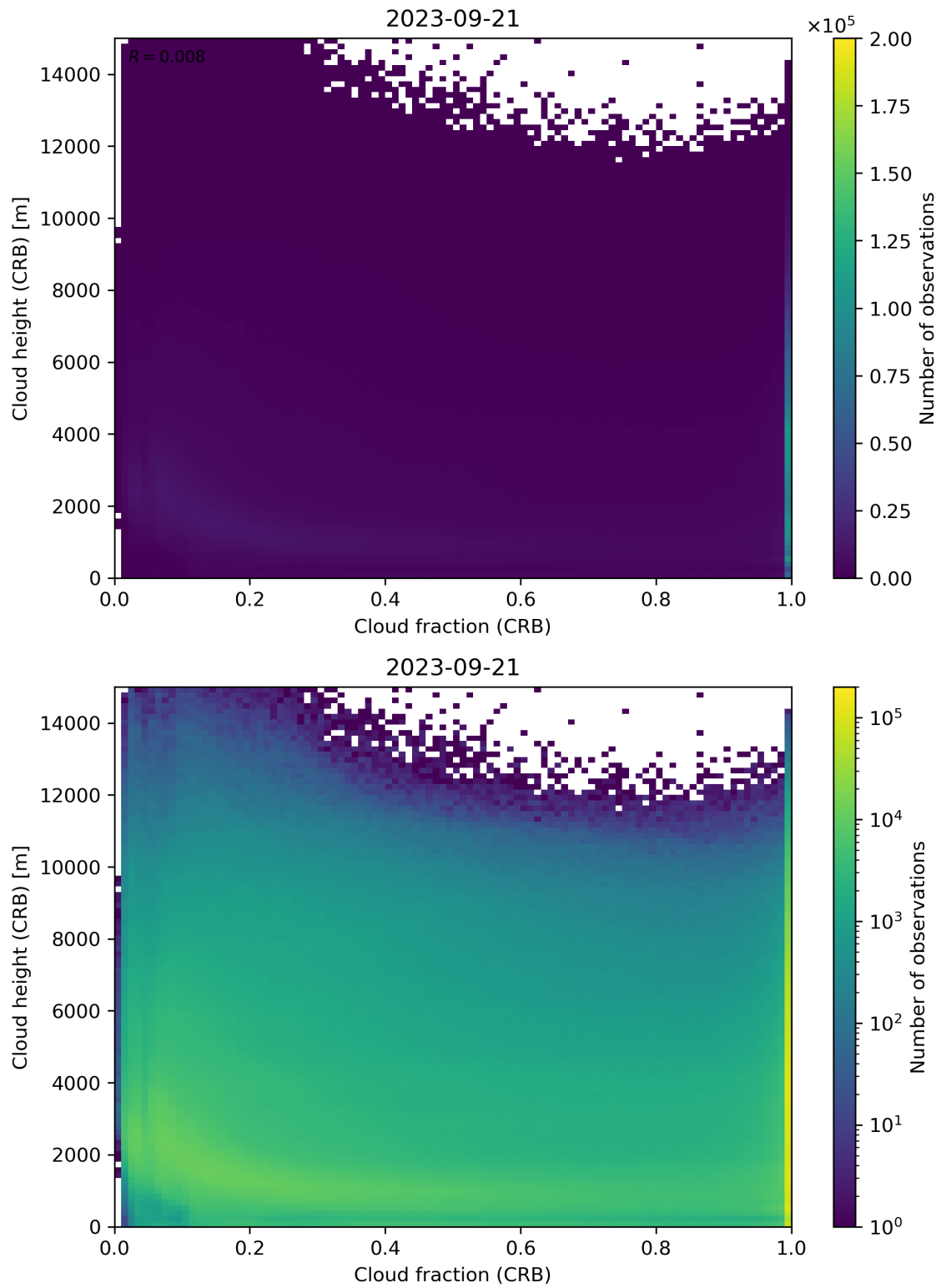
Figure 79: Scatter density plot of “Cloud fraction (CRB)” against “Cloud height (CRB)” for 2023-09-20 to 2023-09-22.
