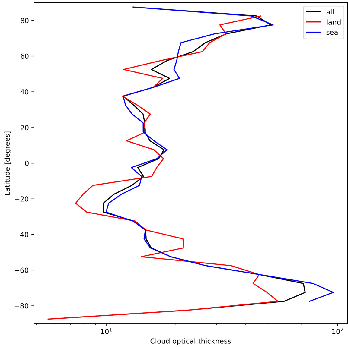
Figure 25: Zonal average of “Cloud optical thickness” for 2023-09-20 to 2023-09-22.
