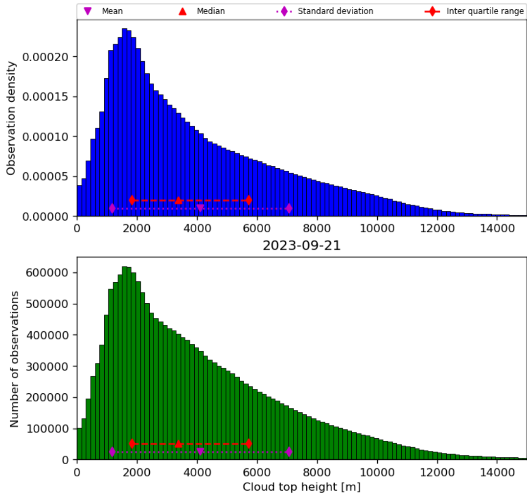
Figure 40: Histogram of “Cloud top height” for 2023-09-20 to 2023-09-22
