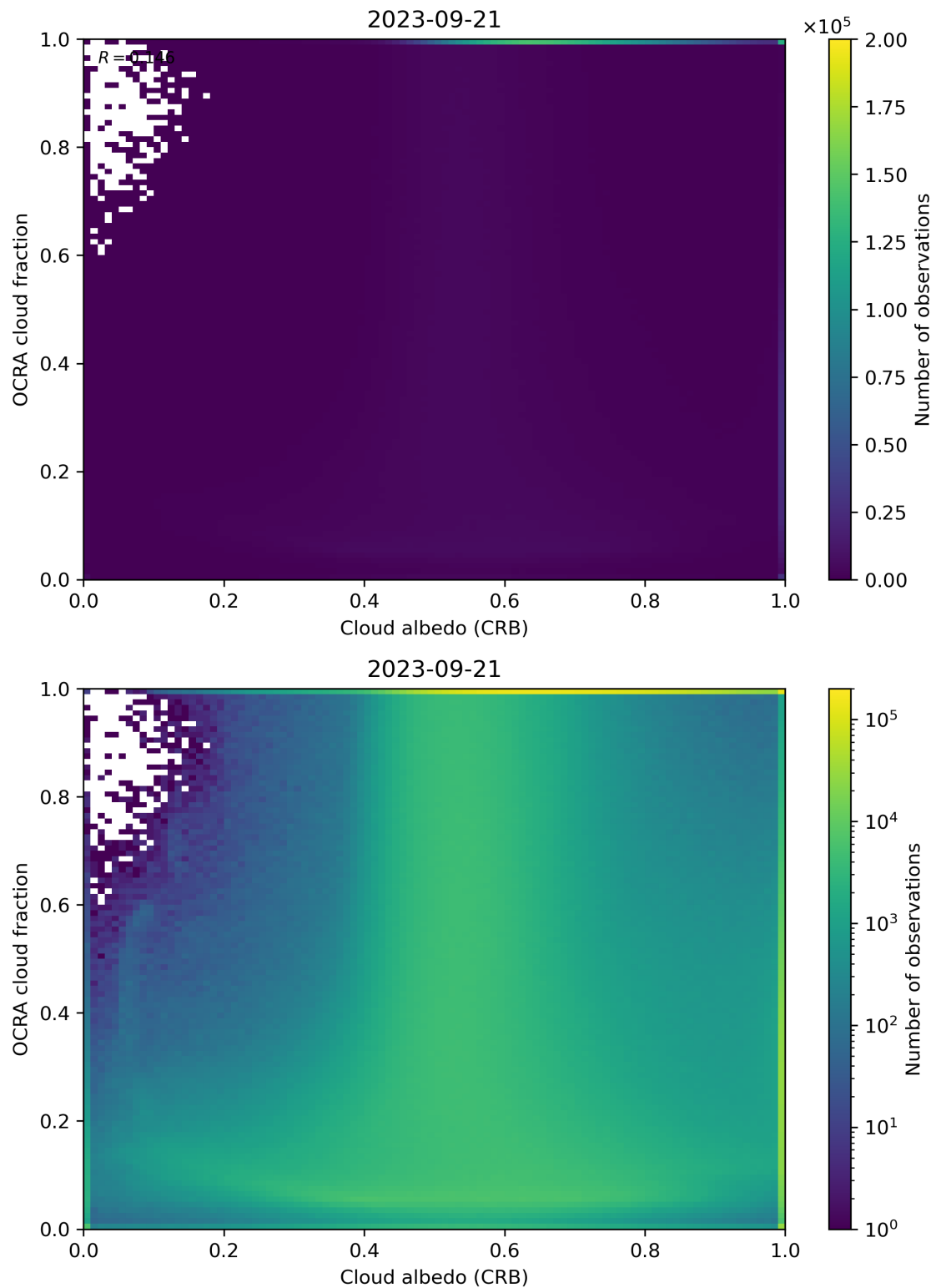
Figure 70: Scatter density plot of “Cloud albedo (CRB)” against “OCRA cloud fraction” for 2023-09-20 to 2023-09-22.
