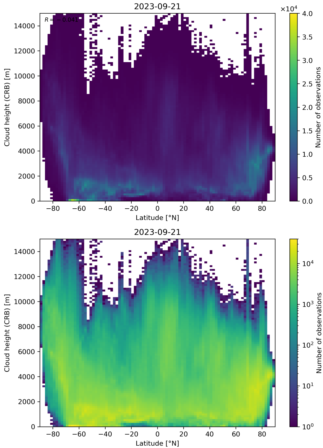
Figure 95: Scatter density plot of “Latitude” against “Cloud height (CRB)” for 2023-09-20 to 2023-09-22.
