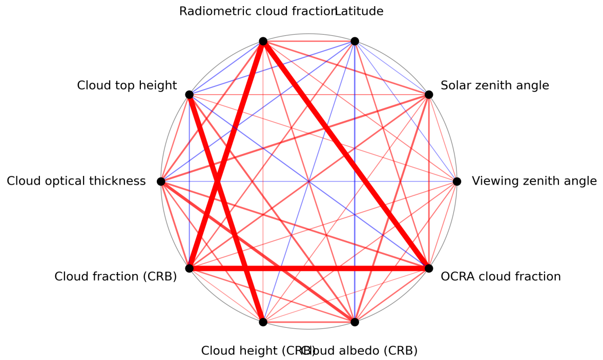
Figure 1: Map of correlation graph for 2023-09-20 to 2023-09-22.
