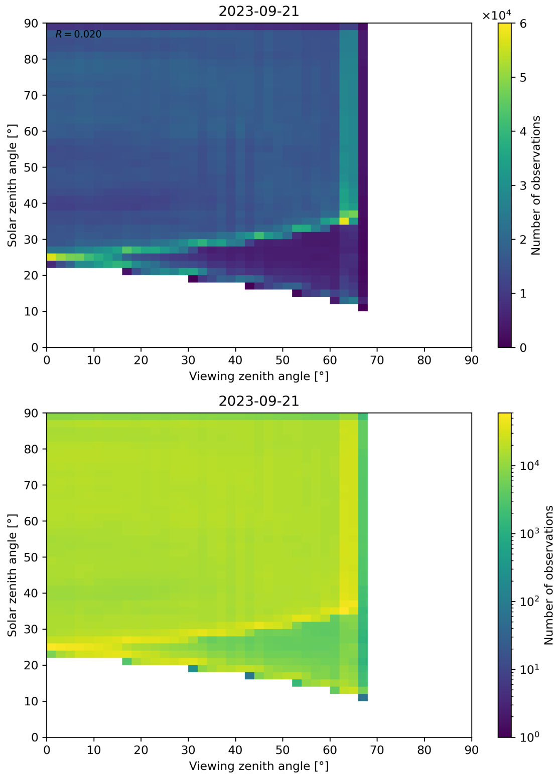
Figure 114: Scatter density plot of “Viewing zenith angle” against “Solar zenith angle” for 2023-09-20 to 2023-09-22.
