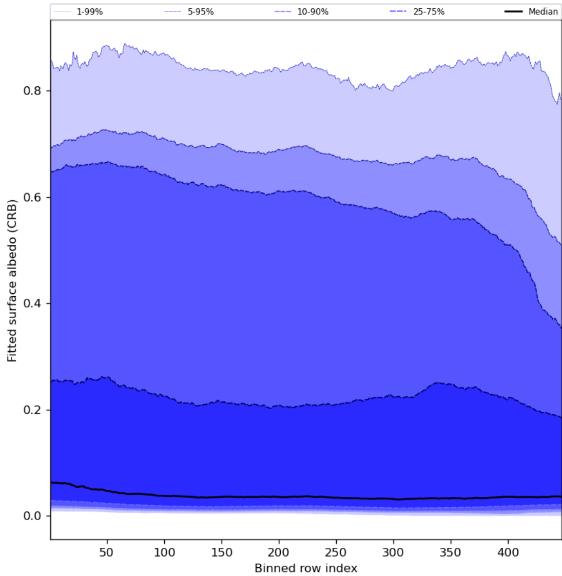
Figure 62: Along track statistics of “Fitted surface albedo (CRB)” for 2023-09-20 to 2023-09-22
