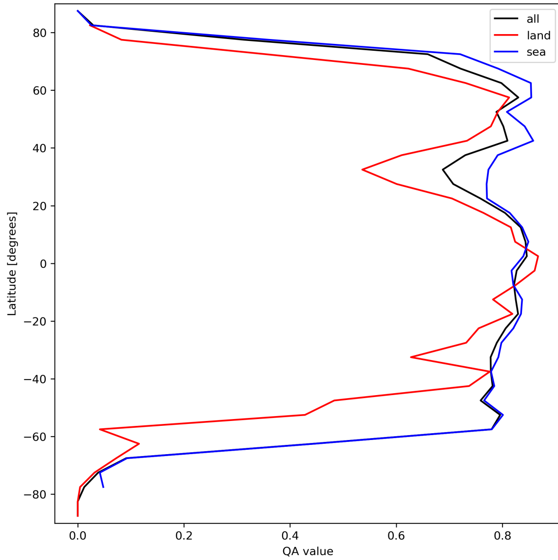
Figure 22: Zonal average of “QA value” for 2023-09-20 to 2023-09-22.
