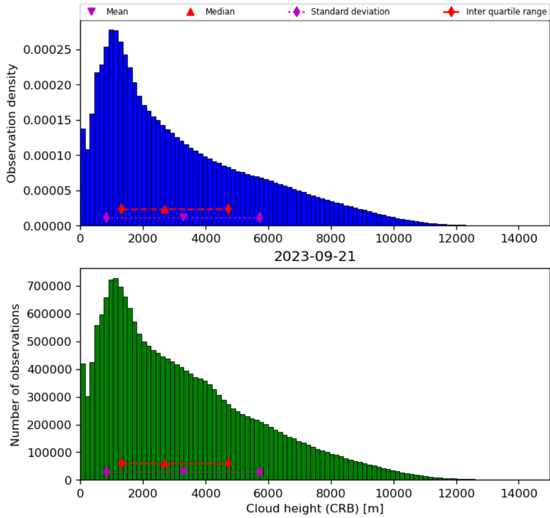
Figure 43: Histogram of “Cloud height (CRB)” for 2023-09-20 to 2023-09-22
