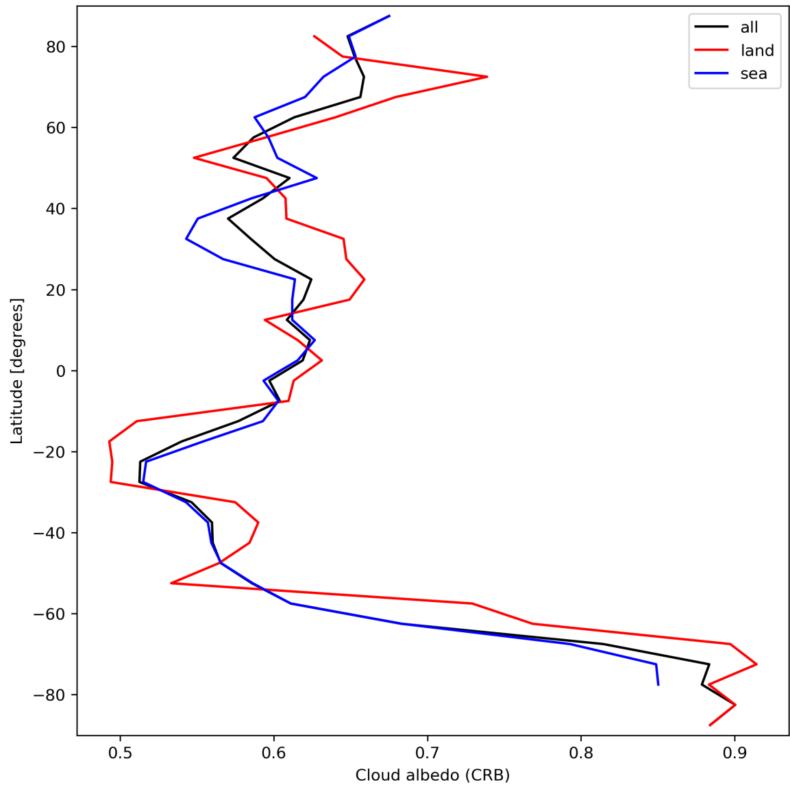
Figure 28: Zonal average of “Cloud albedo (CRB)” for 2023-09-20 to 2023-09-22.
