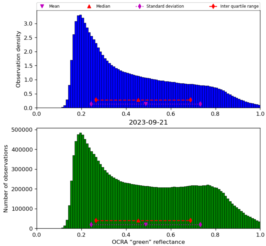
Figure 52: Histogram of “OCRA “green” reflectance” for 2023-09-20 to 2023-09-22
