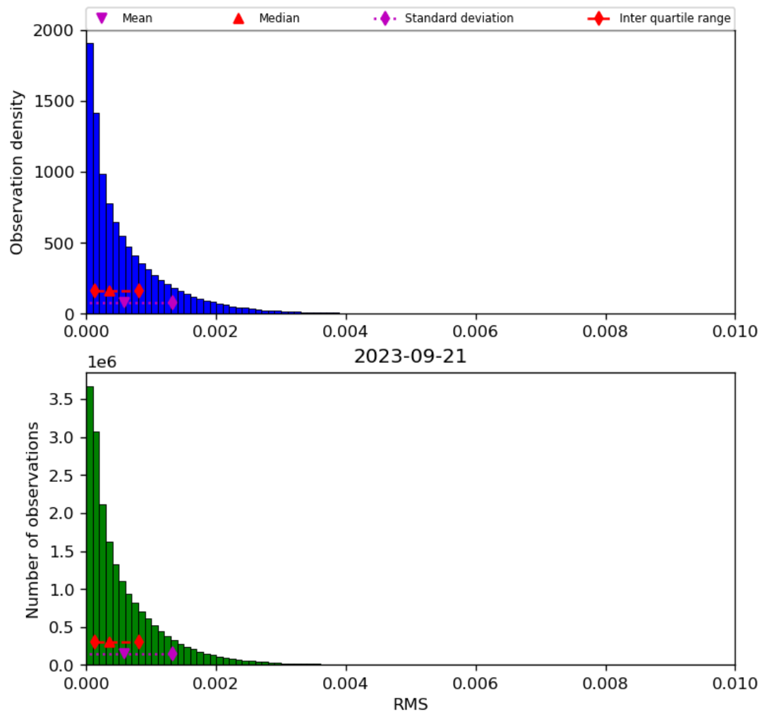
Figure 47: Histogram of “RMS” for 2023-09-20 to 2023-09-22
