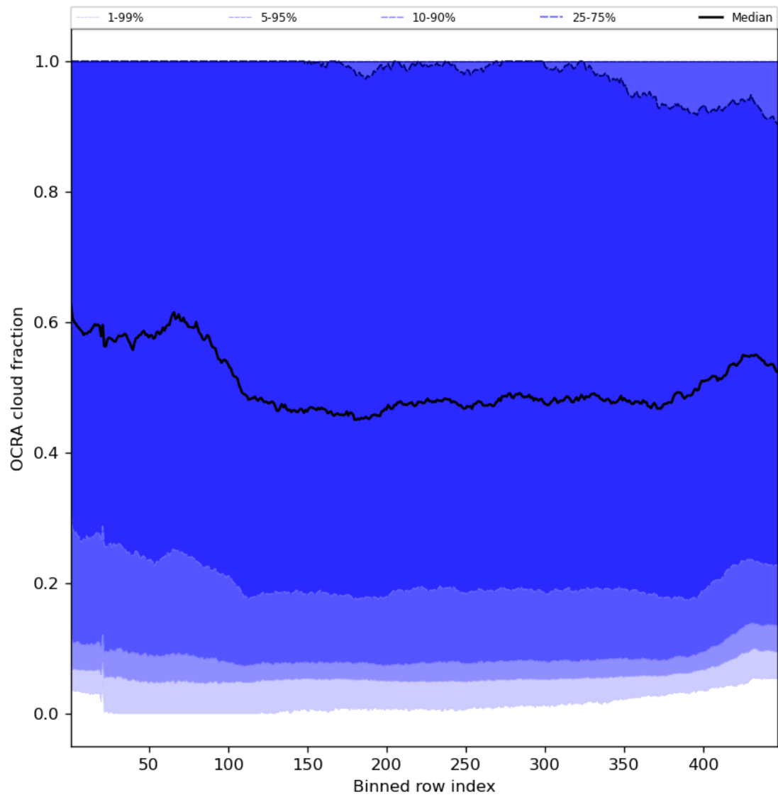
Figure 66: Along track statistics of “OCRA cloud fraction” for 2023-09-20 to 2023-09-22
