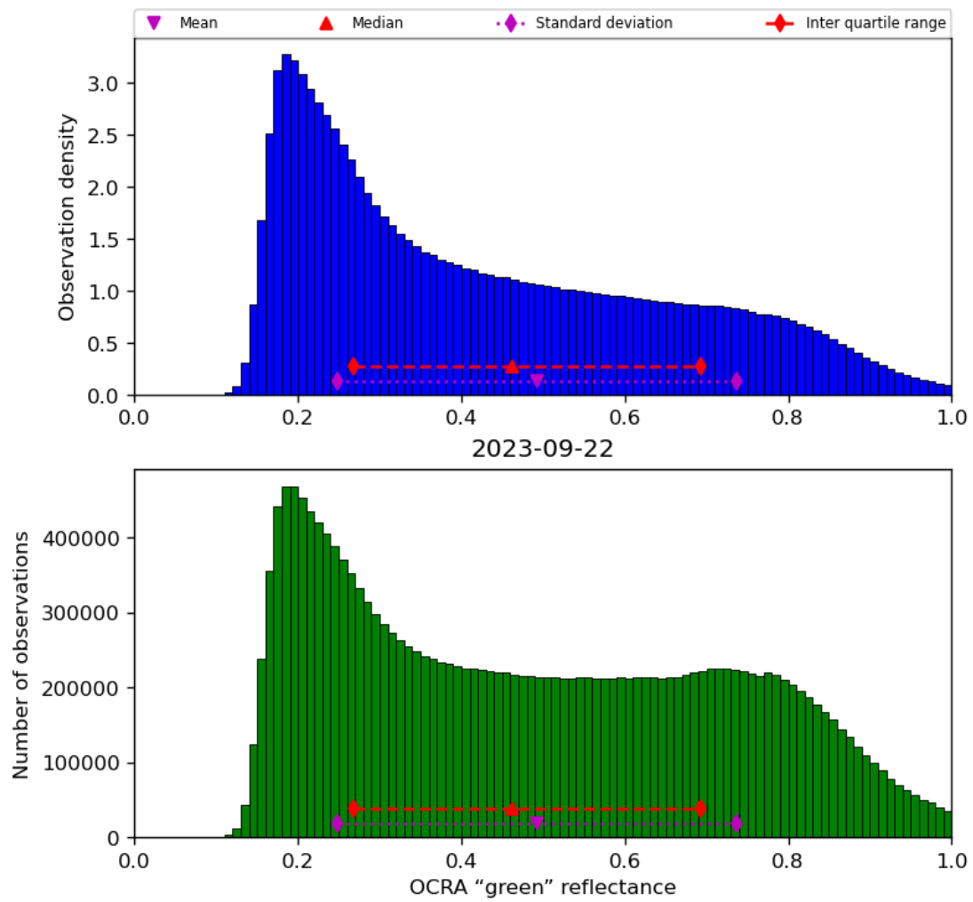
Figure 52: Histogram of “OCRA “green” reflectance” for 2023-09-21 to 2023-09-23
