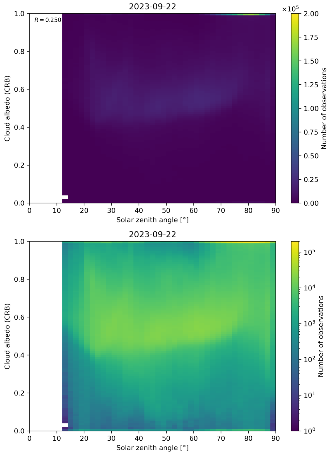
Figure 98: Scatter density plot of “Solar zenith angle” against “Cloud albedo (CRB)” for 2023-09-21 to 2023-09-23.
