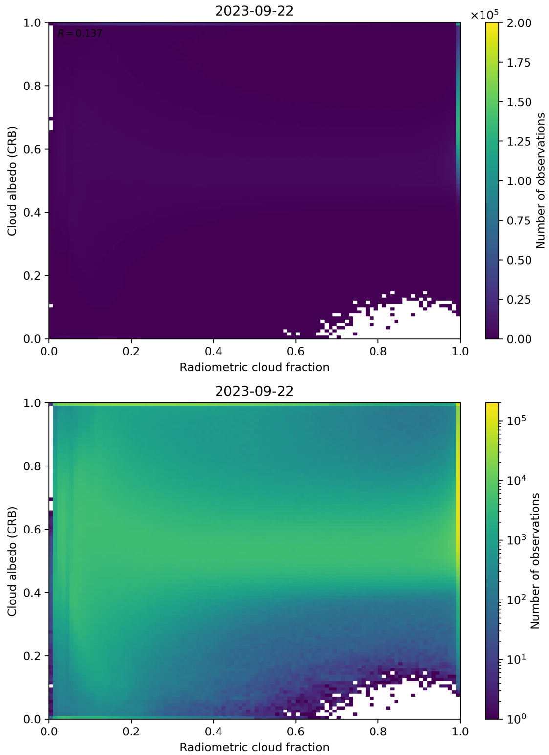
Figure 71: Scatter density plot of “Radiometric cloud fraction” against “Cloud albedo (CRB)” for 2023-09-21 to 2023-09-23.
