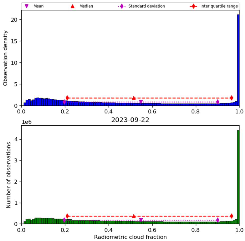
Figure 39: Histogram of “Radiometric cloud fraction” for 2023-09-21 to 2023-09-23
