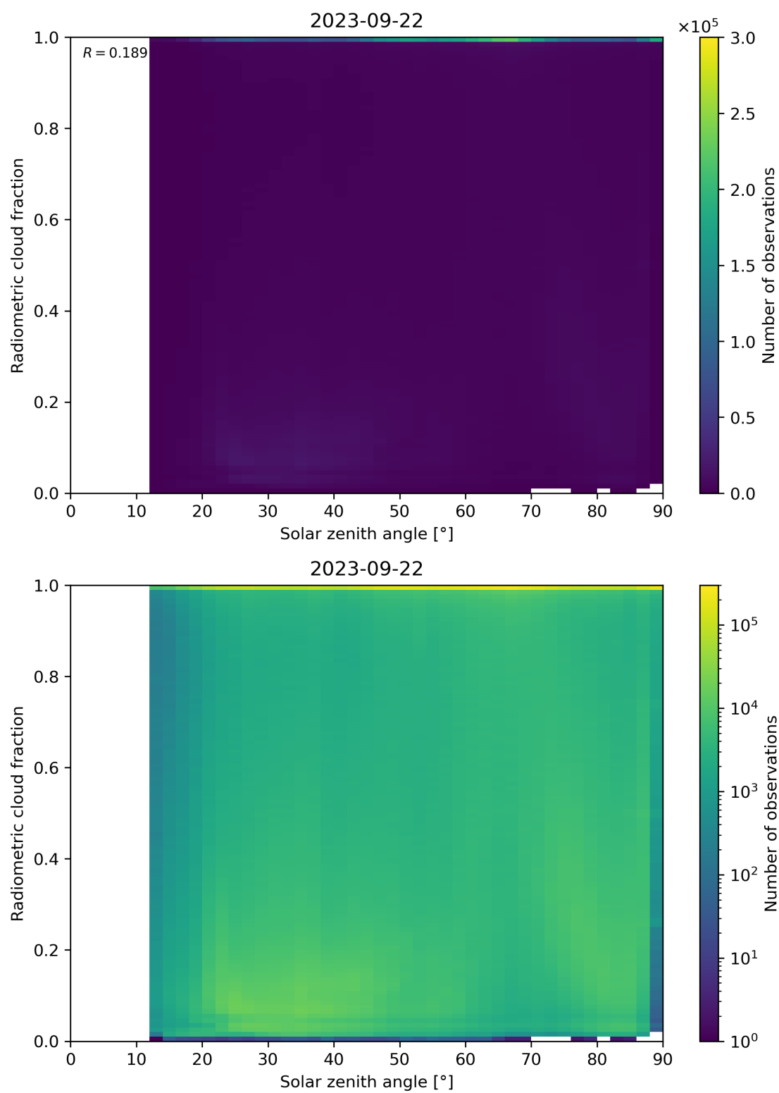
Figure 99: Scatter density plot of “Solar zenith angle” against “Radiometric cloud fraction” for 2023-09-21 to 2023-09-23.
