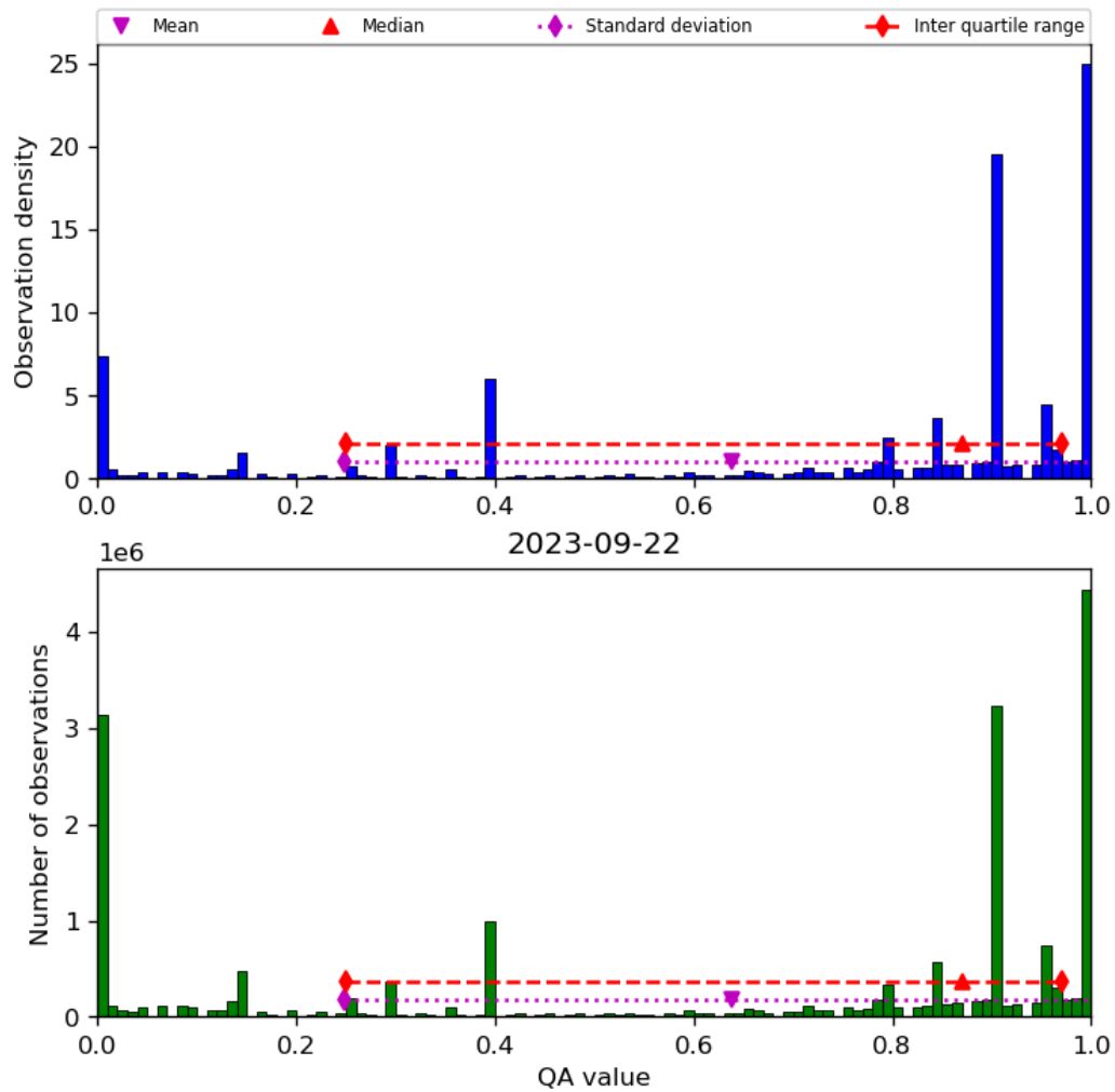
Figure 38: Histogram of “QA value” for 2023-09-21 to 2023-09-23
