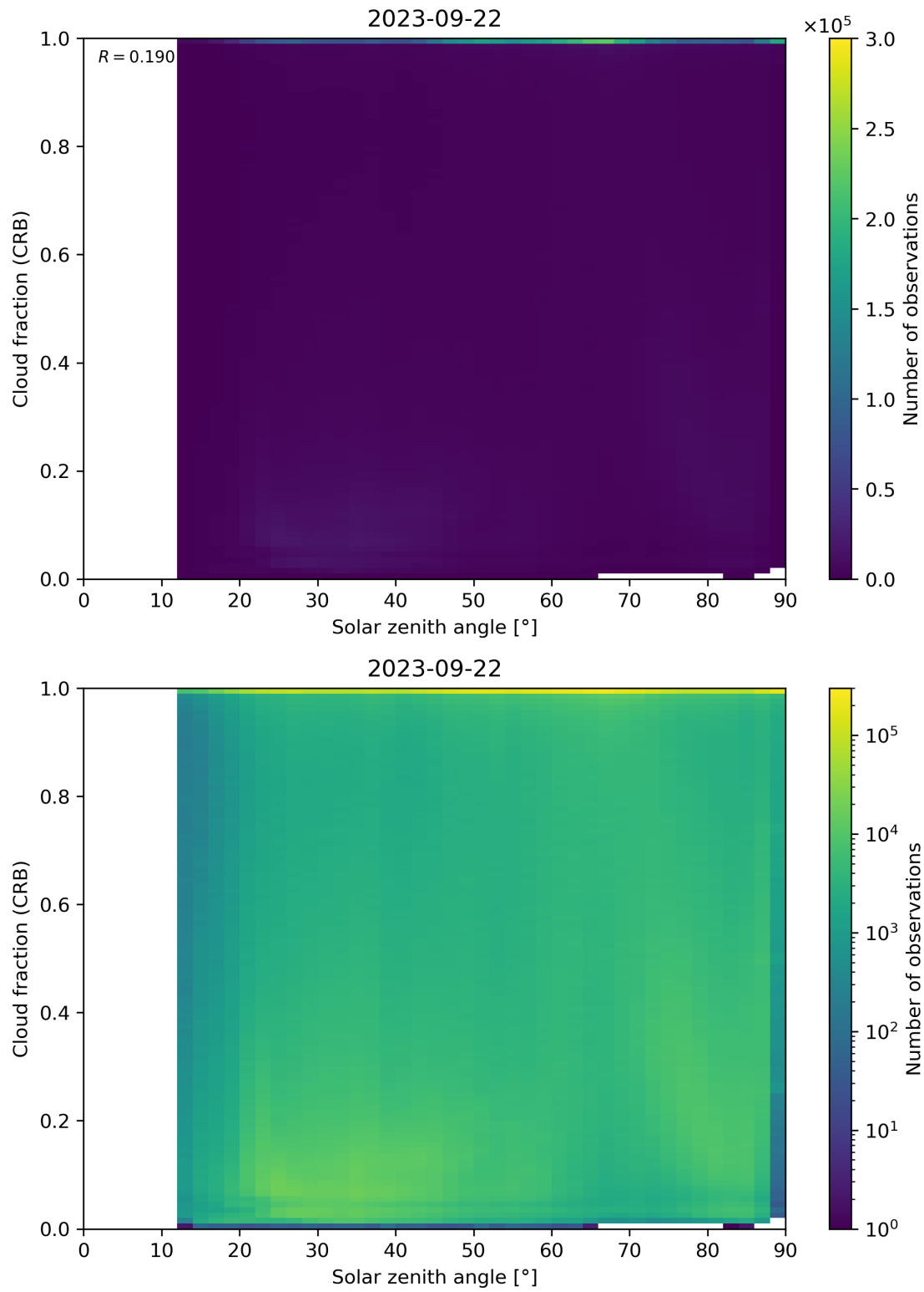
Figure 101: Scatter density plot of “Solar zenith angle” against “Cloud fraction (CRB)” for 2023-09-21 to 2023-09-23.
