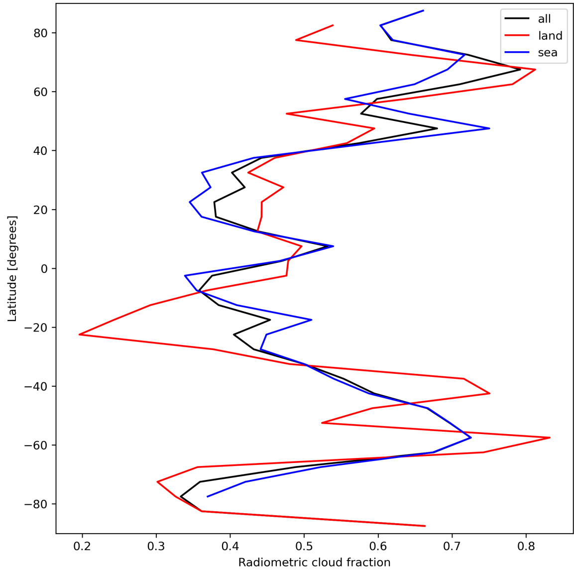
Figure 23: Zonal average of “Radiometric cloud fraction” for 2023-09-21 to 2023-09-23.
