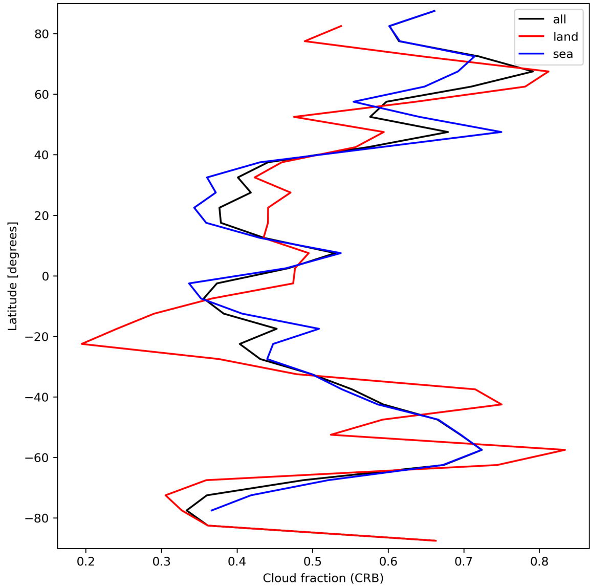
Figure 26: Zonal average of “Cloud fraction (CRB)” for 2023-09-21 to 2023-09-23.
