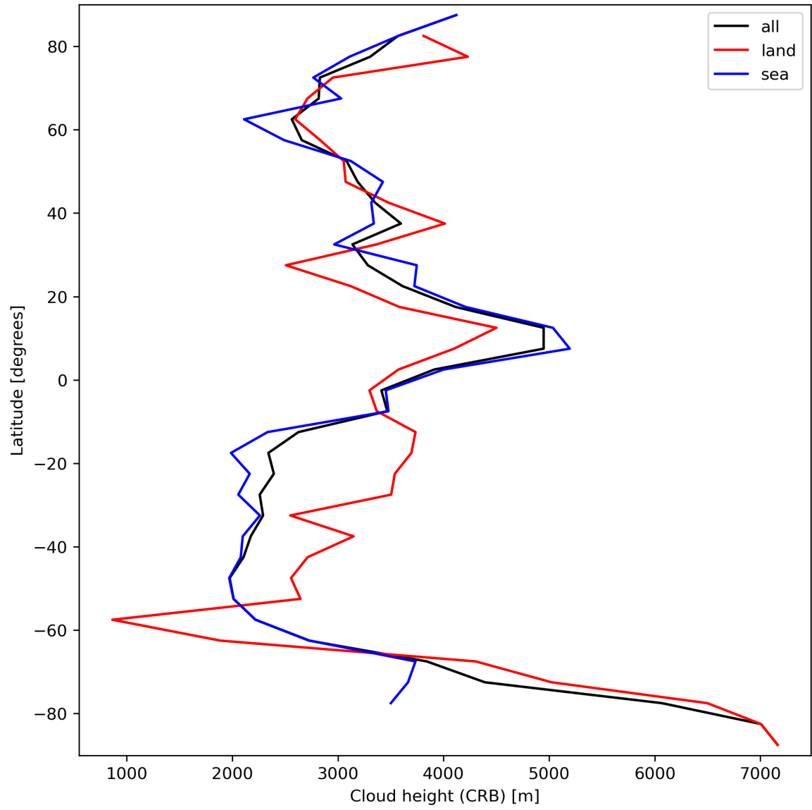
Figure 27: Zonal average of “Cloud height (CRB)” for 2023-09-21 to 2023-09-23.
