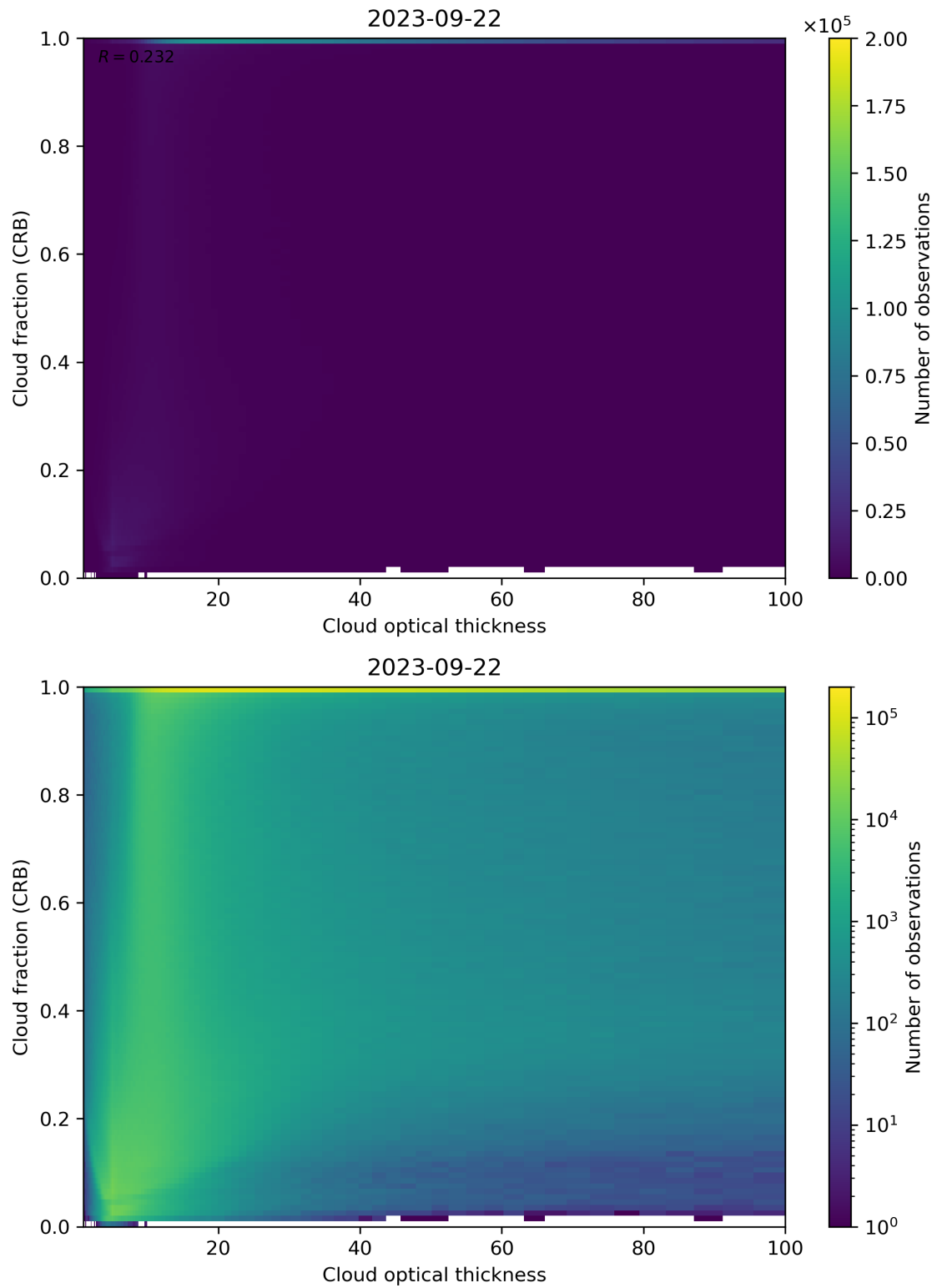
Figure 84: Scatter density plot of “Cloud optical thickness” against “Cloud fraction (CRB)” for 2023-09-21 to 2023-09-23.
