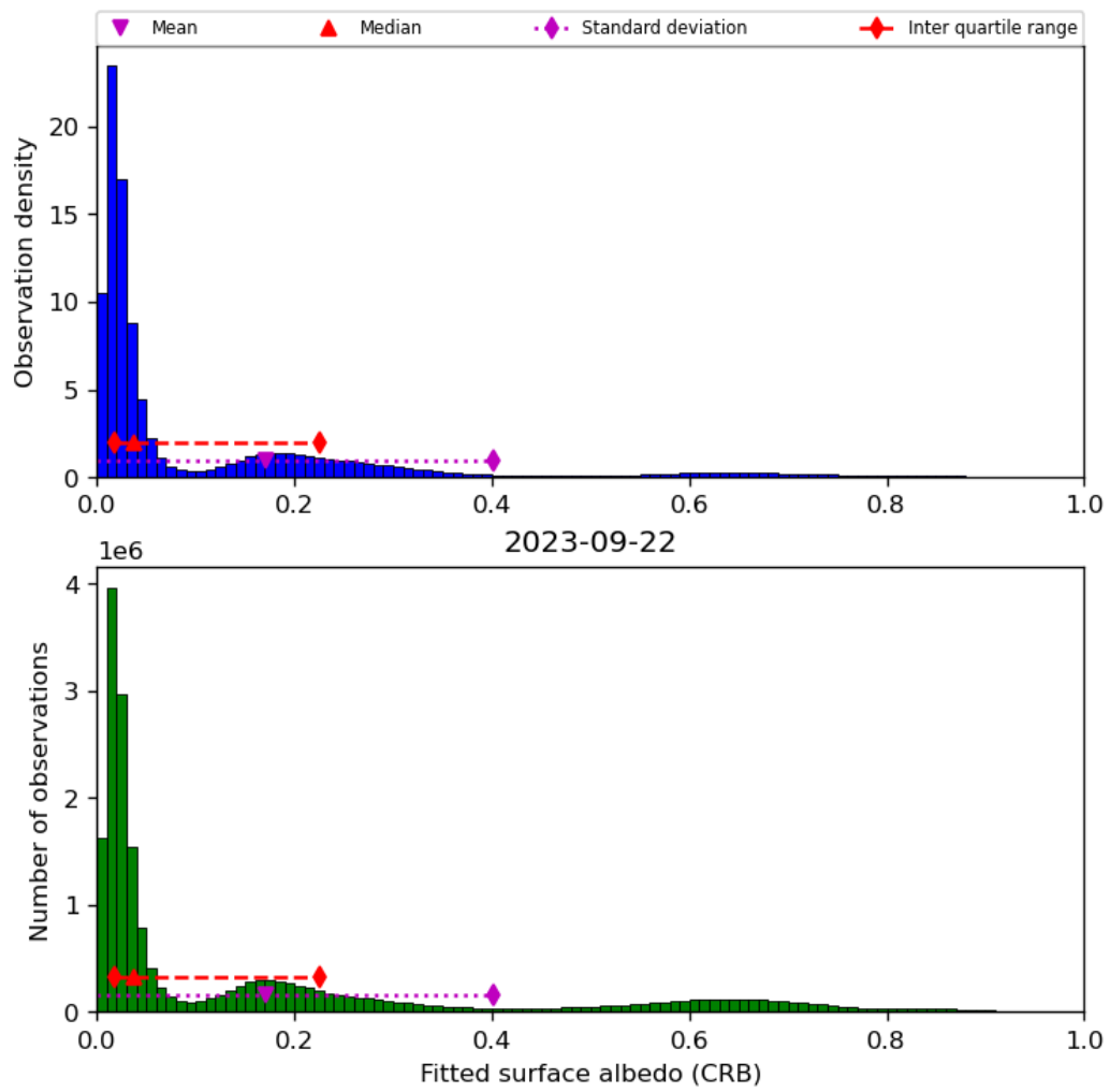
Figure 46: Histogram of “Fitted surface albedo (CRB)” for 2023-09-21 to 2023-09-23
