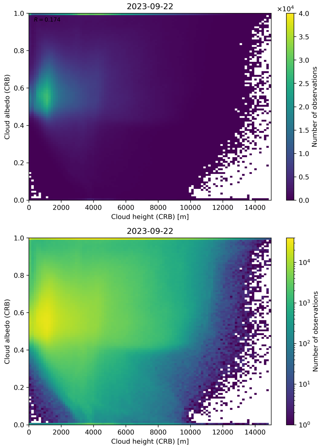
Figure 80: Scatter density plot of “Cloud height (CRB)” against “Cloud albedo (CRB)” for 2023-09-21 to 2023-09-23.
