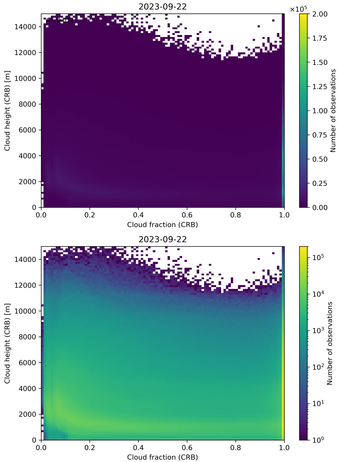
Figure 79: Scatter density plot of “Cloud fraction (CRB)” against “Cloud height (CRB)” for 2023-09-21 to 2023-09-23.
