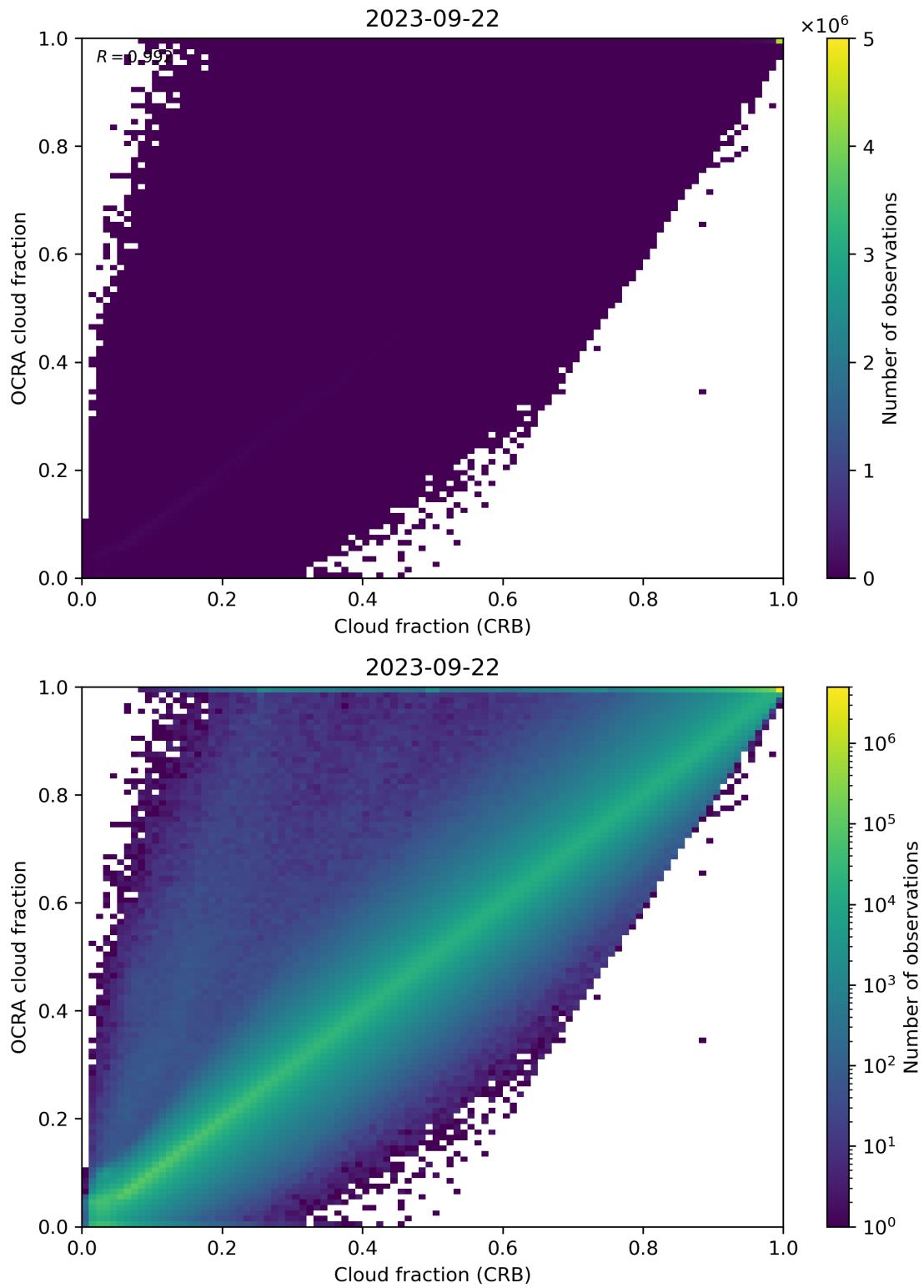
Figure 78: Scatter density plot of “Cloud fraction (CRB)” against “OCRA cloud fraction” for 2023-09-21 to 2023-09-23.
