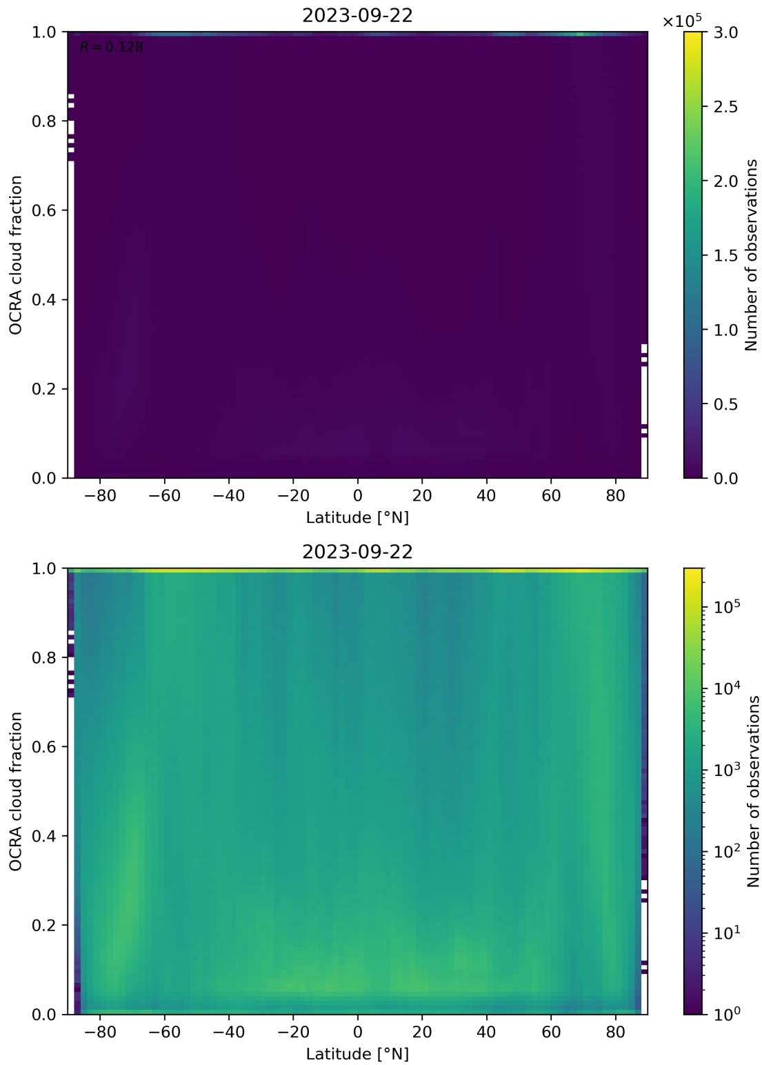
Figure 93: Scatter density plot of “Latitude” against “OCRA cloud fraction” for 2023-09-21 to 2023-09-23.
