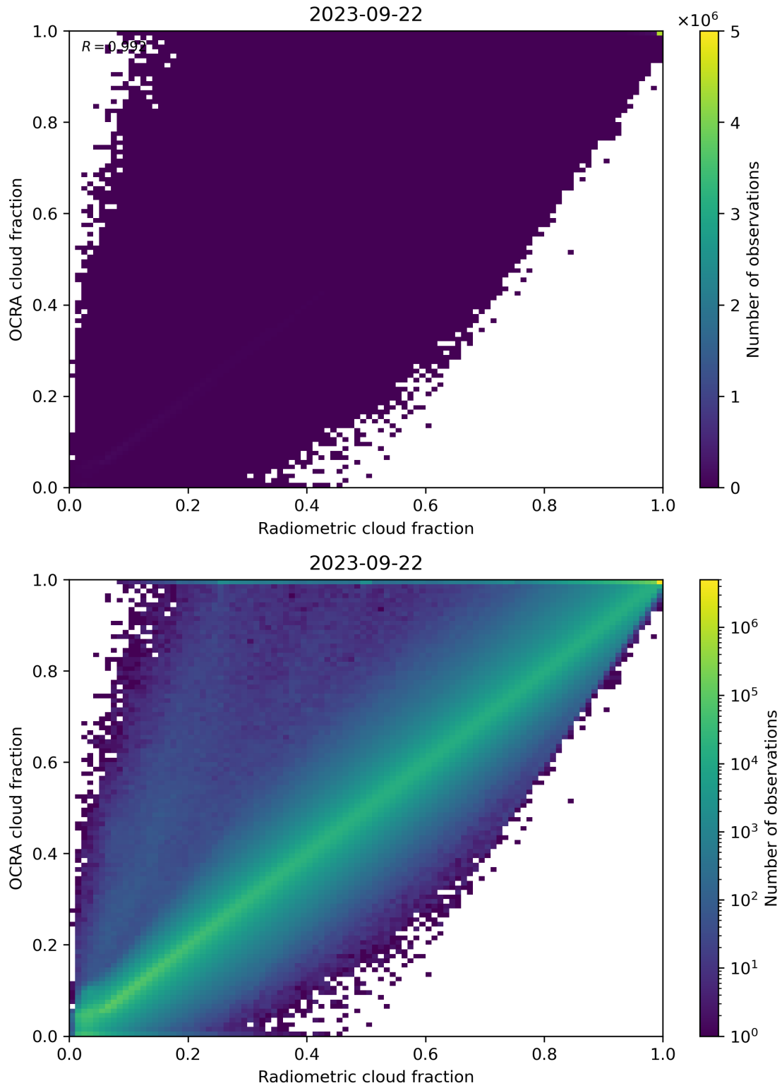
Figure 72: Scatter density plot of “Radiometric cloud fraction” against “OCRA cloud fraction” for 2023-09-21 to 2023-09-23.
