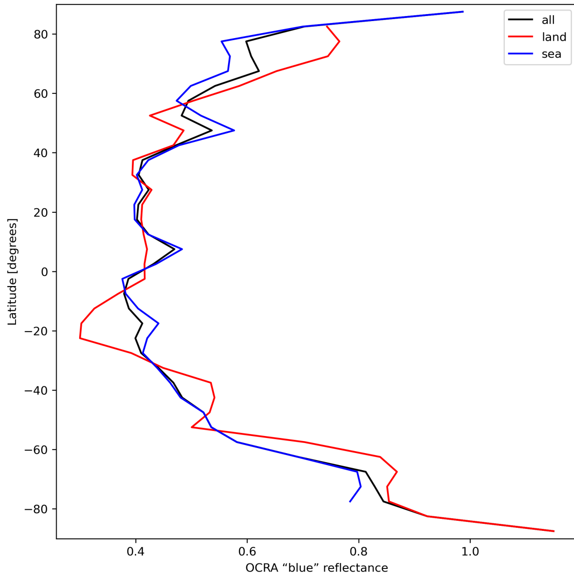
Figure 35: Zonal average of “OCRA “blue” reflectance” for 2023-09-21 to 2023-09-23.
