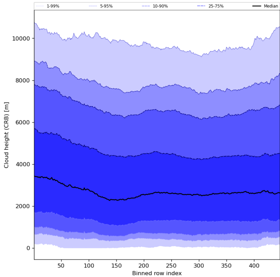
Figure 59: Along track statistics of “Cloud height (CRB)” for 2023-09-21 to 2023-09-23
