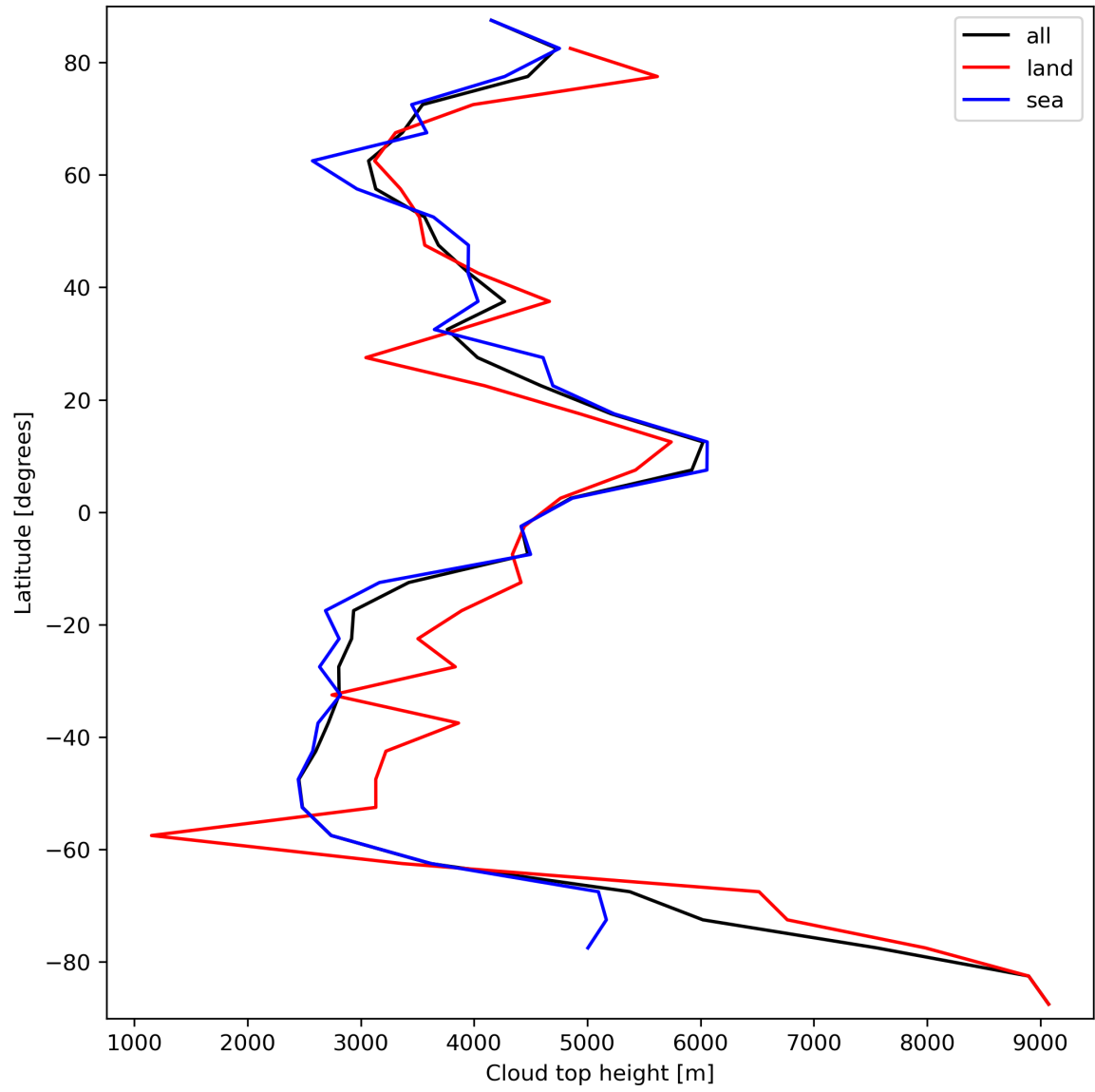
Figure 24: Zonal average of “Cloud top height” for 2023-09-21 to 2023-09-23.
