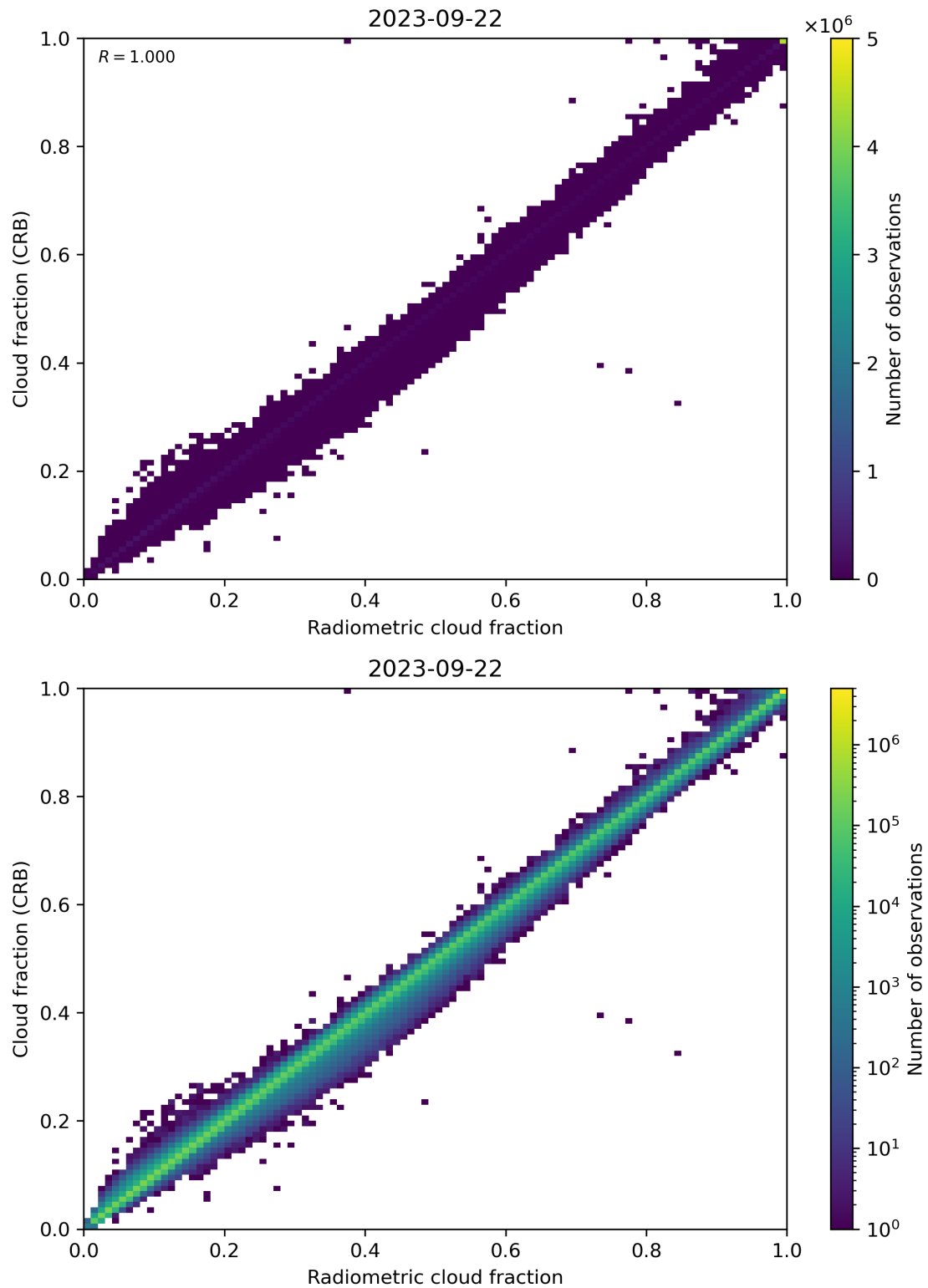
Figure 73: Scatter density plot of “Radiometric cloud fraction” against “Cloud fraction (CRB)” for 2023-09-21 to 2023-09-23.
