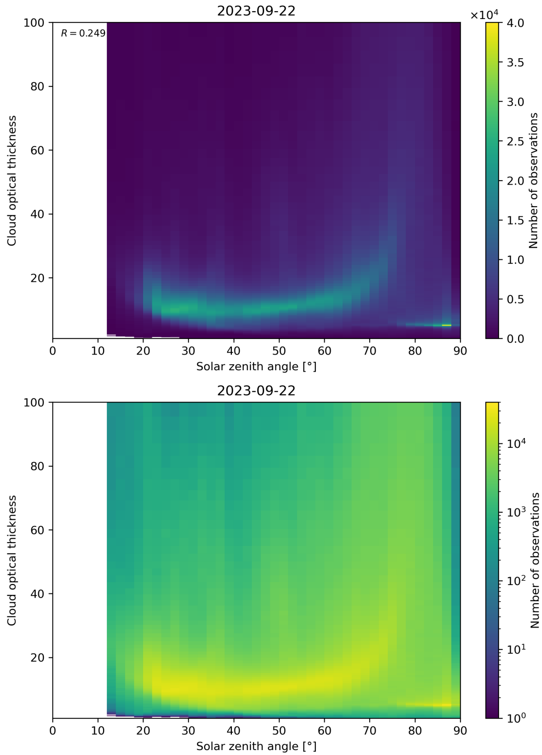
Figure 103: Scatter density plot of “Solar zenith angle” against “Cloud optical thickness” for 2023-09-21 to 2023-09-23.
