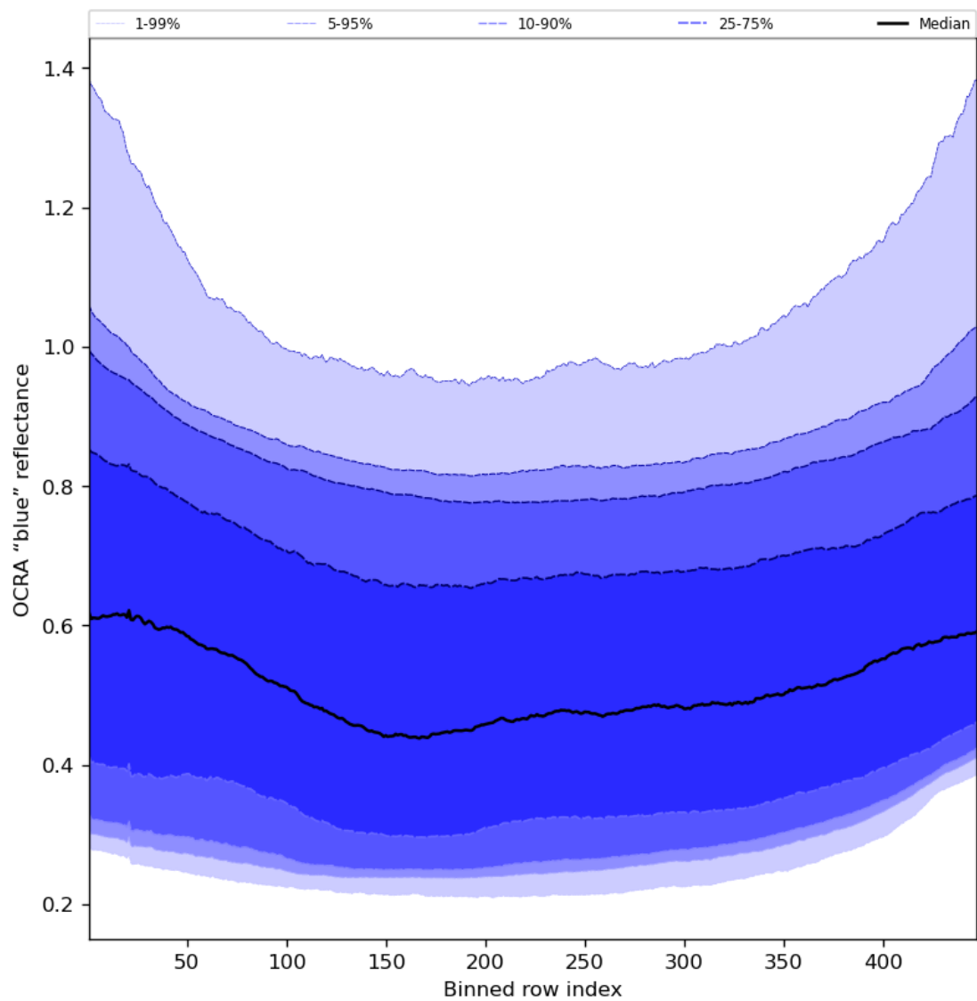
Figure 67: Along track statistics of “OCRA “blue” reflectance” for 2023-09-21 to 2023-09-23
