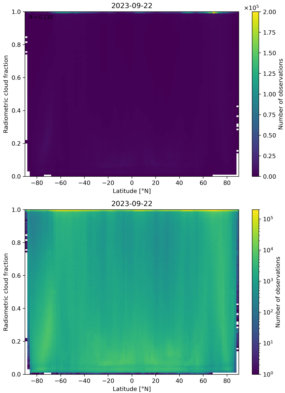
Figure 92: Scatter density plot of “Latitude” against “Radiometric cloud fraction” for 2023-09-21 to 2023-09-23.
