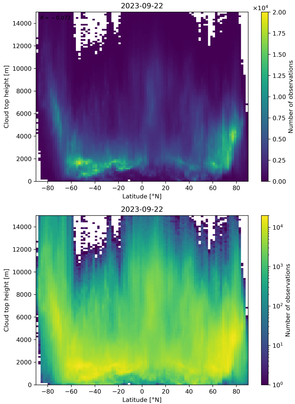
Figure 97: Scatter density plot of “Latitude” against “Cloud top height” for 2023-09-21 to 2023-09-23.
