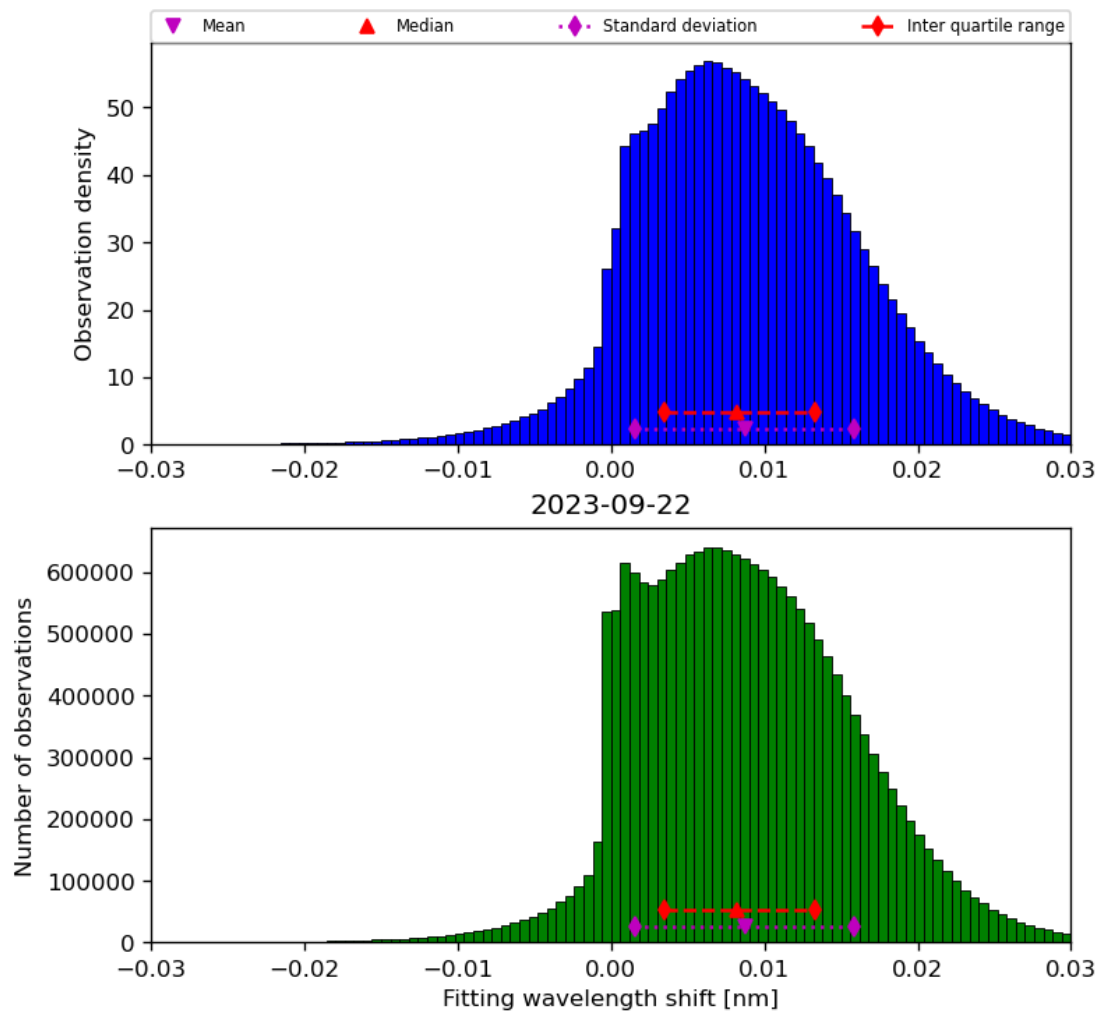
Figure 49: Histogram of “Fitting wavelength shift” for 2023-09-21 to 2023-09-23
