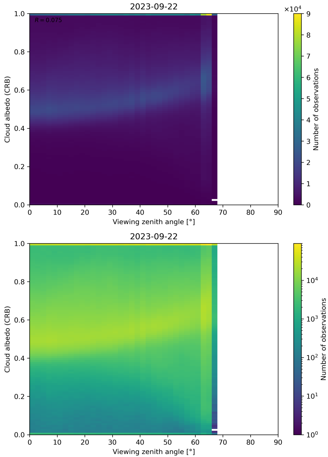
Figure 106: Scatter density plot of “Viewing zenith angle” against “Cloud albedo (CRB)” for 2023-09-21 to 2023-09-23.
