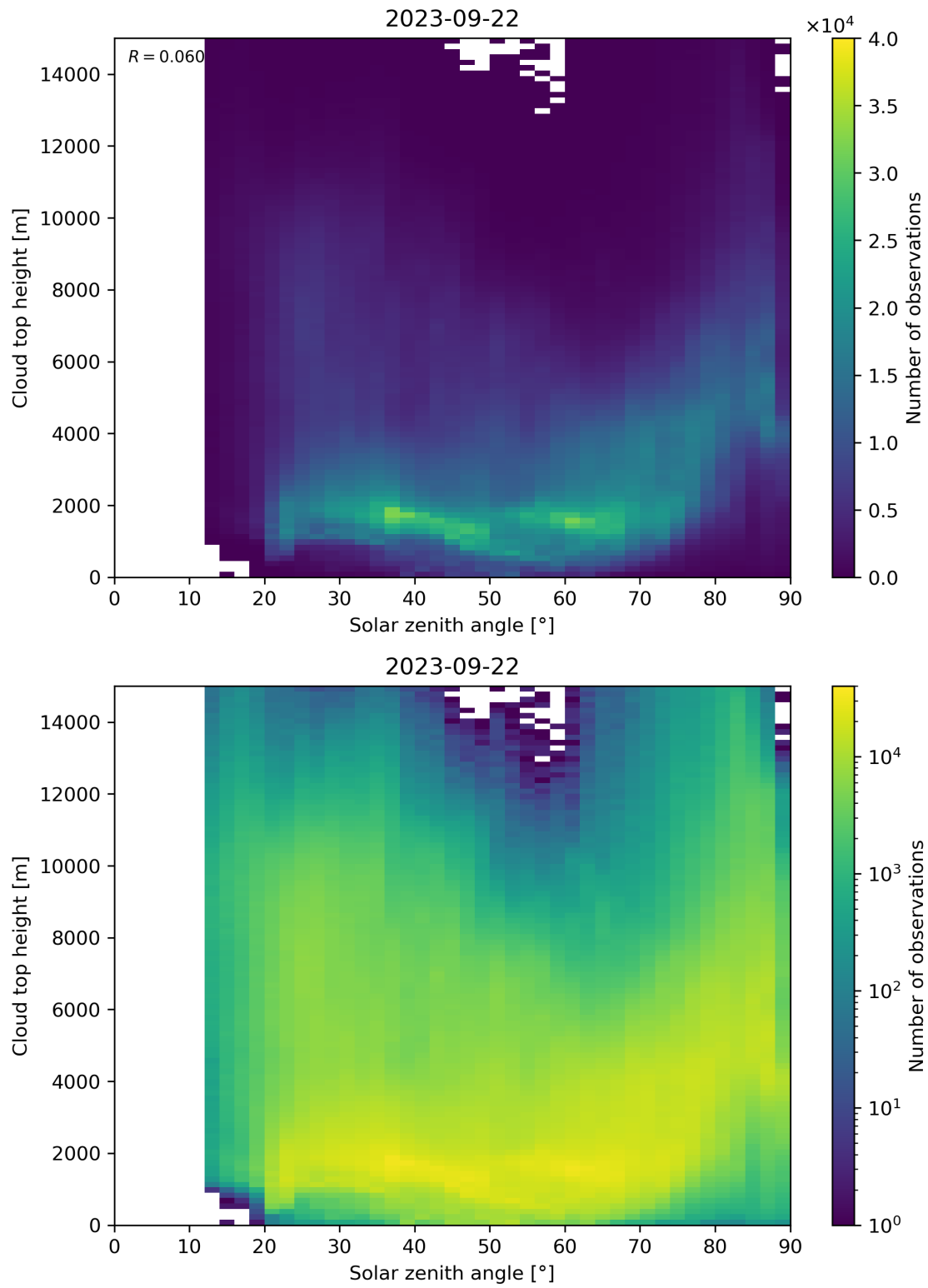
Figure 104: Scatter density plot of “Solar zenith angle” against “Cloud top height” for 2023-09-21 to 2023-09-23.
