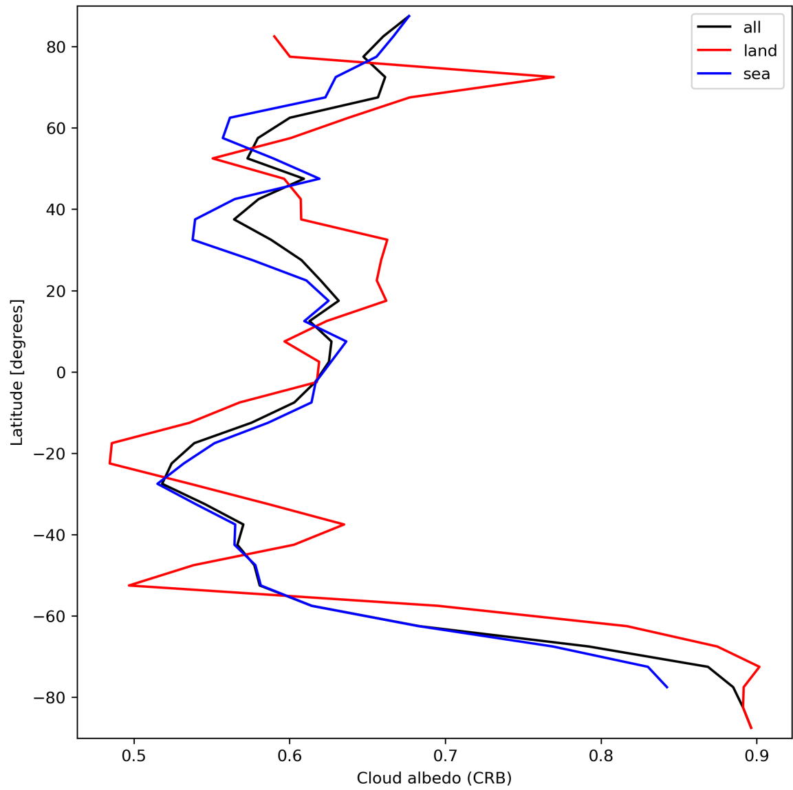
Figure 28: Zonal average of “Cloud albedo (CRB)” for 2023-09-21 to 2023-09-23.
