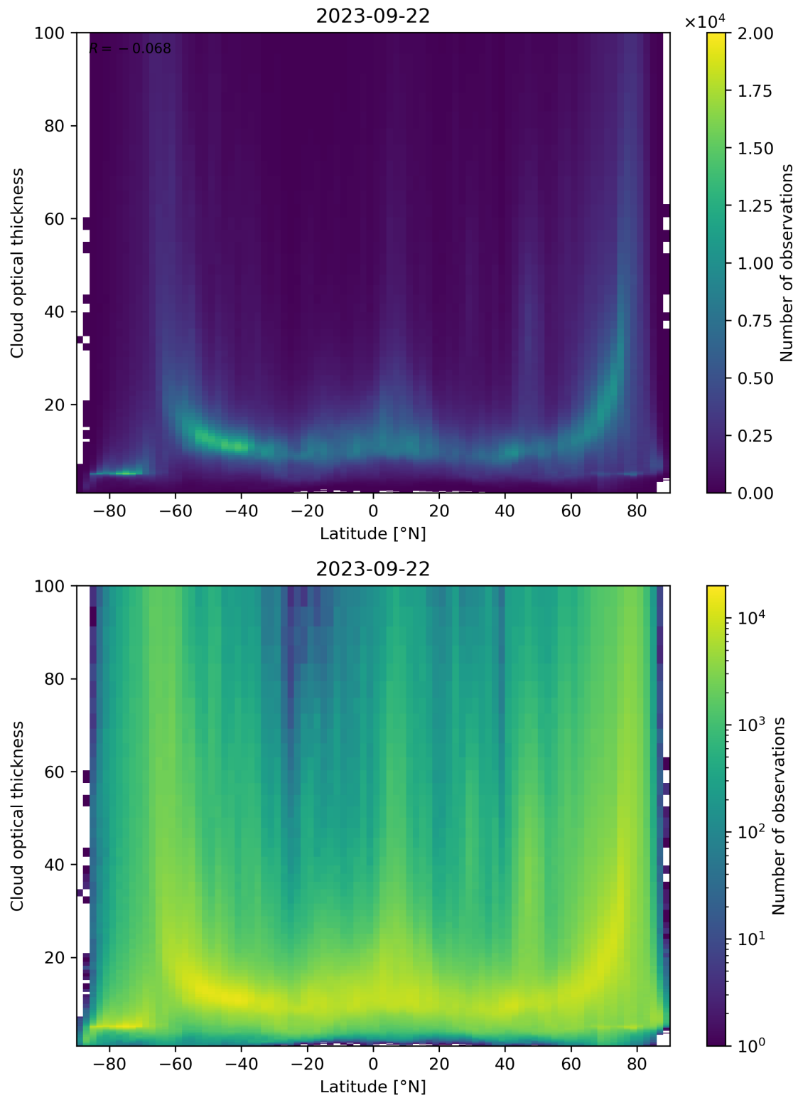
Figure 96: Scatter density plot of “Latitude” against “Cloud optical thickness” for 2023-09-21 to 2023-09-23.
