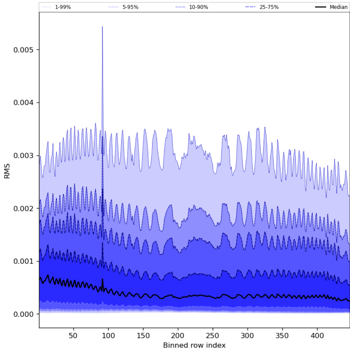
Figure 63: Along track statistics of “RMS” for 2023-09-21 to 2023-09-23
