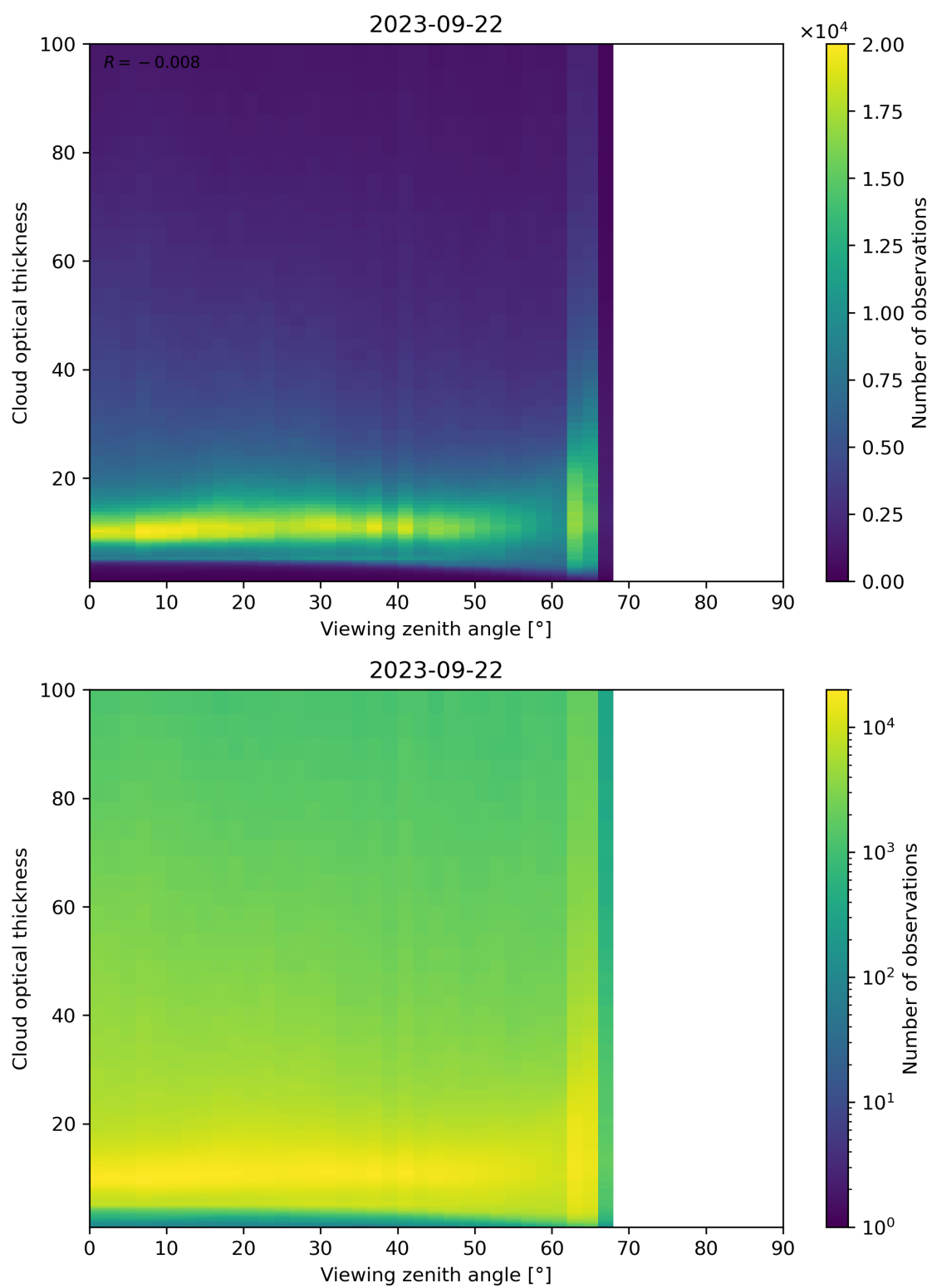
Figure 111: Scatter density plot of “Viewing zenith angle” against “Cloud optical thickness” for 2023-09-21 to 2023-09-23.
