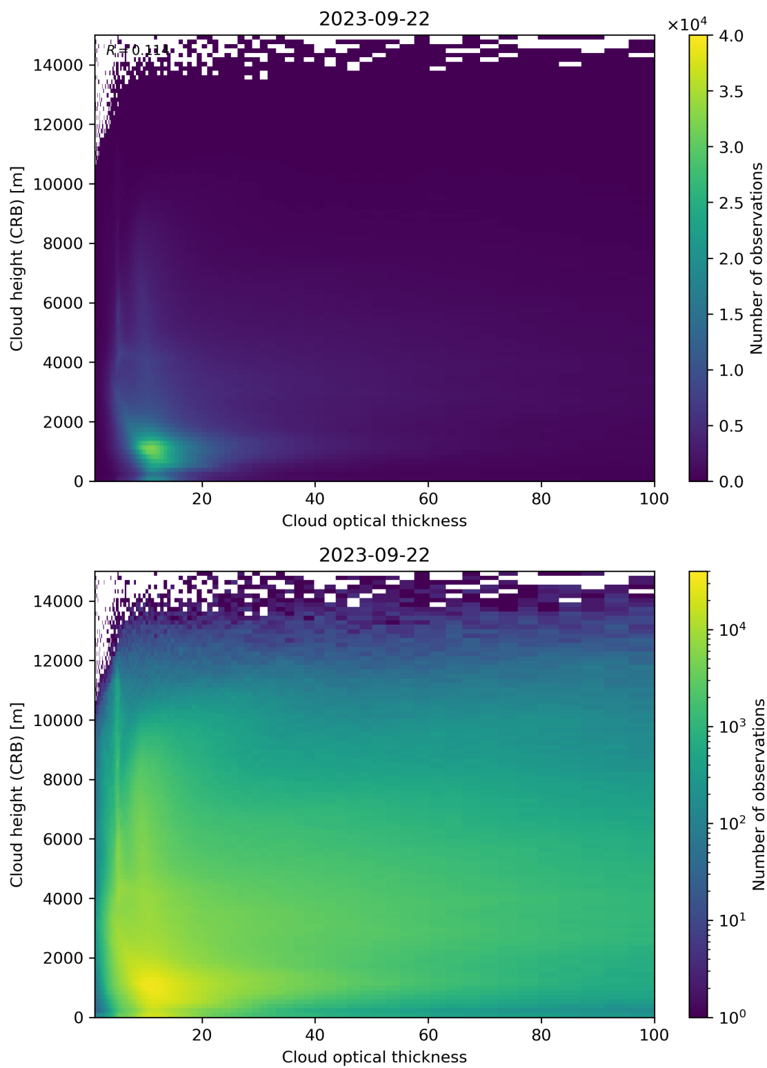
Figure 85: Scatter density plot of “Cloud optical thickness” against “Cloud height (CRB)” for 2023-09-21 to 2023-09-23.
