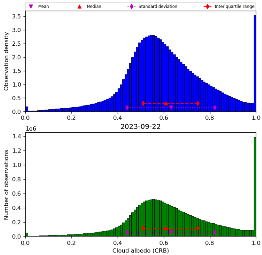
Figure 44: Histogram of “Cloud albedo (CRB)” for 2023-09-21 to 2023-09-23
