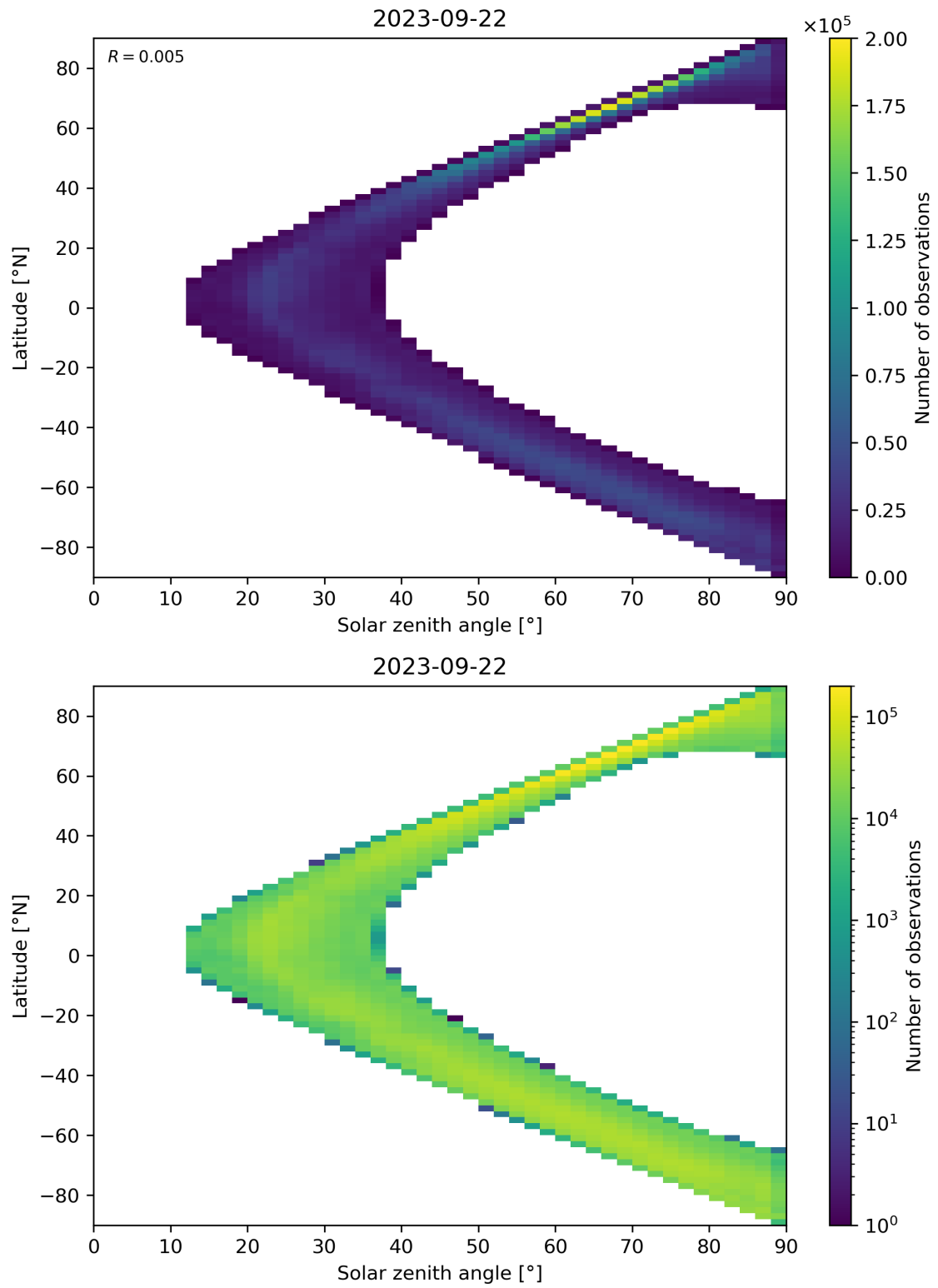
Figure 105: Scatter density plot of “Solar zenith angle” against “Latitude” for 2023-09-21 to 2023-09-23.
