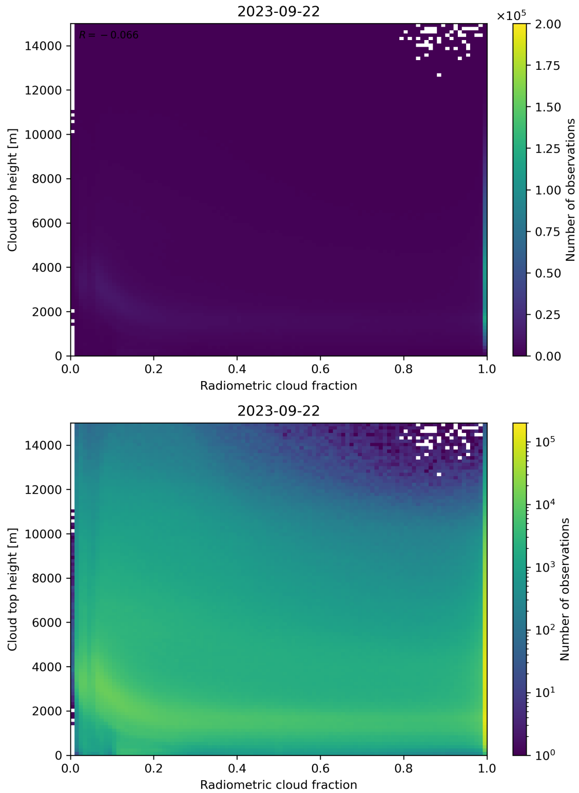
Figure 76: Scatter density plot of “Radiometric cloud fraction” against “Cloud top height” for 2023-09-21 to 2023-09-23.
