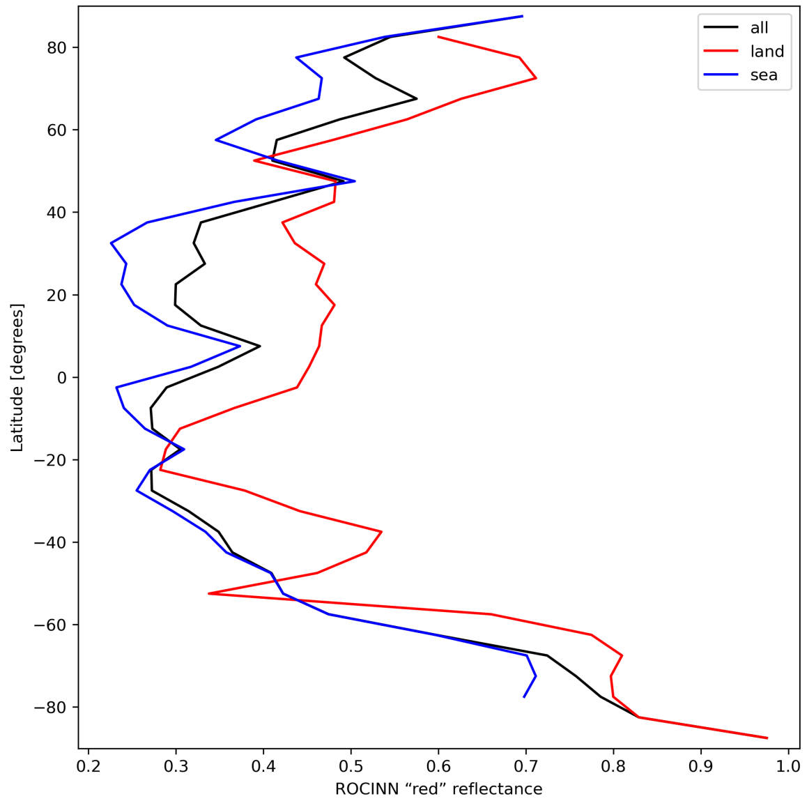
Figure 37: Zonal average of “ROCINN “red” reflectance” for 2023-09-21 to 2023-09-23.
