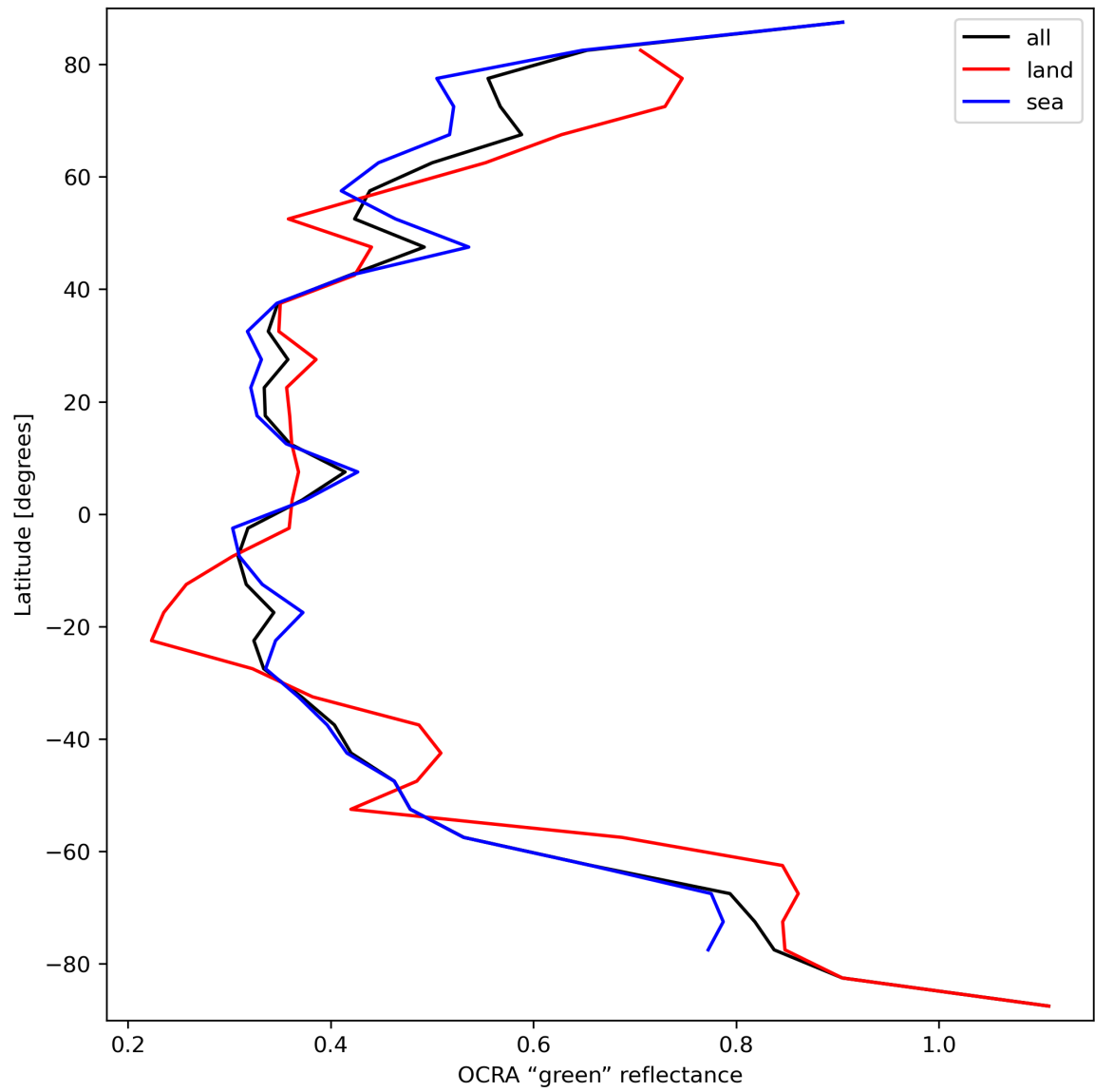
Figure 36: Zonal average of “OCRA “green” reflectance” for 2023-09-21 to 2023-09-23.
