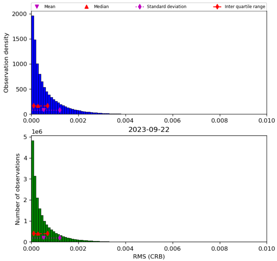
Figure 48: Histogram of “RMS (CRB)” for 2023-09-21 to 2023-09-23
