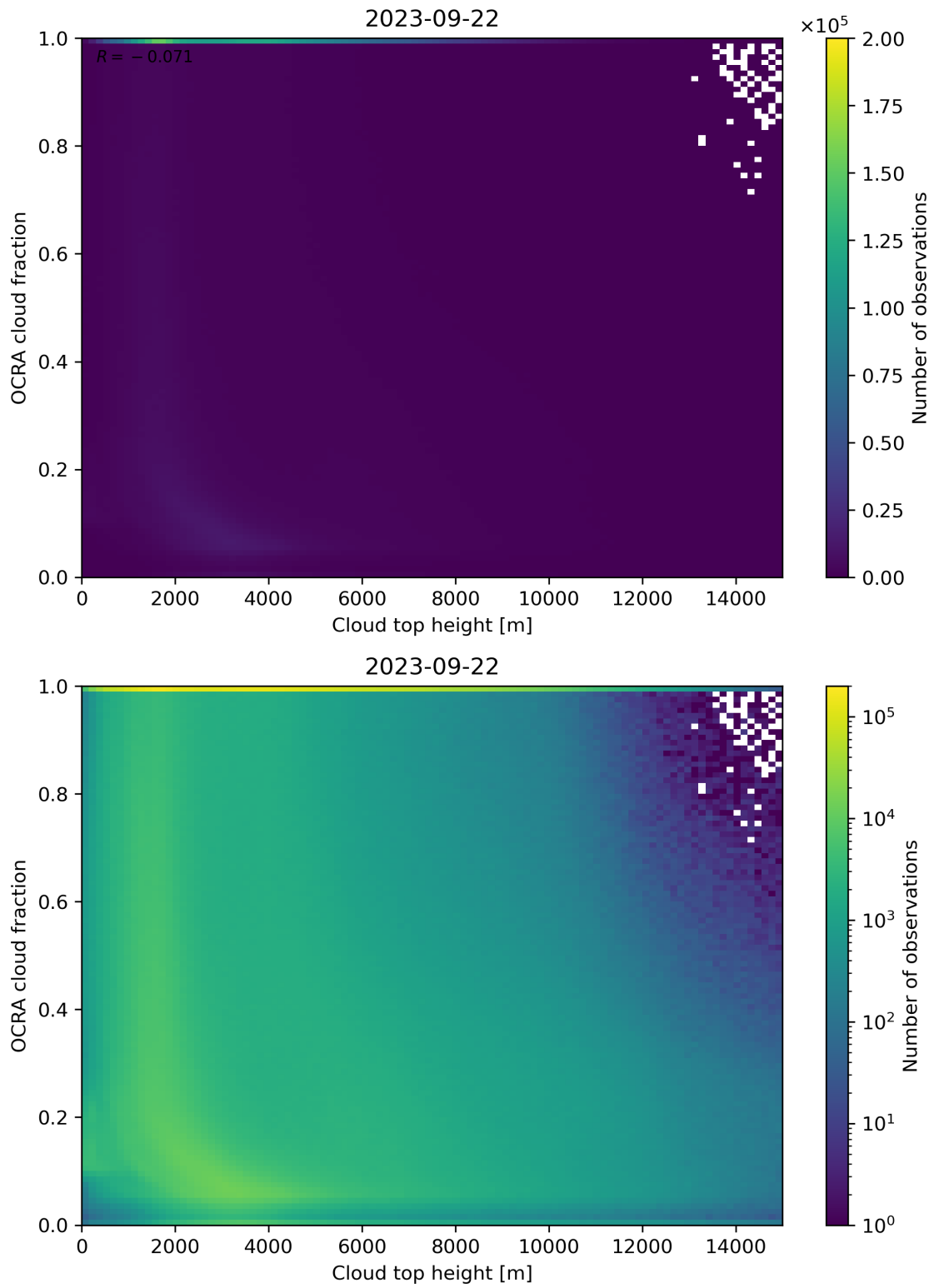
Figure 87: Scatter density plot of “Cloud top height” against “OCRA cloud fraction” for 2023-09-21 to 2023-09-23.
