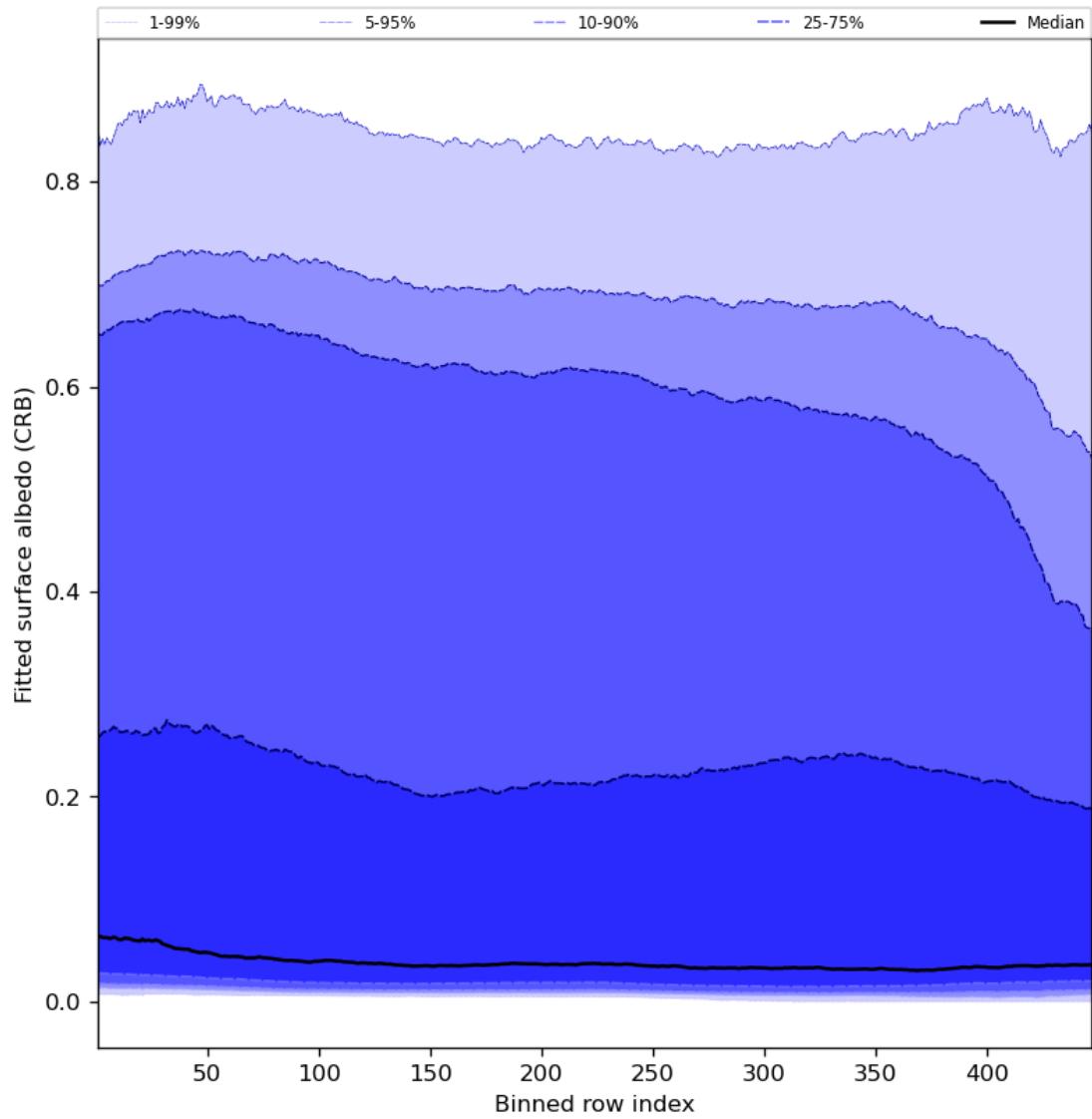
Figure 62: Along track statistics of “Fitted surface albedo (CRB)” for 2023-09-21 to 2023-09-23
