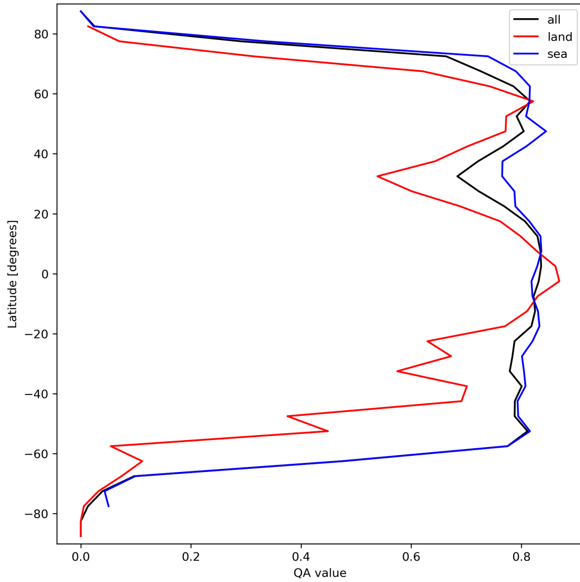
Figure 22: Zonal average of “QA value” for 2023-09-21 to 2023-09-23.
