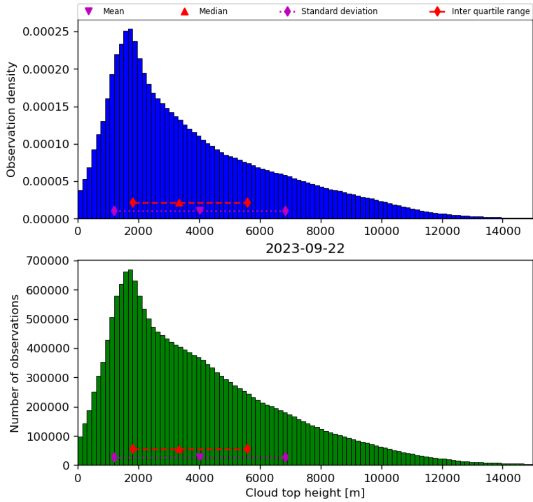
Figure 40: Histogram of “Cloud top height” for 2023-09-21 to 2023-09-23
