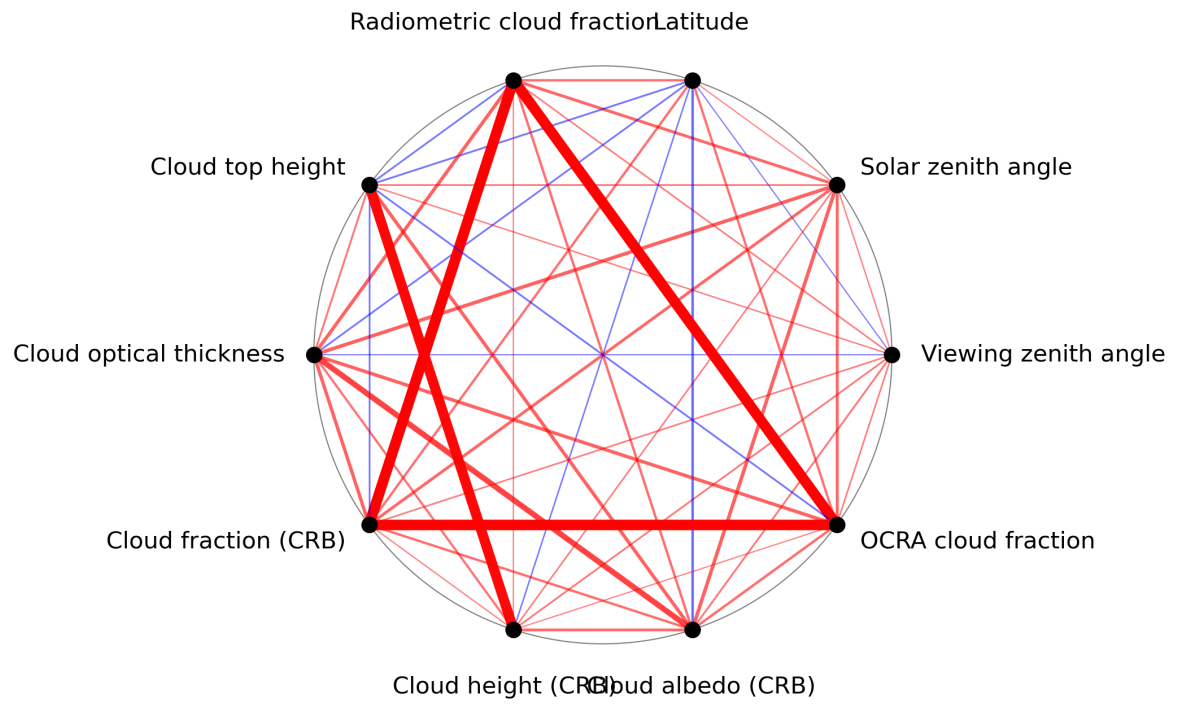
Figure 1: Map of correlation graph for 2023-09-21 to 2023-09-23.
