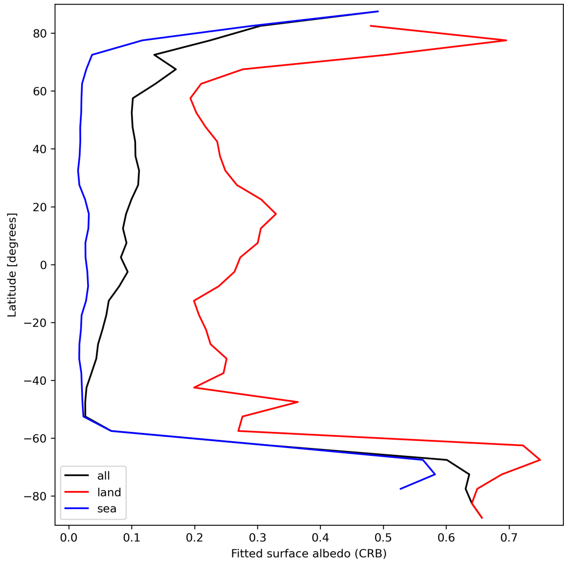
Figure 30: Zonal average of “Fitted surface albedo (CRB)” for 2023-09-21 to 2023-09-23.
