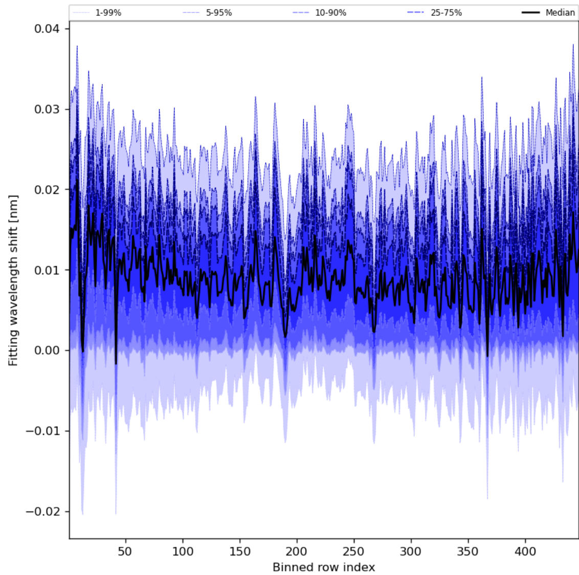
Figure 65: Along track statistics of “Fitting wavelength shift” for 2023-09-21 to 2023-09-23
