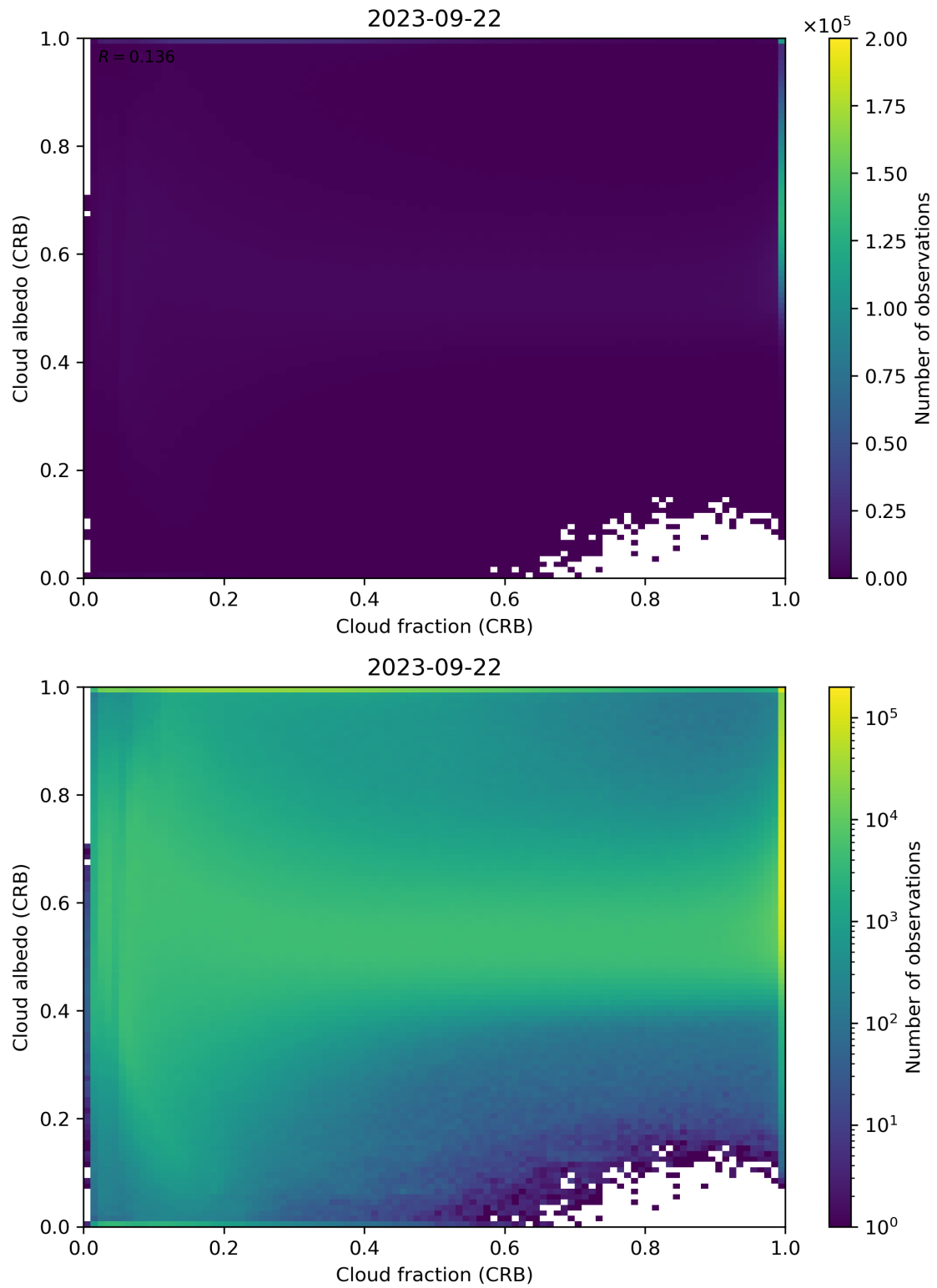
Figure 77: Scatter density plot of “Cloud fraction (CRB)” against “Cloud albedo (CRB)” for 2023-09-21 to 2023-09-23.
