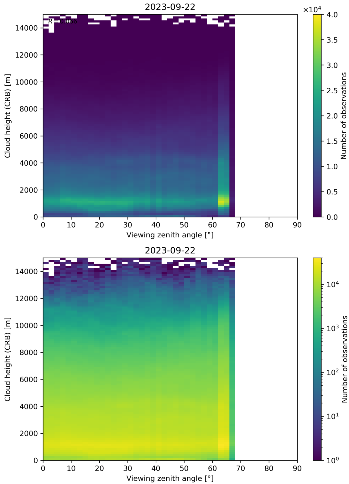
Figure 110: Scatter density plot of “Viewing zenith angle” against “Cloud height (CRB)” for 2023-09-21 to 2023-09-23.
