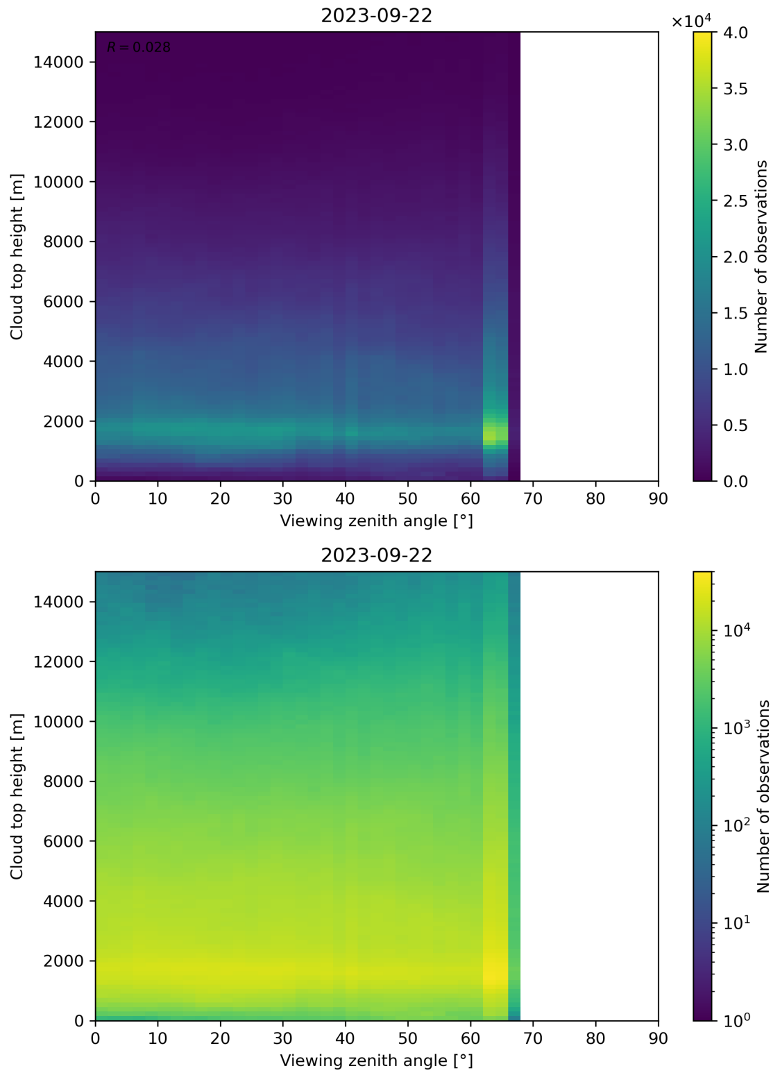
Figure 112: Scatter density plot of “Viewing zenith angle” against “Cloud top height” for 2023-09-21 to 2023-09-23.
