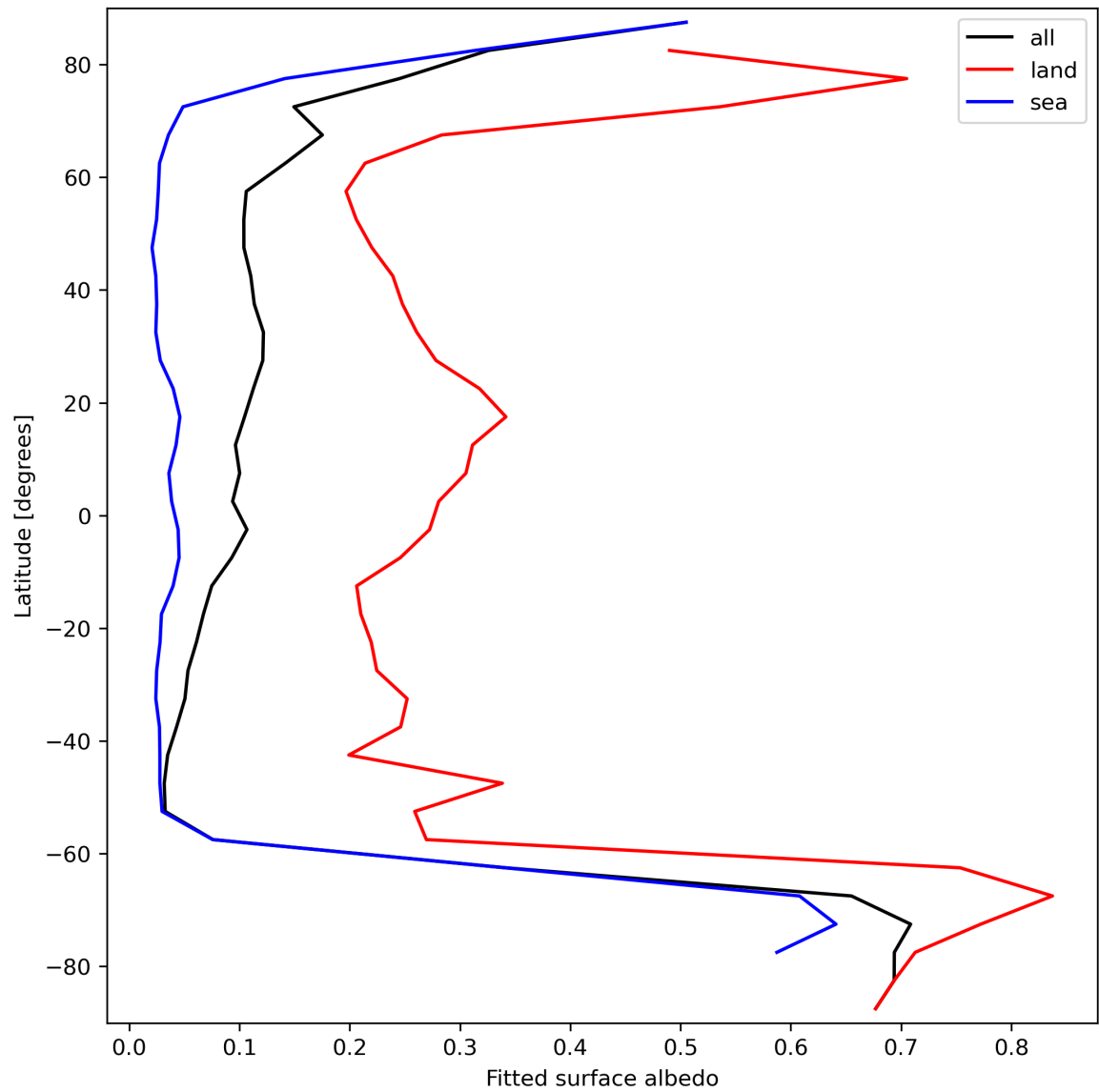
Figure 29: Zonal average of “Fitted surface albedo” for 2023-09-21 to 2023-09-23.
