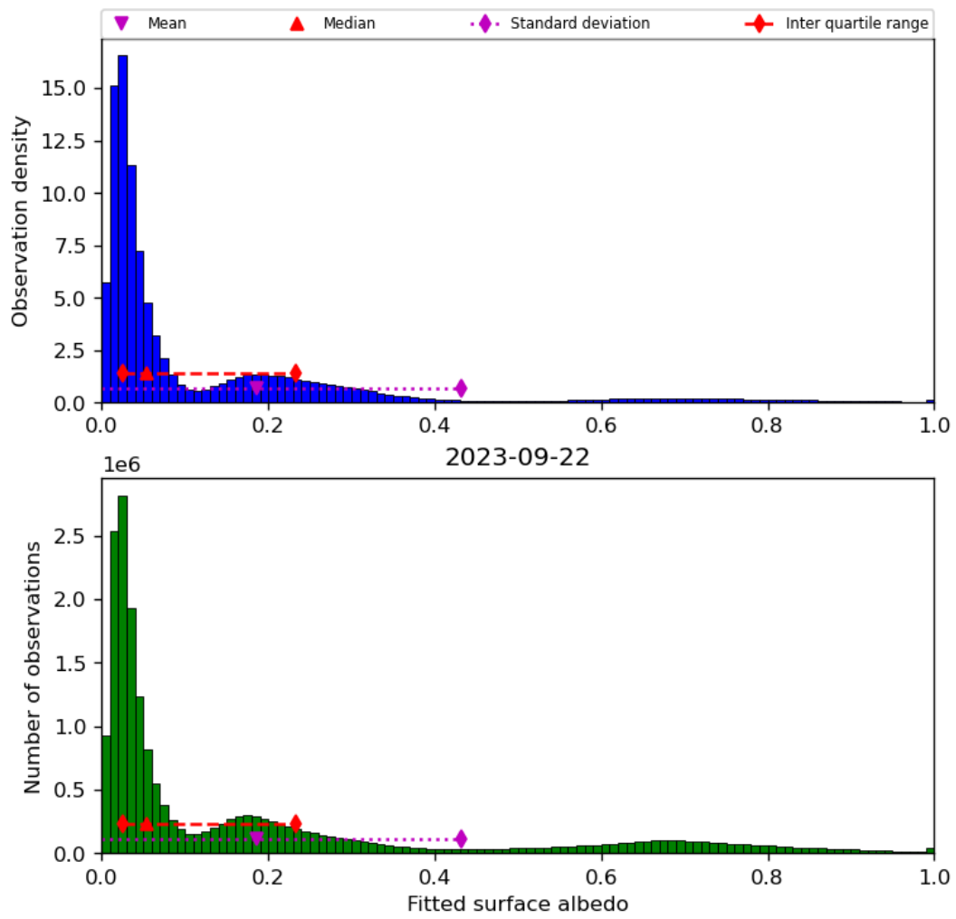
Figure 45: Histogram of “Fitted surface albedo” for 2023-09-21 to 2023-09-23
