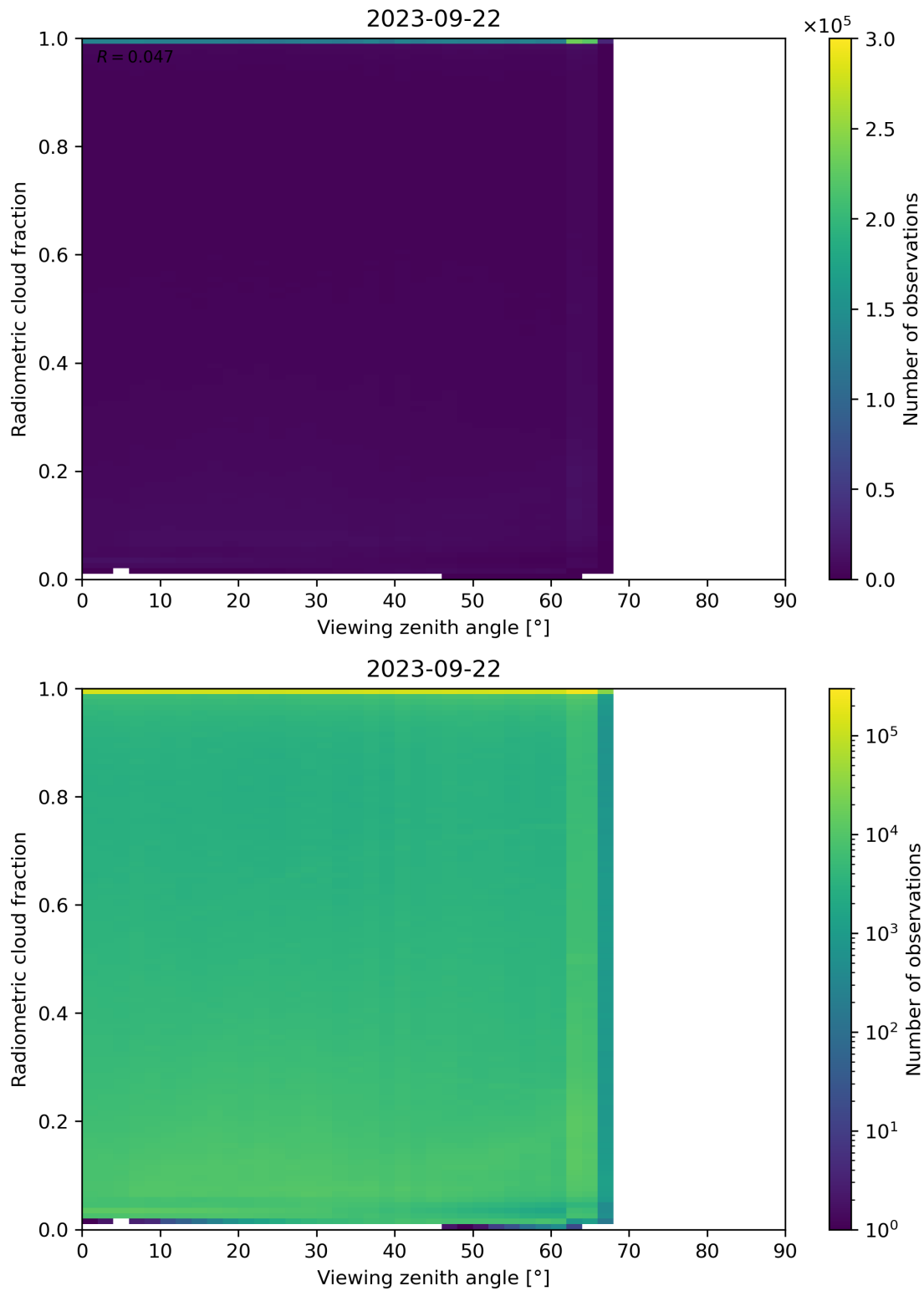
Figure 107: Scatter density plot of “Viewing zenith angle” against “Radiometric cloud fraction” for 2023-09-21 to 2023-09-23.
