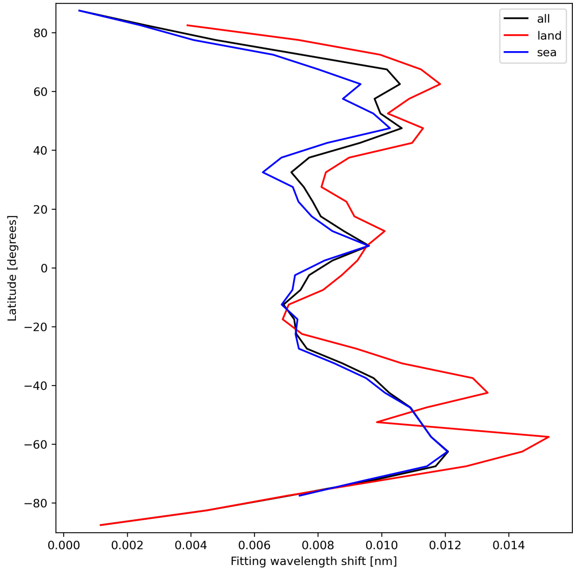
Figure 33: Zonal average of “Fitting wavelength shift” for 2023-09-21 to 2023-09-23.
