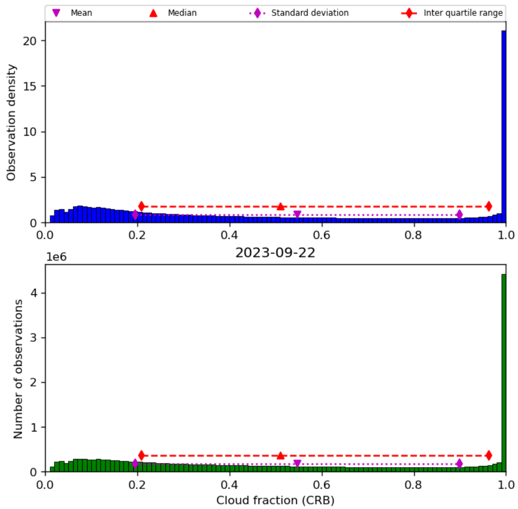
Figure 42: Histogram of “Cloud fraction (CRB)” for 2023-09-21 to 2023-09-23
