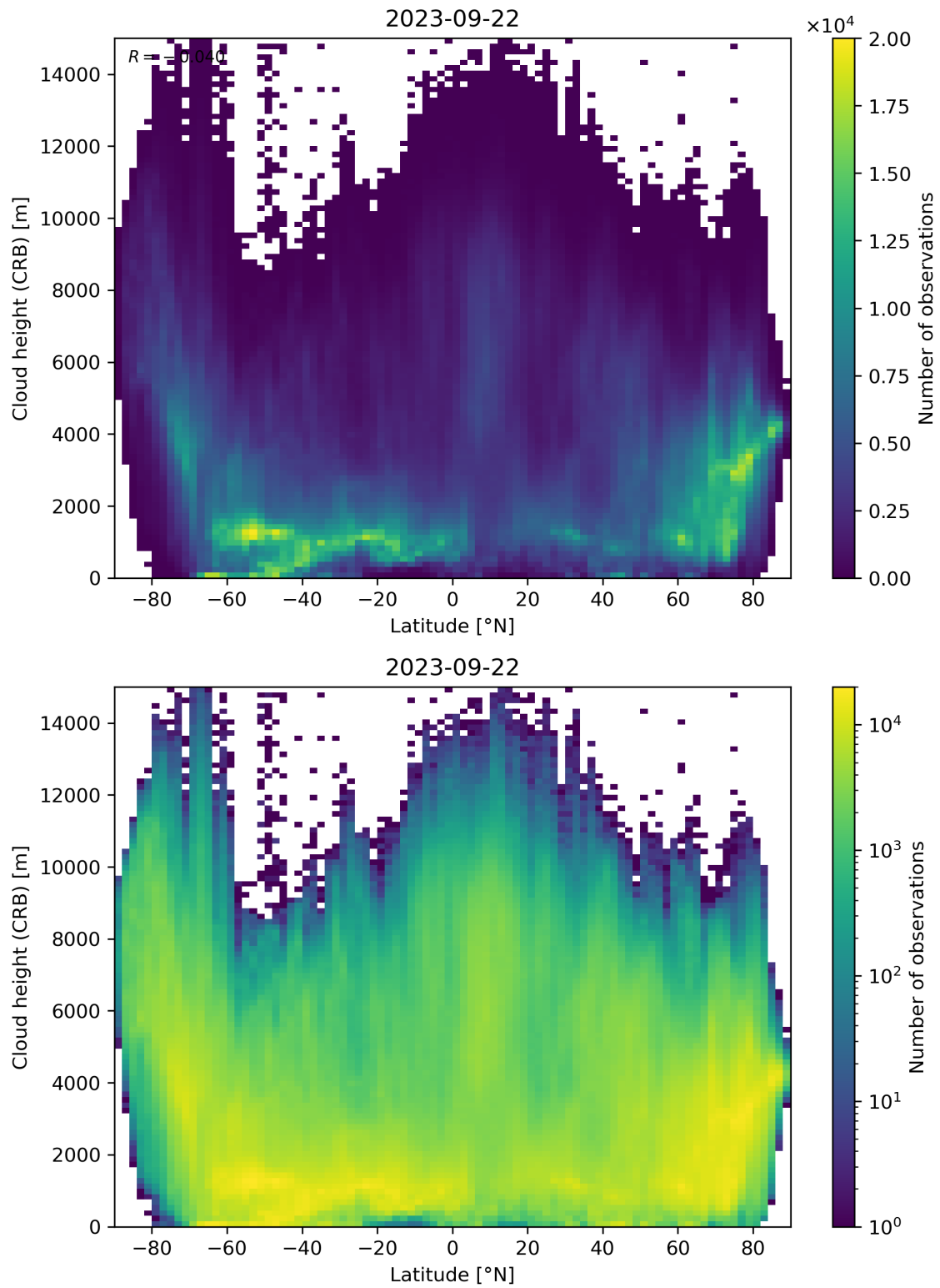
Figure 95: Scatter density plot of “Latitude” against “Cloud height (CRB)” for 2023-09-21 to 2023-09-23.
