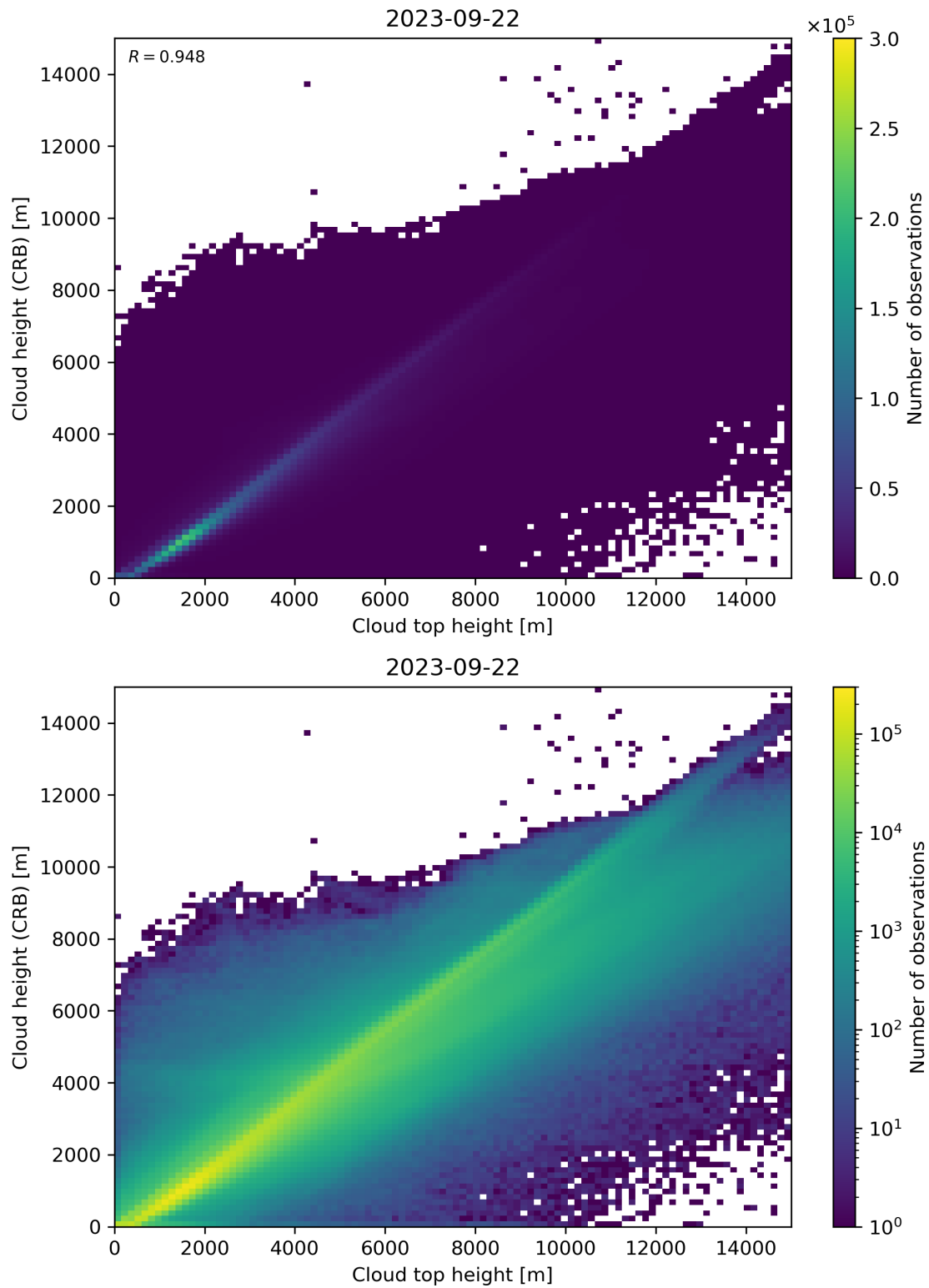
Figure 89: Scatter density plot of “Cloud top height” against “Cloud height (CRB)” for 2023-09-21 to 2023-09-23.
