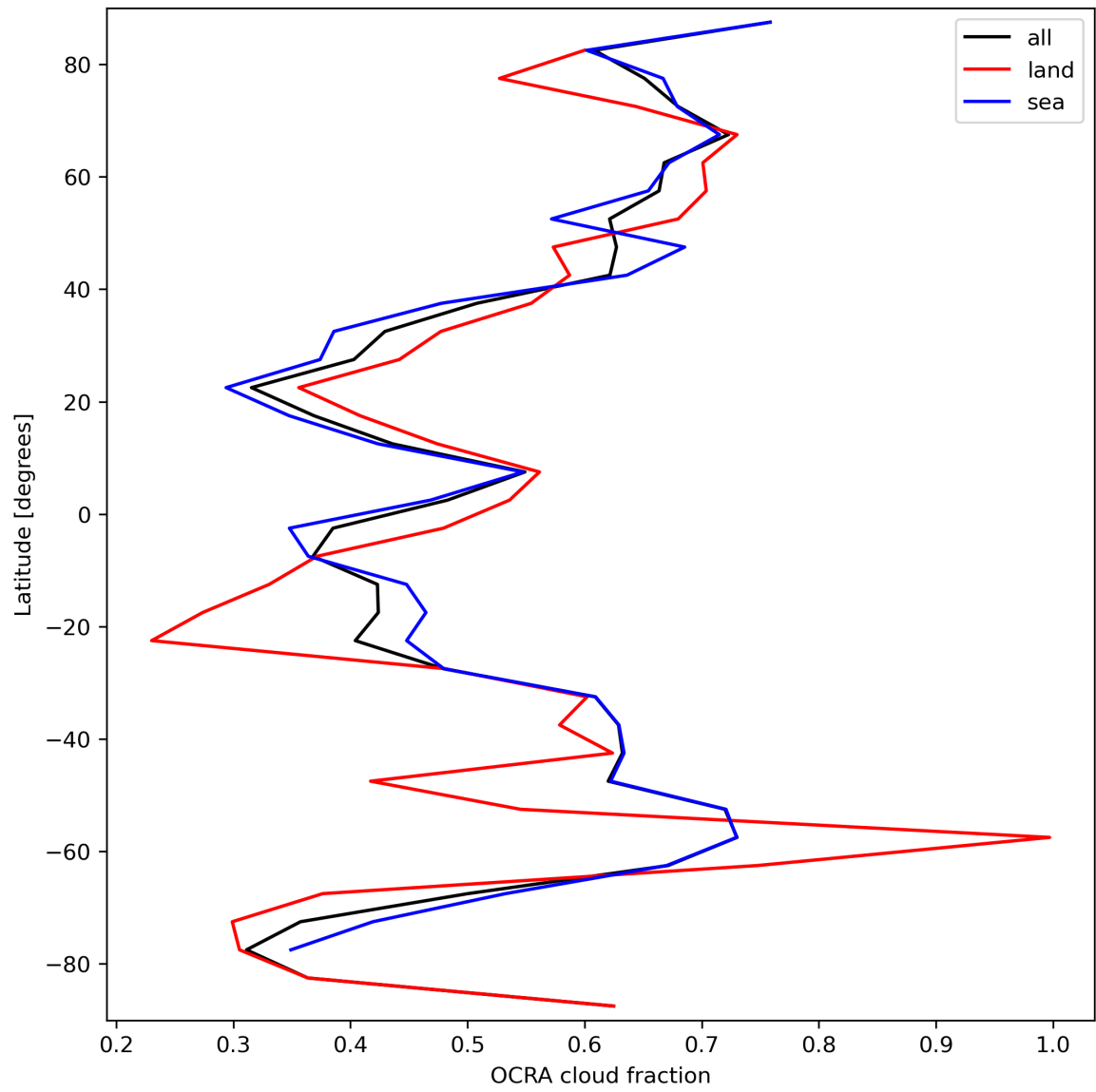
Figure 34: Zonal average of “OCRA cloud fraction” for 2023-09-23 to 2023-09-25.
