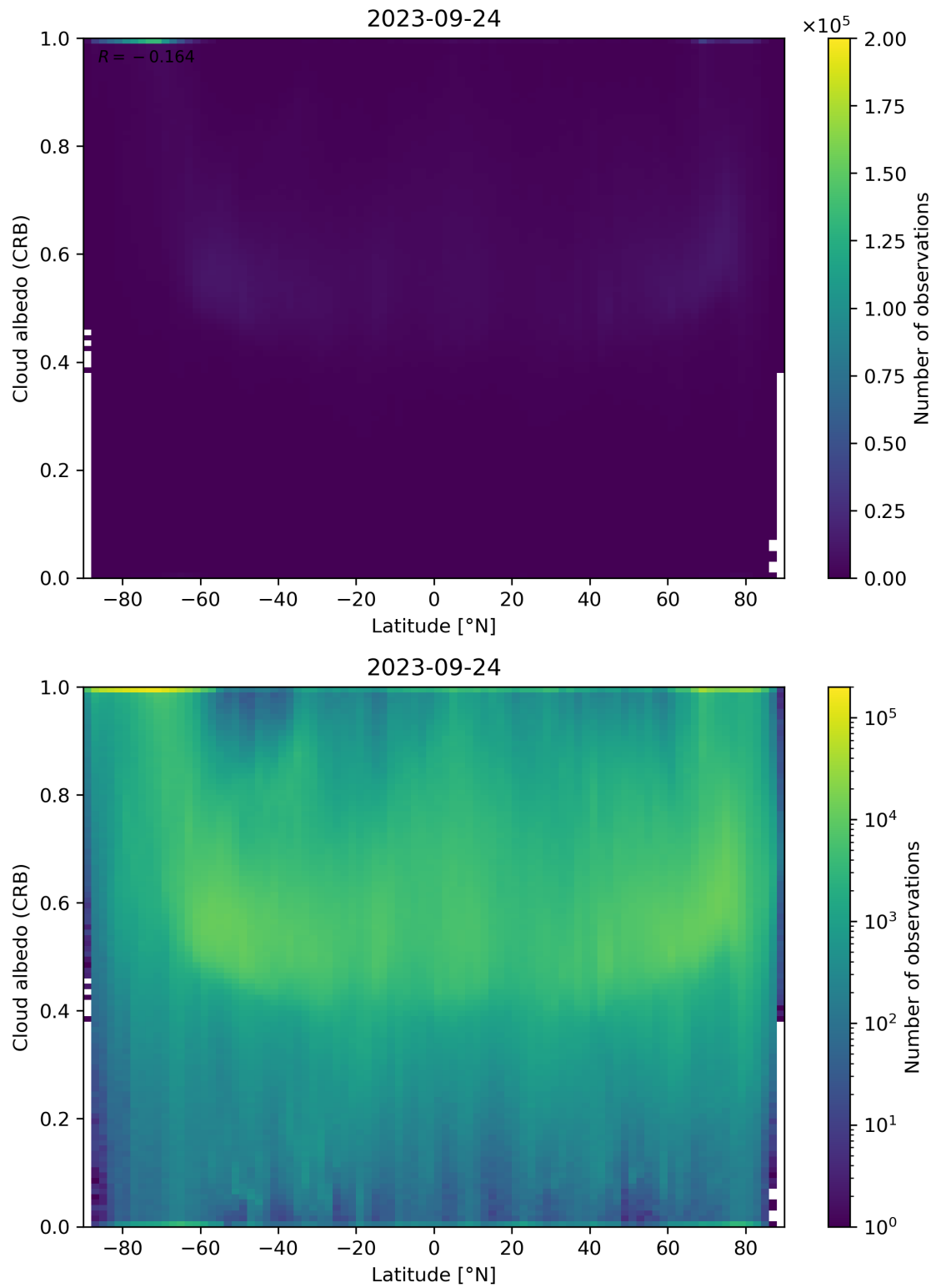
Figure 91: Scatter density plot of “Latitude” against “Cloud albedo (CRB)” for 2023-09-23 to 2023-09-25.
