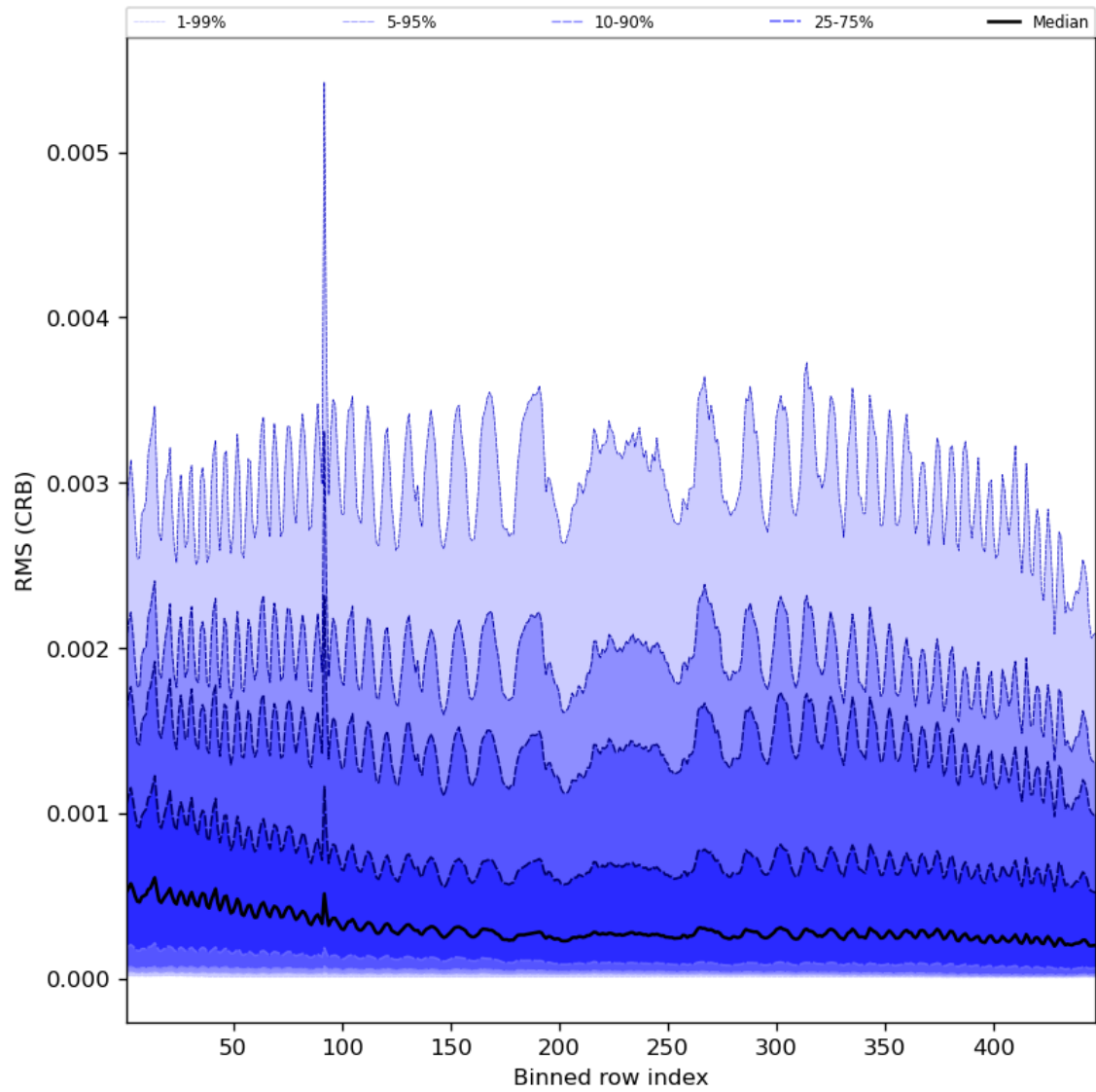
Figure 64: Along track statistics of “RMS (CRB)” for 2023-09-23 to 2023-09-25
