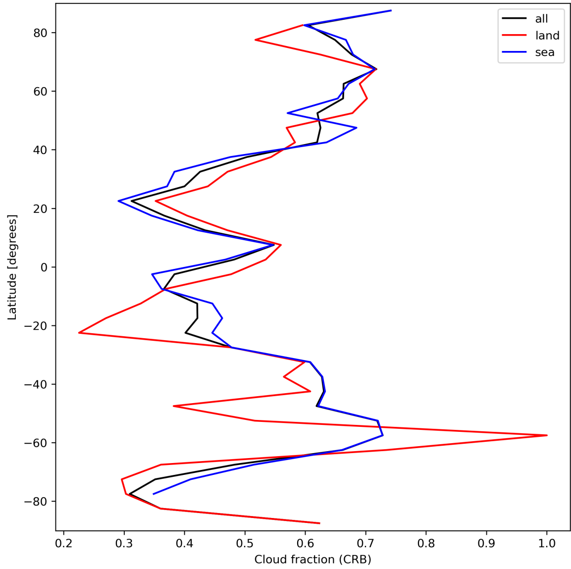
Figure 26: Zonal average of “Cloud fraction (CRB)” for 2023-09-23 to 2023-09-25.
