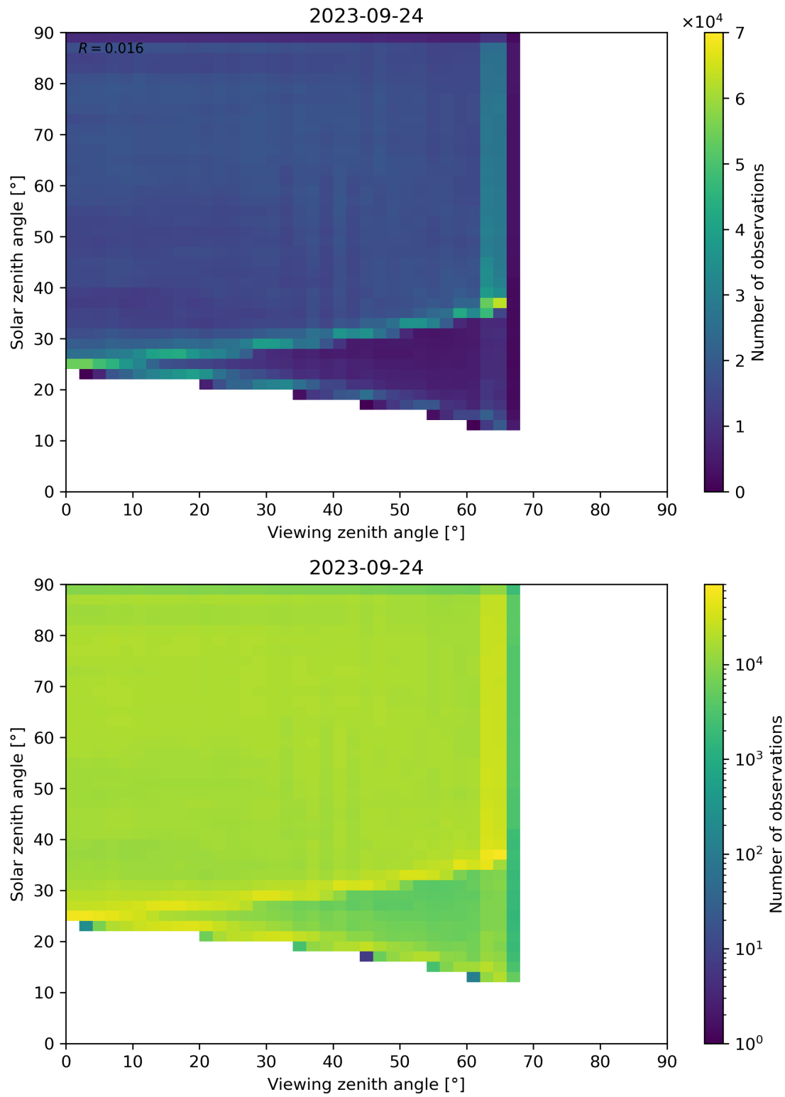
Figure 114: Scatter density plot of “Viewing zenith angle” against “Solar zenith angle” for 2023-09-23 to 2023-09-25.
