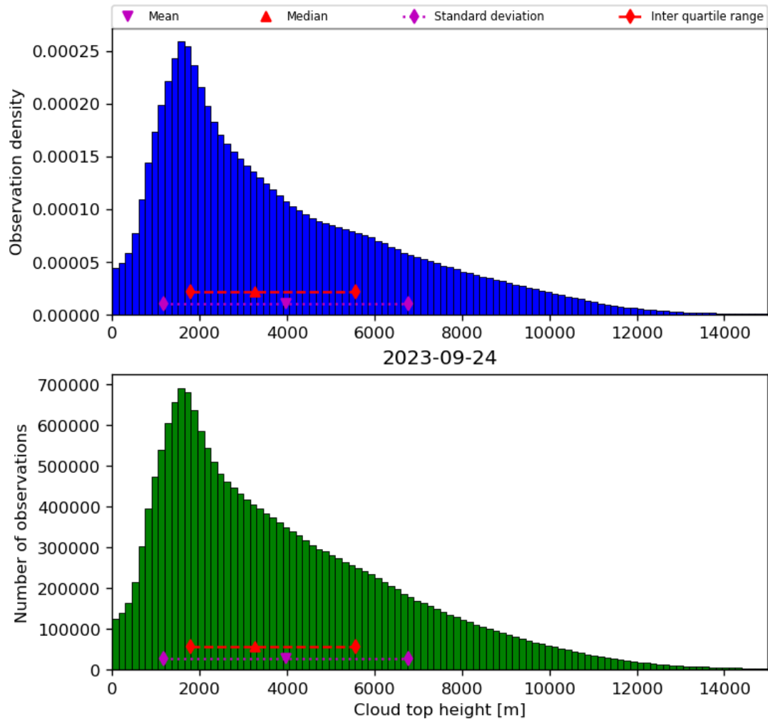
Figure 40: Histogram of “Cloud top height” for 2023-09-23 to 2023-09-25
