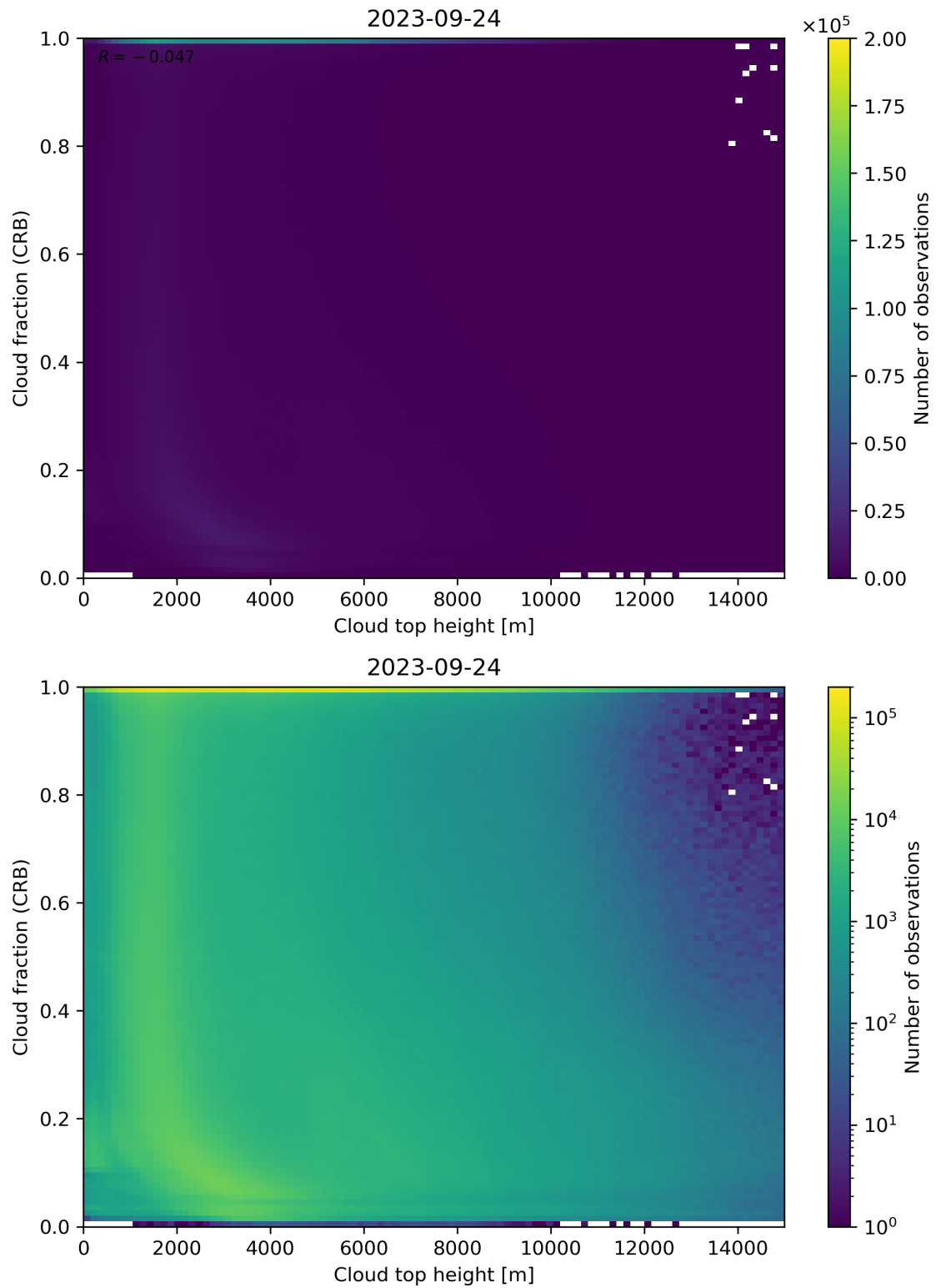
Figure 88: Scatter density plot of “Cloud top height” against “Cloud fraction (CRB)” for 2023-09-23 to 2023-09-25.
