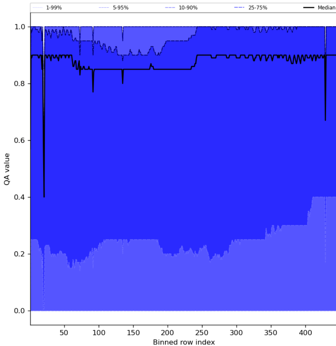
Figure 54: Along track statistics of “QA value” for 2023-09-23 to 2023-09-25
