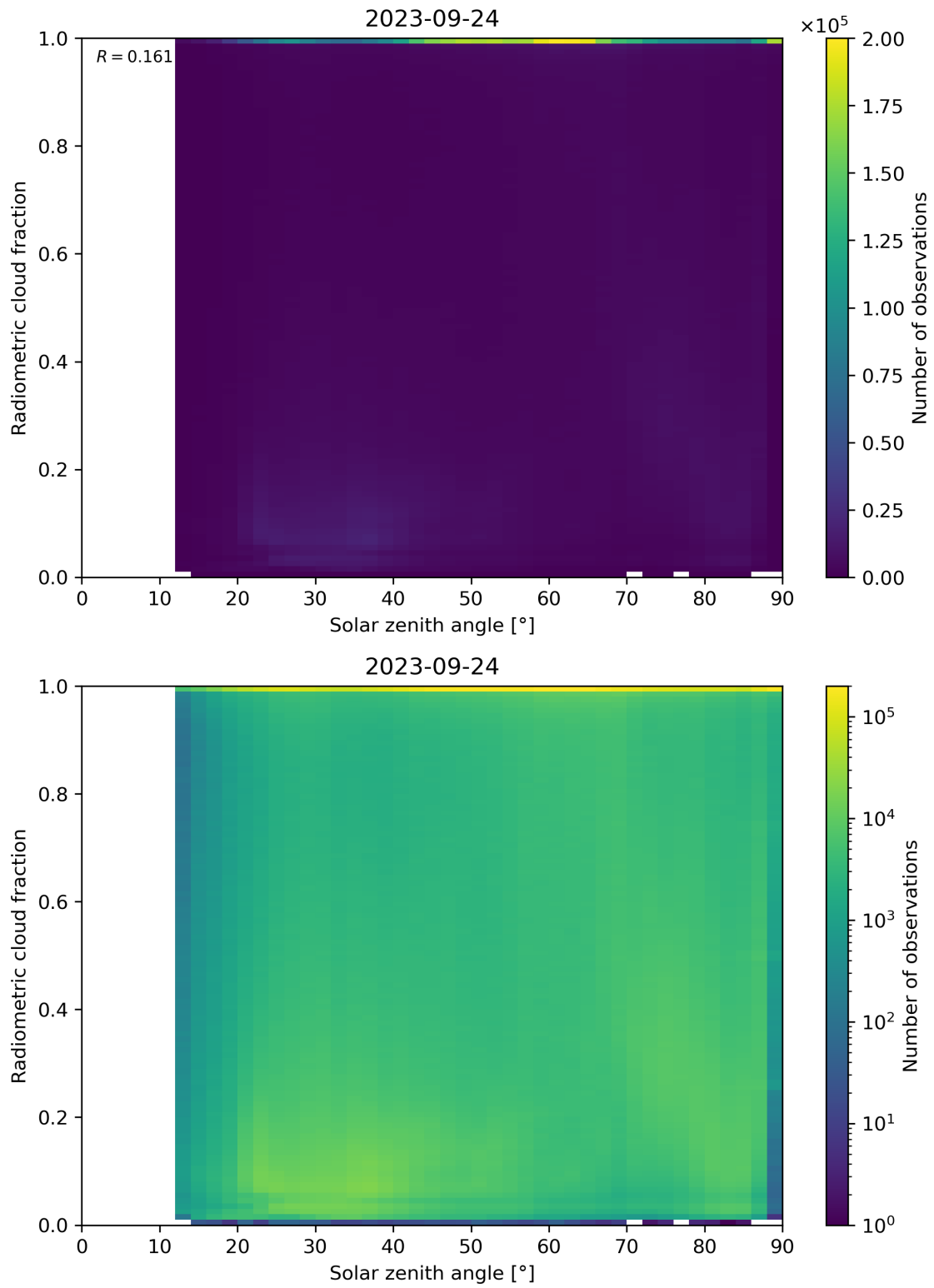
Figure 99: Scatter density plot of “Solar zenith angle” against “Radiometric cloud fraction” for 2023-09-23 to 2023-09-25.
