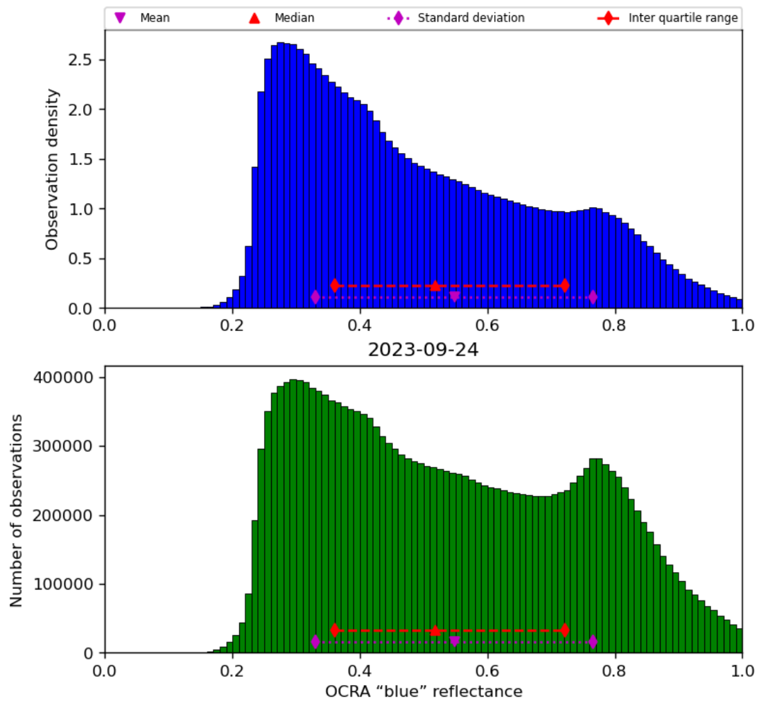
Figure 51: Histogram of “OCRA “blue” reflectance” for 2023-09-23 to 2023-09-25
