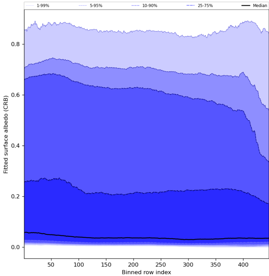
Figure 62: Along track statistics of “Fitted surface albedo (CRB)” for 2023-09-23 to 2023-09-25
