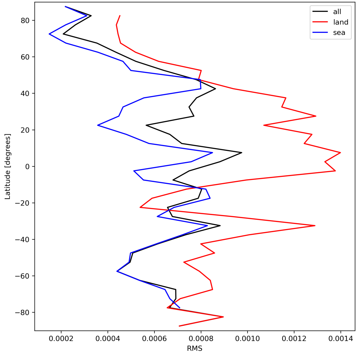
Figure 31: Zonal average of “RMS” for 2023-09-23 to 2023-09-25.
