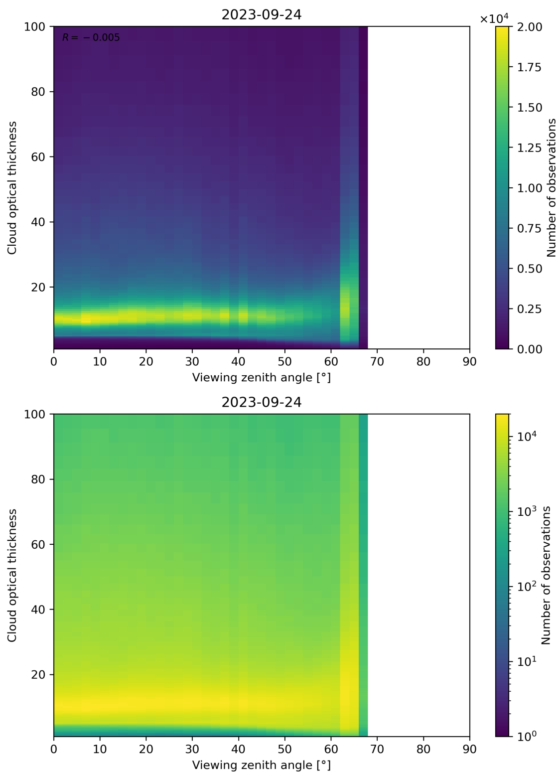
Figure 111: Scatter density plot of “Viewing zenith angle” against “Cloud optical thickness” for 2023-09-23 to 2023-09-25.
