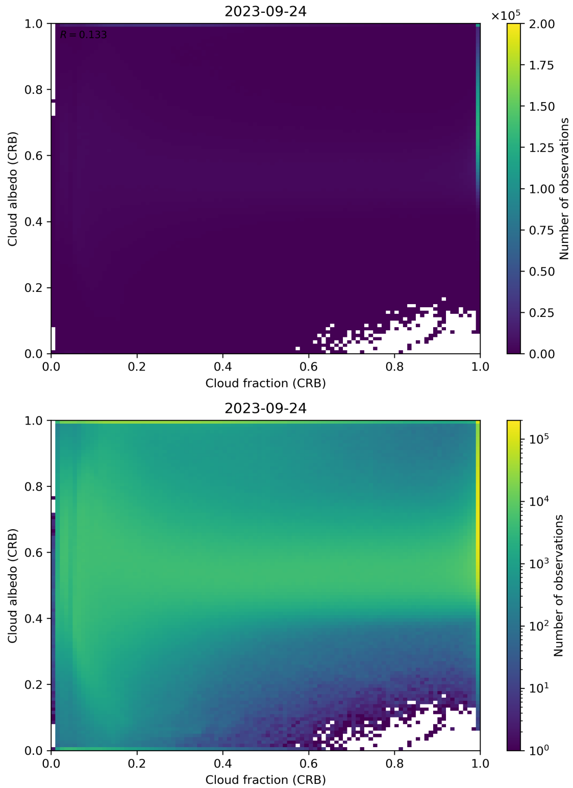
Figure 77: Scatter density plot of “Cloud fraction (CRB)” against “Cloud albedo (CRB)” for 2023-09-23 to 2023-09-25.
