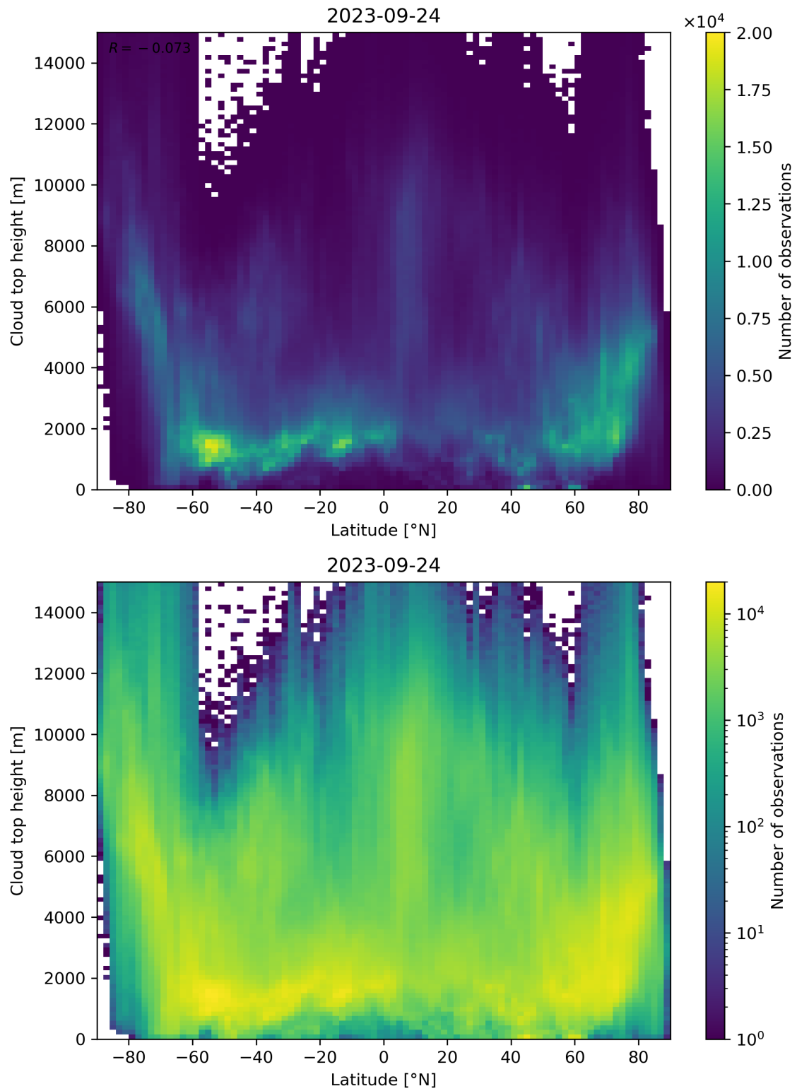
Figure 97: Scatter density plot of “Latitude” against “Cloud top height” for 2023-09-23 to 2023-09-25.
