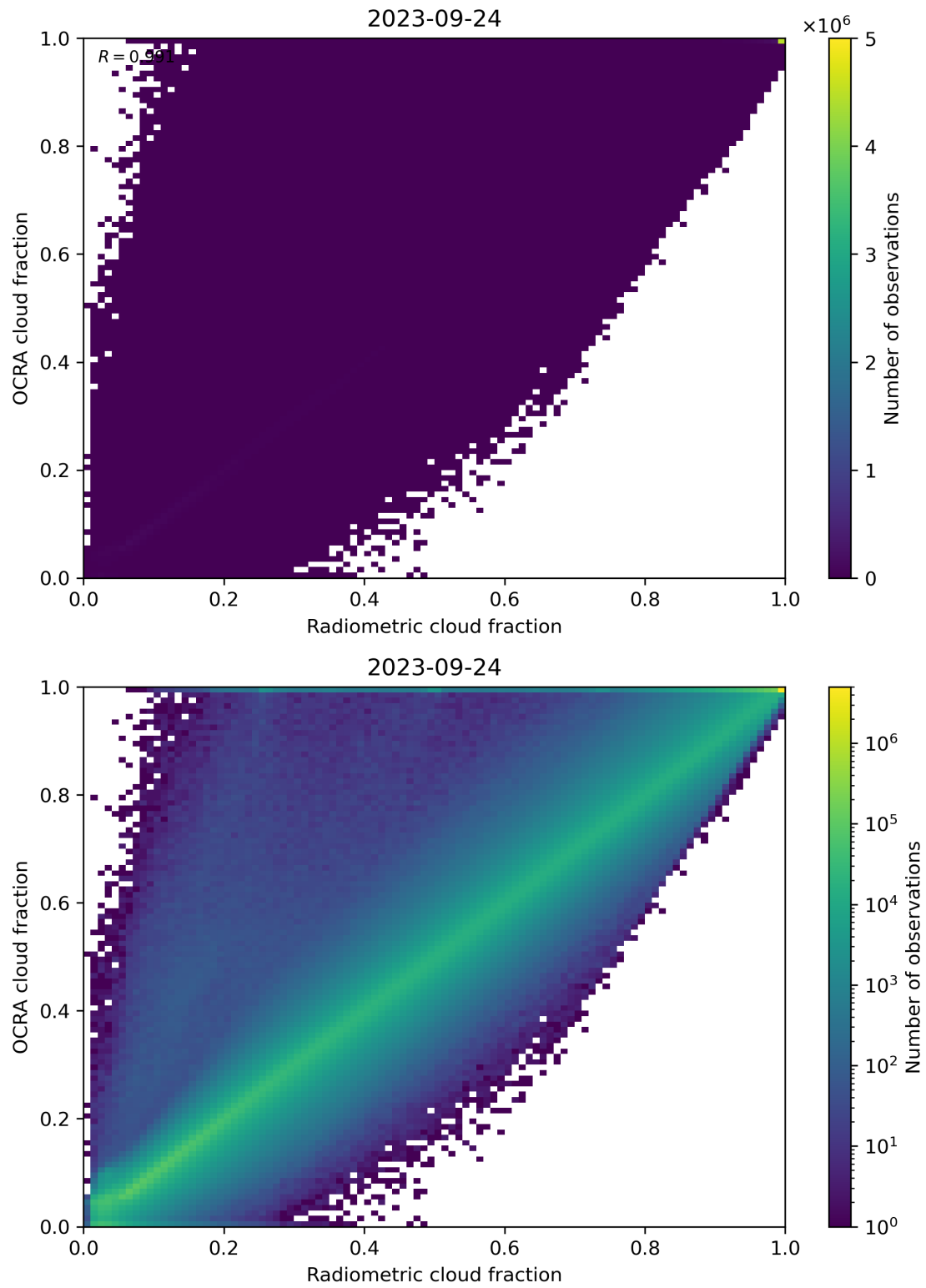
Figure 72: Scatter density plot of “Radiometric cloud fraction” against “OCRA cloud fraction” for 2023-09-23 to 2023-09-25.
