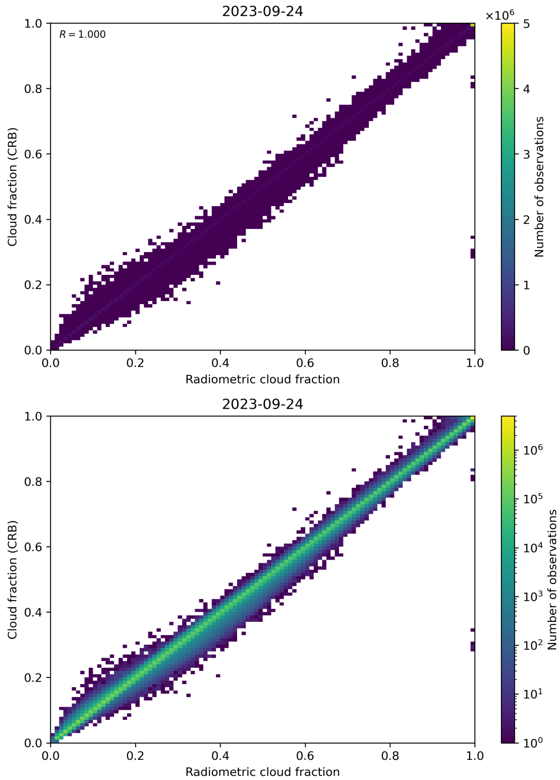
Figure 73: Scatter density plot of “Radiometric cloud fraction” against “Cloud fraction (CRB)” for 2023-09-23 to 2023-09-25.
