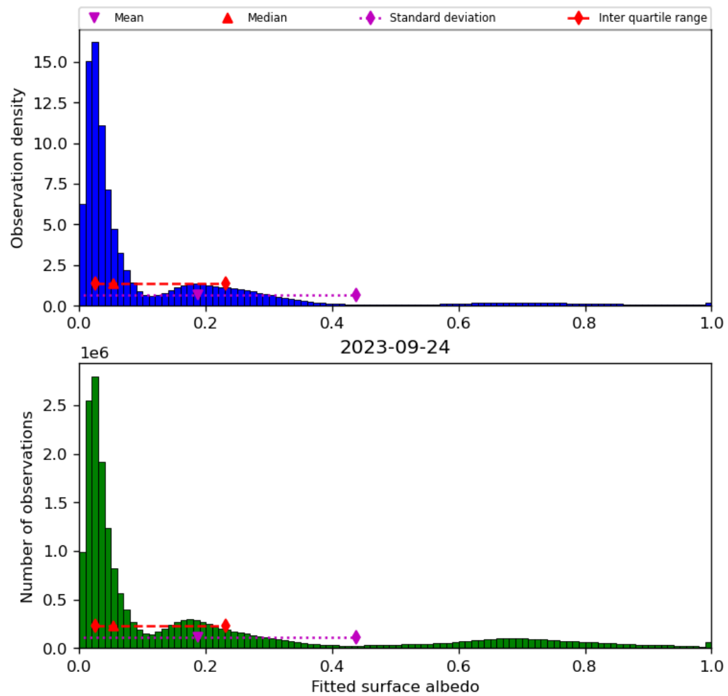
Figure 45: Histogram of “Fitted surface albedo” for 2023-09-23 to 2023-09-25
