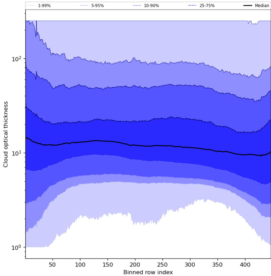
Figure 57: Along track statistics of “Cloud optical thickness” for 2023-09-23 to 2023-09-25
