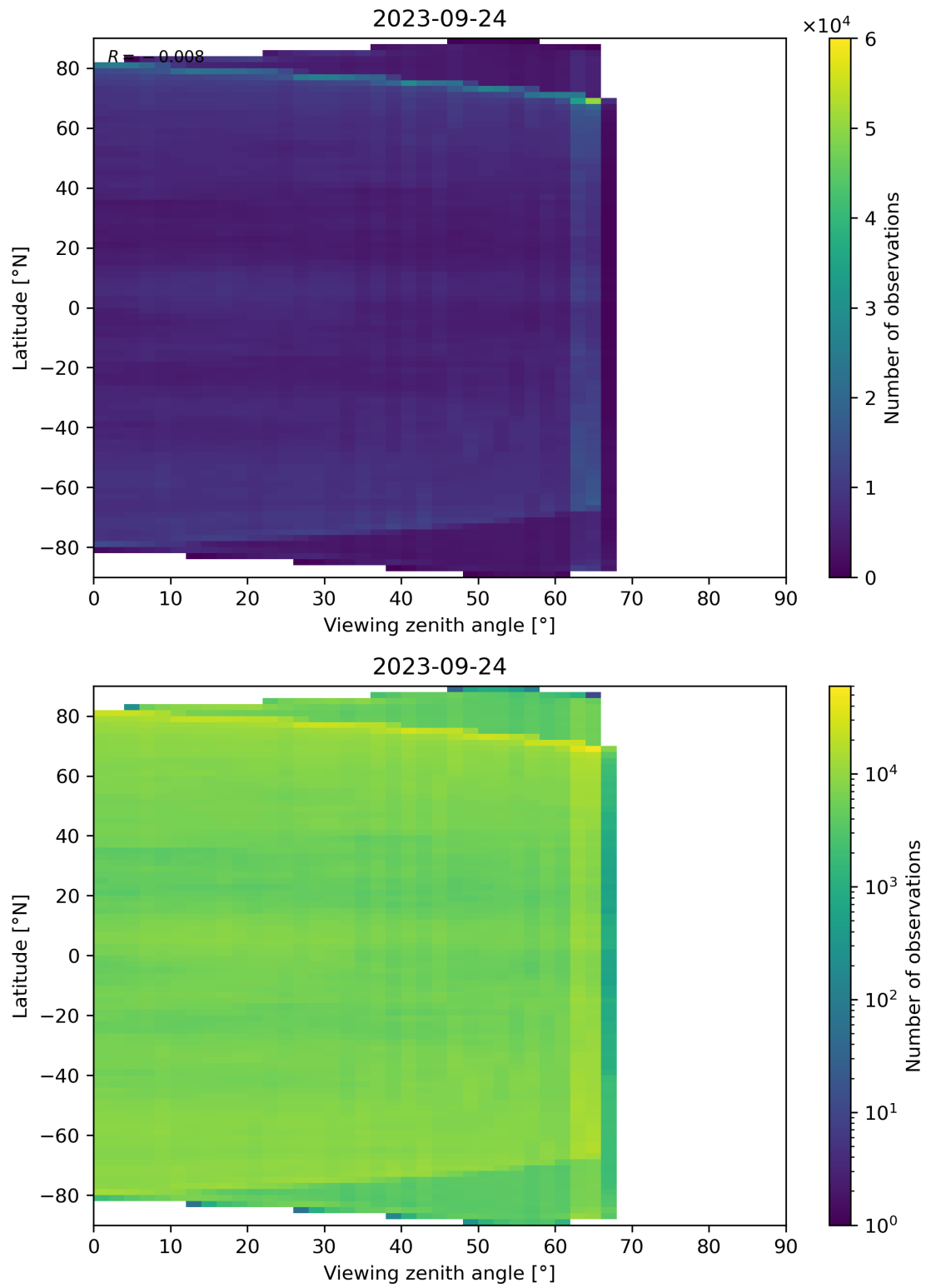
Figure 113: Scatter density plot of “Viewing zenith angle” against “Latitude” for 2023-09-23 to 2023-09-25.
