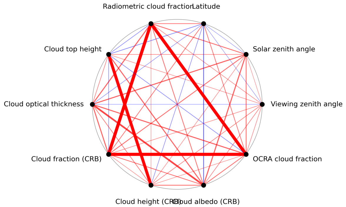
Figure 1: Map of correlation graph for 2023-09-23 to 2023-09-25.
