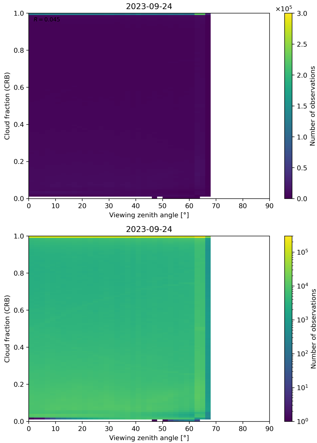
Figure 109: Scatter density plot of “Viewing zenith angle” against “Cloud fraction (CRB)” for 2023-09-23 to 2023-09-25.
