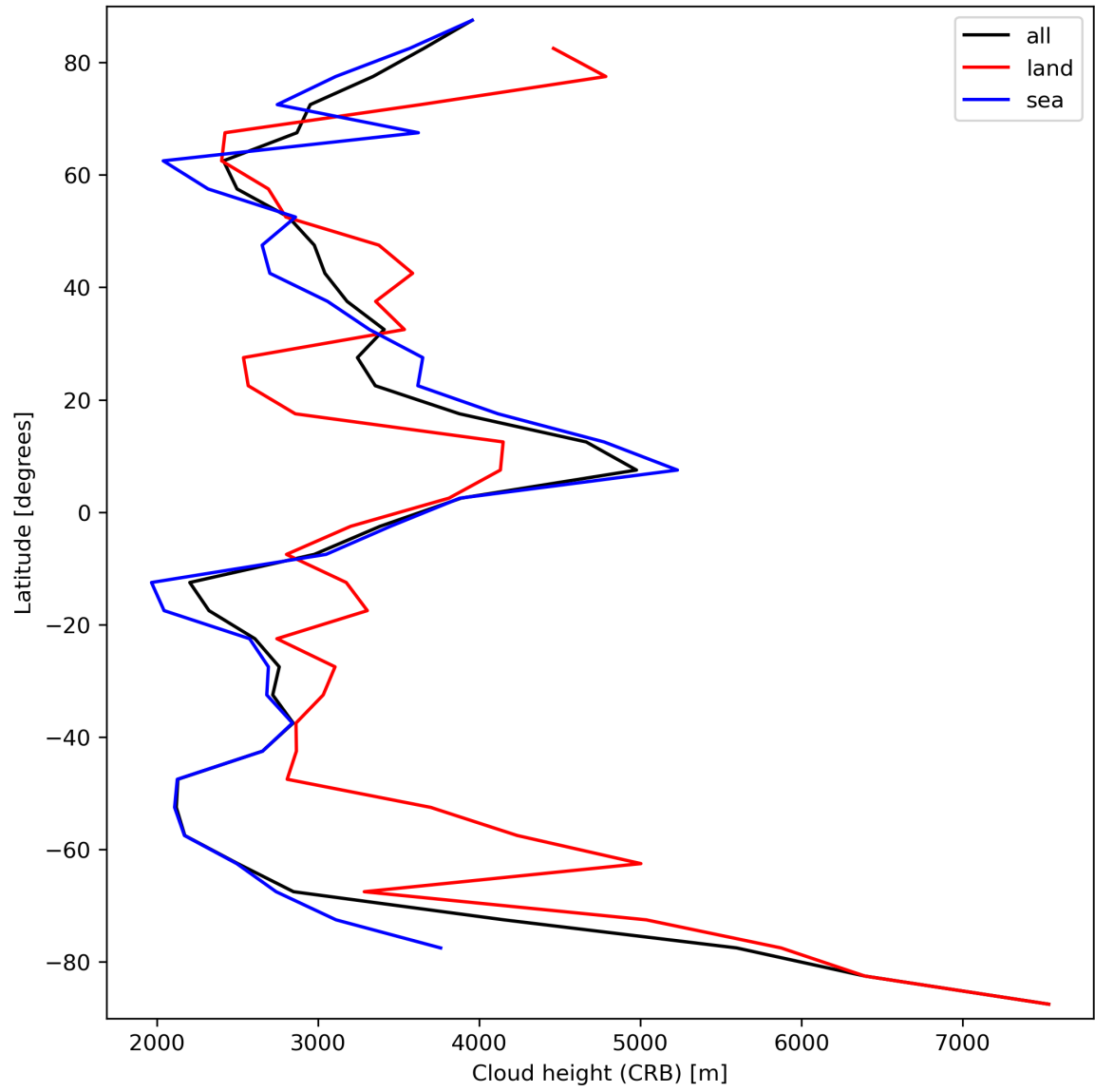
Figure 27: Zonal average of “Cloud height (CRB)” for 2023-09-23 to 2023-09-25.
