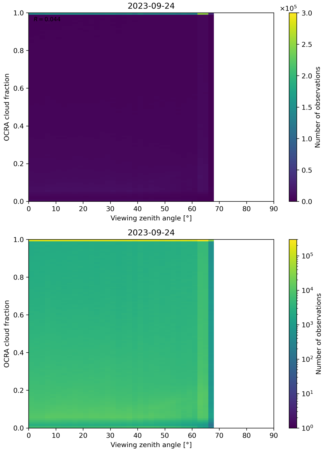
Figure 108: Scatter density plot of “Viewing zenith angle” against “OCRA cloud fraction” for 2023-09-23 to 2023-09-25.
