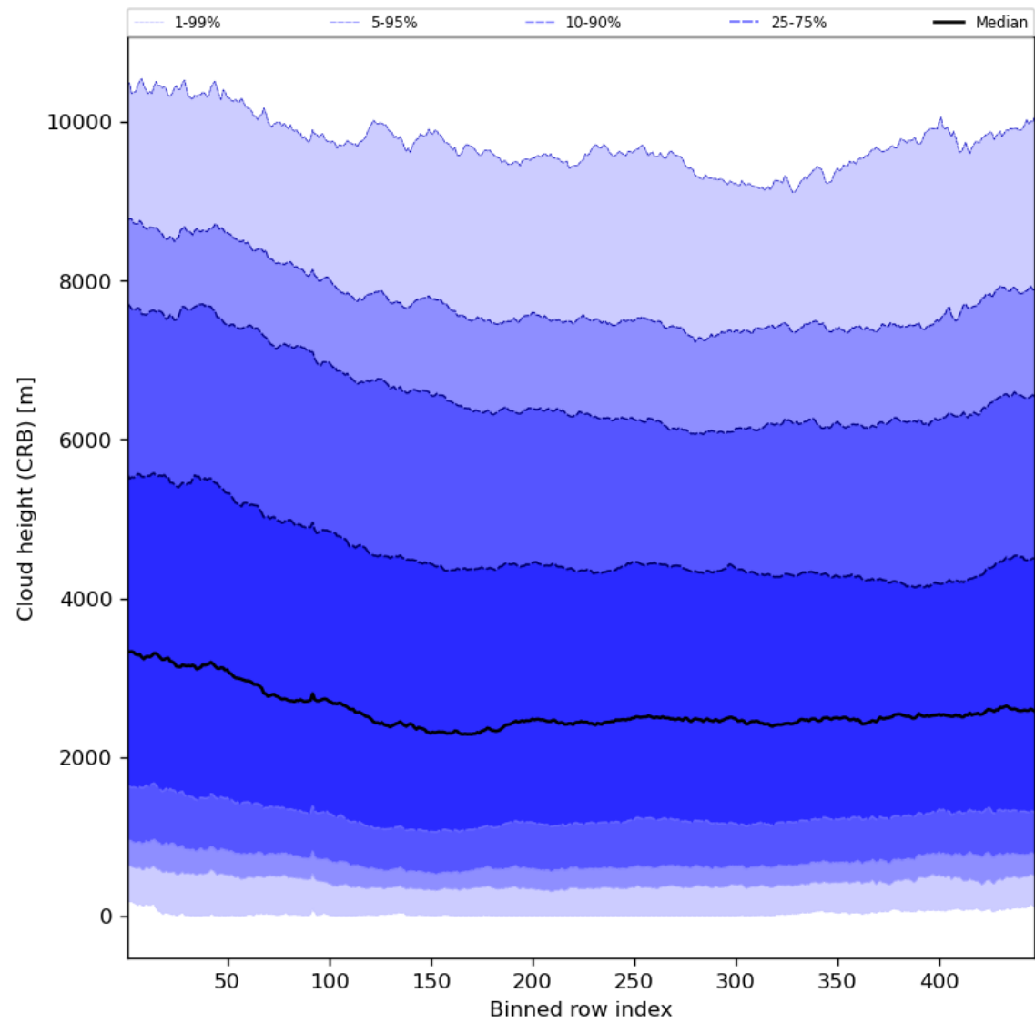
Figure 59: Along track statistics of “Cloud height (CRB)” for 2023-09-23 to 2023-09-25
