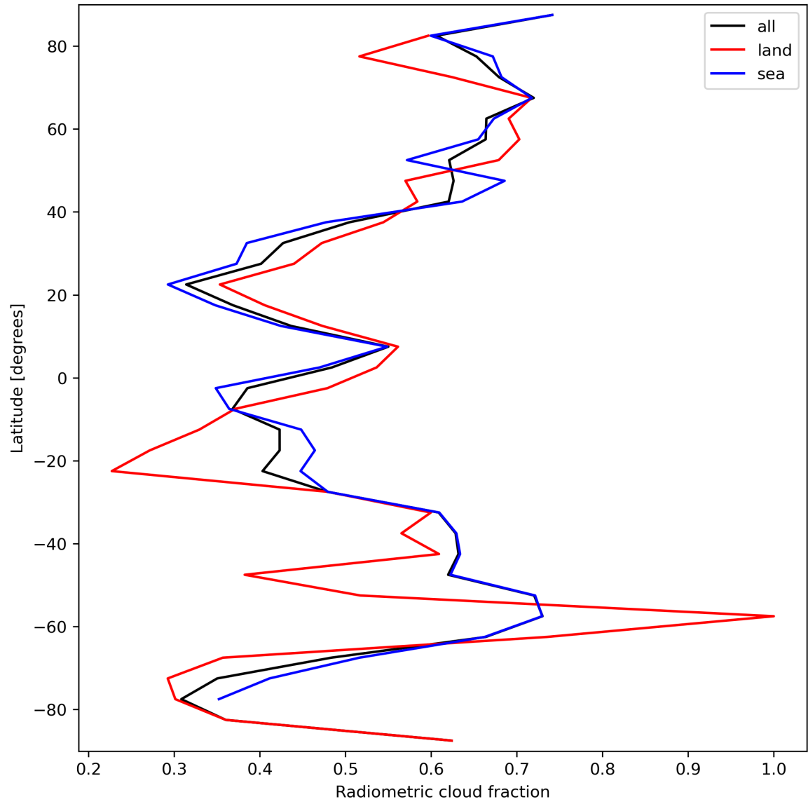
Figure 23: Zonal average of “Radiometric cloud fraction” for 2023-09-23 to 2023-09-25.
