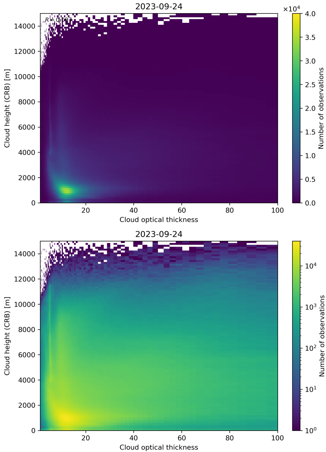
Figure 85: Scatter density plot of “Cloud optical thickness” against “Cloud height (CRB)” for 2023-09-23 to 2023-09-25.
