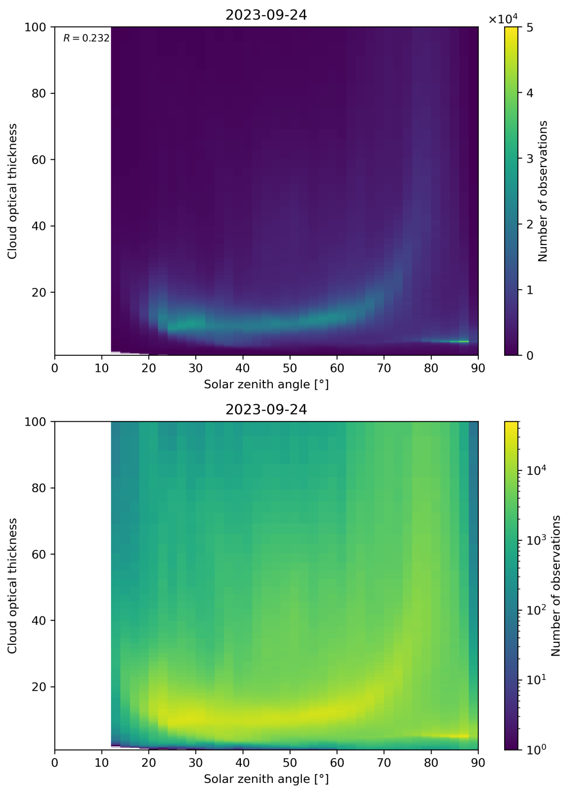
Figure 103: Scatter density plot of “Solar zenith angle” against “Cloud optical thickness” for 2023-09-23 to 2023-09-25.
