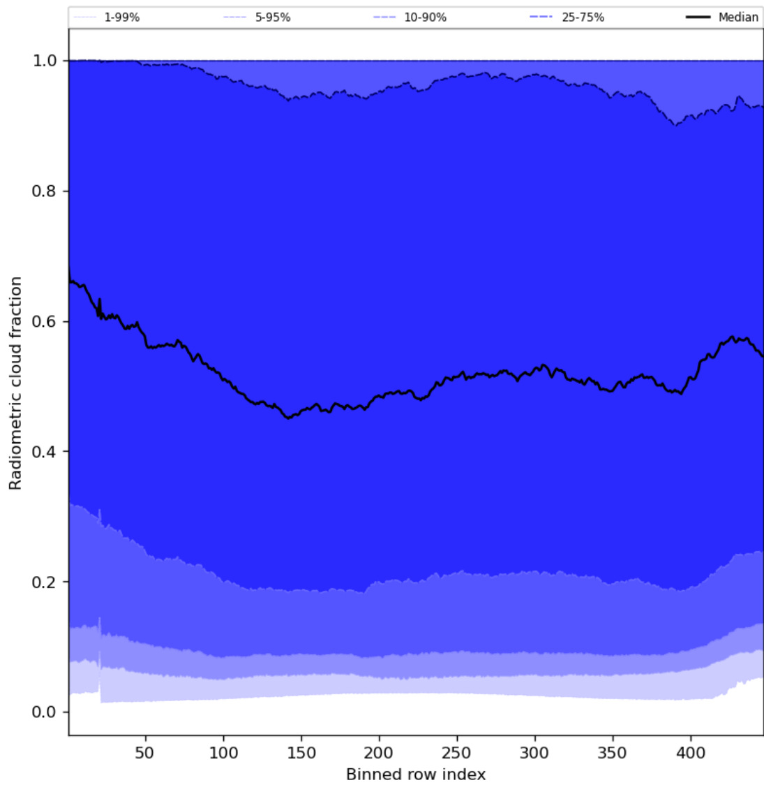
Figure 55: Along track statistics of “Radiometric cloud fraction” for 2023-09-23 to 2023-09-25
