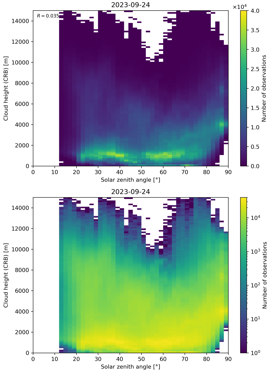
Figure 102: Scatter density plot of “Solar zenith angle” against “Cloud height (CRB)” for 2023-09-23 to 2023-09-25.
