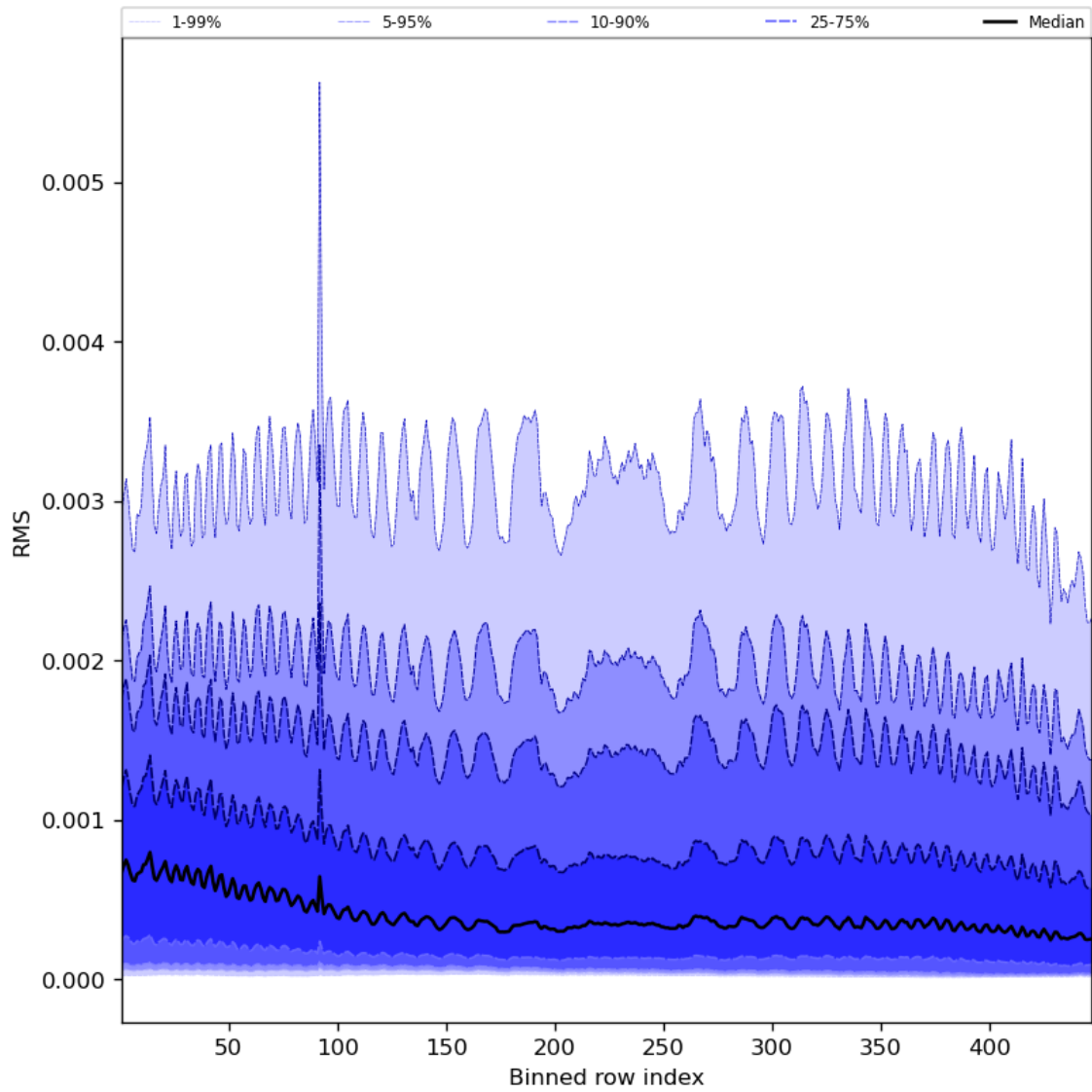
Figure 63: Along track statistics of “RMS” for 2023-09-23 to 2023-09-25
