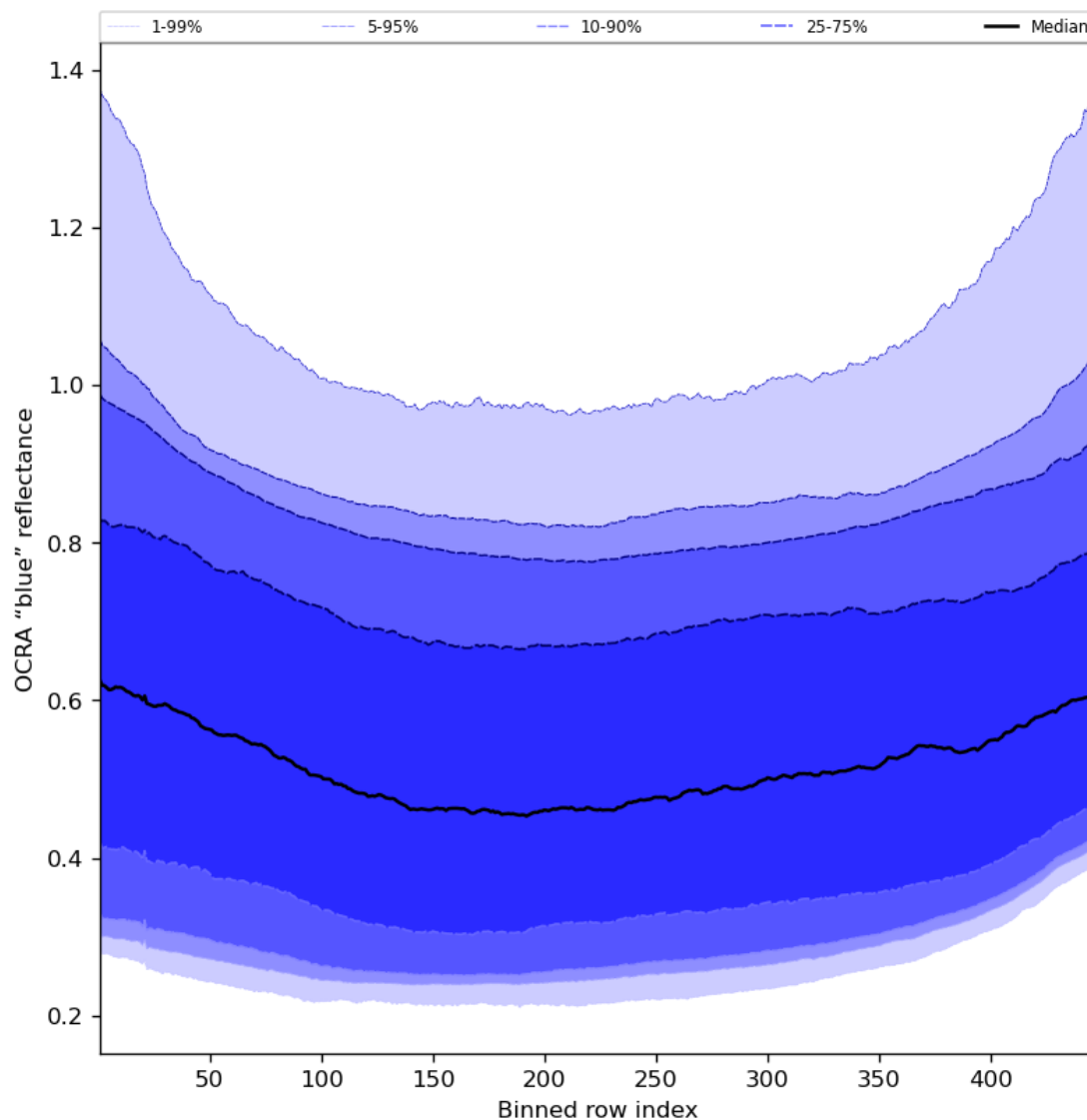
Figure 67: Along track statistics of “OCRA “blue” reflectance” for 2023-09-23 to 2023-09-25
