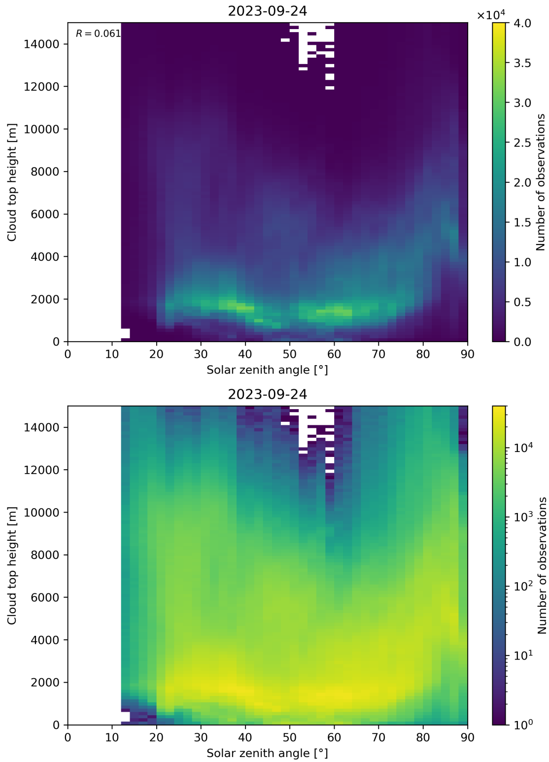
Figure 104: Scatter density plot of “Solar zenith angle” against “Cloud top height” for 2023-09-23 to 2023-09-25.
