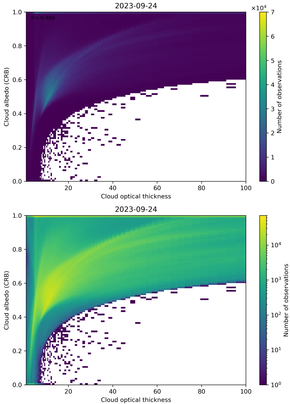
Figure 82: Scatter density plot of “Cloud optical thickness” against “Cloud albedo (CRB)” for 2023-09-23 to 2023-09-25.
