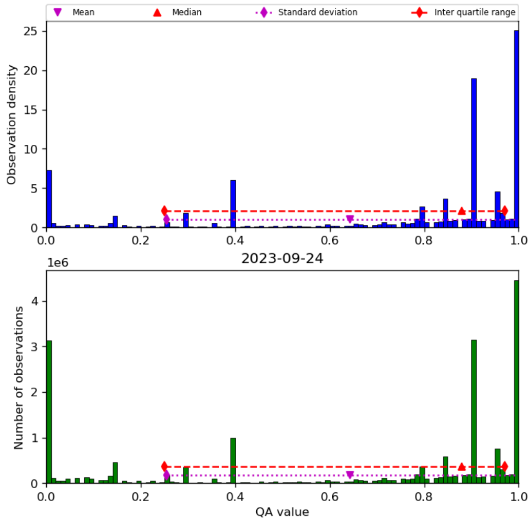
Figure 38: Histogram of “QA value” for 2023-09-23 to 2023-09-25
