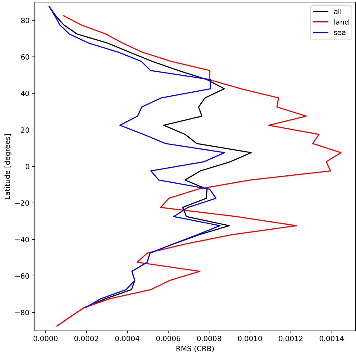
Figure 32: Zonal average of “RMS (CRB)” for 2023-09-23 to 2023-09-25.
