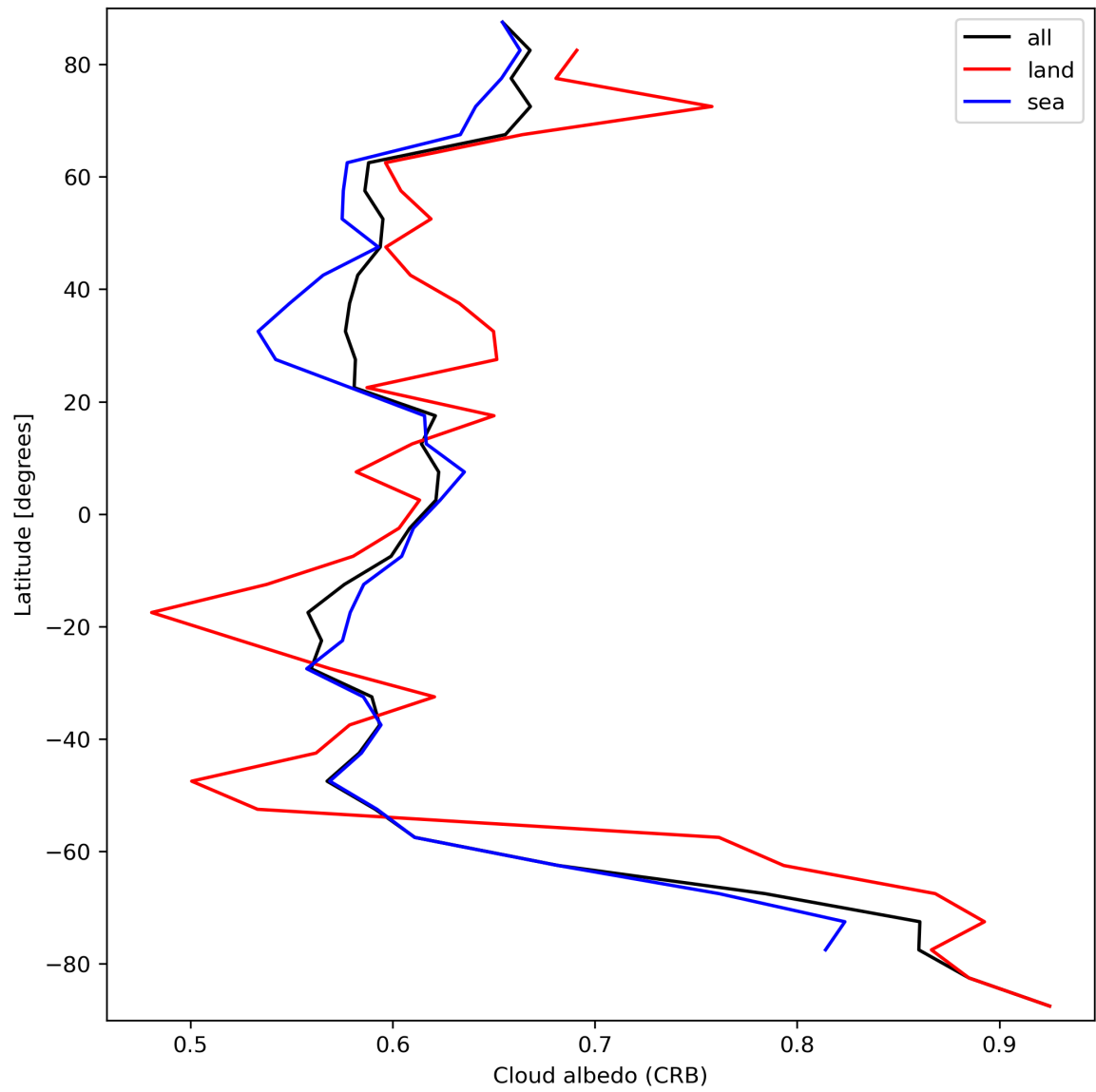
Figure 28: Zonal average of “Cloud albedo (CRB)” for 2023-09-23 to 2023-09-25.
