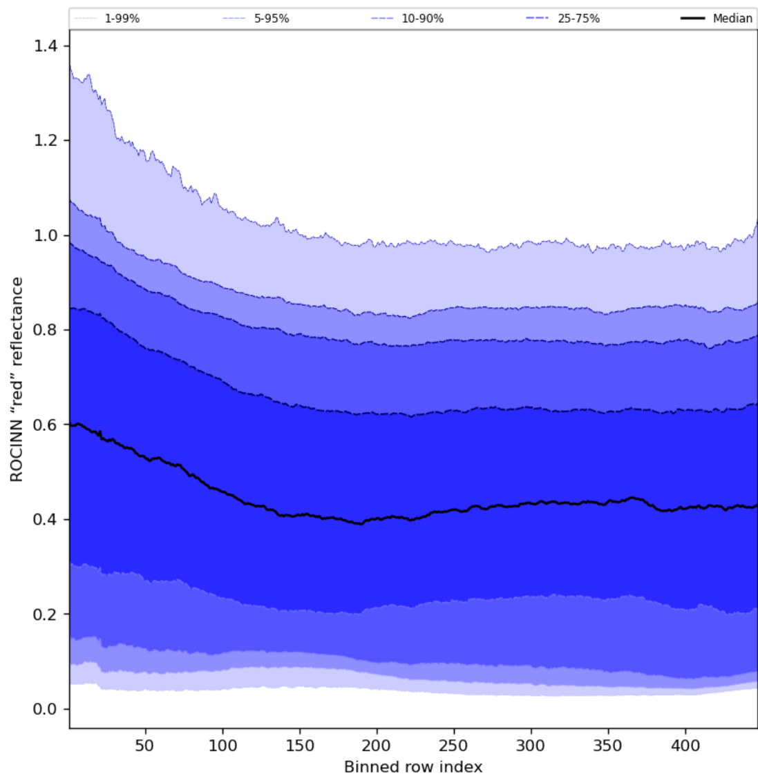
Figure 69: Along track statistics of “ROCINN “red” reflectance” for 2023-09-23 to 2023-09-25
