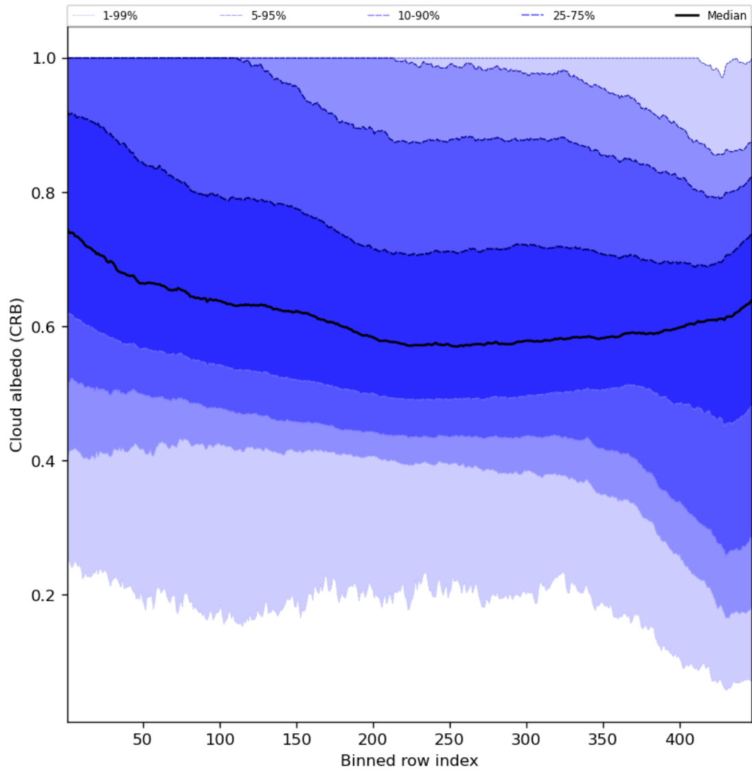
Figure 60: Along track statistics of “Cloud albedo (CRB)” for 2023-09-23 to 2023-09-25
