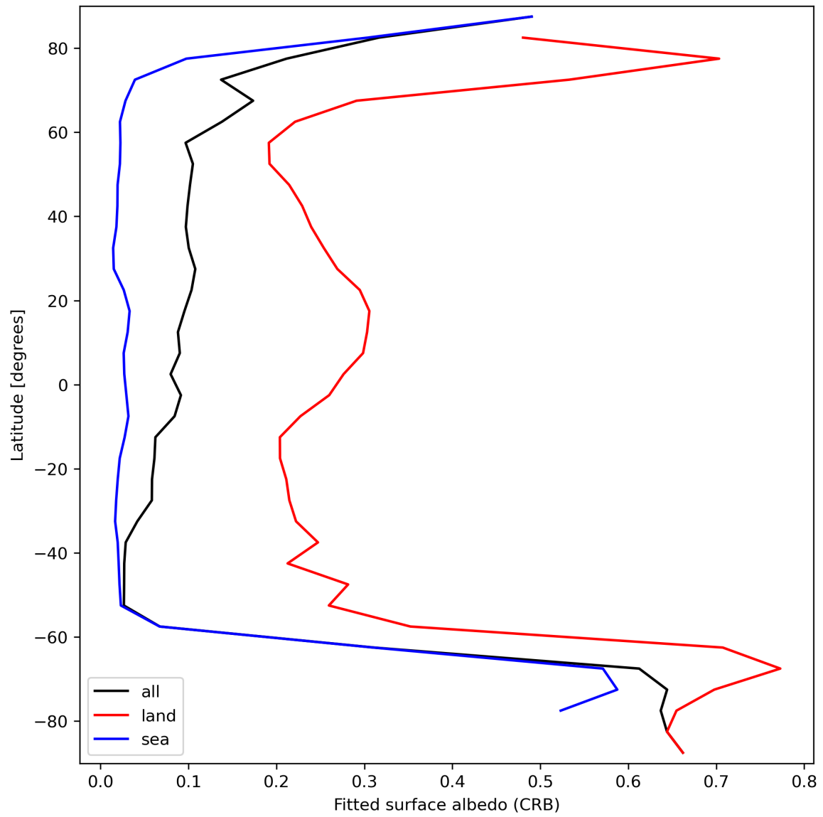
Figure 30: Zonal average of “Fitted surface albedo (CRB)” for 2023-09-23 to 2023-09-25.
