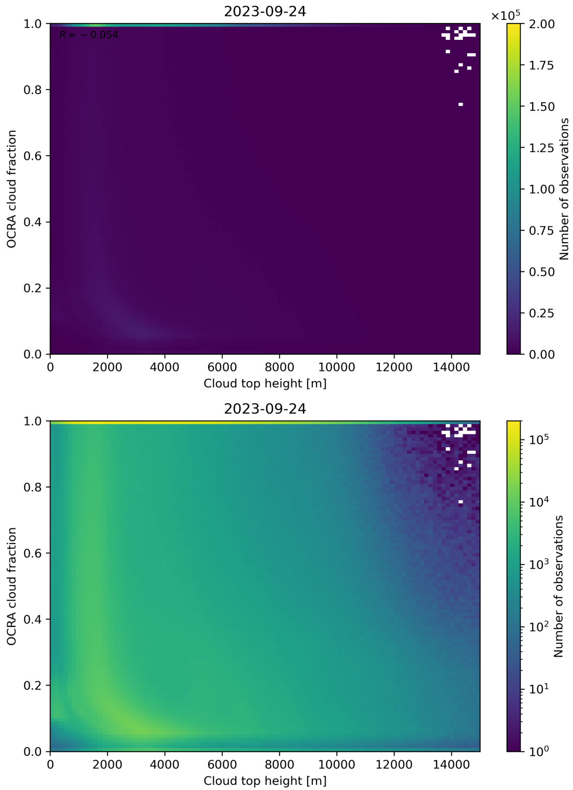
Figure 87: Scatter density plot of “Cloud top height” against “OCRA cloud fraction” for 2023-09-23 to 2023-09-25.
