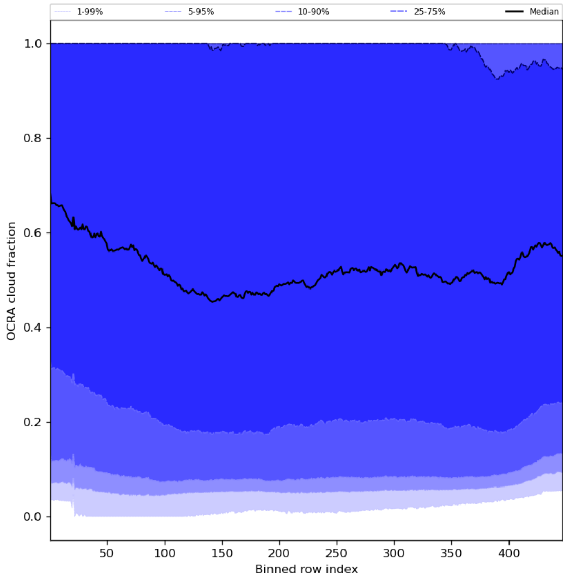
Figure 66: Along track statistics of “OCRA cloud fraction” for 2023-09-23 to 2023-09-25
