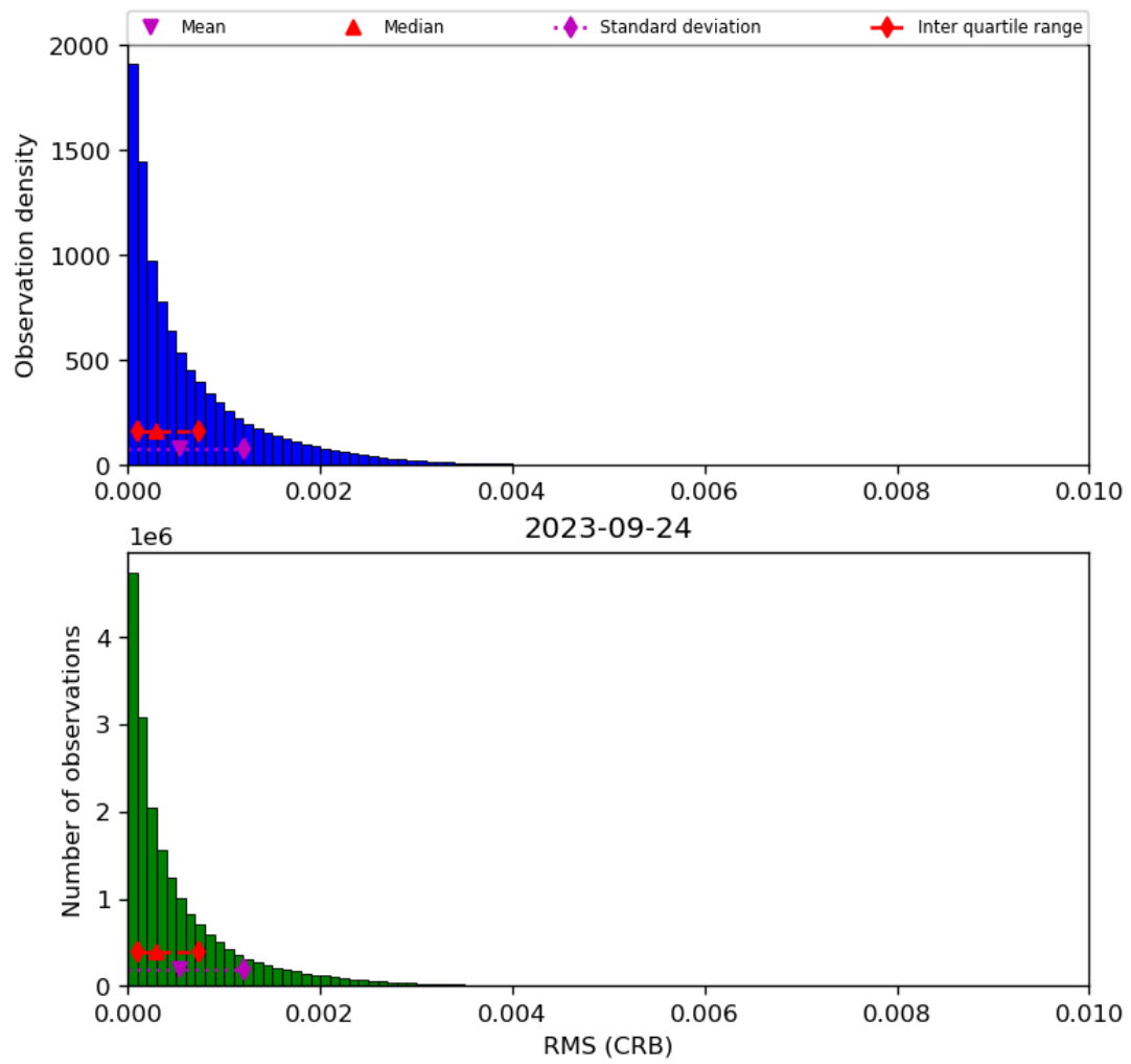
Figure 48: Histogram of “RMS (CRB)” for 2023-09-23 to 2023-09-25
