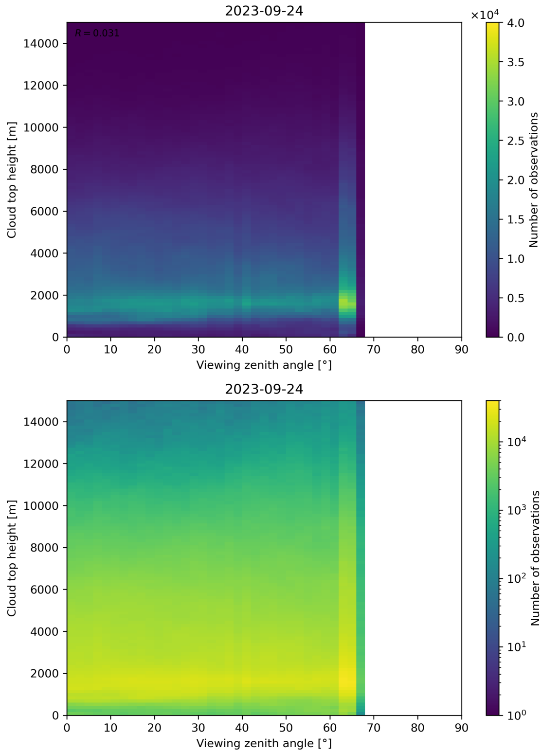
Figure 112: Scatter density plot of “Viewing zenith angle” against “Cloud top height” for 2023-09-23 to 2023-09-25.
