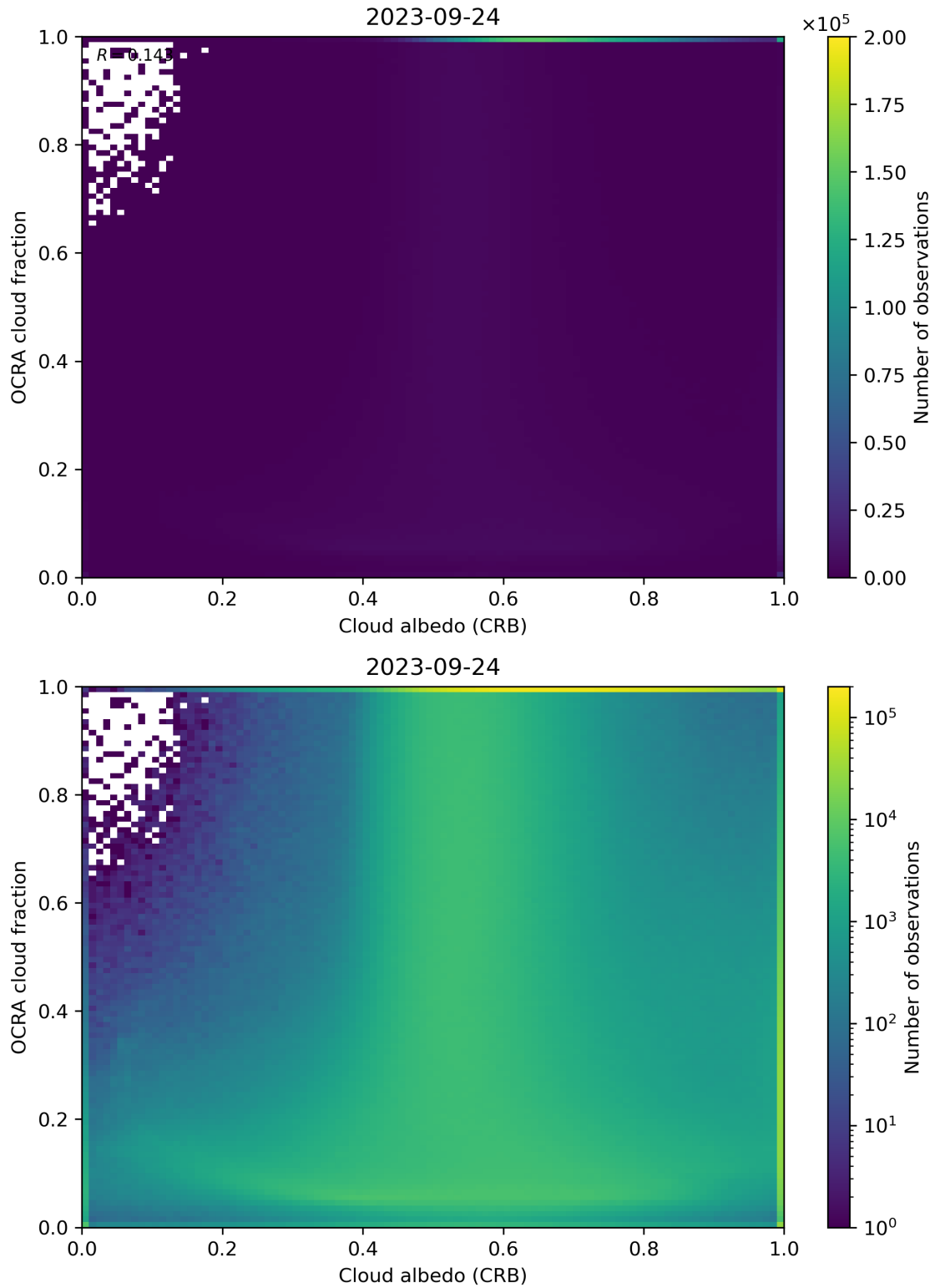
Figure 70: Scatter density plot of “Cloud albedo (CRB)” against “OCRA cloud fraction” for 2023-09-23 to 2023-09-25.
