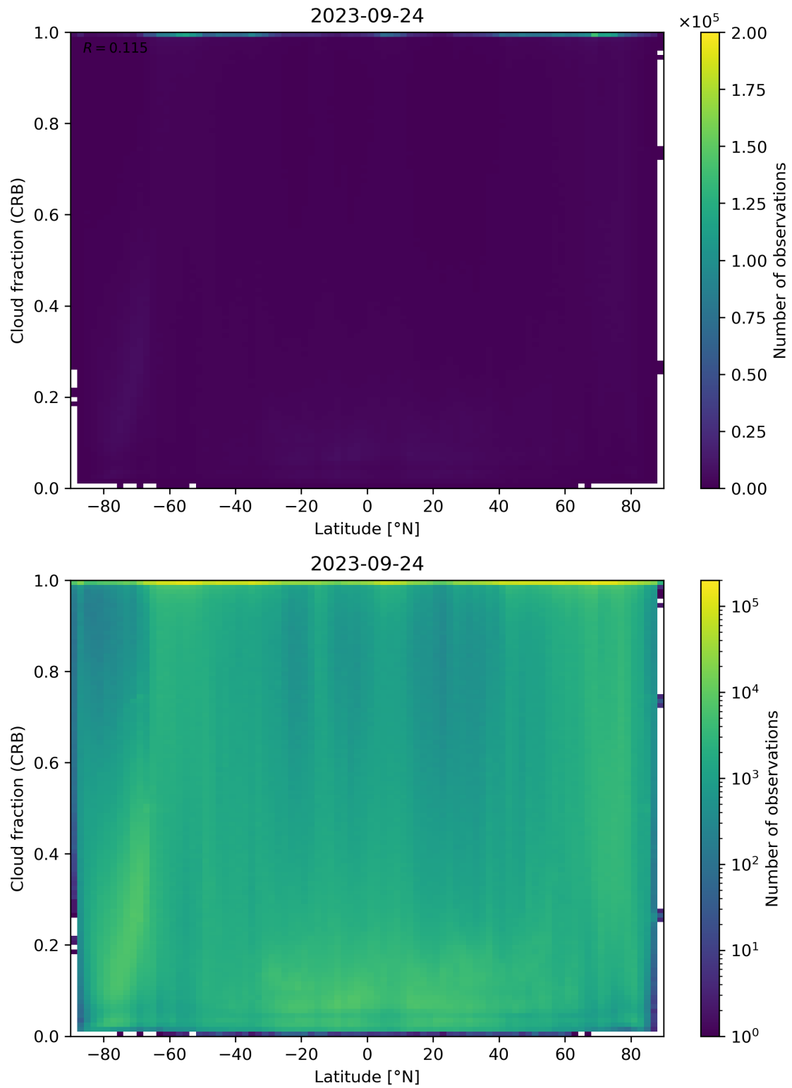
Figure 94: Scatter density plot of “Latitude” against “Cloud fraction (CRB)” for 2023-09-23 to 2023-09-25.
