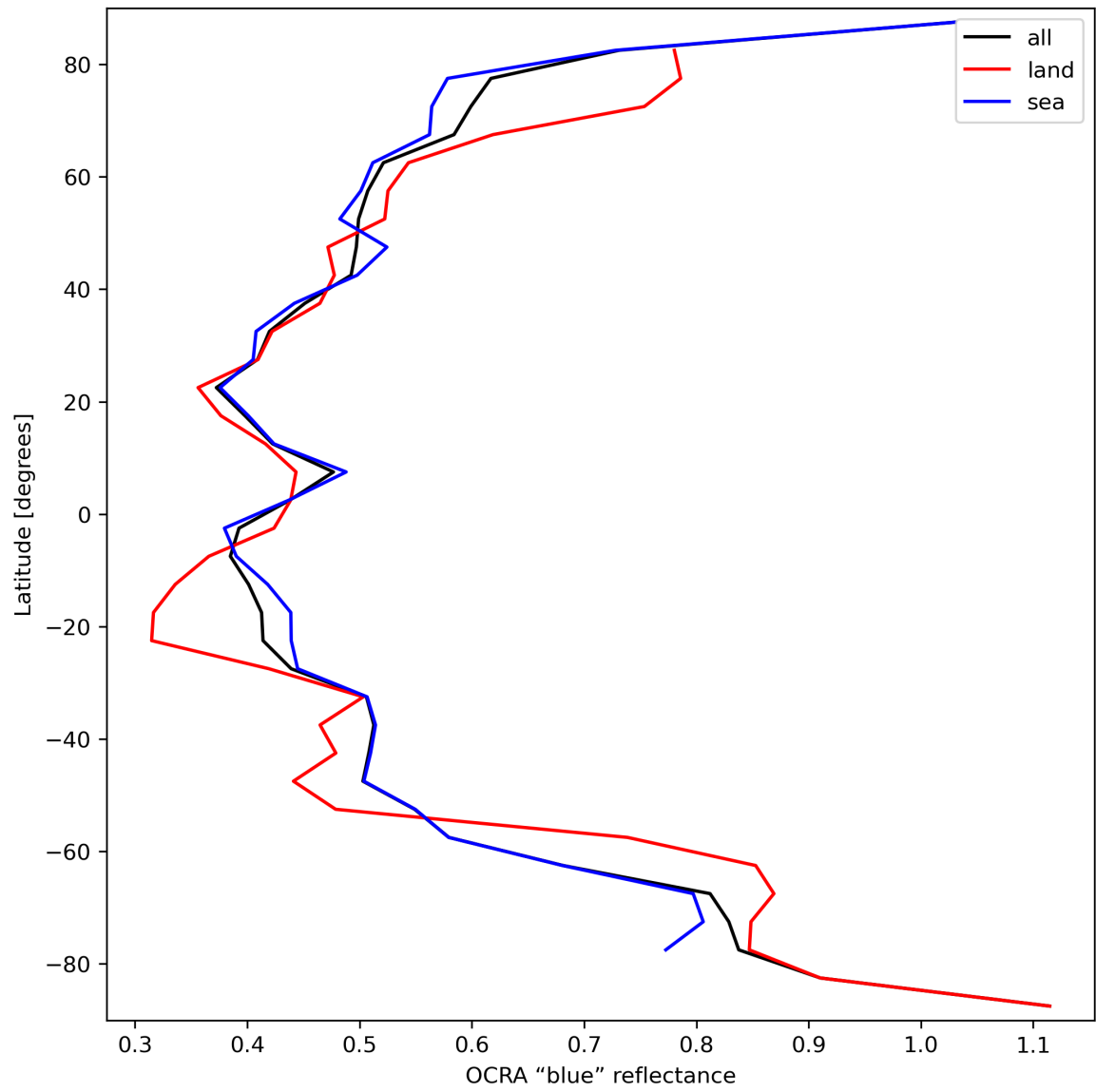
Figure 35: Zonal average of “OCRA “blue” reflectance” for 2023-09-23 to 2023-09-25.
