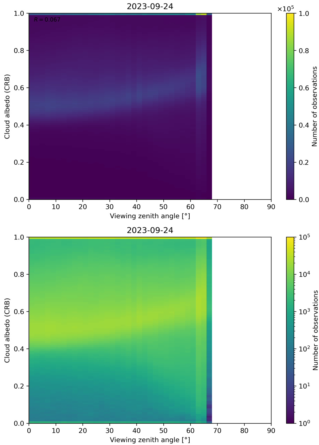
Figure 106: Scatter density plot of “Viewing zenith angle” against “Cloud albedo (CRB)” for 2023-09-23 to 2023-09-25.
