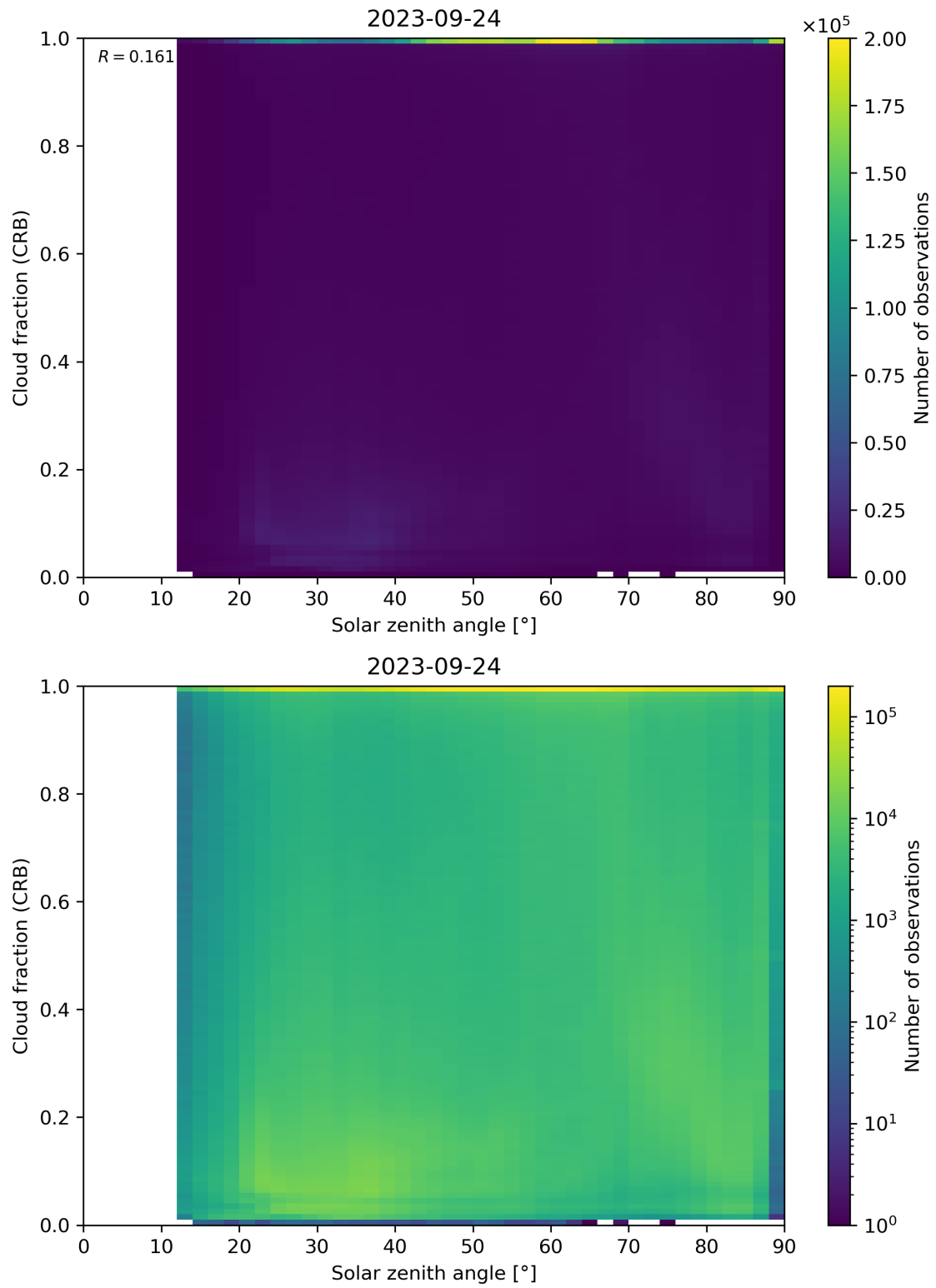
Figure 101: Scatter density plot of “Solar zenith angle” against “Cloud fraction (CRB)” for 2023-09-23 to 2023-09-25.
