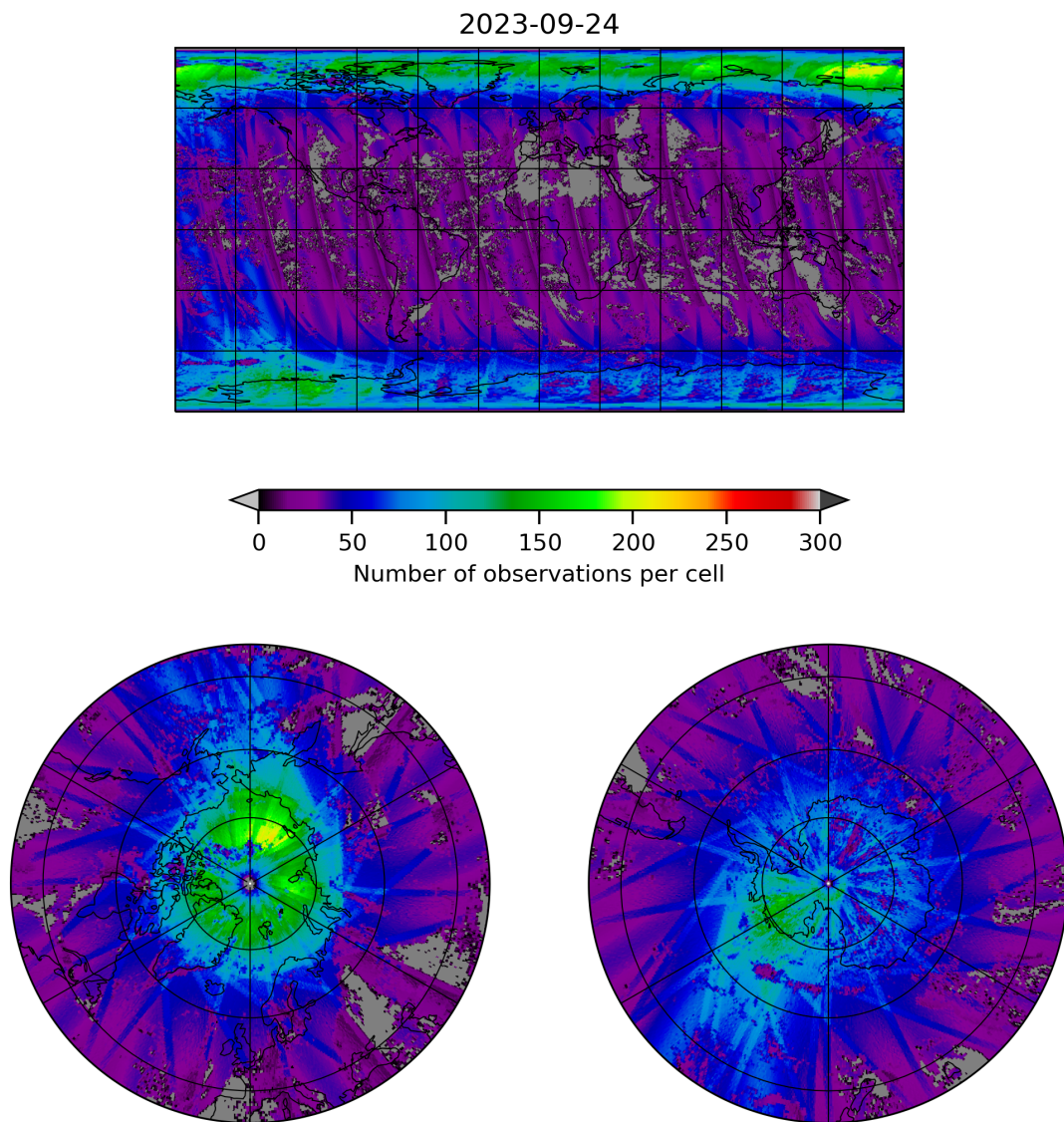
Figure 21: Map of the number of observations for 2023-09-23 to 2023-09-25
