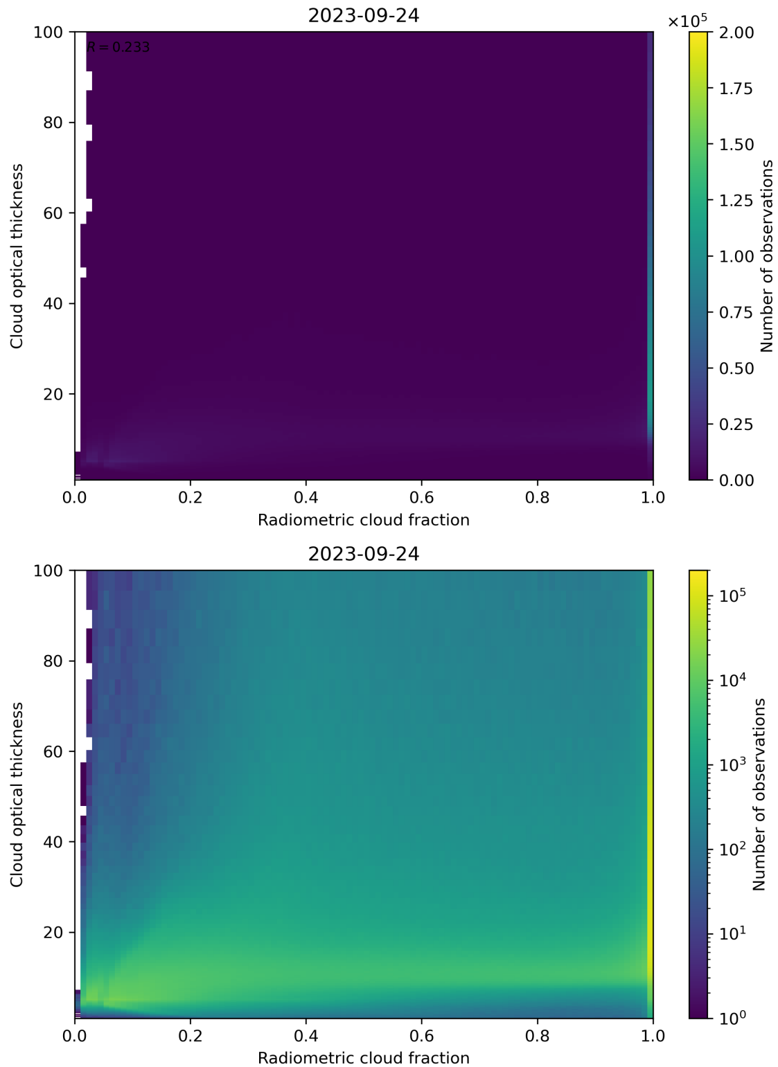
Figure 75: Scatter density plot of “Radiometric cloud fraction” against “Cloud optical thickness” for 2023-09-23 to 2023-09-25.
