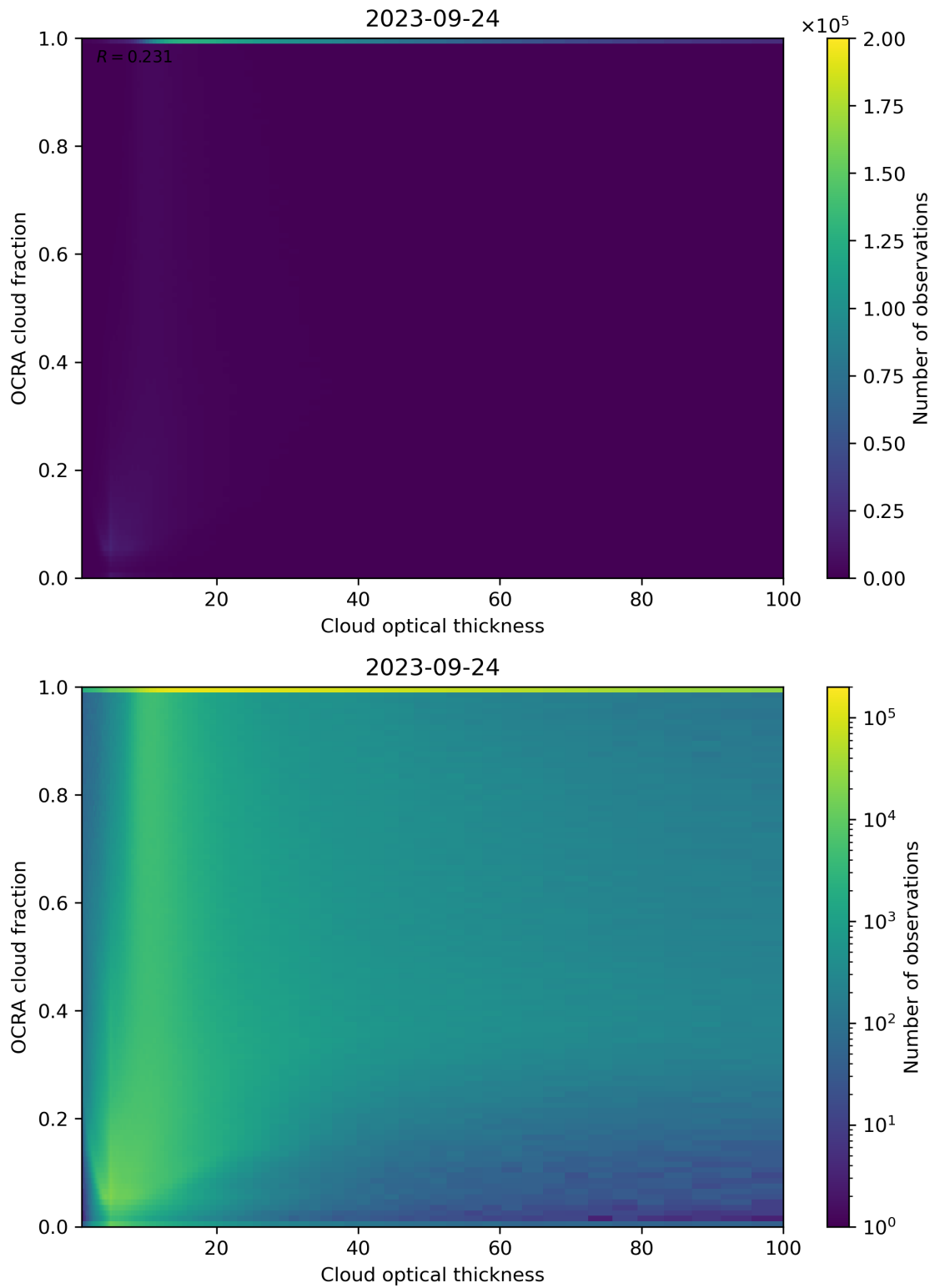
Figure 83: Scatter density plot of “Cloud optical thickness” against “OCRA cloud fraction” for 2023-09-23 to 2023-09-25.
