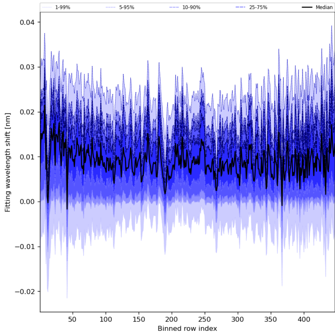
Figure 65: Along track statistics of “Fitting wavelength shift” for 2023-09-23 to 2023-09-25
