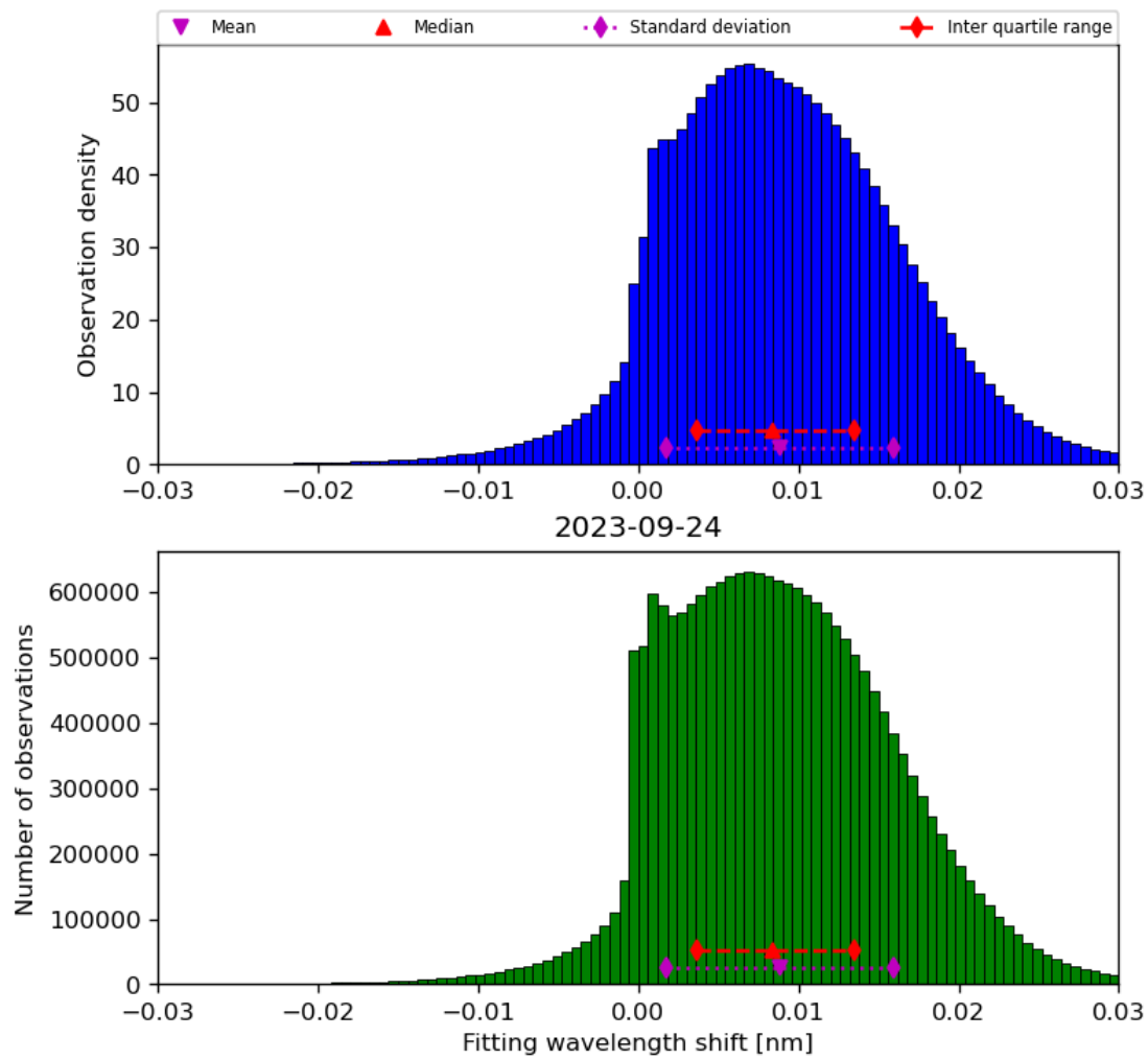
Figure 49: Histogram of “Fitting wavelength shift” for 2023-09-23 to 2023-09-25
