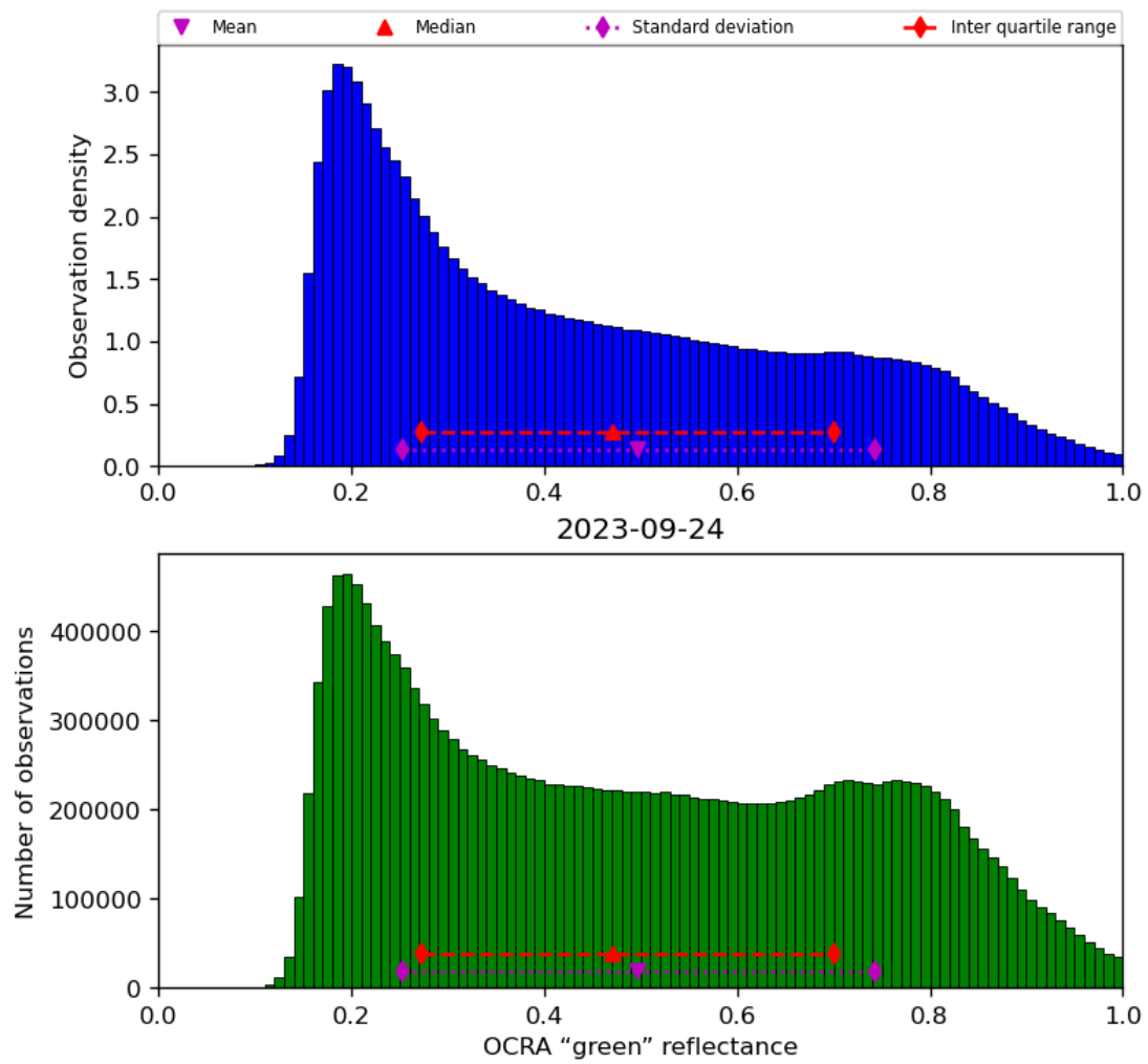
Figure 52: Histogram of “OCRA “green” reflectance” for 2023-09-23 to 2023-09-25
