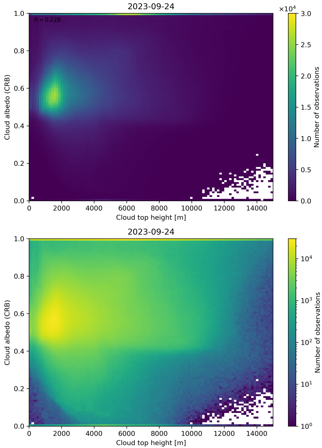
Figure 86: Scatter density plot of “Cloud top height” against “Cloud albedo (CRB)” for 2023-09-23 to 2023-09-25.
