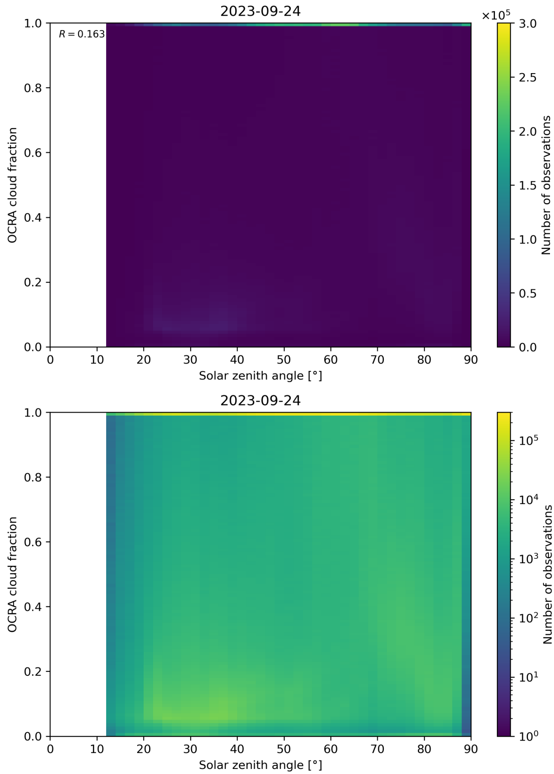
Figure 100: Scatter density plot of “Solar zenith angle” against “OCRA cloud fraction” for 2023-09-23 to 2023-09-25.
