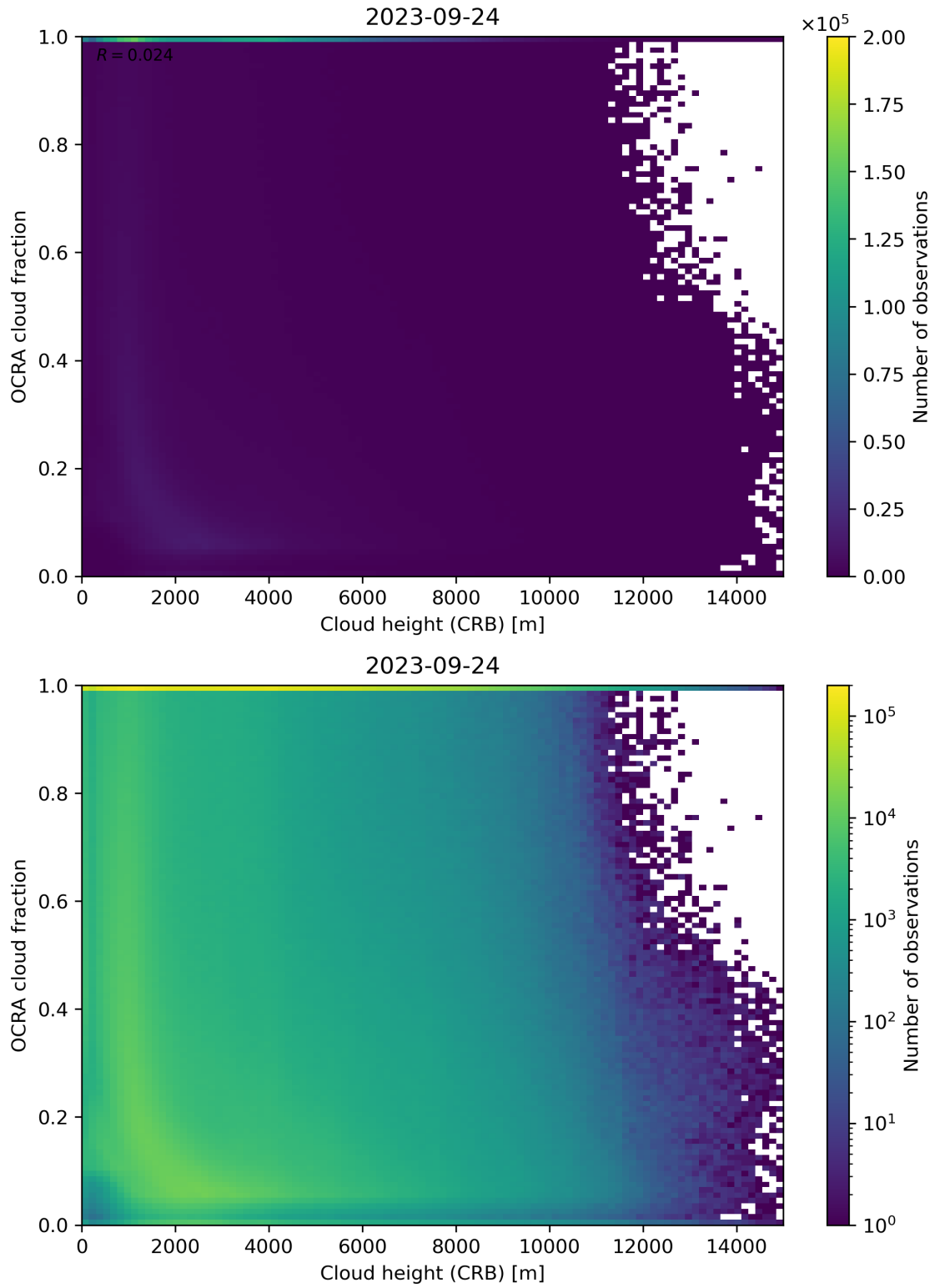
Figure 81: Scatter density plot of “Cloud height (CRB)” against “OCRA cloud fraction” for 2023-09-23 to 2023-09-25.
