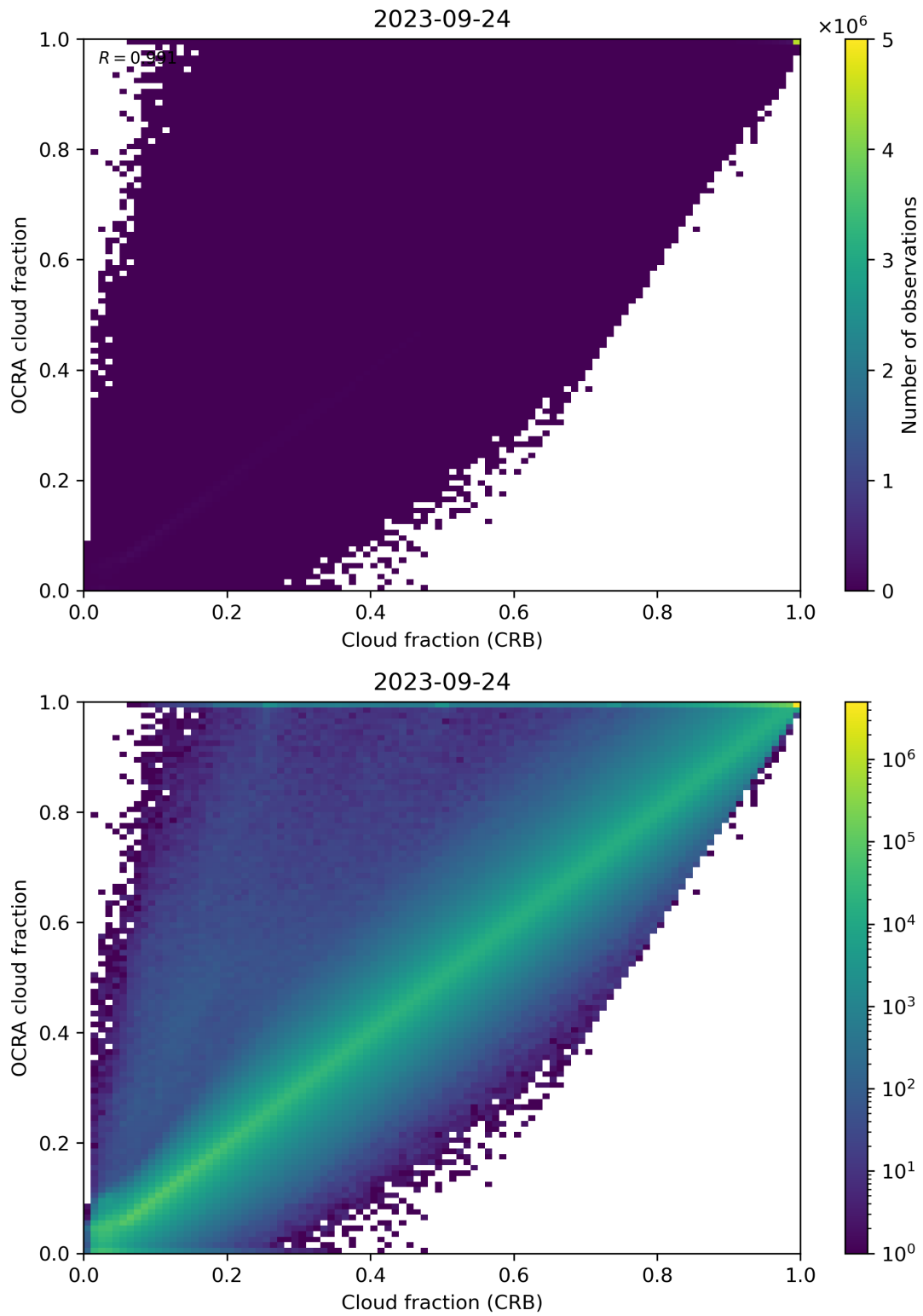
Figure 78: Scatter density plot of “Cloud fraction (CRB)” against “OCRA cloud fraction” for 2023-09-23 to 2023-09-25.
