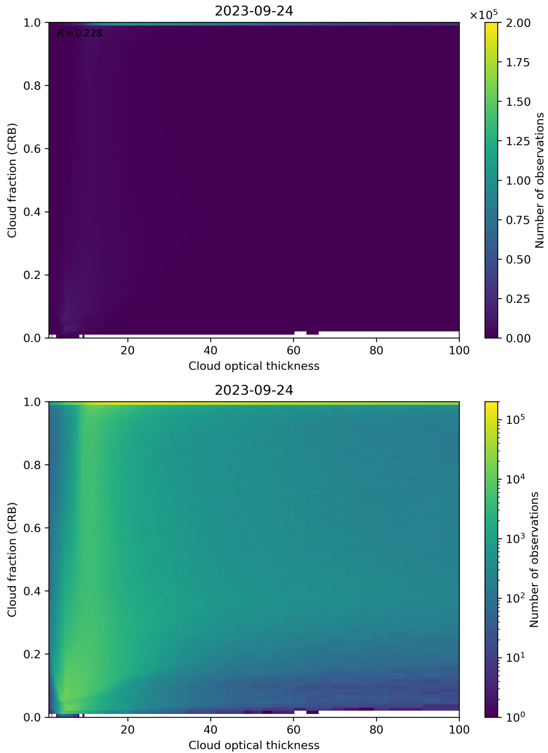
Figure 84: Scatter density plot of “Cloud optical thickness” against “Cloud fraction (CRB)” for 2023-09-23 to 2023-09-25.
