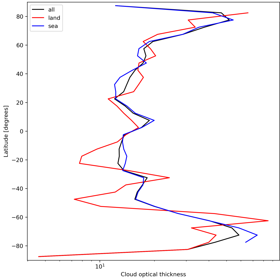
Figure 25: Zonal average of “Cloud optical thickness” for 2023-09-23 to 2023-09-25.
