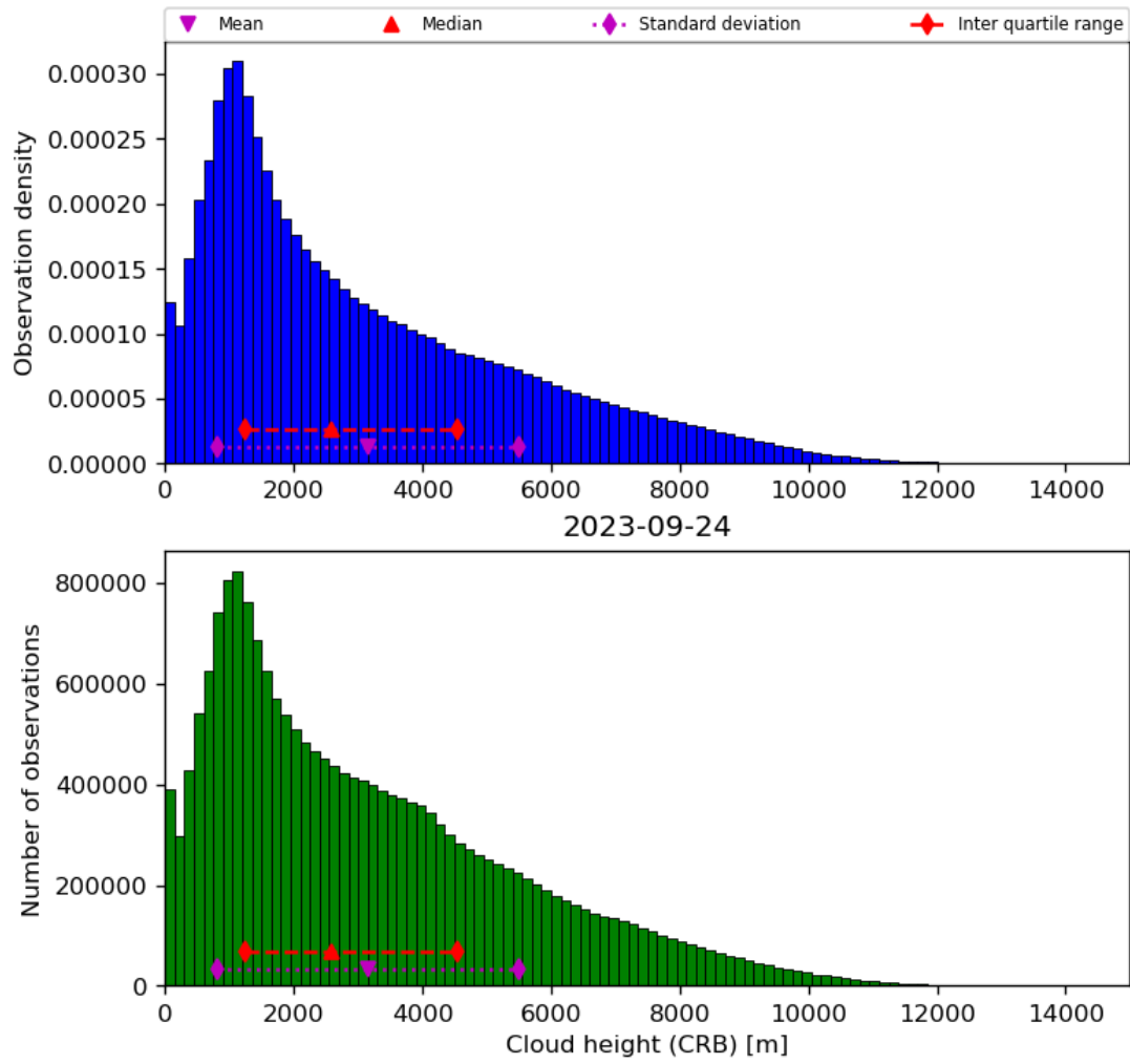
Figure 43: Histogram of “Cloud height (CRB)” for 2023-09-23 to 2023-09-25
