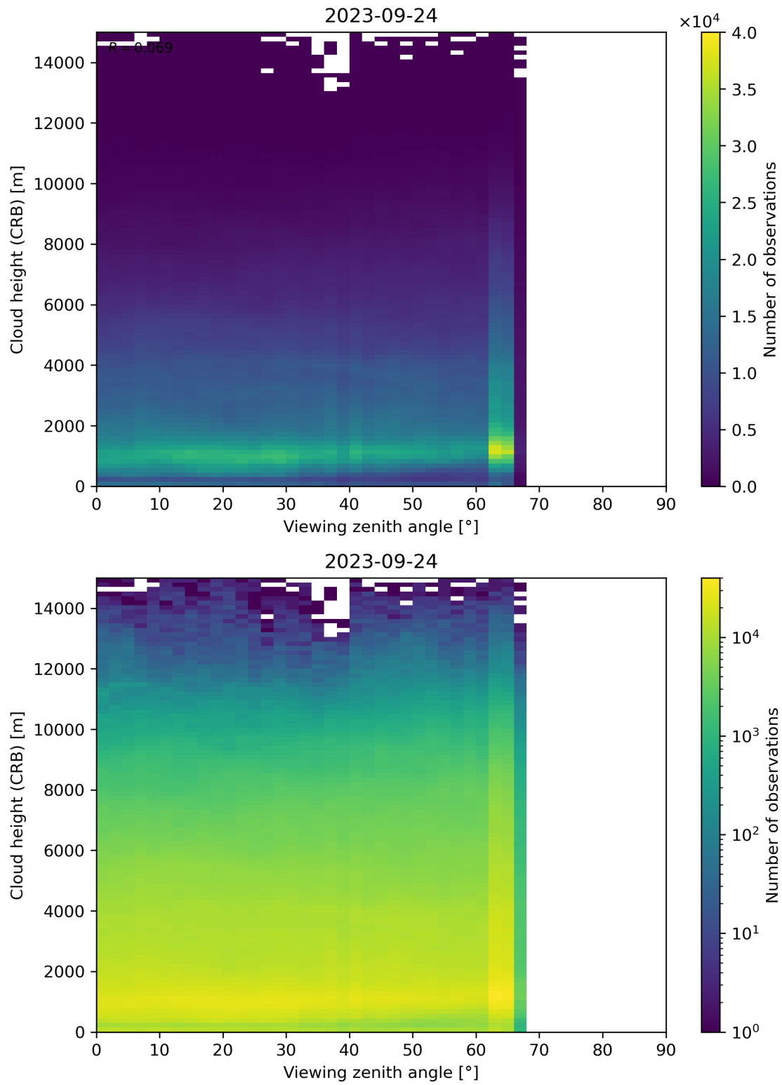
Figure 110: Scatter density plot of “Viewing zenith angle” against “Cloud height (CRB)” for 2023-09-23 to 2023-09-25.
