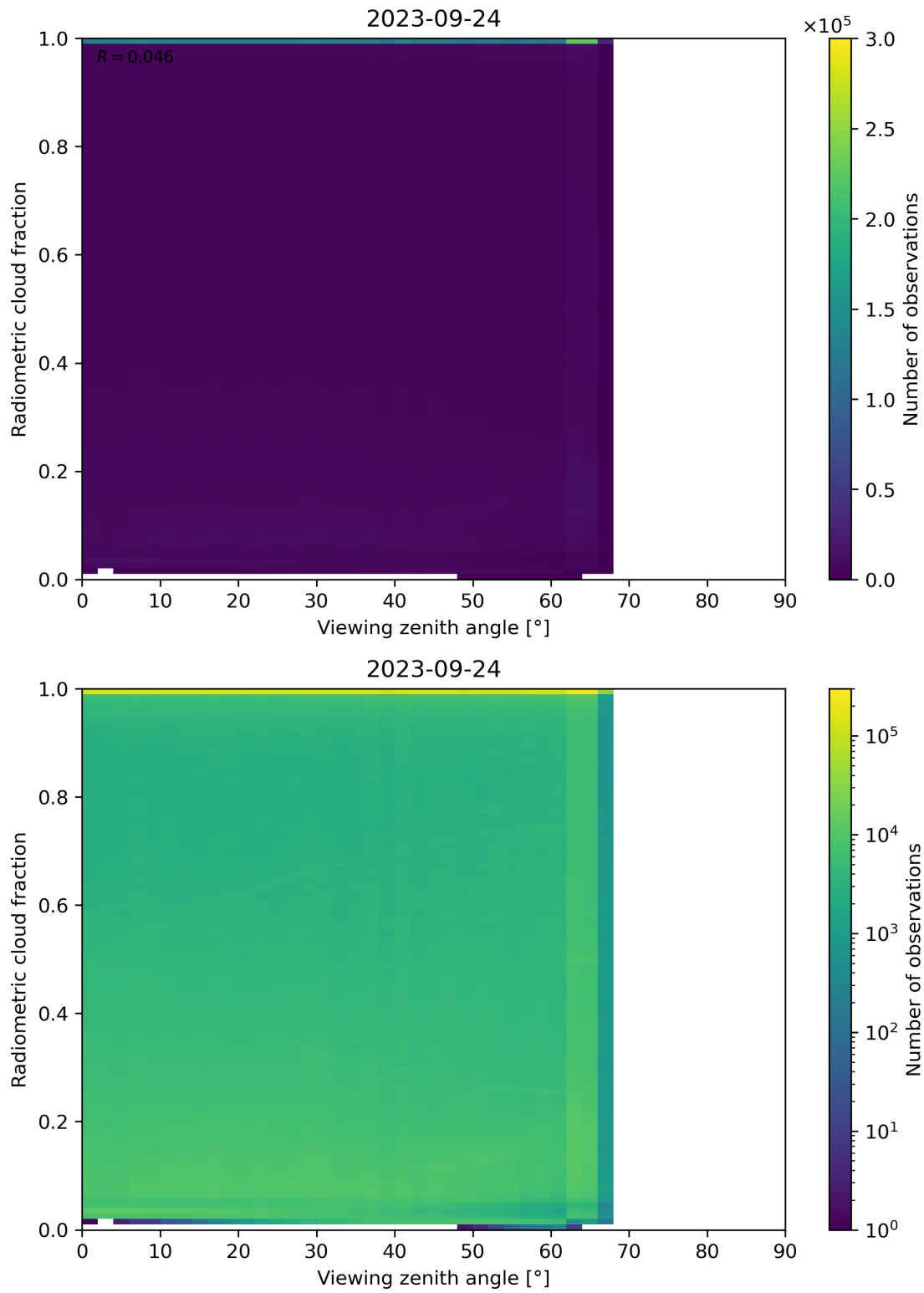
Figure 107: Scatter density plot of “Viewing zenith angle” against “Radiometric cloud fraction” for 2023-09-23 to 2023-09-25.
