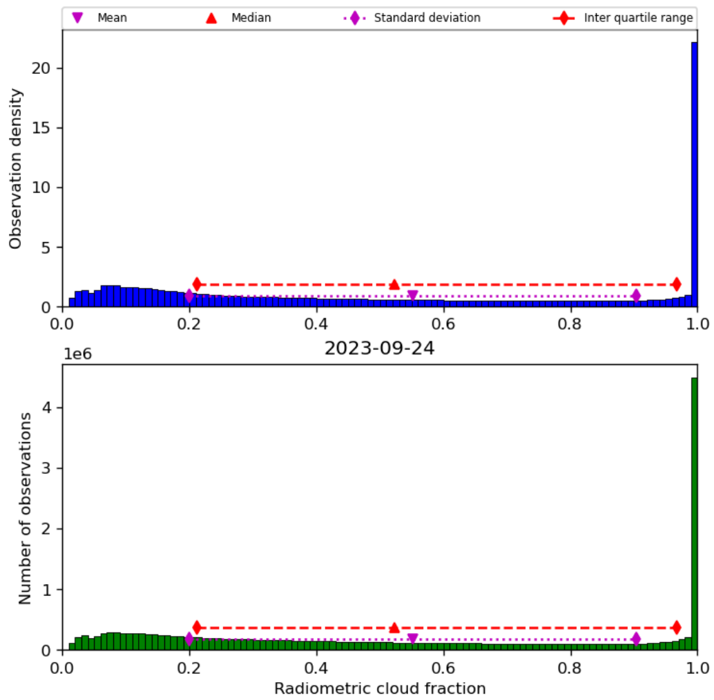
Figure 39: Histogram of “Radiometric cloud fraction” for 2023-09-23 to 2023-09-25
