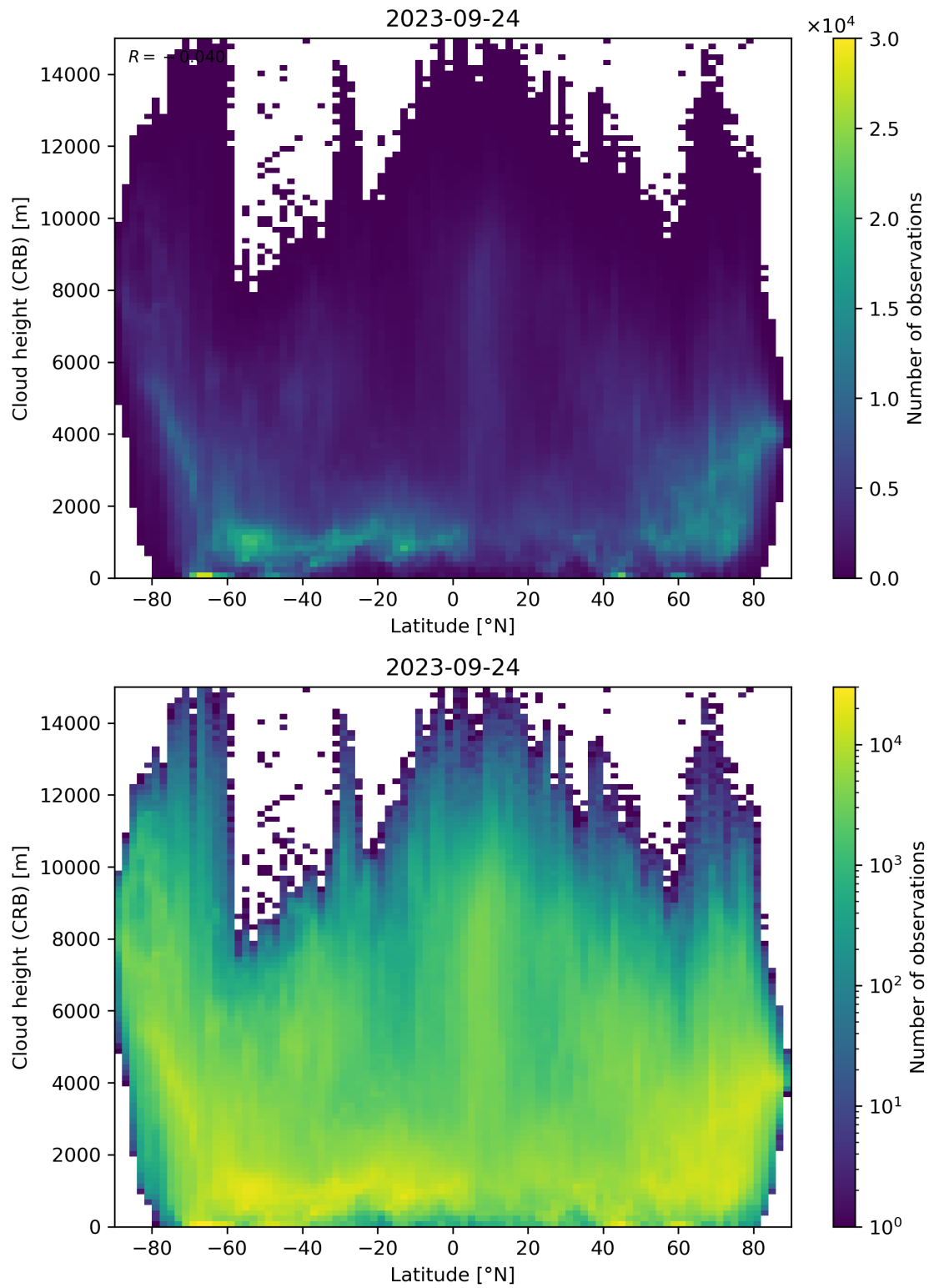
Figure 95: Scatter density plot of “Latitude” against “Cloud height (CRB)” for 2023-09-23 to 2023-09-25.
