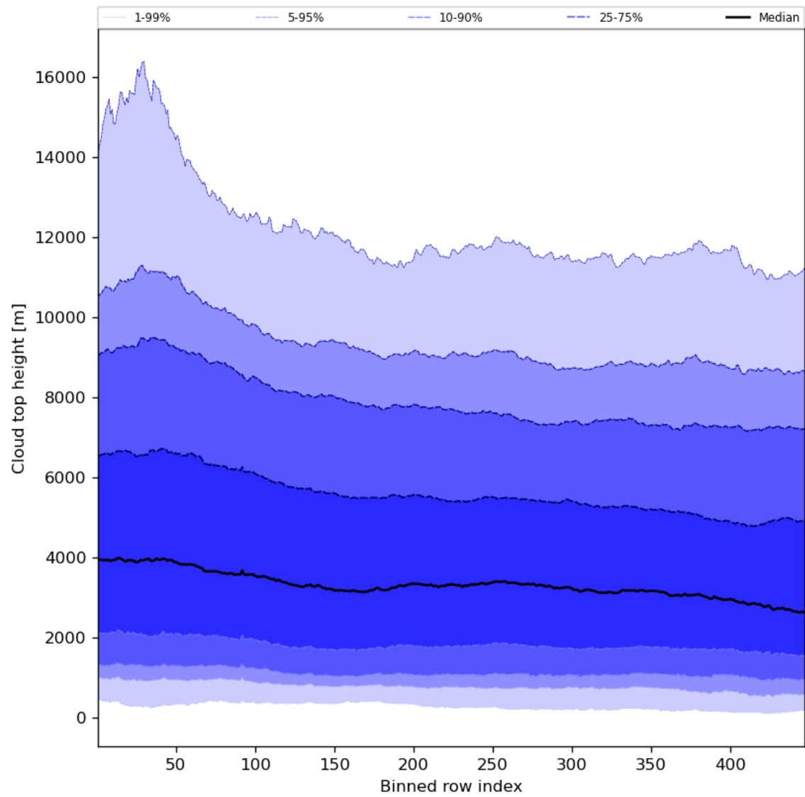
Figure 56: Along track statistics of “Cloud top height” for 2023-09-23 to 2023-09-25
