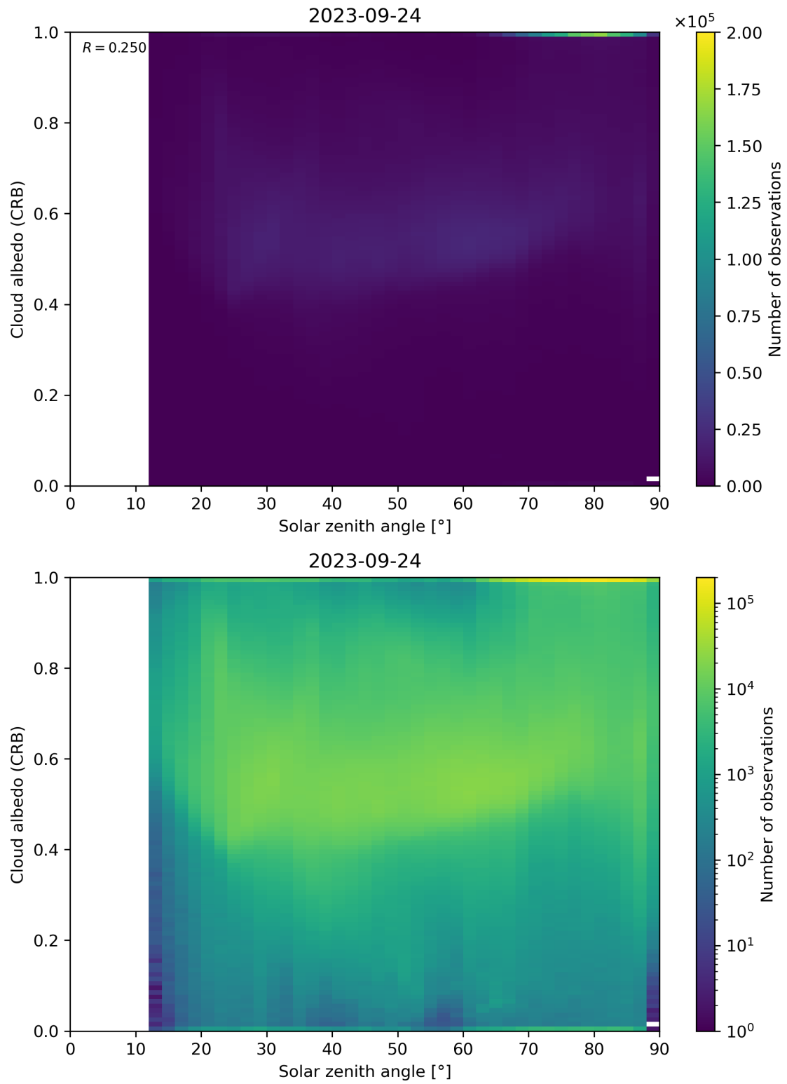
Figure 98: Scatter density plot of “Solar zenith angle” against “Cloud albedo (CRB)” for 2023-09-23 to 2023-09-25.
