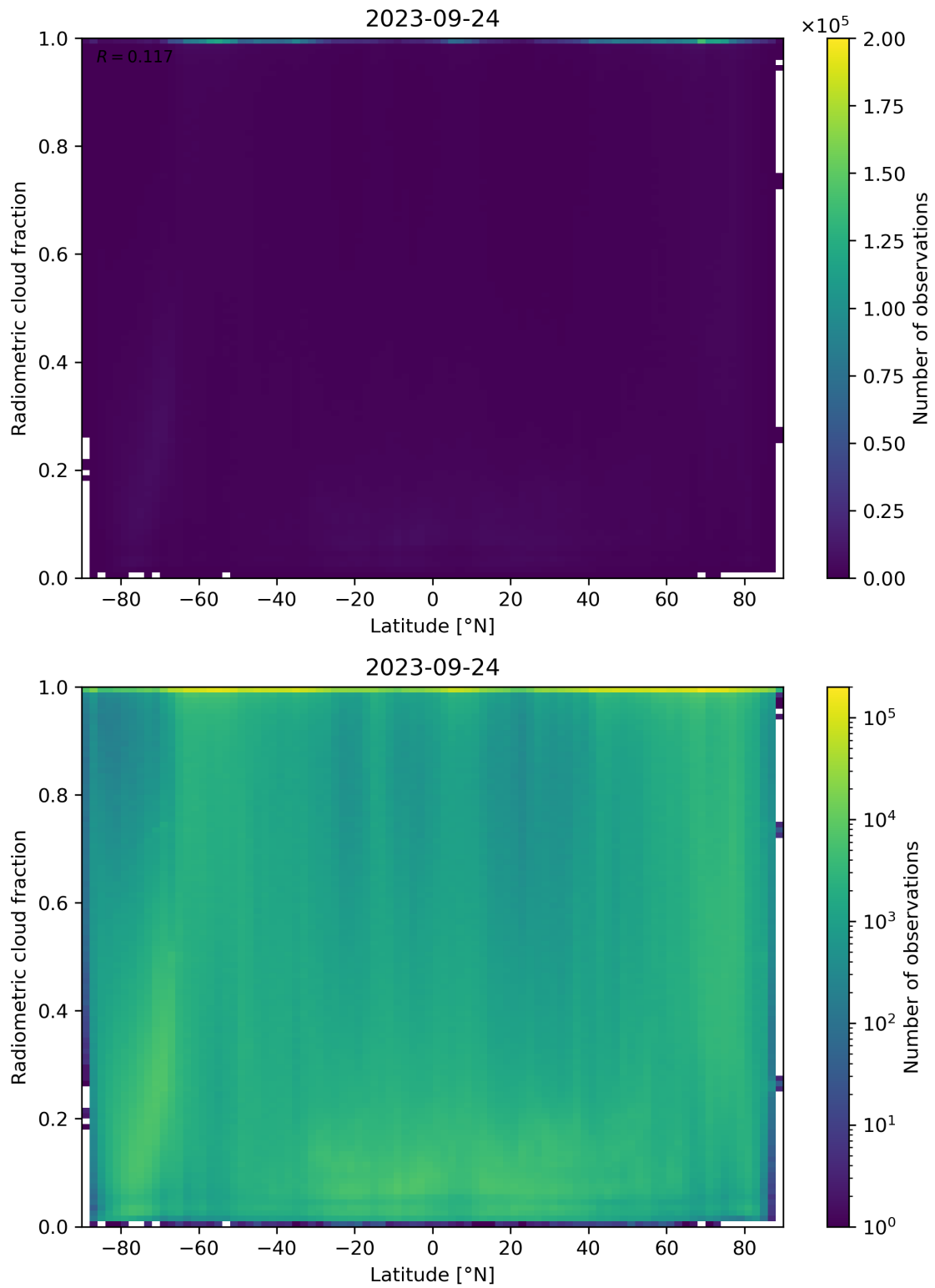
Figure 92: Scatter density plot of “Latitude” against “Radiometric cloud fraction” for 2023-09-23 to 2023-09-25.
