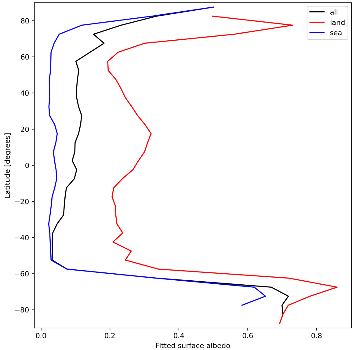
Figure 29: Zonal average of “Fitted surface albedo” for 2023-09-23 to 2023-09-25.
