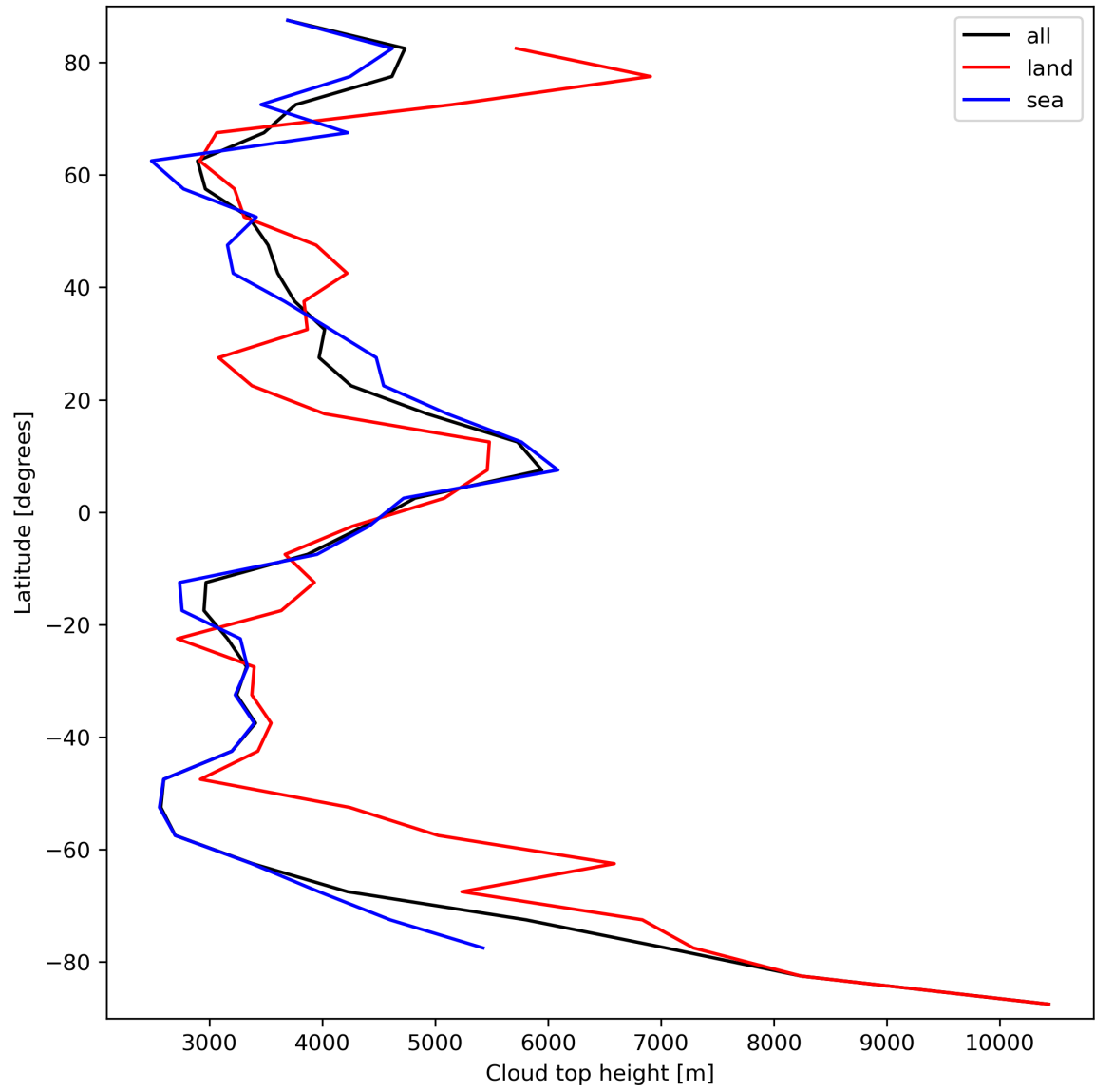
Figure 24: Zonal average of “Cloud top height” for 2023-09-23 to 2023-09-25.
