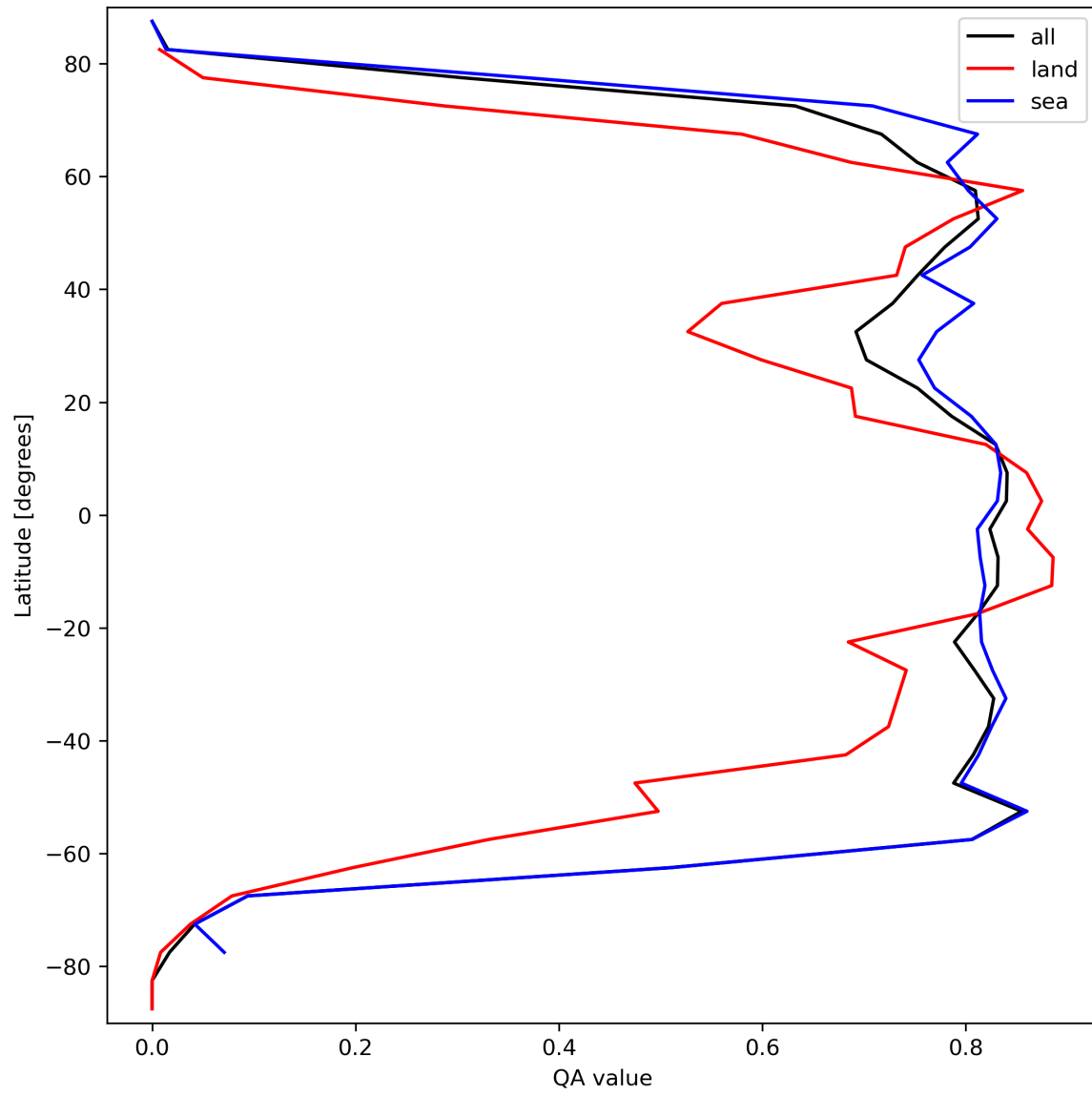
Figure 22: Zonal average of “QA value” for 2023-09-23 to 2023-09-25.
