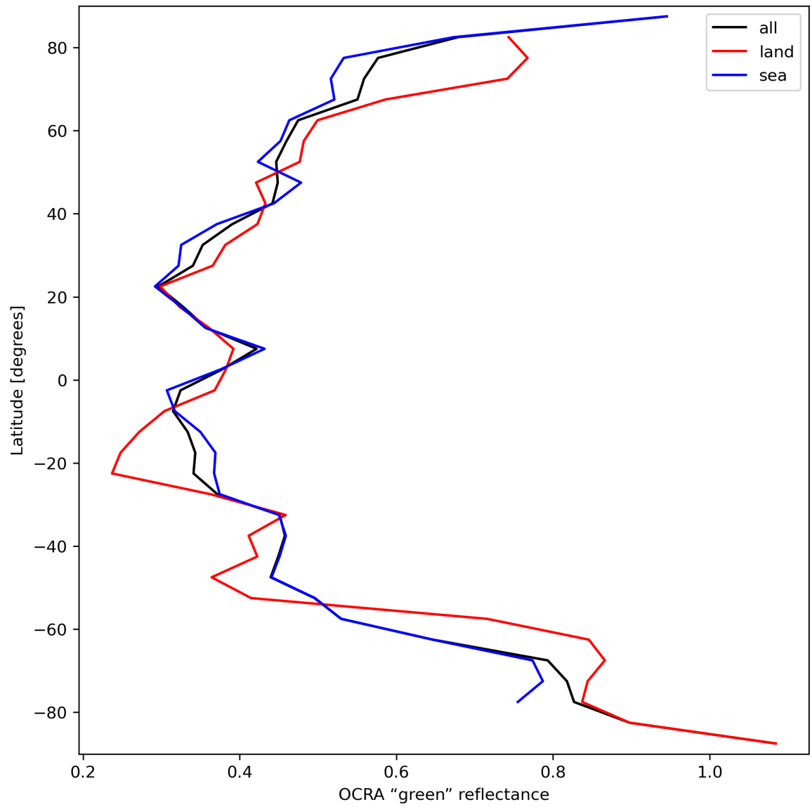
Figure 36: Zonal average of “OCRA “green” reflectance” for 2023-09-23 to 2023-09-25.
