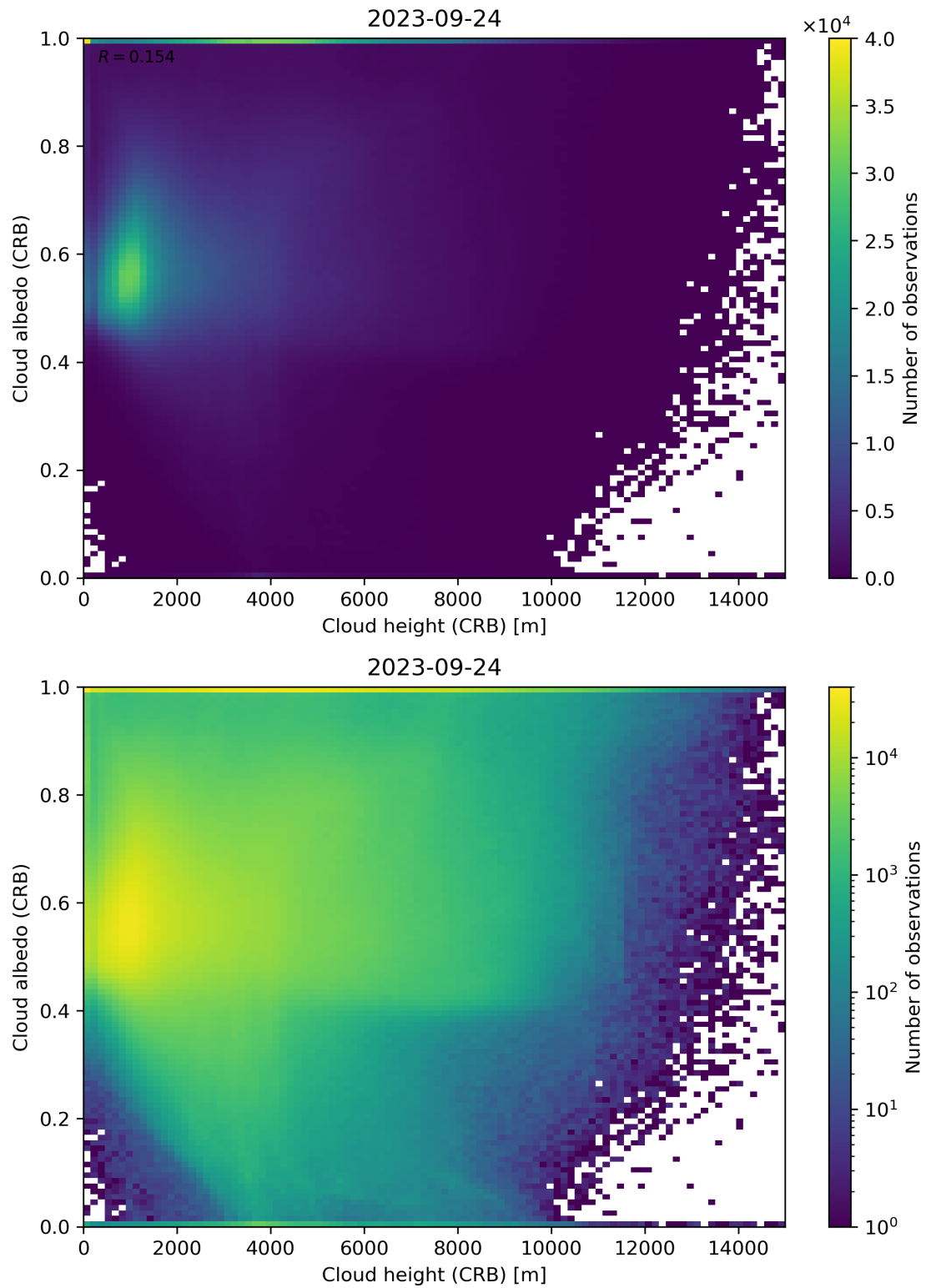
Figure 80: Scatter density plot of “Cloud height (CRB)” against “Cloud albedo (CRB)” for 2023-09-23 to 2023-09-25.
