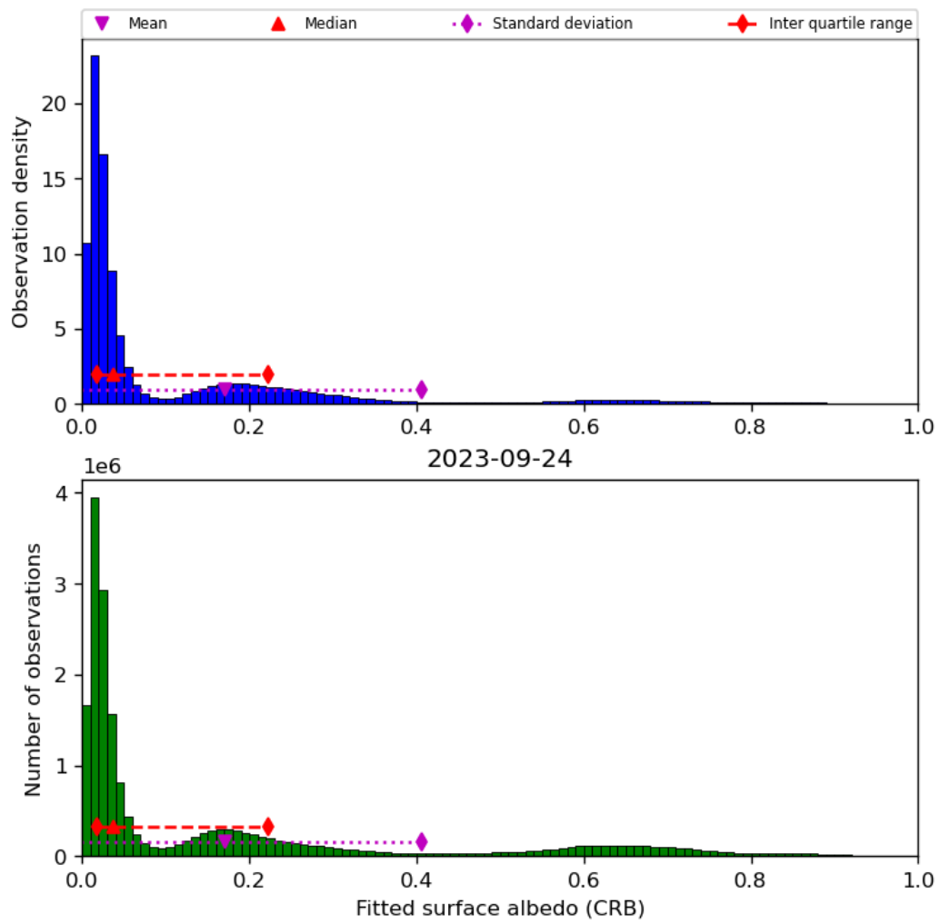
Figure 46: Histogram of “Fitted surface albedo (CRB)” for 2023-09-23 to 2023-09-25
