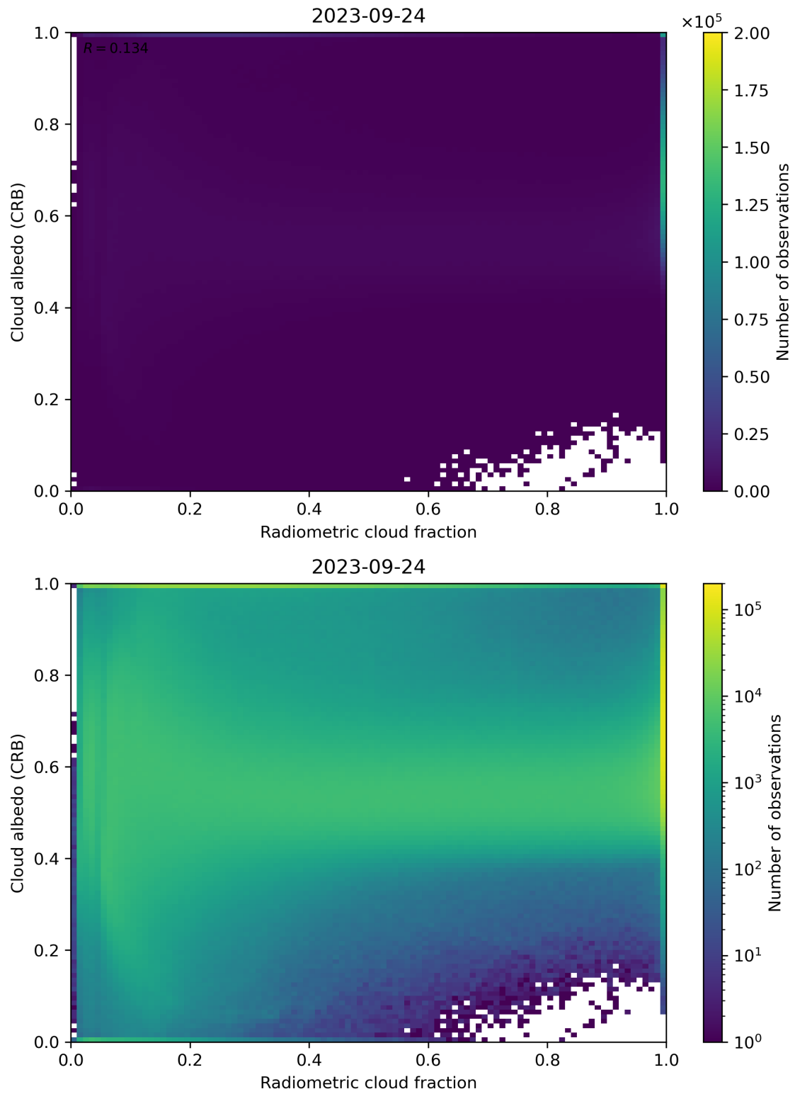
Figure 71: Scatter density plot of “Radiometric cloud fraction” against “Cloud albedo (CRB)” for 2023-09-23 to 2023-09-25.
