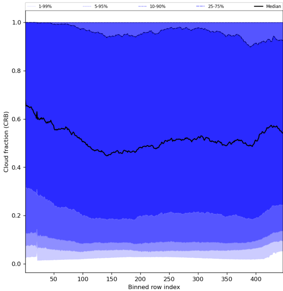
Figure 58: Along track statistics of “Cloud fraction (CRB)” for 2023-09-23 to 2023-09-25
