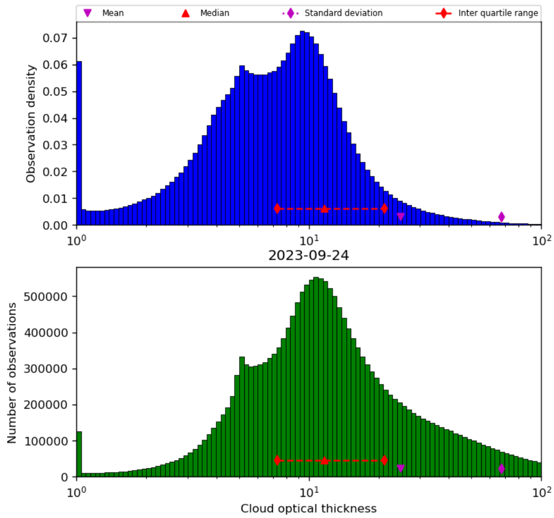
Figure 41: Histogram of “Cloud optical thickness” for 2023-09-23 to 2023-09-25
