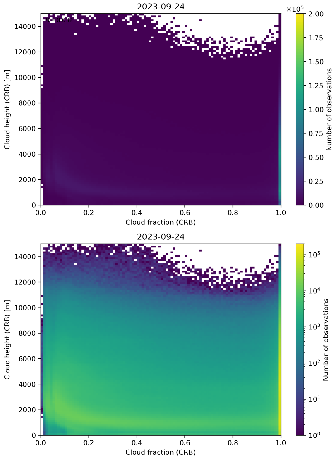
Figure 79: Scatter density plot of “Cloud fraction (CRB)” against “Cloud height (CRB)” for 2023-09-23 to 2023-09-25.
