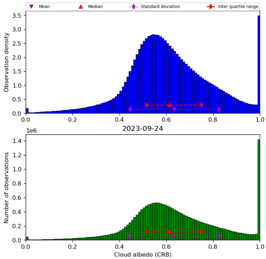
Figure 44: Histogram of “Cloud albedo (CRB)” for 2023-09-23 to 2023-09-25
