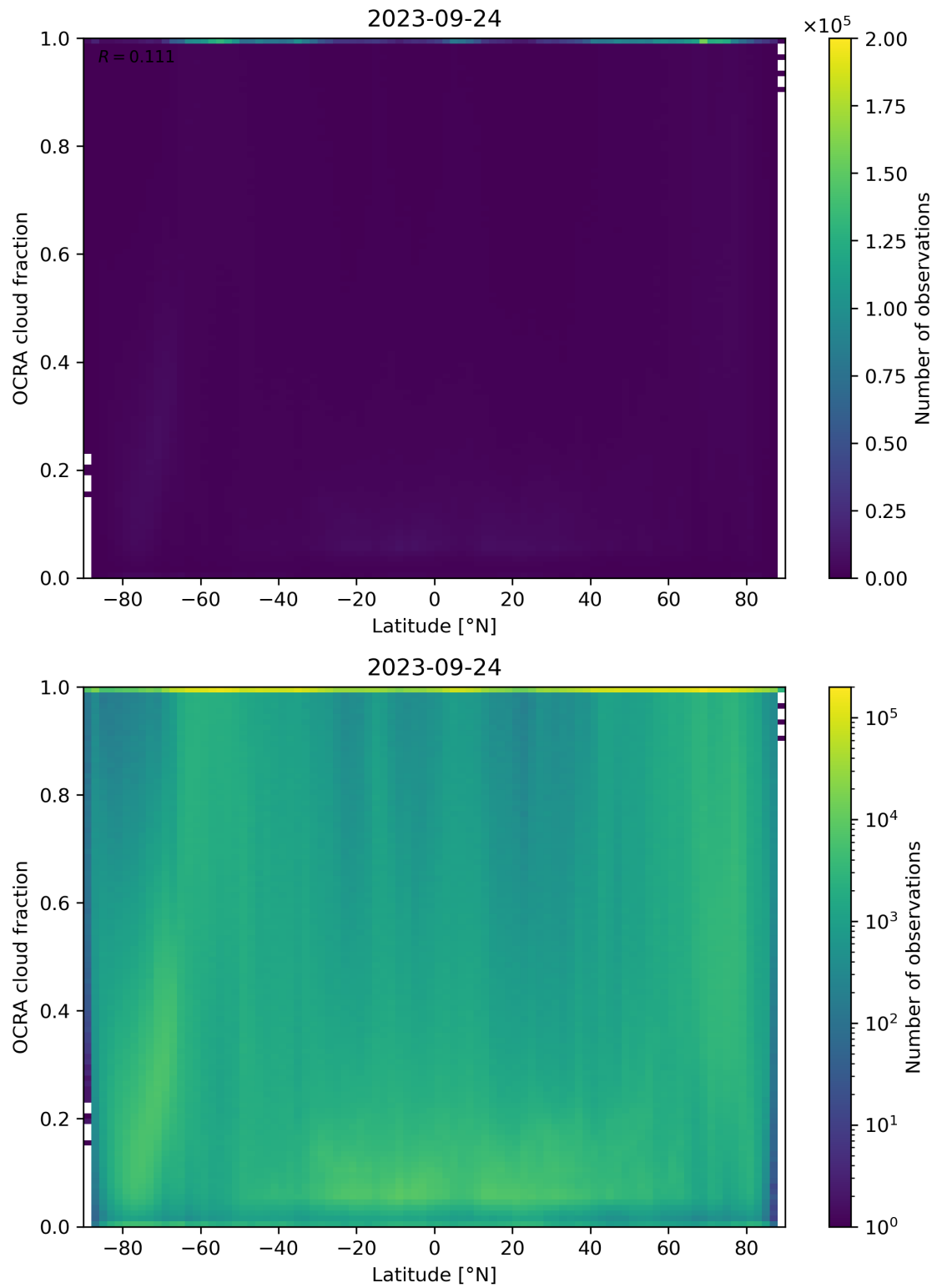
Figure 93: Scatter density plot of “Latitude” against “OCRA cloud fraction” for 2023-09-23 to 2023-09-25.
