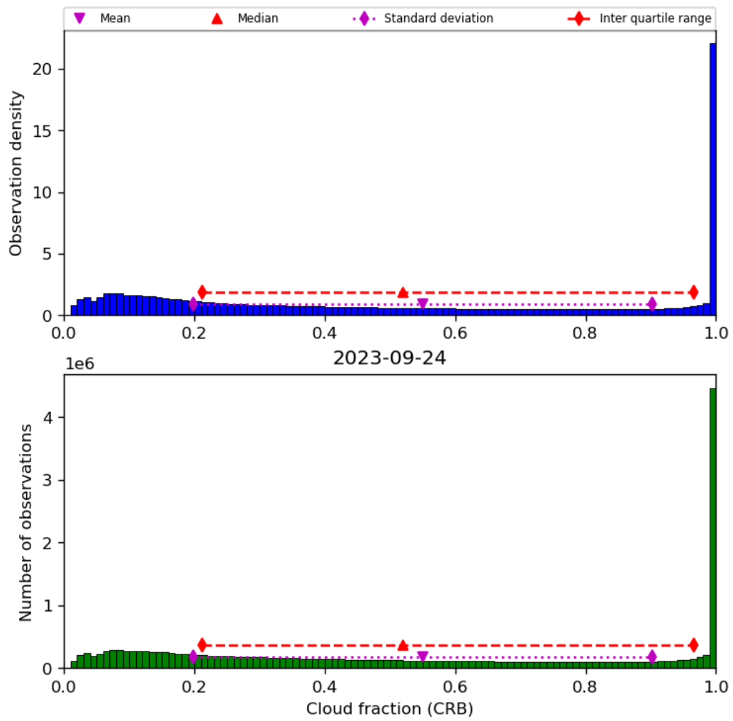
Figure 42: Histogram of “Cloud fraction (CRB)” for 2023-09-23 to 2023-09-25
