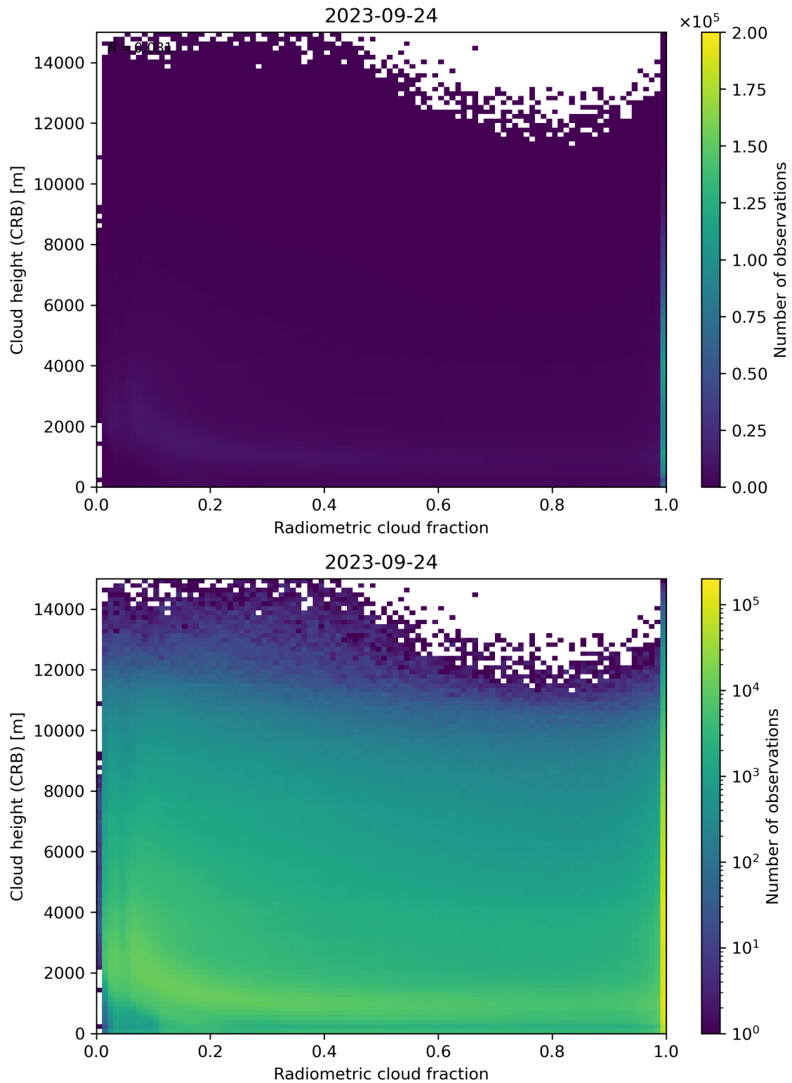
Figure 74: Scatter density plot of “Radiometric cloud fraction” against “Cloud height (CRB)” for 2023-09-23 to 2023-09-25.
