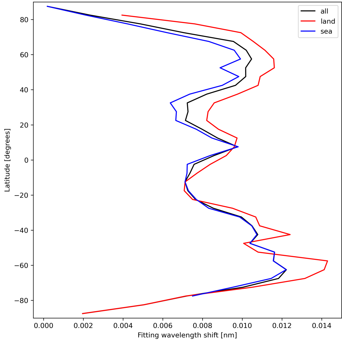
Figure 33: Zonal average of “Fitting wavelength shift” for 2023-09-23 to 2023-09-25.
