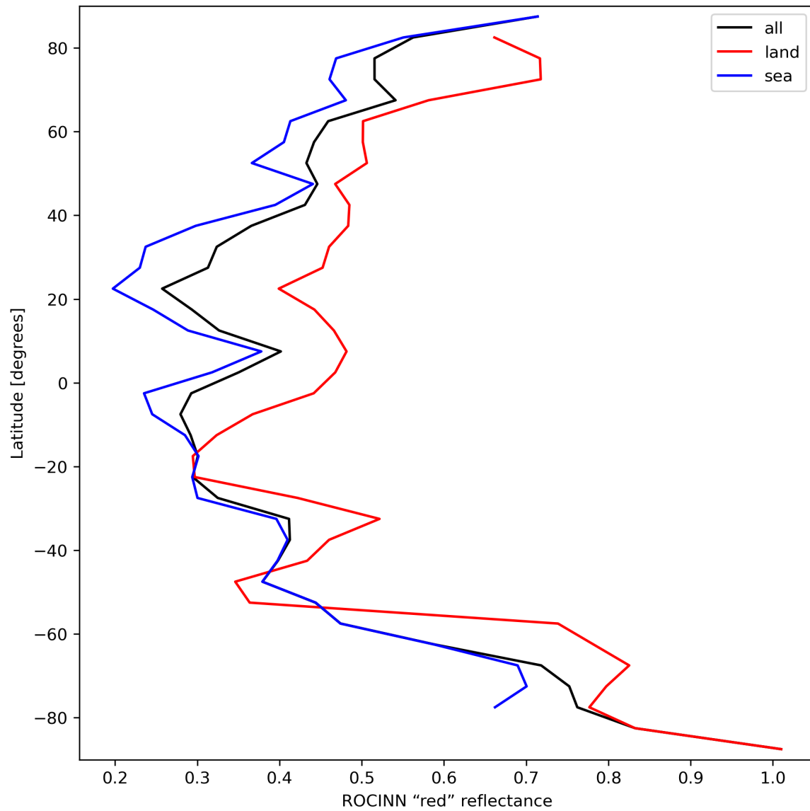
Figure 37: Zonal average of "ROCINN "red" reflectance" for 2023-09-23 to 2023-09-25.
