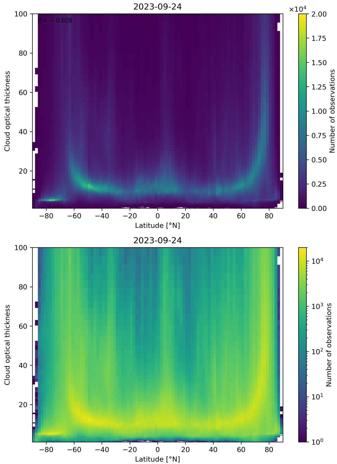
Figure 96: Scatter density plot of “Latitude” against “Cloud optical thickness” for 2023-09-23 to 2023-09-25.
