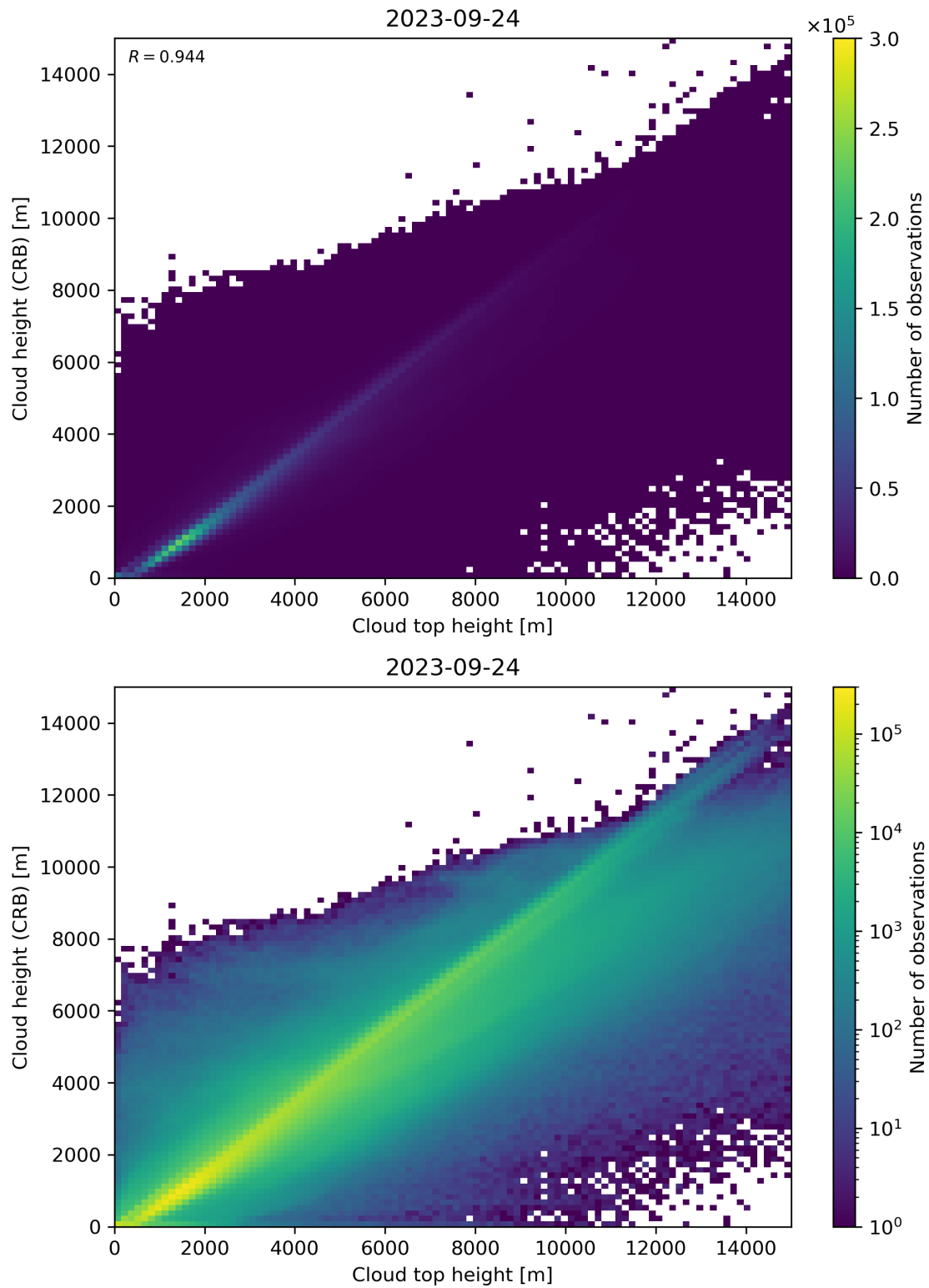
Figure 89: Scatter density plot of “Cloud top height” against “Cloud height (CRB)” for 2023-09-23 to 2023-09-25.
