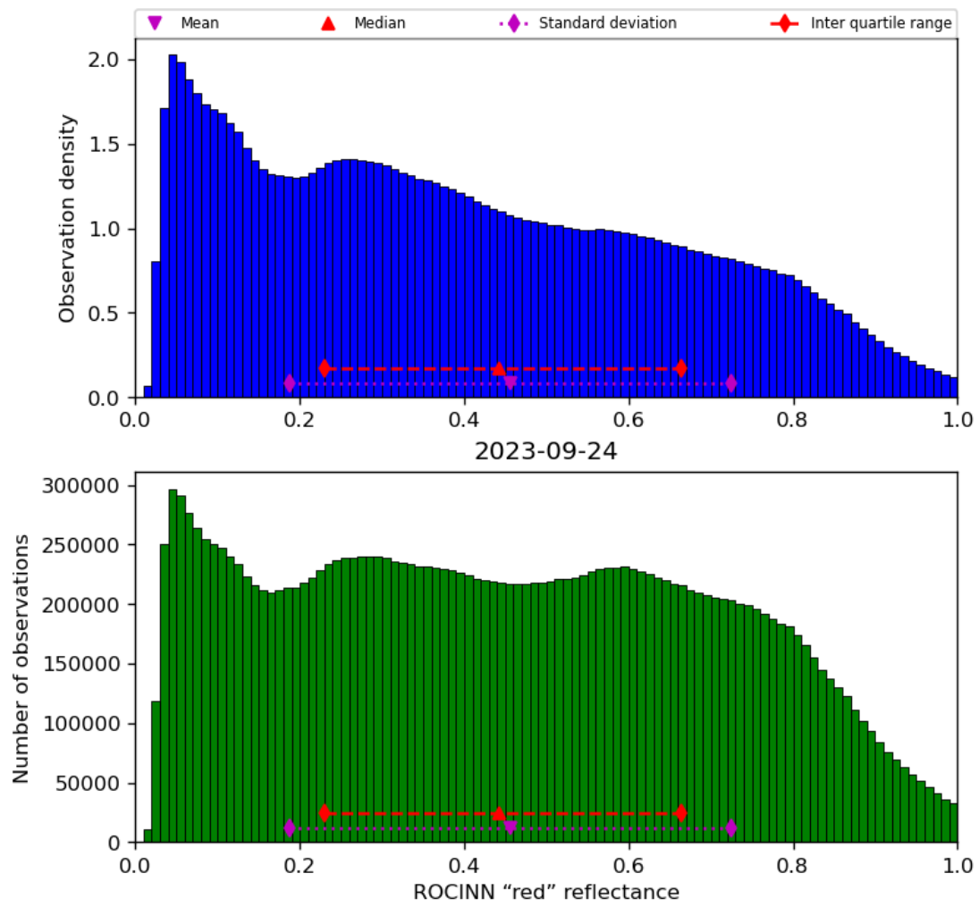
Figure 53: Histogram of “ROCINN “red” reflectance” for 2023-09-23 to 2023-09-25
