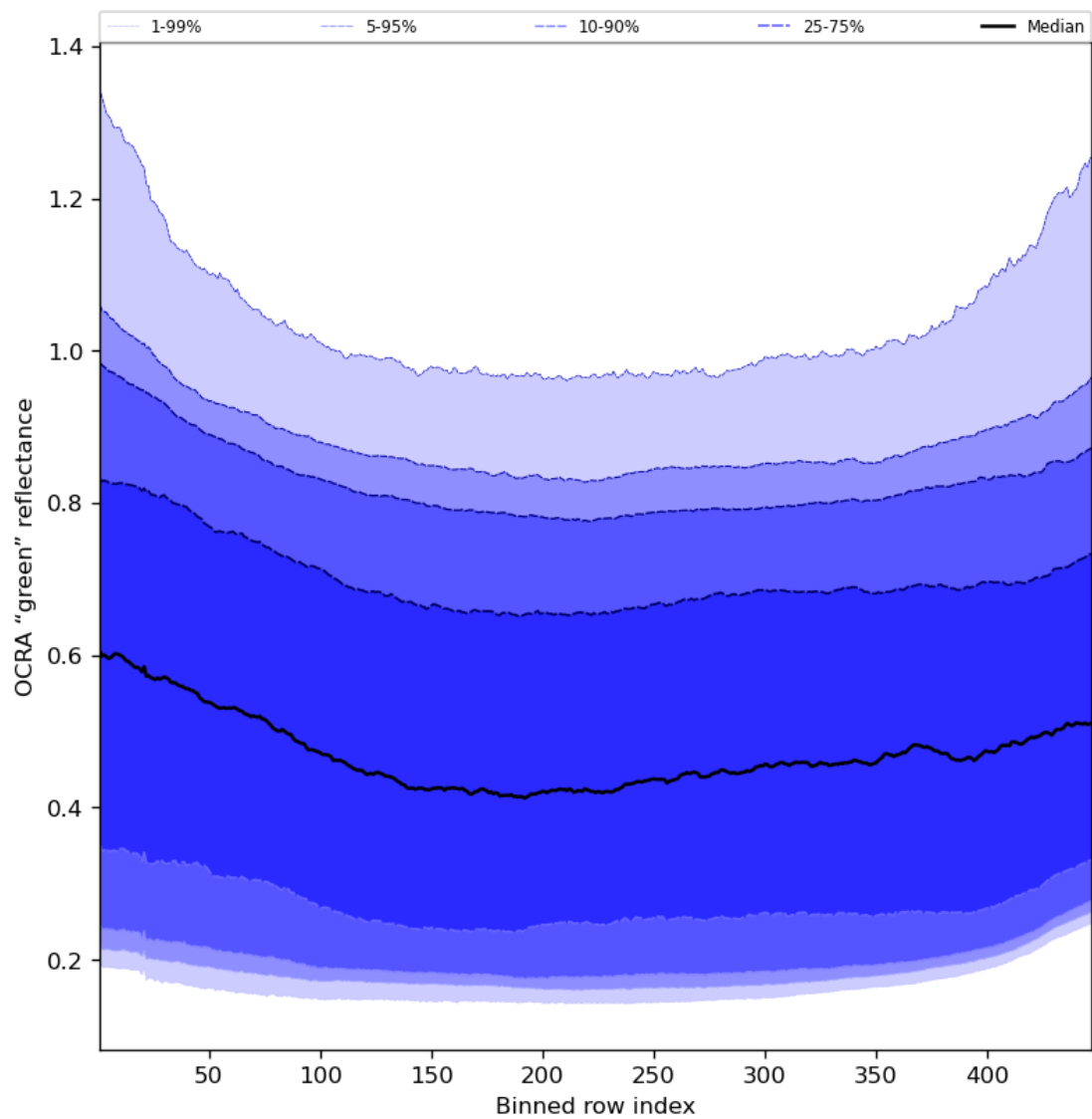
Figure 68: Along track statistics of “OCRA “green” reflectance” for 2023-09-23 to 2023-09-25
