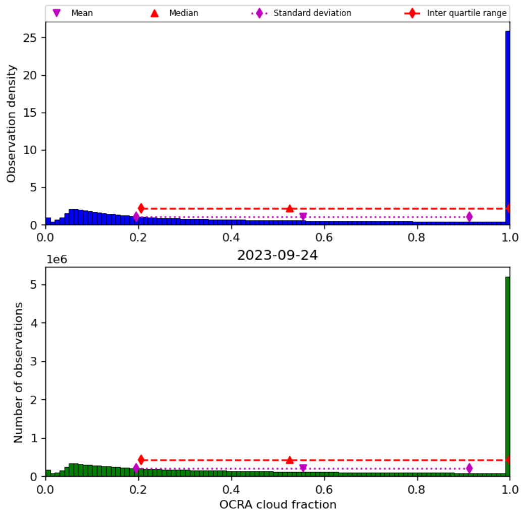
Figure 50: Histogram of “OCRA cloud fraction” for 2023-09-23 to 2023-09-25
