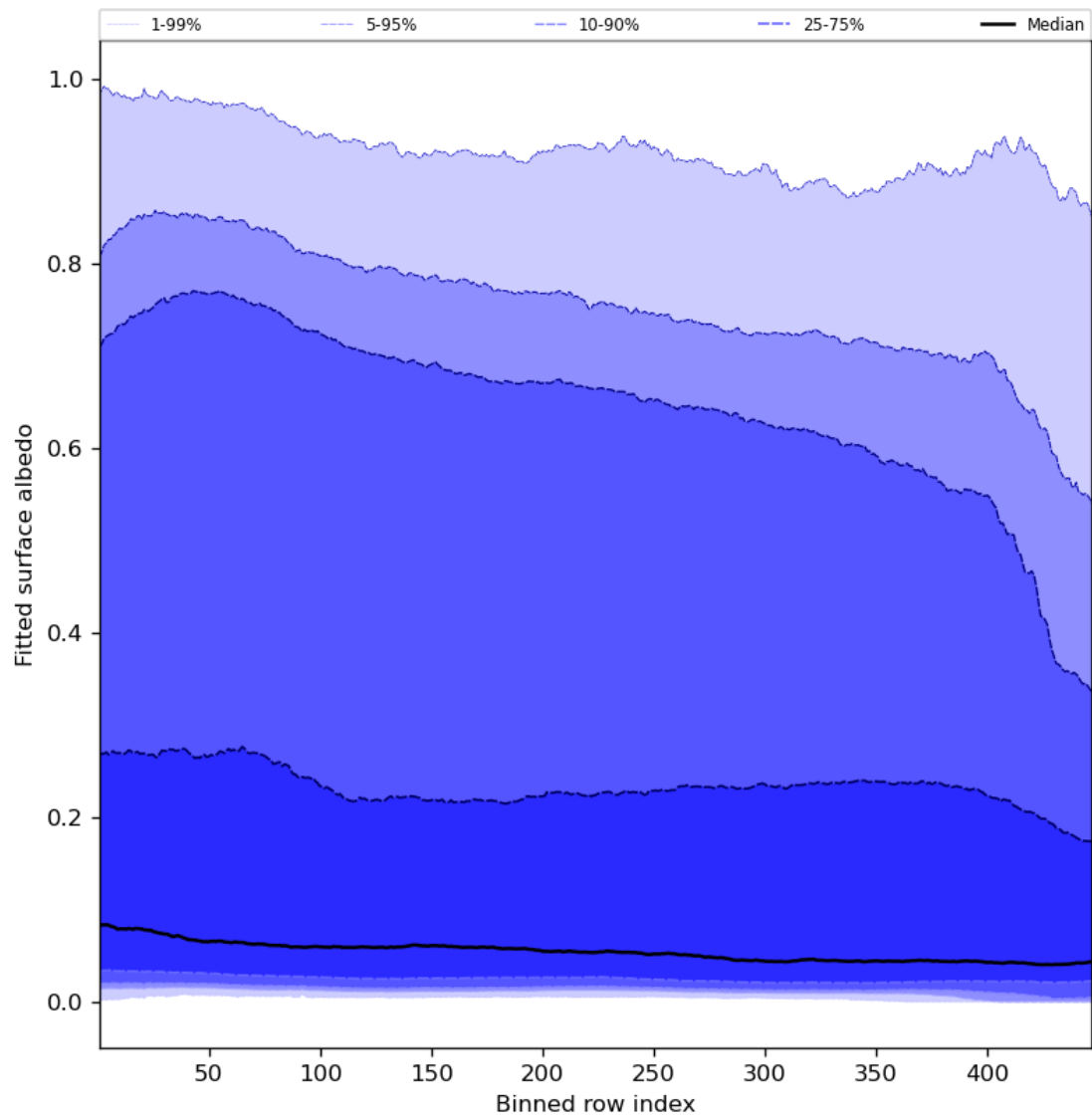
Figure 61: Along track statistics of “Fitted surface albedo” for 2023-09-23 to 2023-09-25
