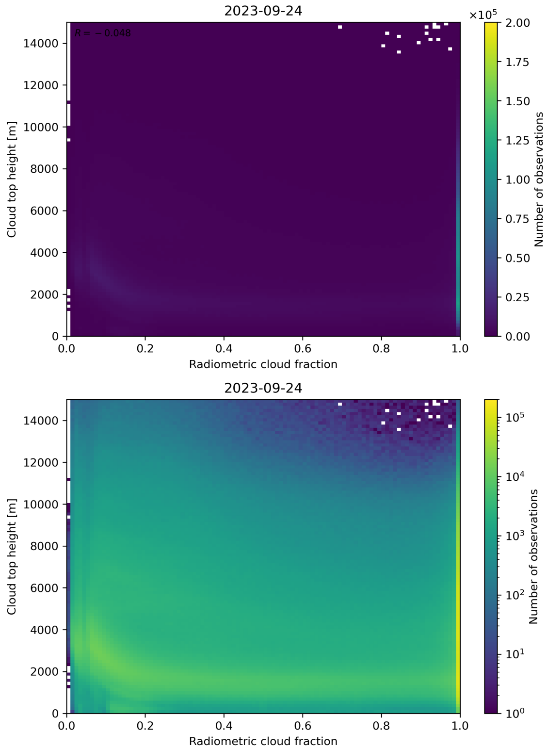
Figure 76: Scatter density plot of “Radiometric cloud fraction” against “Cloud top height” for 2023-09-23 to 2023-09-25.
