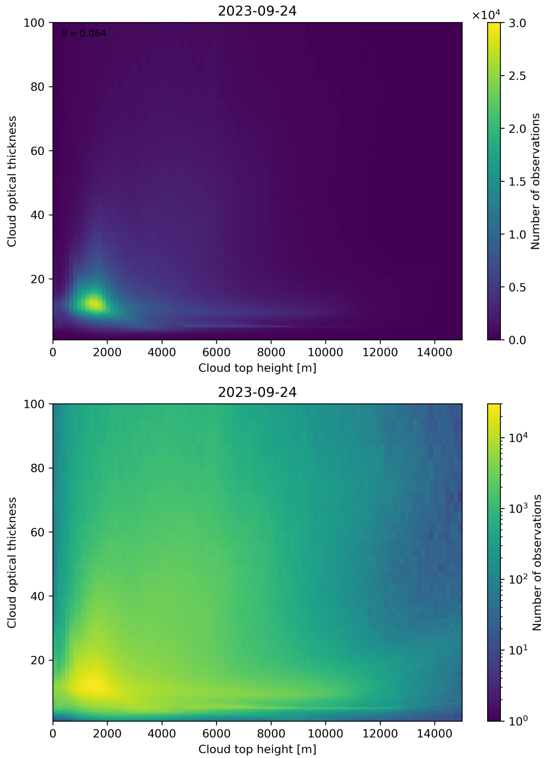
Figure 90: Scatter density plot of “Cloud top height” against “Cloud optical thickness” for 2023-09-23 to 2023-09-25.
