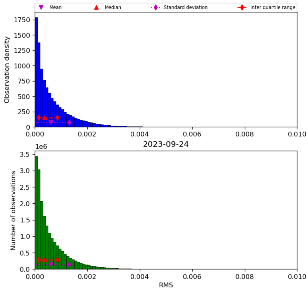
Figure 47: Histogram of “RMS” for 2023-09-23 to 2023-09-25
