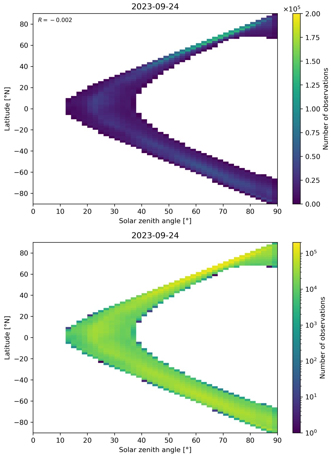
Figure 105: Scatter density plot of “Solar zenith angle” against “Latitude” for 2023-09-23 to 2023-09-25.
