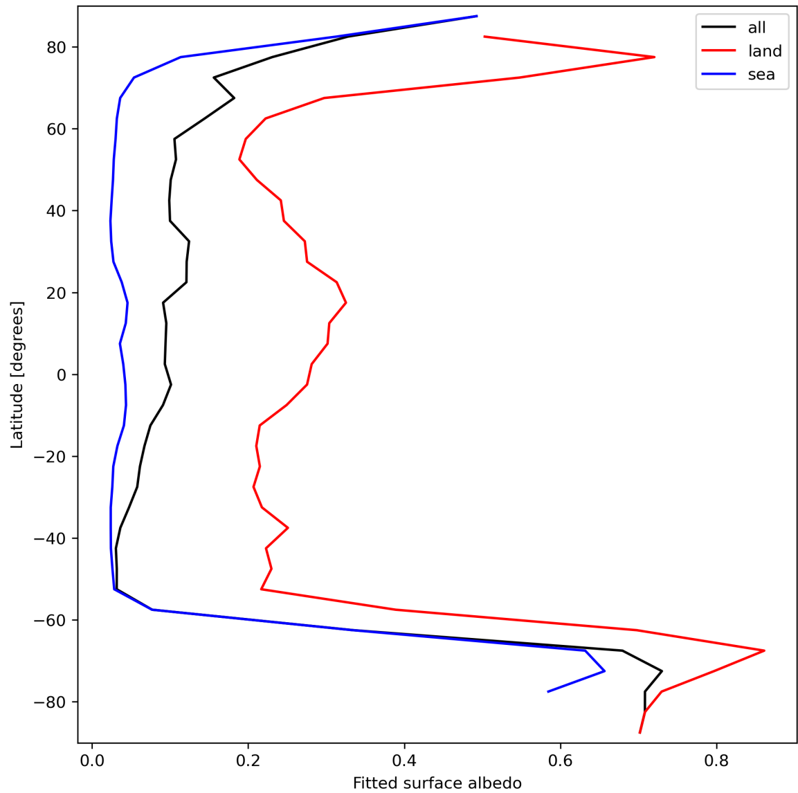
Figure 29: Zonal average of “Fitted surface albedo” for 2023-09-26 to 2023-09-27.
