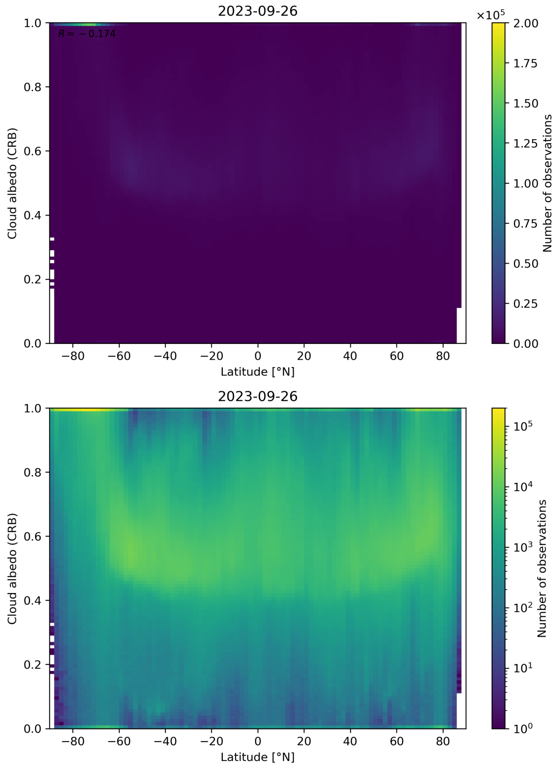
Figure 91: Scatter density plot of “Latitude” against “Cloud albedo (CRB)” for 2023-09-26 to 2023-09-27.
