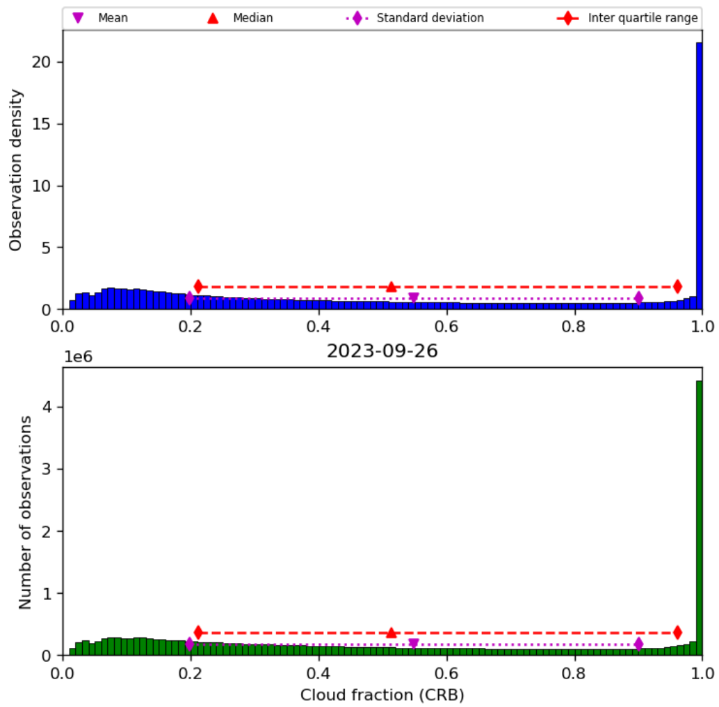
Figure 42: Histogram of “Cloud fraction (CRB)” for 2023-09-26 to 2023-09-27
