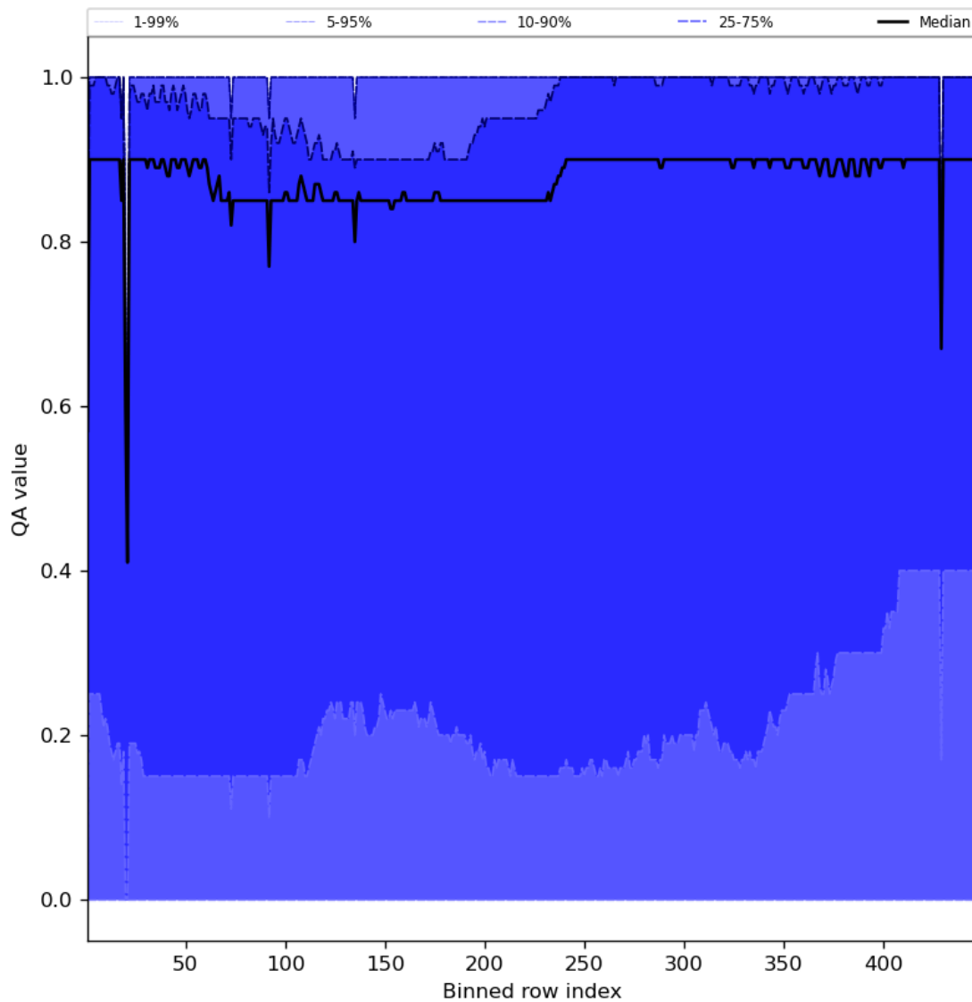
Figure 54: Along track statistics of “QA value” for 2023-09-26 to 2023-09-27
