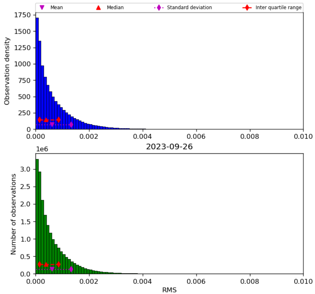
Figure 47: Histogram of “RMS” for 2023-09-26 to 2023-09-27
