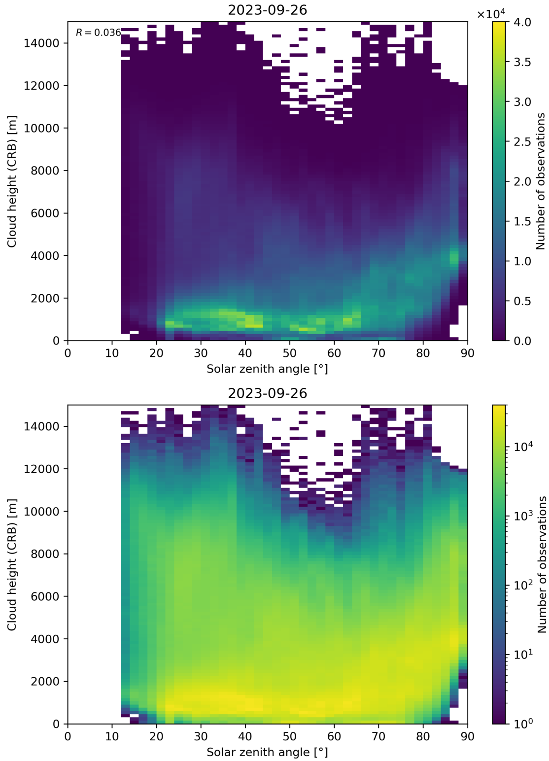
Figure 102: Scatter density plot of “Solar zenith angle” against “Cloud height (CRB)” for 2023-09-26 to 2023-09-27.
