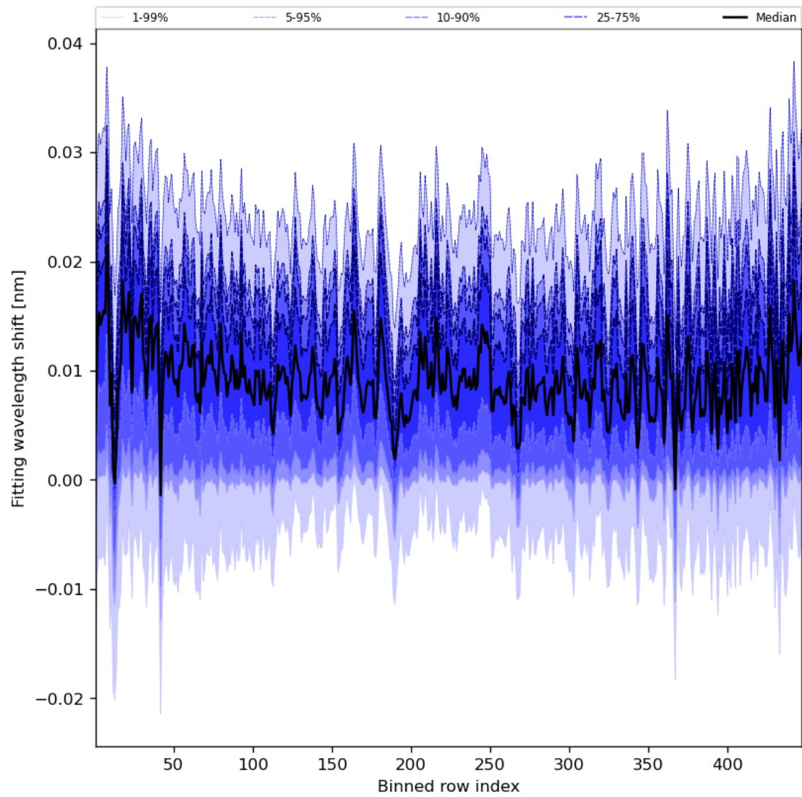
Figure 65: Along track statistics of “Fitting wavelength shift” for 2023-09-26 to 2023-09-27
