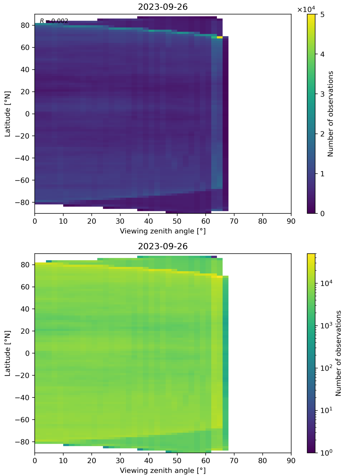
Figure 113: Scatter density plot of “Viewing zenith angle” against “Latitude” for 2023-09-26 to 2023-09-27.
