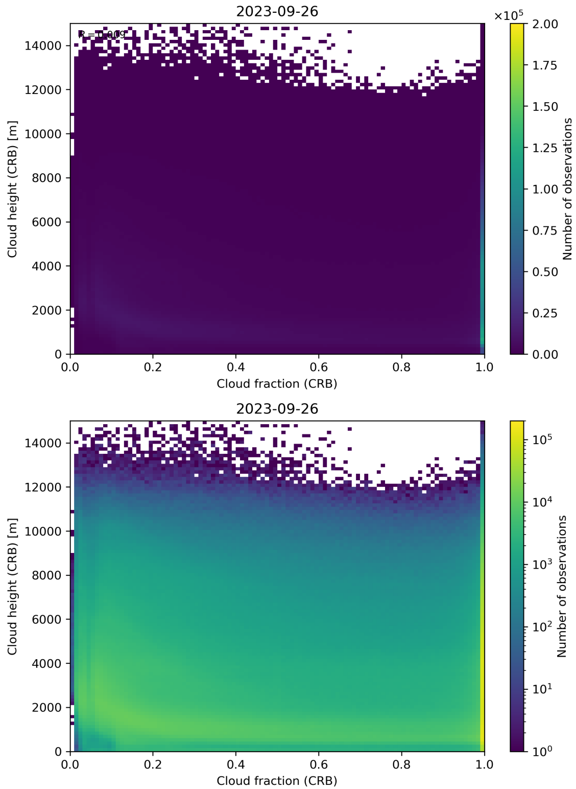
Figure 79: Scatter density plot of “Cloud fraction (CRB)” against “Cloud height (CRB)” for 2023-09-26 to 2023-09-27.
