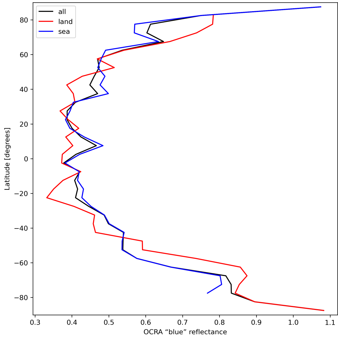
Figure 35: Zonal average of “OCRA “blue” reflectance” for 2023-09-26 to 2023-09-27.
