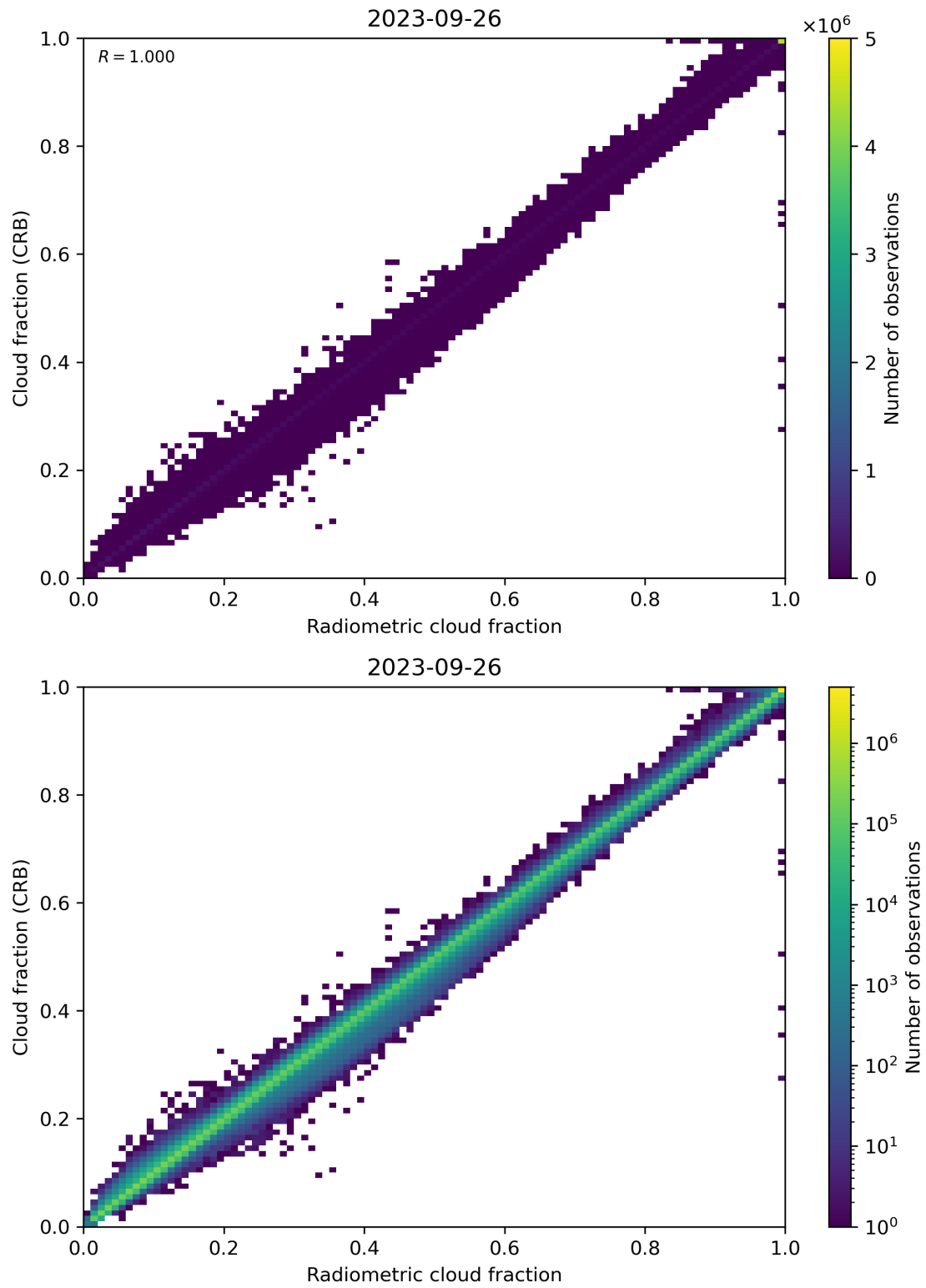
Figure 73: Scatter density plot of “Radiometric cloud fraction” against “Cloud fraction (CRB)” for 2023-09-26 to 2023-09-27.
