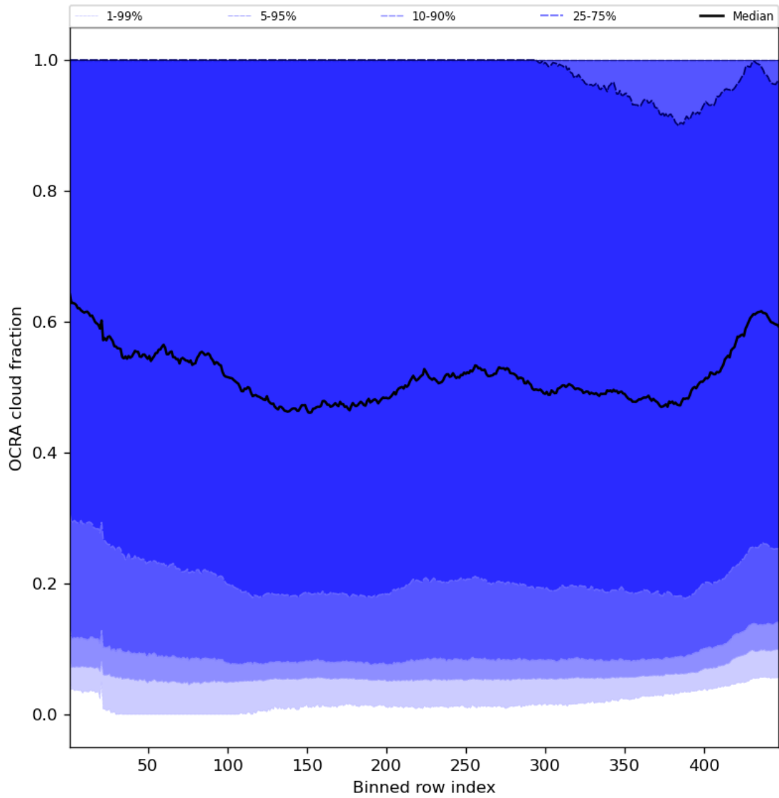
Figure 66: Along track statistics of “OCRA cloud fraction” for 2023-09-26 to 2023-09-27
