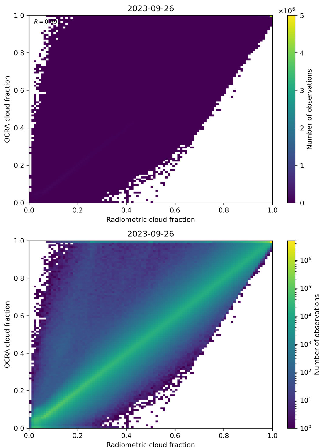
Figure 72: Scatter density plot of “Radiometric cloud fraction” against “OCRA cloud fraction” for 2023-09-26 to 2023-09-27.
