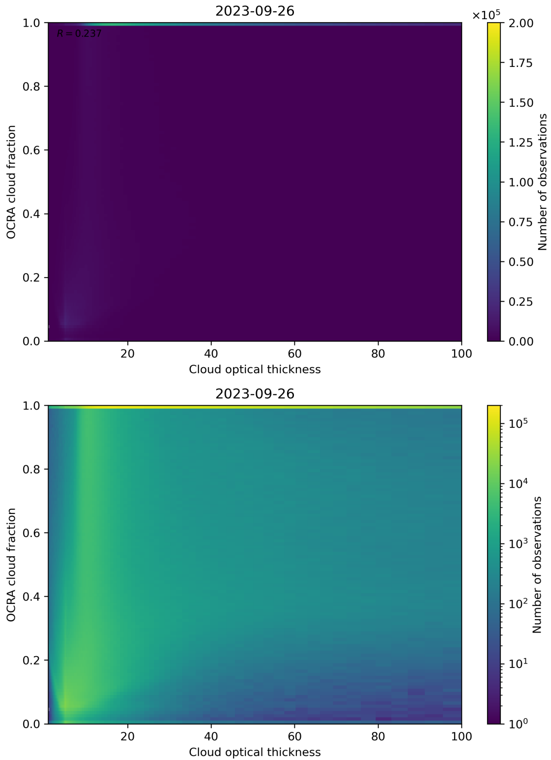
Figure 83: Scatter density plot of “Cloud optical thickness” against “OCRA cloud fraction” for 2023-09-26 to 2023-09-27.
