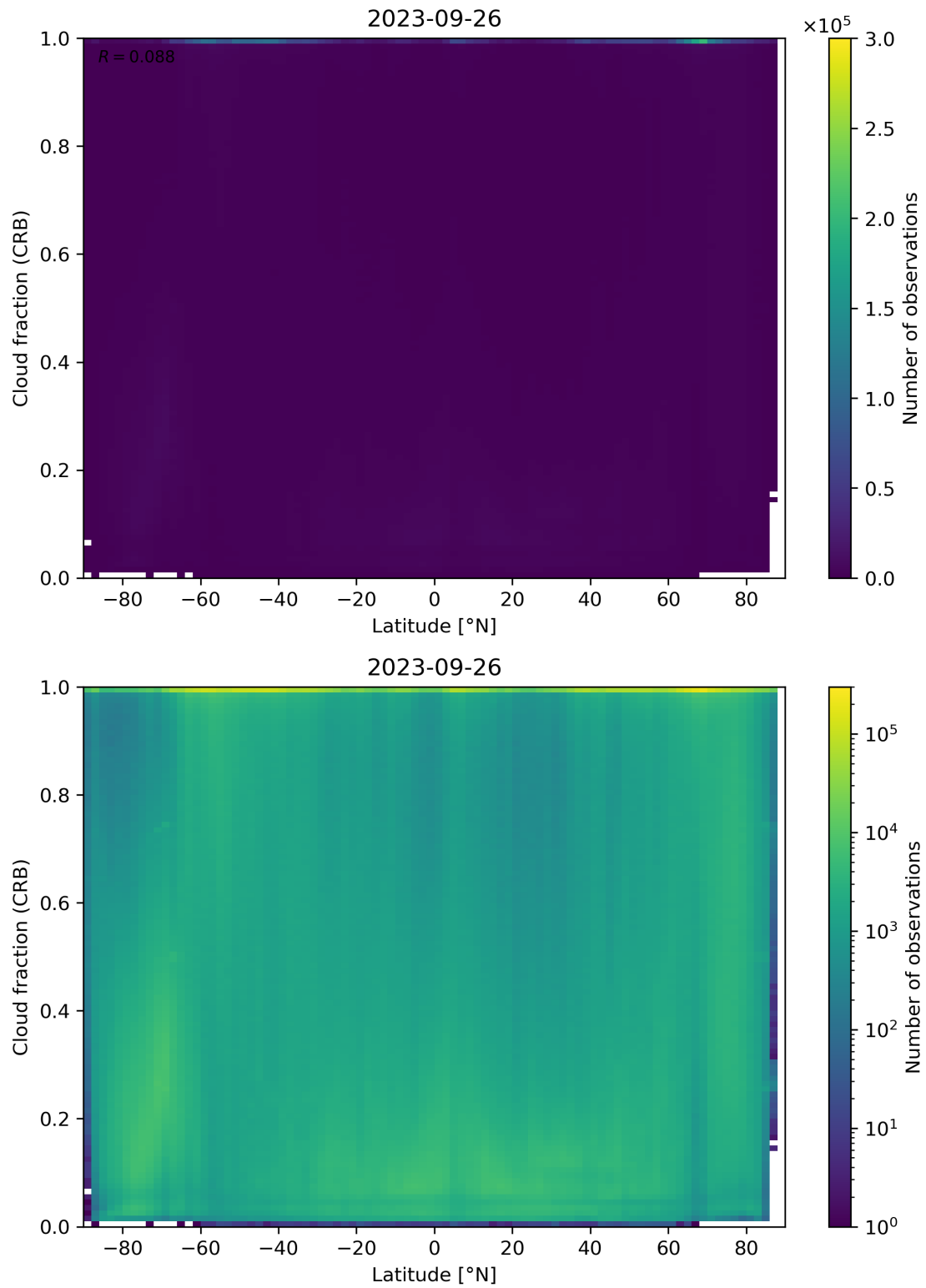
Figure 94: Scatter density plot of “Latitude” against “Cloud fraction (CRB)” for 2023-09-26 to 2023-09-27.
