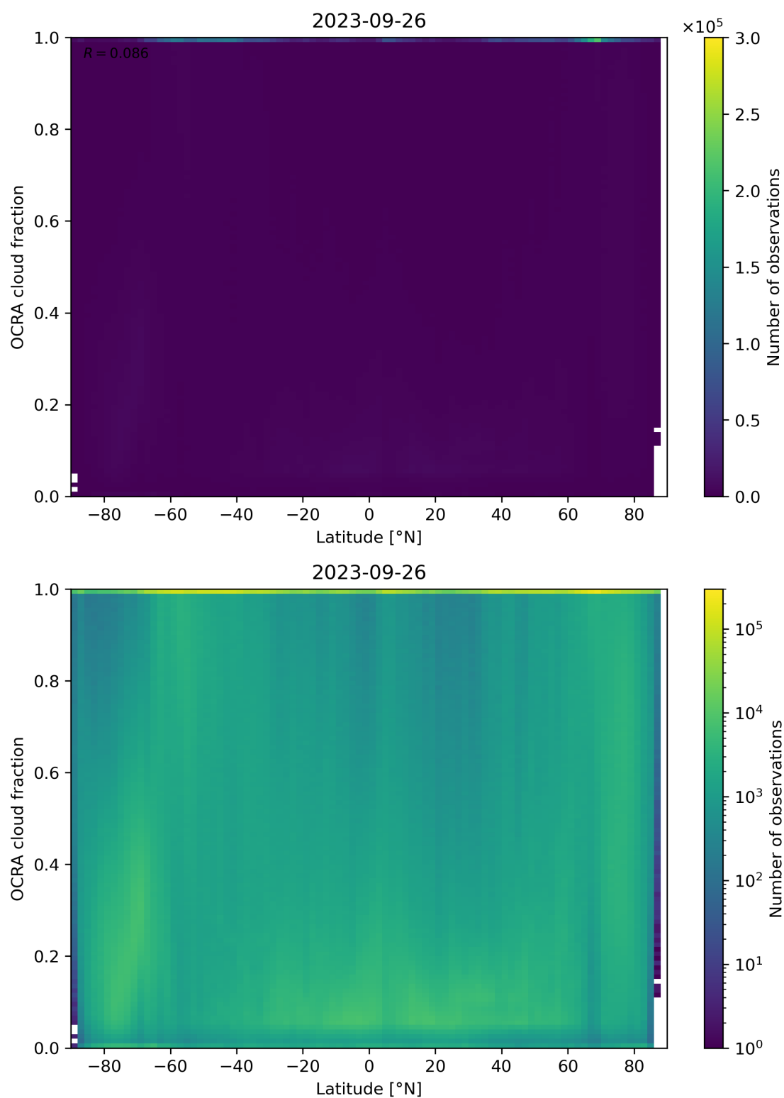
Figure 93: Scatter density plot of “Latitude” against “OCRA cloud fraction” for 2023-09-26 to 2023-09-27.
