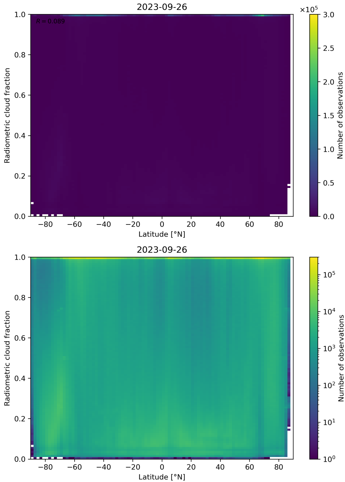
Figure 92: Scatter density plot of “Latitude” against “Radiometric cloud fraction” for 2023-09-26 to 2023-09-27.
