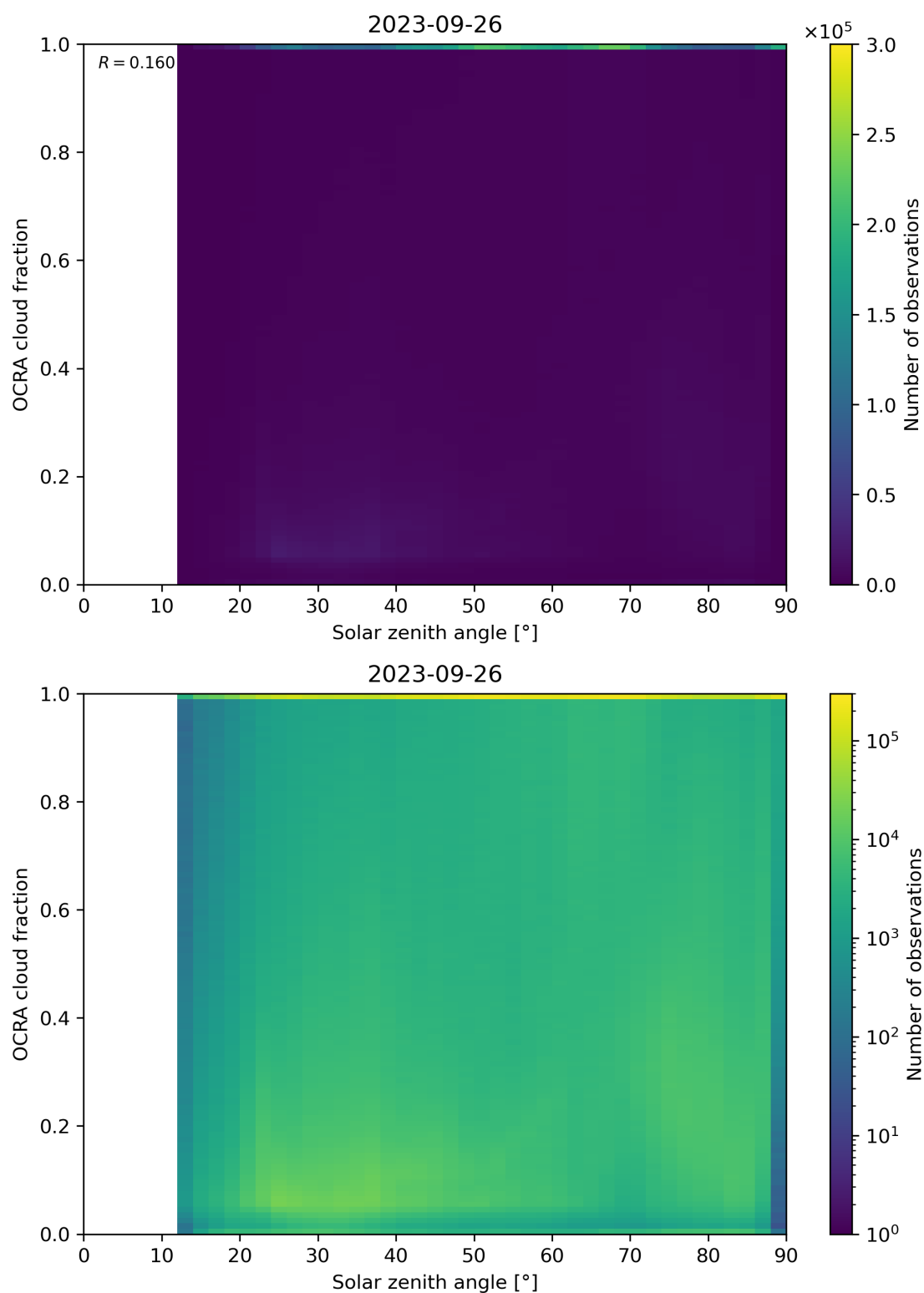
Figure 100: Scatter density plot of “Solar zenith angle” against “OCRA cloud fraction” for 2023-09-26 to 2023-09-27.
