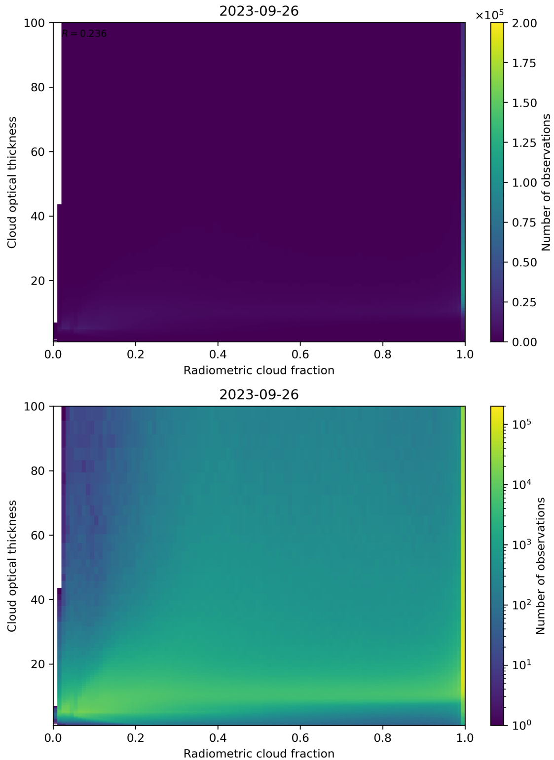
Figure 75: Scatter density plot of “Radiometric cloud fraction” against “Cloud optical thickness” for 2023-09-26 to 2023-09-27.
