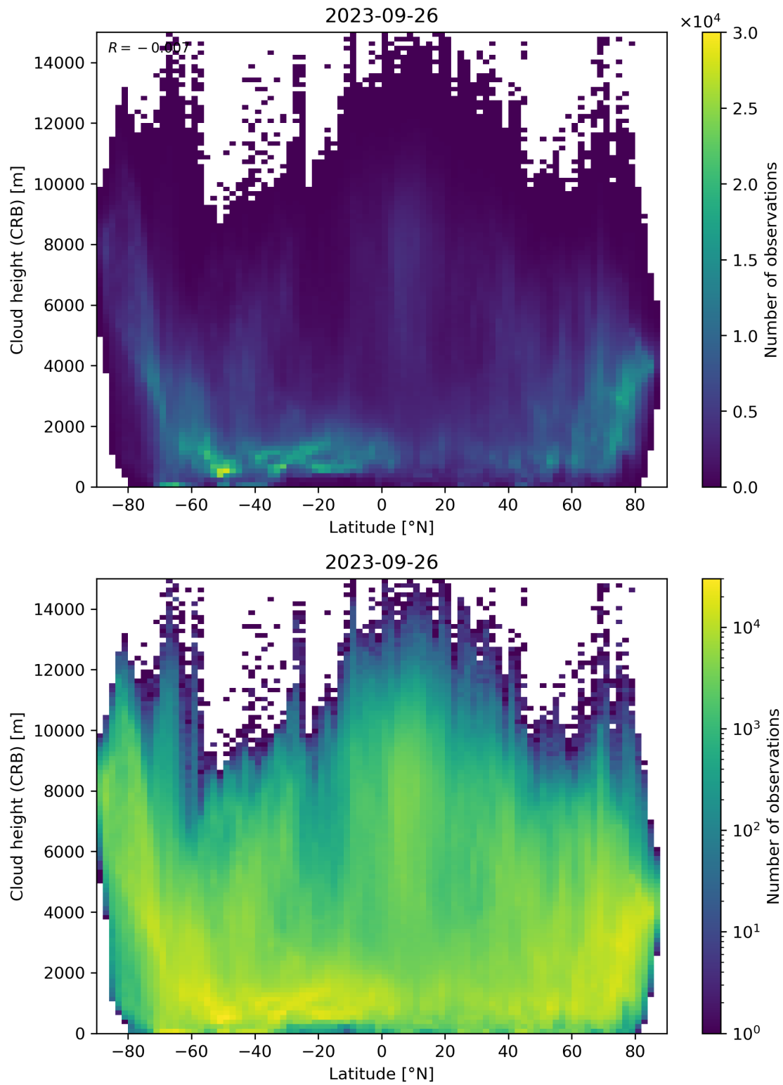
Figure 95: Scatter density plot of “Latitude” against “Cloud height (CRB)” for 2023-09-26 to 2023-09-27.
