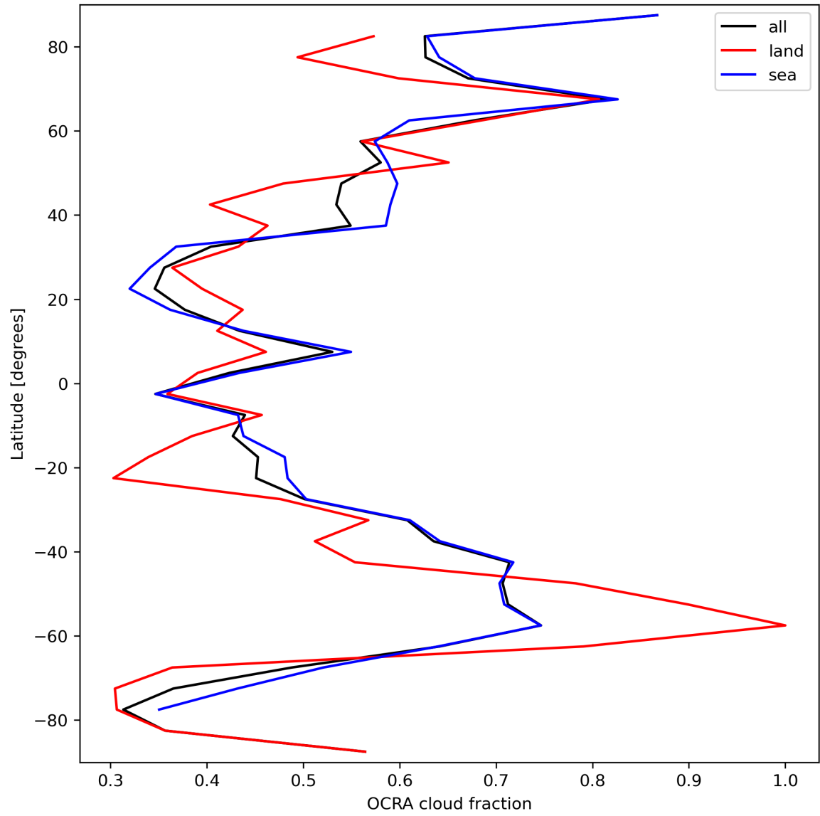
Figure 34: Zonal average of “OCRA cloud fraction” for 2023-09-26 to 2023-09-27.
