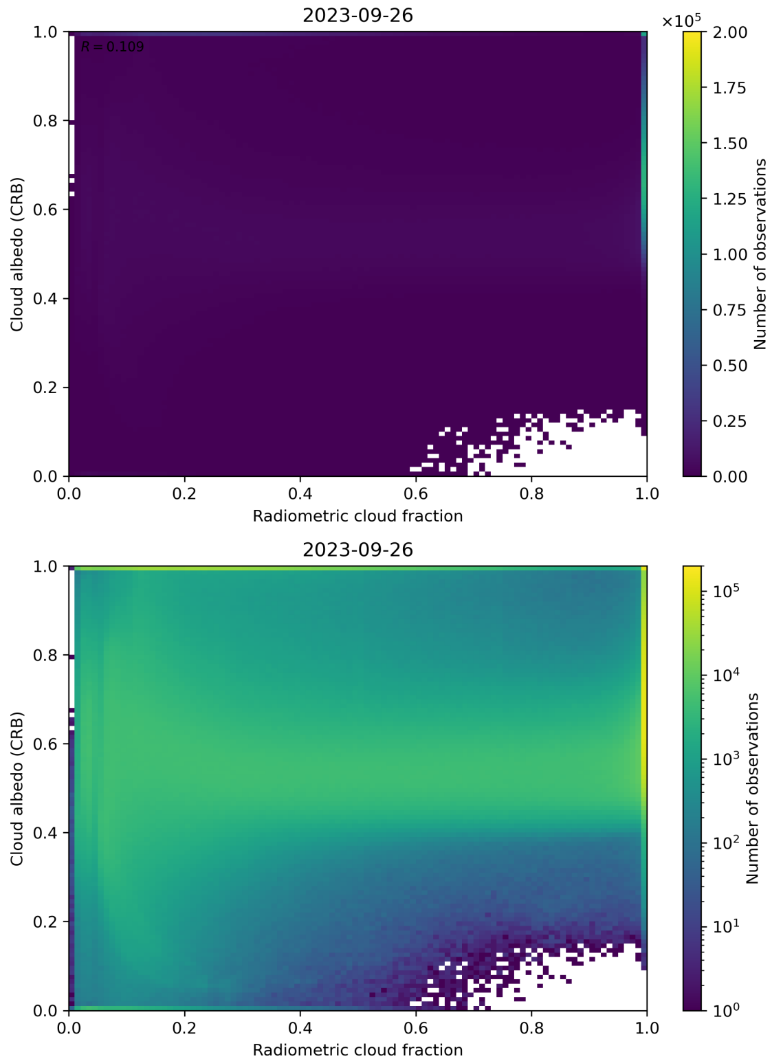
Figure 71: Scatter density plot of “Radiometric cloud fraction” against “Cloud albedo (CRB)” for 2023-09-26 to 2023-09-27.
