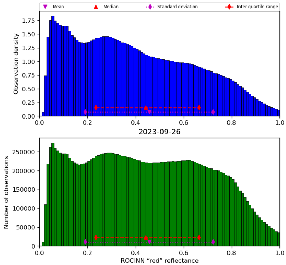
Figure 53: Histogram of “ROCINN “red” reflectance” for 2023-09-26 to 2023-09-27
