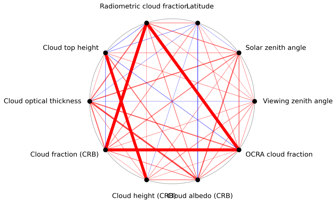
Figure 1: Map of correlation graph for 2023-09-26 to 2023-09-27.
