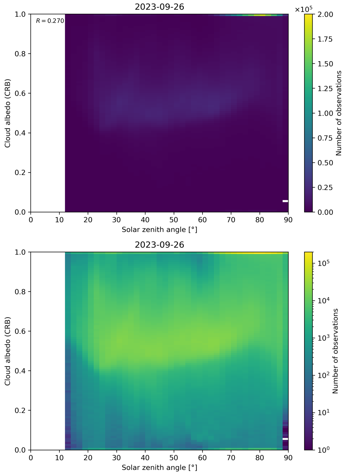
Figure 98: Scatter density plot of “Solar zenith angle” against “Cloud albedo (CRB)” for 2023-09-26 to 2023-09-27.
