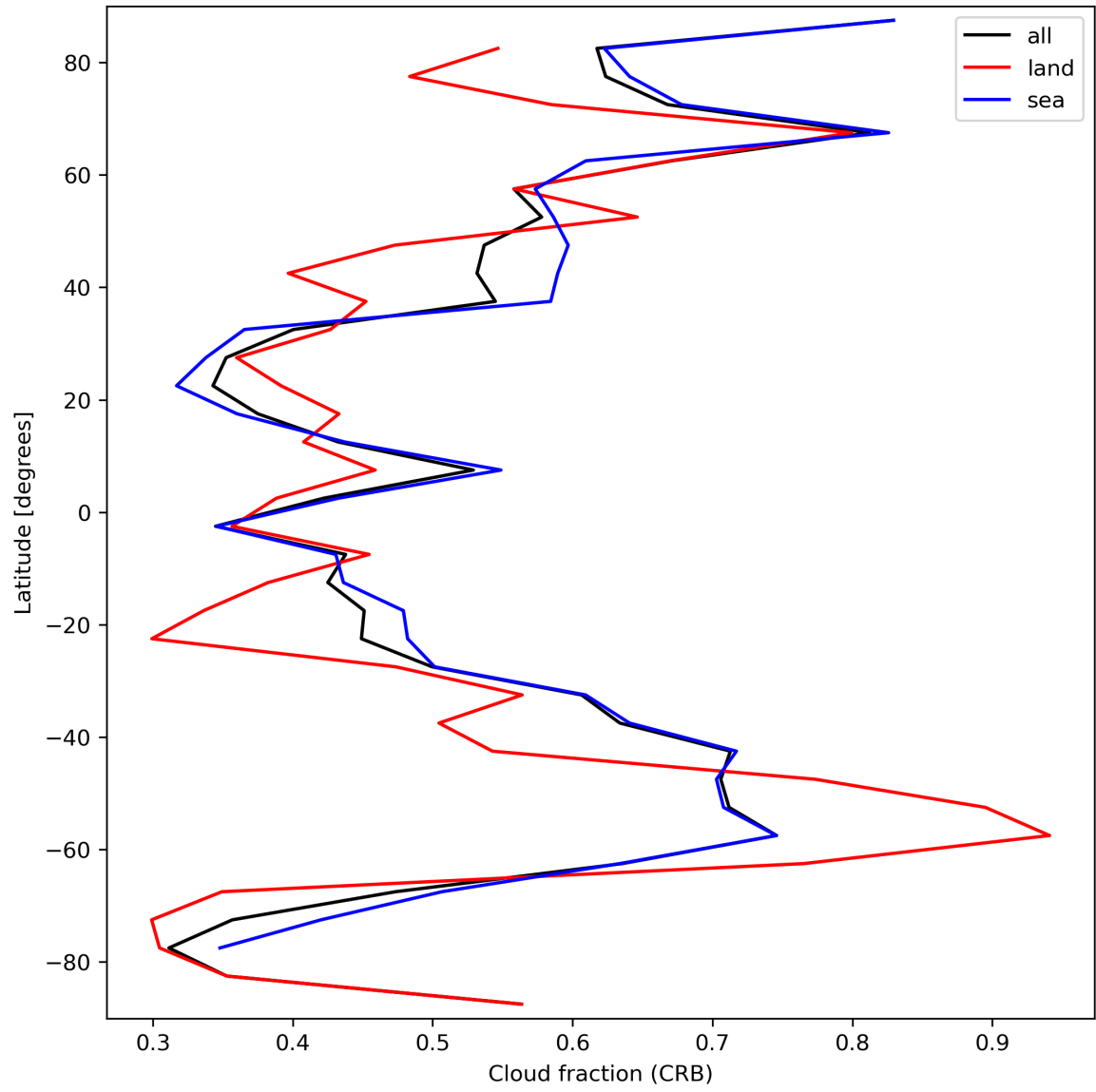
Figure 26: Zonal average of “Cloud fraction (CRB)” for 2023-09-26 to 2023-09-27.
