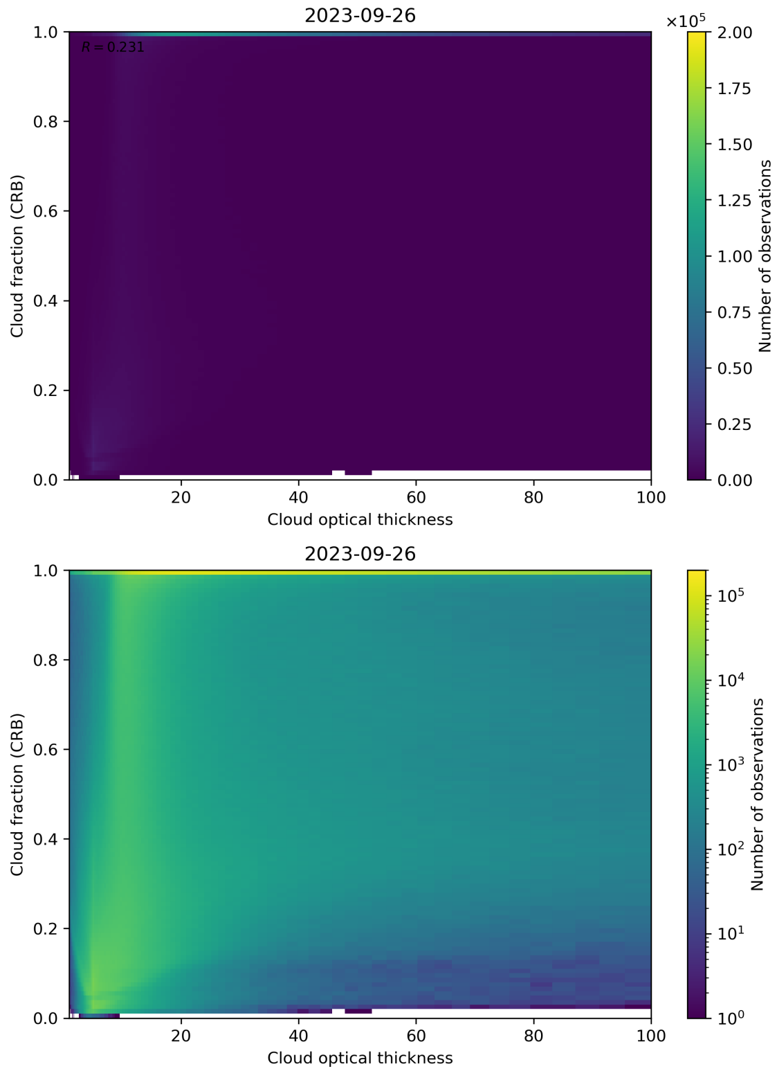
Figure 84: Scatter density plot of “Cloud optical thickness” against “Cloud fraction (CRB)” for 2023-09-26 to 2023-09-27.
