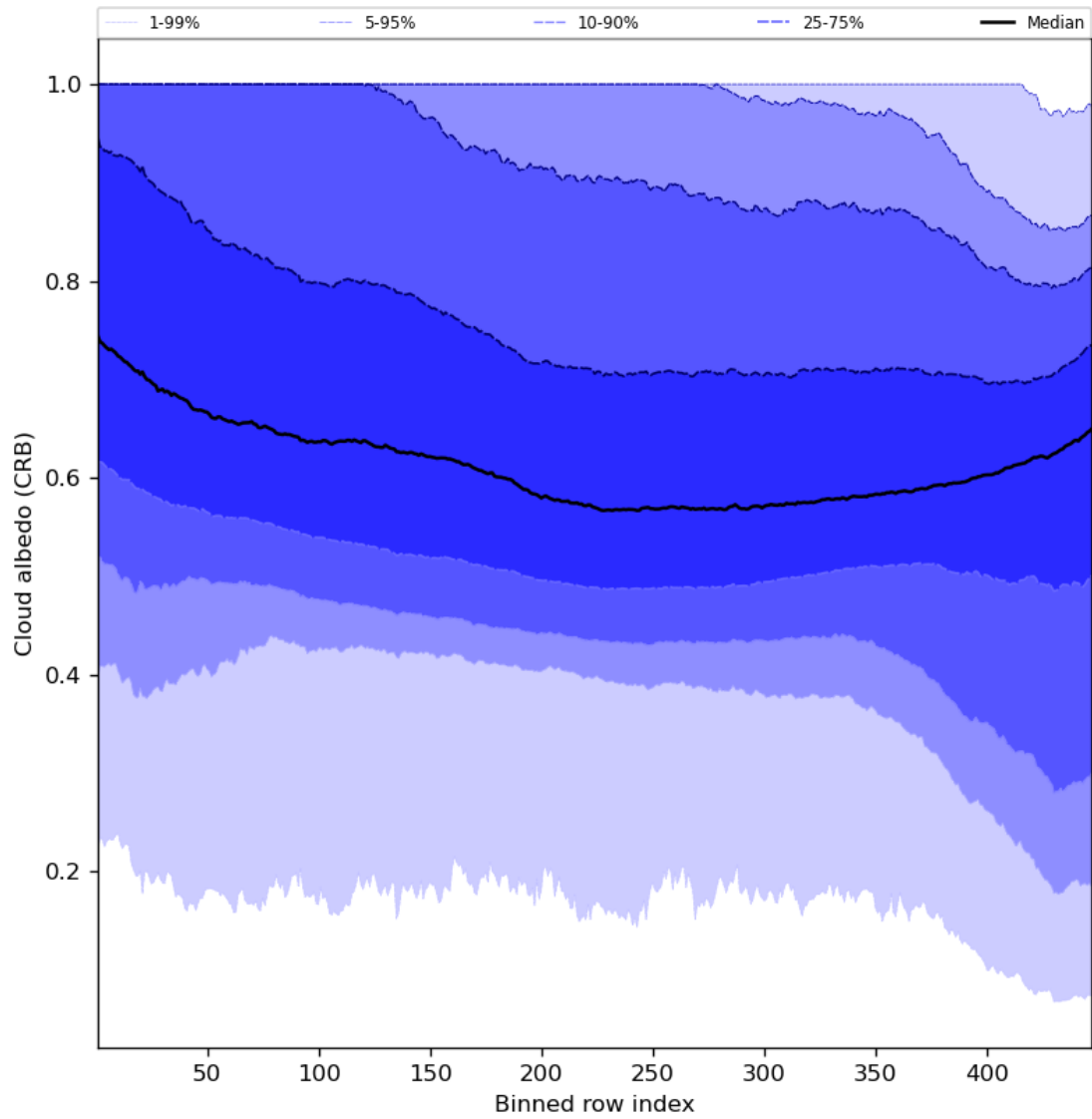
Figure 60: Along track statistics of “Cloud albedo (CRB)” for 2023-09-26 to 2023-09-27
