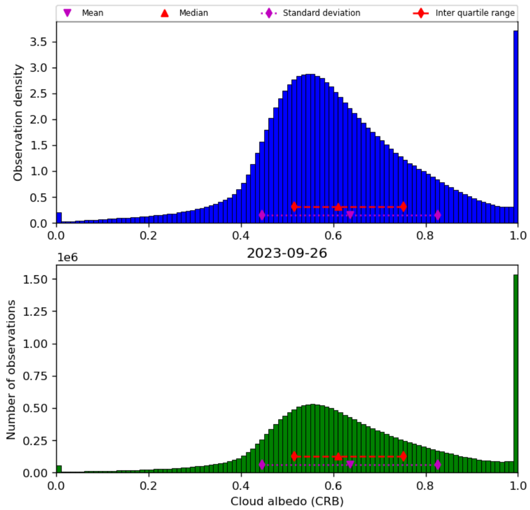
Figure 44: Histogram of “Cloud albedo (CRB)” for 2023-09-26 to 2023-09-27
