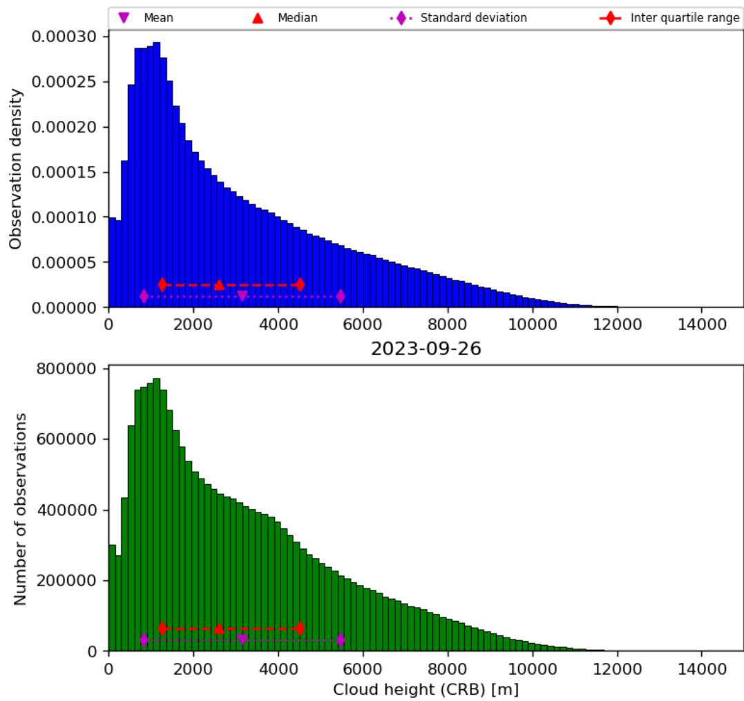
Figure 43: Histogram of “Cloud height (CRB)” for 2023-09-26 to 2023-09-27
