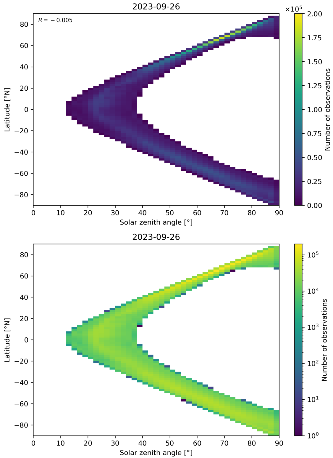
Figure 105: Scatter density plot of “Solar zenith angle” against “Latitude” for 2023-09-26 to 2023-09-27.
