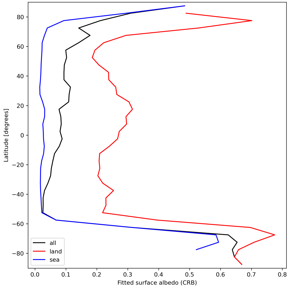
Figure 30: Zonal average of “Fitted surface albedo (CRB)” for 2023-09-26 to 2023-09-27.
