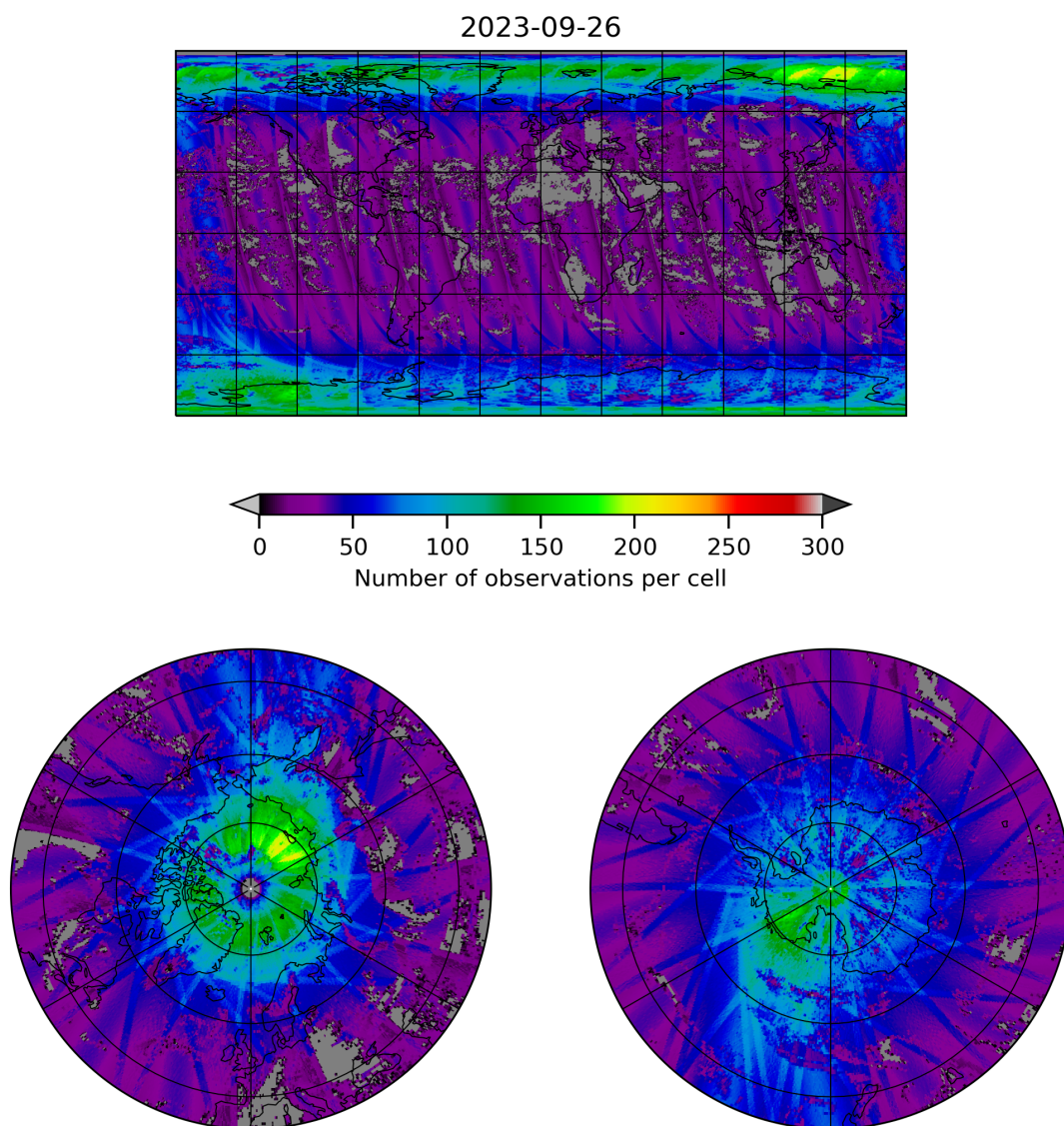
Figure 21: Map of the number of observations for 2023-09-26 to 2023-09-27
