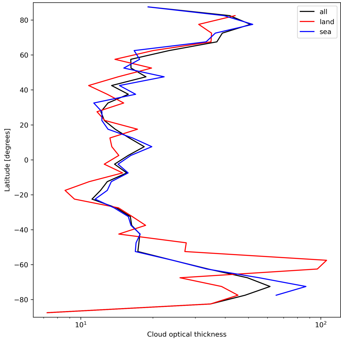
Figure 25: Zonal average of “Cloud optical thickness” for 2023-09-26 to 2023-09-27.
