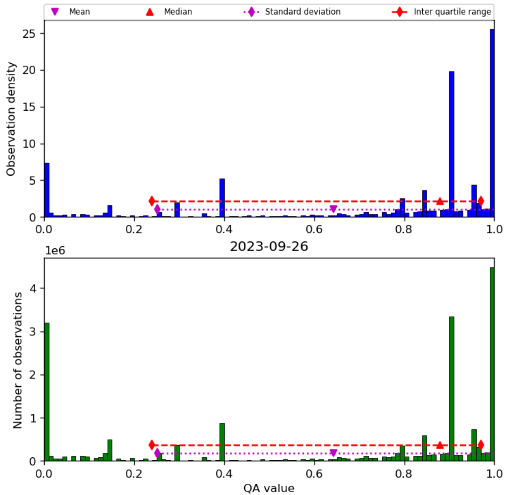
Figure 38: Histogram of “QA value” for 2023-09-26 to 2023-09-27
