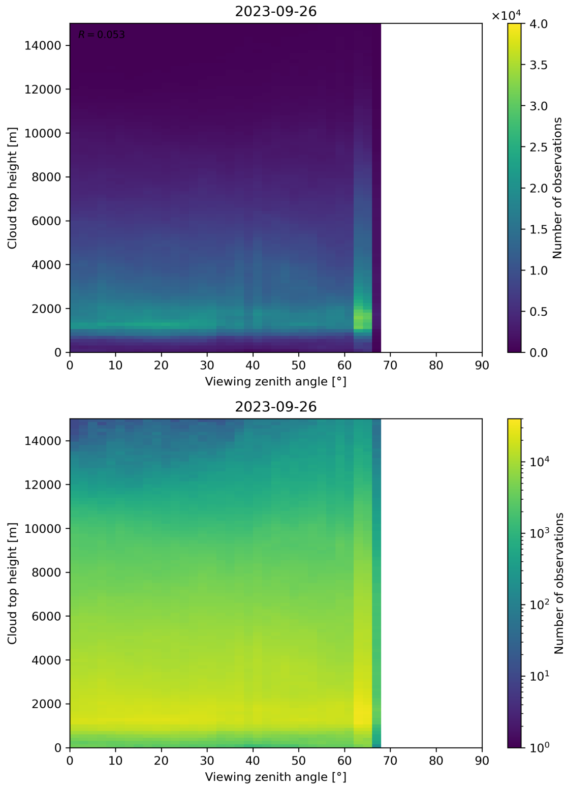
Figure 112: Scatter density plot of “Viewing zenith angle” against “Cloud top height” for 2023-09-26 to 2023-09-27.
