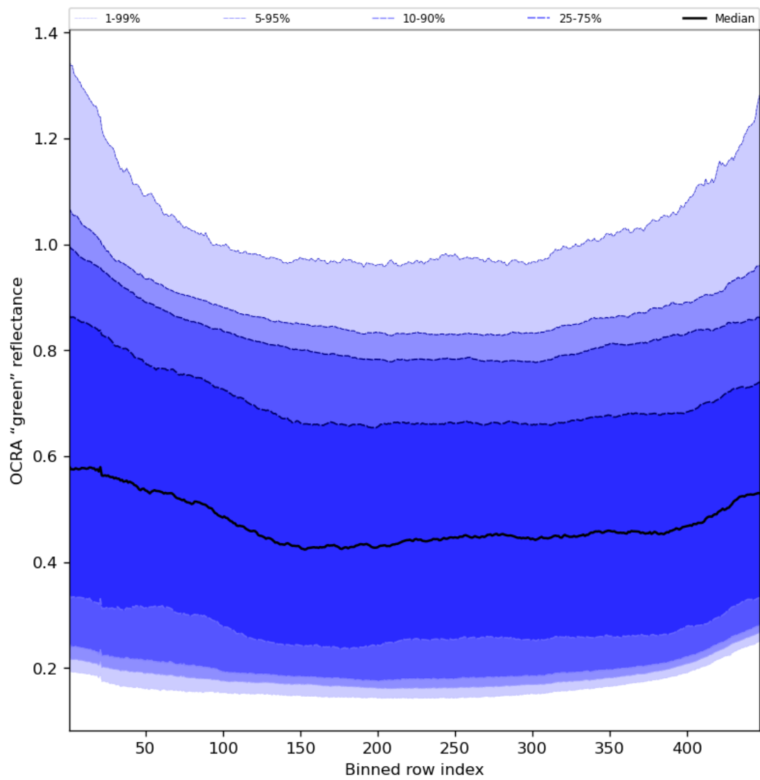
Figure 68: Along track statistics of “OCRA “green” reflectance” for 2023-09-26 to 2023-09-27
