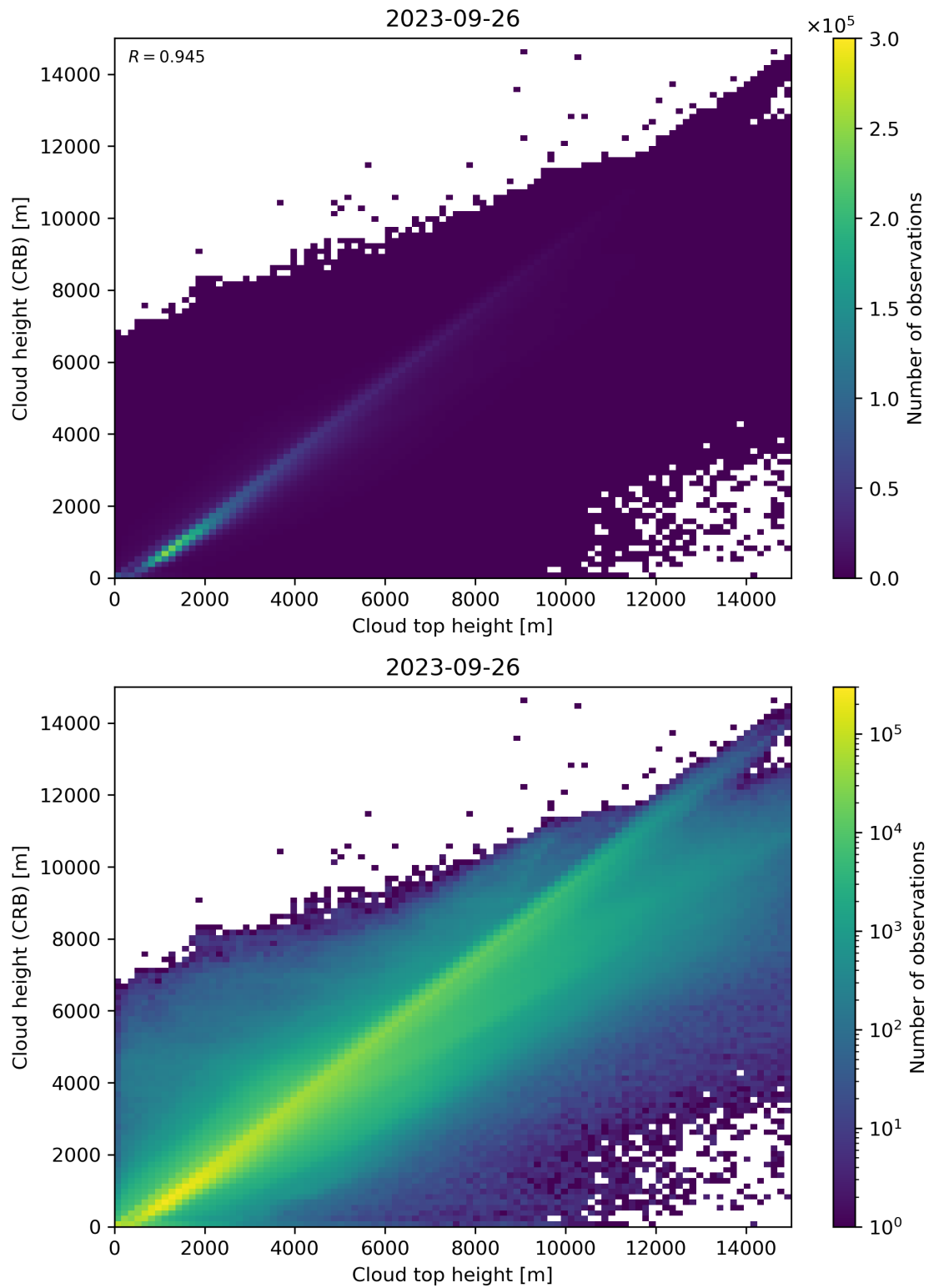
Figure 89: Scatter density plot of “Cloud top height” against “Cloud height (CRB)” for 2023-09-26 to 2023-09-27.
