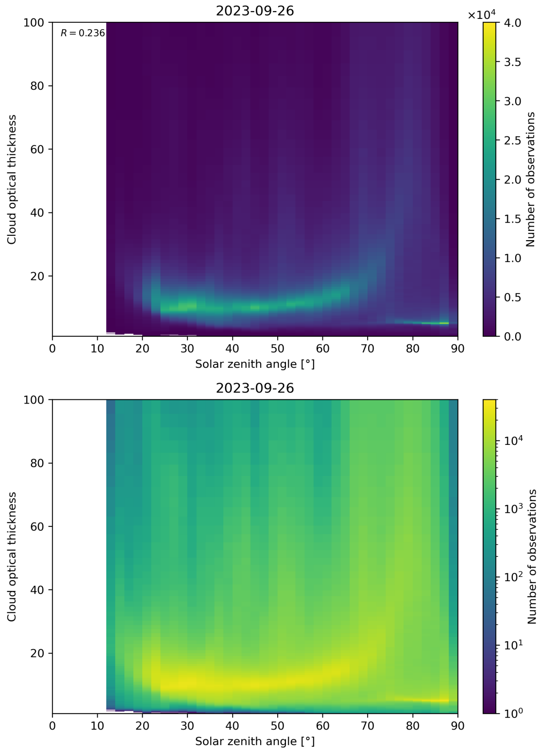
Figure 103: Scatter density plot of “Solar zenith angle” against “Cloud optical thickness” for 2023-09-26 to 2023-09-27.
