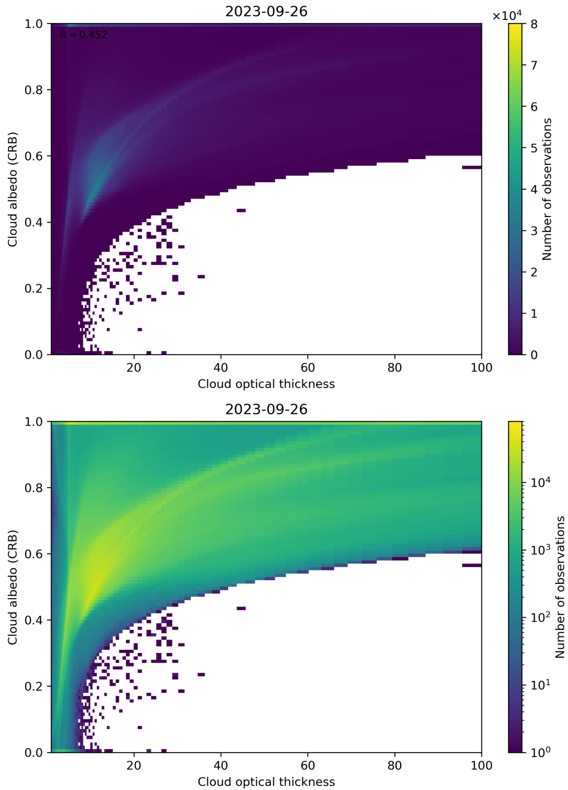
Figure 82: Scatter density plot of “Cloud optical thickness” against “Cloud albedo (CRB)” for 2023-09-26 to 2023-09-27.
