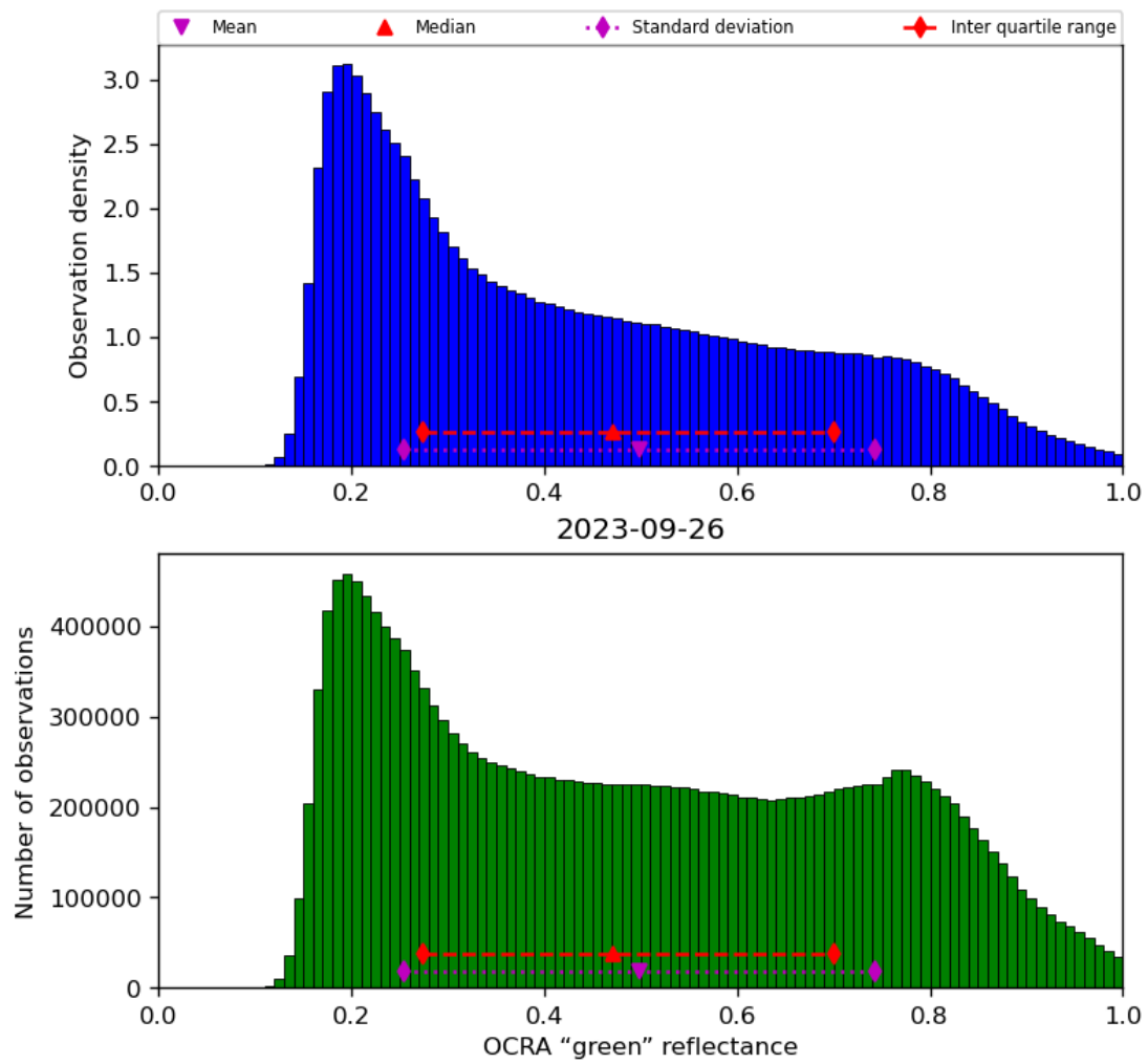
Figure 52: Histogram of “OCRA “green” reflectance” for 2023-09-26 to 2023-09-27
