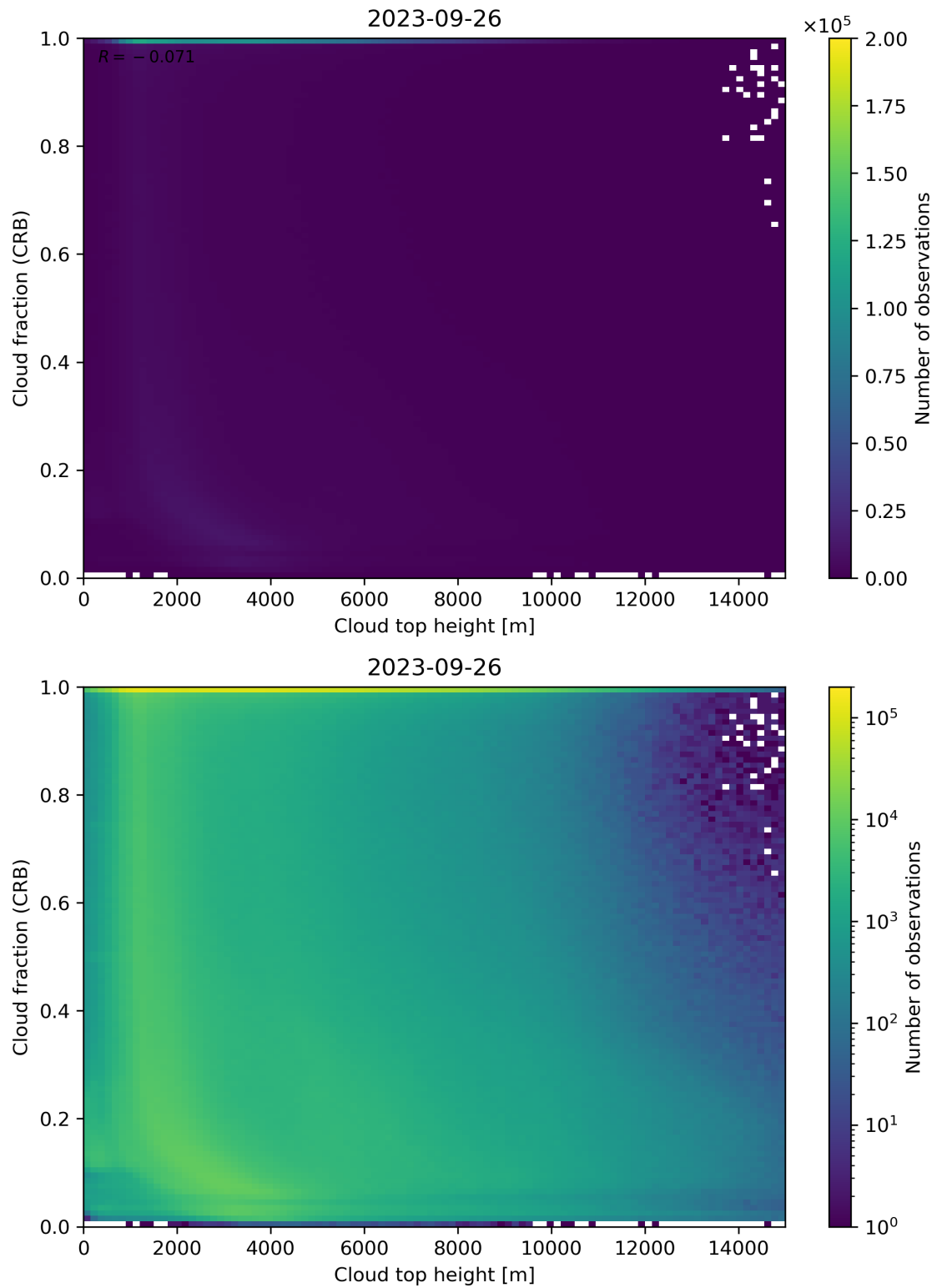
Figure 88: Scatter density plot of “Cloud top height” against “Cloud fraction (CRB)” for 2023-09-26 to 2023-09-27.
