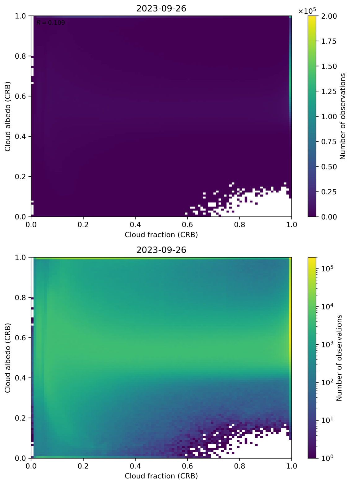
Figure 77: Scatter density plot of “Cloud fraction (CRB)” against “Cloud albedo (CRB)” for 2023-09-26 to 2023-09-27.
