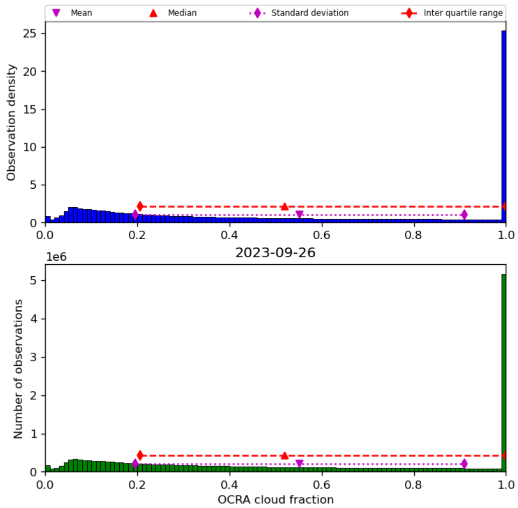
Figure 50: Histogram of “OCRA cloud fraction” for 2023-09-26 to 2023-09-27
