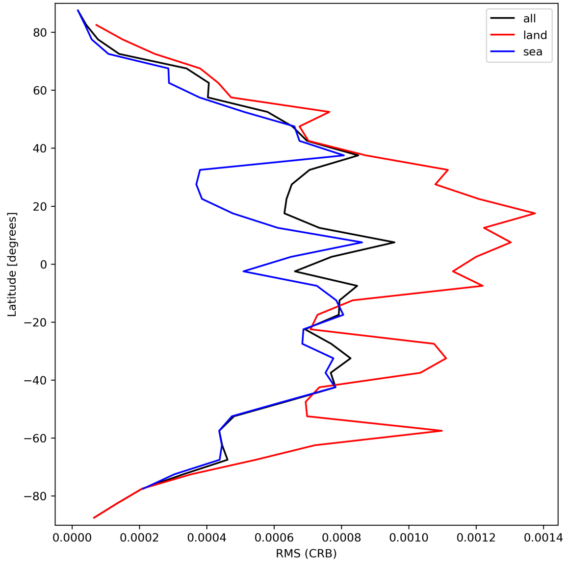
Figure 32: Zonal average of “RMS (CRB)” for 2023-09-26 to 2023-09-27.
