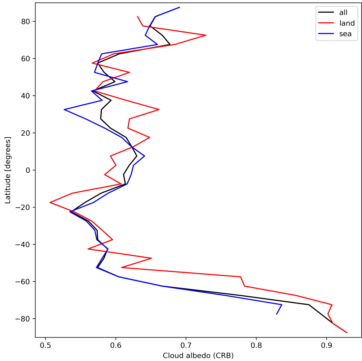
Figure 28: Zonal average of “Cloud albedo (CRB)” for 2023-09-26 to 2023-09-27.
