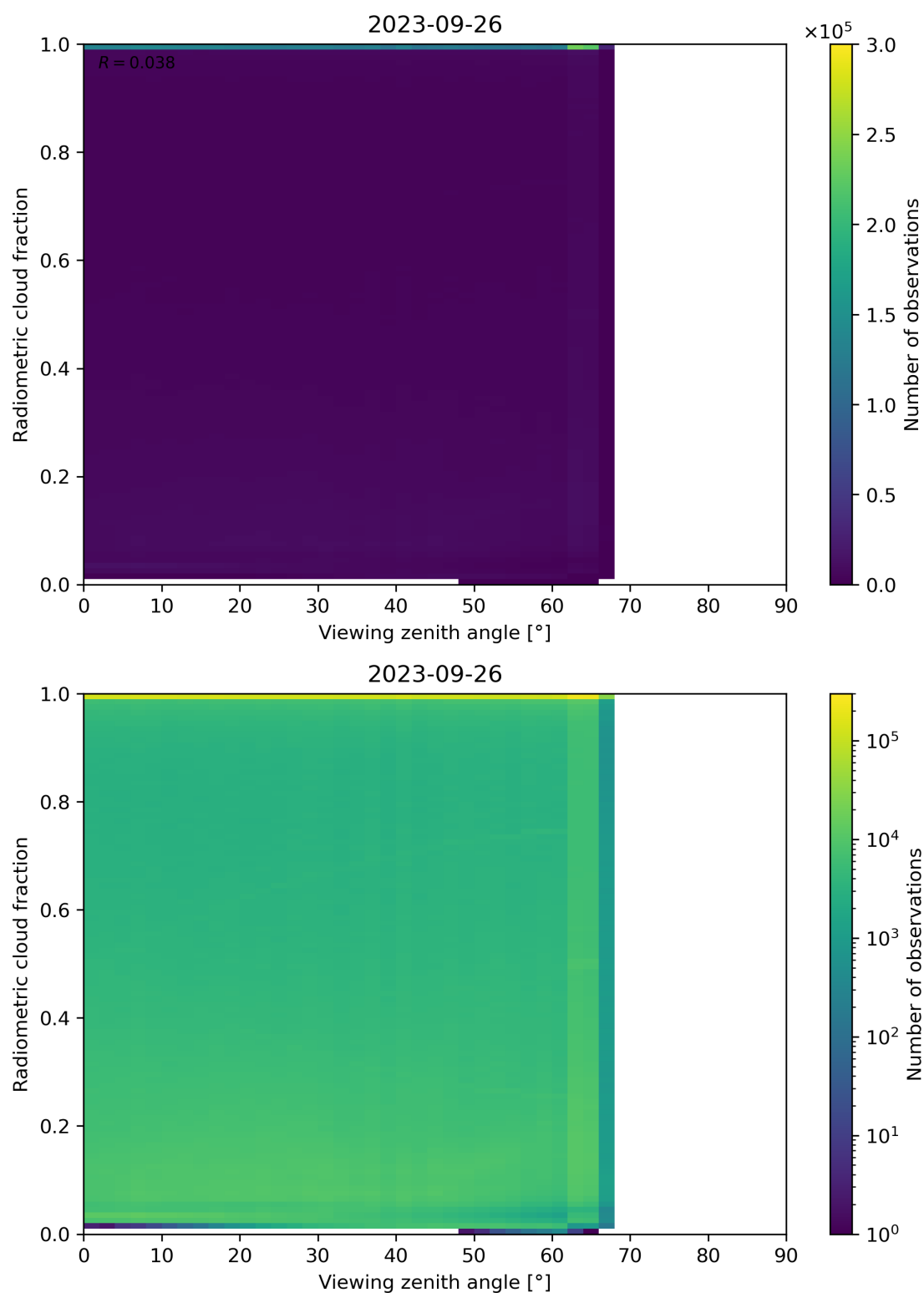
Figure 107: Scatter density plot of “Viewing zenith angle” against “Radiometric cloud fraction” for 2023-09-26 to 2023-09-27.
