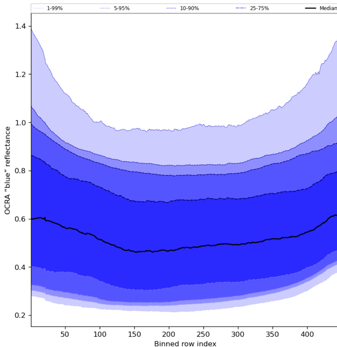
Figure 67: Along track statistics of “OCRA “blue” reflectance” for 2023-09-26 to 2023-09-27
