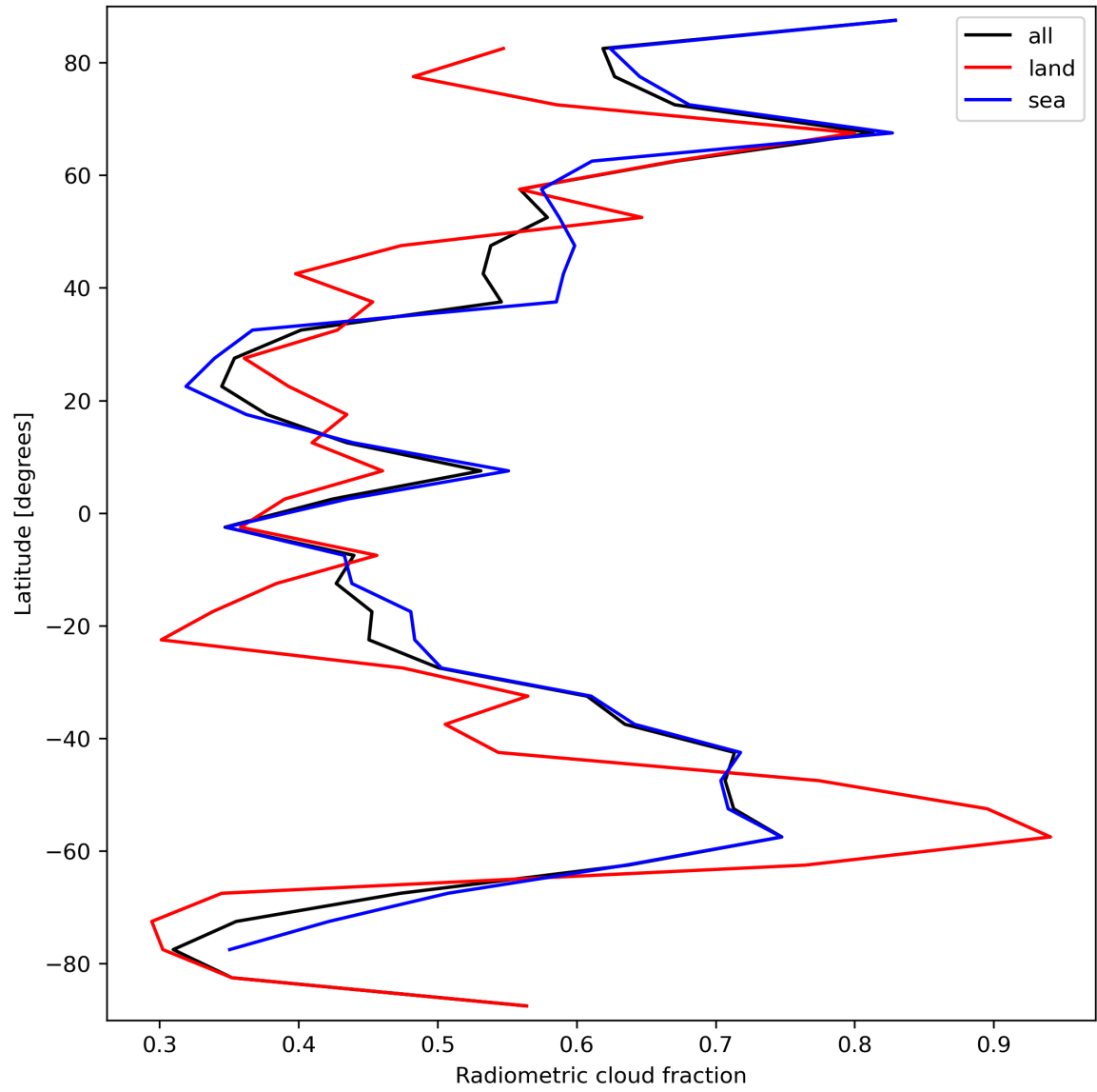
Figure 23: Zonal average of “Radiometric cloud fraction” for 2023-09-26 to 2023-09-27.
