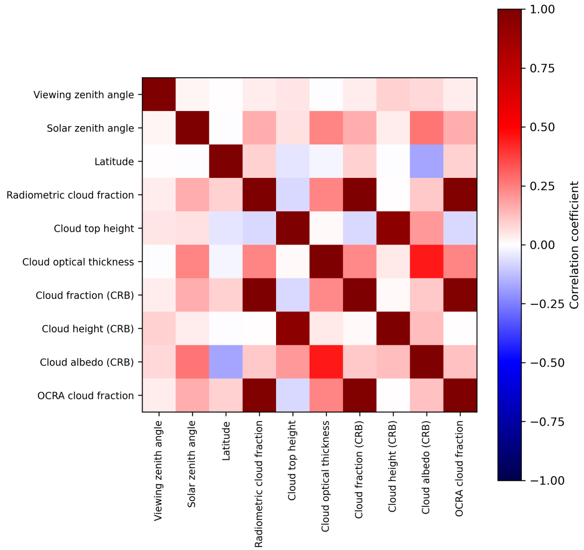
Figure 2: Map of correlation matrix for 2023-09-26 to 2023-09-27.
