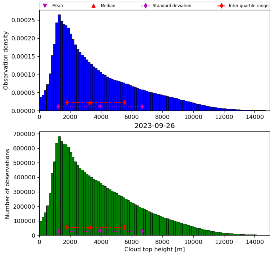
Figure 40: Histogram of “Cloud top height” for 2023-09-26 to 2023-09-27
