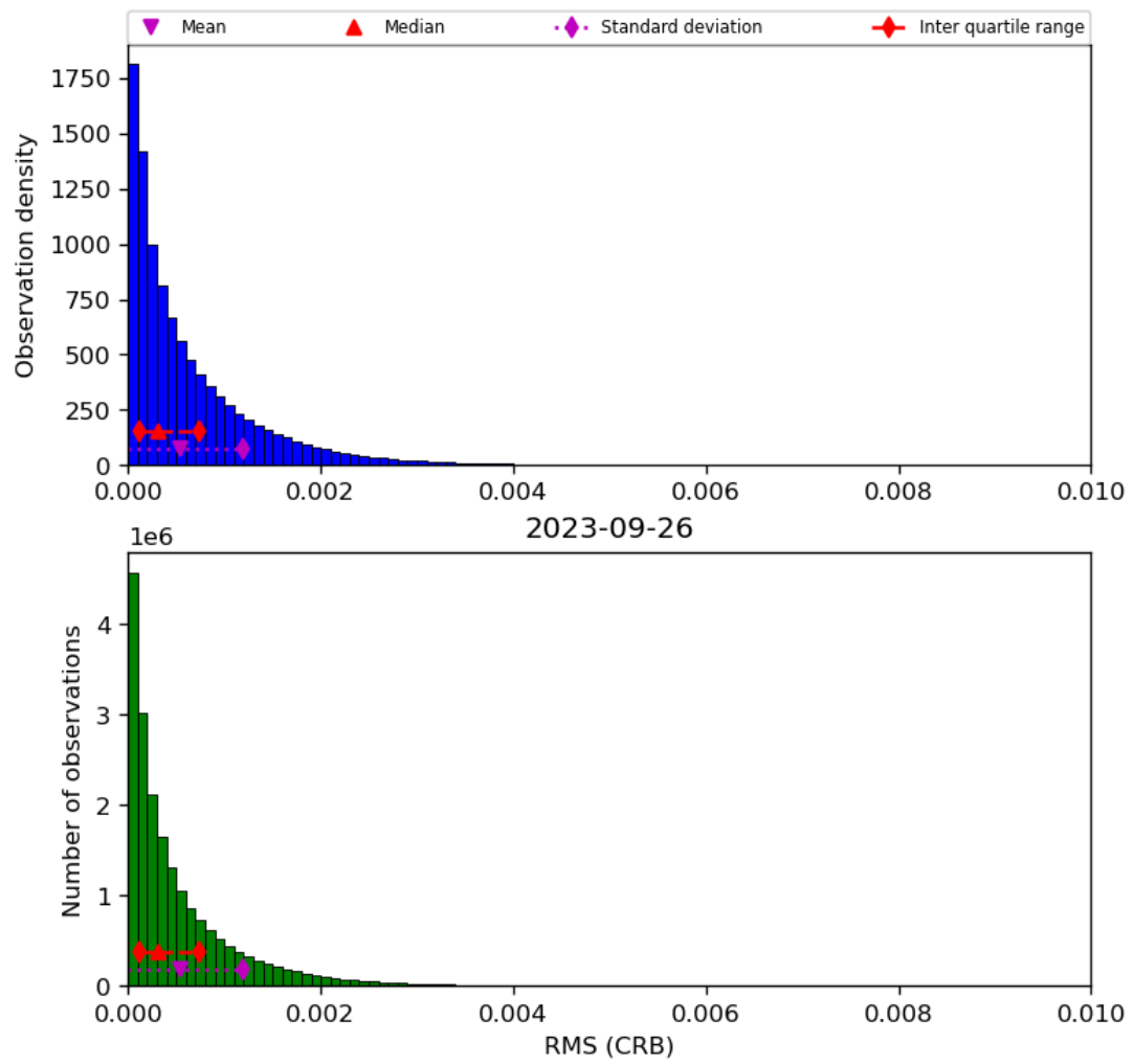
Figure 48: Histogram of "RMS (CRB)" for 2023-09-26 to 2023-09-27
