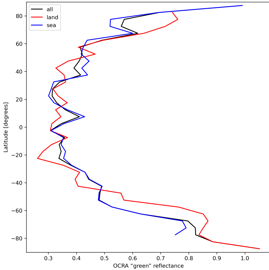
Figure 36: Zonal average of “OCRA “green” reflectance” for 2023-09-26 to 2023-09-27.
