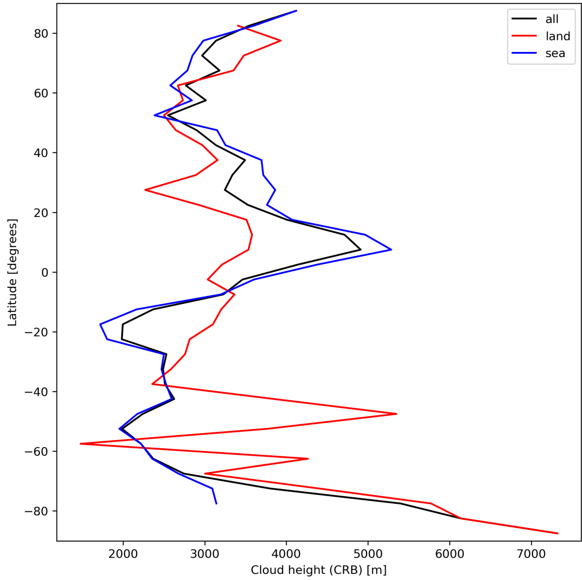
Figure 27: Zonal average of “Cloud height (CRB)” for 2023-09-26 to 2023-09-27.
