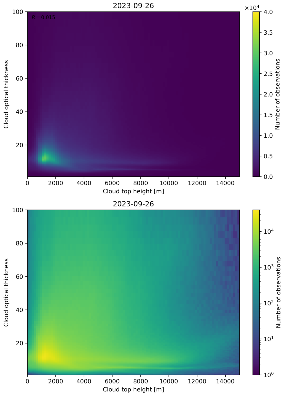
Figure 90: Scatter density plot of “Cloud top height” against “Cloud optical thickness” for 2023-09-26 to 2023-09-27.
