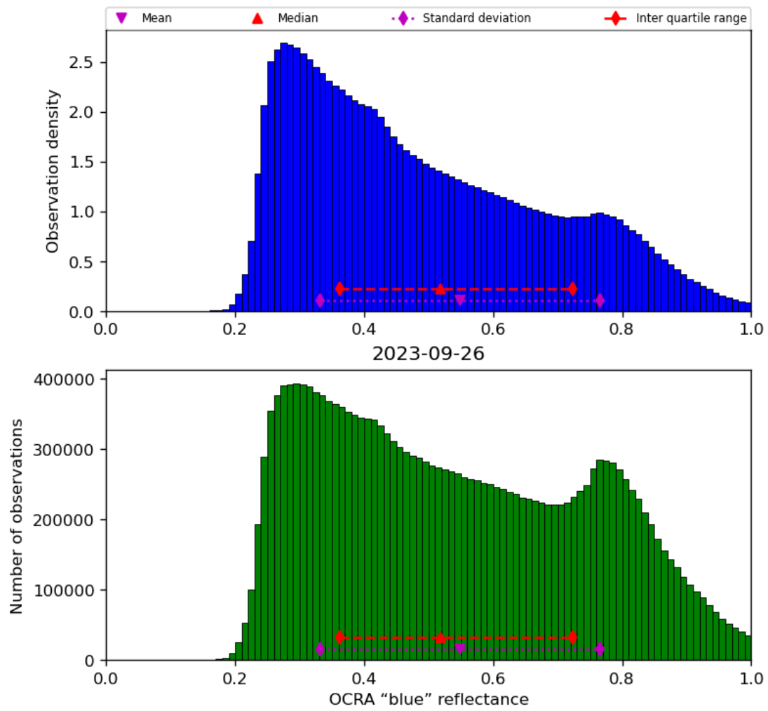
Figure 51: Histogram of “OCRA “blue” reflectance” for 2023-09-26 to 2023-09-27
