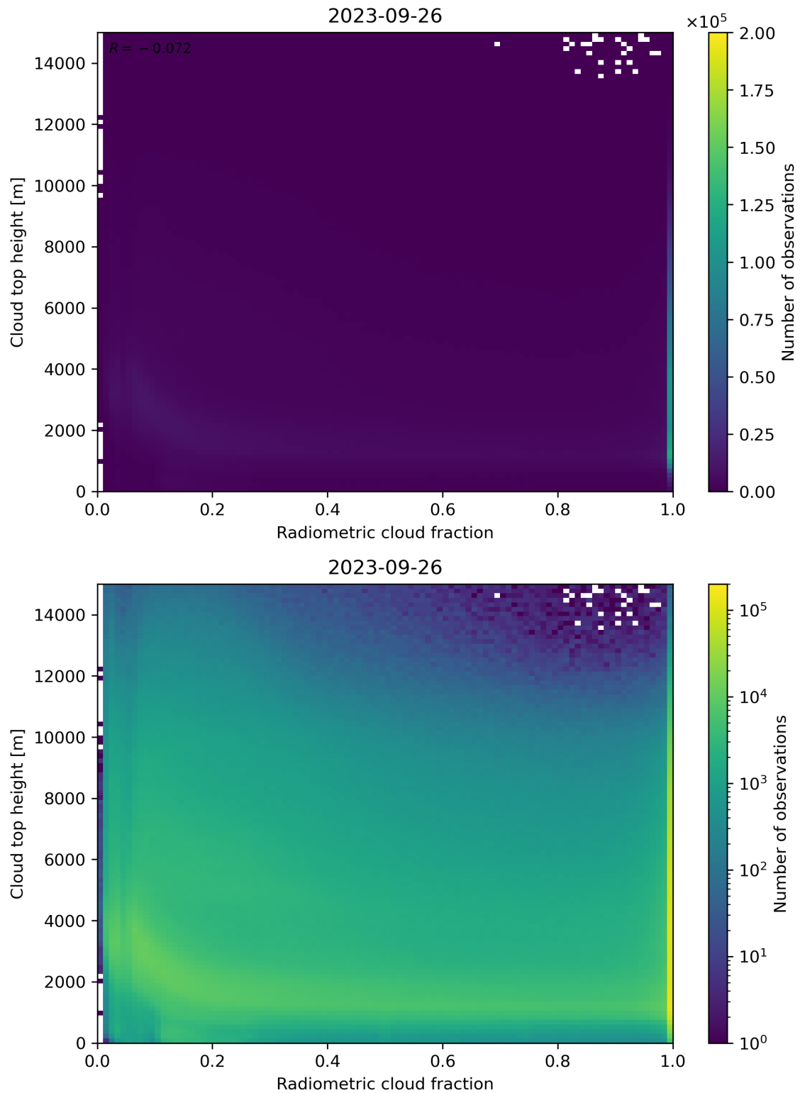
Figure 76: Scatter density plot of “Radiometric cloud fraction” against “Cloud top height” for 2023-09-26 to 2023-09-27.
