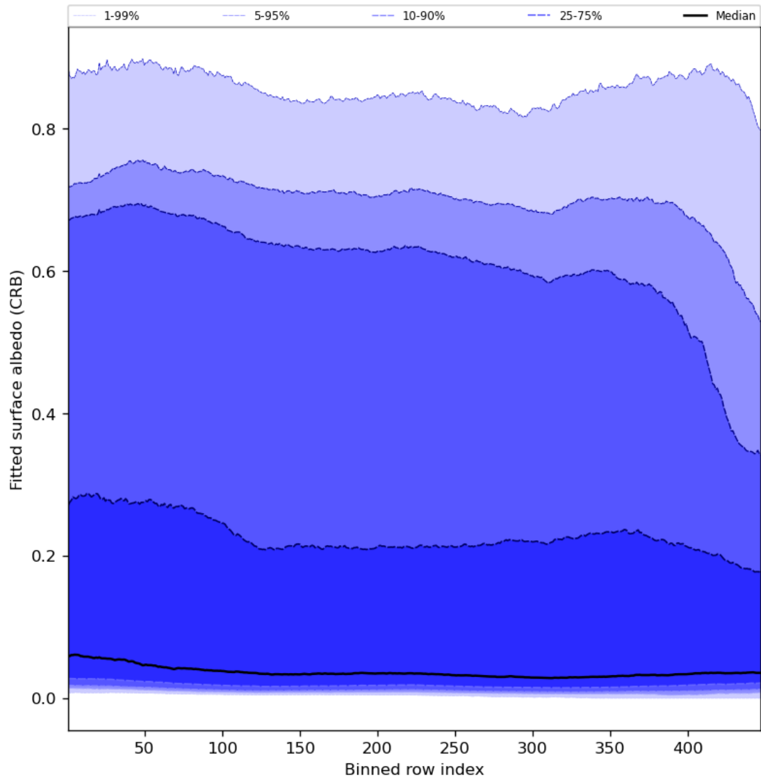
Figure 62: Along track statistics of “Fitted surface albedo (CRB)” for 2023-09-26 to 2023-09-27
