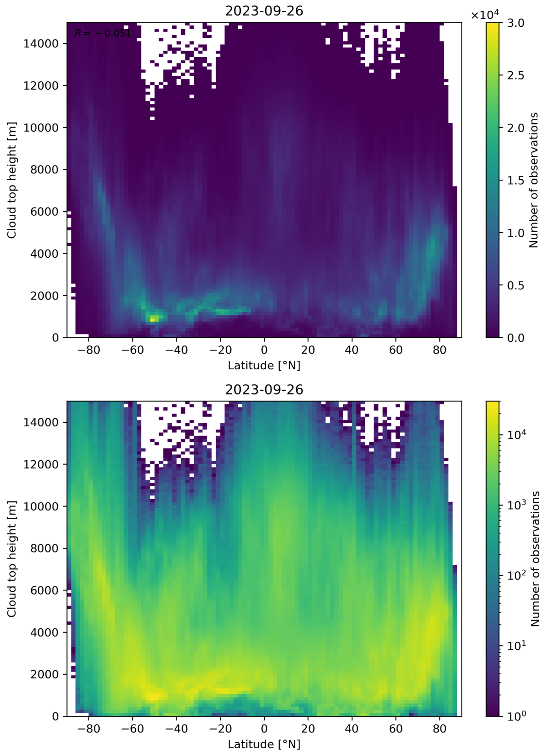
Figure 97: Scatter density plot of “Latitude” against “Cloud top height” for 2023-09-26 to 2023-09-27.
