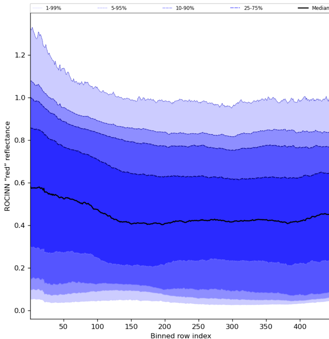
Figure 69: Along track statistics of “ROCINN “red” reflectance” for 2023-09-26 to 2023-09-27
