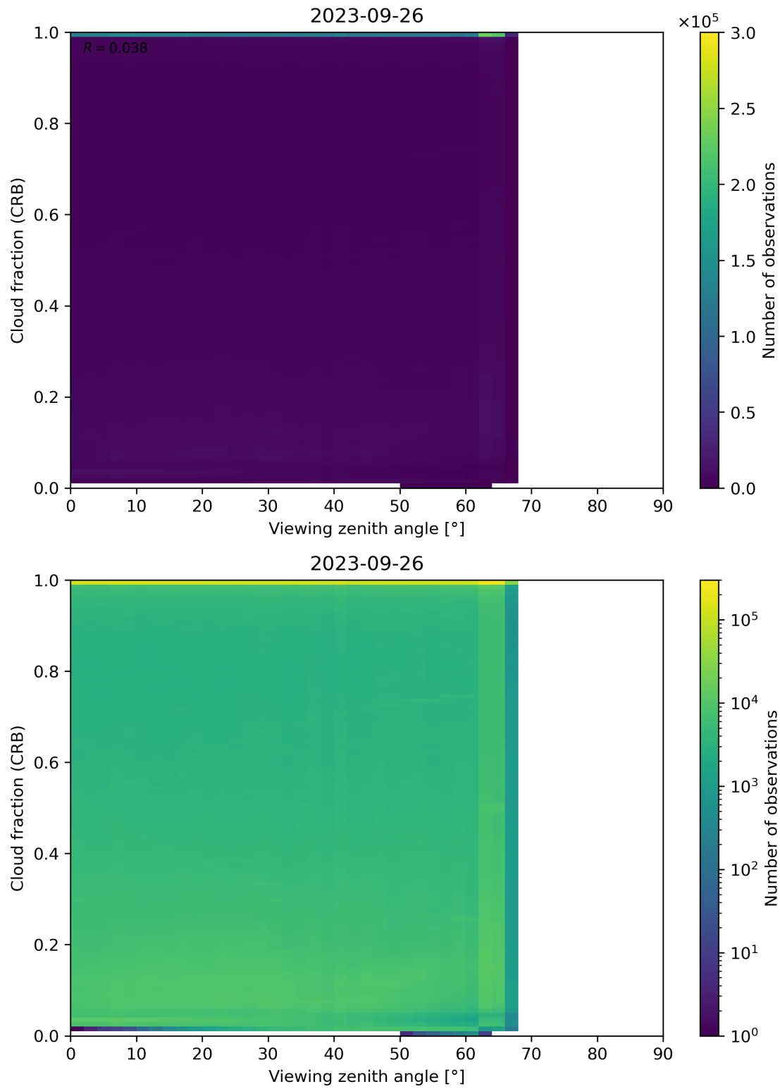
Figure 109: Scatter density plot of “Viewing zenith angle” against “Cloud fraction (CRB)” for 2023-09-26 to 2023-09-27.
