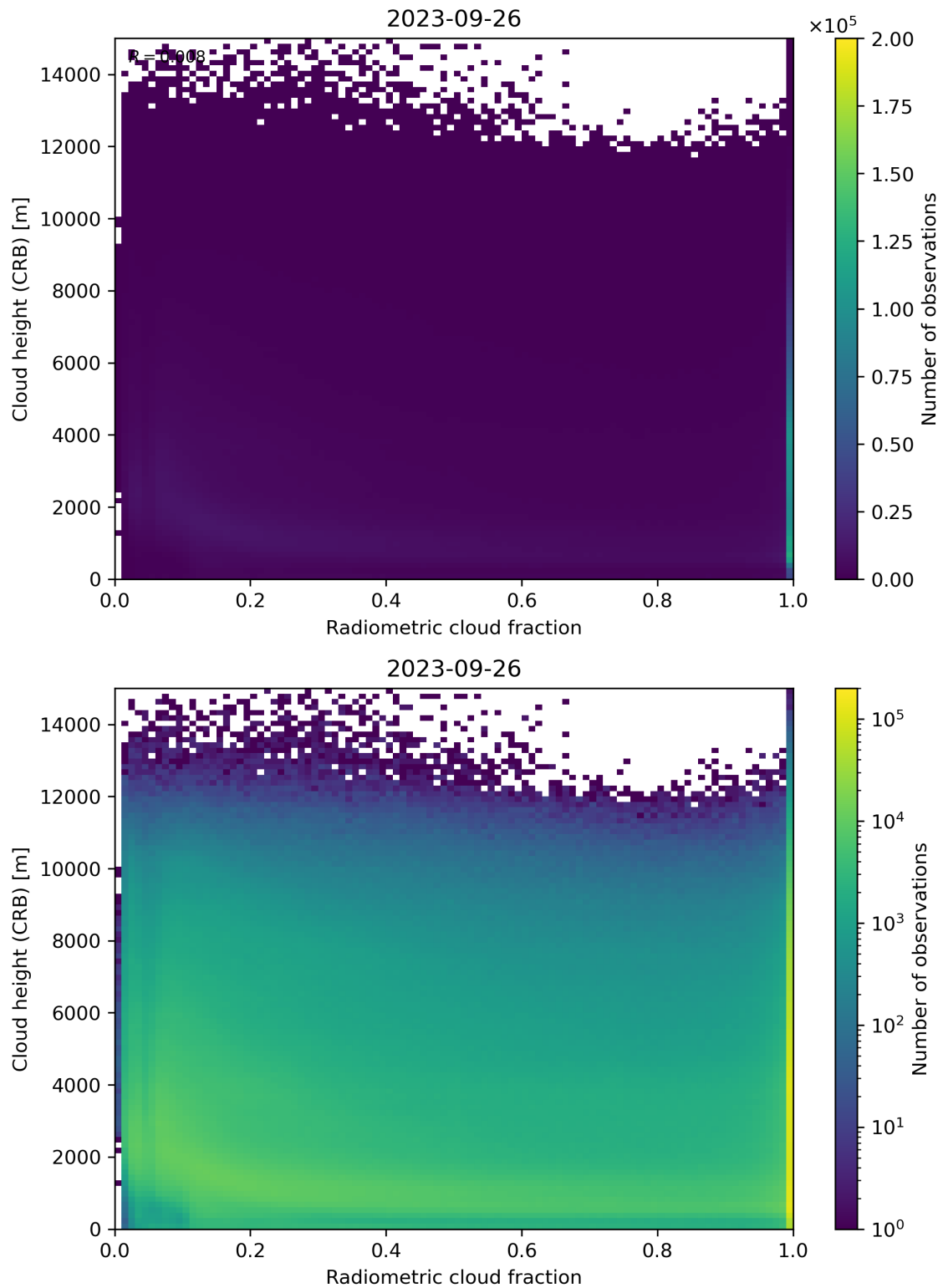
Figure 74: Scatter density plot of “Radiometric cloud fraction” against “Cloud height (CRB)” for 2023-09-26 to 2023-09-27.
