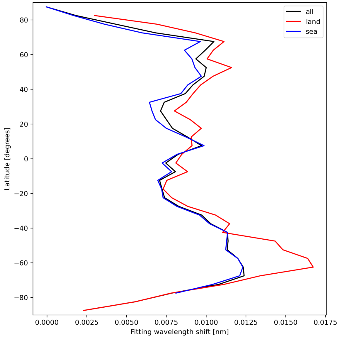
Figure 33: Zonal average of “Fitting wavelength shift” for 2023-09-26 to 2023-09-27.
