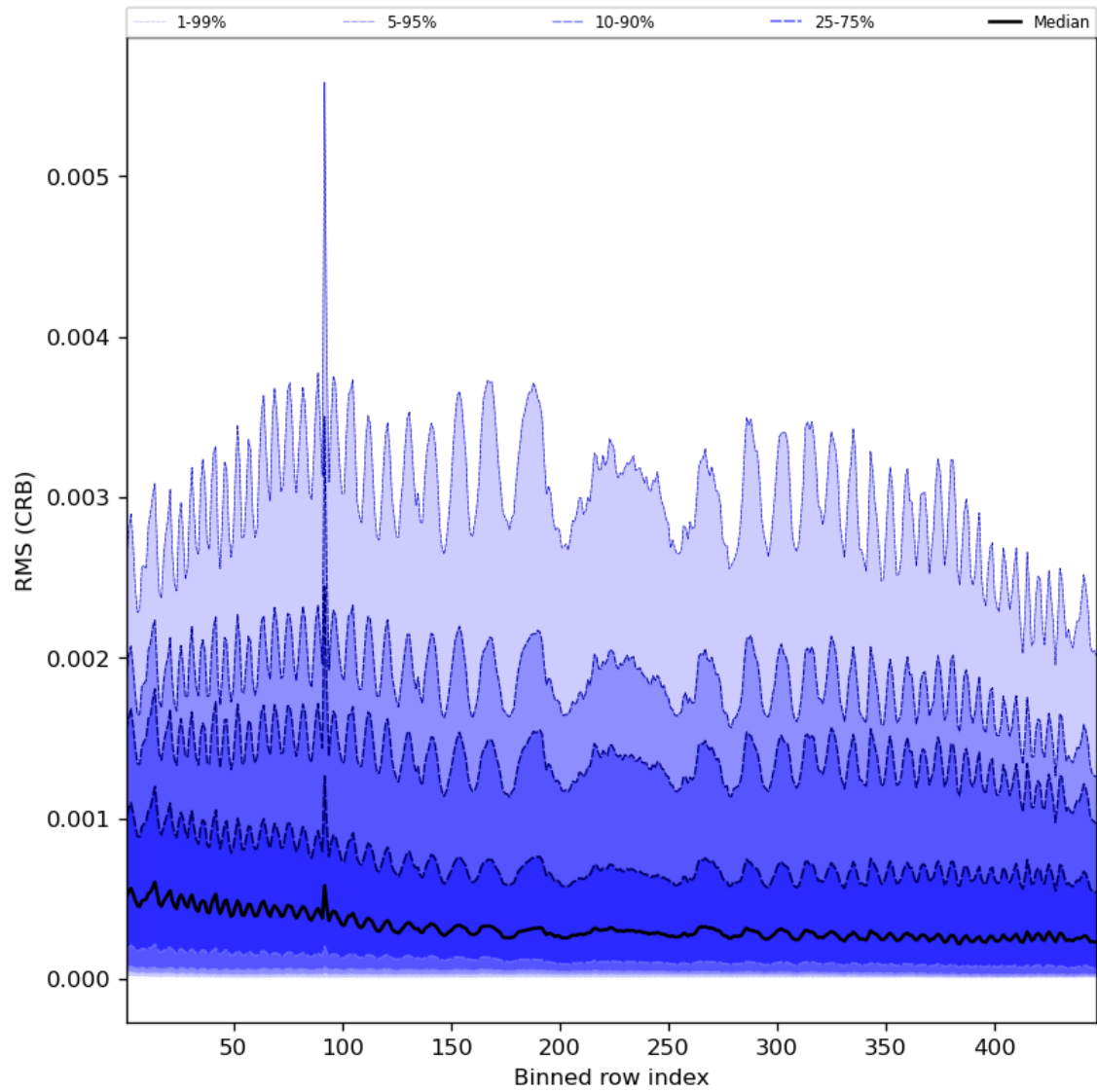
Figure 64: Along track statistics of “RMS (CRB)” for 2023-09-26 to 2023-09-27
