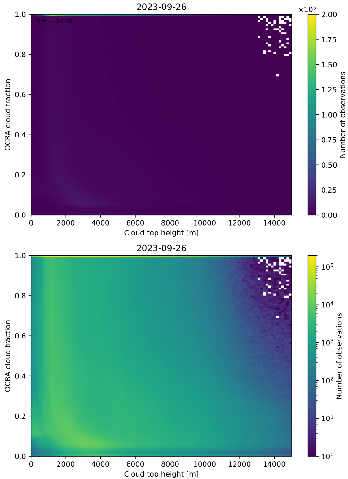
Figure 87: Scatter density plot of “Cloud top height” against “OCRA cloud fraction” for 2023-09-26 to 2023-09-27.
