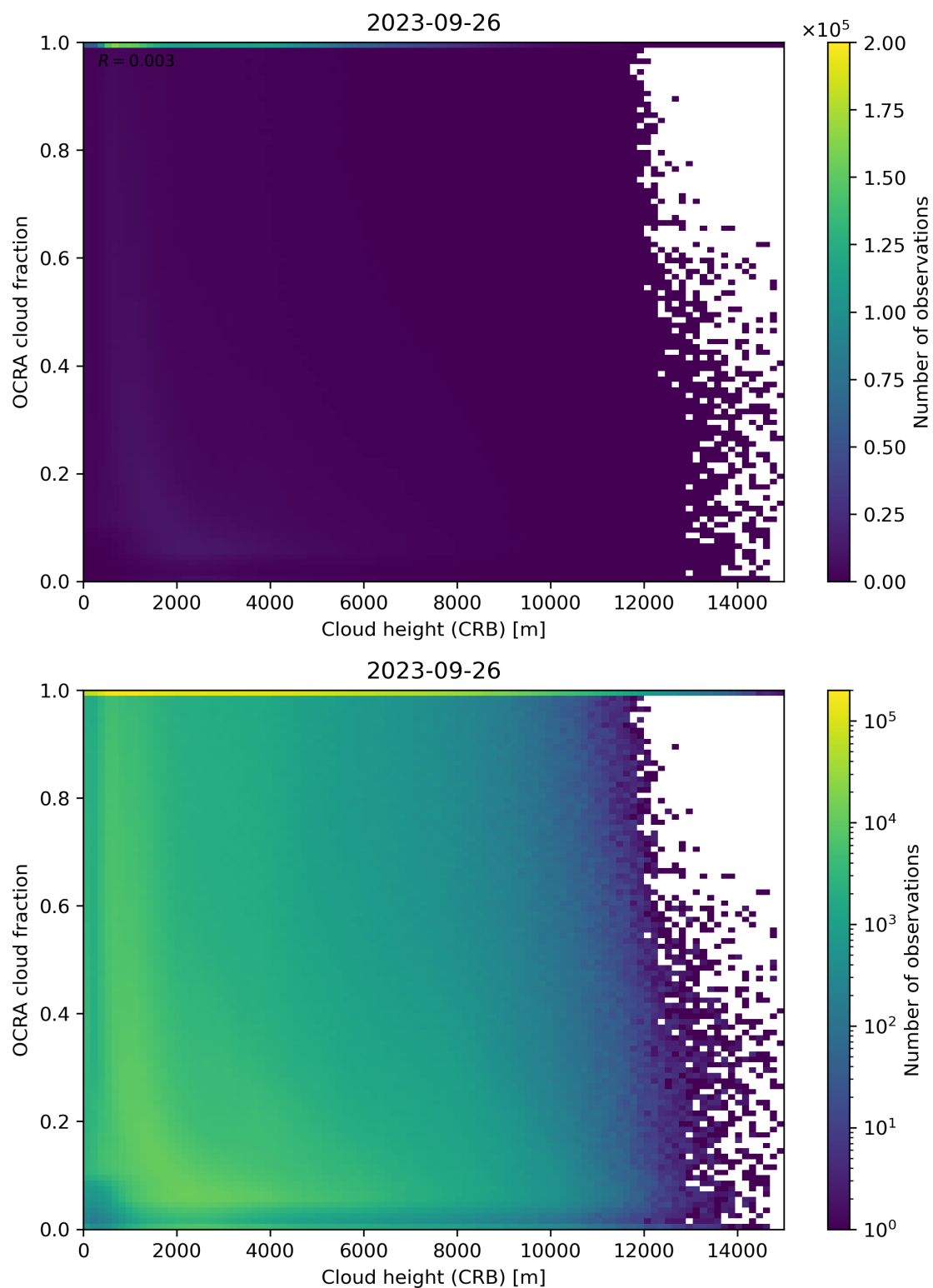
Figure 81: Scatter density plot of “Cloud height (CRB)” against “OCRA cloud fraction” for 2023-09-26 to 2023-09-27.
