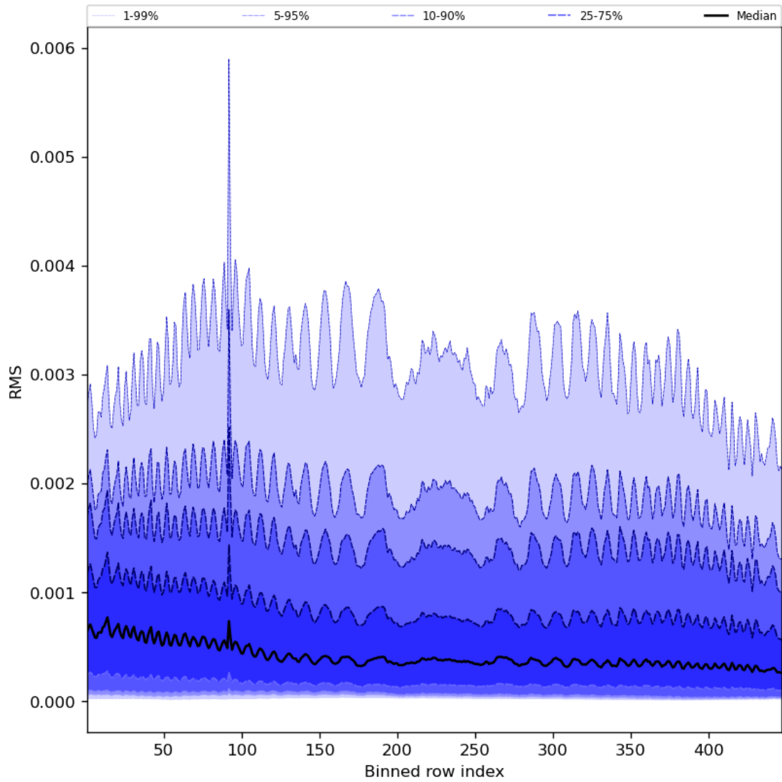
Figure 63: Along track statistics of “RMS” for 2023-09-26 to 2023-09-27
