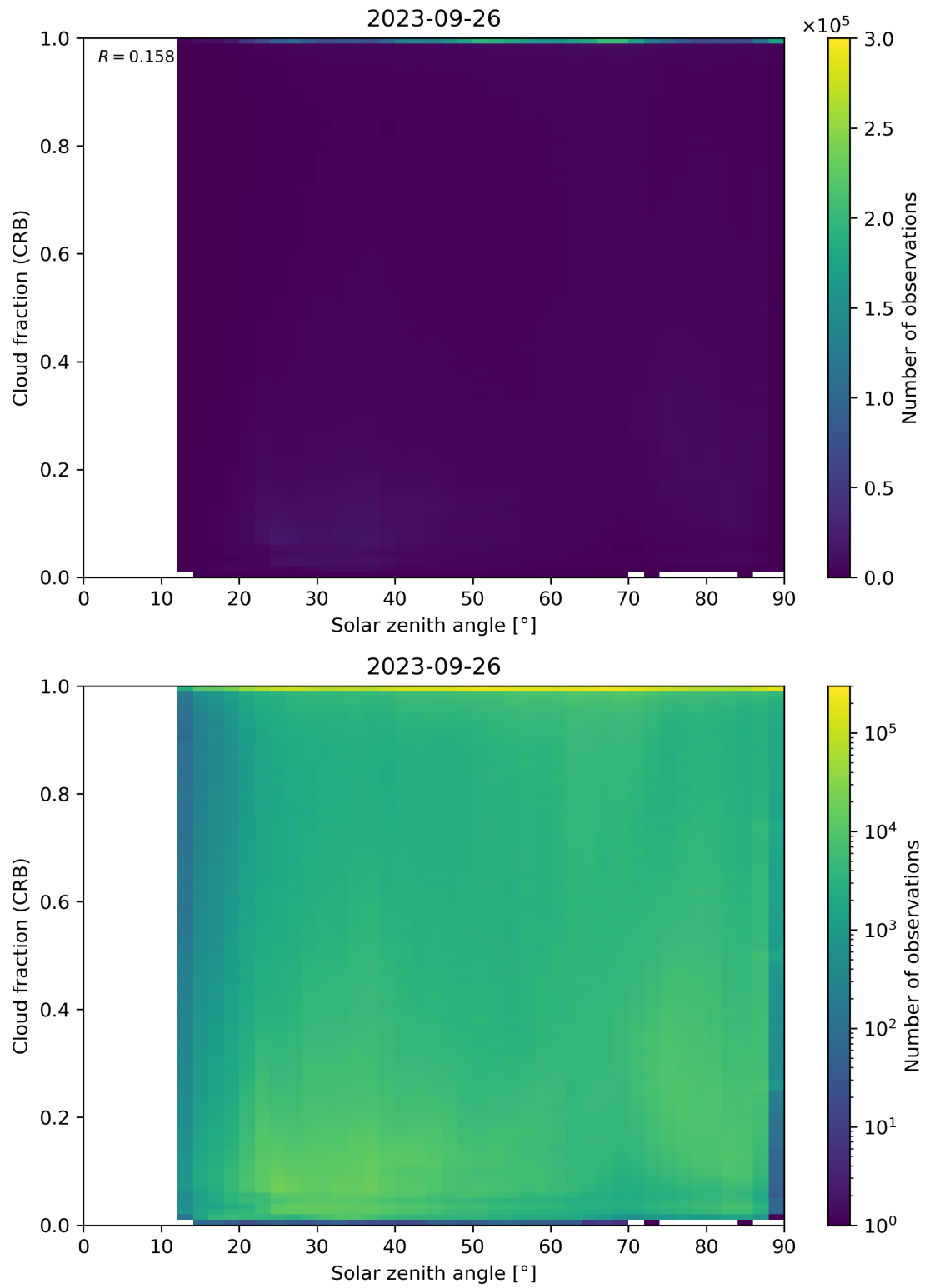
Figure 101: Scatter density plot of “Solar zenith angle” against “Cloud fraction (CRB)” for 2023-09-26 to 2023-09-27.
