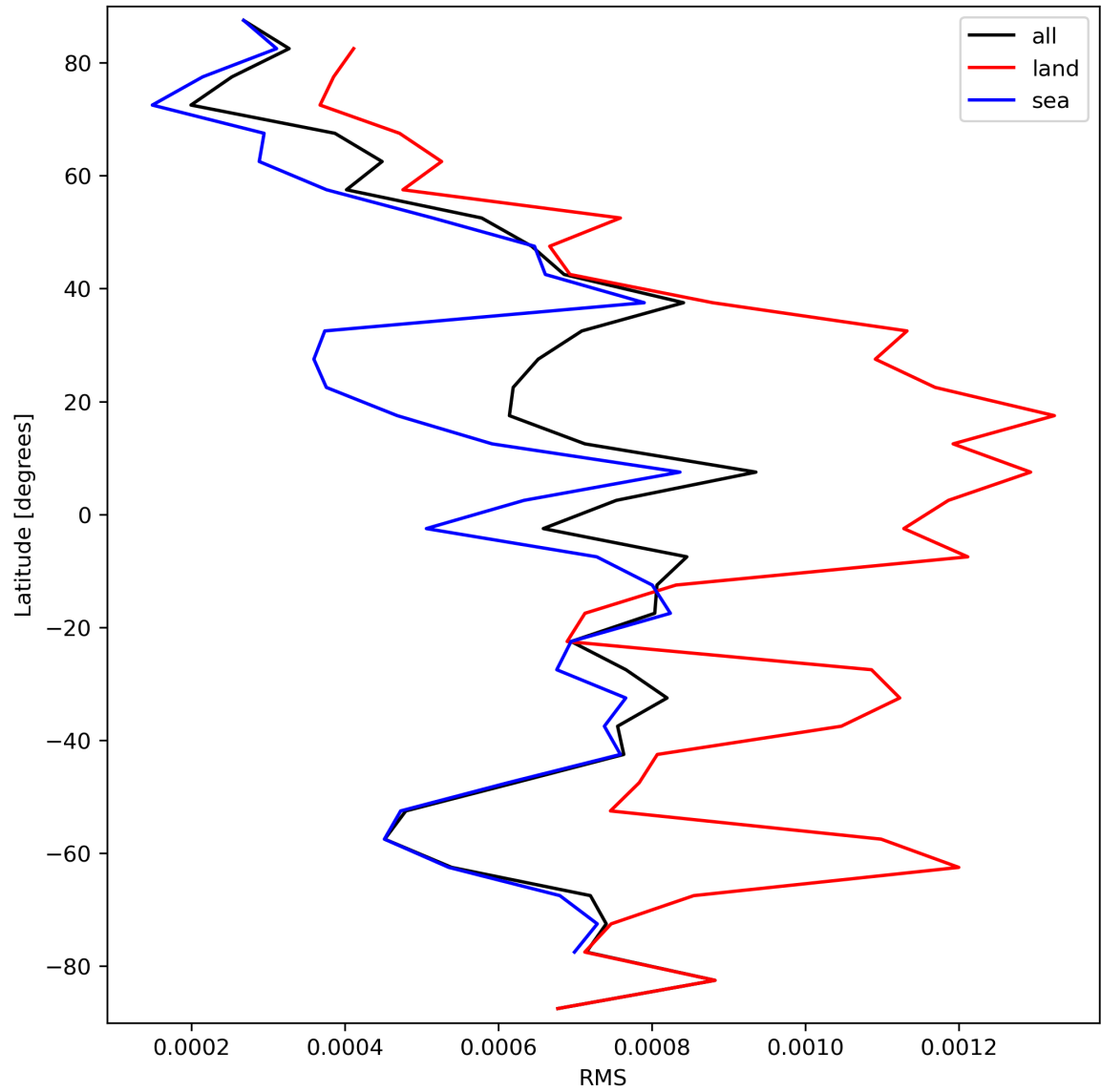
Figure 31: Zonal average of “RMS” for 2023-09-26 to 2023-09-27.
