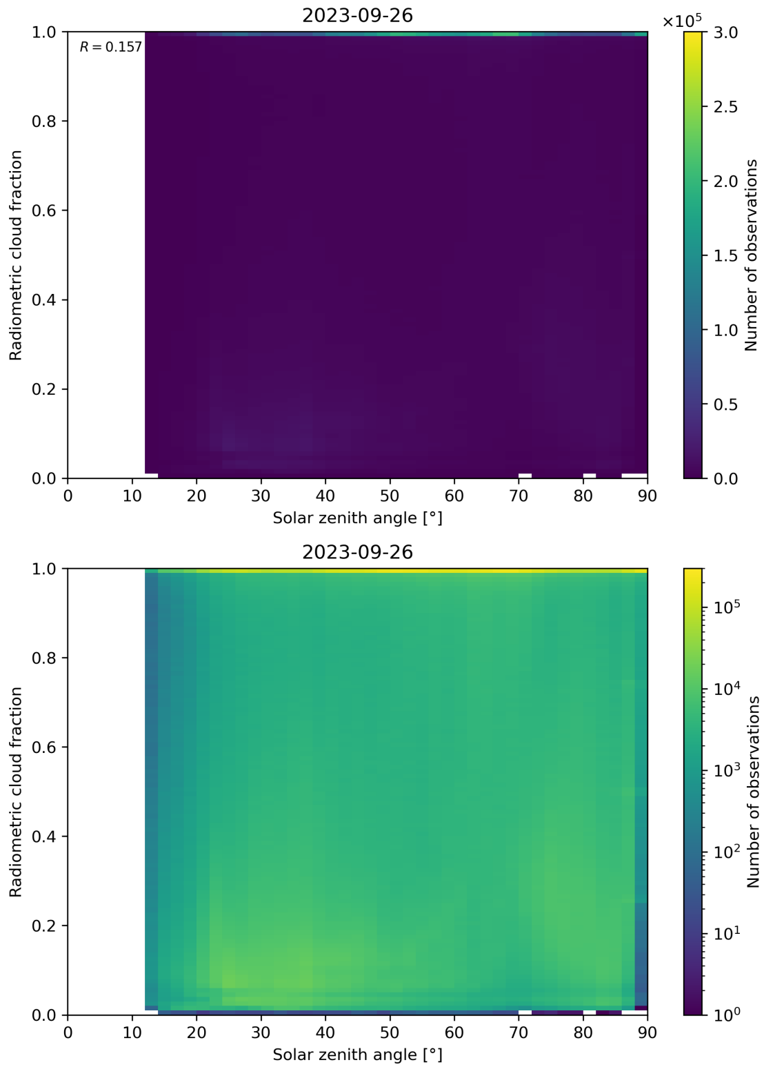
Figure 99: Scatter density plot of “Solar zenith angle” against “Radiometric cloud fraction” for 2023-09-26 to 2023-09-27.
