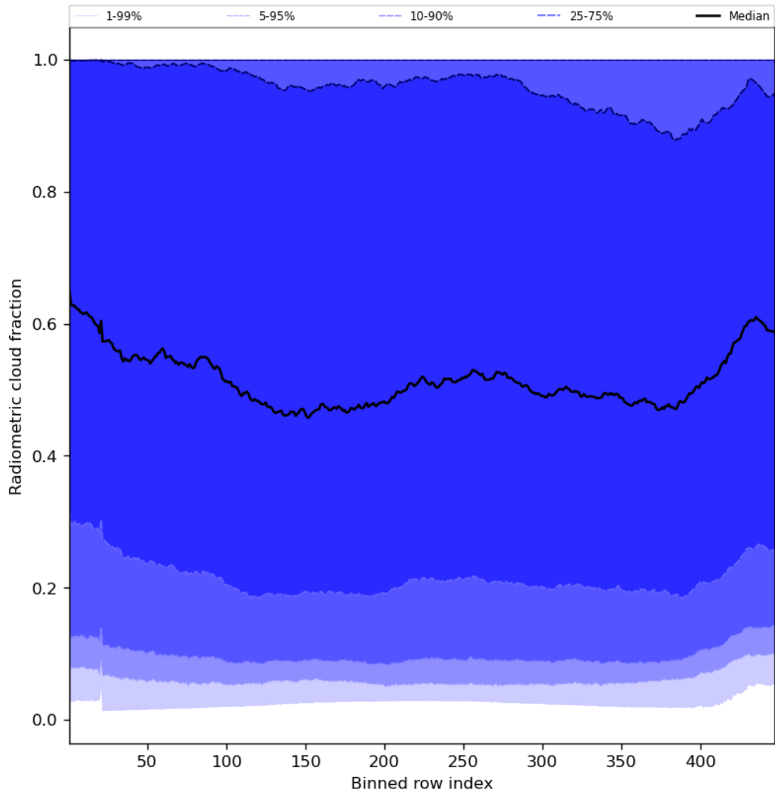
Figure 55: Along track statistics of “Radiometric cloud fraction” for 2023-09-26 to 2023-09-27
