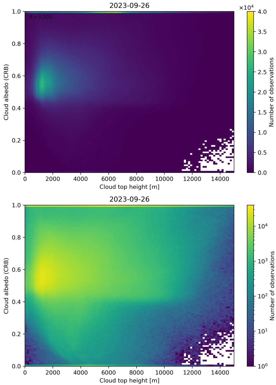
Figure 86: Scatter density plot of “Cloud top height” against “Cloud albedo (CRB)” for 2023-09-26 to 2023-09-27.
