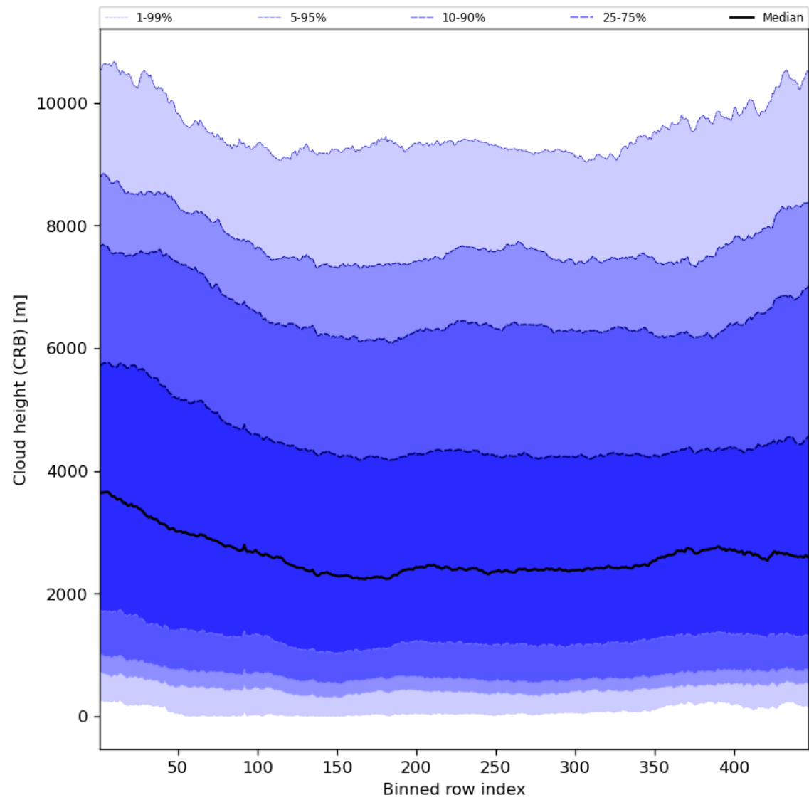
Figure 59: Along track statistics of “Cloud height (CRB)” for 2023-09-26 to 2023-09-27
