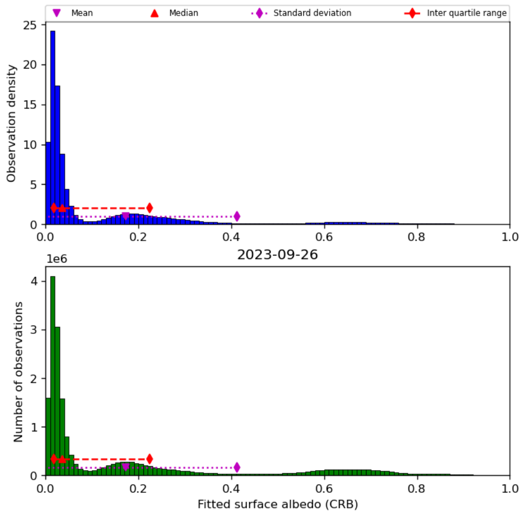
Figure 46: Histogram of “Fitted surface albedo (CRB)” for 2023-09-26 to 2023-09-27
