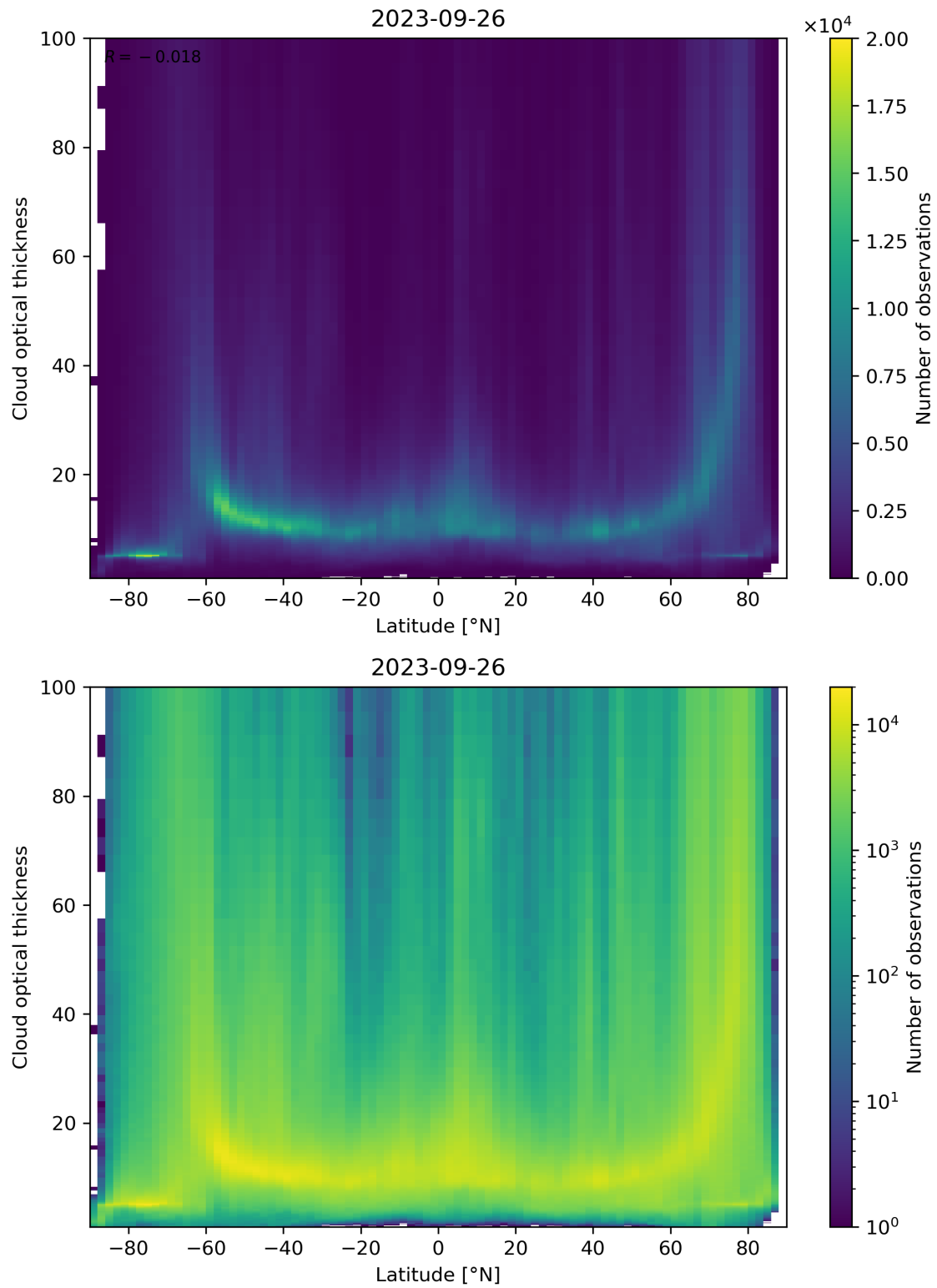
Figure 96: Scatter density plot of “Latitude” against “Cloud optical thickness” for 2023-09-26 to 2023-09-27.
