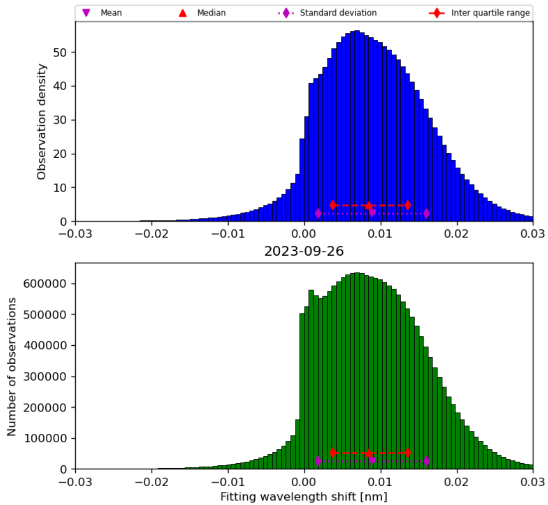
Figure 49: Histogram of “Fitting wavelength shift” for 2023-09-26 to 2023-09-27
