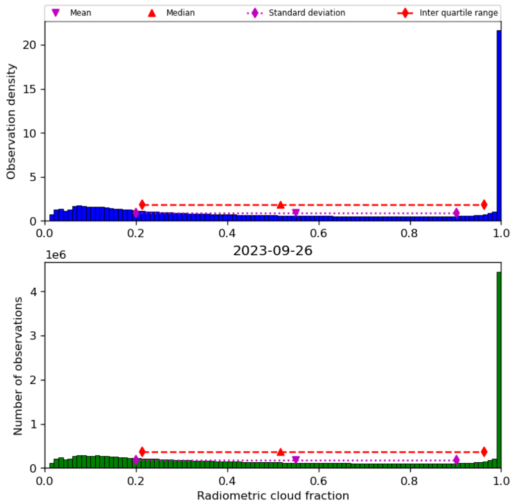
Figure 39: Histogram of “Radiometric cloud fraction” for 2023-09-26 to 2023-09-27
