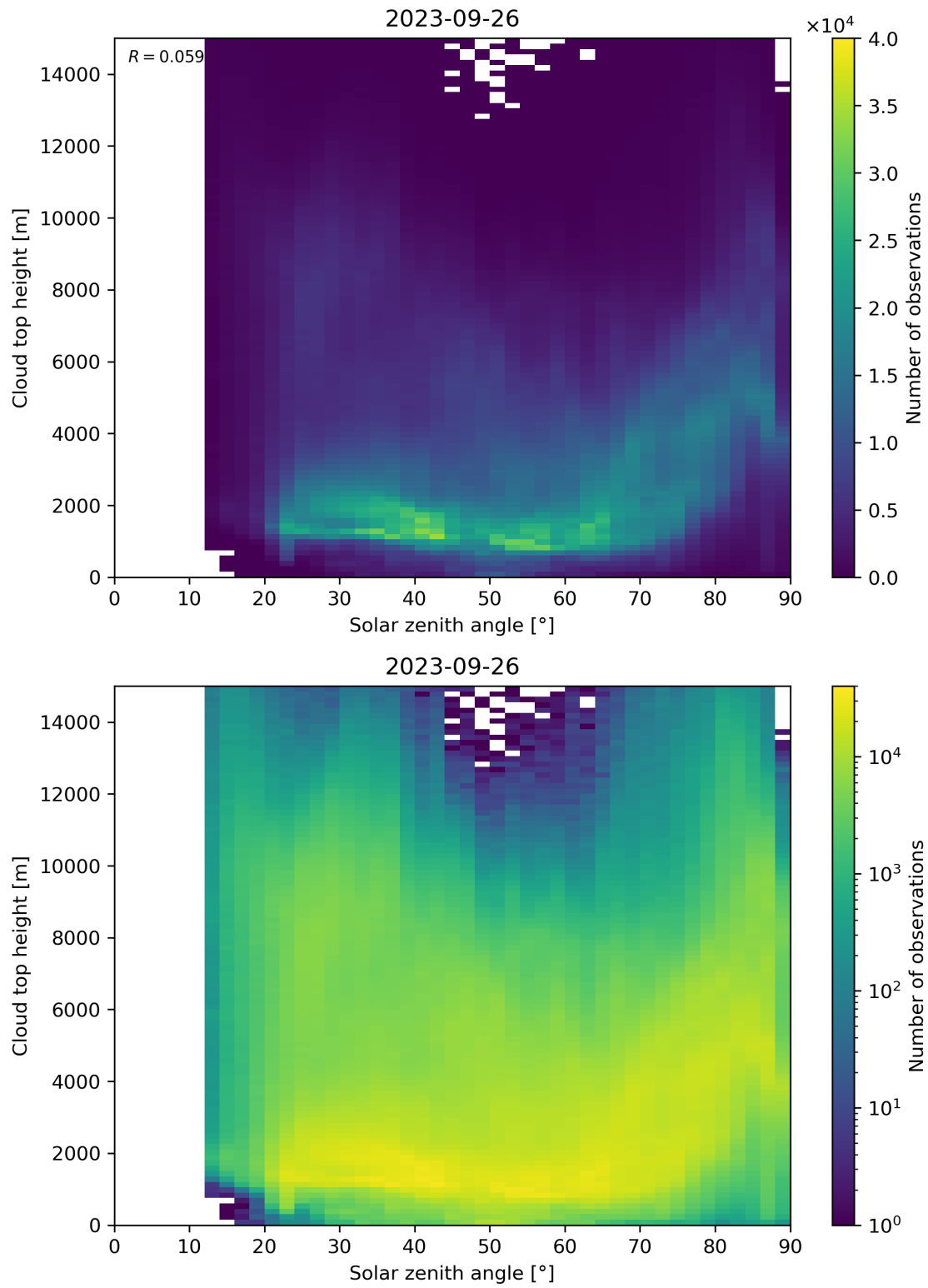
Figure 104: Scatter density plot of “Solar zenith angle” against “Cloud top height” for 2023-09-26 to 2023-09-27.
