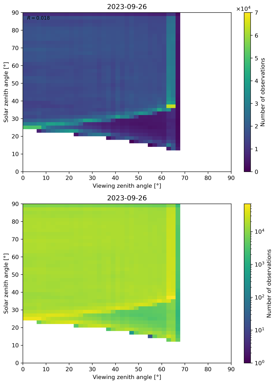
Figure 114: Scatter density plot of “Viewing zenith angle” against “Solar zenith angle” for 2023-09-26 to 2023-09-27.
