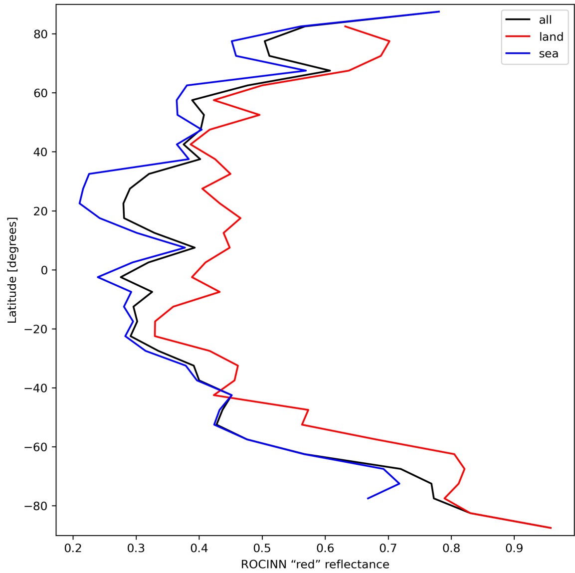
Figure 37: Zonal average of “ROCINN “red” reflectance” for 2023-09-26 to 2023-09-27.
