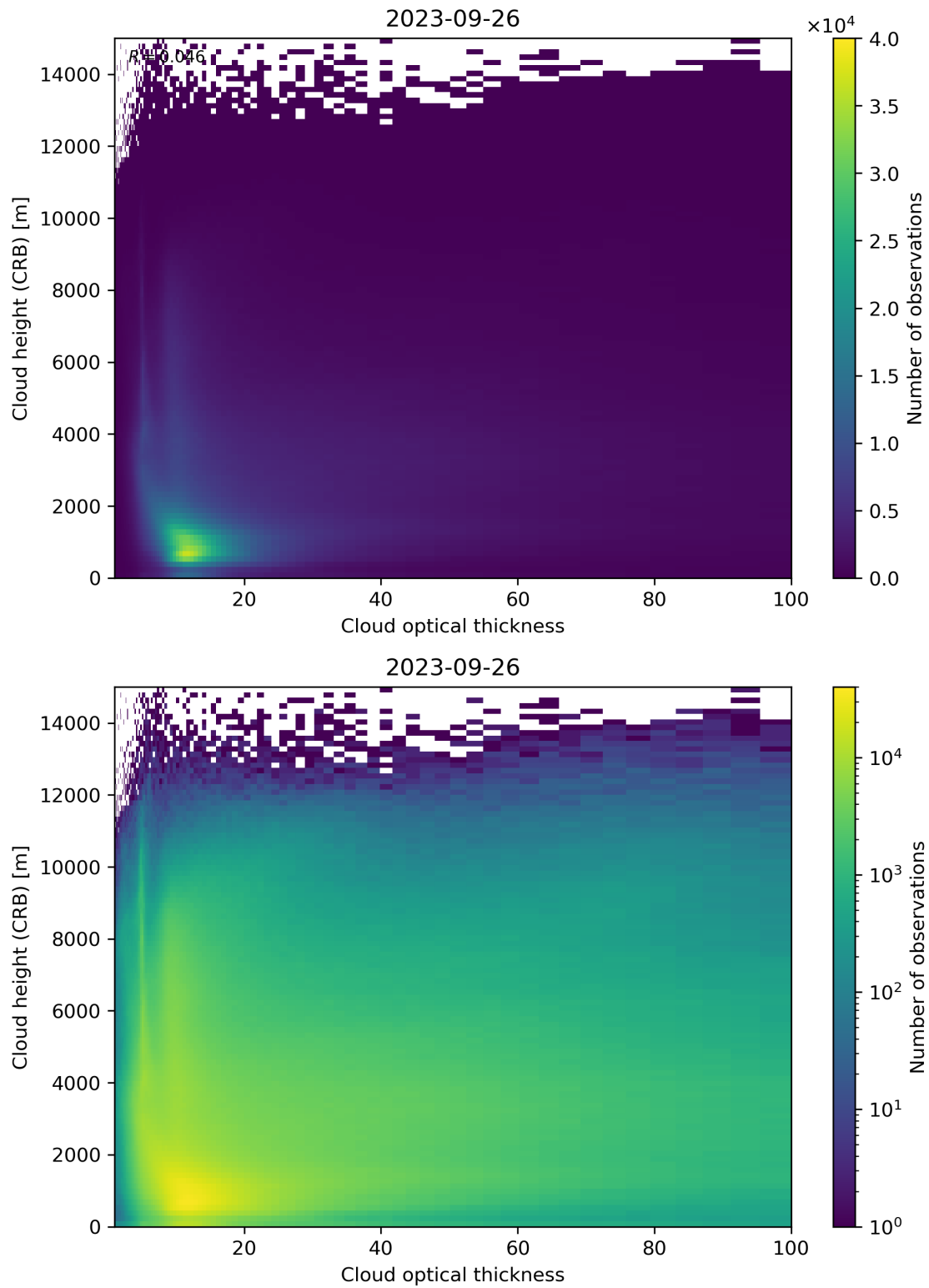
Figure 85: Scatter density plot of “Cloud optical thickness” against “Cloud height (CRB)” for 2023-09-26 to 2023-09-27.
