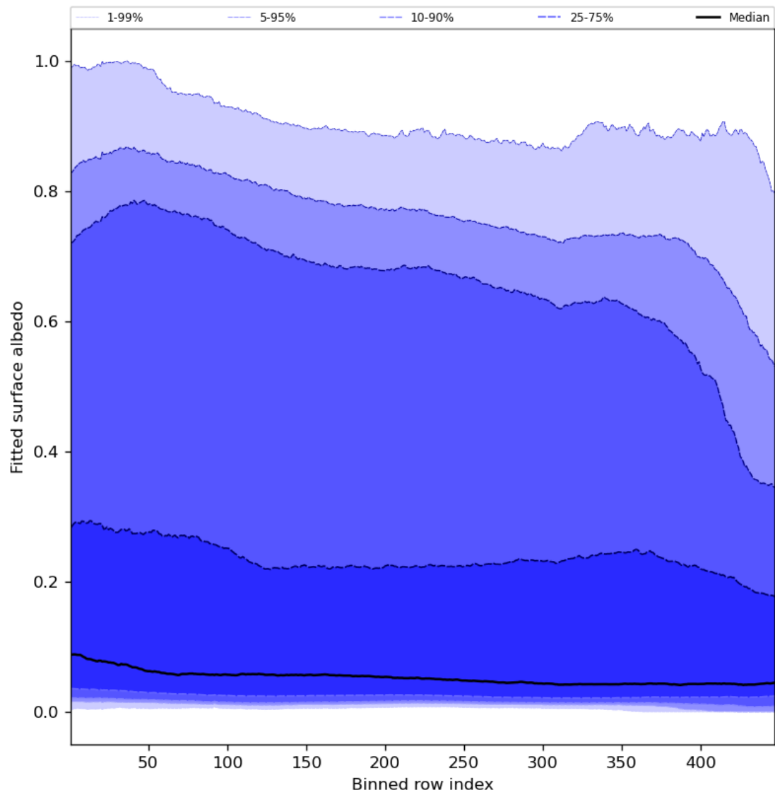
Figure 61: Along track statistics of “Fitted surface albedo” for 2023-09-26 to 2023-09-27
