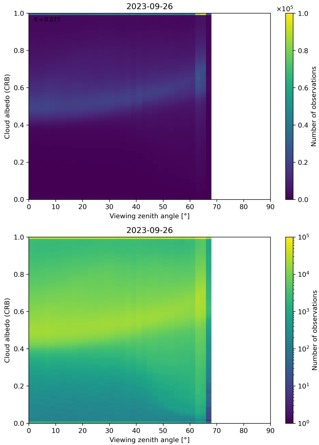
Figure 106: Scatter density plot of “Viewing zenith angle” against “Cloud albedo (CRB)” for 2023-09-26 to 2023-09-27.
