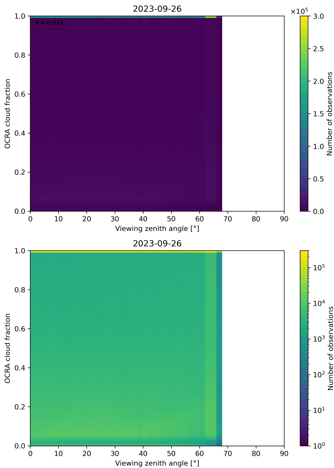
Figure 108: Scatter density plot of “Viewing zenith angle” against “OCRA cloud fraction” for 2023-09-26 to 2023-09-27.
