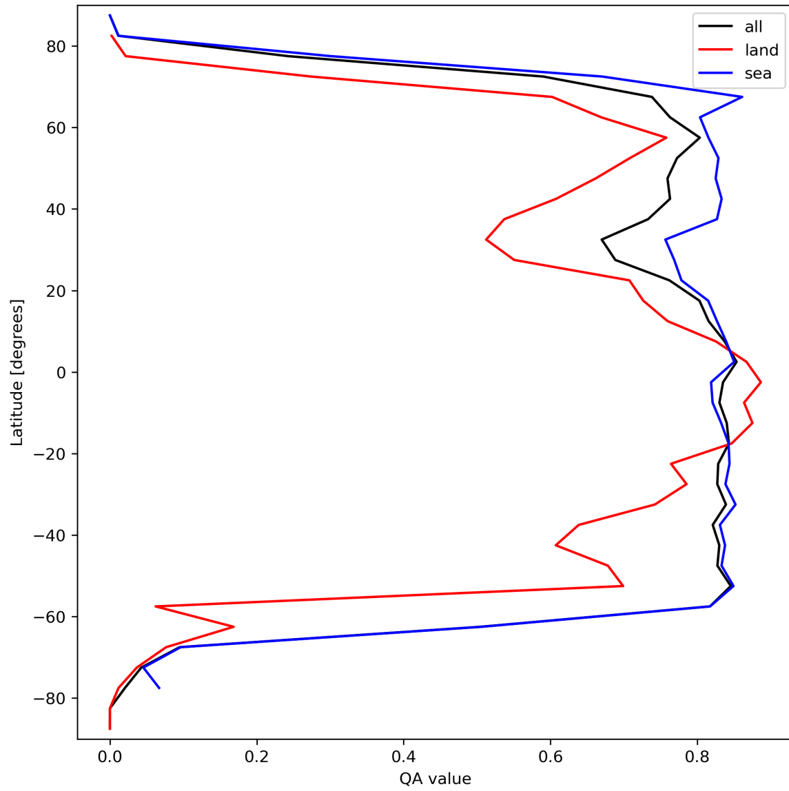
Figure 22: Zonal average of “QA value” for 2023-09-26 to 2023-09-27.
