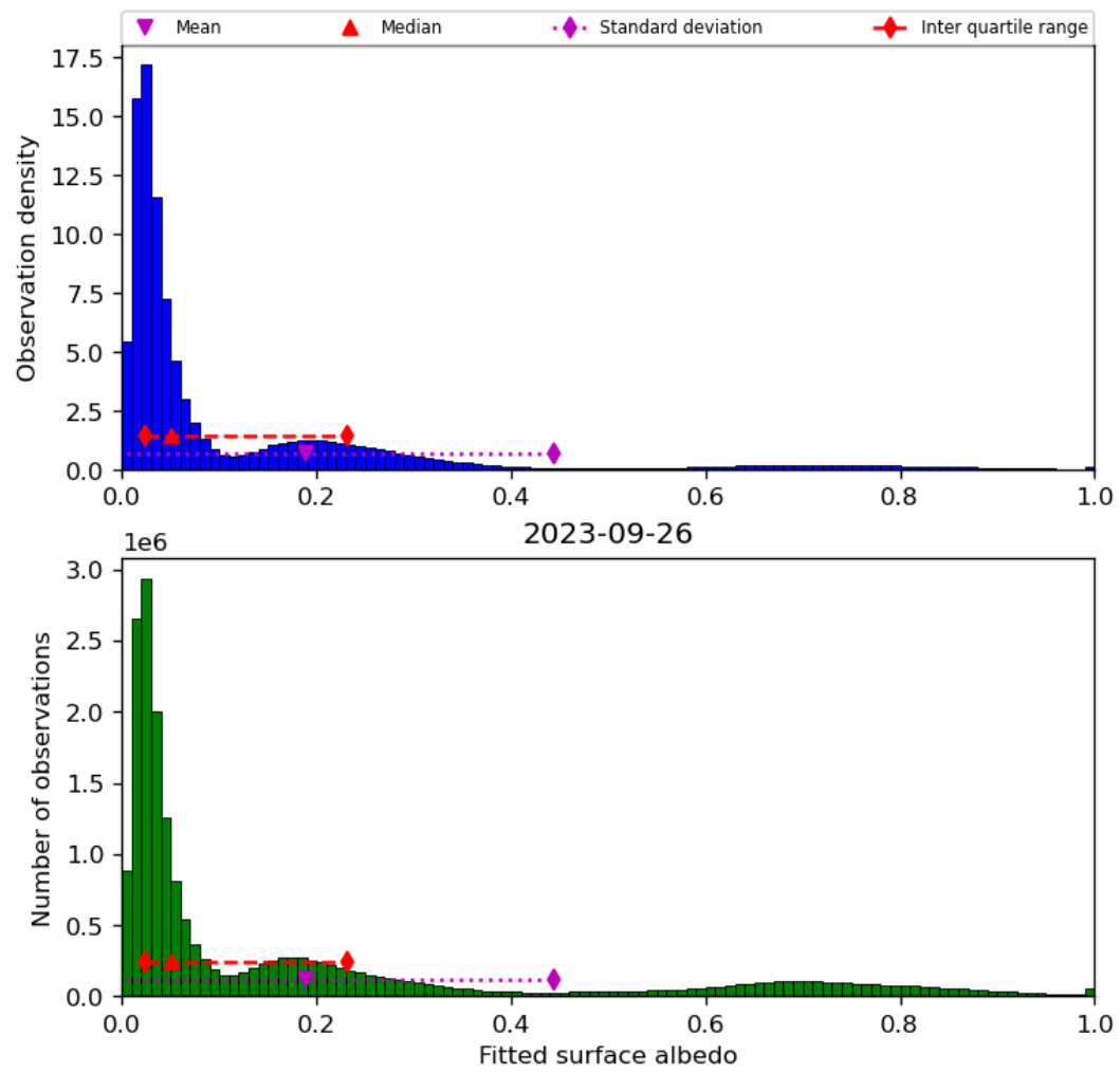
Figure 45: Histogram of “Fitted surface albedo” for 2023-09-26 to 2023-09-27
