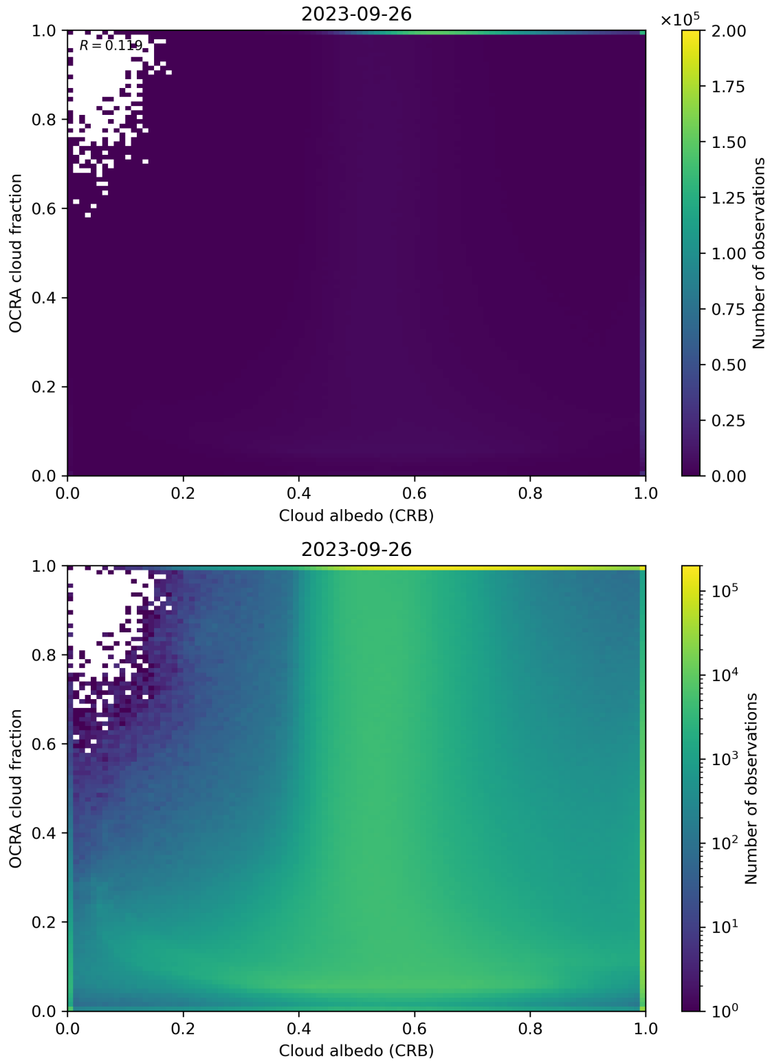
Figure 70: Scatter density plot of “Cloud albedo (CRB)” against “OCRA cloud fraction” for 2023-09-26 to 2023-09-27.
