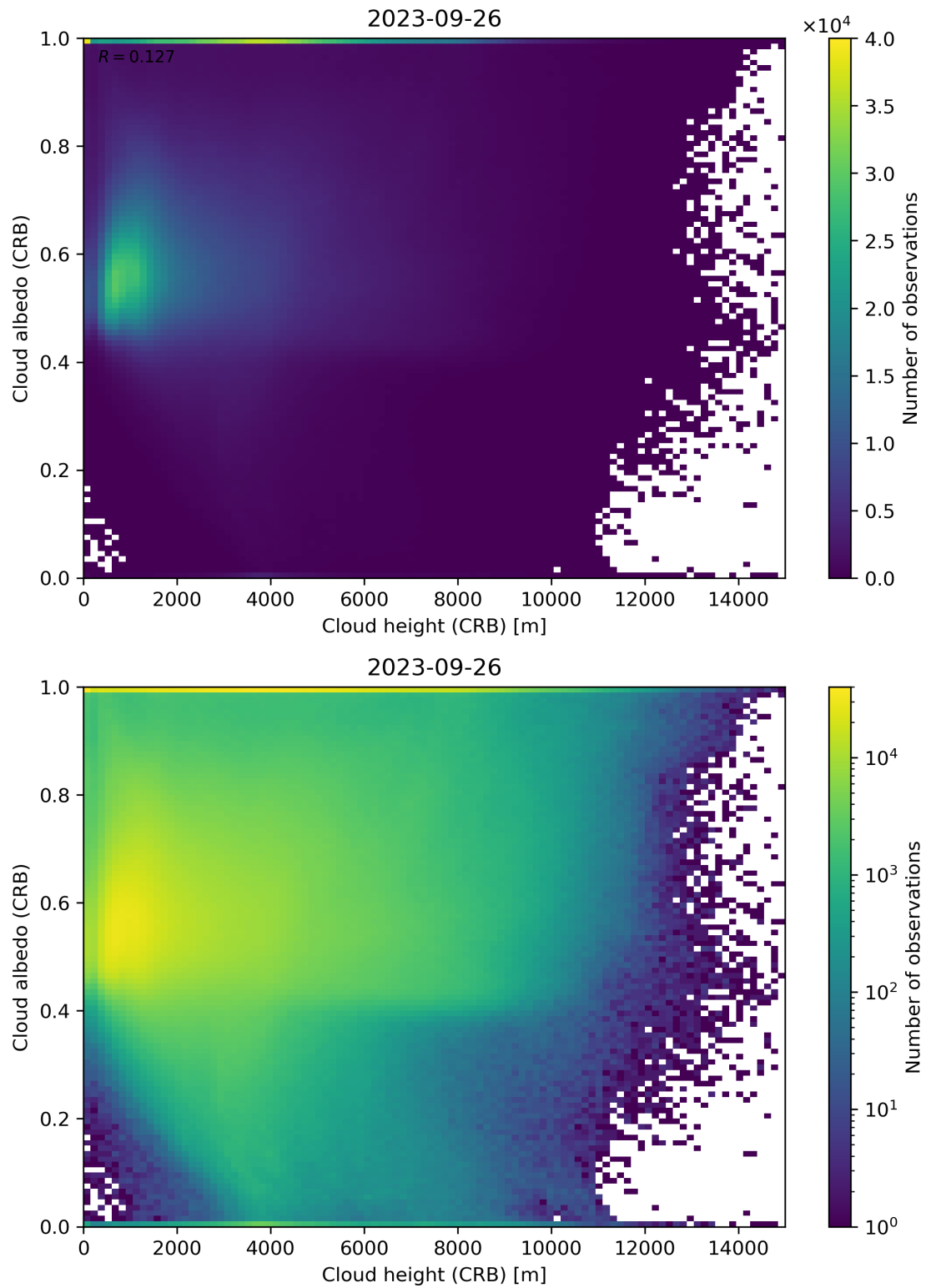
Figure 80: Scatter density plot of “Cloud height (CRB)” against “Cloud albedo (CRB)” for 2023-09-26 to 2023-09-27.
