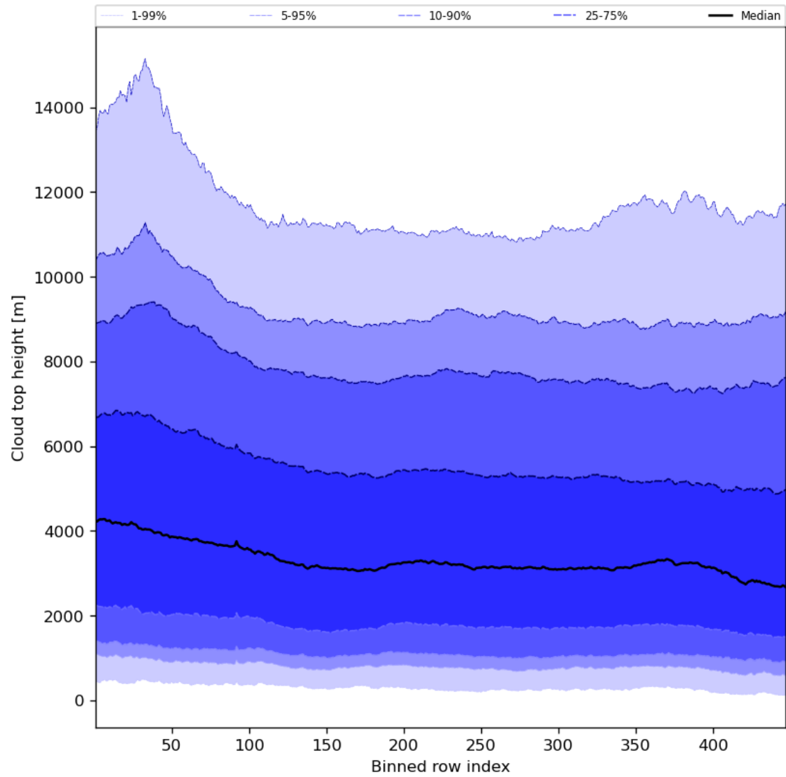
Figure 56: Along track statistics of “Cloud top height” for 2023-09-26 to 2023-09-27
