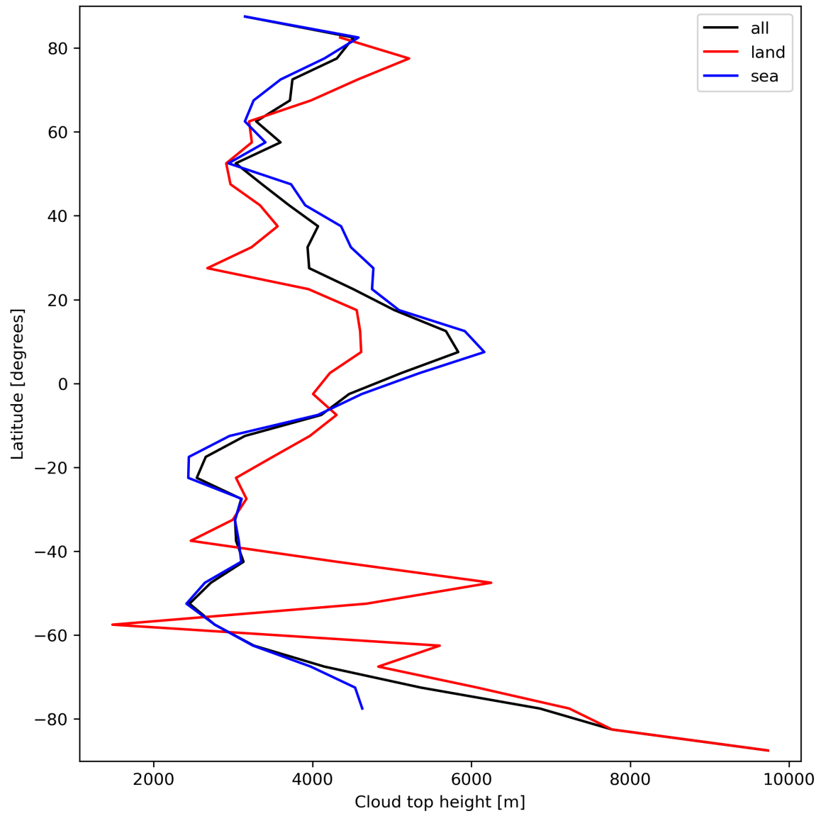
Figure 24: Zonal average of “Cloud top height” for 2023-09-26 to 2023-09-27.
