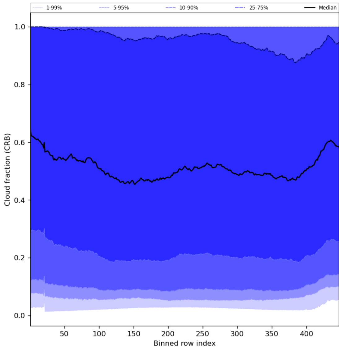
Figure 58: Along track statistics of “Cloud fraction (CRB)” for 2023-09-26 to 2023-09-27
