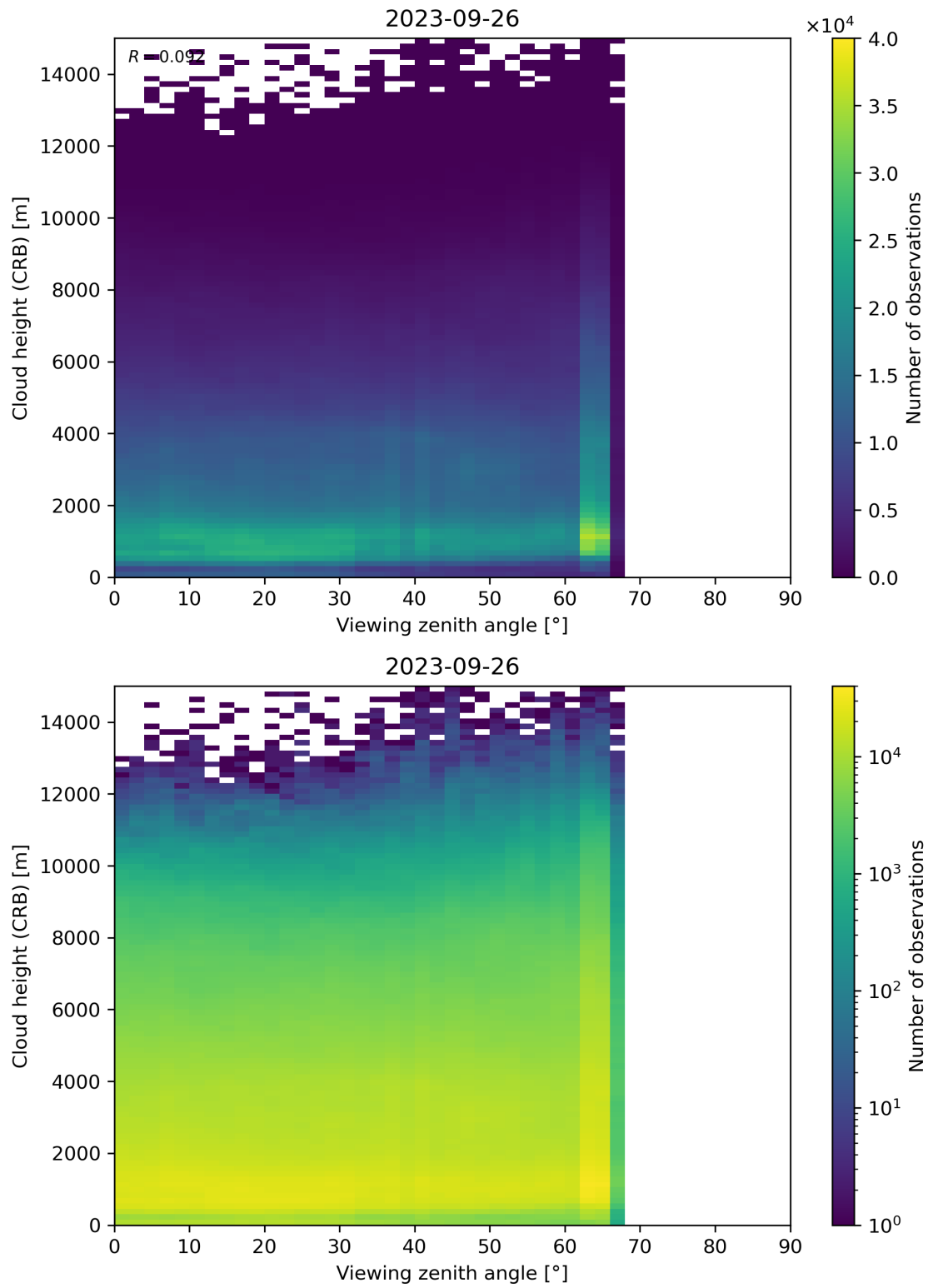
Figure 110: Scatter density plot of “Viewing zenith angle” against “Cloud height (CRB)” for 2023-09-26 to 2023-09-27.
