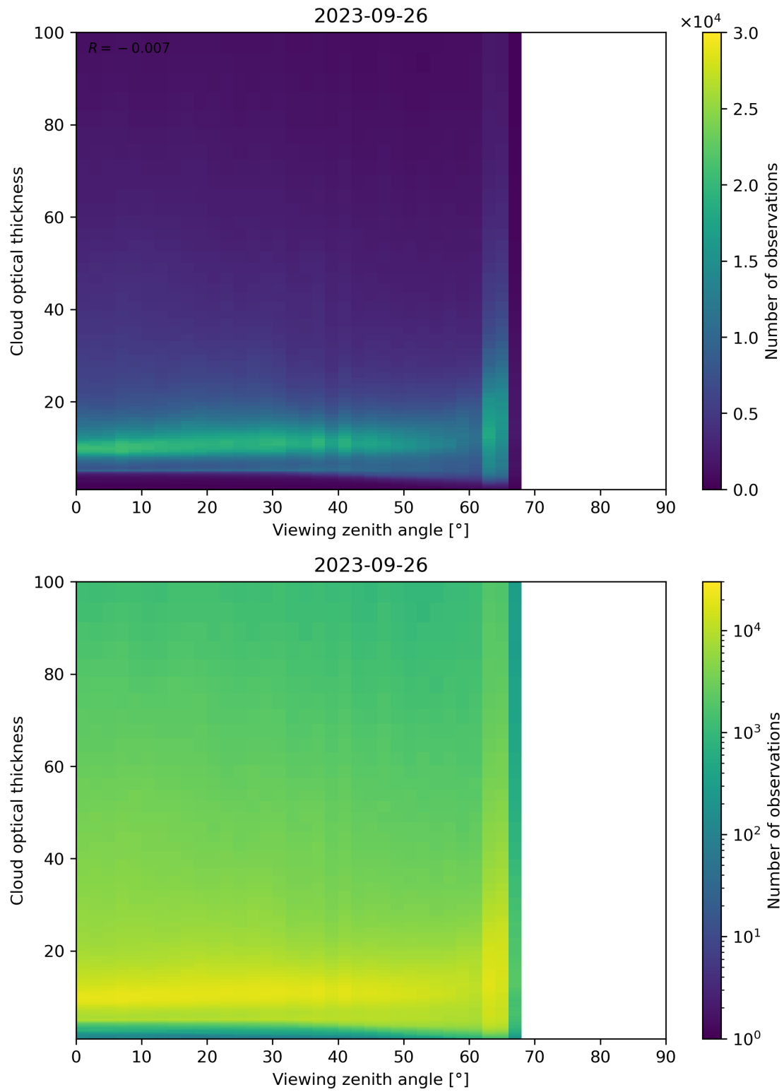
Figure 111: Scatter density plot of “Viewing zenith angle” against “Cloud optical thickness” for 2023-09-26 to 2023-09-27.
