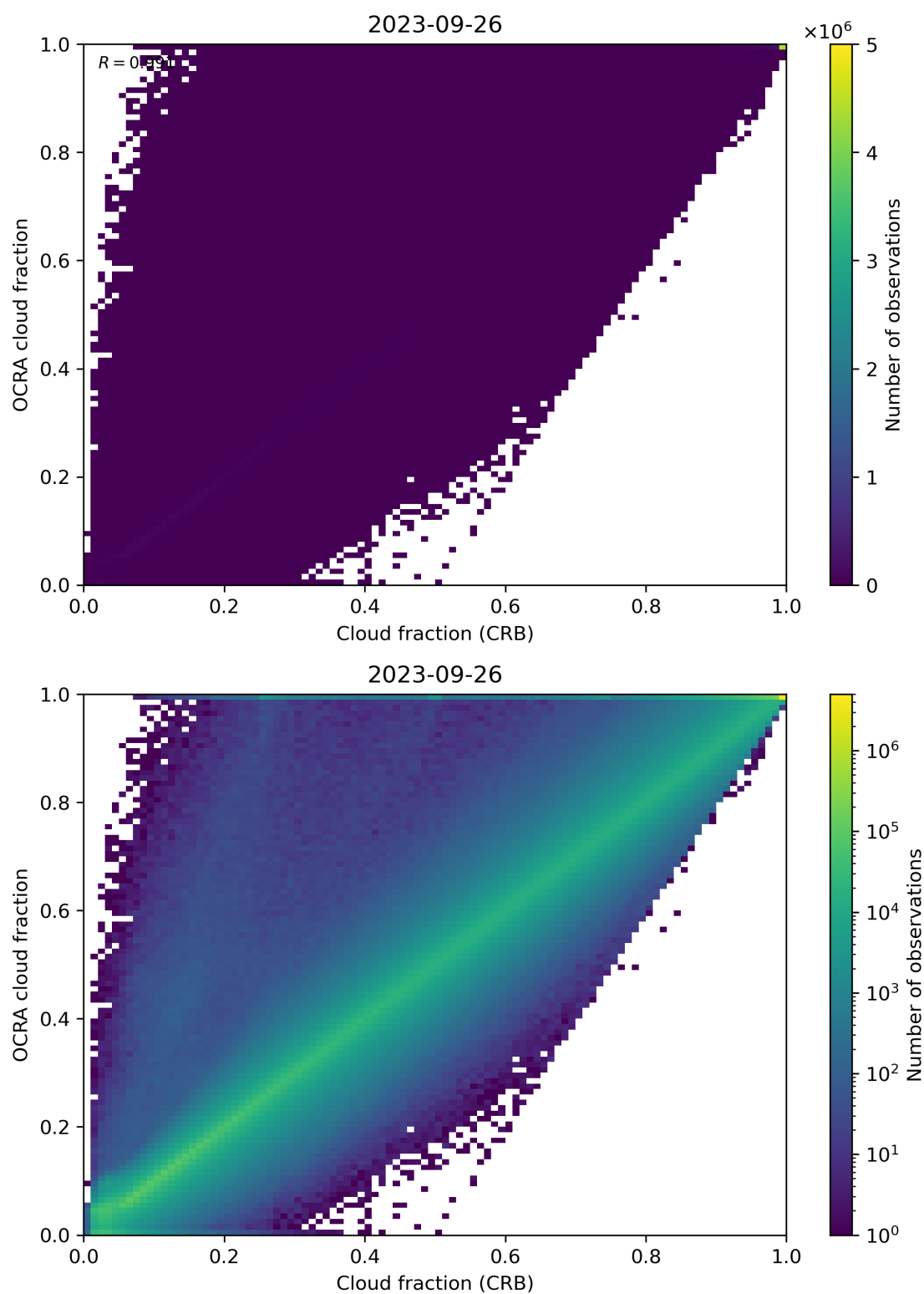
Figure 78: Scatter density plot of “Cloud fraction (CRB)” against “OCRA cloud fraction” for 2023-09-26 to 2023-09-27.
