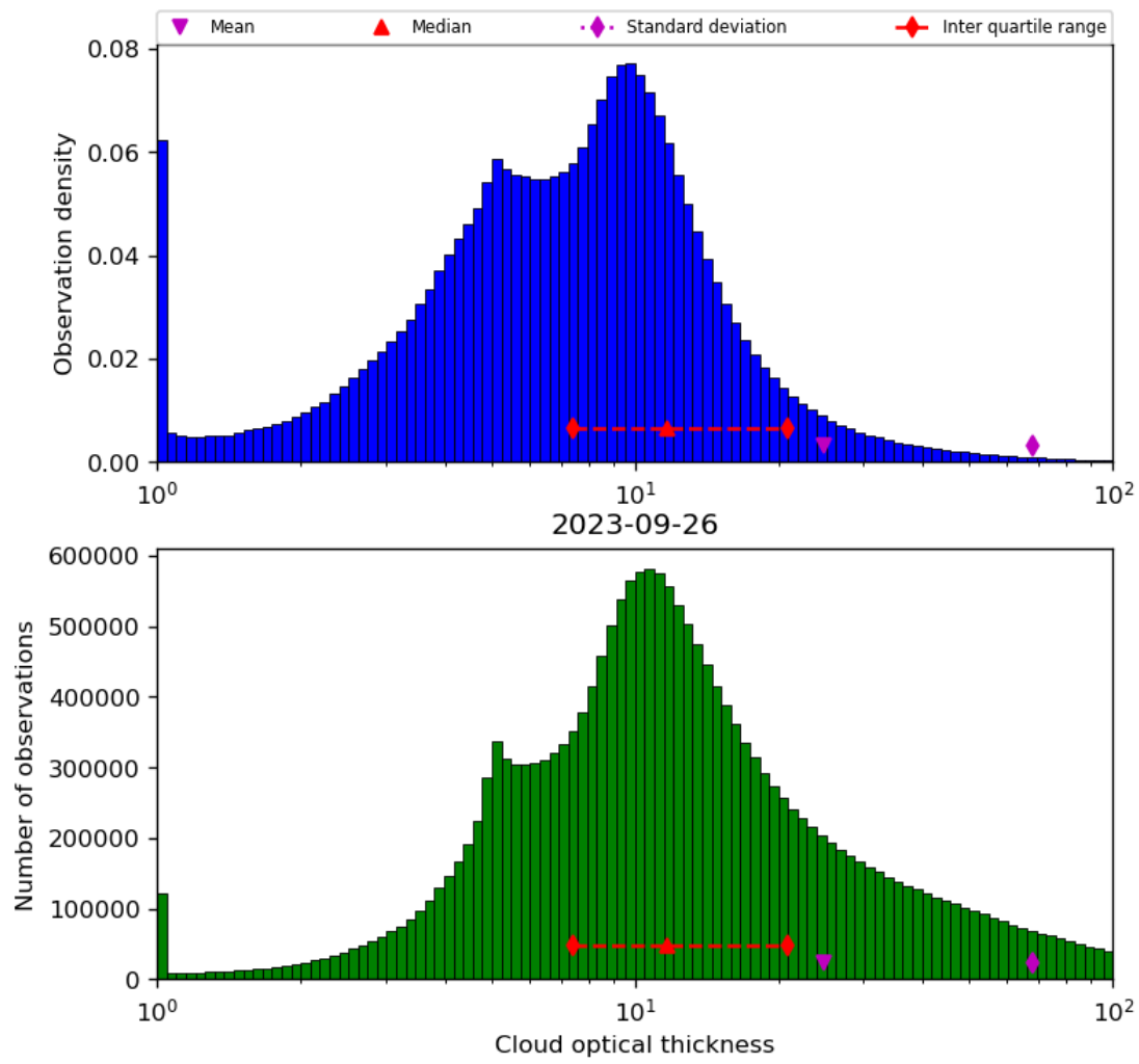
Figure 41: Histogram of “Cloud optical thickness” for 2023-09-26 to 2023-09-27
