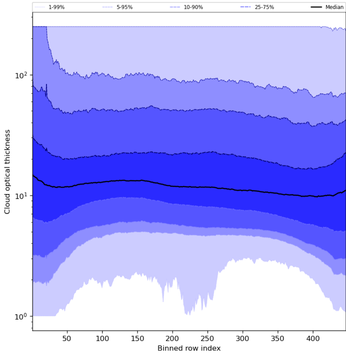
Figure 57: Along track statistics of “Cloud optical thickness” for 2023-09-26 to 2023-09-27
