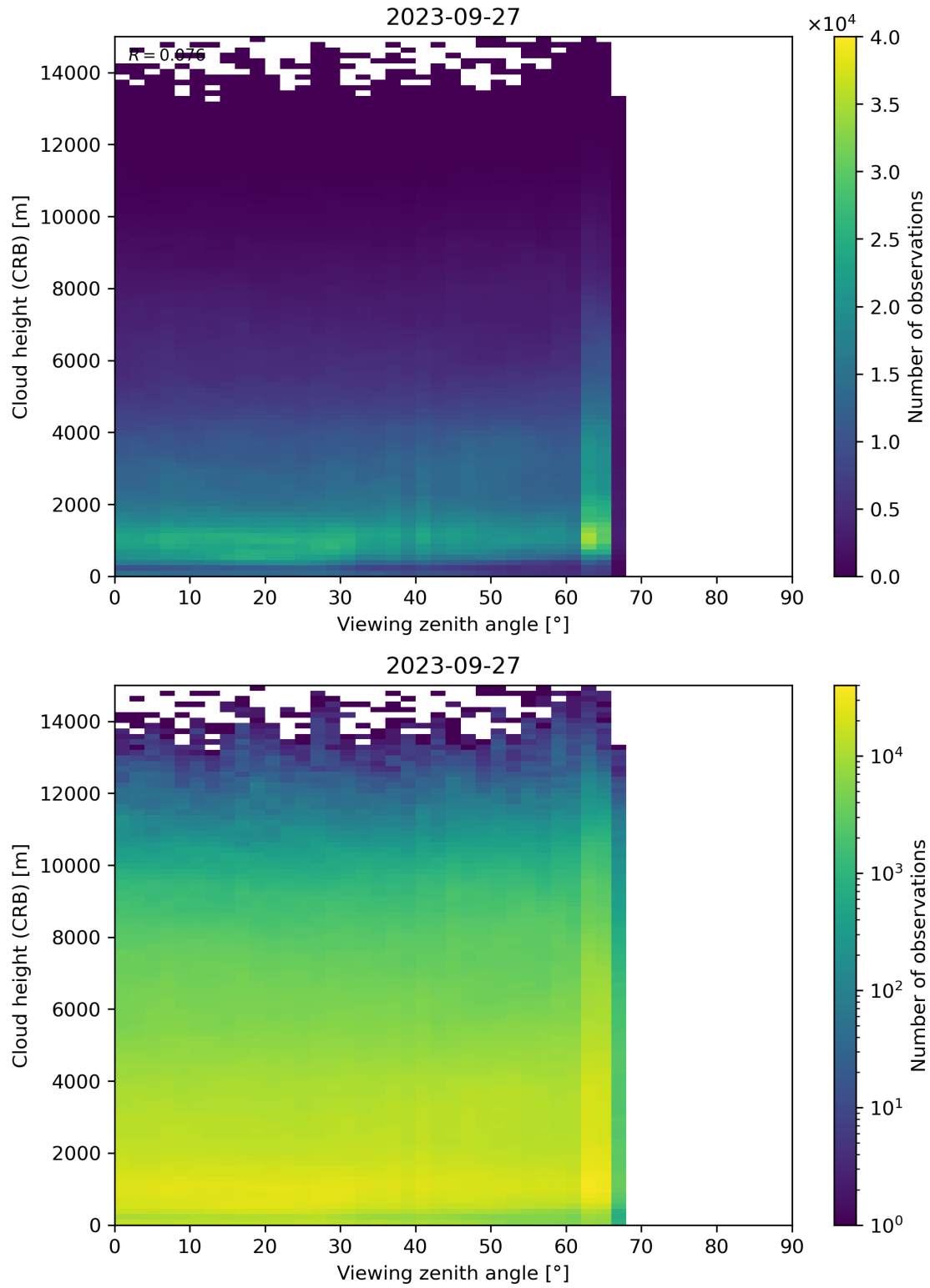
Figure 110: Scatter density plot of “Viewing zenith angle” against “Cloud height (CRB)” for 2023-09-26 to 2023-09-28.
