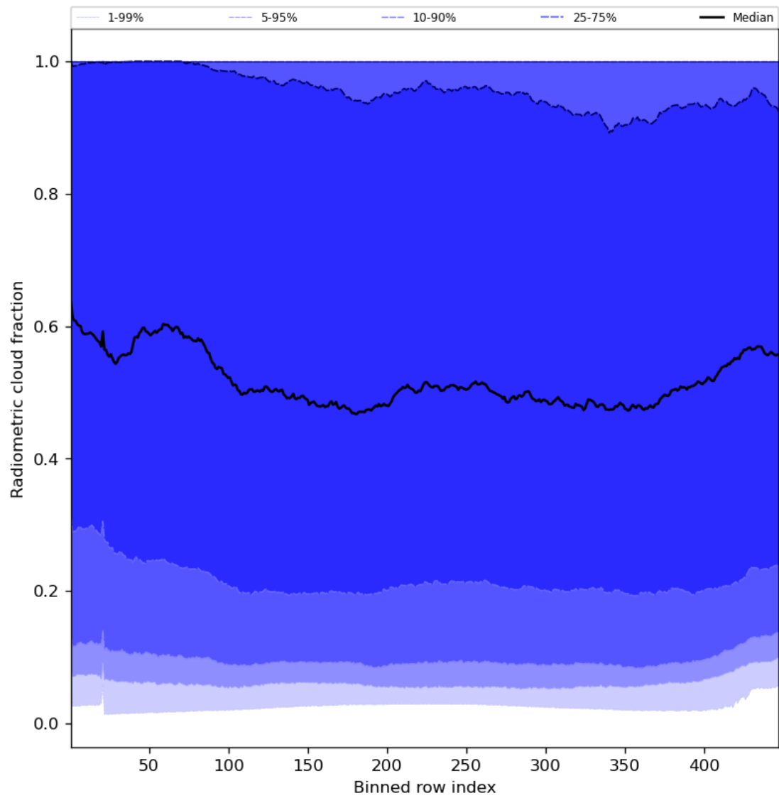
Figure 55: Along track statistics of “Radiometric cloud fraction” for 2023-09-26 to 2023-09-28
