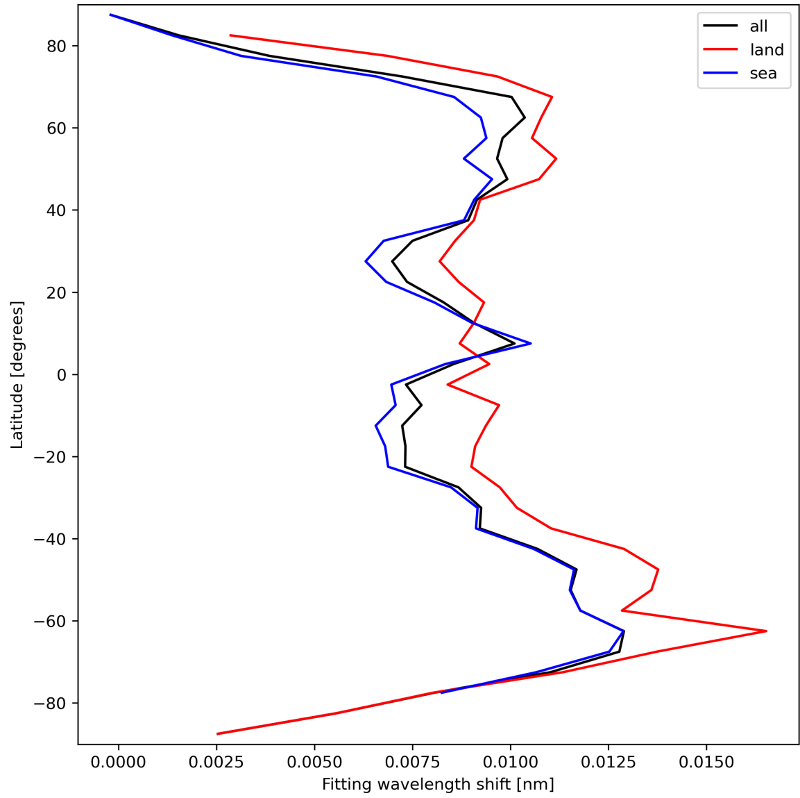
Figure 33: Zonal average of “Fitting wavelength shift” for 2023-09-26 to 2023-09-28.
