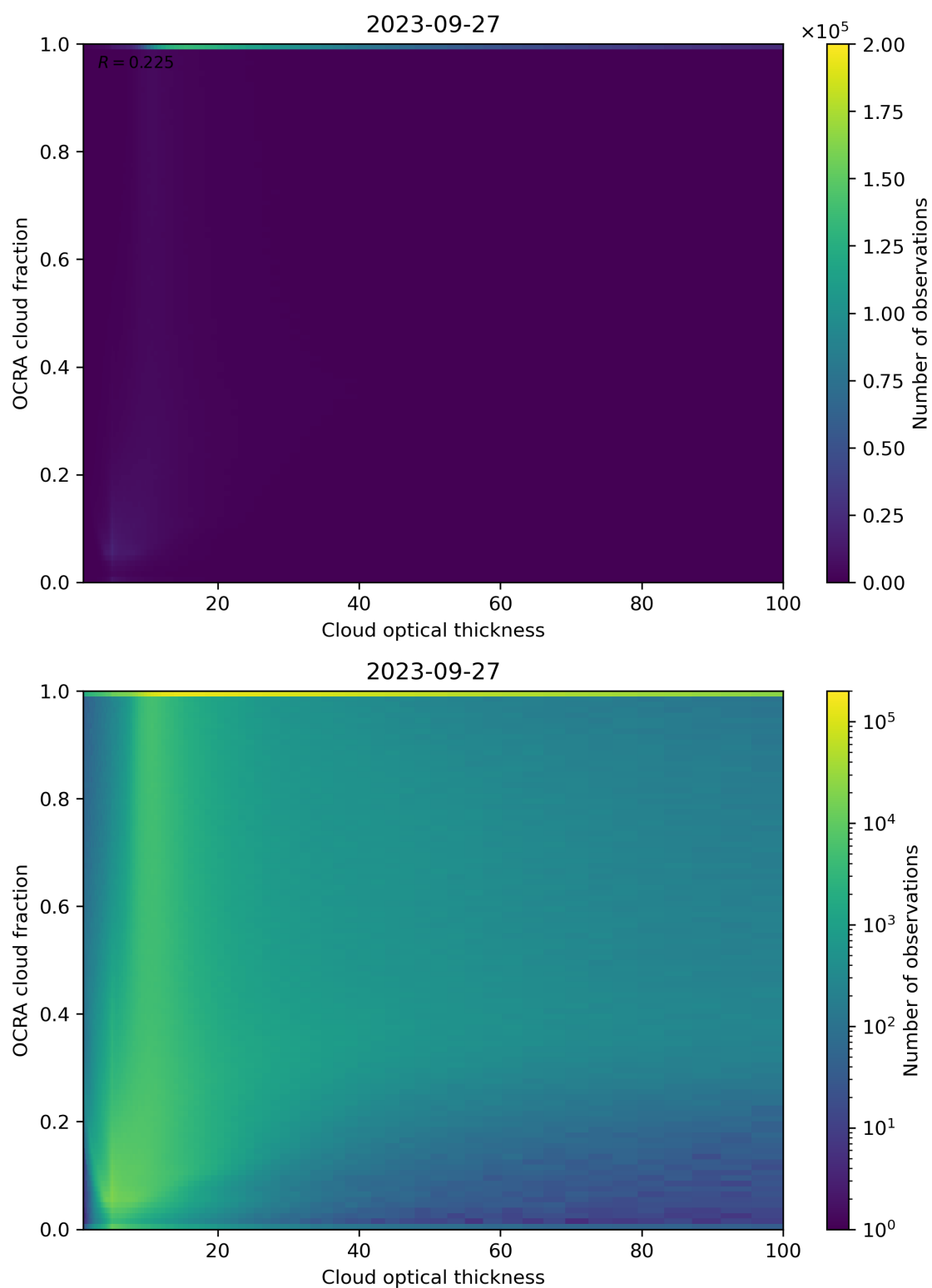
Figure 83: Scatter density plot of “Cloud optical thickness” against “OCRA cloud fraction” for 2023-09-26 to 2023-09-28.
