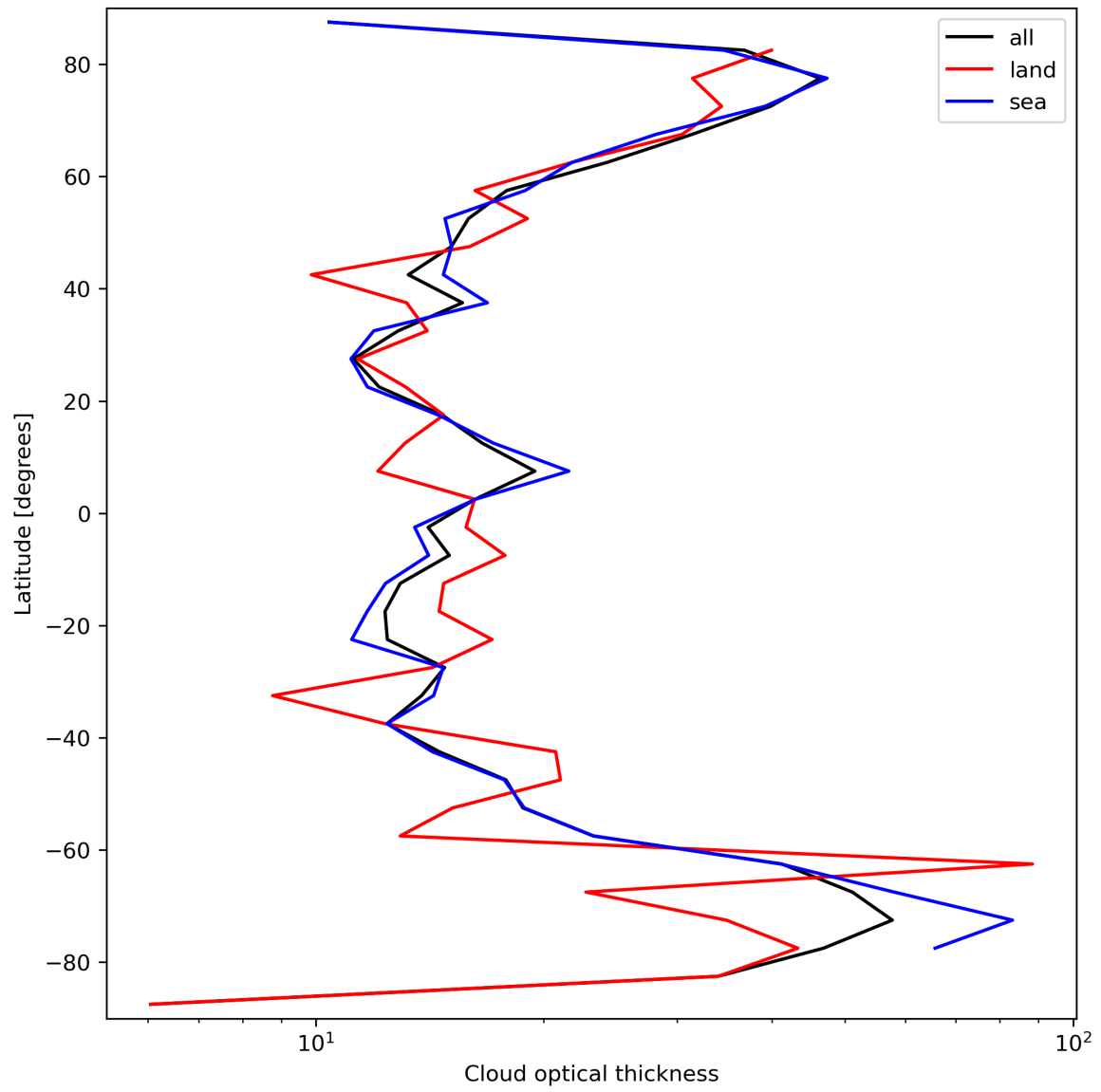
Figure 25: Zonal average of “Cloud optical thickness” for 2023-09-26 to 2023-09-28.
