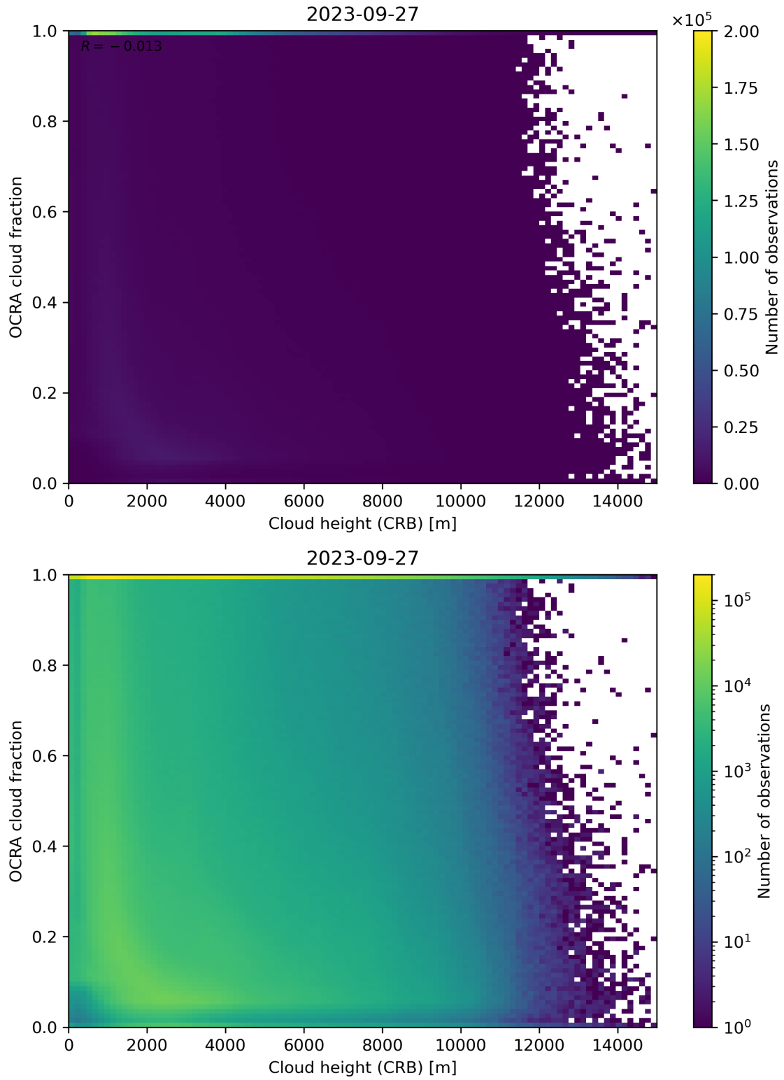
Figure 81: Scatter density plot of “Cloud height (CRB)” against “OCRA cloud fraction” for 2023-09-26 to 2023-09-28.
