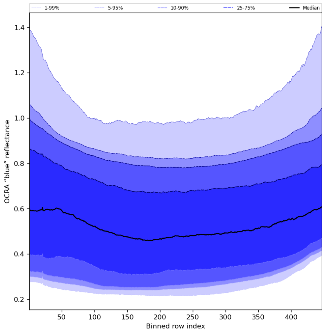
Figure 67: Along track statistics of “OCRA “blue” reflectance” for 2023-09-26 to 2023-09-28
