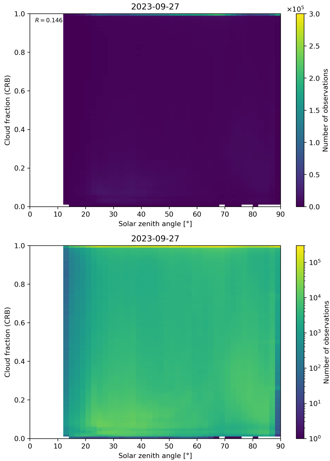
Figure 101: Scatter density plot of “Solar zenith angle” against “Cloud fraction (CRB)” for 2023-09-26 to 2023-09-28.
