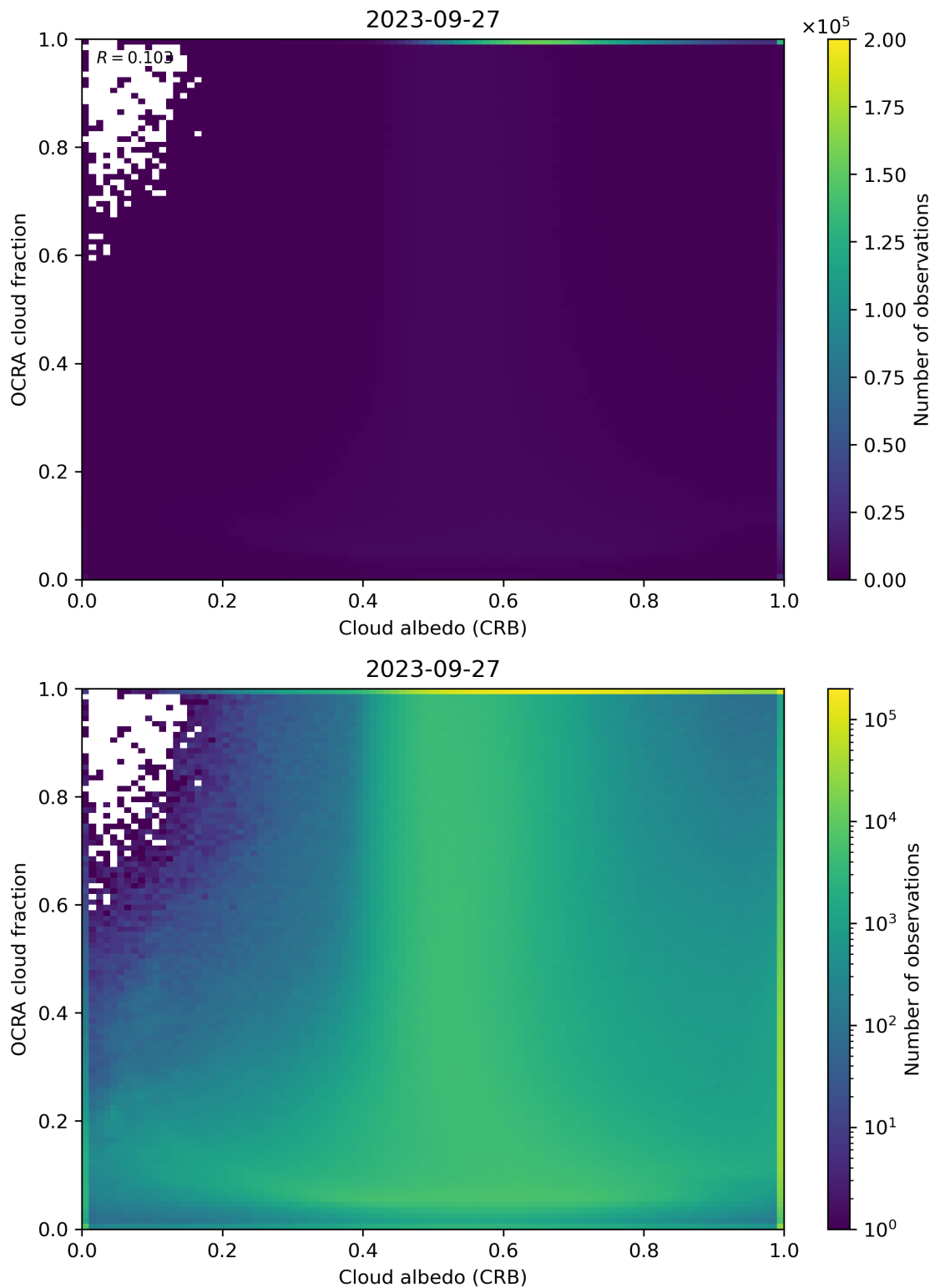
Figure 70: Scatter density plot of “Cloud albedo (CRB)” against “OCRA cloud fraction” for 2023-09-26 to 2023-09-28.
