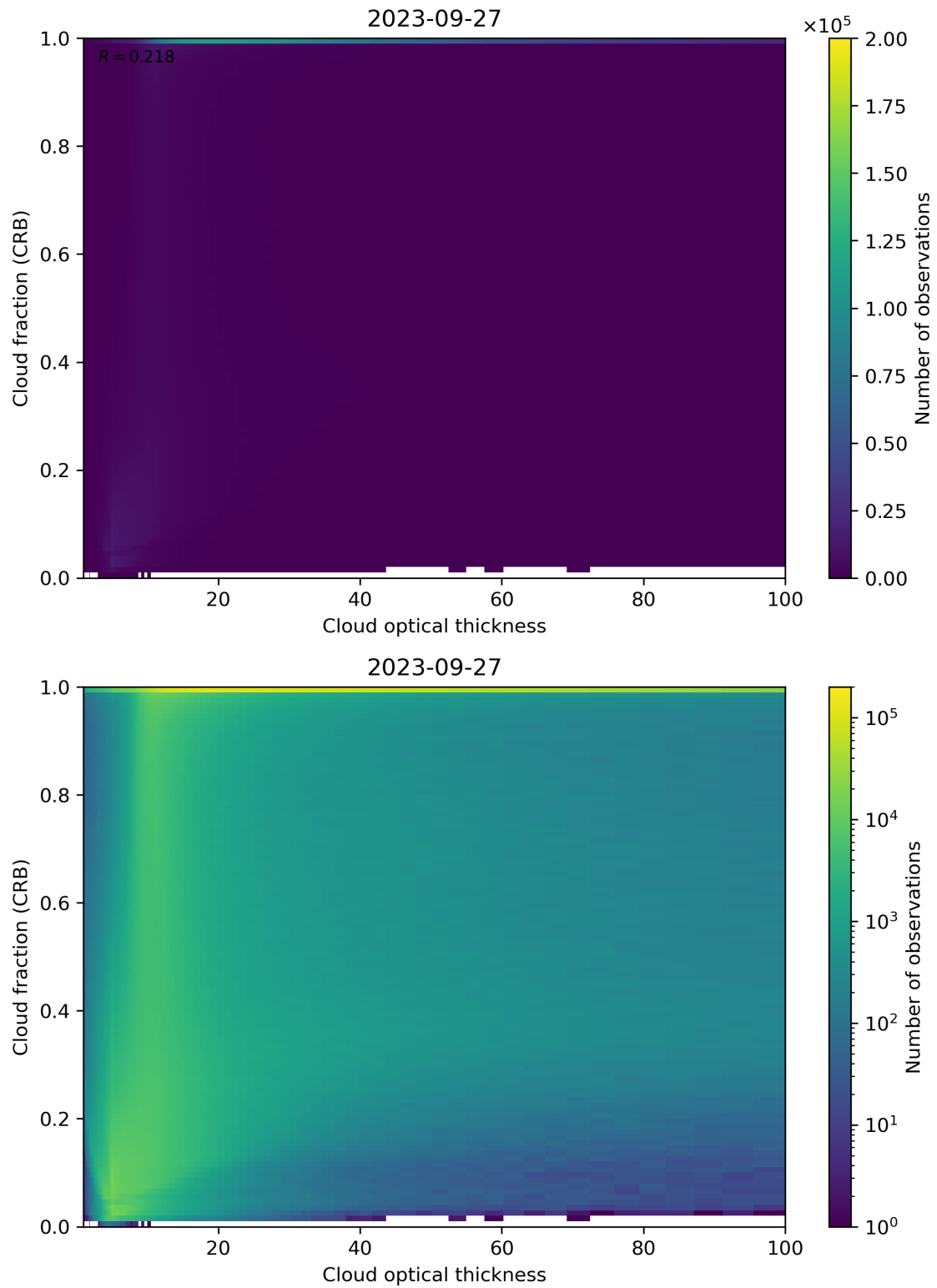
Figure 84: Scatter density plot of “Cloud optical thickness” against “Cloud fraction (CRB)” for 2023-09-26 to 2023-09-28.
