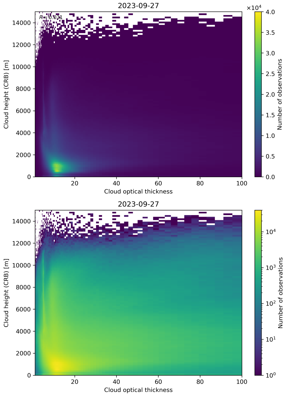
Figure 85: Scatter density plot of “Cloud optical thickness” against “Cloud height (CRB)” for 2023-09-26 to 2023-09-28.
