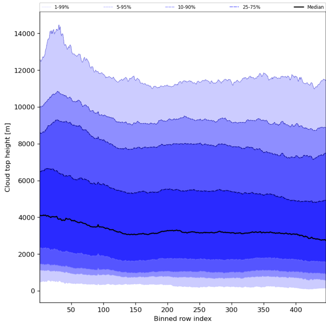
Figure 56: Along track statistics of “Cloud top height” for 2023-09-26 to 2023-09-28
