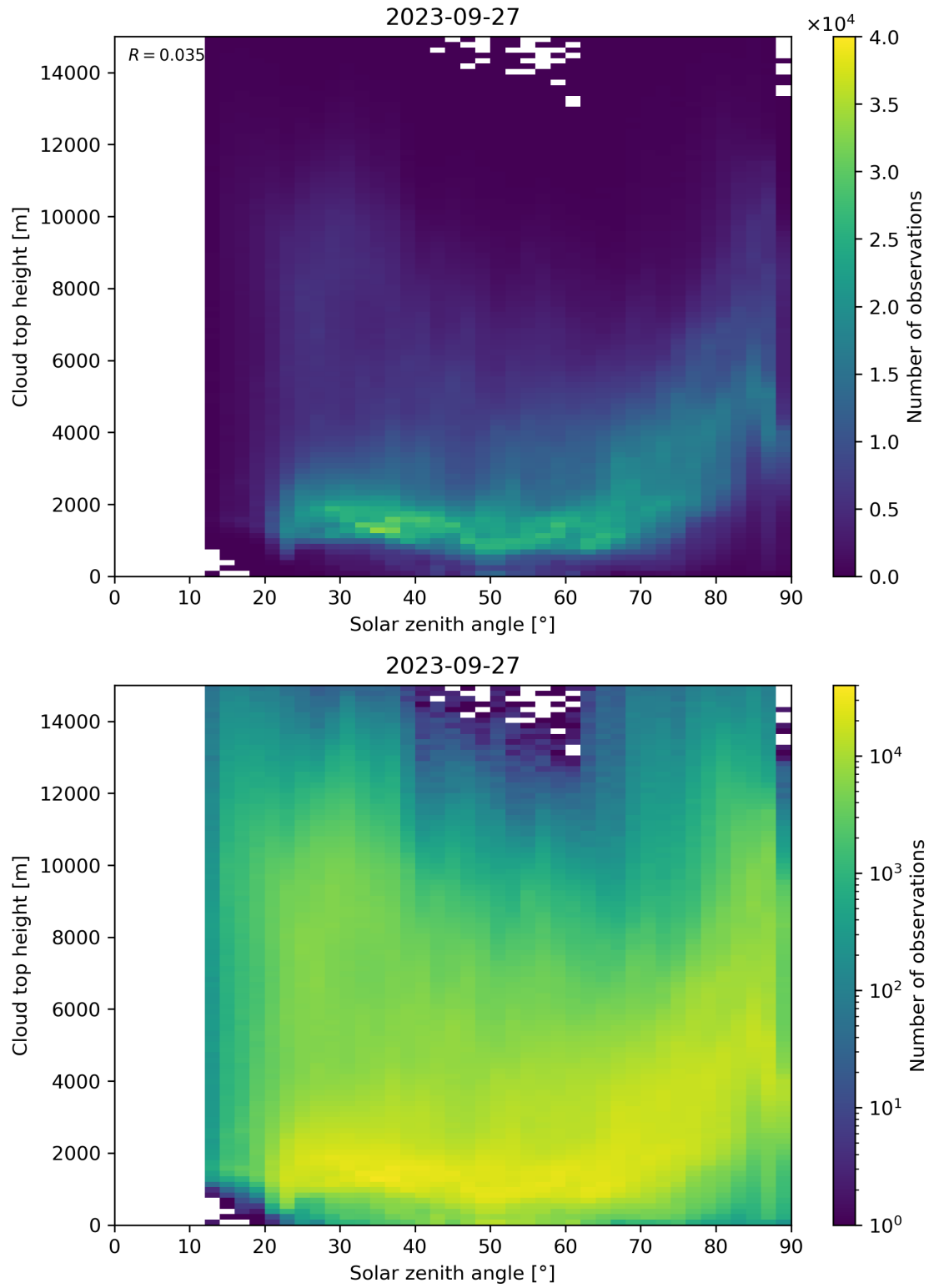
Figure 104: Scatter density plot of “Solar zenith angle” against “Cloud top height” for 2023-09-26 to 2023-09-28.
