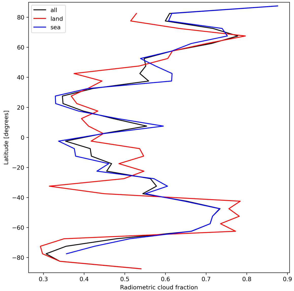
Figure 23: Zonal average of “Radiometric cloud fraction” for 2023-09-26 to 2023-09-28.
