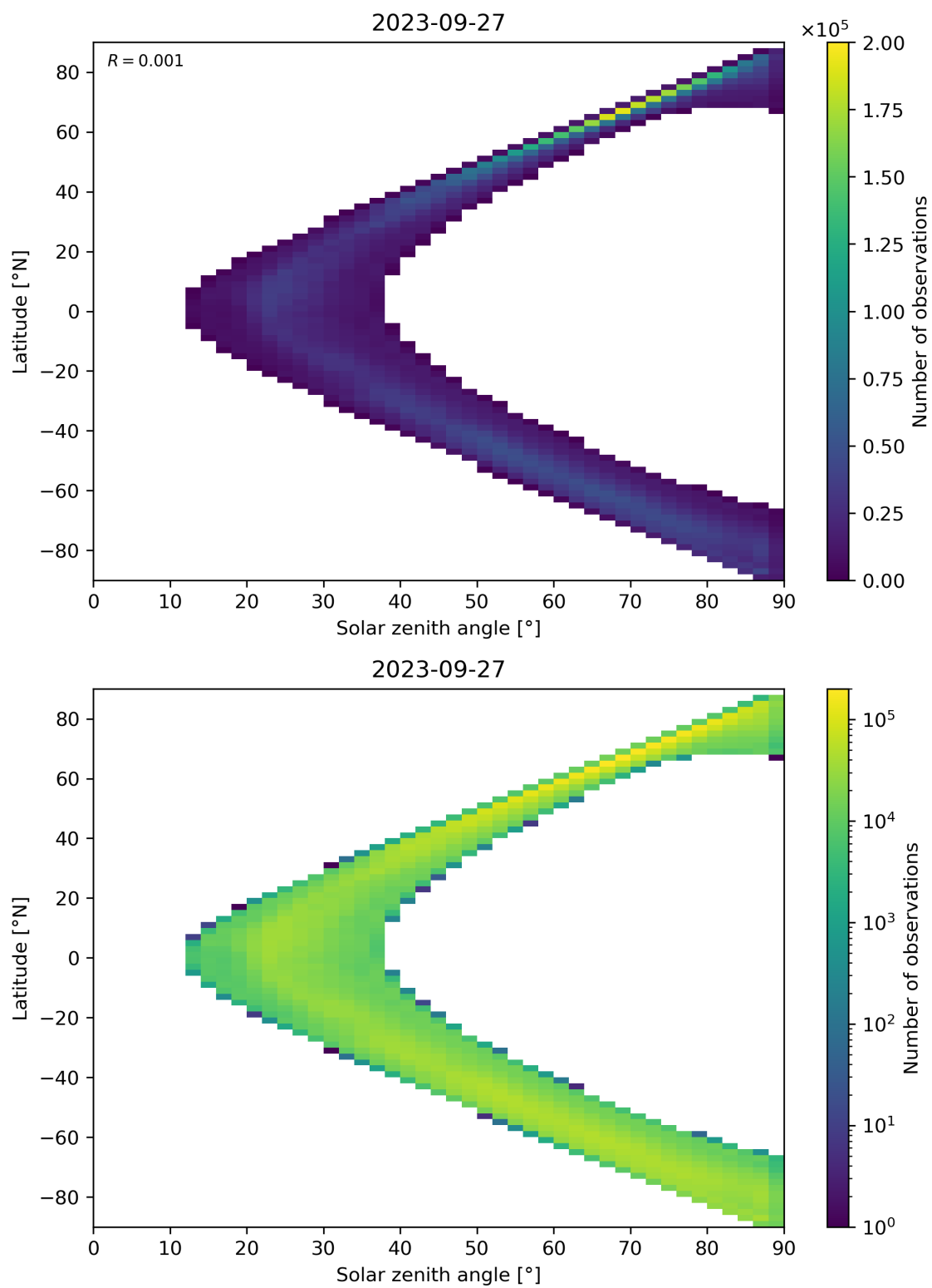
Figure 105: Scatter density plot of “Solar zenith angle” against “Latitude” for 2023-09-26 to 2023-09-28.
