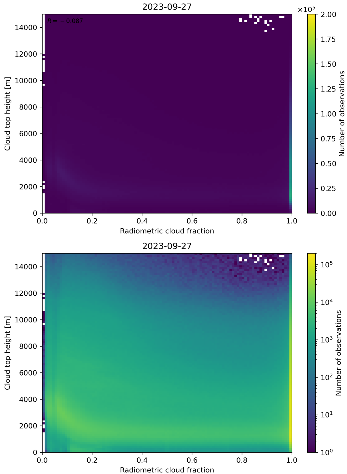
Figure 76: Scatter density plot of “Radiometric cloud fraction” against “Cloud top height” for 2023-09-26 to 2023-09-28.
