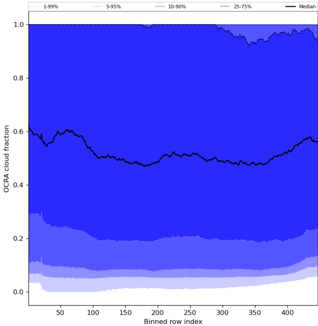
Figure 66: Along track statistics of “OCRA cloud fraction” for 2023-09-26 to 2023-09-28
