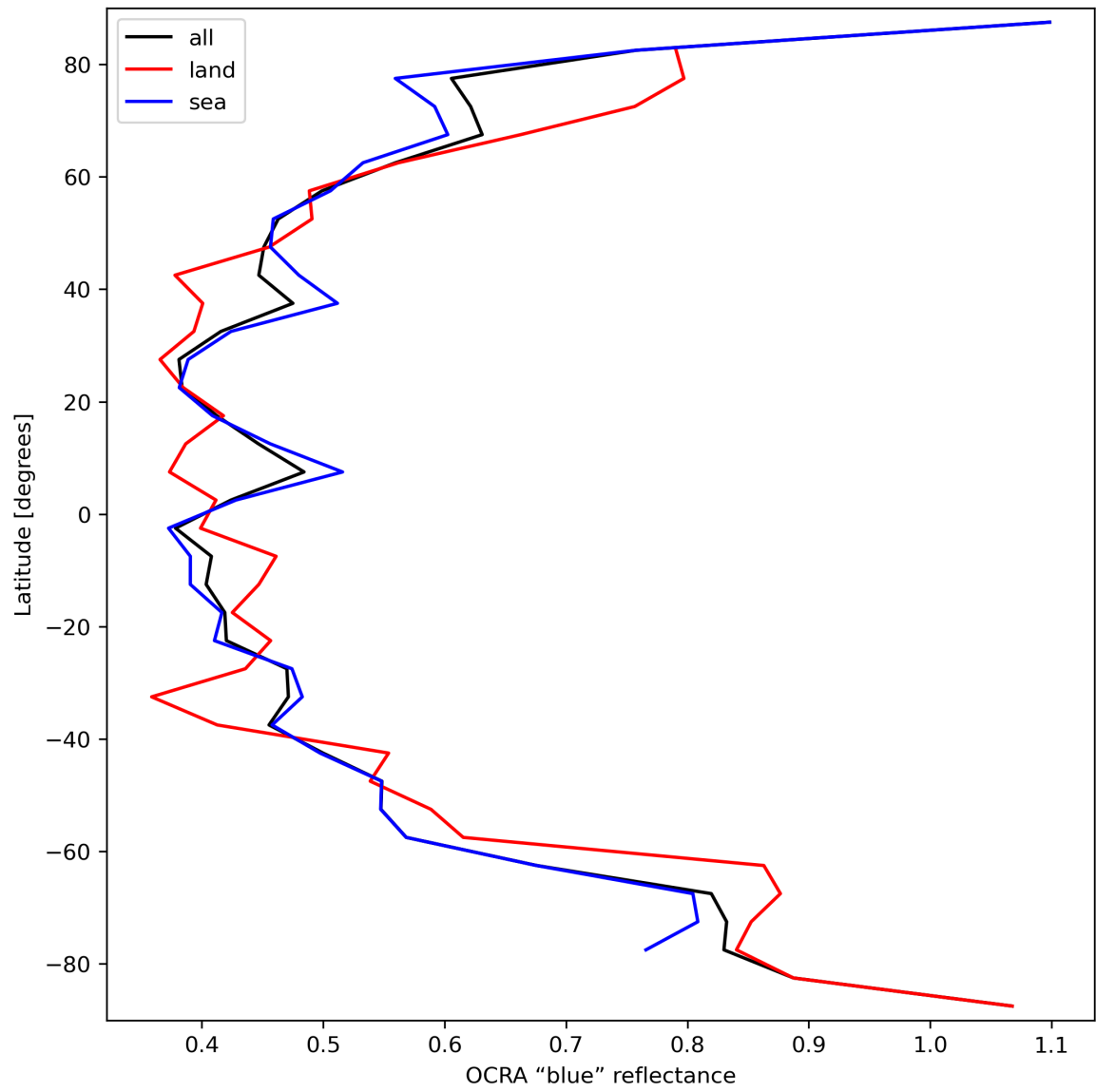
Figure 35: Zonal average of “OCRA “blue” reflectance” for 2023-09-26 to 2023-09-28.
