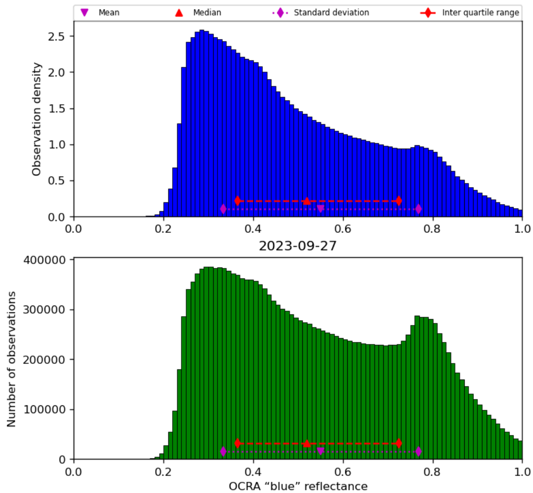
Figure 51: Histogram of “OCRA “blue” reflectance” for 2023-09-26 to 2023-09-28
