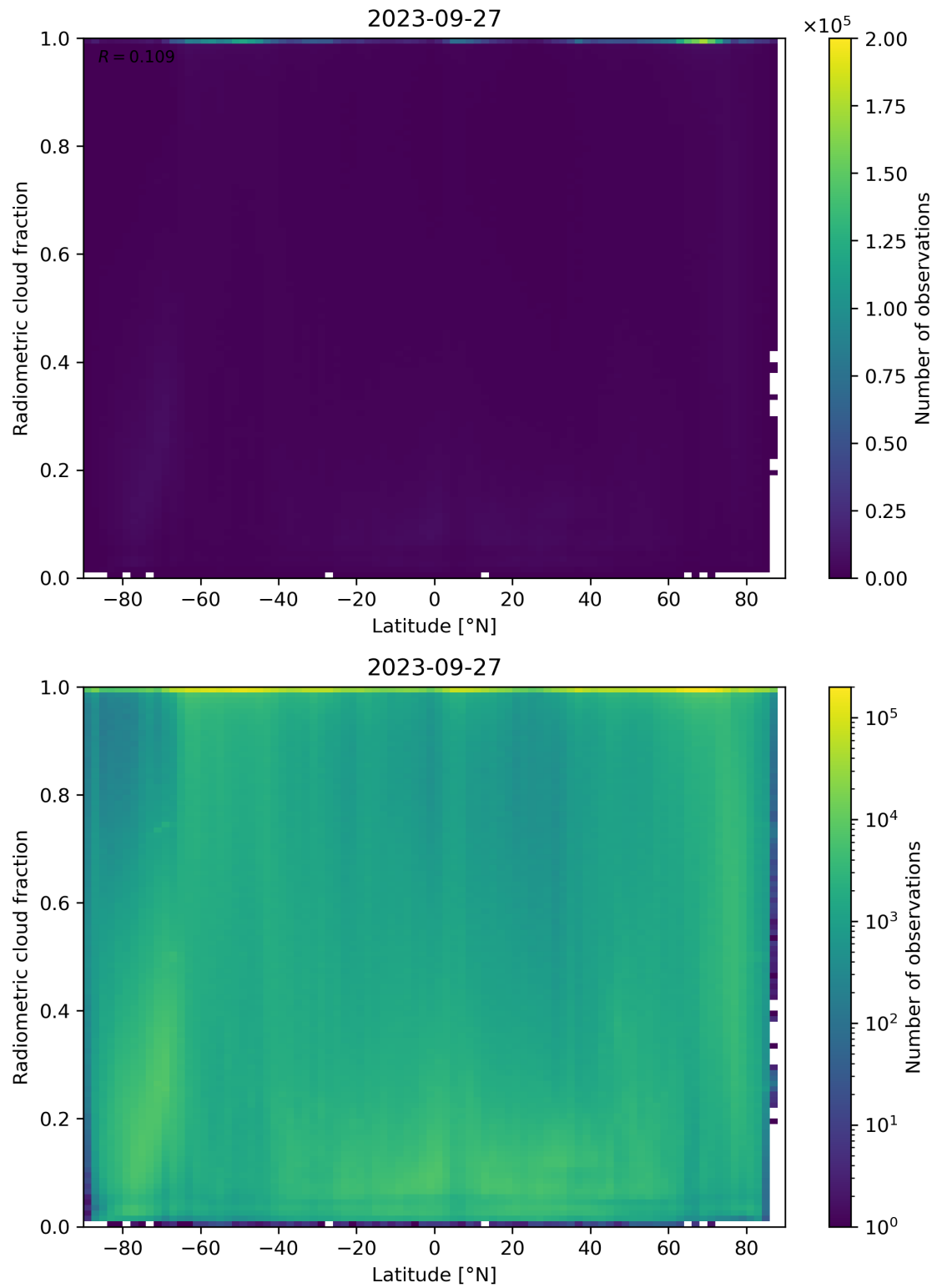
Figure 92: Scatter density plot of “Latitude” against “Radiometric cloud fraction” for 2023-09-26 to 2023-09-28.
