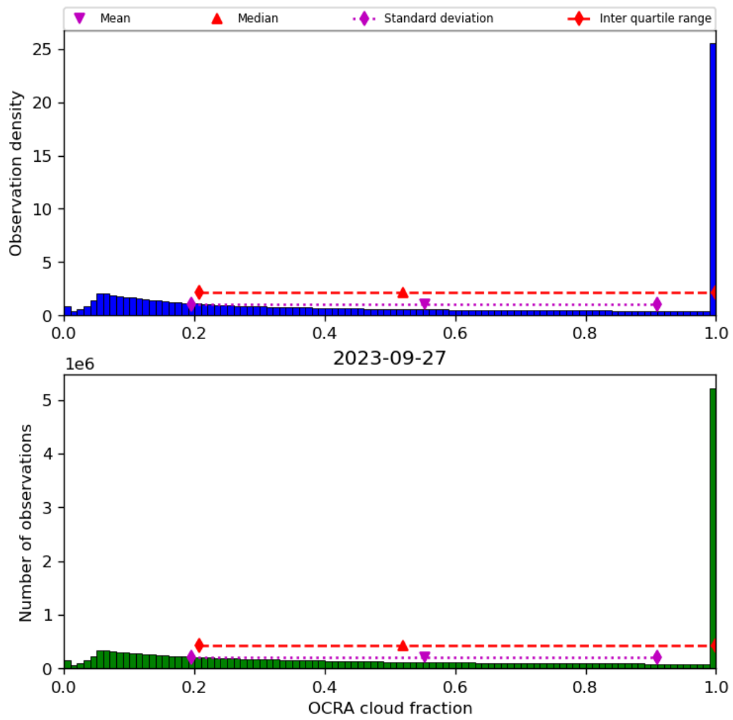
Figure 50: Histogram of “OCRA cloud fraction” for 2023-09-26 to 2023-09-28
