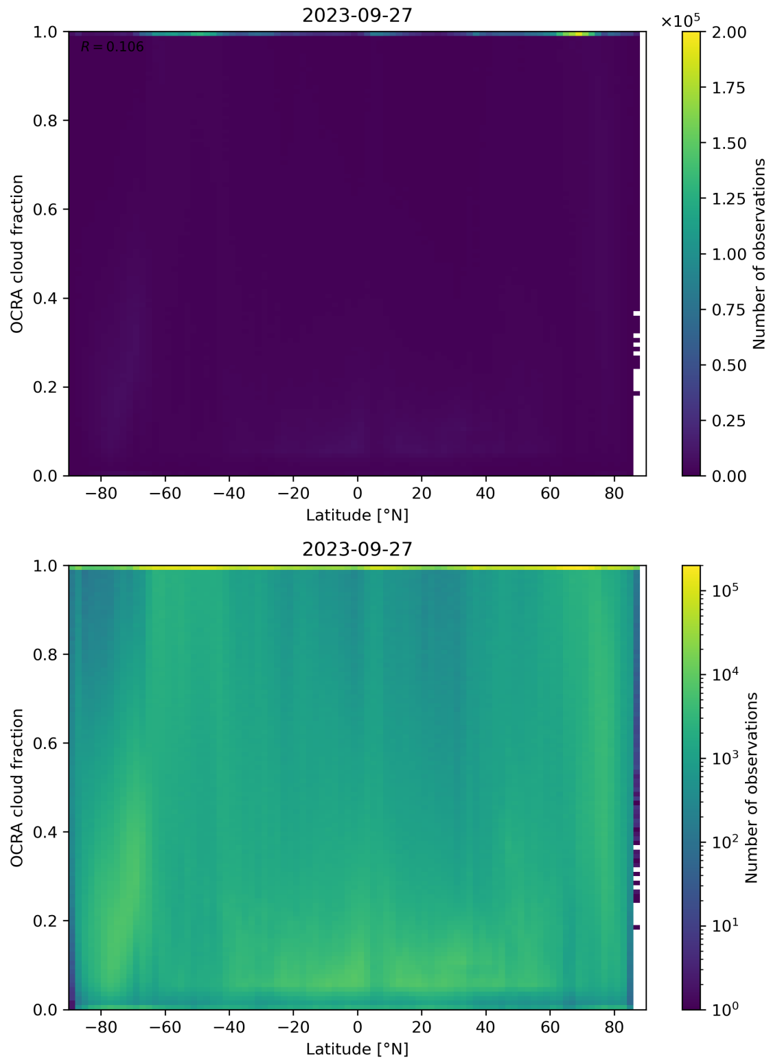
Figure 93: Scatter density plot of “Latitude” against “OCRA cloud fraction” for 2023-09-26 to 2023-09-28.
