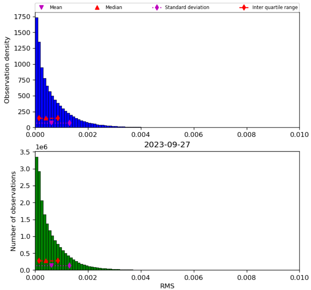
Figure 47: Histogram of “RMS” for 2023-09-26 to 2023-09-28
