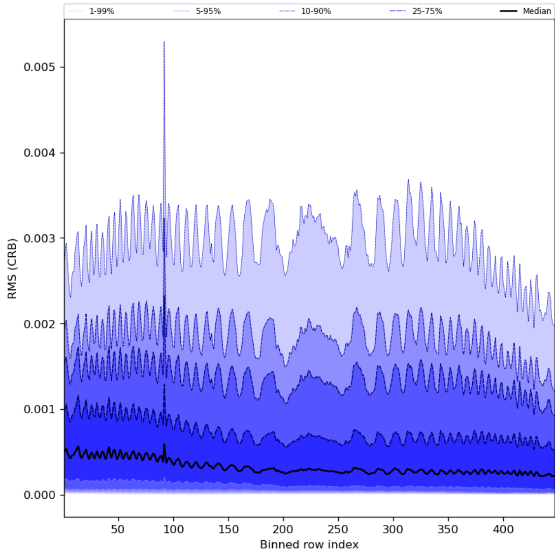
Figure 64: Along track statistics of “RMS (CRB)” for 2023-09-26 to 2023-09-28
