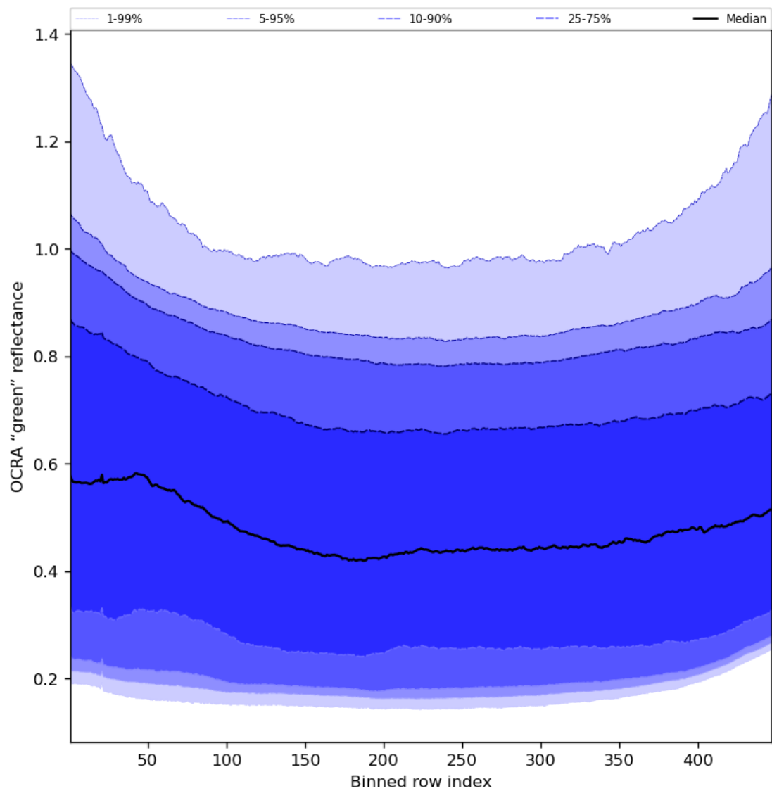
Figure 68: Along track statistics of “OCRA “green” reflectance” for 2023-09-26 to 2023-09-28
