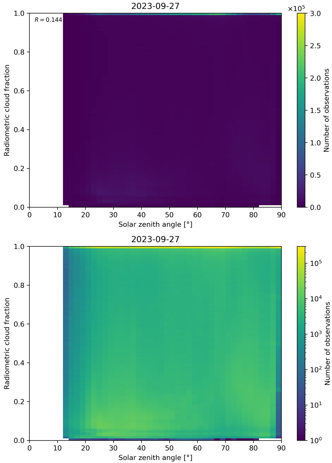
Figure 99: Scatter density plot of “Solar zenith angle” against “Radiometric cloud fraction” for 2023-09-26 to 2023-09-28.
