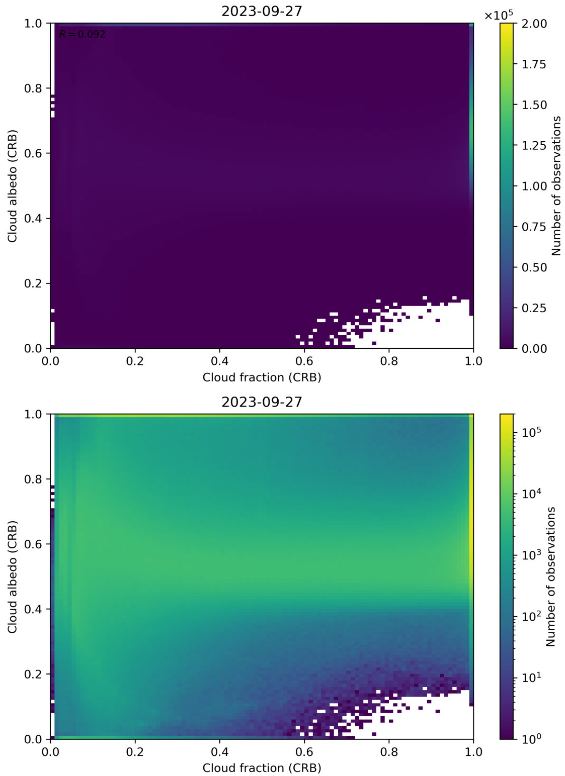
Figure 77: Scatter density plot of “Cloud fraction (CRB)” against “Cloud albedo (CRB)” for 2023-09-26 to 2023-09-28.
