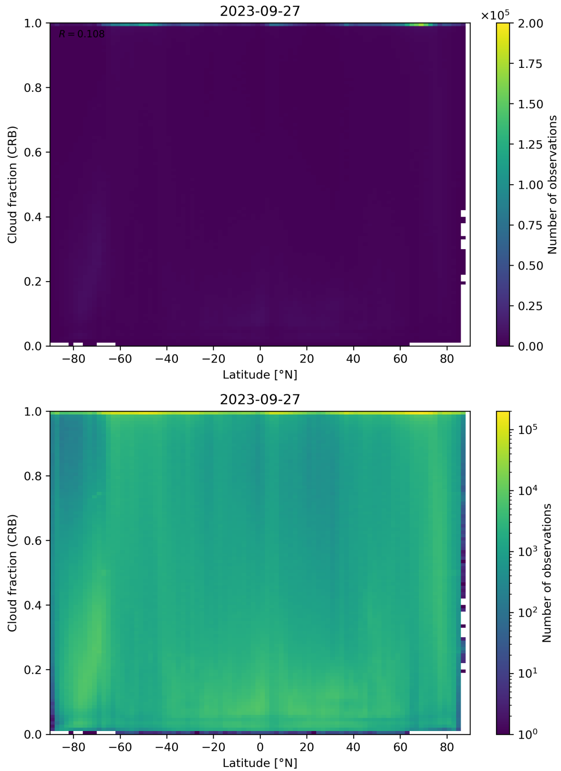
Figure 94: Scatter density plot of “Latitude” against “Cloud fraction (CRB)” for 2023-09-26 to 2023-09-28.
