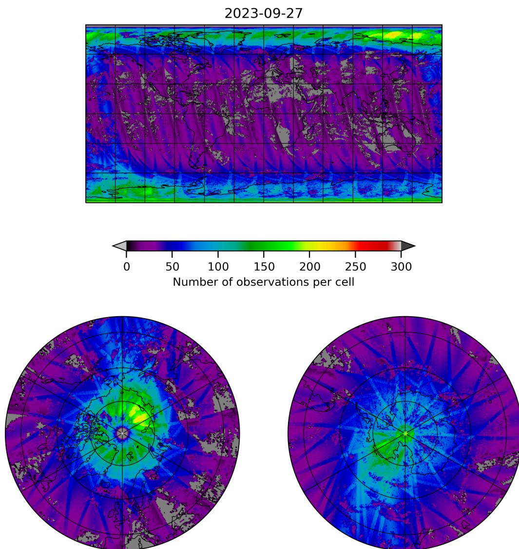
Figure 21: Map of the number of observations for 2023-09-26 to 2023-09-28
