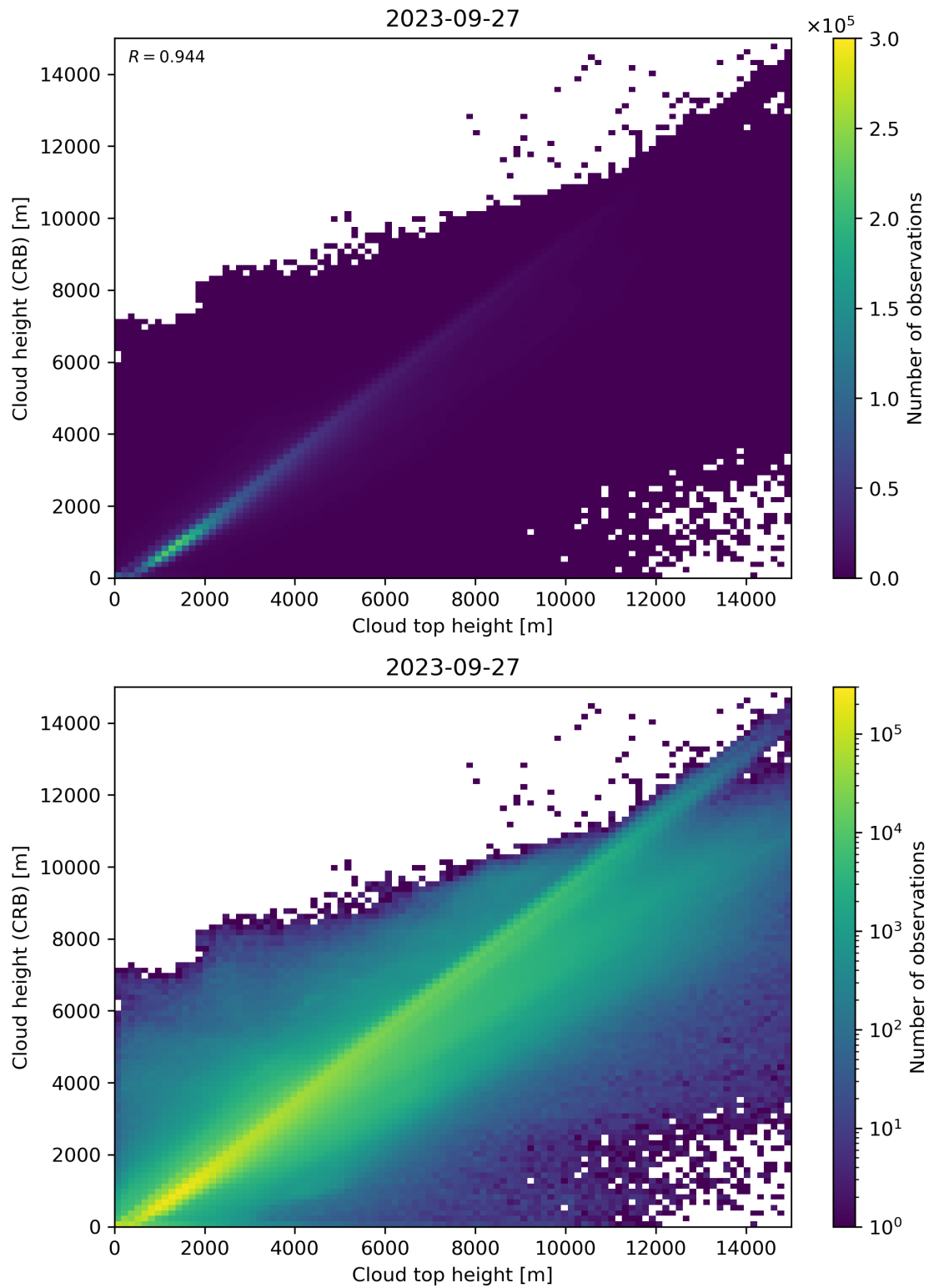
Figure 89: Scatter density plot of “Cloud top height” against “Cloud height (CRB)” for 2023-09-26 to 2023-09-28.
