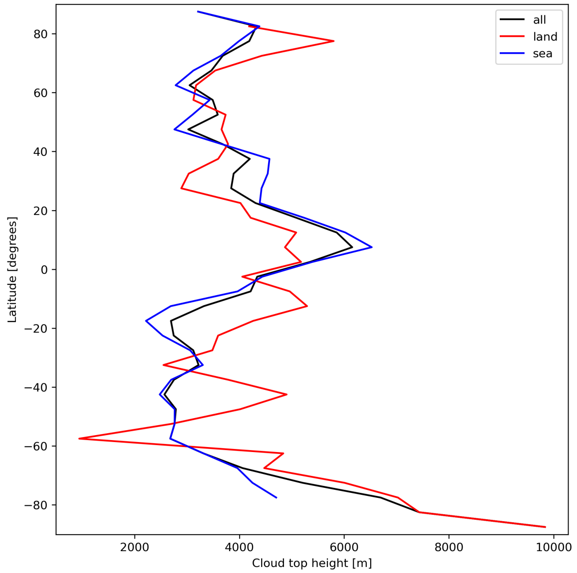
Figure 24: Zonal average of “Cloud top height” for 2023-09-26 to 2023-09-28.
