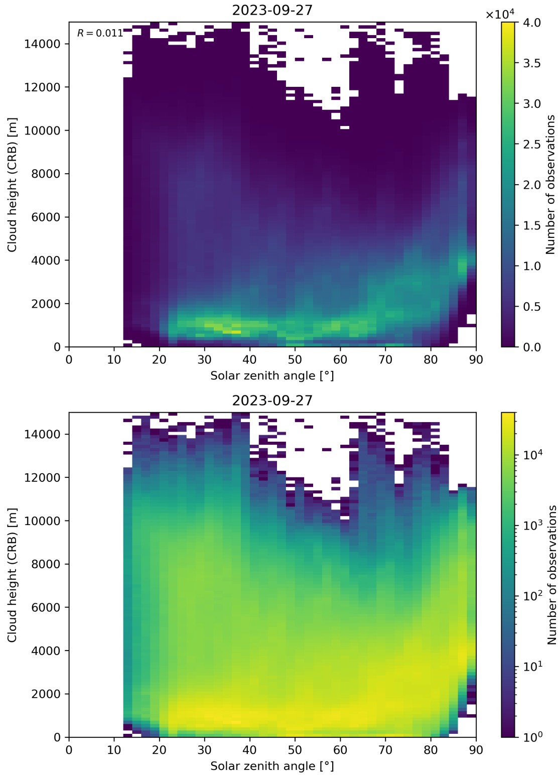
Figure 102: Scatter density plot of “Solar zenith angle” against “Cloud height (CRB)” for 2023-09-26 to 2023-09-28.
