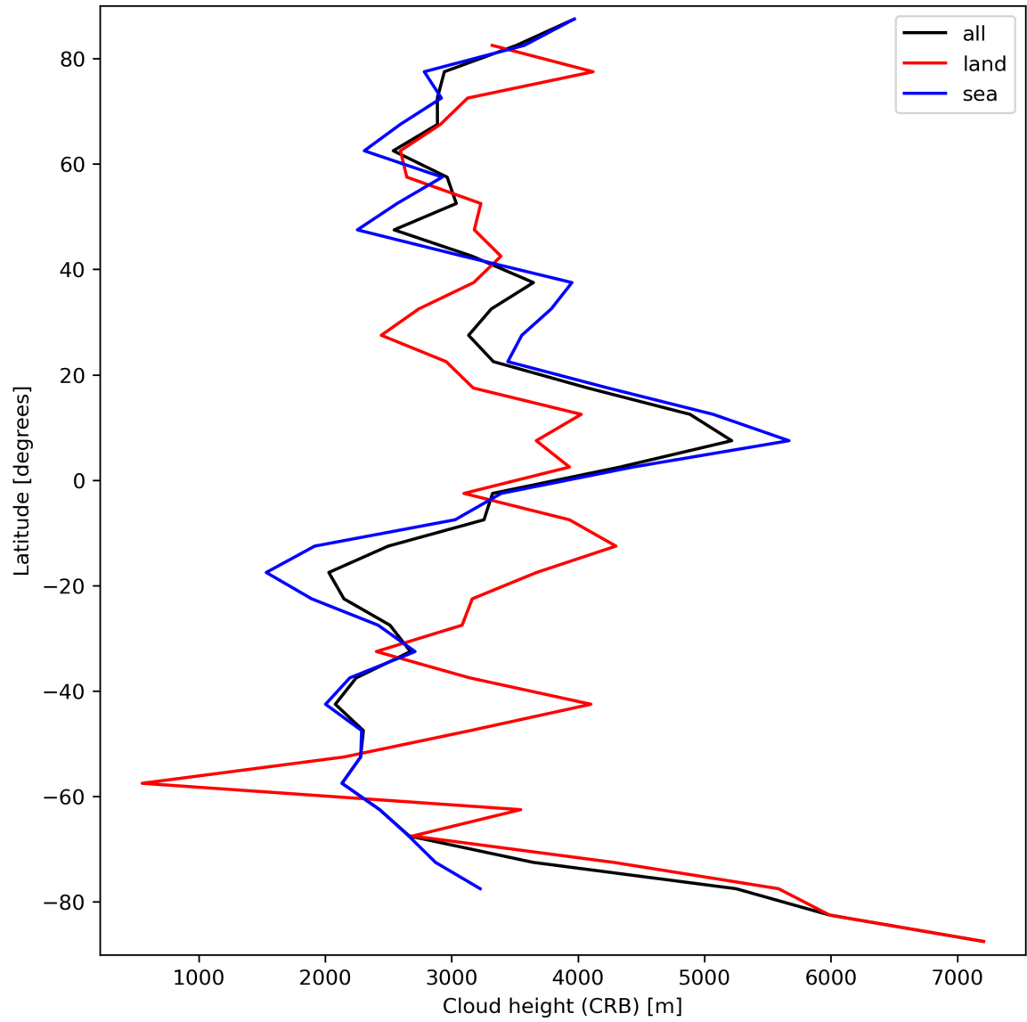
Figure 27: Zonal average of “Cloud height (CRB)” for 2023-09-26 to 2023-09-28.
