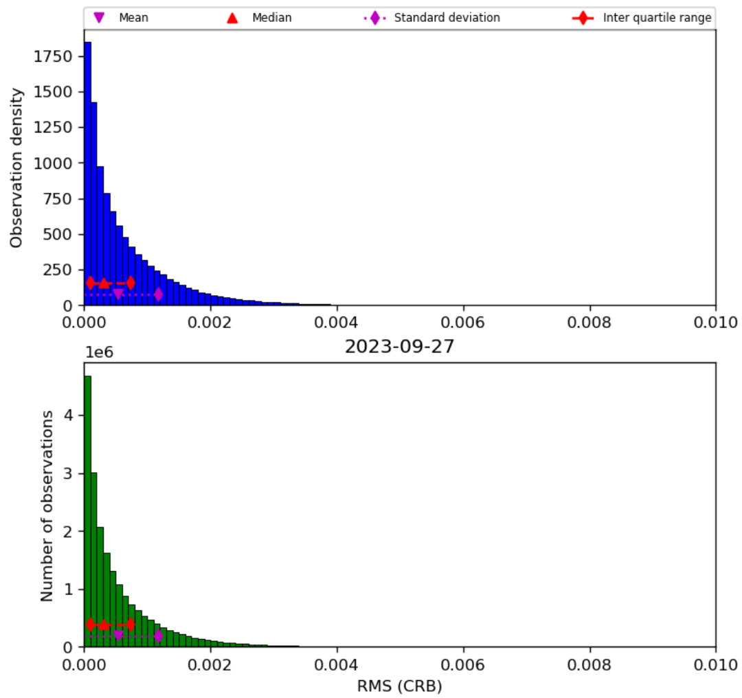
Figure 48: Histogram of “RMS (CRB)” for 2023-09-26 to 2023-09-28
