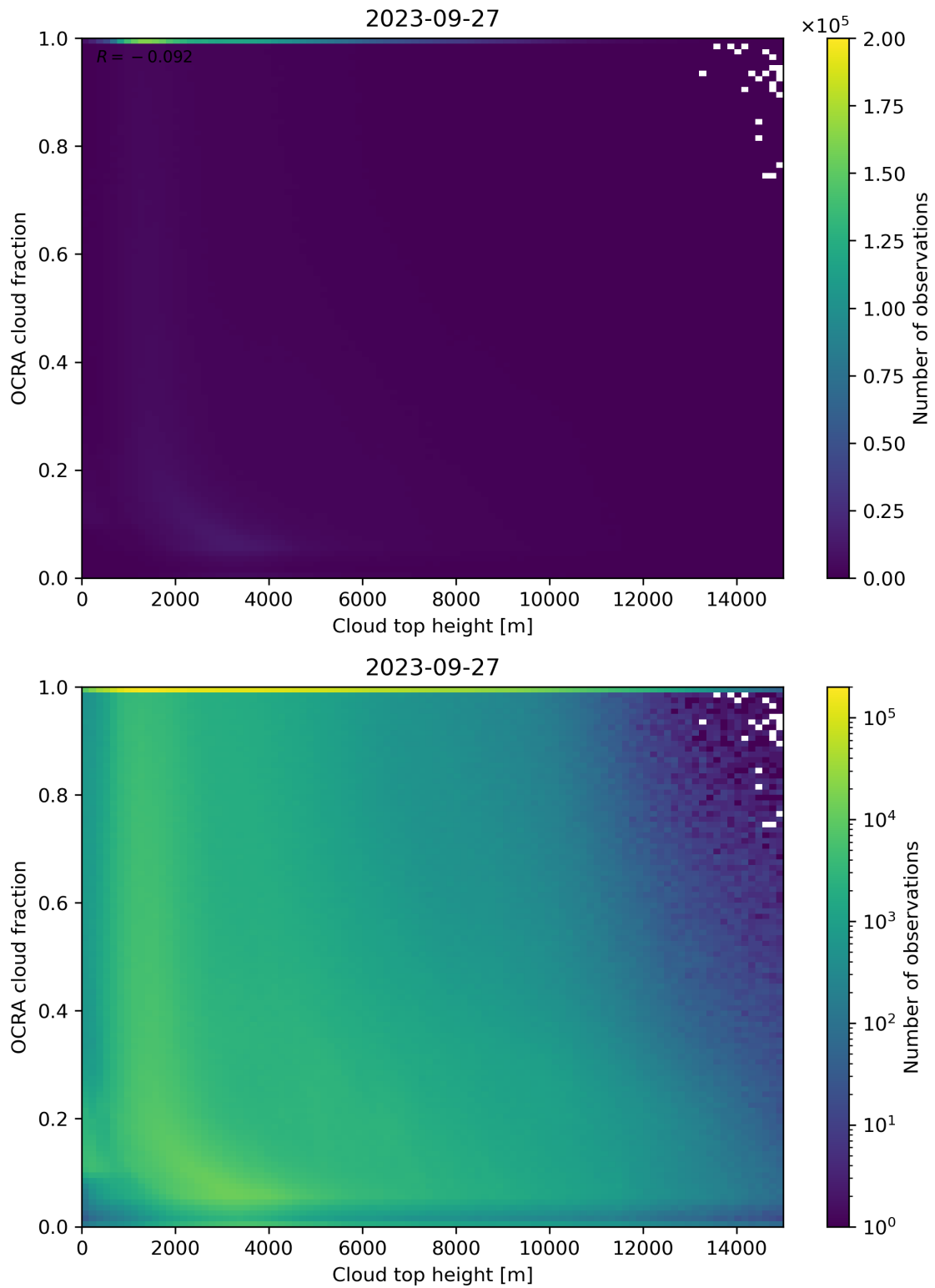
Figure 87: Scatter density plot of “Cloud top height” against “OCRA cloud fraction” for 2023-09-26 to 2023-09-28.
