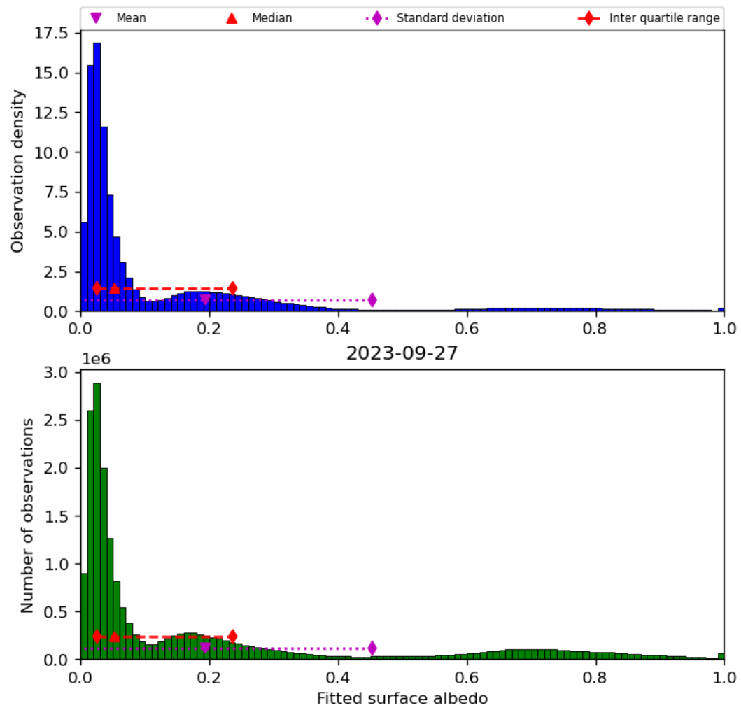
Figure 45: Histogram of “Fitted surface albedo” for 2023-09-26 to 2023-09-28
