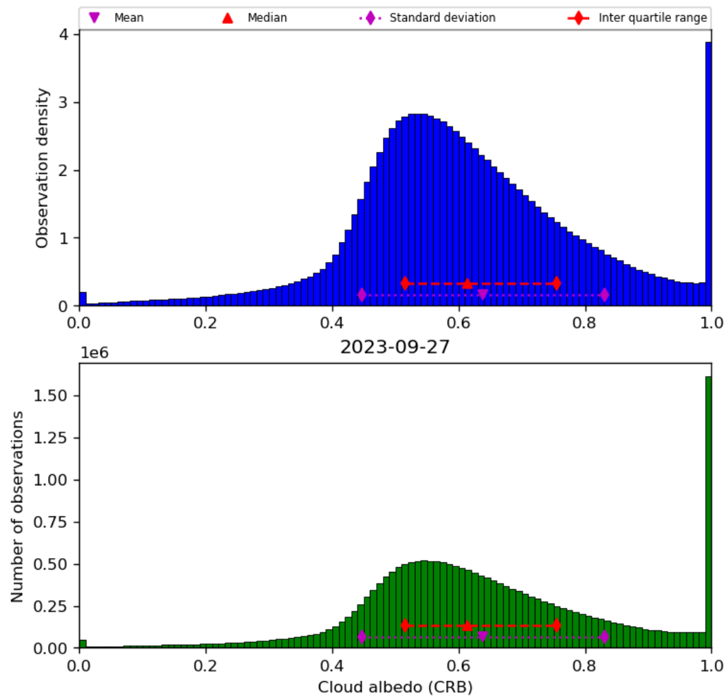
Figure 44: Histogram of “Cloud albedo (CRB)” for 2023-09-26 to 2023-09-28
