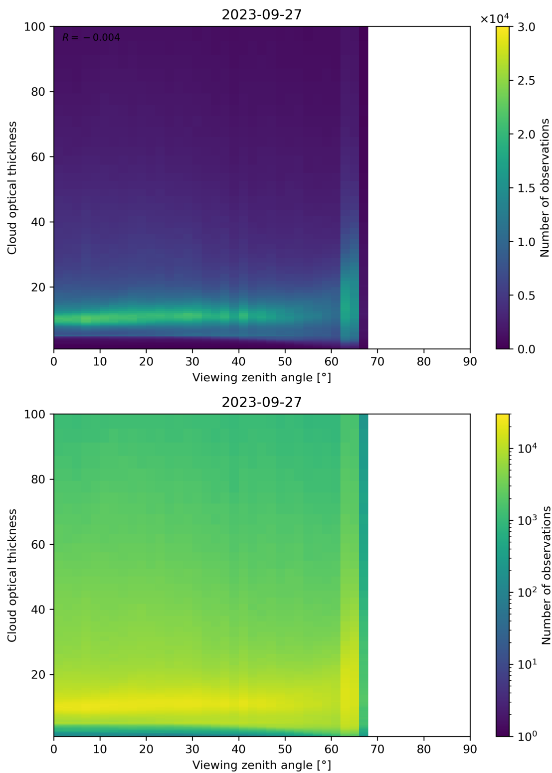
Figure 111: Scatter density plot of “Viewing zenith angle” against “Cloud optical thickness” for 2023-09-26 to 2023-09-28.
