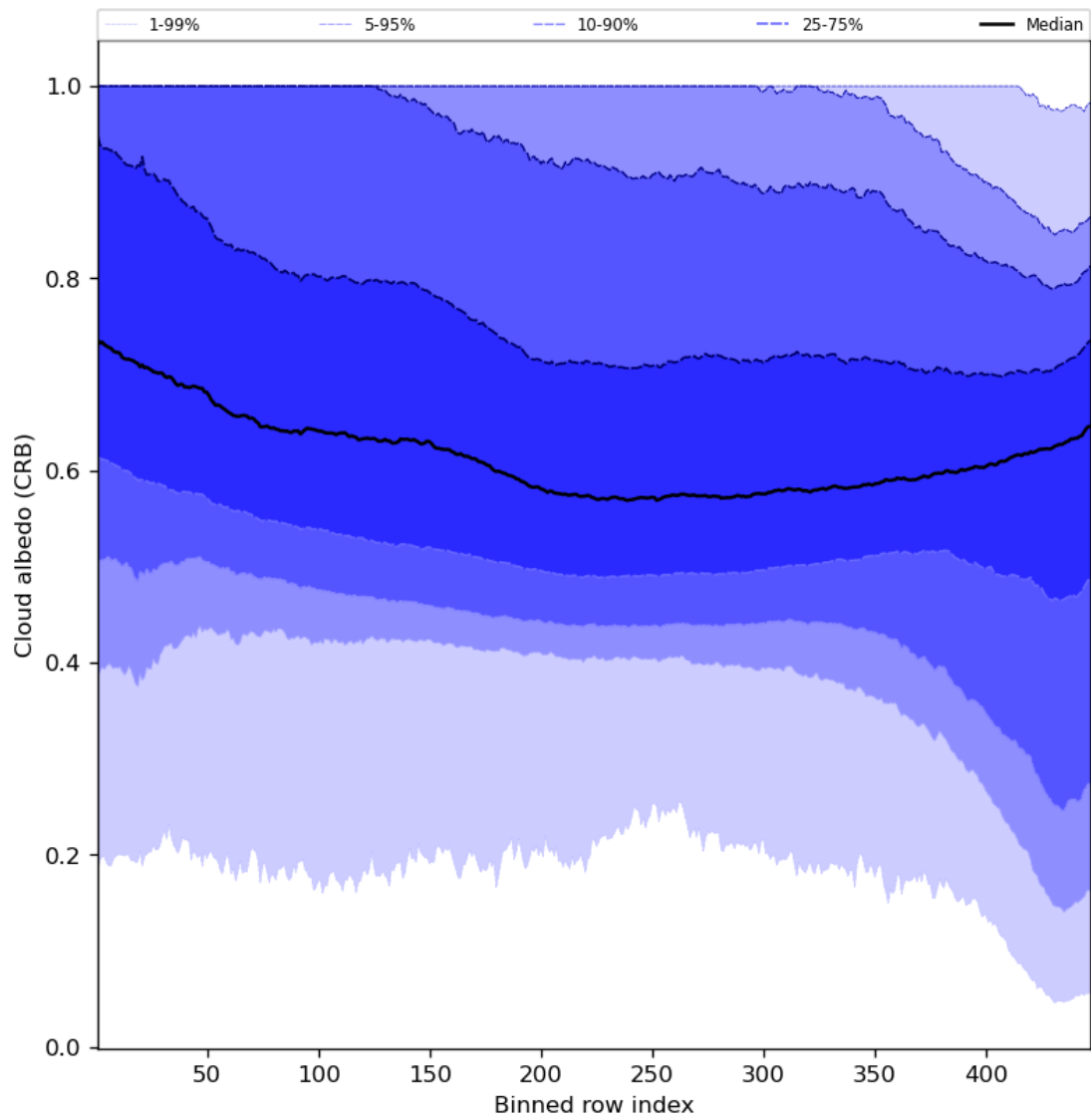
Figure 60: Along track statistics of “Cloud albedo (CRB)” for 2023-09-26 to 2023-09-28
