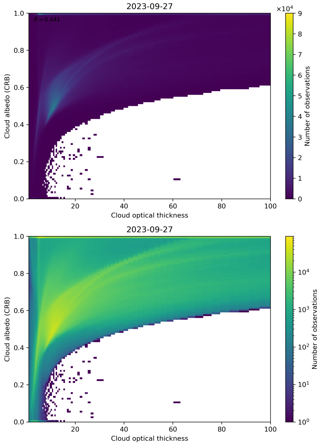
Figure 82: Scatter density plot of “Cloud optical thickness” against “Cloud albedo (CRB)” for 2023-09-26 to 2023-09-28.
