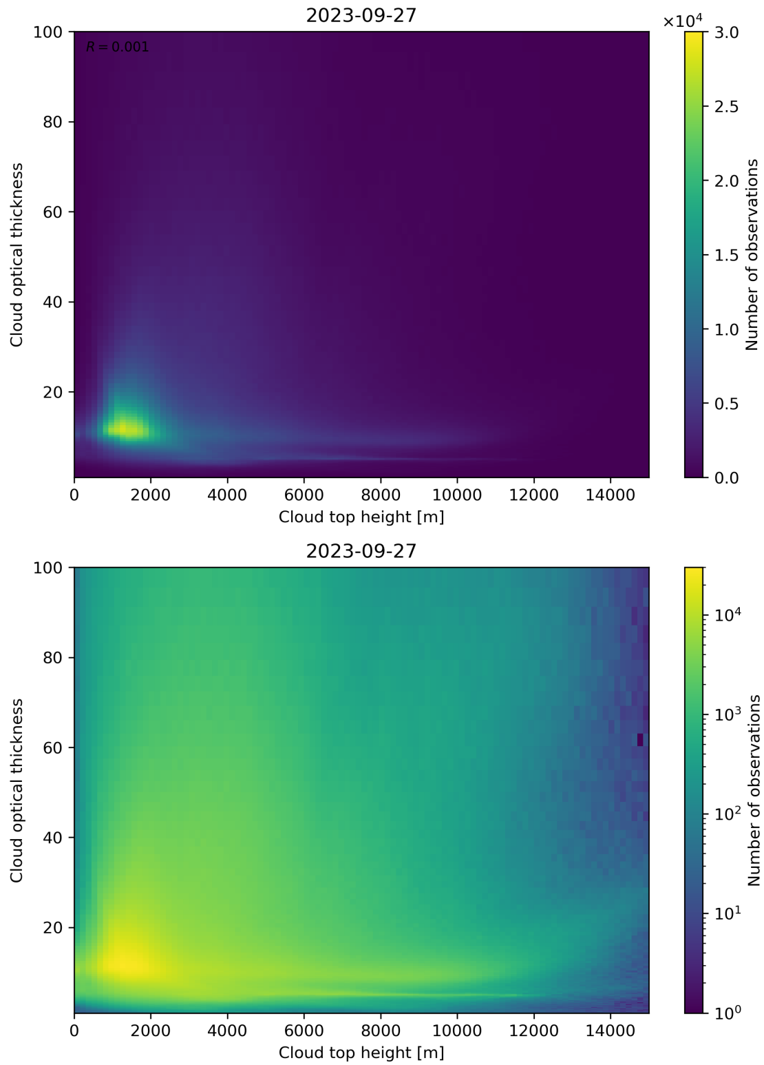
Figure 90: Scatter density plot of “Cloud top height” against “Cloud optical thickness” for 2023-09-26 to 2023-09-28.
