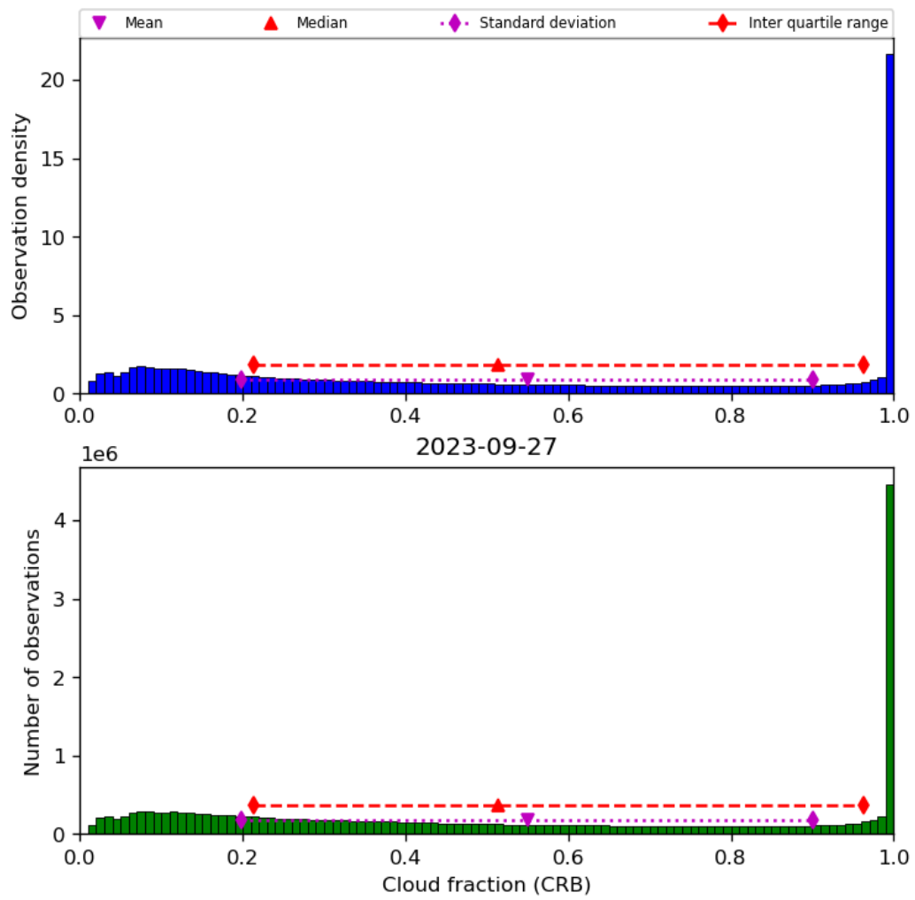
Figure 42: Histogram of “Cloud fraction (CRB)” for 2023-09-26 to 2023-09-28
