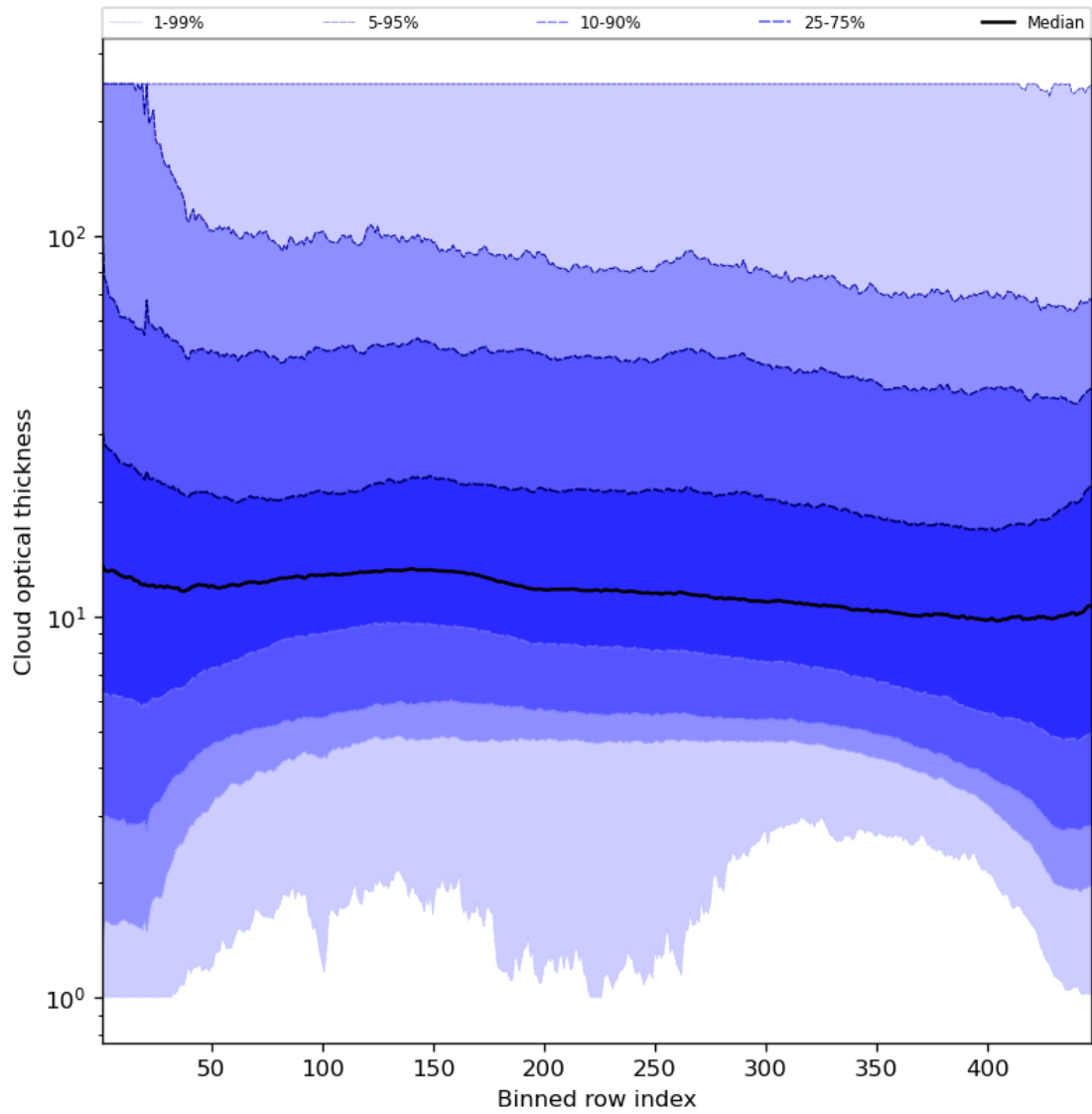
Figure 57: Along track statistics of “Cloud optical thickness” for 2023-09-26 to 2023-09-28
