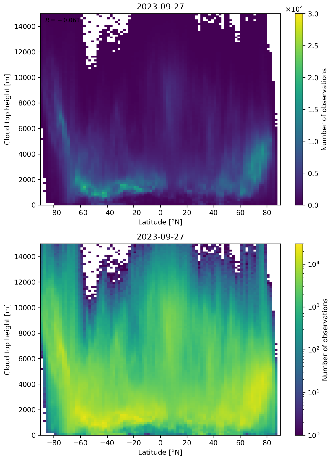
Figure 97: Scatter density plot of “Latitude” against “Cloud top height” for 2023-09-26 to 2023-09-28.
