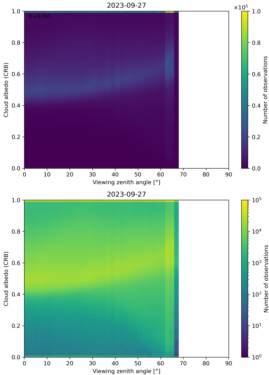
Figure 106: Scatter density plot of “Viewing zenith angle” against “Cloud albedo (CRB)” for 2023-09-26 to 2023-09-28.
