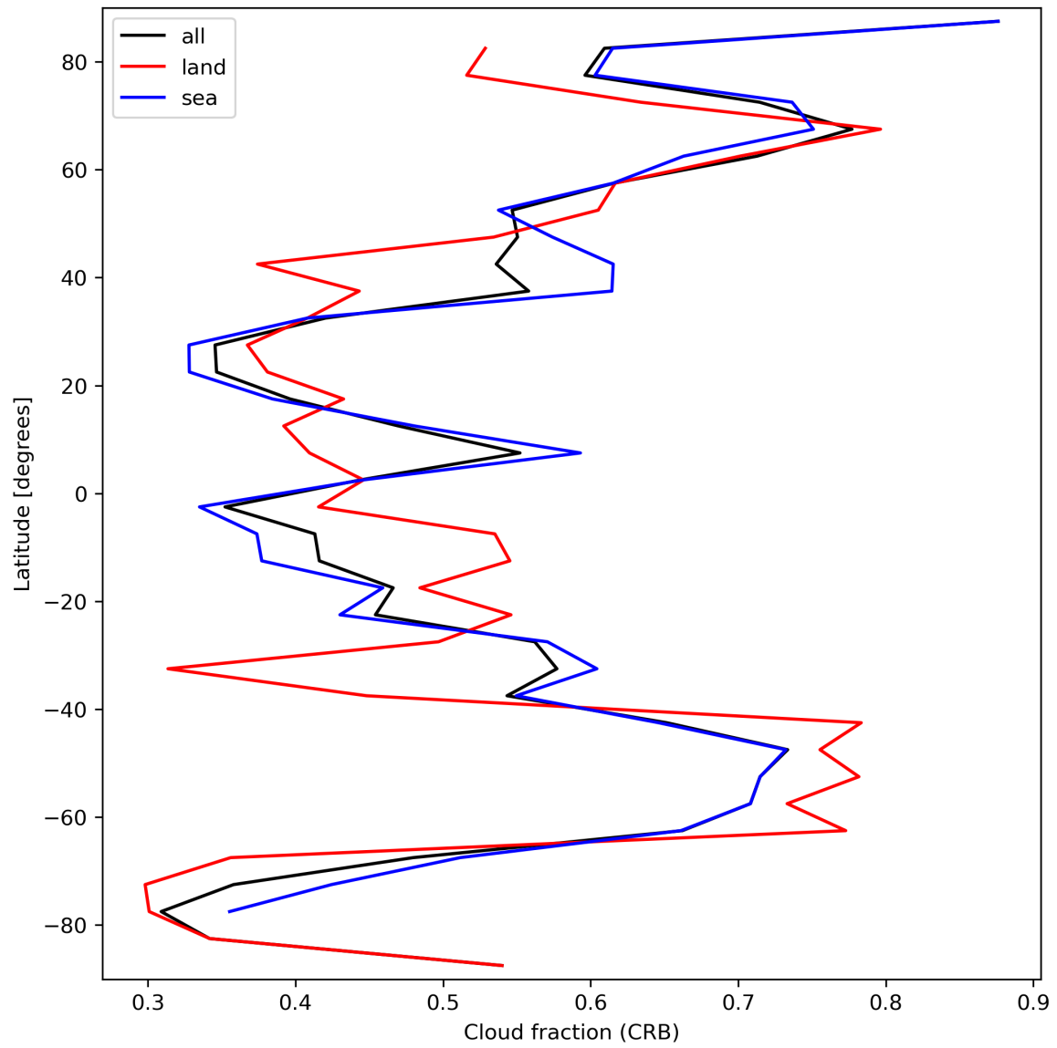
Figure 26: Zonal average of “Cloud fraction (CRB)” for 2023-09-26 to 2023-09-28.
