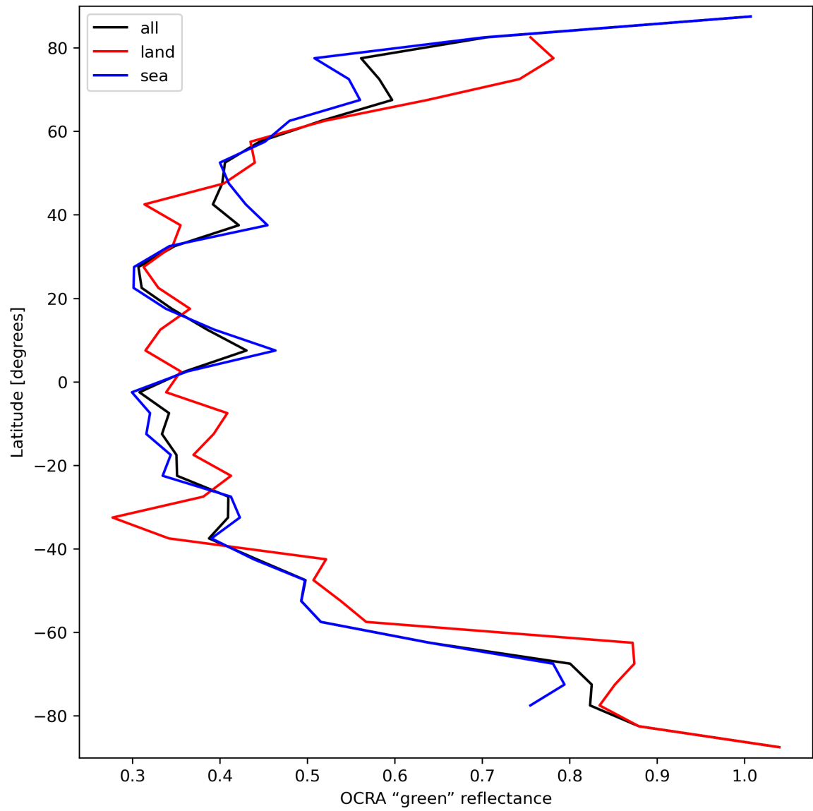
Figure 36: Zonal average of “OCRA “green” reflectance” for 2023-09-26 to 2023-09-28.
