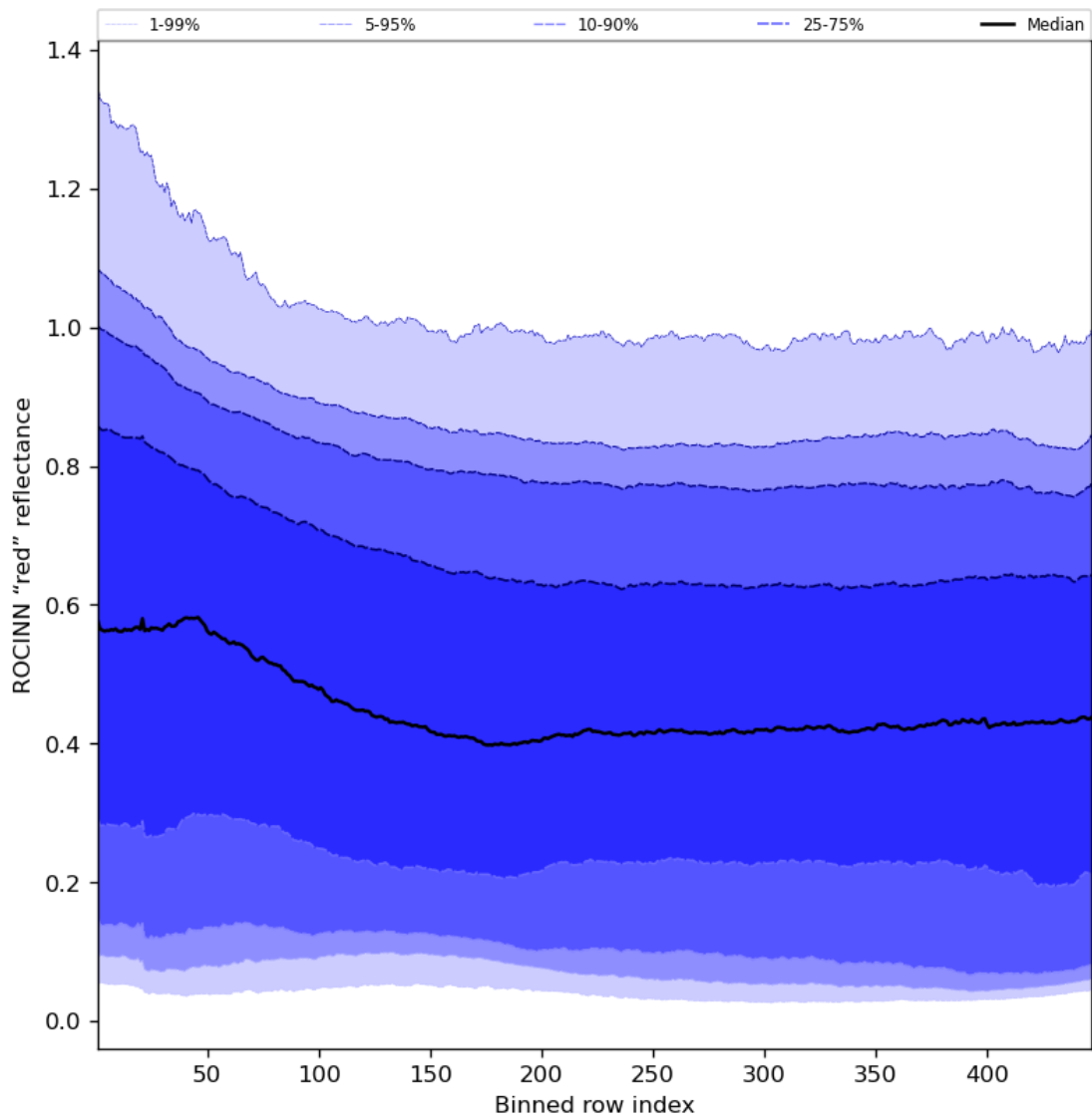
Figure 69: Along track statistics of “ROCINN “red” reflectance” for 2023-09-26 to 2023-09-28
