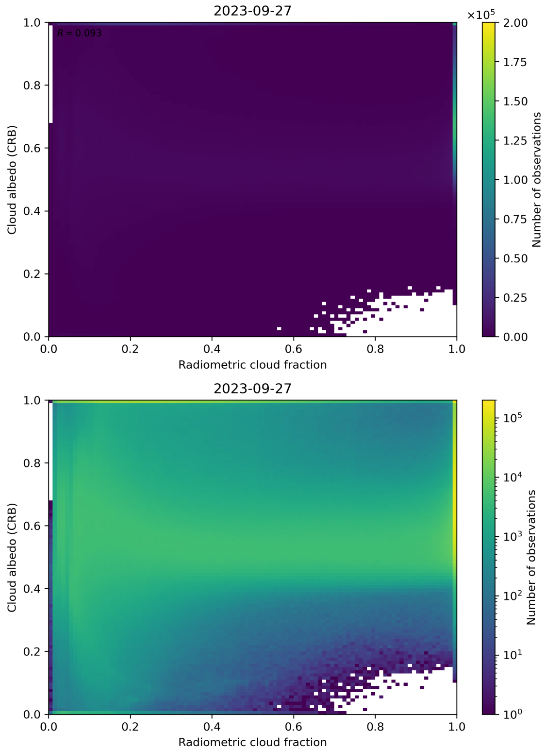
Figure 71: Scatter density plot of “Radiometric cloud fraction” against “Cloud albedo (CRB)” for 2023-09-26 to 2023-09-28.
