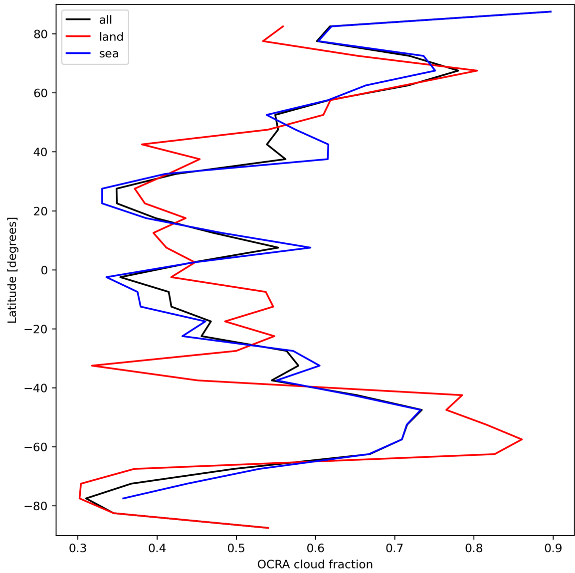
Figure 34: Zonal average of “OCRA cloud fraction” for 2023-09-26 to 2023-09-28.
