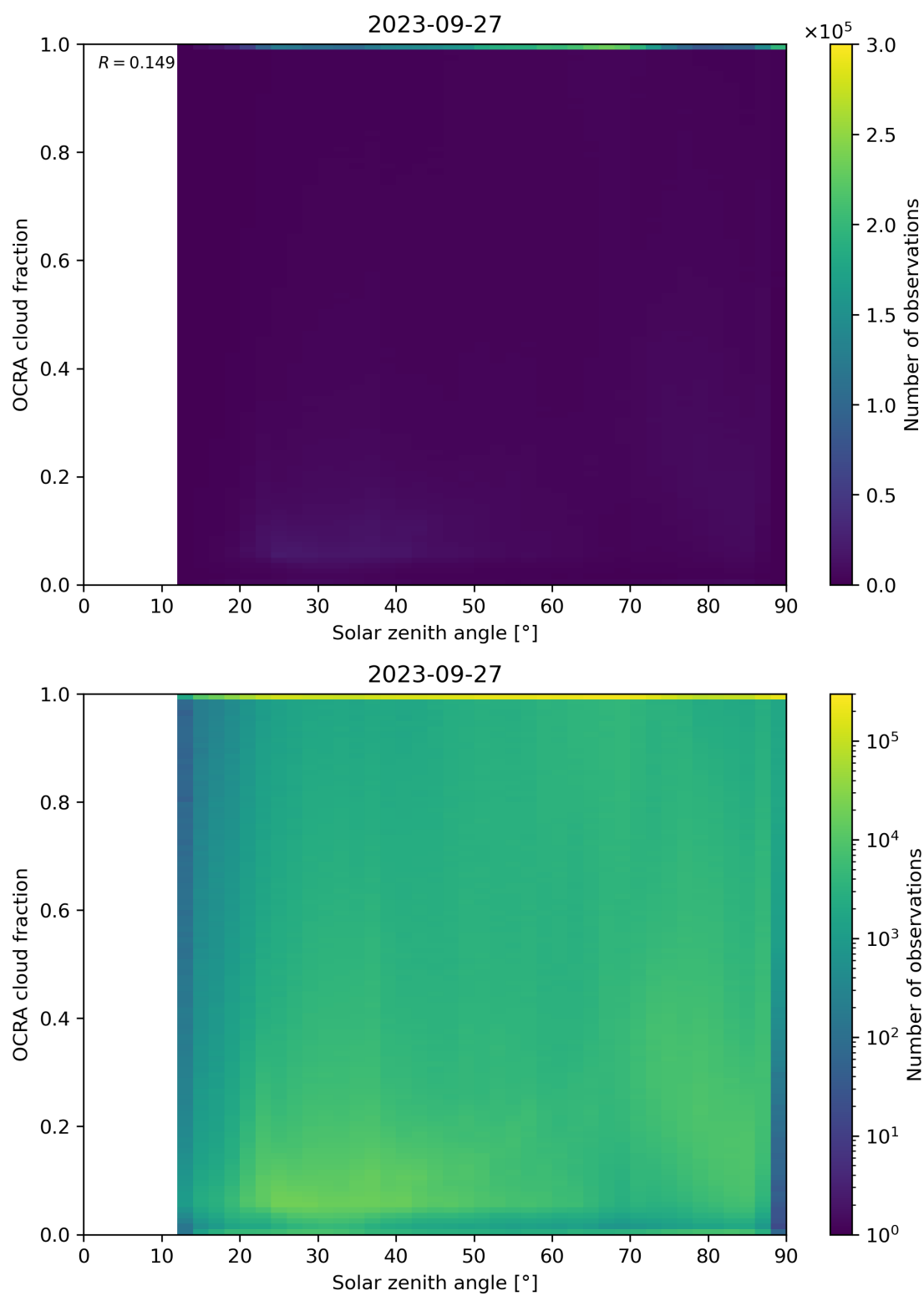
Figure 100: Scatter density plot of “Solar zenith angle” against “OCRA cloud fraction” for 2023-09-26 to 2023-09-28.
