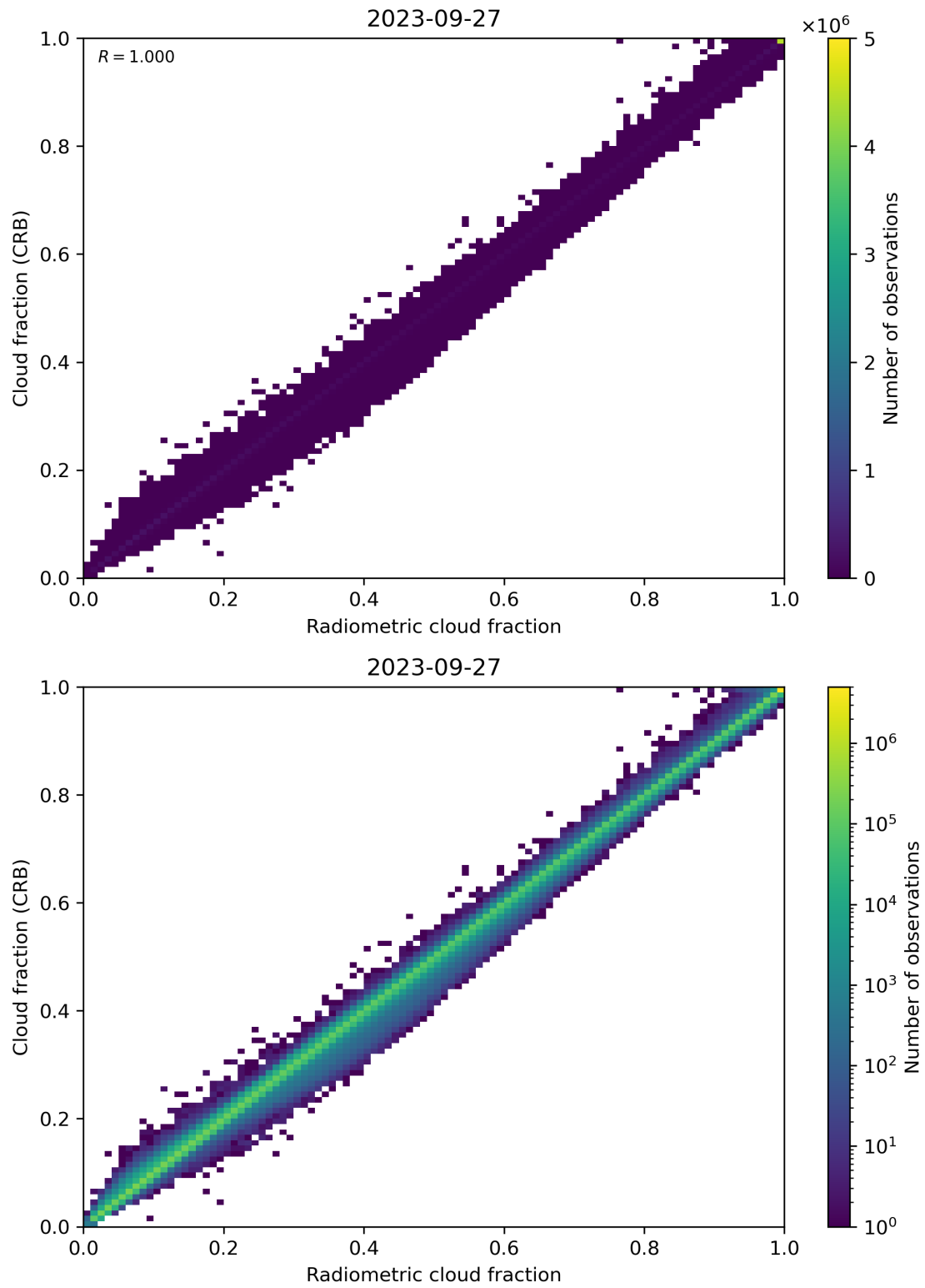
Figure 73: Scatter density plot of “Radiometric cloud fraction” against “Cloud fraction (CRB)” for 2023-09-26 to 2023-09-28.
