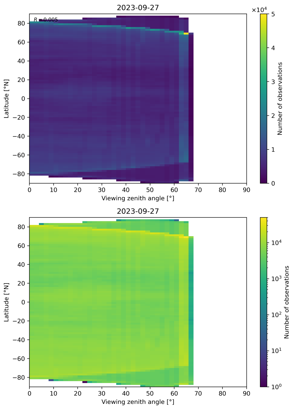
Figure 113: Scatter density plot of “Viewing zenith angle” against “Latitude” for 2023-09-26 to 2023-09-28.
