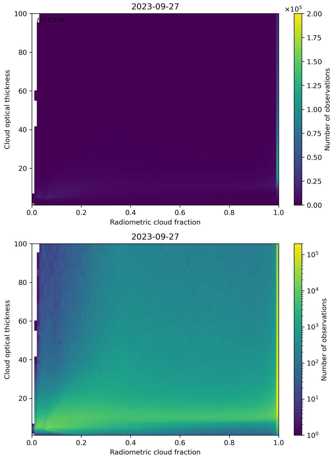
Figure 75: Scatter density plot of “Radiometric cloud fraction” against “Cloud optical thickness” for 2023-09-26 to 2023-09-28.
