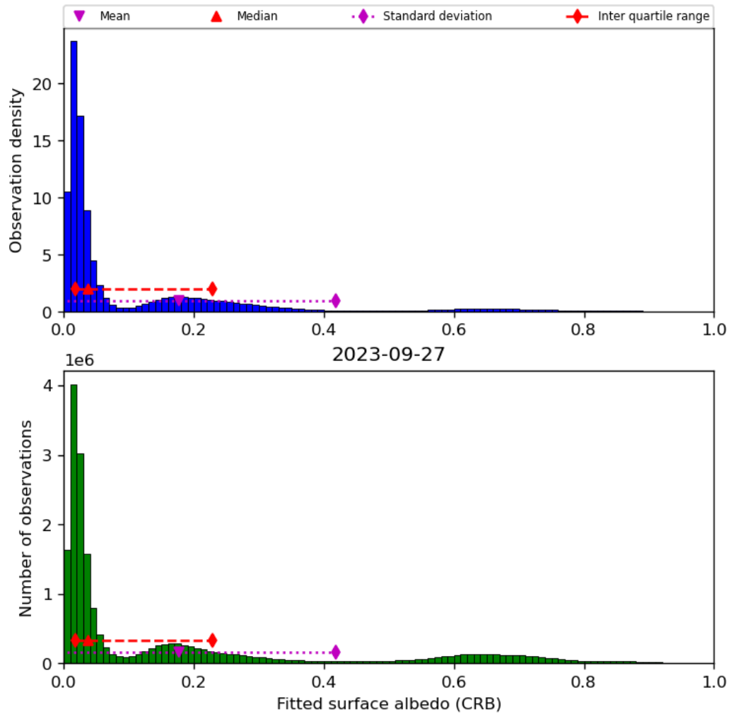
Figure 46: Histogram of “Fitted surface albedo (CRB)” for 2023-09-26 to 2023-09-28
