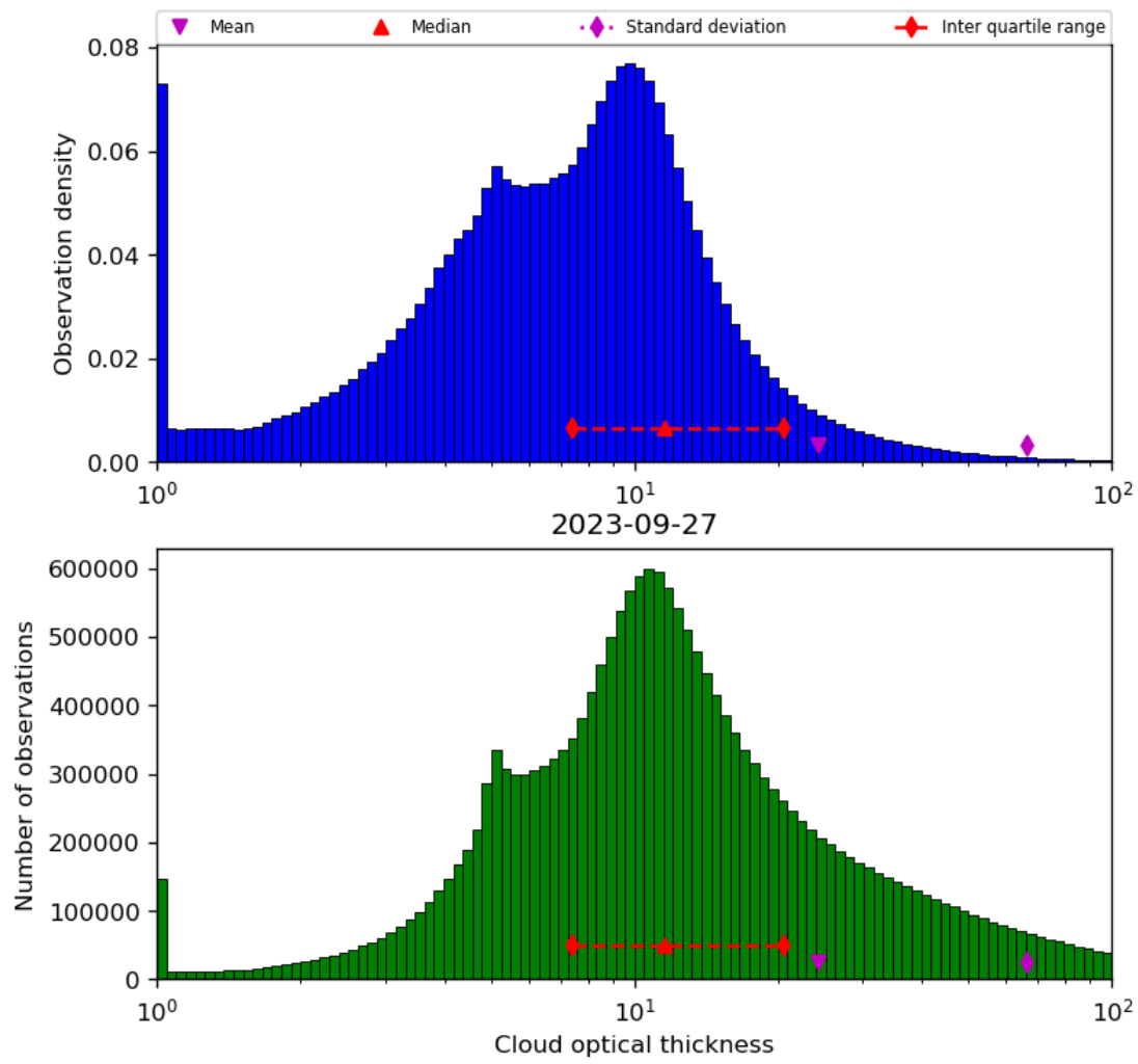
Figure 41: Histogram of “Cloud optical thickness” for 2023-09-26 to 2023-09-28
