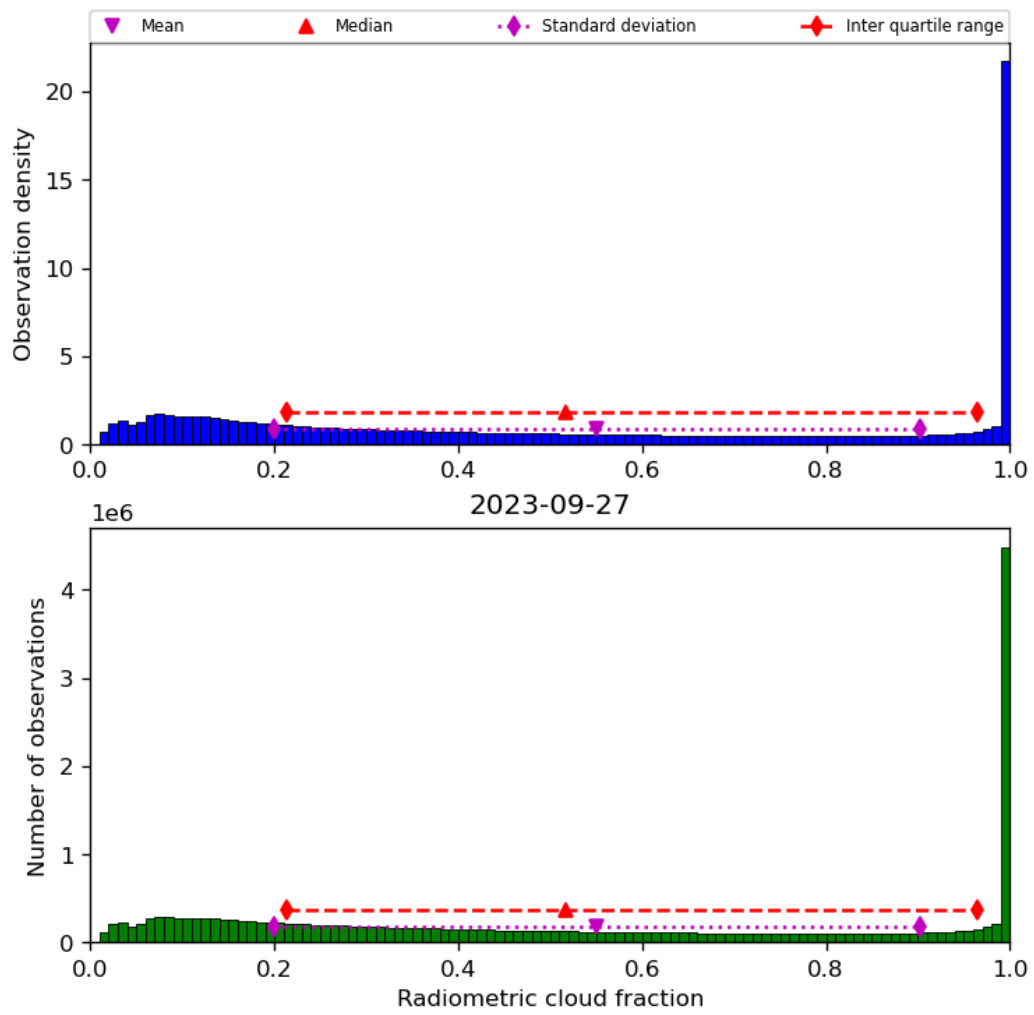
Figure 39: Histogram of “Radiometric cloud fraction” for 2023-09-26 to 2023-09-28
