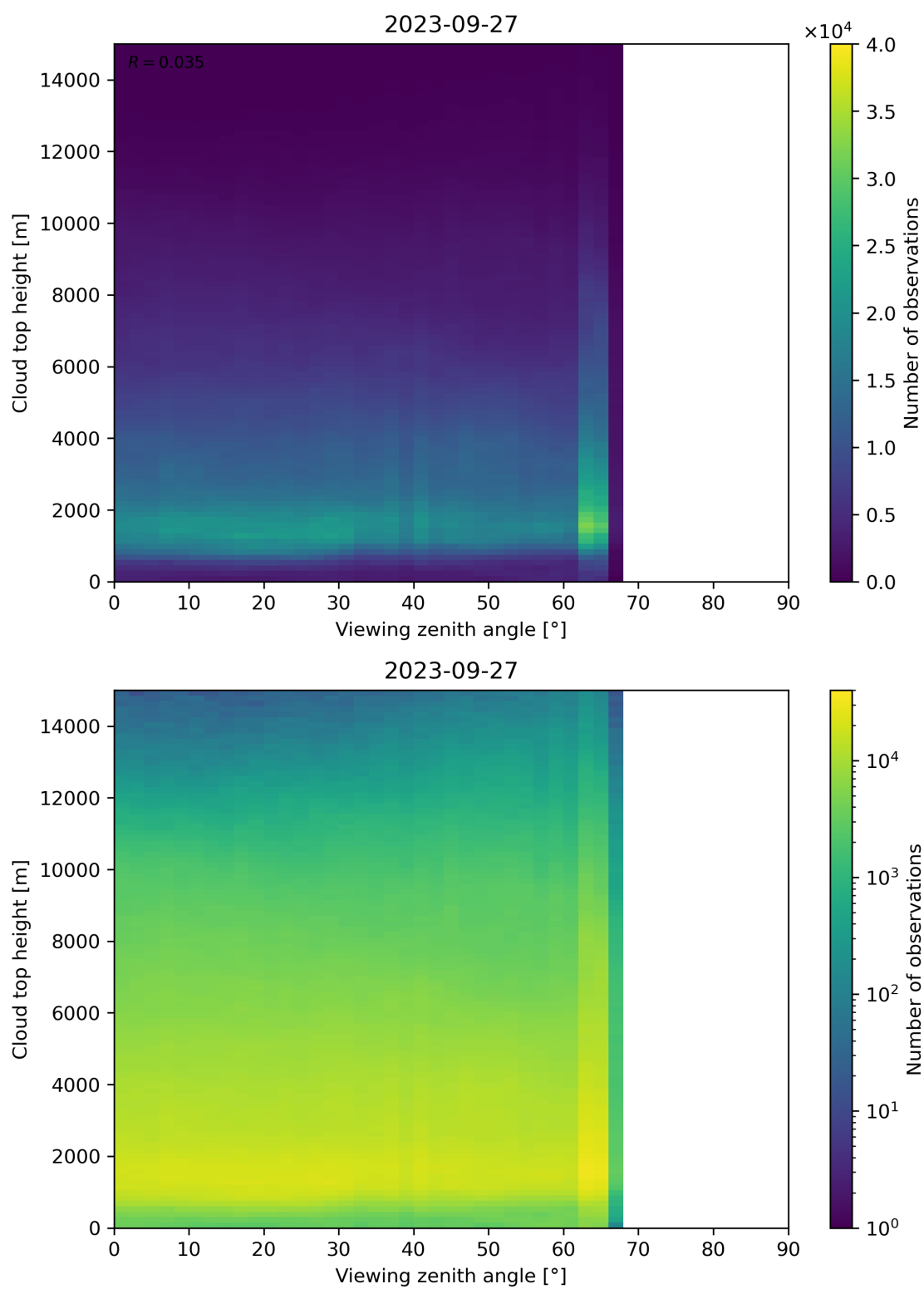
Figure 112: Scatter density plot of “Viewing zenith angle” against “Cloud top height” for 2023-09-26 to 2023-09-28.
