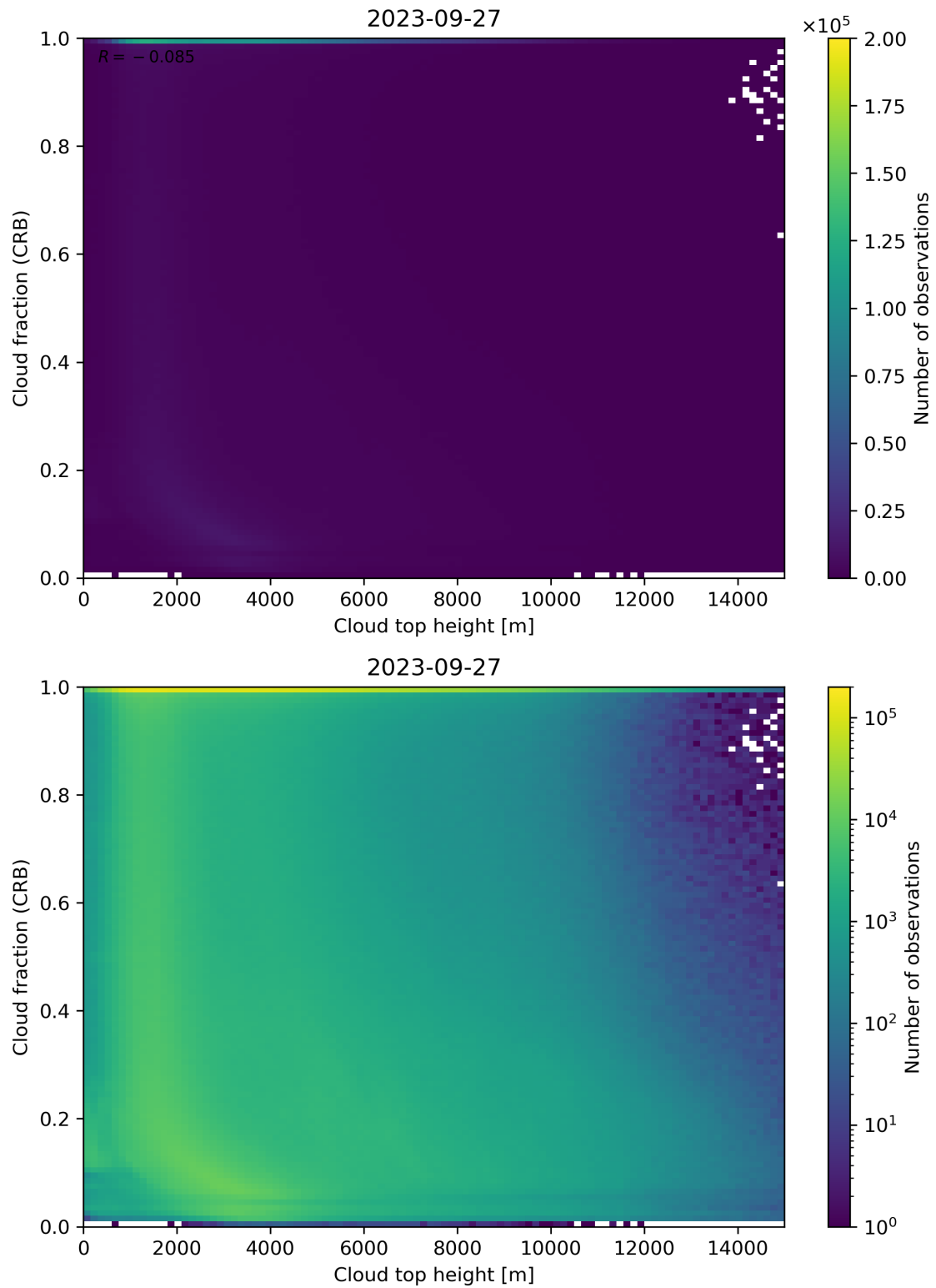
Figure 88: Scatter density plot of “Cloud top height” against “Cloud fraction (CRB)” for 2023-09-26 to 2023-09-28.
