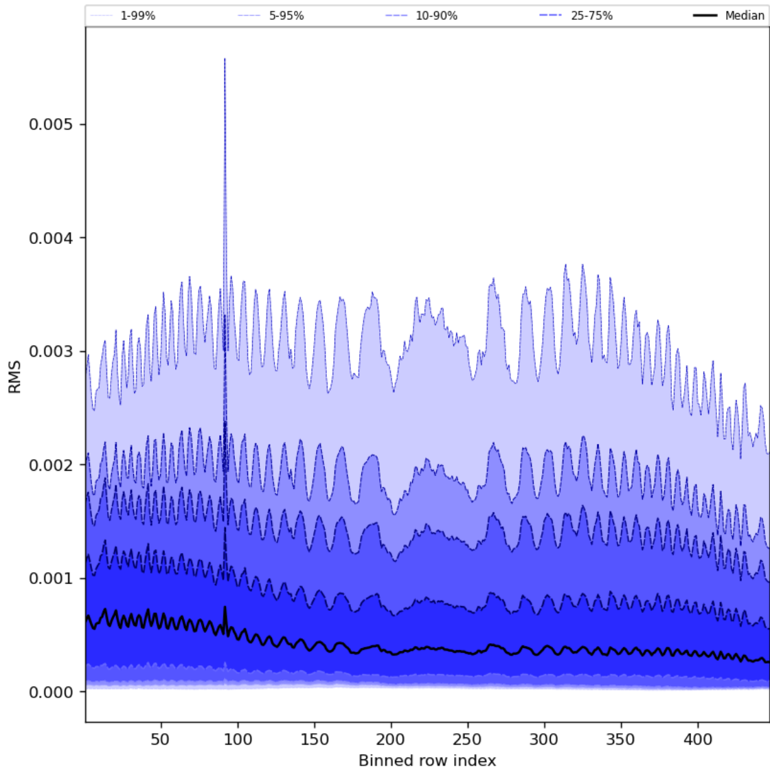
Figure 63: Along track statistics of “RMS” for 2023-09-26 to 2023-09-28
