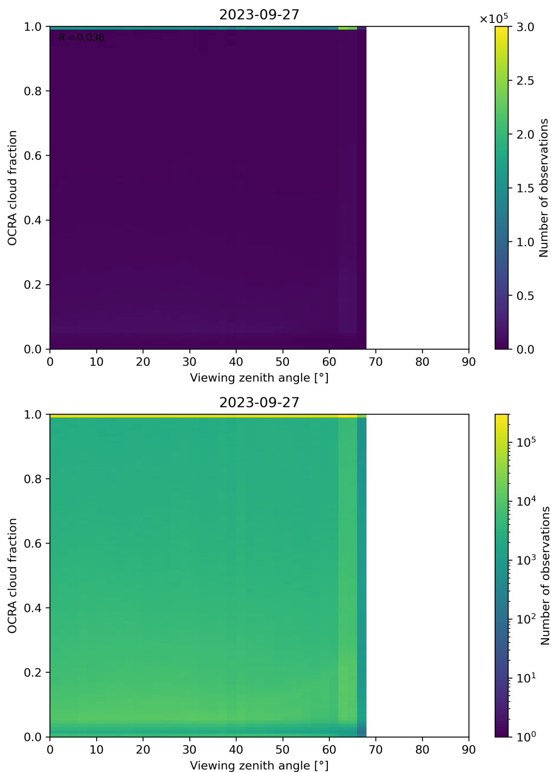
Figure 108: Scatter density plot of “Viewing zenith angle” against “OCRA cloud fraction” for 2023-09-26 to 2023-09-28.
