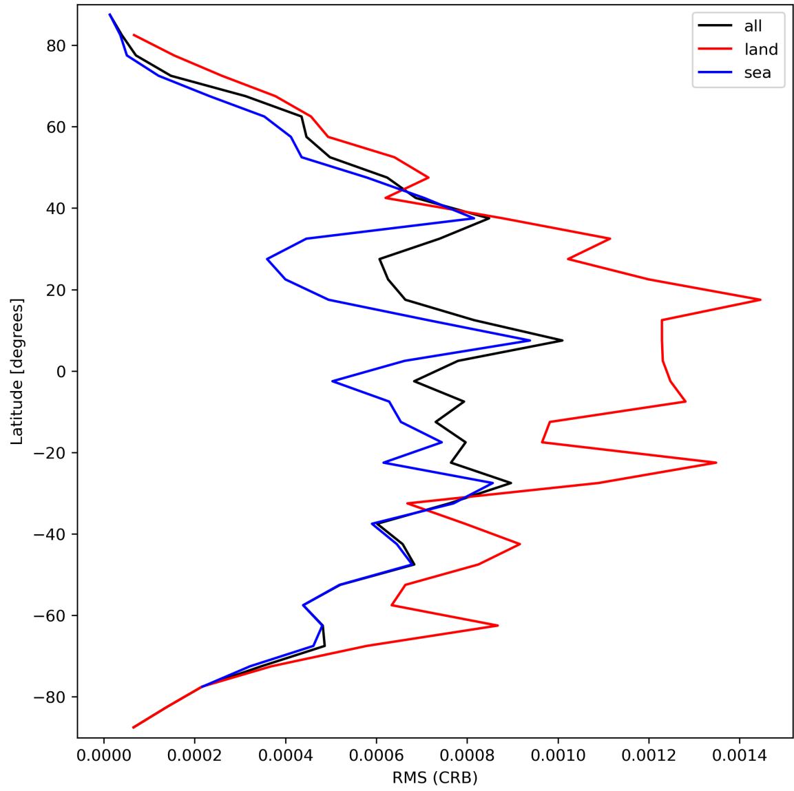
Figure 32: Zonal average of “RMS (CRB)” for 2023-09-26 to 2023-09-28.
