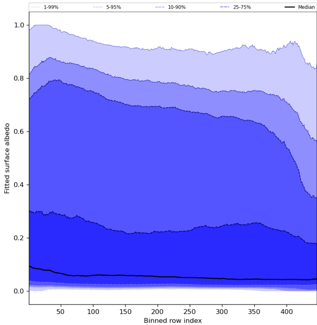
Figure 61: Along track statistics of “Fitted surface albedo” for 2023-09-26 to 2023-09-28
