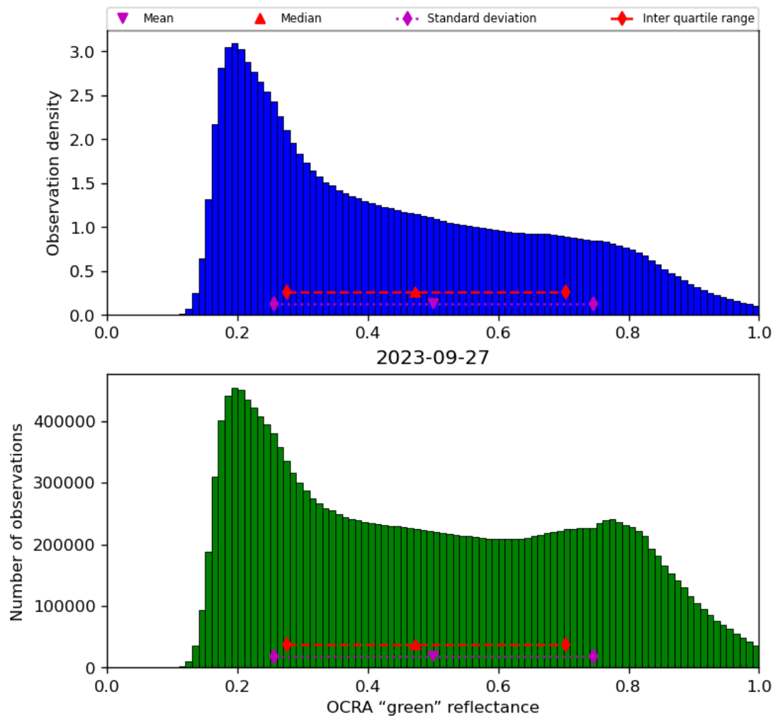
Figure 52: Histogram of “OCRA “green” reflectance” for 2023-09-26 to 2023-09-28
