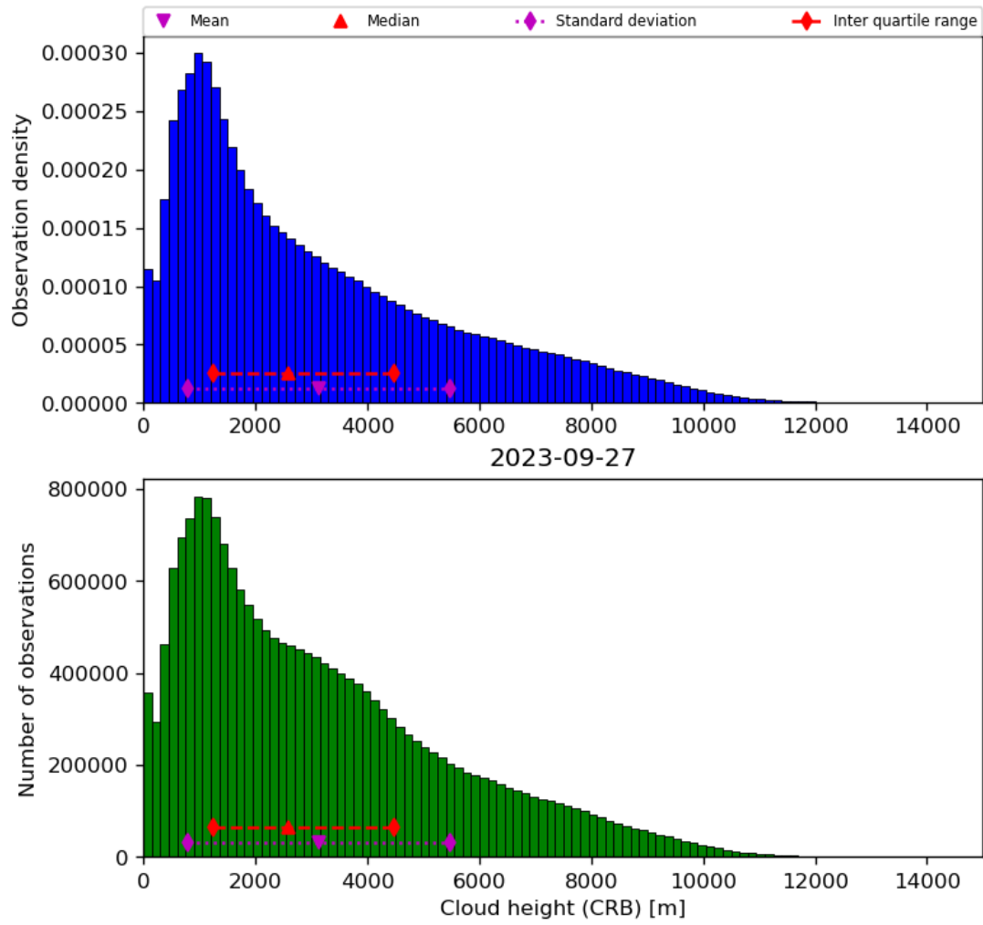
Figure 43: Histogram of “Cloud height (CRB)” for 2023-09-26 to 2023-09-28
