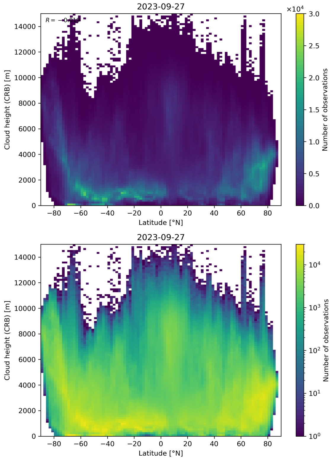
Figure 95: Scatter density plot of “Latitude” against “Cloud height (CRB)” for 2023-09-26 to 2023-09-28.
