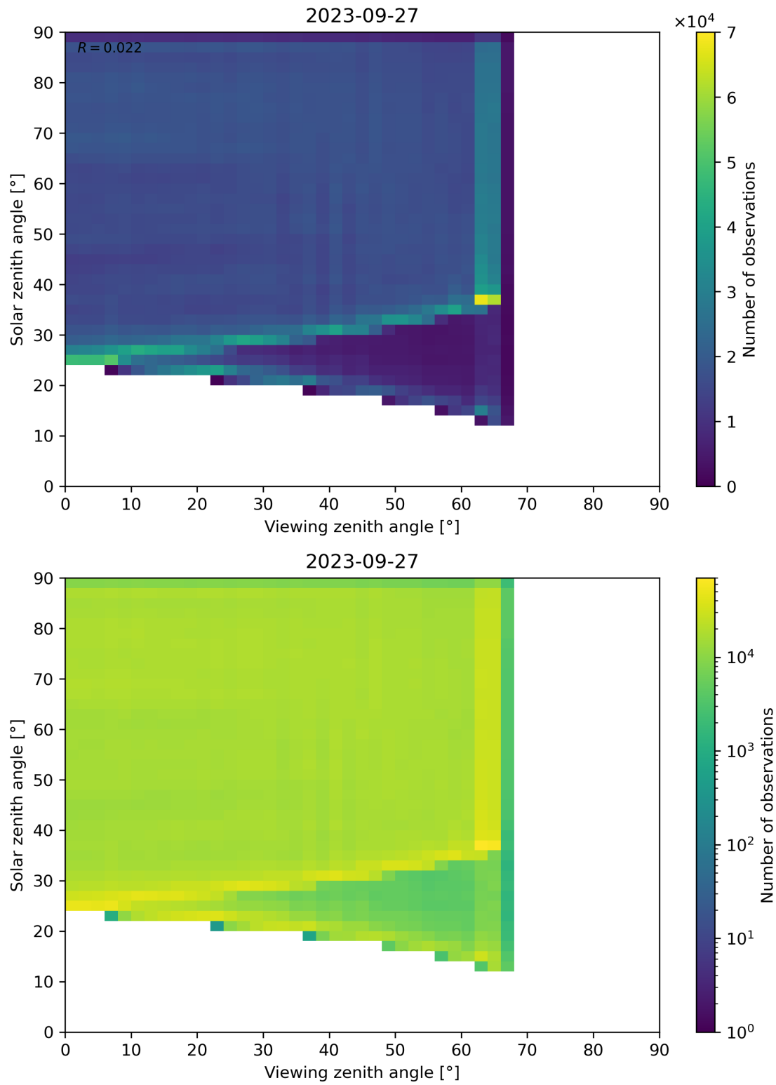
Figure 114: Scatter density plot of “Viewing zenith angle” against “Solar zenith angle” for 2023-09-26 to 2023-09-28.
