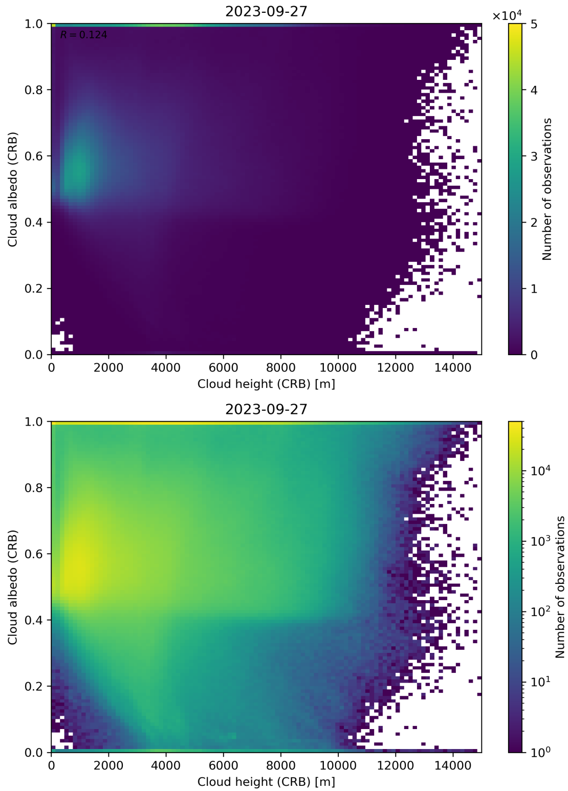
Figure 80: Scatter density plot of “Cloud height (CRB)” against “Cloud albedo (CRB)” for 2023-09-26 to 2023-09-28.
