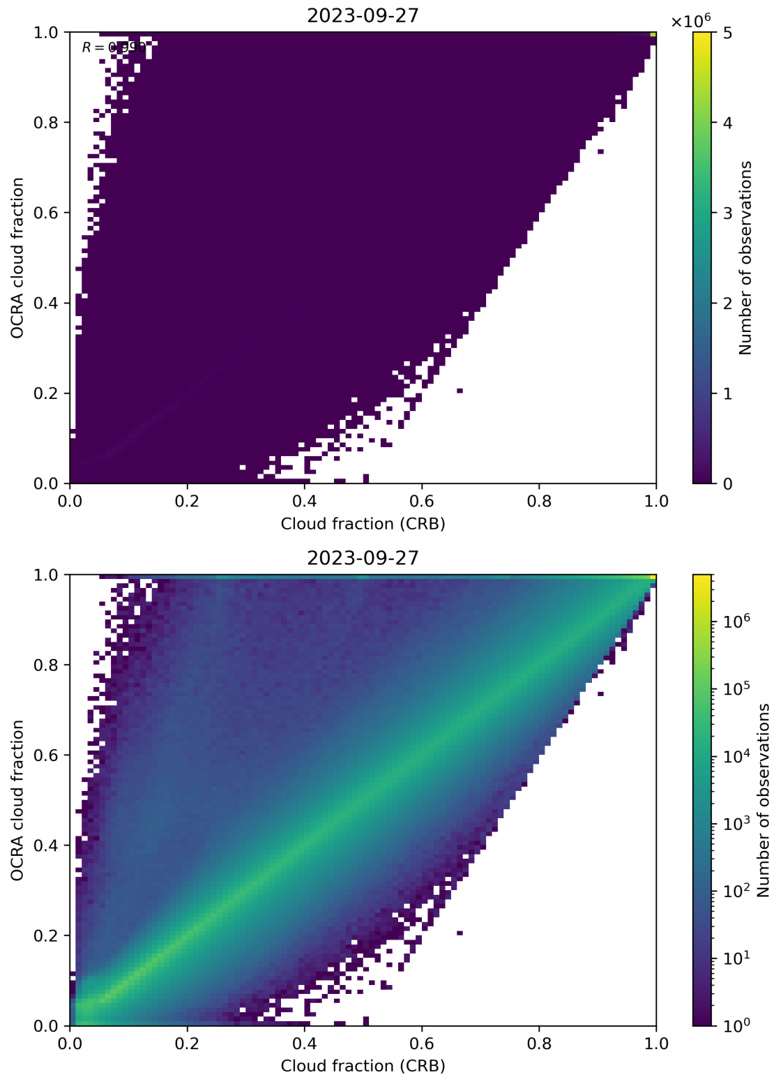
Figure 78: Scatter density plot of “Cloud fraction (CRB)” against “OCRA cloud fraction” for 2023-09-26 to 2023-09-28.
