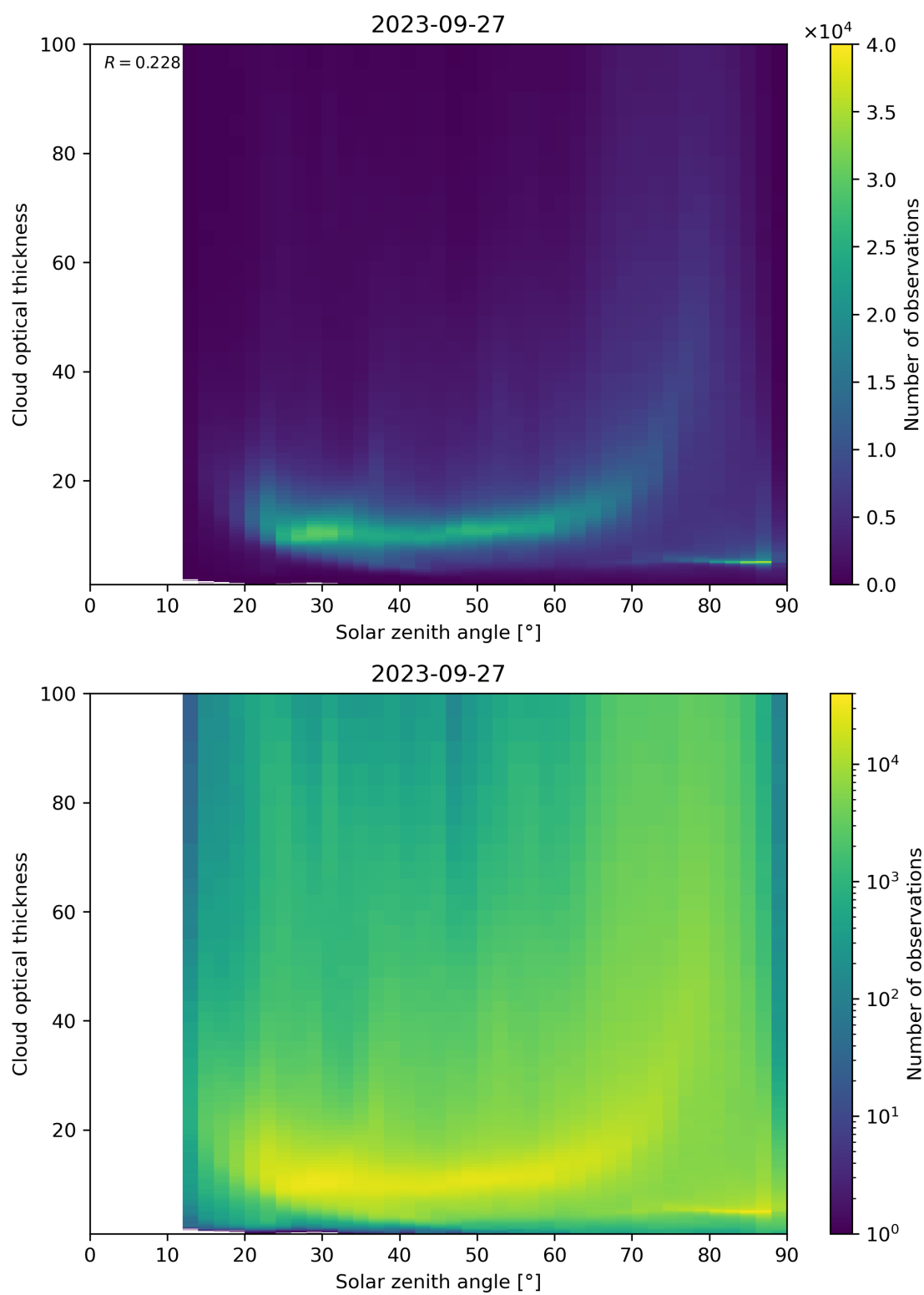
Figure 103: Scatter density plot of “Solar zenith angle” against “Cloud optical thickness” for 2023-09-26 to 2023-09-28.
