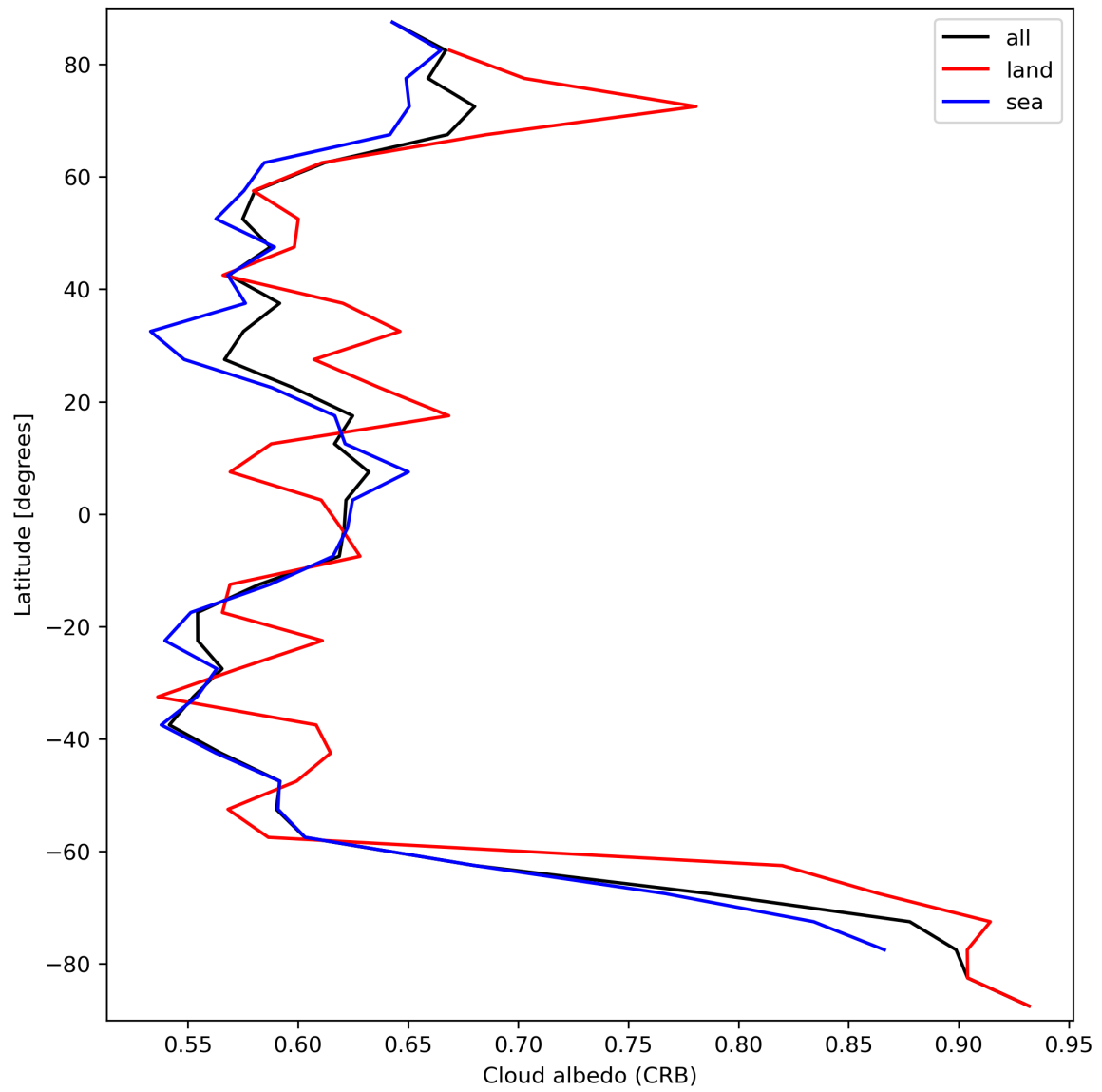
Figure 28: Zonal average of “Cloud albedo (CRB)” for 2023-09-26 to 2023-09-28.
