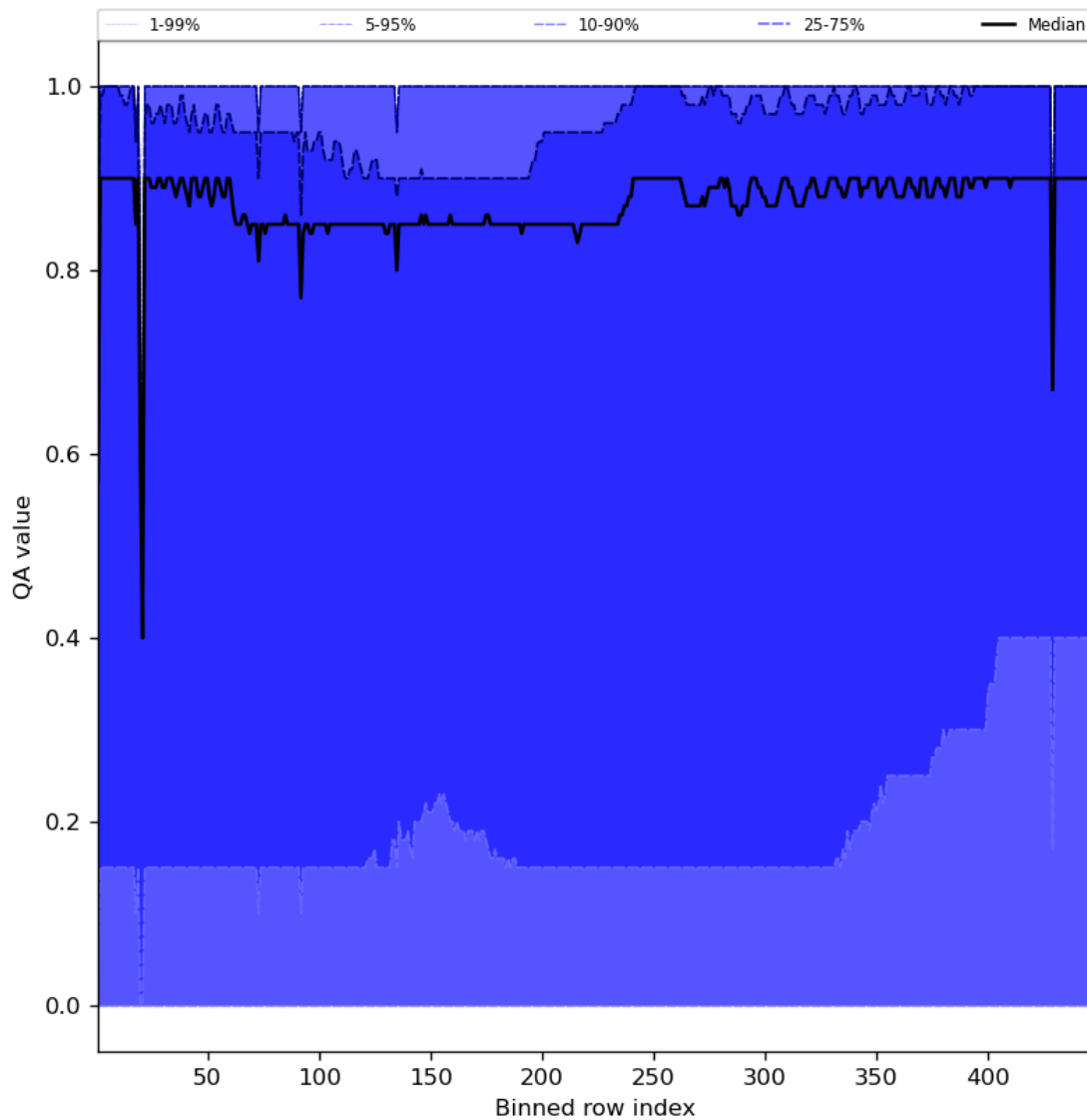
Figure 54: Along track statistics of “QA value” for 2023-09-26 to 2023-09-28
