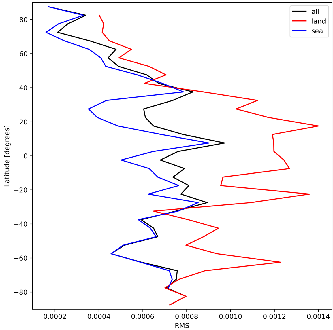
Figure 31: Zonal average of “RMS” for 2023-09-26 to 2023-09-28.
