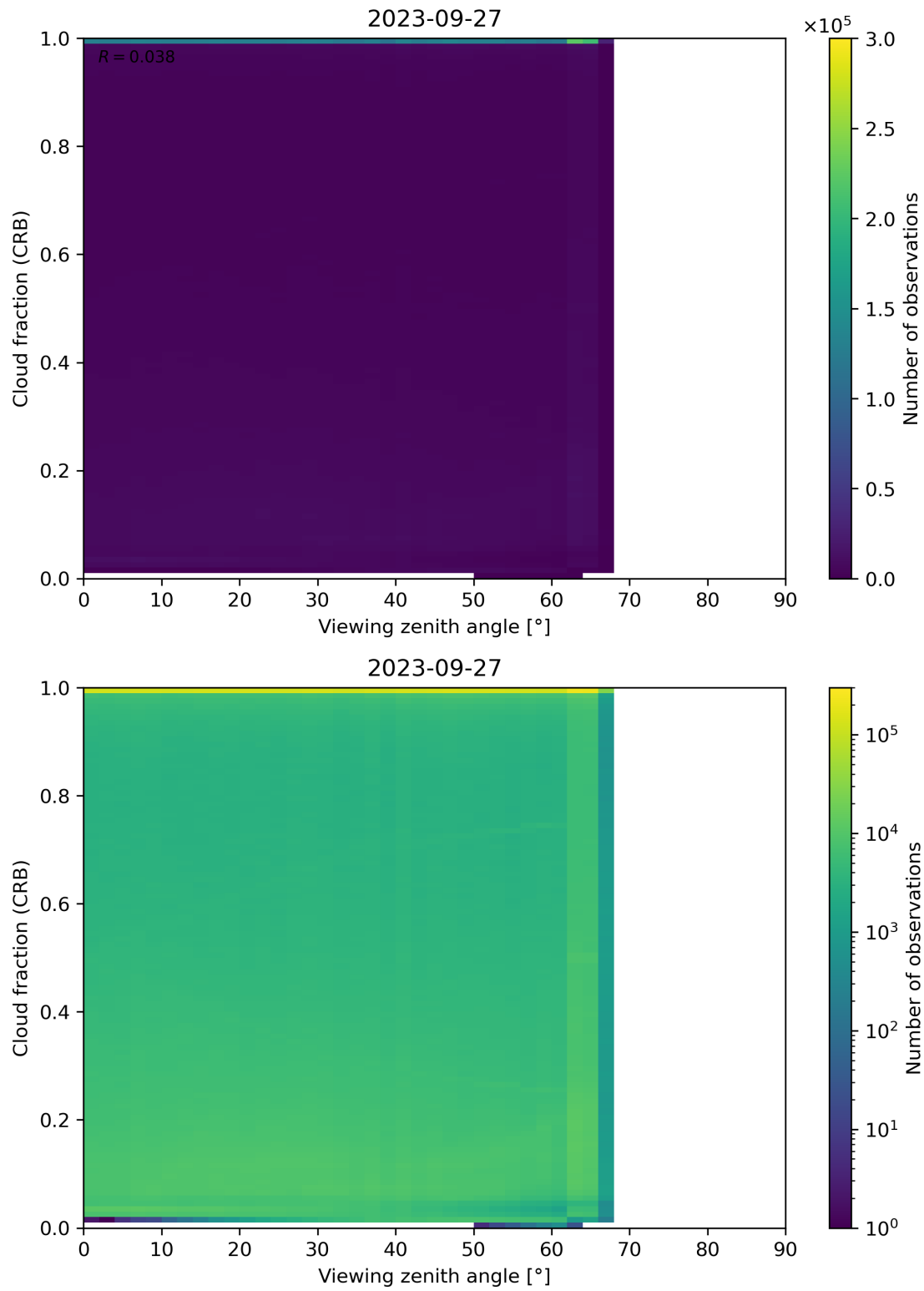
Figure 109: Scatter density plot of “Viewing zenith angle” against “Cloud fraction (CRB)” for 2023-09-26 to 2023-09-28.
