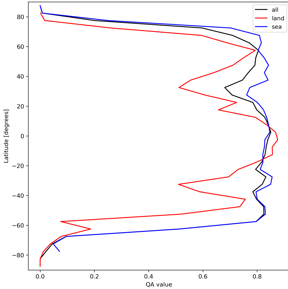
Figure 22: Zonal average of “QA value” for 2023-09-26 to 2023-09-28.
