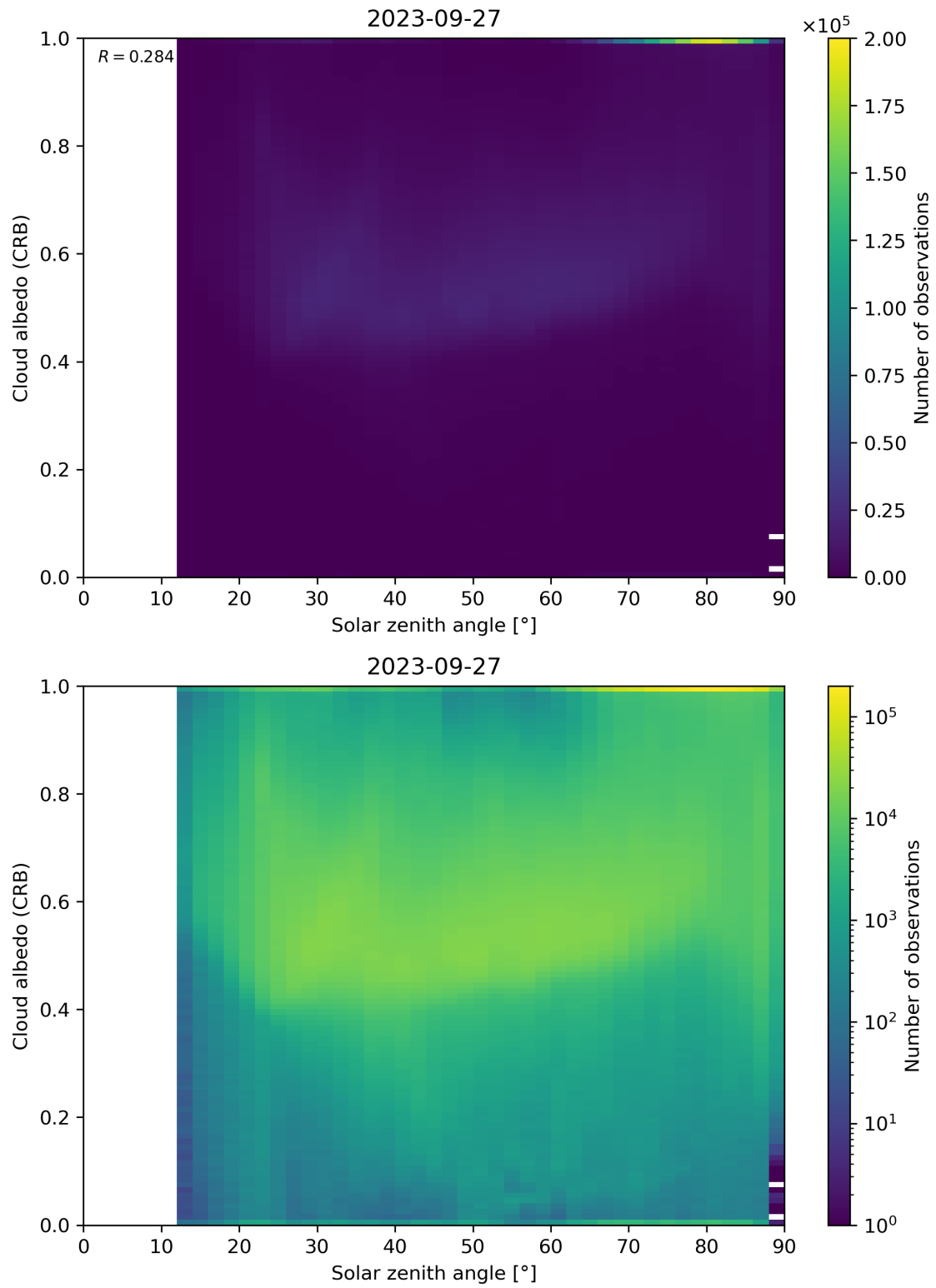
Figure 98: Scatter density plot of “Solar zenith angle” against “Cloud albedo (CRB)” for 2023-09-26 to 2023-09-28.
