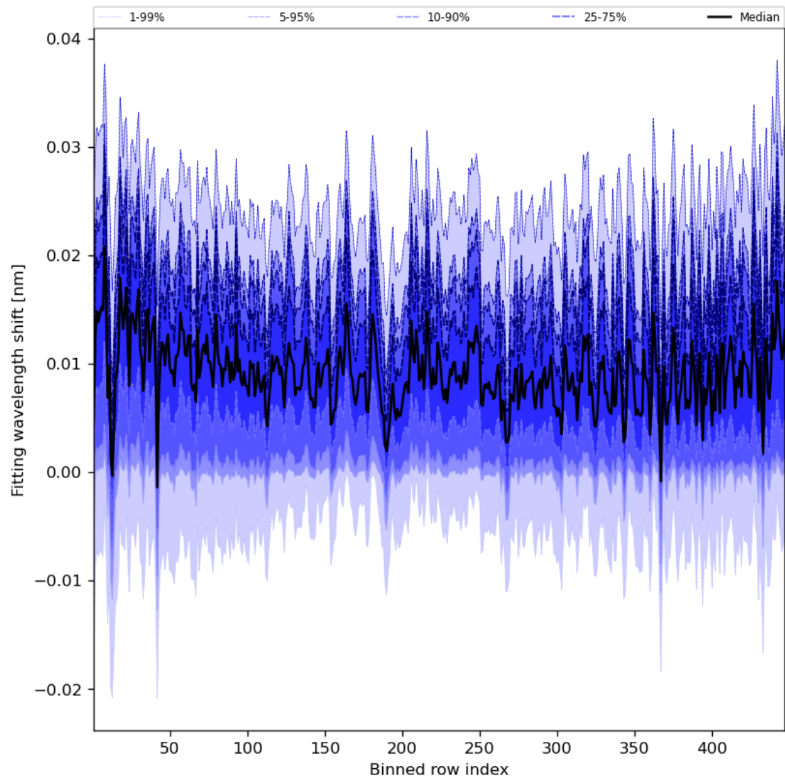
Figure 65: Along track statistics of “Fitting wavelength shift” for 2023-09-26 to 2023-09-28
