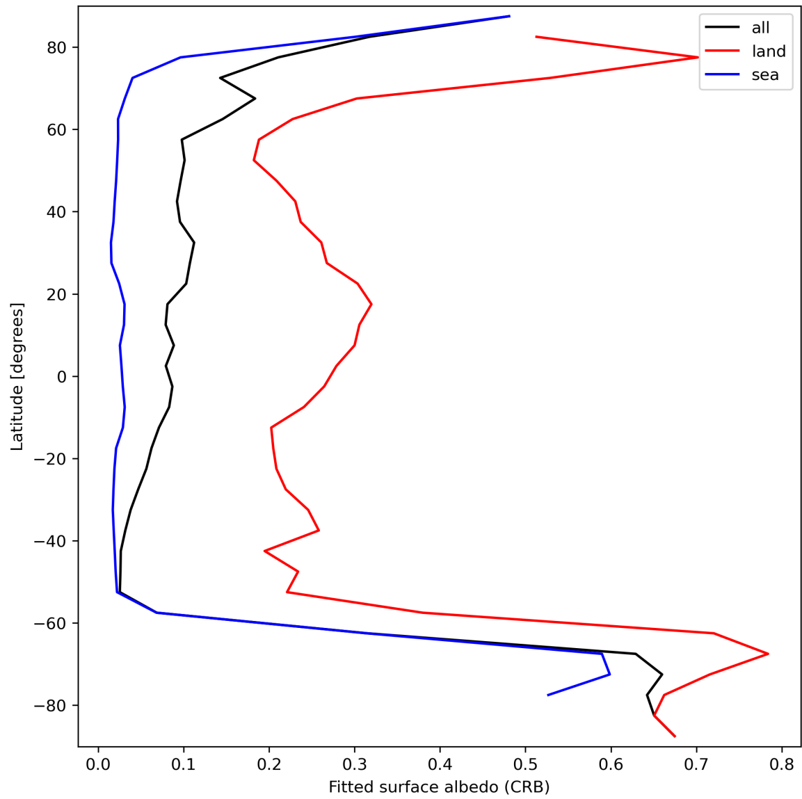
Figure 30: Zonal average of “Fitted surface albedo (CRB)” for 2023-09-26 to 2023-09-28.
