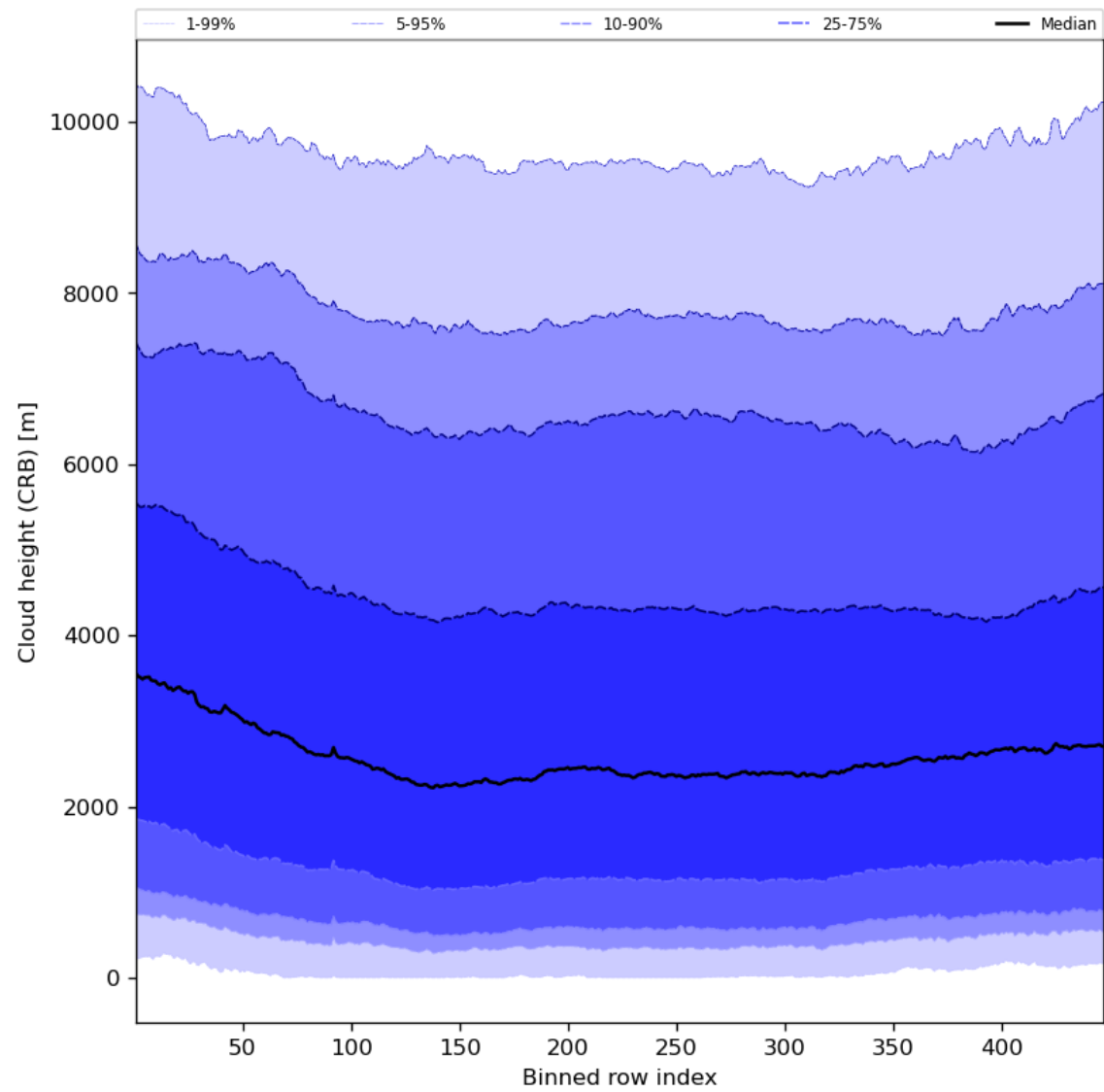
Figure 59: Along track statistics of “Cloud height (CRB)” for 2023-09-26 to 2023-09-28
