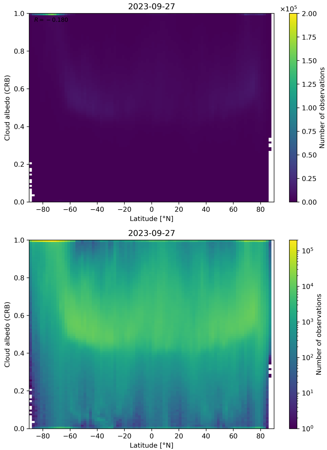
Figure 91: Scatter density plot of “Latitude” against “Cloud albedo (CRB)” for 2023-09-26 to 2023-09-28.
