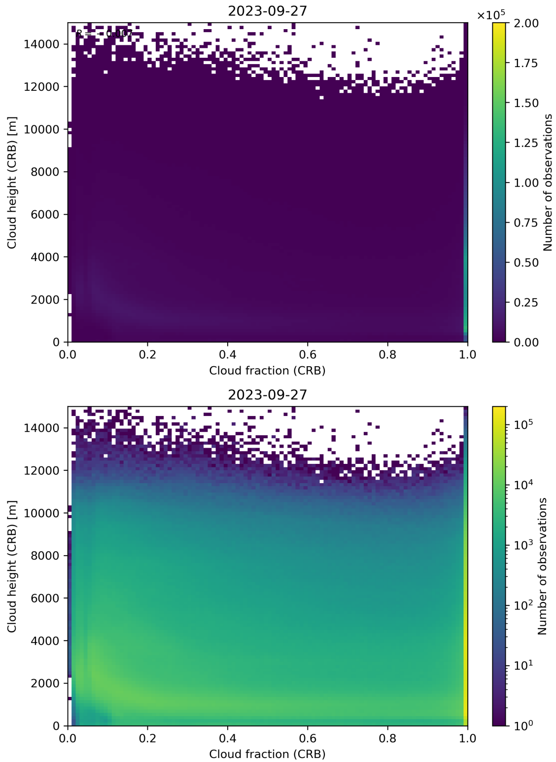
Figure 79: Scatter density plot of “Cloud fraction (CRB)” against “Cloud height (CRB)” for 2023-09-26 to 2023-09-28.
