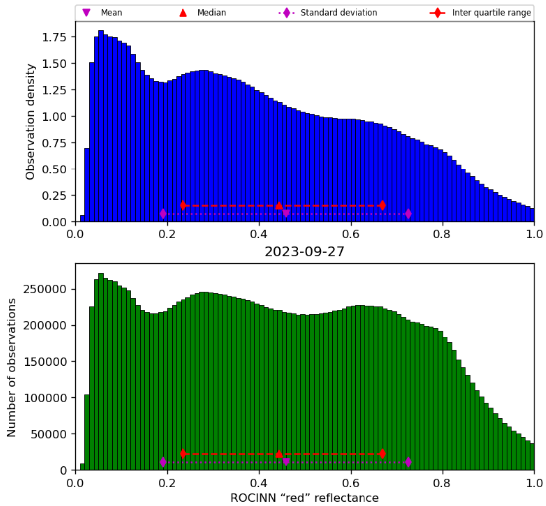
Figure 53: Histogram of “ROCINN “red” reflectance” for 2023-09-26 to 2023-09-28
