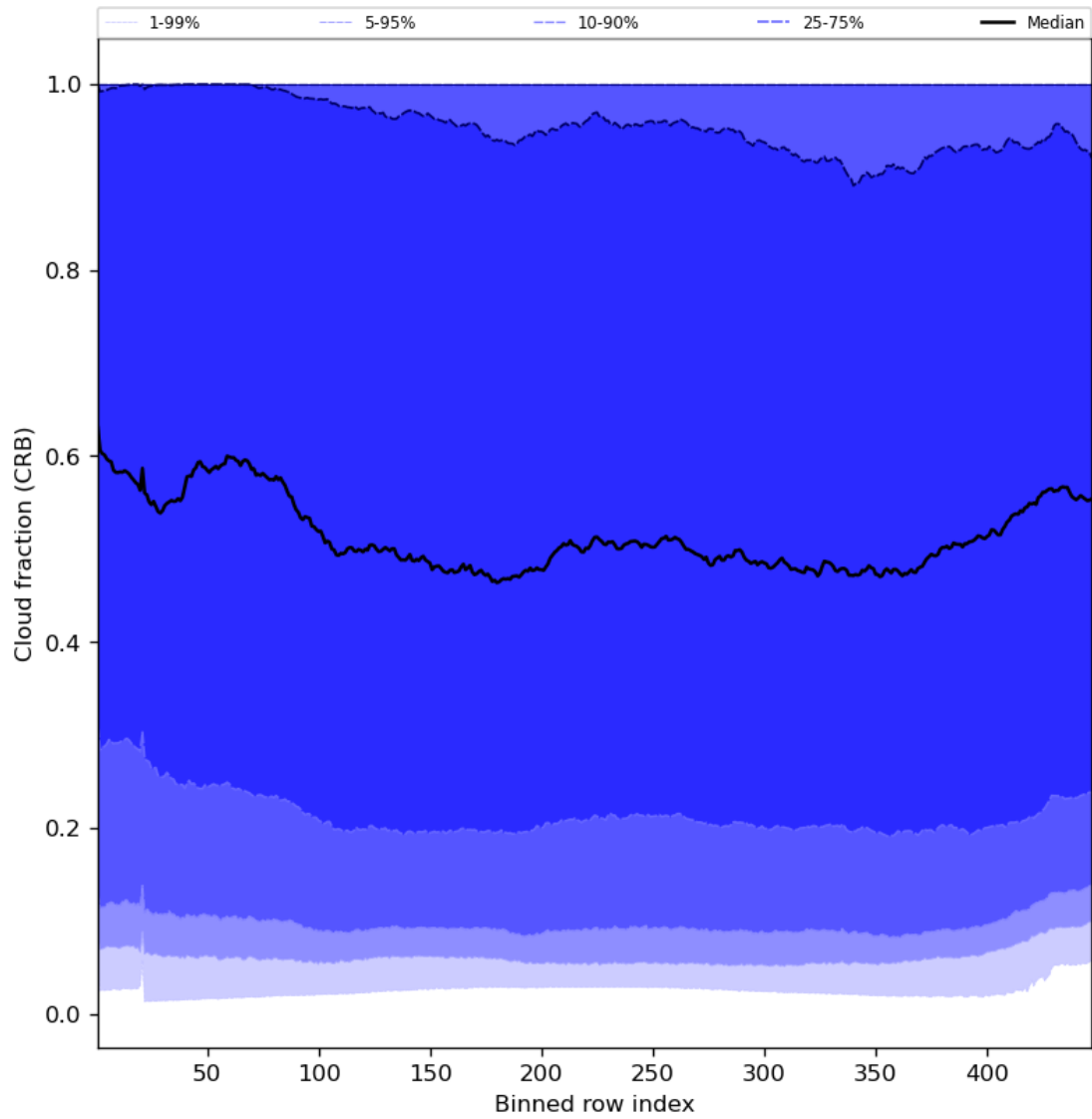
Figure 58: Along track statistics of “Cloud fraction (CRB)” for 2023-09-26 to 2023-09-28
