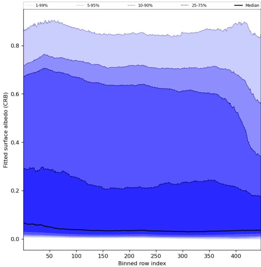
Figure 62: Along track statistics of “Fitted surface albedo (CRB)” for 2023-09-26 to 2023-09-28
