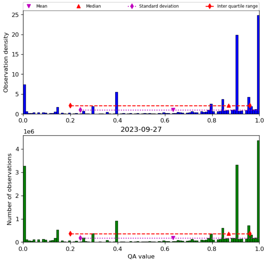
Figure 38: Histogram of “QA value” for 2023-09-26 to 2023-09-28
