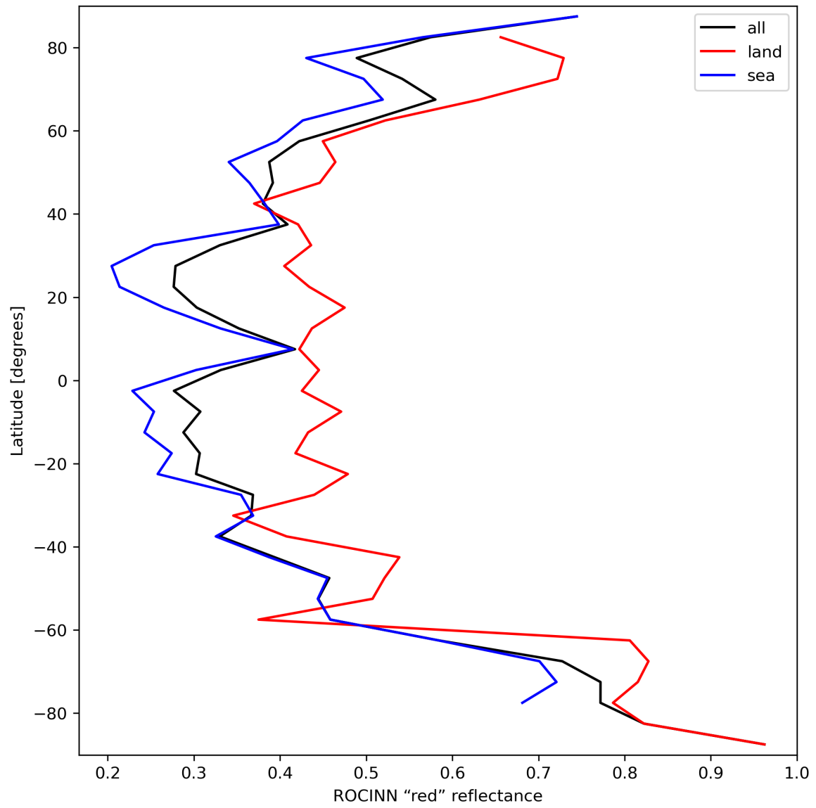
Figure 37: Zonal average of “ROCINN “red” reflectance” for 2023-09-26 to 2023-09-28.
