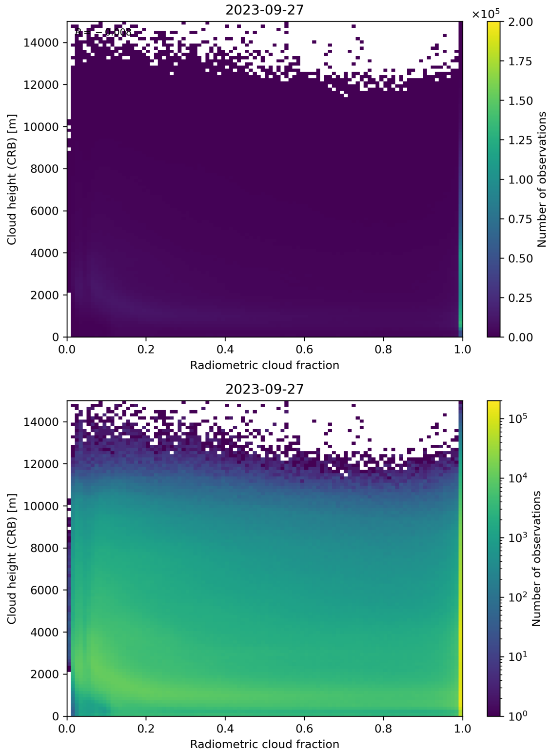
Figure 74: Scatter density plot of “Radiometric cloud fraction” against “Cloud height (CRB)” for 2023-09-26 to 2023-09-28.
