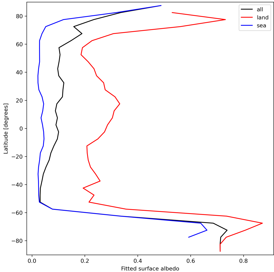
Figure 29: Zonal average of “Fitted surface albedo” for 2023-09-26 to 2023-09-28.
