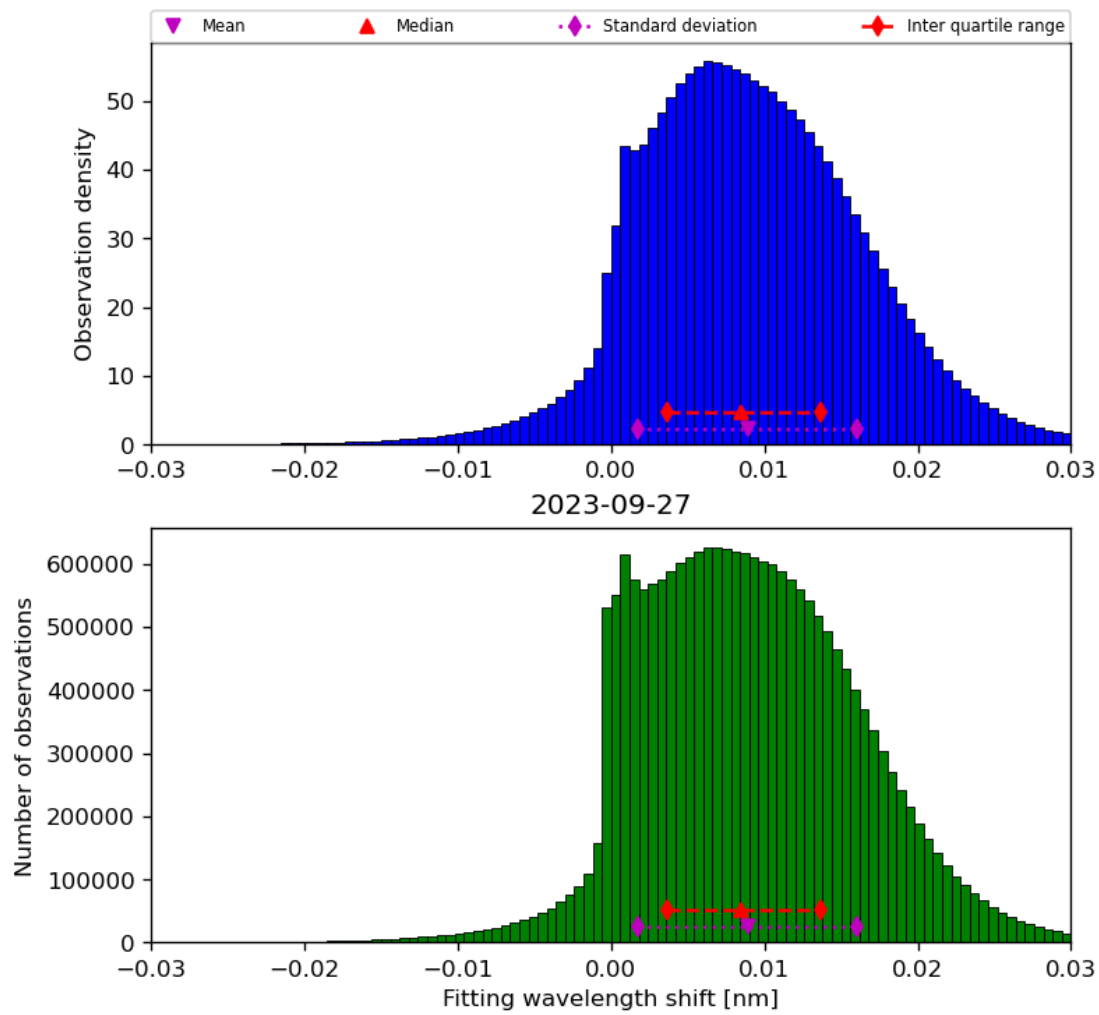
Figure 49: Histogram of “Fitting wavelength shift” for 2023-09-26 to 2023-09-28
