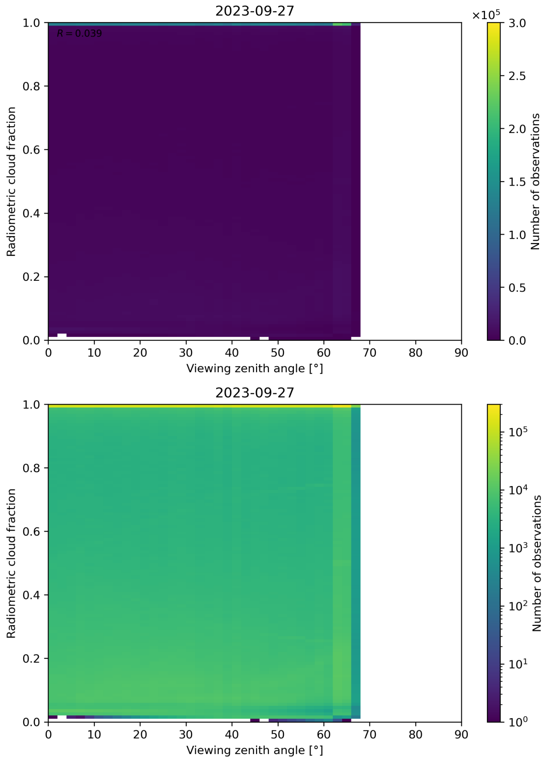
Figure 107: Scatter density plot of “Viewing zenith angle” against “Radiometric cloud fraction” for 2023-09-26 to 2023-09-28.
