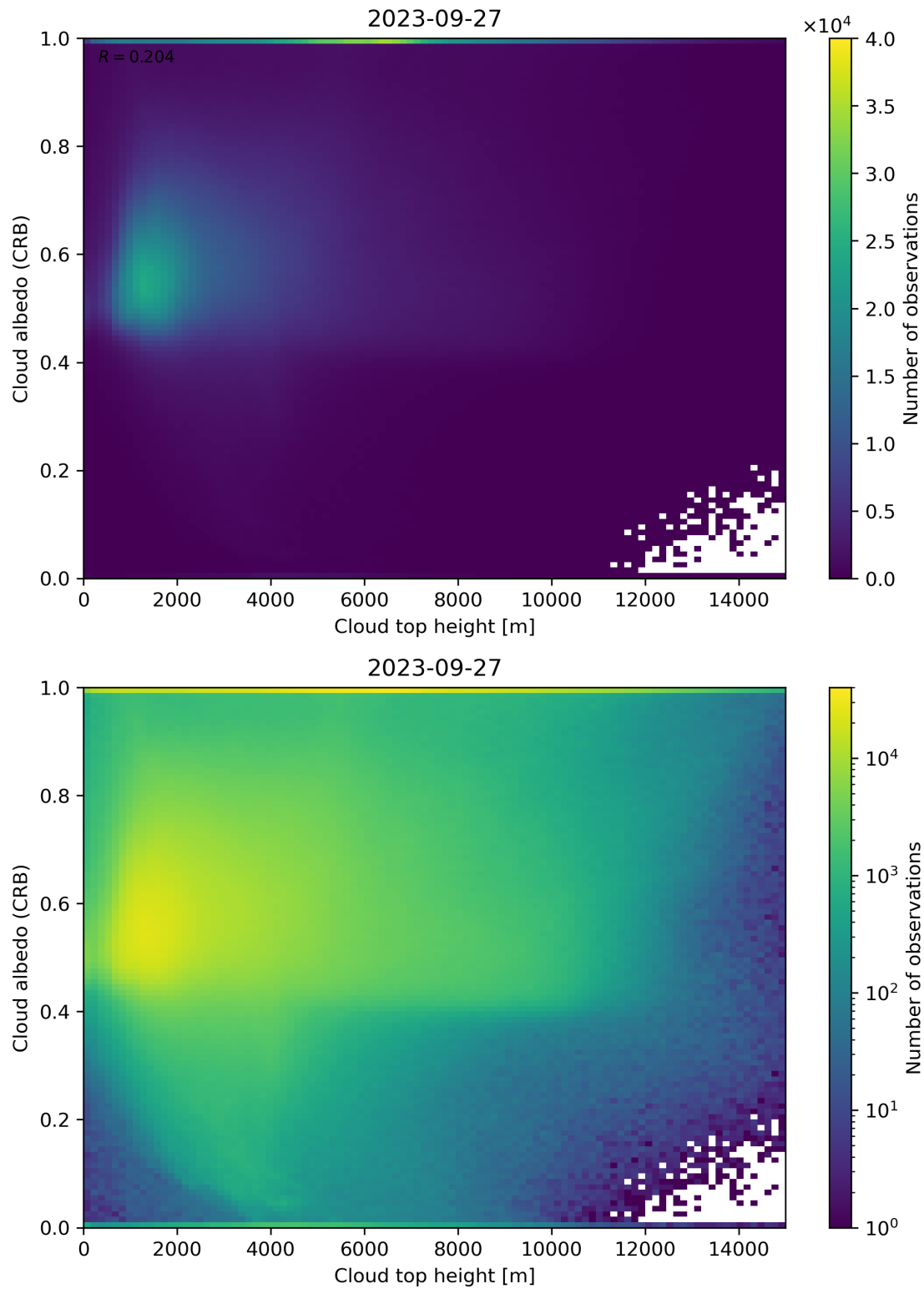
Figure 86: Scatter density plot of “Cloud top height” against “Cloud albedo (CRB)” for 2023-09-26 to 2023-09-28.
