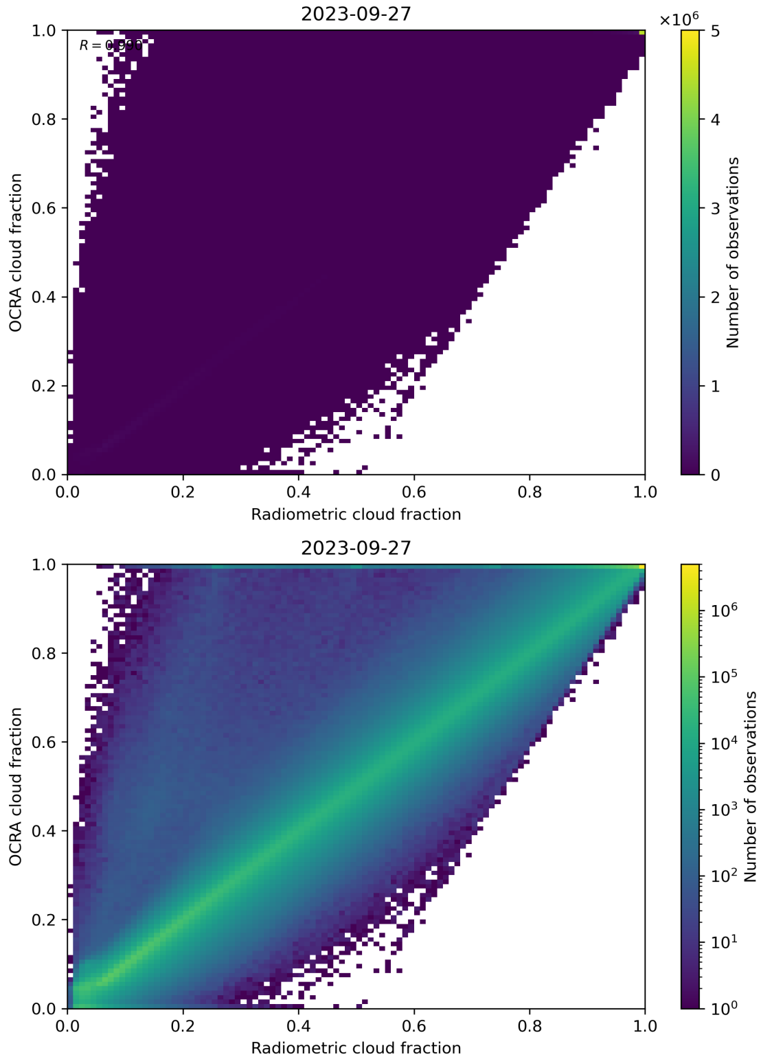
Figure 72: Scatter density plot of “Radiometric cloud fraction” against “OCRA cloud fraction” for 2023-09-26 to 2023-09-28.
