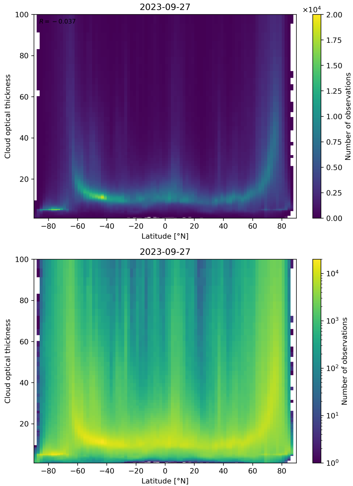
Figure 96: Scatter density plot of “Latitude” against “Cloud optical thickness” for 2023-09-26 to 2023-09-28.
