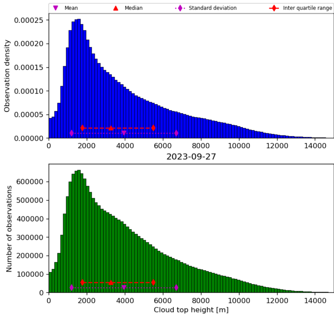
Figure 40: Histogram of “Cloud top height” for 2023-09-26 to 2023-09-28
