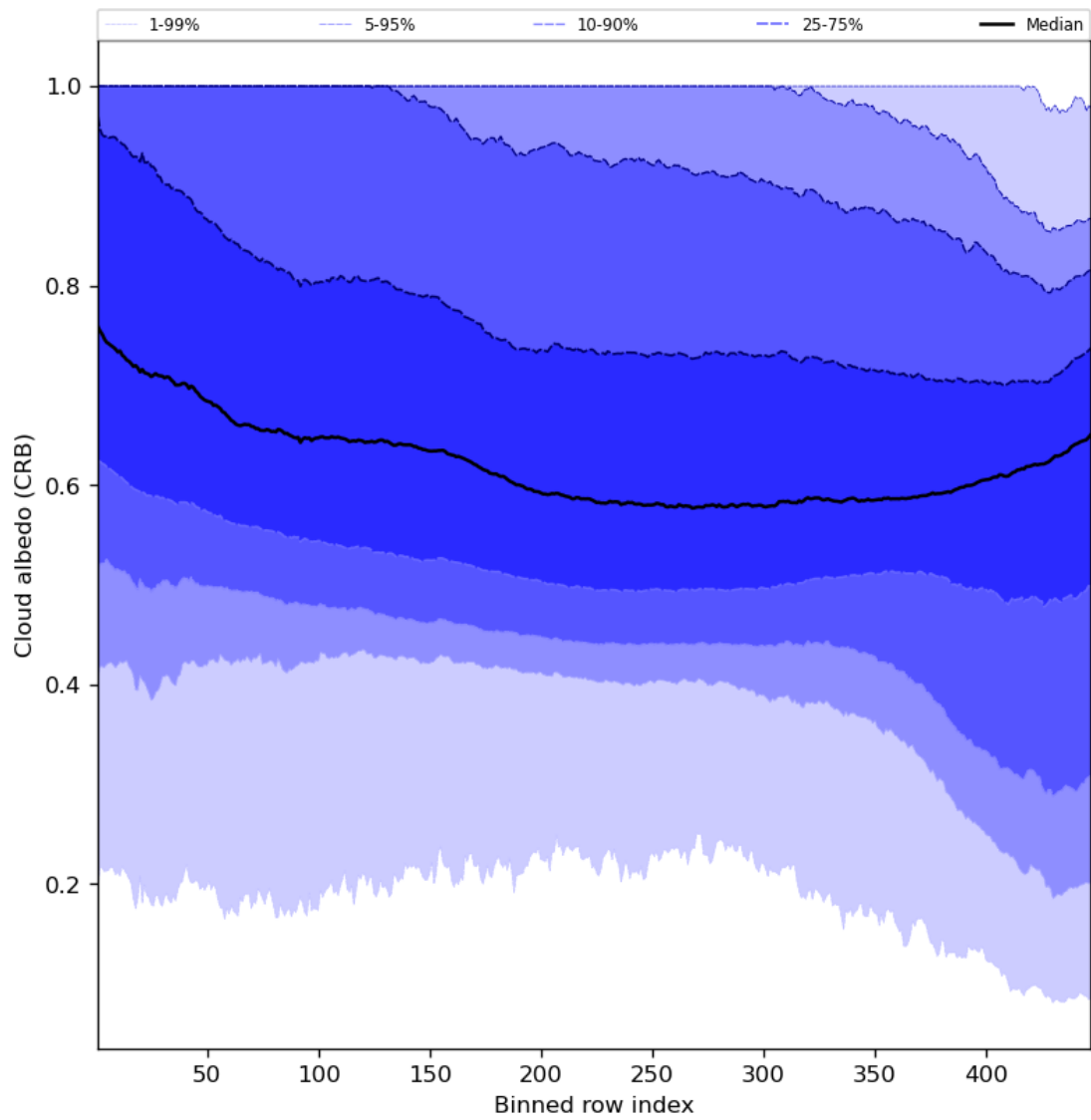
Figure 60: Along track statistics of “Cloud albedo (CRB)” for 2023-10-01 to 2023-10-02
