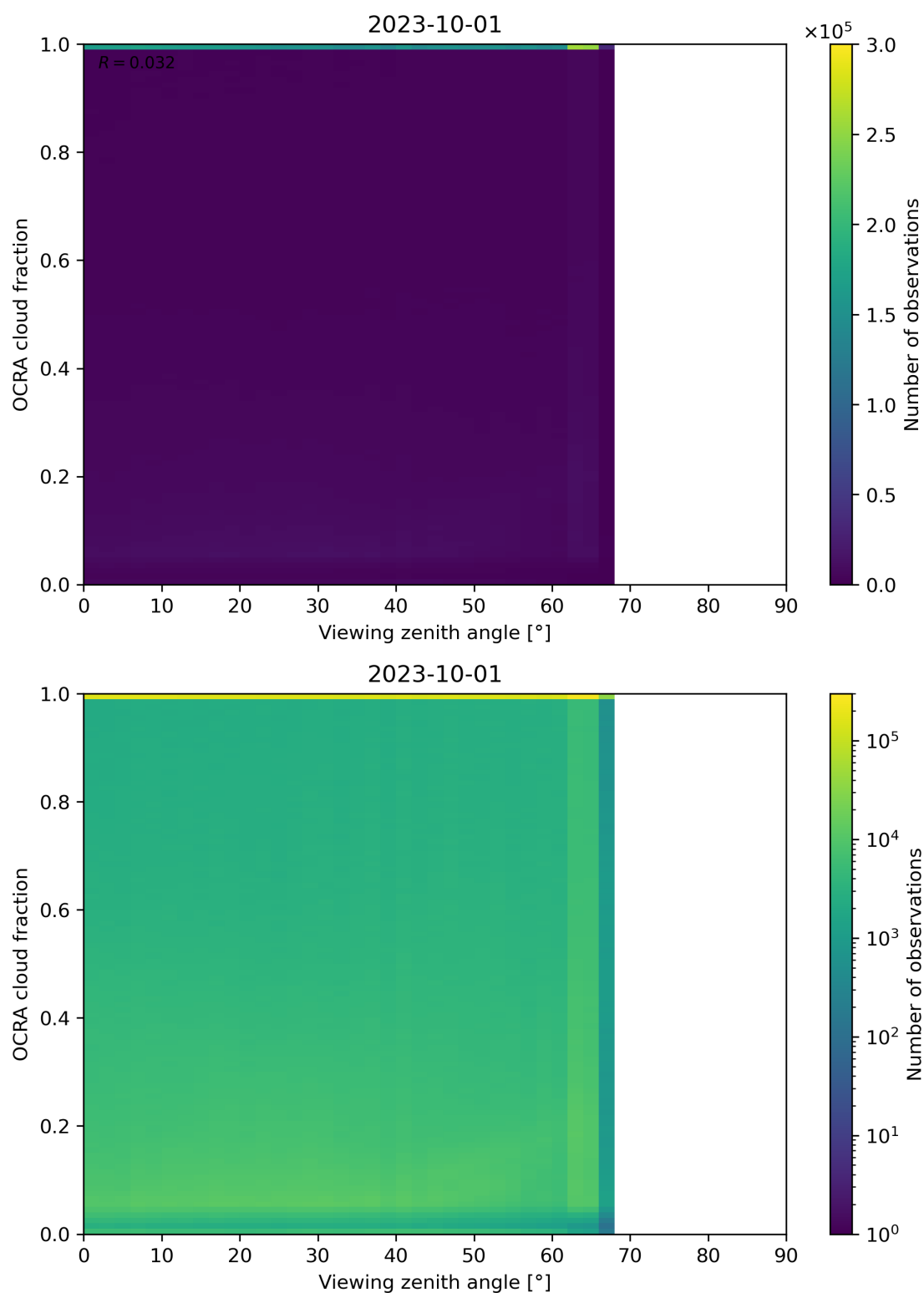
Figure 108: Scatter density plot of “Viewing zenith angle” against “OCRA cloud fraction” for 2023-10-01 to 2023-10-02.
