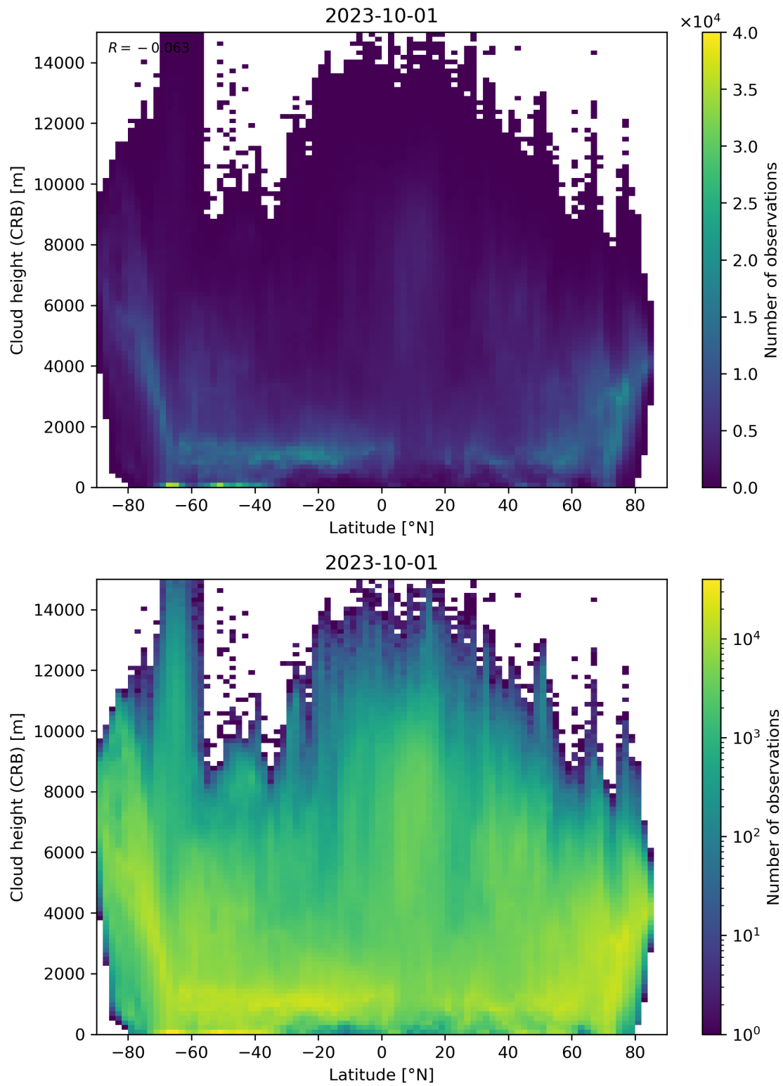
Figure 95: Scatter density plot of “Latitude” against “Cloud height (CRB)” for 2023-10-01 to 2023-10-02.
