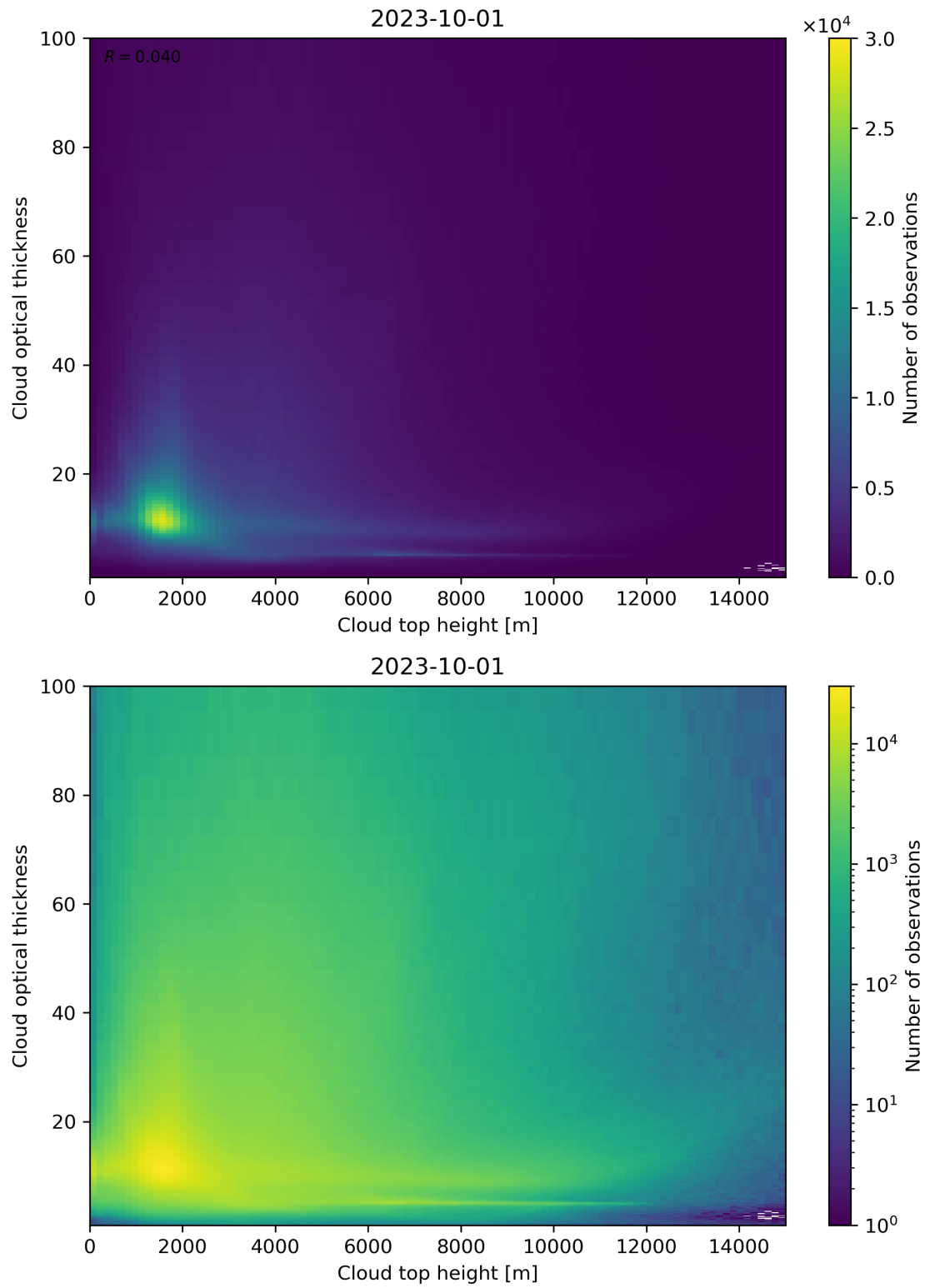
Figure 90: Scatter density plot of “Cloud top height” against “Cloud optical thickness” for 2023-10-01 to 2023-10-02.
