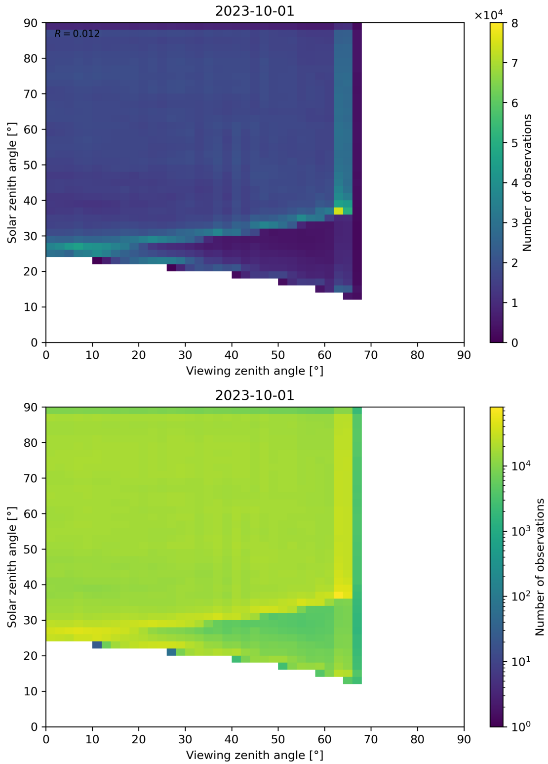
Figure 114: Scatter density plot of “Viewing zenith angle” against “Solar zenith angle” for 2023-10-01 to 2023-10-02.
