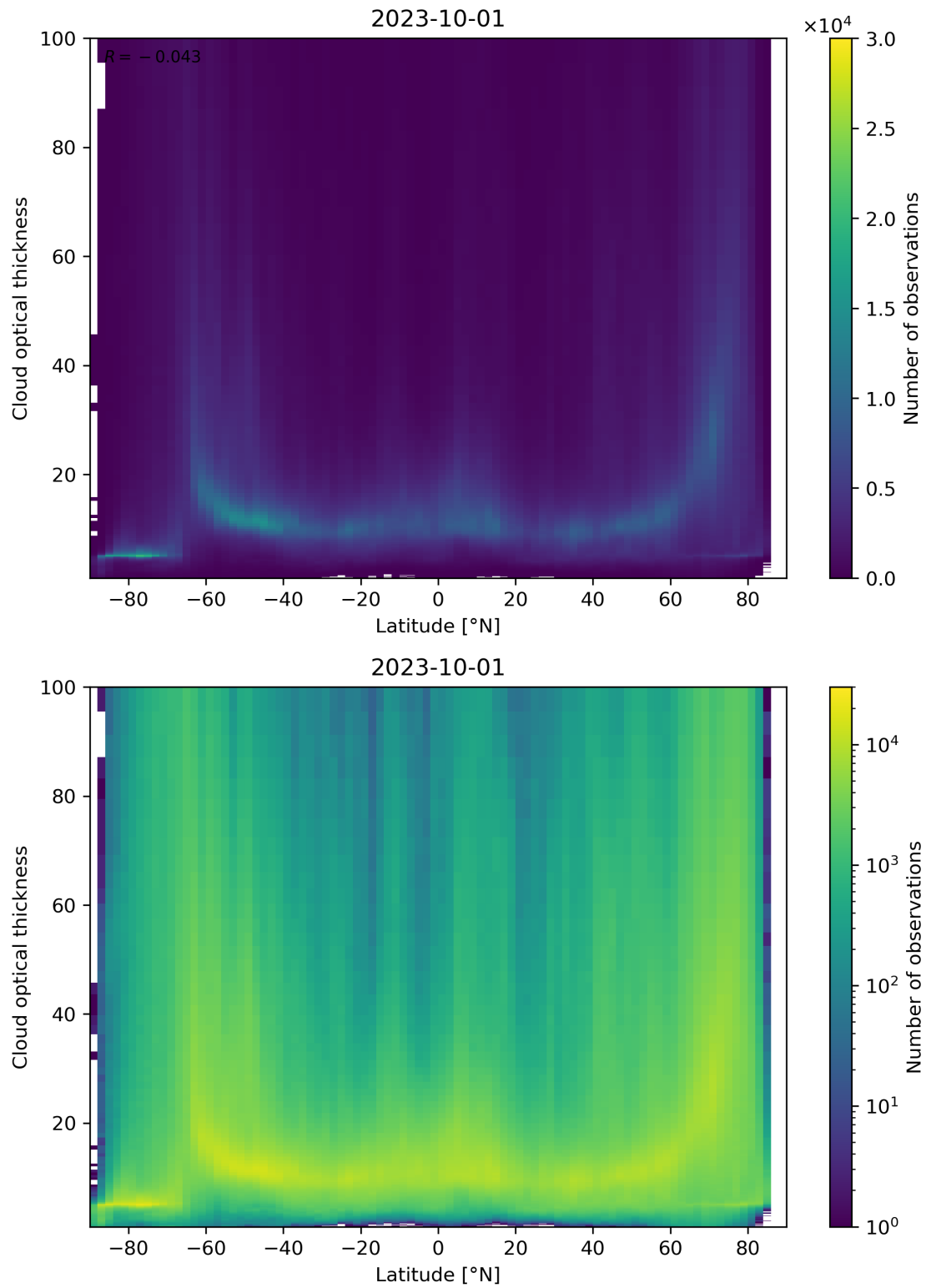
Figure 96: Scatter density plot of “Latitude” against “Cloud optical thickness” for 2023-10-01 to 2023-10-02.
