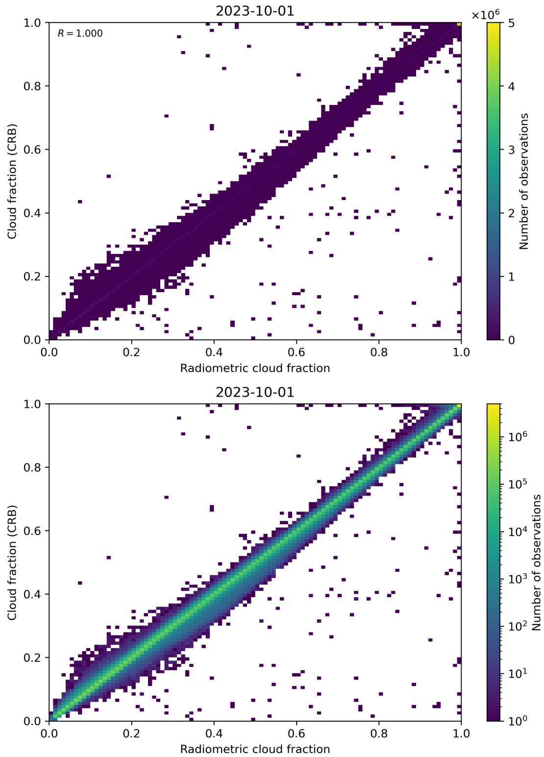
Figure 73: Scatter density plot of “Radiometric cloud fraction” against “Cloud fraction (CRB)” for 2023-10-01 to 2023-10-02.
