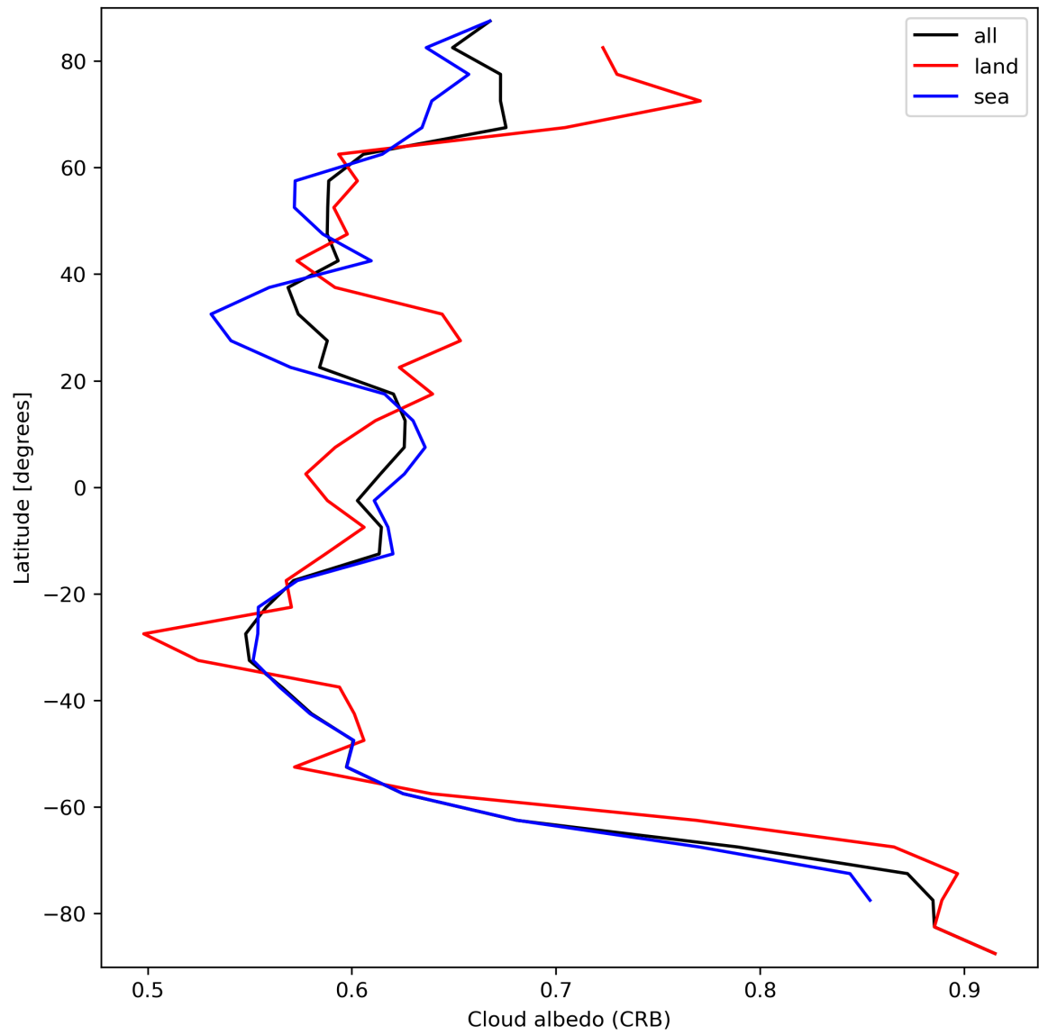
Figure 28: Zonal average of “Cloud albedo (CRB)” for 2023-10-01 to 2023-10-02.
