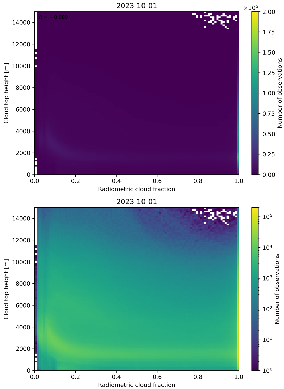
Figure 76: Scatter density plot of “Radiometric cloud fraction” against “Cloud top height” for 2023-10-01 to 2023-10-02.
