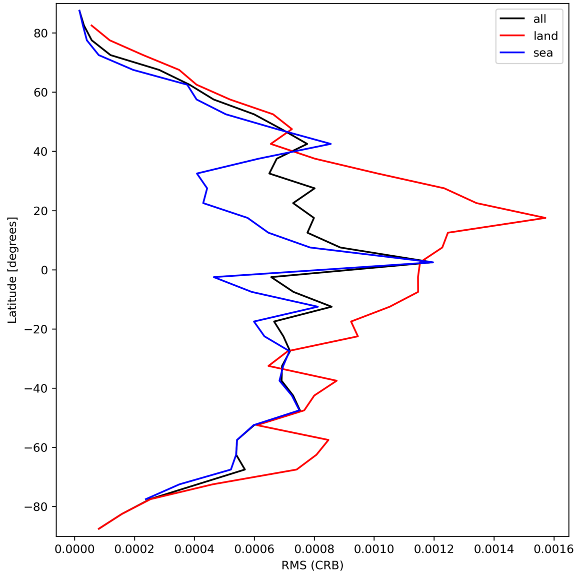
Figure 32: Zonal average of “RMS (CRB)” for 2023-10-01 to 2023-10-02.
