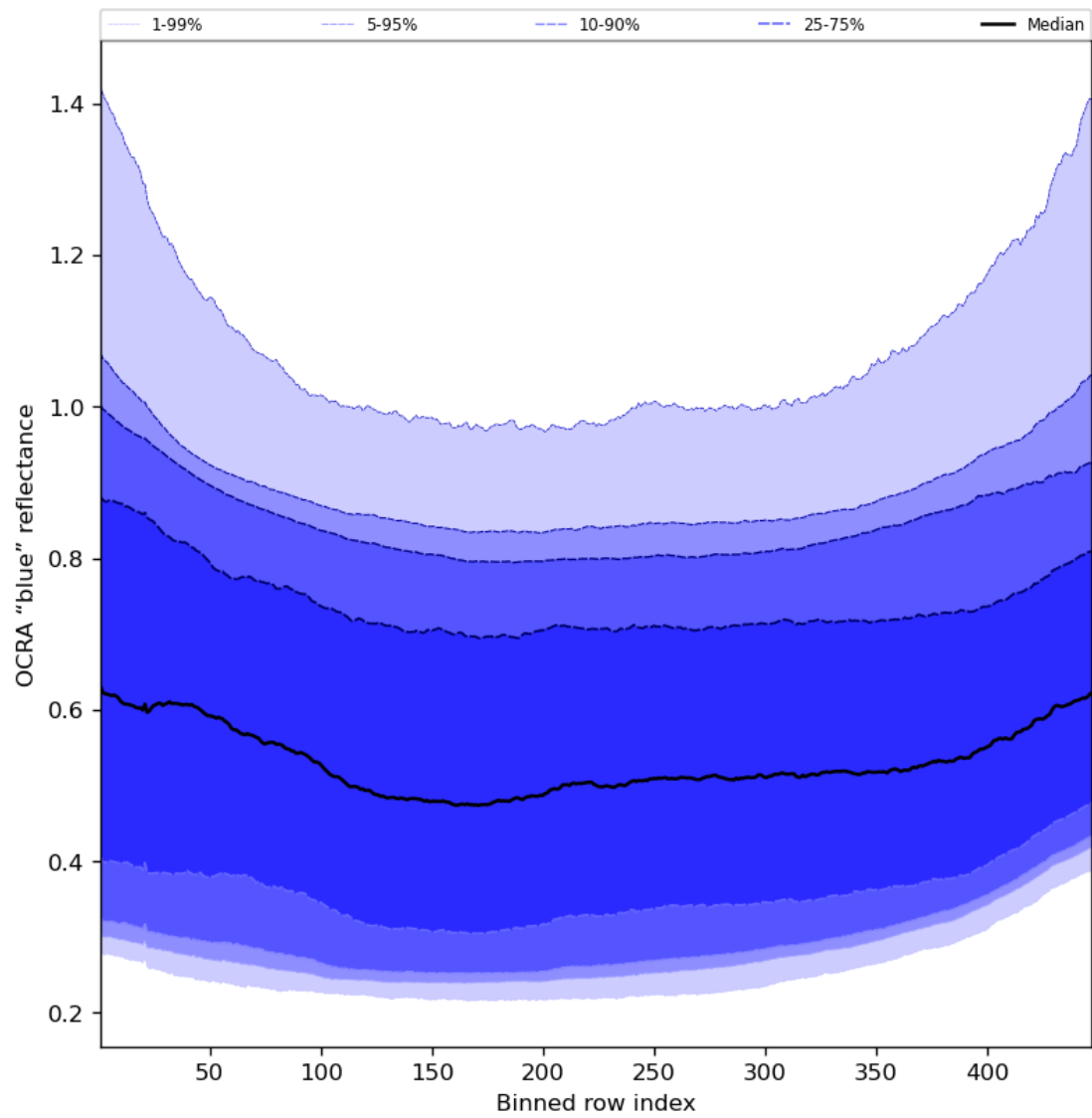
Figure 67: Along track statistics of “OCRA “blue” reflectance” for 2023-10-01 to 2023-10-02
