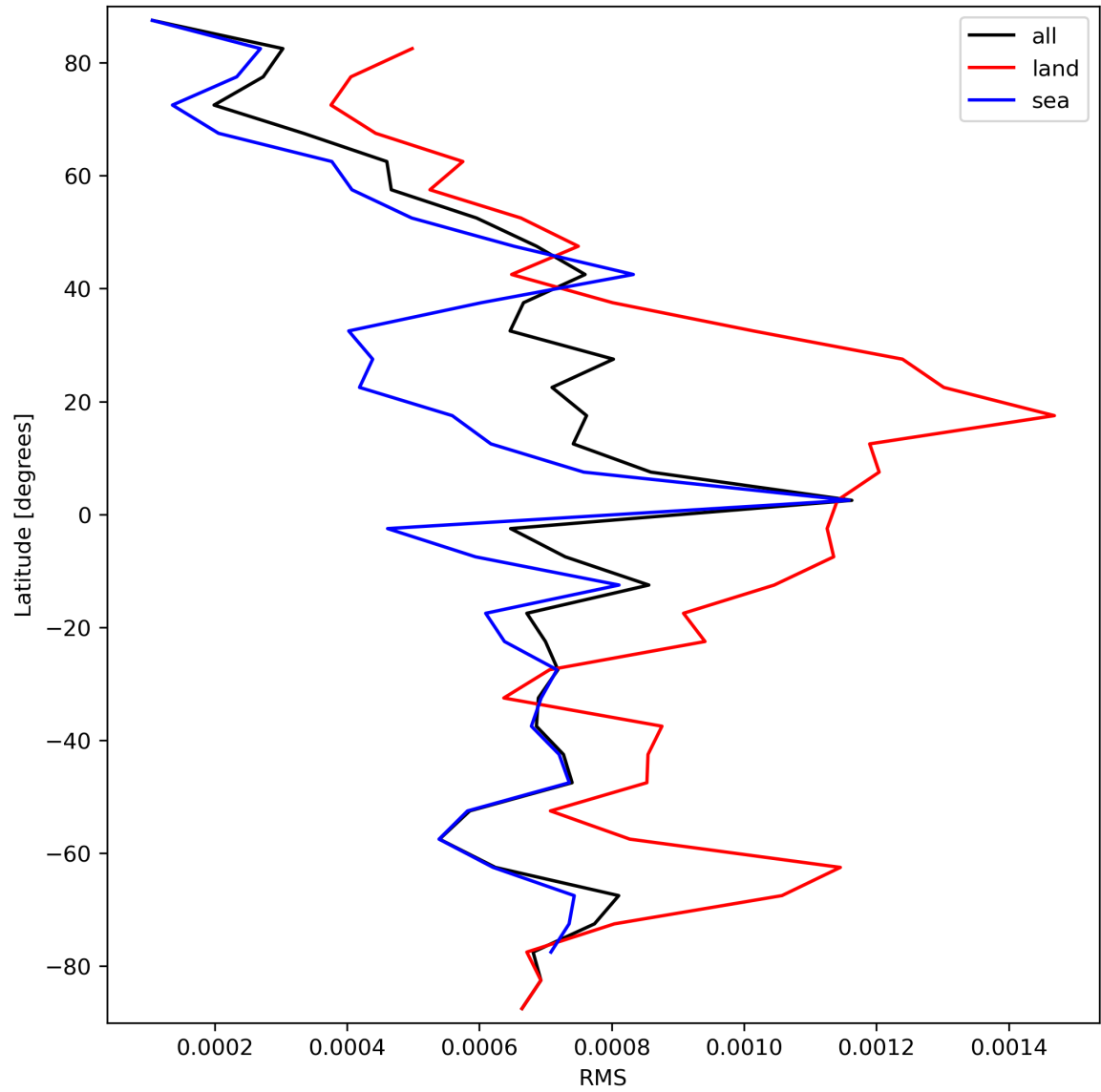
Figure 31: Zonal average of “RMS” for 2023-10-01 to 2023-10-02.
