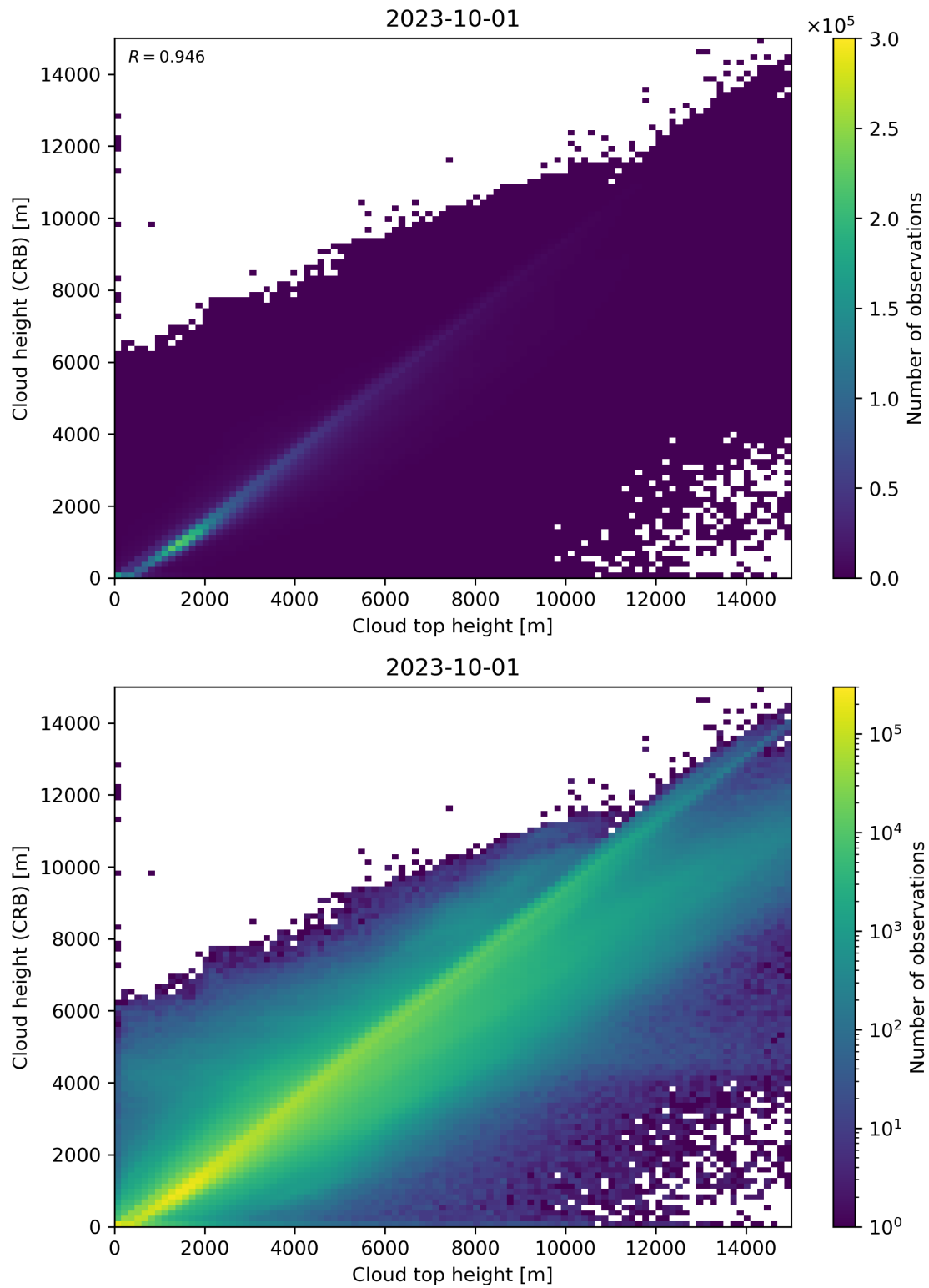
Figure 89: Scatter density plot of “Cloud top height” against “Cloud height (CRB)” for 2023-10-01 to 2023-10-02.
