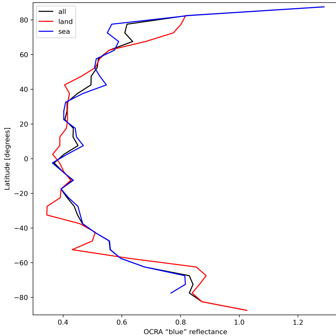
Figure 35: Zonal average of “OCRA “blue” reflectance” for 2023-10-01 to 2023-10-02.
