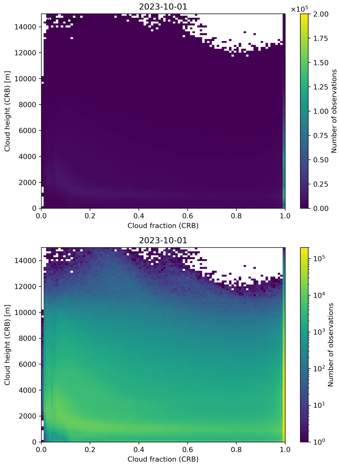
Figure 79: Scatter density plot of “Cloud fraction (CRB)” against “Cloud height (CRB)” for 2023-10-01 to 2023-10-02.
