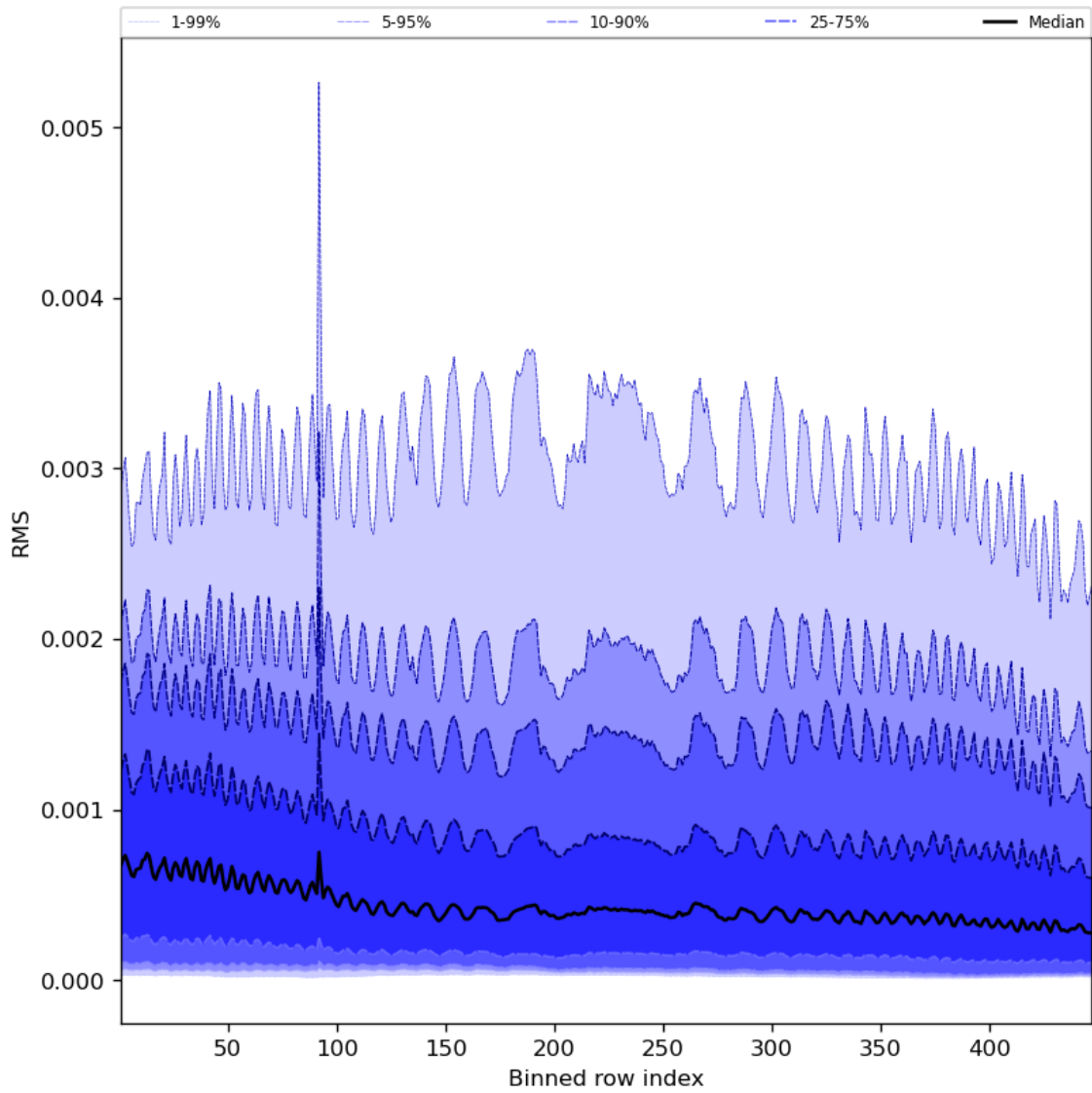
Figure 63: Along track statistics of “RMS” for 2023-10-01 to 2023-10-02
