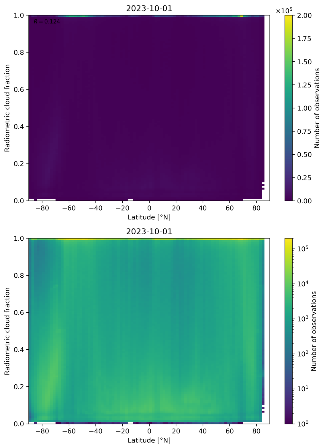
Figure 92: Scatter density plot of “Latitude” against “Radiometric cloud fraction” for 2023-10-01 to 2023-10-02.
