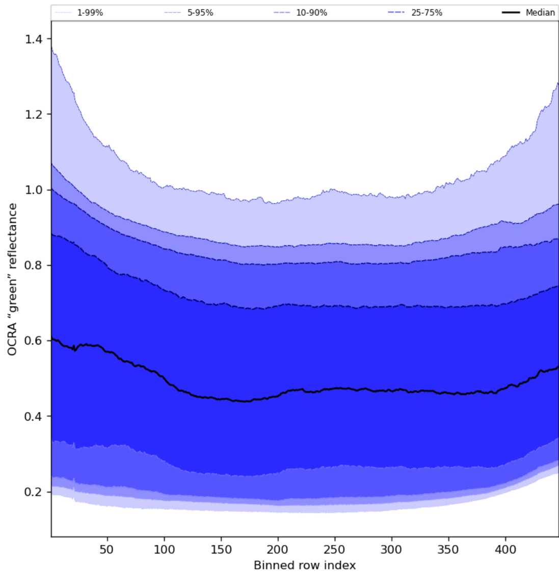
Figure 68: Along track statistics of “OCRA “green” reflectance” for 2023-10-01 to 2023-10-02
