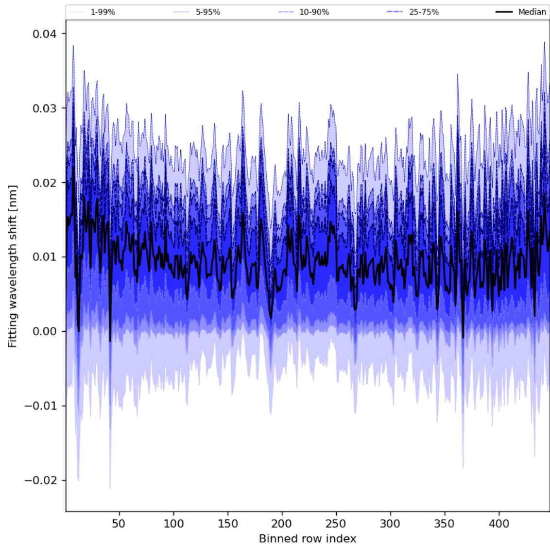
Figure 65: Along track statistics of “Fitting wavelength shift” for 2023-10-01 to 2023-10-02
