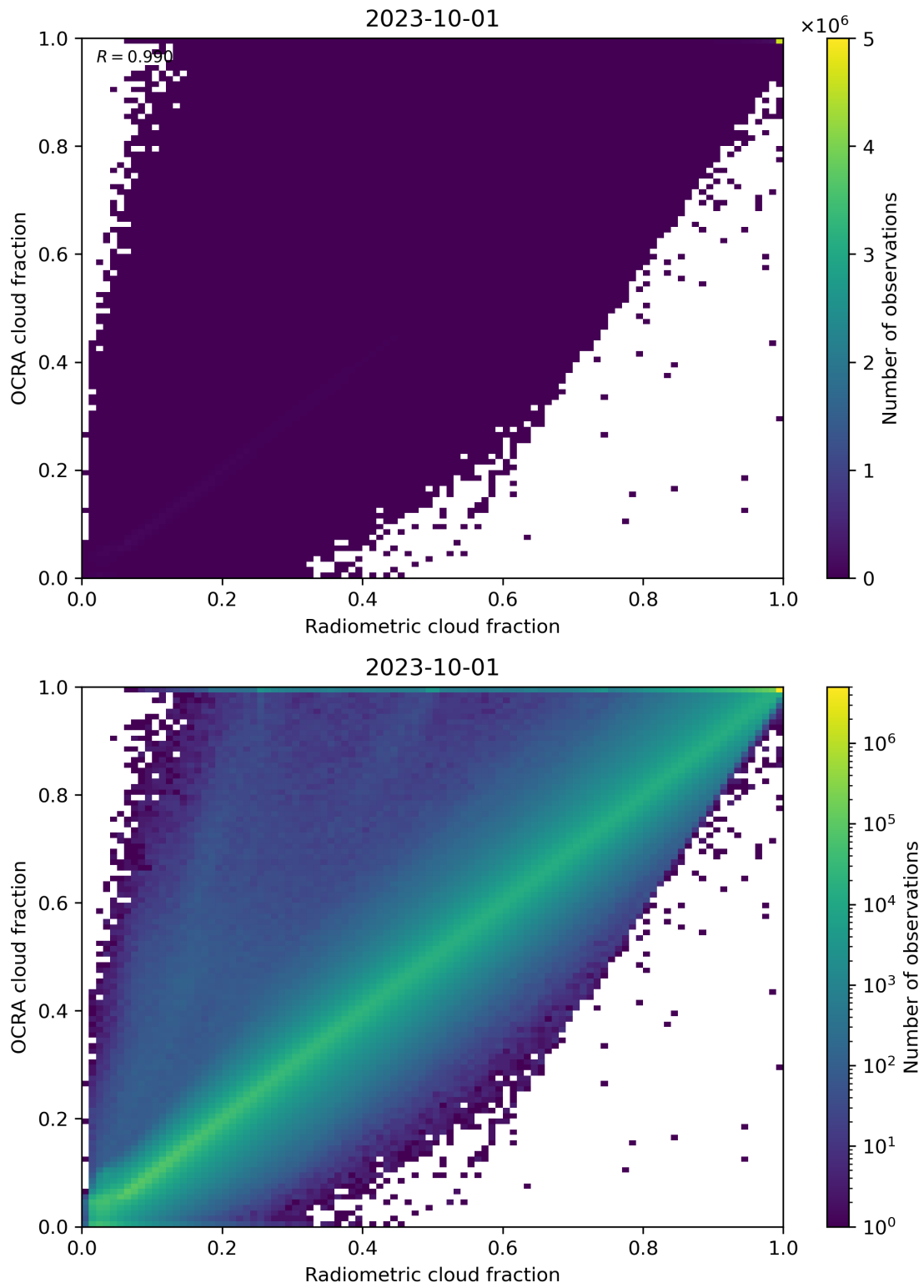
Figure 72: Scatter density plot of “Radiometric cloud fraction” against “OCRA cloud fraction” for 2023-10-01 to 2023-10-02.
