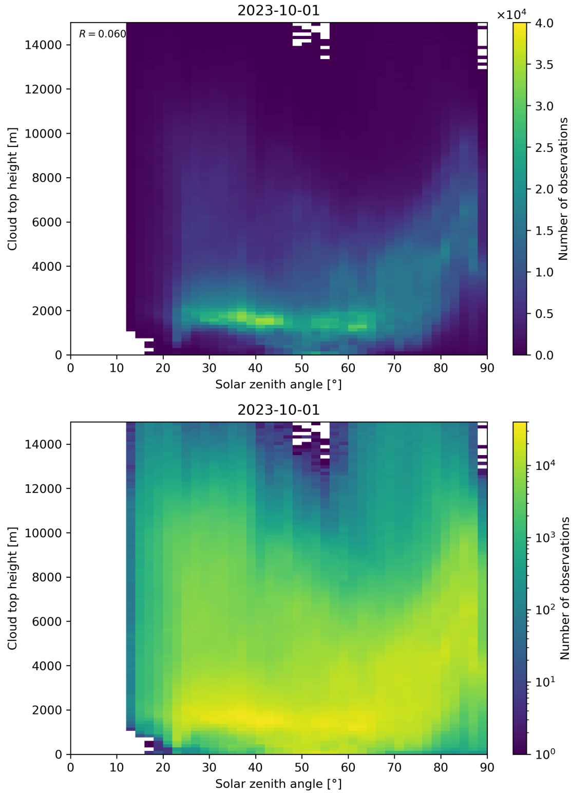
Figure 104: Scatter density plot of “Solar zenith angle” against “Cloud top height” for 2023-10-01 to 2023-10-02.
