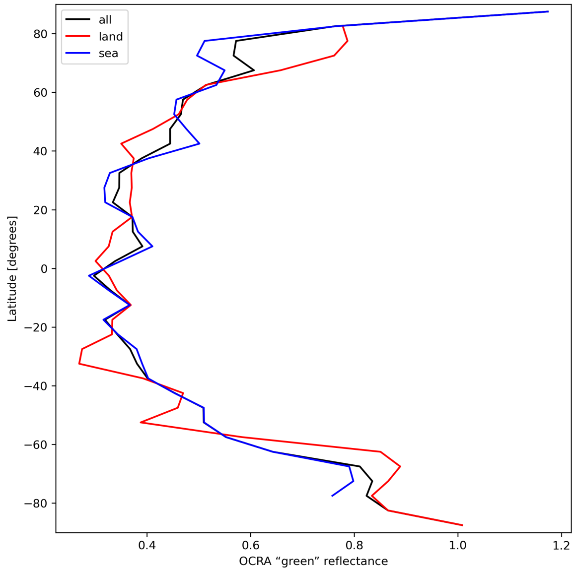
Figure 36: Zonal average of “OCRA “green” reflectance” for 2023-10-01 to 2023-10-02.
