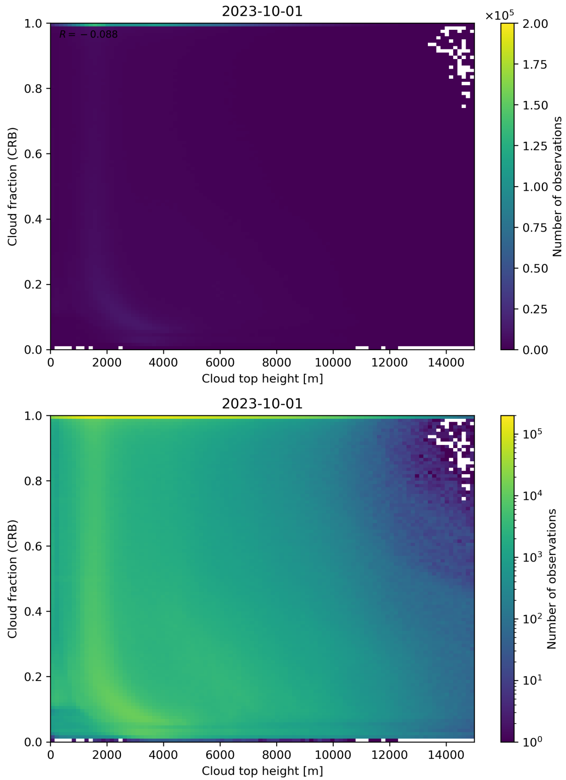
Figure 88: Scatter density plot of “Cloud top height” against “Cloud fraction (CRB)” for 2023-10-01 to 2023-10-02.
