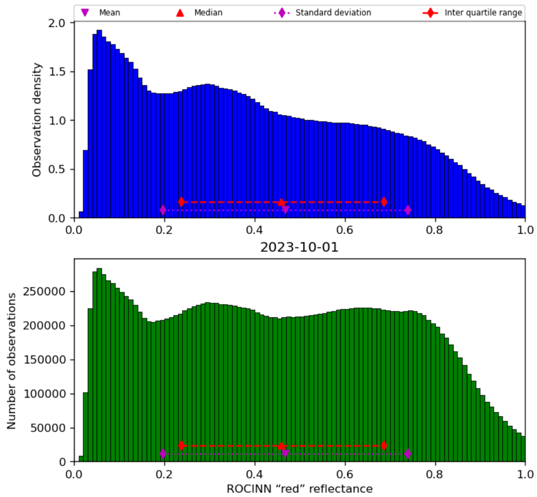
Figure 53: Histogram of “ROCINN “red” reflectance” for 2023-10-01 to 2023-10-02
