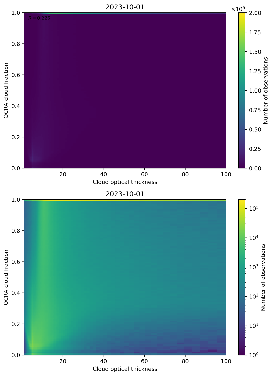
Figure 83: Scatter density plot of “Cloud optical thickness” against “OCRA cloud fraction” for 2023-10-01 to 2023-10-02.
