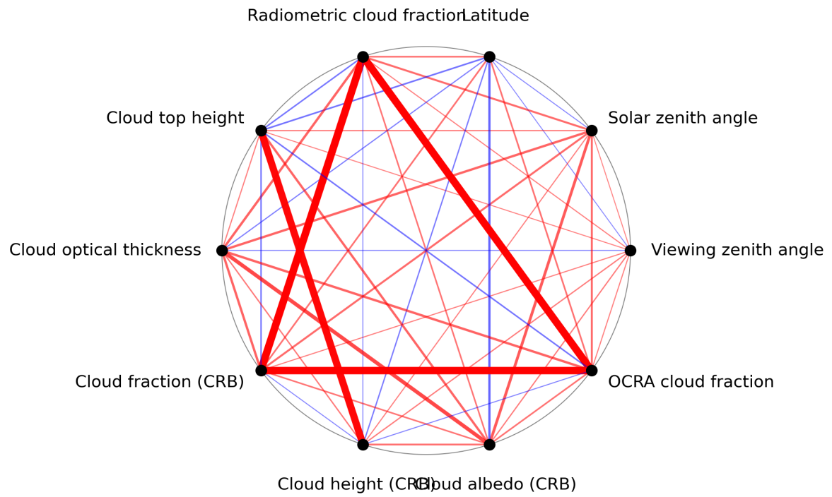
Figure 1: Map of correlation graph for 2023-10-01 to 2023-10-02.
