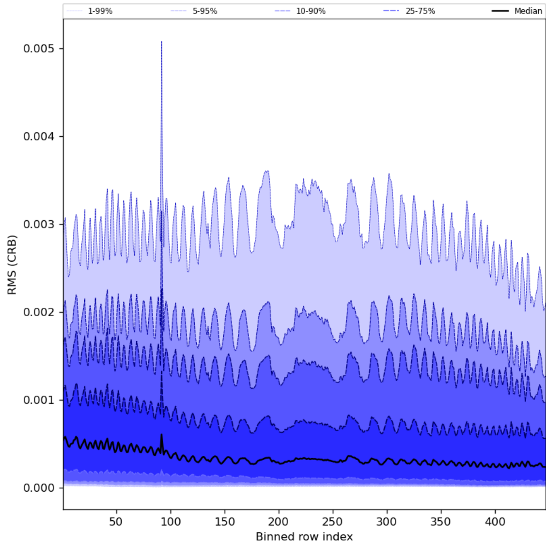
Figure 64: Along track statistics of “RMS (CRB)” for 2023-10-01 to 2023-10-02
