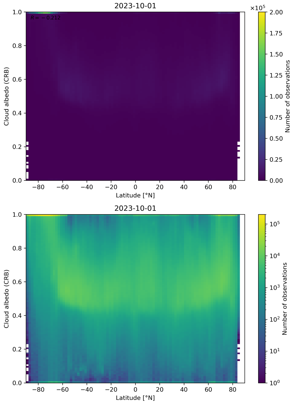
Figure 91: Scatter density plot of “Latitude” against “Cloud albedo (CRB)” for 2023-10-01 to 2023-10-02.
