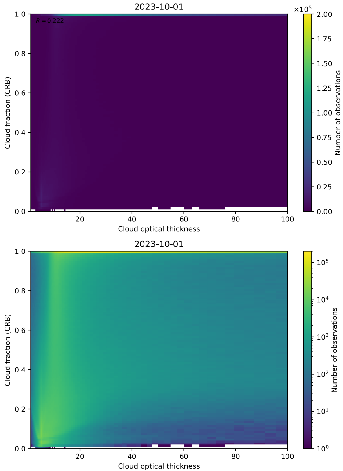
Figure 84: Scatter density plot of “Cloud optical thickness” against “Cloud fraction (CRB)” for 2023-10-01 to 2023-10-02.
