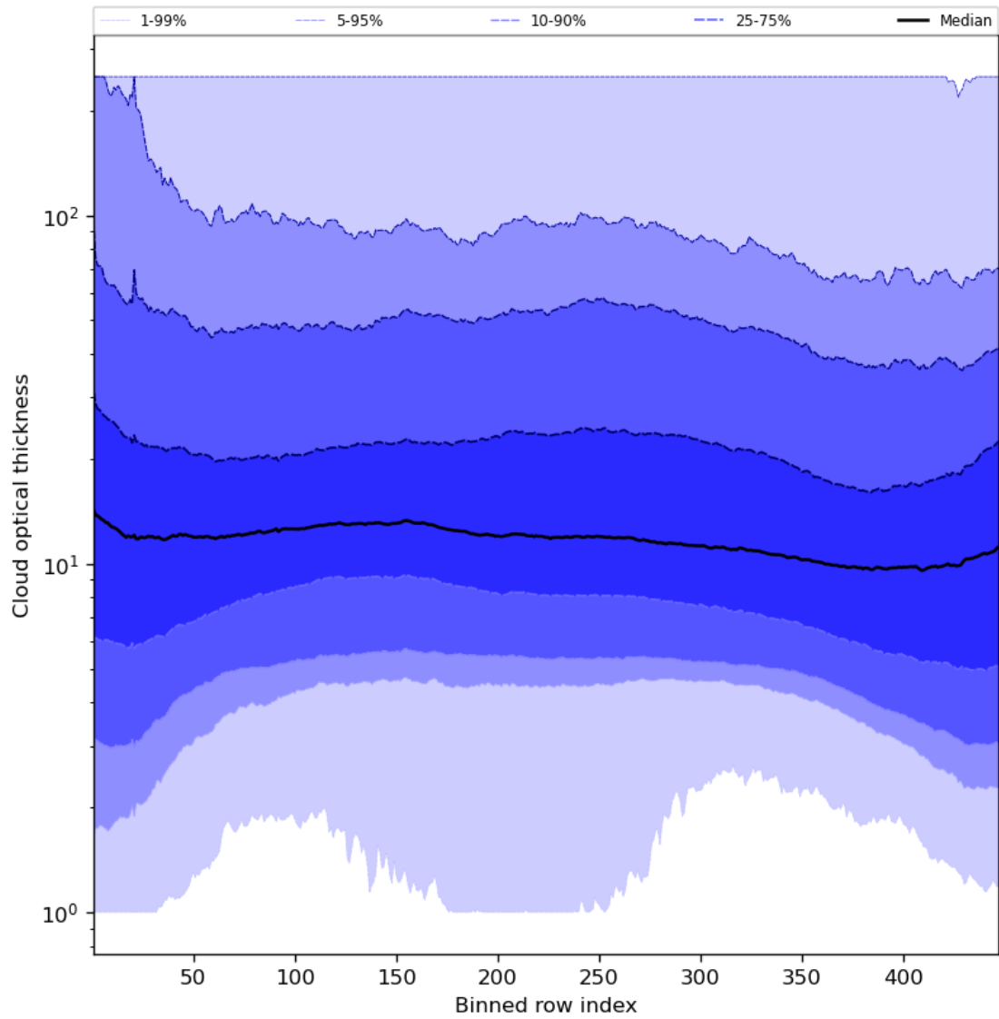
Figure 57: Along track statistics of “Cloud optical thickness” for 2023-10-01 to 2023-10-02
