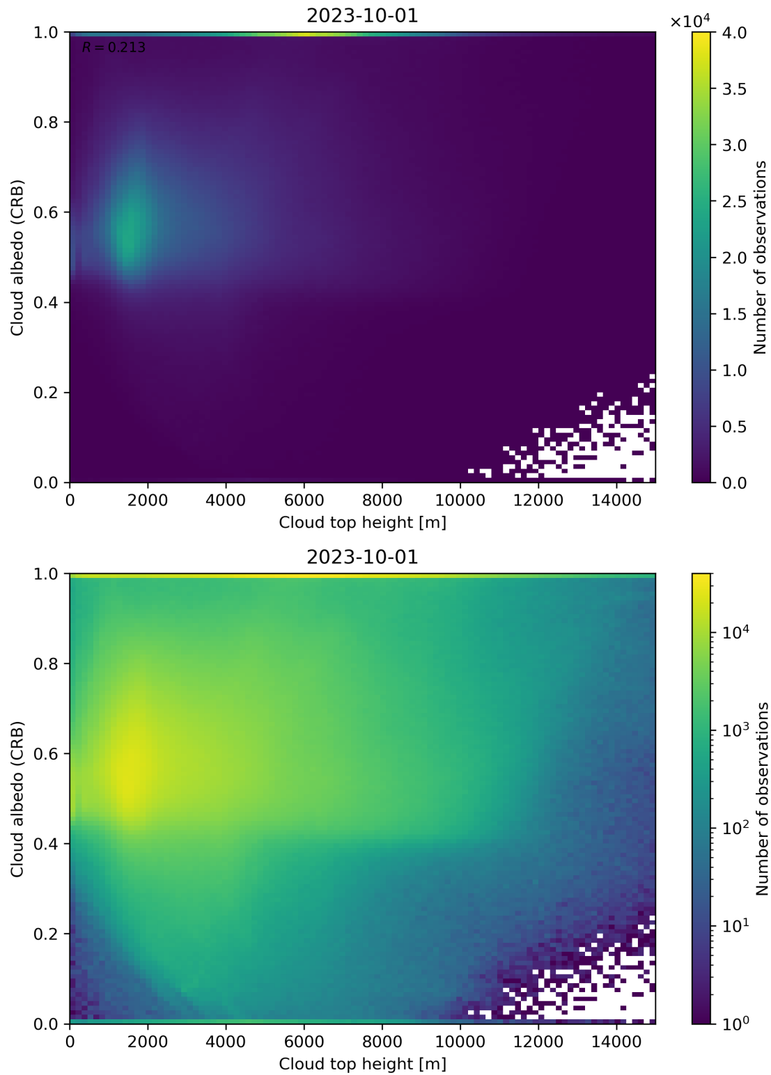
Figure 86: Scatter density plot of “Cloud top height” against “Cloud albedo (CRB)” for 2023-10-01 to 2023-10-02.
