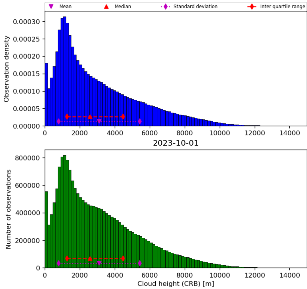
Figure 43: Histogram of “Cloud height (CRB)” for 2023-10-01 to 2023-10-02
