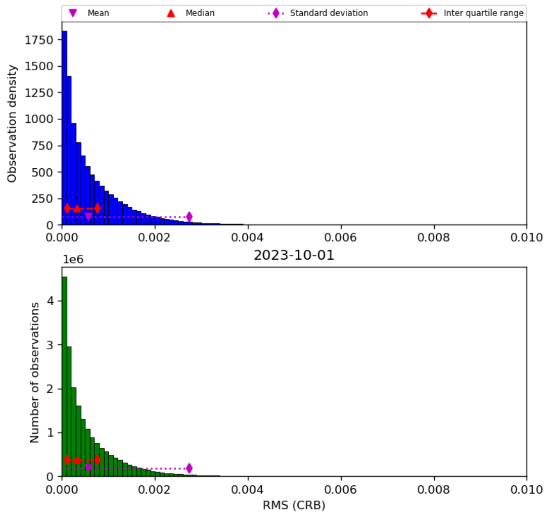
Figure 48: Histogram of "RMS (CRB)" for 2023-10-01 to 2023-10-02
