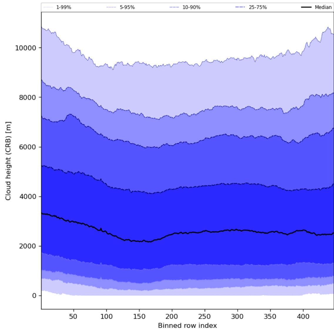
Figure 59: Along track statistics of “Cloud height (CRB)” for 2023-10-01 to 2023-10-02
