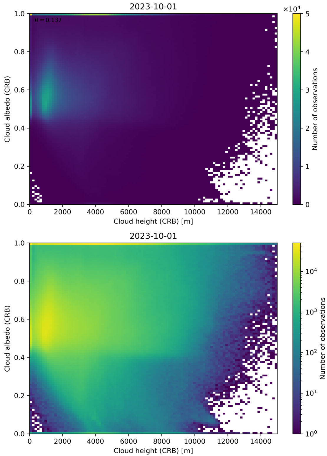
Figure 80: Scatter density plot of “Cloud height (CRB)” against “Cloud albedo (CRB)” for 2023-10-01 to 2023-10-02.
