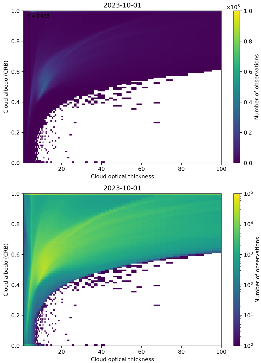
Figure 82: Scatter density plot of “Cloud optical thickness” against “Cloud albedo (CRB)” for 2023-10-01 to 2023-10-02.
