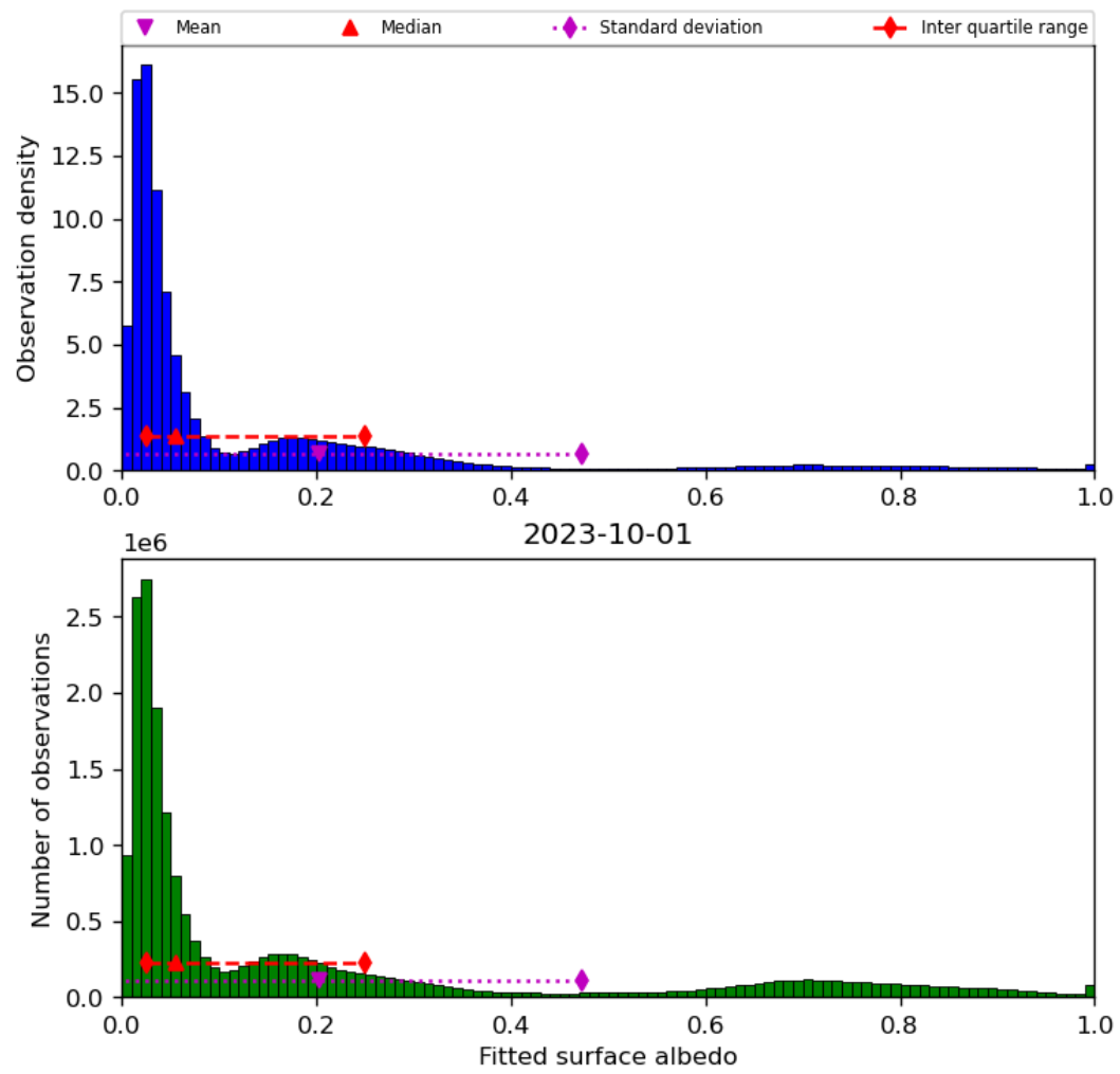
Figure 45: Histogram of “Fitted surface albedo” for 2023-10-01 to 2023-10-02
