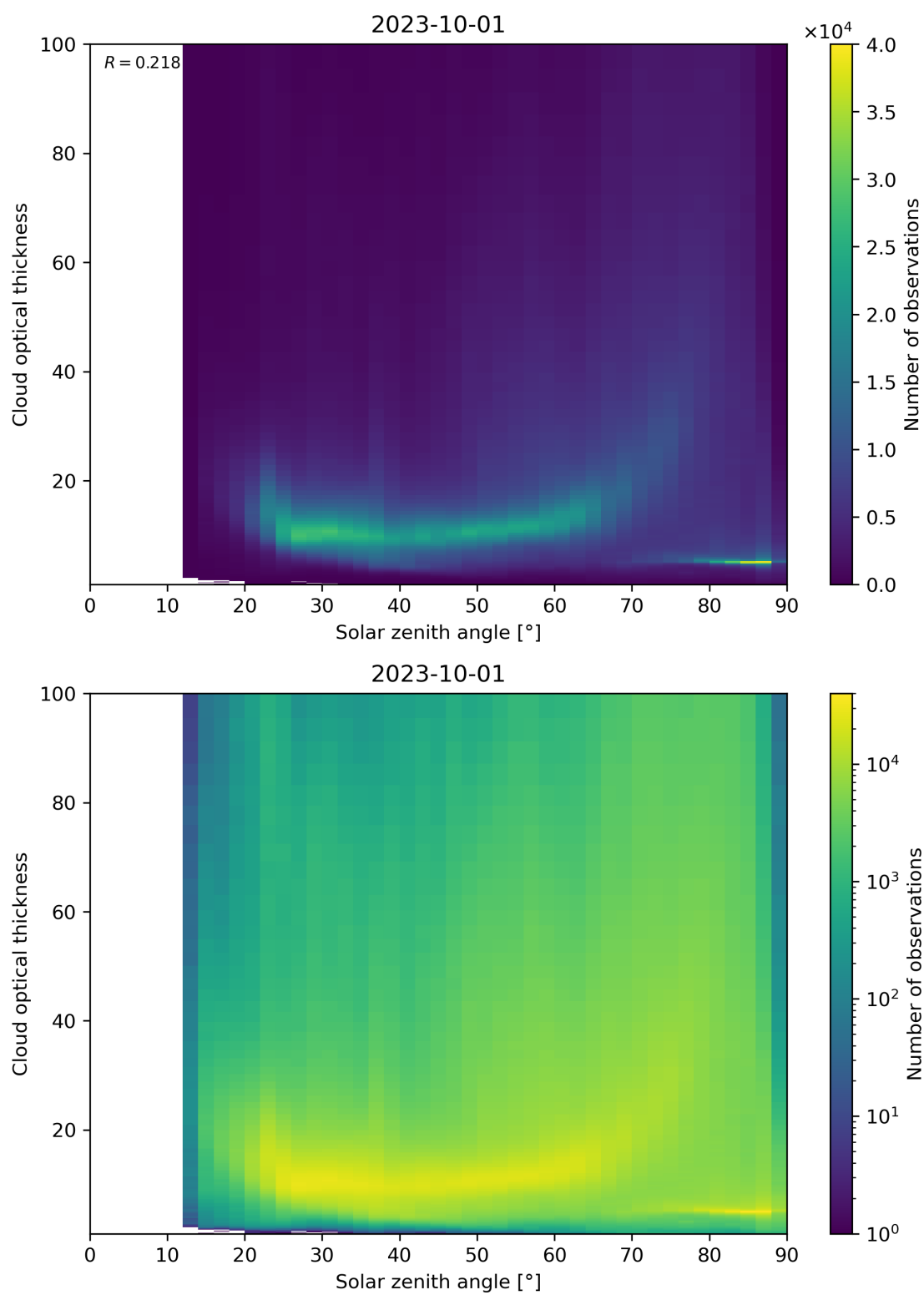
Figure 103: Scatter density plot of “Solar zenith angle” against “Cloud optical thickness” for 2023-10-01 to 2023-10-02.
