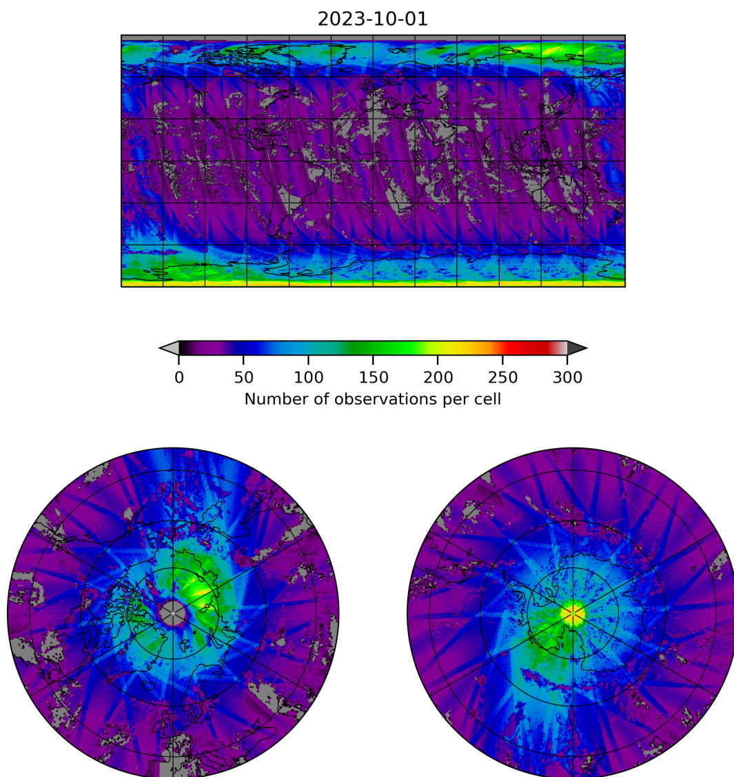
Figure 21: Map of the number of observations for 2023-10-01 to 2023-10-02
