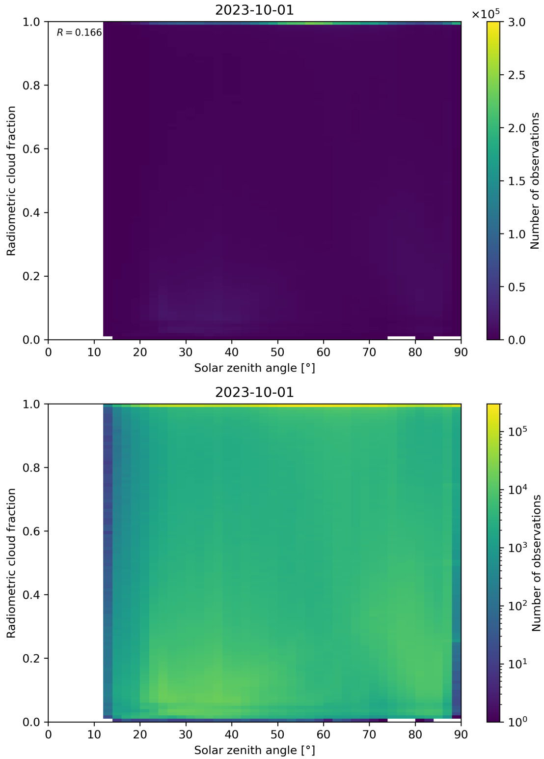
Figure 99: Scatter density plot of “Solar zenith angle” against “Radiometric cloud fraction” for 2023-10-01 to 2023-10-02.
