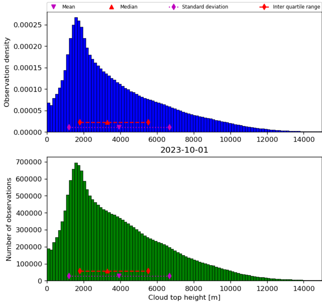
Figure 40: Histogram of “Cloud top height” for 2023-10-01 to 2023-10-02
