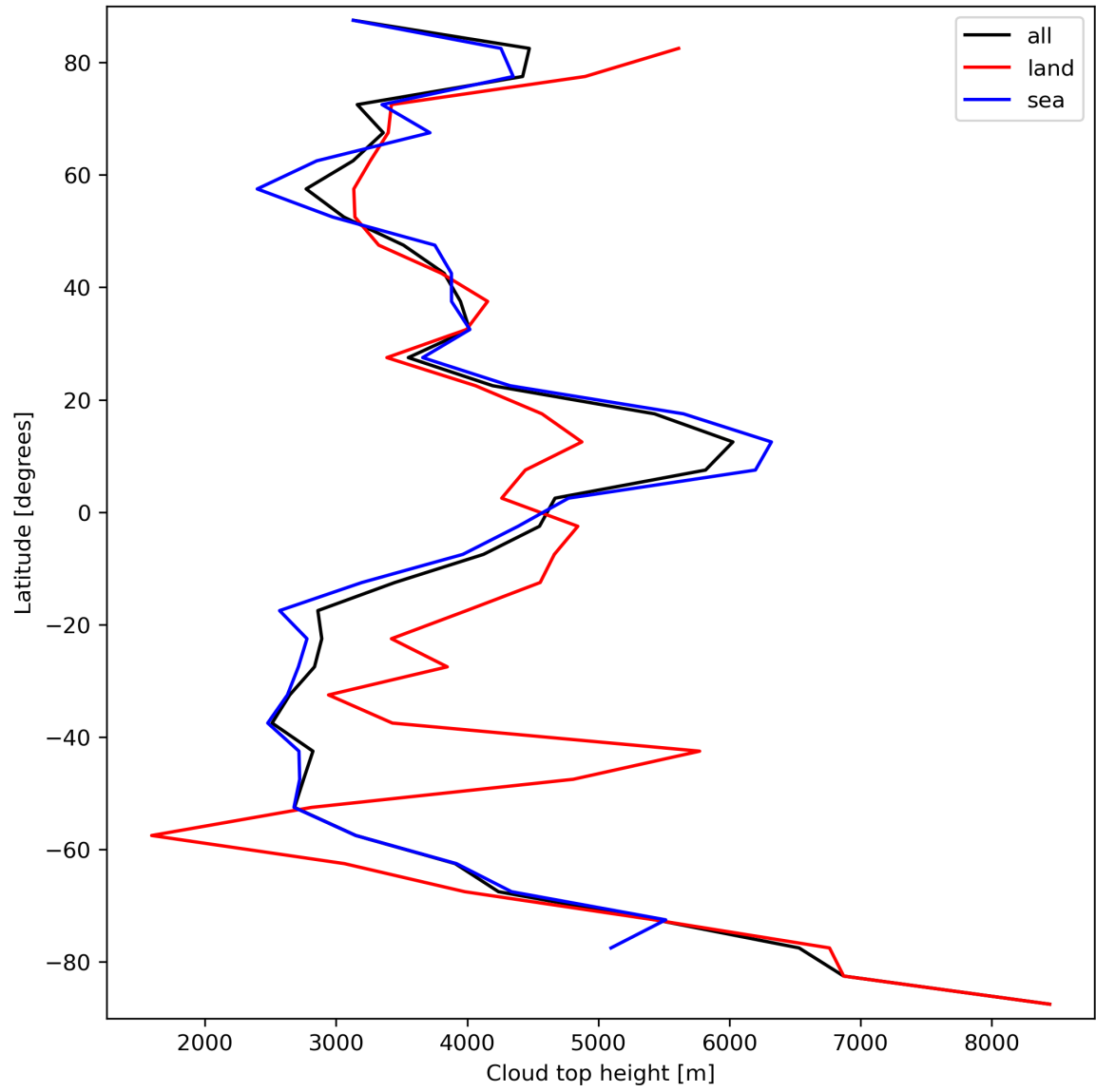
Figure 24: Zonal average of “Cloud top height” for 2023-10-01 to 2023-10-02.
