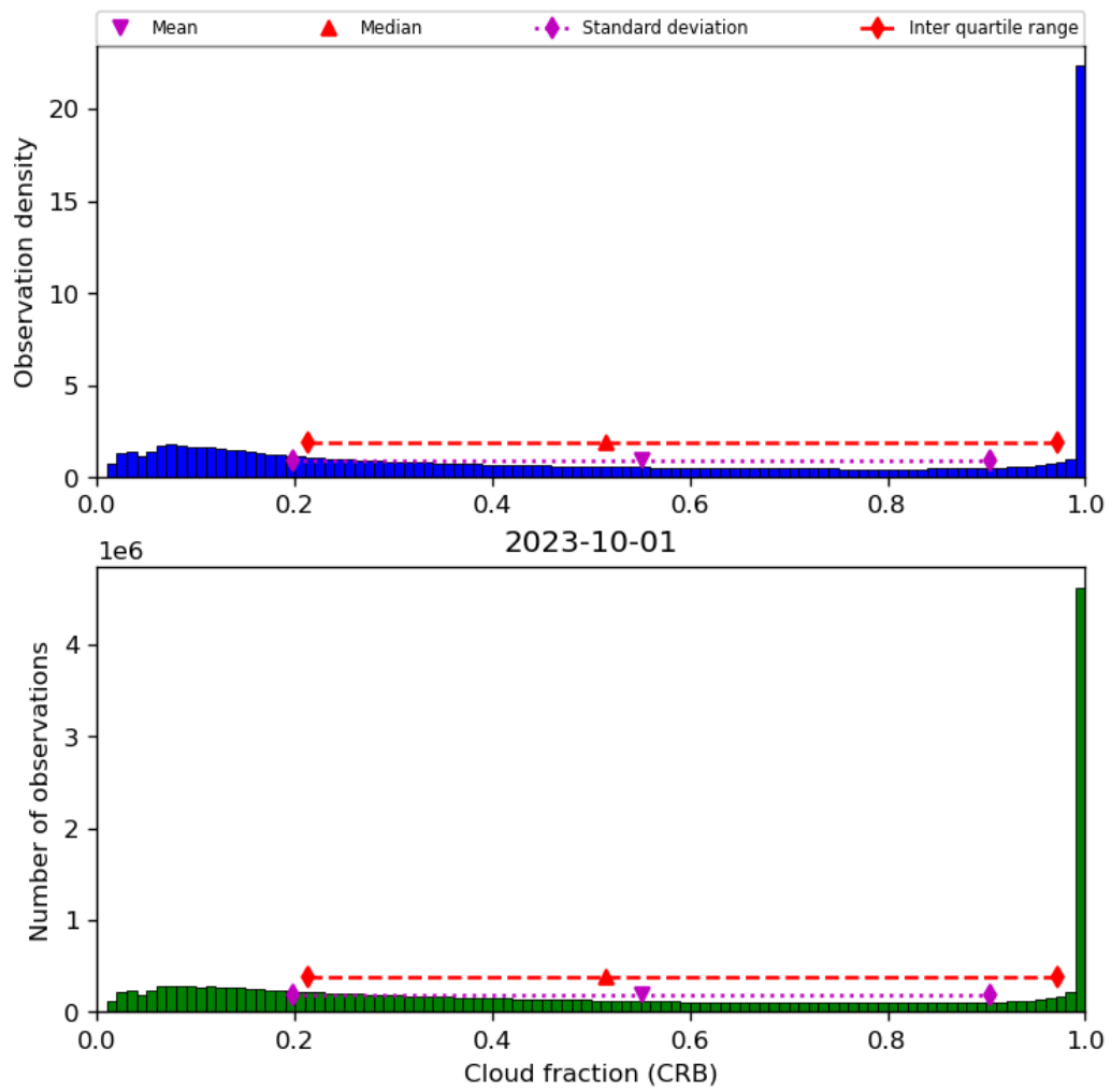
Figure 42: Histogram of “Cloud fraction (CRB)” for 2023-10-01 to 2023-10-02
