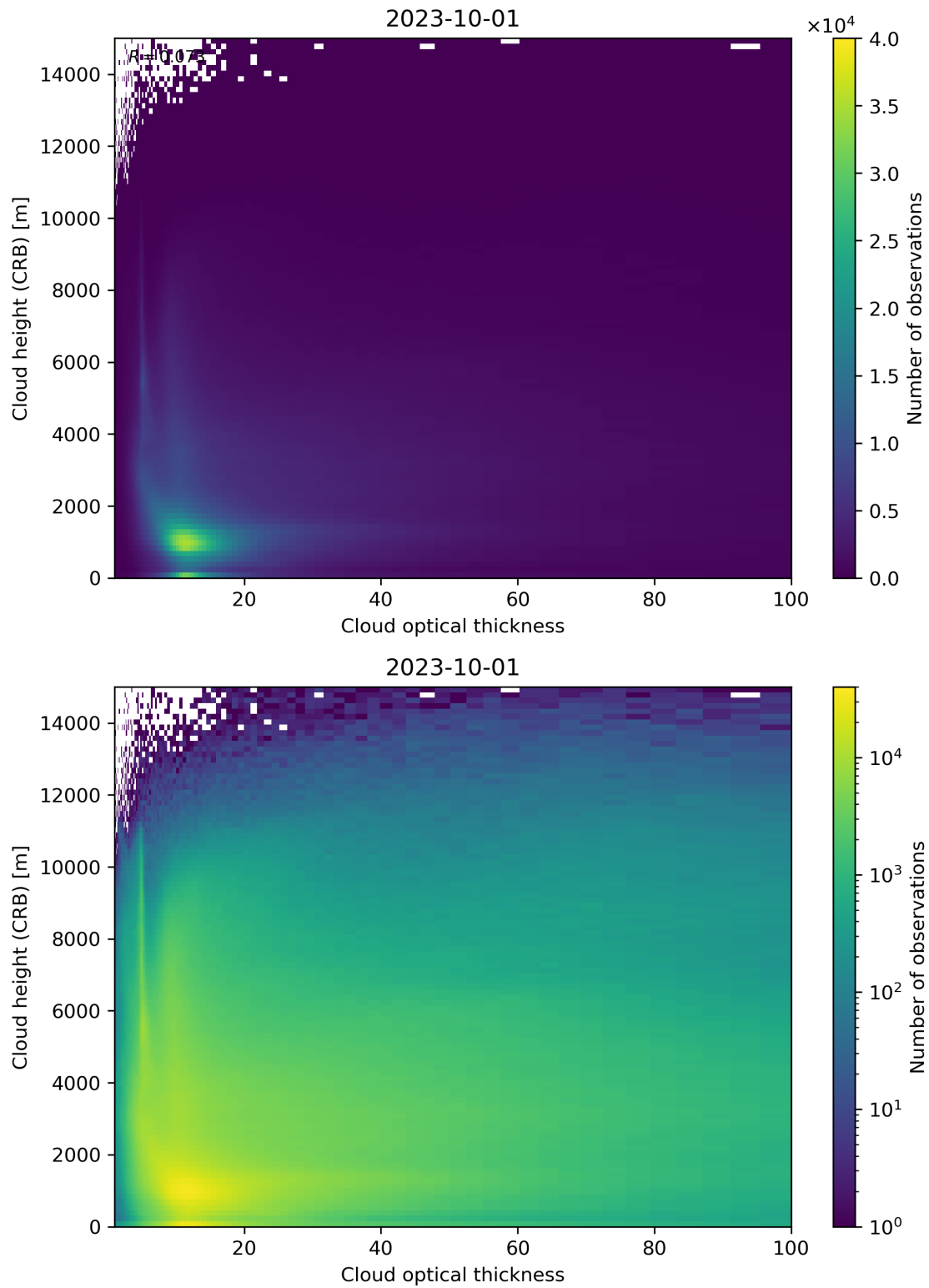
Figure 85: Scatter density plot of “Cloud optical thickness” against “Cloud height (CRB)” for 2023-10-01 to 2023-10-02.
