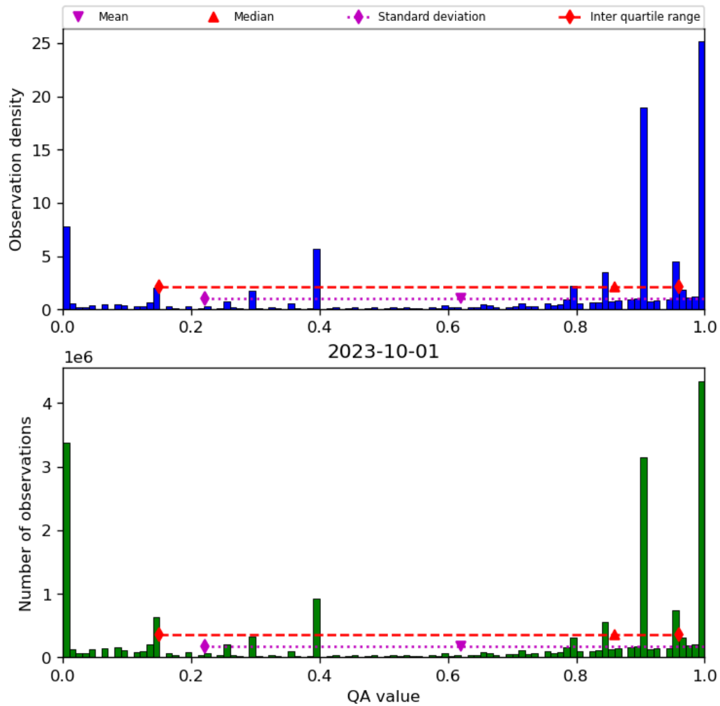
Figure 38: Histogram of “QA value” for 2023-10-01 to 2023-10-02
