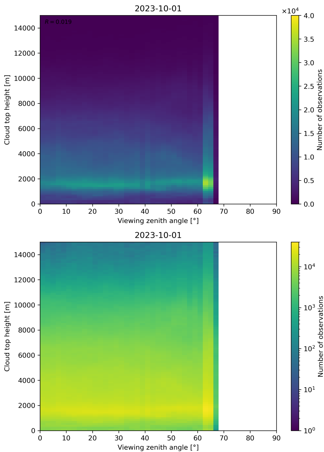
Figure 112: Scatter density plot of “Viewing zenith angle” against “Cloud top height” for 2023-10-01 to 2023-10-02.
