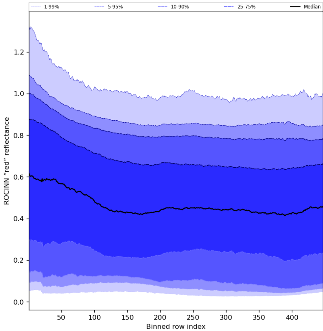
Figure 69: Along track statistics of “ROCINN “red” reflectance” for 2023-10-01 to 2023-10-02
