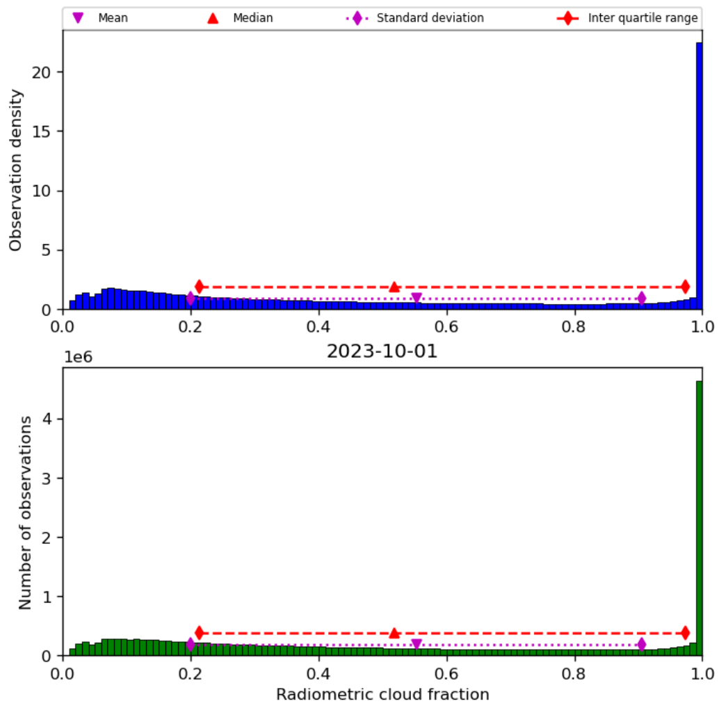
Figure 39: Histogram of “Radiometric cloud fraction” for 2023-10-01 to 2023-10-02
