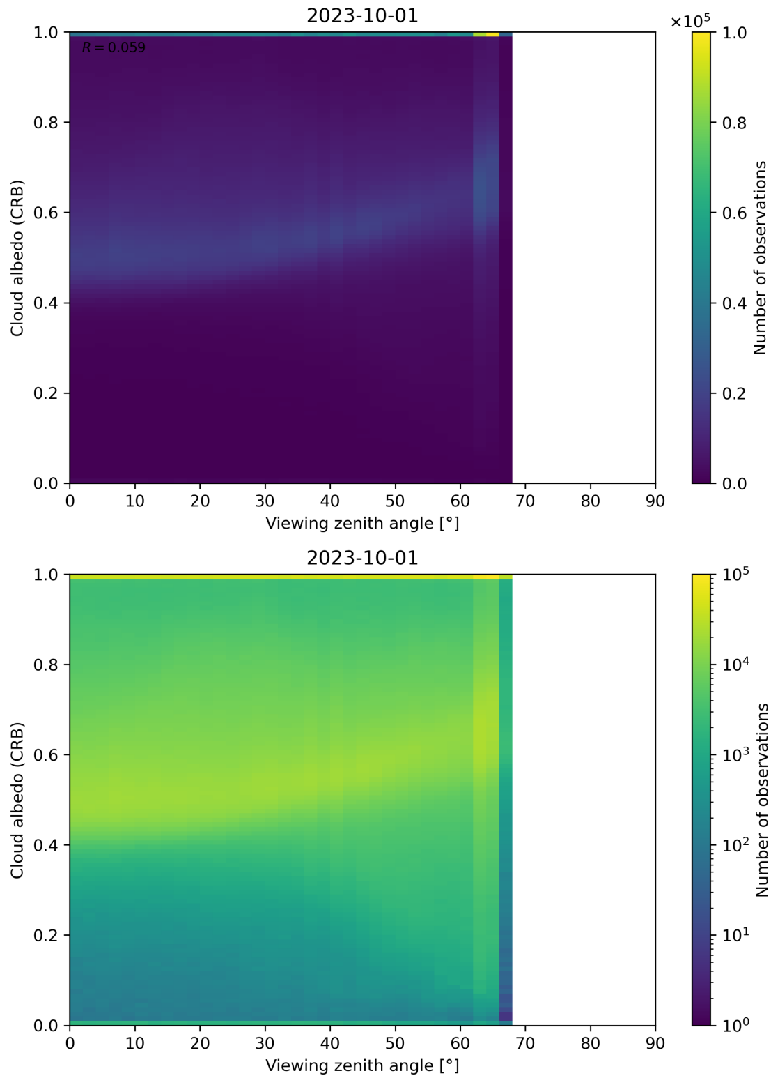
Figure 106: Scatter density plot of “Viewing zenith angle” against “Cloud albedo (CRB)” for 2023-10-01 to 2023-10-02.
