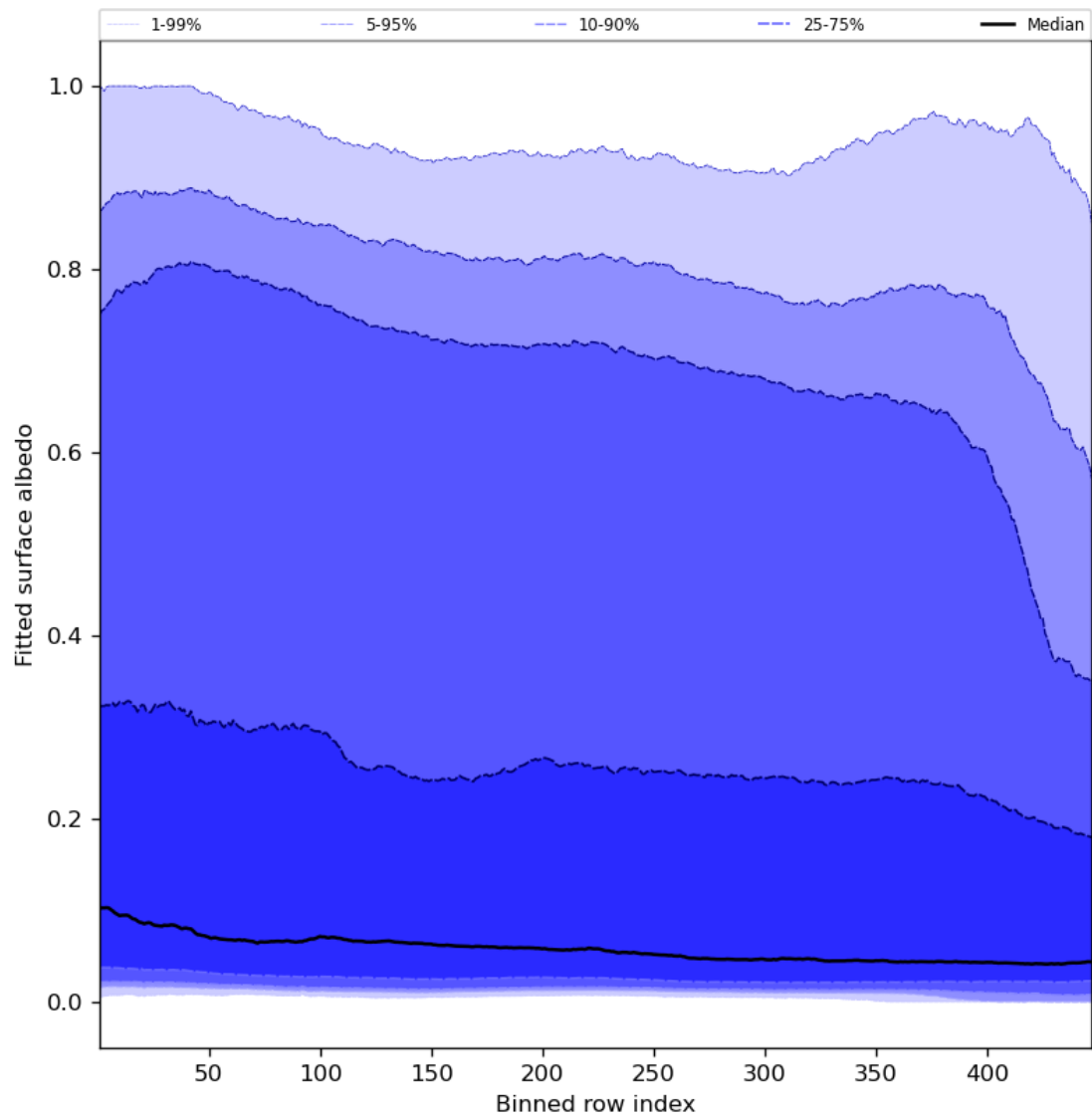
Figure 61: Along track statistics of “Fitted surface albedo” for 2023-10-01 to 2023-10-02
