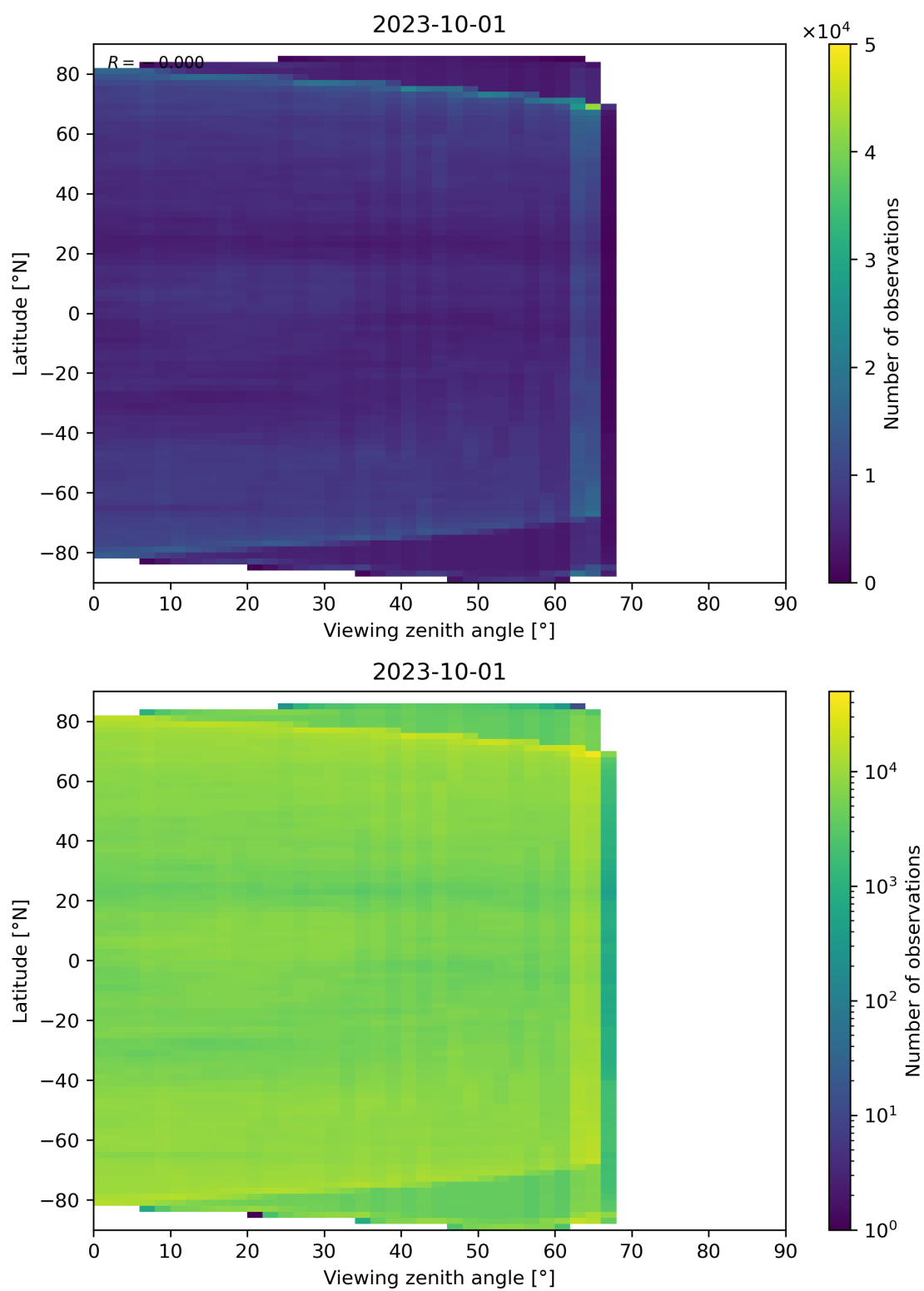
Figure 113: Scatter density plot of “Viewing zenith angle” against “Latitude” for 2023-10-01 to 2023-10-02.
