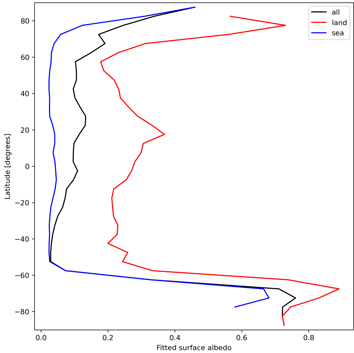
Figure 29: Zonal average of “Fitted surface albedo” for 2023-10-01 to 2023-10-02.
