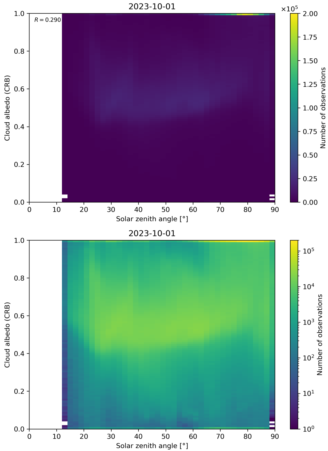
Figure 98: Scatter density plot of “Solar zenith angle” against “Cloud albedo (CRB)” for 2023-10-01 to 2023-10-02.
