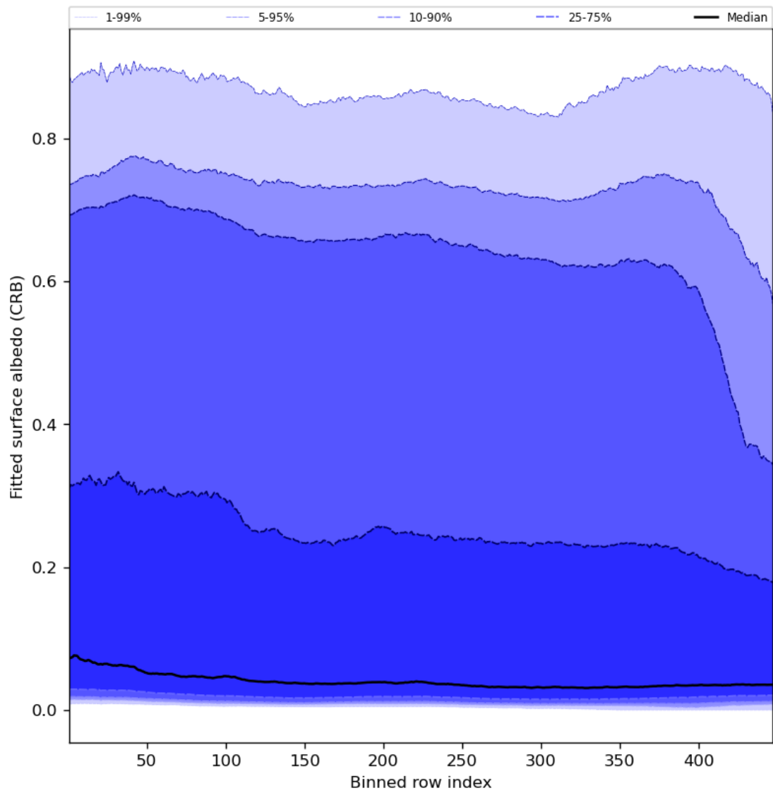
Figure 62: Along track statistics of “Fitted surface albedo (CRB)” for 2023-10-01 to 2023-10-02
