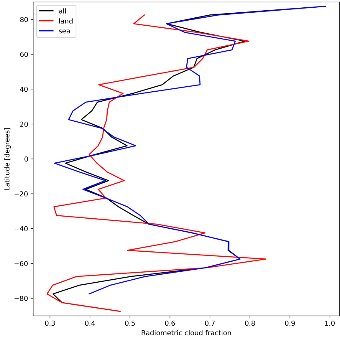
Figure 23: Zonal average of “Radiometric cloud fraction” for 2023-10-01 to 2023-10-02.
