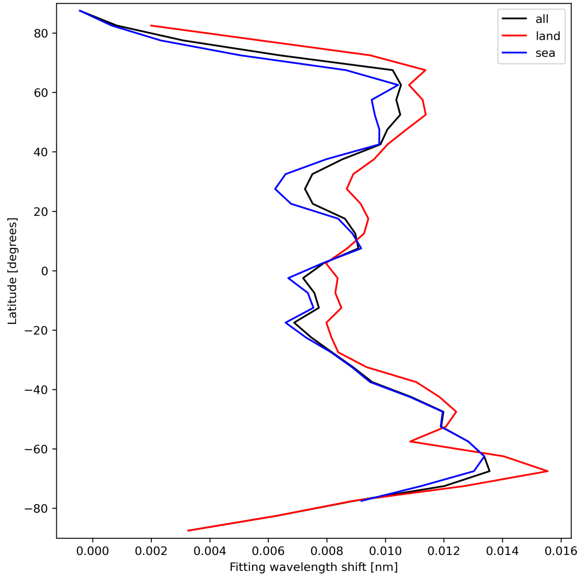
Figure 33: Zonal average of “Fitting wavelength shift” for 2023-10-01 to 2023-10-02.
