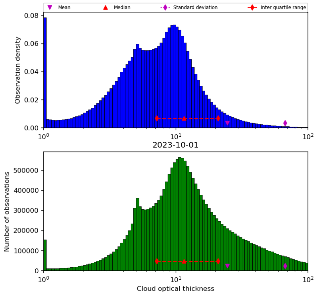
Figure 41: Histogram of “Cloud optical thickness” for 2023-10-01 to 2023-10-02
