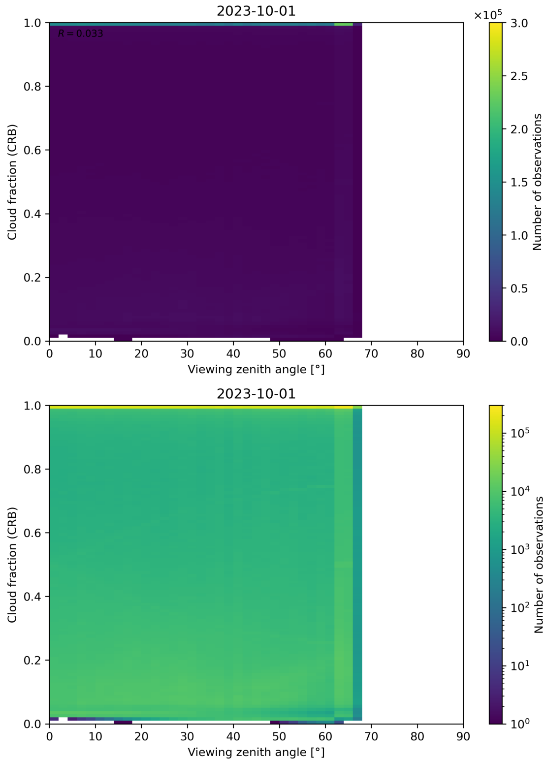
Figure 109: Scatter density plot of “Viewing zenith angle” against “Cloud fraction (CRB)” for 2023-10-01 to 2023-10-02.
