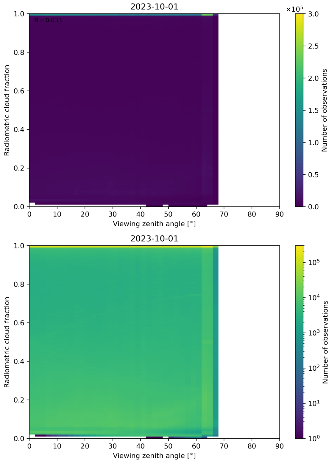
Figure 107: Scatter density plot of “Viewing zenith angle” against “Radiometric cloud fraction” for 2023-10-01 to 2023-10-02.
