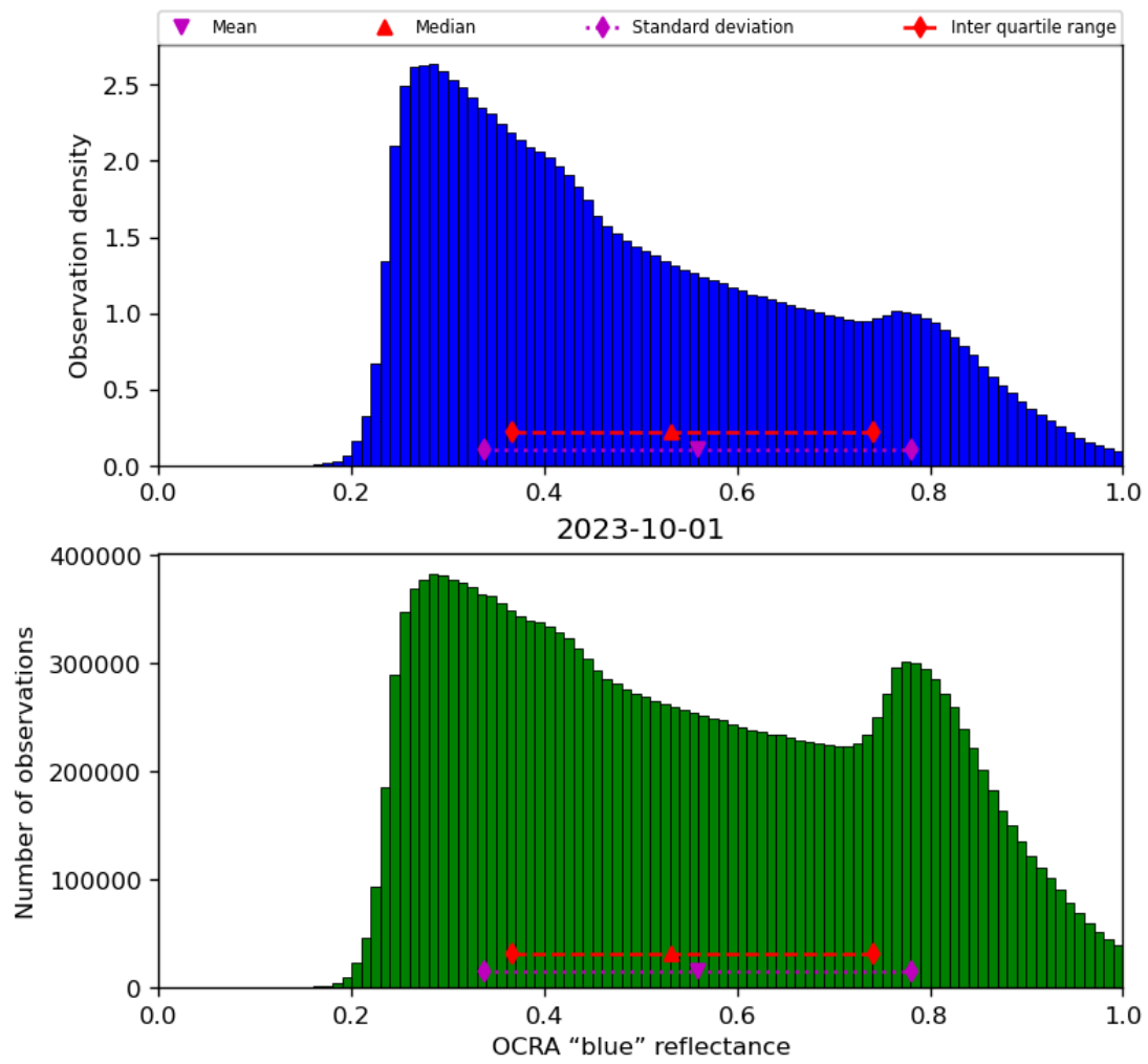
Figure 51: Histogram of “OCRA “blue” reflectance” for 2023-10-01 to 2023-10-02
