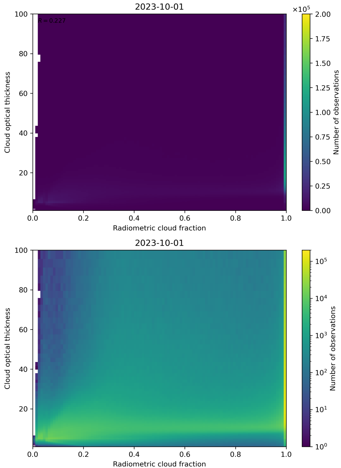
Figure 75: Scatter density plot of “Radiometric cloud fraction” against “Cloud optical thickness” for 2023-10-01 to 2023-10-02.
