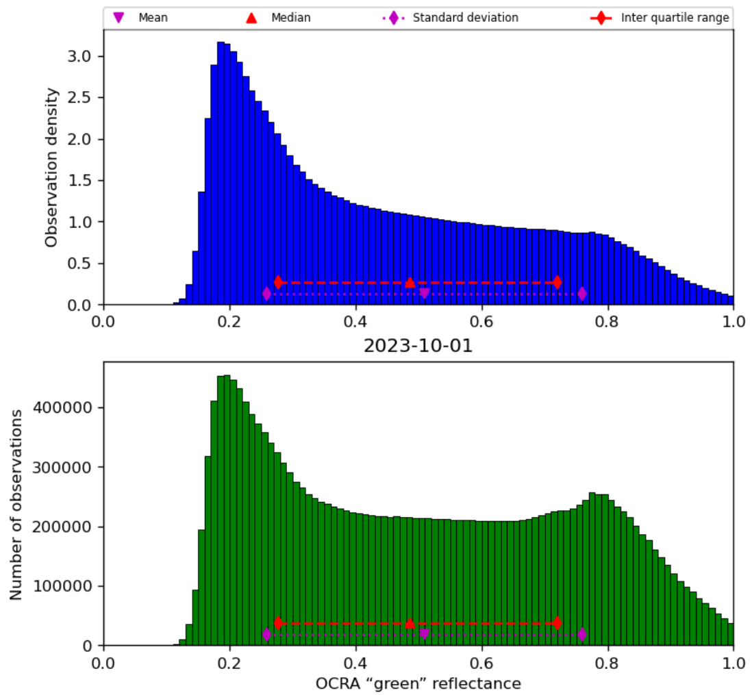
Figure 52: Histogram of “OCRA “green” reflectance” for 2023-10-01 to 2023-10-02
