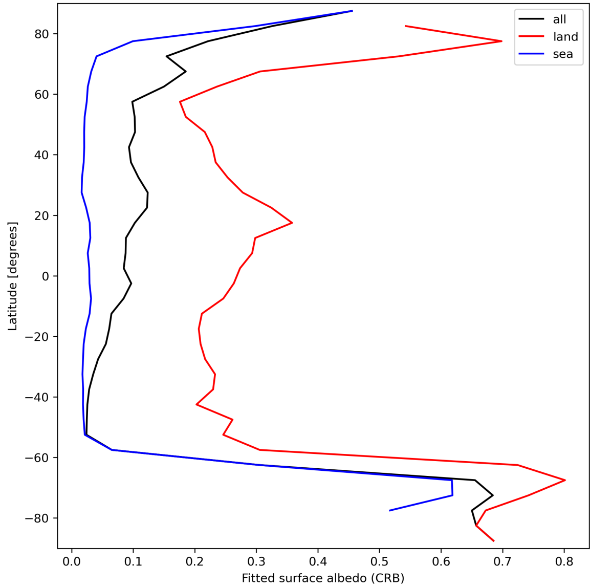
Figure 30: Zonal average of “Fitted surface albedo (CRB)” for 2023-10-01 to 2023-10-02.
