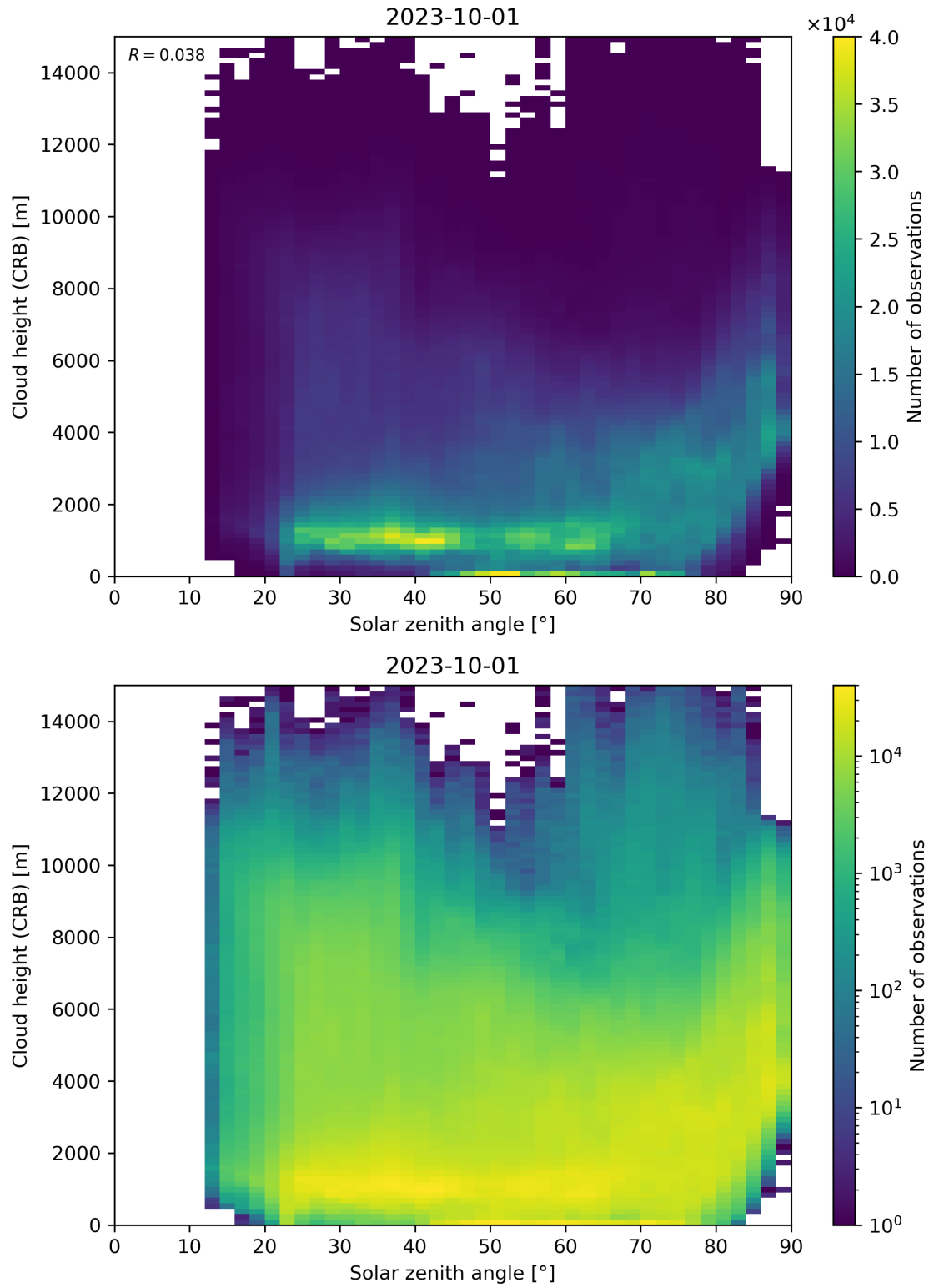
Figure 102: Scatter density plot of “Solar zenith angle” against “Cloud height (CRB)” for 2023-10-01 to 2023-10-02.
