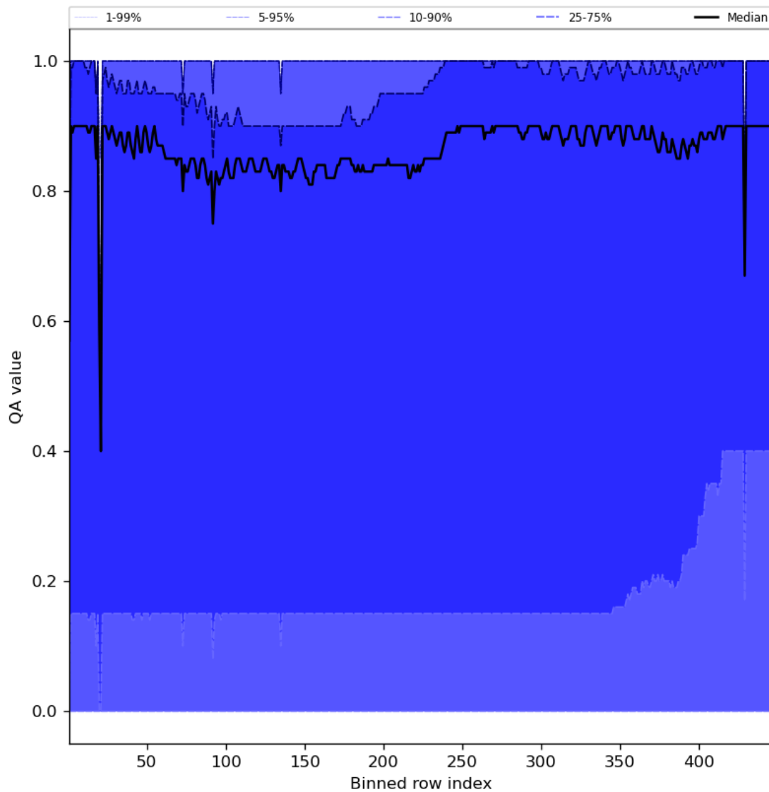
Figure 54: Along track statistics of “QA value” for 2023-10-01 to 2023-10-02
