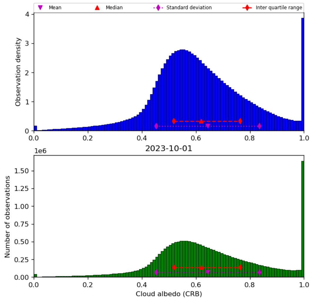
Figure 44: Histogram of “Cloud albedo (CRB)” for 2023-10-01 to 2023-10-02
