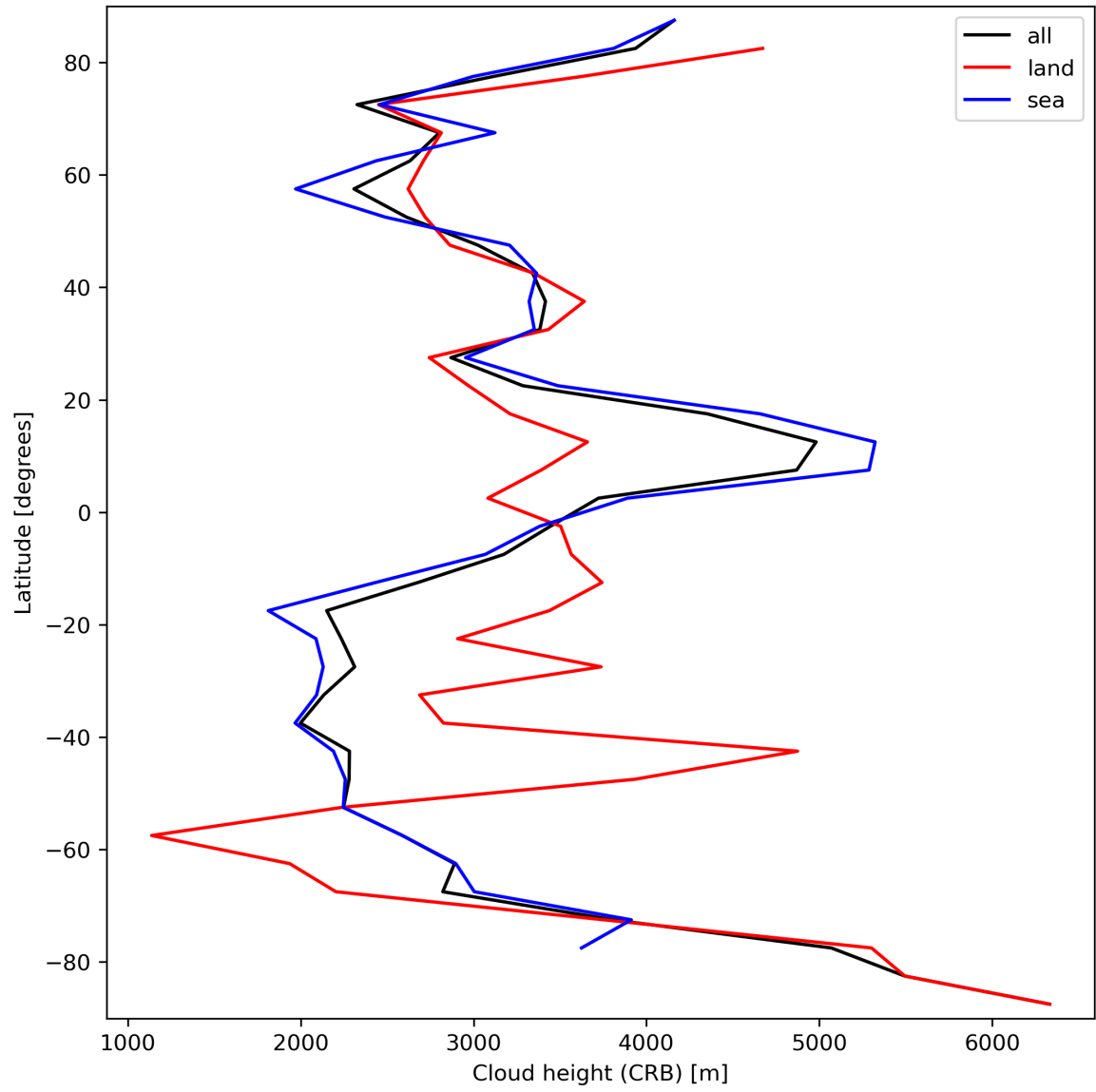
Figure 27: Zonal average of “Cloud height (CRB)” for 2023-10-01 to 2023-10-02.
