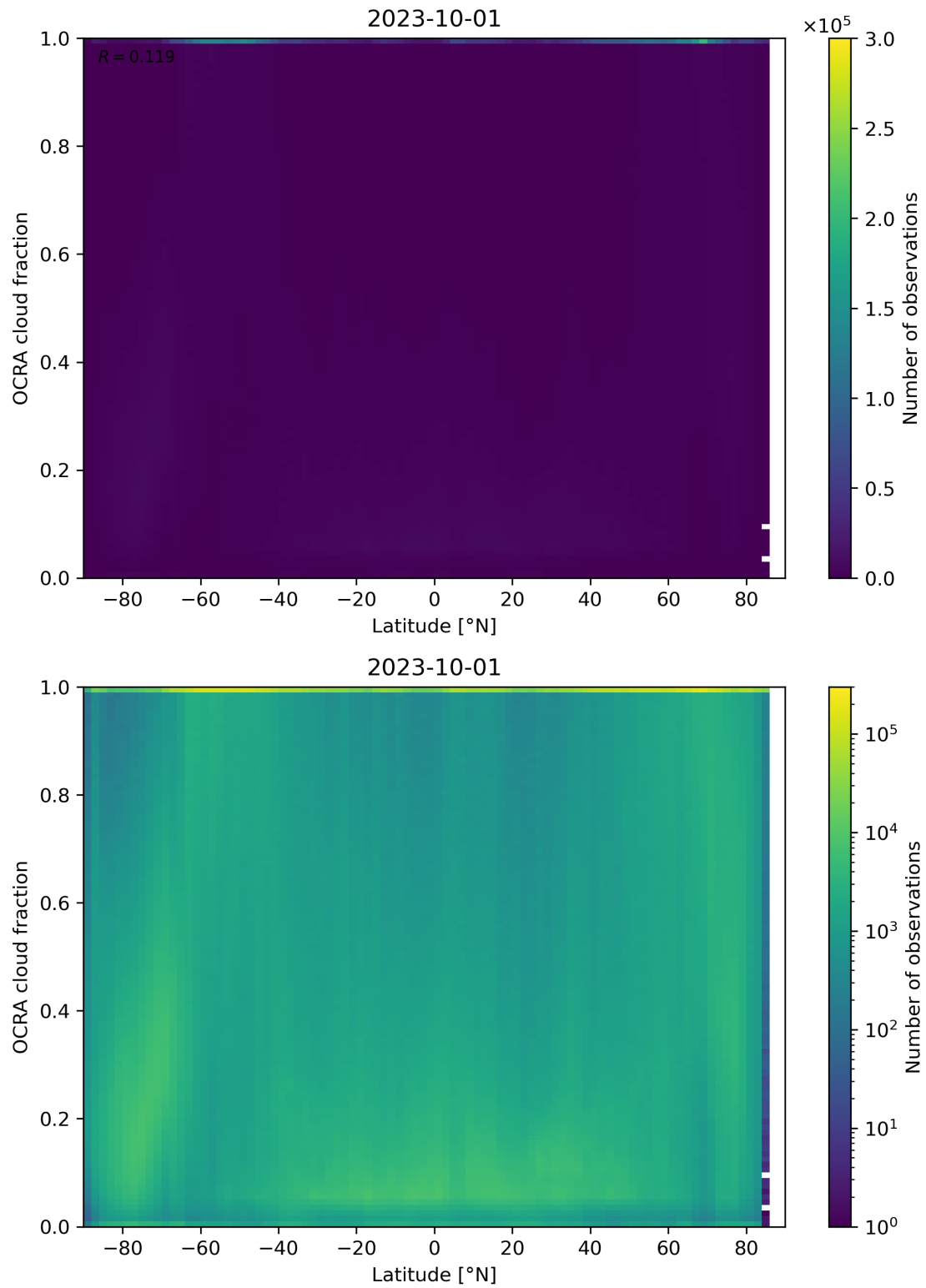
Figure 93: Scatter density plot of “Latitude” against “OCRA cloud fraction” for 2023-10-01 to 2023-10-02.
