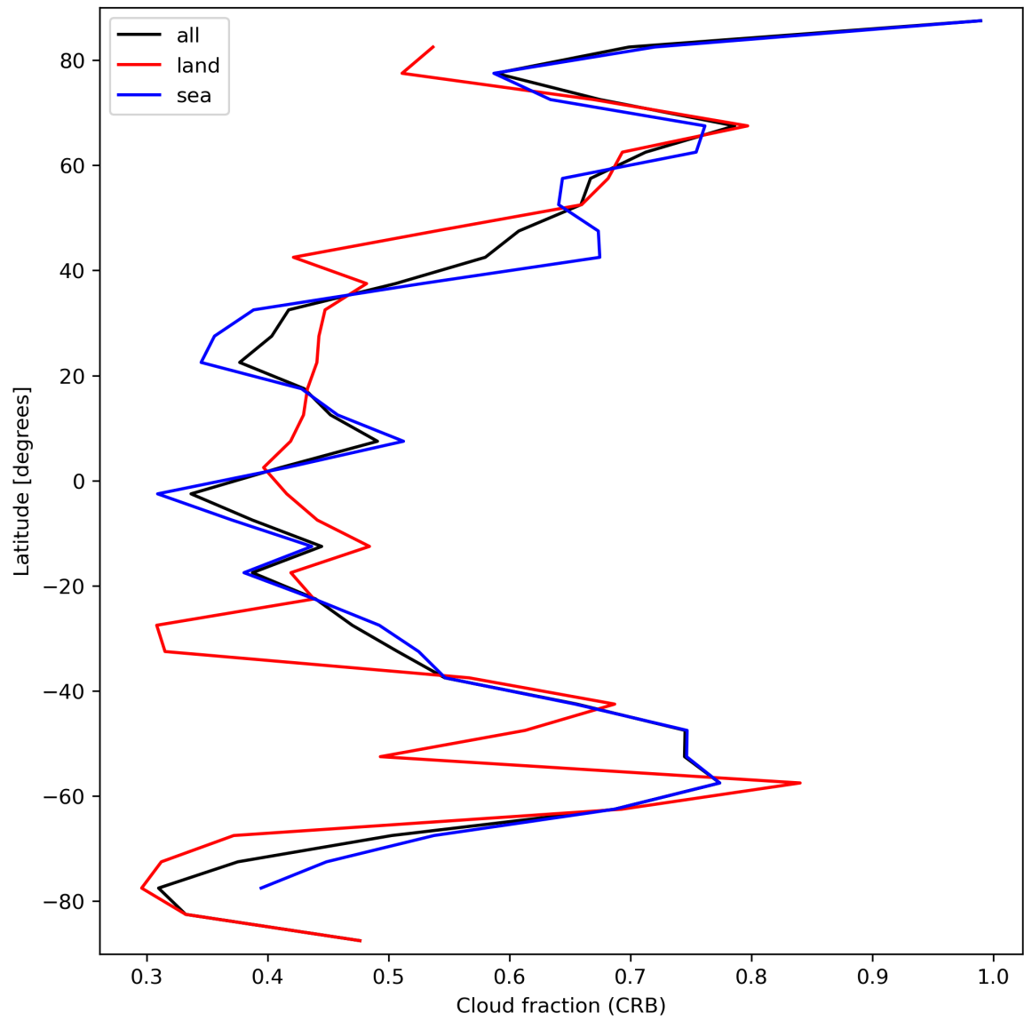
Figure 26: Zonal average of “Cloud fraction (CRB)” for 2023-10-01 to 2023-10-02.
