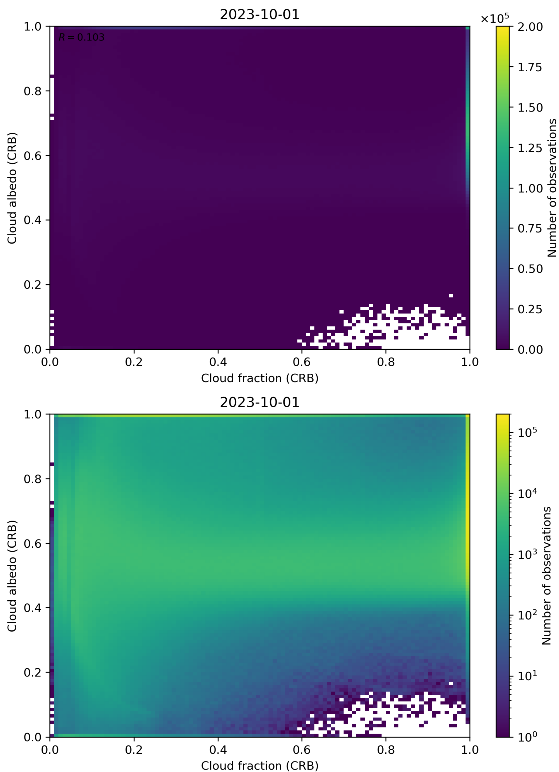
Figure 77: Scatter density plot of “Cloud fraction (CRB)” against “Cloud albedo (CRB)” for 2023-10-01 to 2023-10-02.
