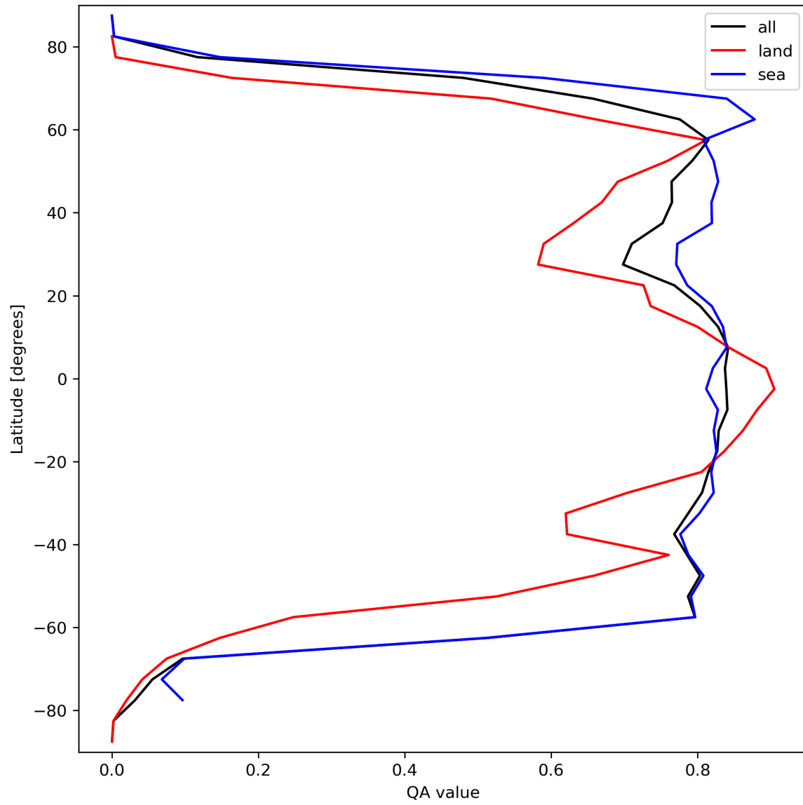
Figure 22: Zonal average of “QA value” for 2023-10-01 to 2023-10-02.
