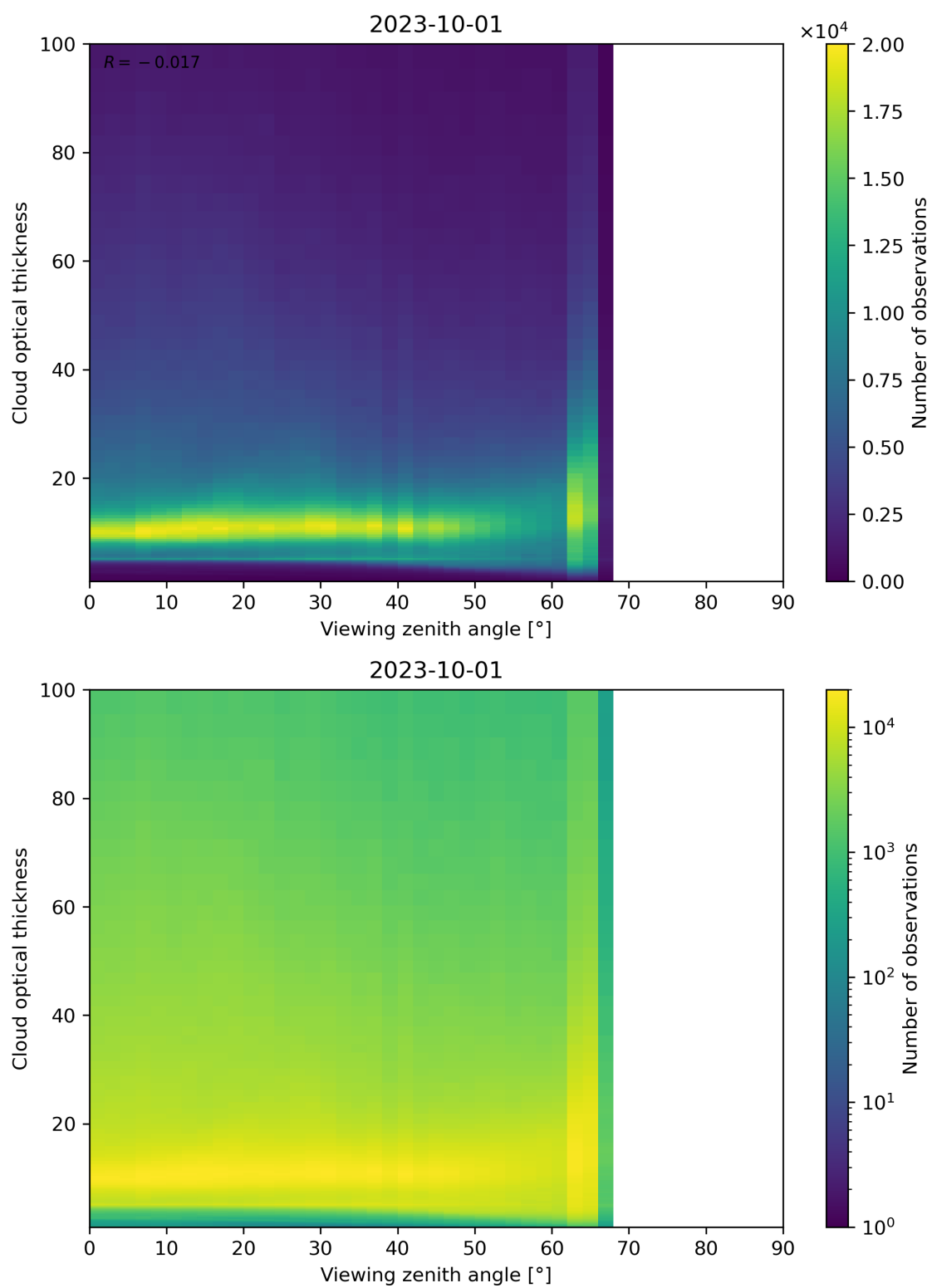
Figure 111: Scatter density plot of “Viewing zenith angle” against “Cloud optical thickness” for 2023-10-01 to 2023-10-02.
