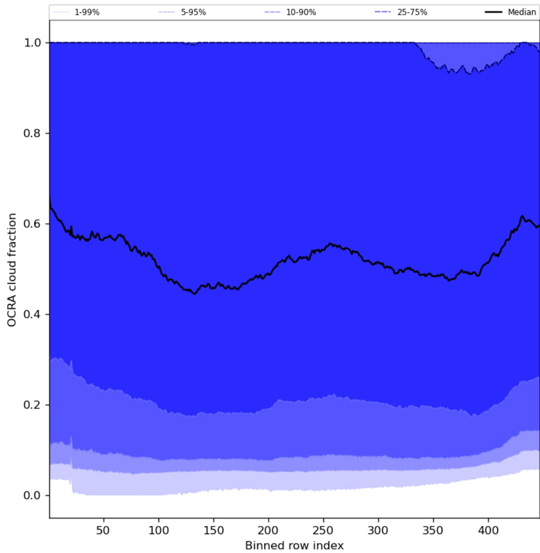
Figure 66: Along track statistics of “OCRA cloud fraction” for 2023-10-01 to 2023-10-02
