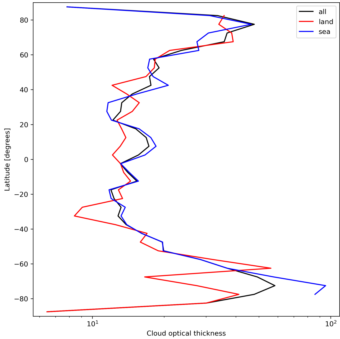
Figure 25: Zonal average of “Cloud optical thickness” for 2023-10-01 to 2023-10-02.
