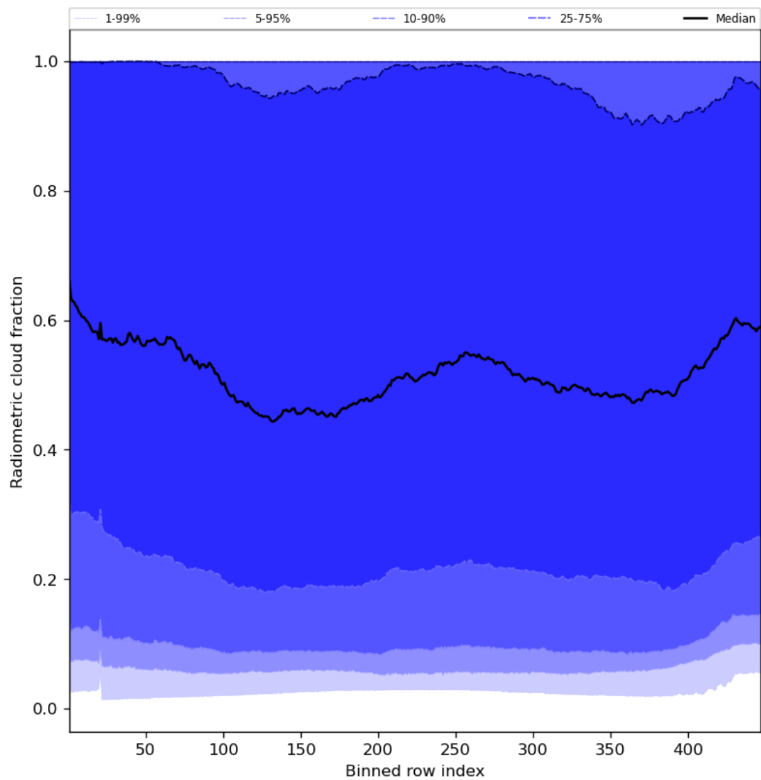
Figure 55: Along track statistics of “Radiometric cloud fraction” for 2023-10-01 to 2023-10-02
