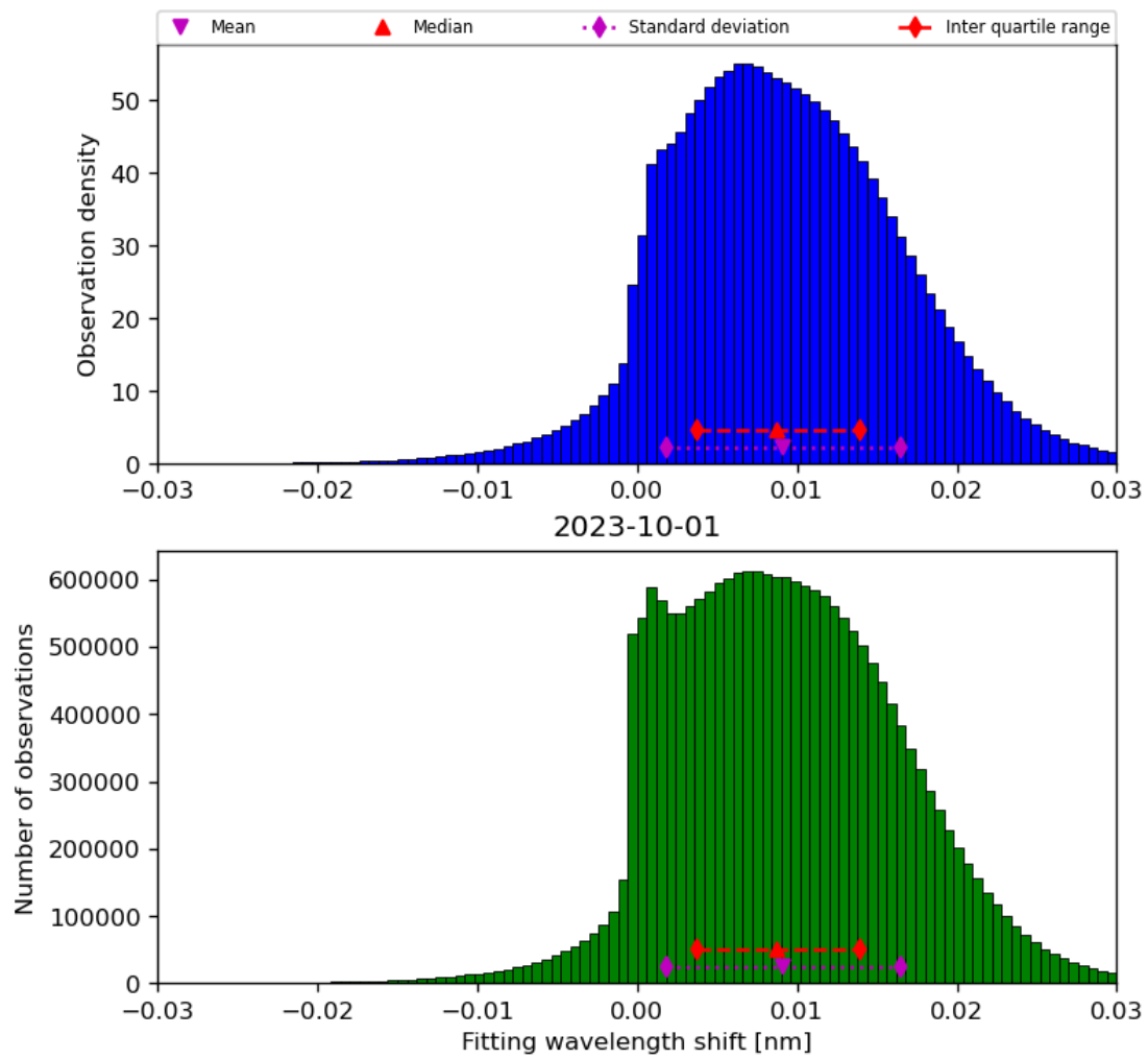
Figure 49: Histogram of “Fitting wavelength shift” for 2023-10-01 to 2023-10-02
