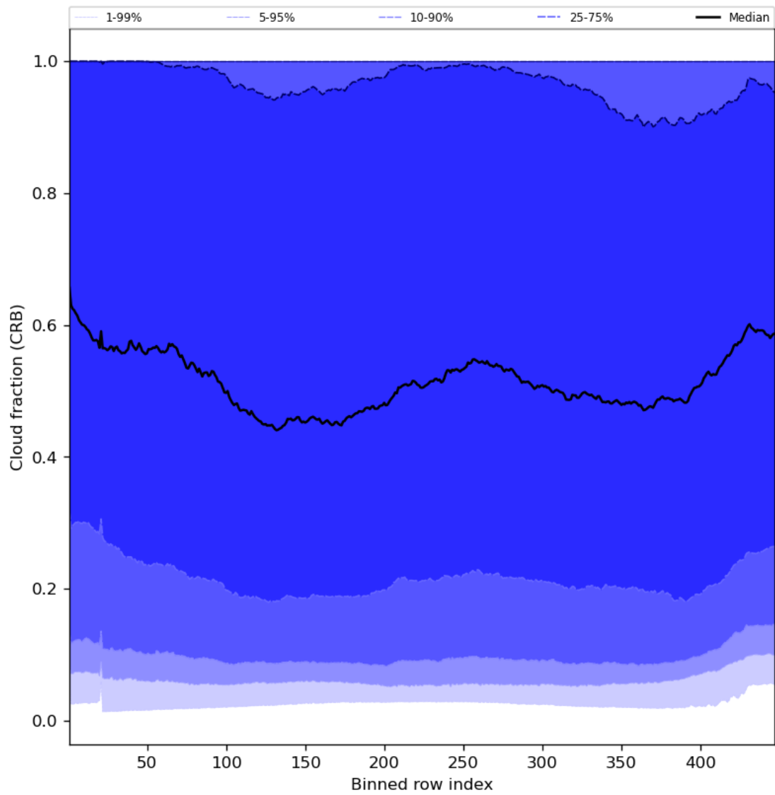
Figure 58: Along track statistics of “Cloud fraction (CRB)” for 2023-10-01 to 2023-10-02
