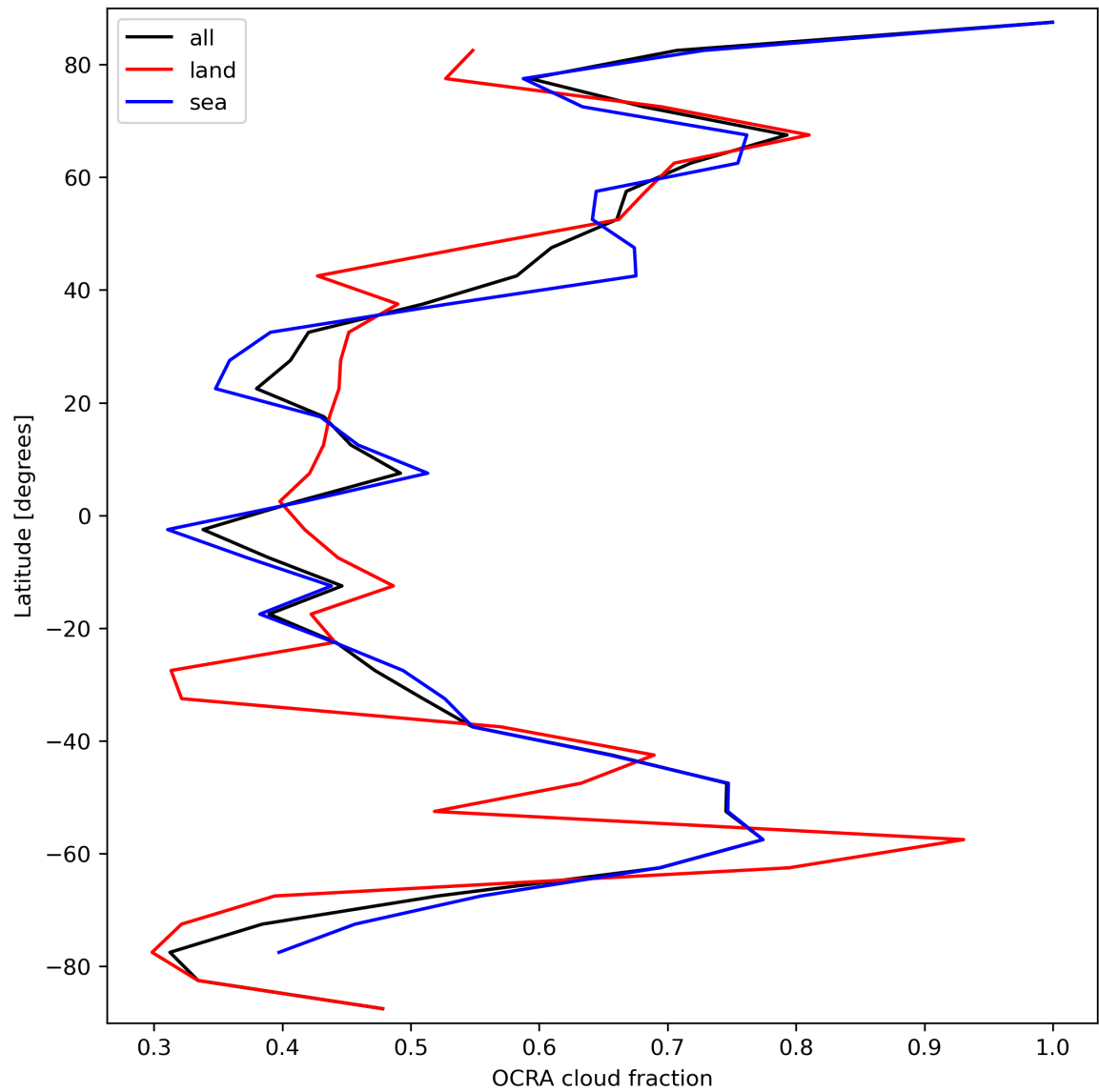
Figure 34: Zonal average of “OCRA cloud fraction” for 2023-10-01 to 2023-10-02.
