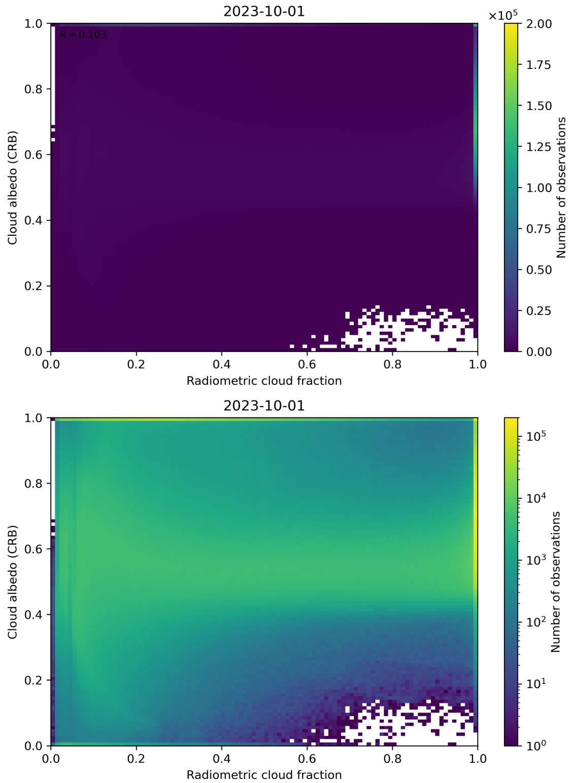
Figure 71: Scatter density plot of “Radiometric cloud fraction” against “Cloud albedo (CRB)” for 2023-10-01 to 2023-10-02.
