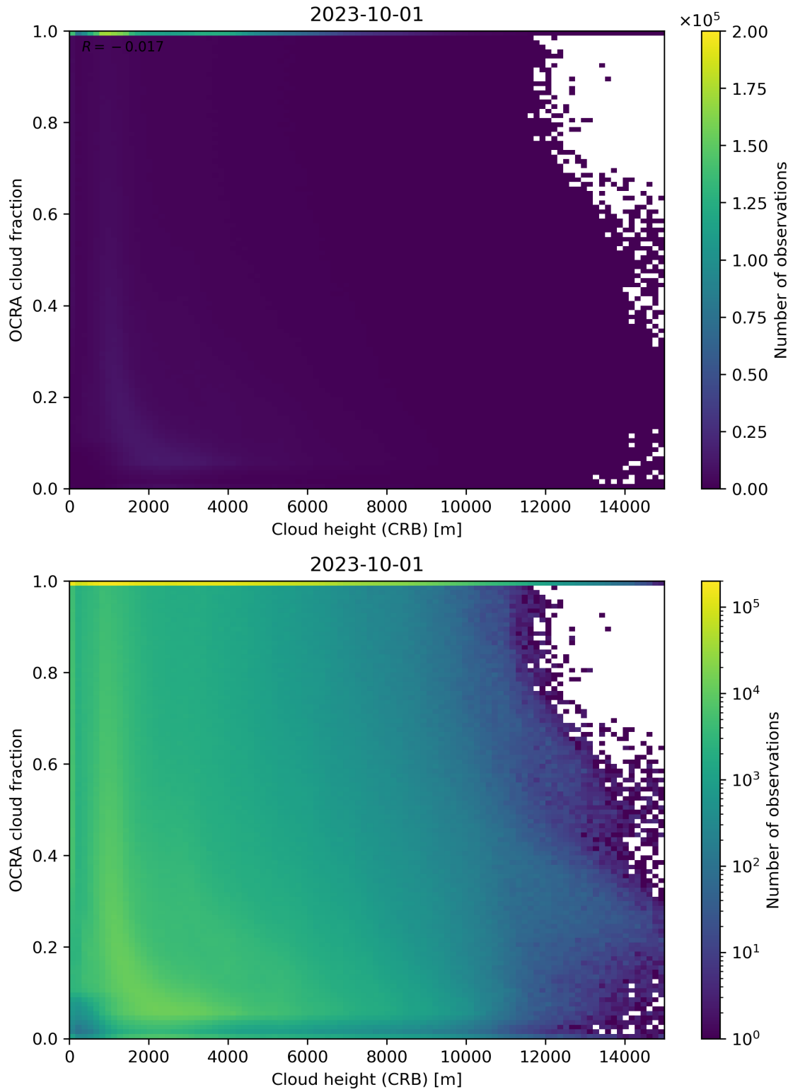
Figure 81: Scatter density plot of “Cloud height (CRB)” against “OCRA cloud fraction” for 2023-10-01 to 2023-10-02.
