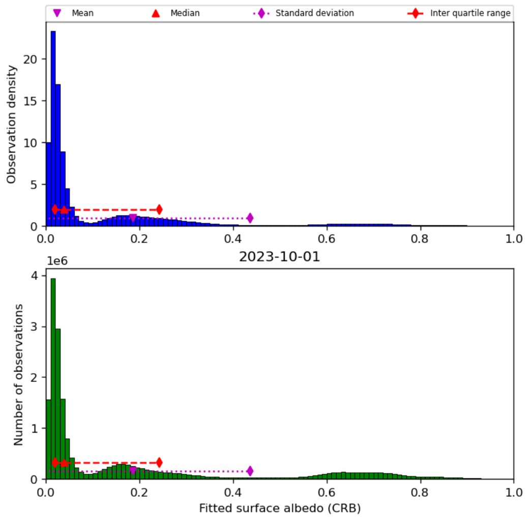
Figure 46: Histogram of “Fitted surface albedo (CRB)” for 2023-10-01 to 2023-10-02
