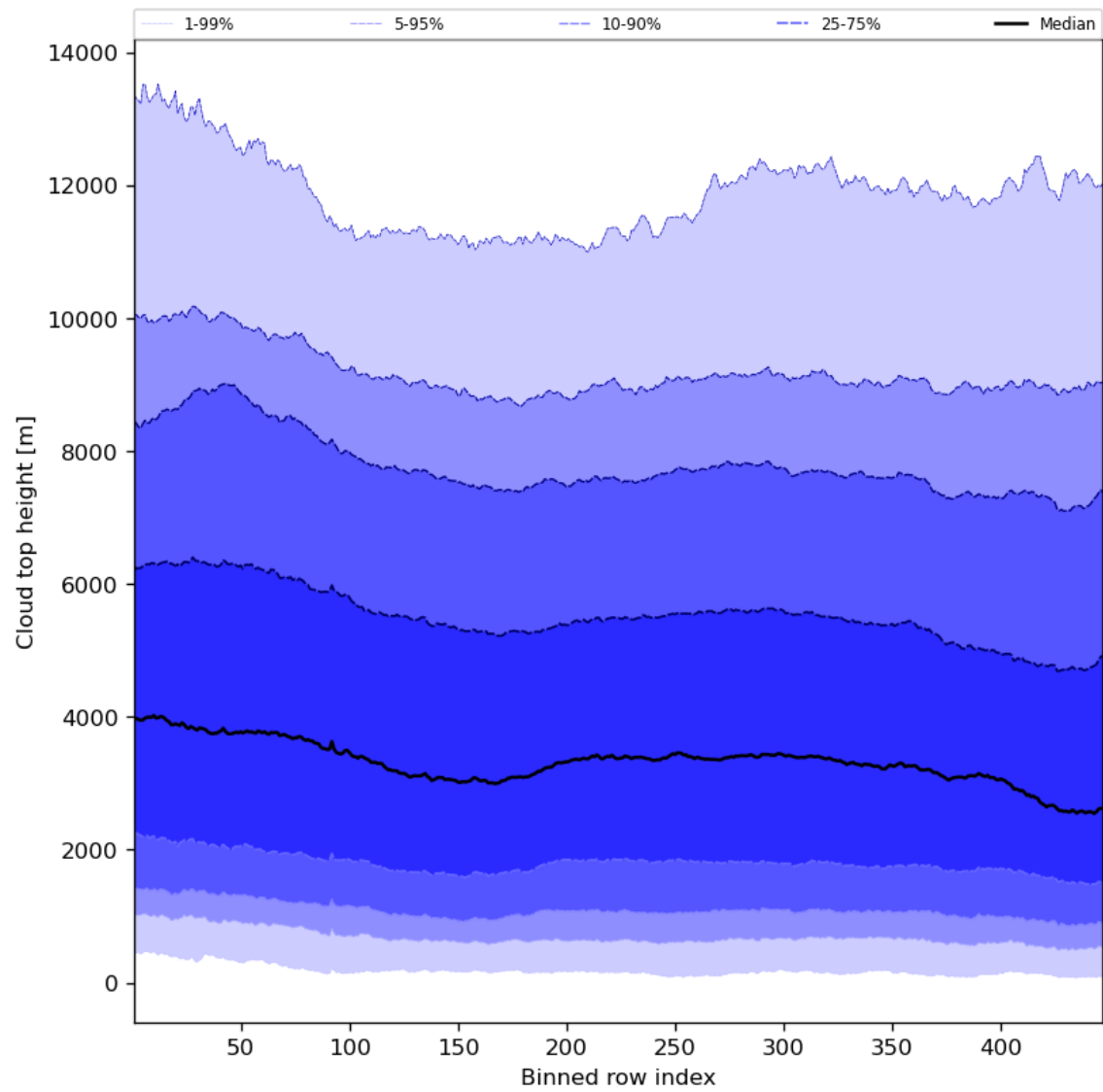
Figure 56: Along track statistics of “Cloud top height” for 2023-10-01 to 2023-10-02
