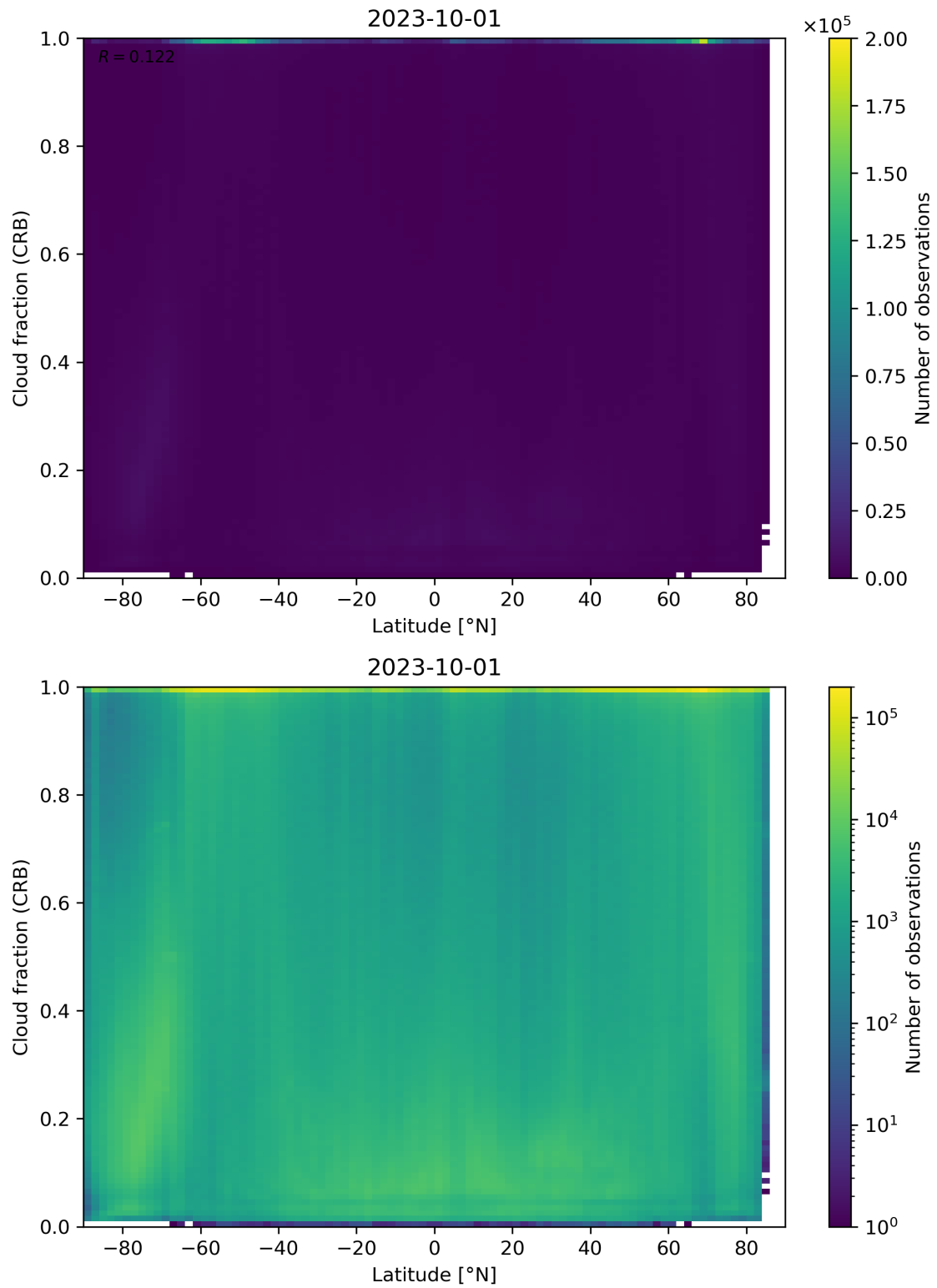
Figure 94: Scatter density plot of “Latitude” against “Cloud fraction (CRB)” for 2023-10-01 to 2023-10-02.
