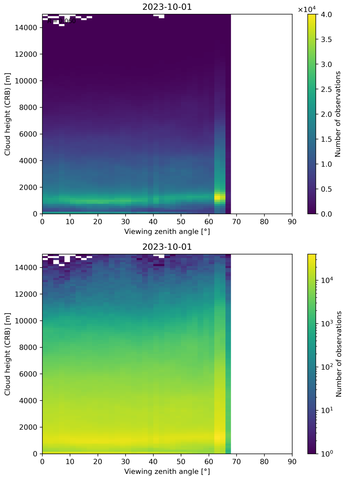
Figure 110: Scatter density plot of “Viewing zenith angle” against “Cloud height (CRB)” for 2023-10-01 to 2023-10-02.
