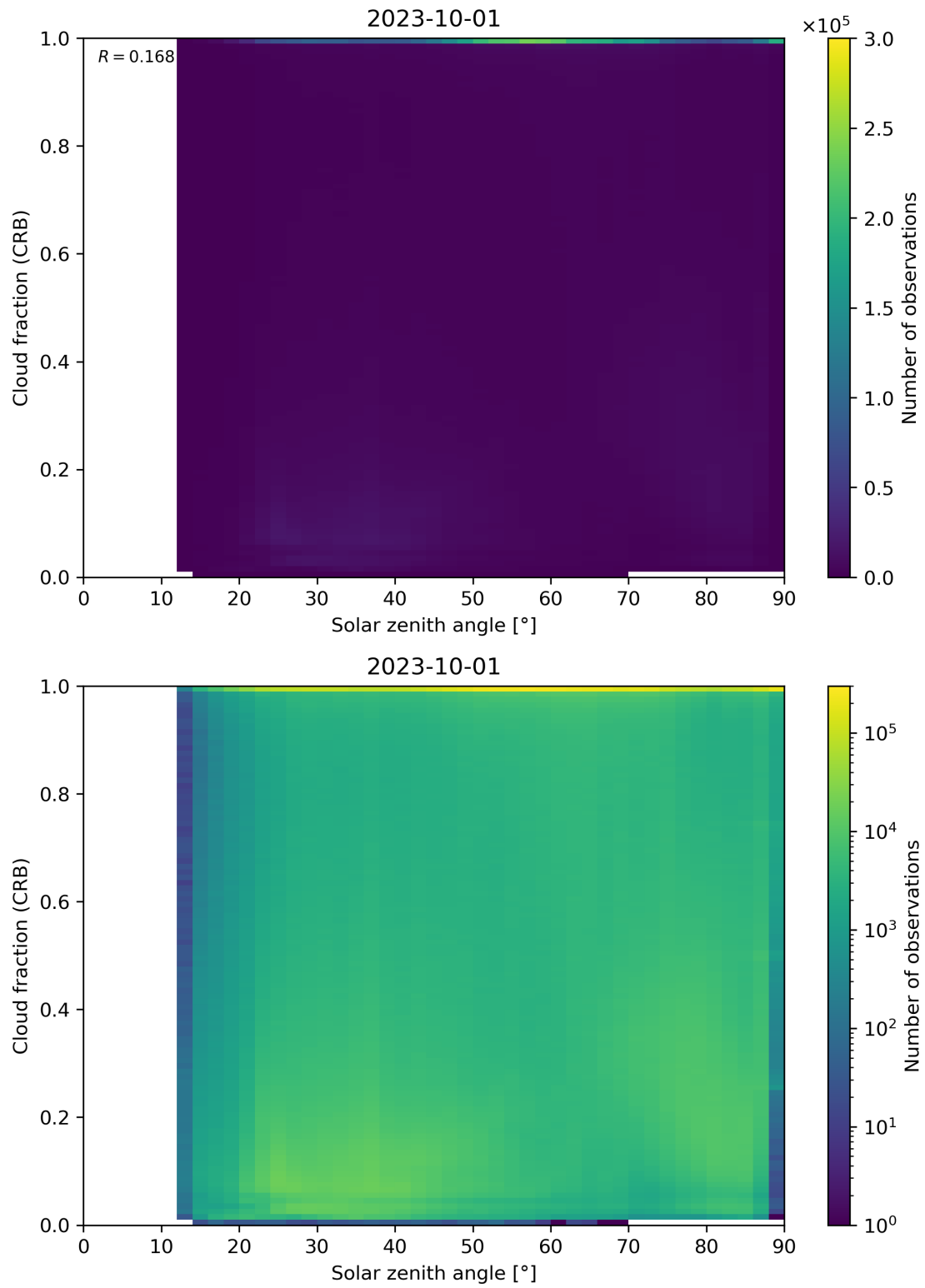
Figure 101: Scatter density plot of “Solar zenith angle” against “Cloud fraction (CRB)” for 2023-10-01 to 2023-10-02.
