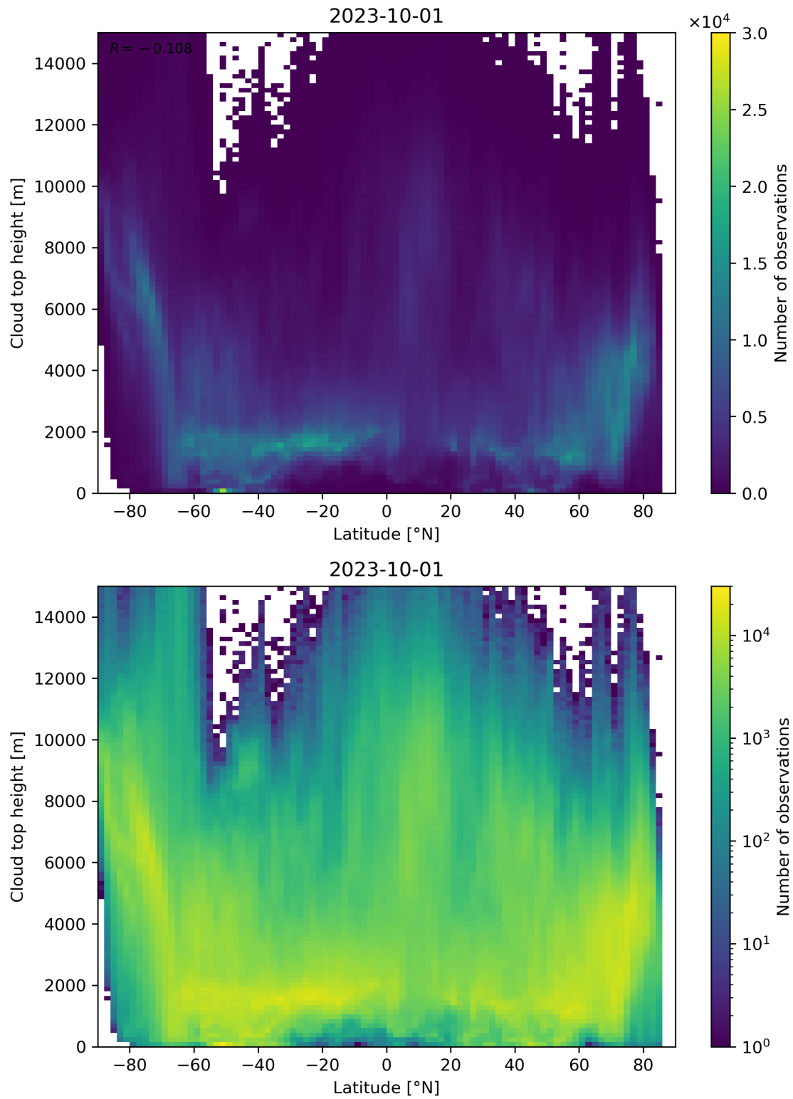
Figure 97: Scatter density plot of “Latitude” against “Cloud top height” for 2023-10-01 to 2023-10-02.
