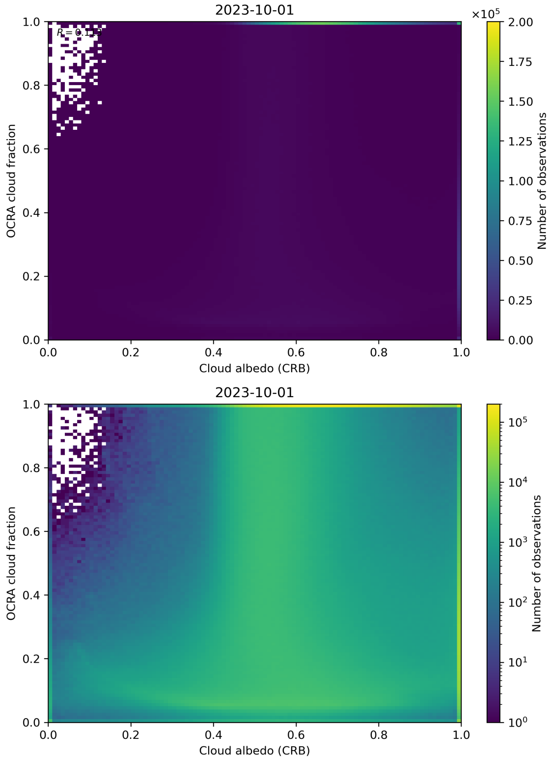
Figure 70: Scatter density plot of “Cloud albedo (CRB)” against “OCRA cloud fraction” for 2023-10-01 to 2023-10-02.
