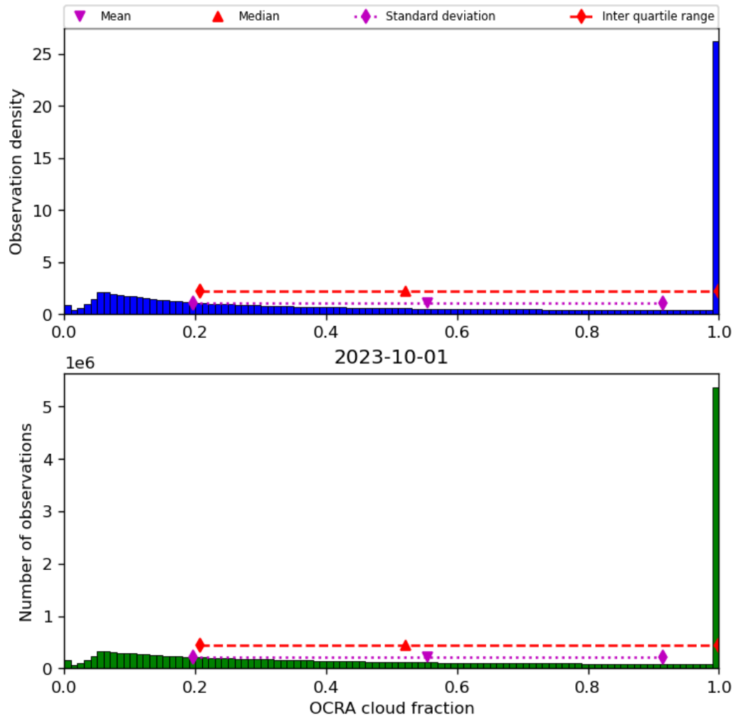
Figure 50: Histogram of “OCRA cloud fraction” for 2023-10-01 to 2023-10-02
