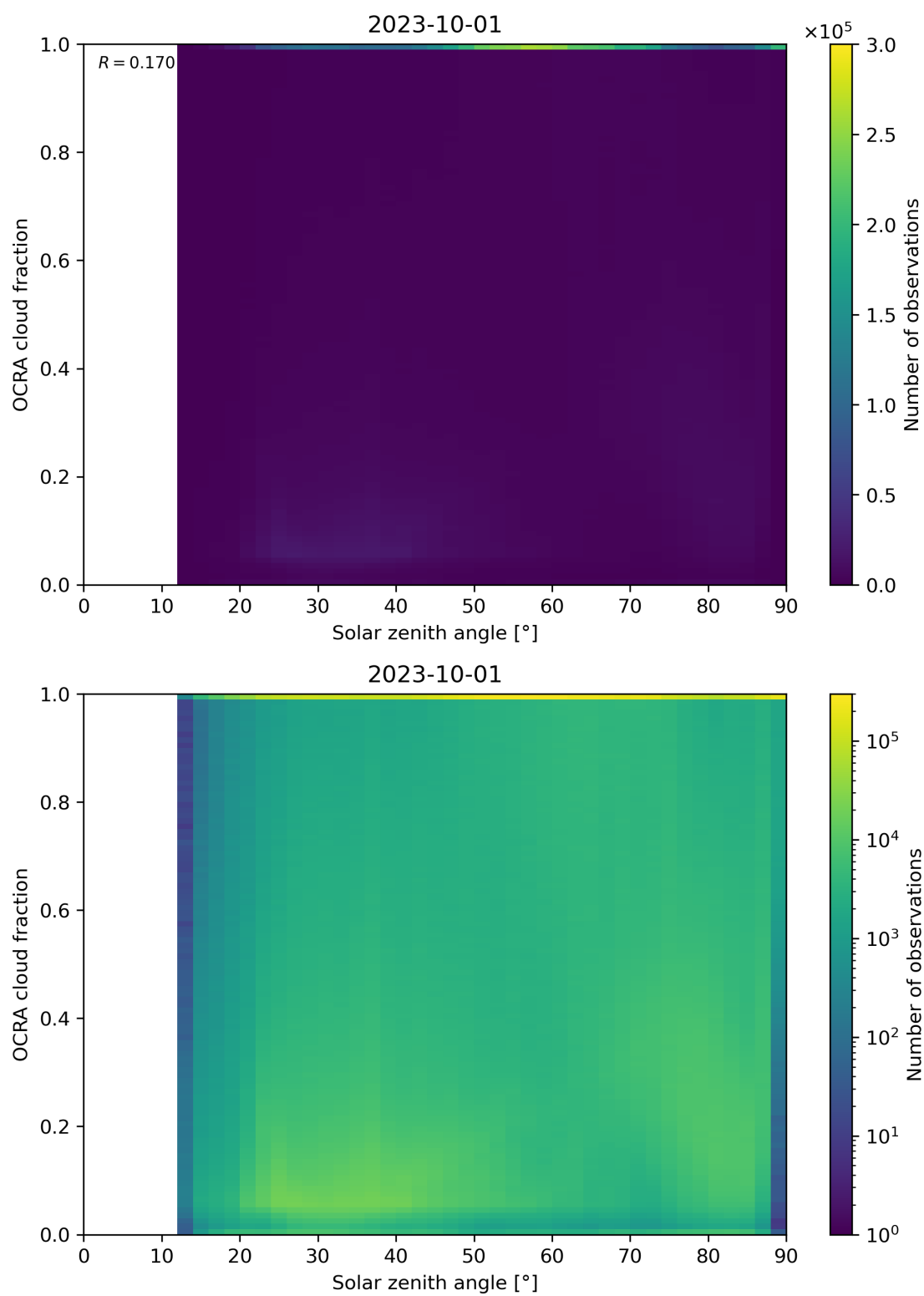
Figure 100: Scatter density plot of “Solar zenith angle” against “OCRA cloud fraction” for 2023-10-01 to 2023-10-02.
