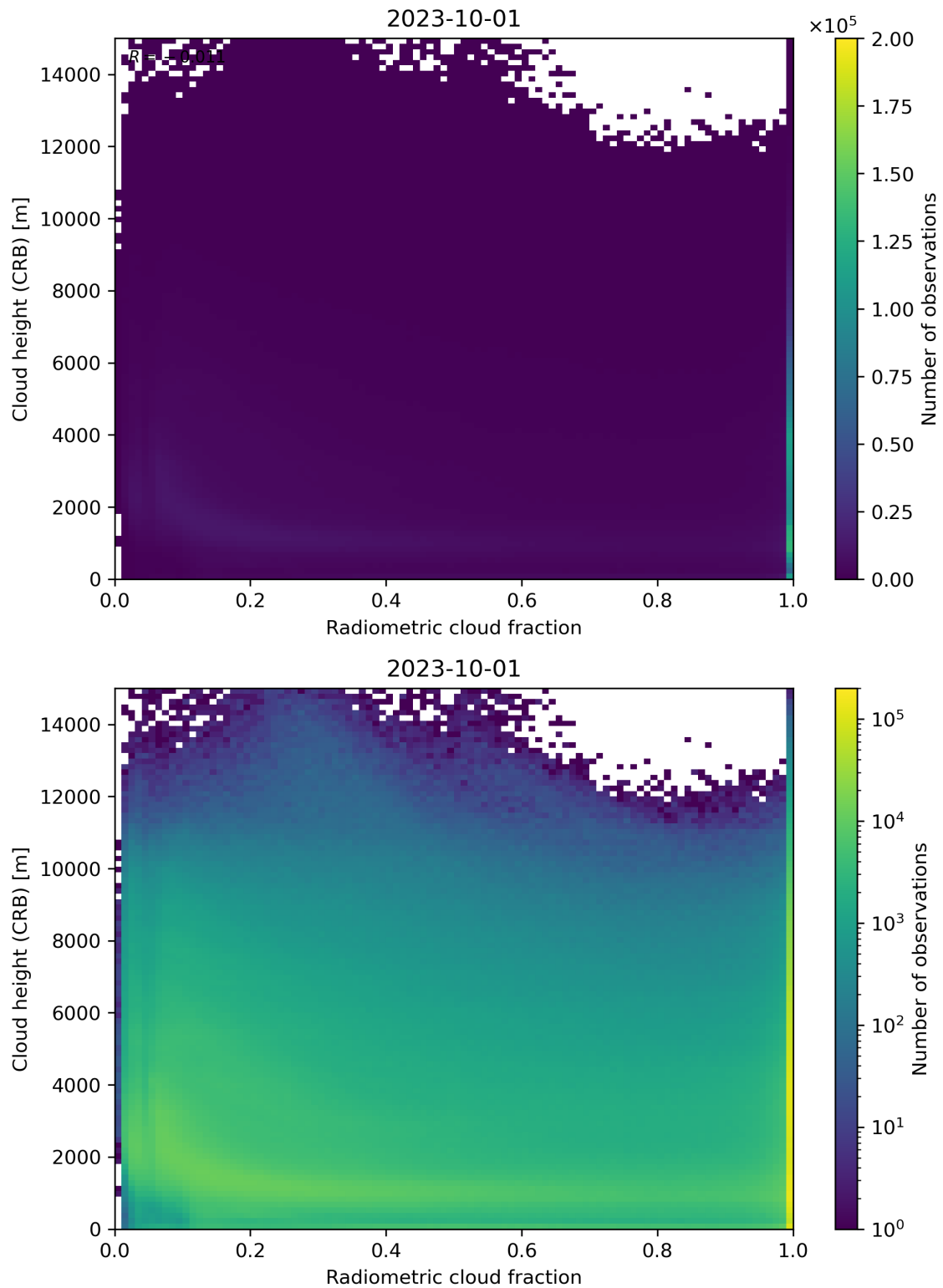
Figure 74: Scatter density plot of “Radiometric cloud fraction” against “Cloud height (CRB)” for 2023-10-01 to 2023-10-02.
