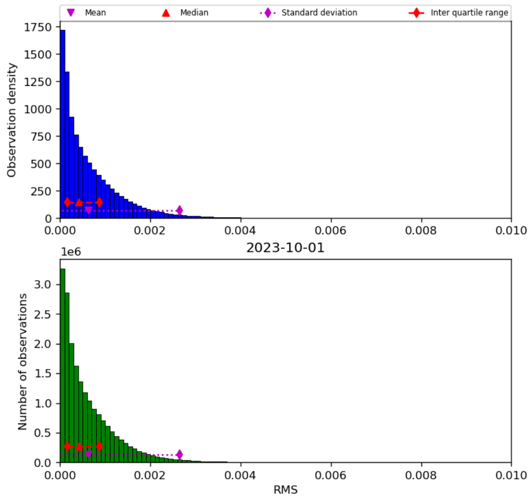
Figure 47: Histogram of “RMS” for 2023-10-01 to 2023-10-02
