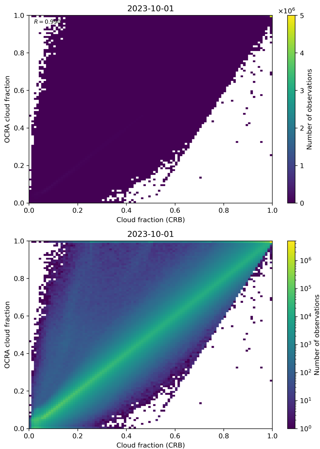
Figure 78: Scatter density plot of “Cloud fraction (CRB)” against “OCRA cloud fraction” for 2023-10-01 to 2023-10-02.
