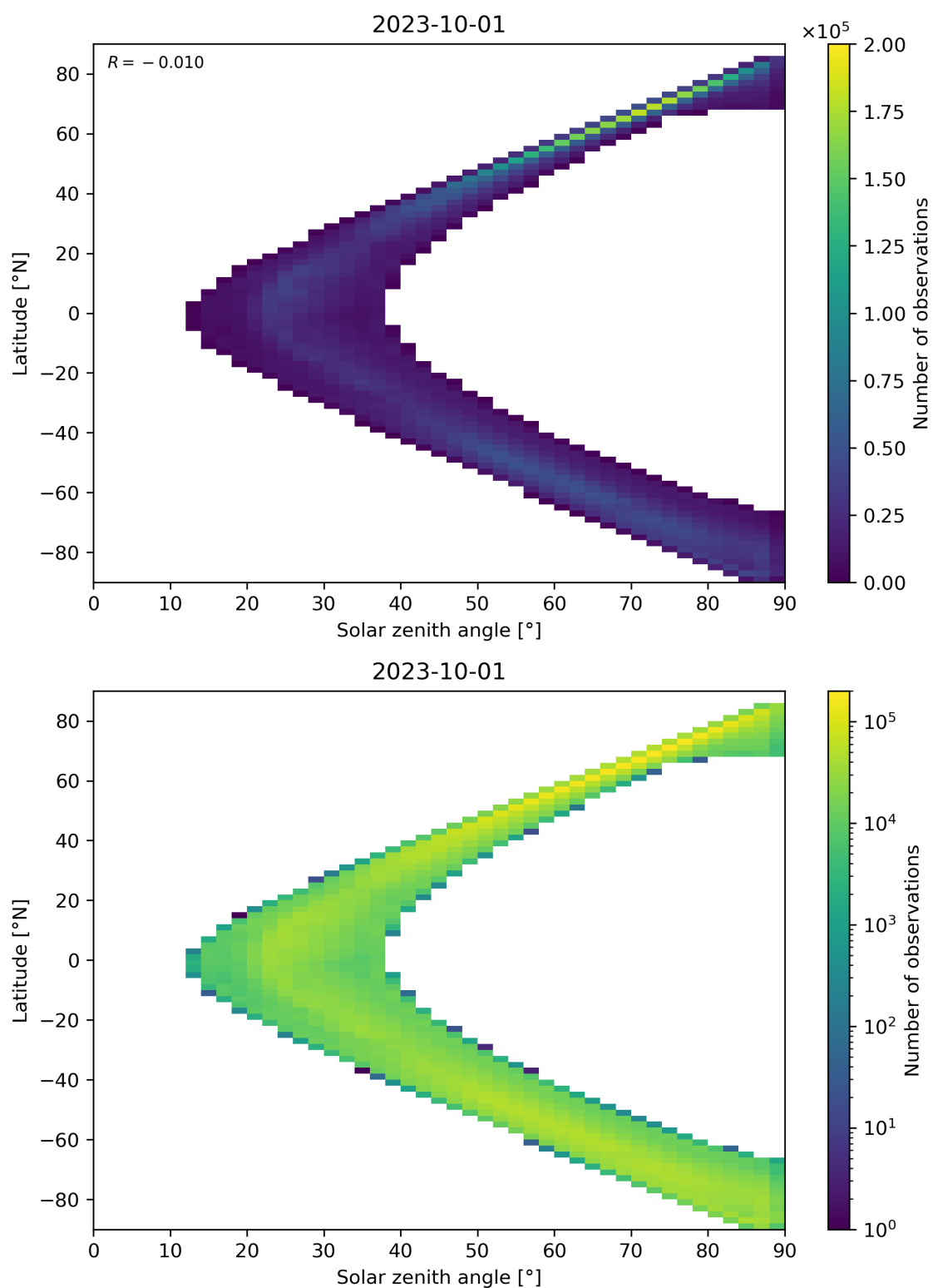
Figure 105: Scatter density plot of “Solar zenith angle” against “Latitude” for 2023-10-01 to 2023-10-02.
