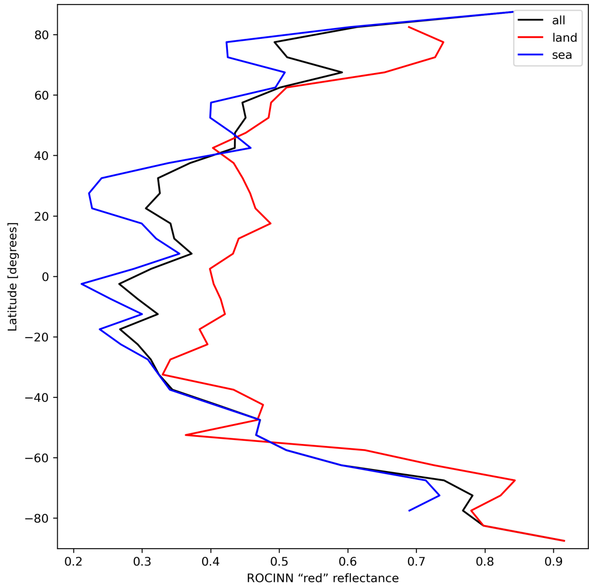
Figure 37: Zonal average of “ROCINN “red” reflectance” for 2023-10-01 to 2023-10-02.
