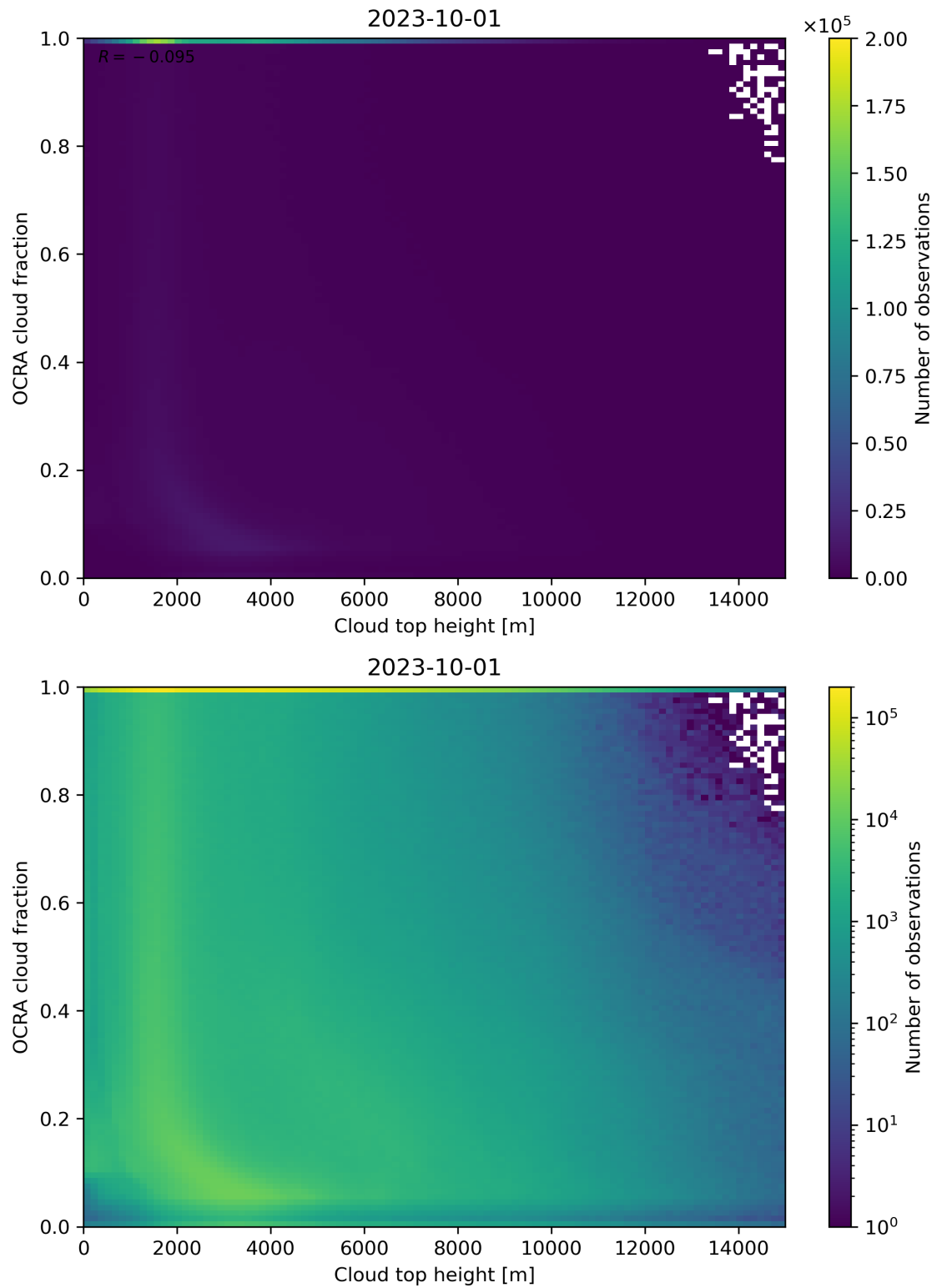
Figure 87: Scatter density plot of “Cloud top height” against “OCRA cloud fraction” for 2023-10-01 to 2023-10-02.
