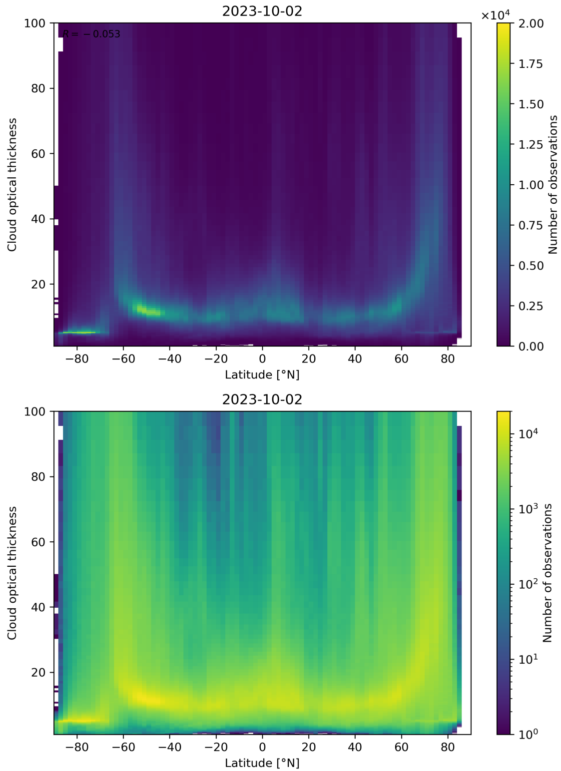
Figure 96: Scatter density plot of “Latitude” against “Cloud optical thickness” for 2023-10-01 to 2023-10-03.
