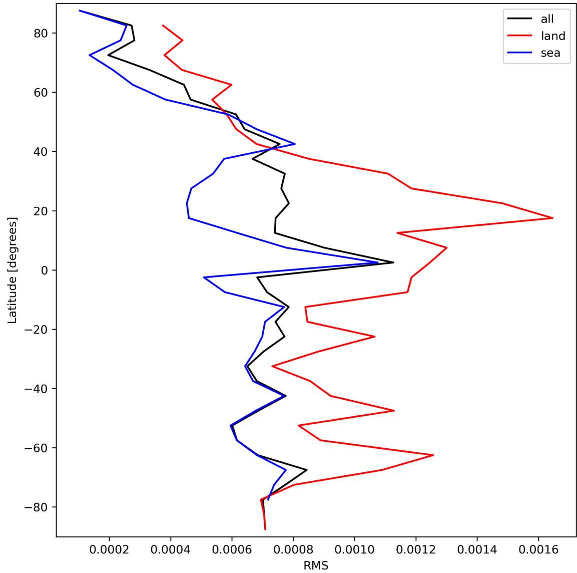
Figure 31: Zonal average of “RMS” for 2023-10-01 to 2023-10-03.
