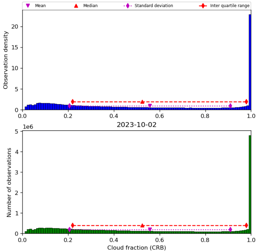
Figure 42: Histogram of “Cloud fraction (CRB)” for 2023-10-01 to 2023-10-03
