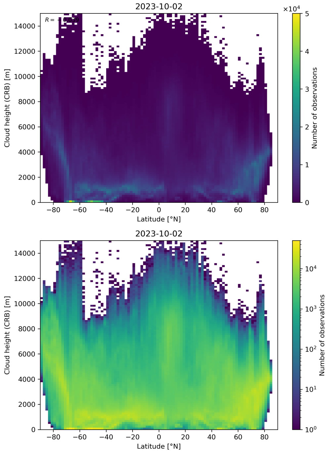
Figure 95: Scatter density plot of “Latitude” against “Cloud height (CRB)” for 2023-10-01 to 2023-10-03.
