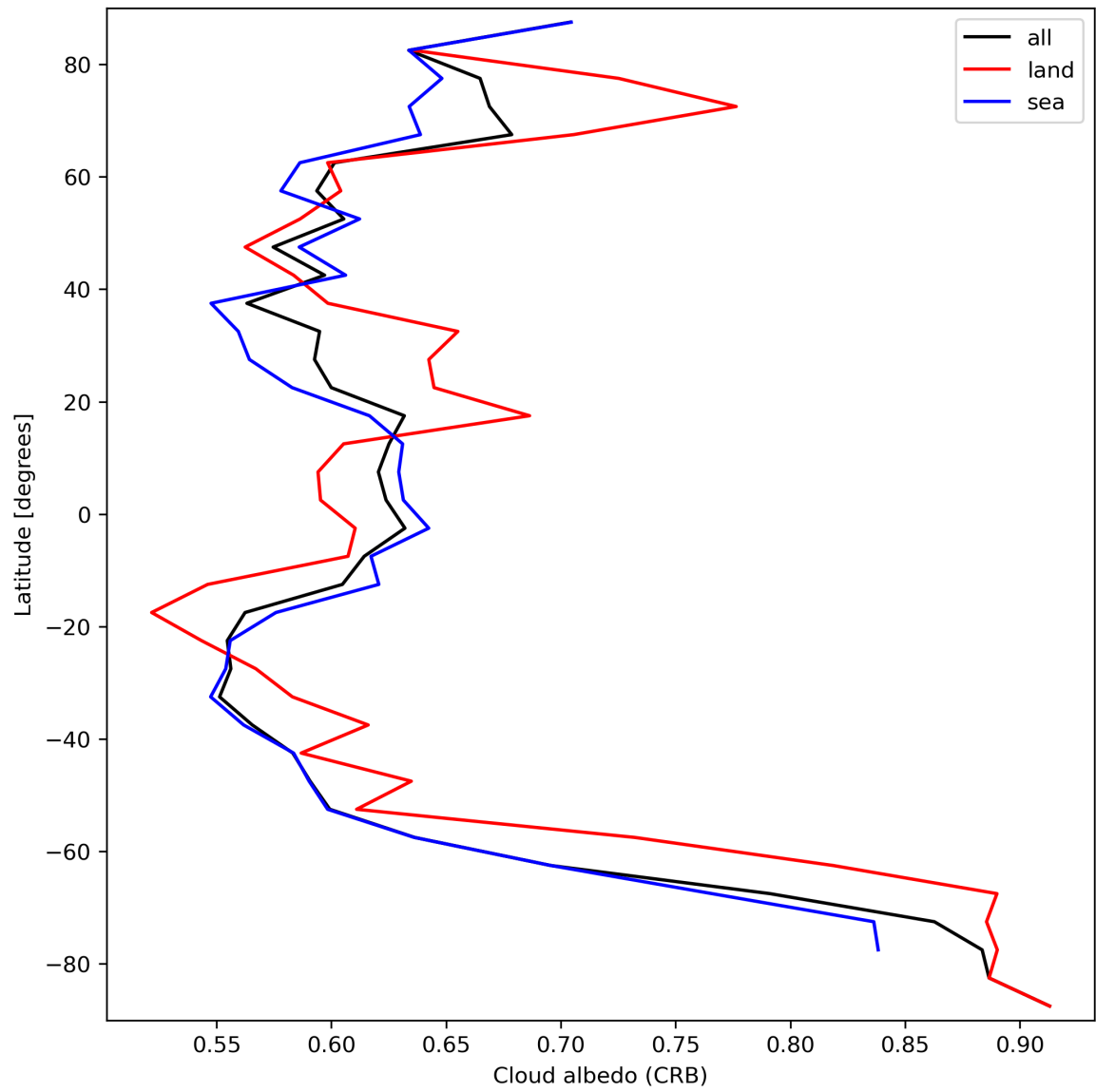
Figure 28: Zonal average of “Cloud albedo (CRB)” for 2023-10-01 to 2023-10-03.
