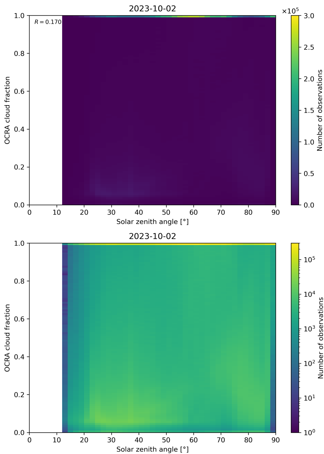
Figure 100: Scatter density plot of “Solar zenith angle” against “OCRA cloud fraction” for 2023-10-01 to 2023-10-03.
