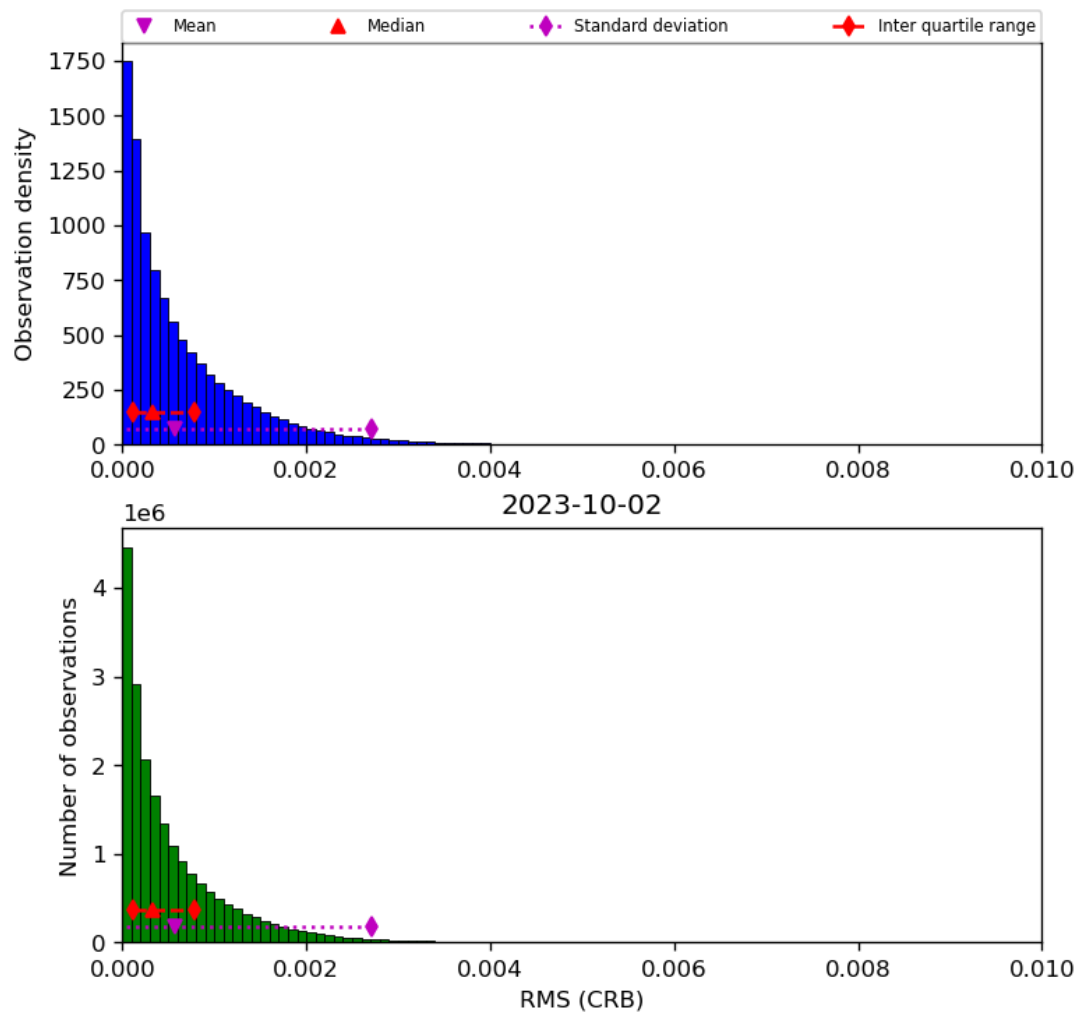
Figure 48: Histogram of “RMS (CRB)” for 2023-10-01 to 2023-10-03
