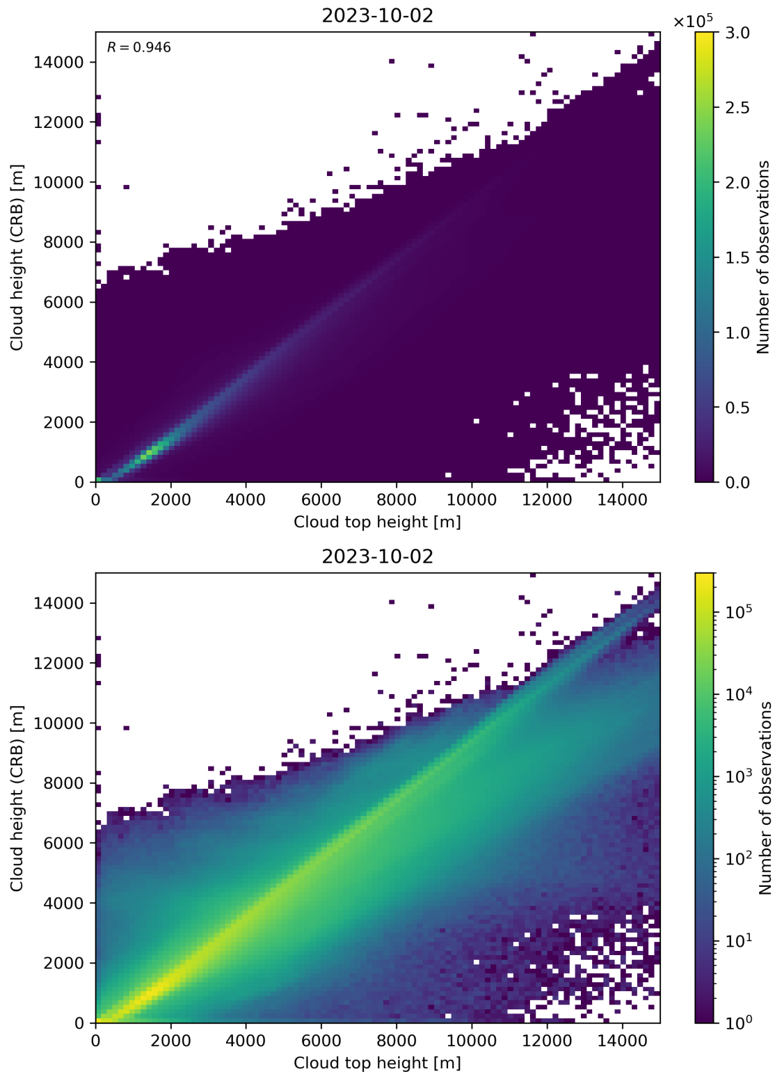
Figure 89: Scatter density plot of “Cloud top height” against “Cloud height (CRB)” for 2023-10-01 to 2023-10-03.
