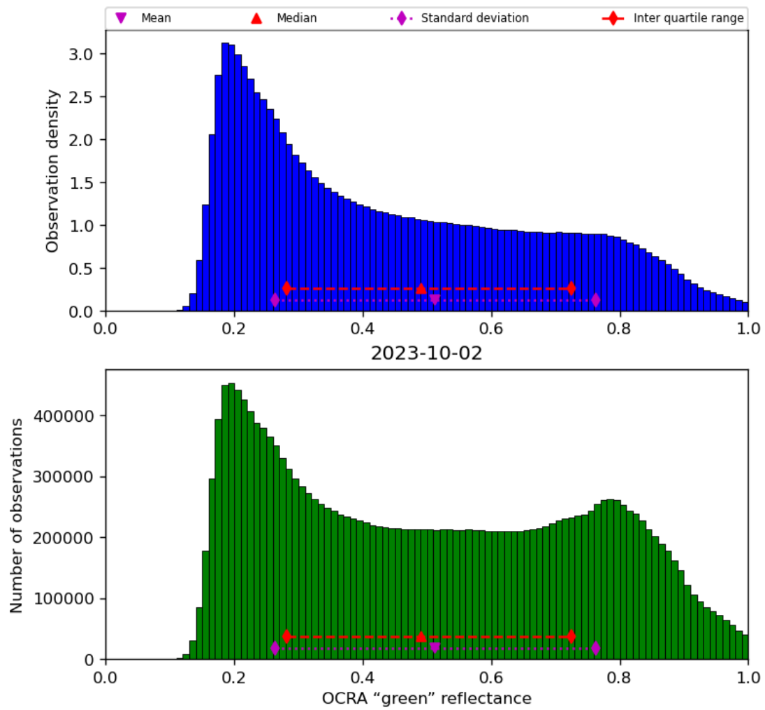
Figure 52: Histogram of “OCRA “green” reflectance” for 2023-10-01 to 2023-10-03
