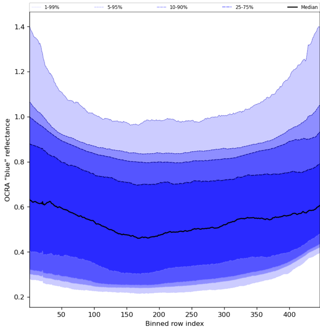
Figure 67: Along track statistics of “OCRA “blue” reflectance” for 2023-10-01 to 2023-10-03
