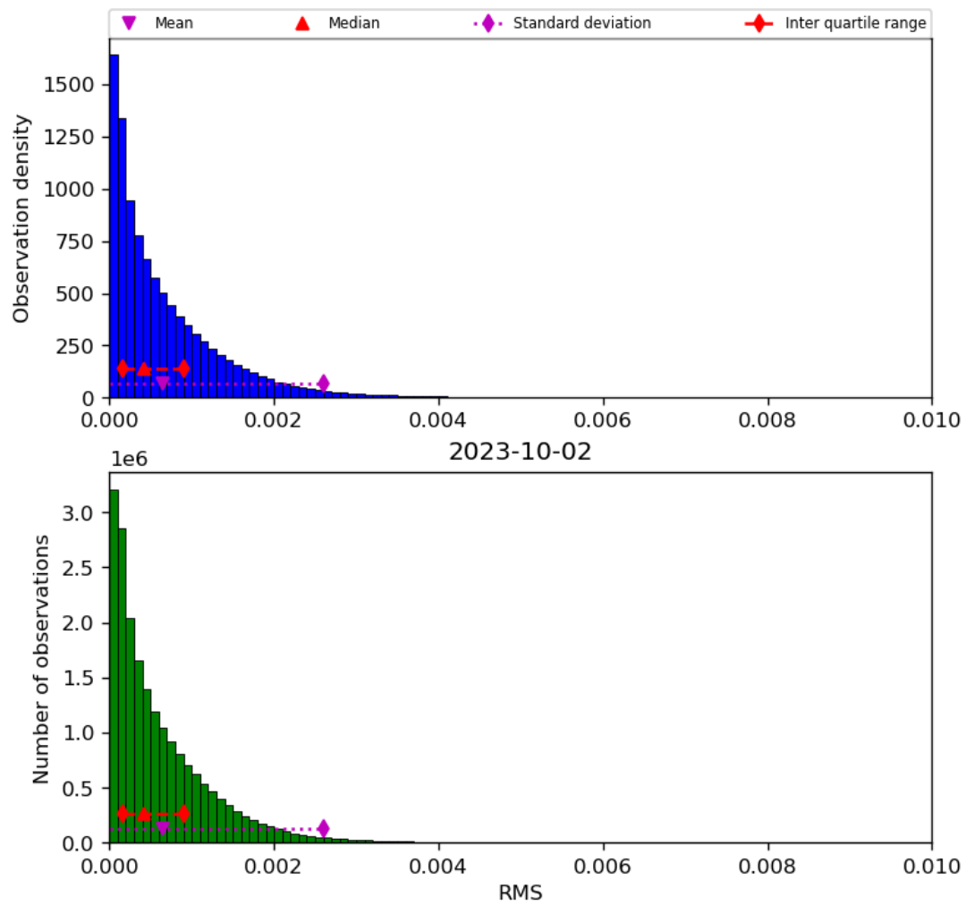
Figure 47: Histogram of “RMS” for 2023-10-01 to 2023-10-03
