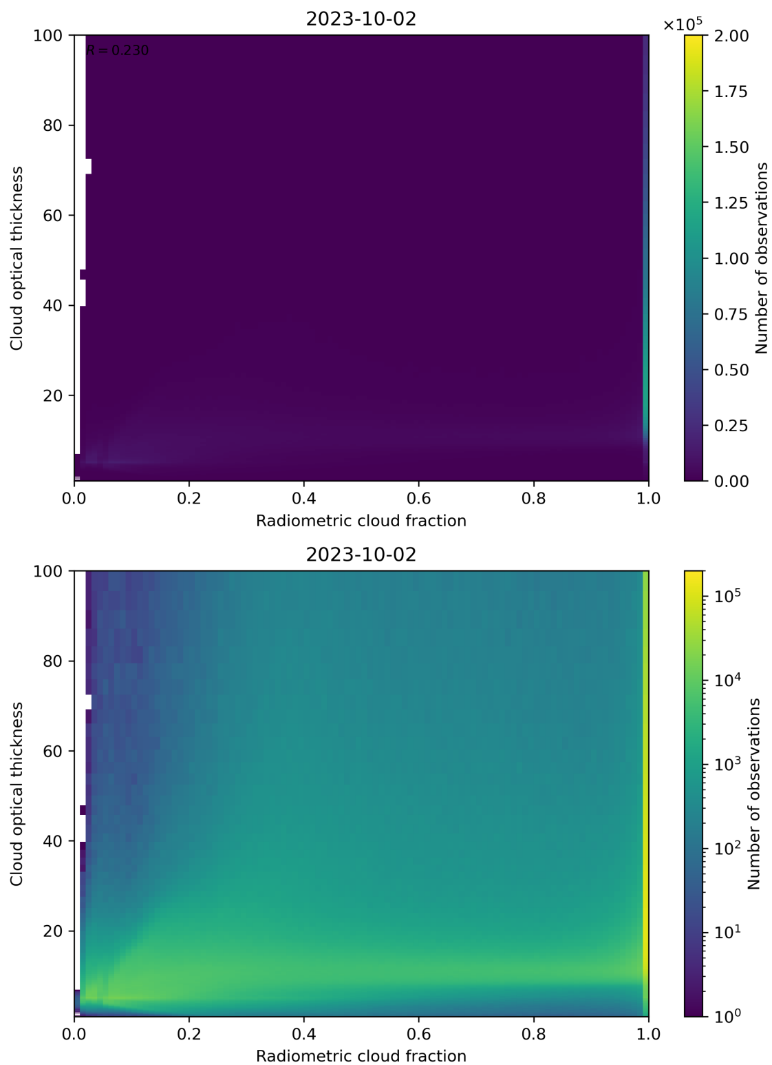
Figure 75: Scatter density plot of “Radiometric cloud fraction” against “Cloud optical thickness” for 2023-10-01 to 2023-10-03.
