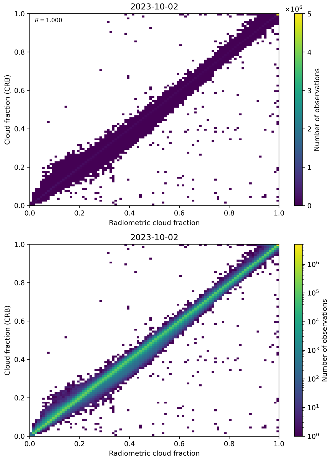
Figure 73: Scatter density plot of “Radiometric cloud fraction” against “Cloud fraction (CRB)” for 2023-10-01 to 2023-10-03.
