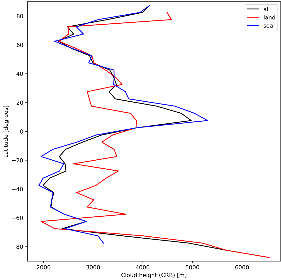
Figure 27: Zonal average of “Cloud height (CRB)” for 2023-10-01 to 2023-10-03.
