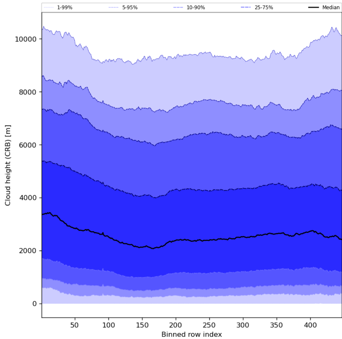
Figure 59: Along track statistics of “Cloud height (CRB)” for 2023-10-01 to 2023-10-03
