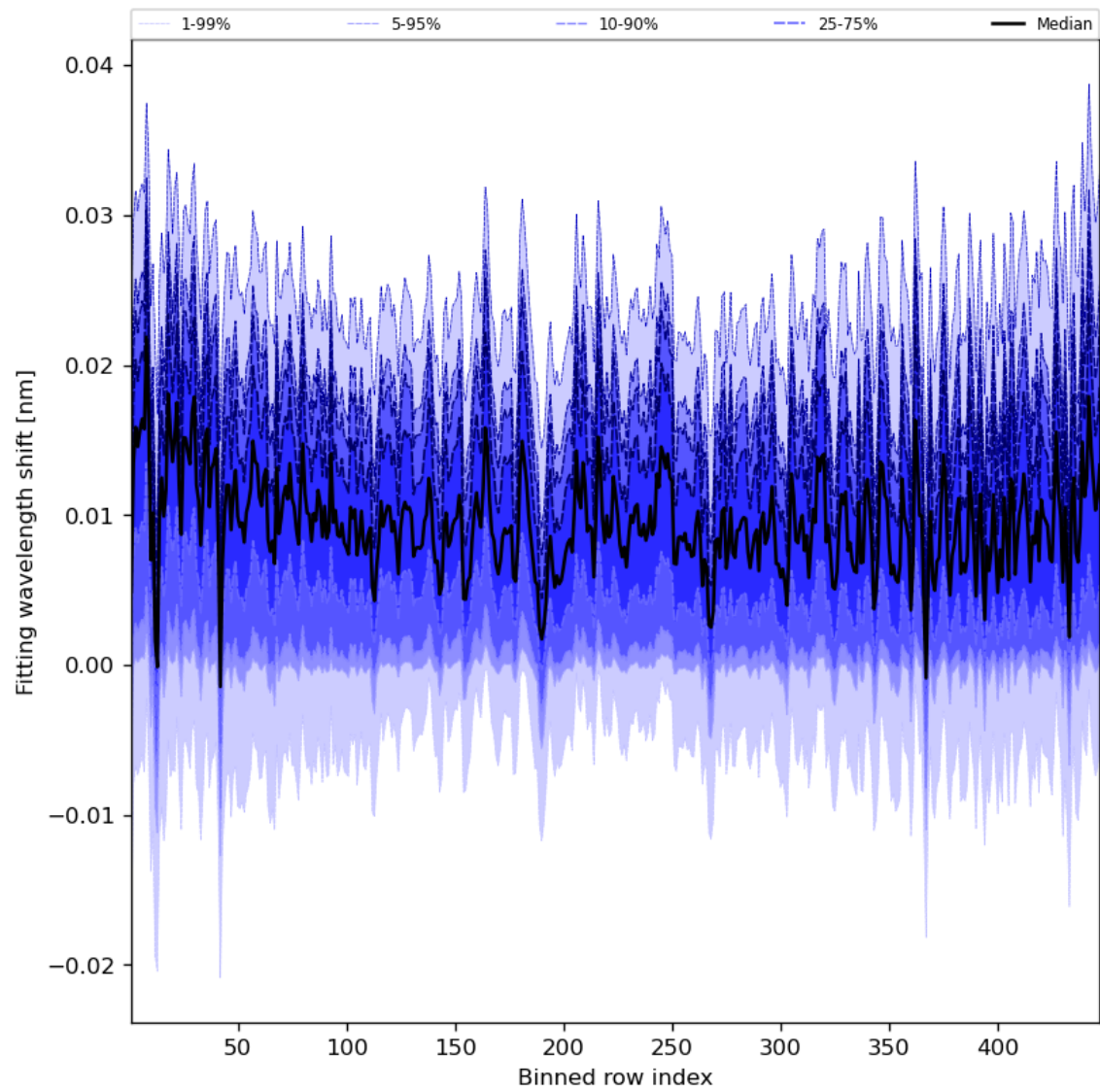
Figure 65: Along track statistics of “Fitting wavelength shift” for 2023-10-01 to 2023-10-03
