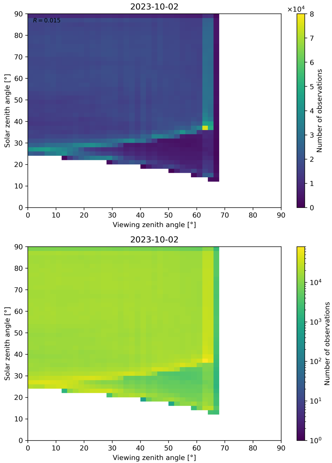
Figure 114: Scatter density plot of “Viewing zenith angle” against “Solar zenith angle” for 2023-10-01 to 2023-10-03.
