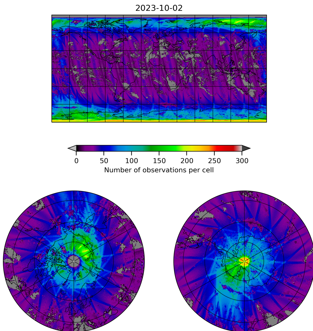
Figure 21: Map of the number of observations for 2023-10-01 to 2023-10-03
