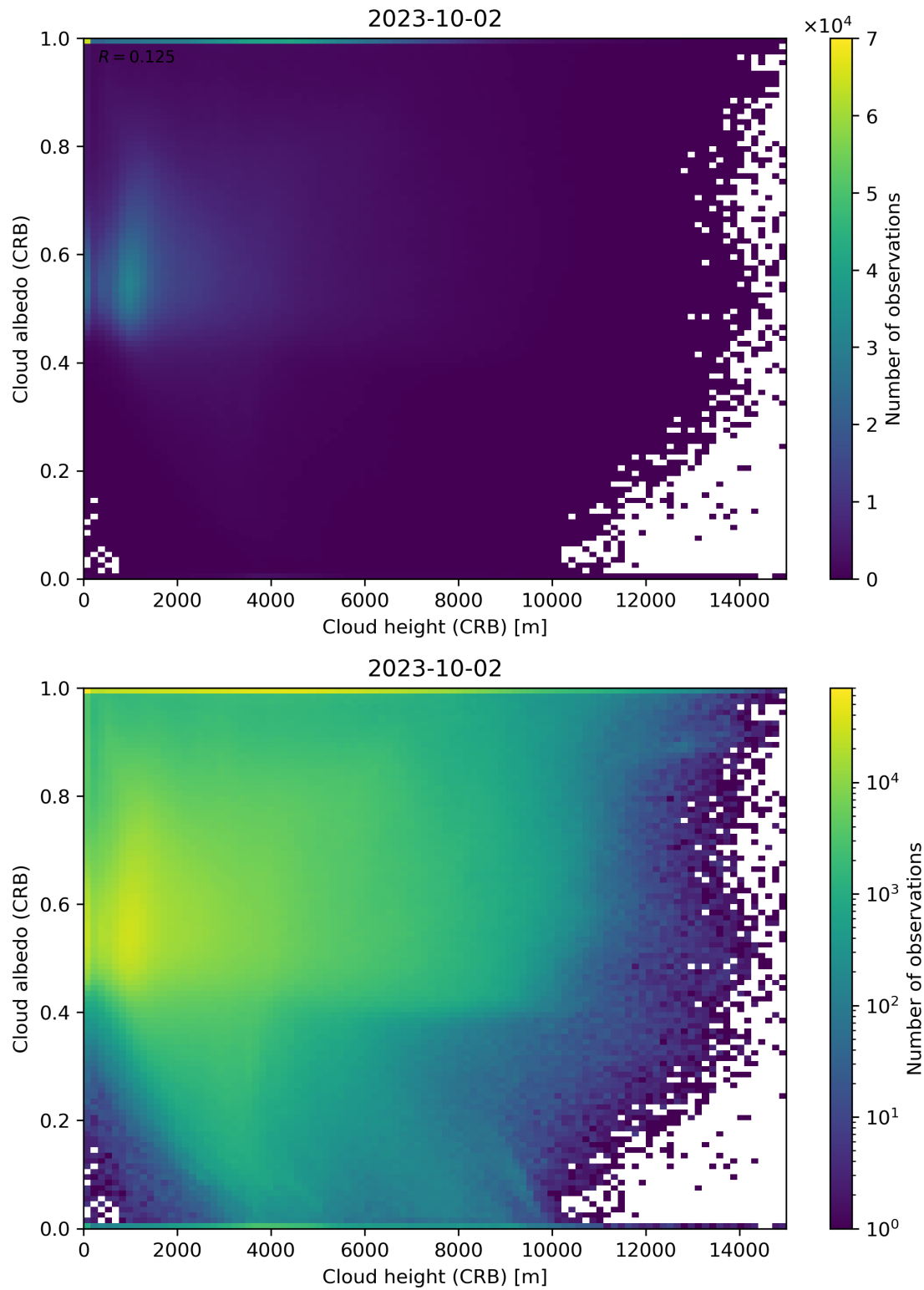
Figure 80: Scatter density plot of “Cloud height (CRB)” against “Cloud albedo (CRB)” for 2023-10-01 to 2023-10-03.
