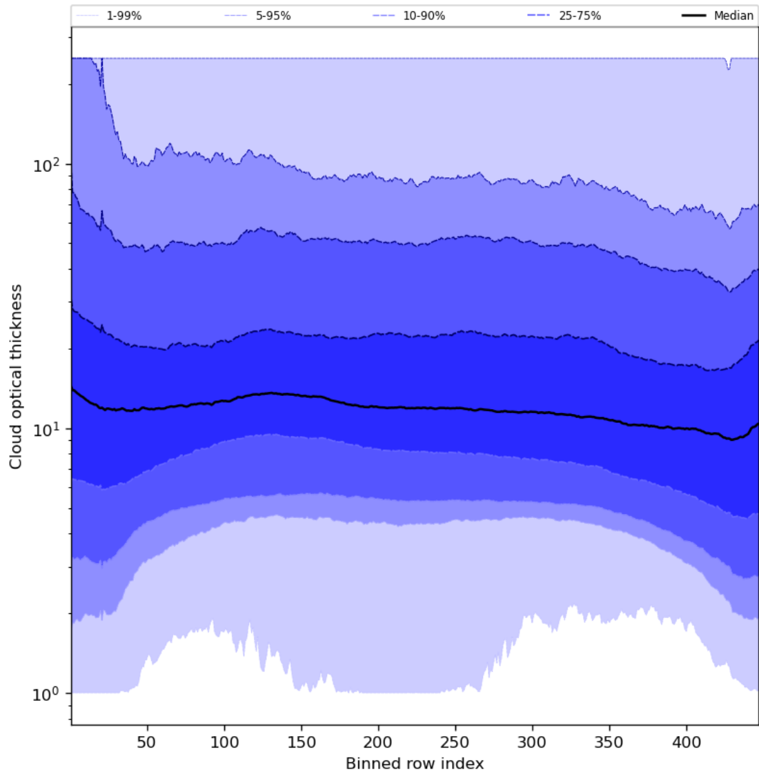
Figure 57: Along track statistics of “Cloud optical thickness” for 2023-10-01 to 2023-10-03
