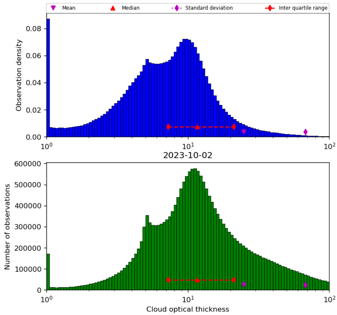
Figure 41: Histogram of “Cloud optical thickness” for 2023-10-01 to 2023-10-03
