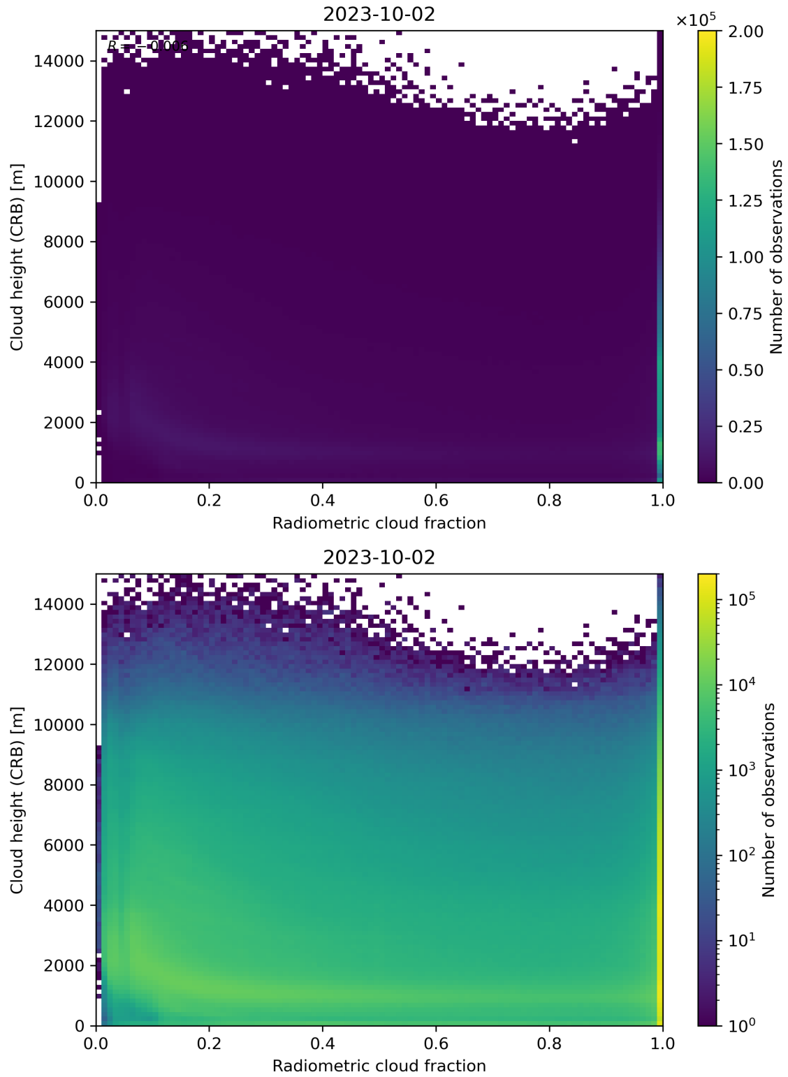
Figure 74: Scatter density plot of “Radiometric cloud fraction” against “Cloud height (CRB)” for 2023-10-01 to 2023-10-03.
