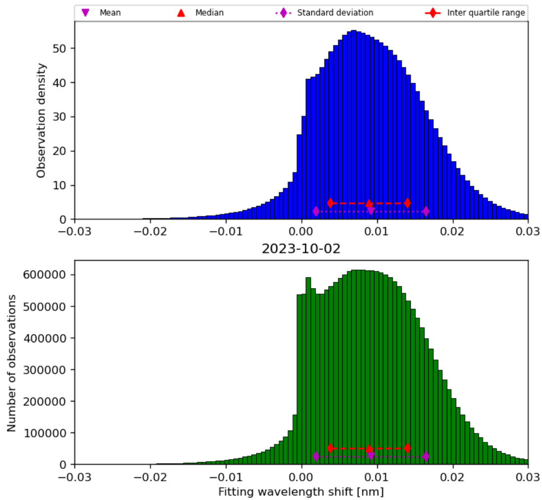
Figure 49: Histogram of “Fitting wavelength shift” for 2023-10-01 to 2023-10-03
