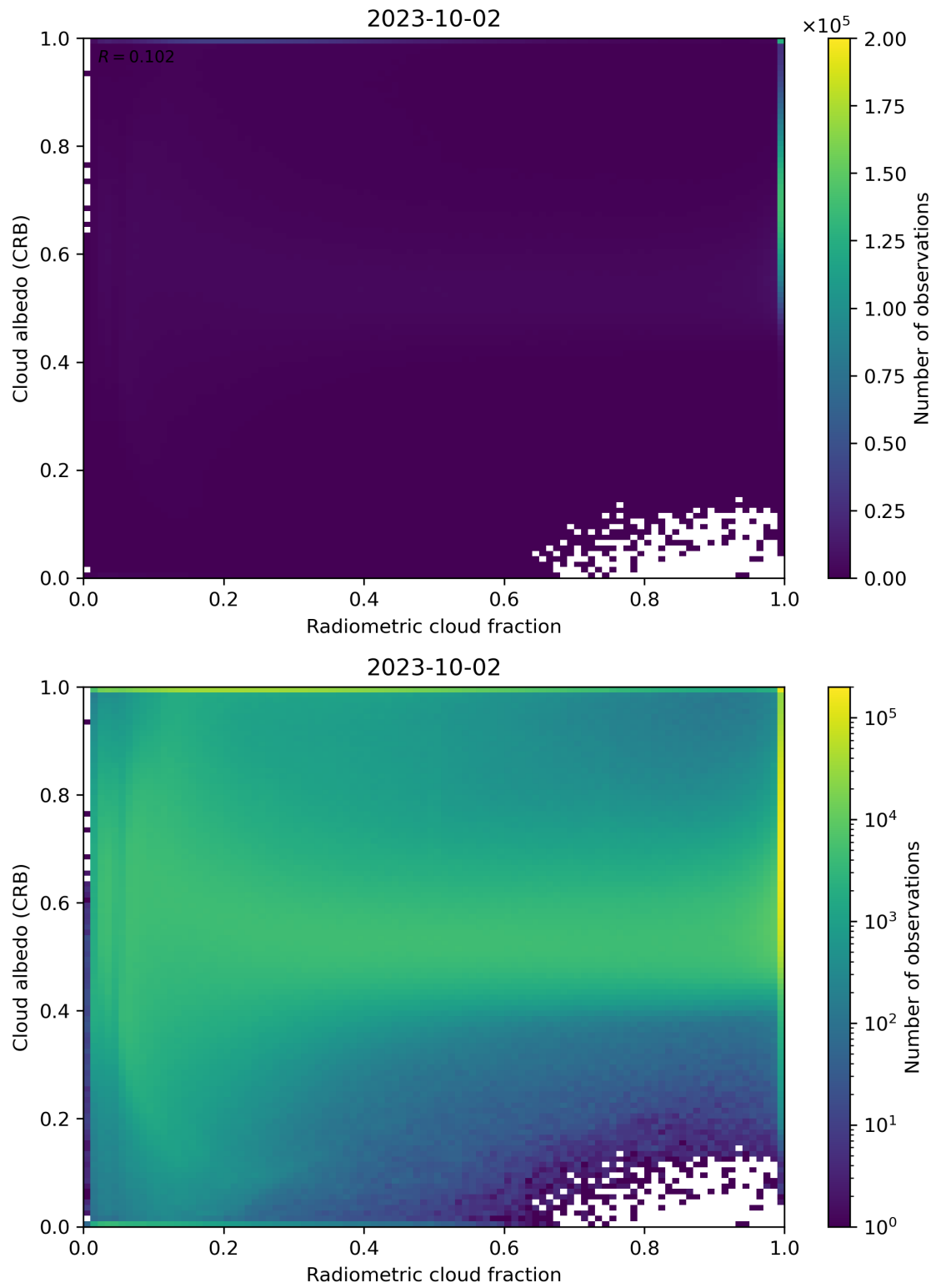
Figure 71: Scatter density plot of “Radiometric cloud fraction” against “Cloud albedo (CRB)” for 2023-10-01 to 2023-10-03.
