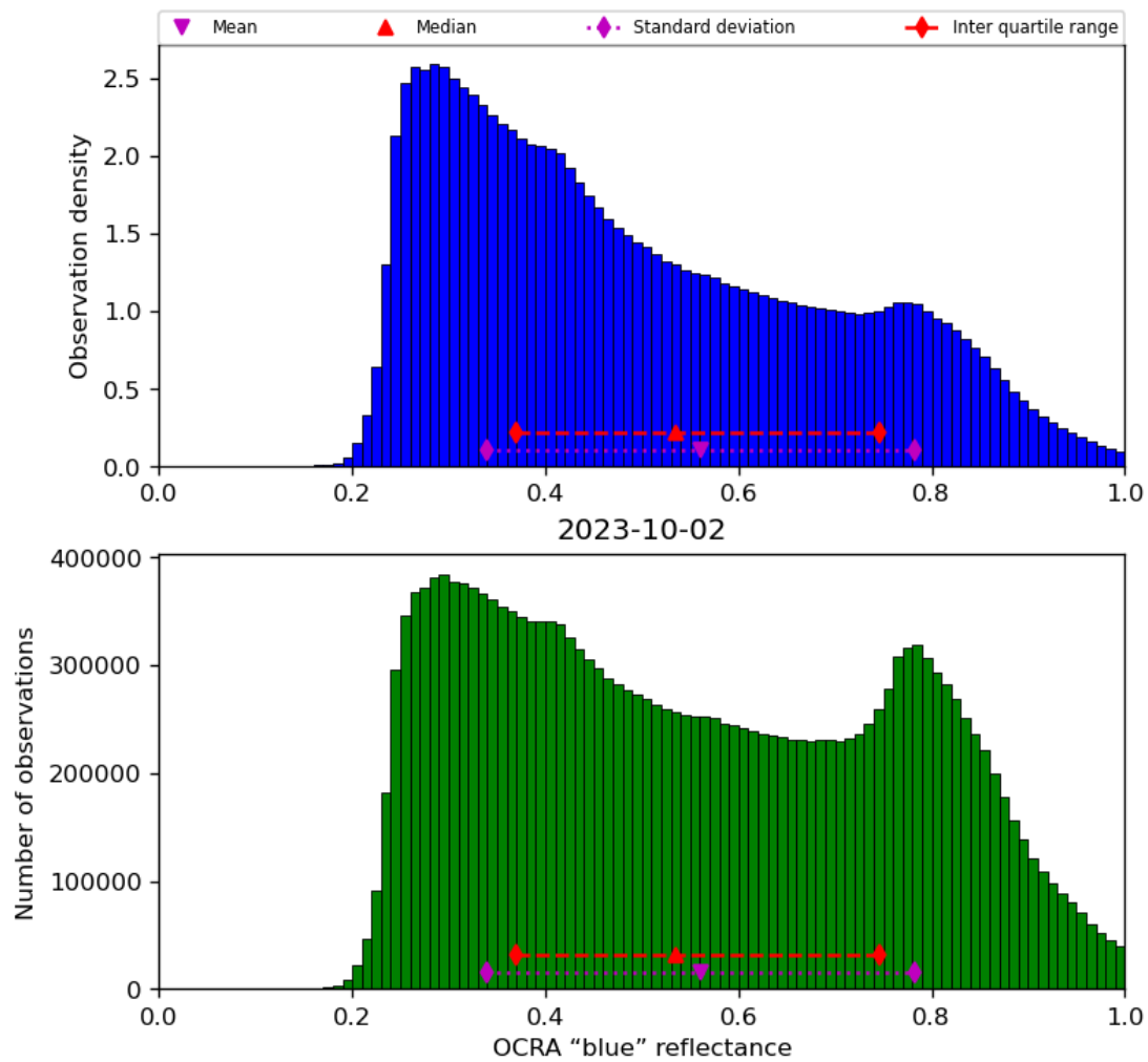
Figure 51: Histogram of “OCRA “blue” reflectance” for 2023-10-01 to 2023-10-03
