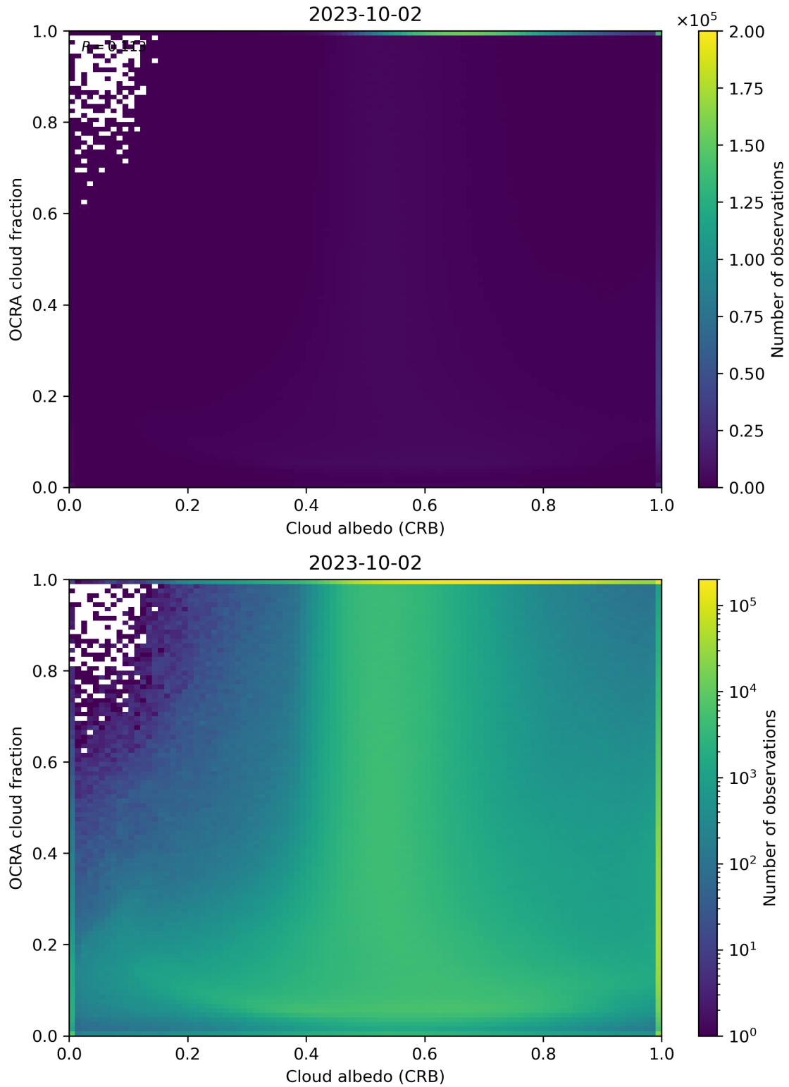
Figure 70: Scatter density plot of “Cloud albedo (CRB)” against “OCRA cloud fraction” for 2023-10-01 to 2023-10-03.
