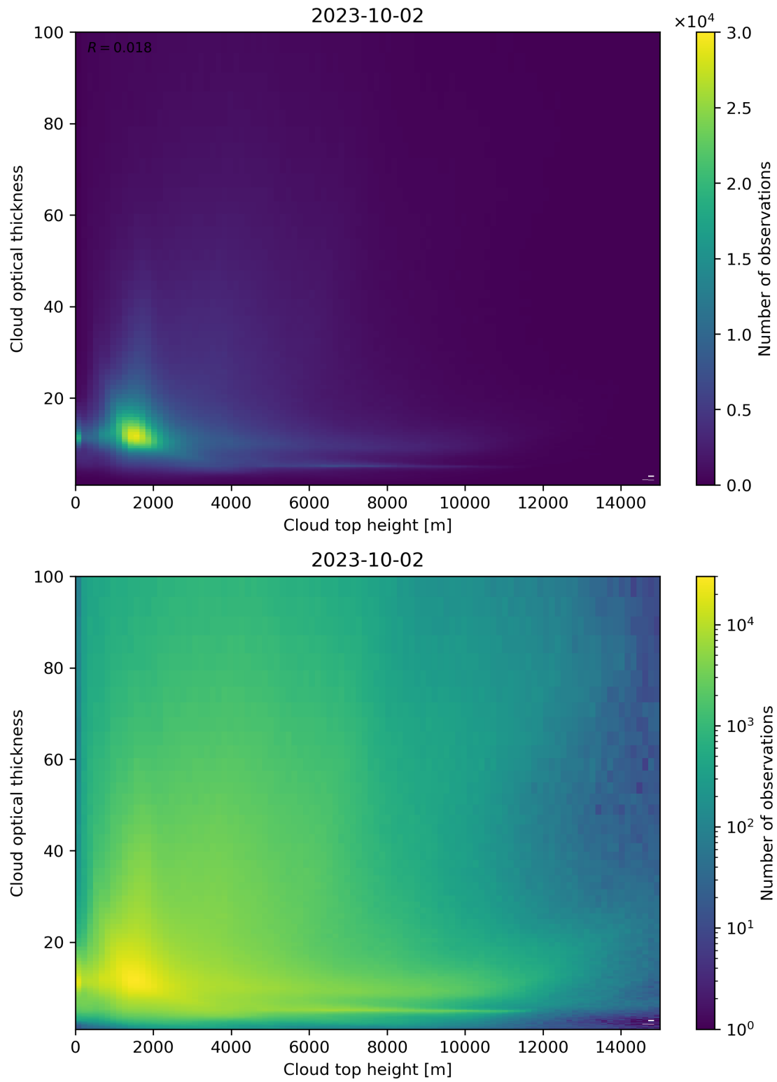
Figure 90: Scatter density plot of “Cloud top height” against “Cloud optical thickness” for 2023-10-01 to 2023-10-03.
