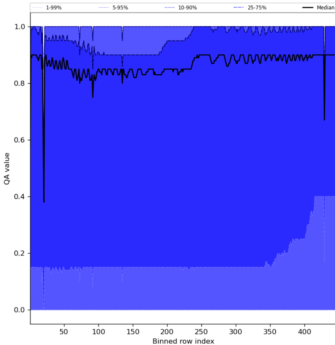
Figure 54: Along track statistics of “QA value” for 2023-10-01 to 2023-10-03
