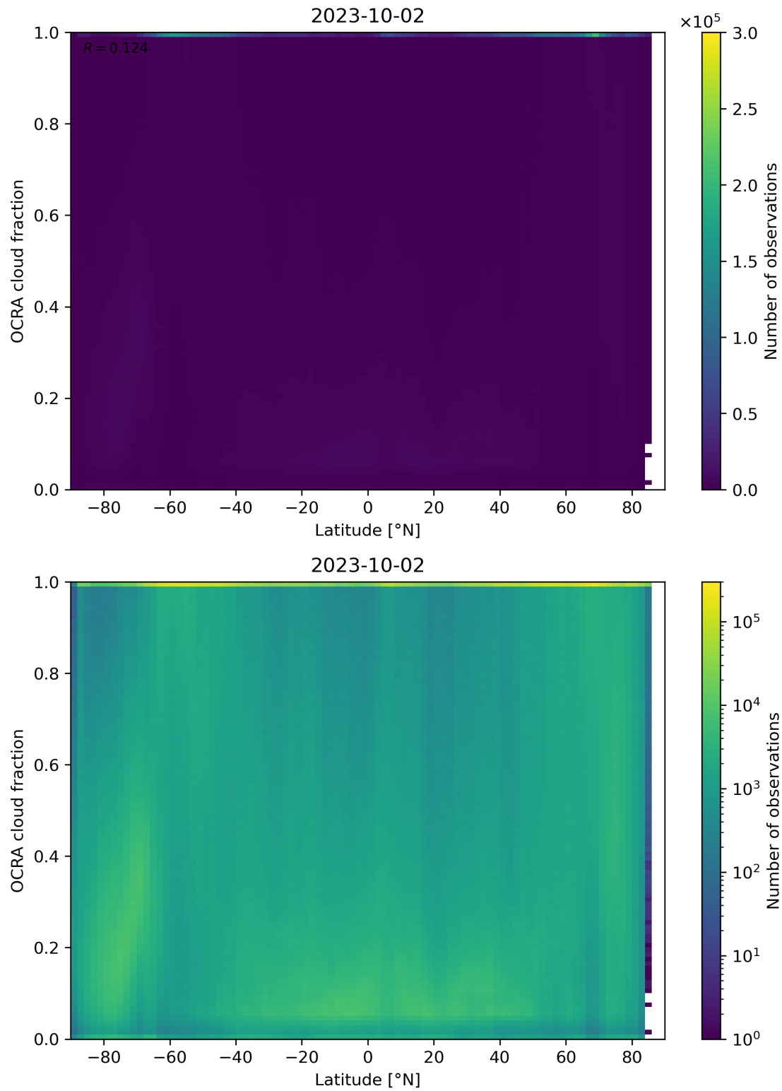
Figure 93: Scatter density plot of “Latitude” against “OCRA cloud fraction” for 2023-10-01 to 2023-10-03.
