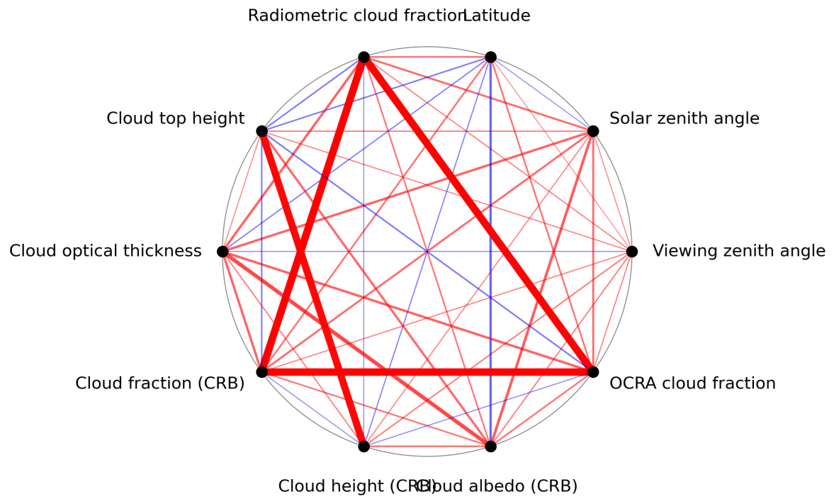
Figure 1: Map of correlation graph for 2023-10-01 to 2023-10-03.
