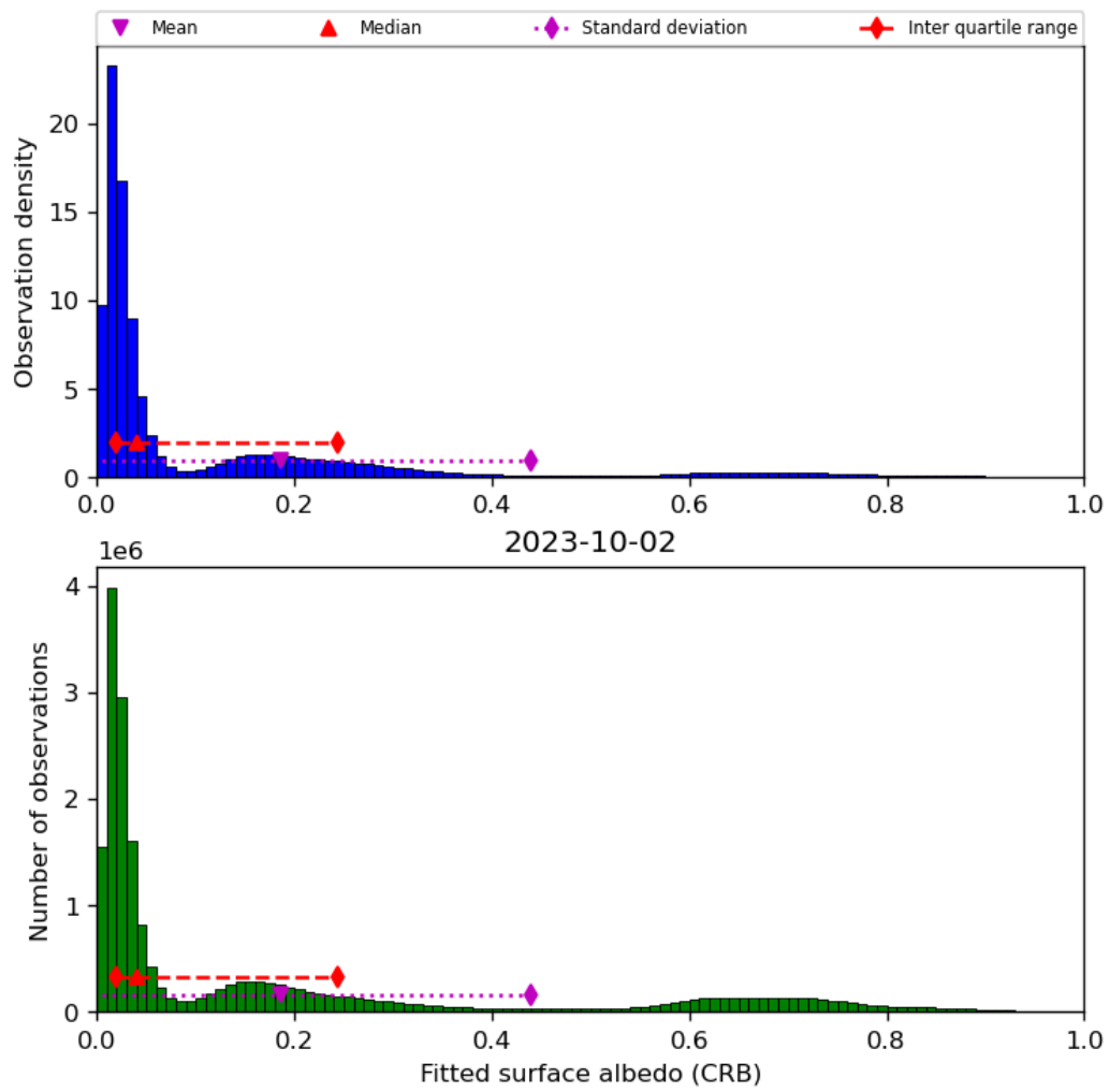
Figure 46: Histogram of “Fitted surface albedo (CRB)” for 2023-10-01 to 2023-10-03
