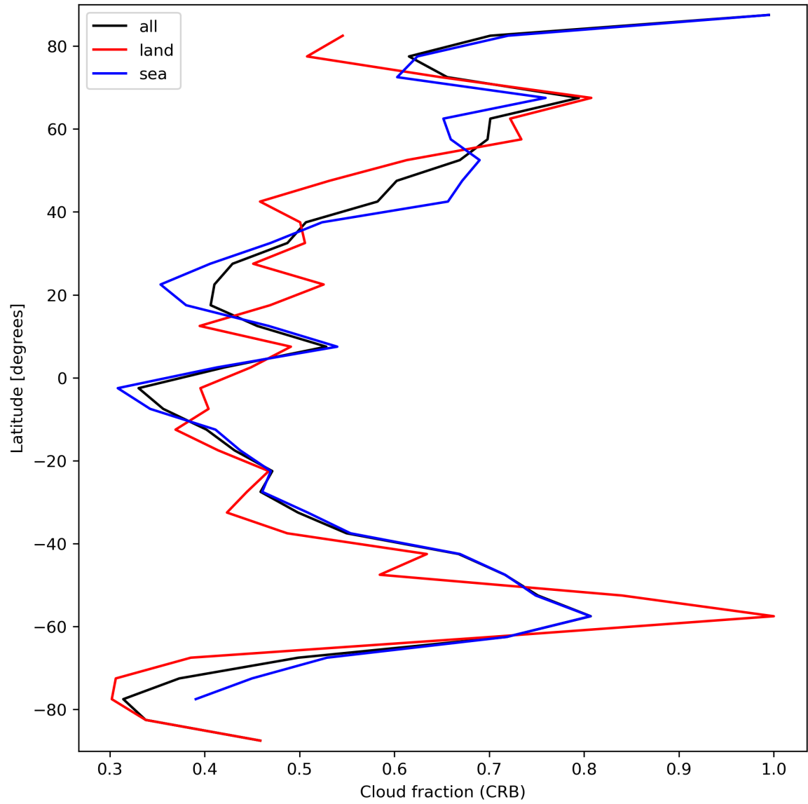
Figure 26: Zonal average of “Cloud fraction (CRB)” for 2023-10-01 to 2023-10-03.
